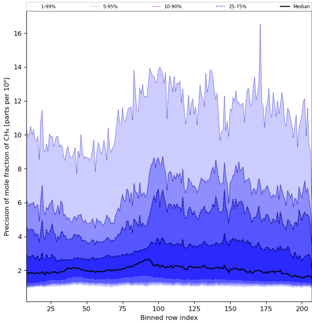
Figure 35: Along track statistics of “Precision of mole fraction of CH 4 ” for 2023-11-23 to 2023-11-25
