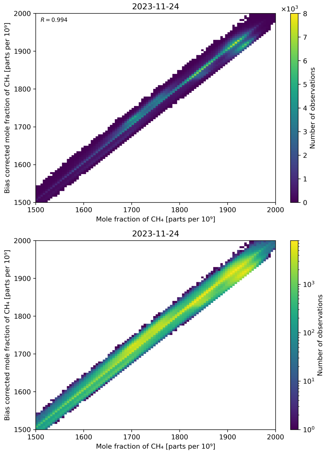
Figure 74: Scatter density plot of “Mole fraction of CH 4 ” against “Bias corrected mole fraction of CH 4 ” for 2023-11-23 to 2023-11-25.
