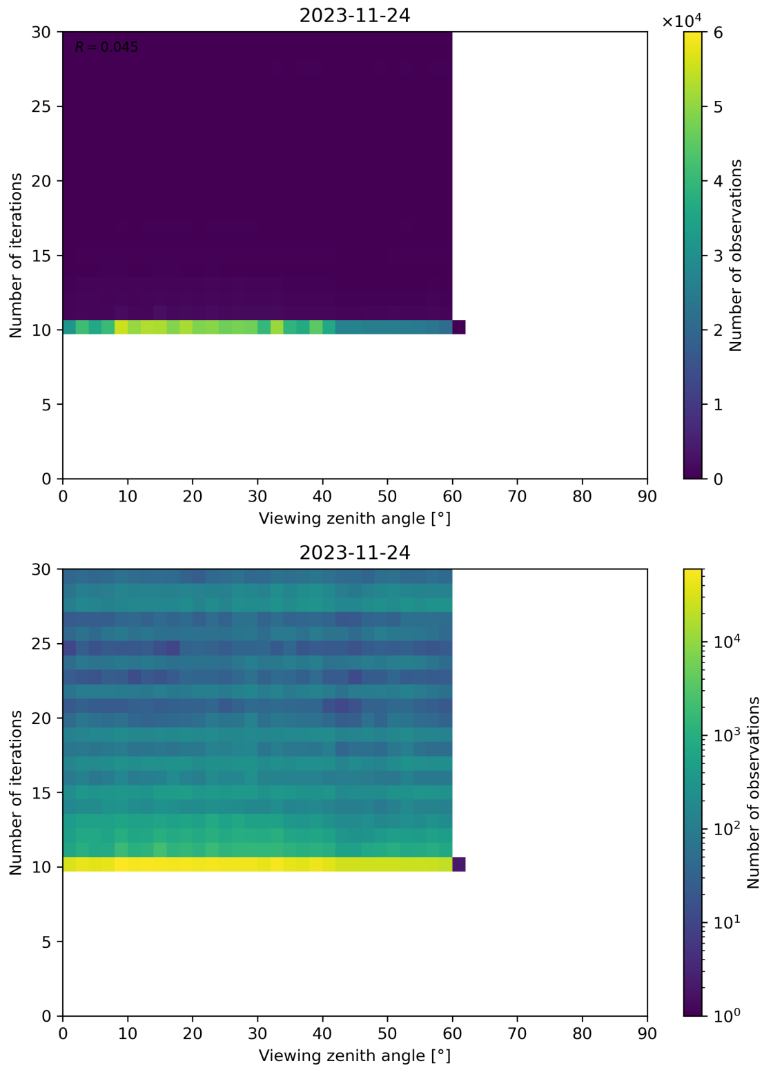
Figure 113: Scatter density plot of “Viewing zenith angle” against “Number of iterations” for 2023-11-23 to 2023-11-25.
