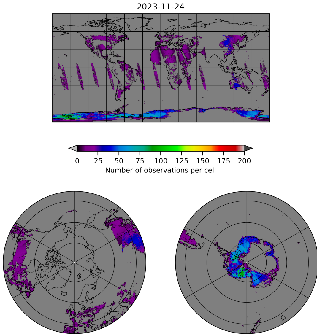
Figure 10: Map of the number of observations for 2023-11-23 to 2023-11-25
