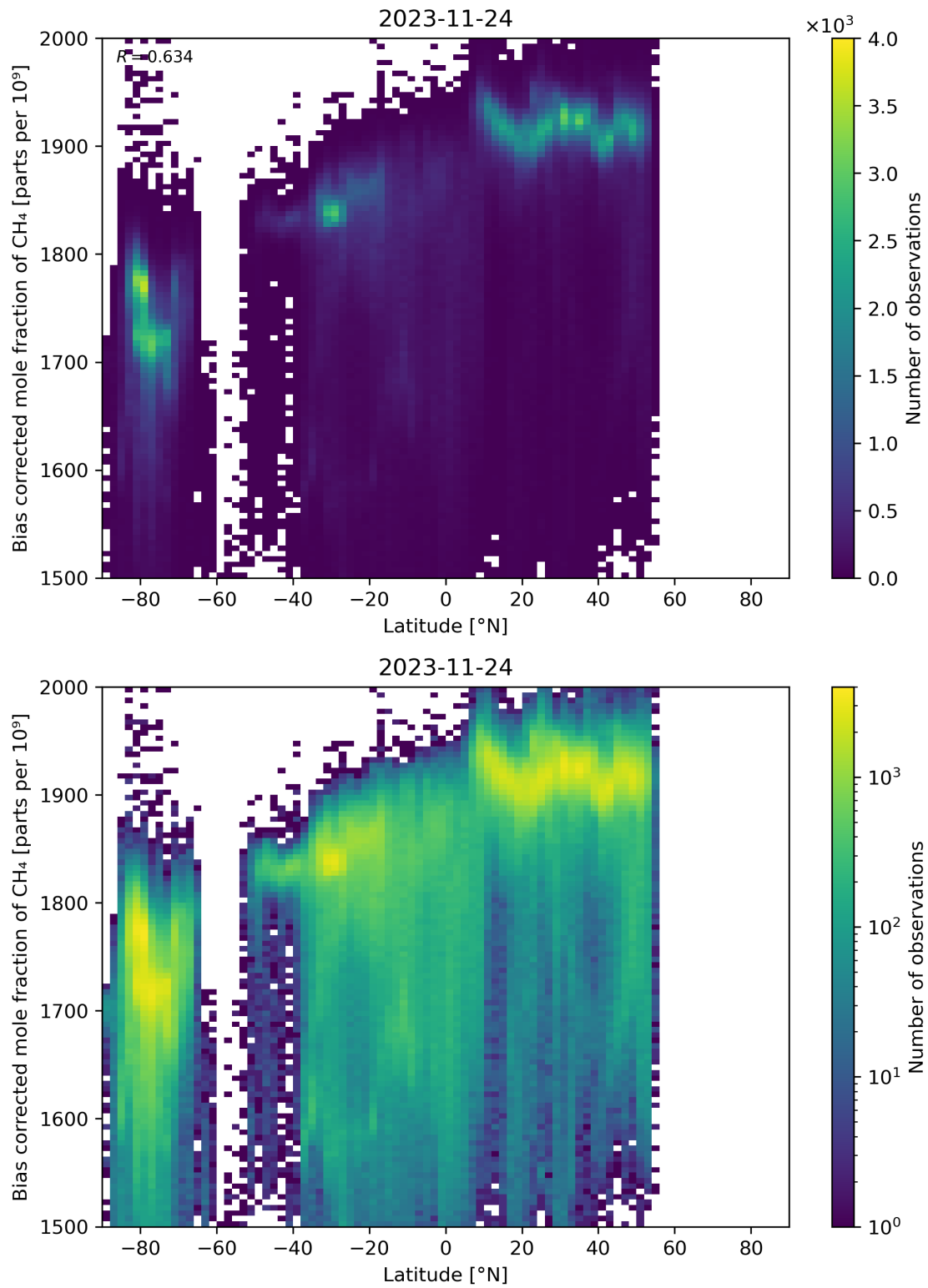
Figure 58: Scatter density plot of “Latitude” against “Bias corrected mole fraction of CH 4 ” for 2023-11-23 to 2023-11-25.
