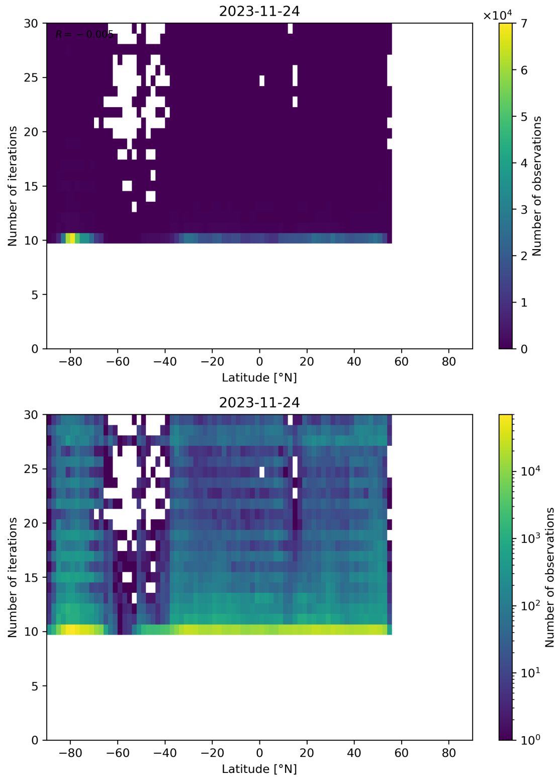
Figure 60: Scatter density plot of “Latitude” against “Number of iterations” for 2023-11-23 to 2023-11-25.
