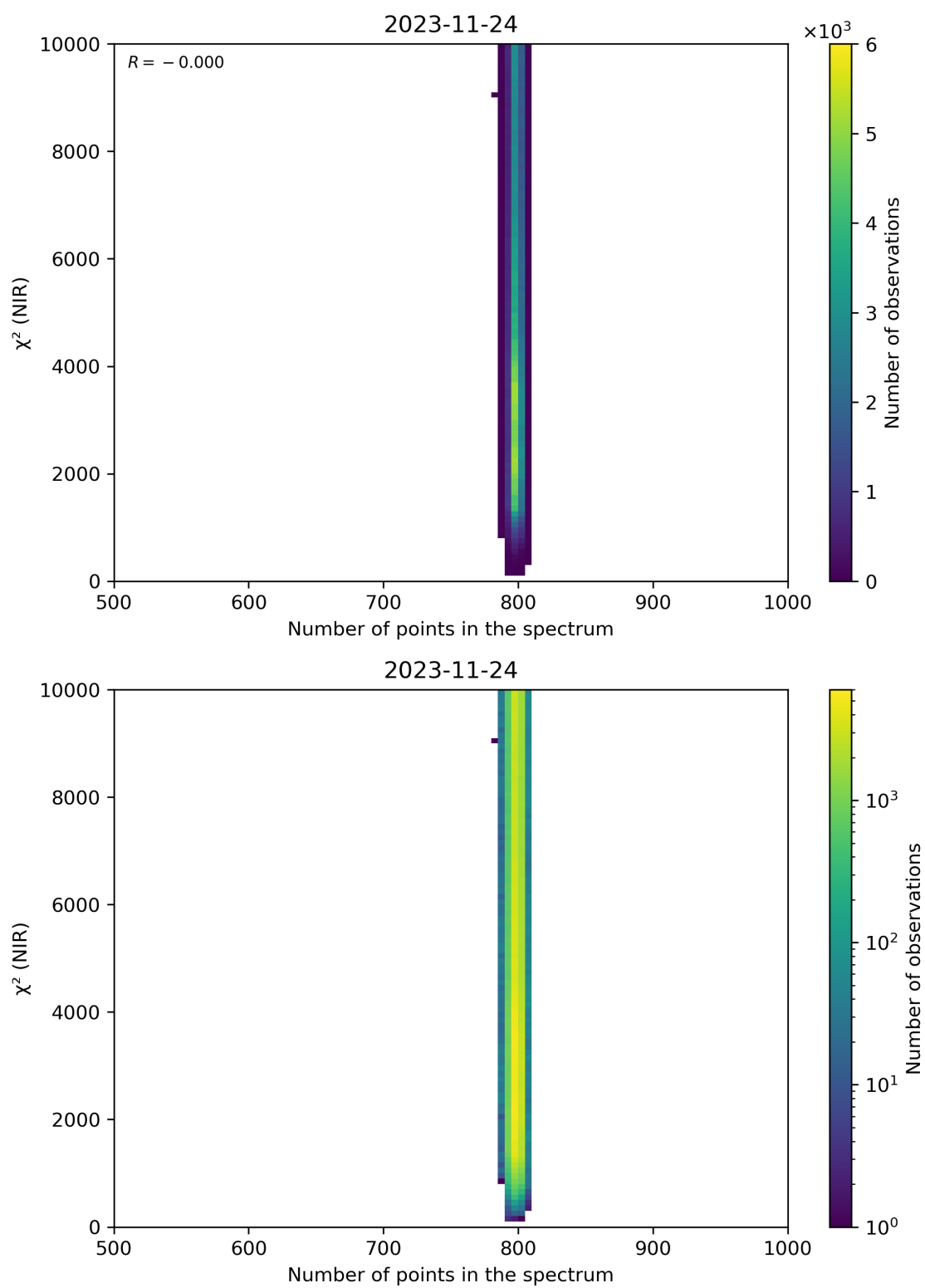
Figure 88: Scatter density plot of “Number of points in the spectrum” against “ \chi^2 (NIR)” for 2023-11-23 to 2023-11-25.
