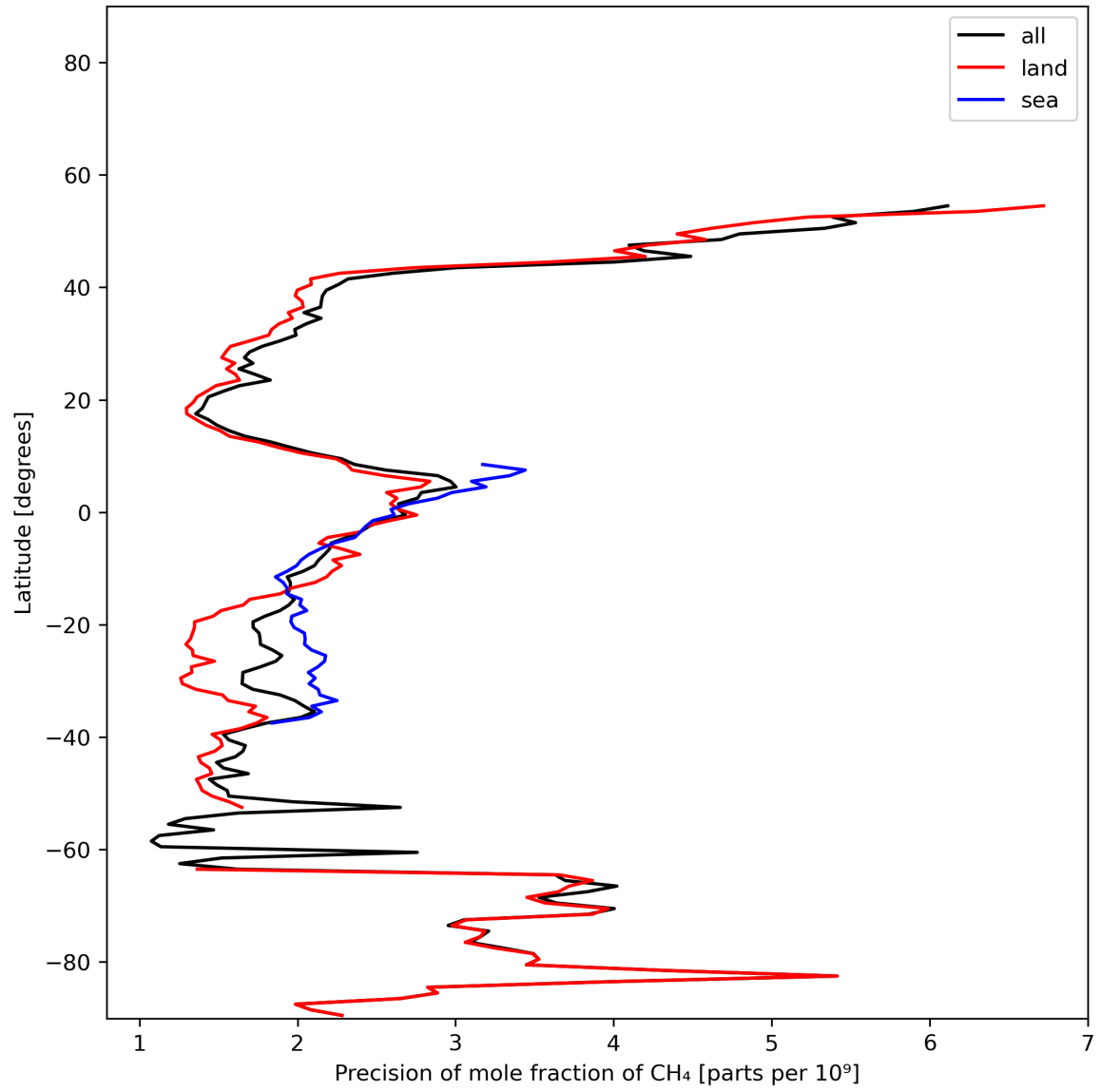
Figure 13: Zonal average of “Precision of mole fraction of CH 4 ” for 2023-11-23 to 2023-11-25.
