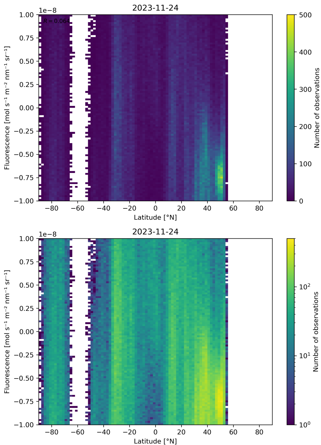
Figure 56: Scatter density plot of “Latitude” against “Fluorescence” for 2023-11-23 to 2023-11-25.
