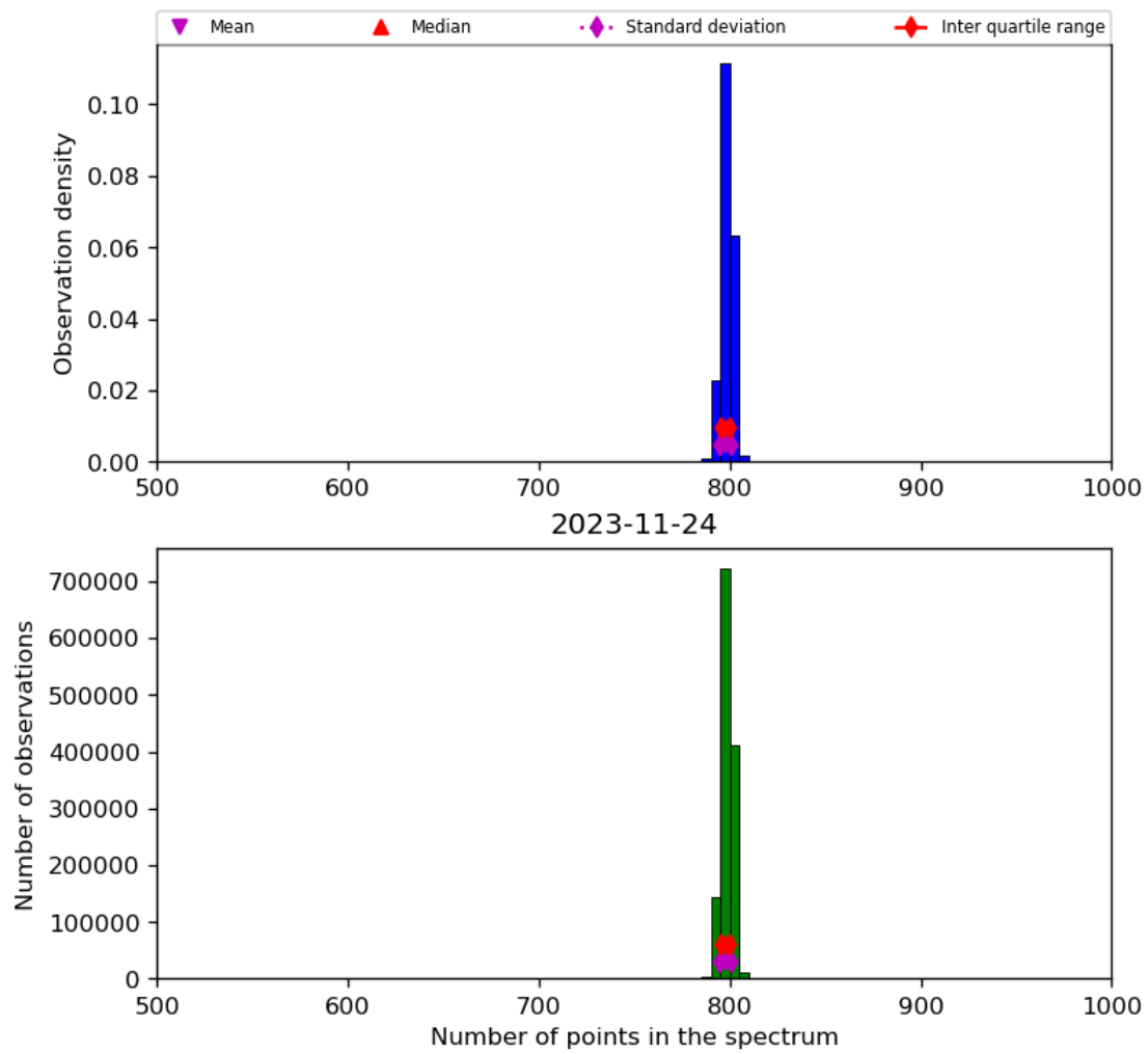
Figure 26: Histogram of “Number of points in the spectrum” for 2023-11-23 to 2023-11-25
