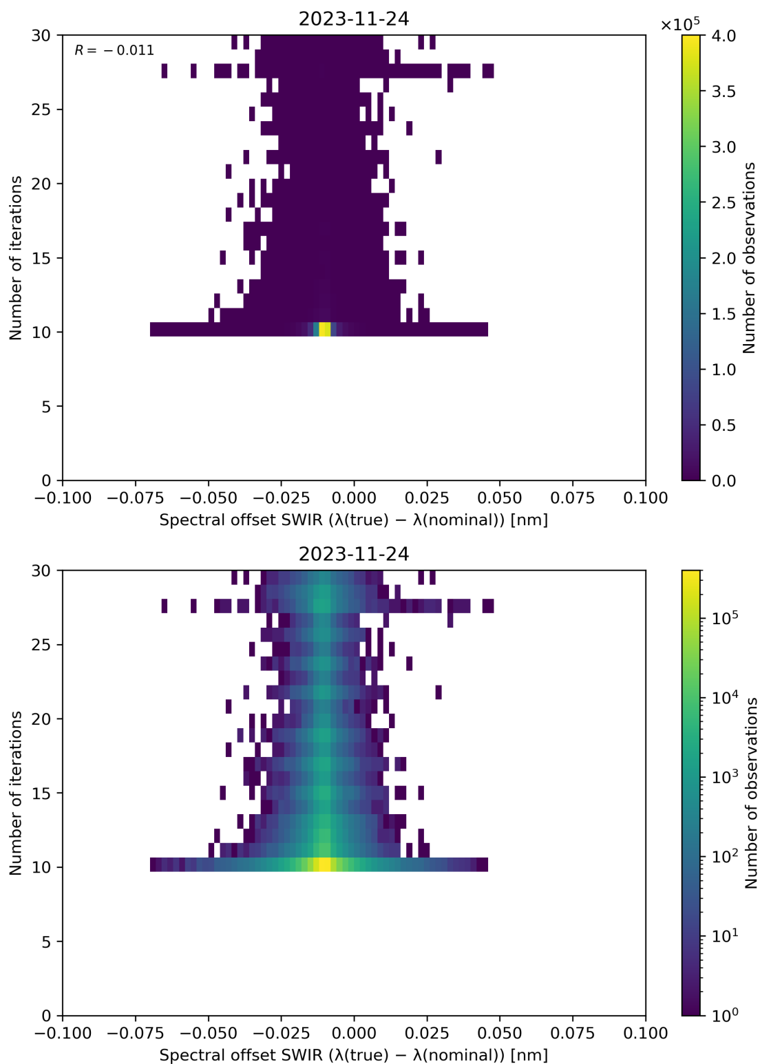
Figure 121: Scatter density plot of “Spectral offset SWIR ( \lambda(\text{true}) - \lambda(\text{nominal}) )” against “Number of iterations” for 2023-11-23 to 2023-11-25.
