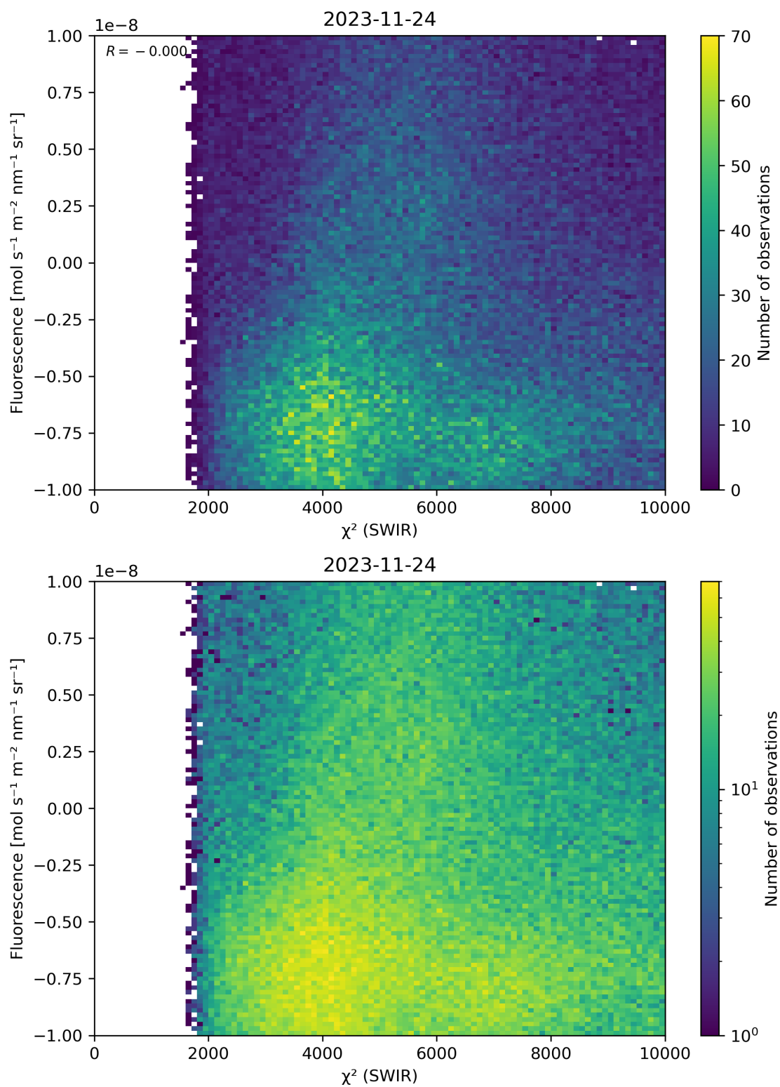
Figure 49: Scatter density plot of “ \chi^2 (SWIR)” against “Fluorescence” for 2023-11-23 to 2023-11-25.
