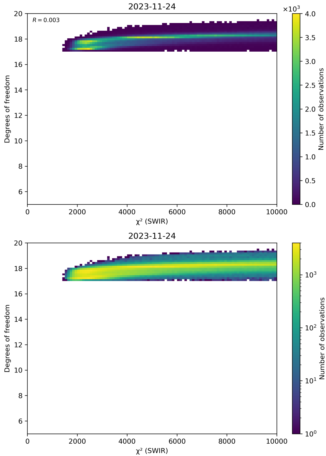
Figure 48: Scatter density plot of “ \chi^2 (SWIR)” against “Degrees of freedom” for 2023-11-23 to 2023-11-25.
