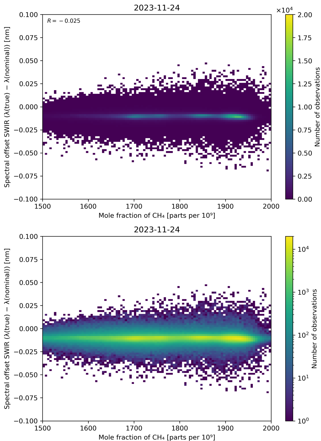
Figure 86: Scatter density plot of “Mole fraction of CH 4 ” against “Spectral offset SWIR ( \lambda(\text{true}) - \lambda(\text{nominal}) )” for 2023-11-23 to 2023-11-25.
