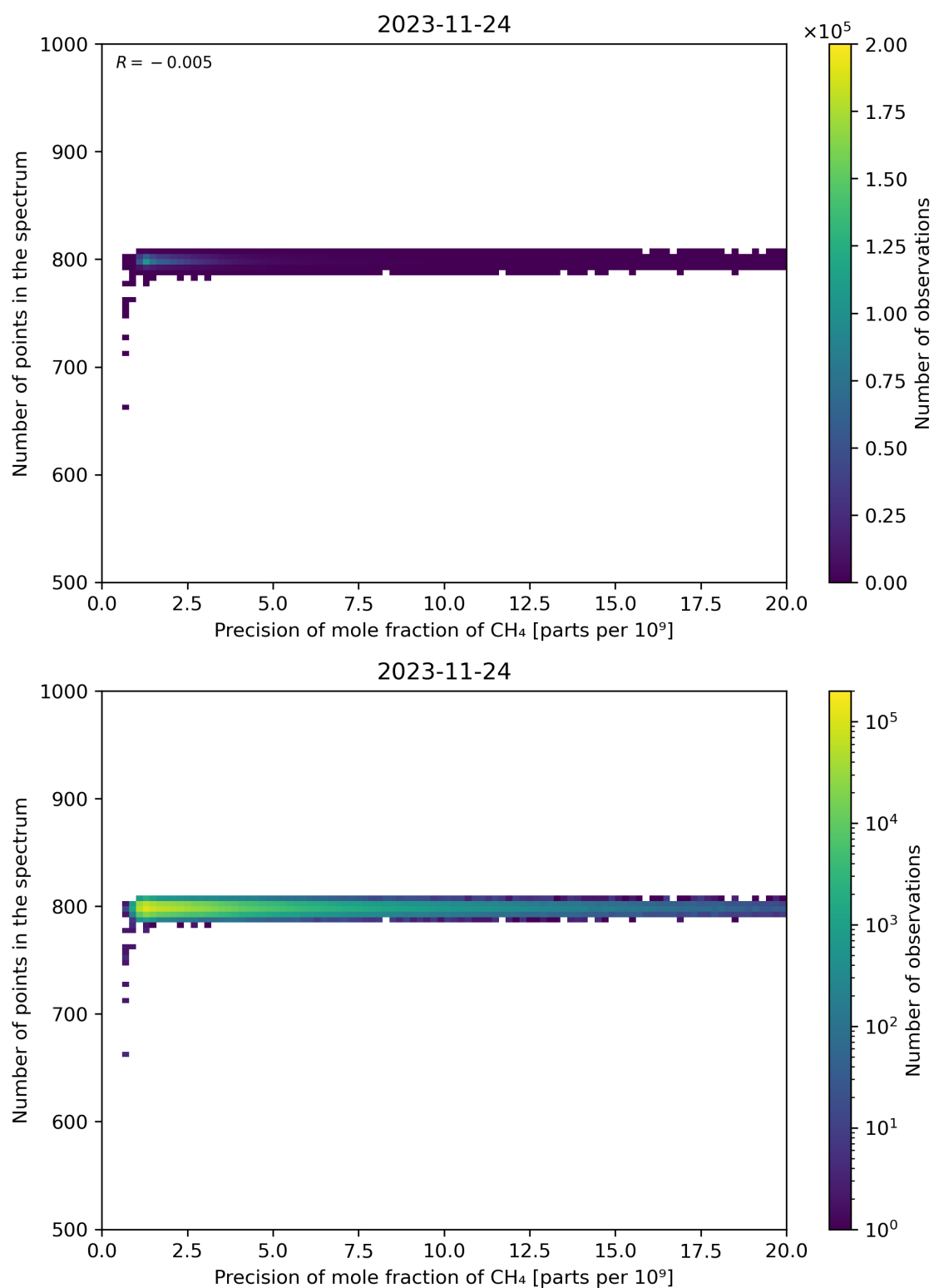
Figure 84: Scatter density plot of “Precision of mole fraction of CH 4 ” against “Number of points in the spectrum” for 2023-11-23 to 2023-11-25.
