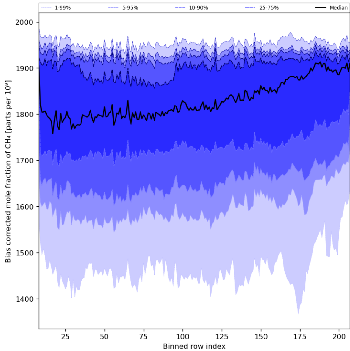
Figure 36: Along track statistics of “Bias corrected mole fraction of CH 4 ” for 2023-11-23 to 2023-11-25
