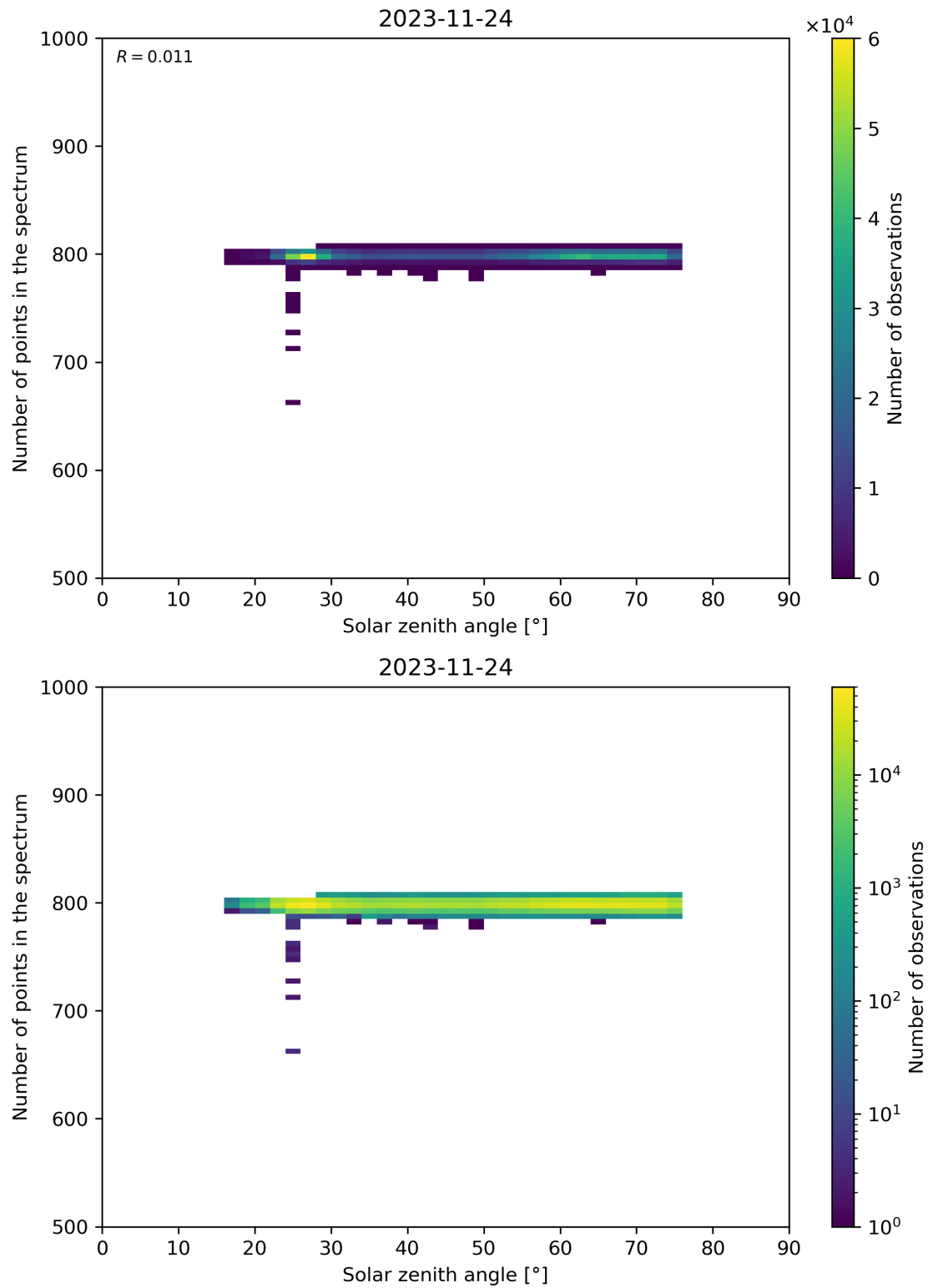
Figure 103: Scatter density plot of “Solar zenith angle” against “Number of points in the spectrum” for 2023-11-23 to 2023-11-25.
