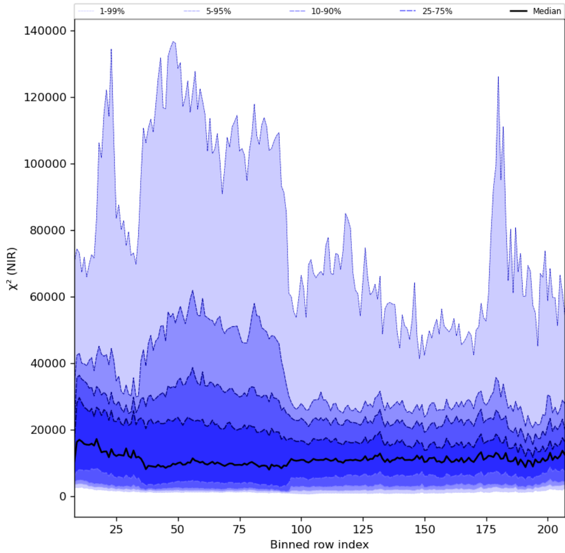
Figure 40: Along track statistics of " \chi^2 (NIR)" for 2023-11-23 to 2023-11-25
