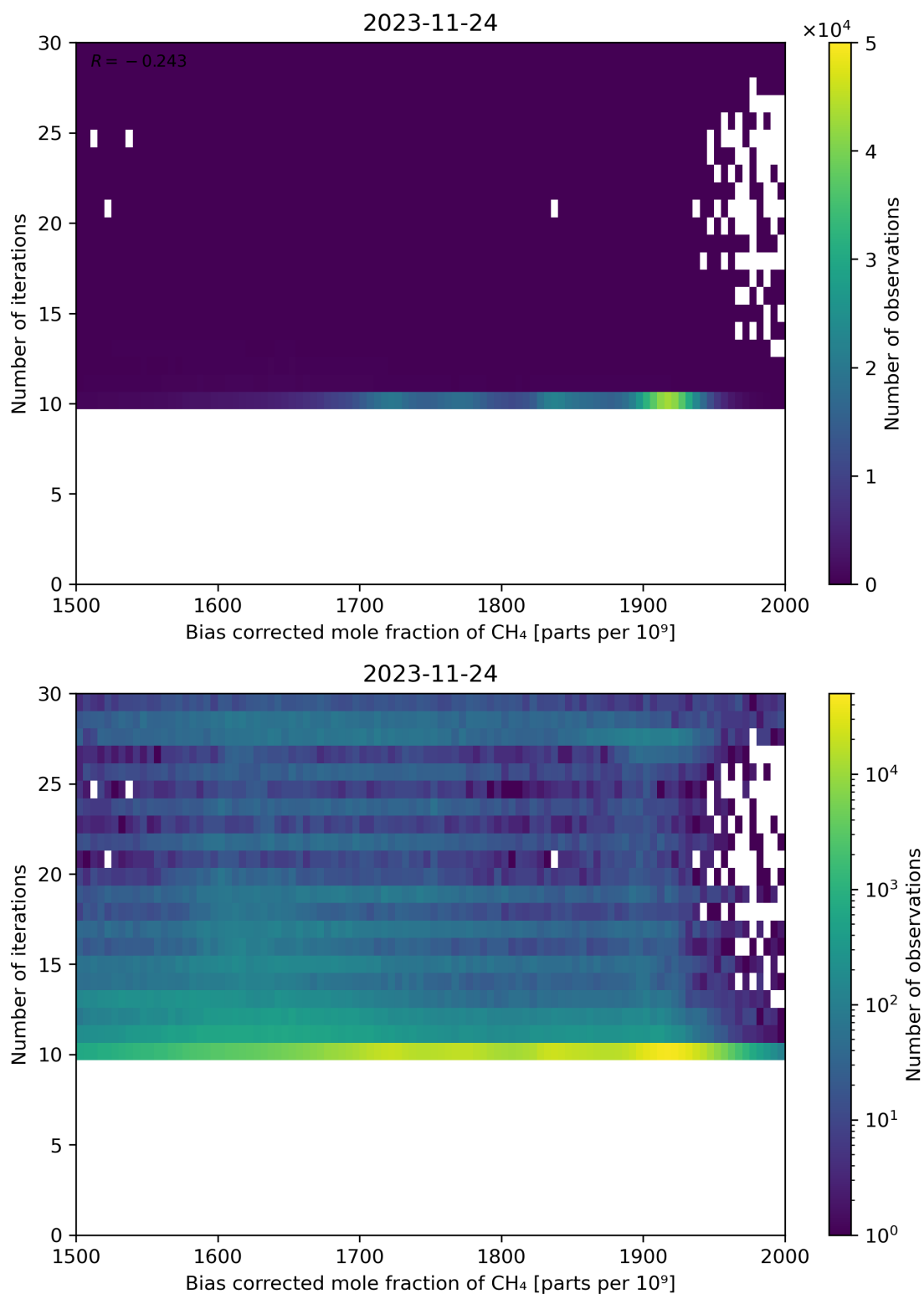
Figure 67: Scatter density plot of “Bias corrected mole fraction of \text{CH}_4 ” against “Number of iterations” for 2023-11-23 to 2023-11-25.
