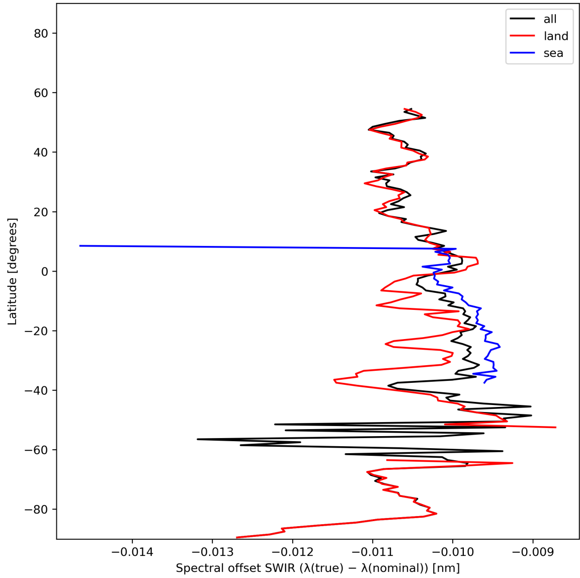
Figure 16: Zonal average of “Spectral offset SWIR ( \lambda(\text{true}) - \lambda(\text{nominal}) )” for 2023-11-23 to 2023-11-25.
