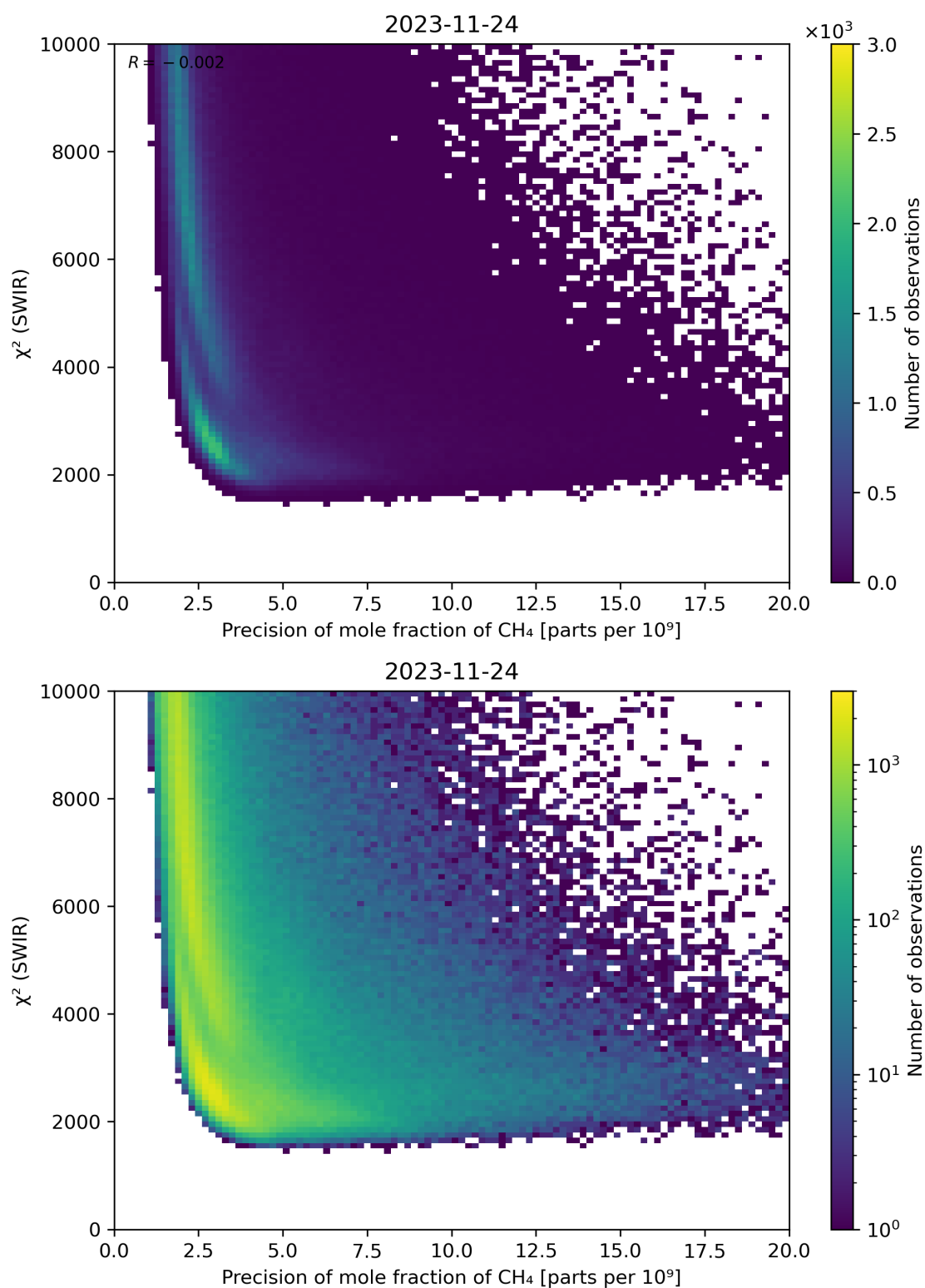
Figure 79: Scatter density plot of “Precision of mole fraction of \text{CH}_4 ” against “ \chi^2 (SWIR)” for 2023-11-23 to 2023-11-25.
