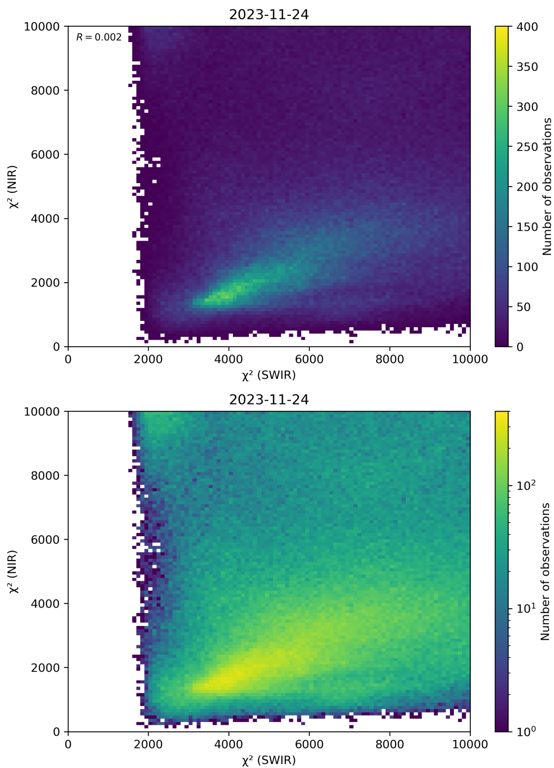
Figure 47: Scatter density plot of “ \chi^2 (SWIR)” against “ \chi^2 (NIR)” for 2023-11-23 to 2023-11-25.
