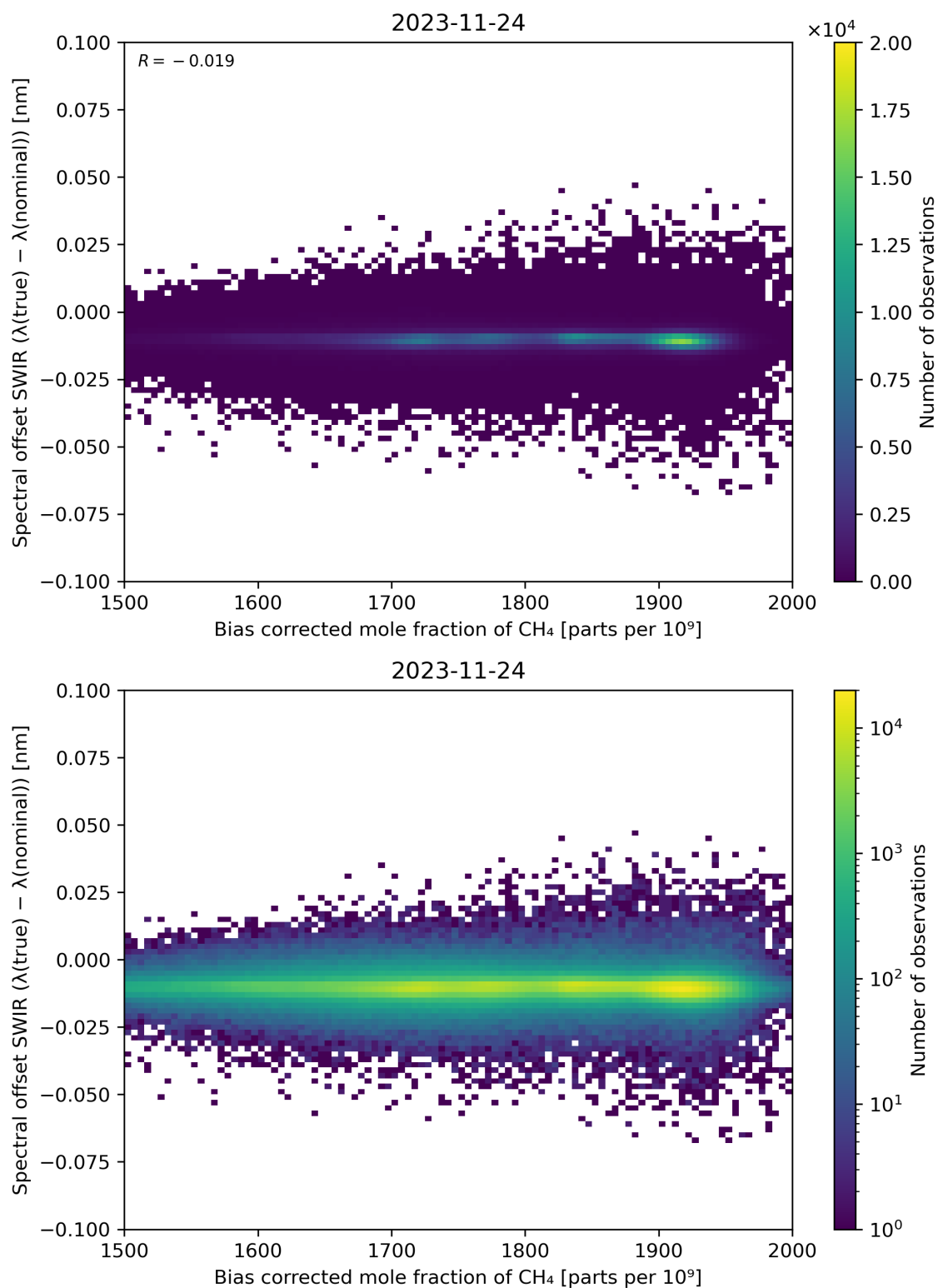
Figure 69: Scatter density plot of “Bias corrected mole fraction of \text{CH}_4 ” against “Spectral offset SWIR ( \lambda(\text{true}) - \lambda(\text{nominal}) )” for 2023-11-23 to 2023-11-25.
