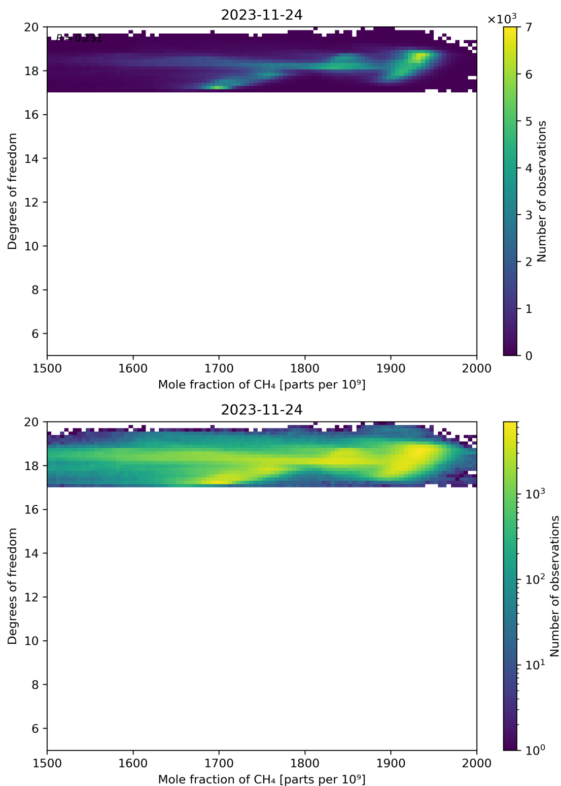
Figure 72: Scatter density plot of “Mole fraction of CH 4 ” against “Degrees of freedom” for 2023-11-23 to 2023-11-25.
