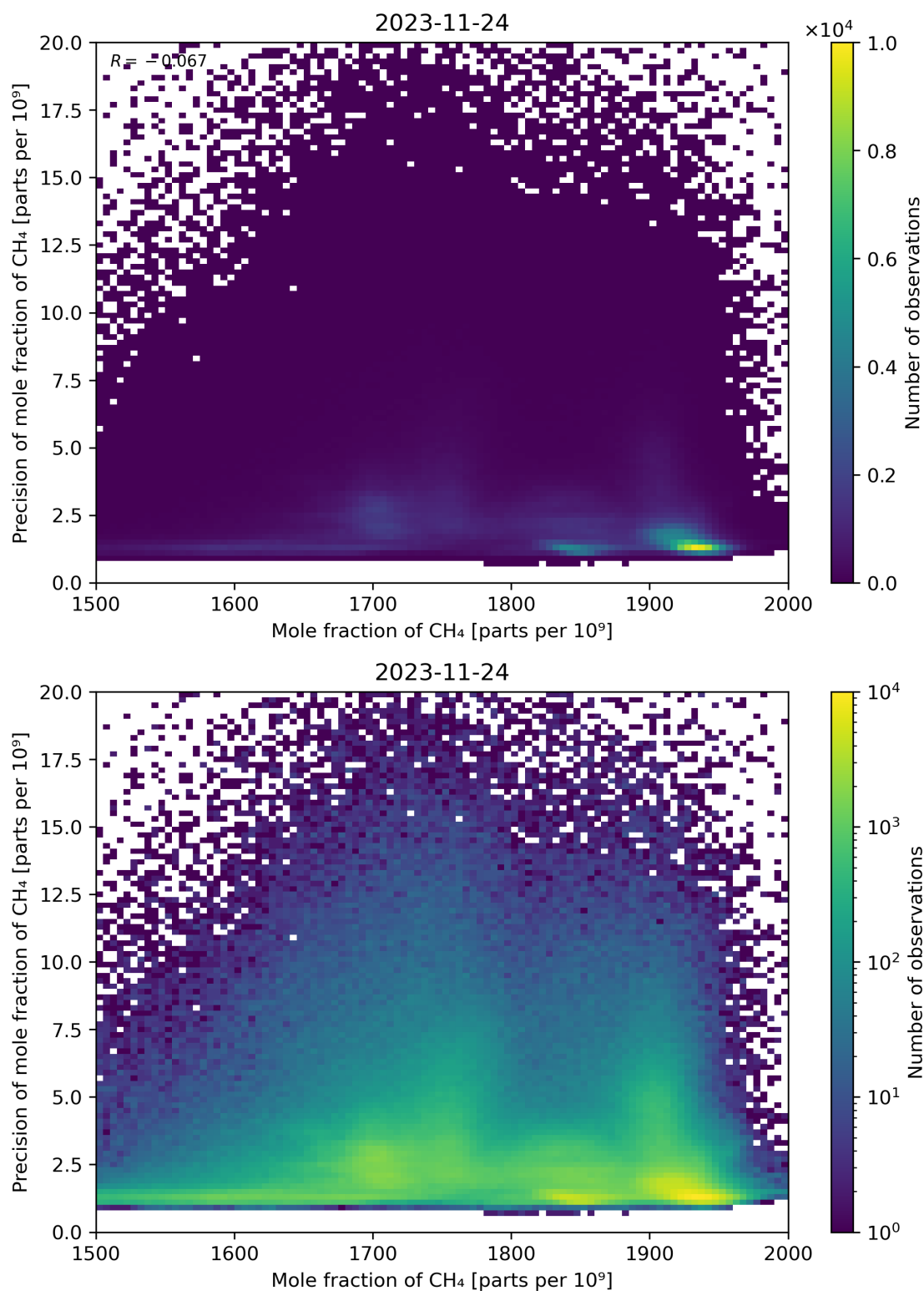
Figure 75: Scatter density plot of “Mole fraction of CH 4 ” against “Precision of mole fraction of CH 4 ” for 2023-11-23 to 2023-11-25.
