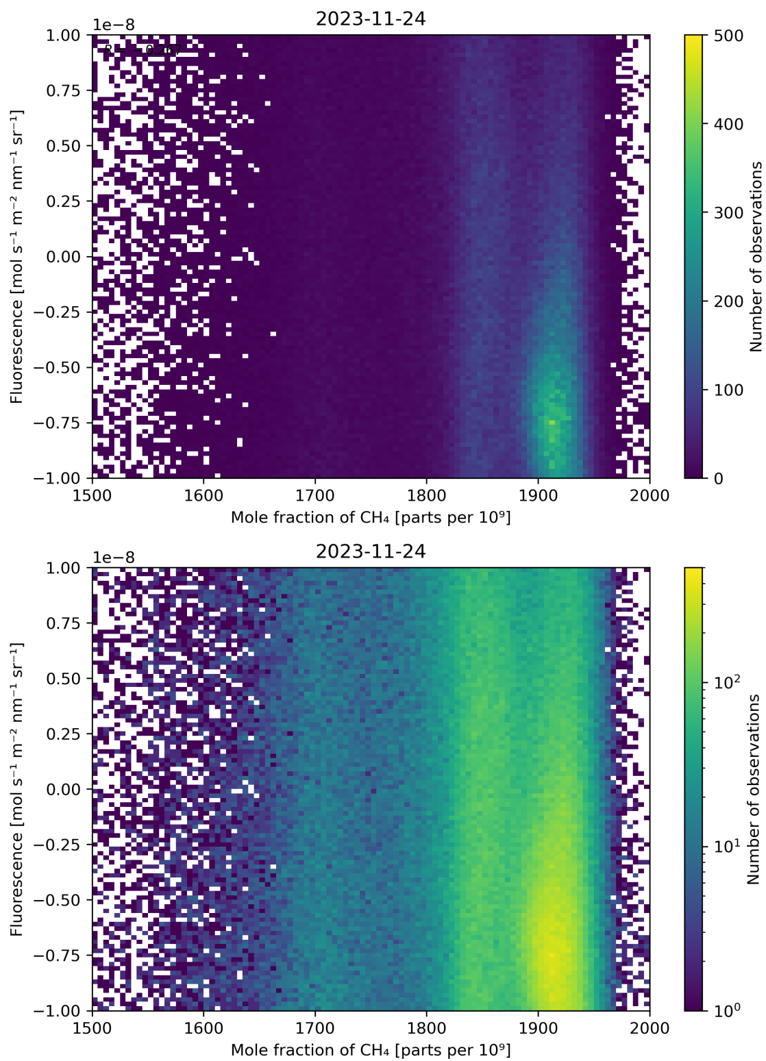
Figure 73: Scatter density plot of “Mole fraction of \text{CH}_4 ” against “Fluorescence” for 2023-11-23 to 2023-11-25.
