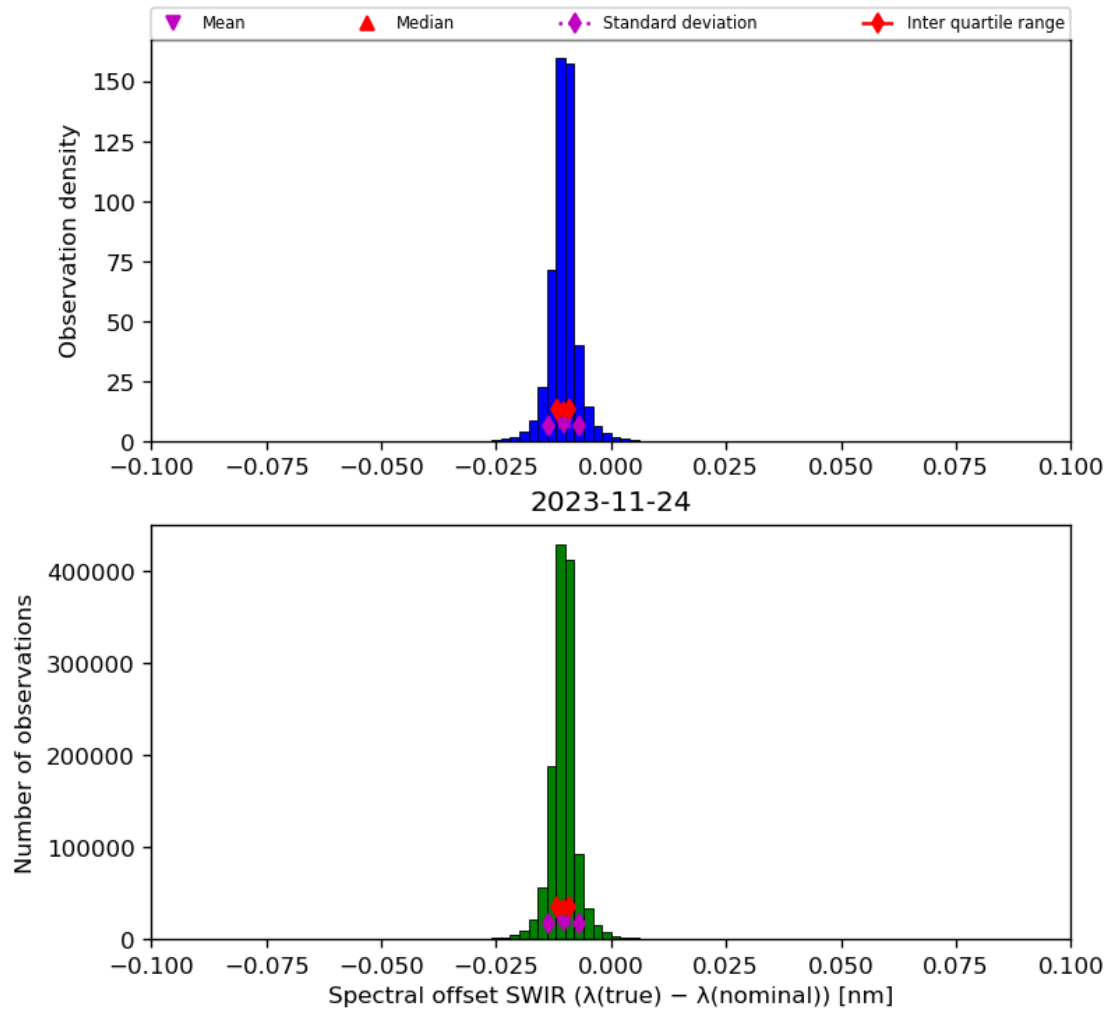
Figure 27: Histogram of “Spectral offset SWIR ( \lambda(\text{true}) - \lambda(\text{nominal}) )” for 2023-11-23 to 2023-11-25
