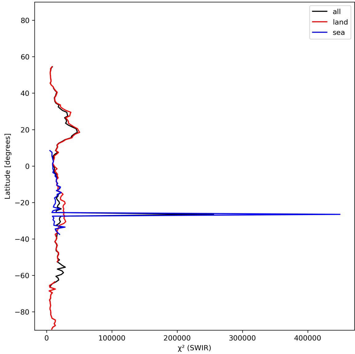
Figure 17: Zonal average of “ \chi^2 (SWIR)” for 2023-11-23 to 2023-11-25.
