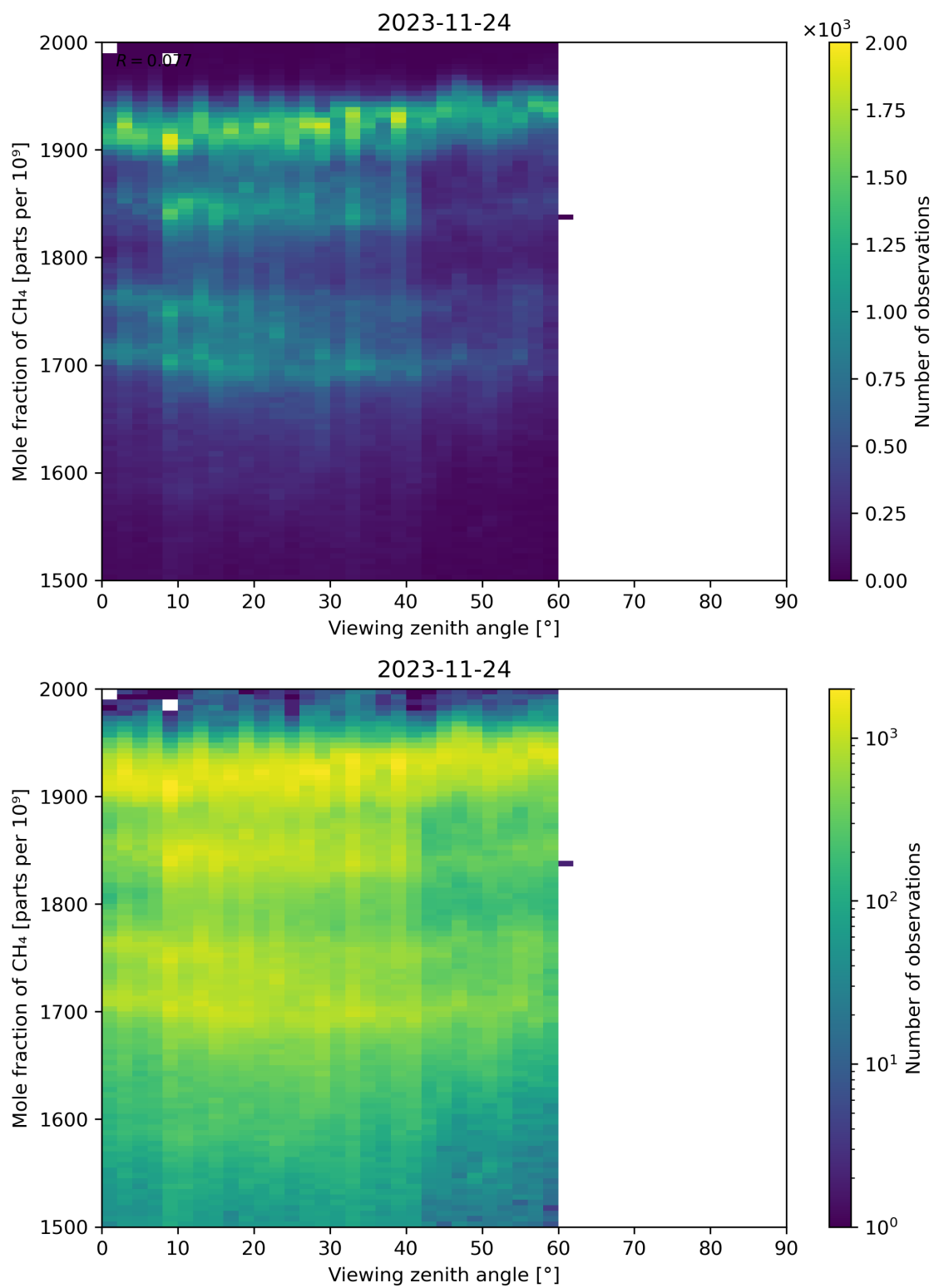
Figure 110: Scatter density plot of “Viewing zenith angle” against “Mole fraction of CH 4 ” for 2023-11-23 to 2023-11-25.
