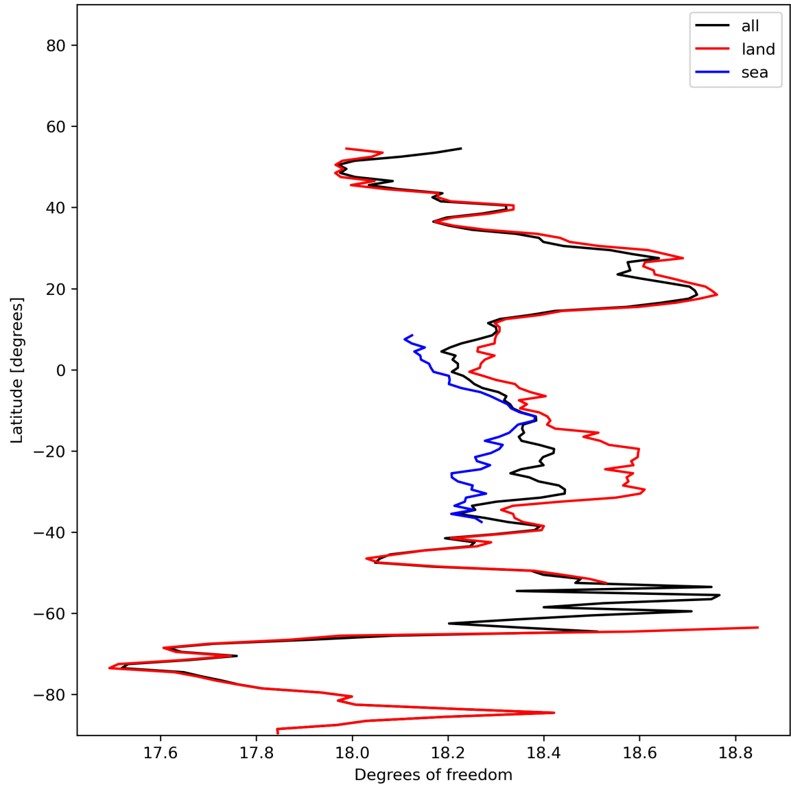
Figure 19: Zonal average of “Degrees of freedom” for 2023-11-23 to 2023-11-25.
