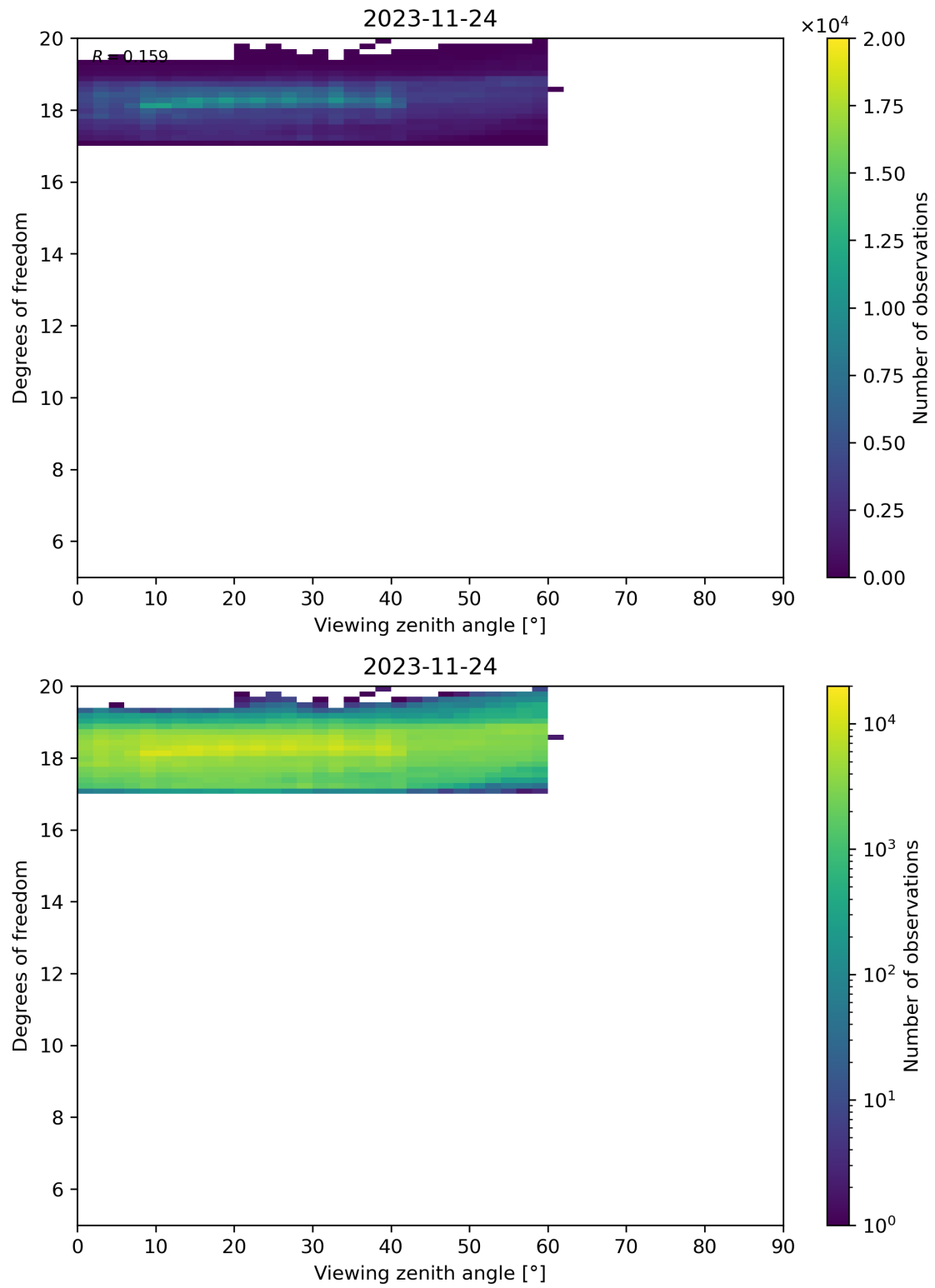
Figure 107: Scatter density plot of “Viewing zenith angle” against “Degrees of freedom” for 2023-11-23 to 2023-11-25.
