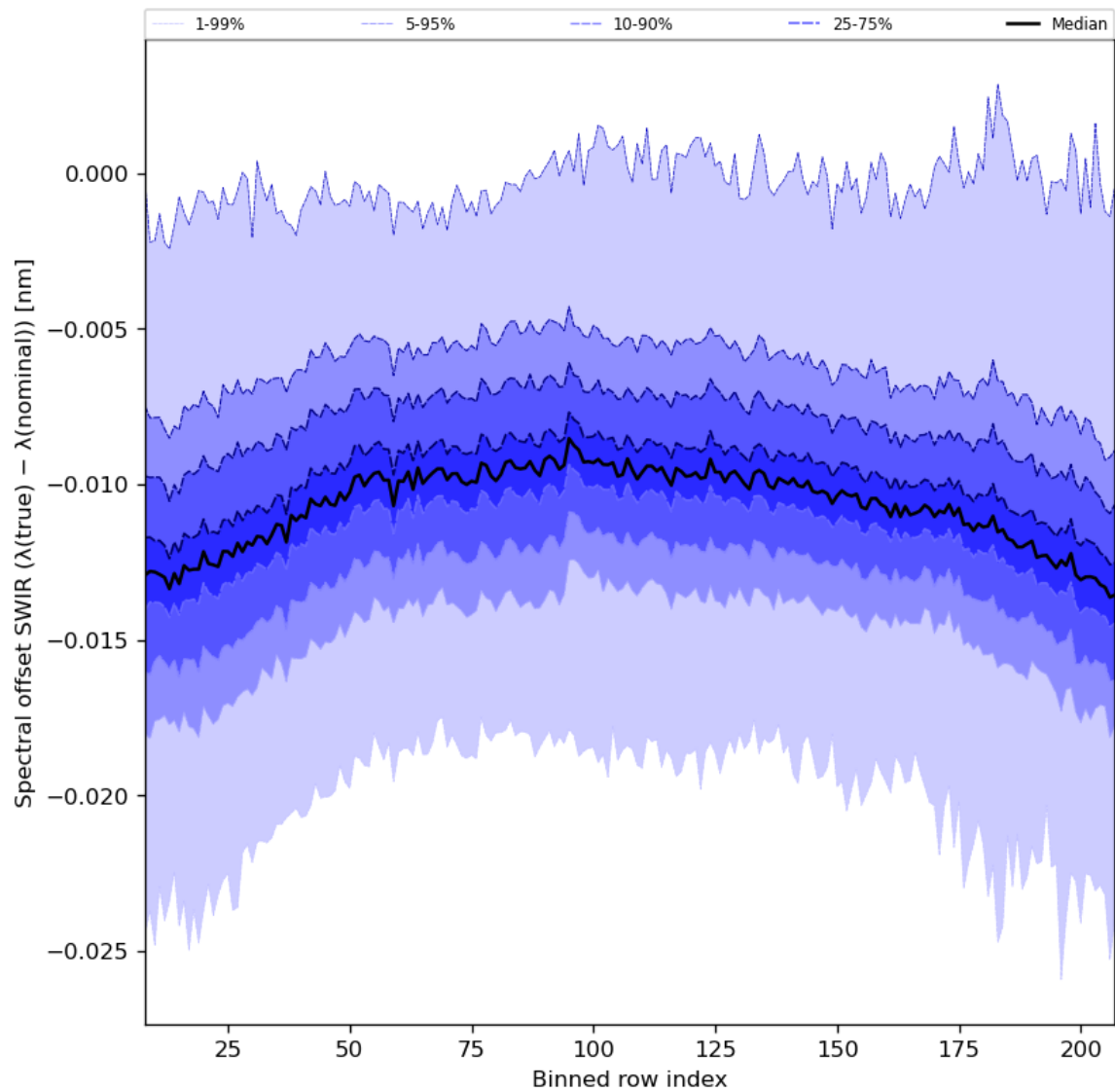
Figure 38: Along track statistics of “Spectral offset SWIR ( \lambda(\text{true}) - \lambda(\text{nominal}) )” for 2023-11-23 to 2023-11-25
