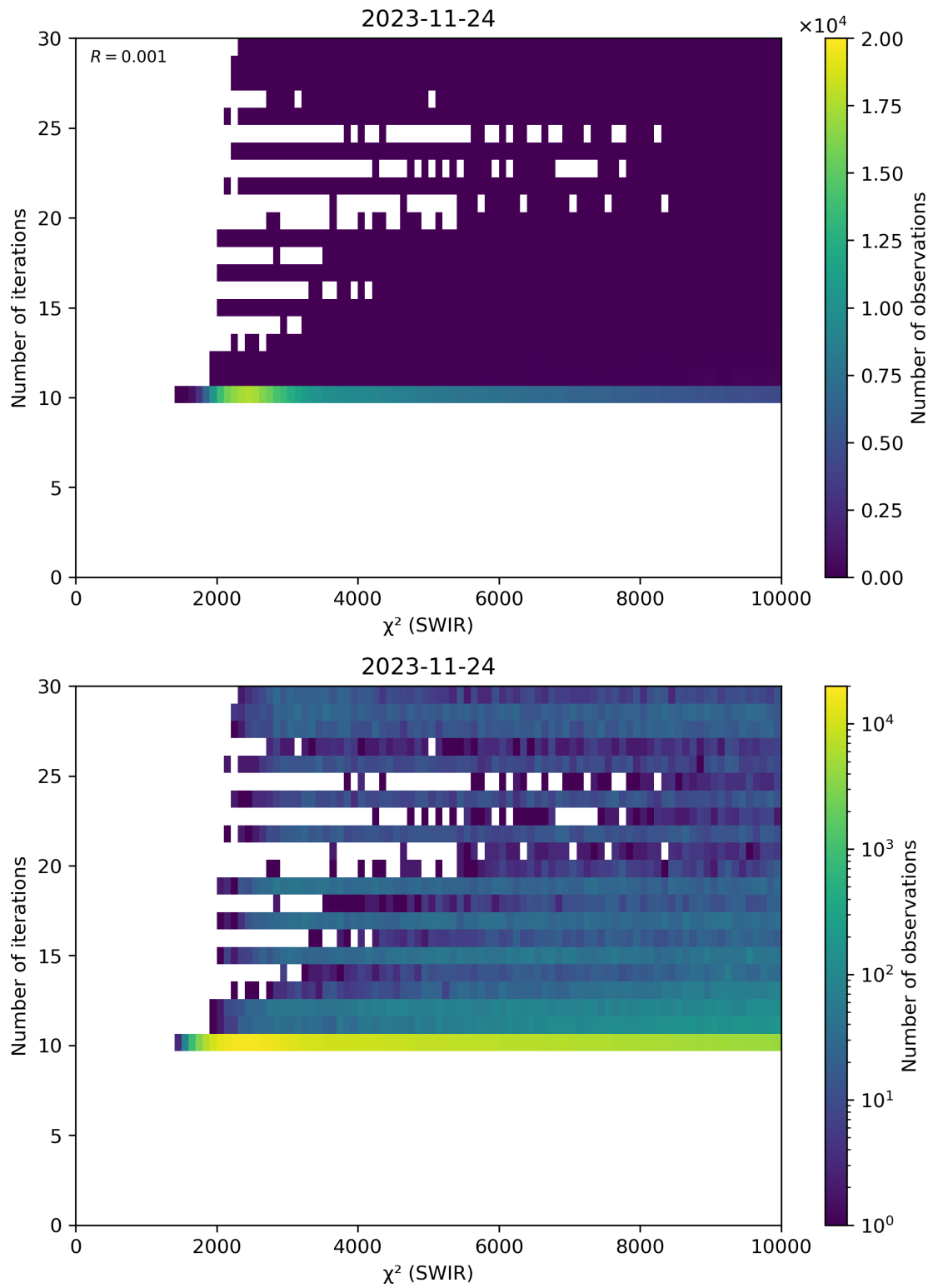
Figure 50: Scatter density plot of “ \chi^2 (SWIR)” against “Number of iterations” for 2023-11-23 to 2023-11-25.
