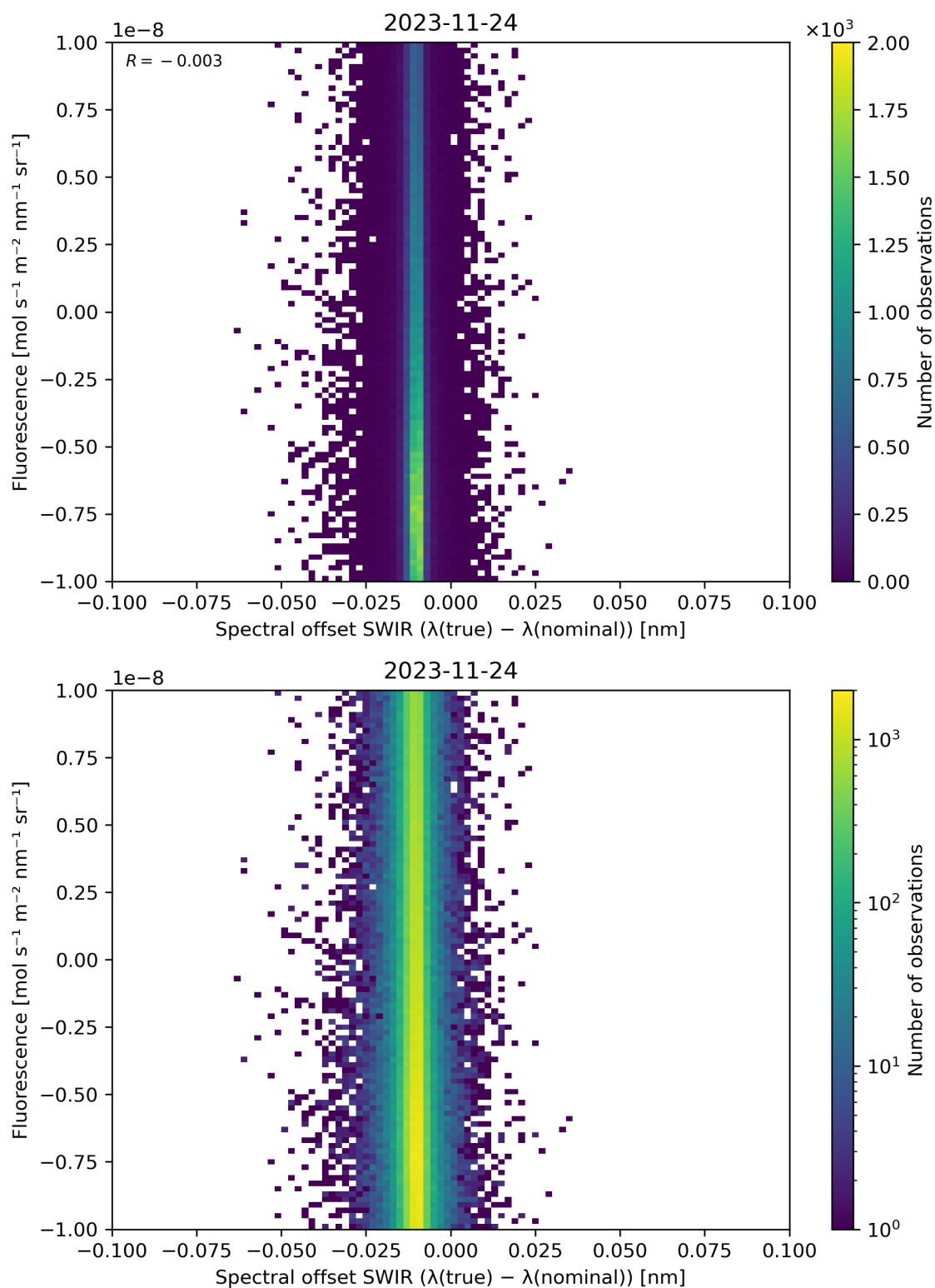
Figure 120: Scatter density plot of “Spectral offset SWIR ( \lambda(\text{true}) - \lambda(\text{nominal}) )” against “Fluorescence” for 2023-11-23 to 2023-11-25.
