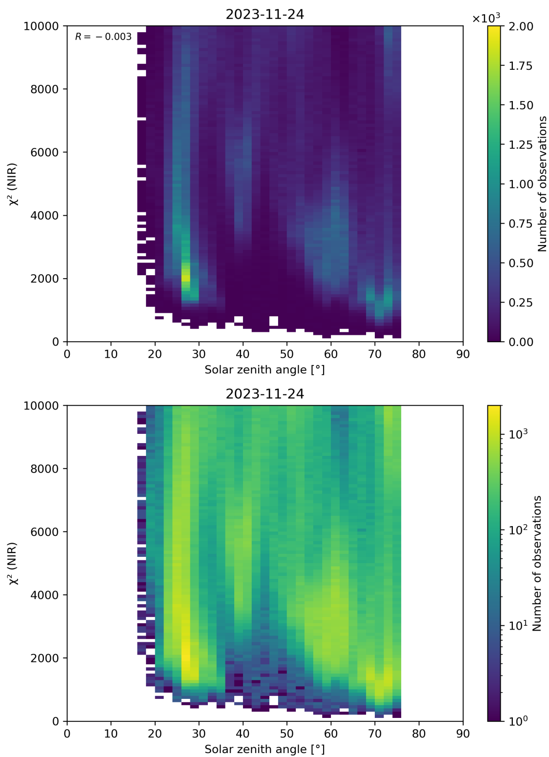
Figure 94: Scatter density plot of “Solar zenith angle” against “ \chi^2 (NIR)” for 2023-11-23 to 2023-11-25.
