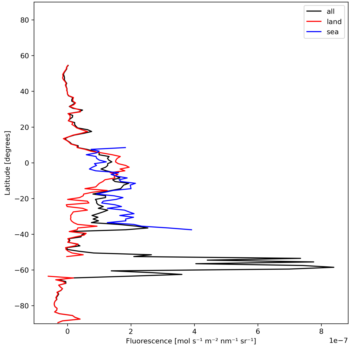
Figure 21: Zonal average of “Fluorescence” for 2023-11-23 to 2023-11-25.
