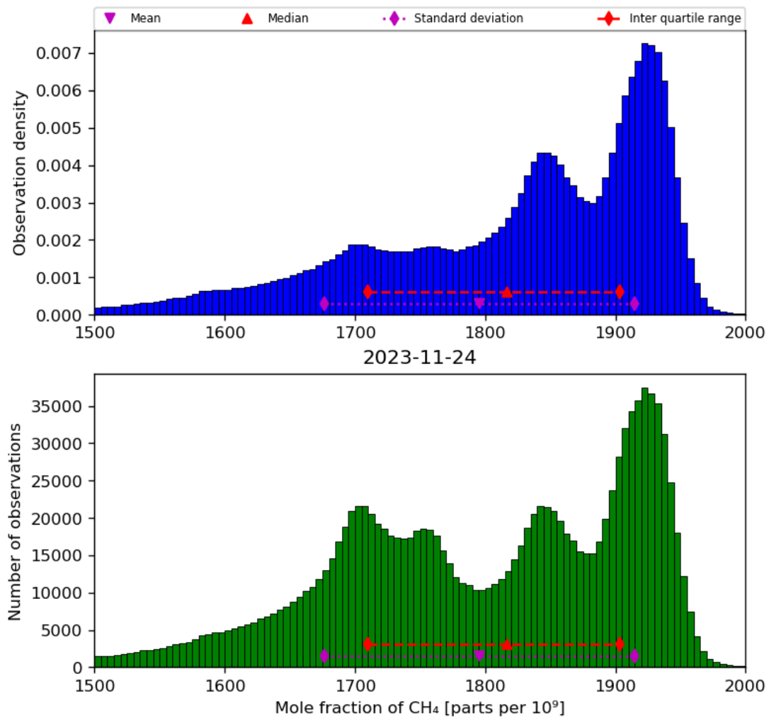
Figure 23: Histogram of “Mole fraction of CH 4 ” for 2023-11-23 to 2023-11-25
