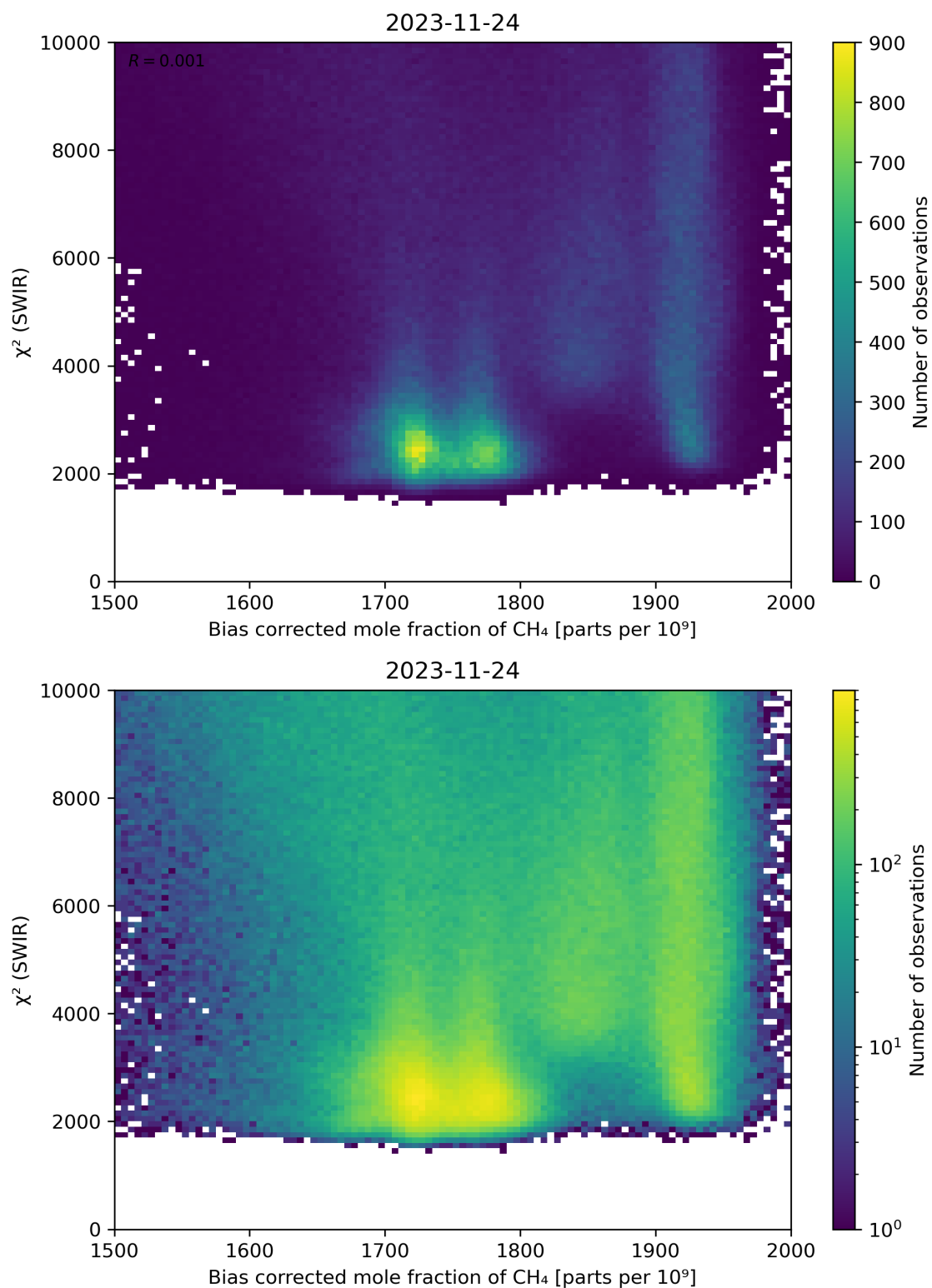
Figure 64: Scatter density plot of “Bias corrected mole fraction of \text{CH}_4 ” against “ \chi^2 (SWIR)” for 2023-11-23 to 2023-11-25.
