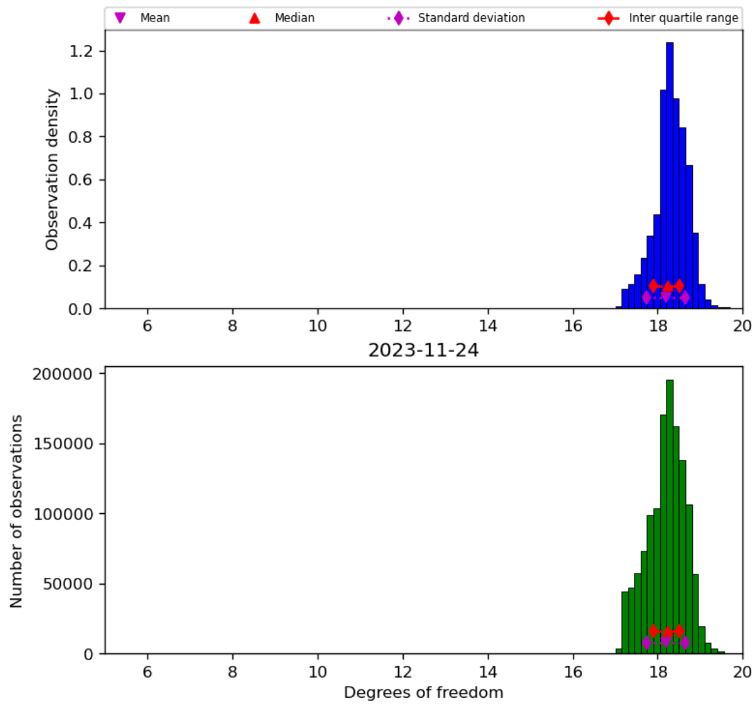
Figure 30: Histogram of “Degrees of freedom” for 2023-11-23 to 2023-11-25
