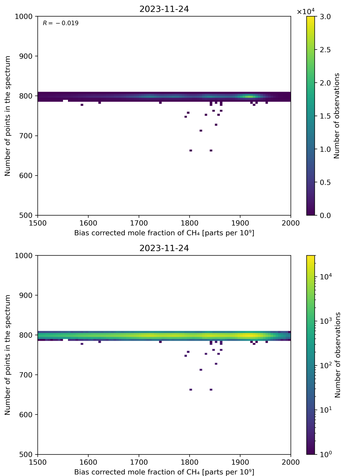
Figure 68: Scatter density plot of “Bias corrected mole fraction of CH 4 ” against “Number of points in the spectrum” for 2023-11-23 to 2023-11-25.
