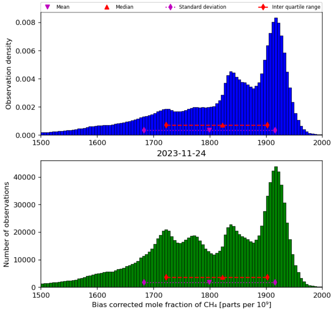
Figure 25: Histogram of “Bias corrected mole fraction of CH 4 ” for 2023-11-23 to 2023-11-25
