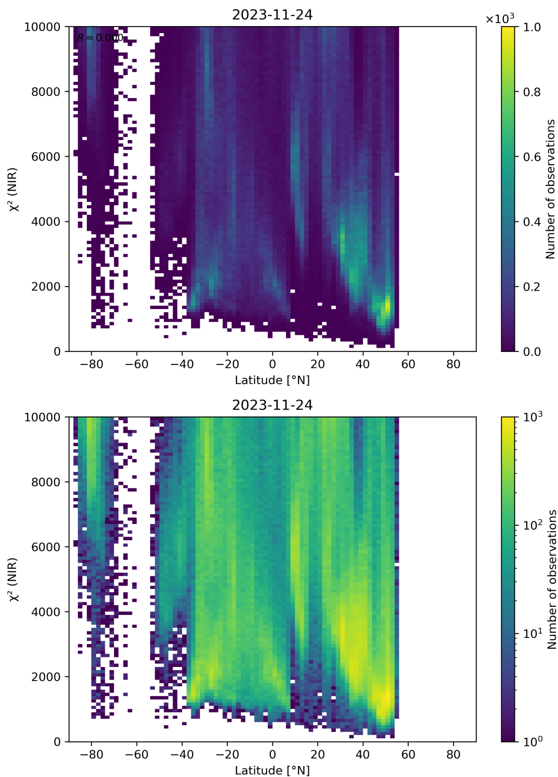
Figure 53: Scatter density plot of “Latitude” against “ \chi^2 (NIR)” for 2023-11-23 to 2023-11-25.
