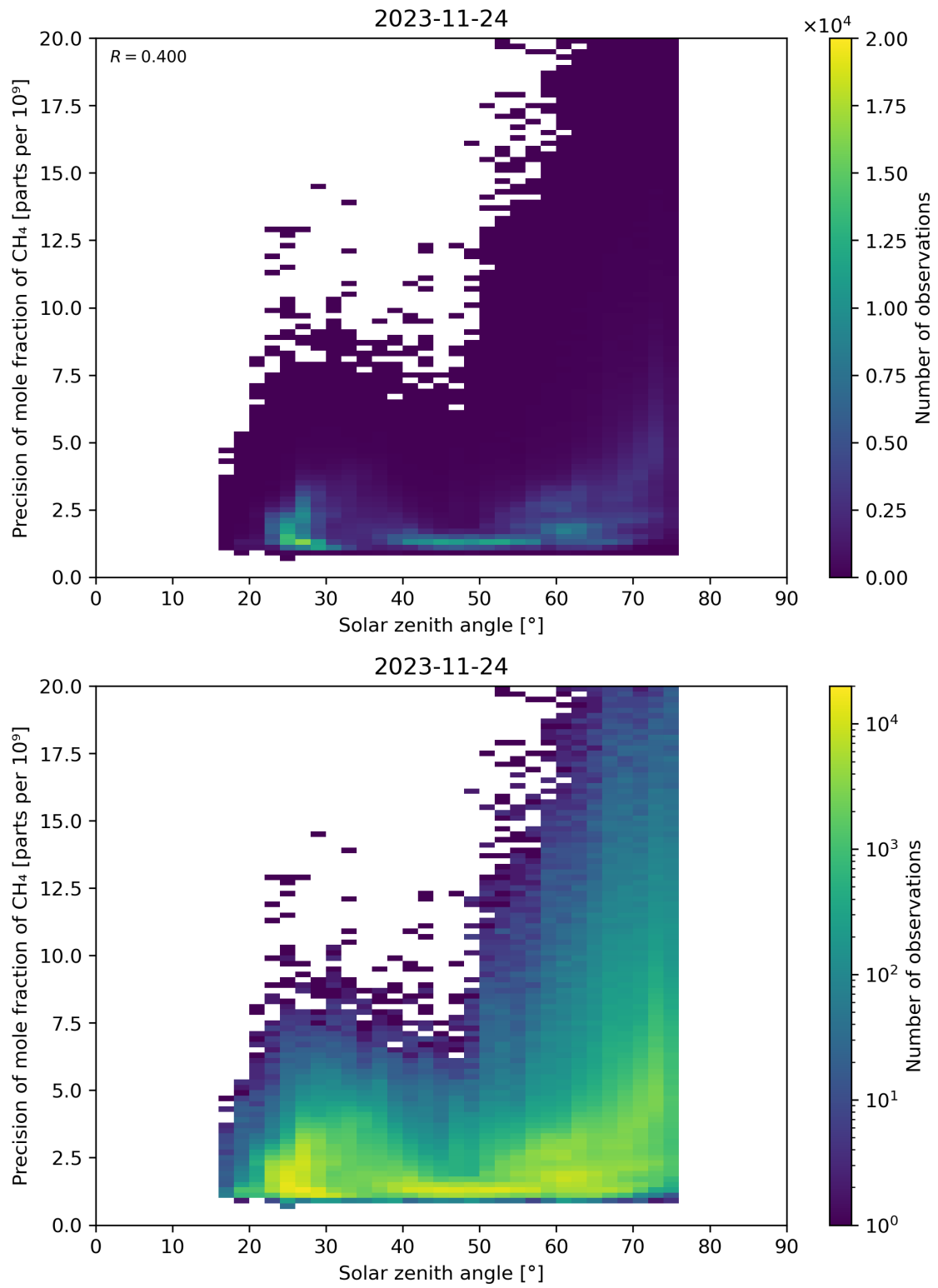
Figure 101: Scatter density plot of “Solar zenith angle” against “Precision of mole fraction of \text{CH}_4 ” for 2023-11-23 to 2023-11-25.
