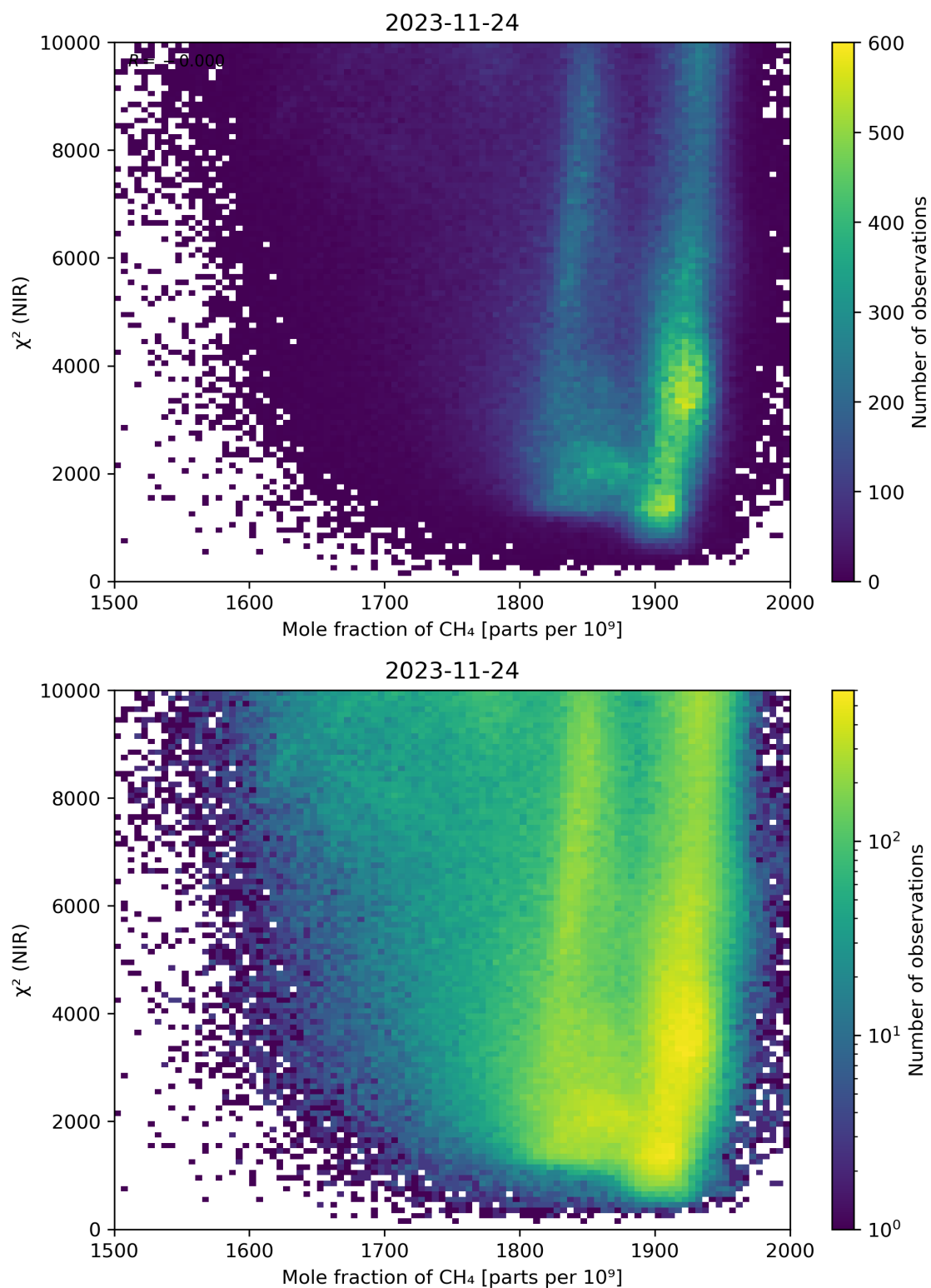
Figure 70: Scatter density plot of “Mole fraction of CH 4 ” against “ \chi^2 (NIR)” for 2023-11-23 to 2023-11-25.
