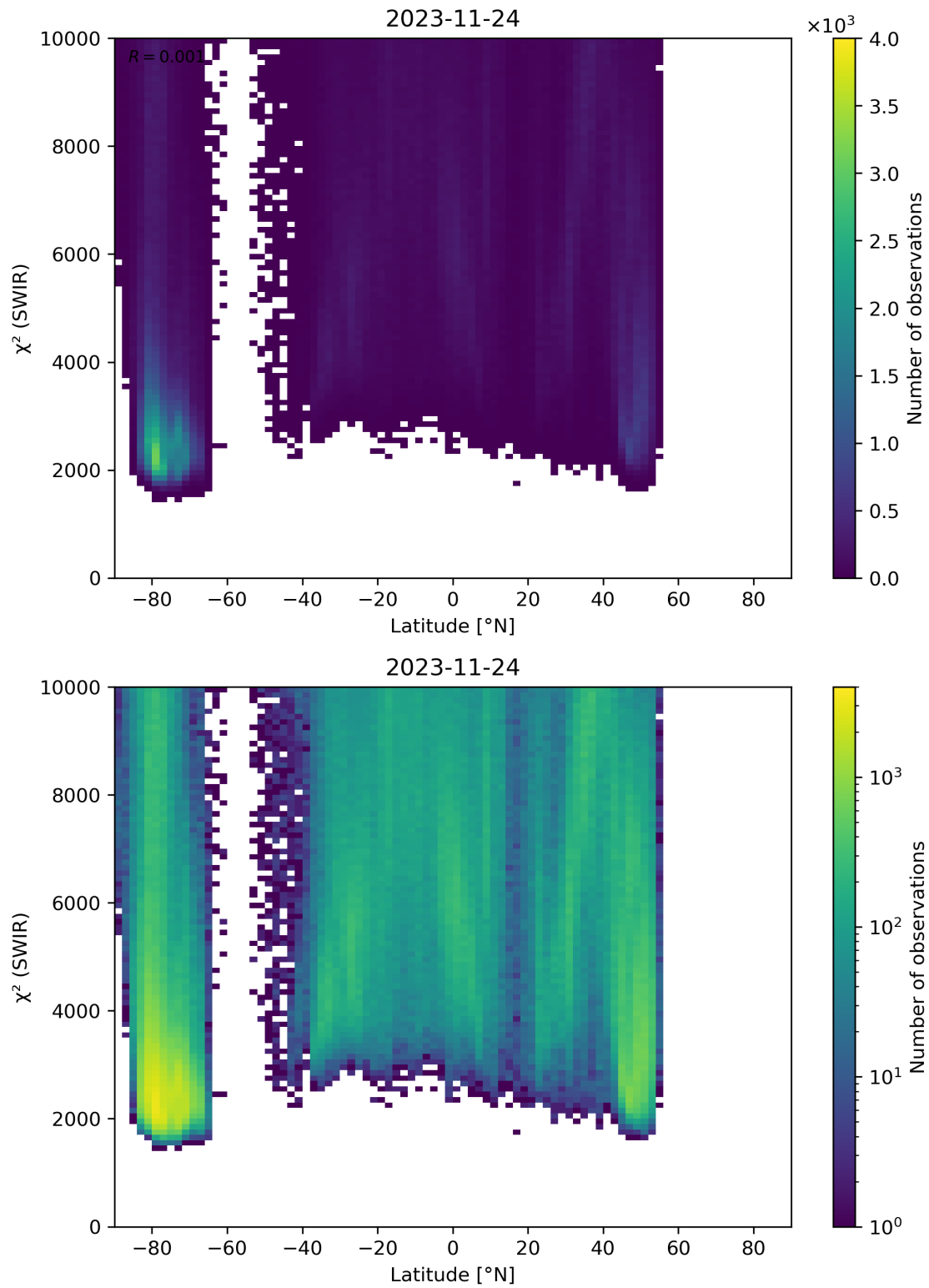
Figure 54: Scatter density plot of “Latitude” against “ \chi^2 (SWIR)” for 2023-11-23 to 2023-11-25.
