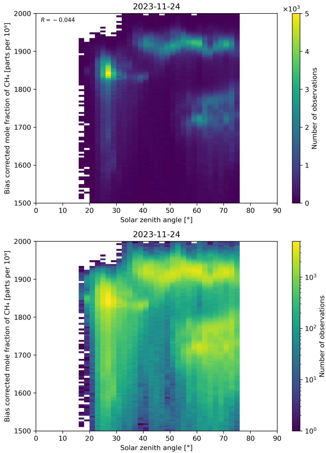
Figure 100: Scatter density plot of “Solar zenith angle” against “Bias corrected mole fraction of CH 4 ” for 2023-11-23 to 2023-11-25.
