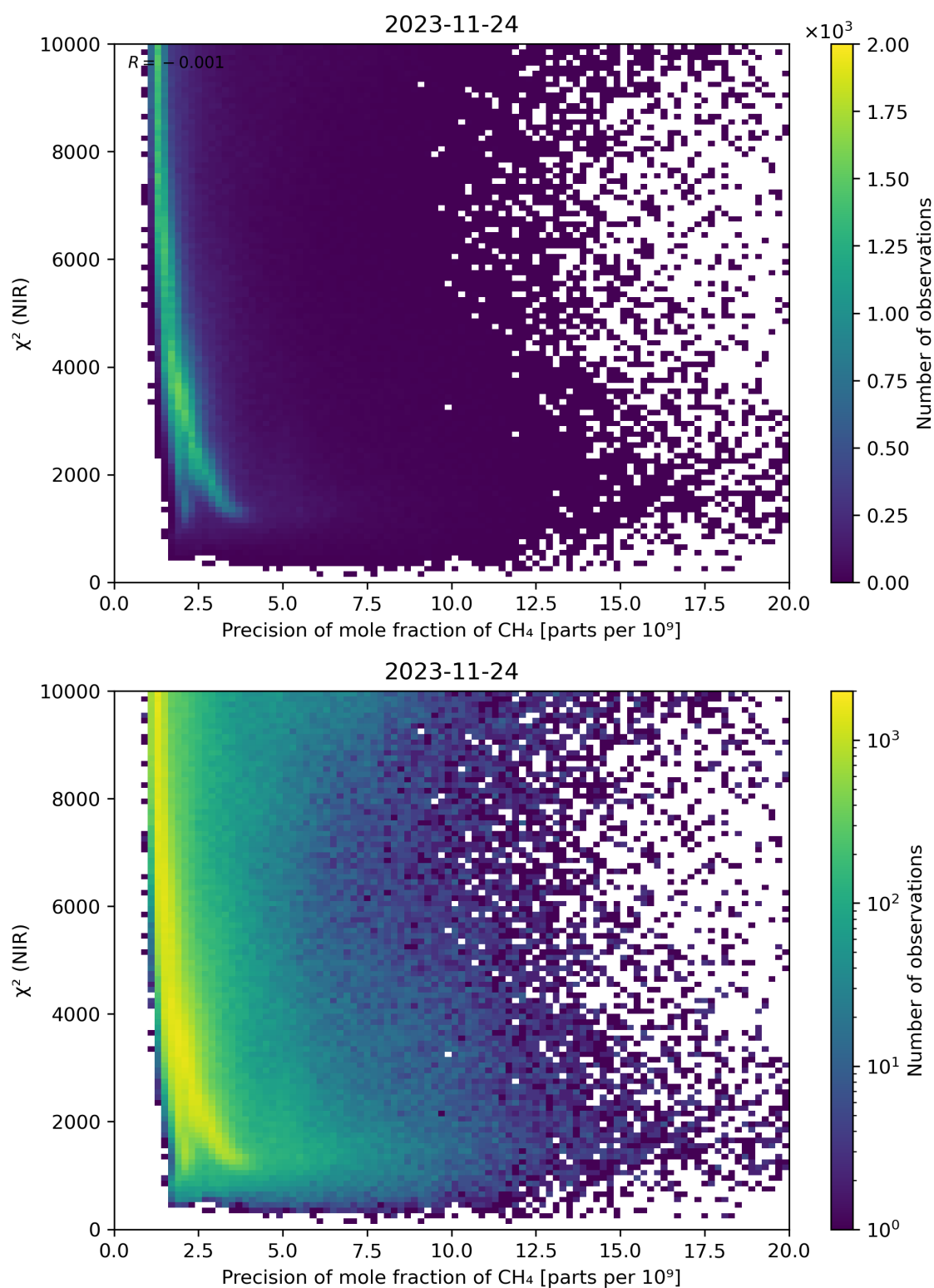
Figure 78: Scatter density plot of “Precision of mole fraction of CH 4 ” against “ \chi^2 (NIR)” for 2023-11-23 to 2023-11-25.
