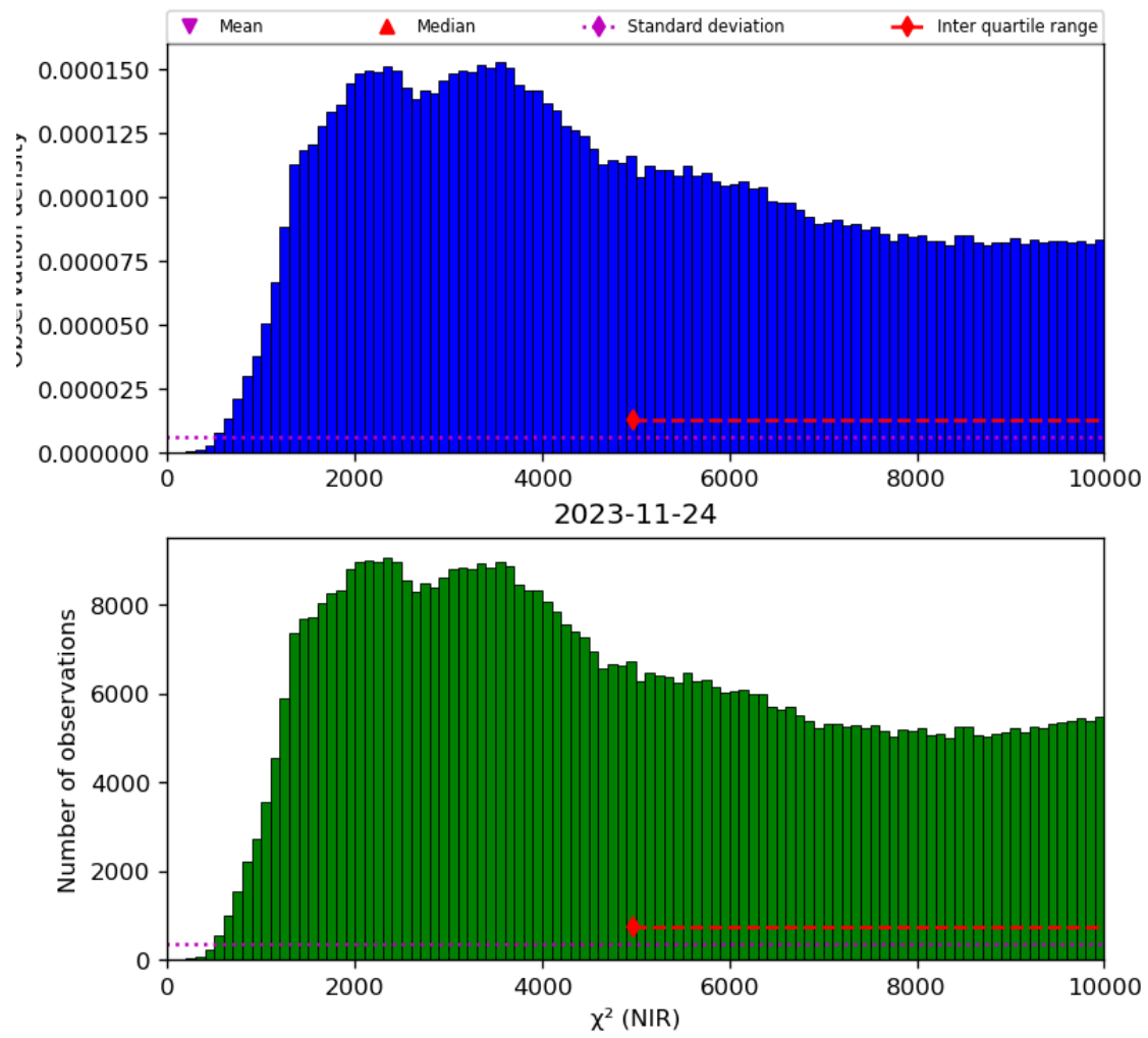
Figure 29: Histogram of “ \chi^2 (NIR)” for 2023-11-23 to 2023-11-25
