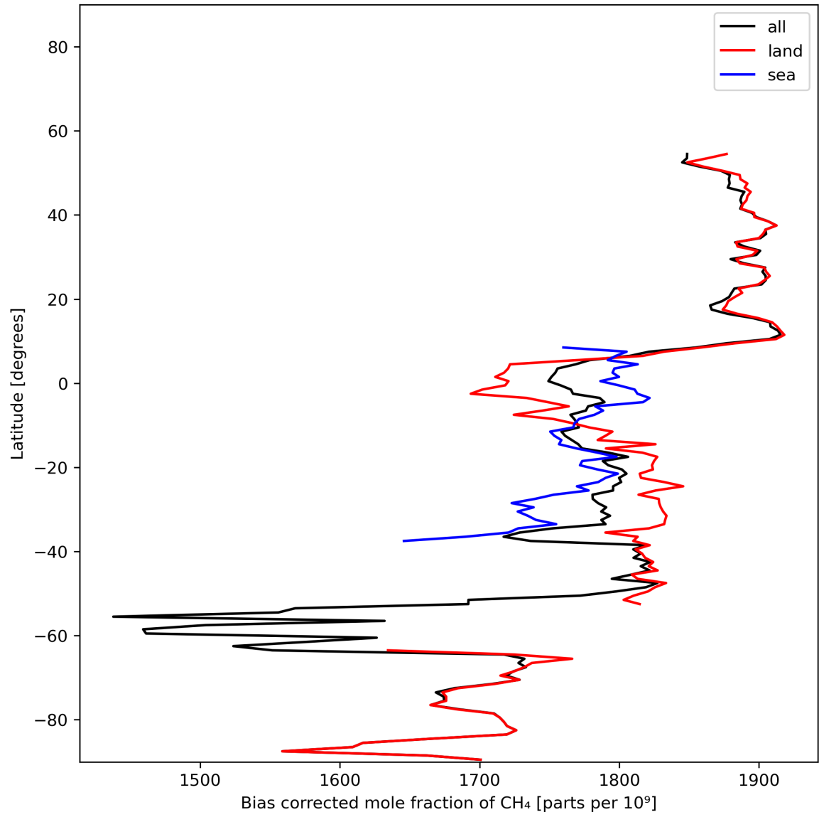
Figure 14: Zonal average of “Bias corrected mole fraction of CH 4 ” for 2023-11-23 to 2023-11-25.
