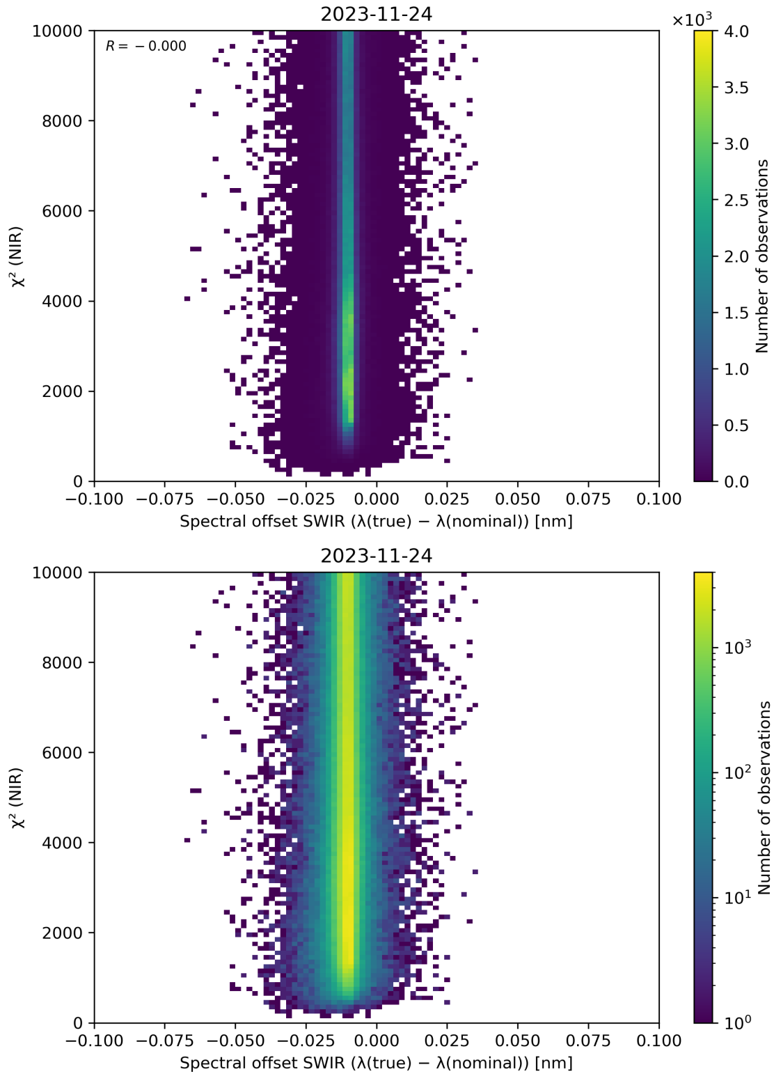
Figure 117: Scatter density plot of “Spectral offset SWIR ( \lambda(\text{true}) - \lambda(\text{nominal}) )” against “ \chi^2 (NIR)” for 2023-11-23 to 2023-11-25.
