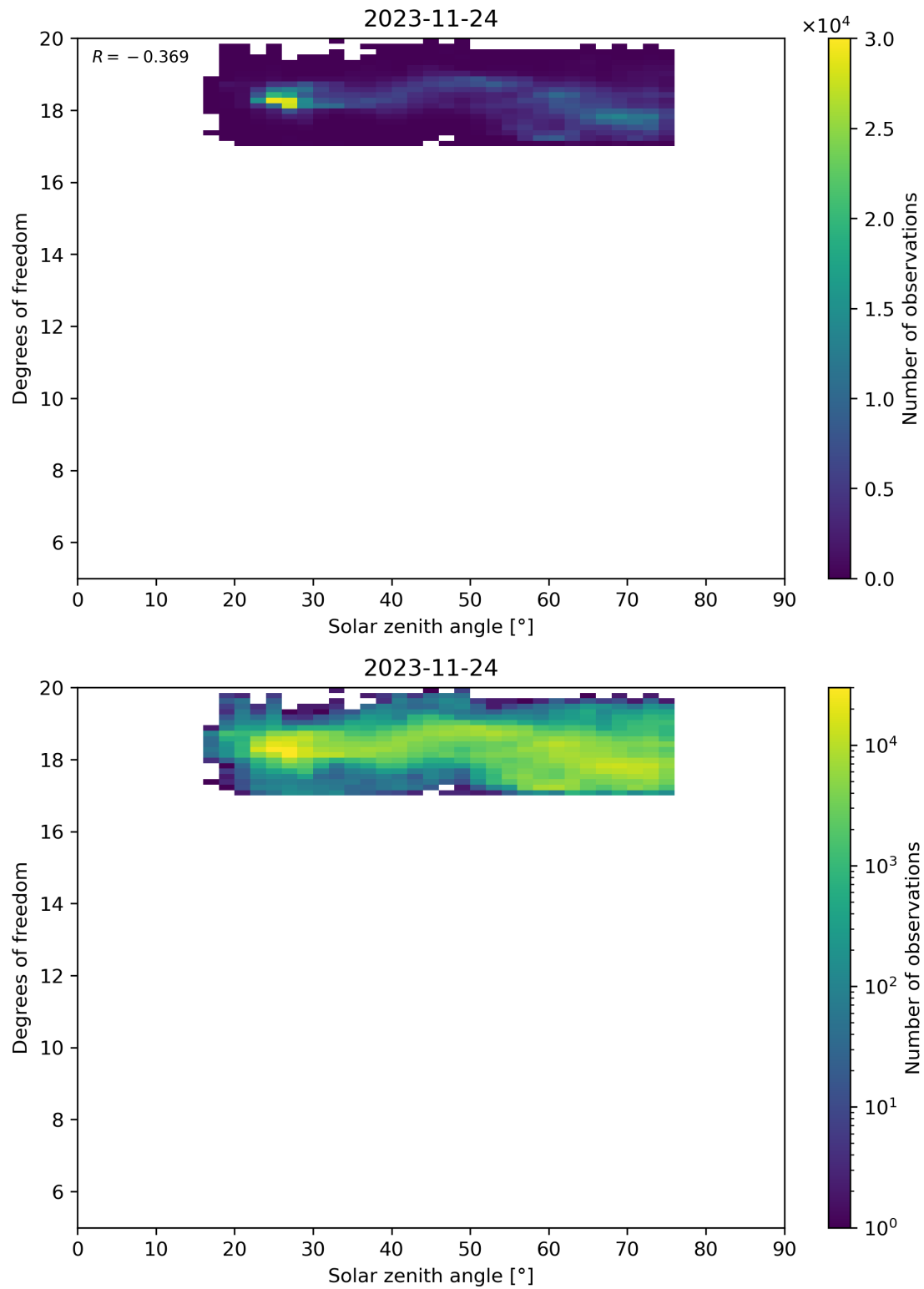
Figure 96: Scatter density plot of “Solar zenith angle” against “Degrees of freedom” for 2023-11-23 to 2023-11-25.
