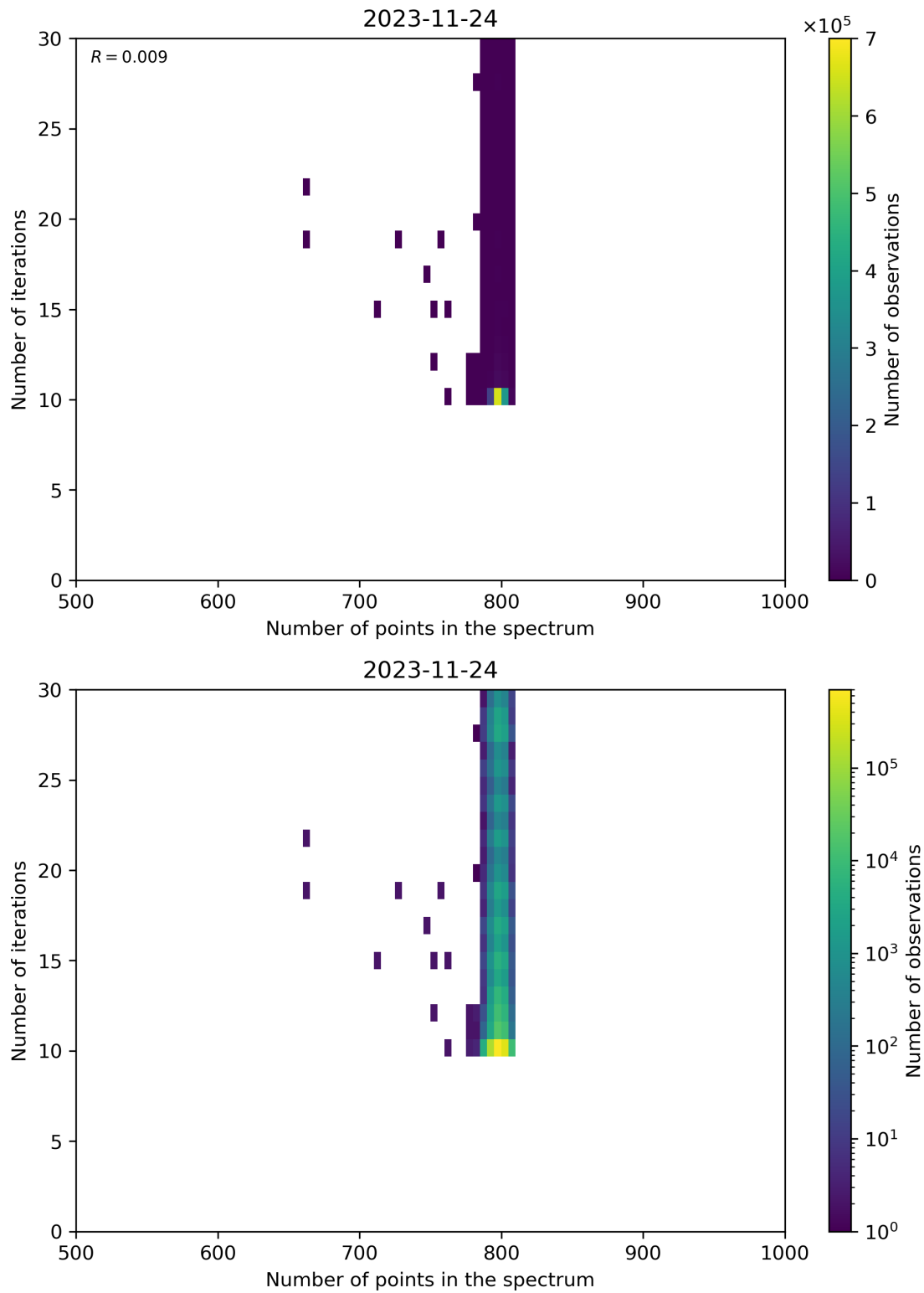
Figure 92: Scatter density plot of “Number of points in the spectrum” against “Number of iterations” for 2023-11-23 to 2023-11-25.
