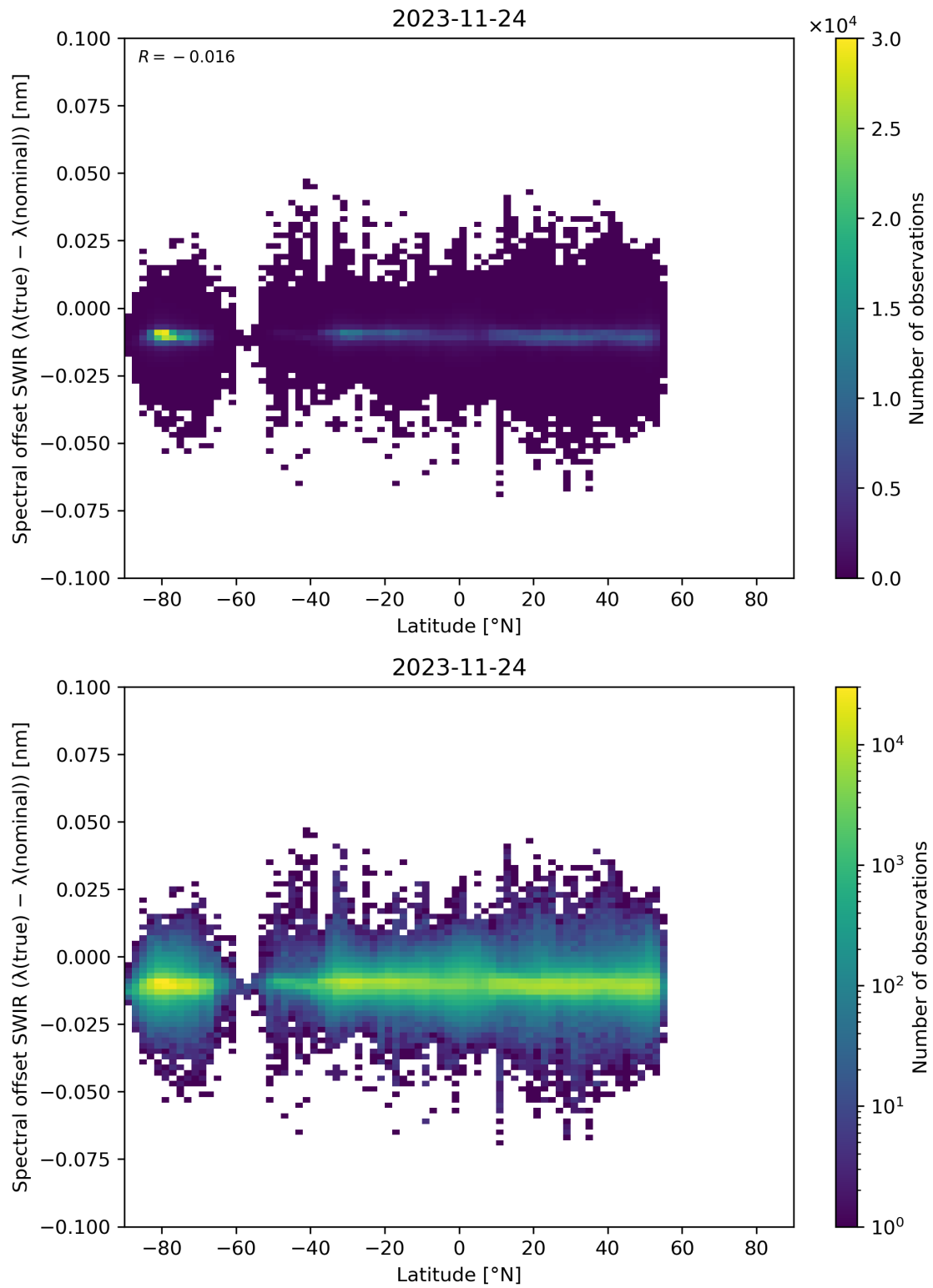
Figure 62: Scatter density plot of “Latitude” against “Spectral offset SWIR ( \lambda(\text{true}) - \lambda(\text{nominal}) )” for 2023-11-23 to 2023-11-25.
