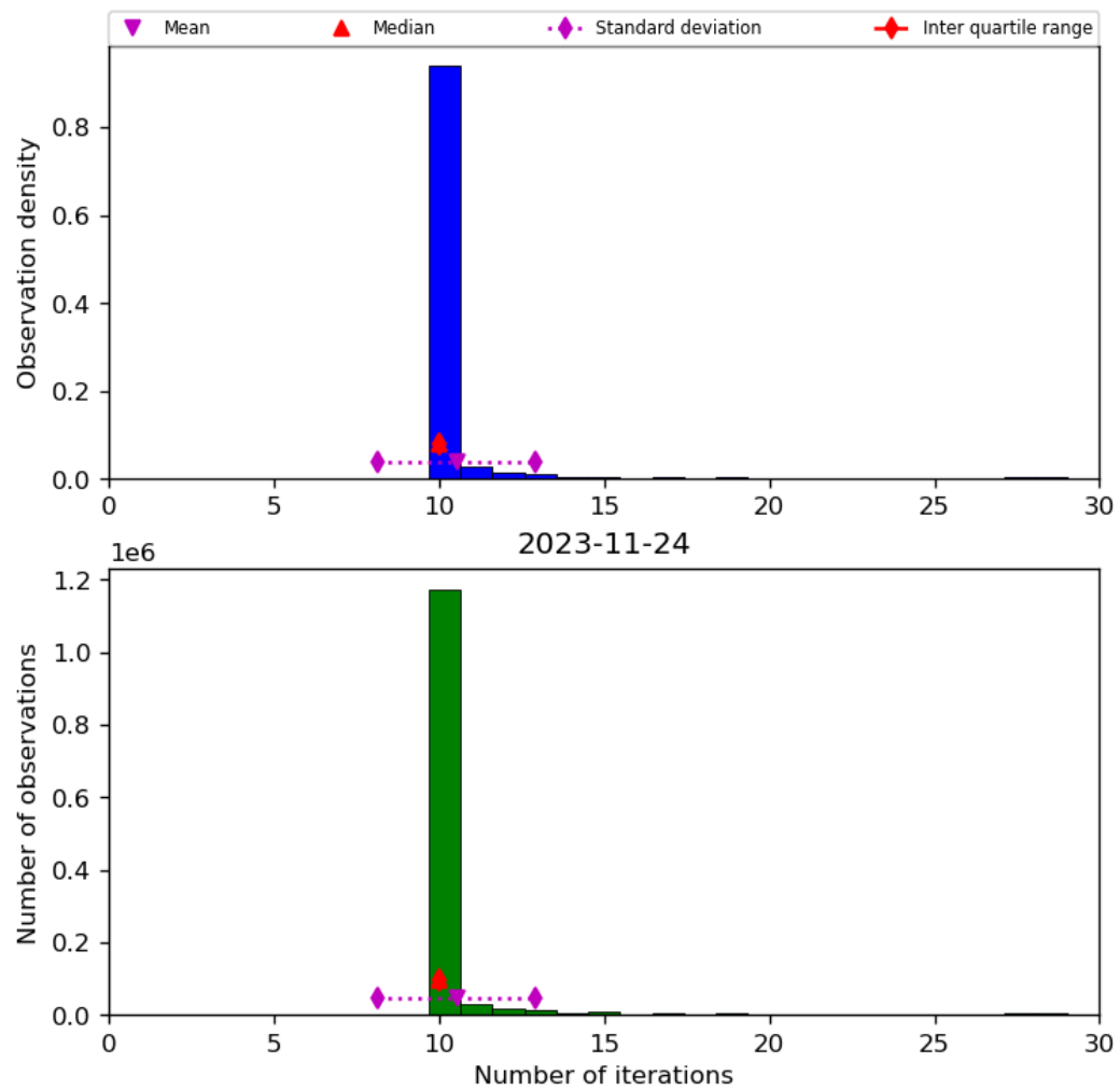
Figure 31: Histogram of “Number of iterations” for 2023-11-23 to 2023-11-25
