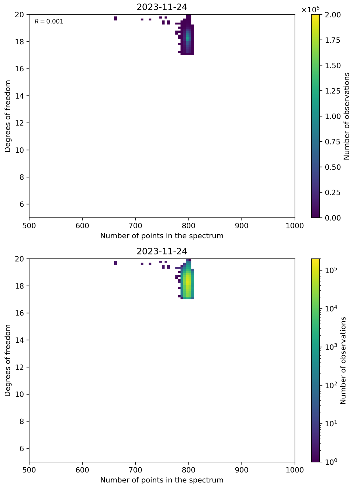
Figure 90: Scatter density plot of “Number of points in the spectrum” against “Degrees of freedom” for 2023-11-23 to 2023-11-25.
