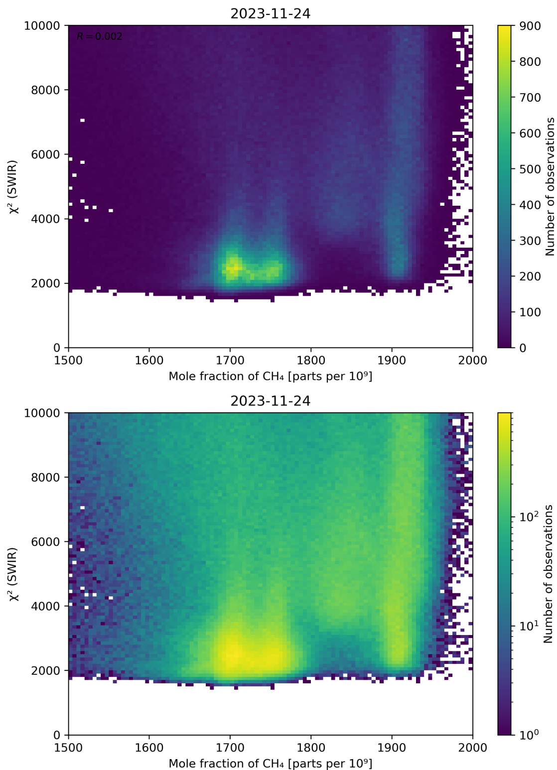
Figure 71: Scatter density plot of “Mole fraction of \text{CH}_4 ” against “ \chi^2 (SWIR)” for 2023-11-23 to 2023-11-25.
