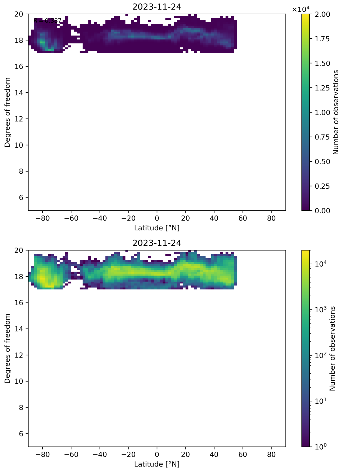
Figure 55: Scatter density plot of “Latitude” against “Degrees of freedom” for 2023-11-23 to 2023-11-25.
