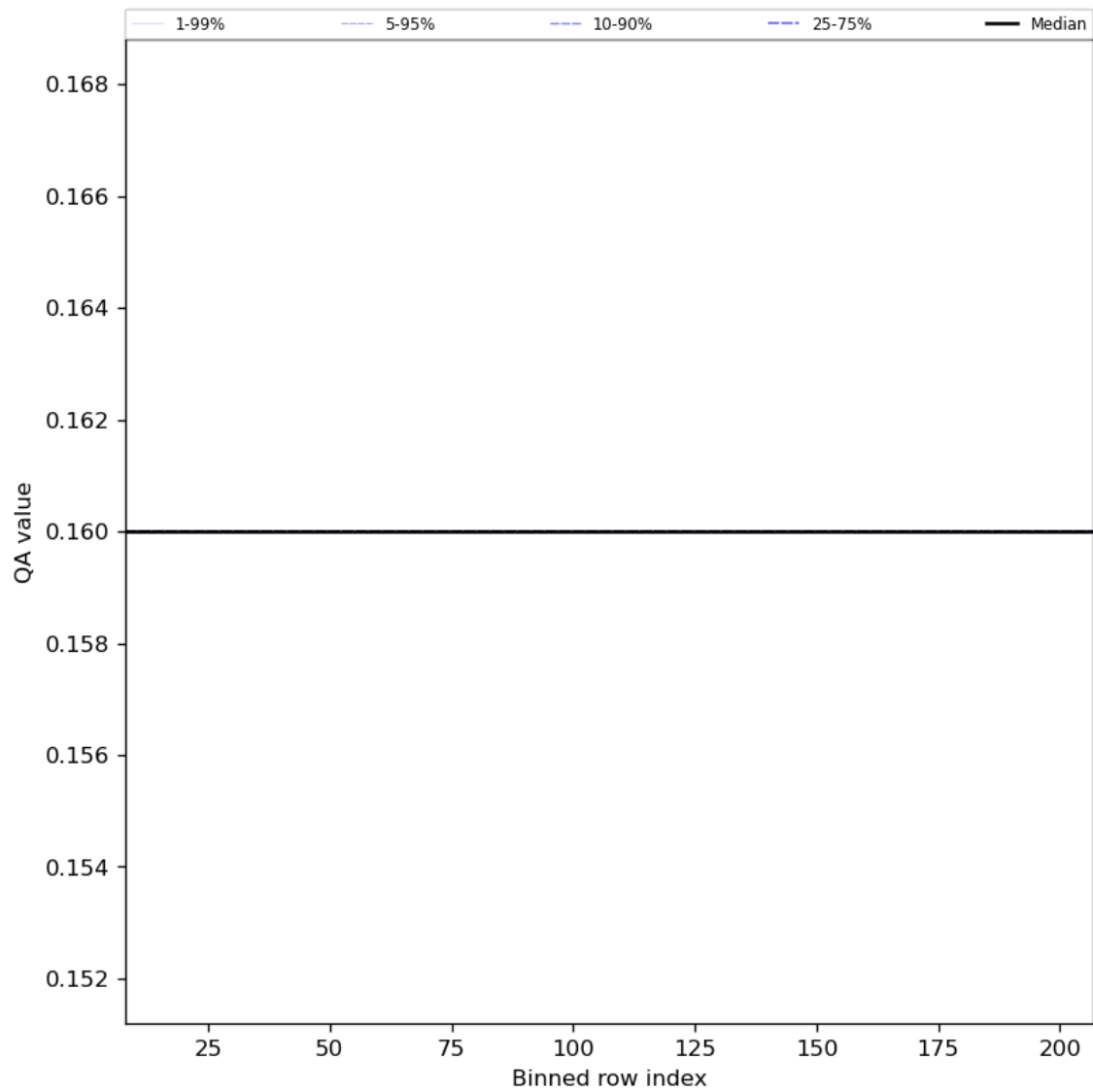
Figure 33: Along track statistics of “QA value” for 2023-11-23 to 2023-11-25
