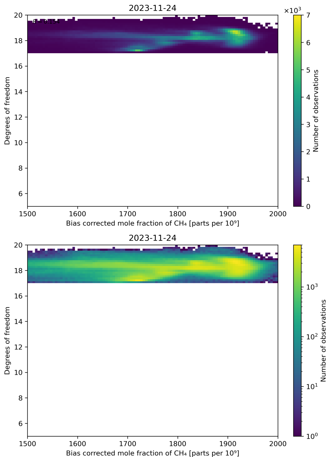
Figure 65: Scatter density plot of “Bias corrected mole fraction of CH 4 ” against “Degrees of freedom” for 2023-11-23 to 2023-11-25.
