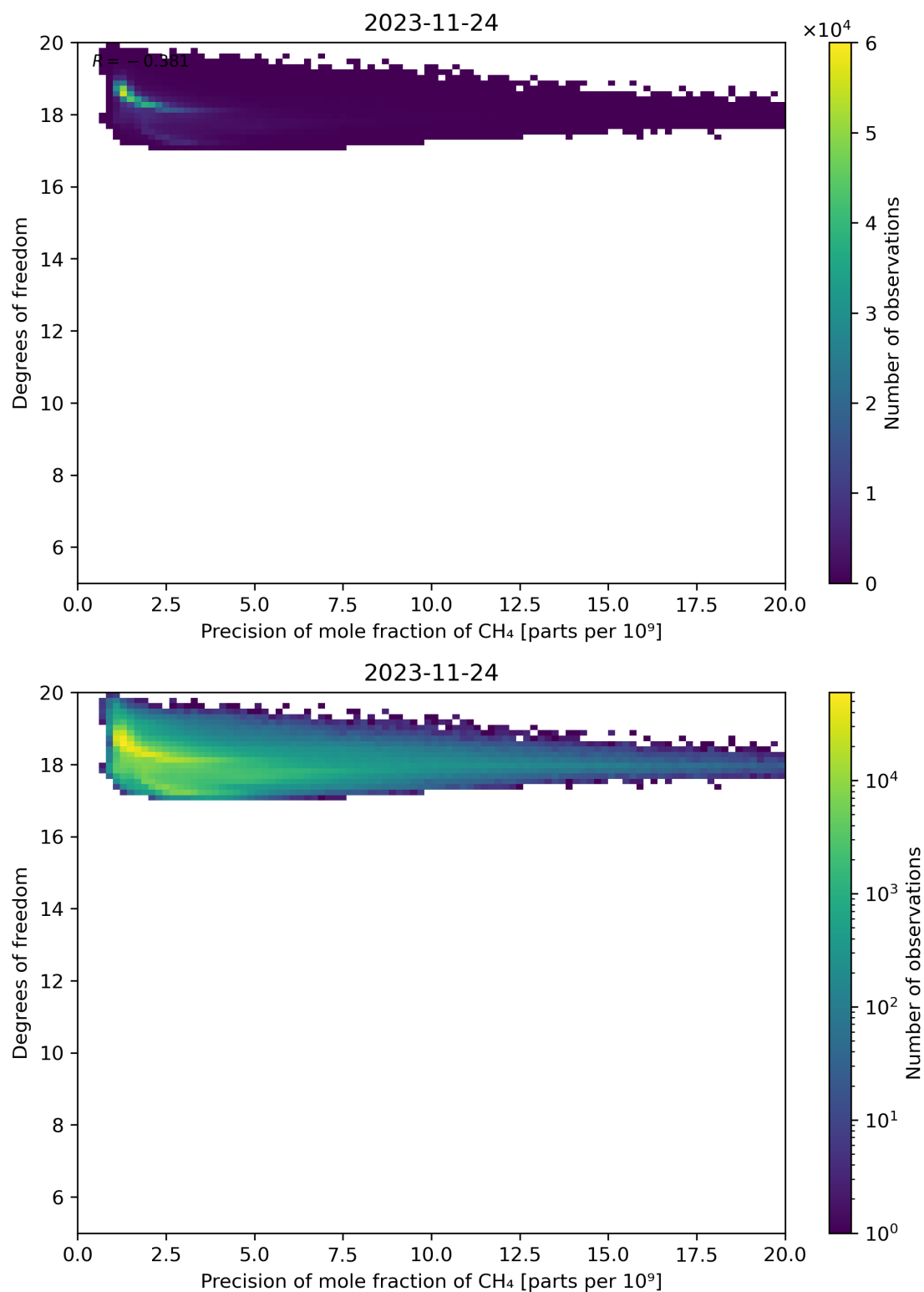
Figure 80: Scatter density plot of “Precision of mole fraction of CH 4 ” against “Degrees of freedom” for 2023-11-23 to 2023-11-25.
