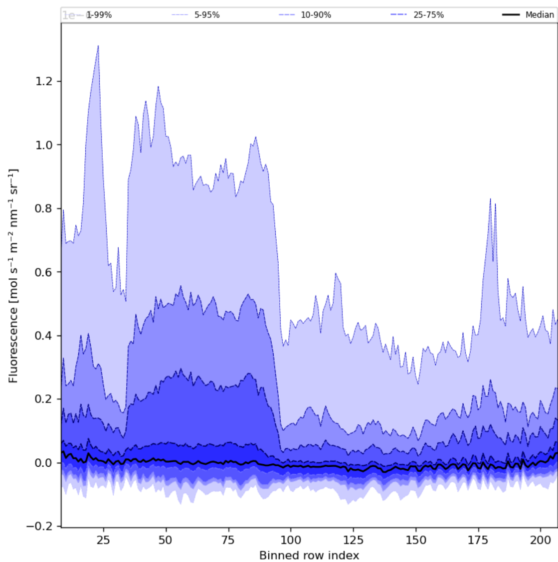
Figure 43: Along track statistics of “Fluorescence” for 2023-11-23 to 2023-11-25
