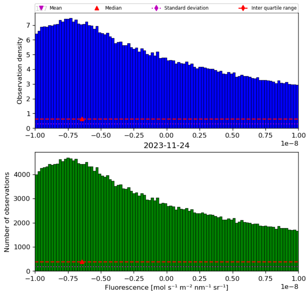
Figure 32: Histogram of “Fluorescence” for 2023-11-23 to 2023-11-25
