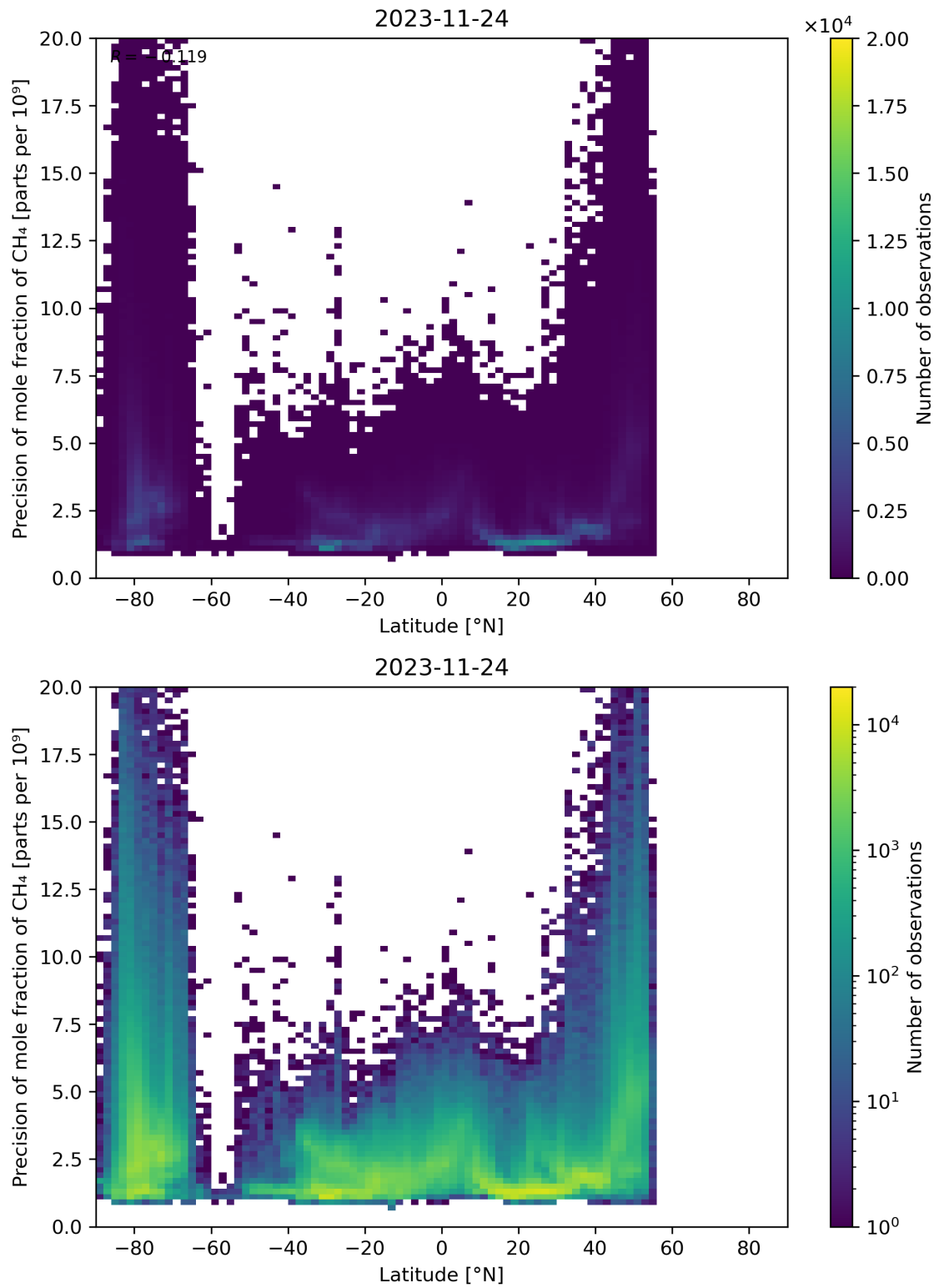
Figure 59: Scatter density plot of “Latitude” against “Precision of mole fraction of CH 4 ” for 2023-11-23 to 2023-11-25.
