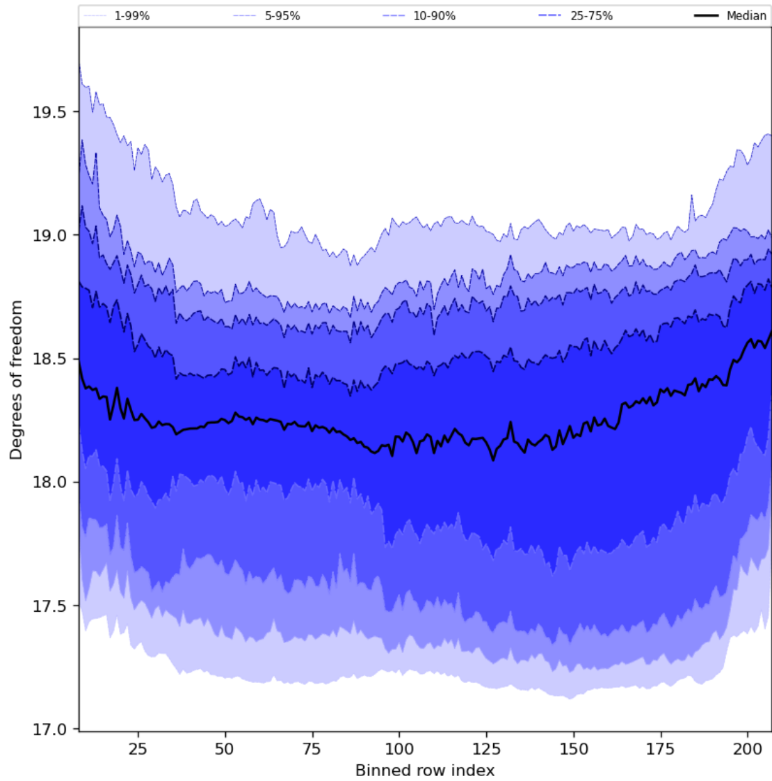
Figure 41: Along track statistics of “Degrees of freedom” for 2023-11-23 to 2023-11-25
