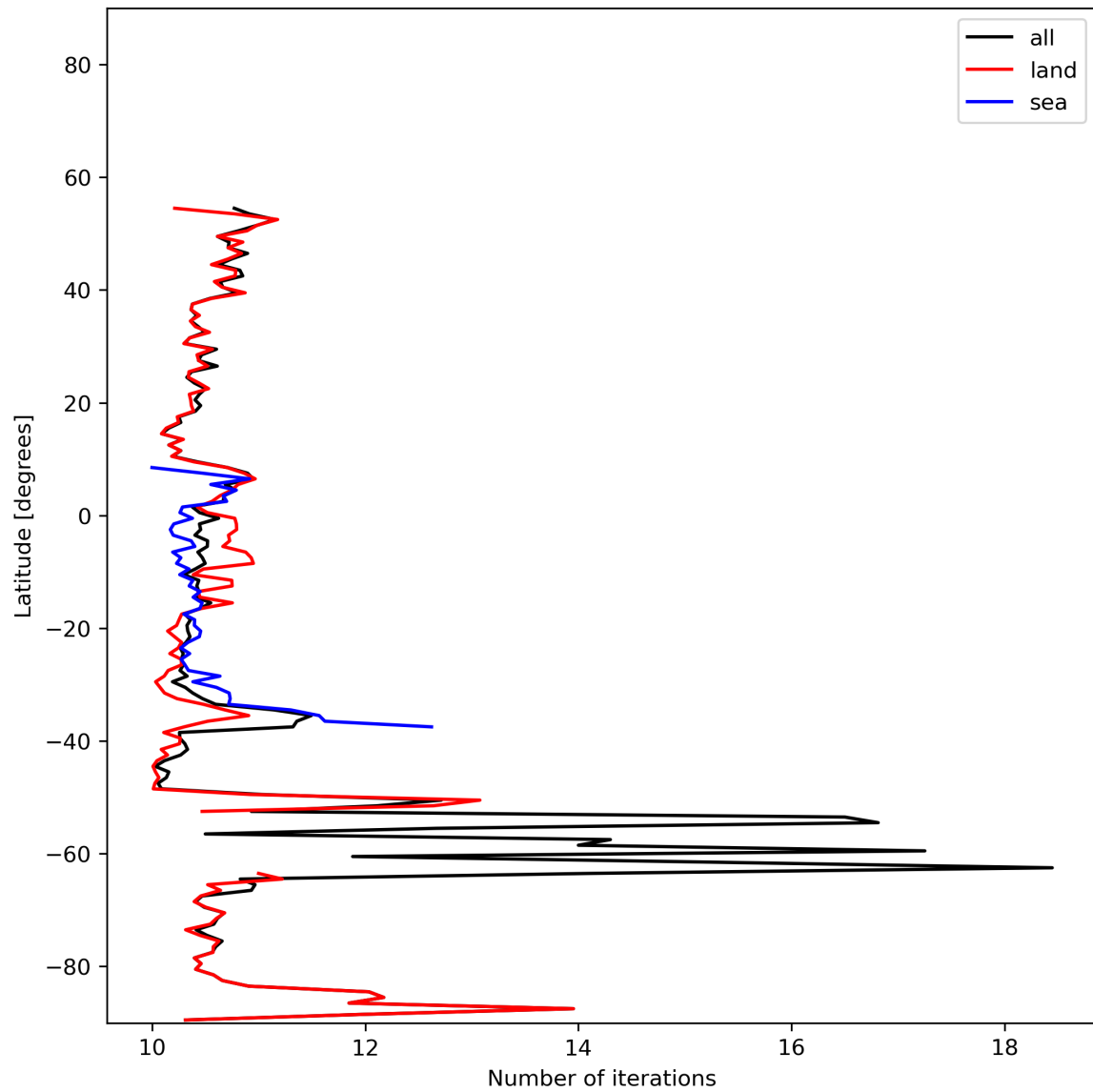
Figure 20: Zonal average of “Number of iterations” for 2023-11-23 to 2023-11-25.
