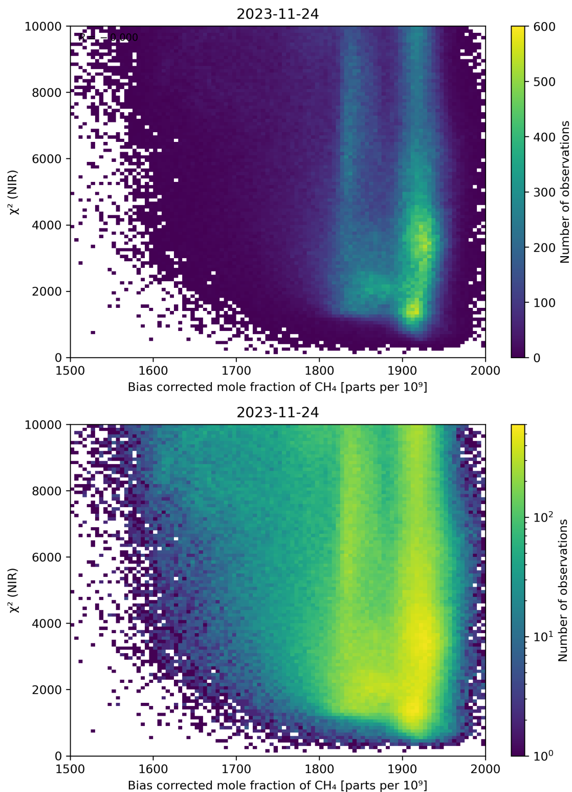
Figure 63: Scatter density plot of “Bias corrected mole fraction of CH 4 ” against “ \chi^2 (NIR)” for 2023-11-23 to 2023-11-25.
