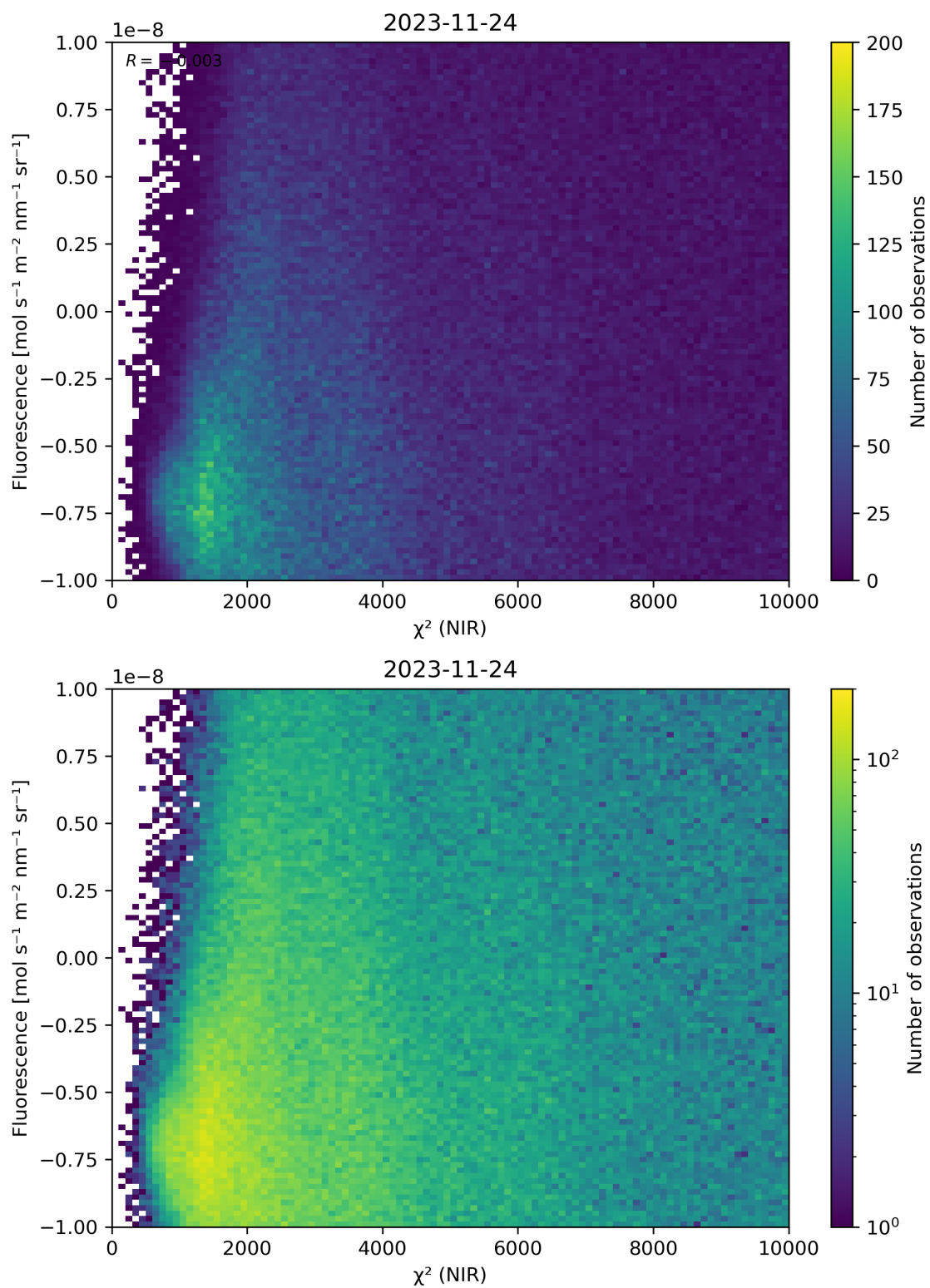
Figure 45: Scatter density plot of “ \chi^2 (NIR)” against “Fluorescence” for 2023-11-23 to 2023-11-25.
