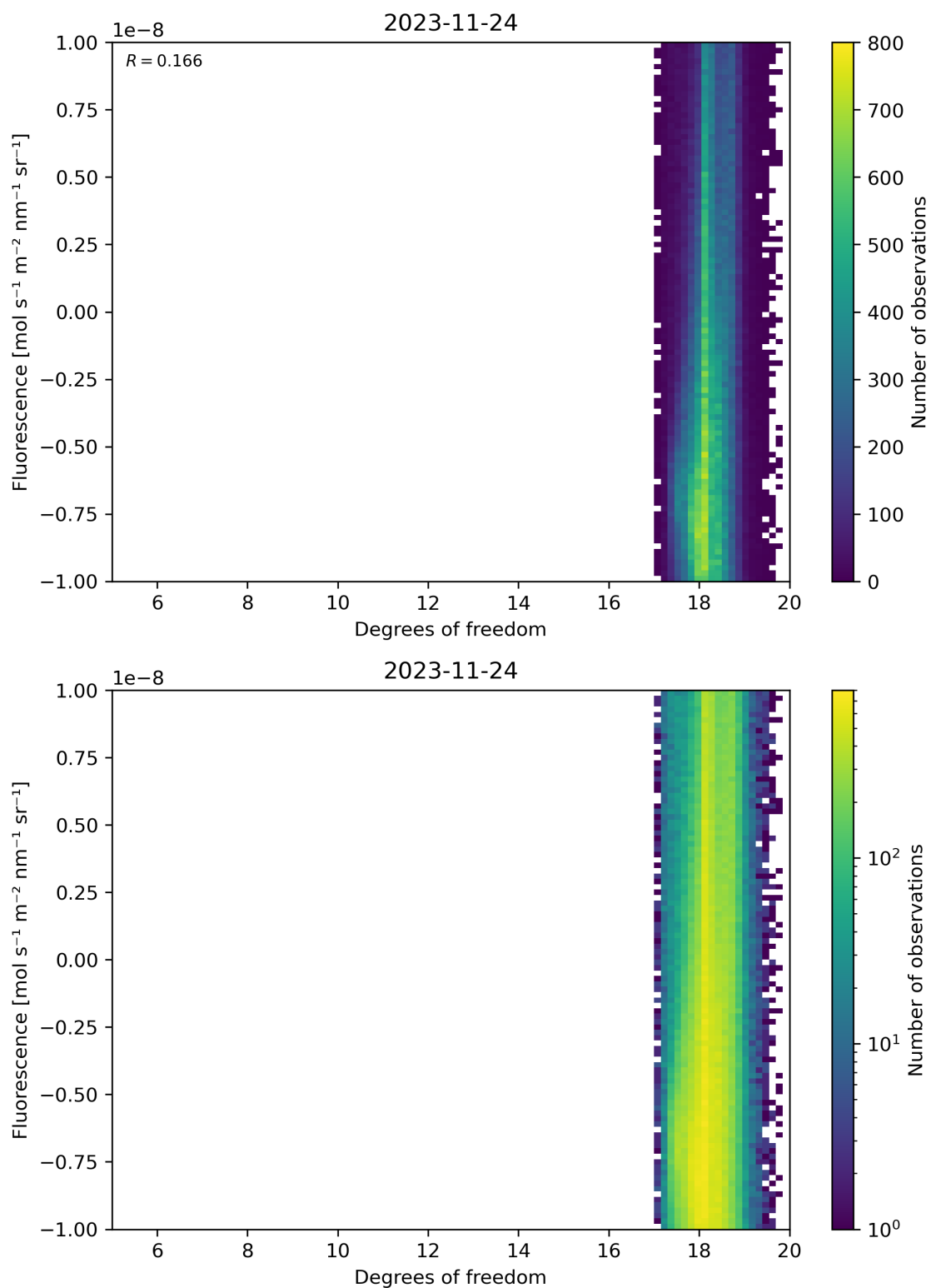
Figure 51: Scatter density plot of “Degrees of freedom” against “Fluorescence” for 2023-11-23 to 2023-11-25.
