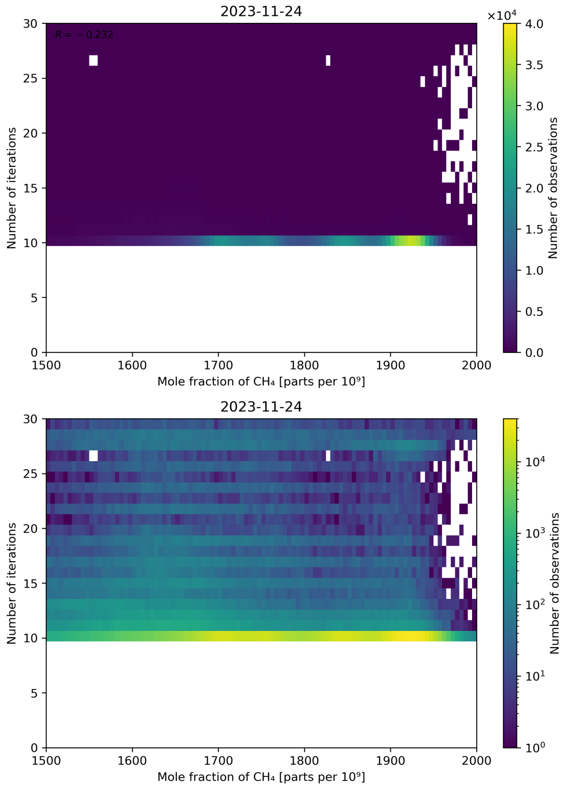
Figure 76: Scatter density plot of “Mole fraction of CH 4 ” against “Number of iterations” for 2023-11-23 to 2023-11-25.
