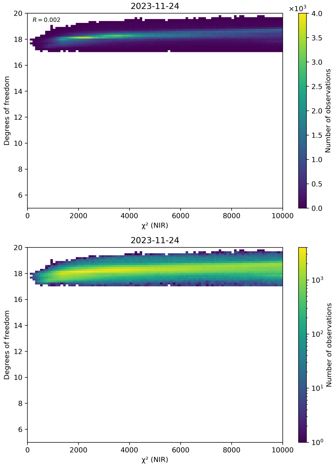
Figure 44: Scatter density plot of “ \chi^2 (NIR)” against “Degrees of freedom” for 2023-11-23 to 2023-11-25.
