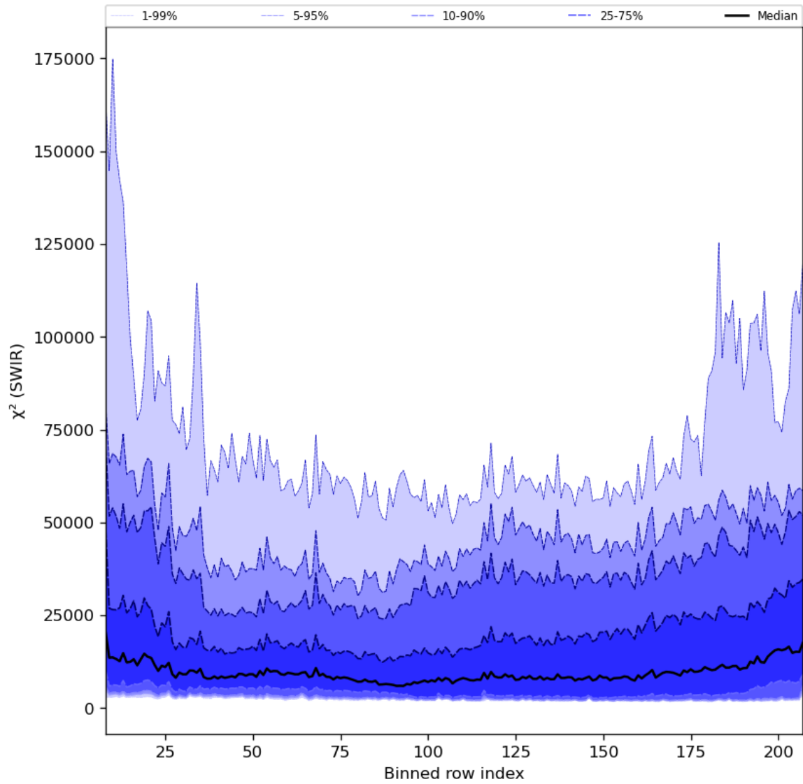
Figure 39: Along track statistics of “ \chi^2 (SWIR)” for 2023-11-23 to 2023-11-25
