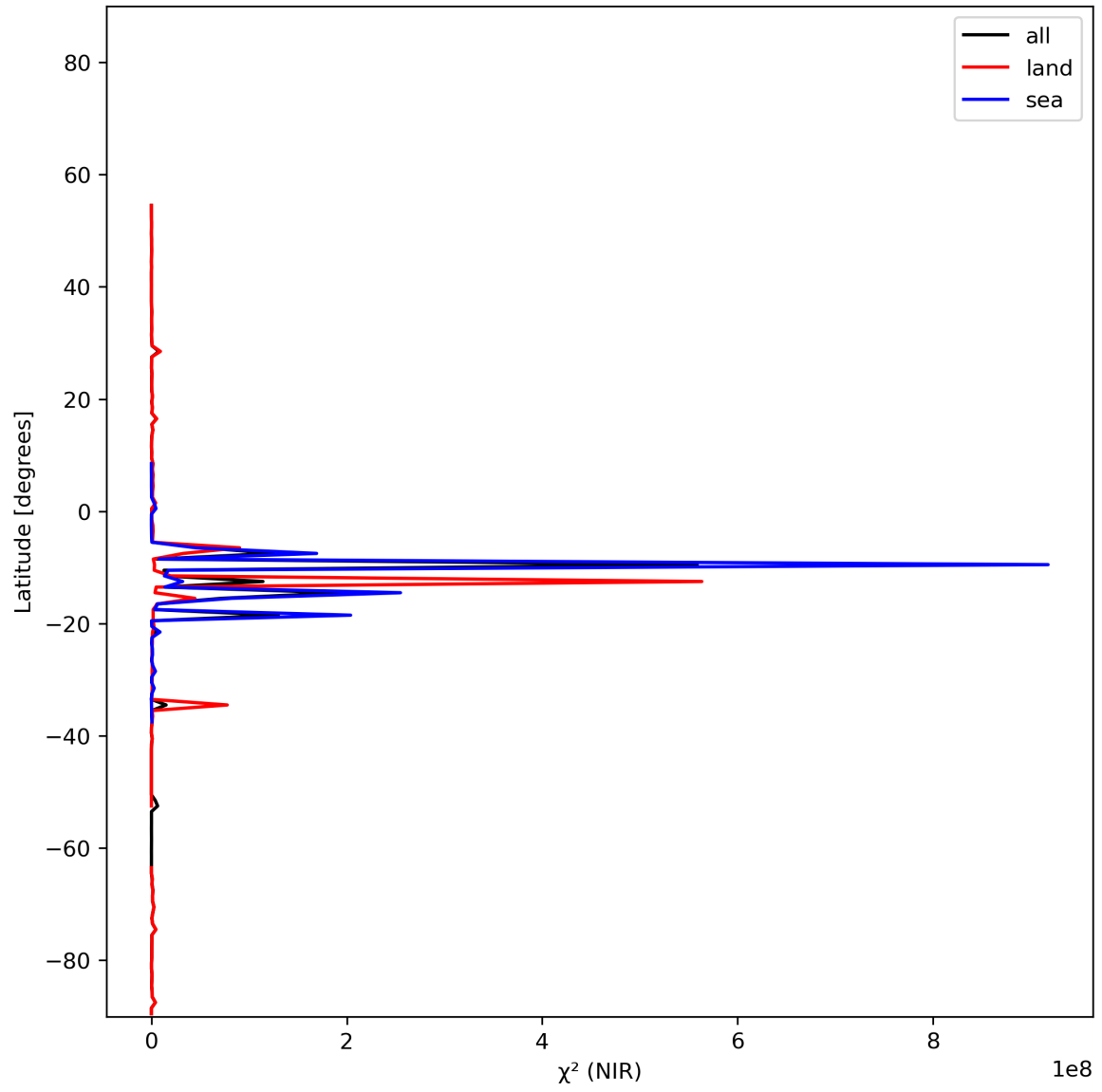
Figure 18: Zonal average of “ \chi^2 (NIR)” for 2023-11-23 to 2023-11-25.
