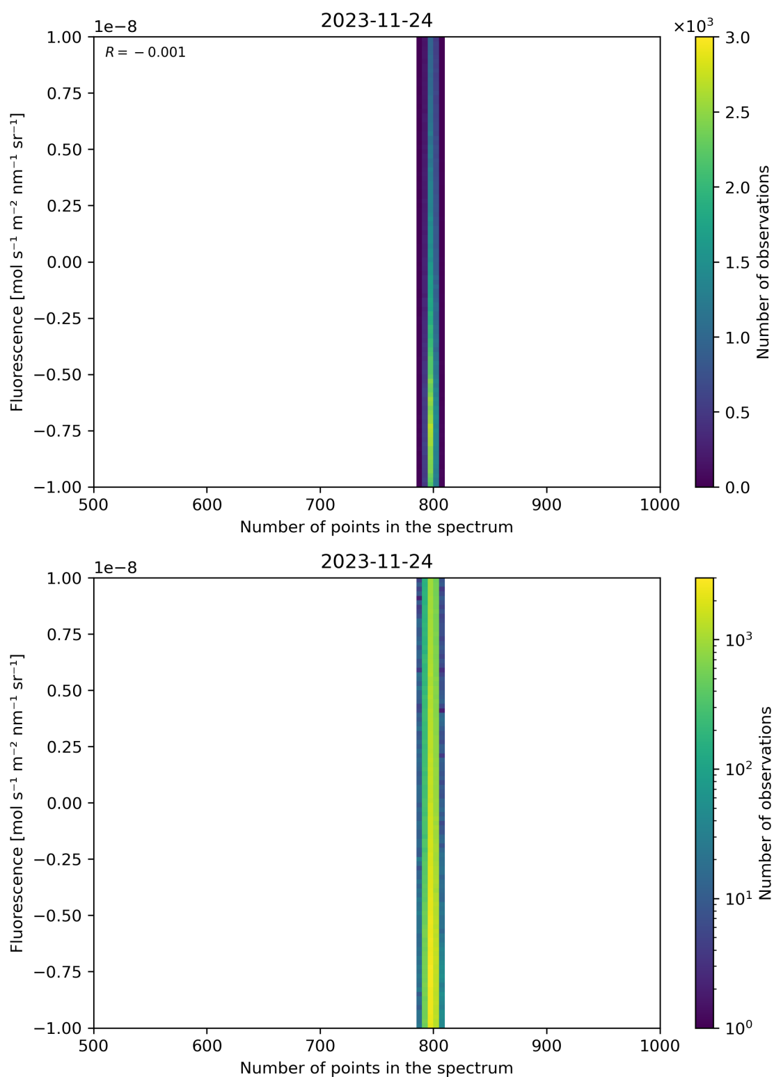
Figure 91: Scatter density plot of “Number of points in the spectrum” against “Fluorescence” for 2023-11-23 to 2023-11-25.
