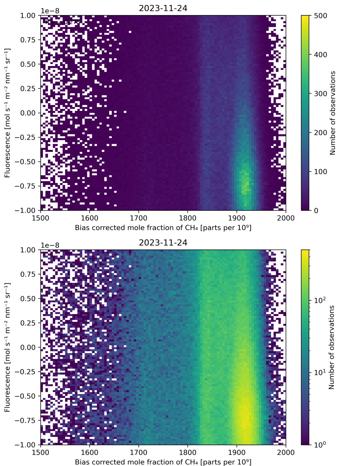
Figure 66: Scatter density plot of “Bias corrected mole fraction of \text{CH}_4 ” against “Fluorescence” for 2023-11-23 to 2023-11-25.
