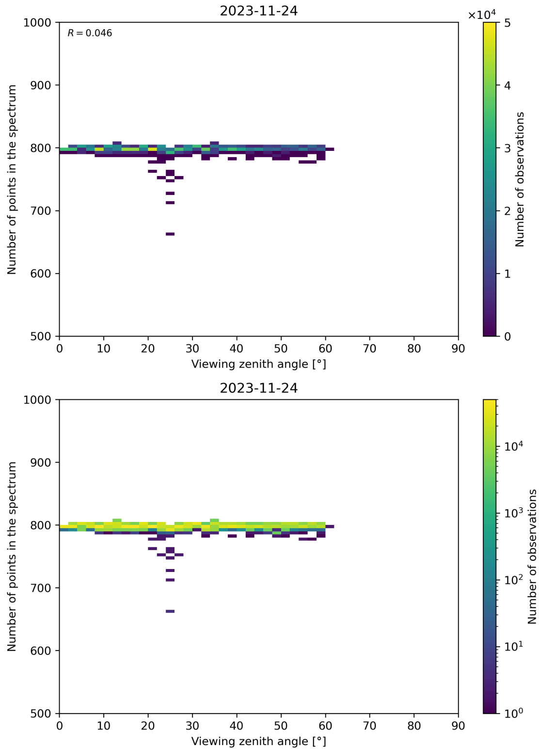
Figure 114: Scatter density plot of “Viewing zenith angle” against “Number of points in the spectrum” for 2023-11-23 to 2023-11-25.
