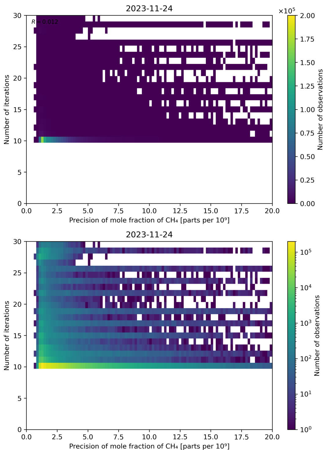
Figure 83: Scatter density plot of “Precision of mole fraction of CH 4 ” against “Number of iterations” for 2023-11-23 to 2023-11-25.
