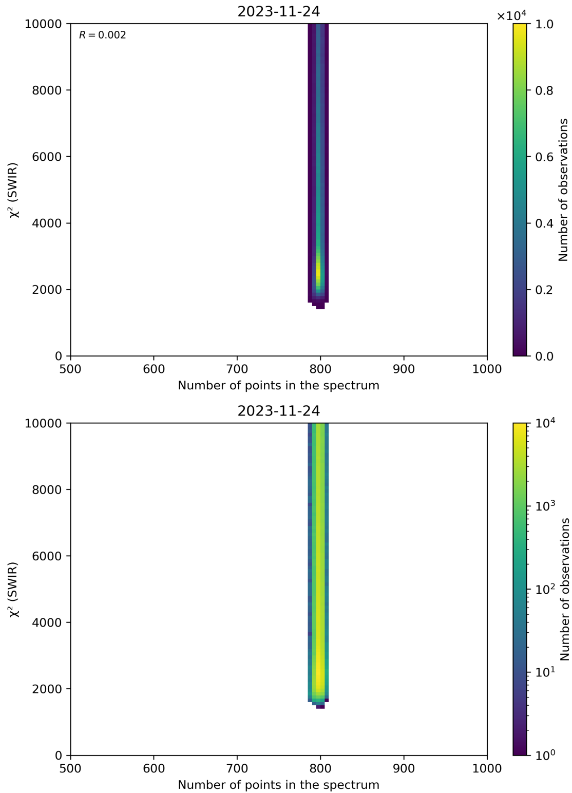
Figure 89: Scatter density plot of “Number of points in the spectrum” against “ \chi^2 (SWIR)” for 2023-11-23 to 2023-11-25.
