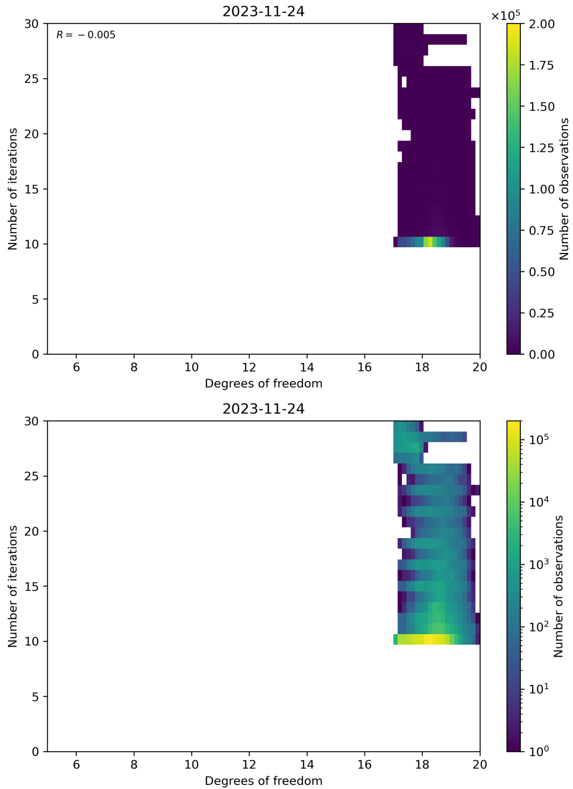
Figure 52: Scatter density plot of “Degrees of freedom” against “Number of iterations” for 2023-11-23 to 2023-11-25.
