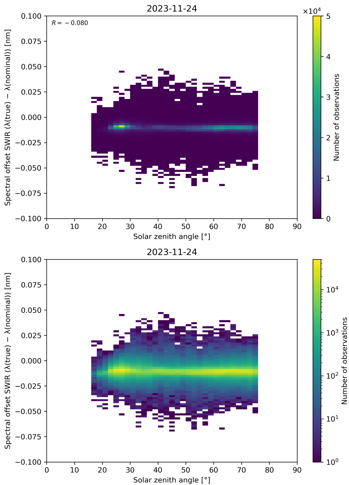
Figure 104: Scatter density plot of “Solar zenith angle” against “Spectral offset SWIR ( \lambda(\text{true}) - \lambda(\text{nominal}) )” for 2023-11-23 to 2023-11-25.
