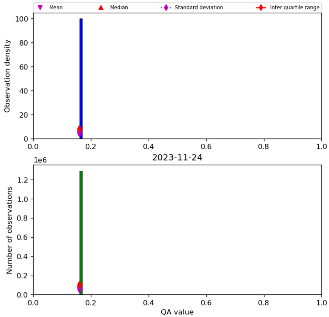
Figure 22: Histogram of “QA value” for 2023-11-23 to 2023-11-25
