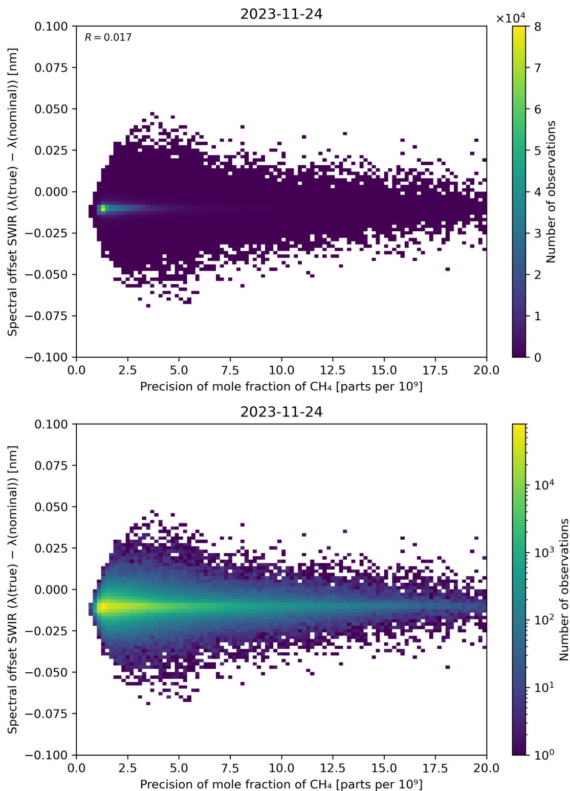
Figure 85: Scatter density plot of “Precision of mole fraction of \text{CH}_4 ” against “Spectral offset SWIR ( \lambda(\text{true}) - \lambda(\text{nominal}) )” for 2023-11-23 to 2023-11-25.
