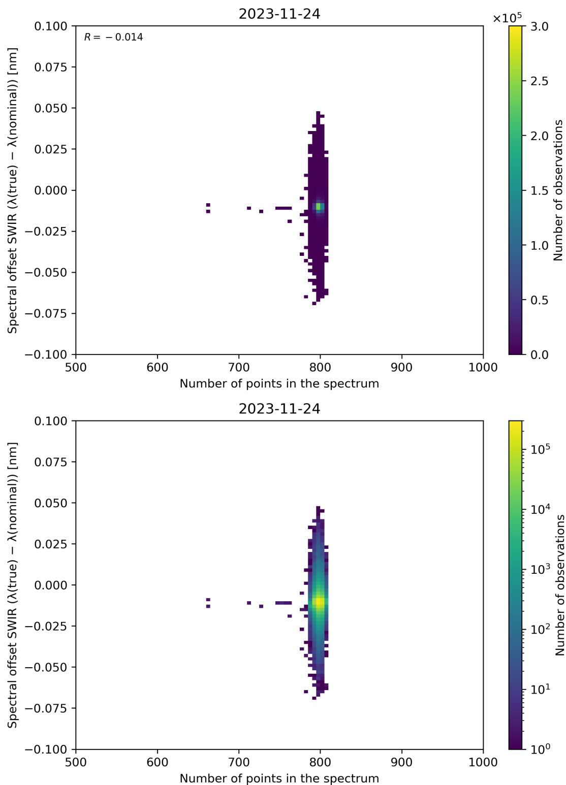
Figure 93: Scatter density plot of “Number of points in the spectrum” against “Spectral offset SWIR ( \lambda(\text{true}) - \lambda(\text{nominal}) )” for 2023-11-23 to 2023-11-25.
