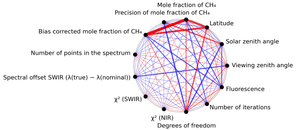
Figure 1: Map of correlation graph for 2023-11-23 to 2023-11-25.
