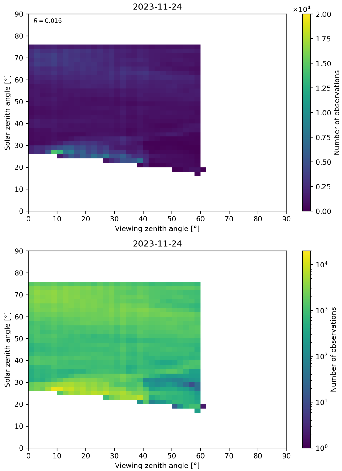
Figure 115: Scatter density plot of “Viewing zenith angle” against “Solar zenith angle” for 2023-11-23 to 2023-11-25.
