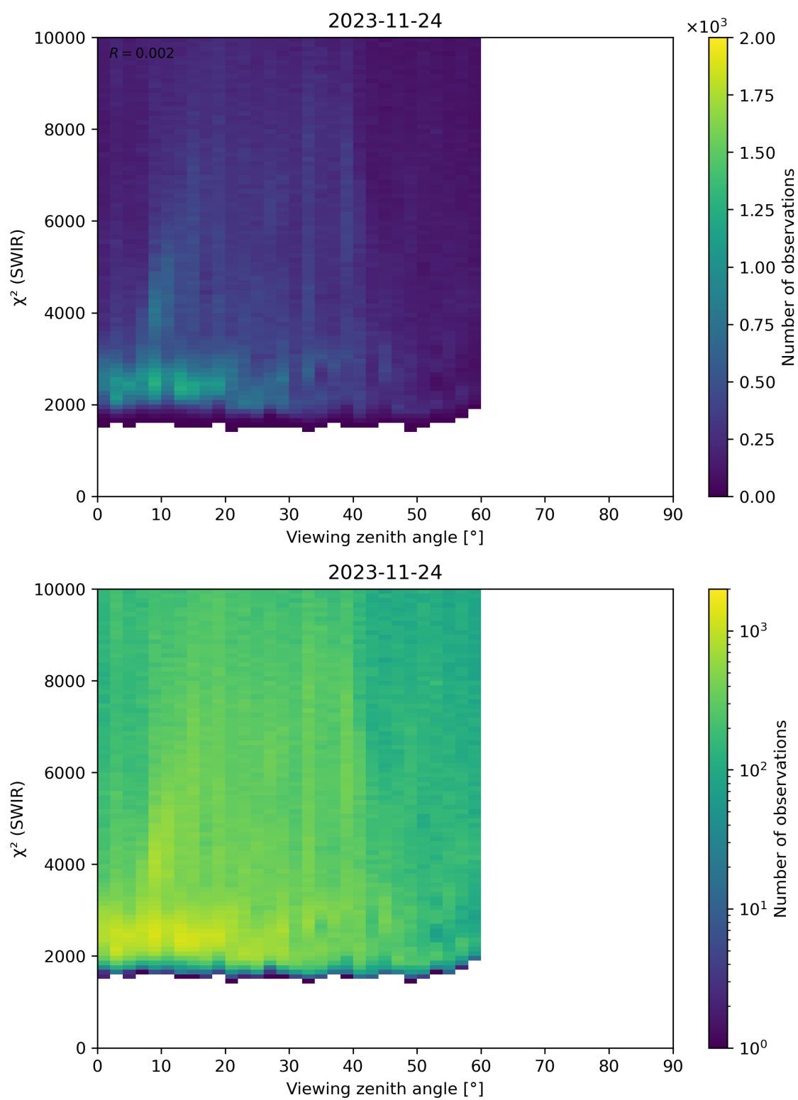
Figure 106: Scatter density plot of “Viewing zenith angle” against “ \chi^2 (SWIR)” for 2023-11-23 to 2023-11-25.
