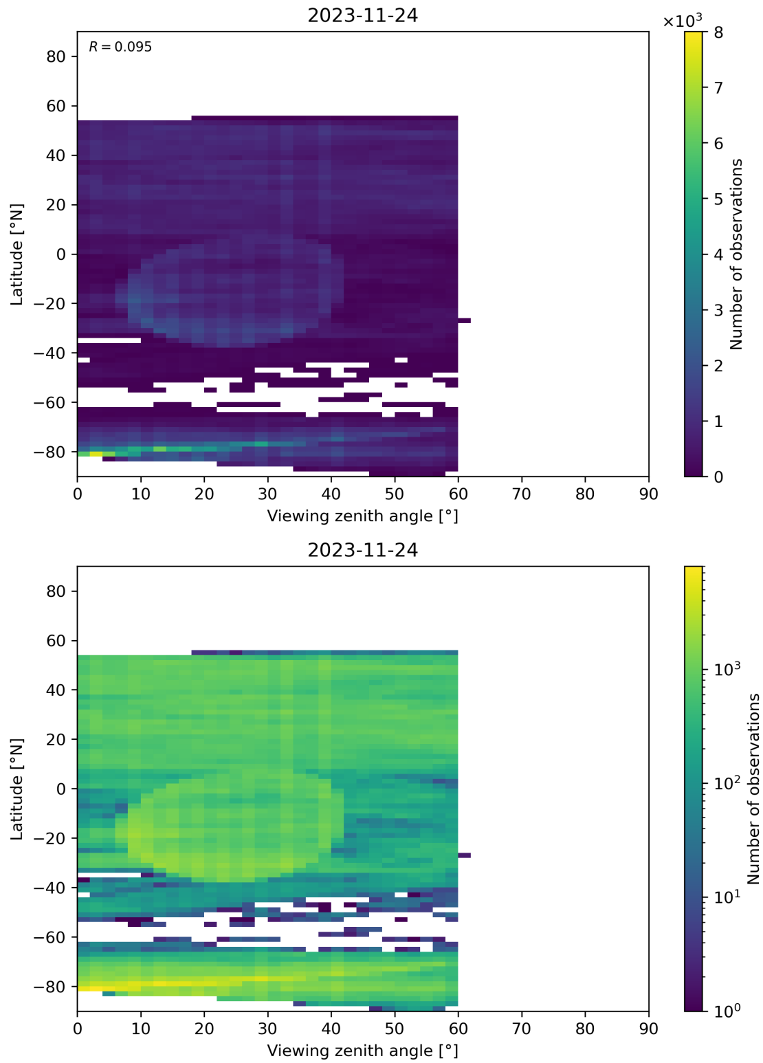
Figure 109: Scatter density plot of “Viewing zenith angle” against “Latitude” for 2023-11-23 to 2023-11-25.
