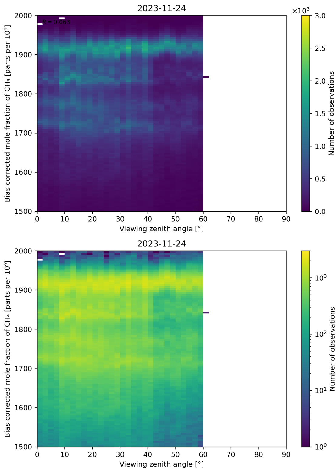
Figure 111: Scatter density plot of “Viewing zenith angle” against “Bias corrected mole fraction of CH 4 ” for 2023-11-23 to 2023-11-25.
