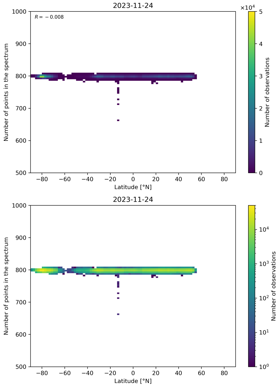
Figure 61: Scatter density plot of “Latitude” against “Number of points in the spectrum” for 2023-11-23 to 2023-11-25.
