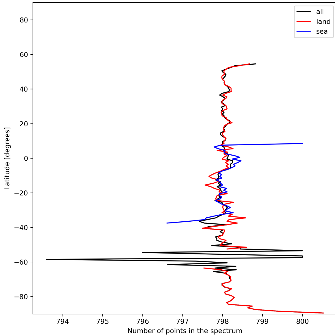
Figure 15: Zonal average of “Number of points in the spectrum” for 2023-11-23 to 2023-11-25.
