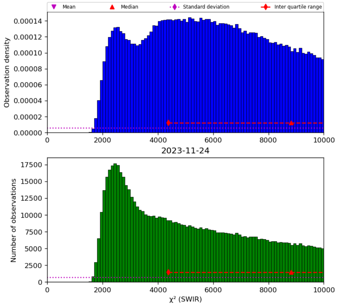
Figure 28: Histogram of “ \chi^2 (SWIR)” for 2023-11-23 to 2023-11-25
