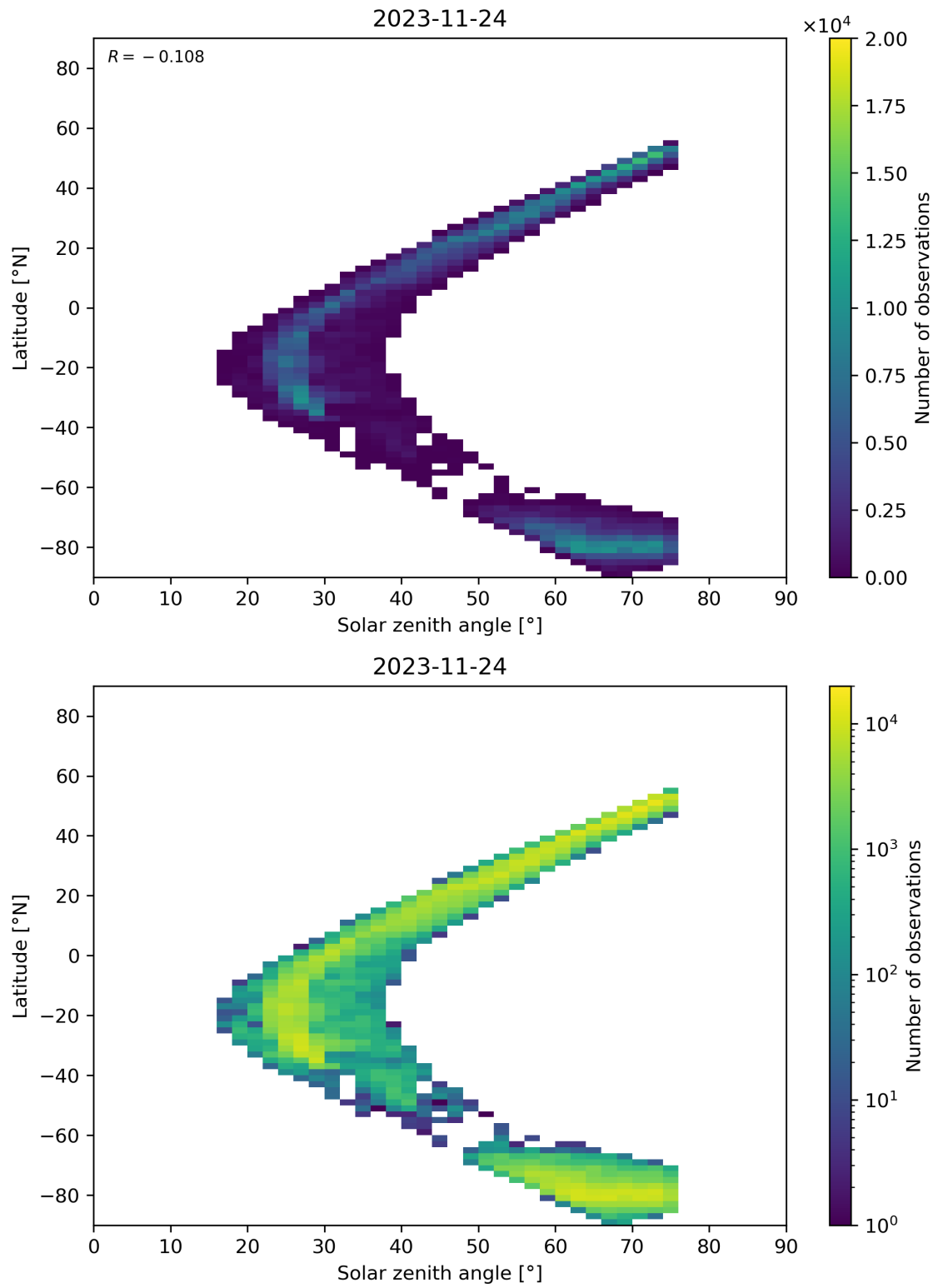
Figure 98: Scatter density plot of “Solar zenith angle” against “Latitude” for 2023-11-23 to 2023-11-25.
