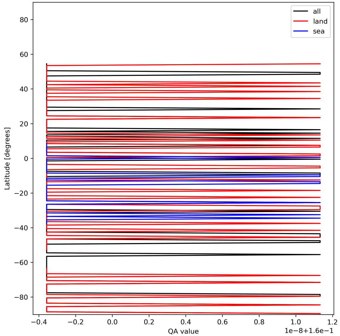
Figure 11: Zonal average of “QA value” for 2023-11-23 to 2023-11-25.
