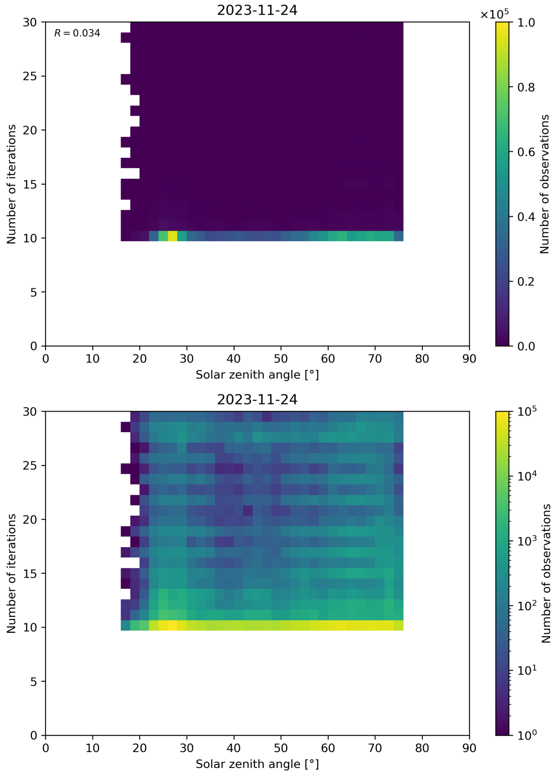
Figure 102: Scatter density plot of “Solar zenith angle” against “Number of iterations” for 2023-11-23 to 2023-11-25.
