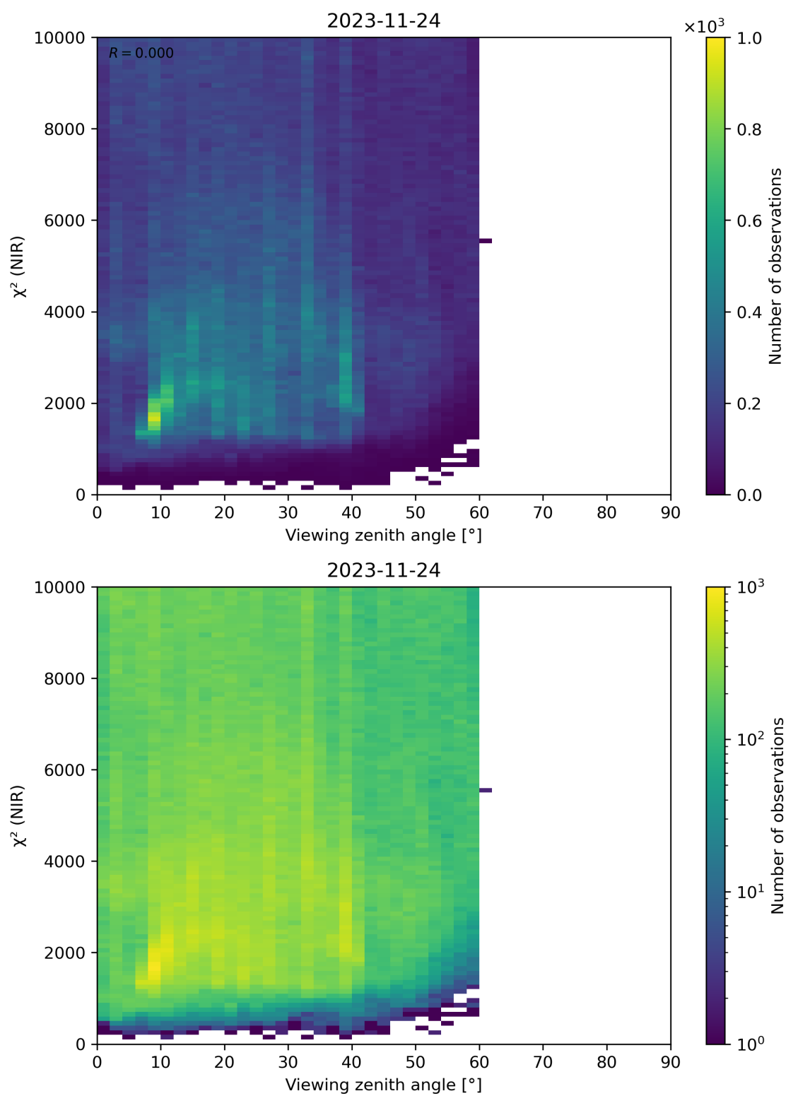
Figure 105: Scatter density plot of “Viewing zenith angle” against “ \chi^2 (NIR)” for 2023-11-23 to 2023-11-25.
