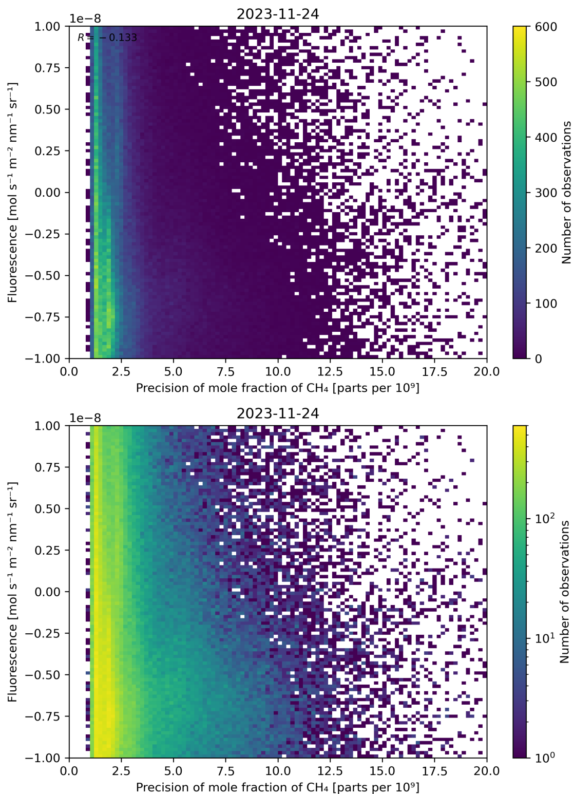
Figure 81: Scatter density plot of “Precision of mole fraction of \text{CH}_4 ” against “Fluorescence” for 2023-11-23 to 2023-11-25.
