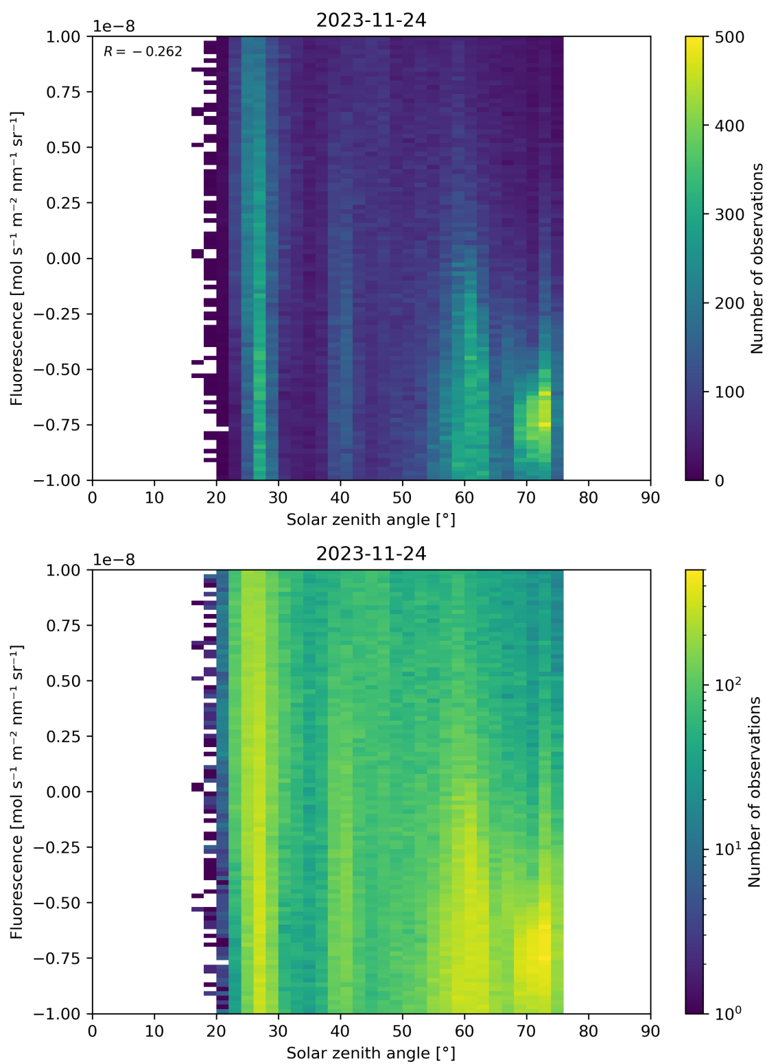
Figure 97: Scatter density plot of “Solar zenith angle” against “Fluorescence” for 2023-11-23 to 2023-11-25.
