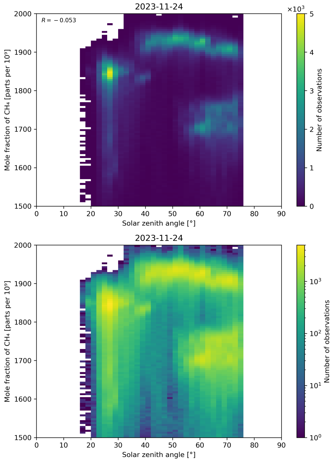
Figure 99: Scatter density plot of “Solar zenith angle” against “Mole fraction of CH 4 ” for 2023-11-23 to 2023-11-25.
