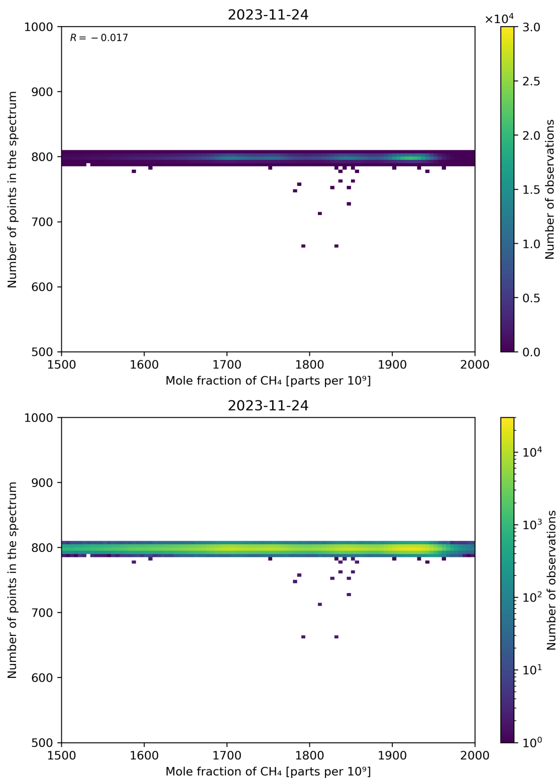
Figure 77: Scatter density plot of “Mole fraction of CH 4 ” against “Number of points in the spectrum” for 2023-11-23 to 2023-11-25.
