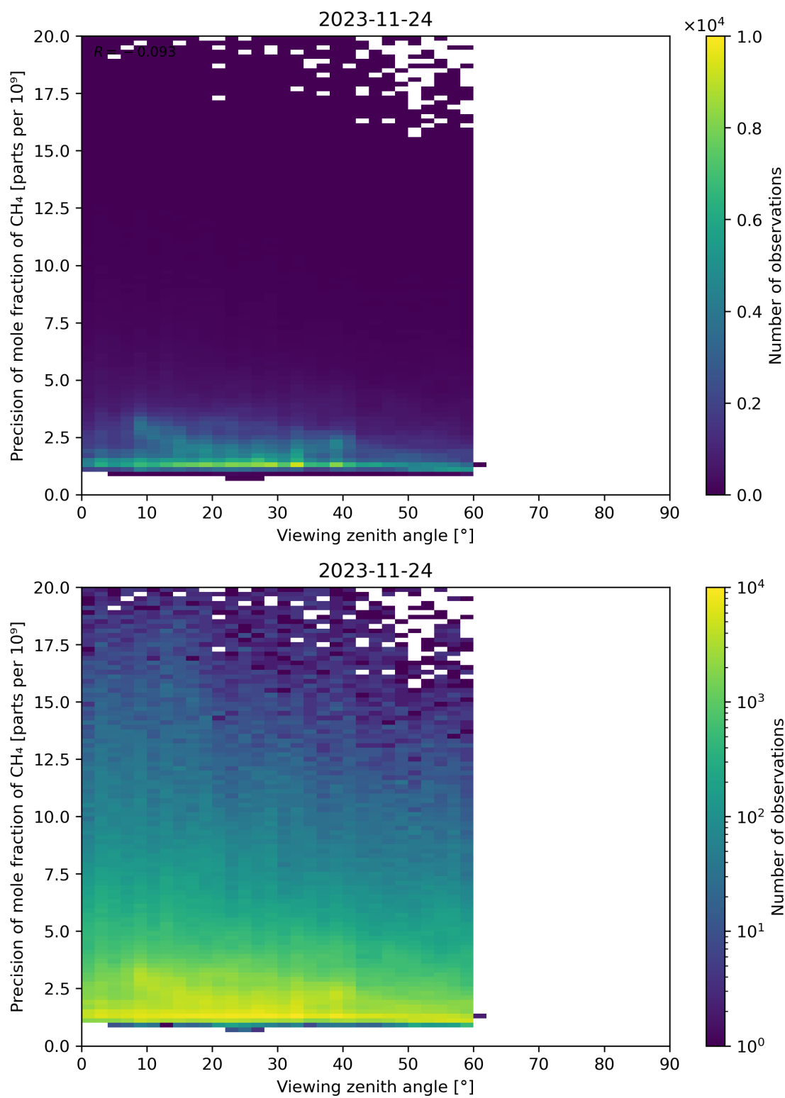
Figure 112: Scatter density plot of “Viewing zenith angle” against “Precision of mole fraction of CH 4 ” for 2023-11-23 to 2023-11-25.
