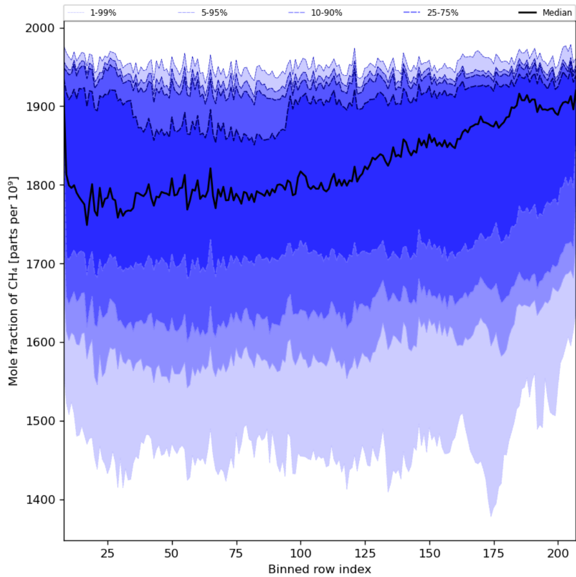
Figure 34: Along track statistics of “Mole fraction of CH 4 ” for 2023-11-23 to 2023-11-25
