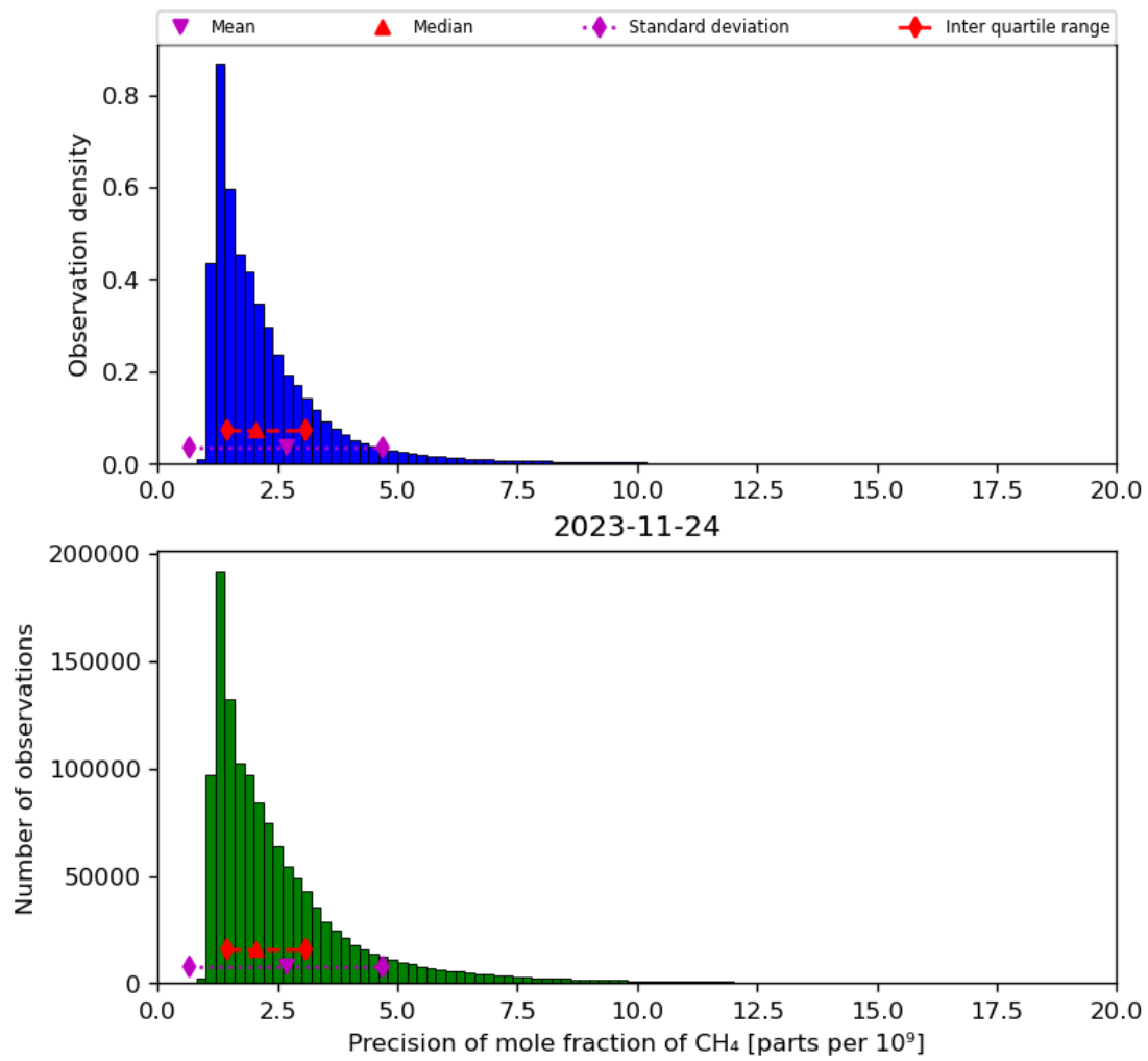
Figure 24: Histogram of “Precision of mole fraction of CH 4 ” for 2023-11-23 to 2023-11-25
