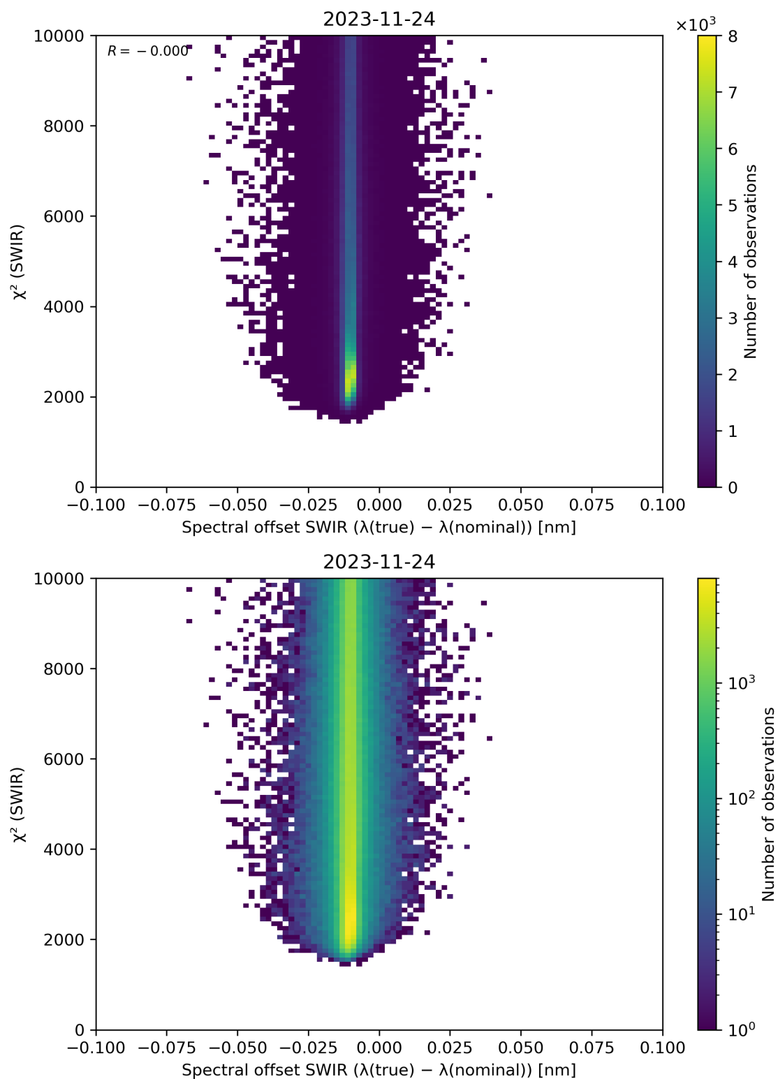
Figure 118: Scatter density plot of “Spectral offset SWIR ( \lambda(\text{true}) - \lambda(\text{nominal}) )” against “ \chi^2 (SWIR)” for 2023-11-23 to 2023-11-25.
