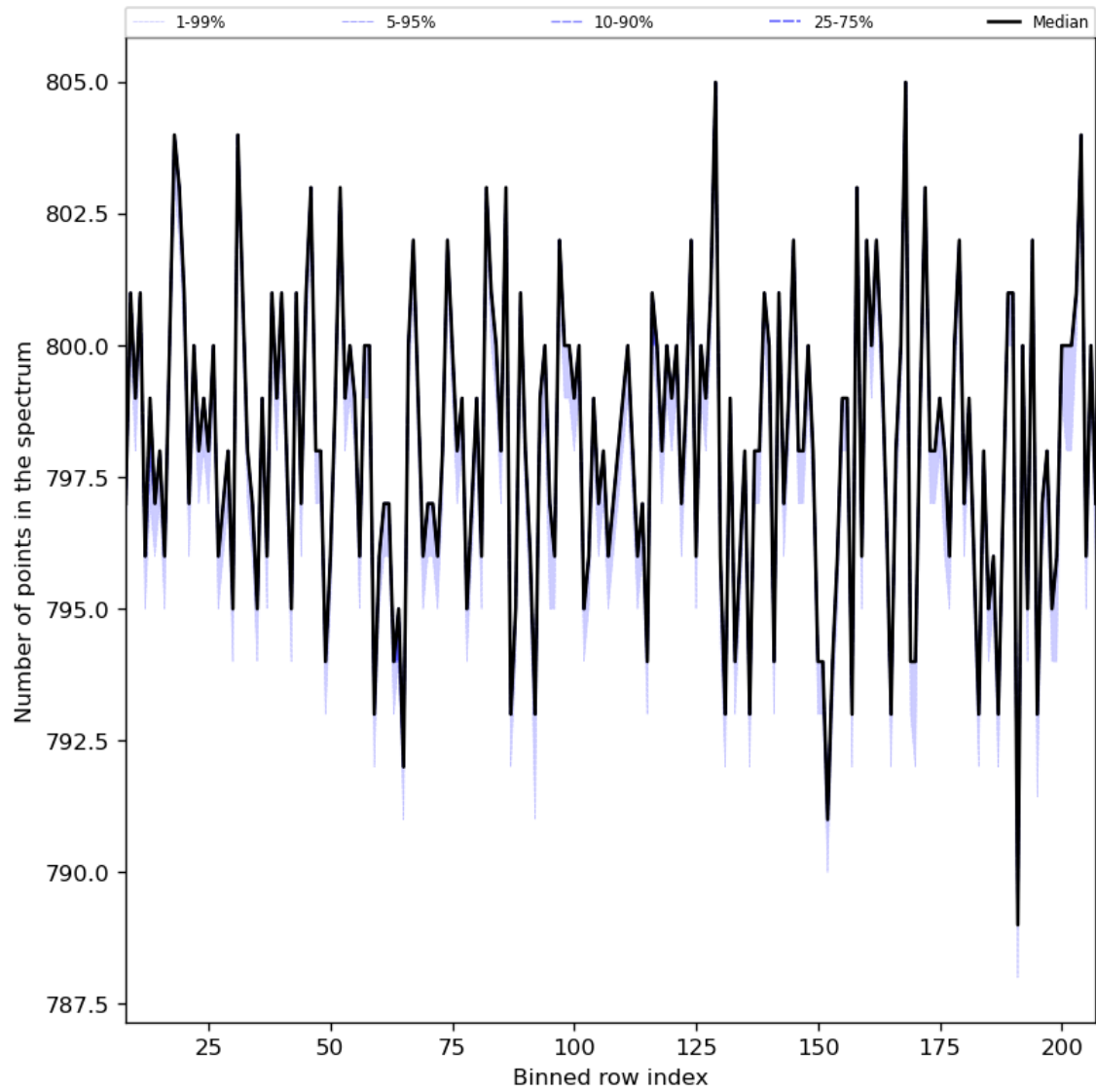
Figure 37: Along track statistics of “Number of points in the spectrum” for 2023-11-23 to 2023-11-25
