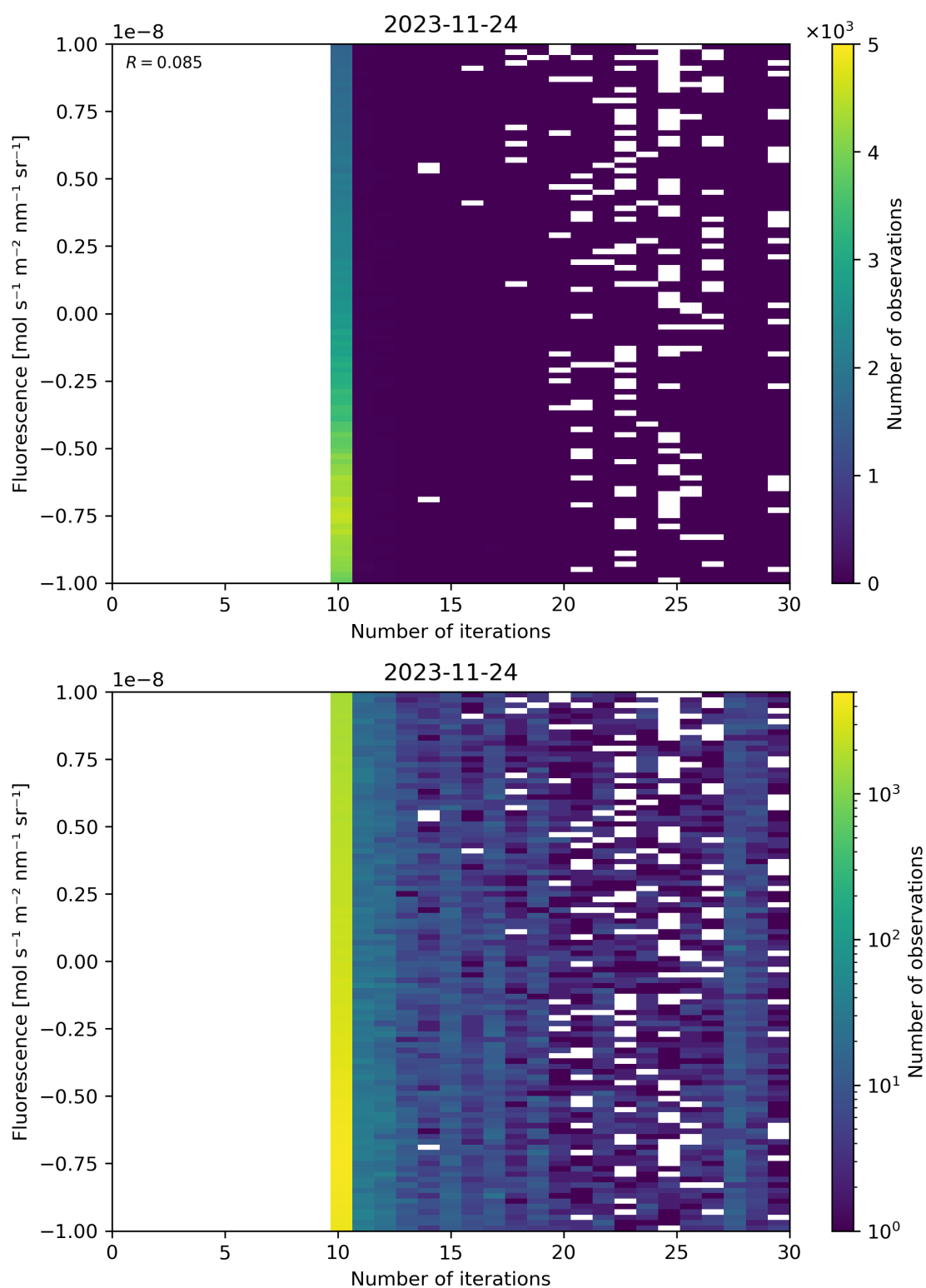
Figure 87: Scatter density plot of “Number of iterations” against “Fluorescence” for 2023-11-23 to 2023-11-25.
