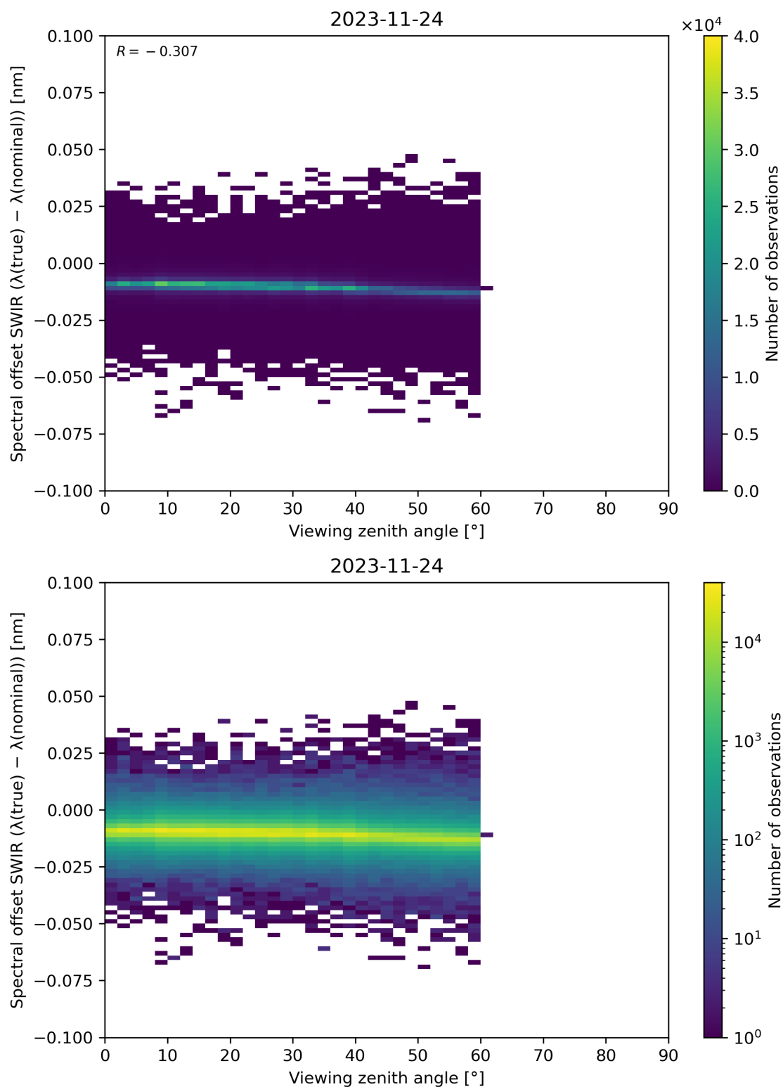
Figure 116: Scatter density plot of “Viewing zenith angle” against “Spectral offset SWIR ( \lambda(\text{true}) - \lambda(\text{nominal}) )” for 2023-11-23 to 2023-11-25.
