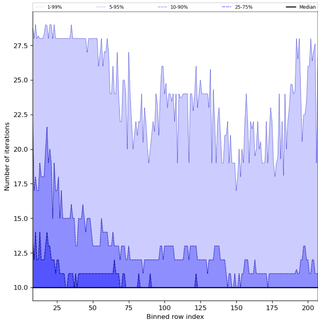
Figure 42: Along track statistics of “Number of iterations” for 2023-11-23 to 2023-11-25
