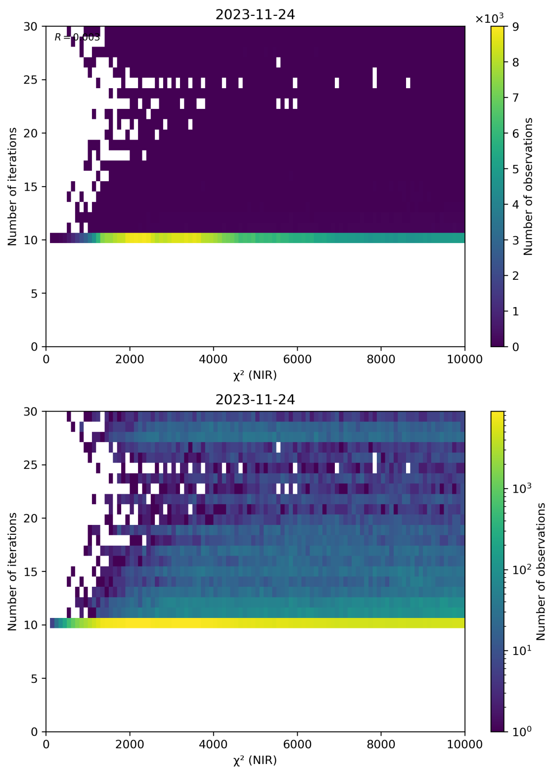
Figure 46: Scatter density plot of “ \chi^2 (NIR)” against “Number of iterations” for 2023-11-23 to 2023-11-25.
