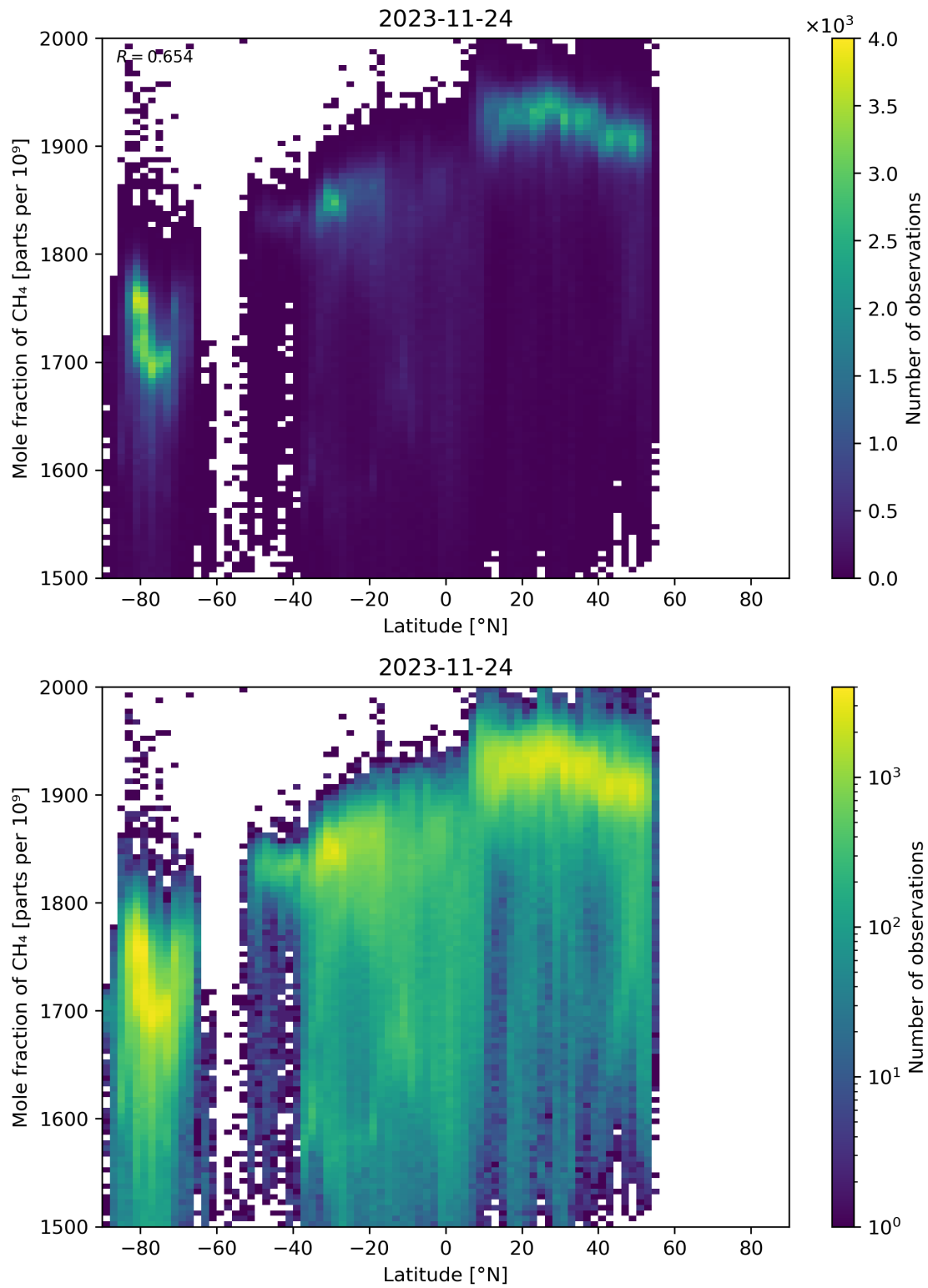
Figure 57: Scatter density plot of “Latitude” against “Mole fraction of CH 4 ” for 2023-11-23 to 2023-11-25.
