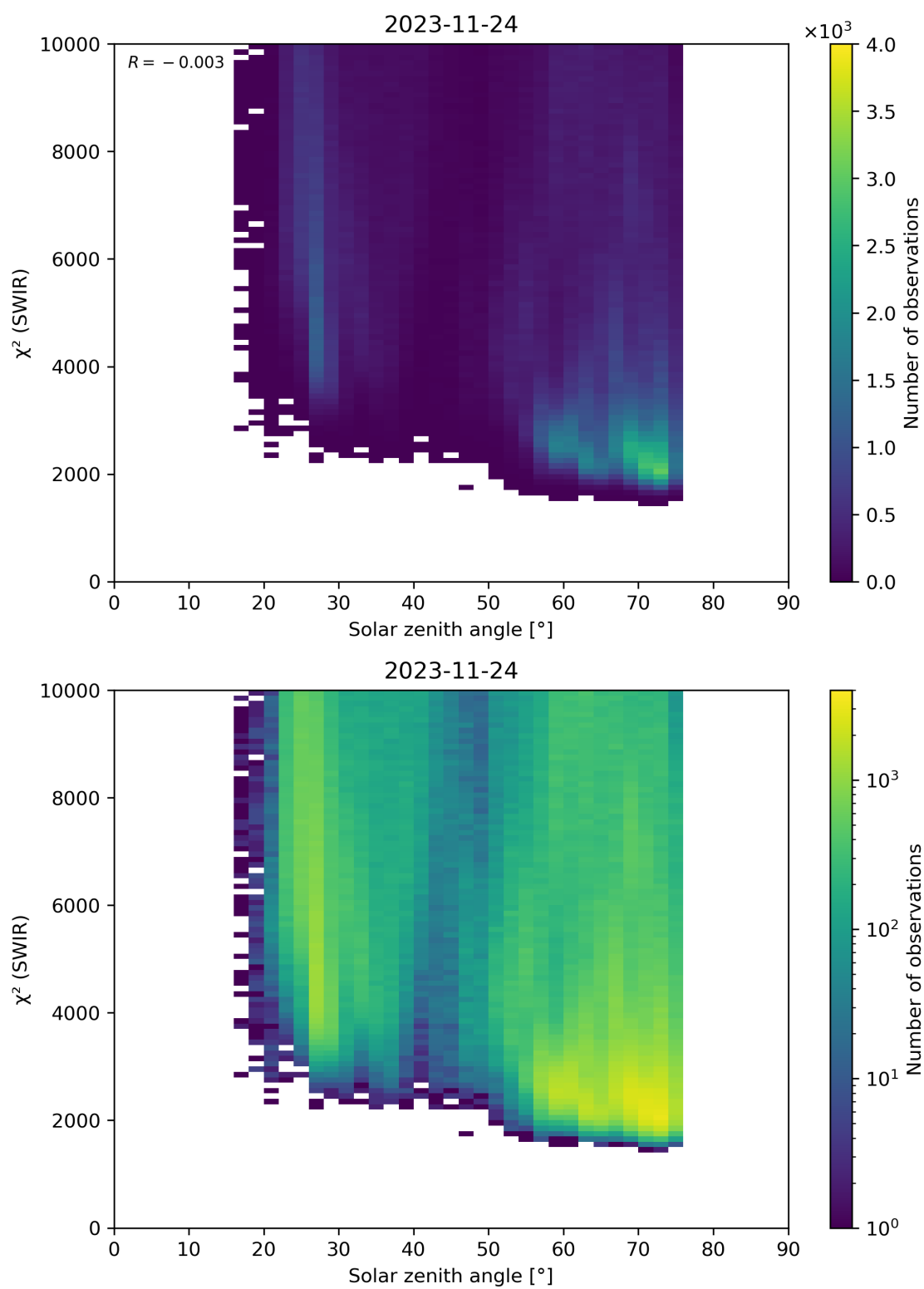
Figure 95: Scatter density plot of “Solar zenith angle” against “ \chi^2 (SWIR)” for 2023-11-23 to 2023-11-25.
