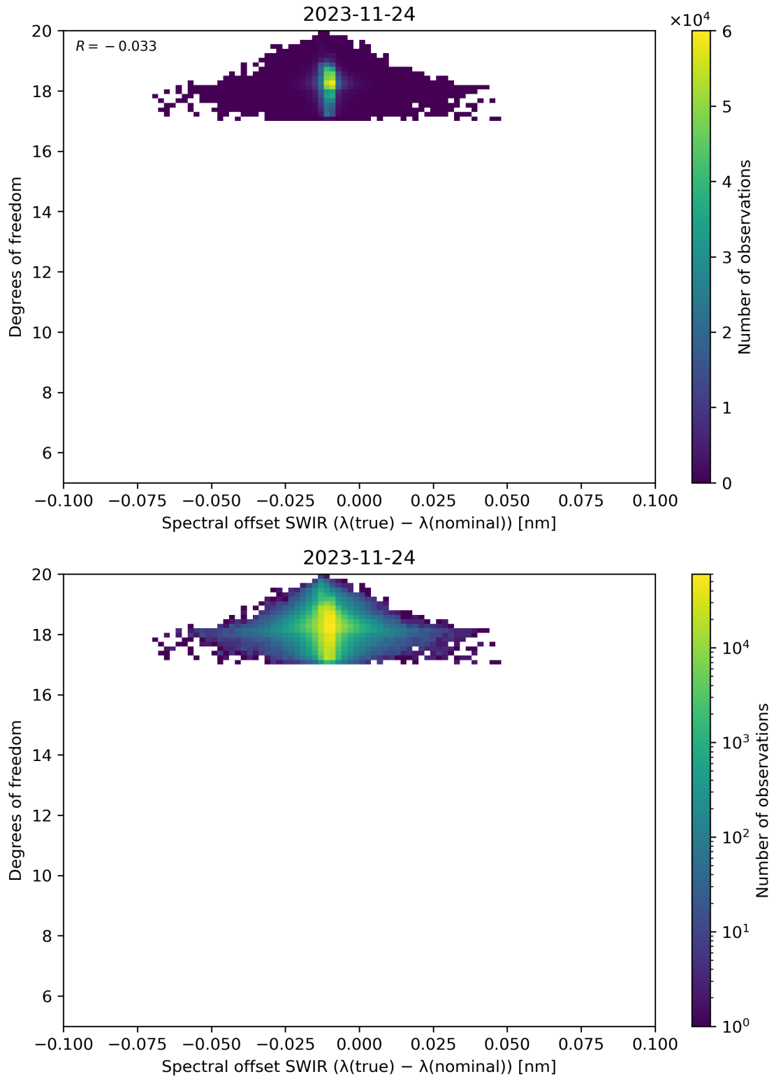
Figure 119: Scatter density plot of “Spectral offset SWIR ( \lambda(\text{true}) - \lambda(\text{nominal}) )” against “Degrees of freedom” for 2023-11-23 to 2023-11-25.
