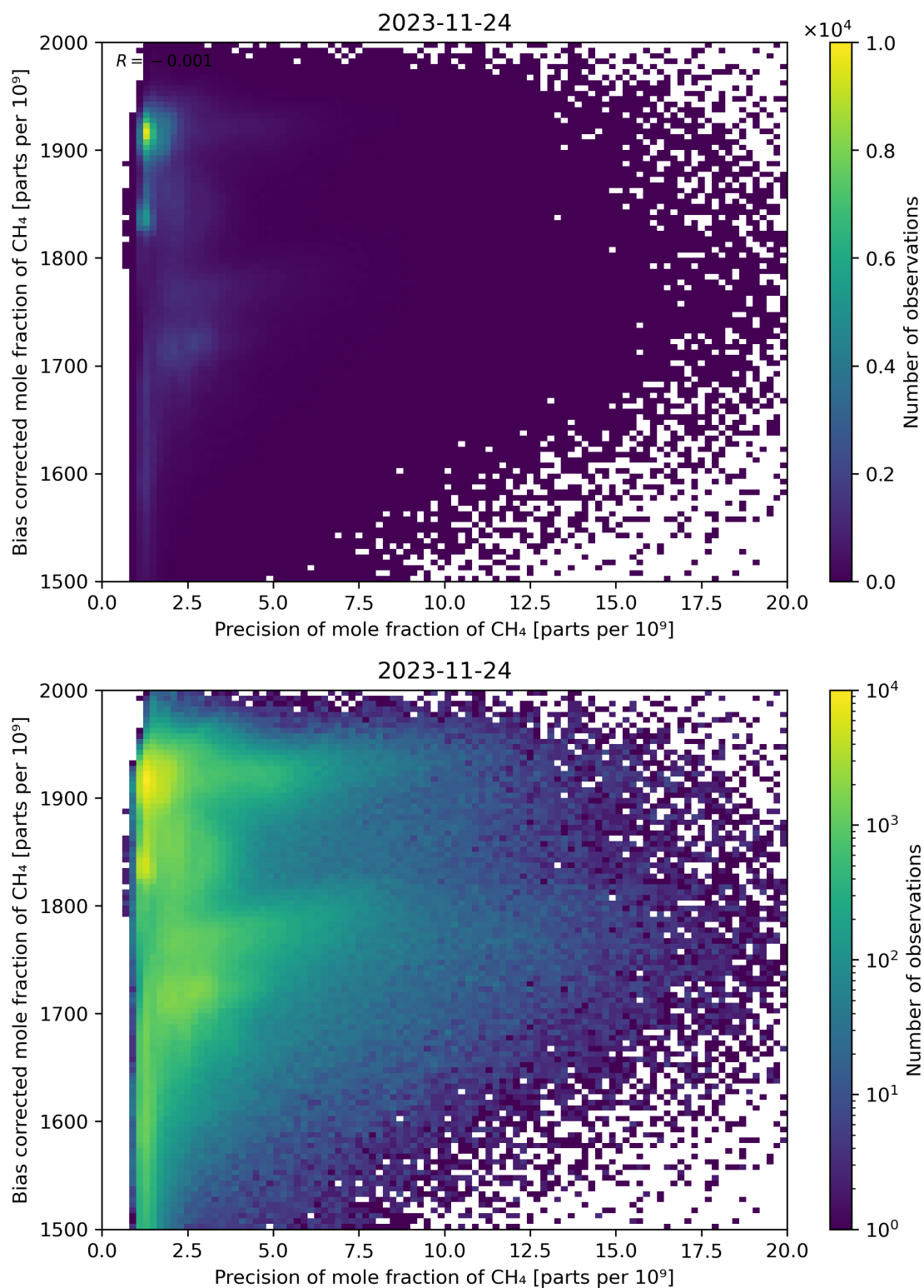
Figure 82: Scatter density plot of “Precision of mole fraction of CH 4 ” against “Bias corrected mole fraction of CH 4 ” for 2023-11-23 to 2023-11-25.
