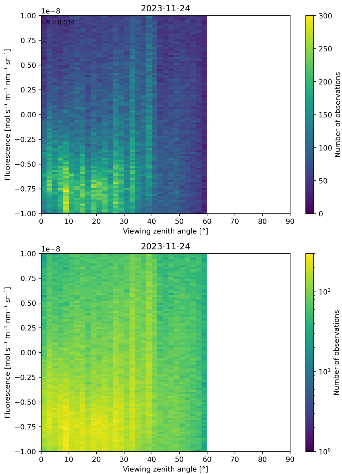
Figure 108: Scatter density plot of “Viewing zenith angle” against “Fluorescence” for 2023-11-23 to 2023-11-25.
