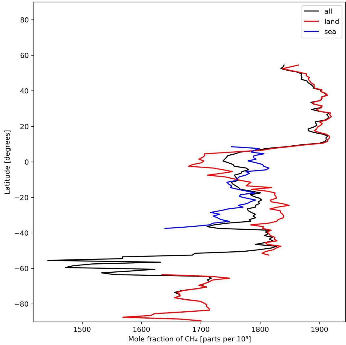
Figure 12: Zonal average of “Mole fraction of \text{CH}_4 ” for 2023-11-23 to 2023-11-25.
