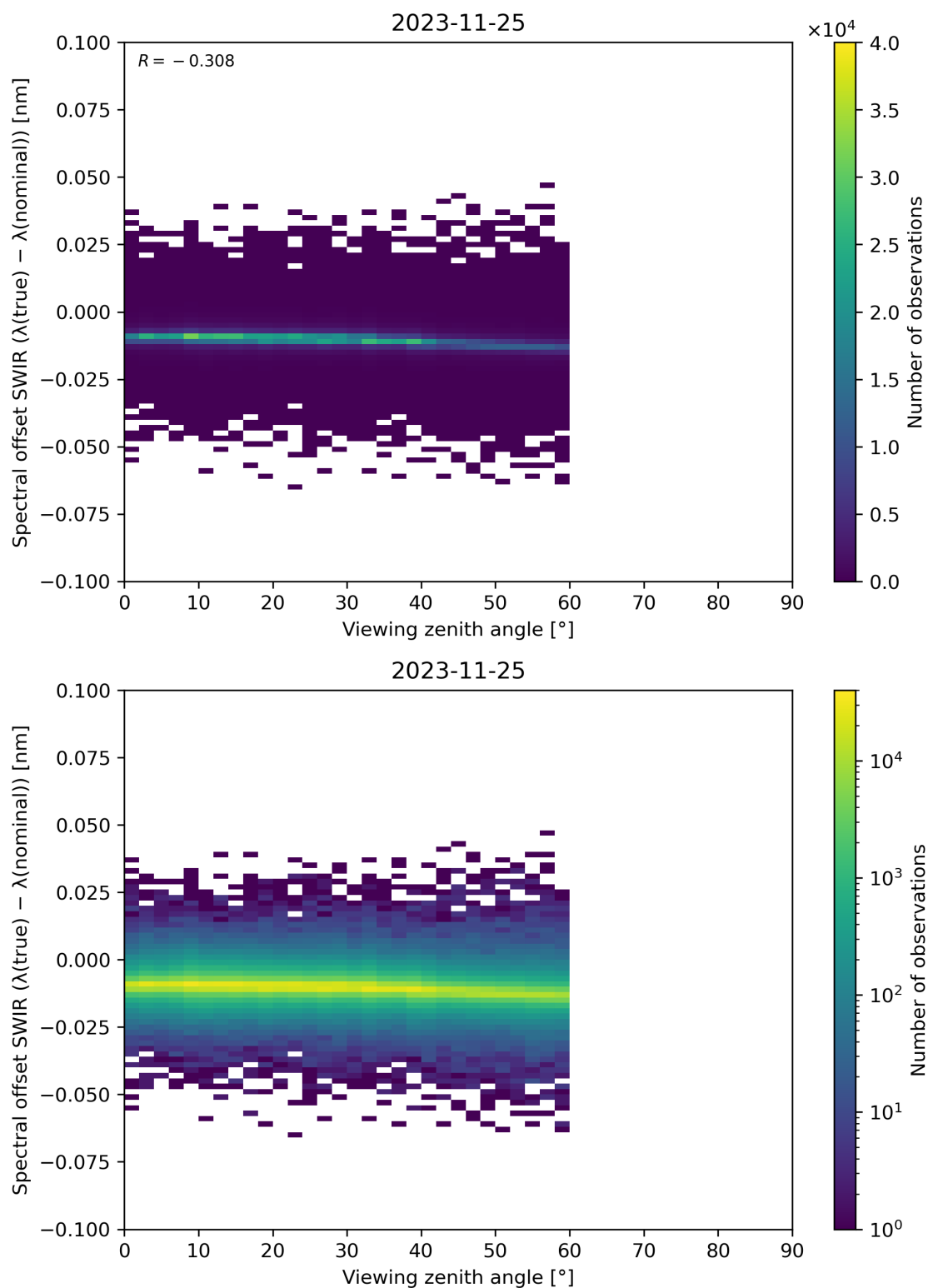
Figure 116: Scatter density plot of “Viewing zenith angle” against “Spectral offset SWIR ( \lambda(\text{true}) - \lambda(\text{nominal}) )” for 2023-11-24 to 2023-11-26.
