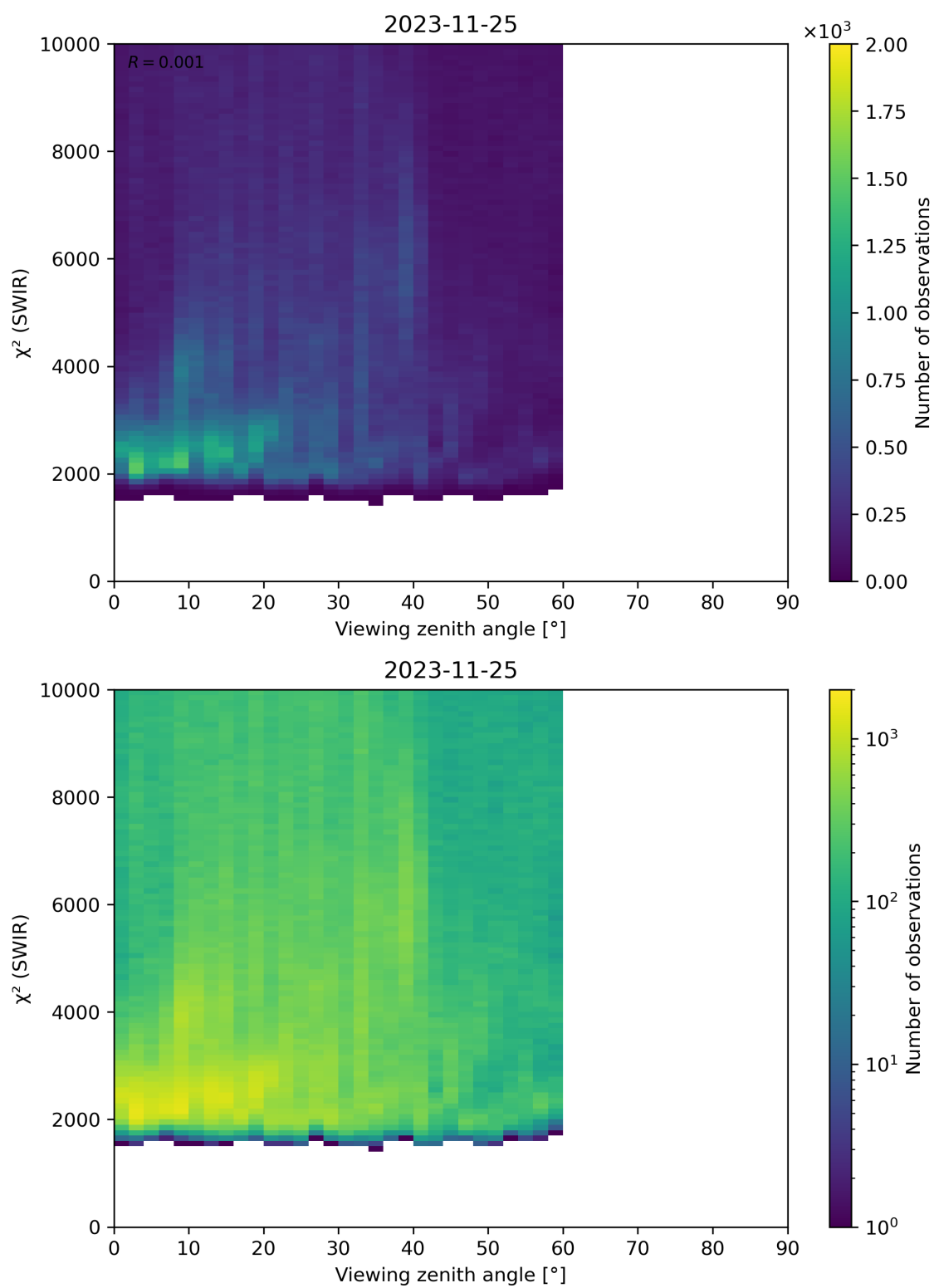
Figure 106: Scatter density plot of “Viewing zenith angle” against “ \chi^2 (SWIR)” for 2023-11-24 to 2023-11-26.
