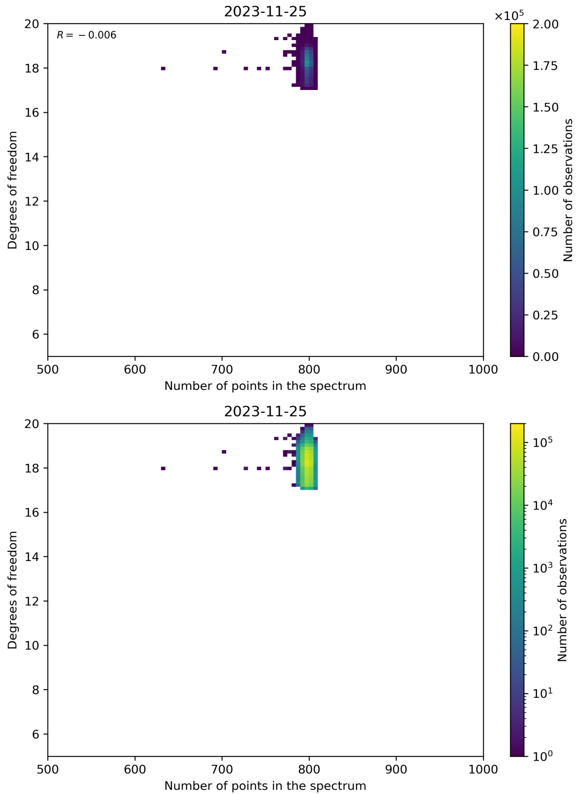
Figure 90: Scatter density plot of “Number of points in the spectrum” against “Degrees of freedom” for 2023-11-24 to 2023-11-26.
