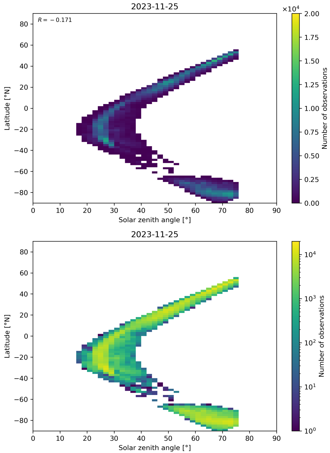
Figure 98: Scatter density plot of “Solar zenith angle” against “Latitude” for 2023-11-24 to 2023-11-26.
