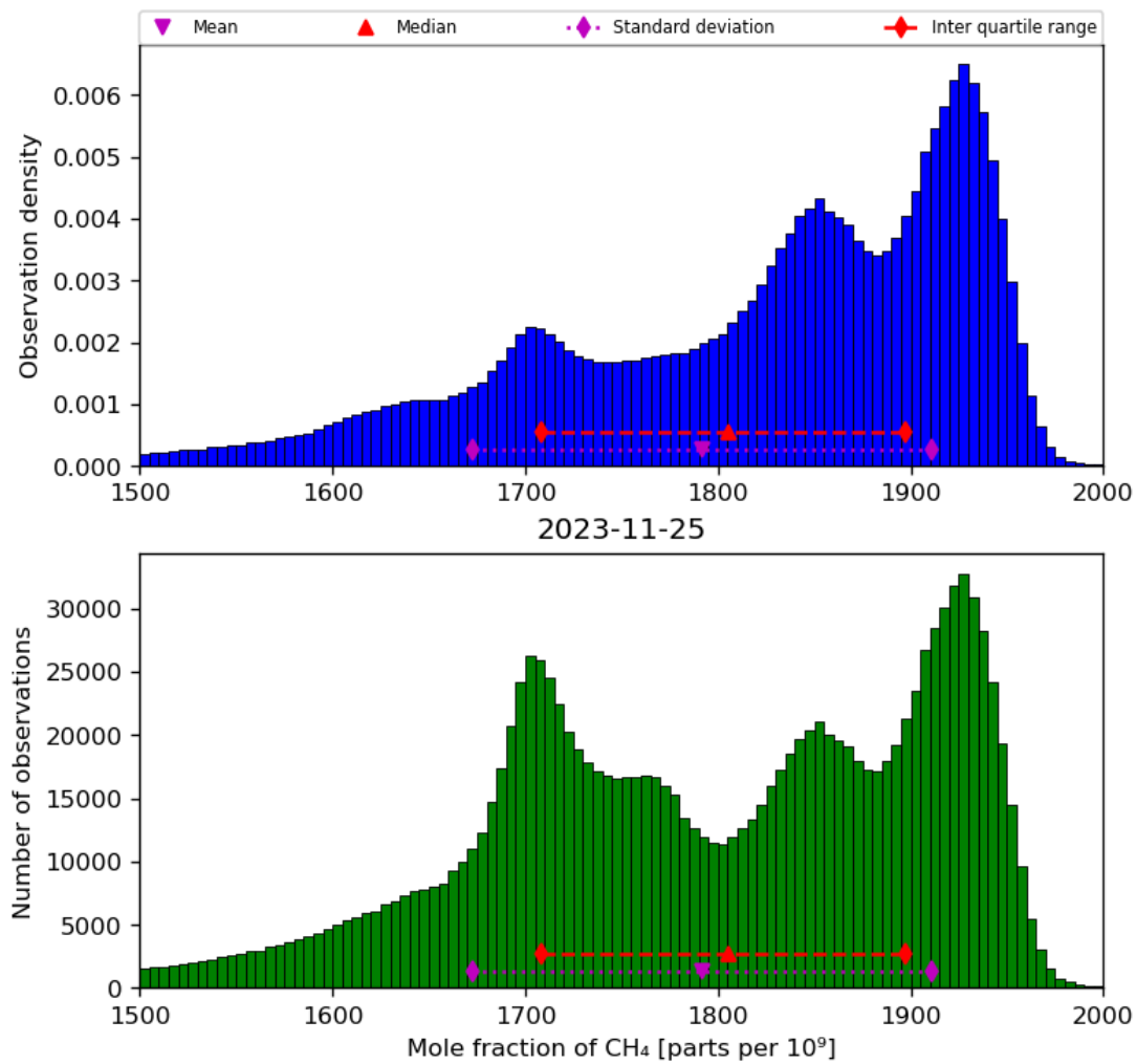
Figure 23: Histogram of “Mole fraction of CH 4 ” for 2023-11-24 to 2023-11-26
