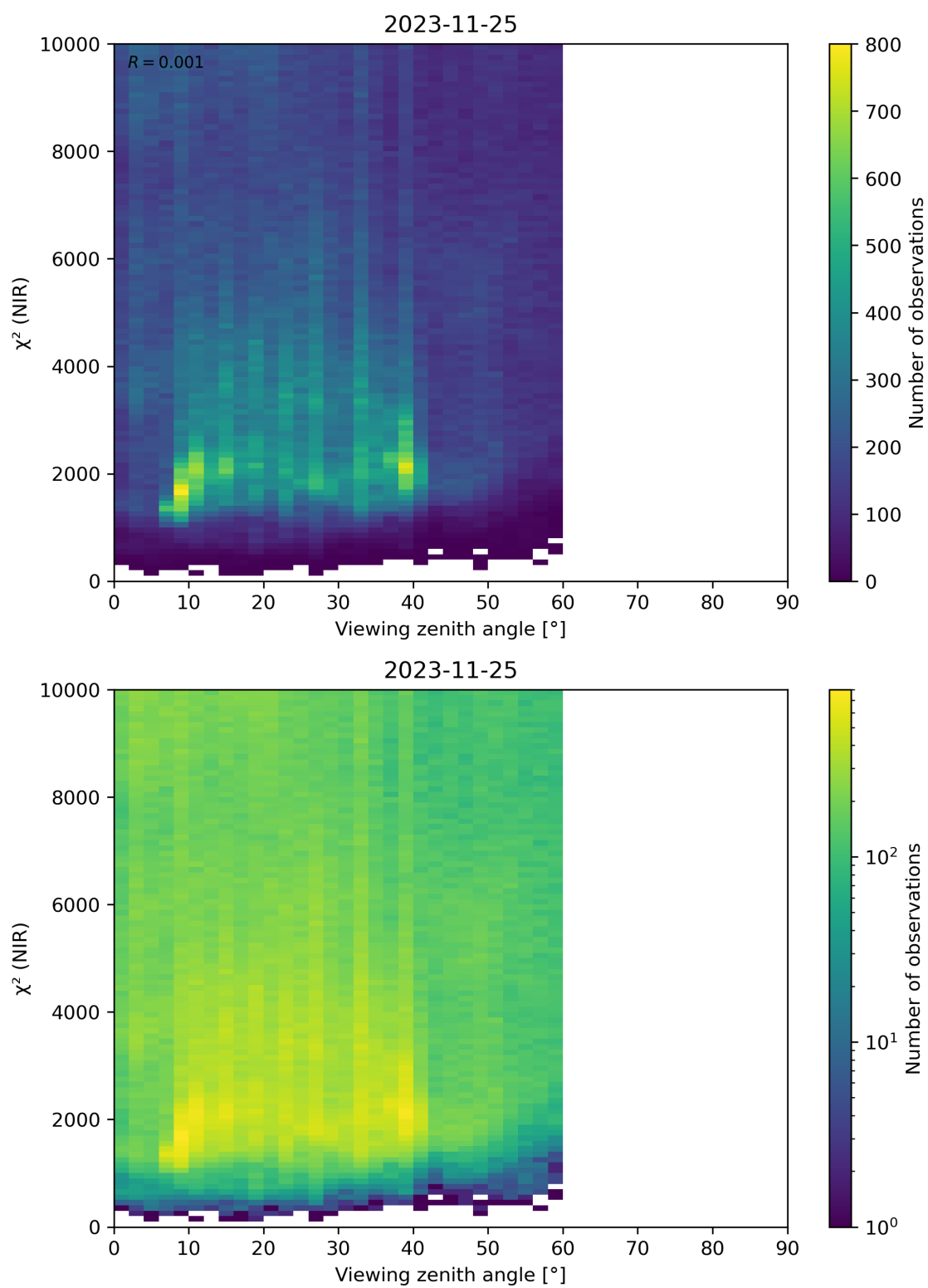
Figure 105: Scatter density plot of “Viewing zenith angle” against “ \chi^2 (NIR)” for 2023-11-24 to 2023-11-26.
