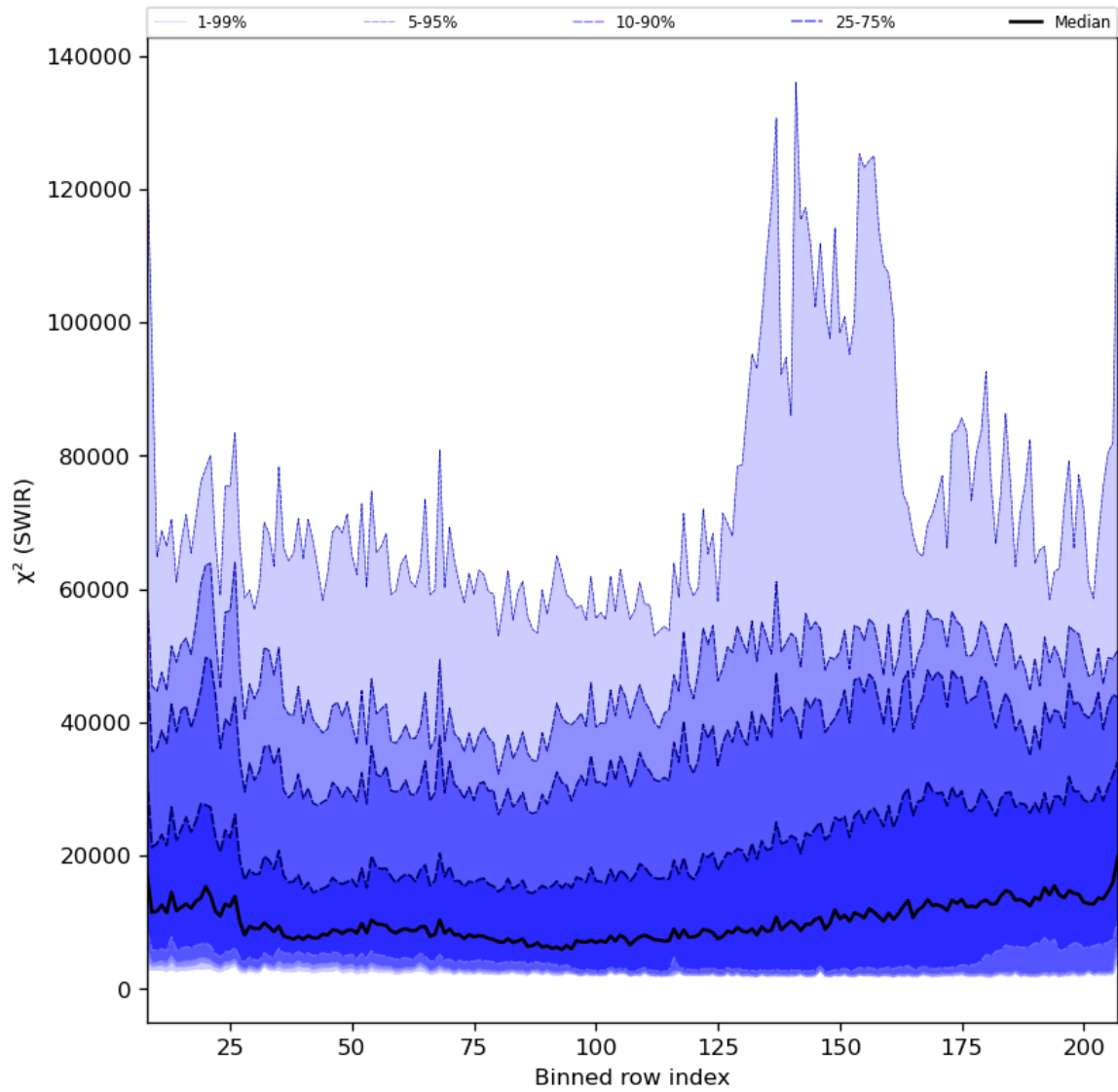
Figure 39: Along track statistics of " \chi^2 (SWIR)" for 2023-11-24 to 2023-11-26
