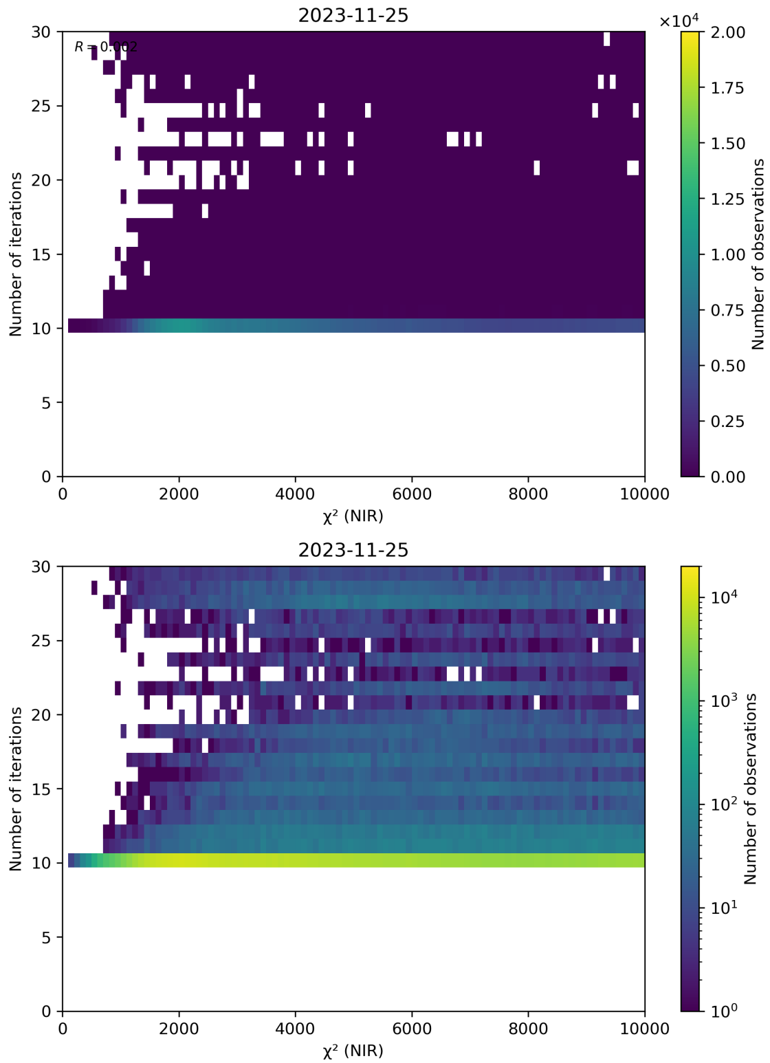
Figure 46: Scatter density plot of “ \chi^2 (NIR)” against “Number of iterations” for 2023-11-24 to 2023-11-26.
