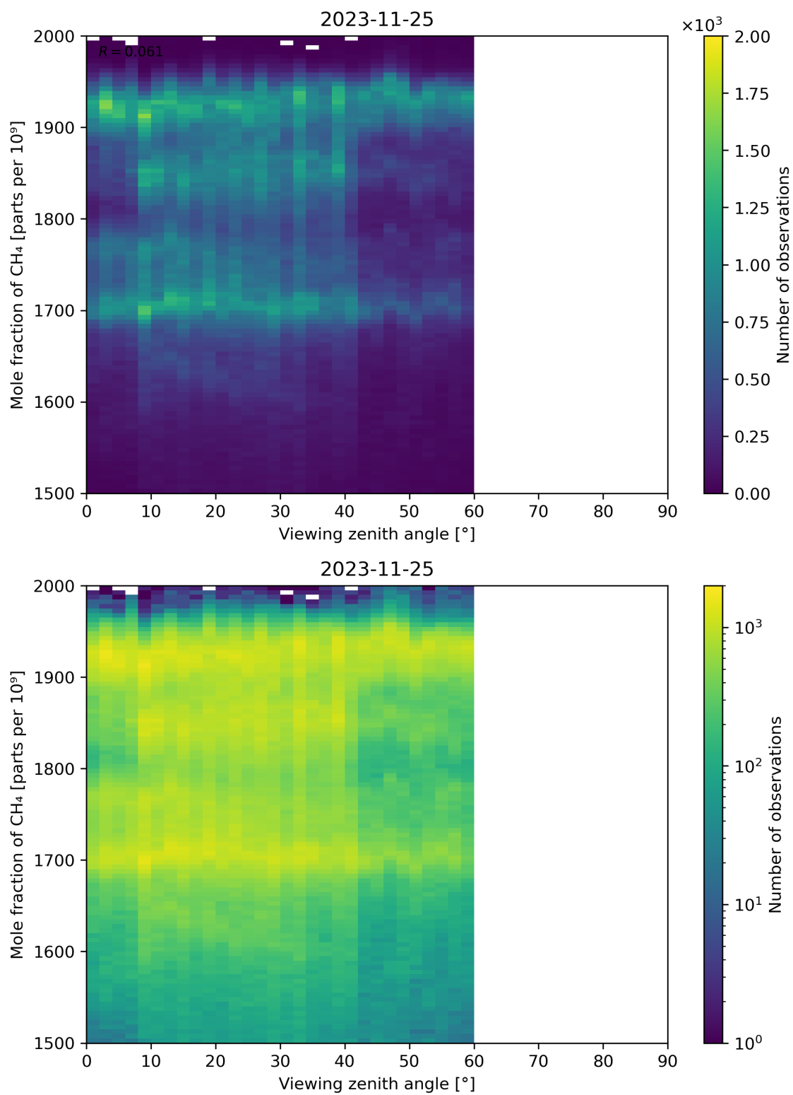
Figure 110: Scatter density plot of “Viewing zenith angle” against “Mole fraction of CH 4 ” for 2023-11-24 to 2023-11-26.
