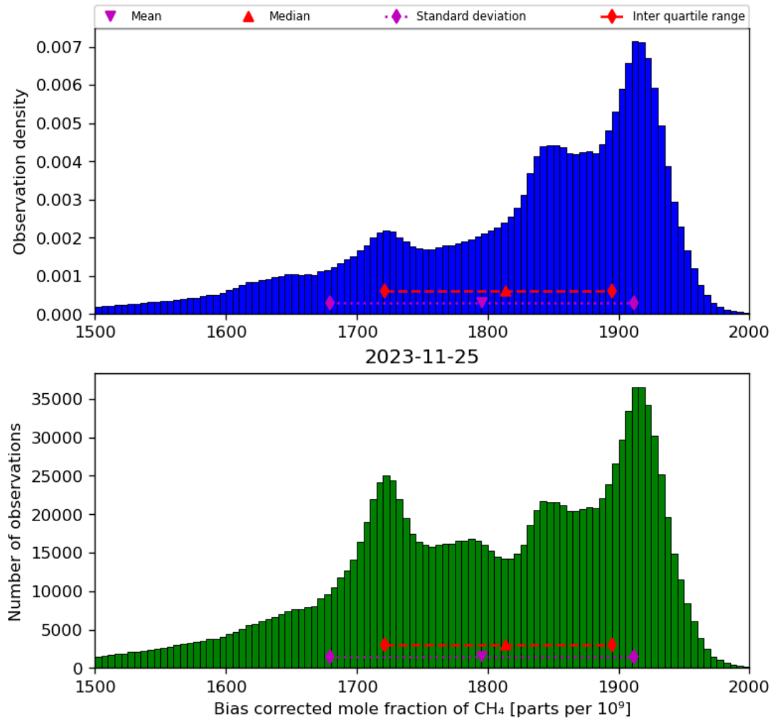
Figure 25: Histogram of “Bias corrected mole fraction of CH 4 ” for 2023-11-24 to 2023-11-26
