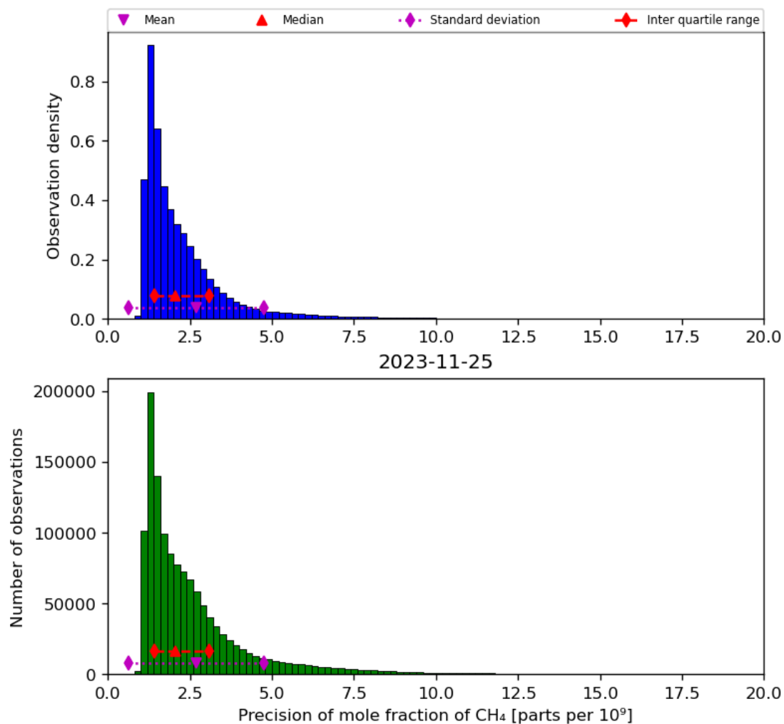
Figure 24: Histogram of “Precision of mole fraction of CH 4 ” for 2023-11-24 to 2023-11-26
