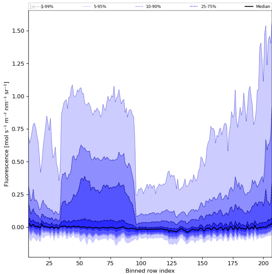
Figure 43: Along track statistics of “Fluorescence” for 2023-11-24 to 2023-11-26
