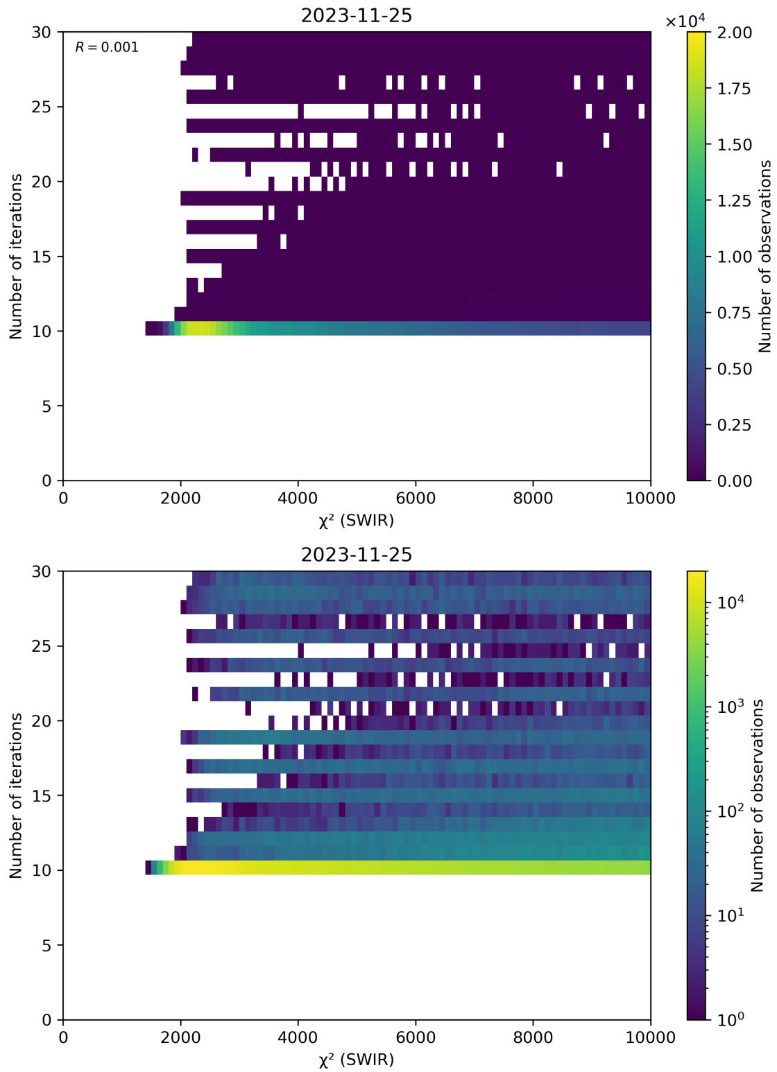
Figure 50: Scatter density plot of “ \chi^2 (SWIR)” against “Number of iterations” for 2023-11-24 to 2023-11-26.
