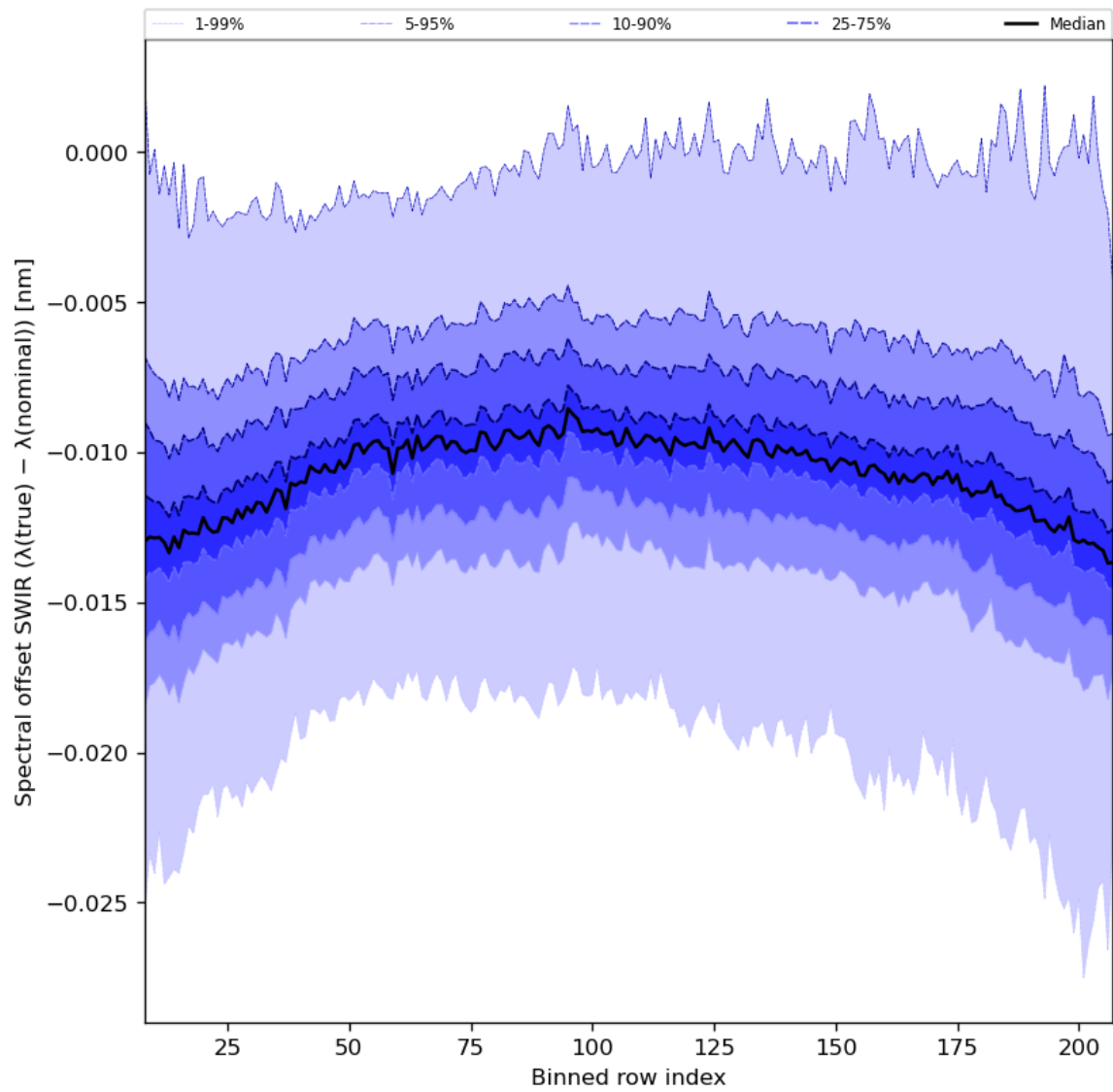
Figure 38: Along track statistics of “Spectral offset SWIR ( \lambda(\text{true}) - \lambda(\text{nominal}) )” for 2023-11-24 to 2023-11-26
