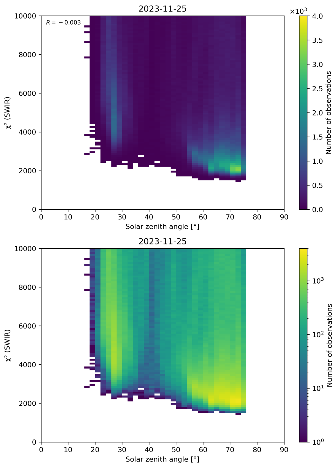
Figure 95: Scatter density plot of “Solar zenith angle” against “ \chi^2 (SWIR)” for 2023-11-24 to 2023-11-26.
