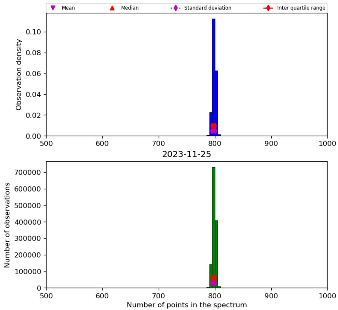
Figure 26: Histogram of “Number of points in the spectrum” for 2023-11-24 to 2023-11-26
