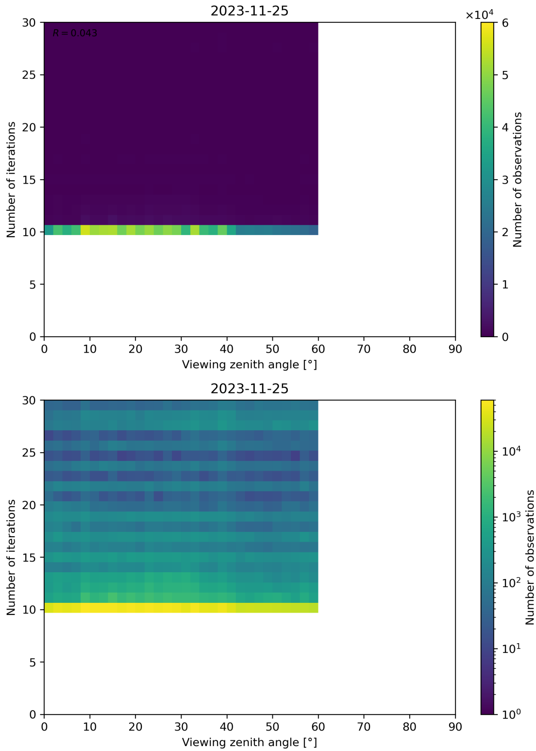
Figure 113: Scatter density plot of “Viewing zenith angle” against “Number of iterations” for 2023-11-24 to 2023-11-26.
