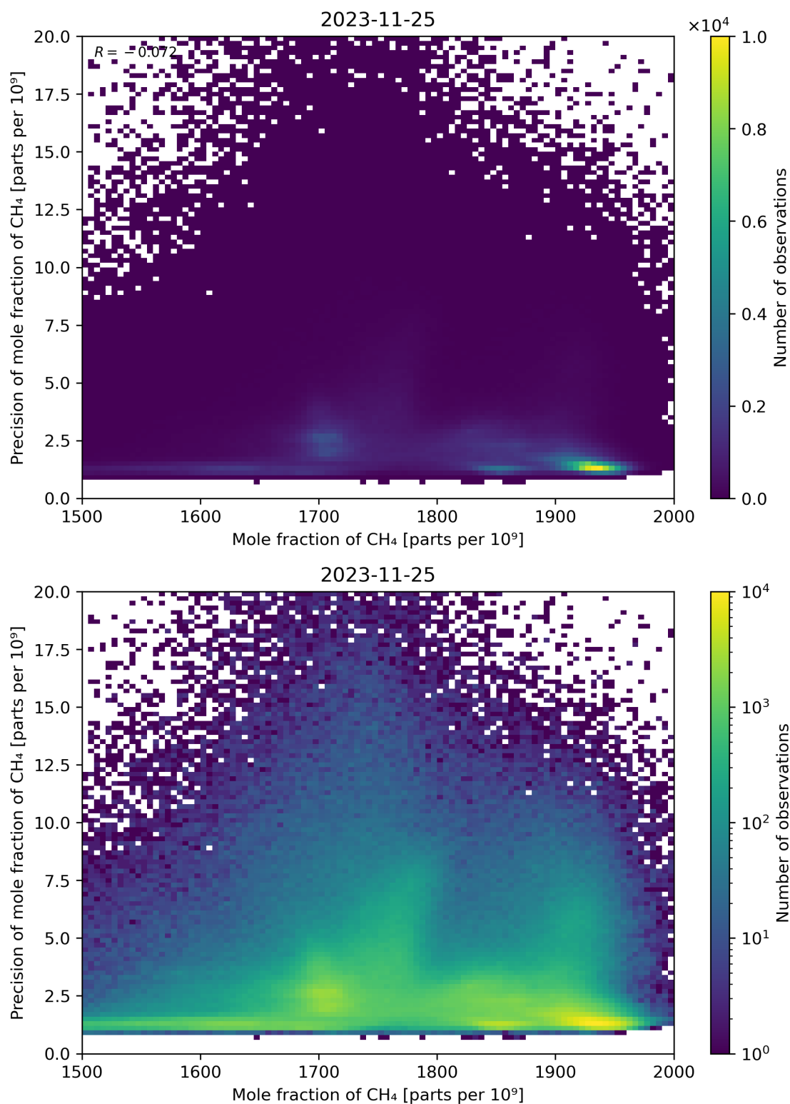
Figure 75: Scatter density plot of “Mole fraction of CH 4 ” against “Precision of mole fraction of CH 4 ” for 2023-11-24 to 2023-11-26.
