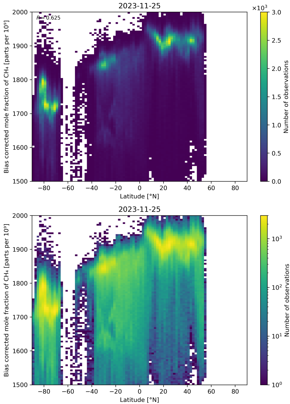
Figure 58: Scatter density plot of “Latitude” against “Bias corrected mole fraction of CH 4 ” for 2023-11-24 to 2023-11-26.
