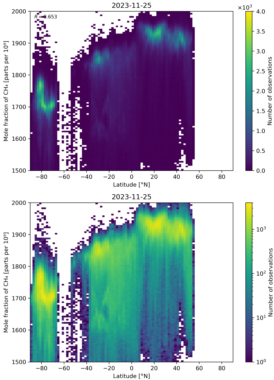
Figure 57: Scatter density plot of “Latitude” against “Mole fraction of CH 4 ” for 2023-11-24 to 2023-11-26.
