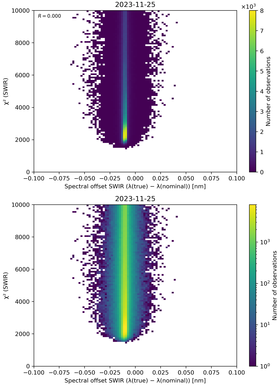
Figure 118: Scatter density plot of “Spectral offset SWIR ( \lambda(\text{true}) - \lambda(\text{nominal}) )” against “ \chi^2 (SWIR)” for 2023-11-24 to 2023-11-26.
