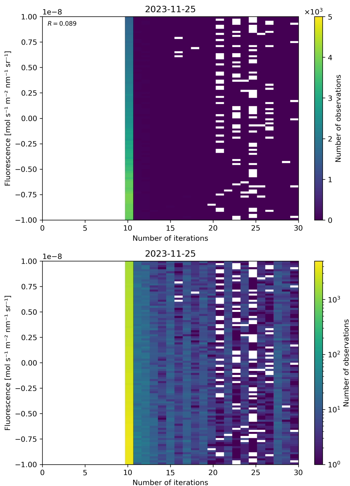
Figure 87: Scatter density plot of “Number of iterations” against “Fluorescence” for 2023-11-24 to 2023-11-26.
