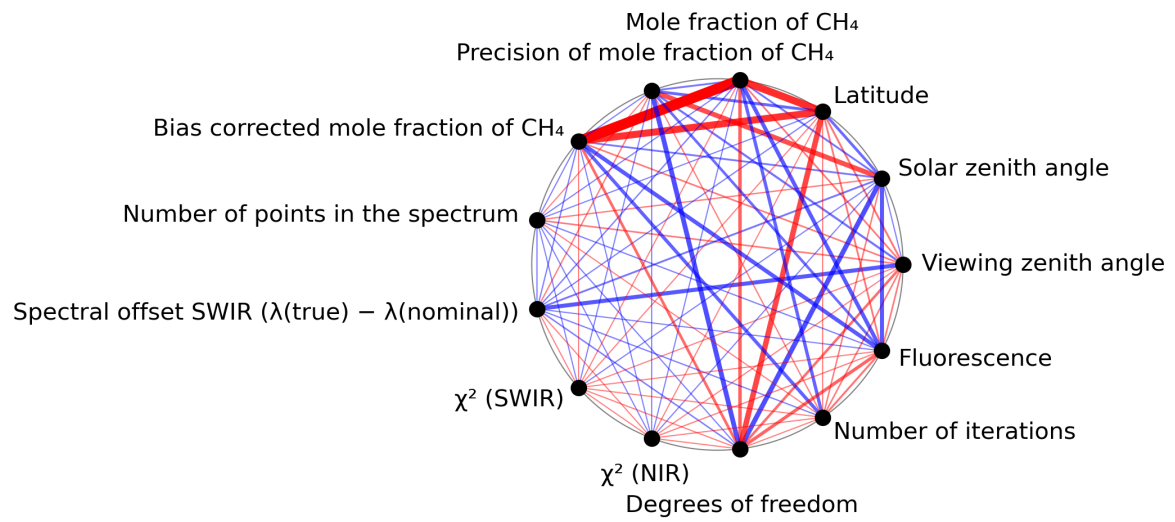
Figure 1: Map of correlation graph for 2023-11-24 to 2023-11-26.
