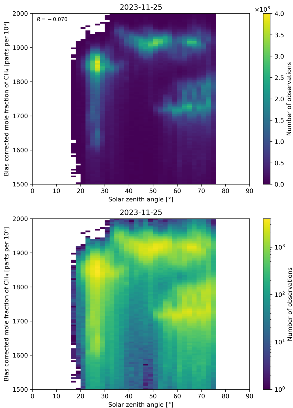
Figure 100: Scatter density plot of “Solar zenith angle” against “Bias corrected mole fraction of CH 4 ” for 2023-11-24 to 2023-11-26.
