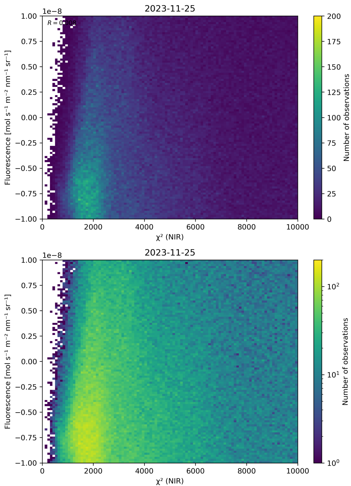
Figure 45: Scatter density plot of “ \chi^2 (NIR)” against “Fluorescence” for 2023-11-24 to 2023-11-26.
