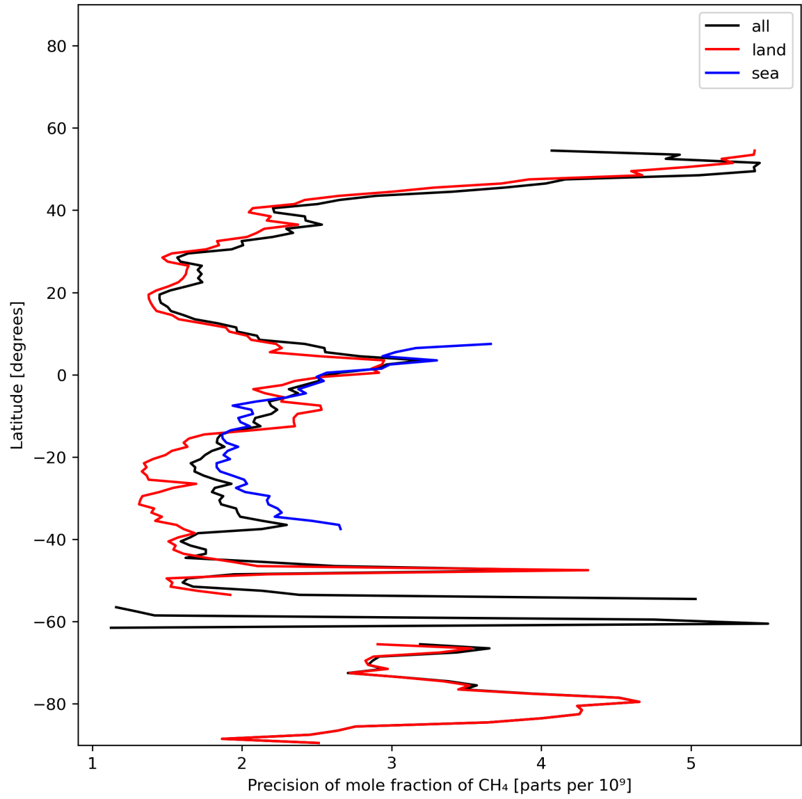
Figure 13: Zonal average of “Precision of mole fraction of CH 4 ” for 2023-11-24 to 2023-11-26.
