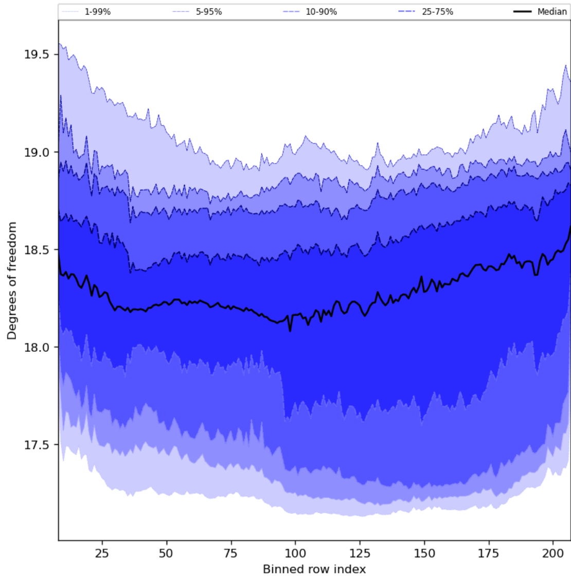
Figure 41: Along track statistics of “Degrees of freedom” for 2023-11-24 to 2023-11-26
