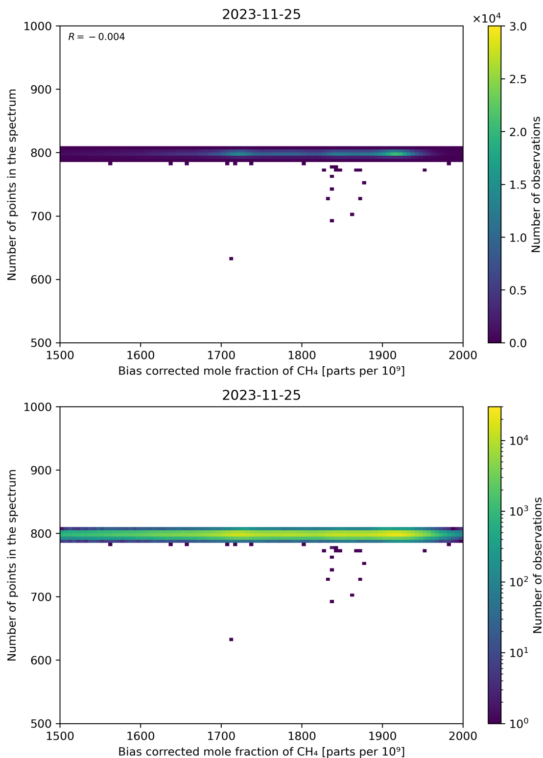
Figure 68: Scatter density plot of “Bias corrected mole fraction of CH 4 ” against “Number of points in the spectrum” for 2023-11-24 to 2023-11-26.
