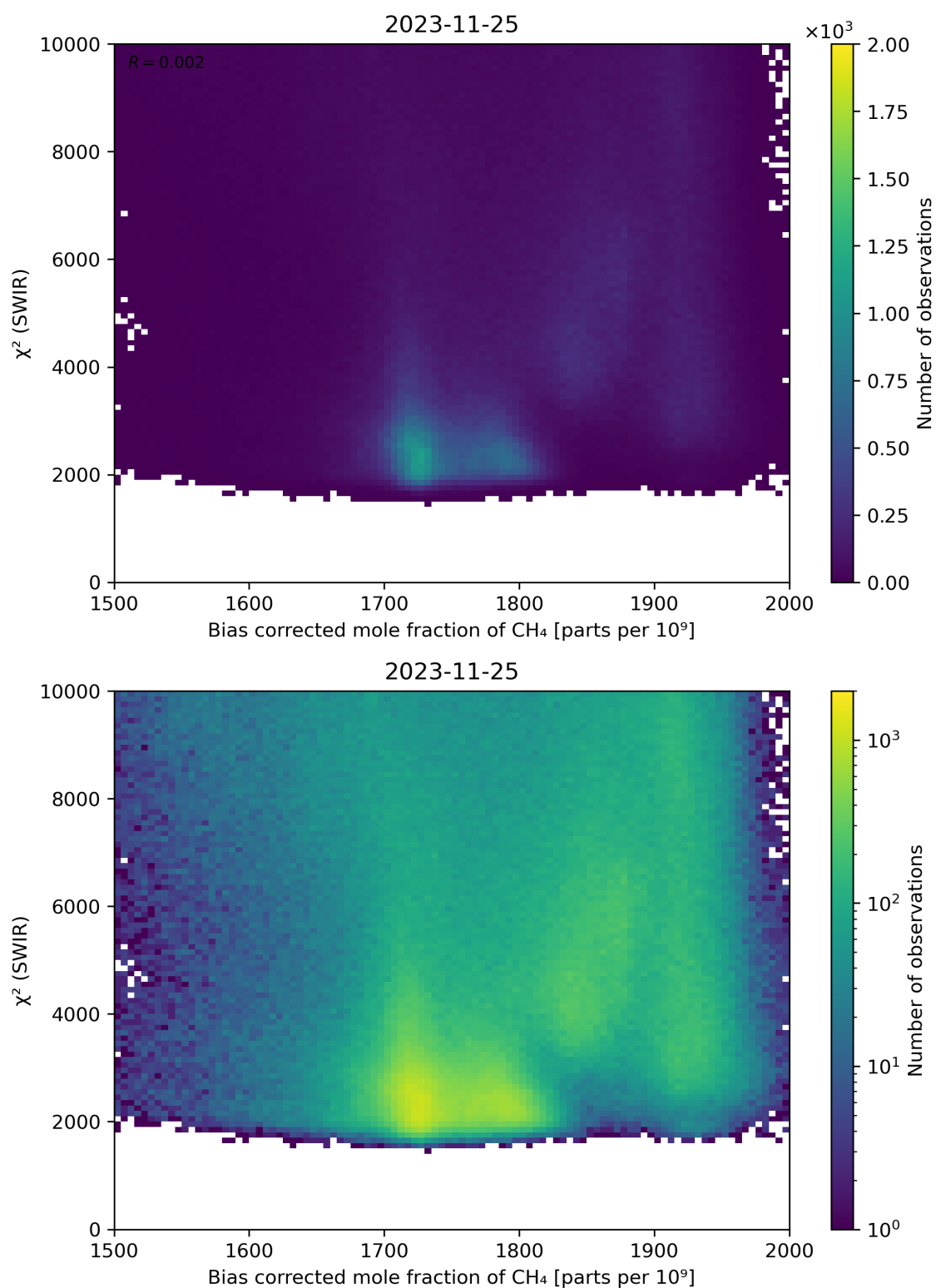
Figure 64: Scatter density plot of “Bias corrected mole fraction of CH 4 ” against “ \chi^2 (SWIR)” for 2023-11-24 to 2023-11-26.
