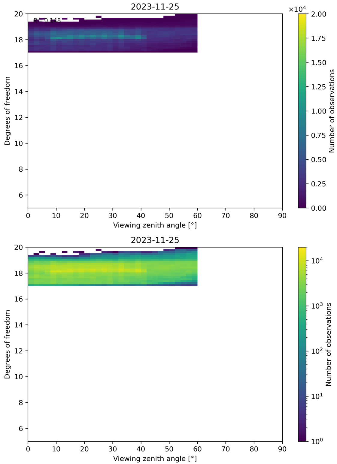
Figure 107: Scatter density plot of “Viewing zenith angle” against “Degrees of freedom” for 2023-11-24 to 2023-11-26.
