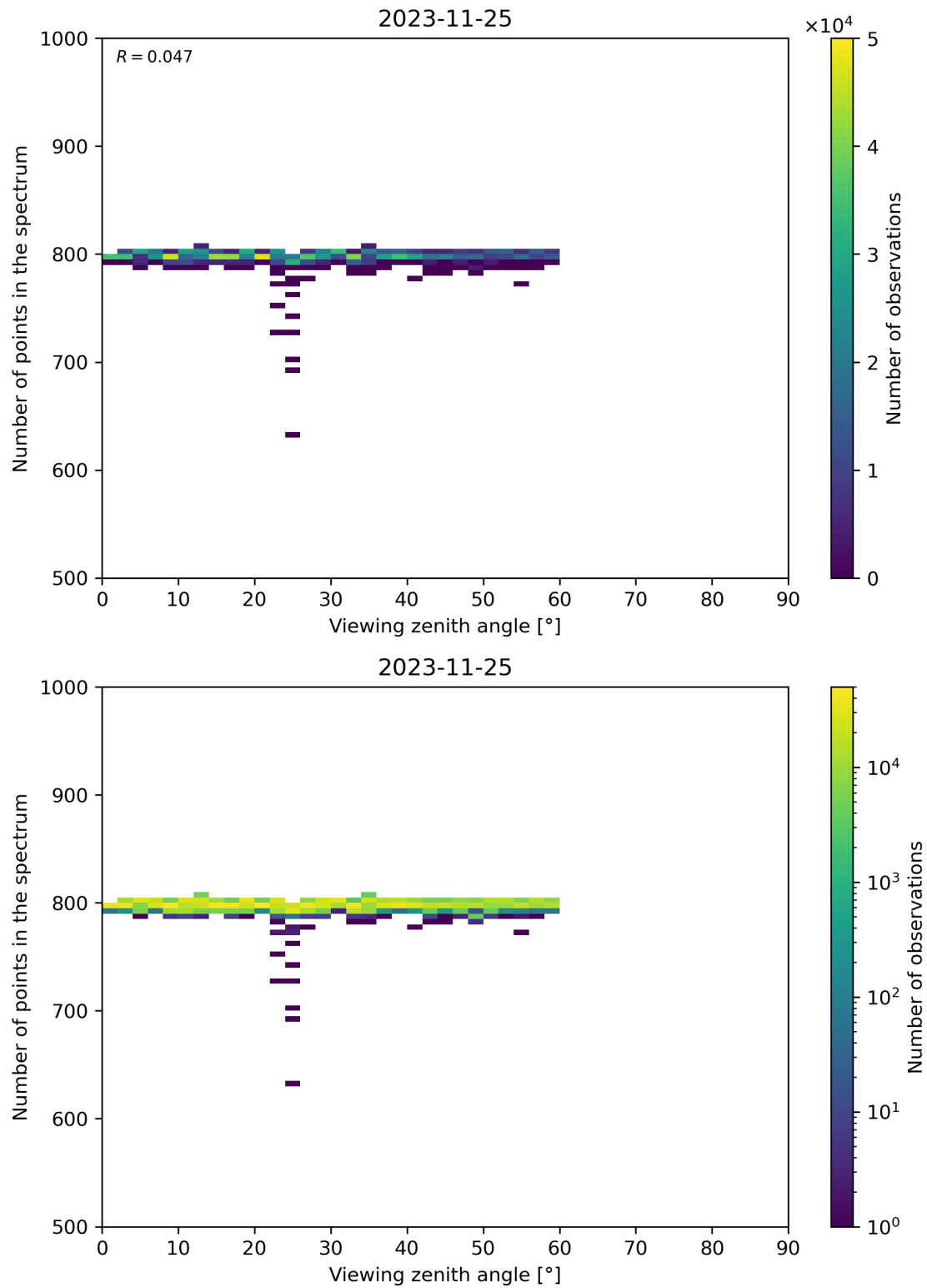
Figure 114: Scatter density plot of “Viewing zenith angle” against “Number of points in the spectrum” for 2023-11-24 to 2023-11-26.
