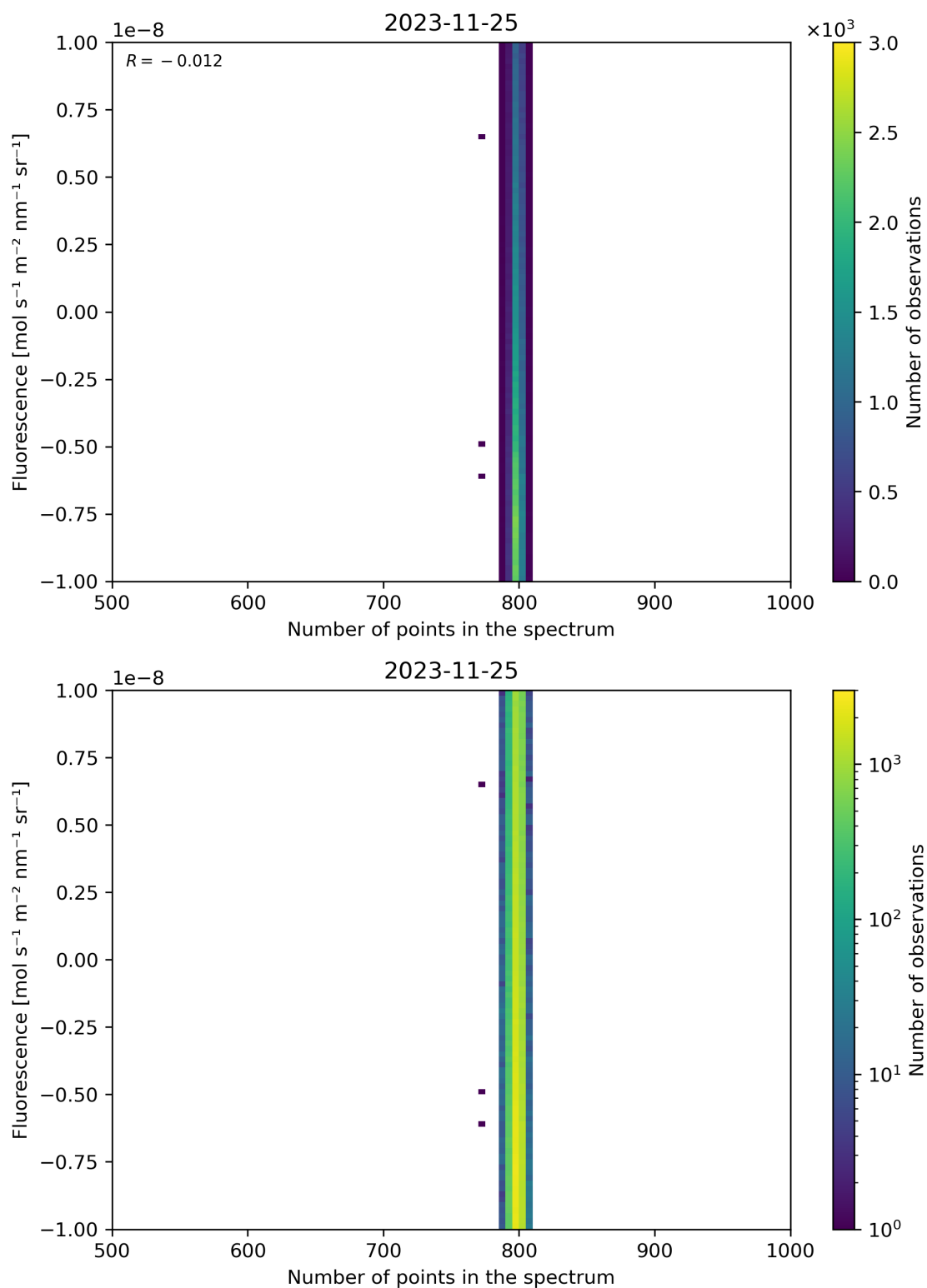
Figure 91: Scatter density plot of “Number of points in the spectrum” against “Fluorescence” for 2023-11-24 to 2023-11-26.
