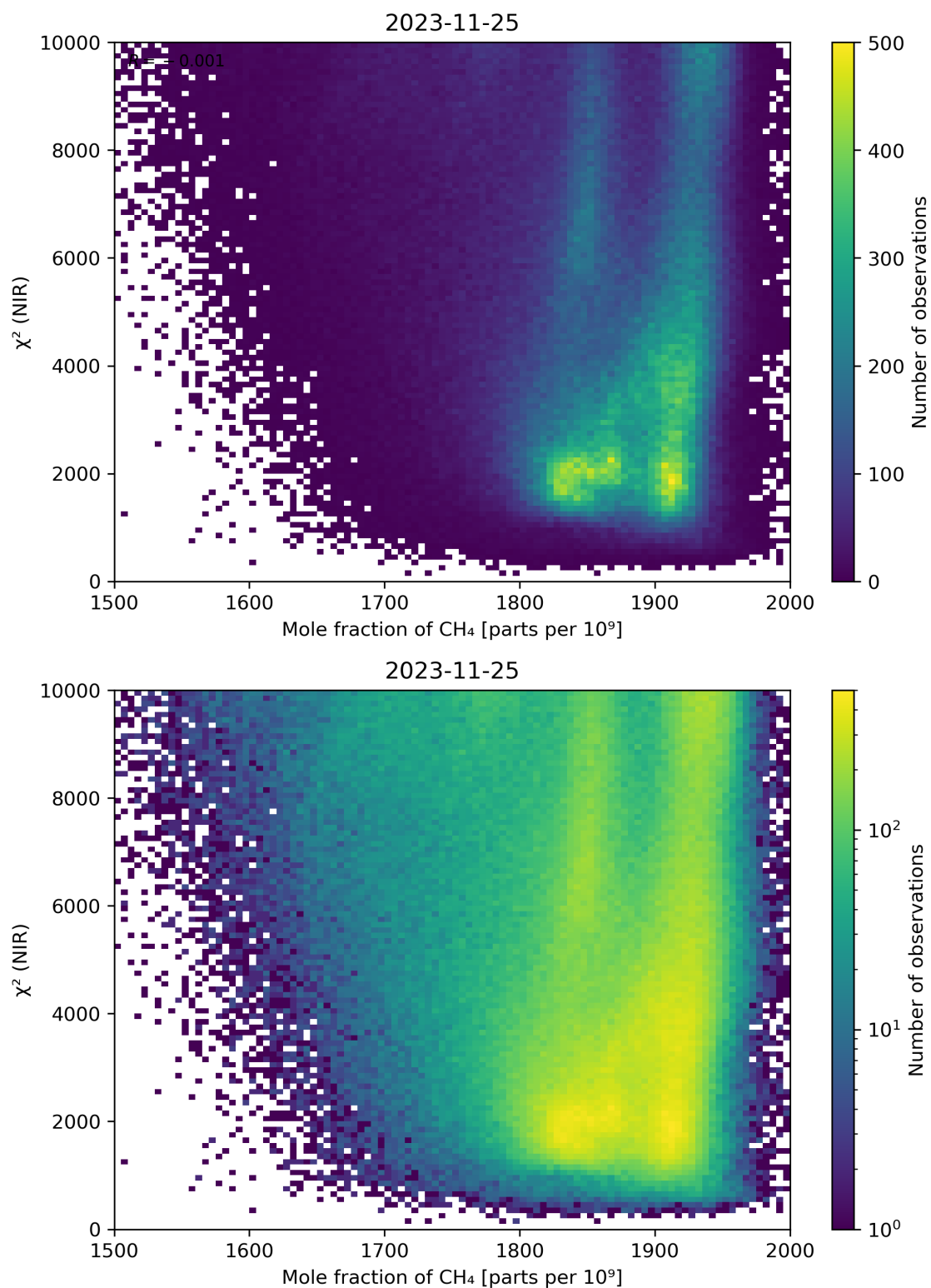
Figure 70: Scatter density plot of “Mole fraction of \text{CH}_4 ” against “ \chi^2 (NIR)” for 2023-11-24 to 2023-11-26.
