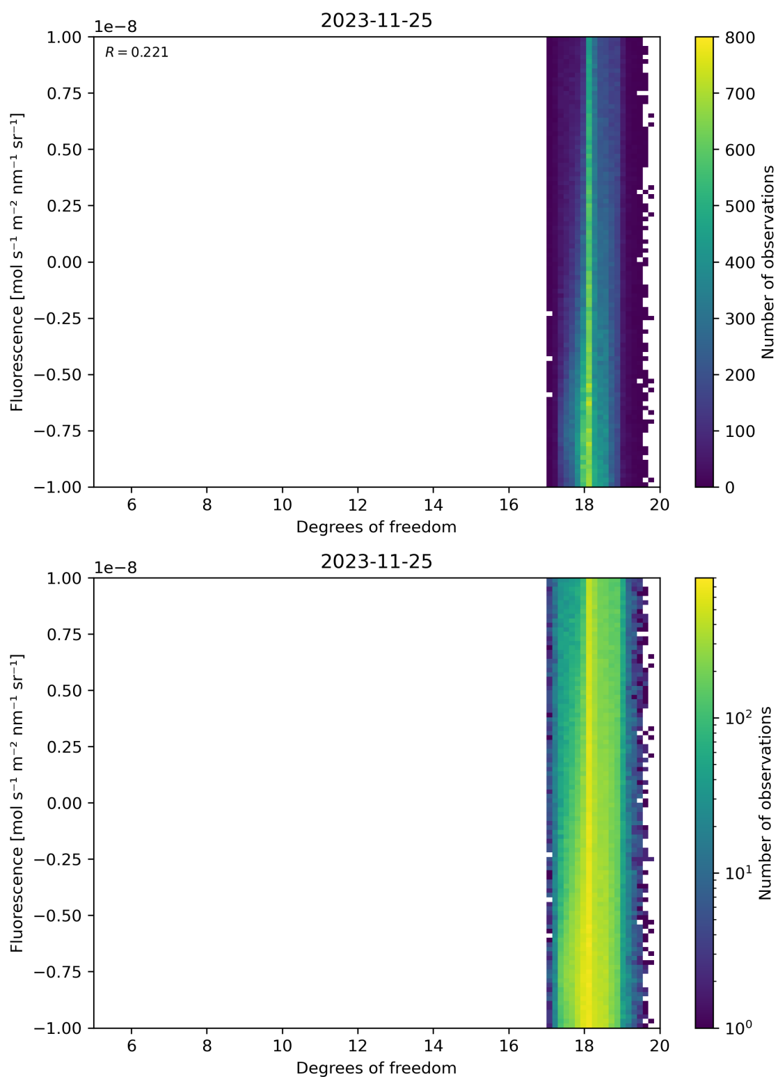
Figure 51: Scatter density plot of “Degrees of freedom” against “Fluorescence” for 2023-11-24 to 2023-11-26.
