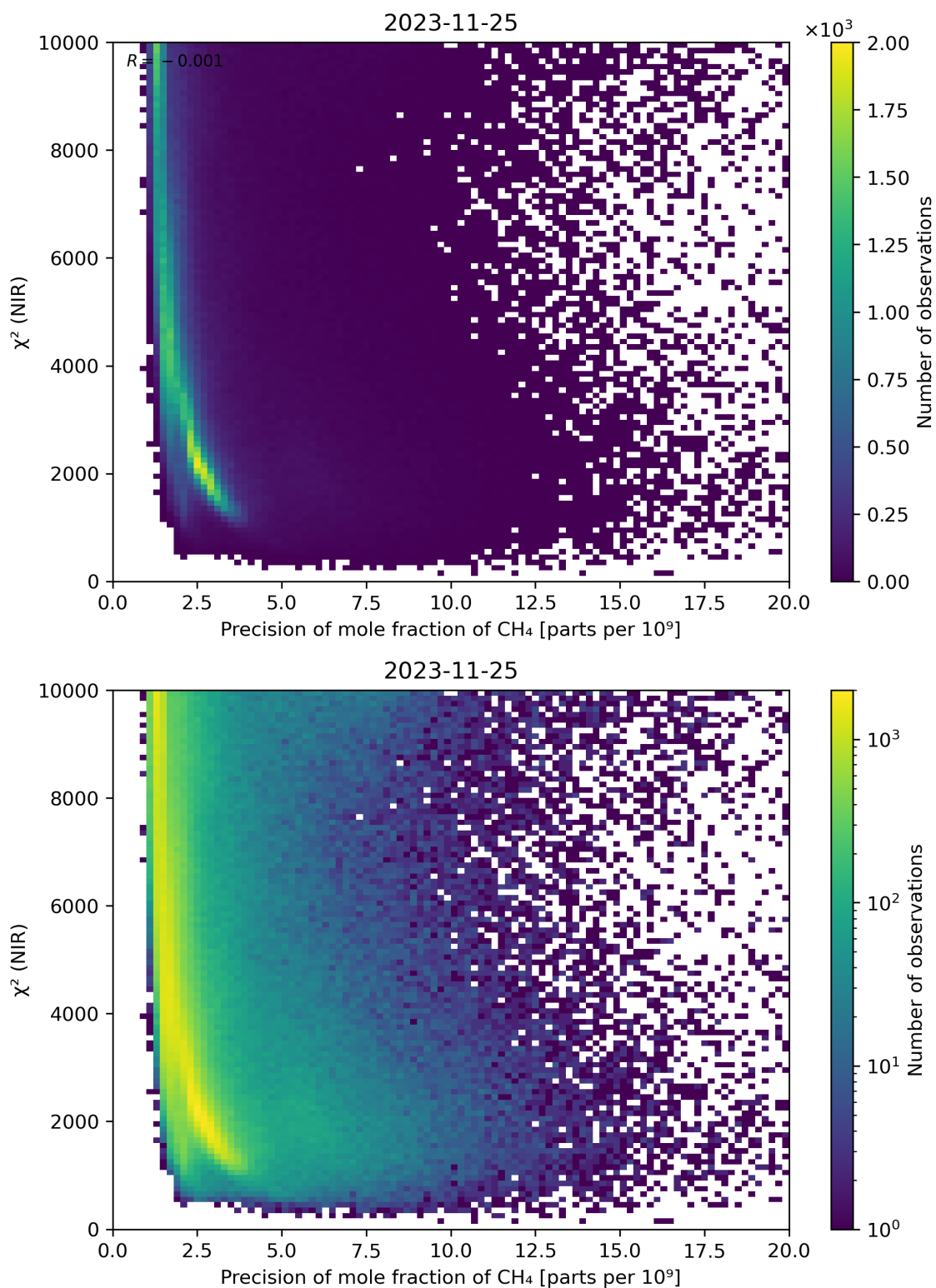
Figure 78: Scatter density plot of “Precision of mole fraction of CH 4 ” against “ \chi^2 (NIR)” for 2023-11-24 to 2023-11-26.
