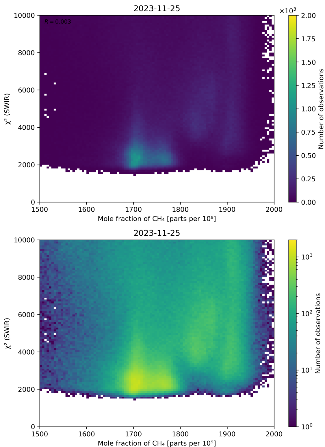
Figure 71: Scatter density plot of “Mole fraction of \text{CH}_4 ” against “ \chi^2 (SWIR)” for 2023-11-24 to 2023-11-26.
