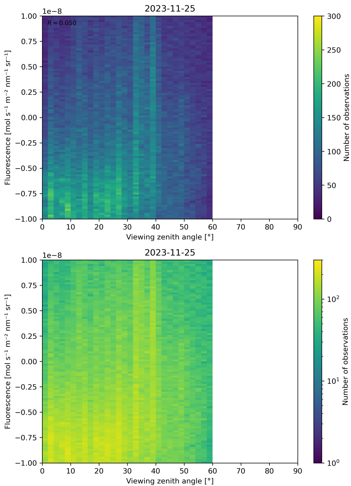
Figure 108: Scatter density plot of “Viewing zenith angle” against “Fluorescence” for 2023-11-24 to 2023-11-26.
