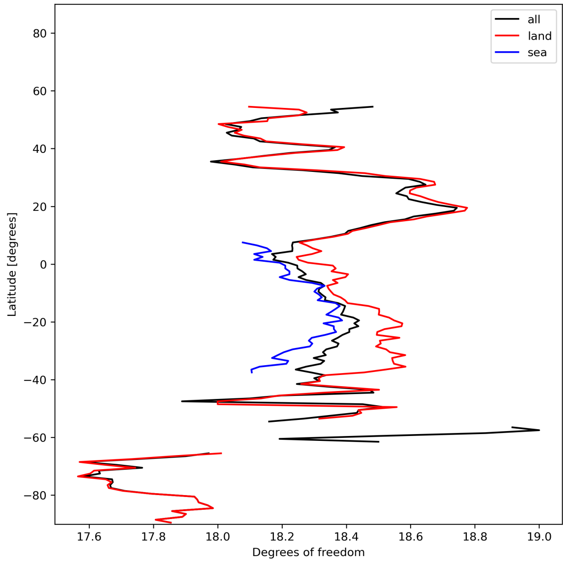
Figure 19: Zonal average of “Degrees of freedom” for 2023-11-24 to 2023-11-26.
