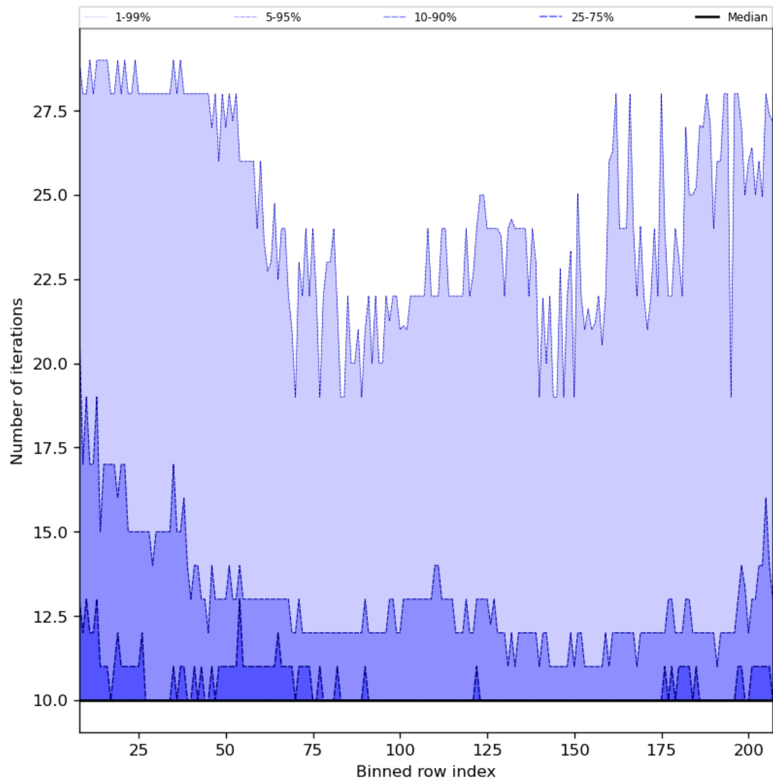
Figure 42: Along track statistics of “Number of iterations” for 2023-11-24 to 2023-11-26
