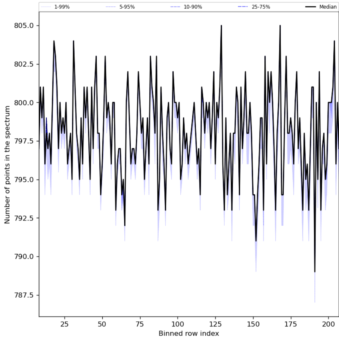
Figure 37: Along track statistics of “Number of points in the spectrum” for 2023-11-24 to 2023-11-26
