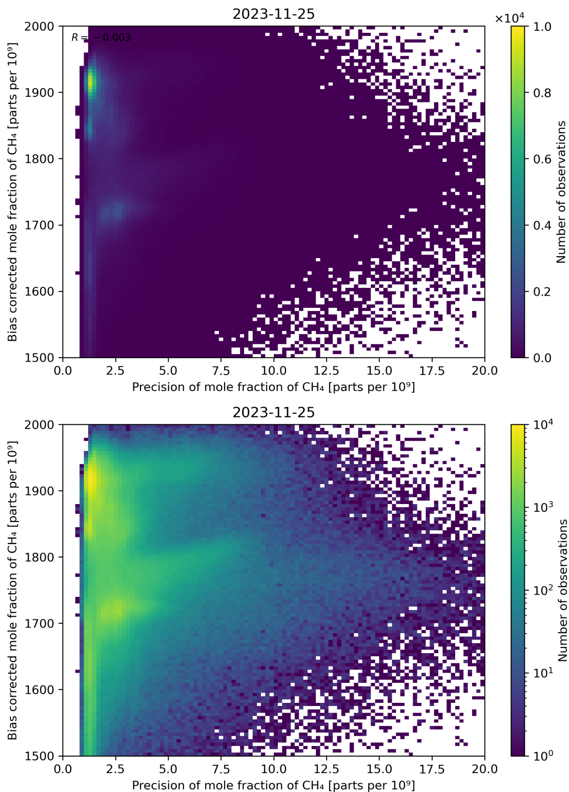
Figure 82: Scatter density plot of “Precision of mole fraction of CH 4 ” against “Bias corrected mole fraction of CH 4 ” for 2023-11-24 to 2023-11-26.
