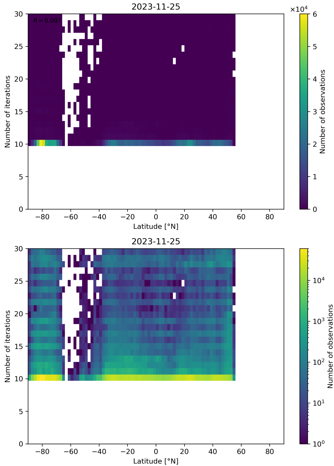
Figure 60: Scatter density plot of “Latitude” against “Number of iterations” for 2023-11-24 to 2023-11-26.
