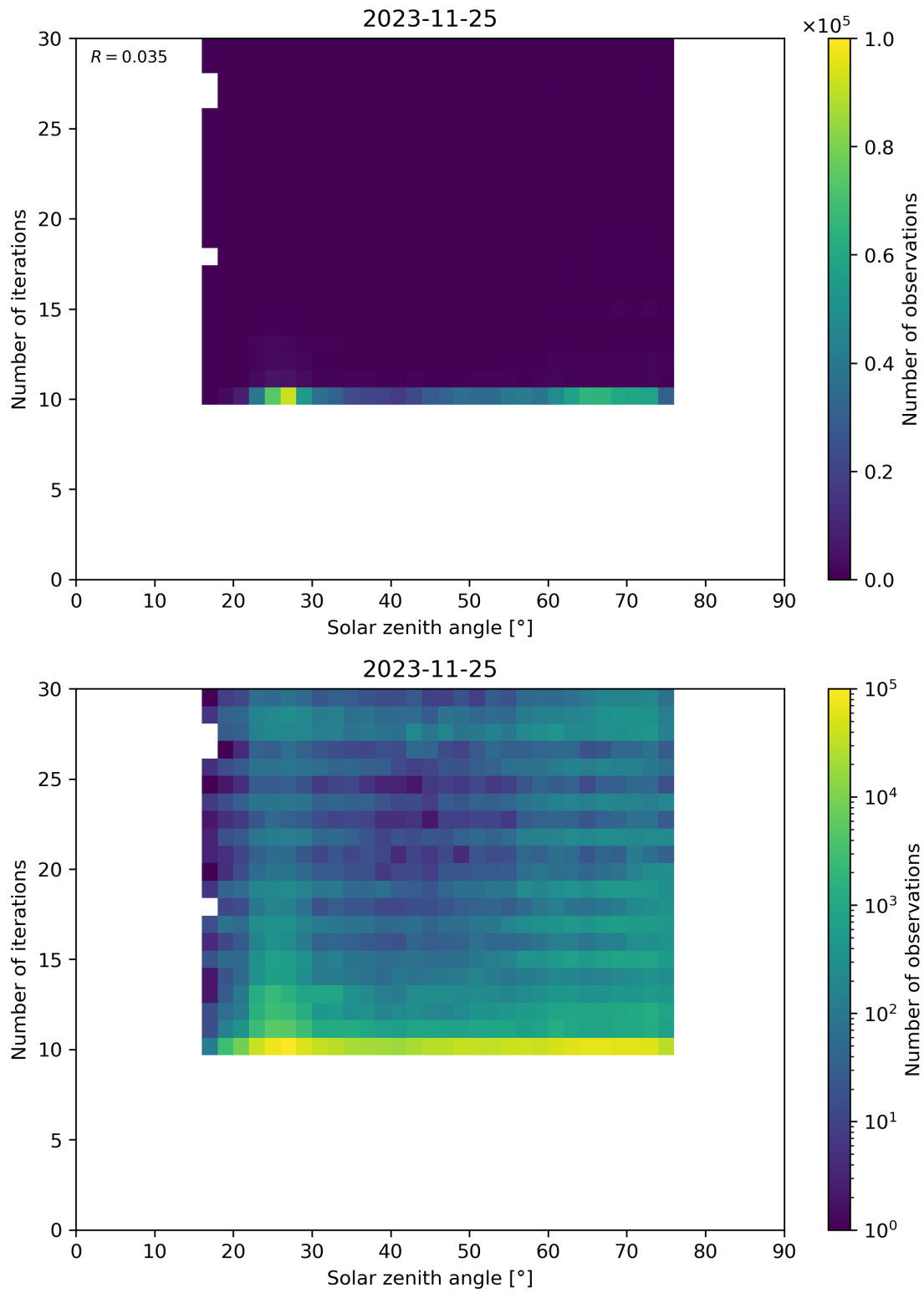
Figure 102: Scatter density plot of “Solar zenith angle” against “Number of iterations” for 2023-11-24 to 2023-11-26.
