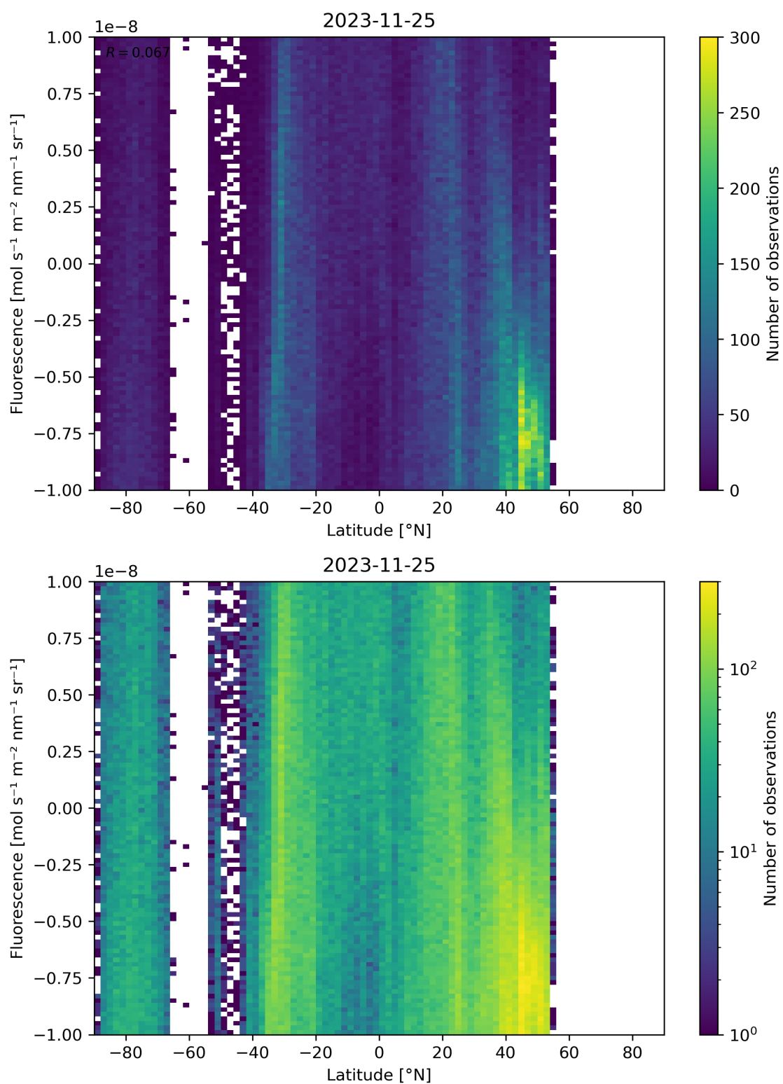
Figure 56: Scatter density plot of “Latitude” against “Fluorescence” for 2023-11-24 to 2023-11-26.
