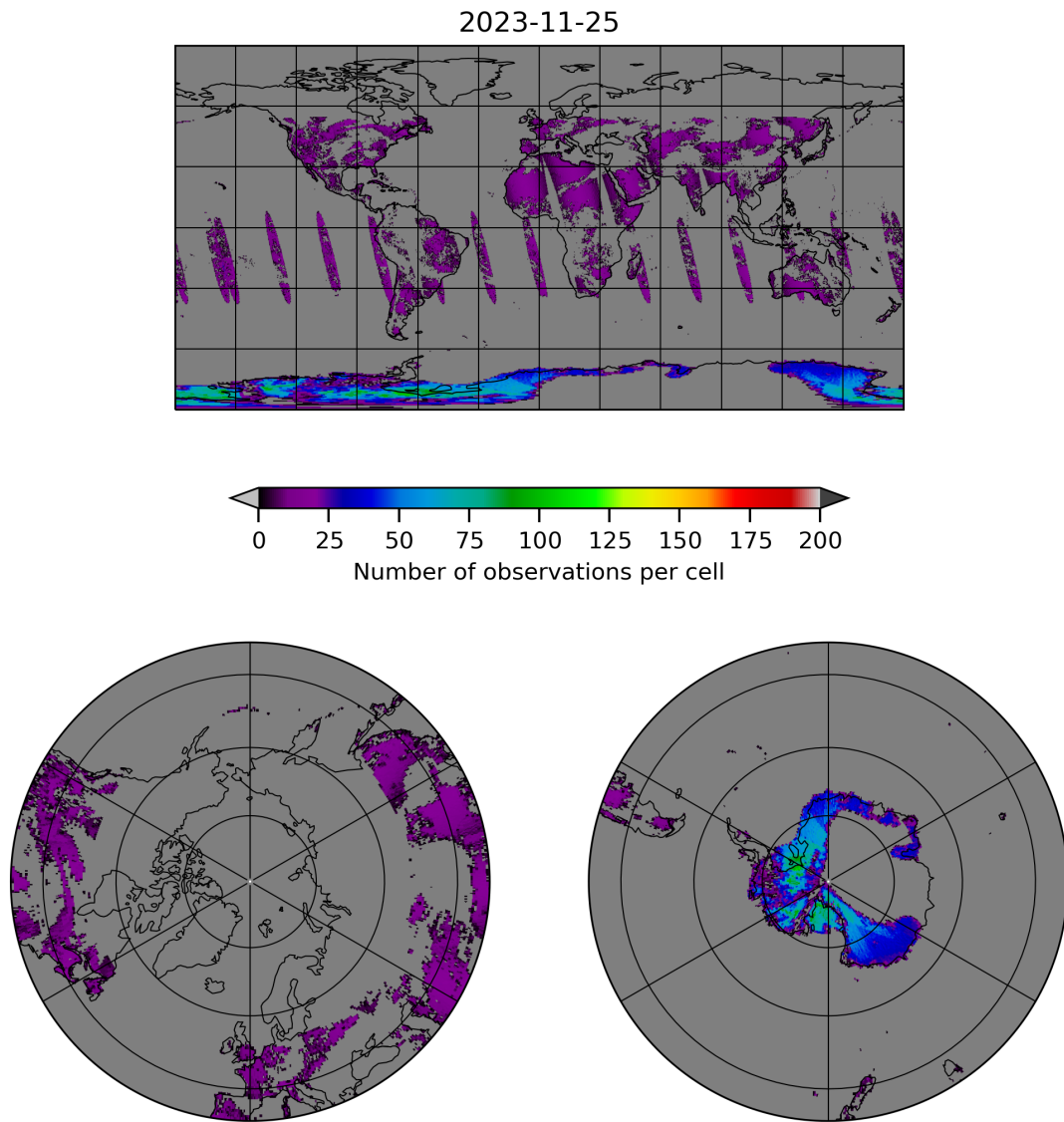
Figure 10: Map of the number of observations for 2023-11-24 to 2023-11-26
