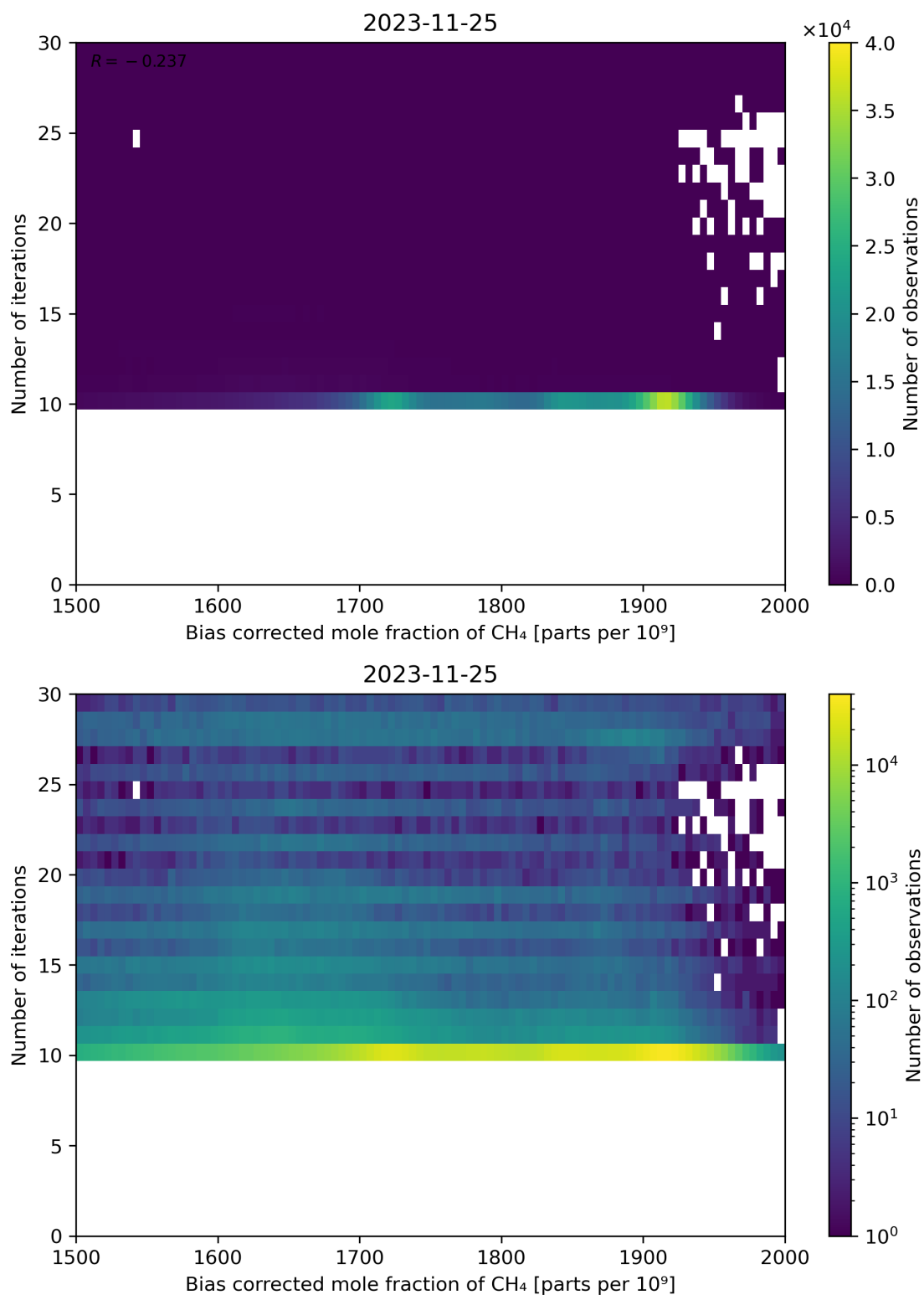
Figure 67: Scatter density plot of “Bias corrected mole fraction of \text{CH}_4 ” against “Number of iterations” for 2023-11-24 to 2023-11-26.
