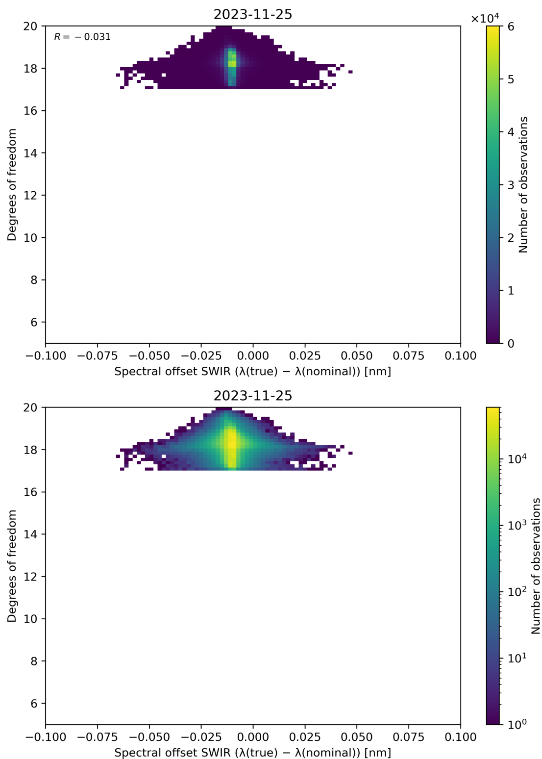
Figure 119: Scatter density plot of “Spectral offset SWIR ( \lambda(\text{true}) - \lambda(\text{nominal}) )” against “Degrees of freedom” for 2023-11-24 to 2023-11-26.
