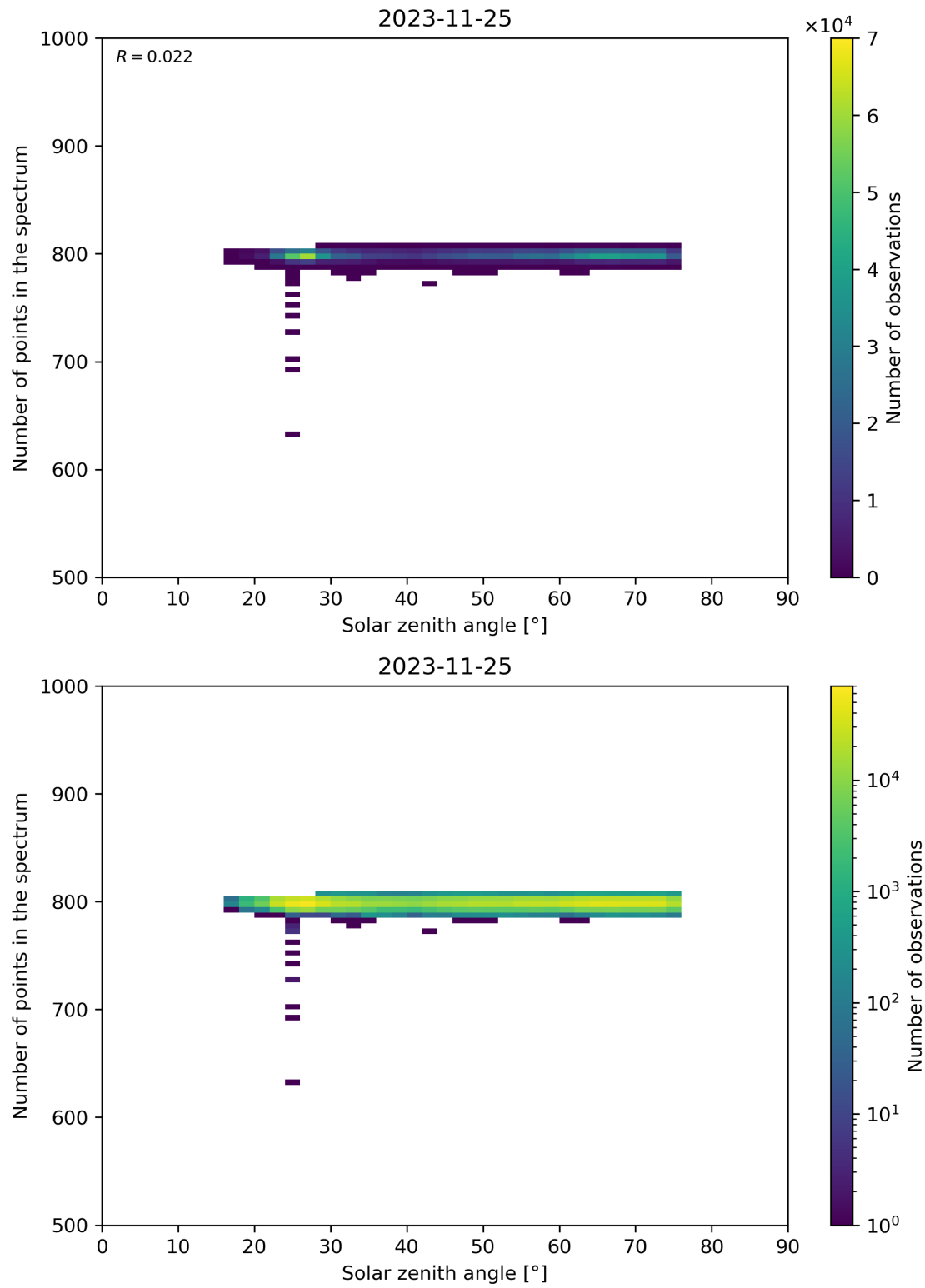
Figure 103: Scatter density plot of “Solar zenith angle” against “Number of points in the spectrum” for 2023-11-24 to 2023-11-26.
