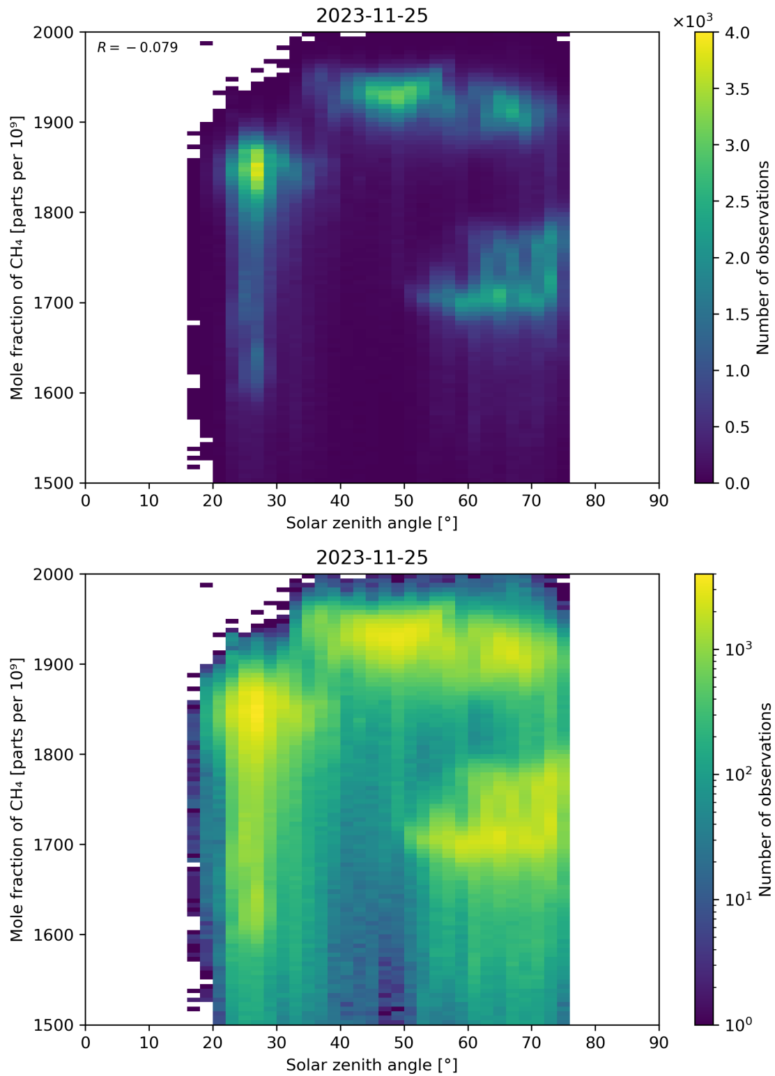
Figure 99: Scatter density plot of “Solar zenith angle” against “Mole fraction of CH 4 ” for 2023-11-24 to 2023-11-26.
