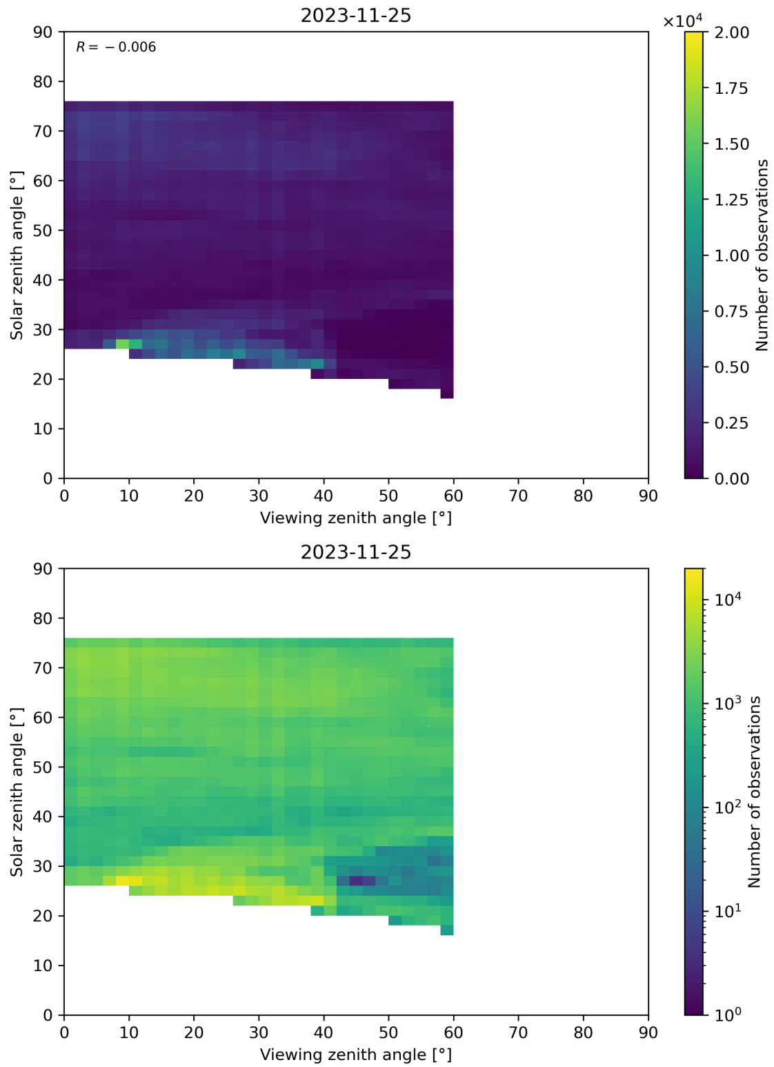
Figure 115: Scatter density plot of “Viewing zenith angle” against “Solar zenith angle” for 2023-11-24 to 2023-11-26.
