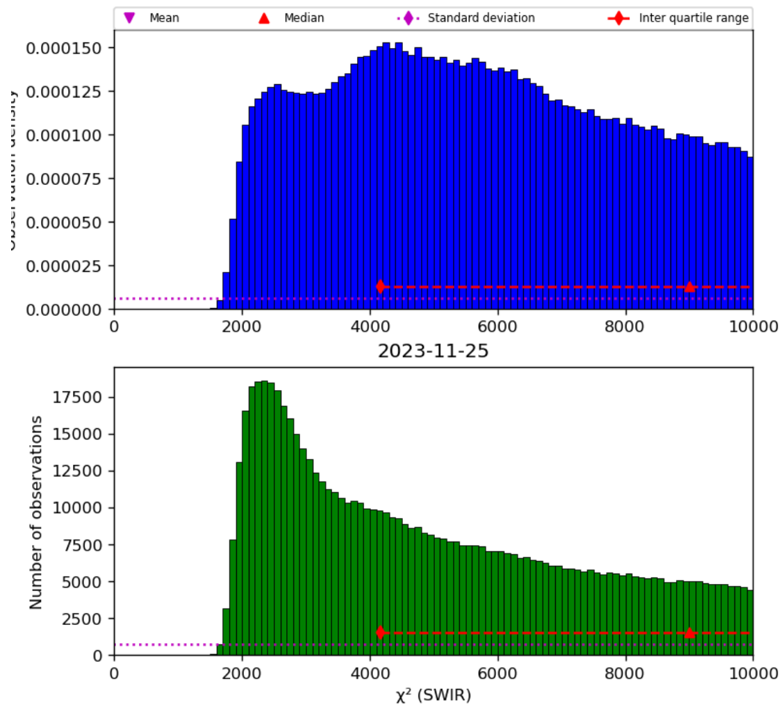
Figure 28: Histogram of “ \chi^2 (SWIR)” for 2023-11-24 to 2023-11-26
