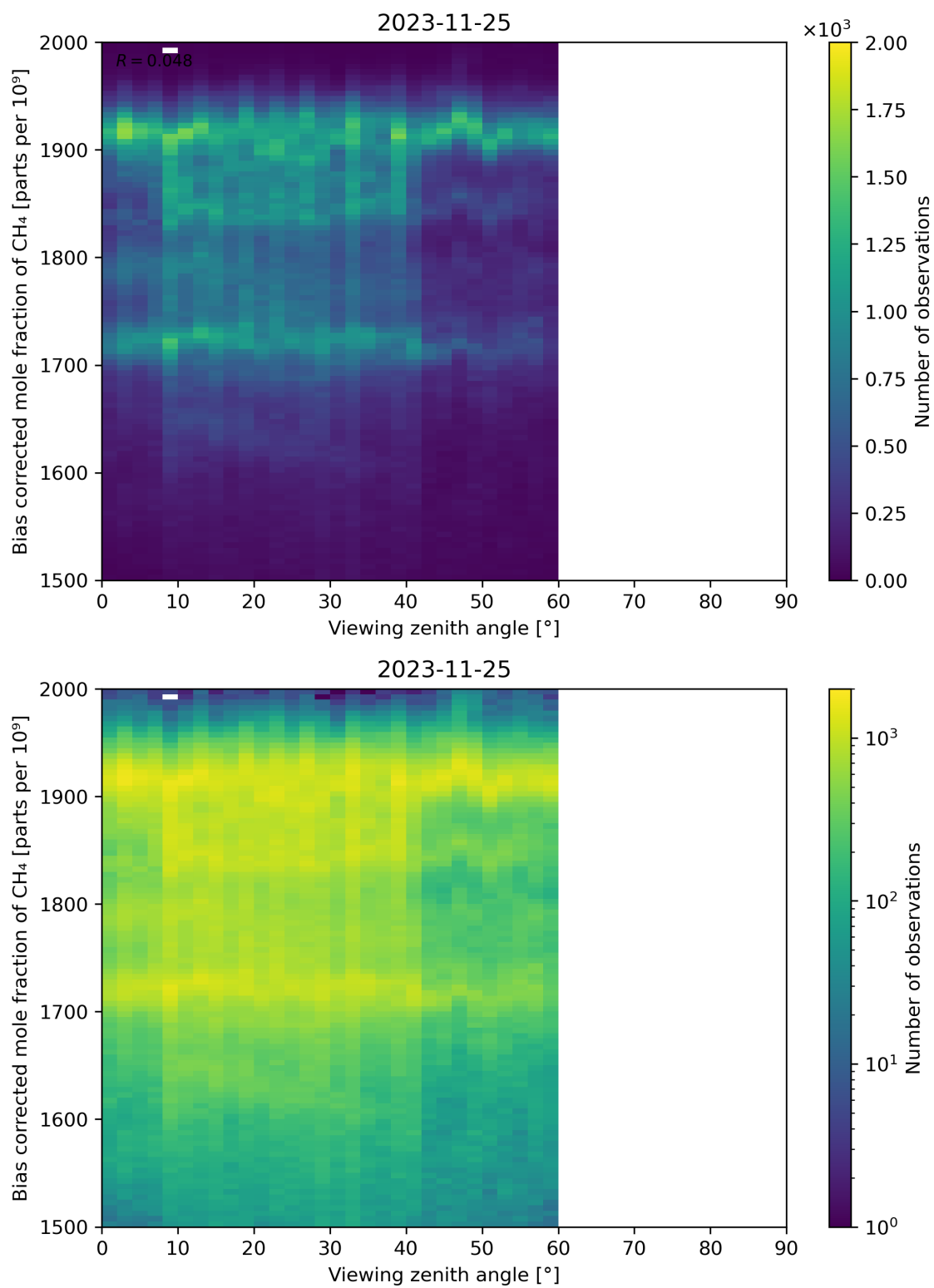
Figure 111: Scatter density plot of “Viewing zenith angle” against “Bias corrected mole fraction of CH 4 ” for 2023-11-24 to 2023-11-26.
