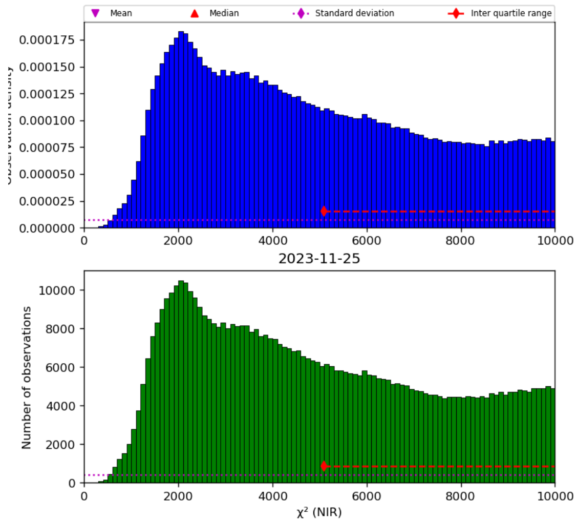
Figure 29: Histogram of “ \chi^2 (NIR)” for 2023-11-24 to 2023-11-26
