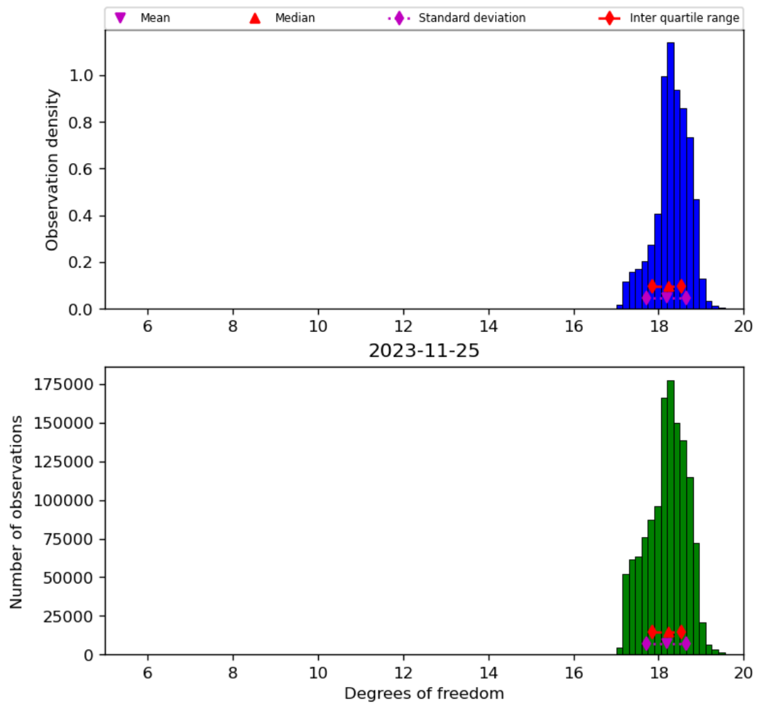
Figure 30: Histogram of “Degrees of freedom” for 2023-11-24 to 2023-11-26
