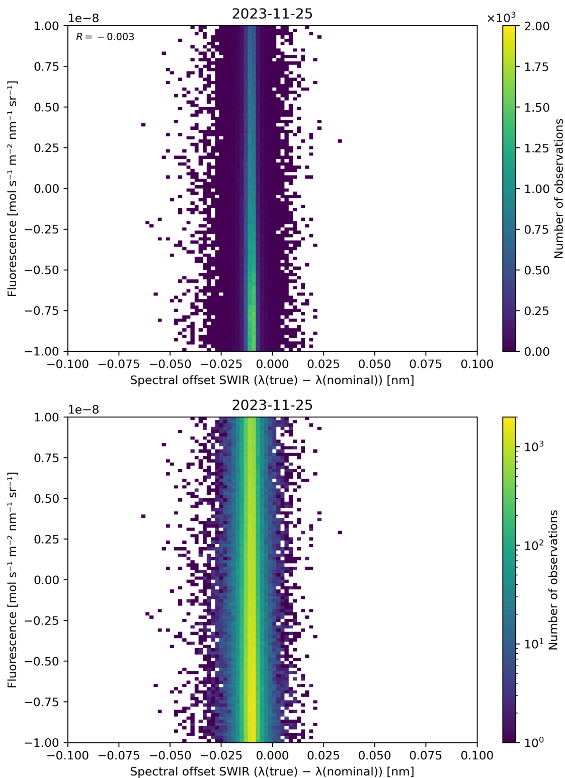
Figure 120: Scatter density plot of “Spectral offset SWIR ( \lambda(\text{true}) - \lambda(\text{nominal}) )” against “Fluorescence” for 2023-11-24 to 2023-11-26.
