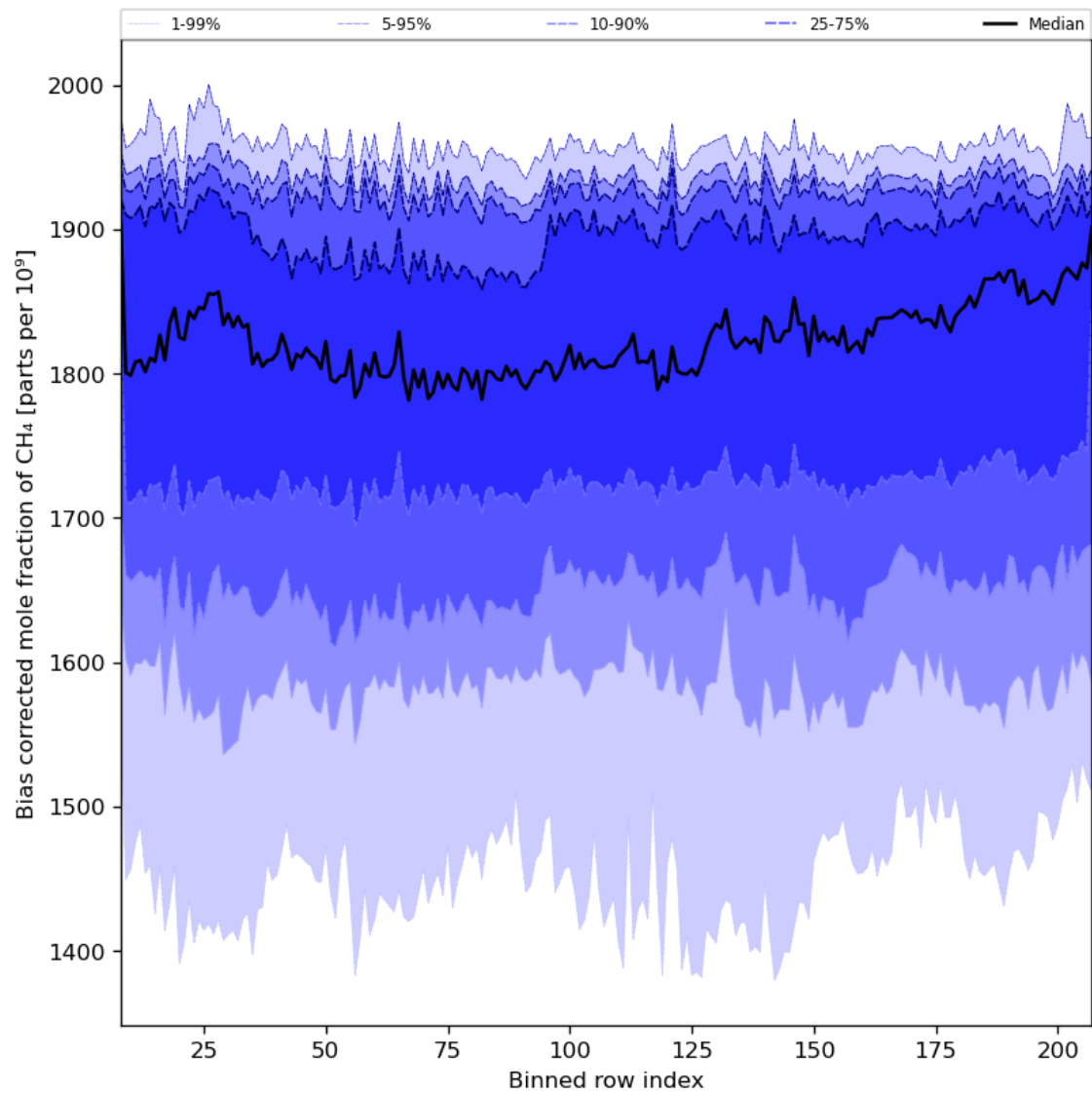
Figure 36: Along track statistics of “Bias corrected mole fraction of CH 4 ” for 2023-11-24 to 2023-11-26
