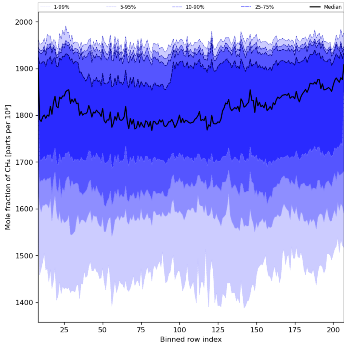
Figure 34: Along track statistics of “Mole fraction of CH 4 ” for 2023-11-24 to 2023-11-26
