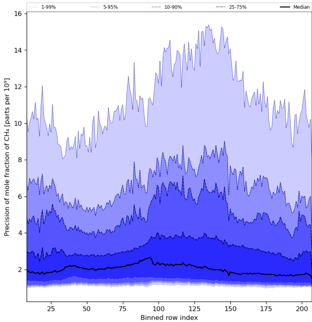
Figure 35: Along track statistics of “Precision of mole fraction of CH 4 ” for 2023-11-24 to 2023-11-26
