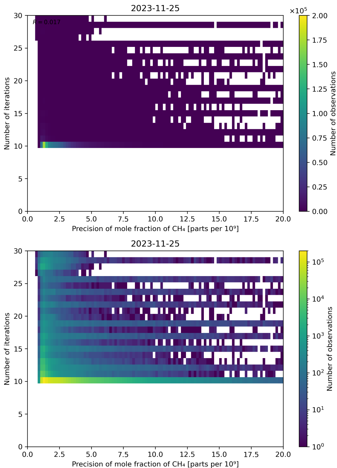
Figure 83: Scatter density plot of “Precision of mole fraction of CH 4 ” against “Number of iterations” for 2023-11-24 to 2023-11-26.
