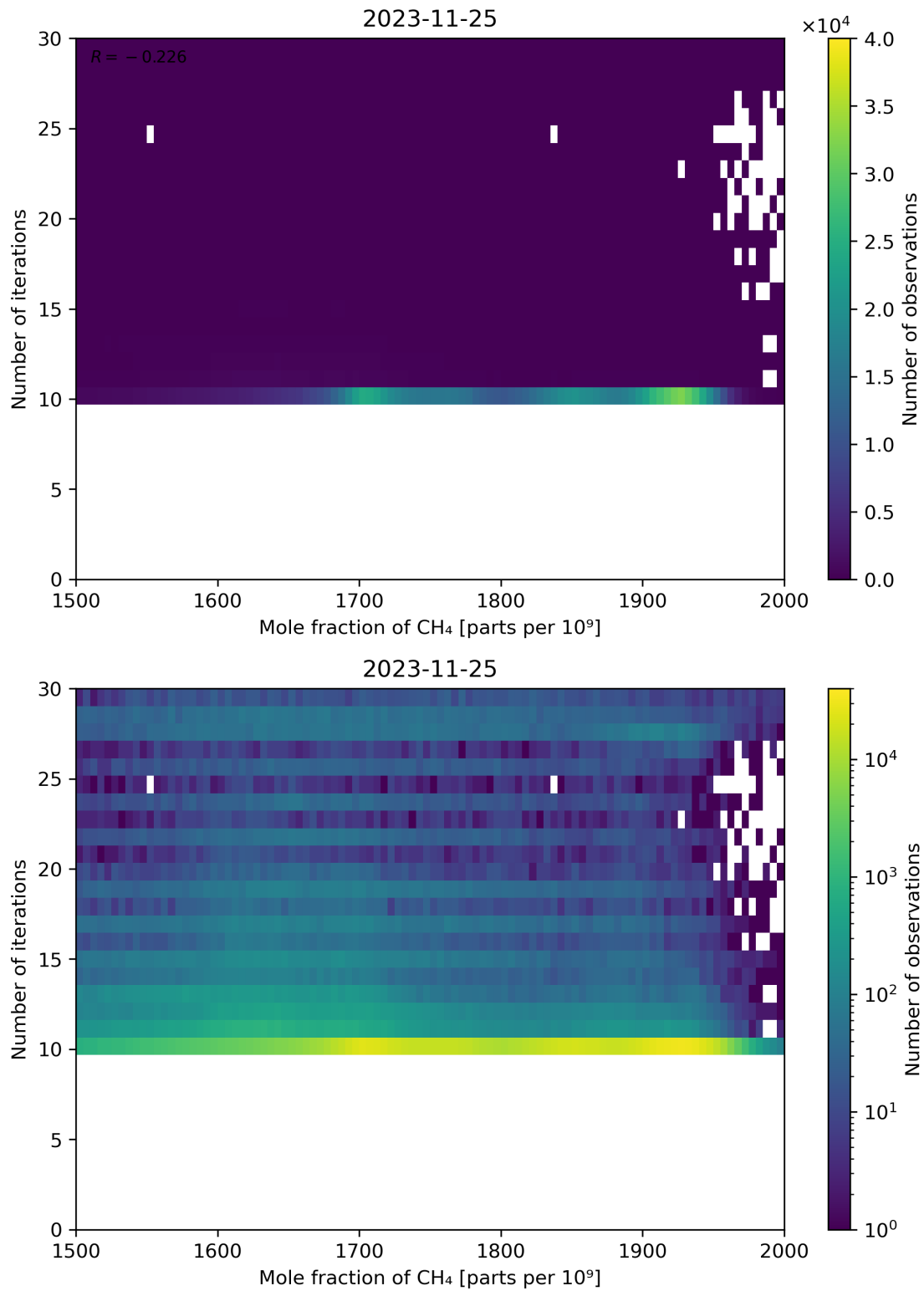
Figure 76: Scatter density plot of “Mole fraction of CH 4 ” against “Number of iterations” for 2023-11-24 to 2023-11-26.
