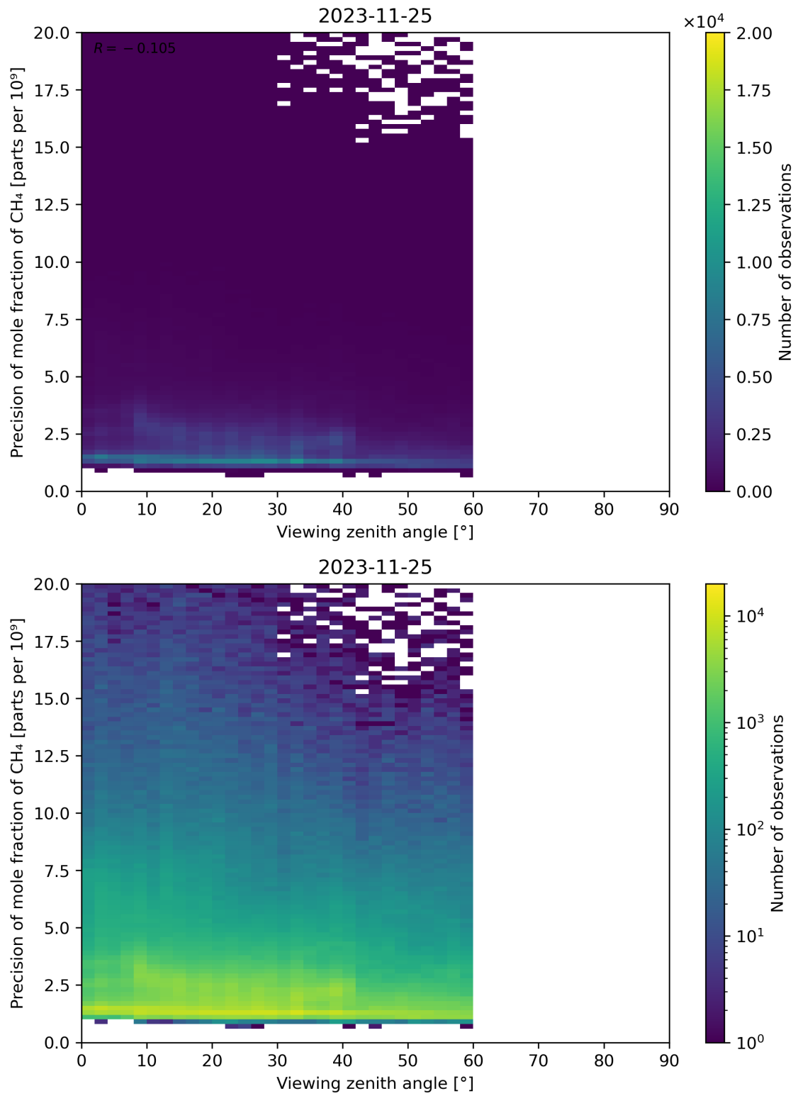
Figure 112: Scatter density plot of “Viewing zenith angle” against “Precision of mole fraction of CH 4 ” for 2023-11-24 to 2023-11-26.
