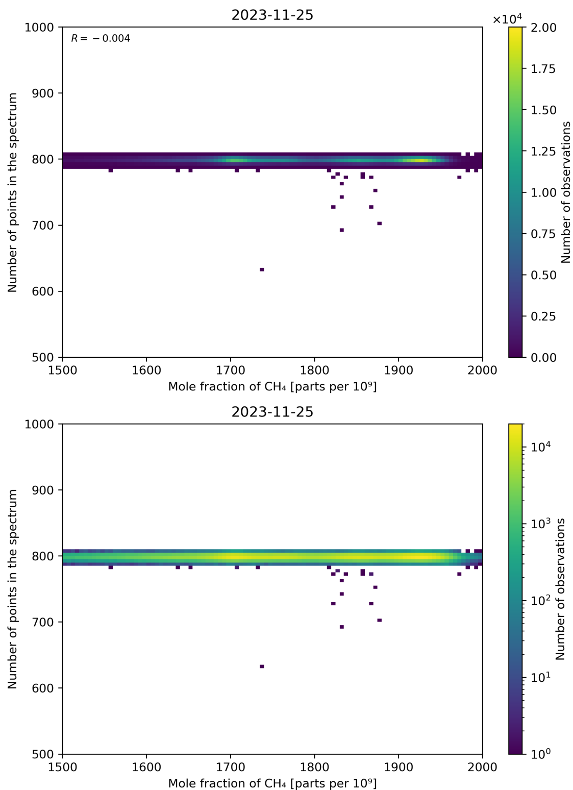
Figure 77: Scatter density plot of “Mole fraction of CH 4 ” against “Number of points in the spectrum” for 2023-11-24 to 2023-11-26.
