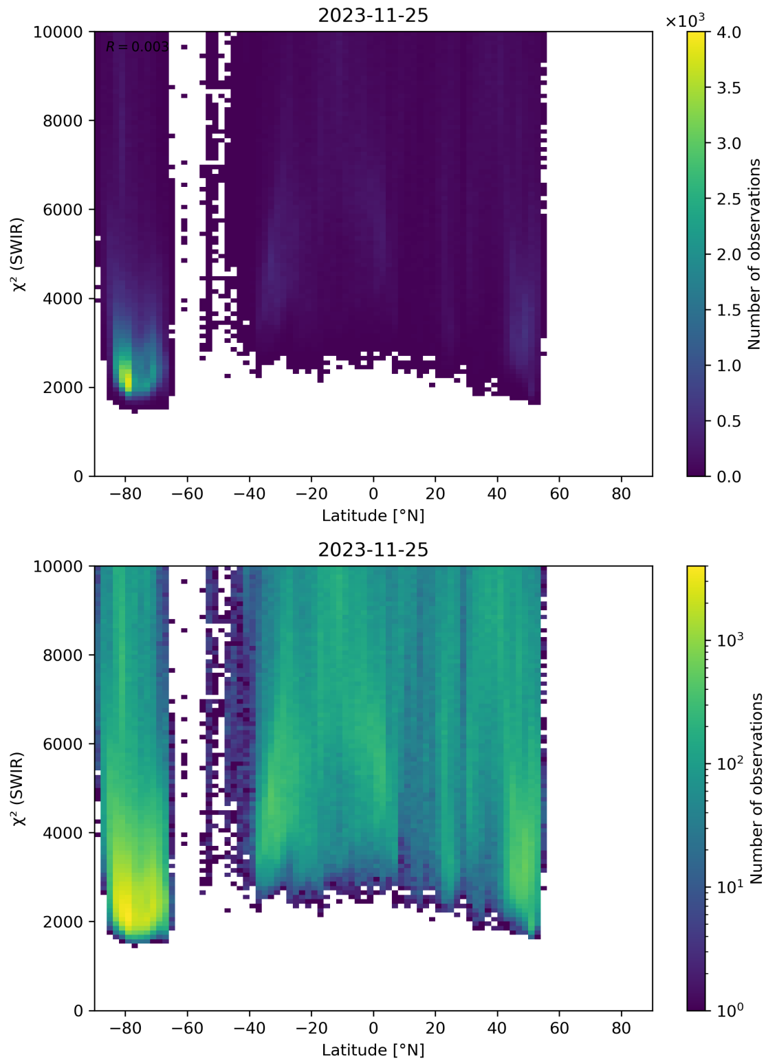
Figure 54: Scatter density plot of “Latitude” against “ \chi^2 (SWIR)” for 2023-11-24 to 2023-11-26.
