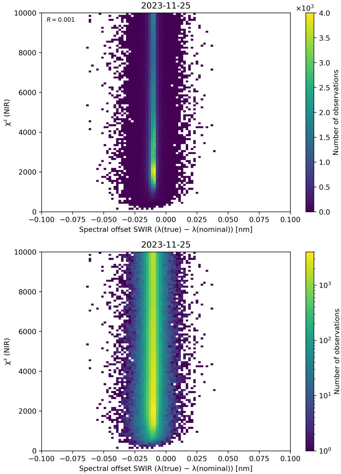
Figure 117: Scatter density plot of “Spectral offset SWIR ( \lambda(\text{true}) - \lambda(\text{nominal}) )” against “ \chi^2 (NIR)” for 2023-11-24 to 2023-11-26.
