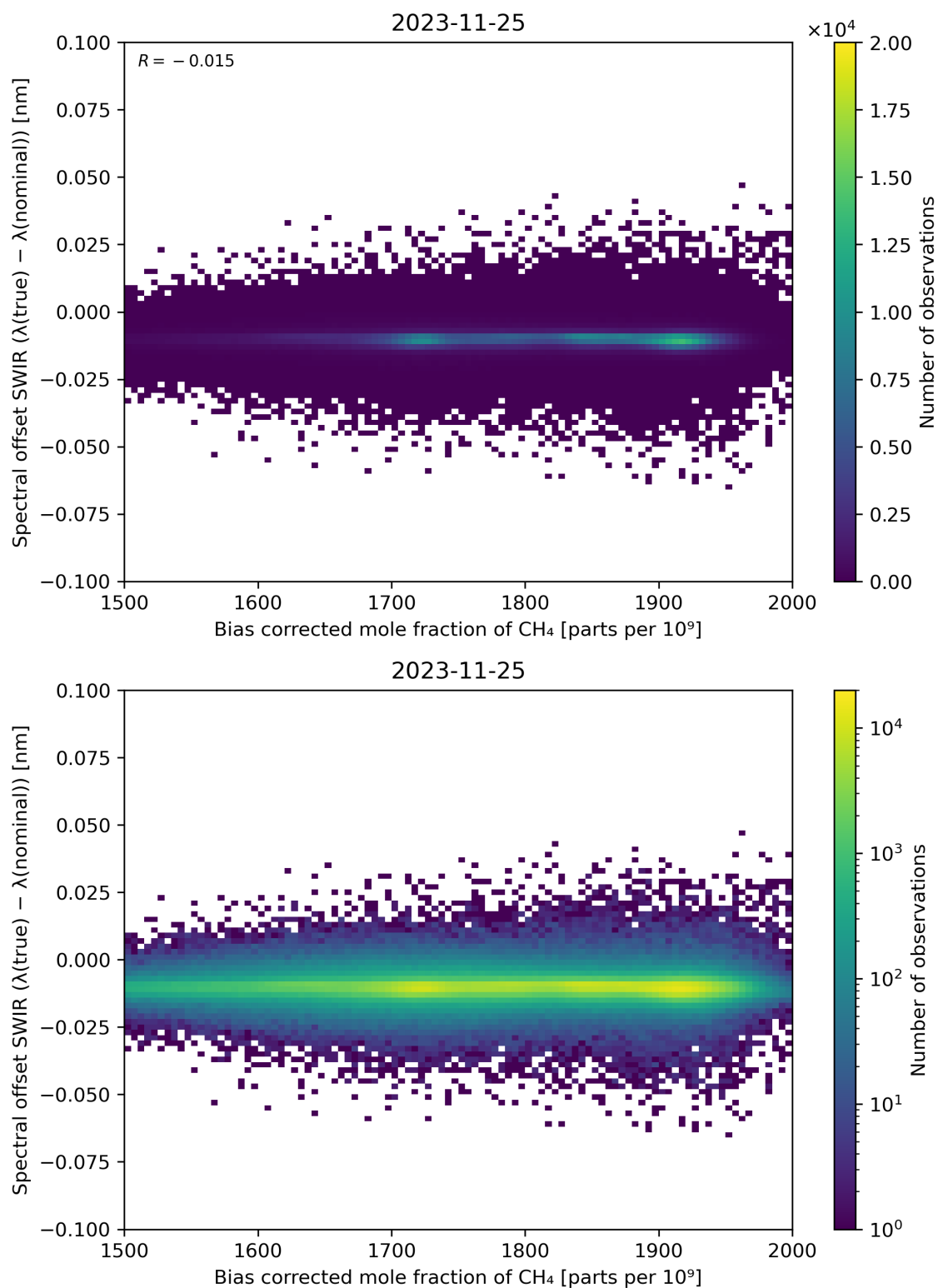
Figure 69: Scatter density plot of “Bias corrected mole fraction of \text{CH}_4 ” against “Spectral offset SWIR ( \lambda(\text{true}) - \lambda(\text{nominal}) )” for 2023-11-24 to 2023-11-26.
