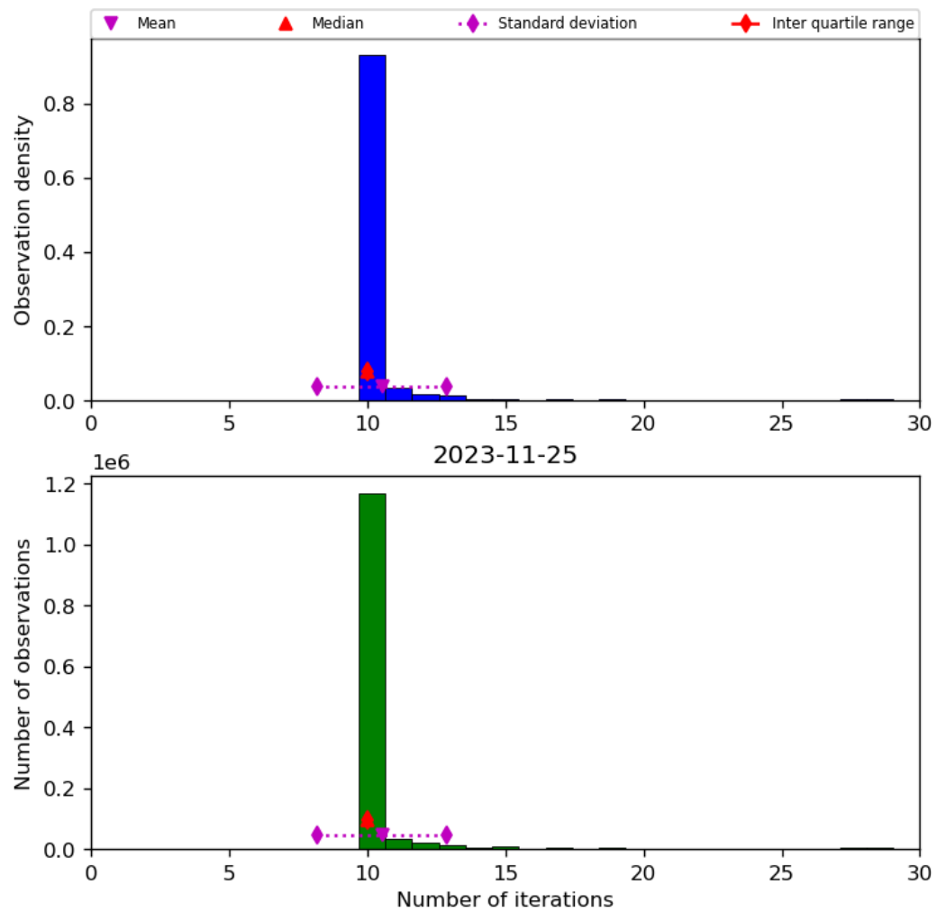
Figure 31: Histogram of “Number of iterations” for 2023-11-24 to 2023-11-26
