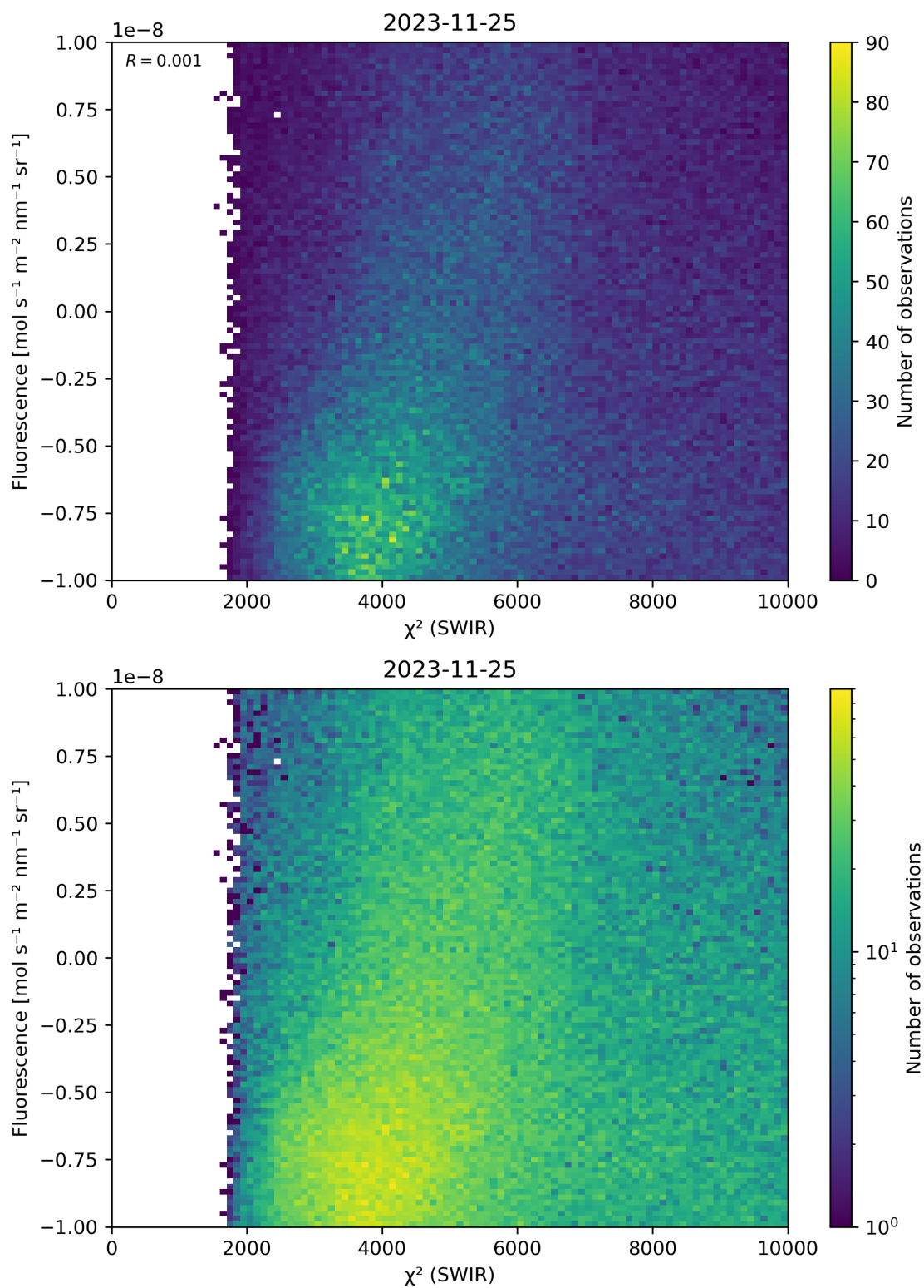
Figure 49: Scatter density plot of “ \chi^2 (SWIR)” against “Fluorescence” for 2023-11-24 to 2023-11-26.
