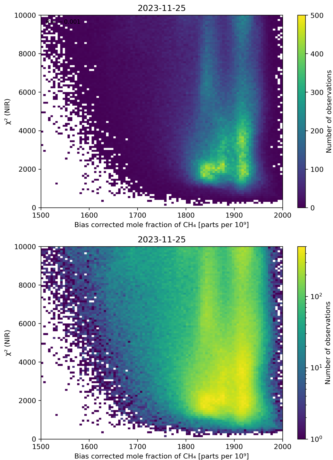
Figure 63: Scatter density plot of “Bias corrected mole fraction of CH 4 ” against “ \chi^2 (NIR)” for 2023-11-24 to 2023-11-26.
