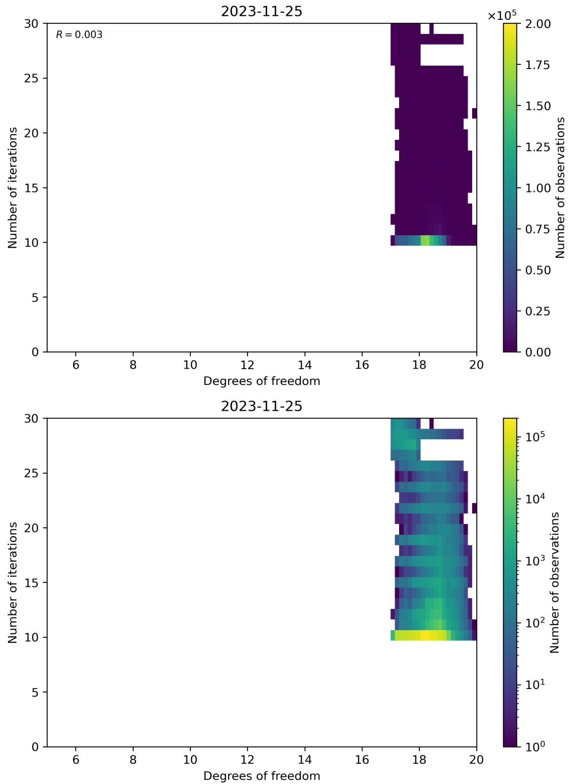
Figure 52: Scatter density plot of “Degrees of freedom” against “Number of iterations” for 2023-11-24 to 2023-11-26.
