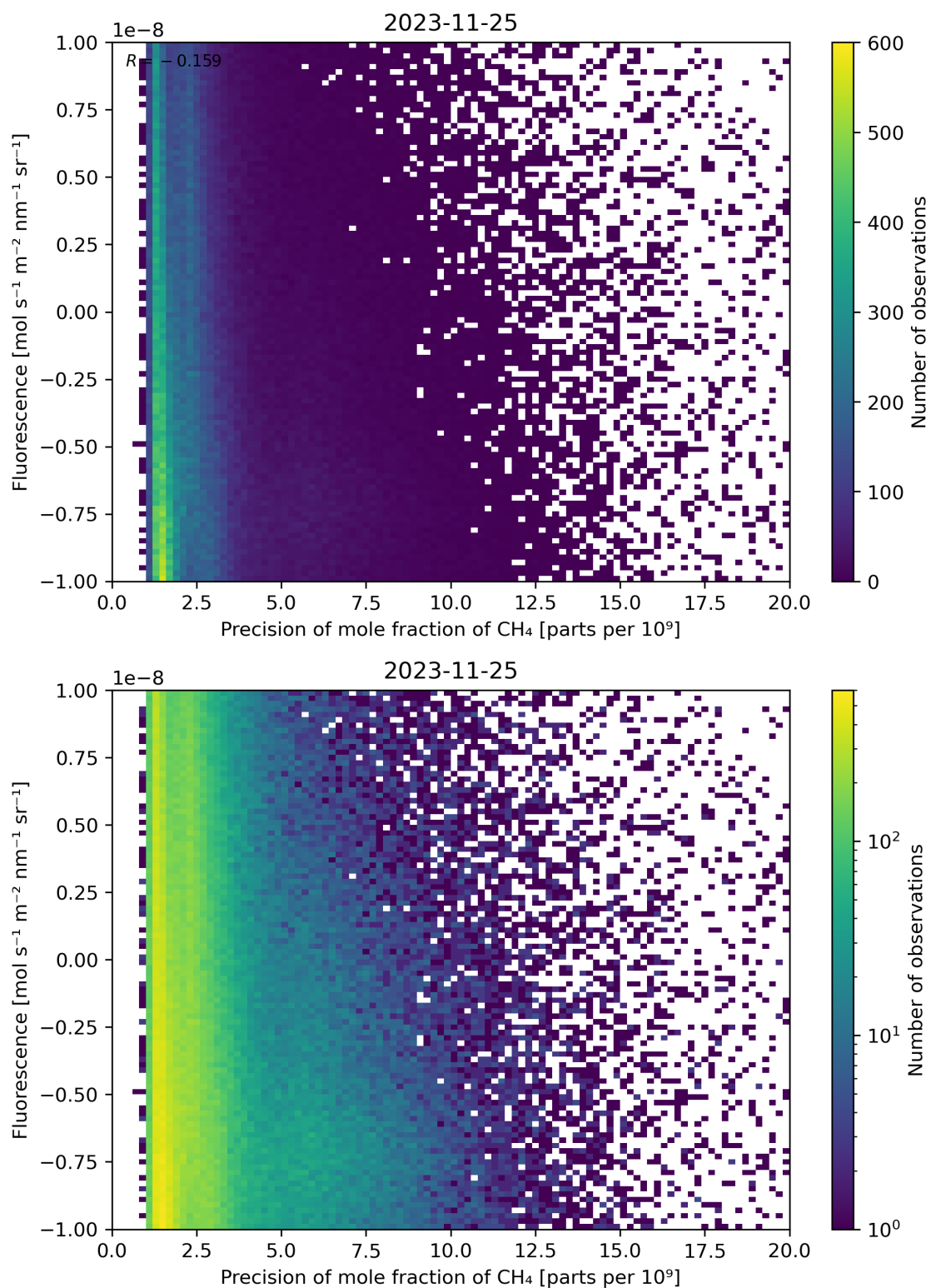
Figure 81: Scatter density plot of “Precision of mole fraction of \text{CH}_4 ” against “Fluorescence” for 2023-11-24 to 2023-11-26.
