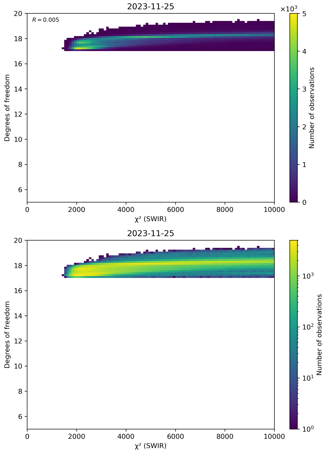
Figure 48: Scatter density plot of “ \chi^2 (SWIR)” against “Degrees of freedom” for 2023-11-24 to 2023-11-26.
