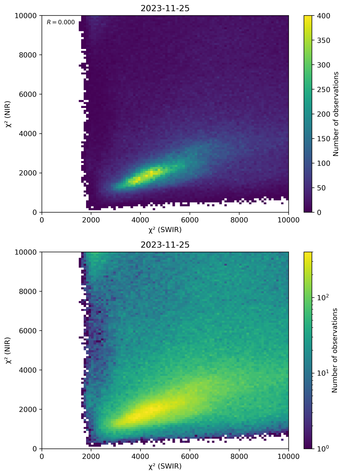
Figure 47: Scatter density plot of “ \chi^2 (SWIR)” against “ \chi^2 (NIR)” for 2023-11-24 to 2023-11-26.
