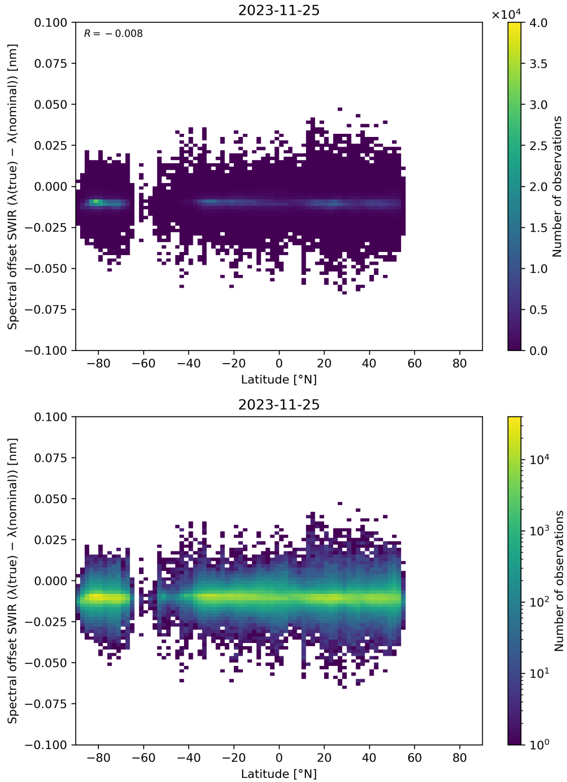
Figure 62: Scatter density plot of “Latitude” against “Spectral offset SWIR ( \lambda(\text{true}) - \lambda(\text{nominal}) )” for 2023-11-24 to 2023-11-26.
