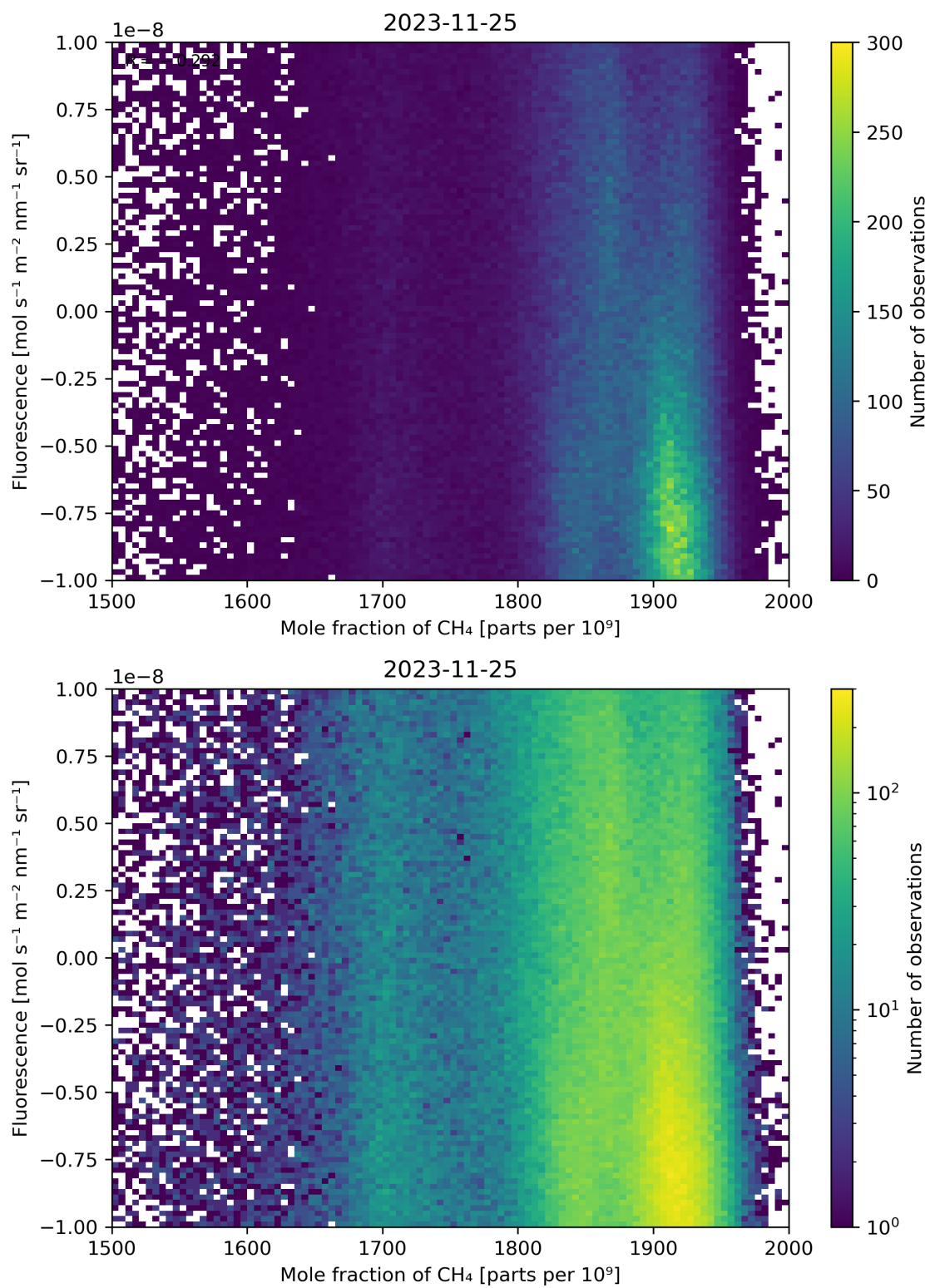
Figure 73: Scatter density plot of “Mole fraction of \text{CH}_4 ” against “Fluorescence” for 2023-11-24 to 2023-11-26.
