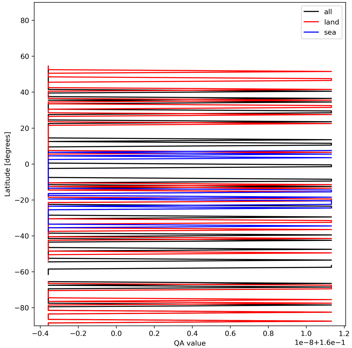
Figure 11: Zonal average of “QA value” for 2023-11-24 to 2023-11-26.
