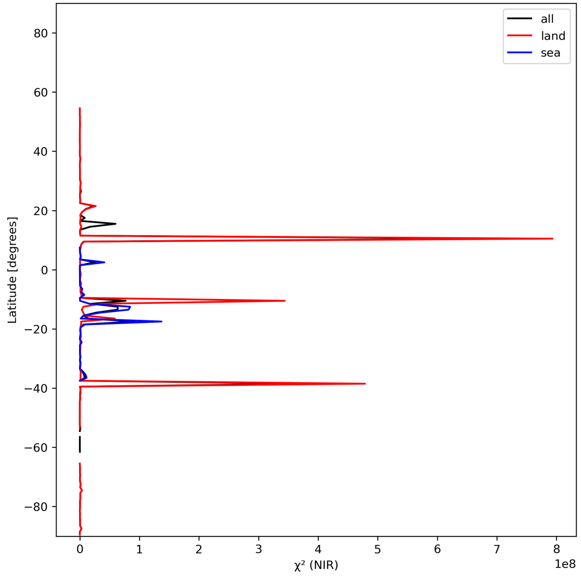
Figure 18: Zonal average of “ \chi^2 (NIR)” for 2023-11-24 to 2023-11-26.
