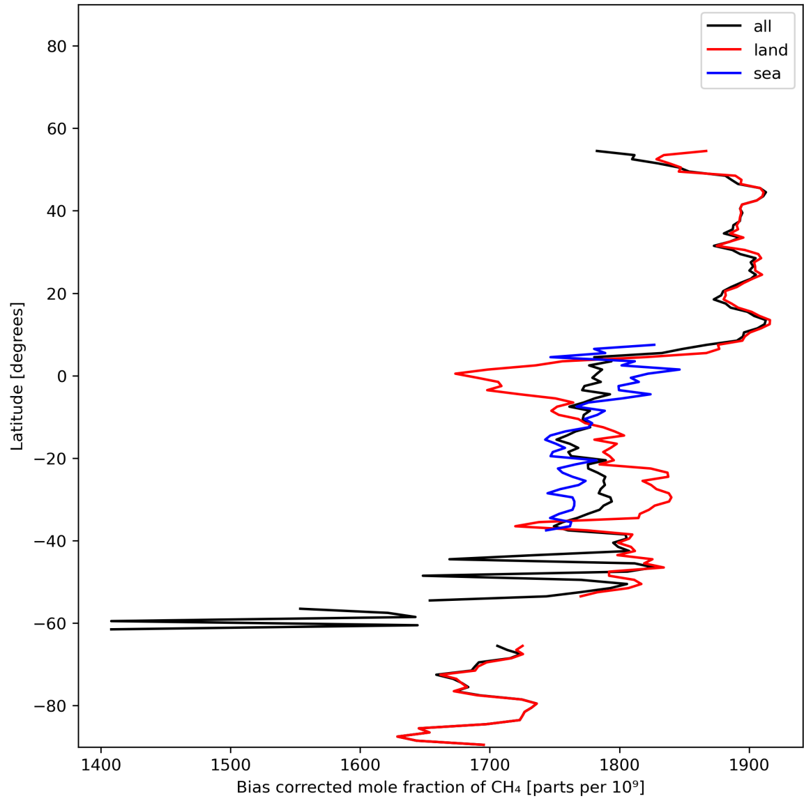
Figure 14: Zonal average of “Bias corrected mole fraction of CH 4 ” for 2023-11-24 to 2023-11-26.
