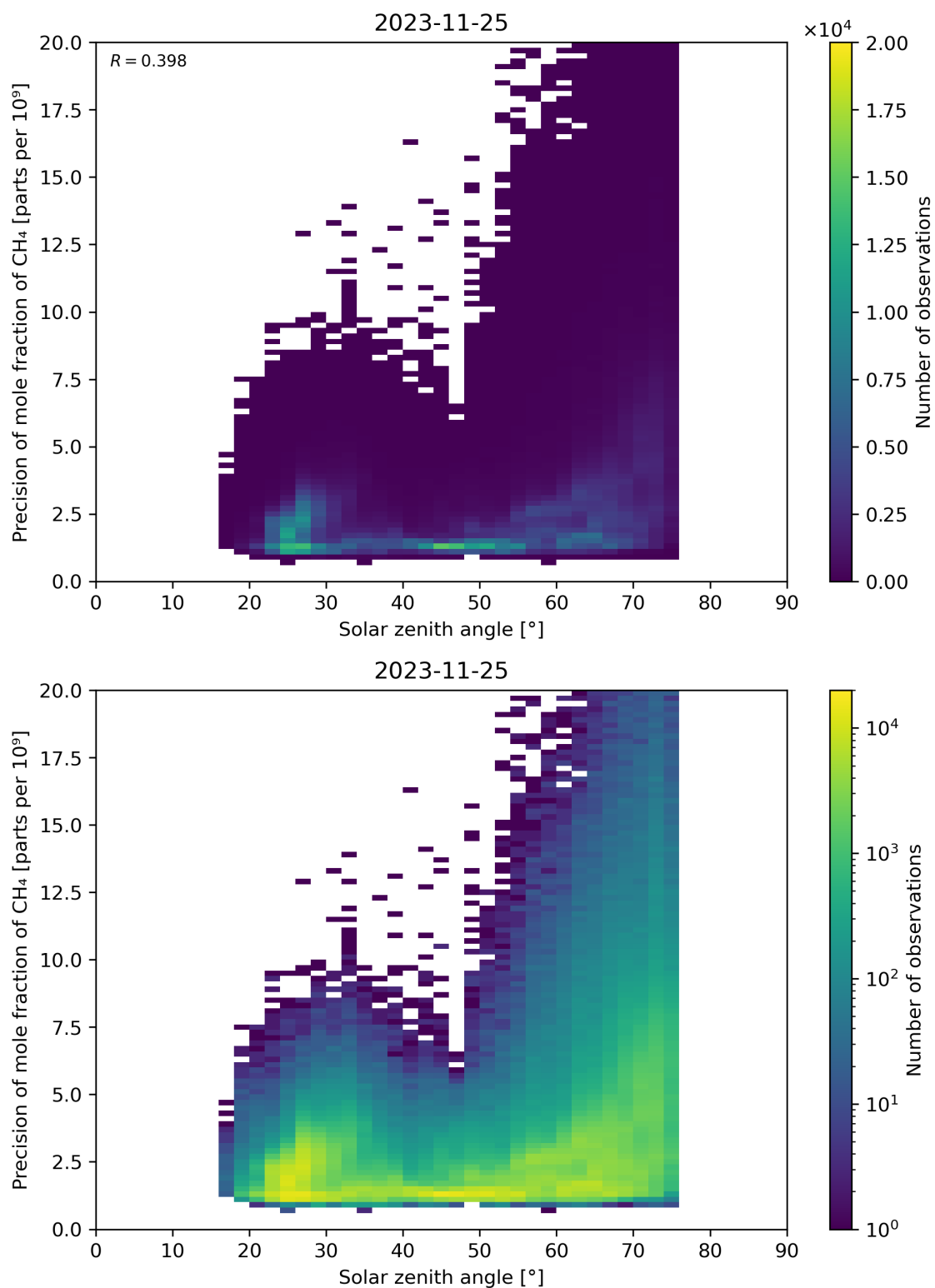
Figure 101: Scatter density plot of “Solar zenith angle” against “Precision of mole fraction of CH 4 ” for 2023-11-24 to 2023-11-26.
