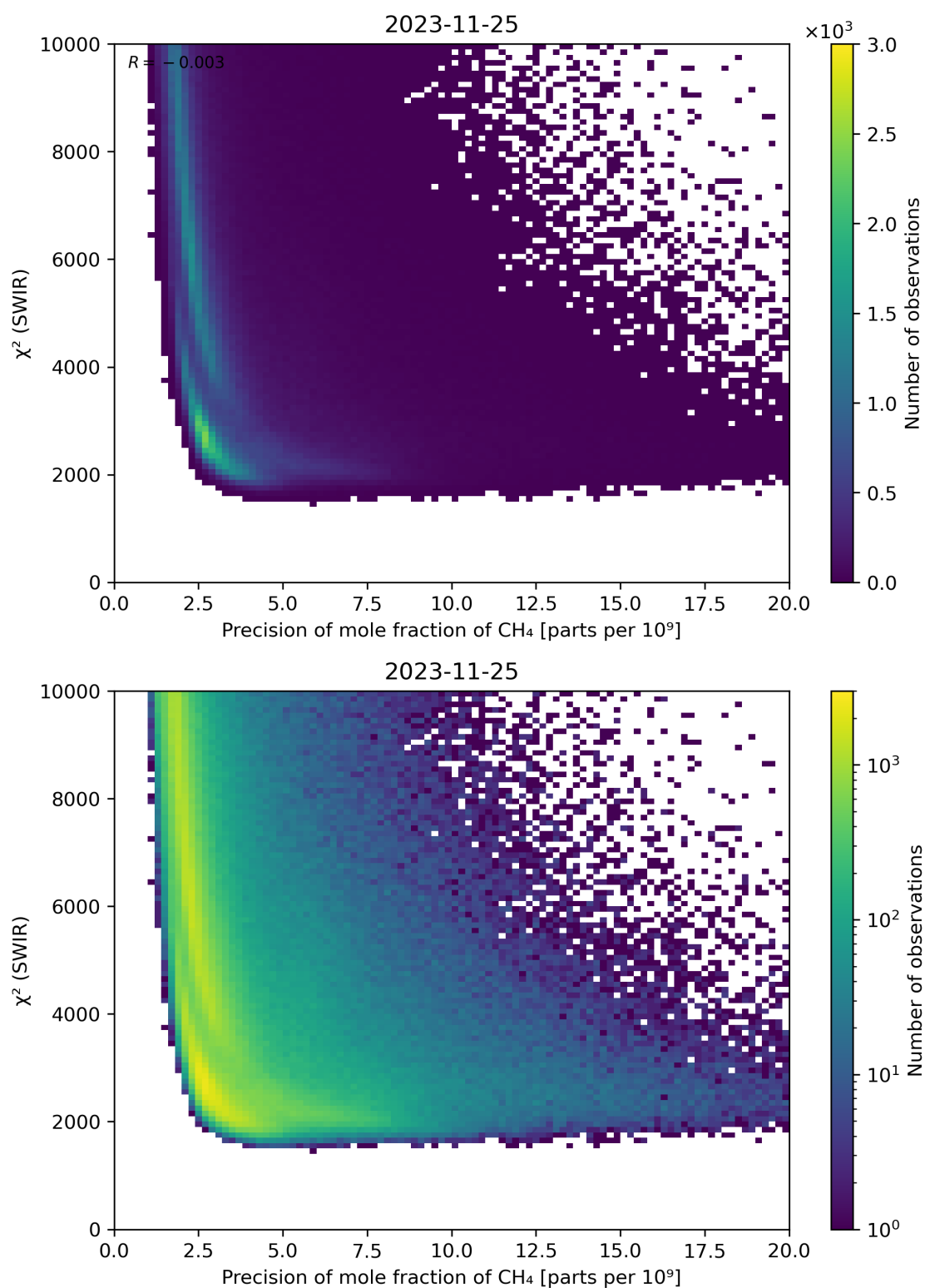
Figure 79: Scatter density plot of “Precision of mole fraction of CH 4 ” against “ \chi^2 (SWIR)” for 2023-11-24 to 2023-11-26.
