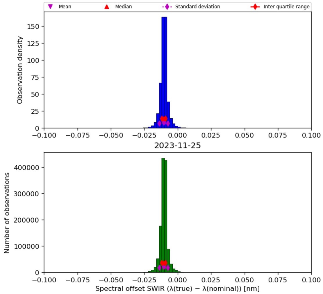
Figure 27: Histogram of “Spectral offset SWIR ( \lambda(\text{true}) - \lambda(\text{nominal}) )” for 2023-11-24 to 2023-11-26
