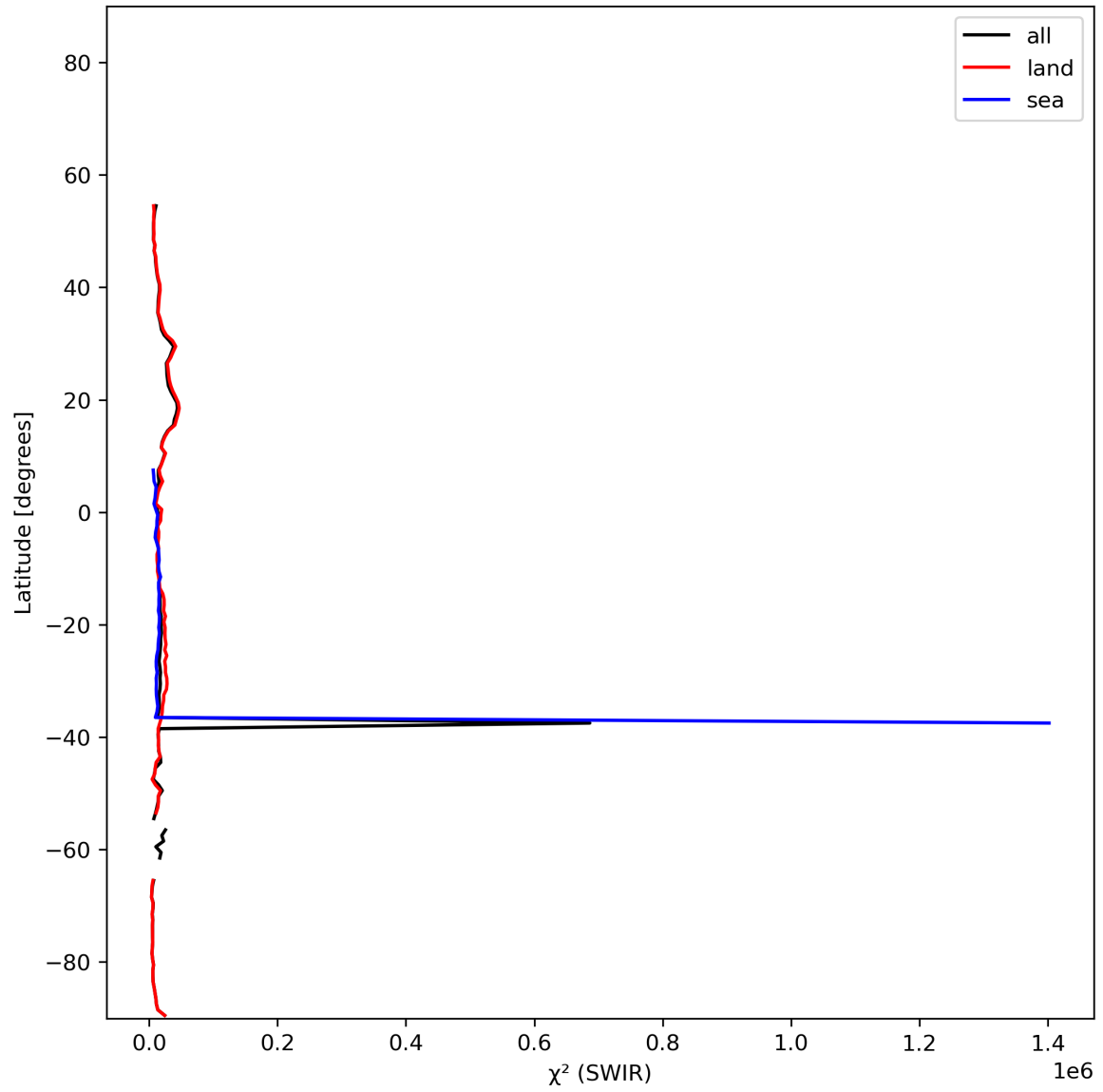
Figure 17: Zonal average of “ \chi^2 (SWIR)” for 2023-11-24 to 2023-11-26.
