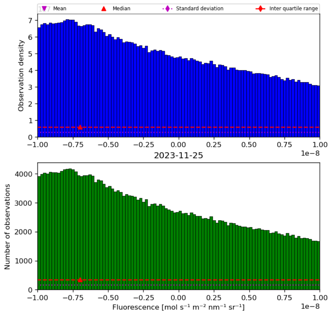
Figure 32: Histogram of “Fluorescence” for 2023-11-24 to 2023-11-26
