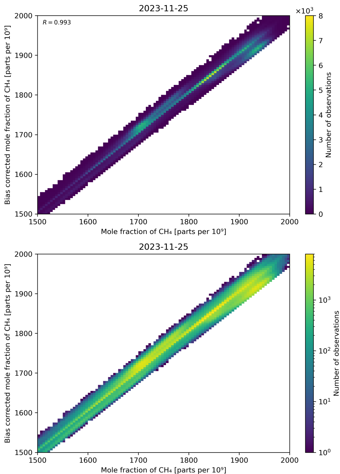
Figure 74: Scatter density plot of “Mole fraction of CH 4 ” against “Bias corrected mole fraction of CH 4 ” for 2023-11-24 to 2023-11-26.
