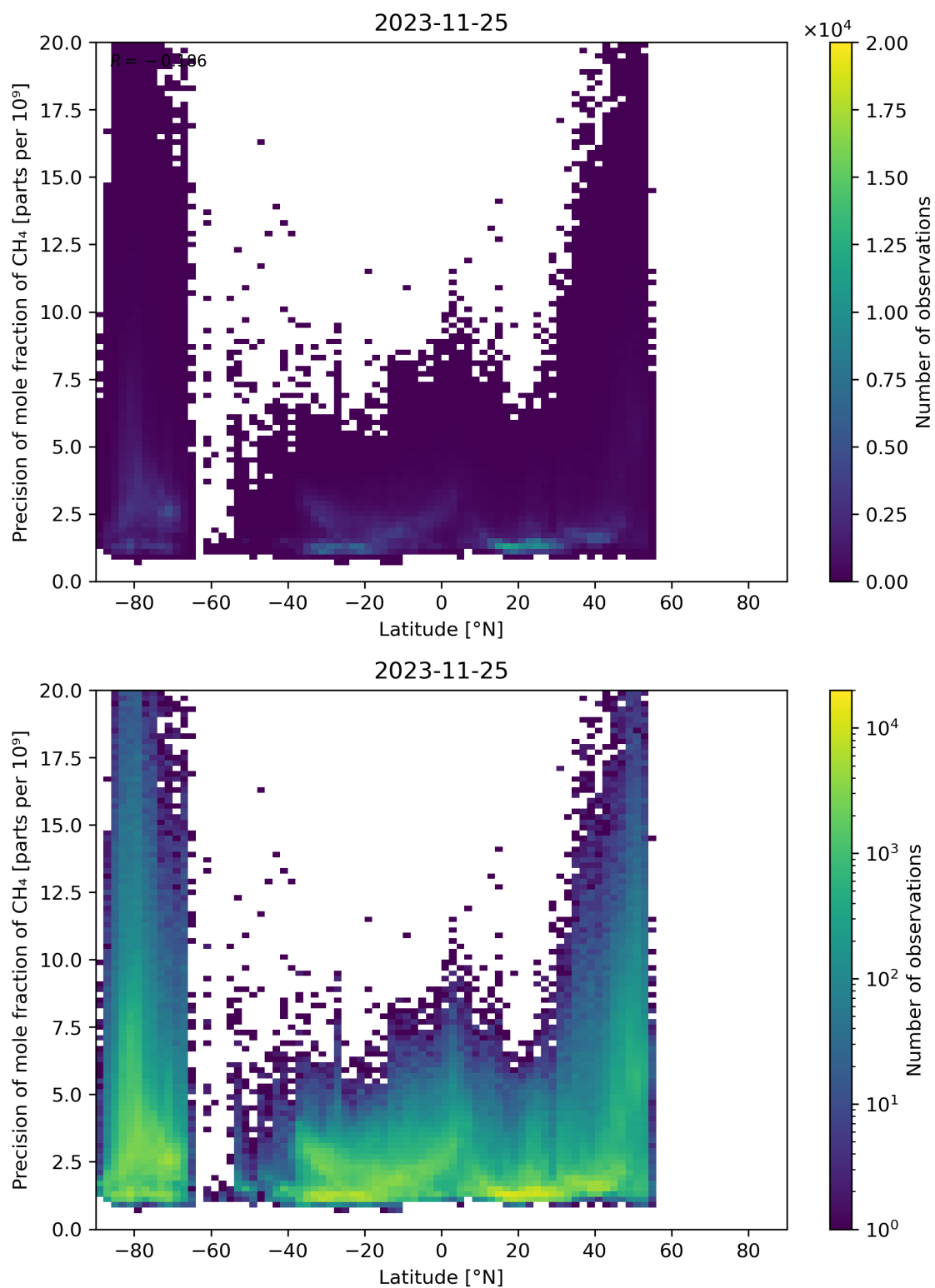
Figure 59: Scatter density plot of “Latitude” against “Precision of mole fraction of \text{CH}_4 ” for 2023-11-24 to 2023-11-26.
