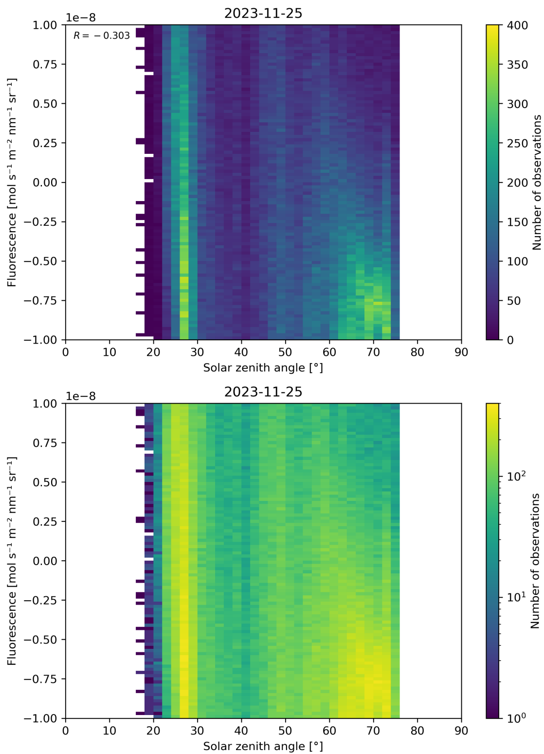
Figure 97: Scatter density plot of “Solar zenith angle” against “Fluorescence” for 2023-11-24 to 2023-11-26.
