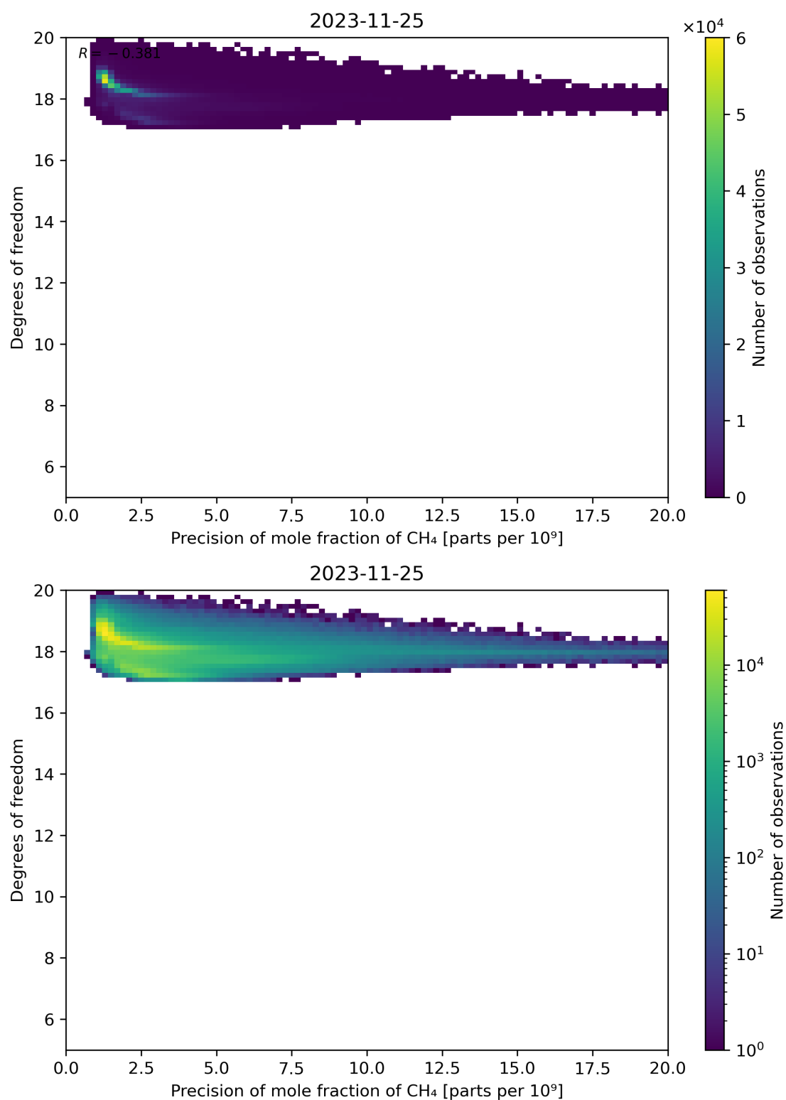
Figure 80: Scatter density plot of “Precision of mole fraction of CH 4 ” against “Degrees of freedom” for 2023-11-24 to 2023-11-26.
