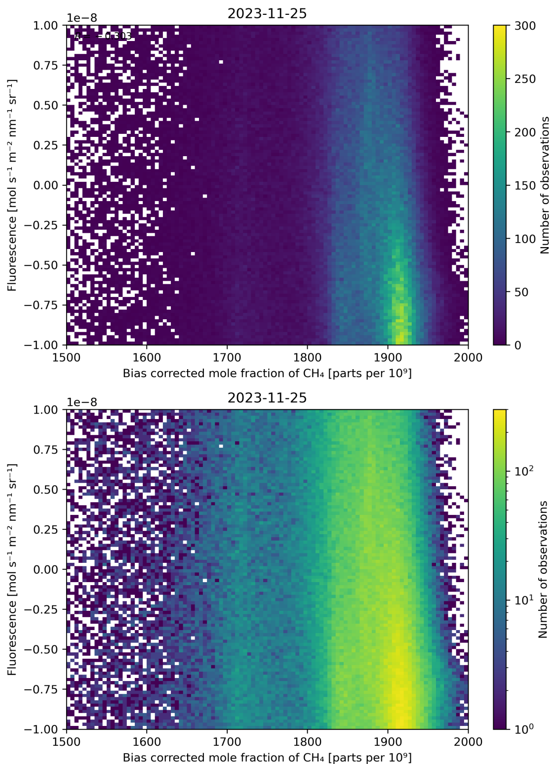
Figure 66: Scatter density plot of “Bias corrected mole fraction of \text{CH}_4 ” against “Fluorescence” for 2023-11-24 to 2023-11-26.
