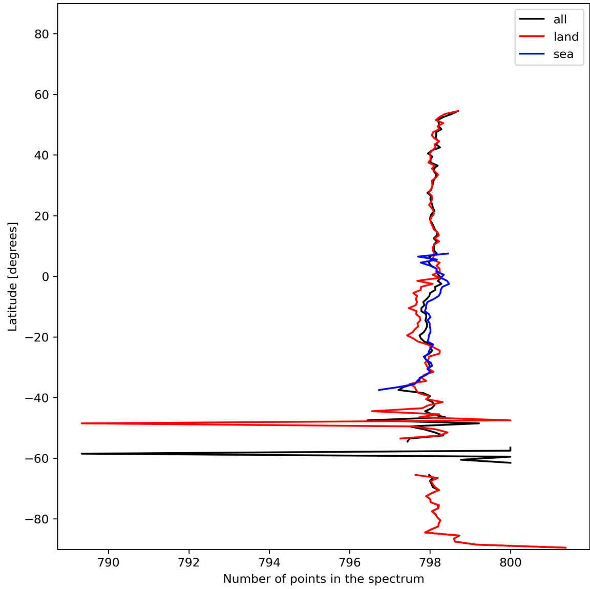
Figure 15: Zonal average of “Number of points in the spectrum” for 2023-11-24 to 2023-11-26.
