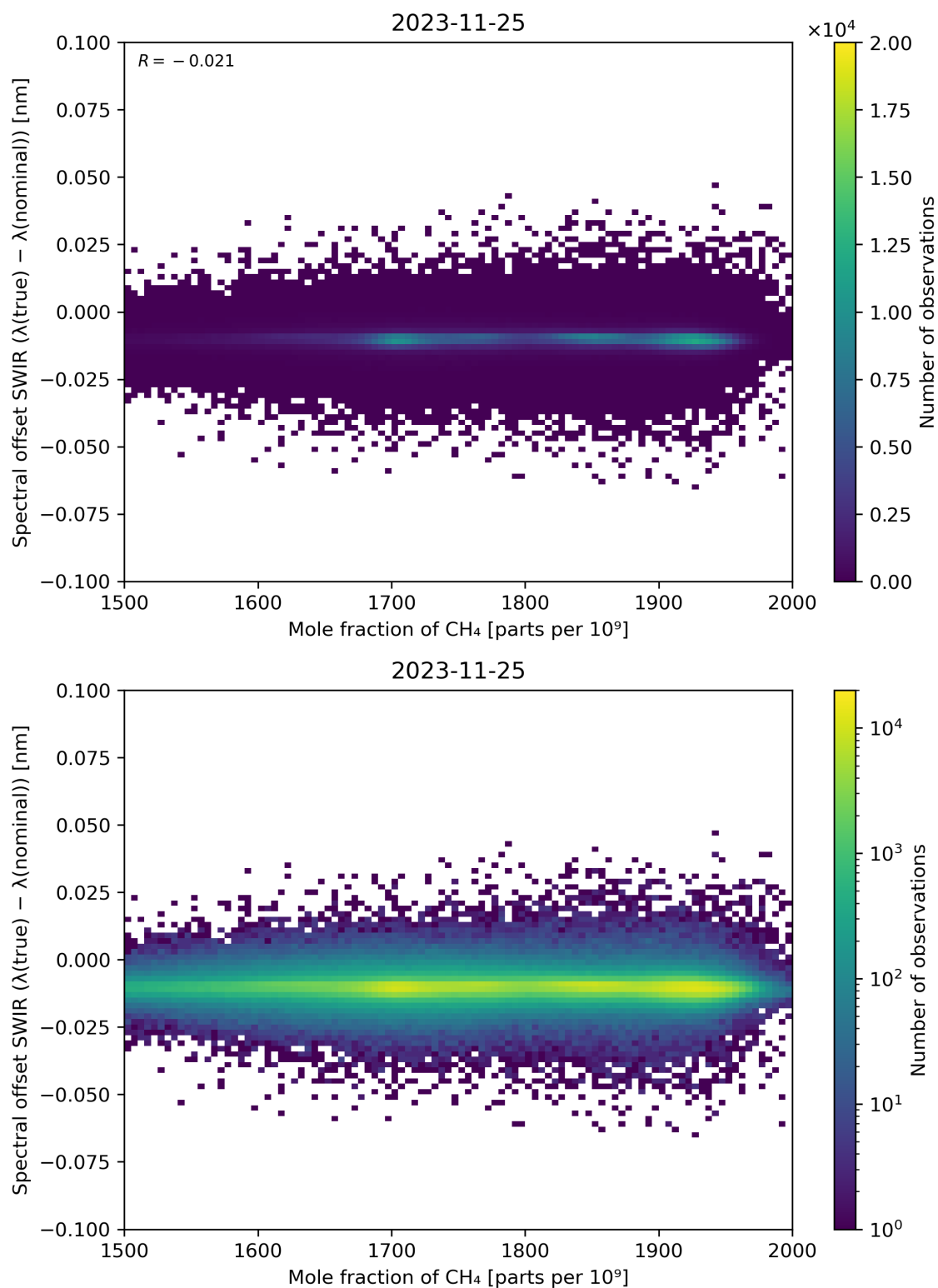
Figure 86: Scatter density plot of “Mole fraction of CH 4 ” against “Spectral offset SWIR ( \lambda(\text{true}) - \lambda(\text{nominal}) )” for 2023-11-24 to 2023-11-26.
