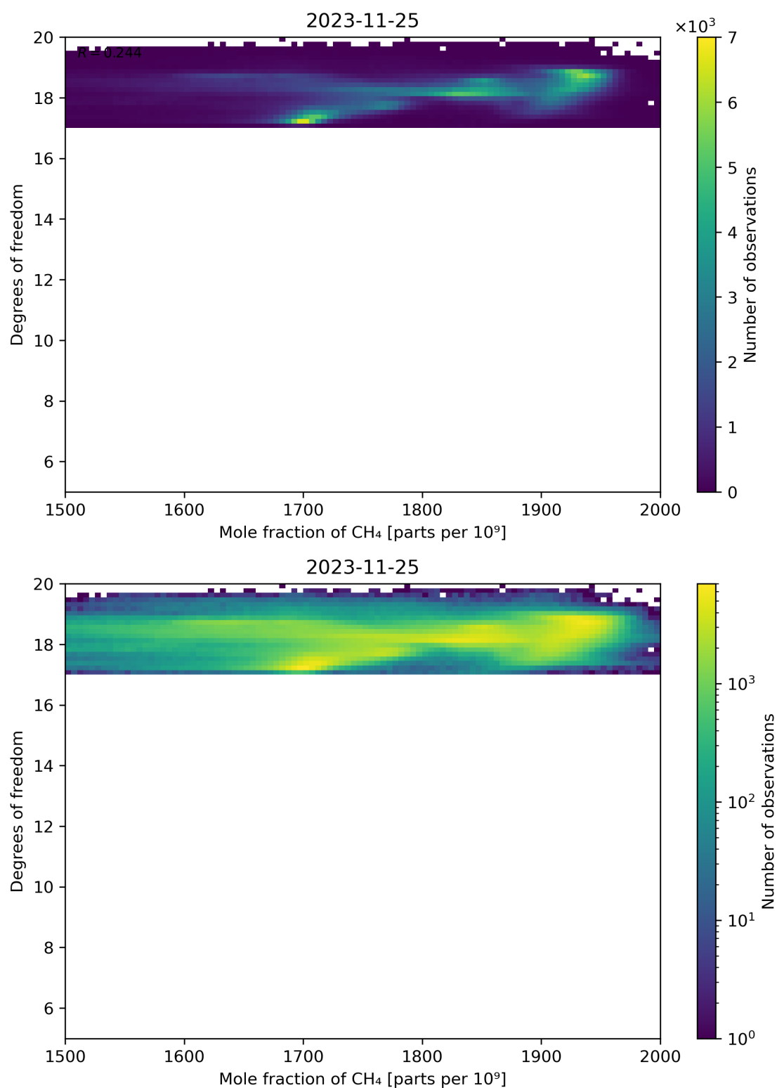
Figure 72: Scatter density plot of “Mole fraction of CH 4 ” against “Degrees of freedom” for 2023-11-24 to 2023-11-26.
