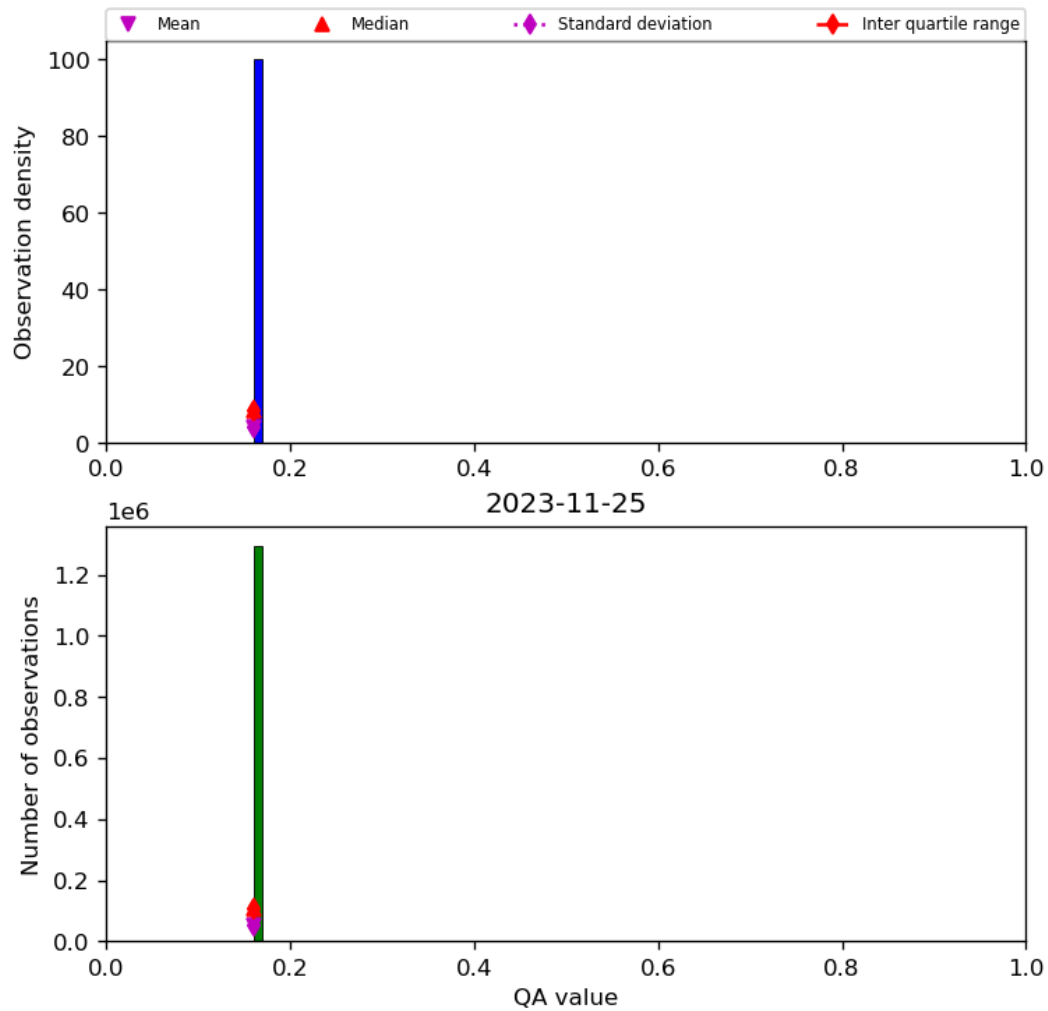
Figure 22: Histogram of “QA value” for 2023-11-24 to 2023-11-26
