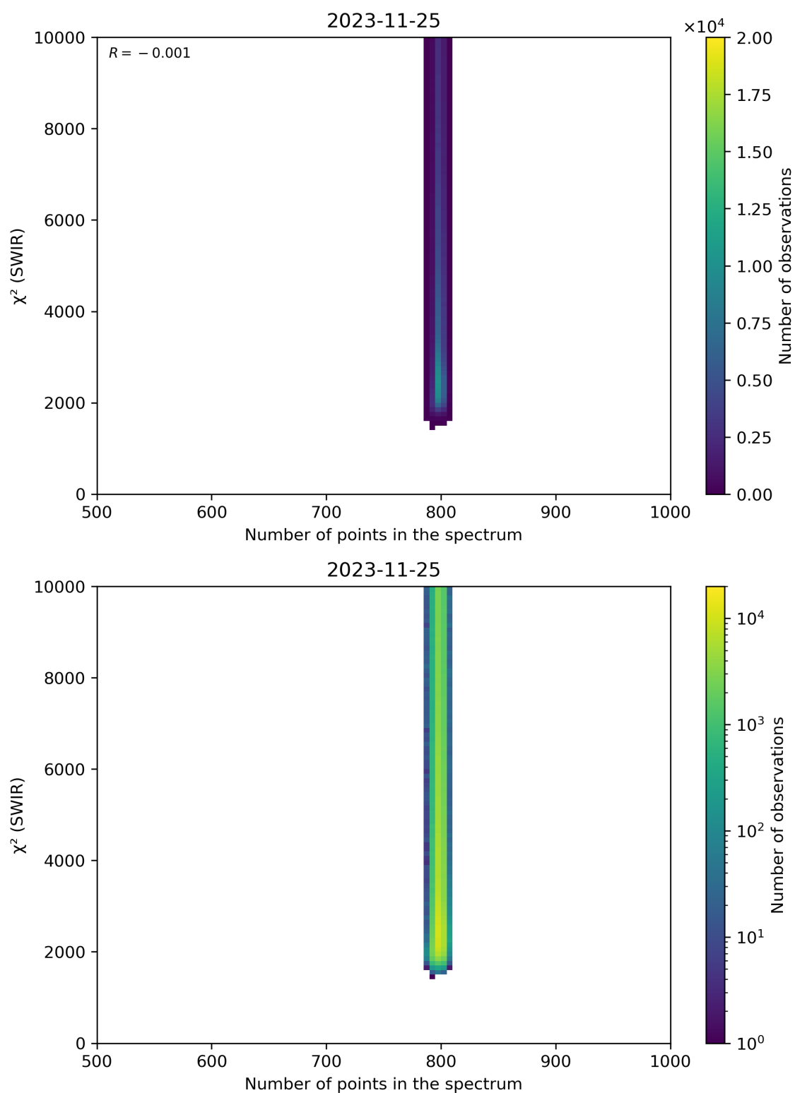
Figure 89: Scatter density plot of “Number of points in the spectrum” against “ \chi^2 (SWIR)” for 2023-11-24 to 2023-11-26.
