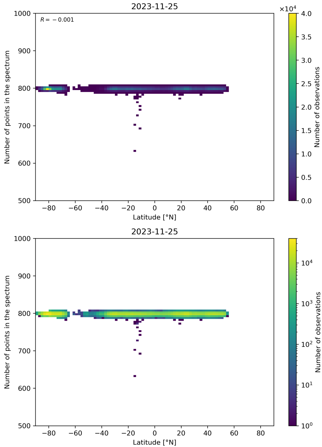
Figure 61: Scatter density plot of “Latitude” against “Number of points in the spectrum” for 2023-11-24 to 2023-11-26.
