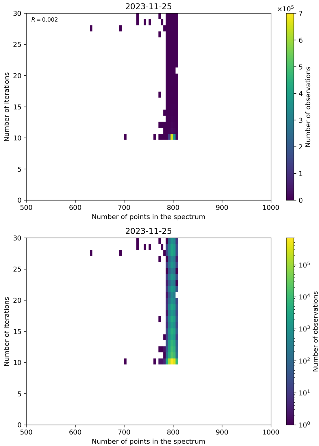
Figure 92: Scatter density plot of “Number of points in the spectrum” against “Number of iterations” for 2023-11-24 to 2023-11-26.
