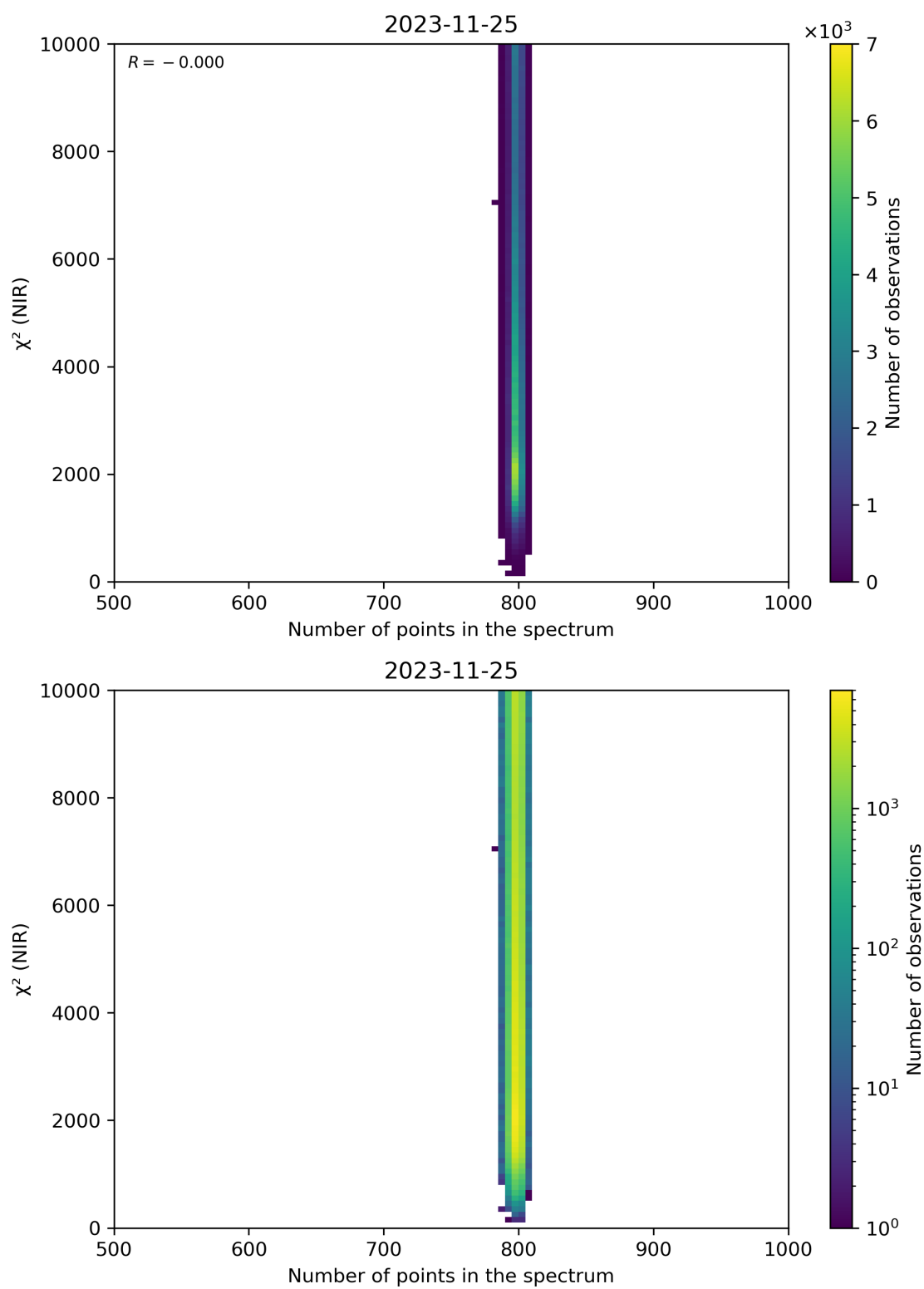
Figure 88: Scatter density plot of “Number of points in the spectrum” against “ \chi^2 (NIR)” for 2023-11-24 to 2023-11-26.
