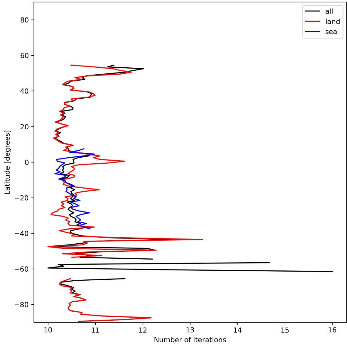
Figure 20: Zonal average of “Number of iterations” for 2023-11-24 to 2023-11-26.
