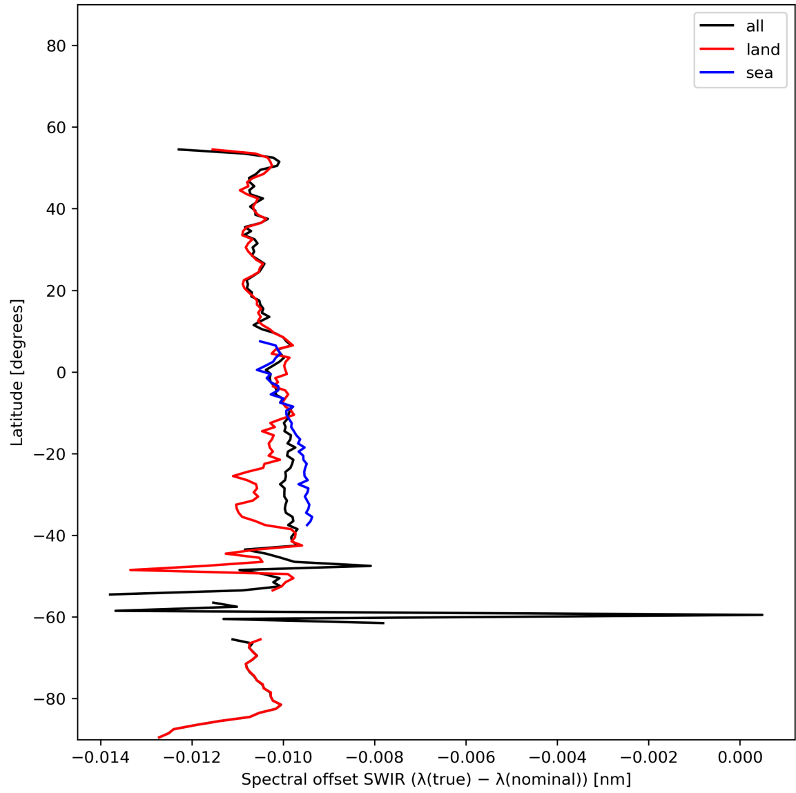
Figure 16: Zonal average of “Spectral offset SWIR ( \lambda(\text{true}) - \lambda(\text{nominal}) )” for 2023-11-24 to 2023-11-26.
