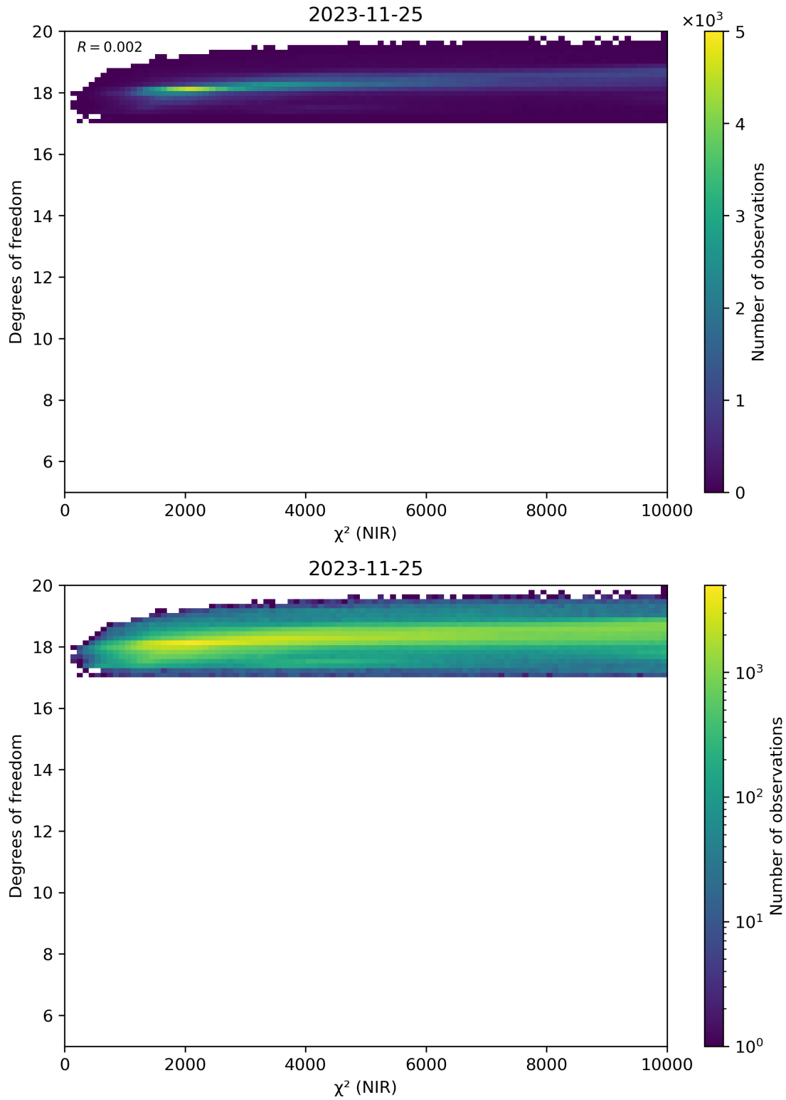
Figure 44: Scatter density plot of “ \chi^2 (NIR)” against “Degrees of freedom” for 2023-11-24 to 2023-11-26.
