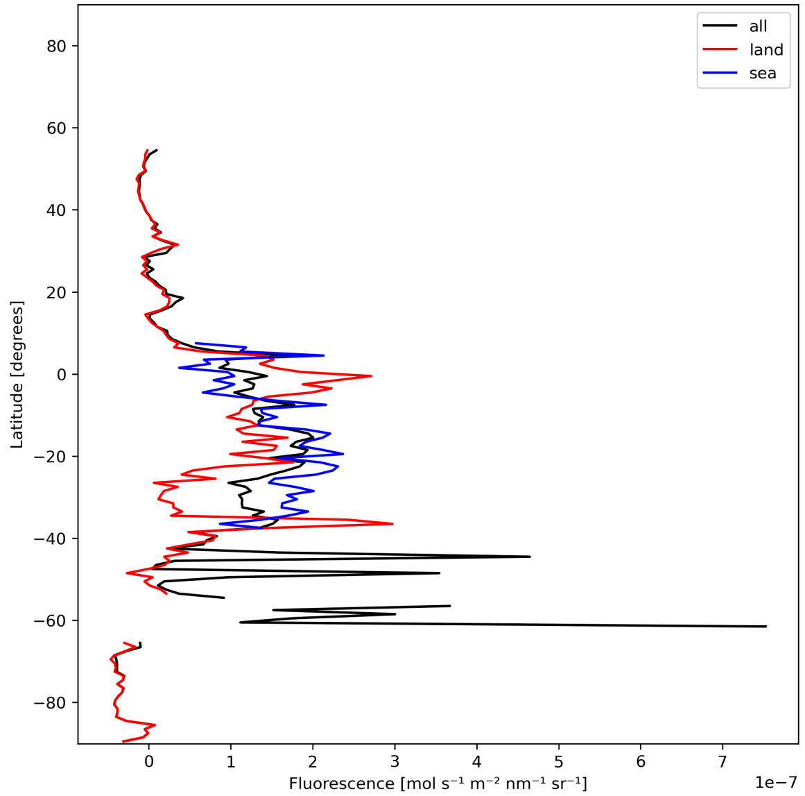
Figure 21: Zonal average of “Fluorescence” for 2023-11-24 to 2023-11-26.
