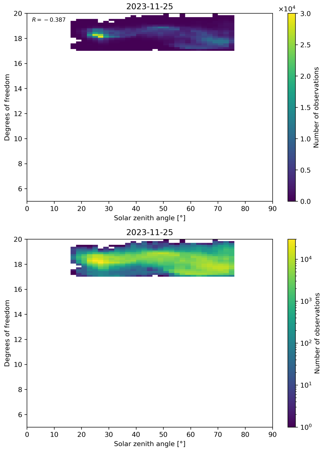
Figure 96: Scatter density plot of “Solar zenith angle” against “Degrees of freedom” for 2023-11-24 to 2023-11-26.
