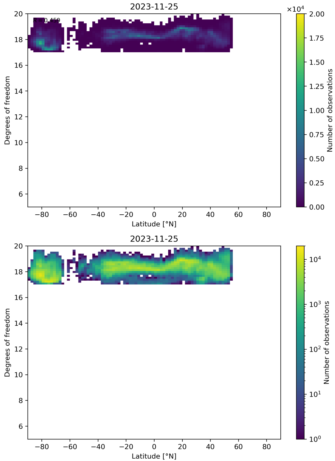
Figure 55: Scatter density plot of “Latitude” against “Degrees of freedom” for 2023-11-24 to 2023-11-26.
