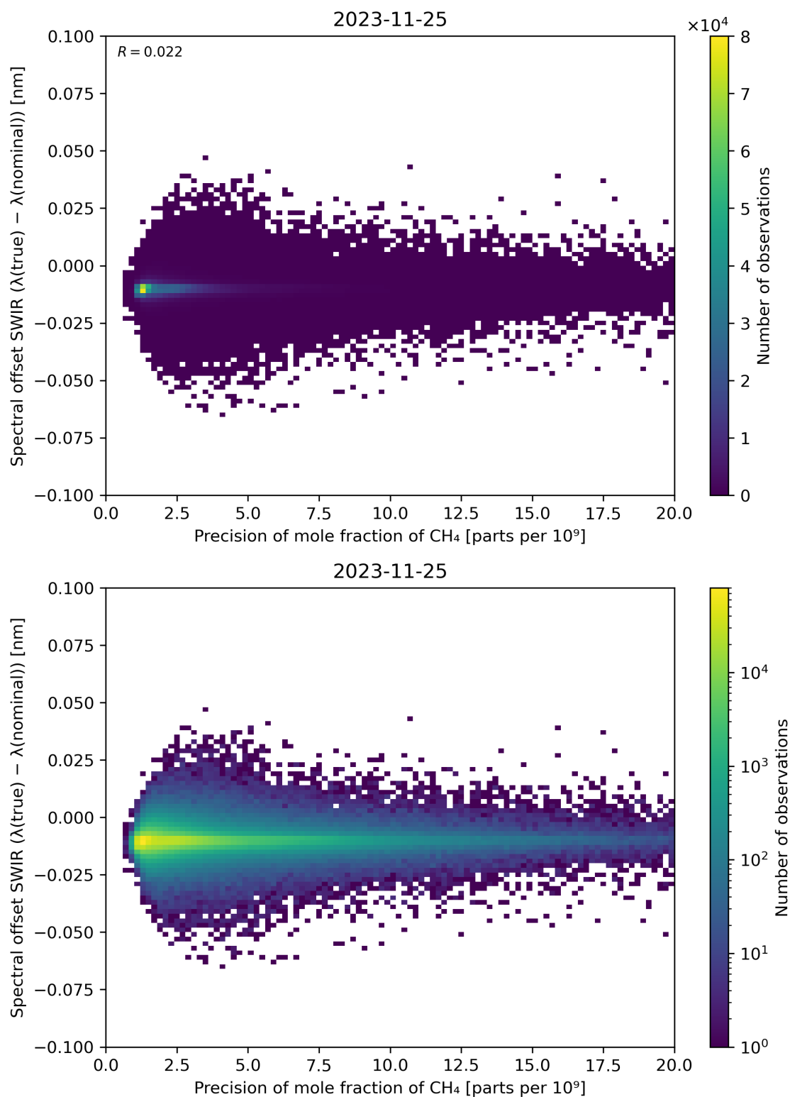
Figure 85: Scatter density plot of “Precision of mole fraction of CH 4 ” against “Spectral offset SWIR ( \lambda(\text{true}) - \lambda(\text{nominal}) )” for 2023-11-24 to 2023-11-26.
