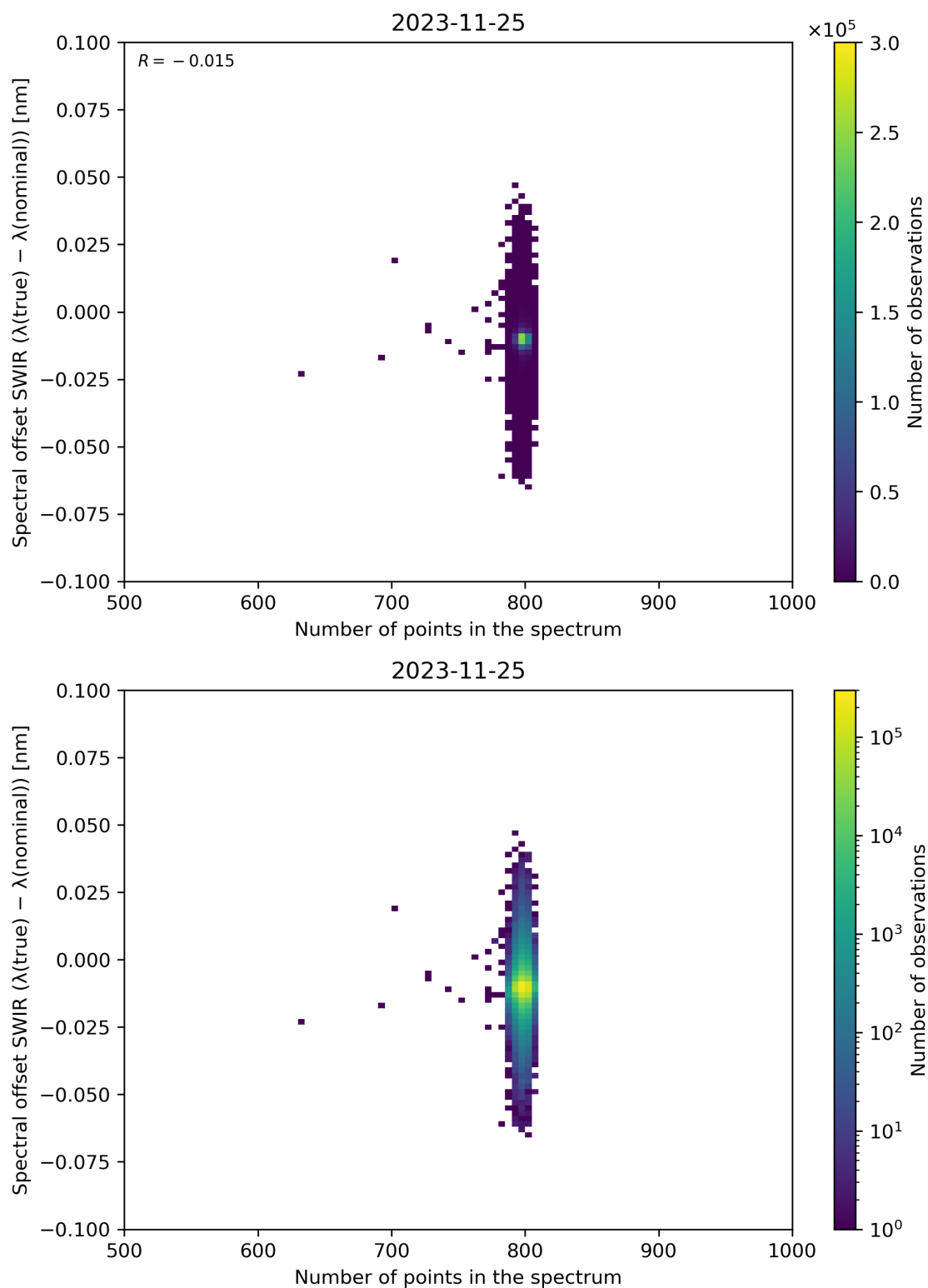
Figure 93: Scatter density plot of “Number of points in the spectrum” against “Spectral offset SWIR ( \lambda(\text{true}) - \lambda(\text{nominal}) )” for 2023-11-24 to 2023-11-26.
