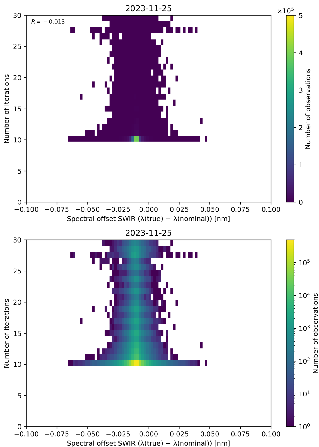
Figure 121: Scatter density plot of “Spectral offset SWIR ( \lambda(\text{true}) - \lambda(\text{nominal}) )” against “Number of iterations” for 2023-11-24 to 2023-11-26.
