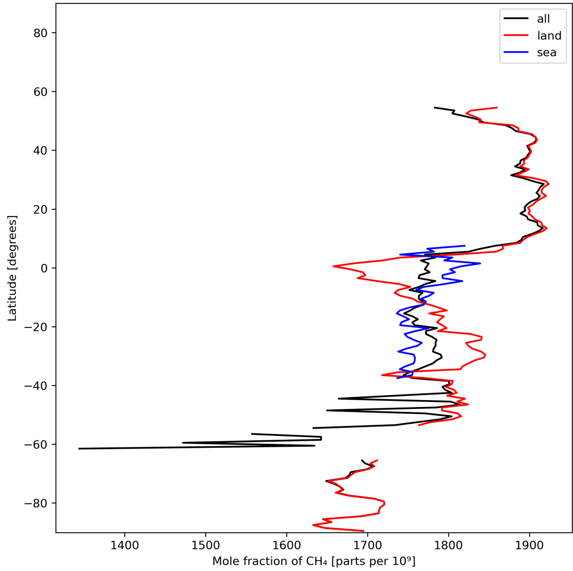
Figure 12: Zonal average of “Mole fraction of CH 4 ” for 2023-11-24 to 2023-11-26.
