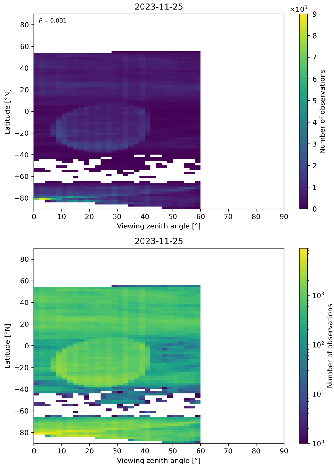
Figure 109: Scatter density plot of “Viewing zenith angle” against “Latitude” for 2023-11-24 to 2023-11-26.
