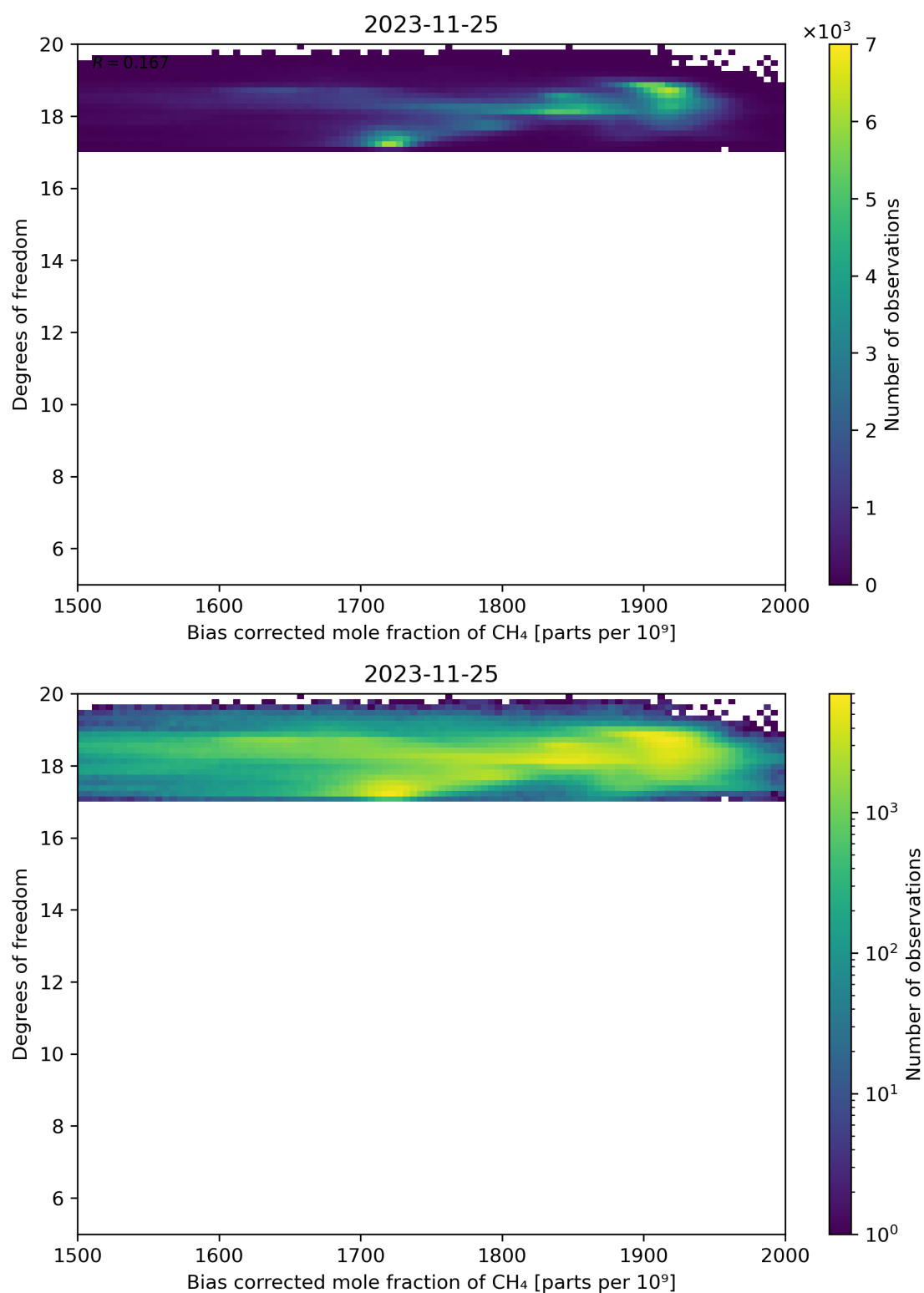
Figure 65: Scatter density plot of “Bias corrected mole fraction of CH 4 ” against “Degrees of freedom” for 2023-11-24 to 2023-11-26.
