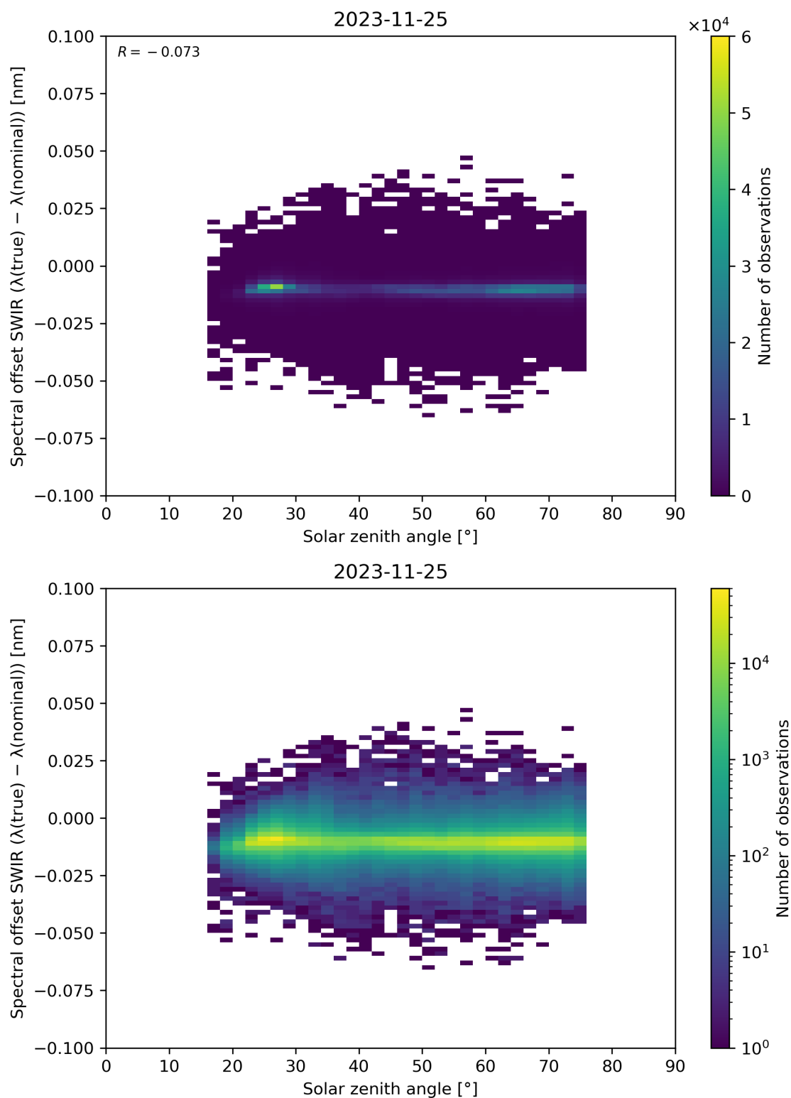
Figure 104: Scatter density plot of “Solar zenith angle” against “Spectral offset SWIR ( \lambda(\text{true}) - \lambda(\text{nominal}) )” for 2023-11-24 to 2023-11-26.
