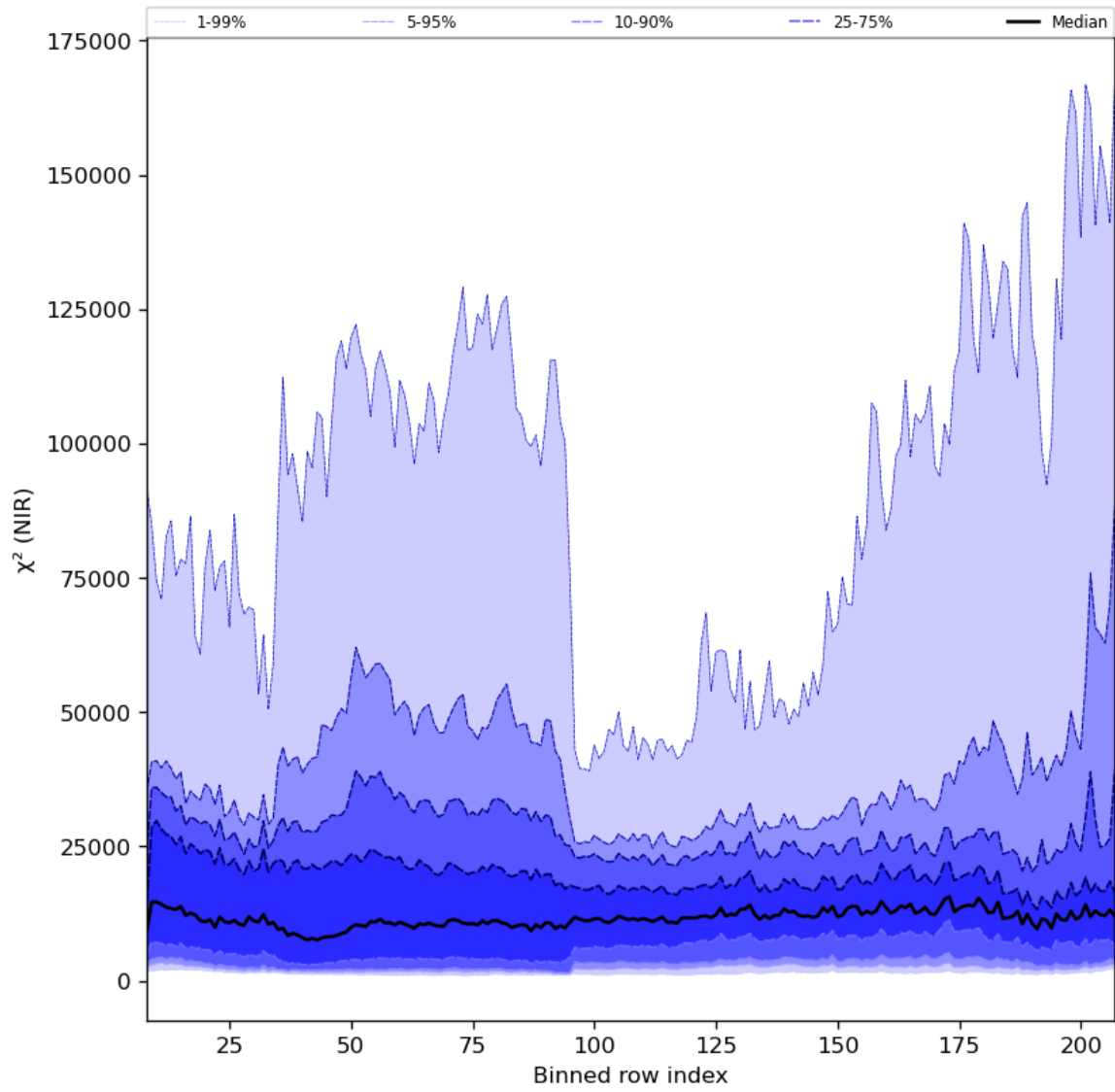
Figure 40: Along track statistics of “ \chi^2 (NIR)” for 2023-11-24 to 2023-11-26
