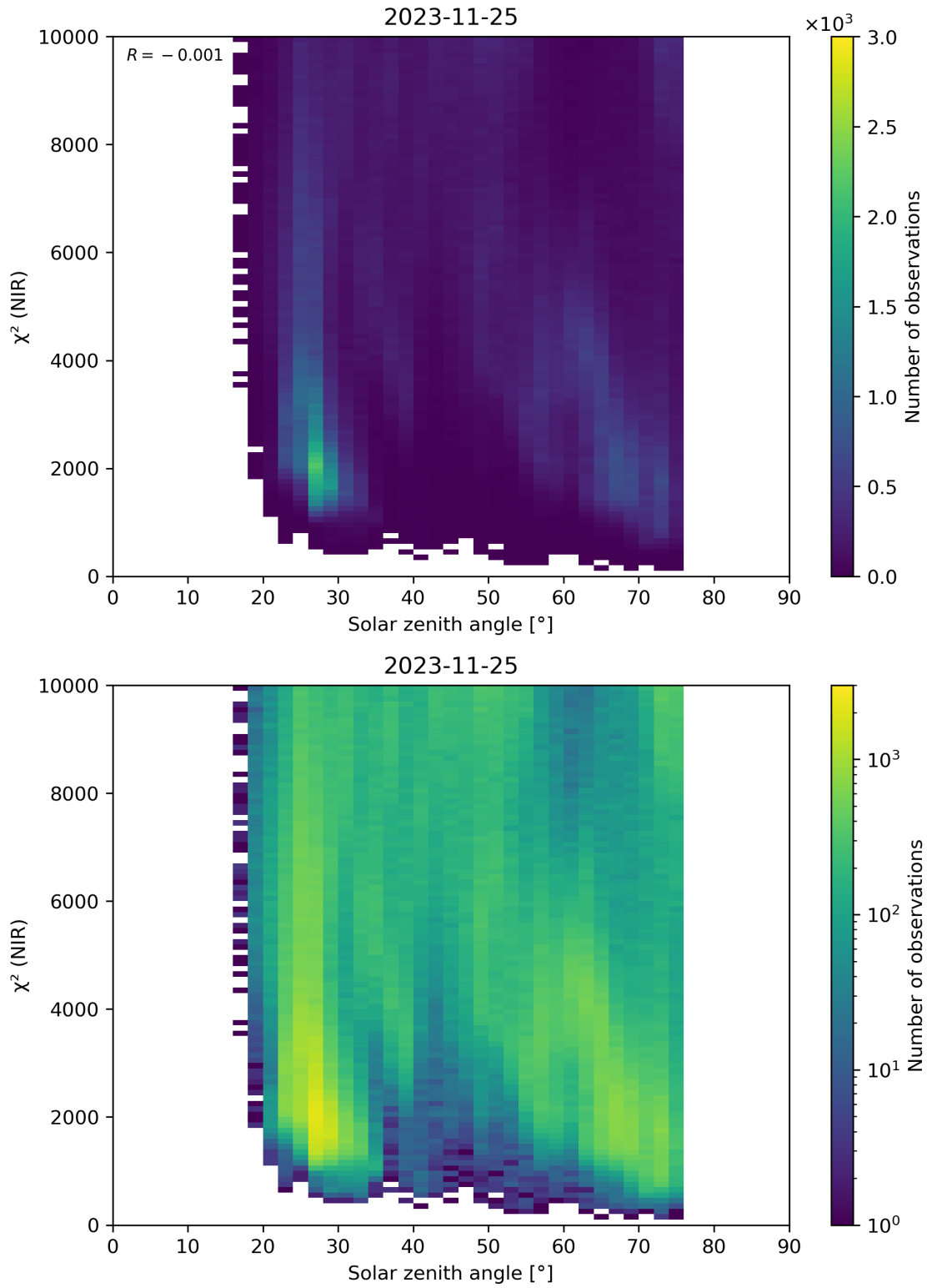
Figure 94: Scatter density plot of “Solar zenith angle” against “ \chi^2 (NIR)” for 2023-11-24 to 2023-11-26.
