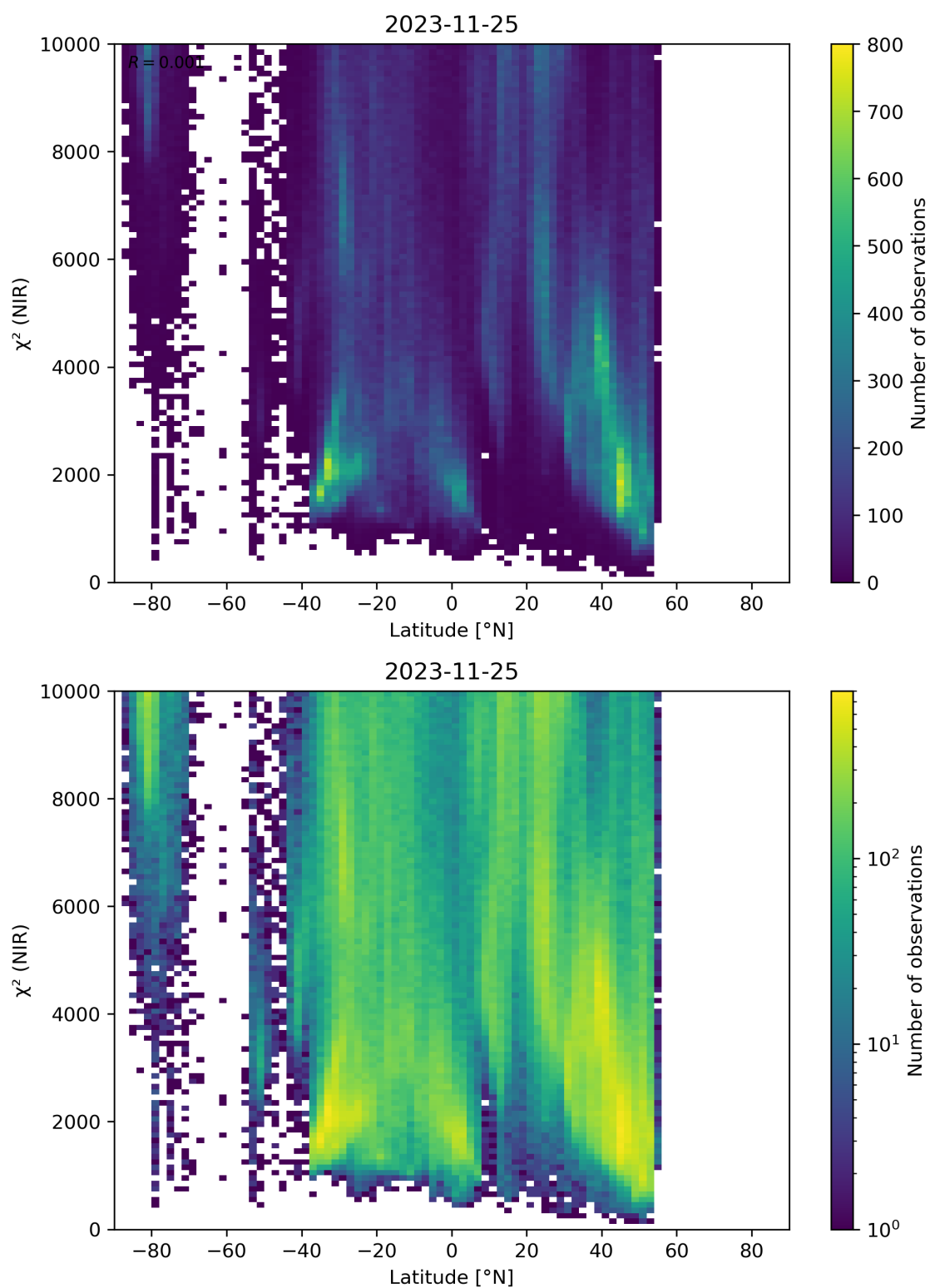
Figure 53: Scatter density plot of “Latitude” against “ \chi^2 (NIR)” for 2023-11-24 to 2023-11-26.
