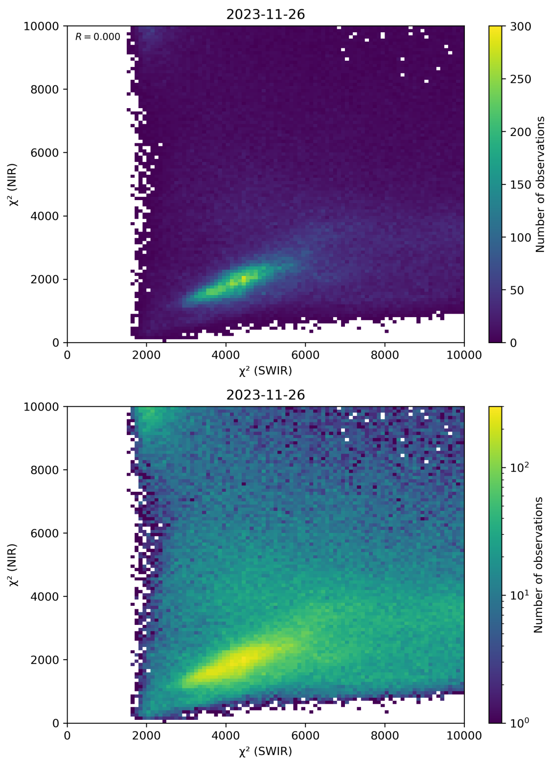
Figure 47: Scatter density plot of “ \chi^2 (SWIR)” against “ \chi^2 (NIR)” for 2023-11-25 to 2023-11-27.
