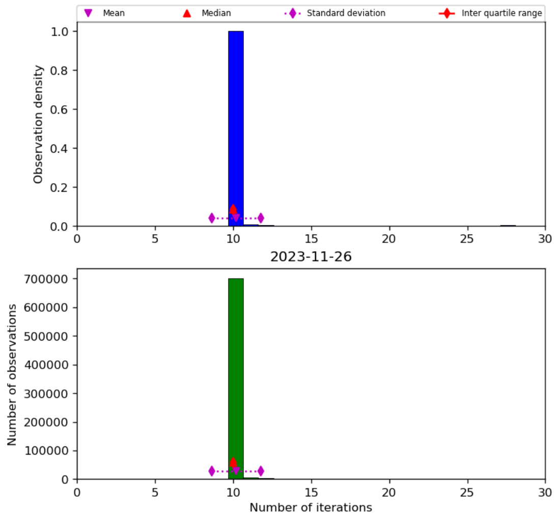
Figure 31: Histogram of “Number of iterations” for 2023-11-25 to 2023-11-27
