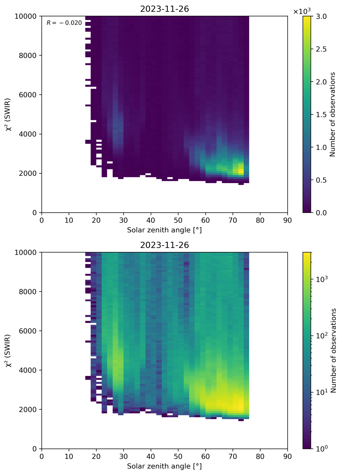
Figure 95: Scatter density plot of “Solar zenith angle” against “ \chi^2 (SWIR)” for 2023-11-25 to 2023-11-27.
