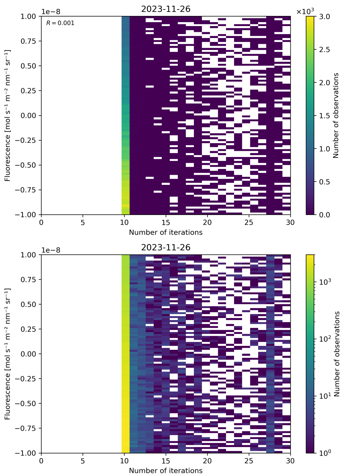
Figure 87: Scatter density plot of “Number of iterations” against “Fluorescence” for 2023-11-25 to 2023-11-27.
