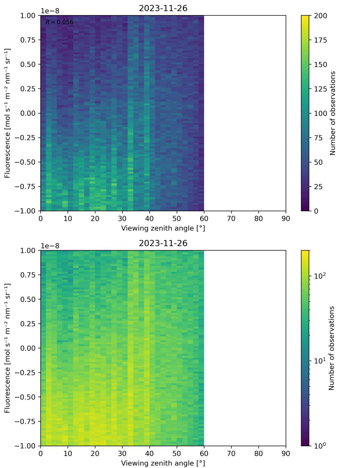
Figure 108: Scatter density plot of “Viewing zenith angle” against “Fluorescence” for 2023-11-25 to 2023-11-27.
