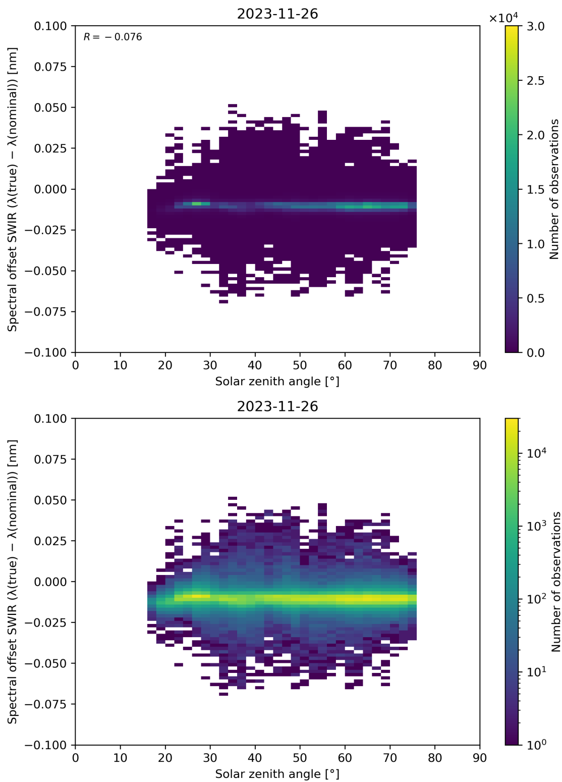
Figure 104: Scatter density plot of “Solar zenith angle” against “Spectral offset SWIR ( \lambda(\text{true}) - \lambda(\text{nominal}) )” for 2023-11-25 to 2023-11-27.
