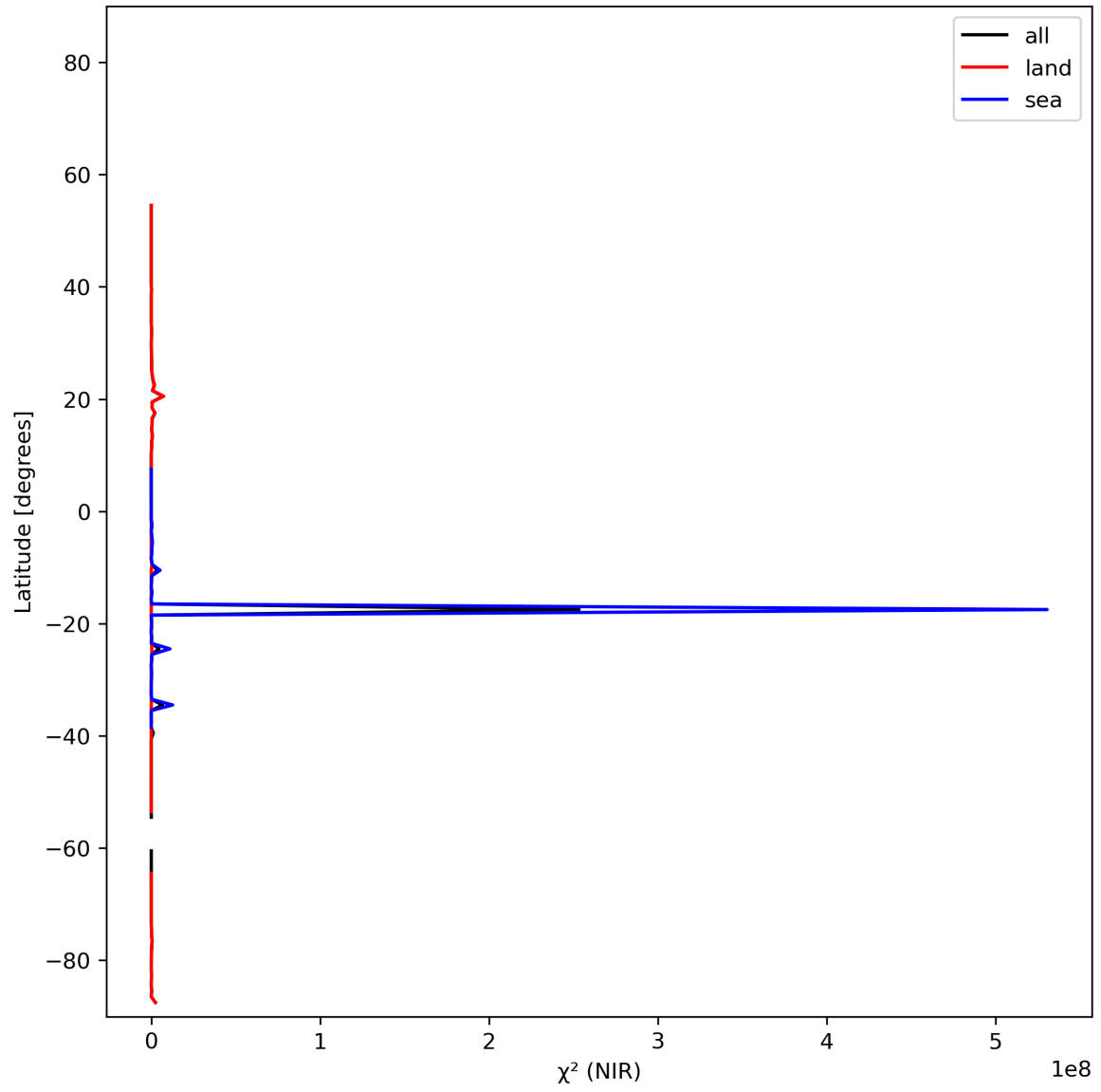
Figure 18: Zonal average of “ \chi^2 (NIR)” for 2023-11-25 to 2023-11-27.
