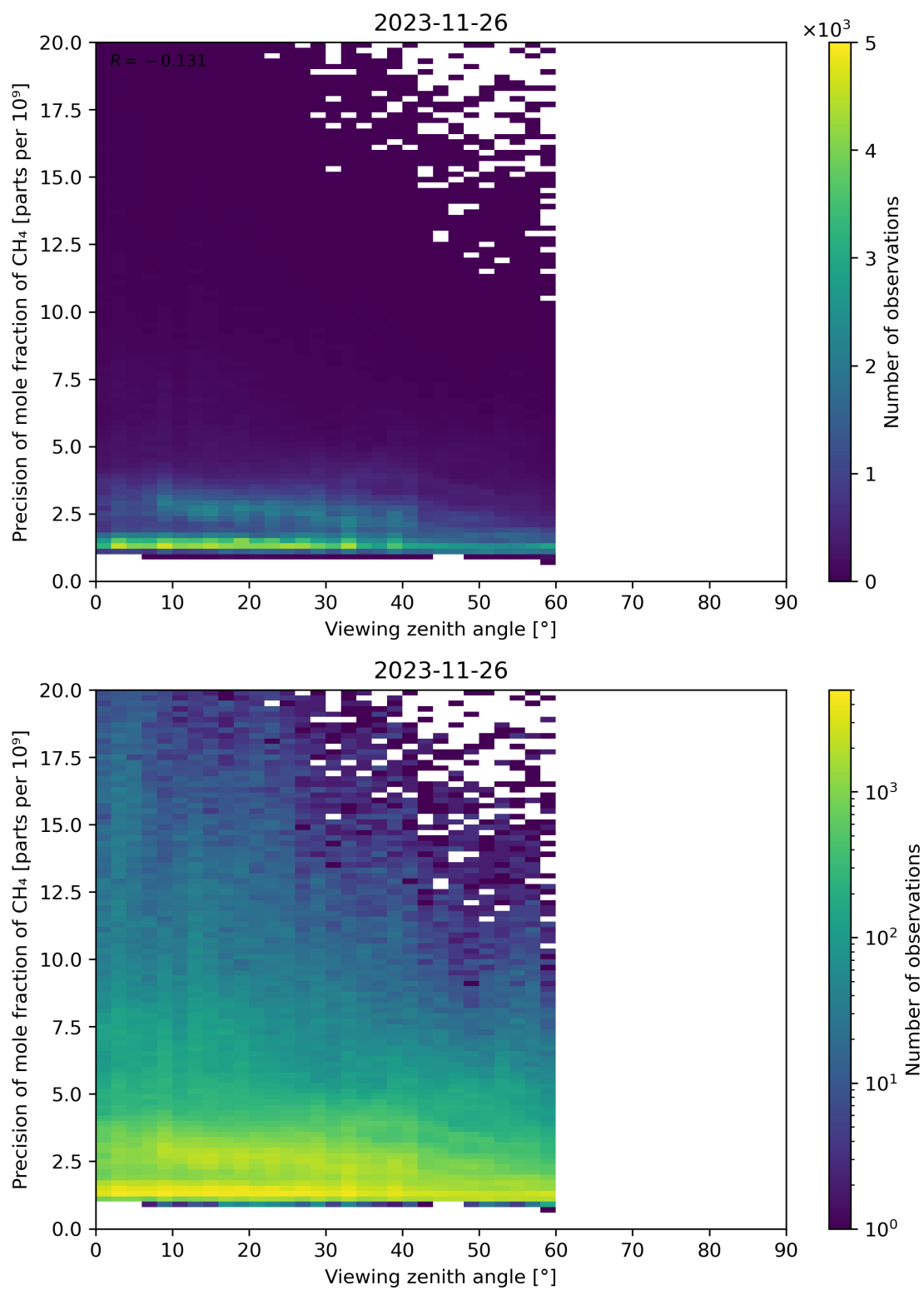
Figure 112: Scatter density plot of “Viewing zenith angle” against “Precision of mole fraction of CH 4 ” for 2023-11-25 to 2023-11-27.
