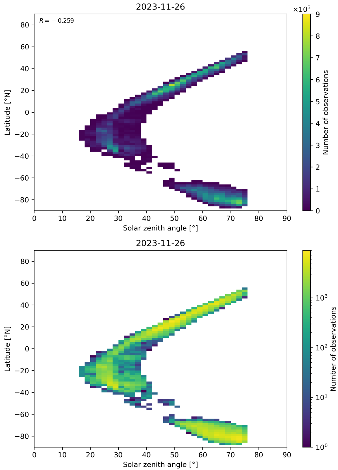
Figure 98: Scatter density plot of “Solar zenith angle” against “Latitude” for 2023-11-25 to 2023-11-27.
