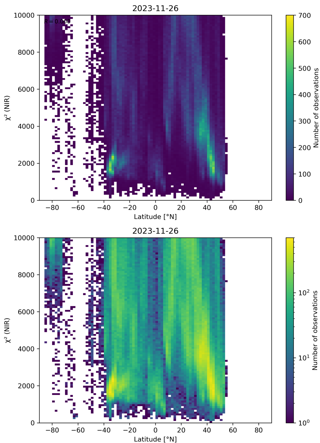
Figure 53: Scatter density plot of “Latitude” against “ \chi^2 (NIR)” for 2023-11-25 to 2023-11-27.
