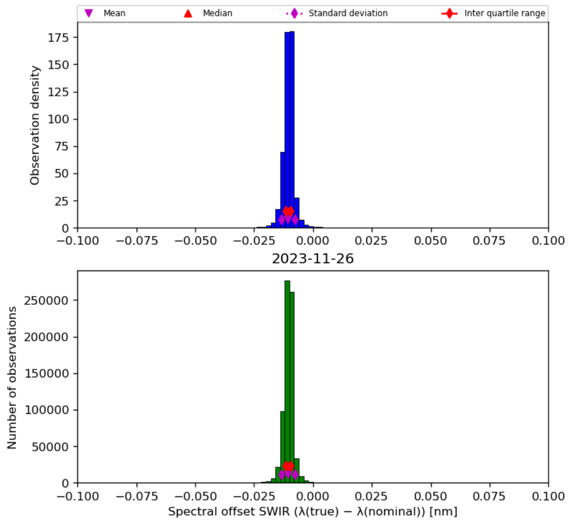
Figure 27: Histogram of “Spectral offset SWIR ( \lambda(\text{true}) - \lambda(\text{nominal}) )” for 2023-11-25 to 2023-11-27
