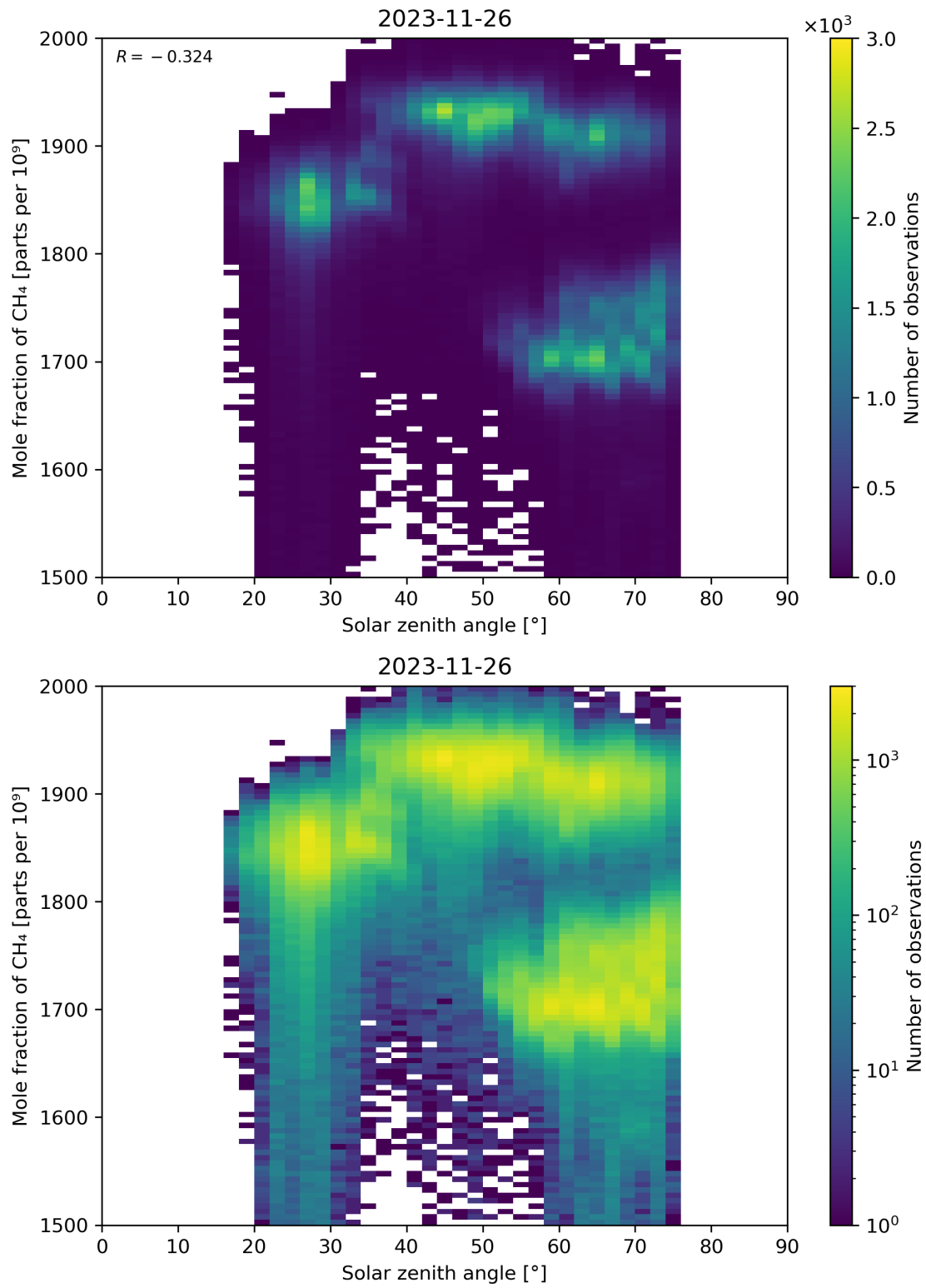
Figure 99: Scatter density plot of “Solar zenith angle” against “Mole fraction of \text{CH}_4 ” for 2023-11-25 to 2023-11-27.
