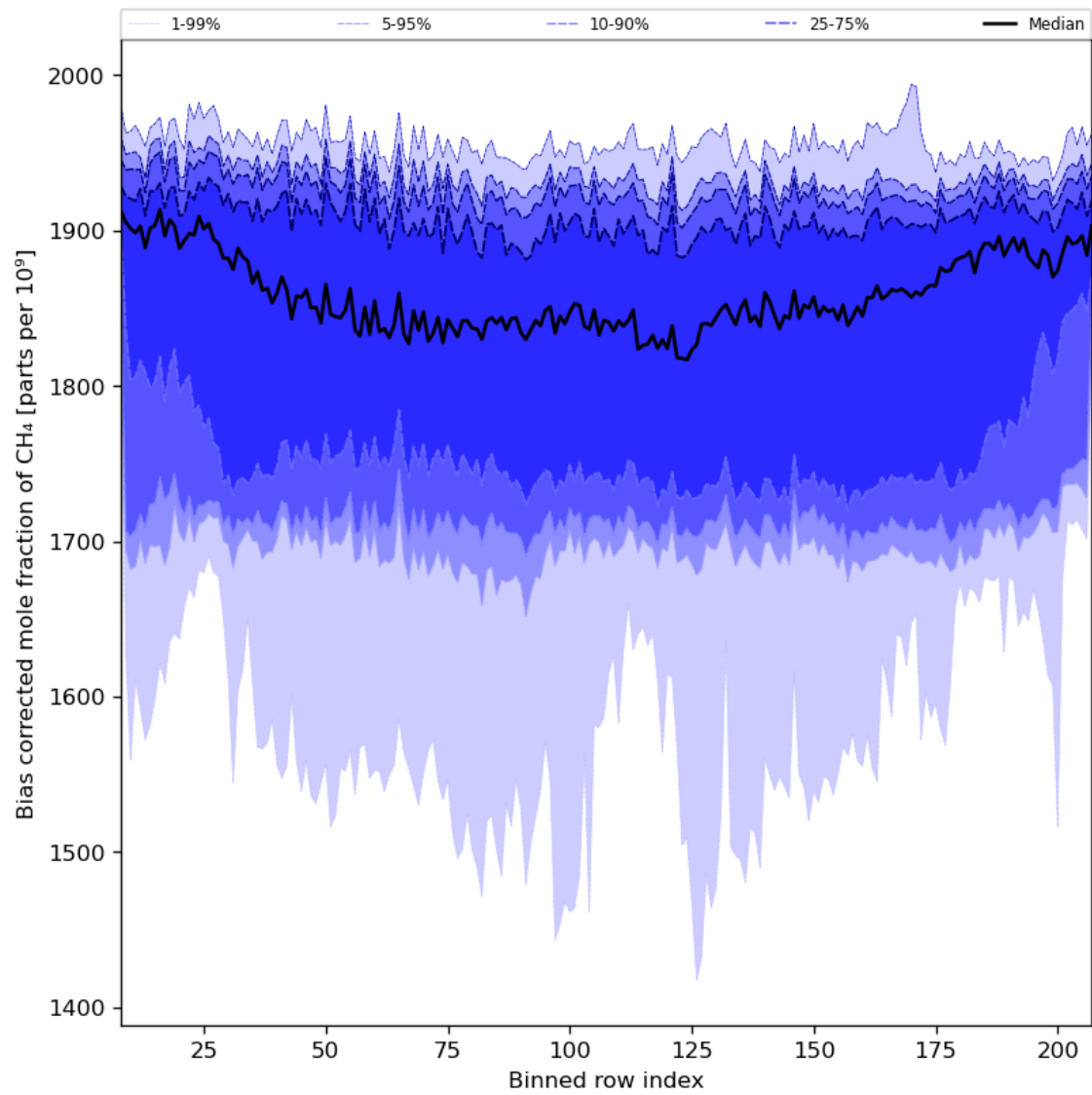
Figure 36: Along track statistics of “Bias corrected mole fraction of CH 4 ” for 2023-11-25 to 2023-11-27
