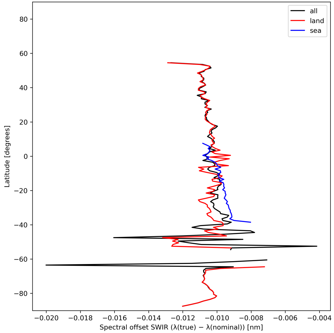
Figure 16: Zonal average of “Spectral offset SWIR ( \lambda(\text{true}) - \lambda(\text{nominal}) )” for 2023-11-25 to 2023-11-27.
