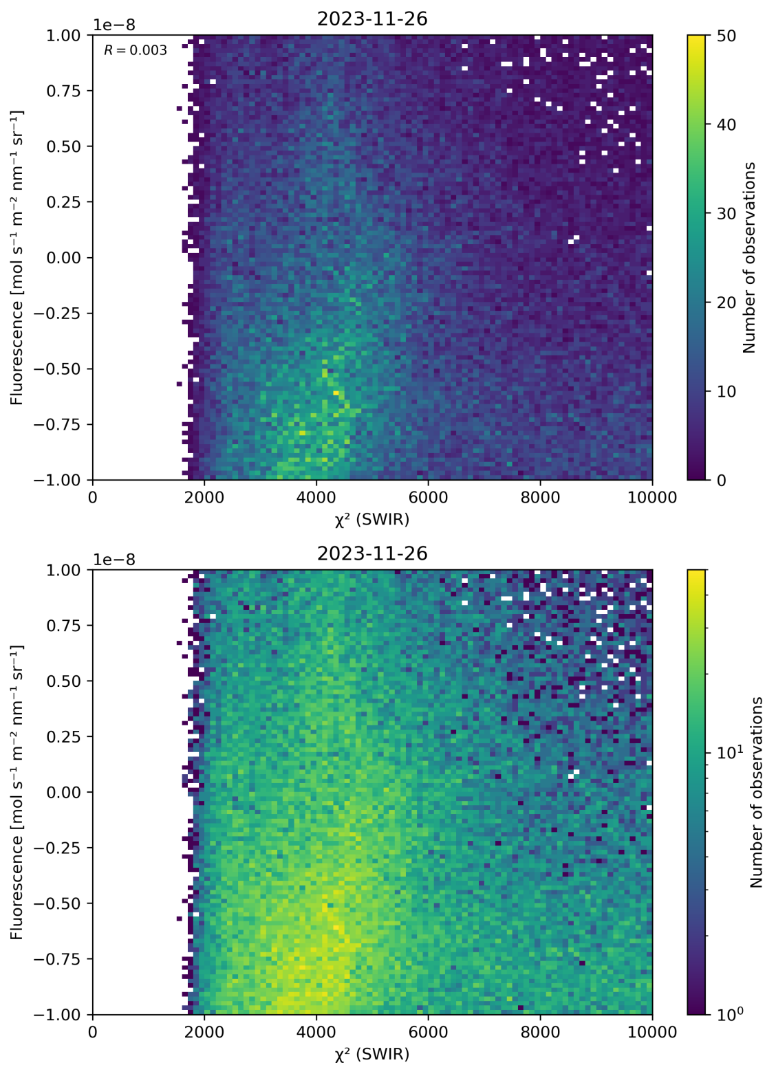
Figure 49: Scatter density plot of “ \chi^2 (SWIR)” against “Fluorescence” for 2023-11-25 to 2023-11-27.
