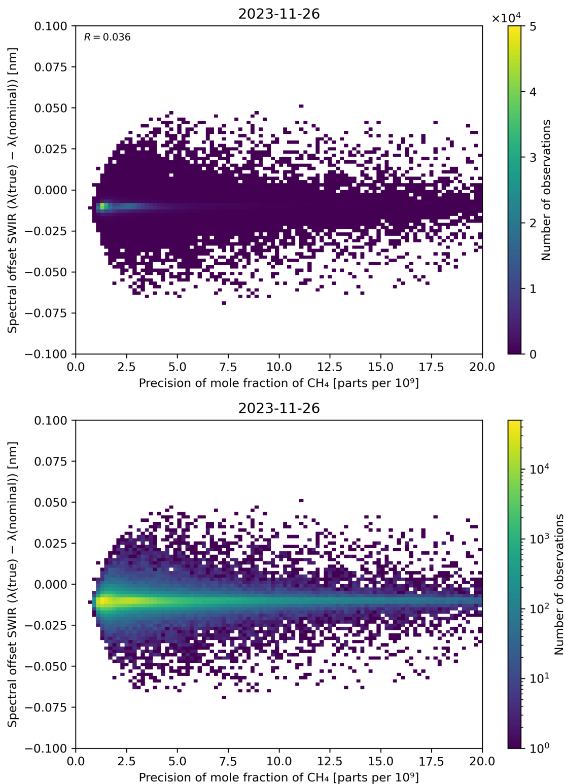
Figure 85: Scatter density plot of “Precision of mole fraction of \text{CH}_4 ” against “Spectral offset SWIR ( \lambda(\text{true}) - \lambda(\text{nominal}) )” for 2023-11-25 to 2023-11-27.
