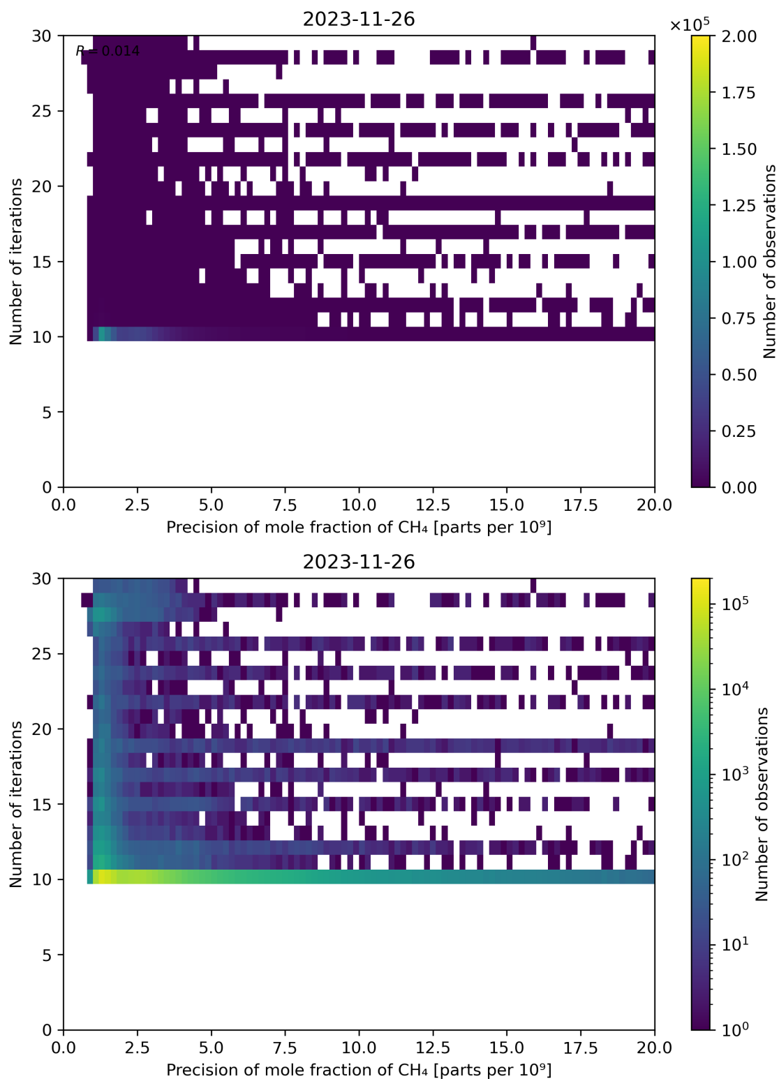
Figure 83: Scatter density plot of “Precision of mole fraction of CH 4 ” against “Number of iterations” for 2023-11-25 to 2023-11-27.
