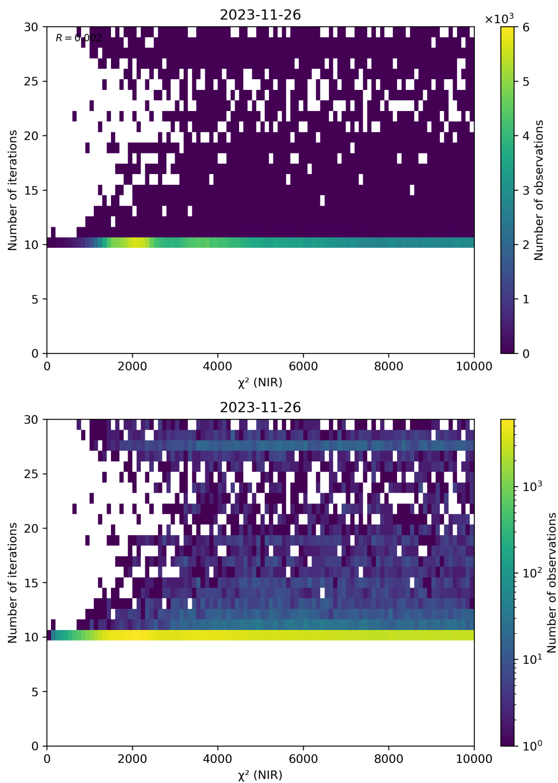
Figure 46: Scatter density plot of “ \chi^2 (NIR)” against “Number of iterations” for 2023-11-25 to 2023-11-27.
