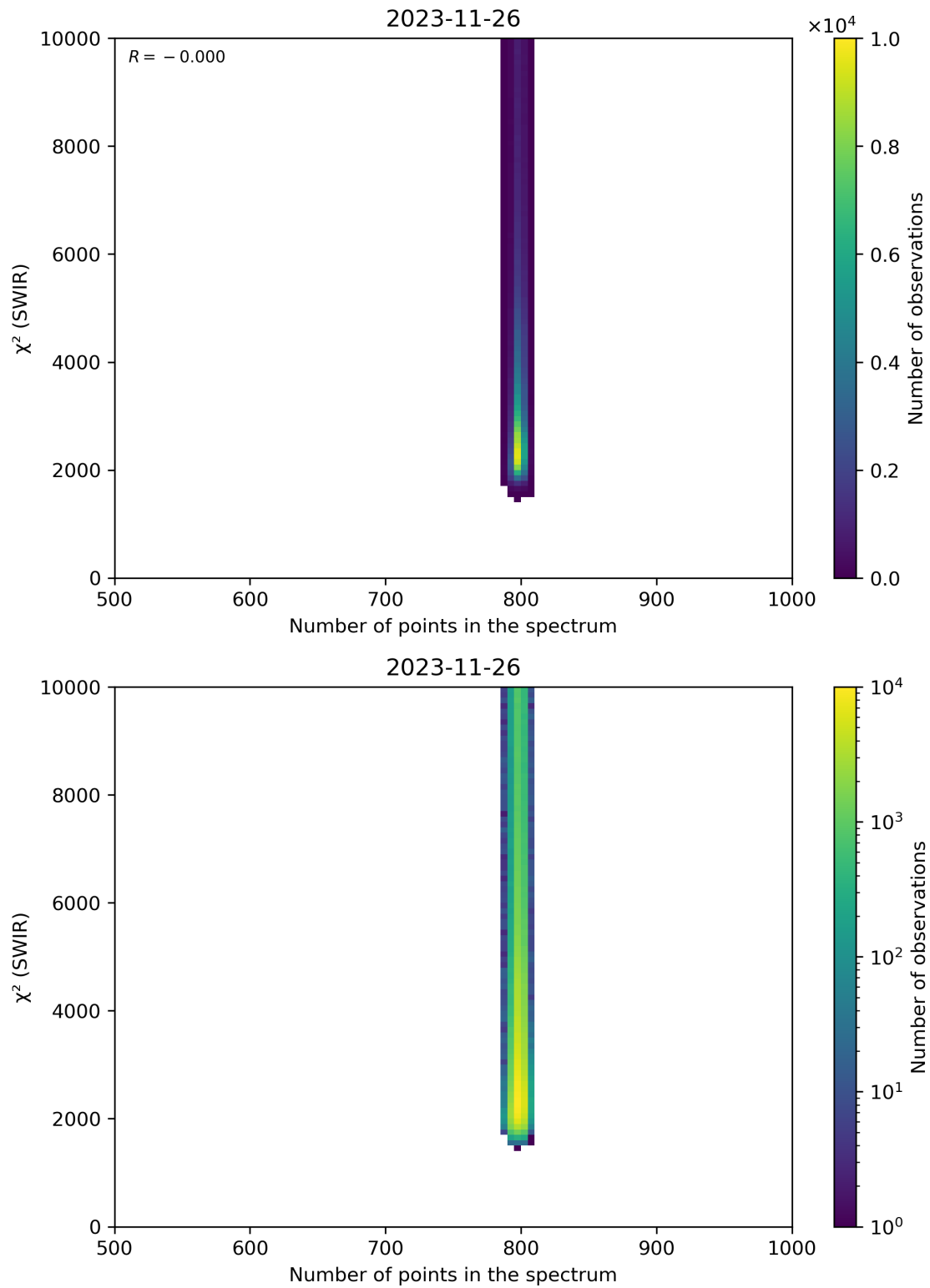
Figure 89: Scatter density plot of “Number of points in the spectrum” against “ \chi^2 (SWIR)” for 2023-11-25 to 2023-11-27.
