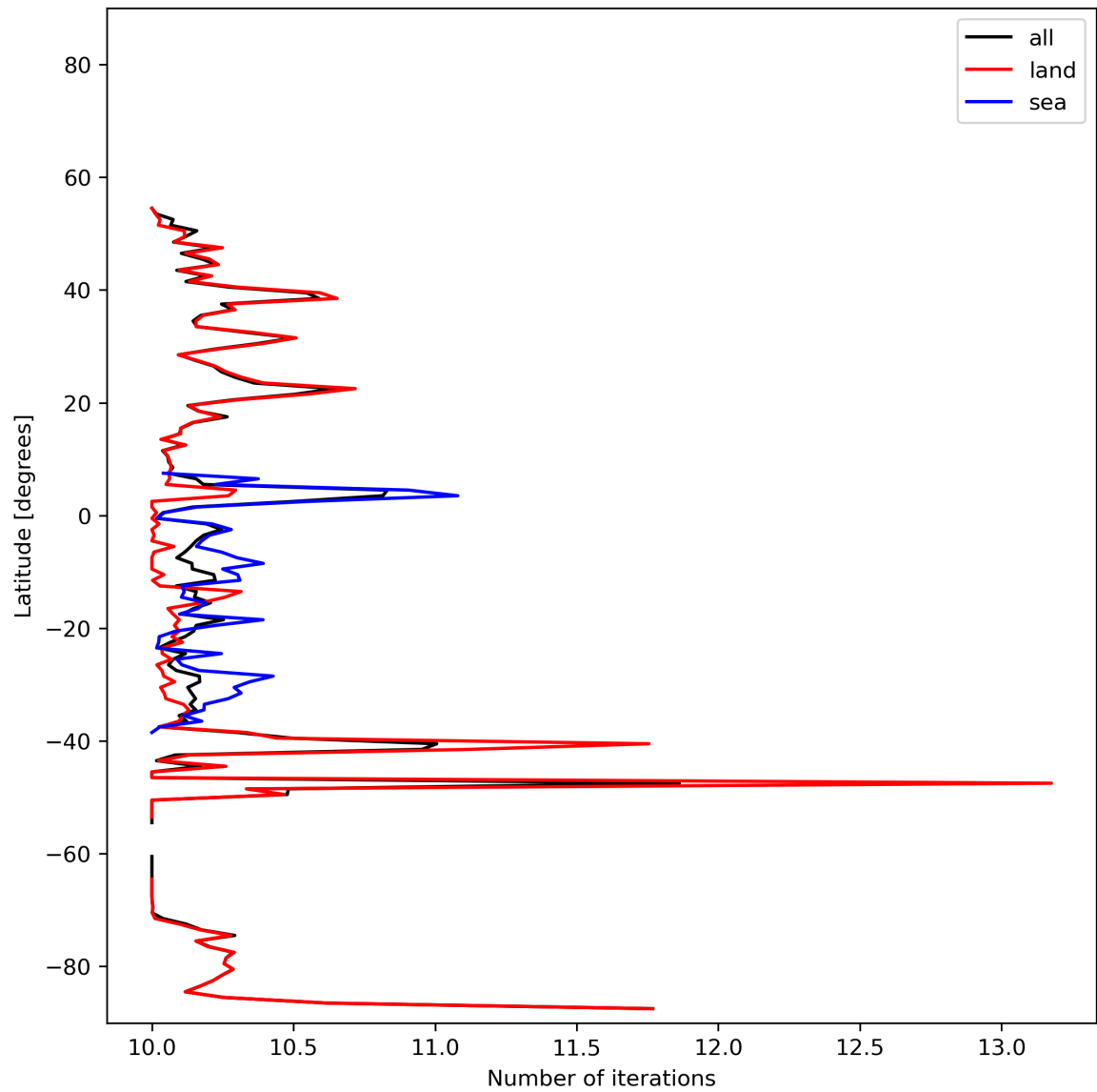
Figure 20: Zonal average of “Number of iterations” for 2023-11-25 to 2023-11-27.
