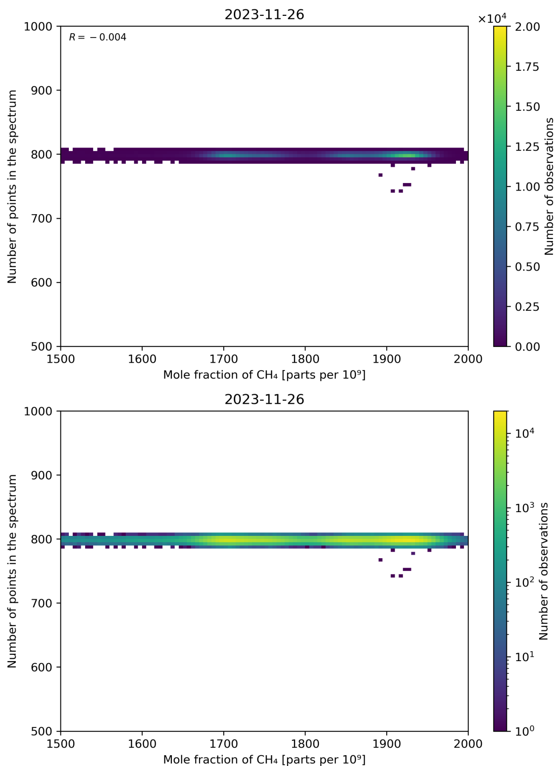
Figure 77: Scatter density plot of “Mole fraction of CH 4 ” against “Number of points in the spectrum” for 2023-11-25 to 2023-11-27.
