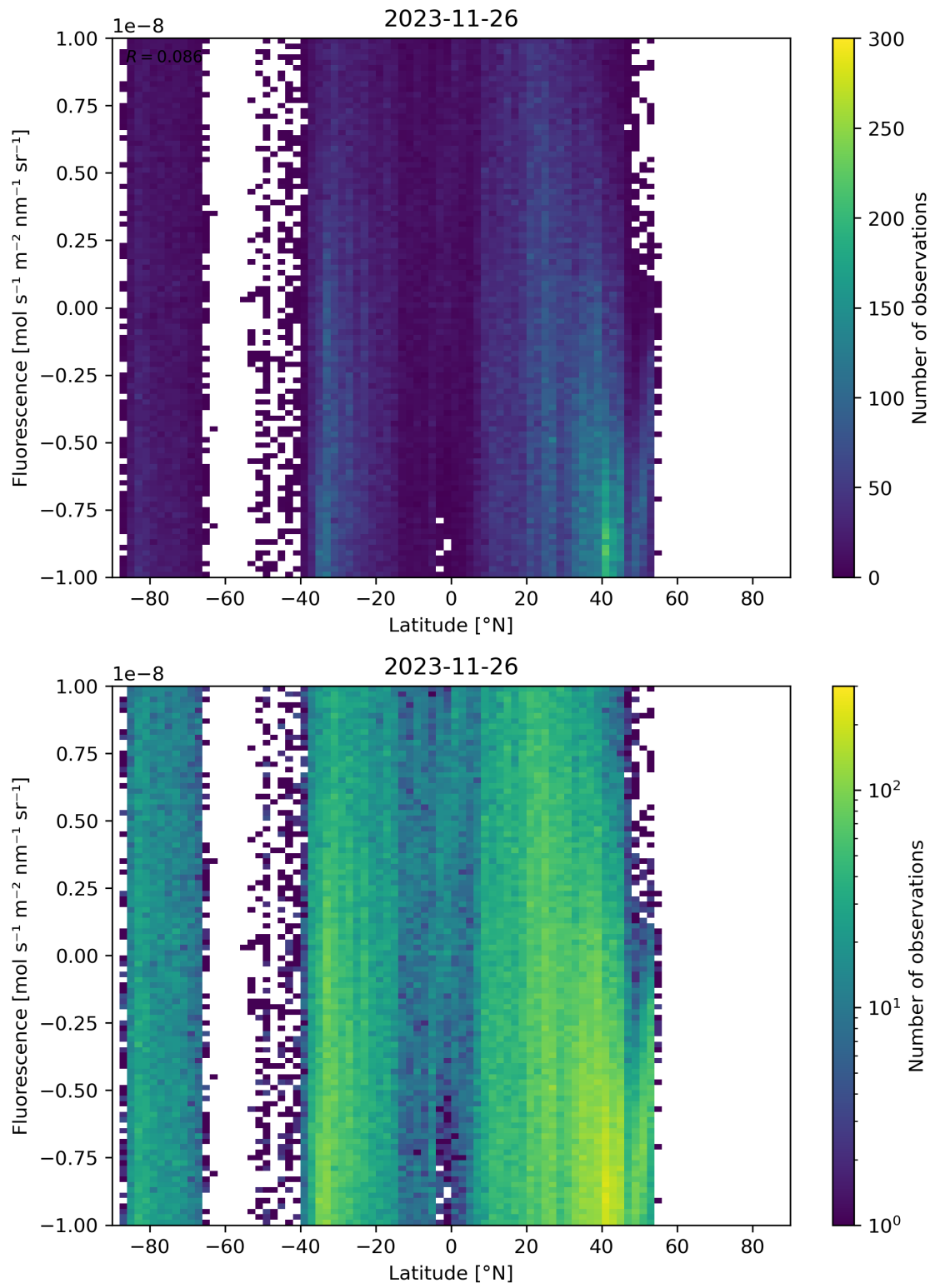
Figure 56: Scatter density plot of “Latitude” against “Fluorescence” for 2023-11-25 to 2023-11-27.
