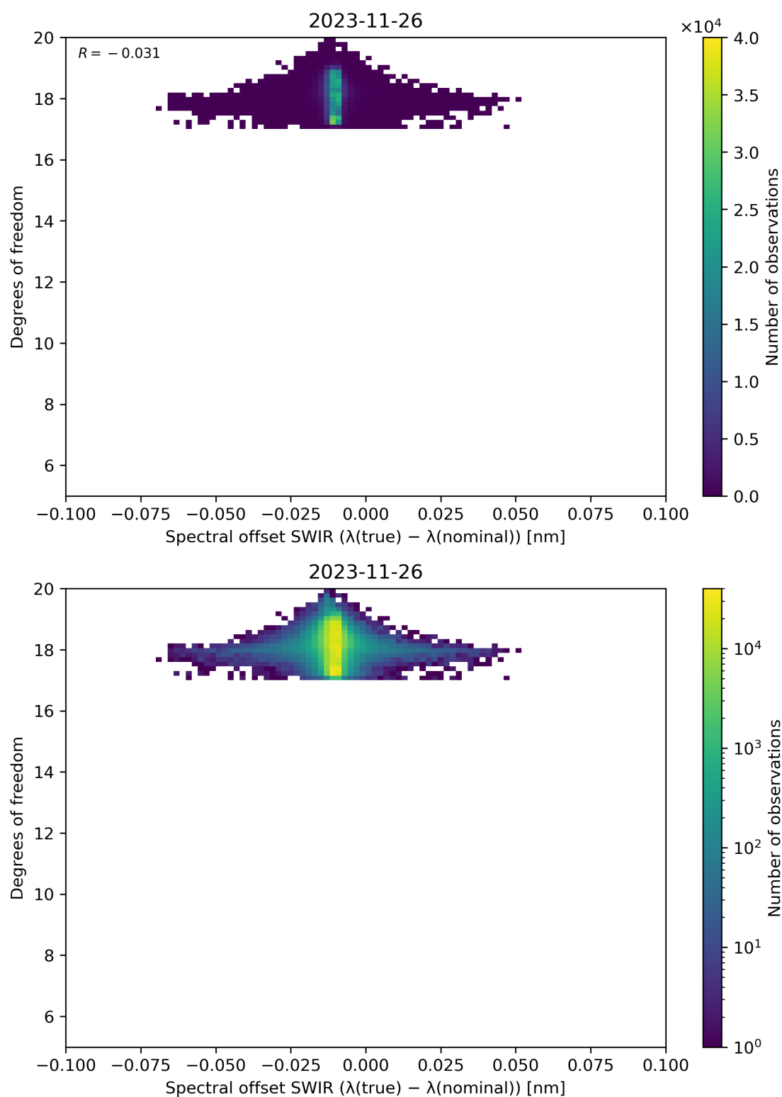
Figure 119: Scatter density plot of “Spectral offset SWIR ( \lambda(\text{true}) - \lambda(\text{nominal}) )” against “Degrees of freedom” for 2023-11-25 to 2023-11-27.
