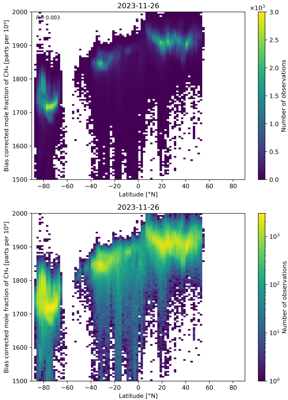
Figure 58: Scatter density plot of “Latitude” against “Bias corrected mole fraction of CH 4 ” for 2023-11-25 to 2023-11-27.
