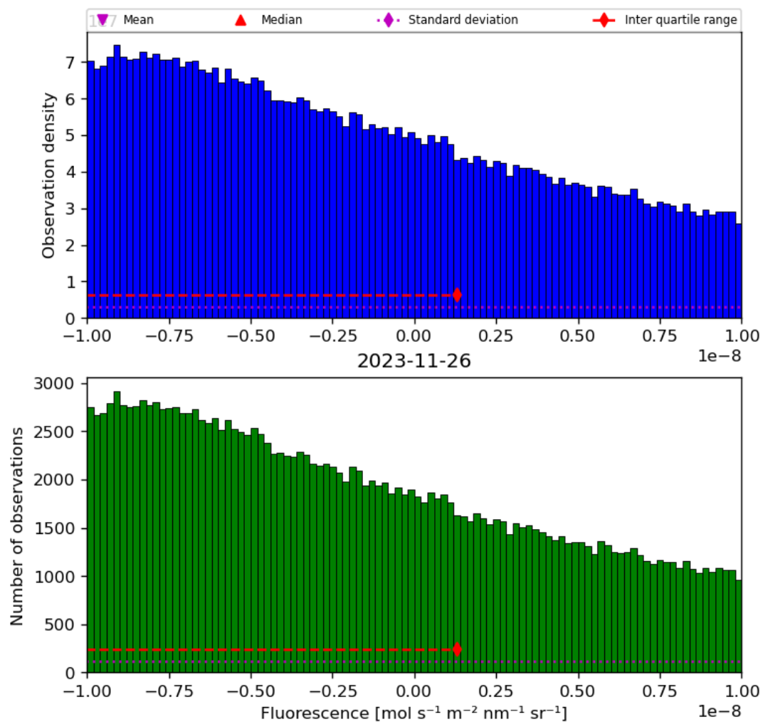
Figure 32: Histogram of “Fluorescence” for 2023-11-25 to 2023-11-27
