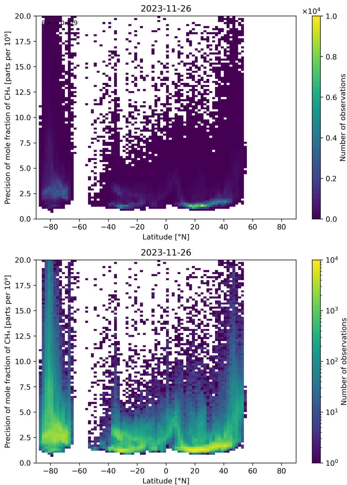
Figure 59: Scatter density plot of “Latitude” against “Precision of mole fraction of CH 4 ” for 2023-11-25 to 2023-11-27.
