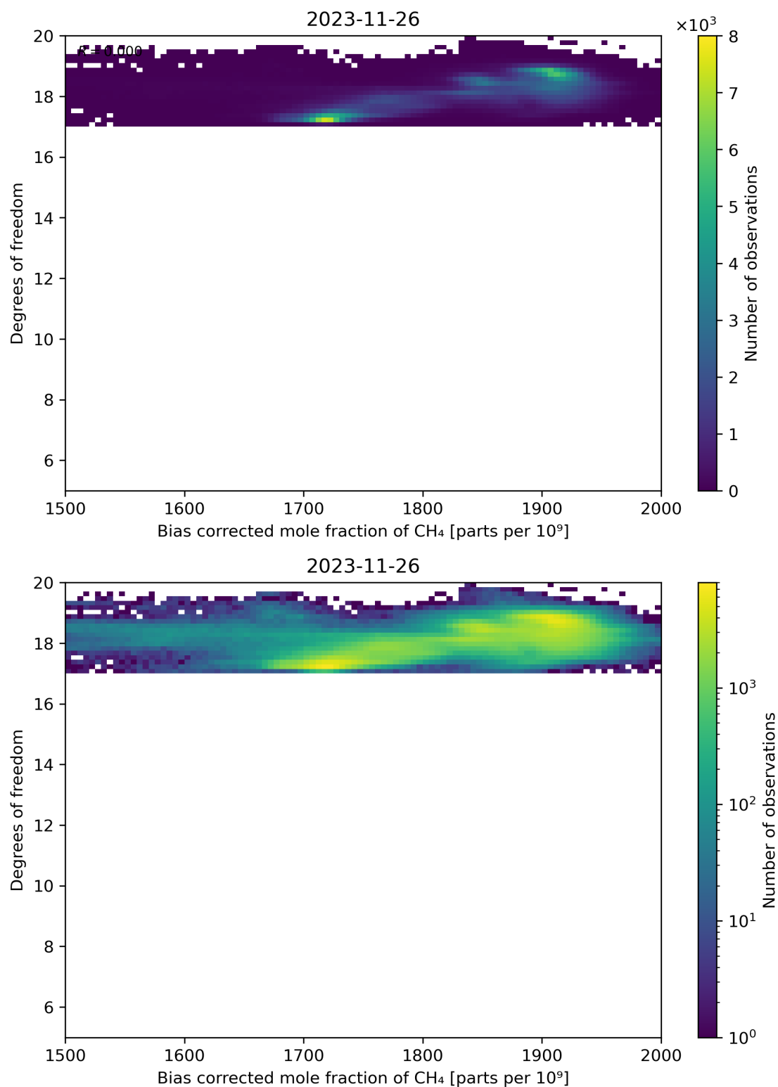
Figure 65: Scatter density plot of “Bias corrected mole fraction of CH 4 ” against “Degrees of freedom” for 2023-11-25 to 2023-11-27.
