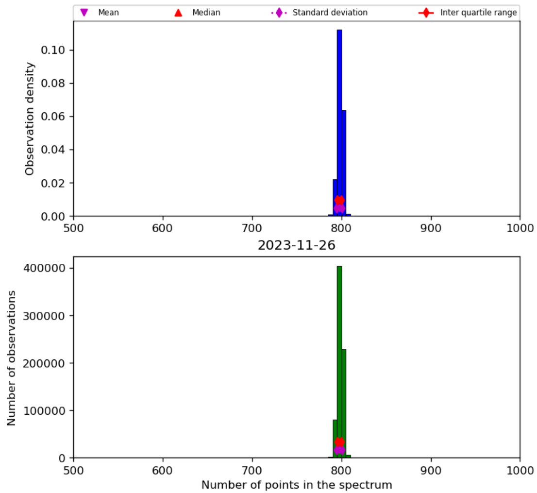
Figure 26: Histogram of “Number of points in the spectrum” for 2023-11-25 to 2023-11-27
