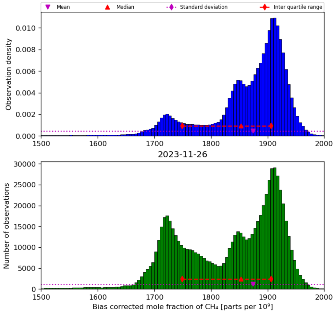
Figure 25: Histogram of “Bias corrected mole fraction of CH 4 ” for 2023-11-25 to 2023-11-27
