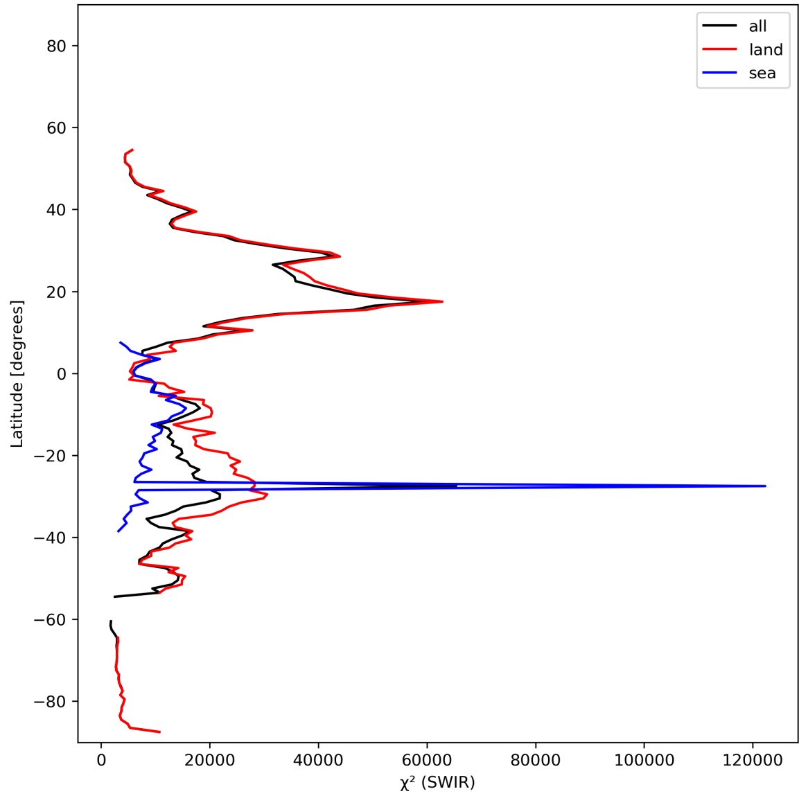
Figure 17: Zonal average of “ \chi^2 (SWIR)” for 2023-11-25 to 2023-11-27.
