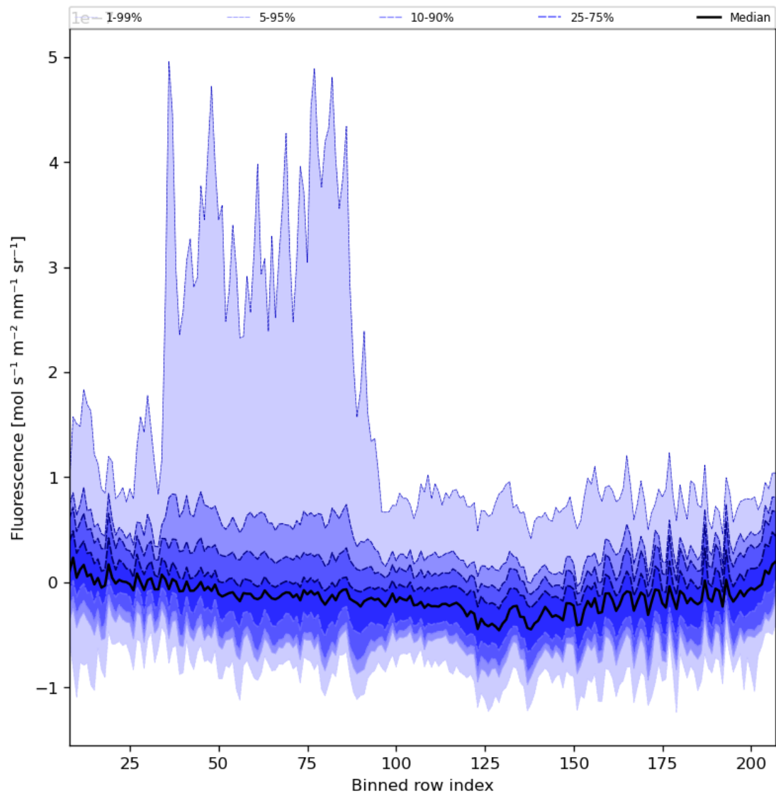
Figure 43: Along track statistics of “Fluorescence” for 2023-11-25 to 2023-11-27
