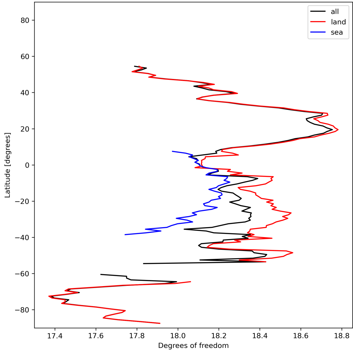
Figure 19: Zonal average of “Degrees of freedom” for 2023-11-25 to 2023-11-27.
