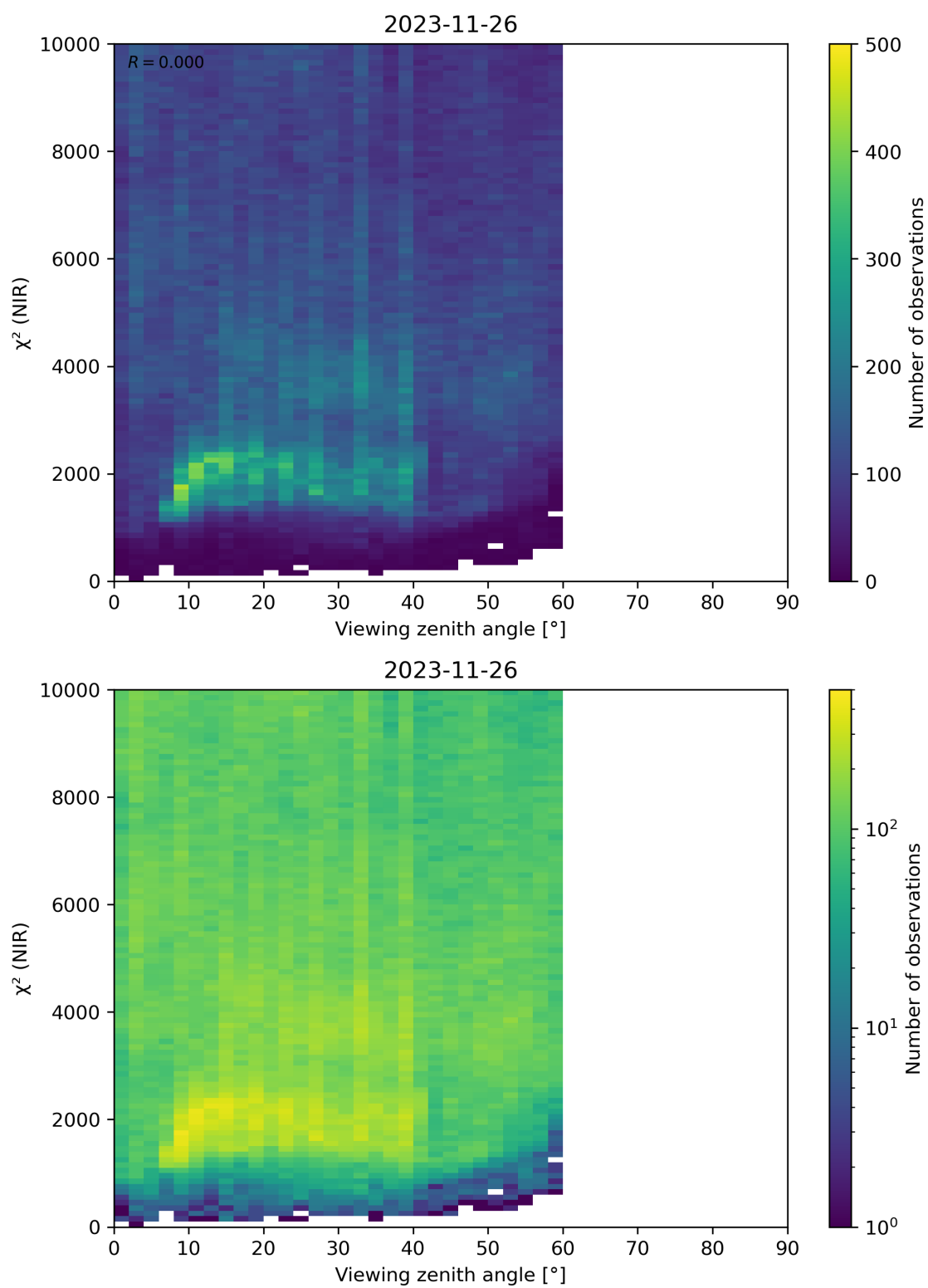
Figure 105: Scatter density plot of “Viewing zenith angle” against “ \chi^2 (NIR)” for 2023-11-25 to 2023-11-27.
