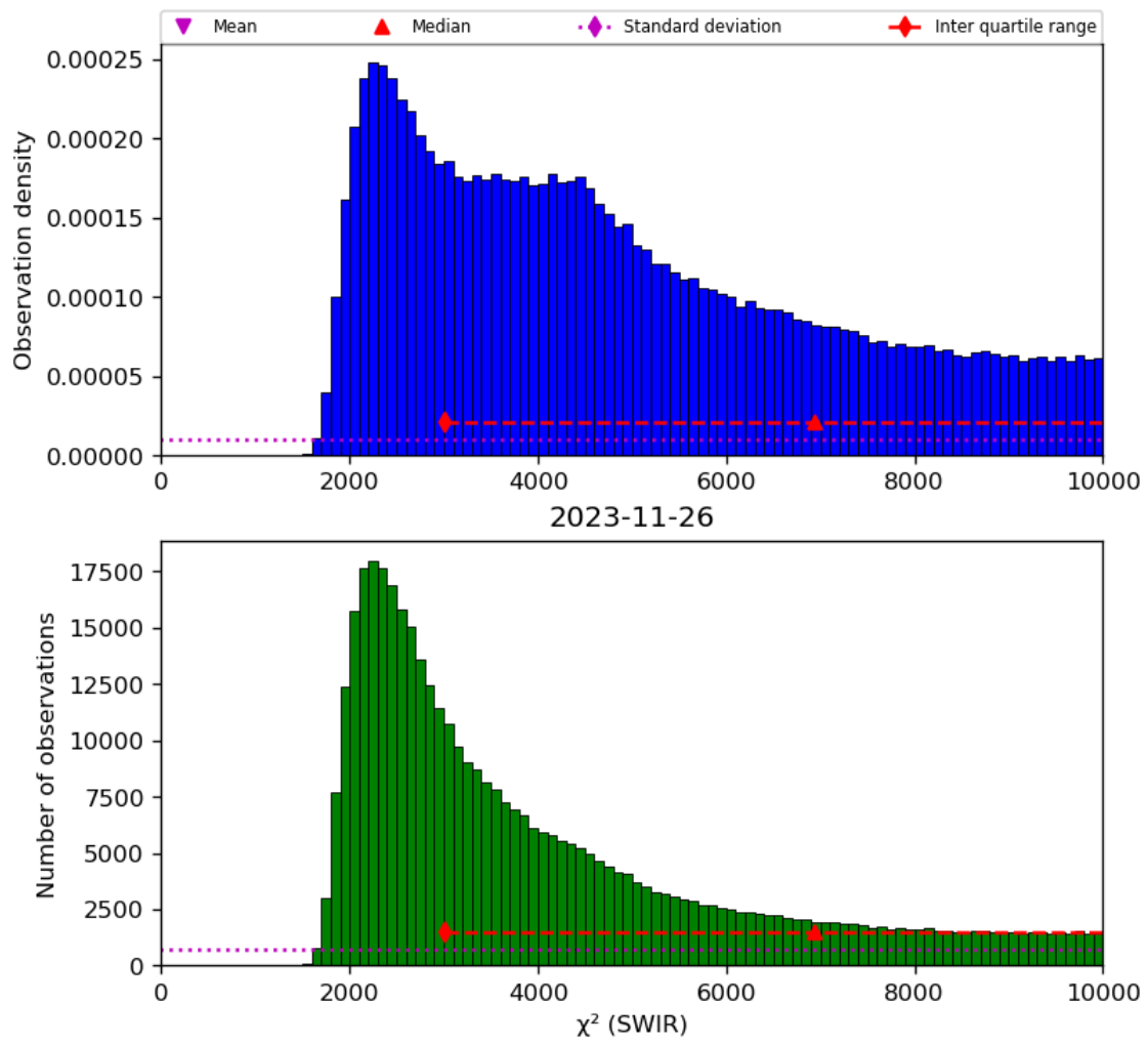
Figure 28: Histogram of “ \chi^2 (SWIR)” for 2023-11-25 to 2023-11-27
