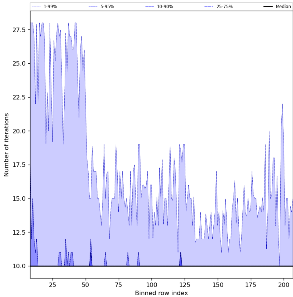
Figure 42: Along track statistics of “Number of iterations” for 2023-11-25 to 2023-11-27
