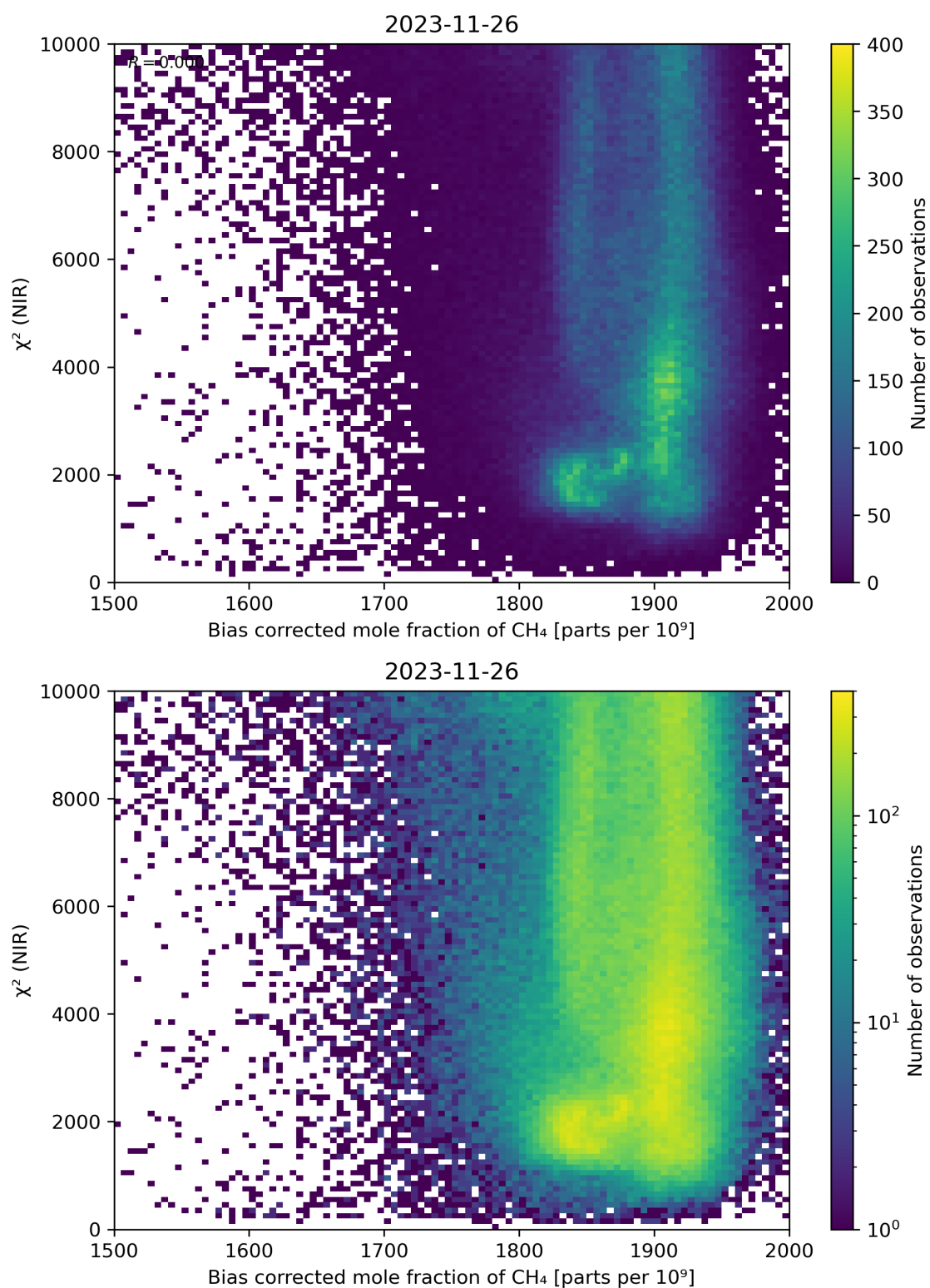
Figure 63: Scatter density plot of “Bias corrected mole fraction of CH 4 ” against “ \chi^2 (NIR)” for 2023-11-25 to 2023-11-27.
