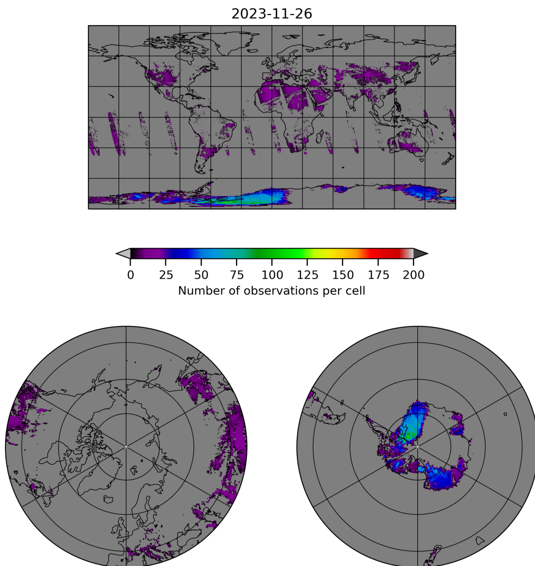
Figure 10: Map of the number of observations for 2023-11-25 to 2023-11-27
