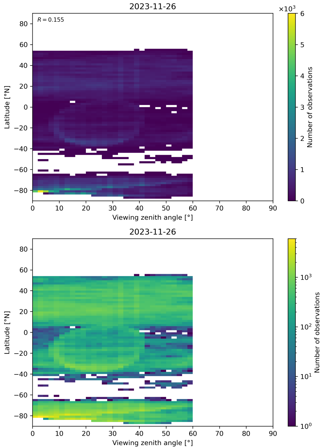
Figure 109: Scatter density plot of “Viewing zenith angle” against “Latitude” for 2023-11-25 to 2023-11-27.
