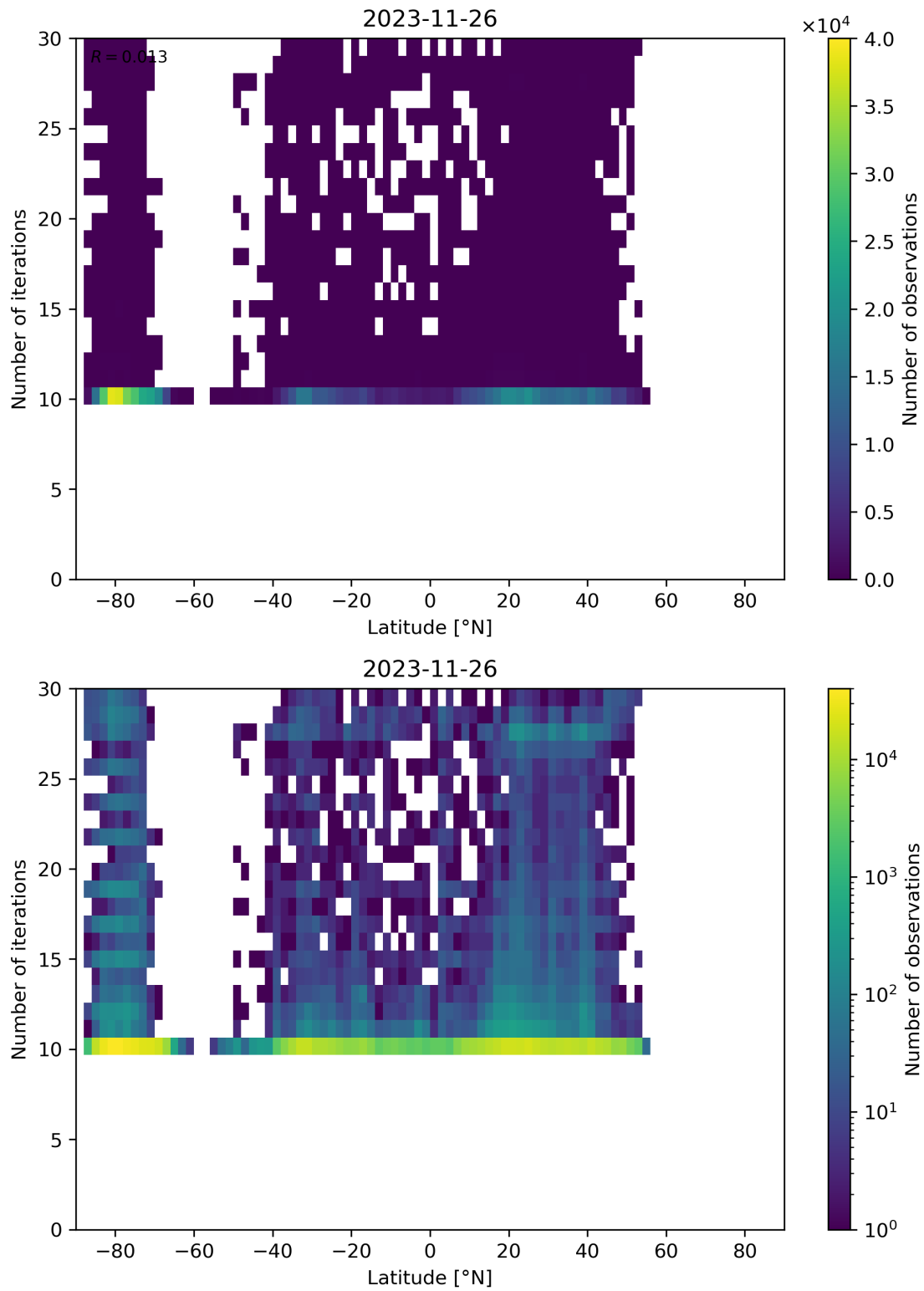
Figure 60: Scatter density plot of “Latitude” against “Number of iterations” for 2023-11-25 to 2023-11-27.
