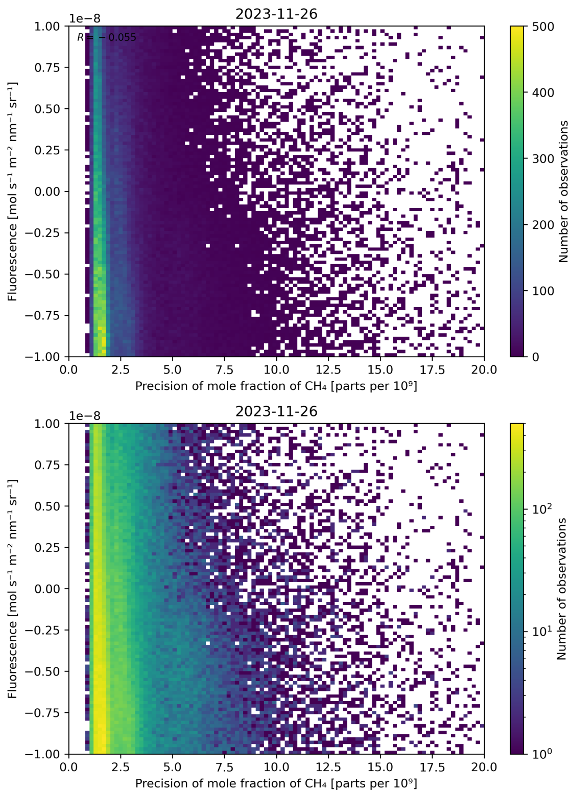
Figure 81: Scatter density plot of “Precision of mole fraction of \text{CH}_4 ” against “Fluorescence” for 2023-11-25 to 2023-11-27.
