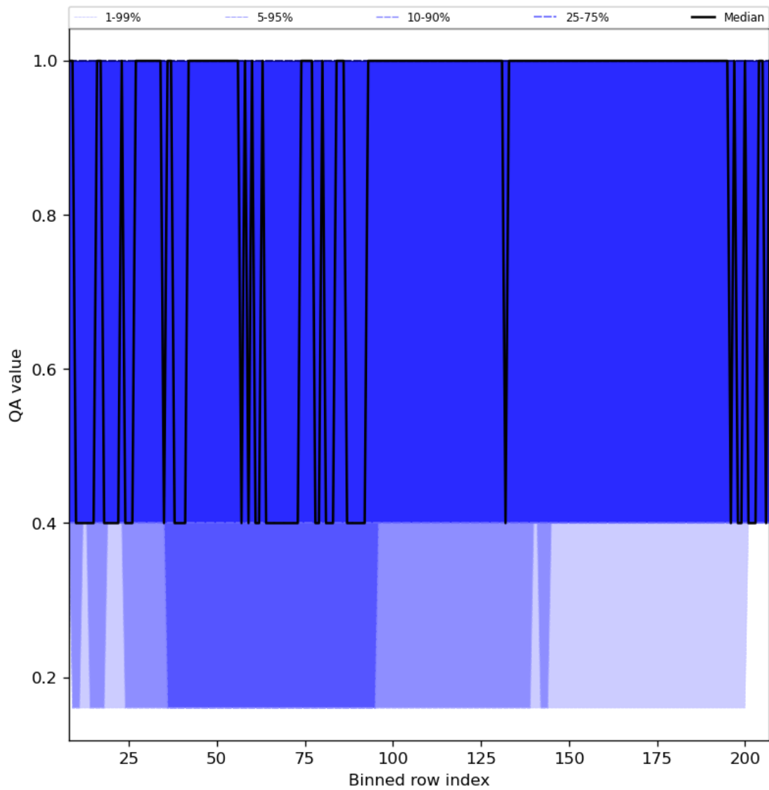
Figure 33: Along track statistics of “QA value” for 2023-11-25 to 2023-11-27
