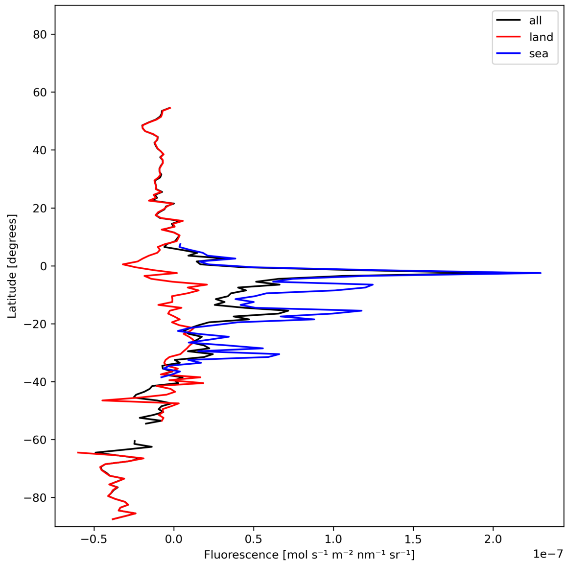
Figure 21: Zonal average of “Fluorescence” for 2023-11-25 to 2023-11-27.
