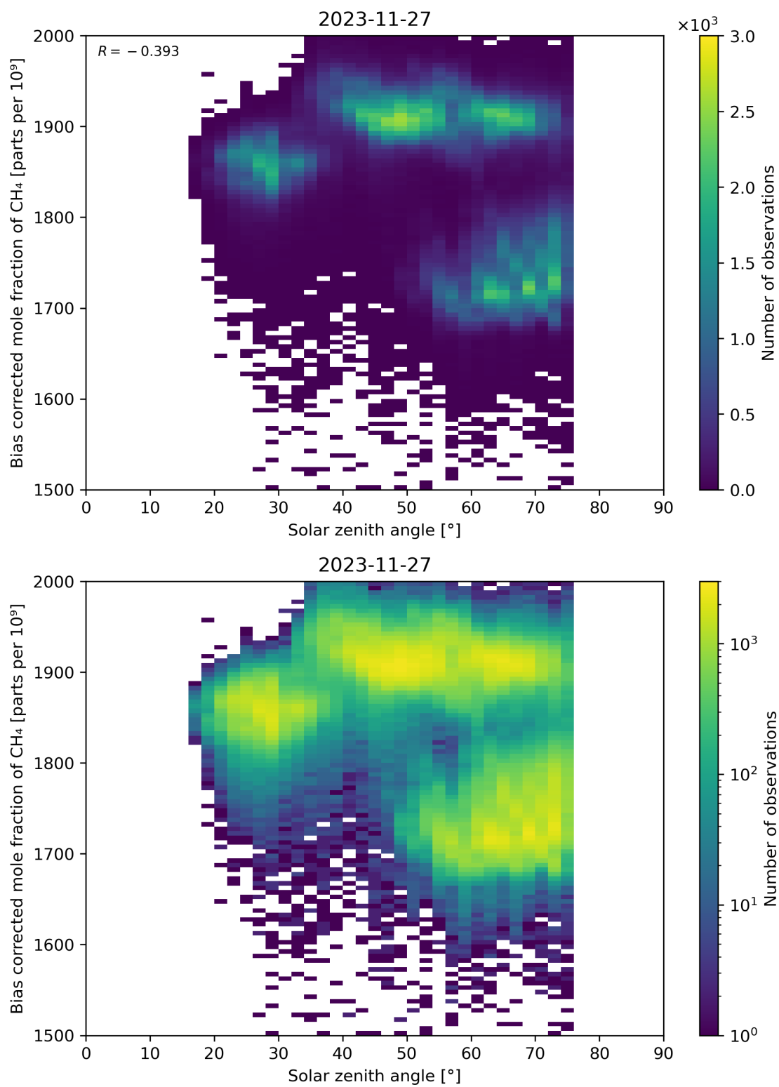
Figure 100: Scatter density plot of “Solar zenith angle” against “Bias corrected mole fraction of CH 4 ” for 2023-11-26 to 2023-11-28.
