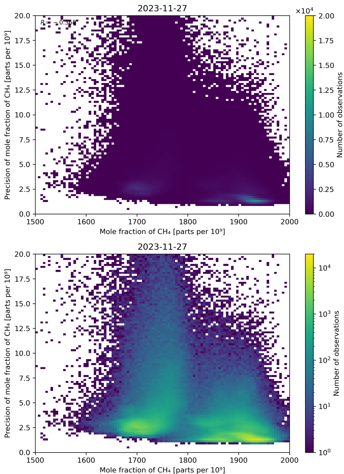
Figure 75: Scatter density plot of “Mole fraction of CH 4 ” against “Precision of mole fraction of CH 4 ” for 2023-11-26 to 2023-11-28.
