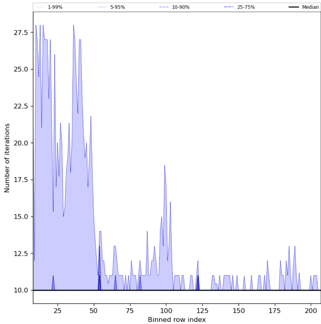
Figure 42: Along track statistics of “Number of iterations” for 2023-11-26 to 2023-11-28
