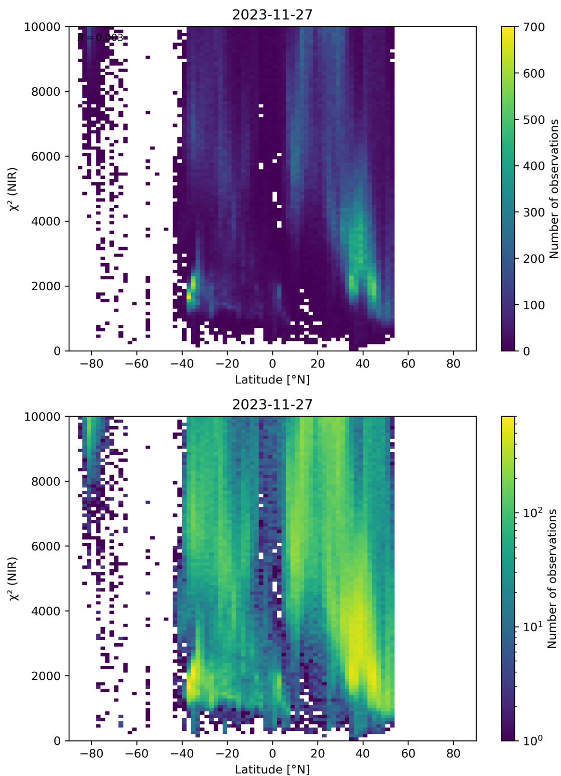
Figure 53: Scatter density plot of “Latitude” against “ \chi^2 (NIR)” for 2023-11-26 to 2023-11-28.
