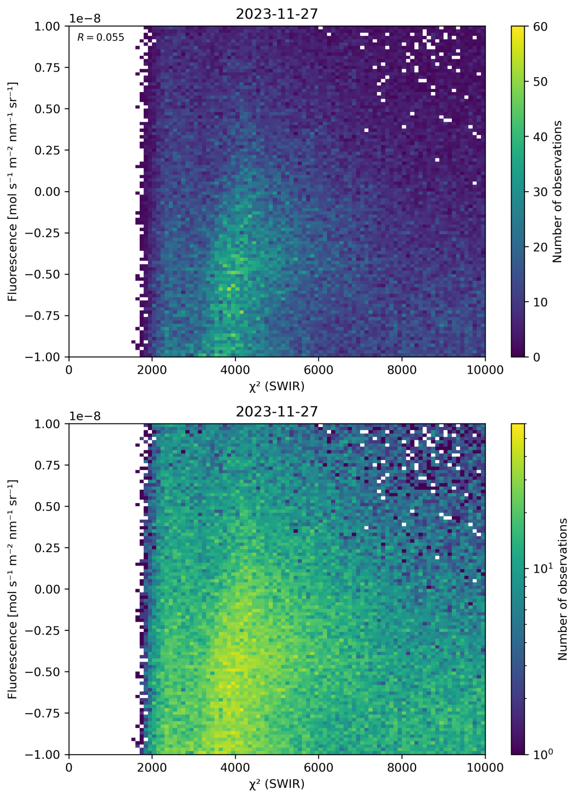
Figure 49: Scatter density plot of “ \chi^2 (SWIR)” against “Fluorescence” for 2023-11-26 to 2023-11-28.
