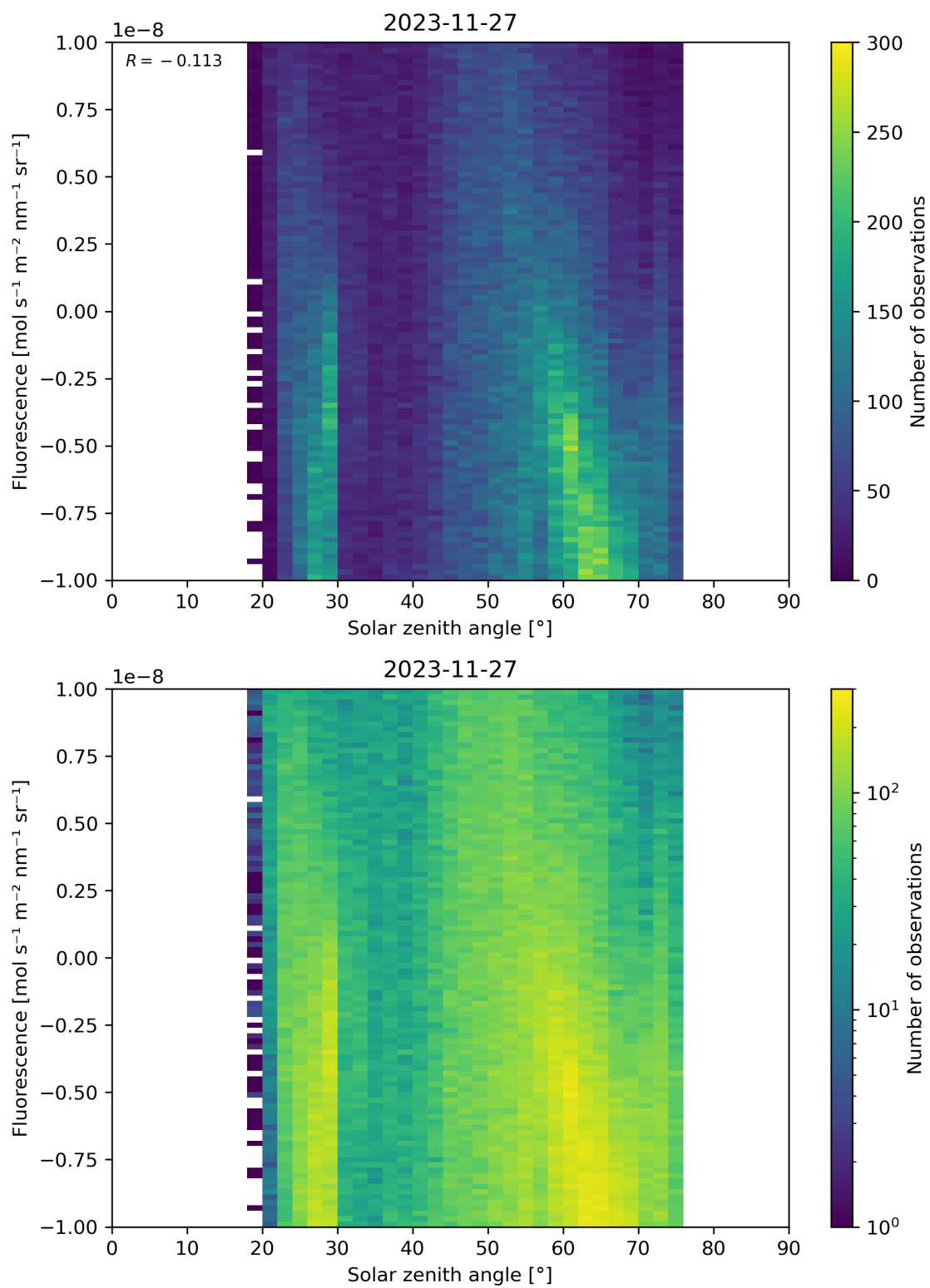
Figure 97: Scatter density plot of “Solar zenith angle” against “Fluorescence” for 2023-11-26 to 2023-11-28.
