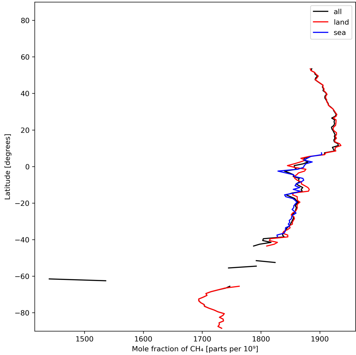
Figure 12: Zonal average of “Mole fraction of CH 4 ” for 2023-11-26 to 2023-11-28.
