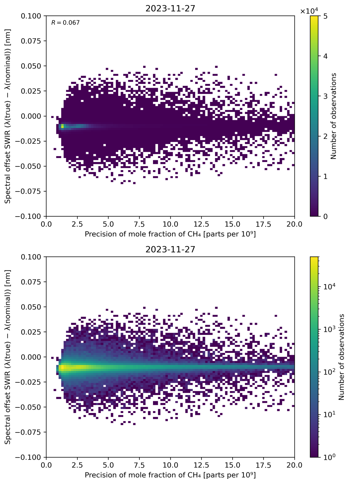
Figure 85: Scatter density plot of “Precision of mole fraction of \text{CH}_4 ” against “Spectral offset SWIR ( \lambda(\text{true}) - \lambda(\text{nominal}) )” for 2023-11-26 to 2023-11-28.
