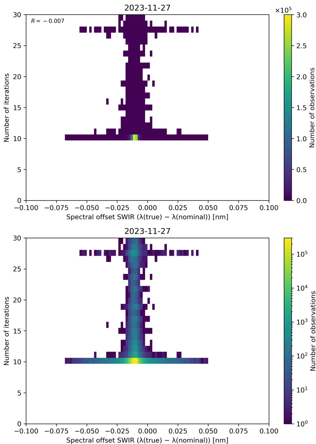
Figure 121: Scatter density plot of “Spectral offset SWIR ( \lambda(\text{true}) - \lambda(\text{nominal}) )” against “Number of iterations” for 2023-11-26 to 2023-11-28.
