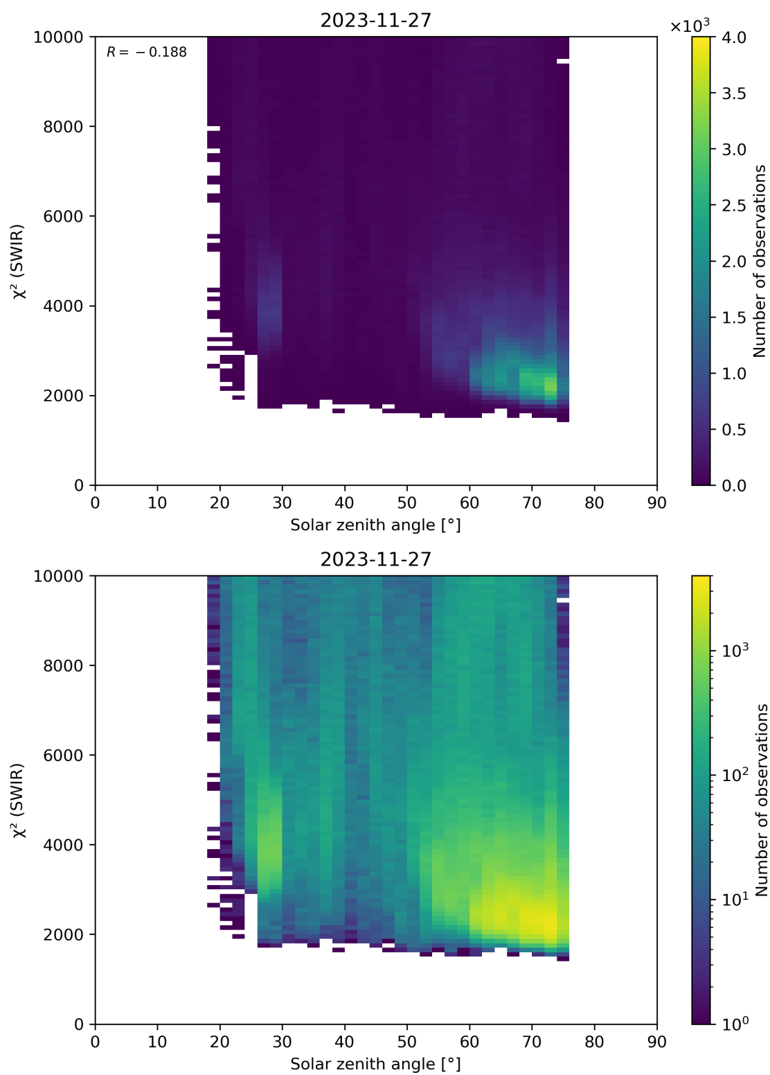
Figure 95: Scatter density plot of “Solar zenith angle” against “ \chi^2 (SWIR)” for 2023-11-26 to 2023-11-28.
