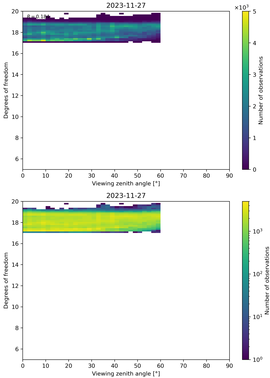
Figure 107: Scatter density plot of “Viewing zenith angle” against “Degrees of freedom” for 2023-11-26 to 2023-11-28.
