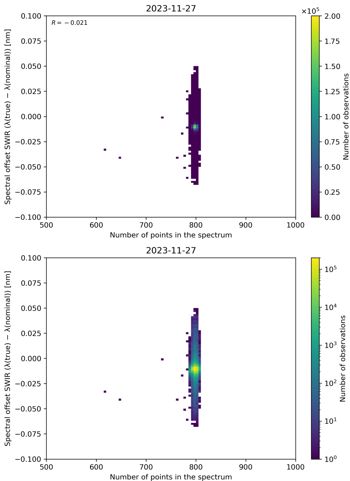
Figure 93: Scatter density plot of “Number of points in the spectrum” against “Spectral offset SWIR ( \lambda(\text{true}) - \lambda(\text{nominal}) )” for 2023-11-26 to 2023-11-28.
