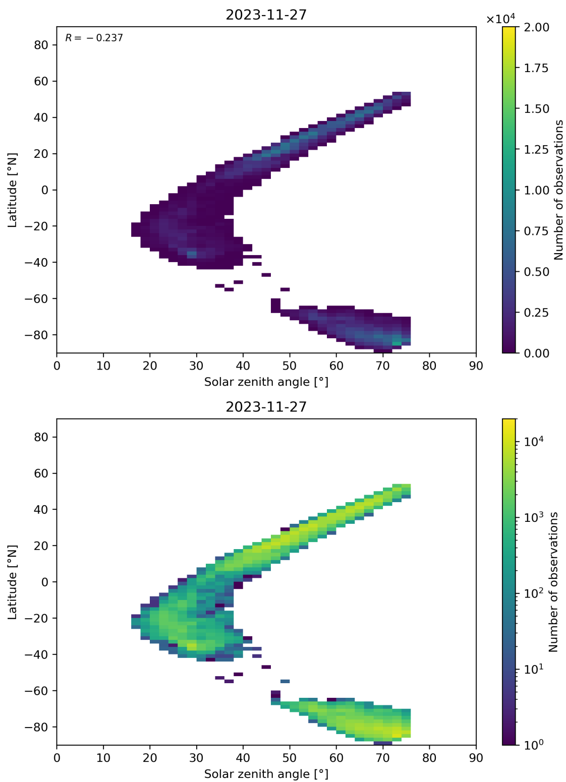
Figure 98: Scatter density plot of “Solar zenith angle” against “Latitude” for 2023-11-26 to 2023-11-28.
