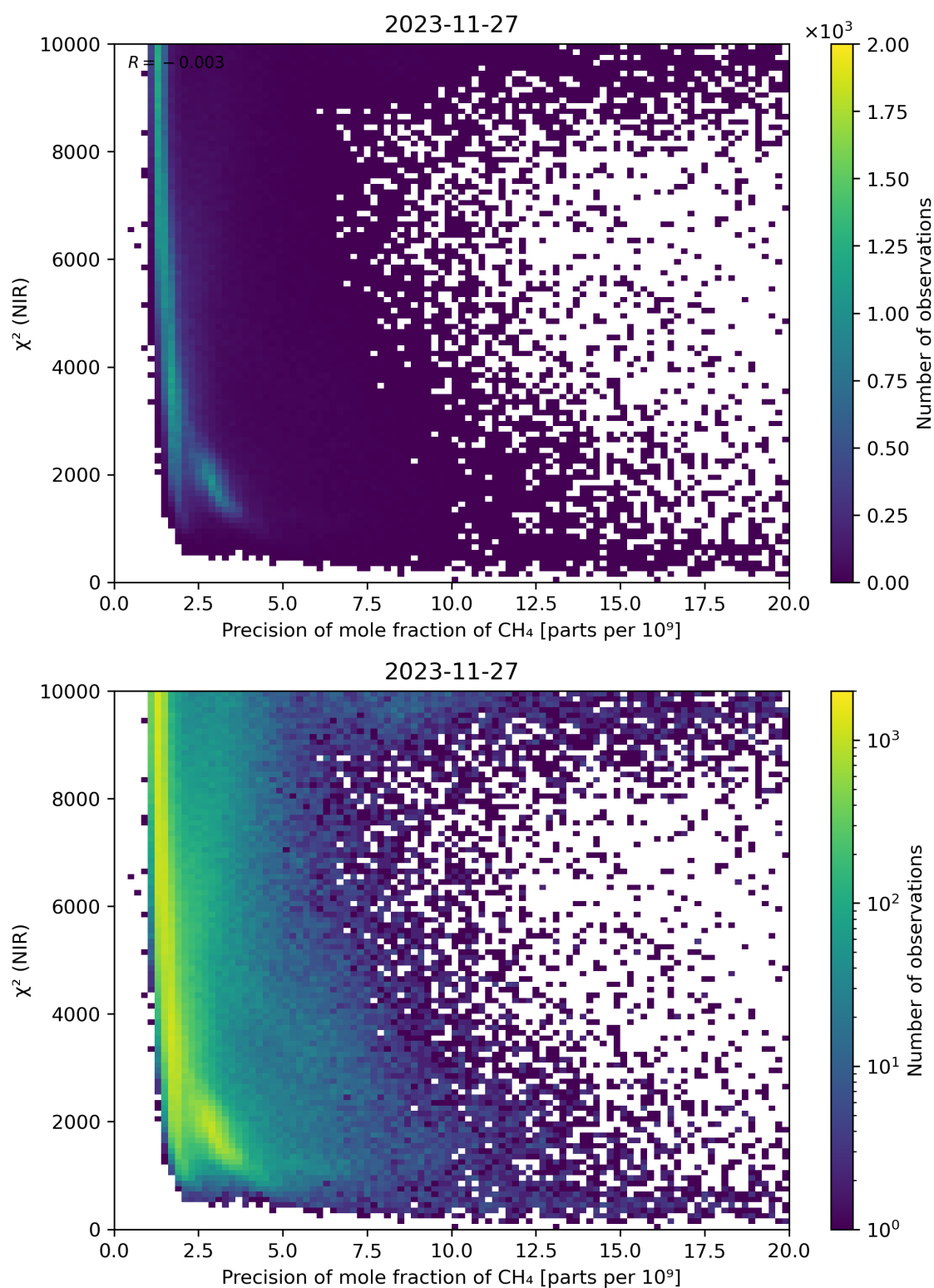
Figure 78: Scatter density plot of “Precision of mole fraction of CH 4 ” against “ \chi^2 (NIR)” for 2023-11-26 to 2023-11-28.
