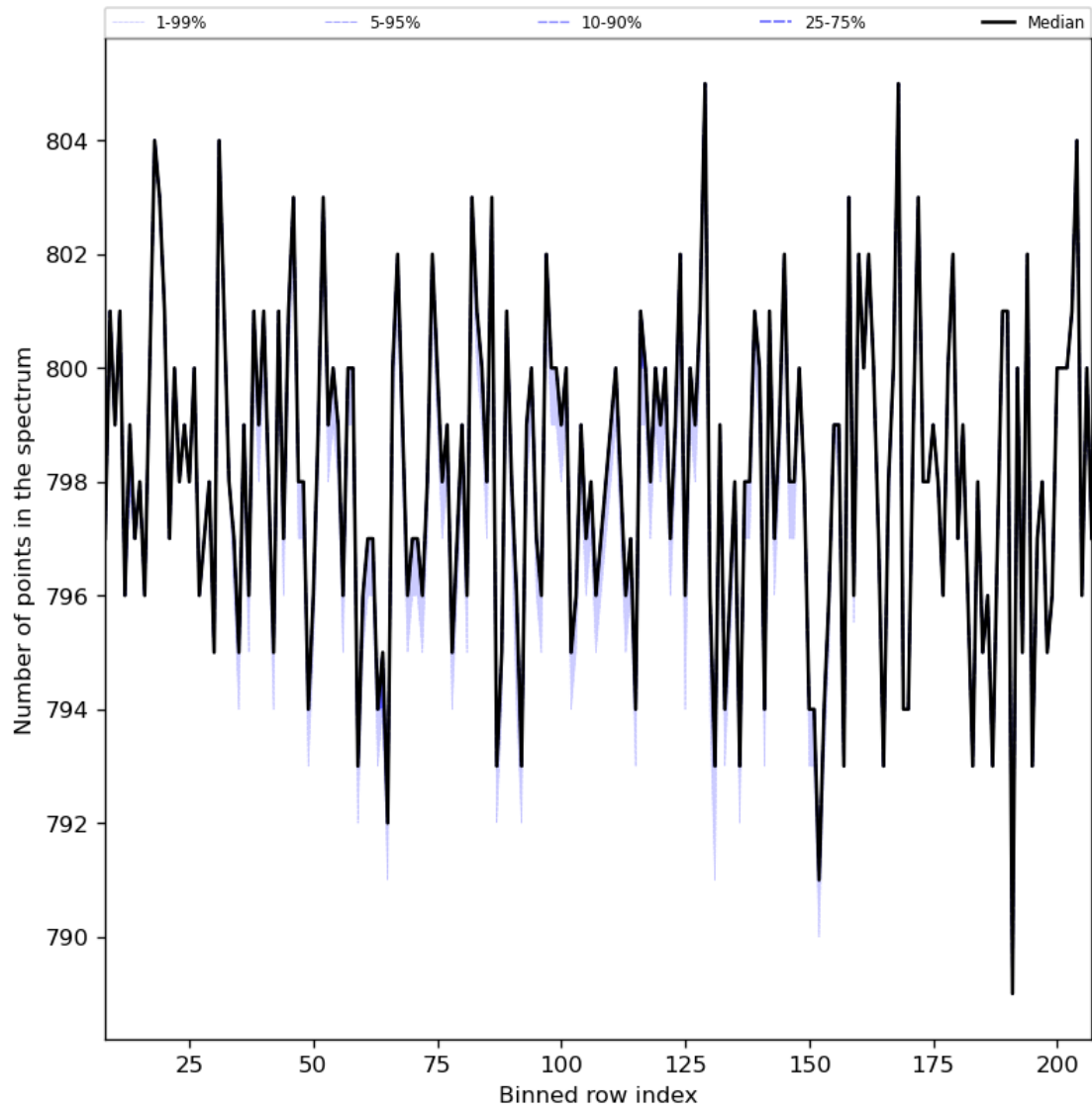
Figure 37: Along track statistics of “Number of points in the spectrum” for 2023-11-26 to 2023-11-28
