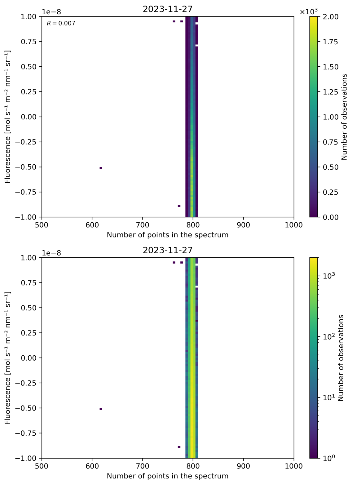
Figure 91: Scatter density plot of “Number of points in the spectrum” against “Fluorescence” for 2023-11-26 to 2023-11-28.
