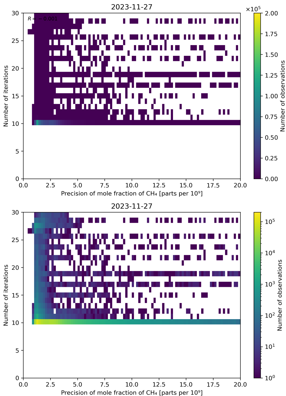
Figure 83: Scatter density plot of “Precision of mole fraction of CH 4 ” against “Number of iterations” for 2023-11-26 to 2023-11-28.
