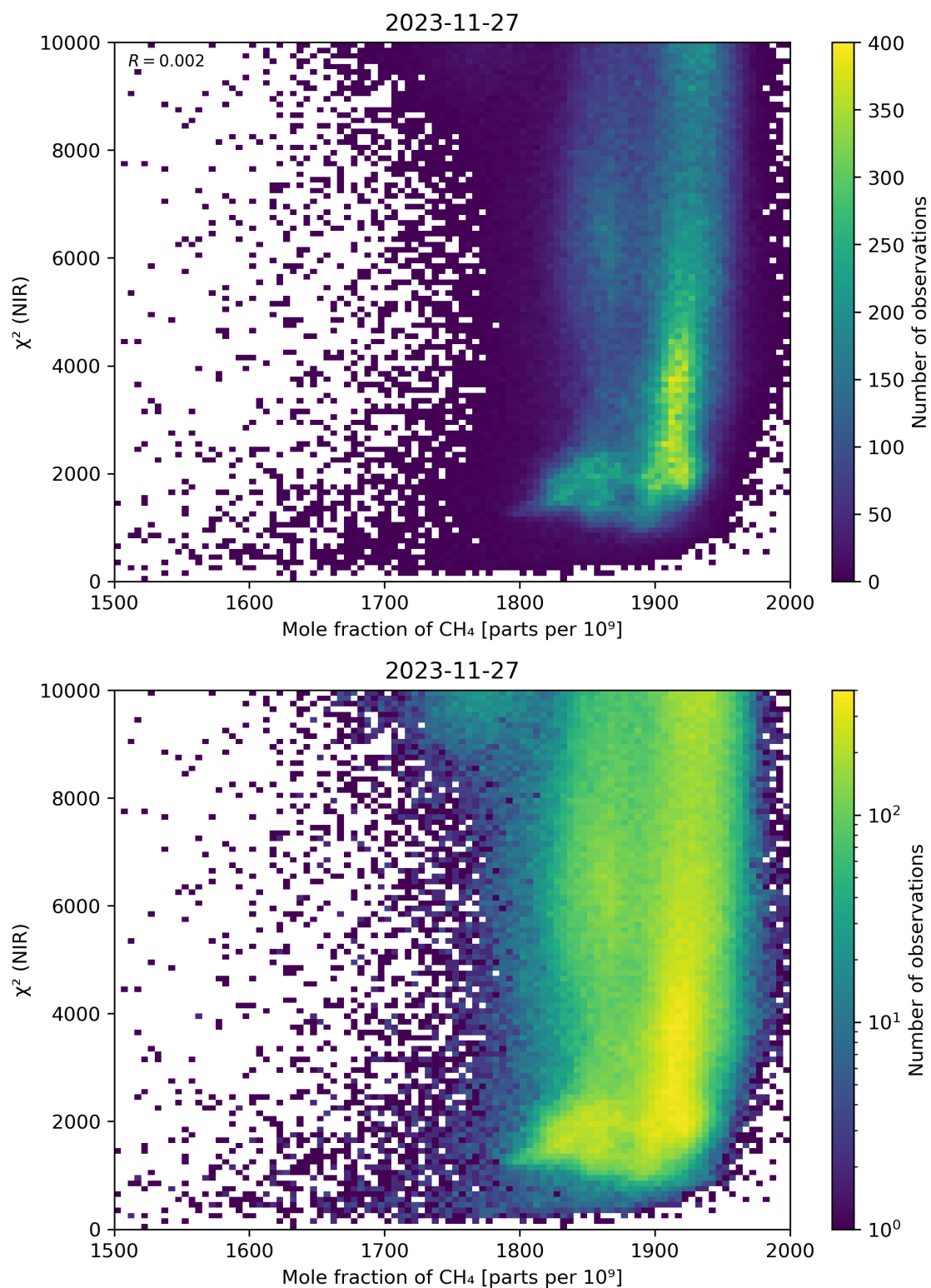
Figure 70: Scatter density plot of “Mole fraction of \text{CH}_4 ” against “ \chi^2 (NIR)” for 2023-11-26 to 2023-11-28.
