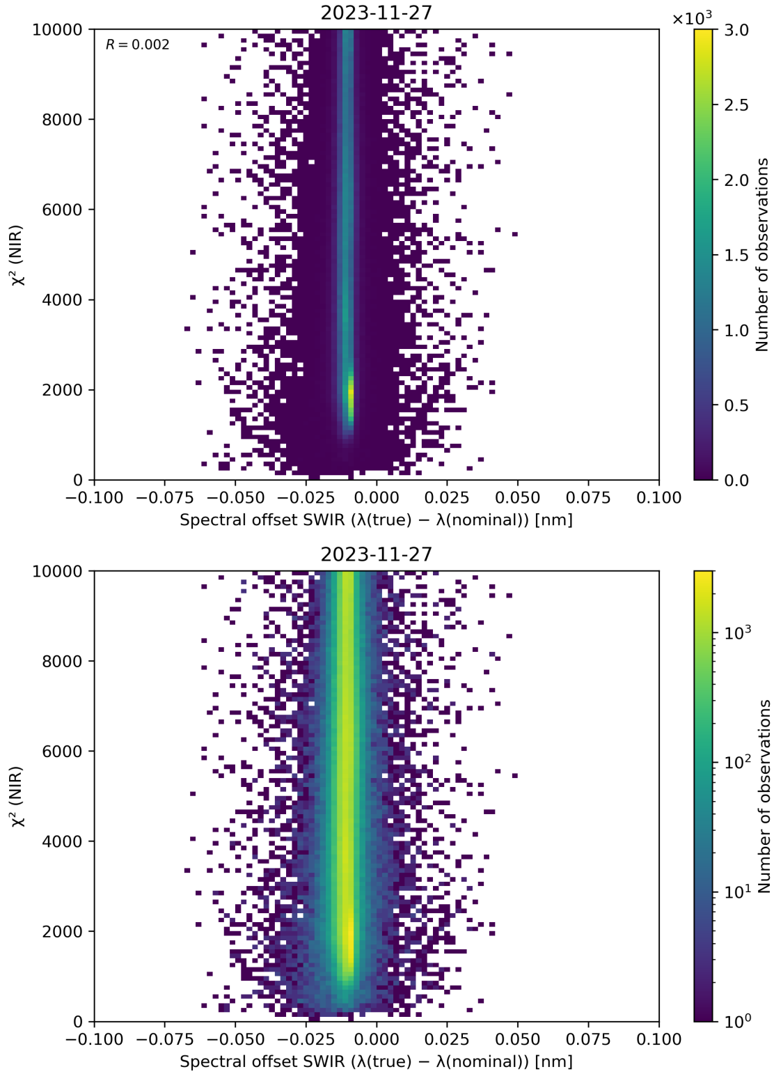
Figure 117: Scatter density plot of “Spectral offset SWIR ( \lambda(\text{true}) - \lambda(\text{nominal}) )” against “ \chi^2 (NIR)” for 2023-11-26 to 2023-11-28.
