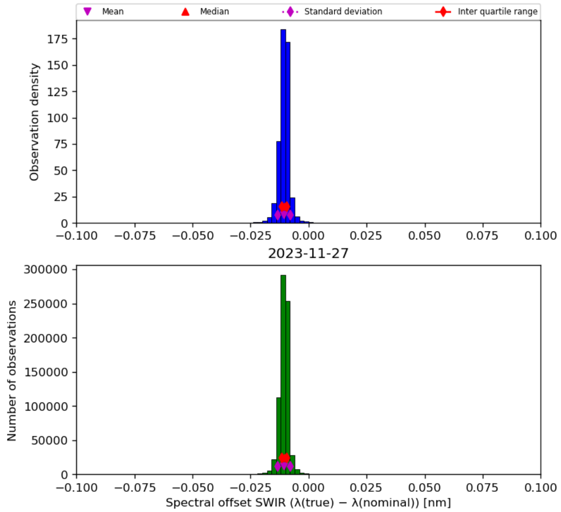
Figure 27: Histogram of “Spectral offset SWIR ( \lambda(\text{true}) - \lambda(\text{nominal}) )” for 2023-11-26 to 2023-11-28
