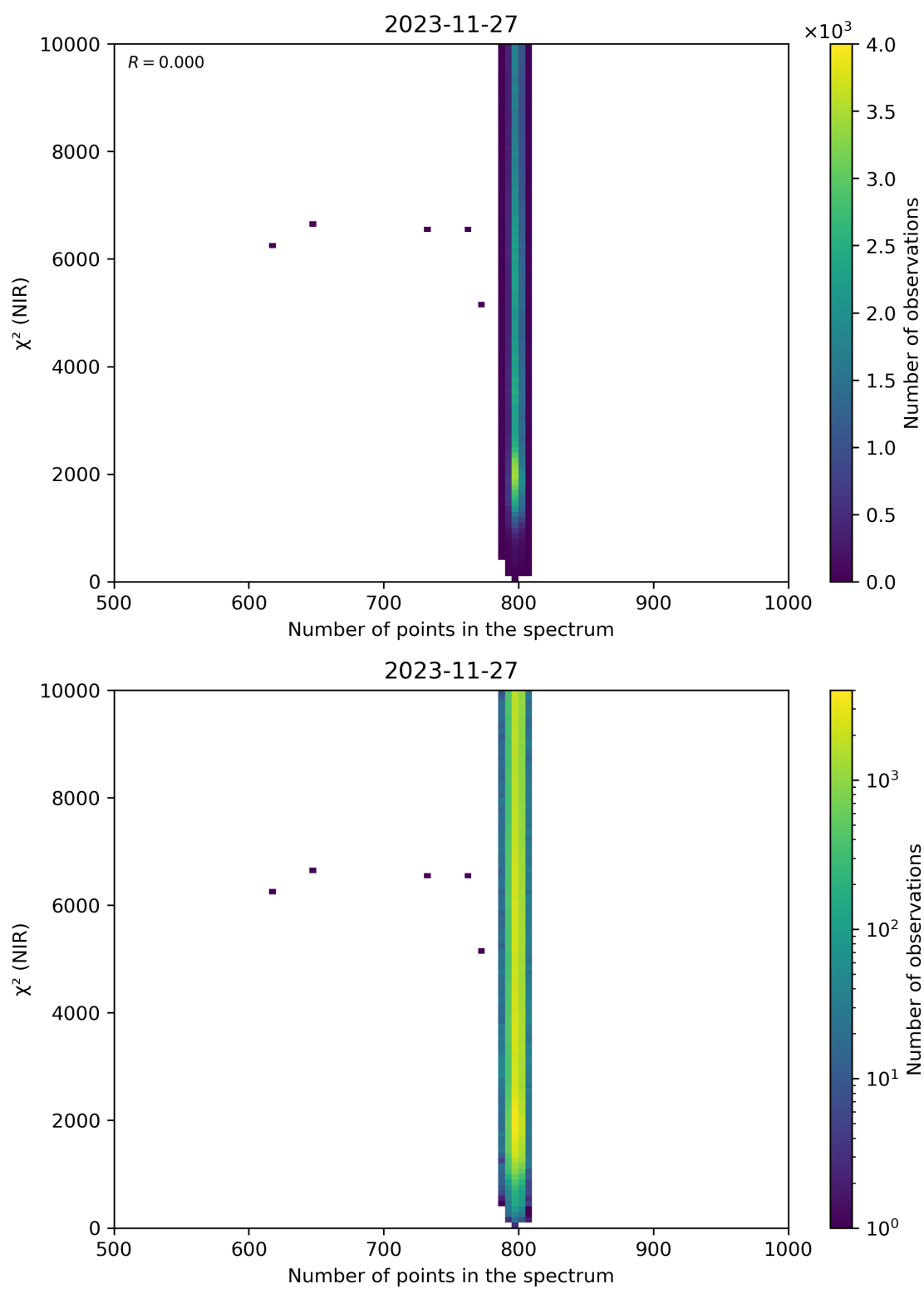
Figure 88: Scatter density plot of “Number of points in the spectrum” against “ \chi^2 (NIR)” for 2023-11-26 to 2023-11-28.
