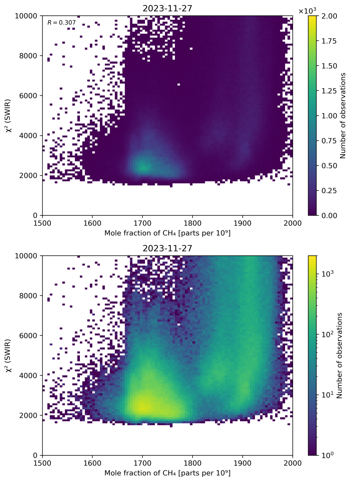
Figure 71: Scatter density plot of “Mole fraction of \text{CH}_4 ” against “ \chi^2 (SWIR)” for 2023-11-26 to 2023-11-28.
