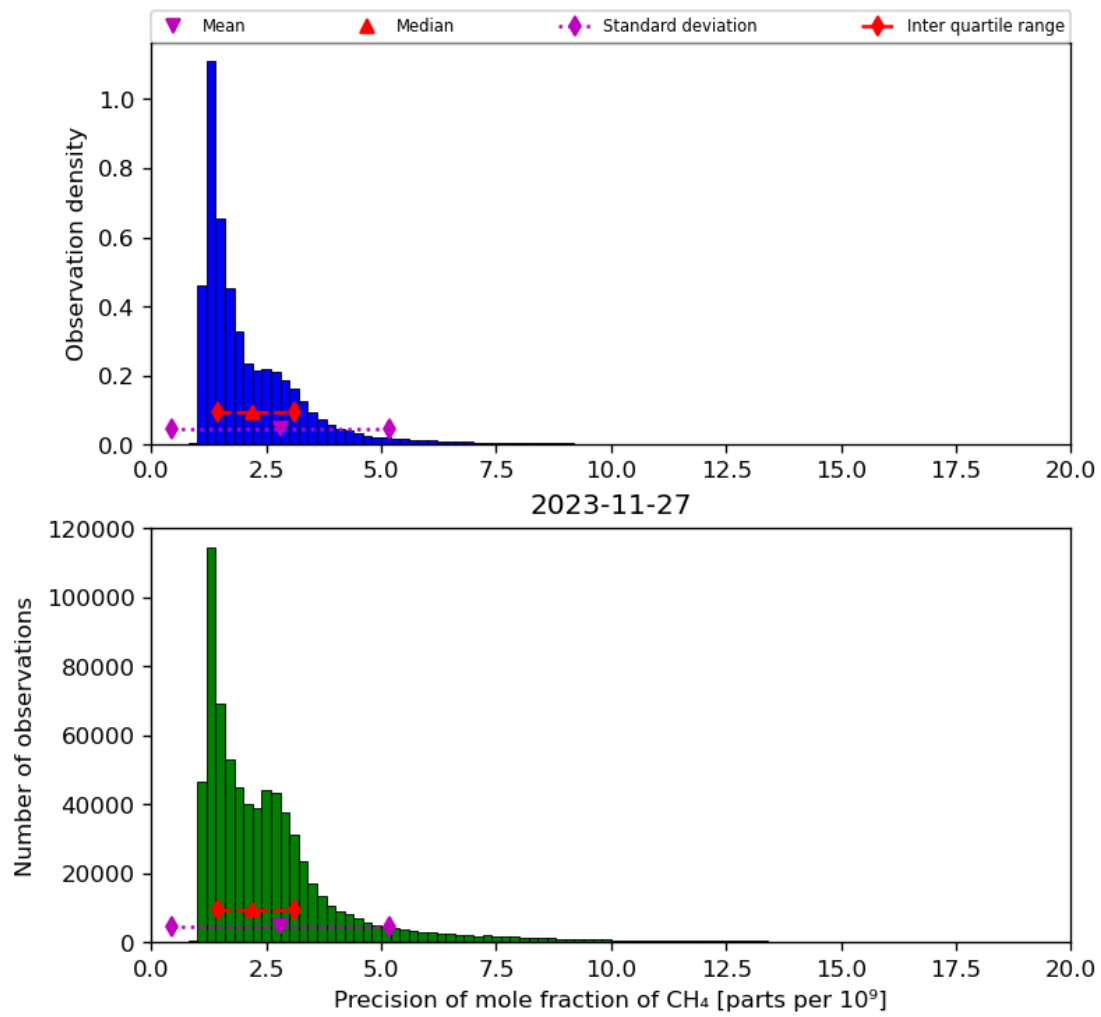
Figure 24: Histogram of “Precision of mole fraction of CH 4 ” for 2023-11-26 to 2023-11-28
