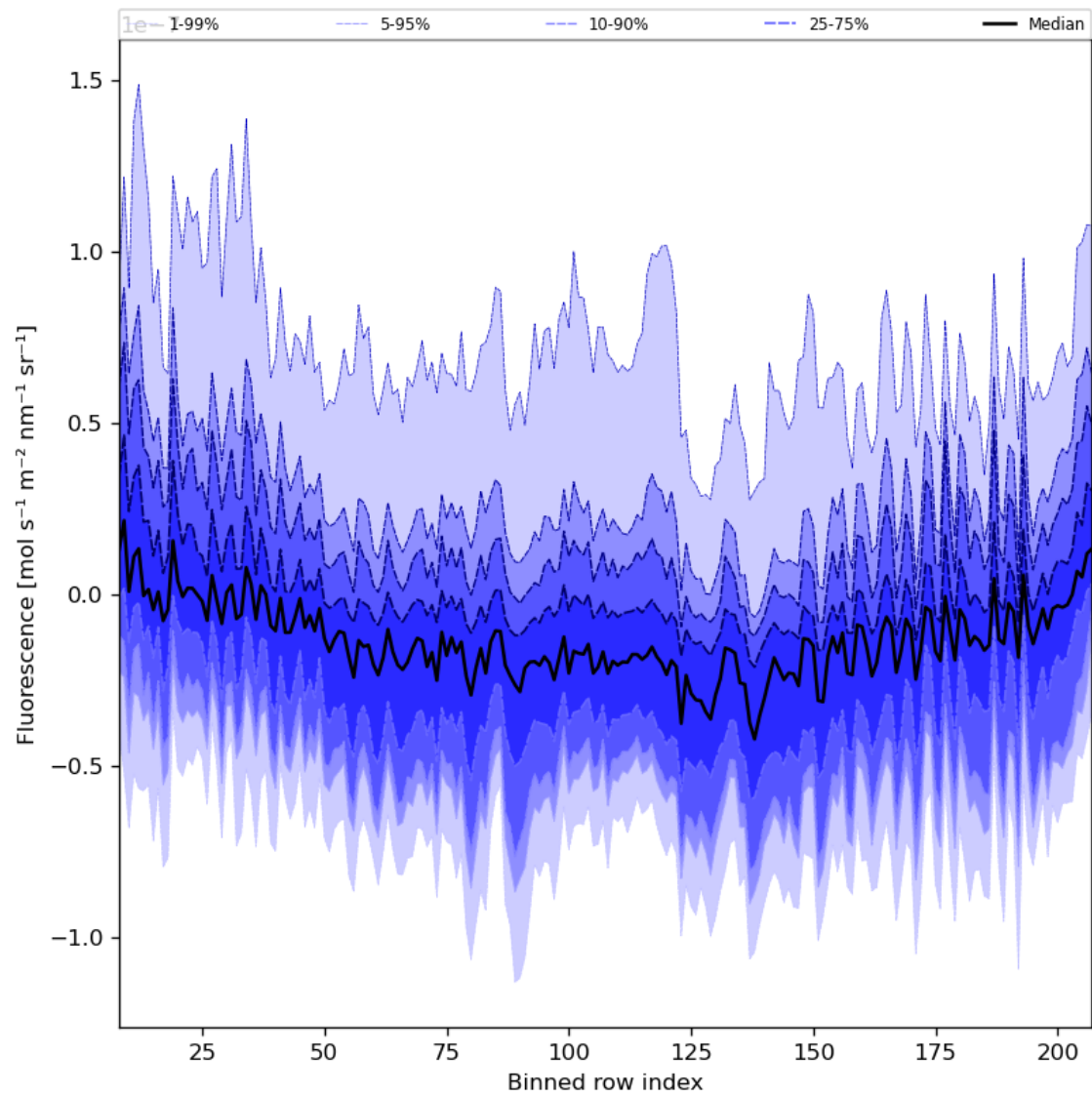
Figure 43: Along track statistics of “Fluorescence” for 2023-11-26 to 2023-11-28
