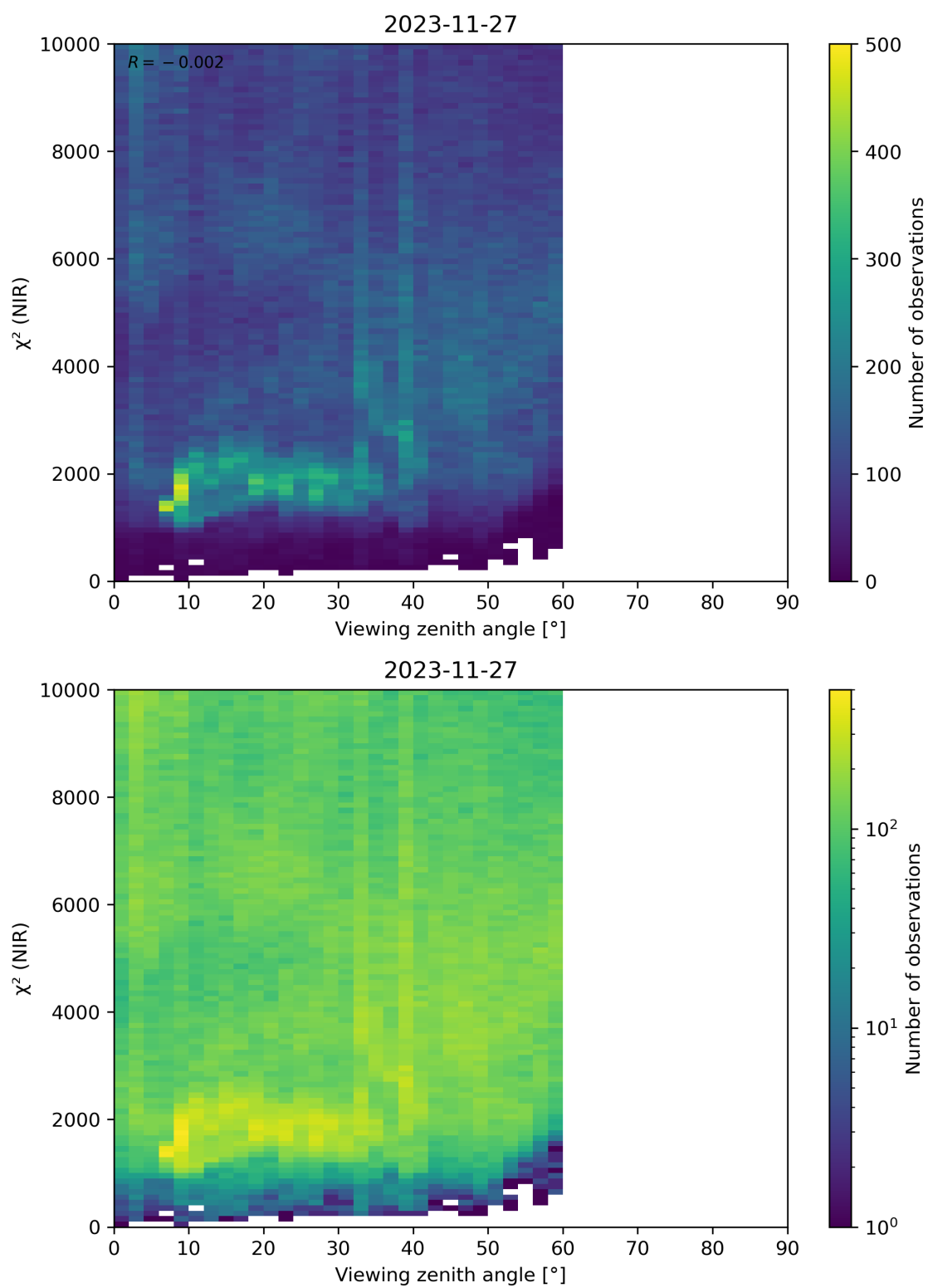
Figure 105: Scatter density plot of “Viewing zenith angle” against “ \chi^2 (NIR)” for 2023-11-26 to 2023-11-28.
