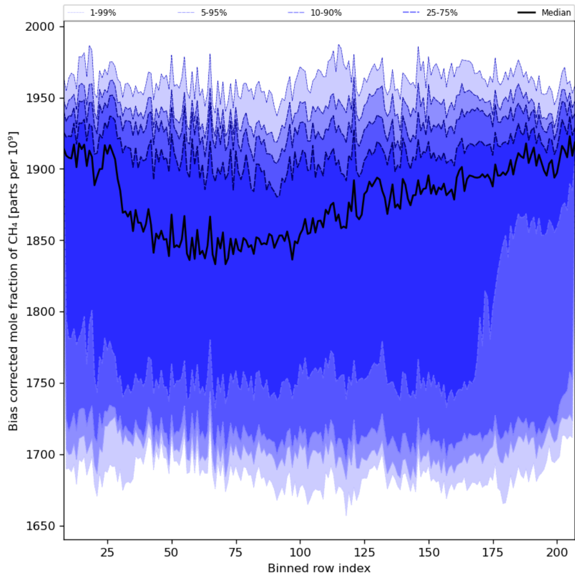
Figure 36: Along track statistics of “Bias corrected mole fraction of CH 4 ” for 2023-11-26 to 2023-11-28
