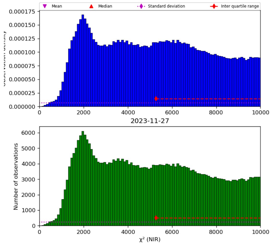
Figure 29: Histogram of “ \chi^2 (NIR)” for 2023-11-26 to 2023-11-28
