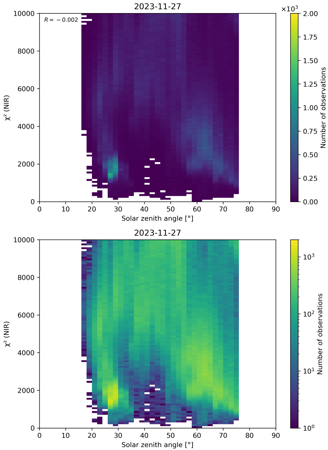
Figure 94: Scatter density plot of “Solar zenith angle” against “ \chi^2 (NIR)” for 2023-11-26 to 2023-11-28.
