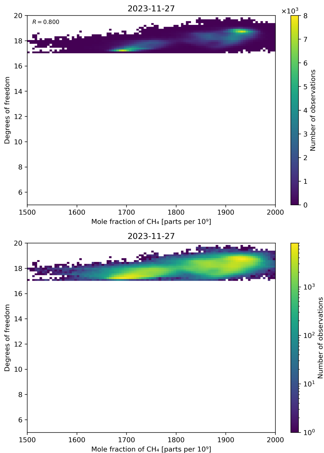
Figure 72: Scatter density plot of “Mole fraction of CH 4 ” against “Degrees of freedom” for 2023-11-26 to 2023-11-28.
