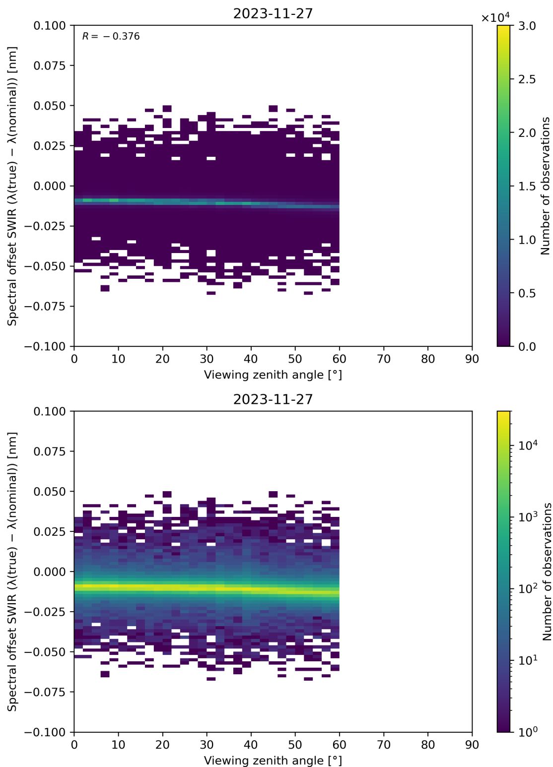
Figure 116: Scatter density plot of “Viewing zenith angle” against “Spectral offset SWIR ( \lambda(\text{true}) - \lambda(\text{nominal}) )” for 2023-11-26 to 2023-11-28.
