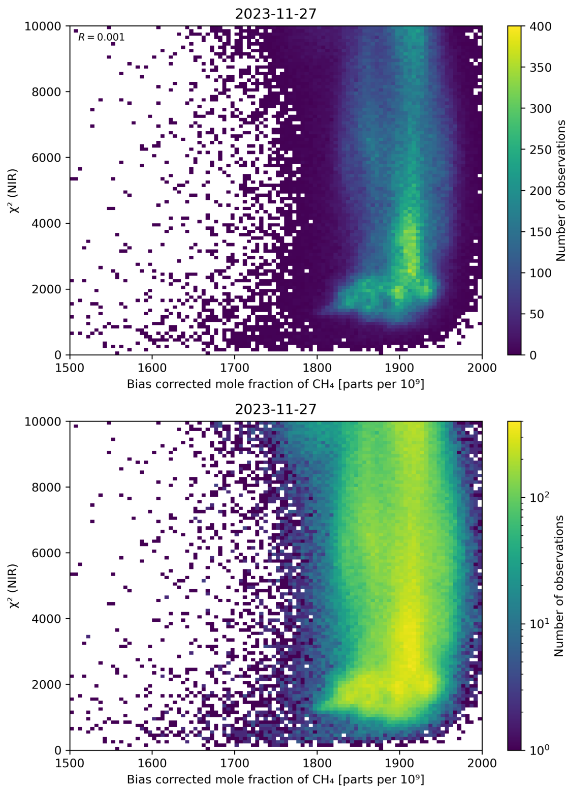
Figure 63: Scatter density plot of “Bias corrected mole fraction of CH 4 ” against “ \chi^2 (NIR)” for 2023-11-26 to 2023-11-28.
