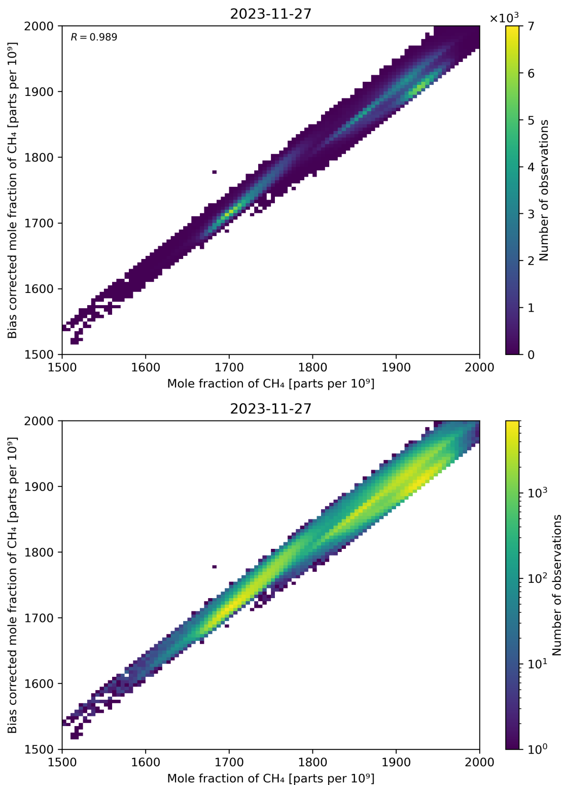
Figure 74: Scatter density plot of “Mole fraction of CH 4 ” against “Bias corrected mole fraction of CH 4 ” for 2023-11-26 to 2023-11-28.
