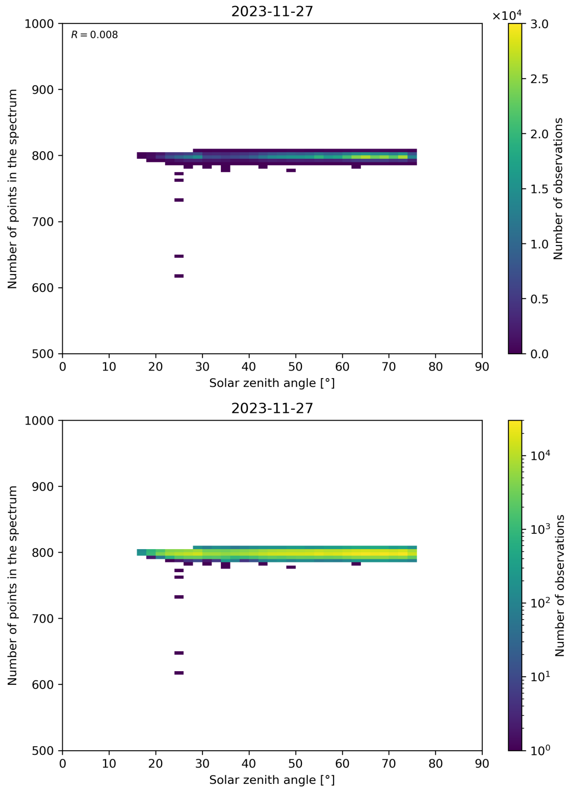
Figure 103: Scatter density plot of “Solar zenith angle” against “Number of points in the spectrum” for 2023-11-26 to 2023-11-28.
