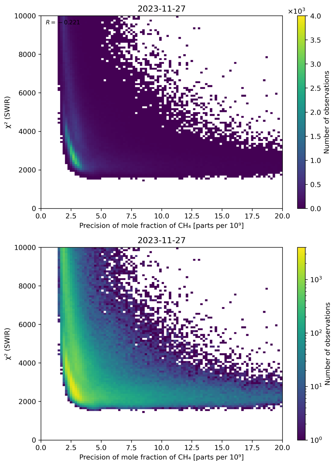
Figure 79: Scatter density plot of “Precision of mole fraction of \text{CH}_4 ” against “ \chi^2 (SWIR)” for 2023-11-26 to 2023-11-28.
