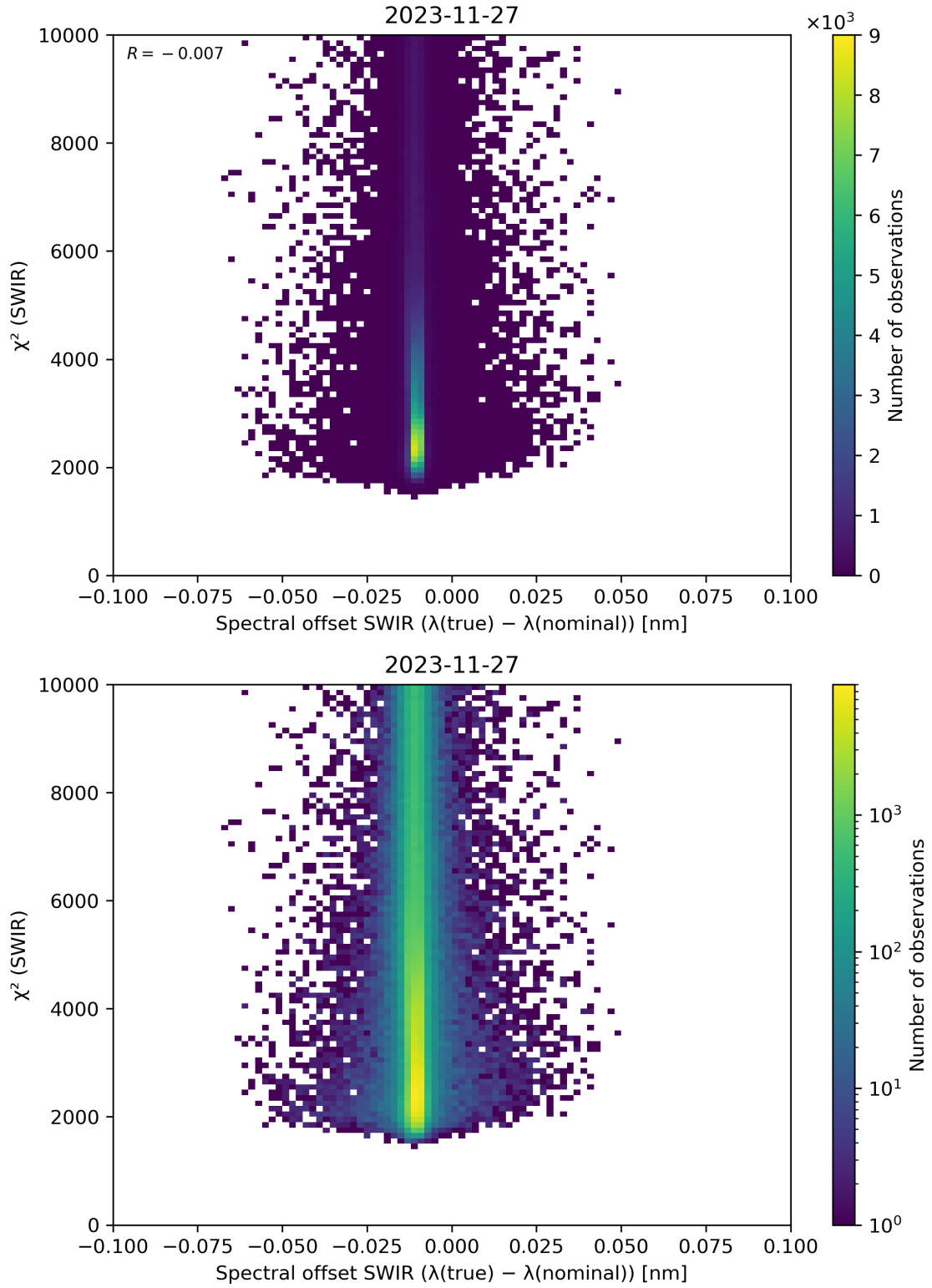
Figure 118: Scatter density plot of “Spectral offset SWIR ( \lambda(\text{true}) - \lambda(\text{nominal}) )” against “ \chi^2 (SWIR)” for 2023-11-26 to 2023-11-28.
