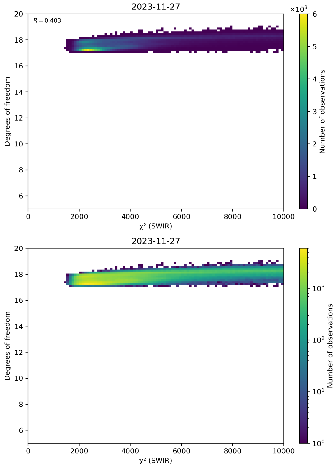
Figure 48: Scatter density plot of “ \chi^2 (SWIR)” against “Degrees of freedom” for 2023-11-26 to 2023-11-28.
