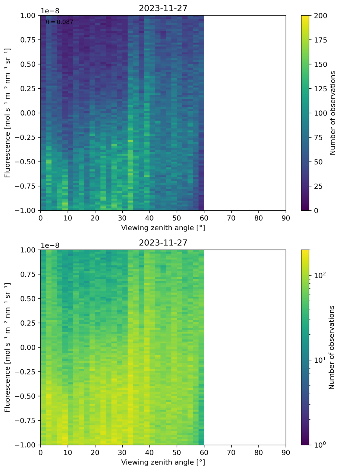
Figure 108: Scatter density plot of “Viewing zenith angle” against “Fluorescence” for 2023-11-26 to 2023-11-28.
