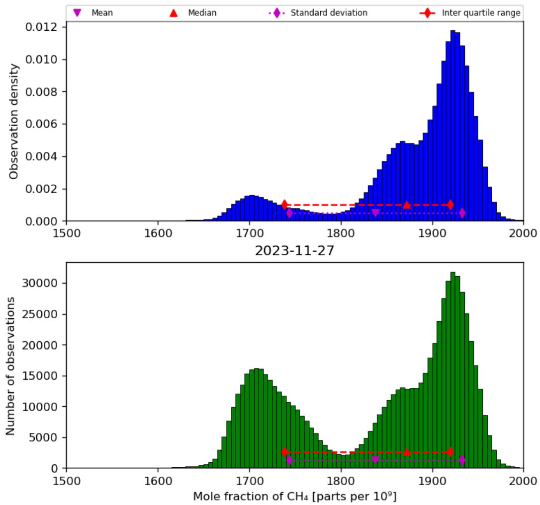
Figure 23: Histogram of “Mole fraction of CH 4 ” for 2023-11-26 to 2023-11-28
