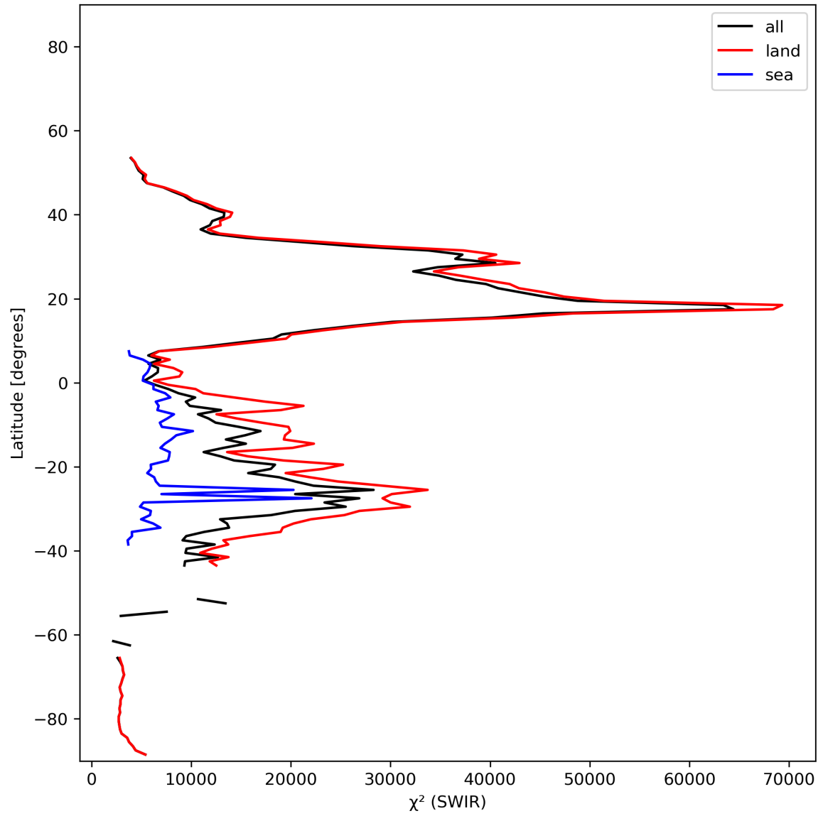
Figure 17: Zonal average of “ \chi^2 (SWIR)” for 2023-11-26 to 2023-11-28.
