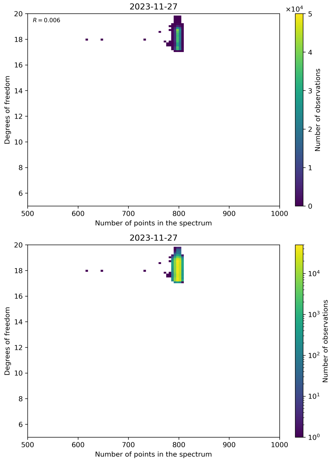
Figure 90: Scatter density plot of “Number of points in the spectrum” against “Degrees of freedom” for 2023-11-26 to 2023-11-28.
