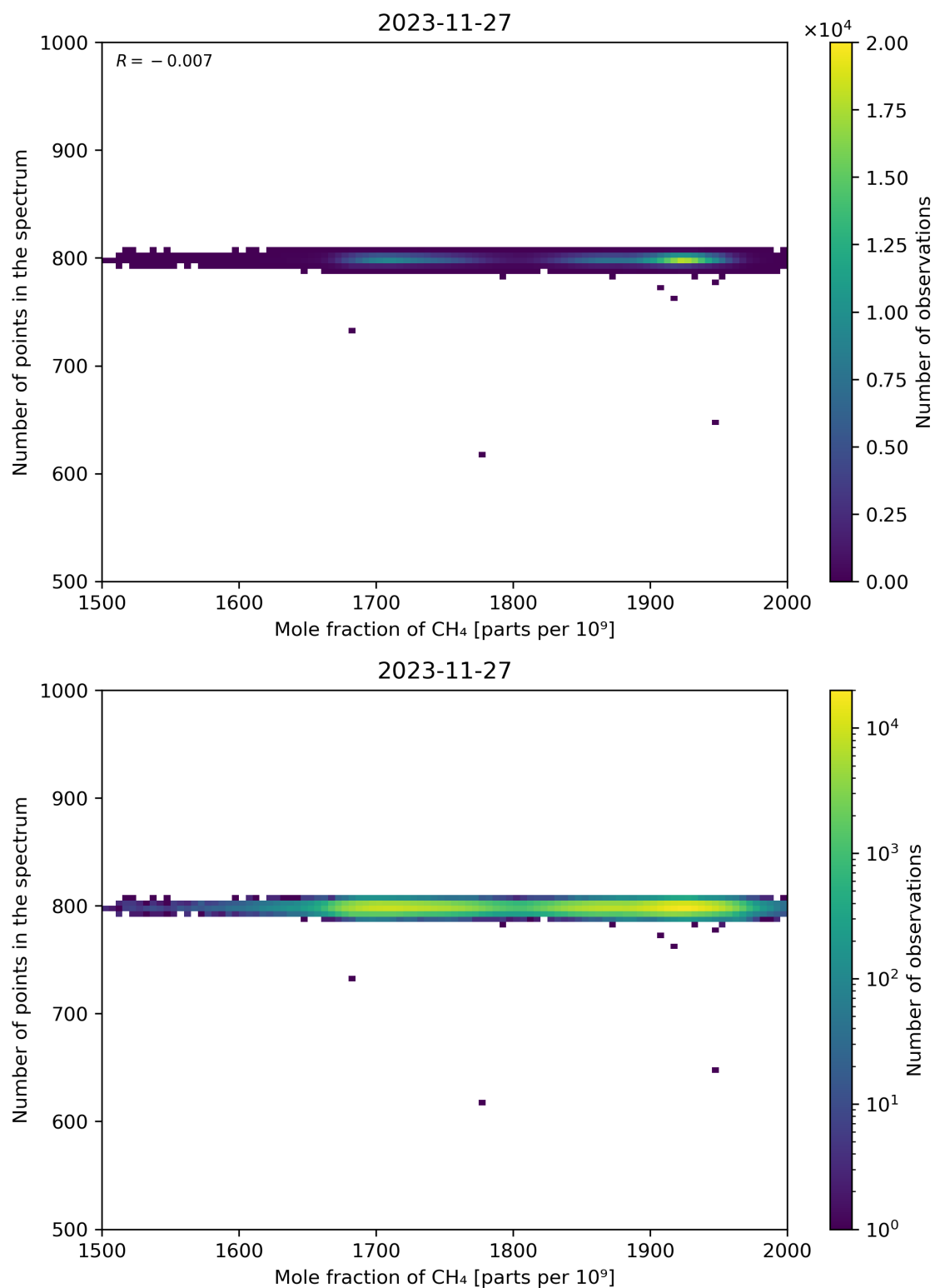
Figure 77: Scatter density plot of “Mole fraction of CH 4 ” against “Number of points in the spectrum” for 2023-11-26 to 2023-11-28.
