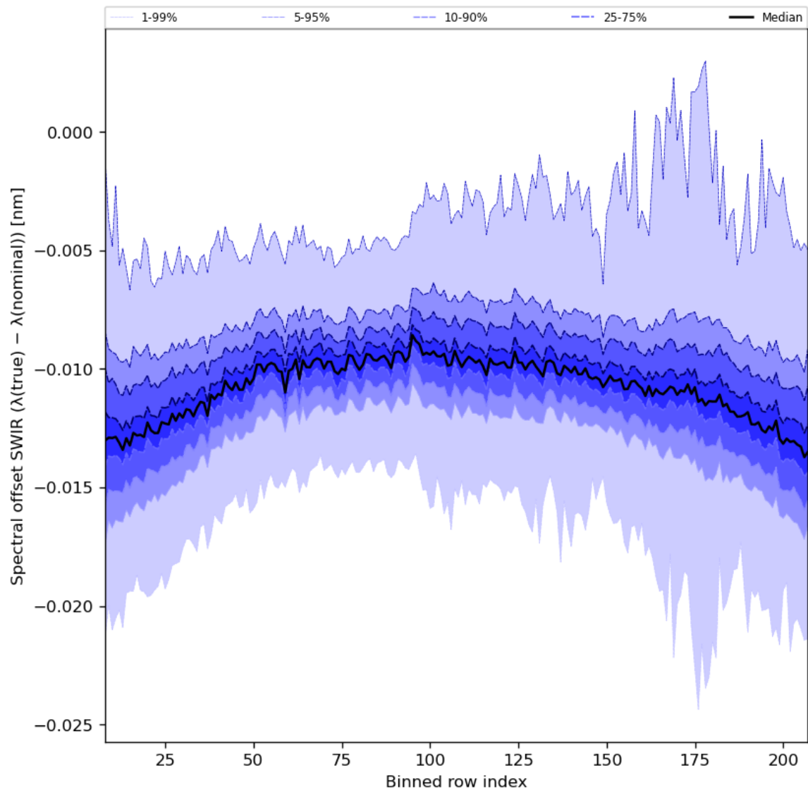
Figure 38: Along track statistics of “Spectral offset SWIR ( \lambda(\text{true}) - \lambda(\text{nominal}) )” for 2023-11-26 to 2023-11-28
