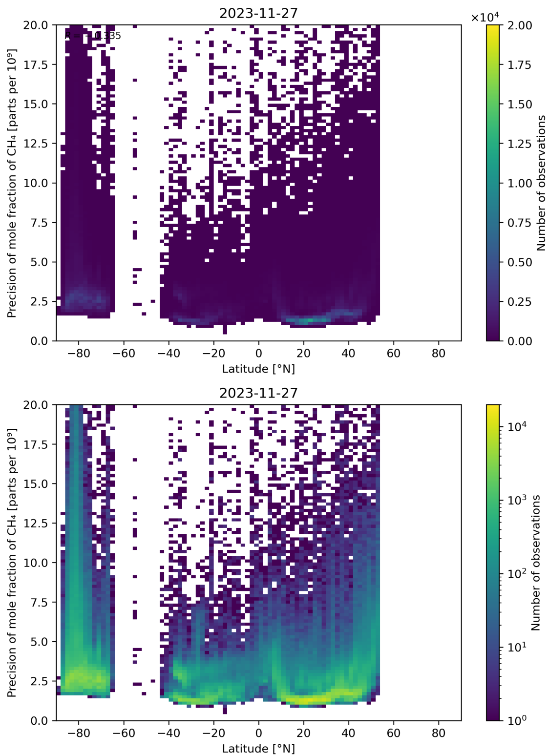
Figure 59: Scatter density plot of “Latitude” against “Precision of mole fraction of CH 4 ” for 2023-11-26 to 2023-11-28.
