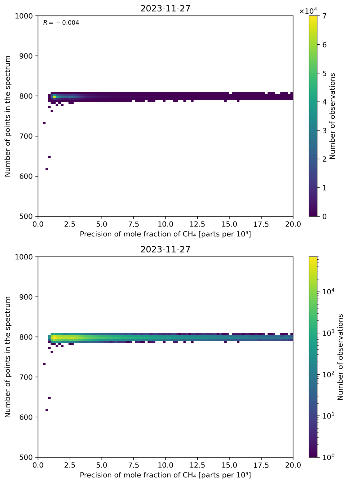
Figure 84: Scatter density plot of “Precision of mole fraction of CH 4 ” against “Number of points in the spectrum” for 2023-11-26 to 2023-11-28.
