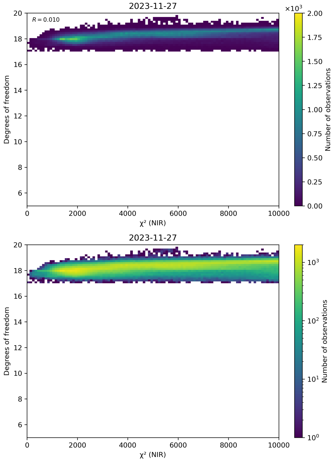
Figure 44: Scatter density plot of “ \chi^2 (NIR)” against “Degrees of freedom” for 2023-11-26 to 2023-11-28.
