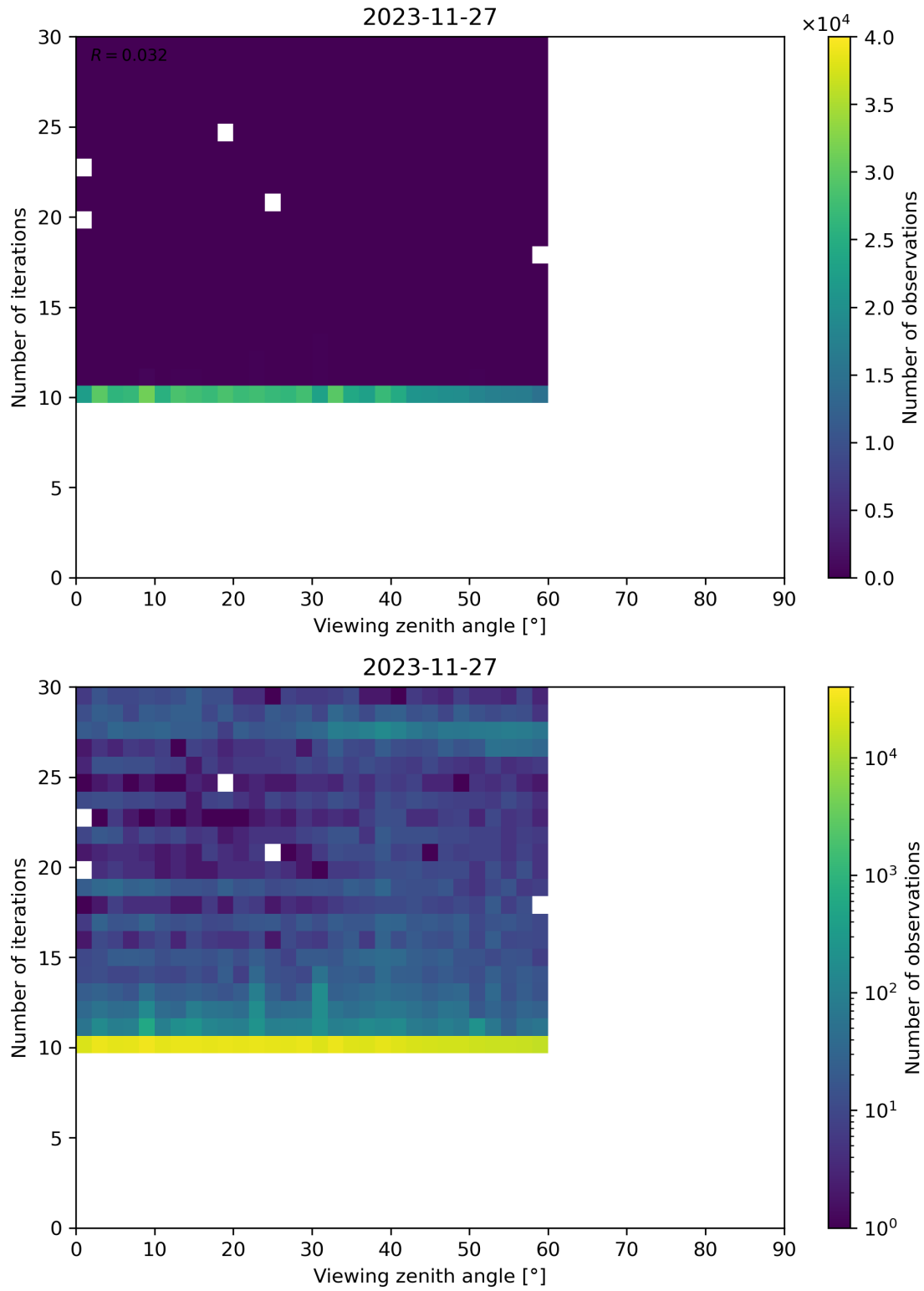
Figure 113: Scatter density plot of “Viewing zenith angle” against “Number of iterations” for 2023-11-26 to 2023-11-28.
