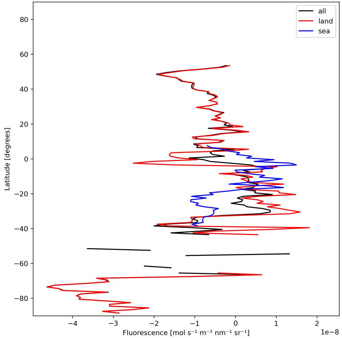
Figure 21: Zonal average of “Fluorescence” for 2023-11-26 to 2023-11-28.
