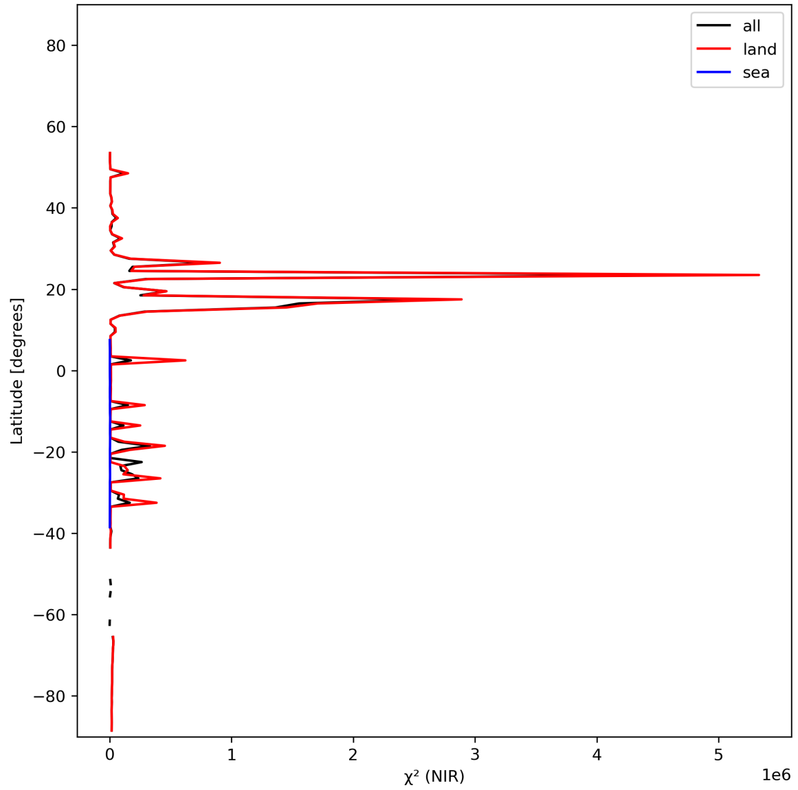
Figure 18: Zonal average of “ \chi^2 (NIR)” for 2023-11-26 to 2023-11-28.
