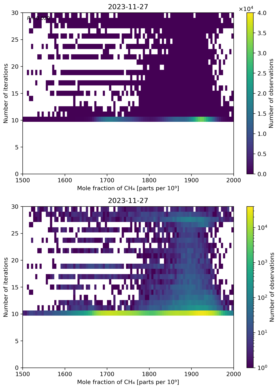
Figure 76: Scatter density plot of “Mole fraction of CH 4 ” against “Number of iterations” for 2023-11-26 to 2023-11-28.
