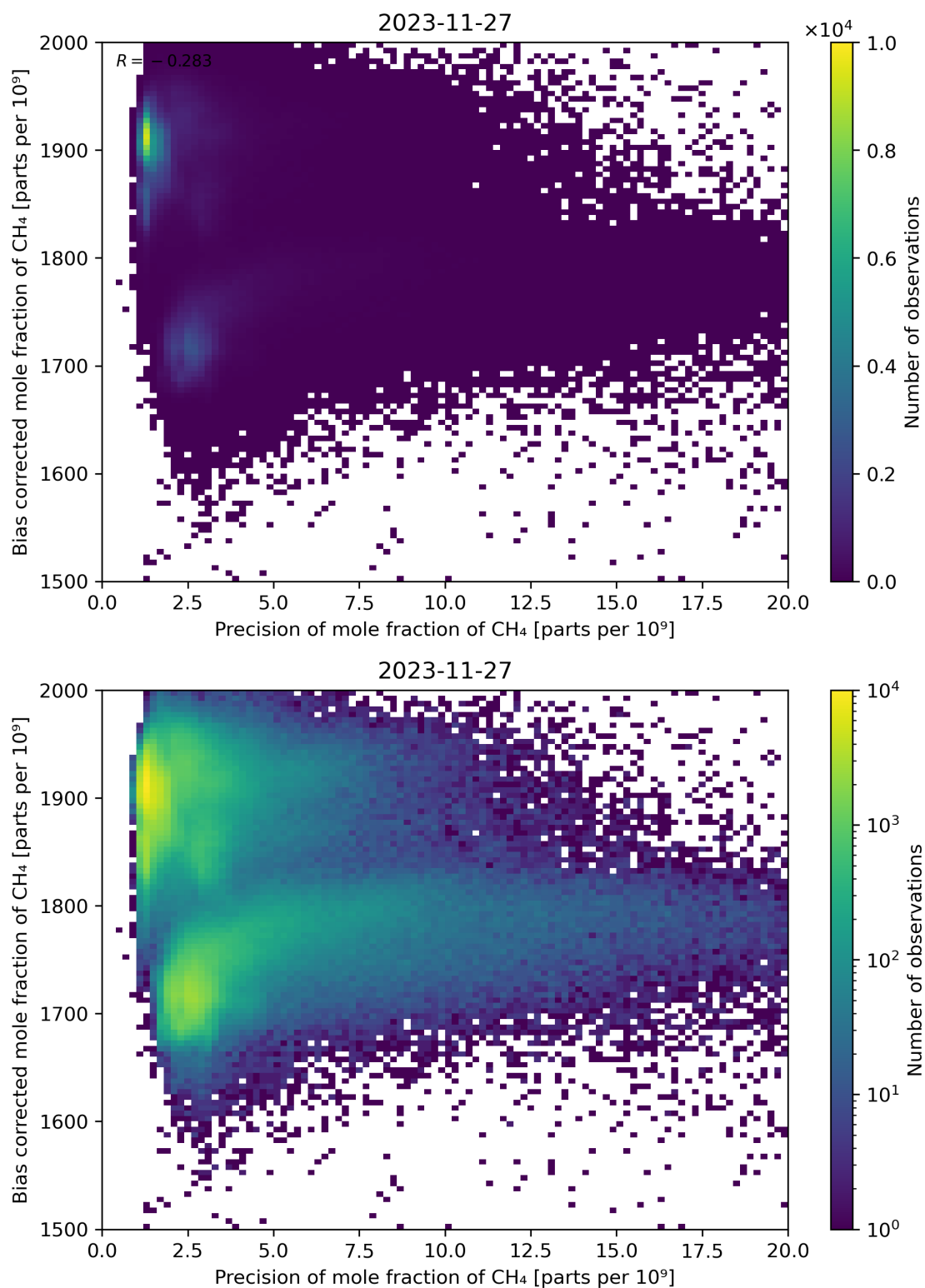
Figure 82: Scatter density plot of “Precision of mole fraction of CH 4 ” against “Bias corrected mole fraction of CH 4 ” for 2023-11-26 to 2023-11-28.
