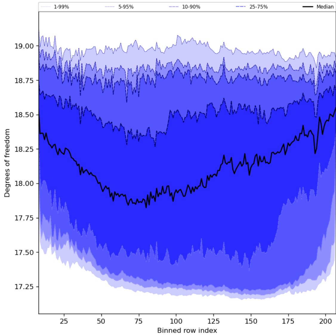
Figure 41: Along track statistics of “Degrees of freedom” for 2023-11-26 to 2023-11-28
