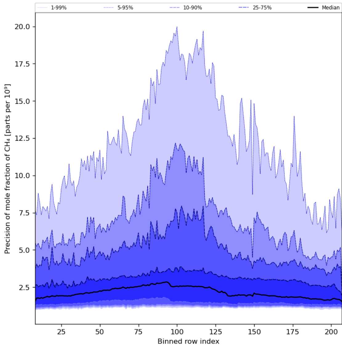
Figure 35: Along track statistics of “Precision of mole fraction of CH 4 ” for 2023-11-26 to 2023-11-28
