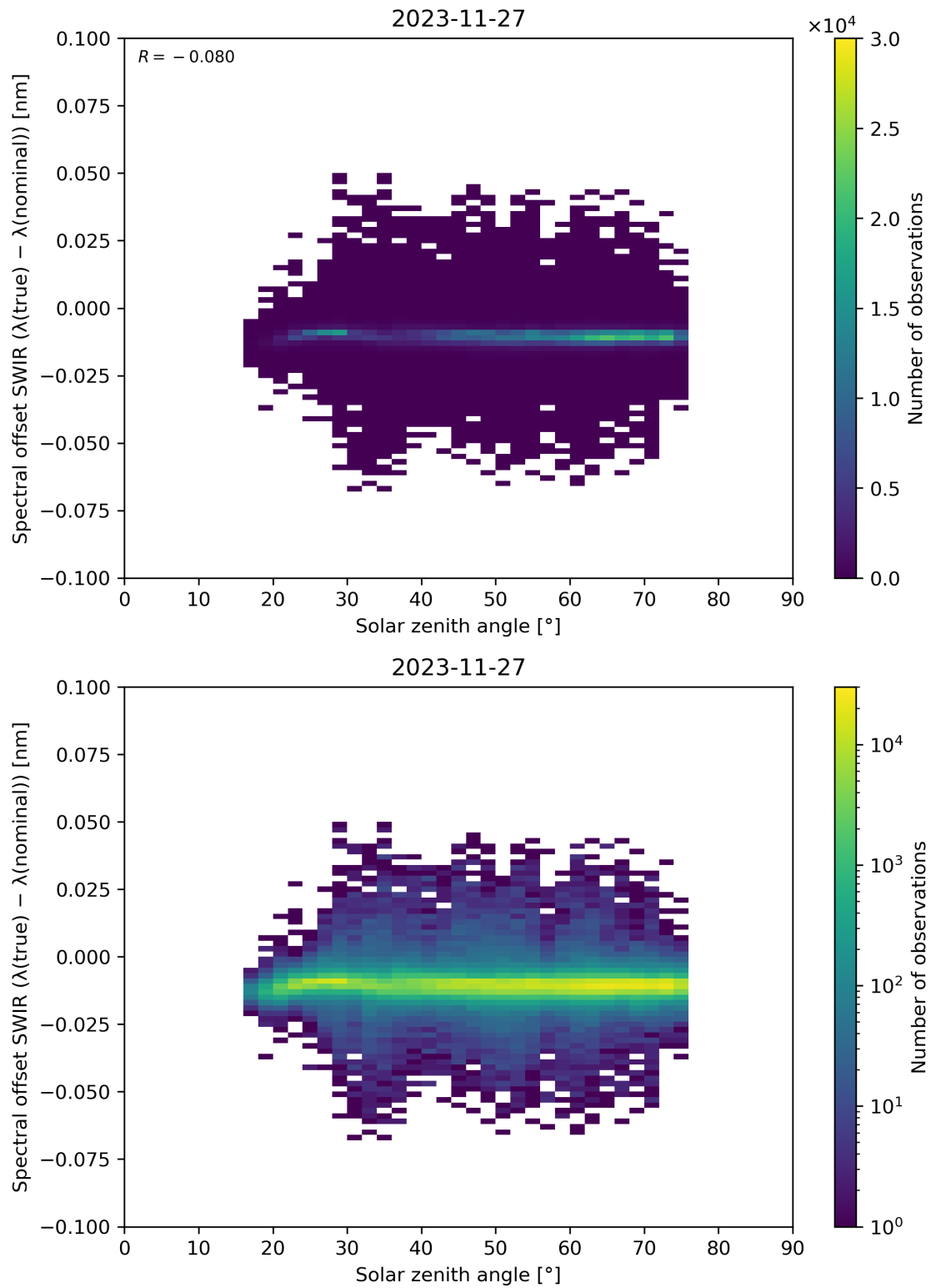
Figure 104: Scatter density plot of “Solar zenith angle” against “Spectral offset SWIR ( \lambda(\text{true}) - \lambda(\text{nominal}) )” for 2023-11-26 to 2023-11-28.
