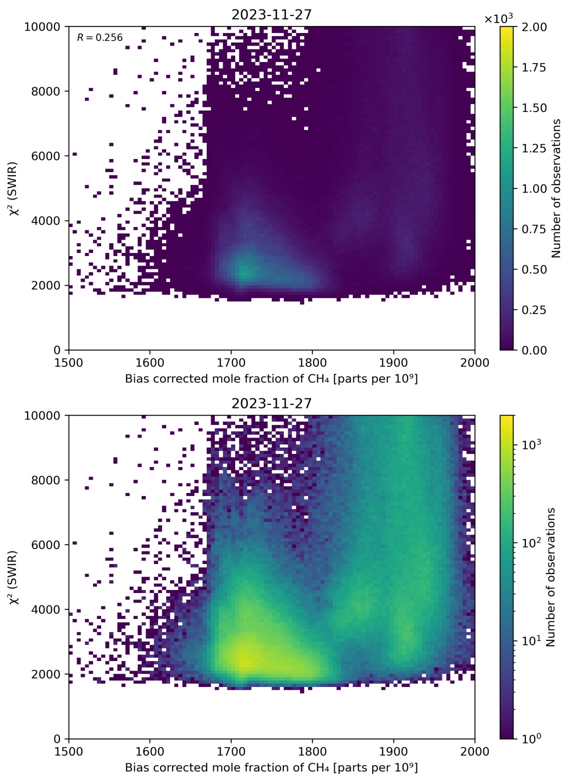
Figure 64: Scatter density plot of “Bias corrected mole fraction of \text{CH}_4 ” against “ \chi^2 (SWIR)” for 2023-11-26 to 2023-11-28.
