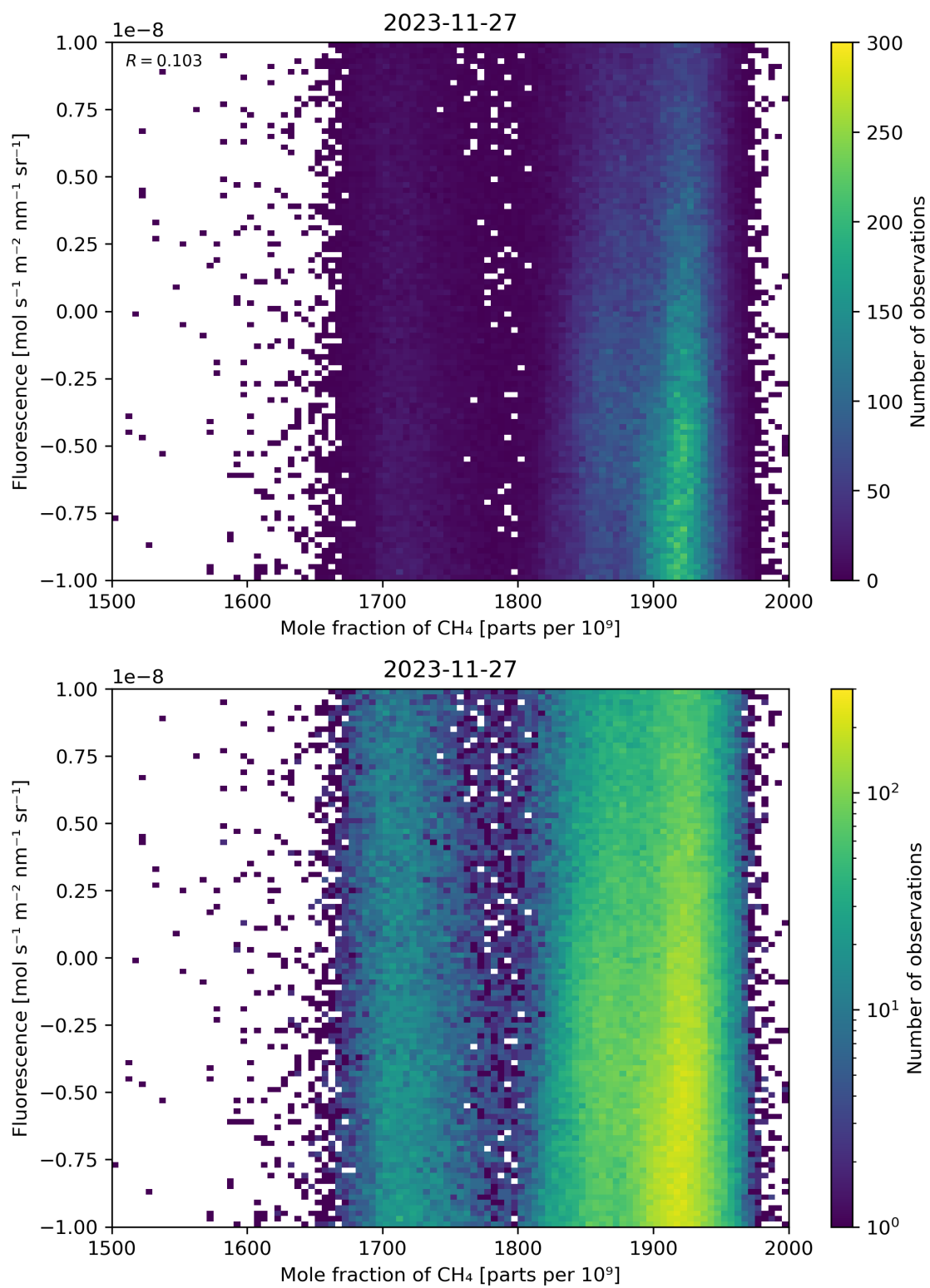
Figure 73: Scatter density plot of “Mole fraction of \text{CH}_4 ” against “Fluorescence” for 2023-11-26 to 2023-11-28.
