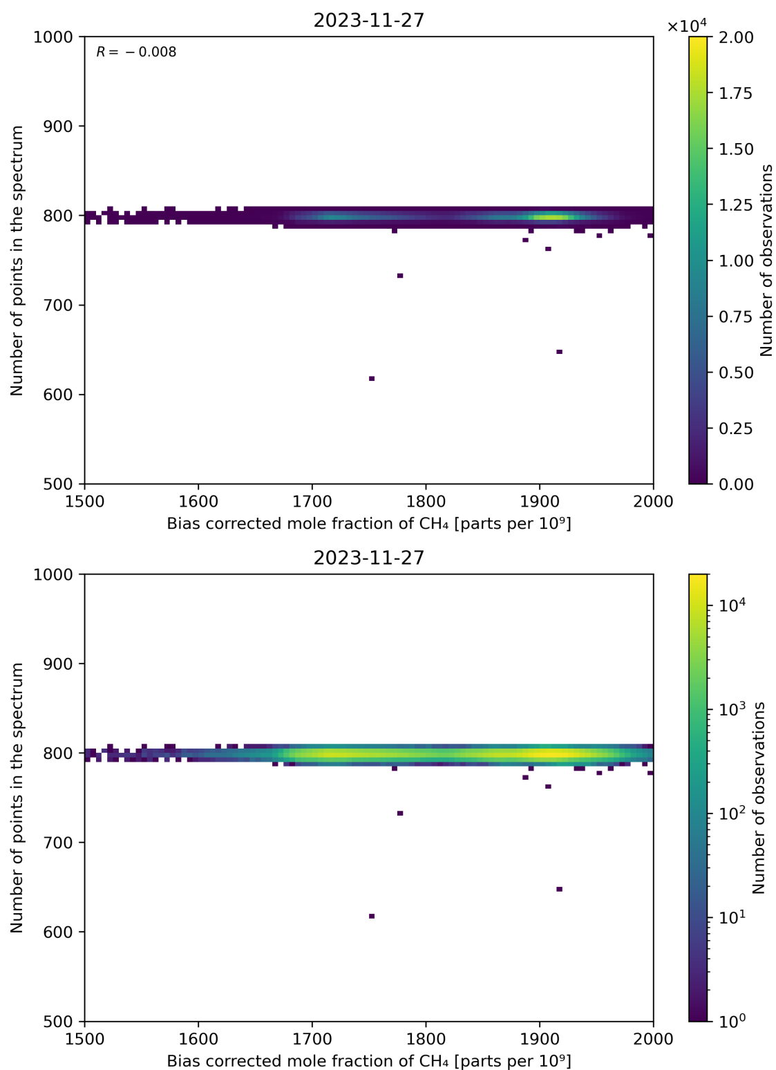
Figure 68: Scatter density plot of “Bias corrected mole fraction of CH 4 ” against “Number of points in the spectrum” for 2023-11-26 to 2023-11-28.
