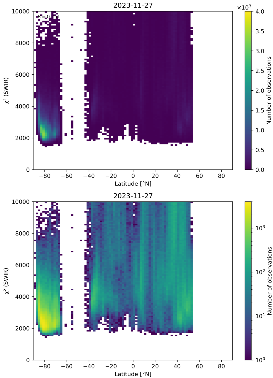
Figure 54: Scatter density plot of “Latitude” against “ \chi^2 (SWIR)” for 2023-11-26 to 2023-11-28.
