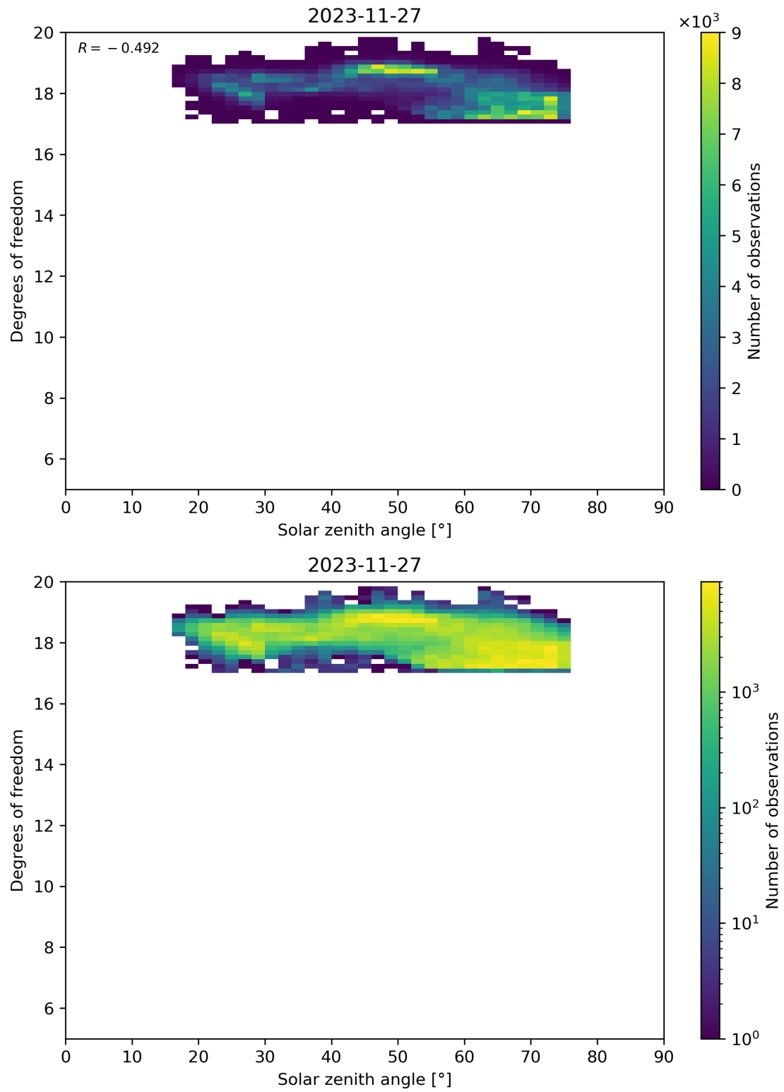
Figure 96: Scatter density plot of “Solar zenith angle” against “Degrees of freedom” for 2023-11-26 to 2023-11-28.
