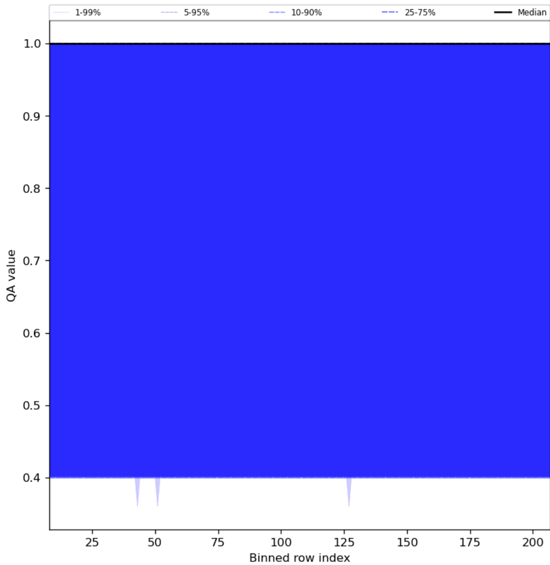
Figure 33: Along track statistics of “QA value” for 2023-11-26 to 2023-11-28
