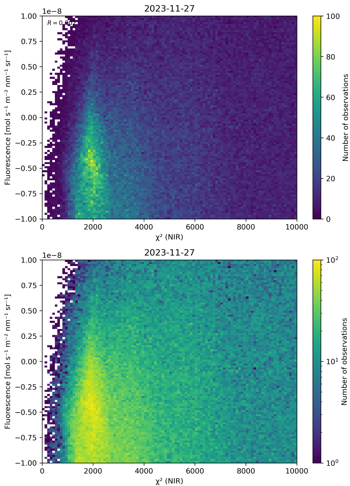
Figure 45: Scatter density plot of “ \chi^2 (NIR)” against “Fluorescence” for 2023-11-26 to 2023-11-28.
