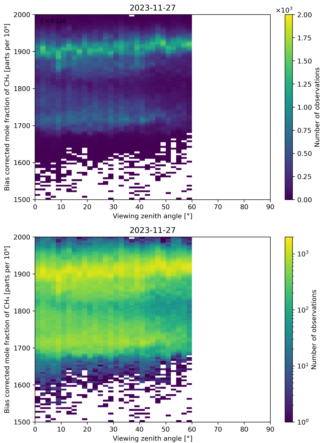
Figure 111: Scatter density plot of “Viewing zenith angle” against “Bias corrected mole fraction of CH 4 ” for 2023-11-26 to 2023-11-28.
