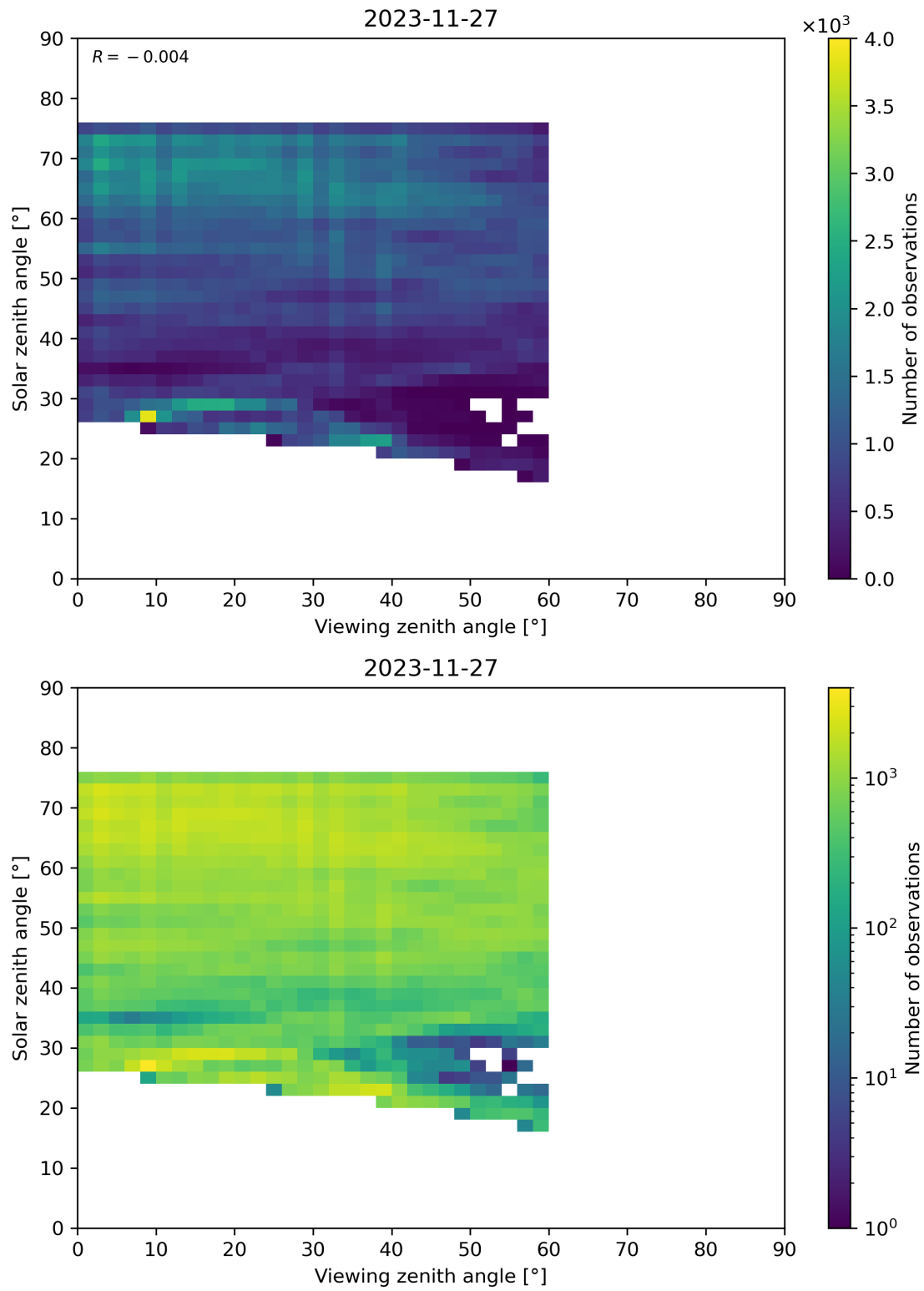
Figure 115: Scatter density plot of “Viewing zenith angle” against “Solar zenith angle” for 2023-11-26 to 2023-11-28.
