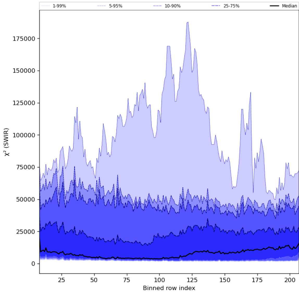
Figure 39: Along track statistics of “ \chi^2 (SWIR)” for 2023-11-26 to 2023-11-28
