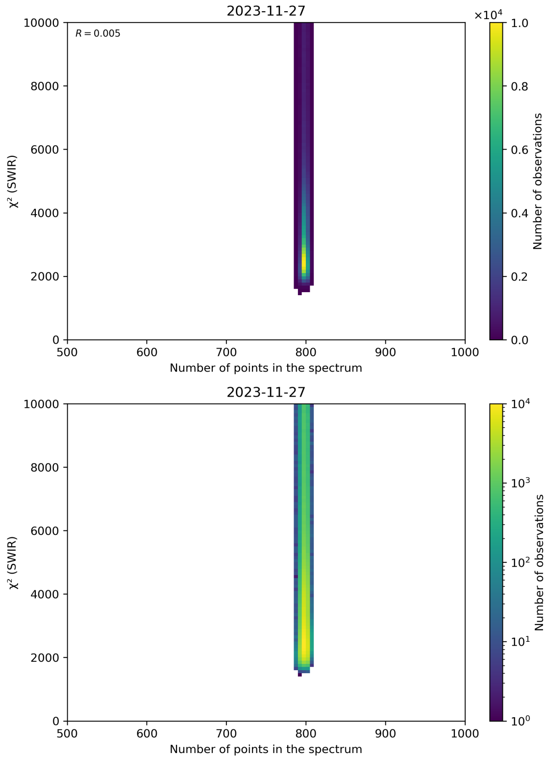
Figure 89: Scatter density plot of “Number of points in the spectrum” against “ \chi^2 (SWIR)” for 2023-11-26 to 2023-11-28.
