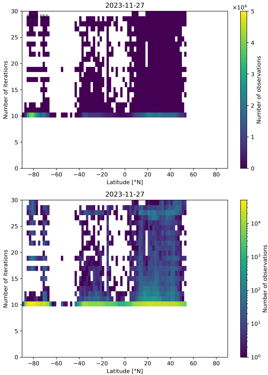
Figure 60: Scatter density plot of “Latitude” against “Number of iterations” for 2023-11-26 to 2023-11-28.
