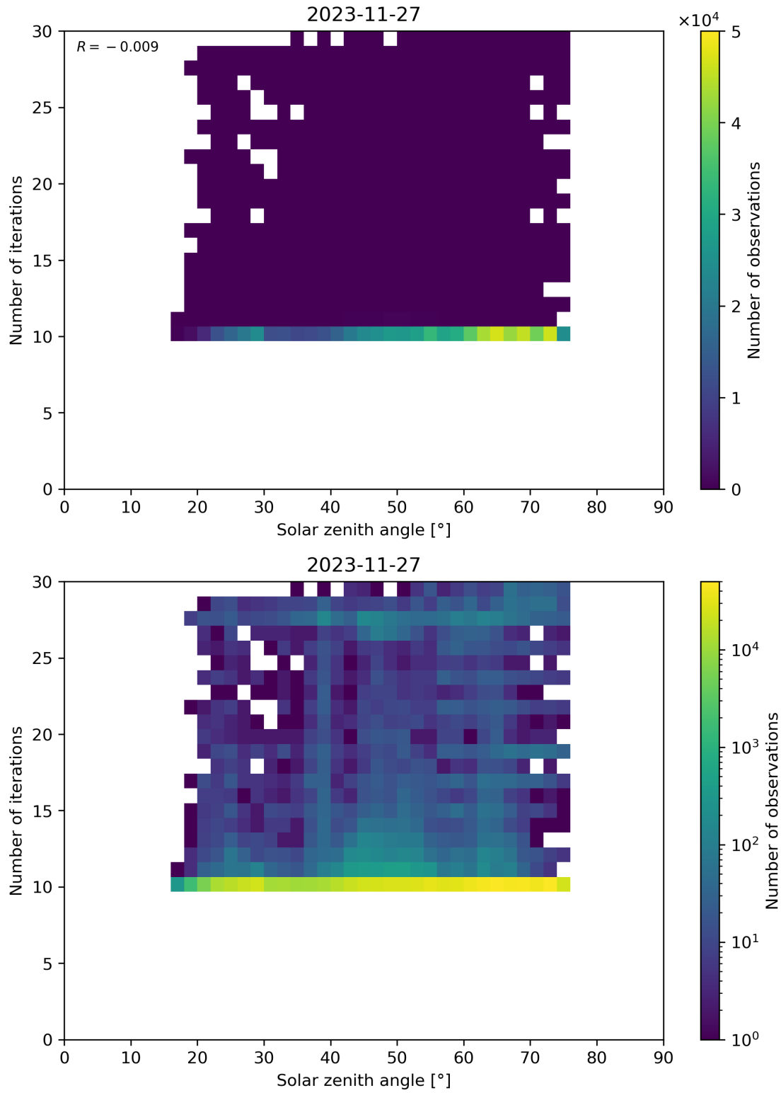
Figure 102: Scatter density plot of “Solar zenith angle” against “Number of iterations” for 2023-11-26 to 2023-11-28.
