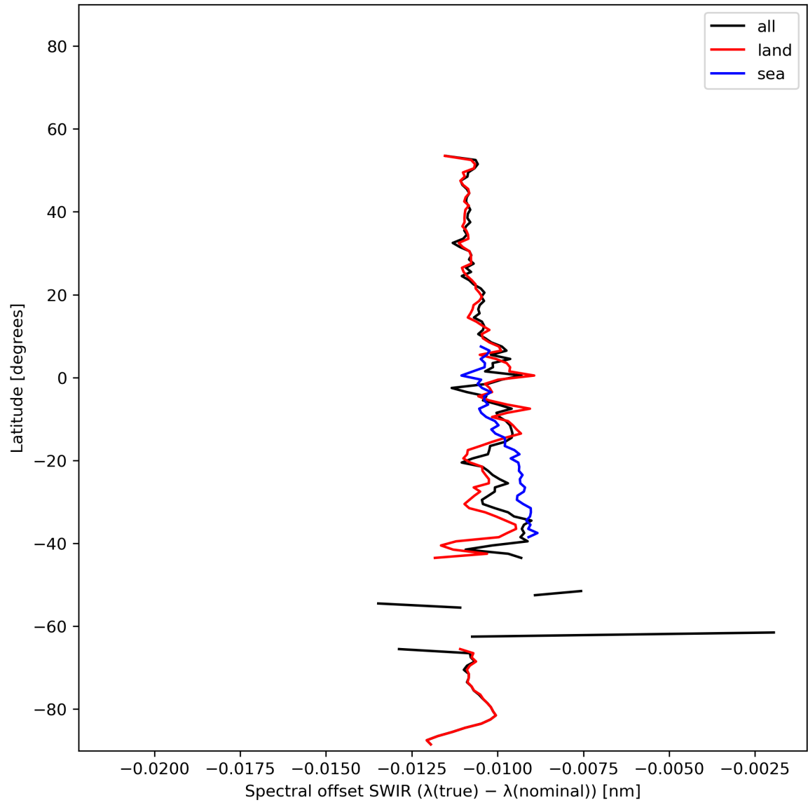
Figure 16: Zonal average of “Spectral offset SWIR ( \lambda(\text{true}) - \lambda(\text{nominal}) )” for 2023-11-26 to 2023-11-28.
