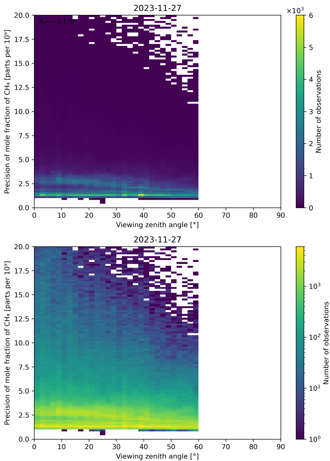
Figure 112: Scatter density plot of “Viewing zenith angle” against “Precision of mole fraction of \text{CH}_4 ” for 2023-11-26 to 2023-11-28.
