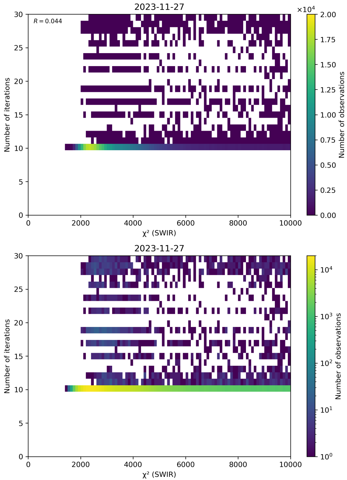
Figure 50: Scatter density plot of “ \chi^2 (SWIR)” against “Number of iterations” for 2023-11-26 to 2023-11-28.
