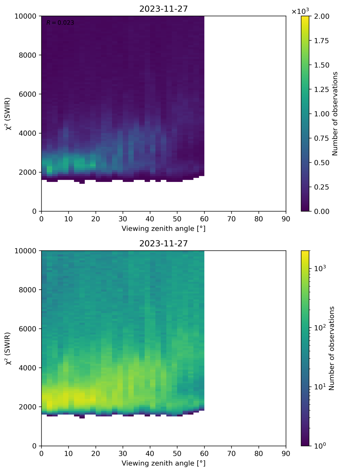
Figure 106: Scatter density plot of “Viewing zenith angle” against “ \chi^2 (SWIR)” for 2023-11-26 to 2023-11-28.
