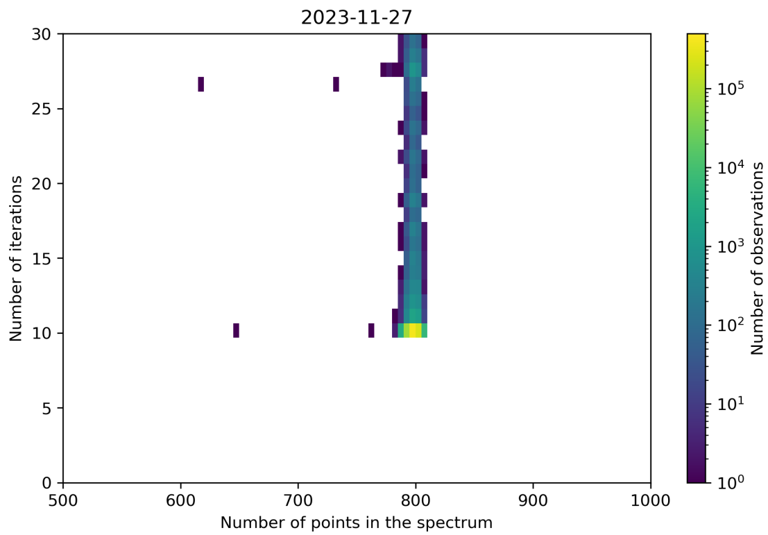
Figure 92: Scatter density plot of “Number of points in the spectrum” against “Number of iterations” for 2023-11-26 to 2023-11-28.
