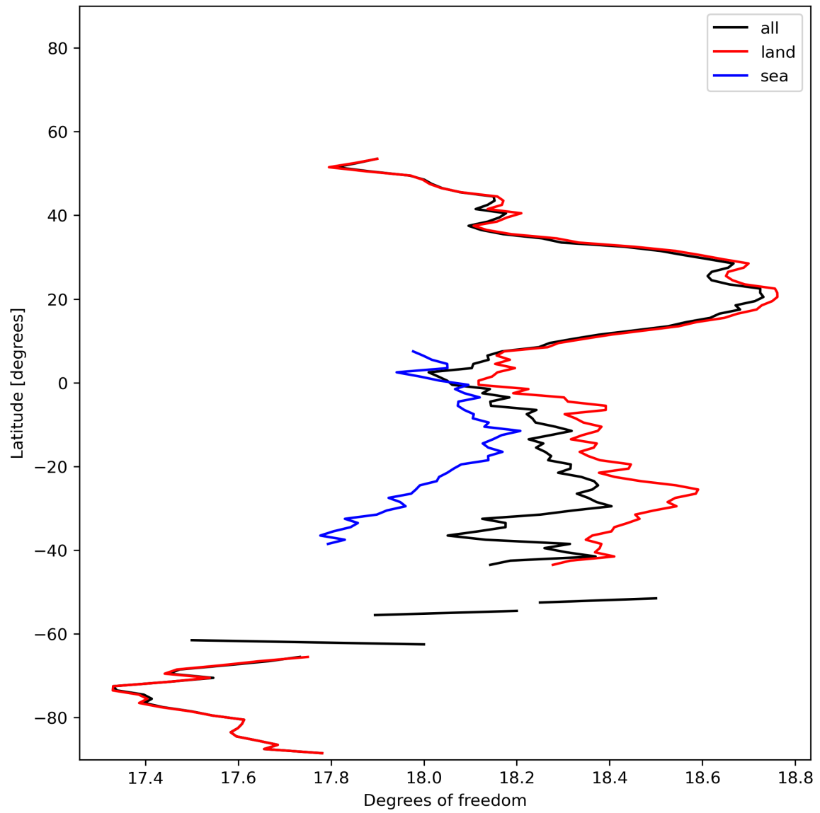
Figure 19: Zonal average of “Degrees of freedom” for 2023-11-26 to 2023-11-28.
