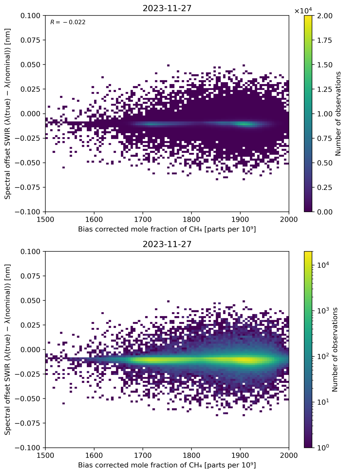
Figure 69: Scatter density plot of “Bias corrected mole fraction of \text{CH}_4 ” against “Spectral offset SWIR ( \lambda(\text{true}) - \lambda(\text{nominal}) )” for 2023-11-26 to 2023-11-28.
