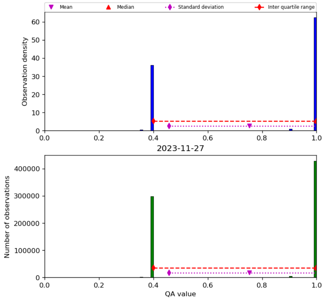
Figure 22: Histogram of “QA value” for 2023-11-26 to 2023-11-28
