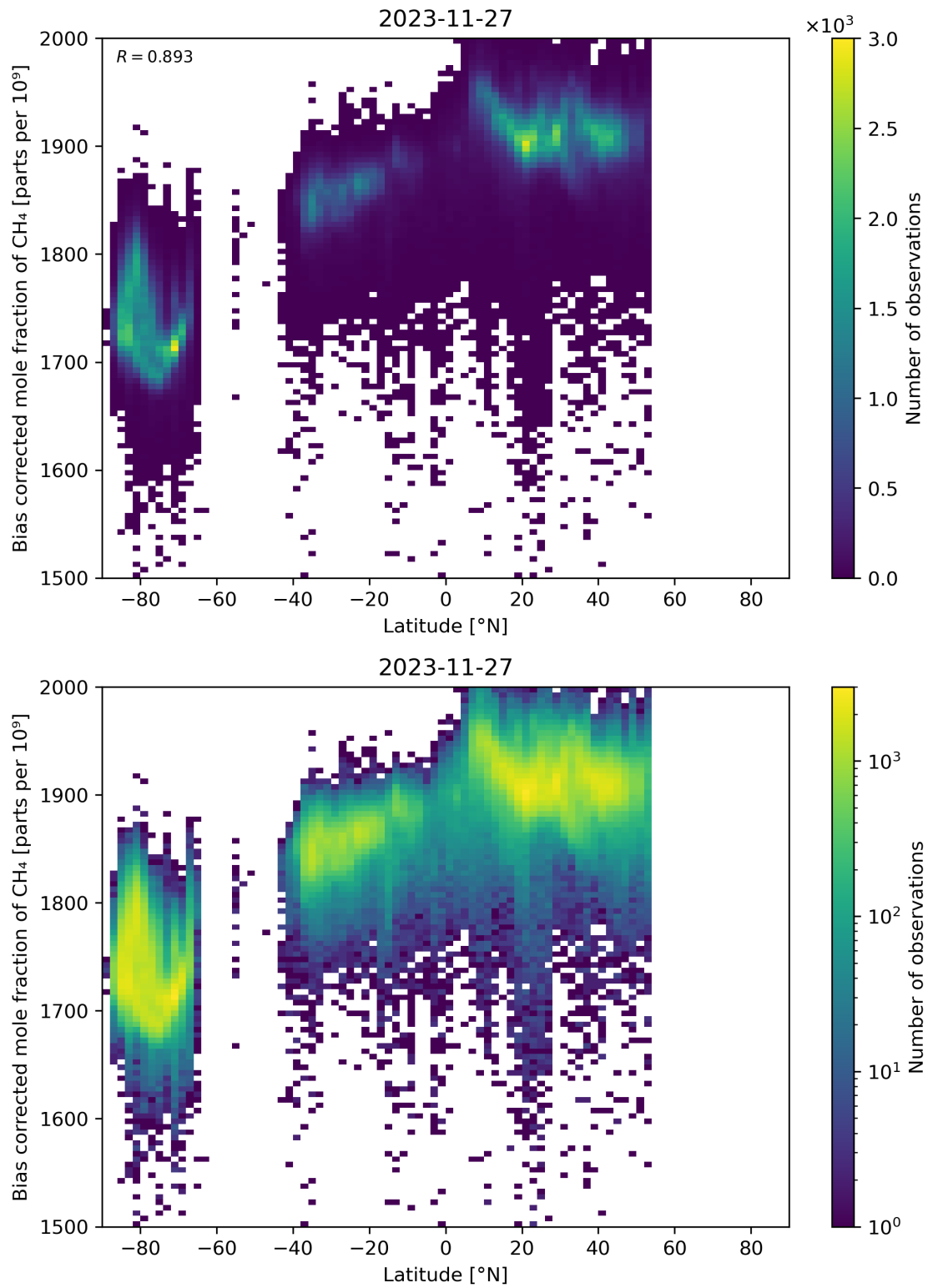
Figure 58: Scatter density plot of “Latitude” against “Bias corrected mole fraction of CH 4 ” for 2023-11-26 to 2023-11-28.
