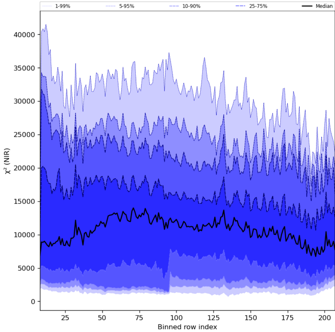
Figure 40: Along track statistics of “ \chi^2 (NIR)” for 2023-11-26 to 2023-11-28
