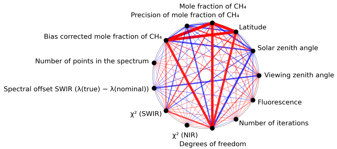
Figure 1: Map of correlation graph for 2023-11-26 to 2023-11-28.
