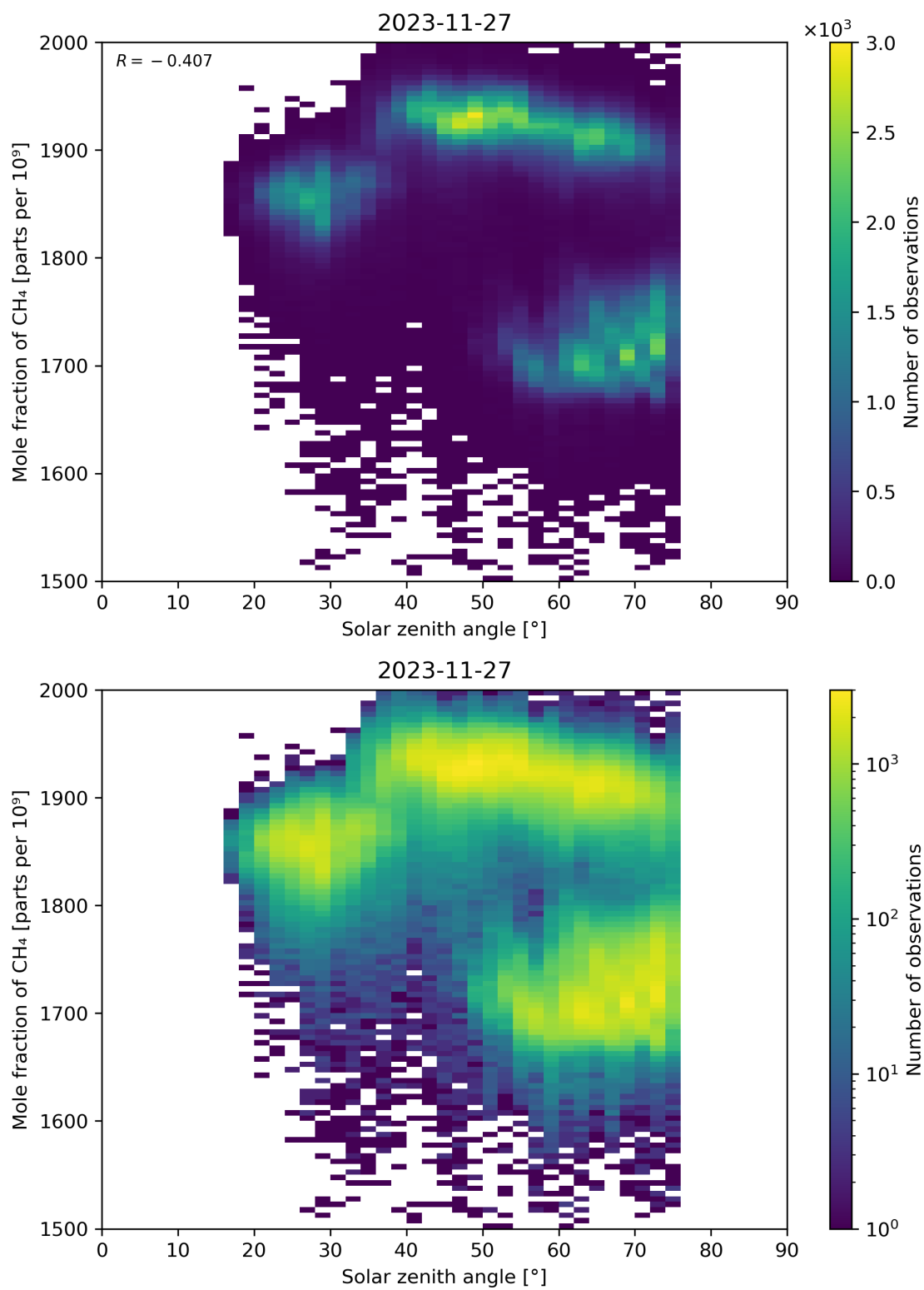
Figure 99: Scatter density plot of “Solar zenith angle” against “Mole fraction of CH 4 ” for 2023-11-26 to 2023-11-28.
