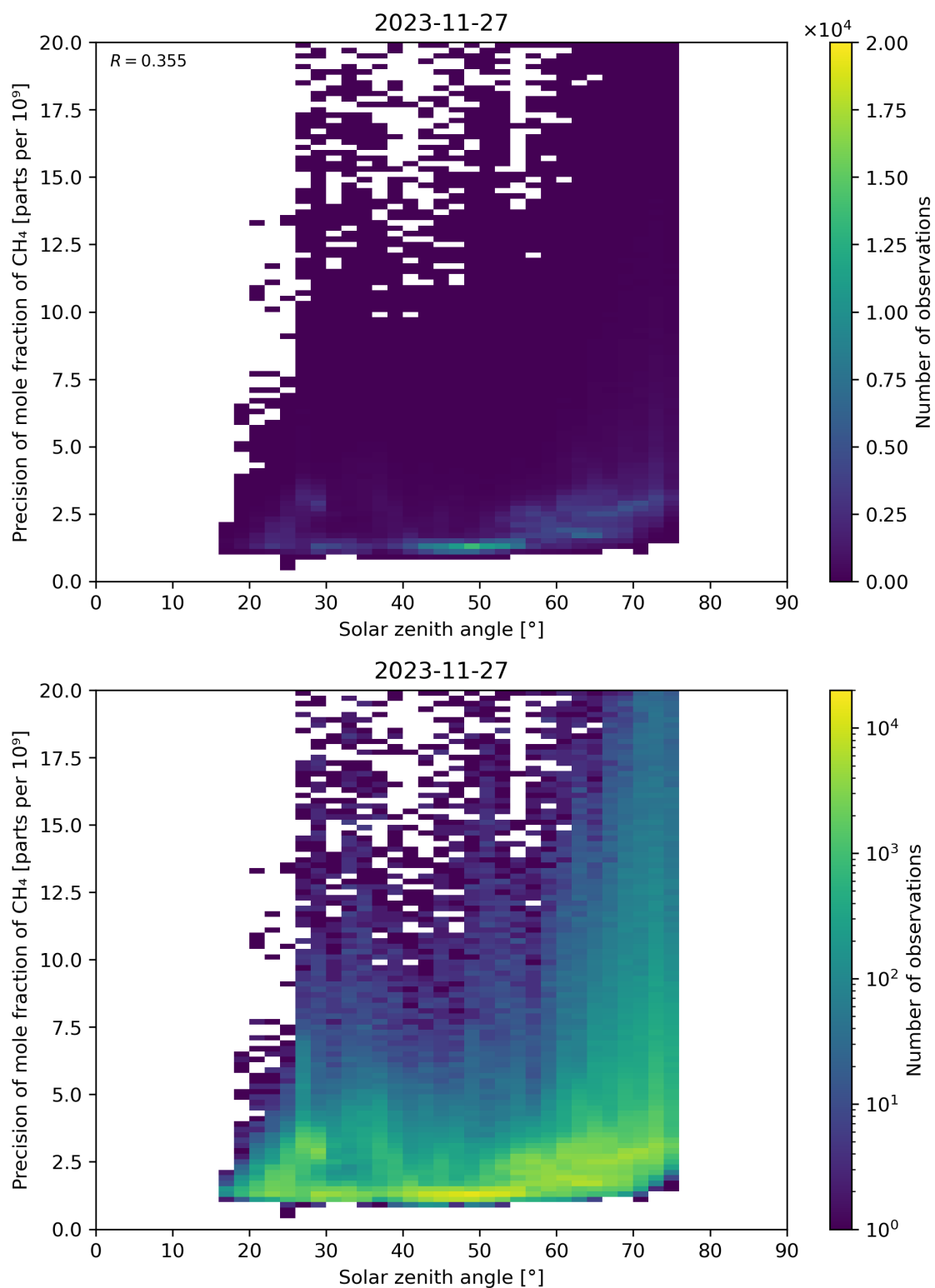
Figure 101: Scatter density plot of “Solar zenith angle” against “Precision of mole fraction of \text{CH}_4 ” for 2023-11-26 to 2023-11-28.
