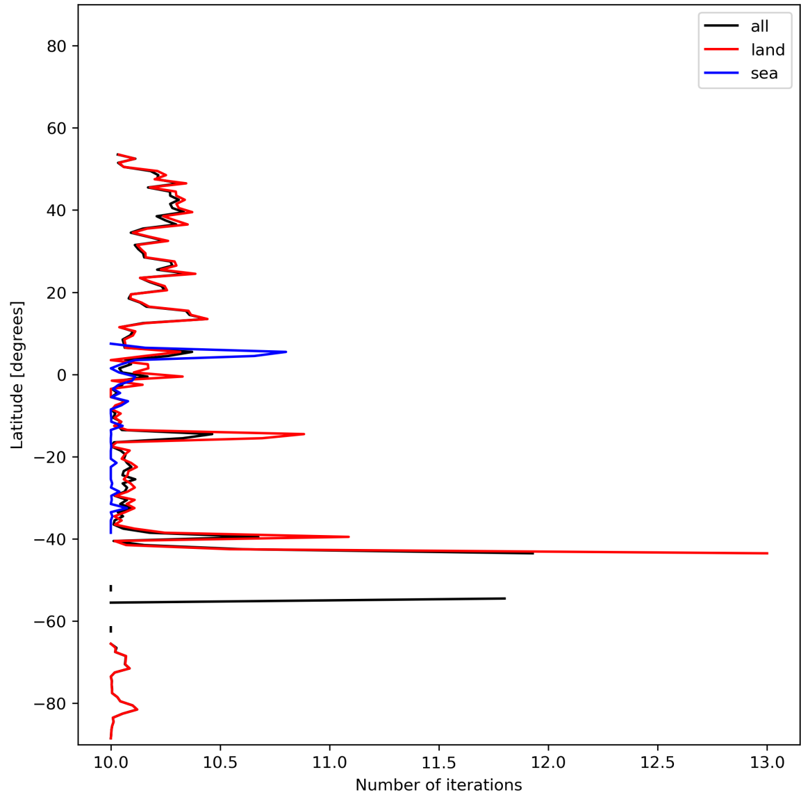
Figure 20: Zonal average of “Number of iterations” for 2023-11-26 to 2023-11-28.
