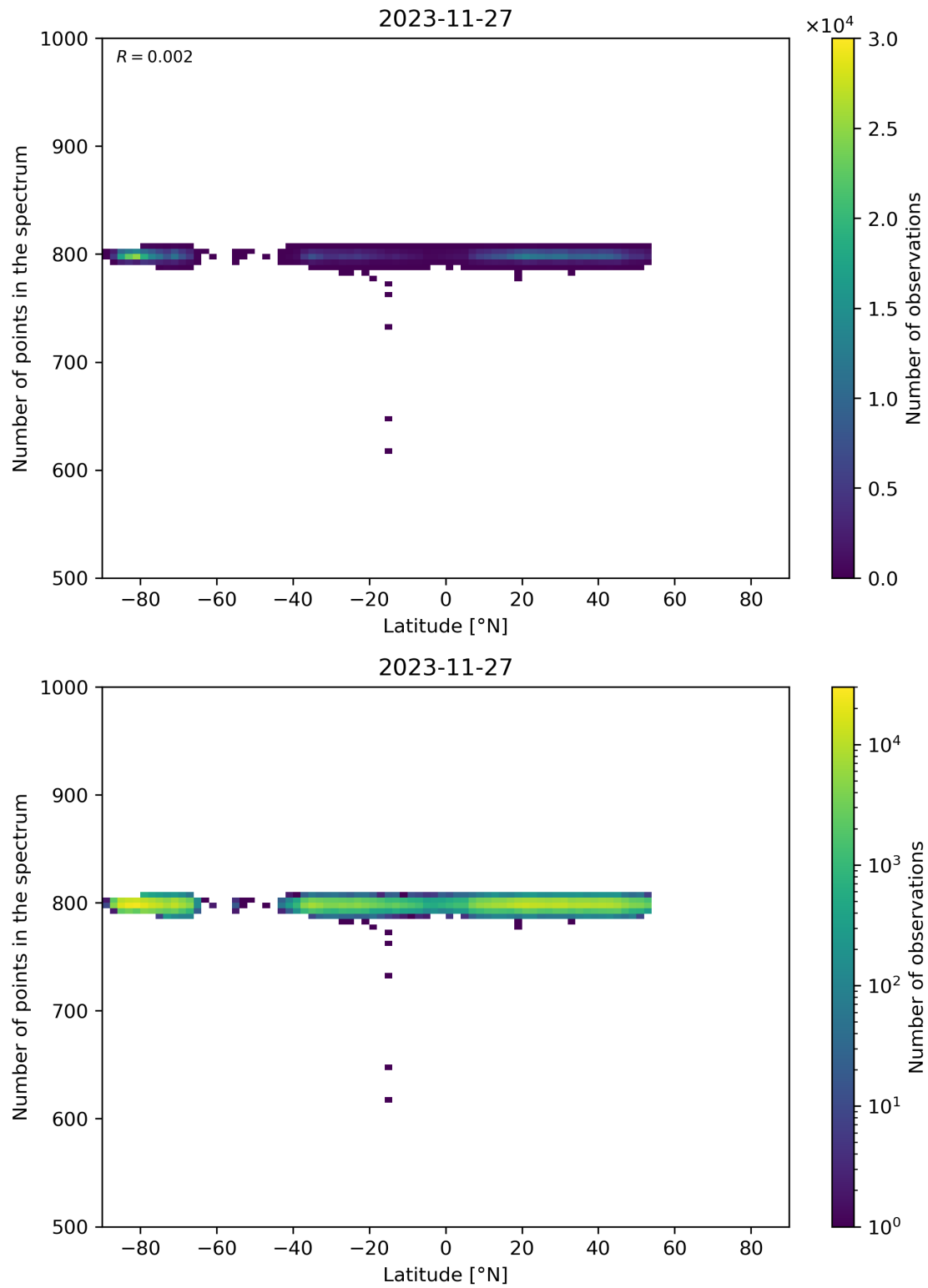
Figure 61: Scatter density plot of “Latitude” against “Number of points in the spectrum” for 2023-11-26 to 2023-11-28.
