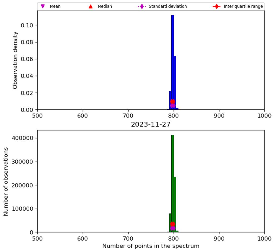
Figure 26: Histogram of “Number of points in the spectrum” for 2023-11-26 to 2023-11-28
