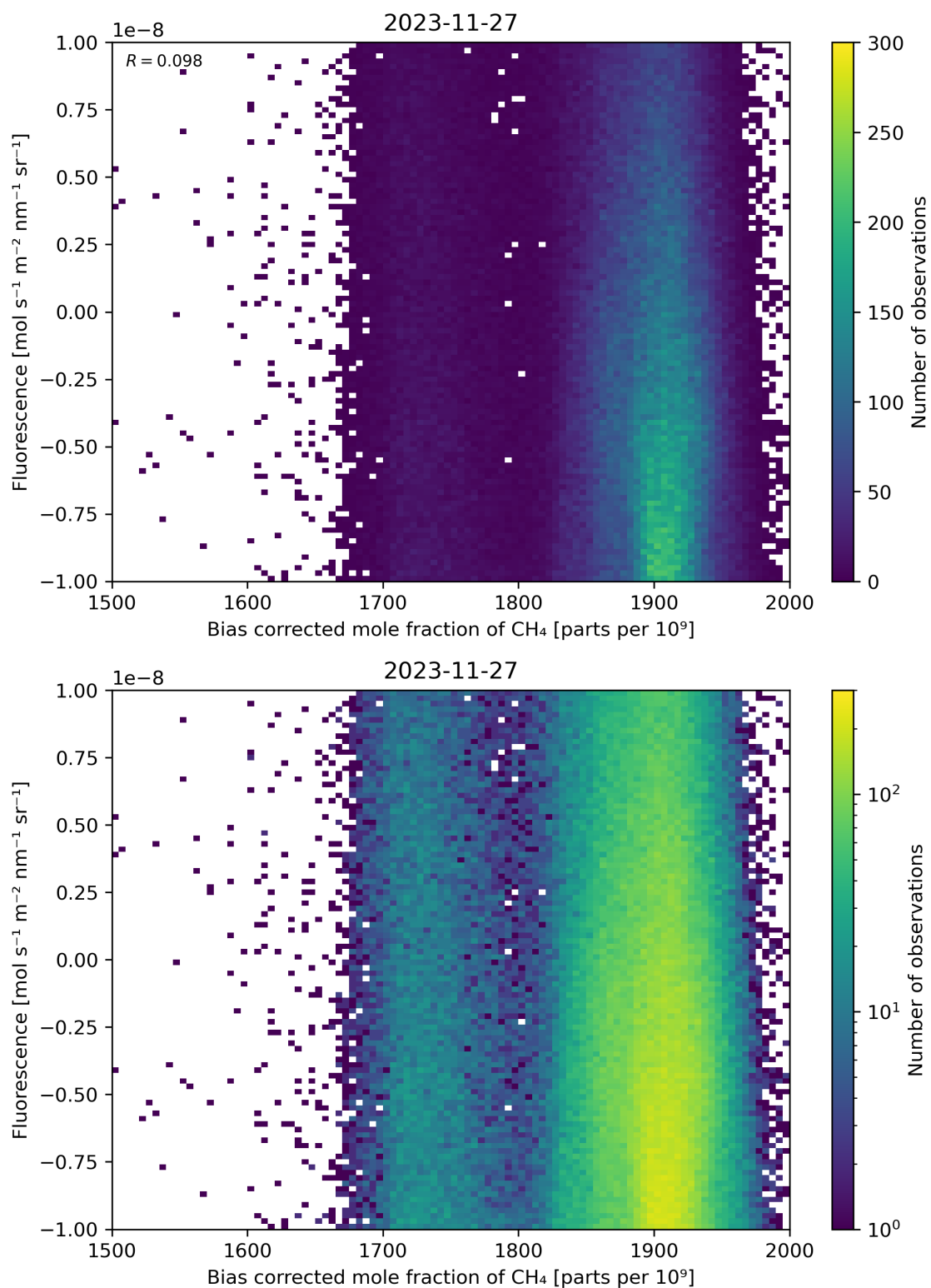
Figure 66: Scatter density plot of “Bias corrected mole fraction of \text{CH}_4 ” against “Fluorescence” for 2023-11-26 to 2023-11-28.
