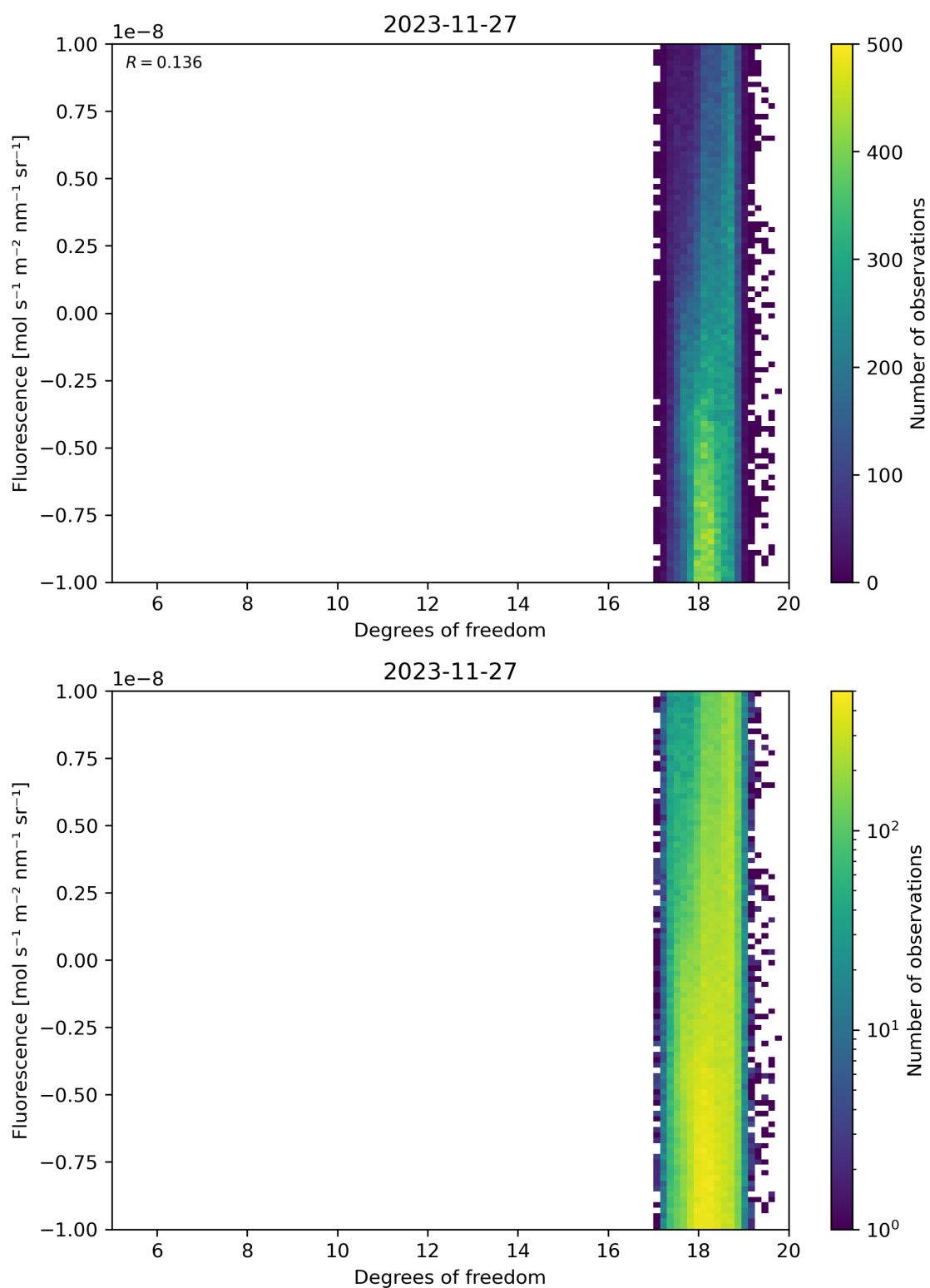
Figure 51: Scatter density plot of “Degrees of freedom” against “Fluorescence” for 2023-11-26 to 2023-11-28.
