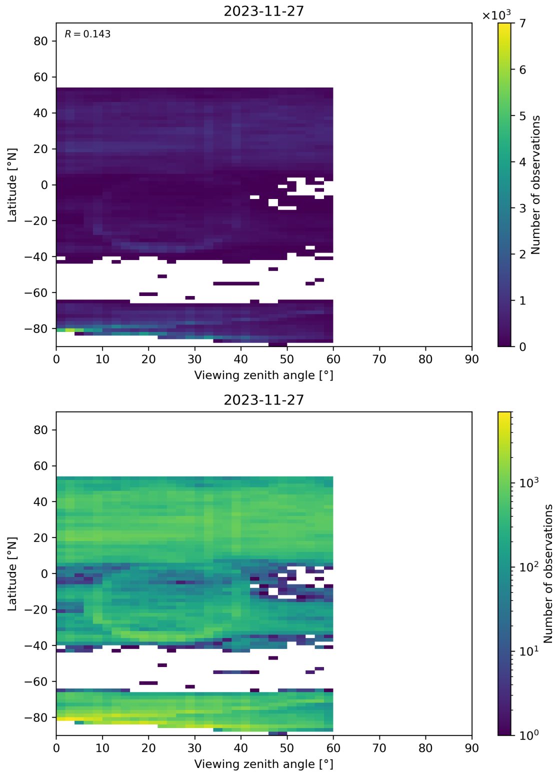
Figure 109: Scatter density plot of “Viewing zenith angle” against “Latitude” for 2023-11-26 to 2023-11-28.
