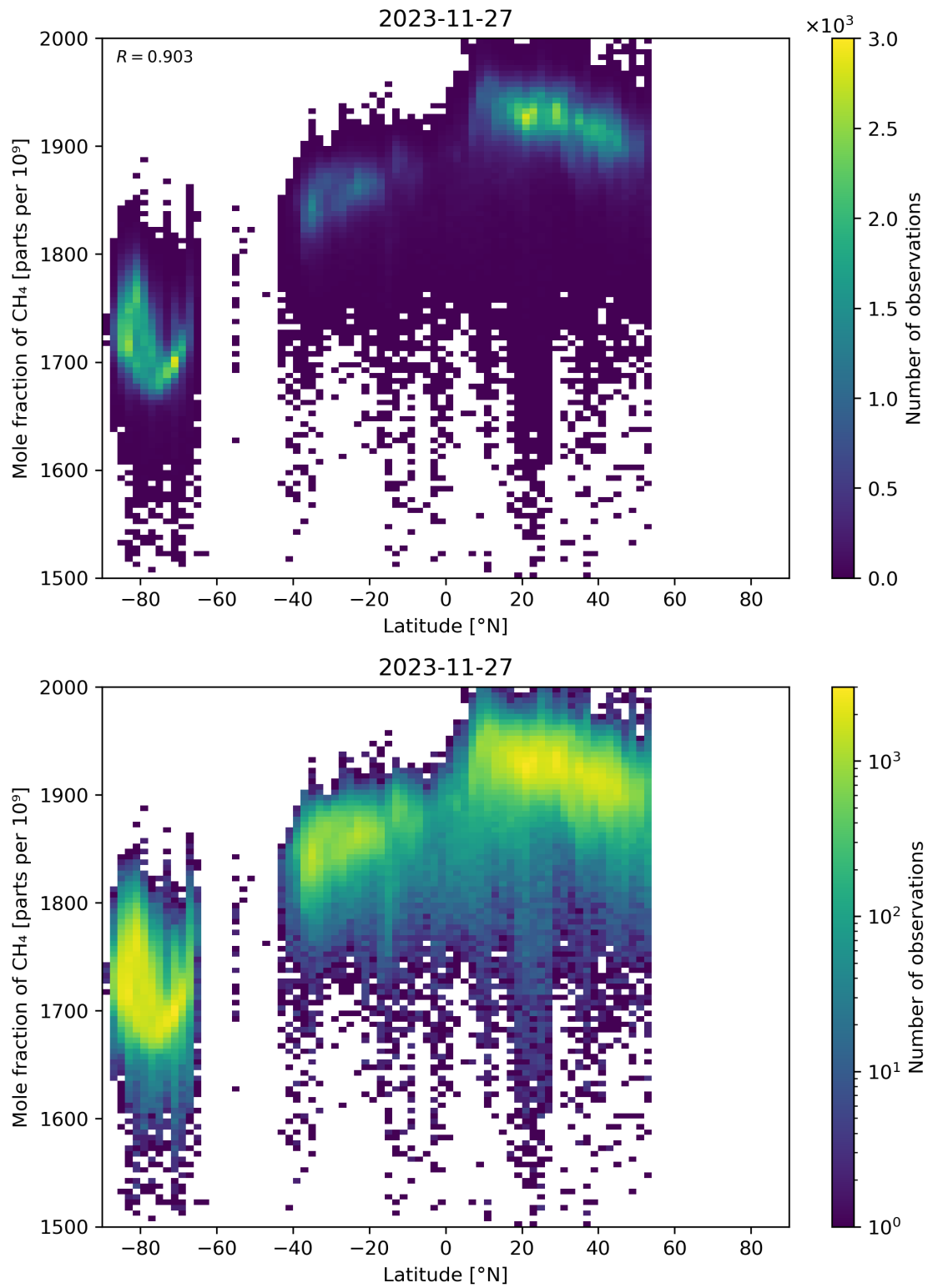
Figure 57: Scatter density plot of “Latitude” against “Mole fraction of \text{CH}_4 ” for 2023-11-26 to 2023-11-28.
