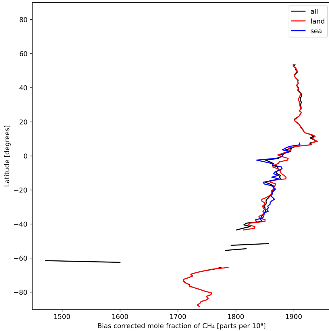
Figure 14: Zonal average of “Bias corrected mole fraction of CH 4 ” for 2023-11-26 to 2023-11-28.
