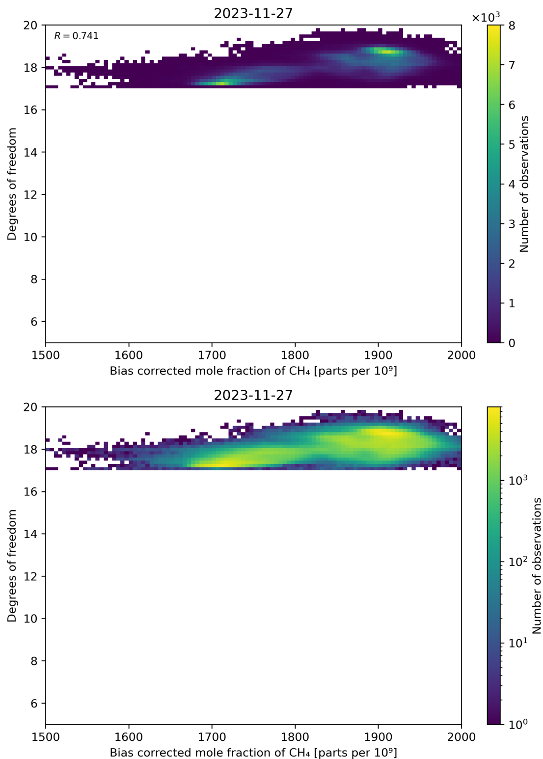
Figure 65: Scatter density plot of “Bias corrected mole fraction of CH 4 ” against “Degrees of freedom” for 2023-11-26 to 2023-11-28.
