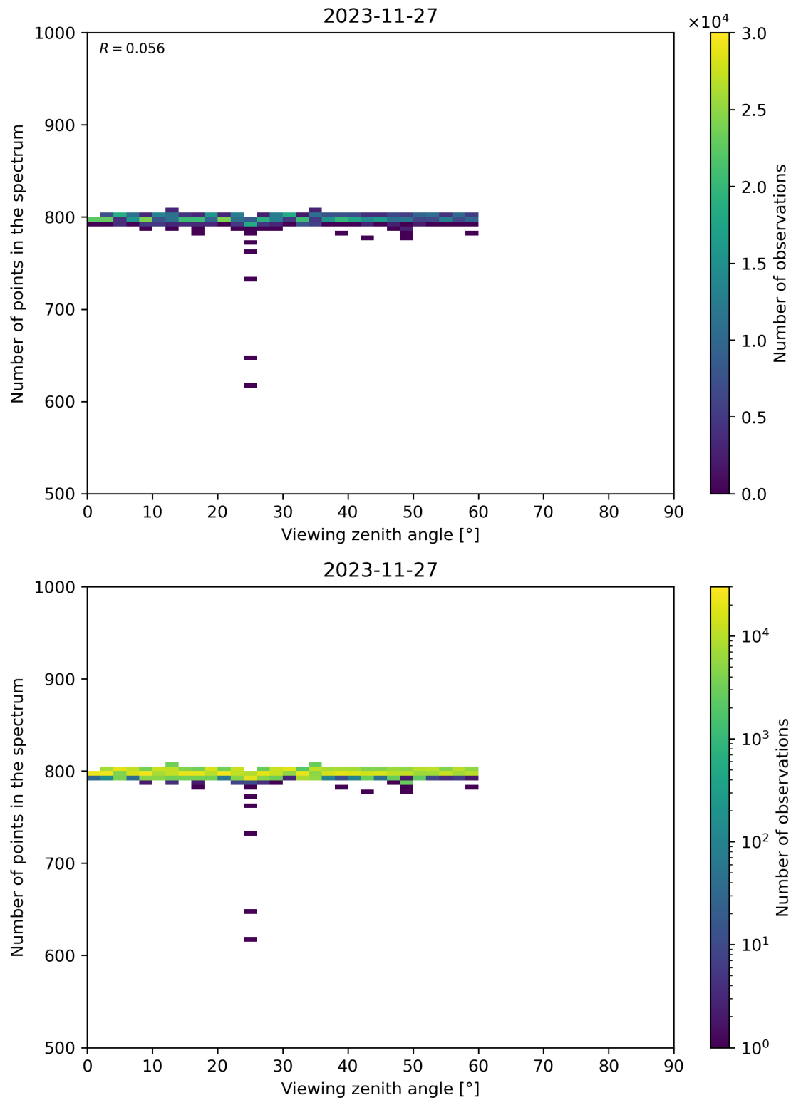
Figure 114: Scatter density plot of “Viewing zenith angle” against “Number of points in the spectrum” for 2023-11-26 to 2023-11-28.
