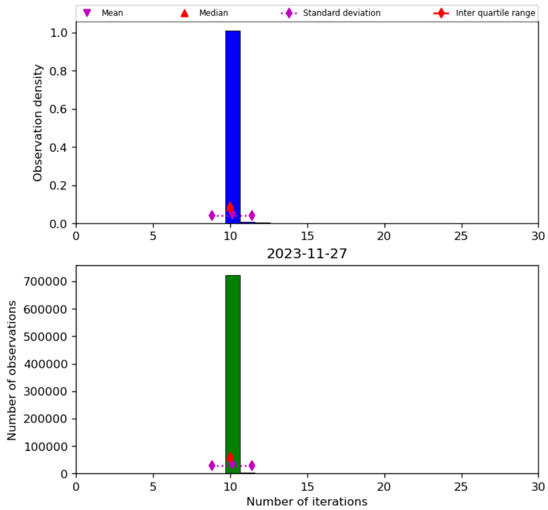
Figure 31: Histogram of “Number of iterations” for 2023-11-26 to 2023-11-28
