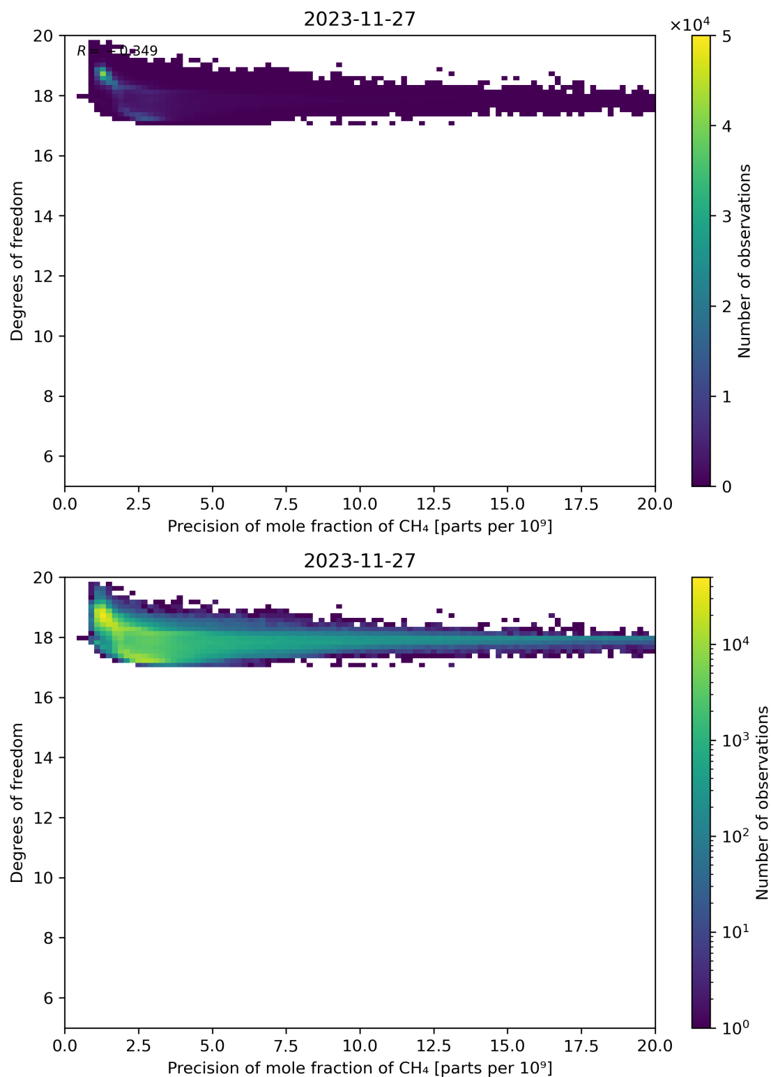
Figure 80: Scatter density plot of “Precision of mole fraction of CH 4 ” against “Degrees of freedom” for 2023-11-26 to 2023-11-28.
