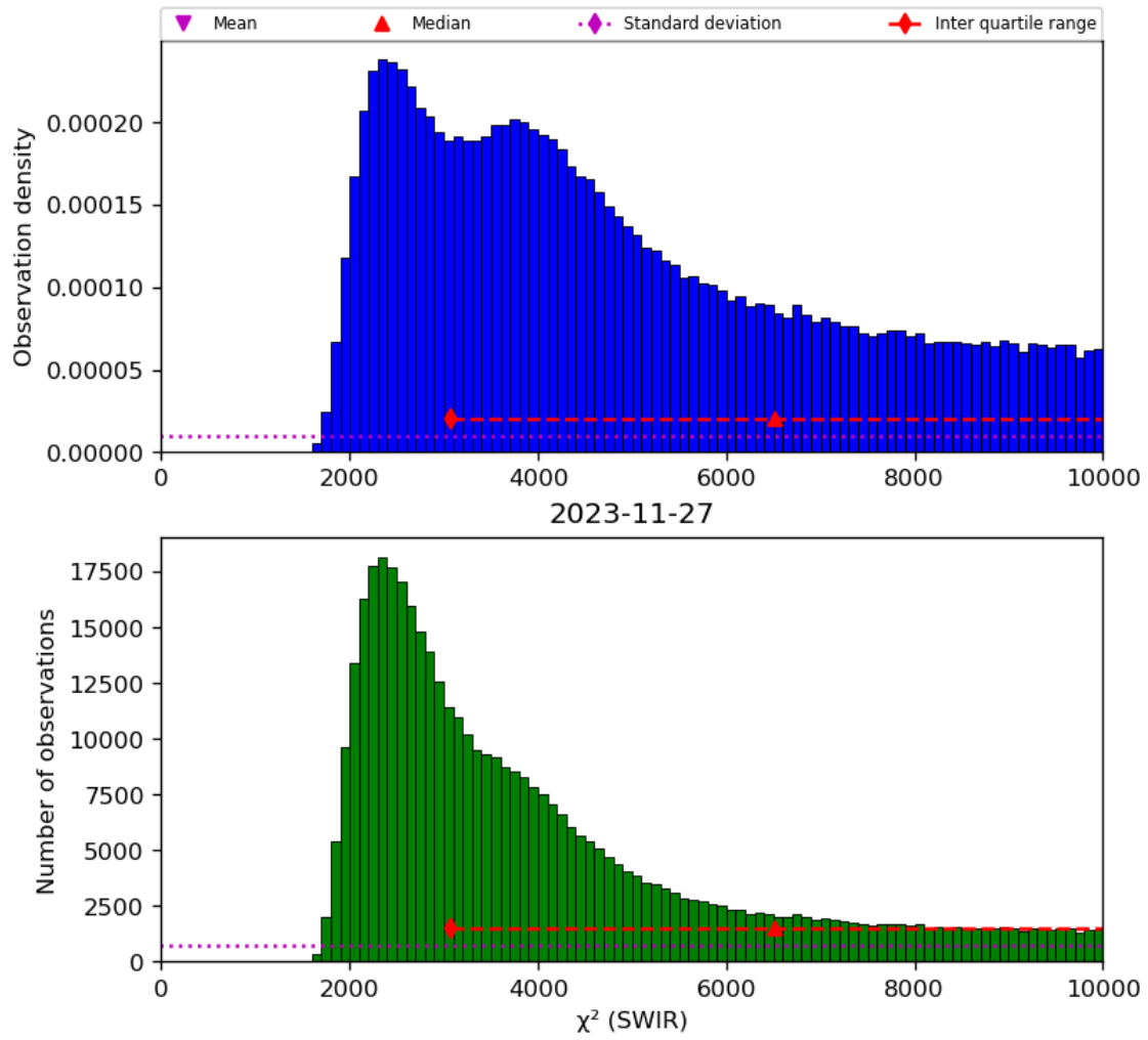
Figure 28: Histogram of “ \chi^2 (SWIR)” for 2023-11-26 to 2023-11-28
