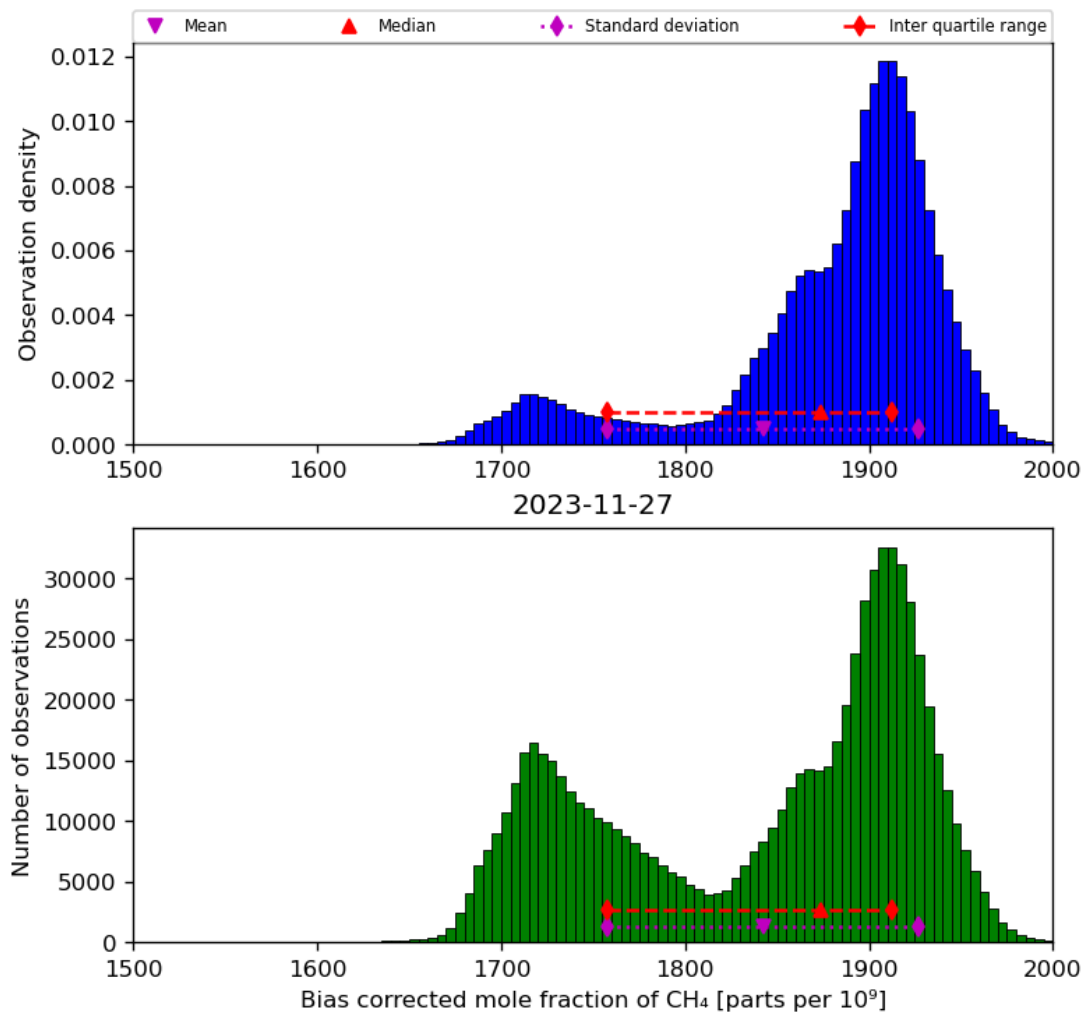
Figure 25: Histogram of “Bias corrected mole fraction of CH 4 ” for 2023-11-26 to 2023-11-28
