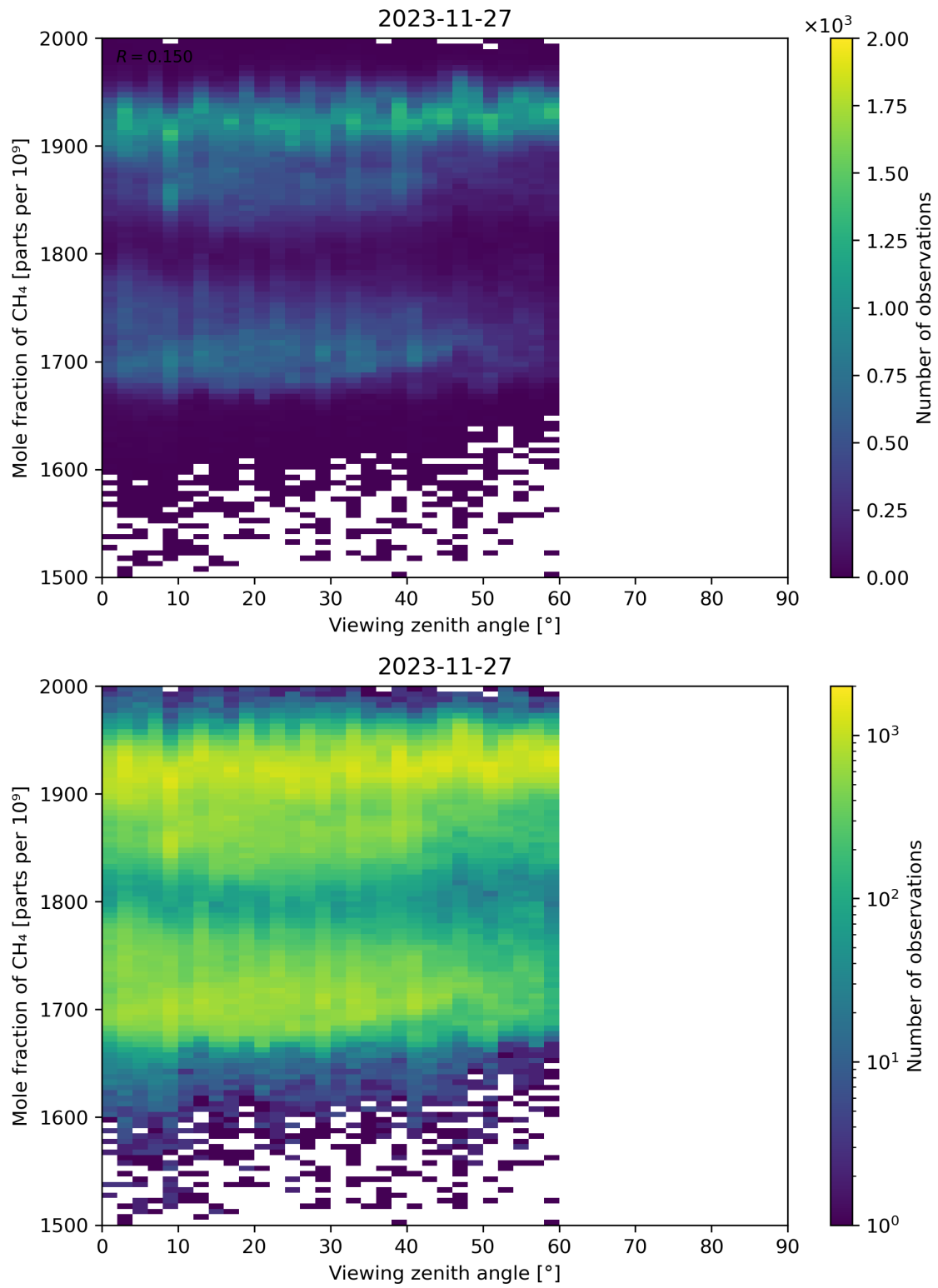
Figure 110: Scatter density plot of “Viewing zenith angle” against “Mole fraction of \text{CH}_4 ” for 2023-11-26 to 2023-11-28.
