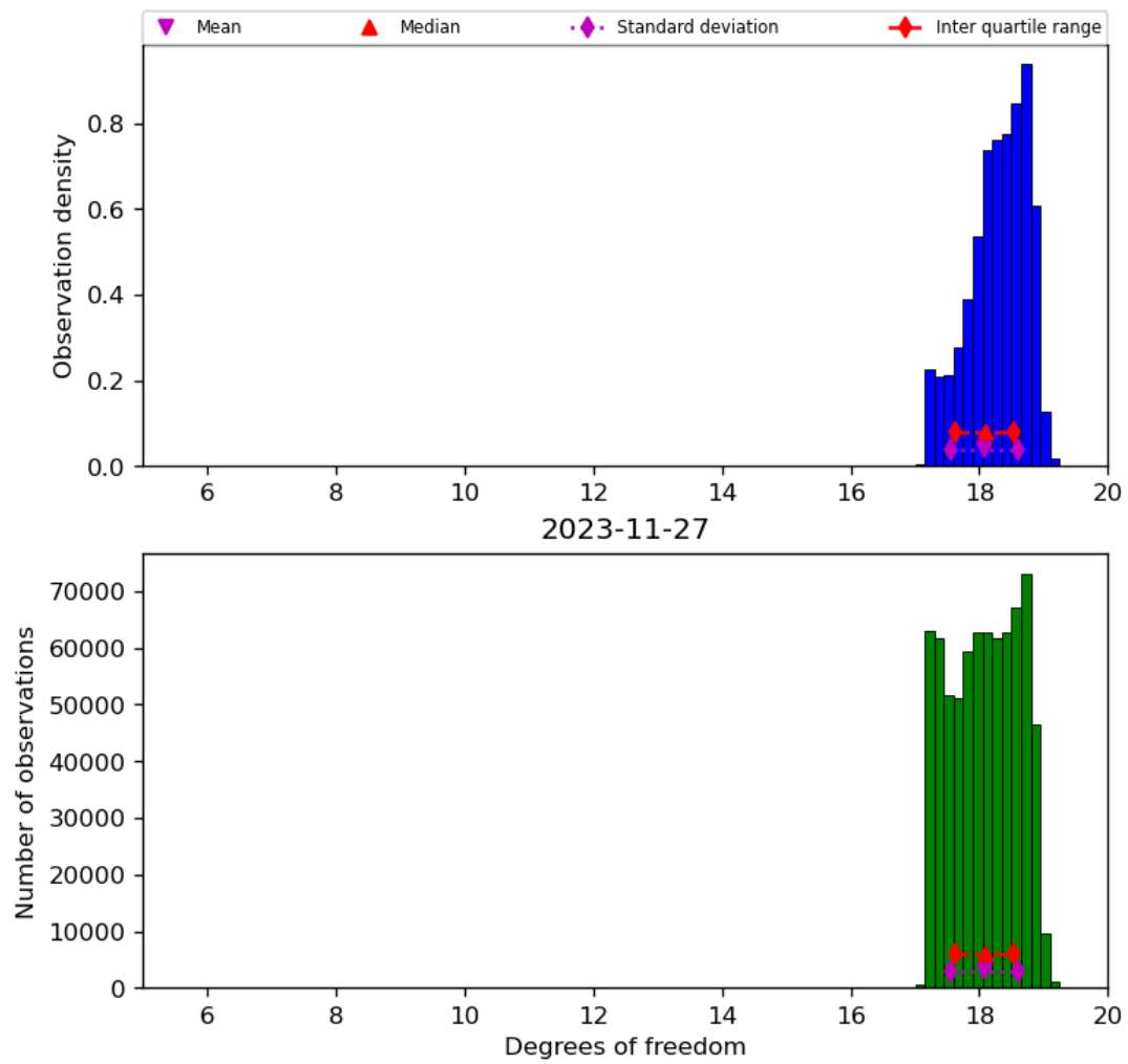
Figure 30: Histogram of “Degrees of freedom” for 2023-11-26 to 2023-11-28
