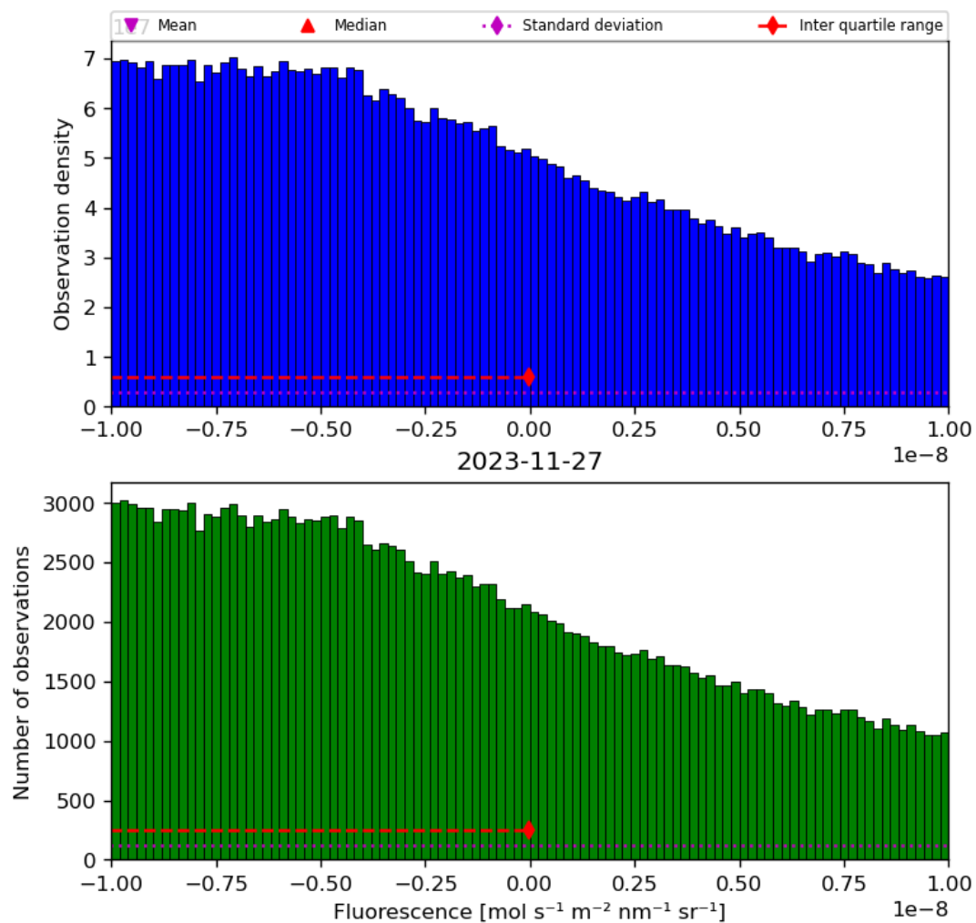
Figure 32: Histogram of “Fluorescence” for 2023-11-26 to 2023-11-28
