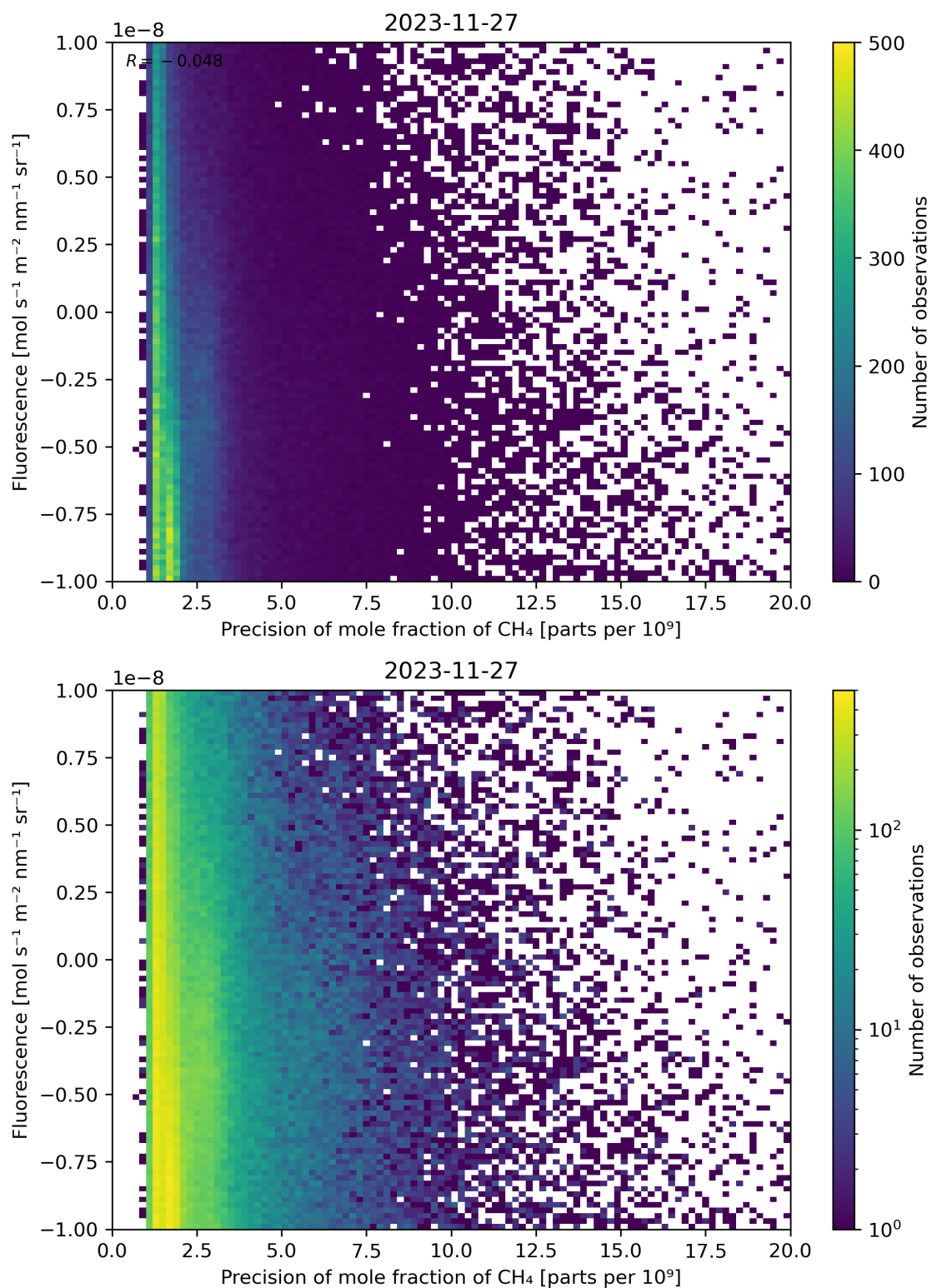
Figure 81: Scatter density plot of “Precision of mole fraction of \text{CH}_4 ” against “Fluorescence” for 2023-11-26 to 2023-11-28.
