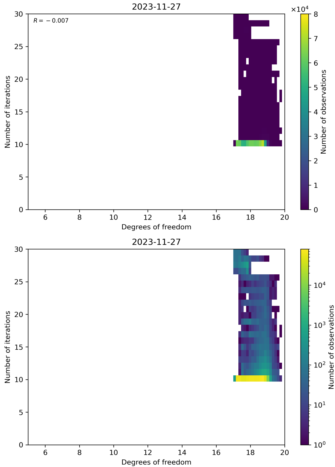
Figure 52: Scatter density plot of “Degrees of freedom” against “Number of iterations” for 2023-11-26 to 2023-11-28.
