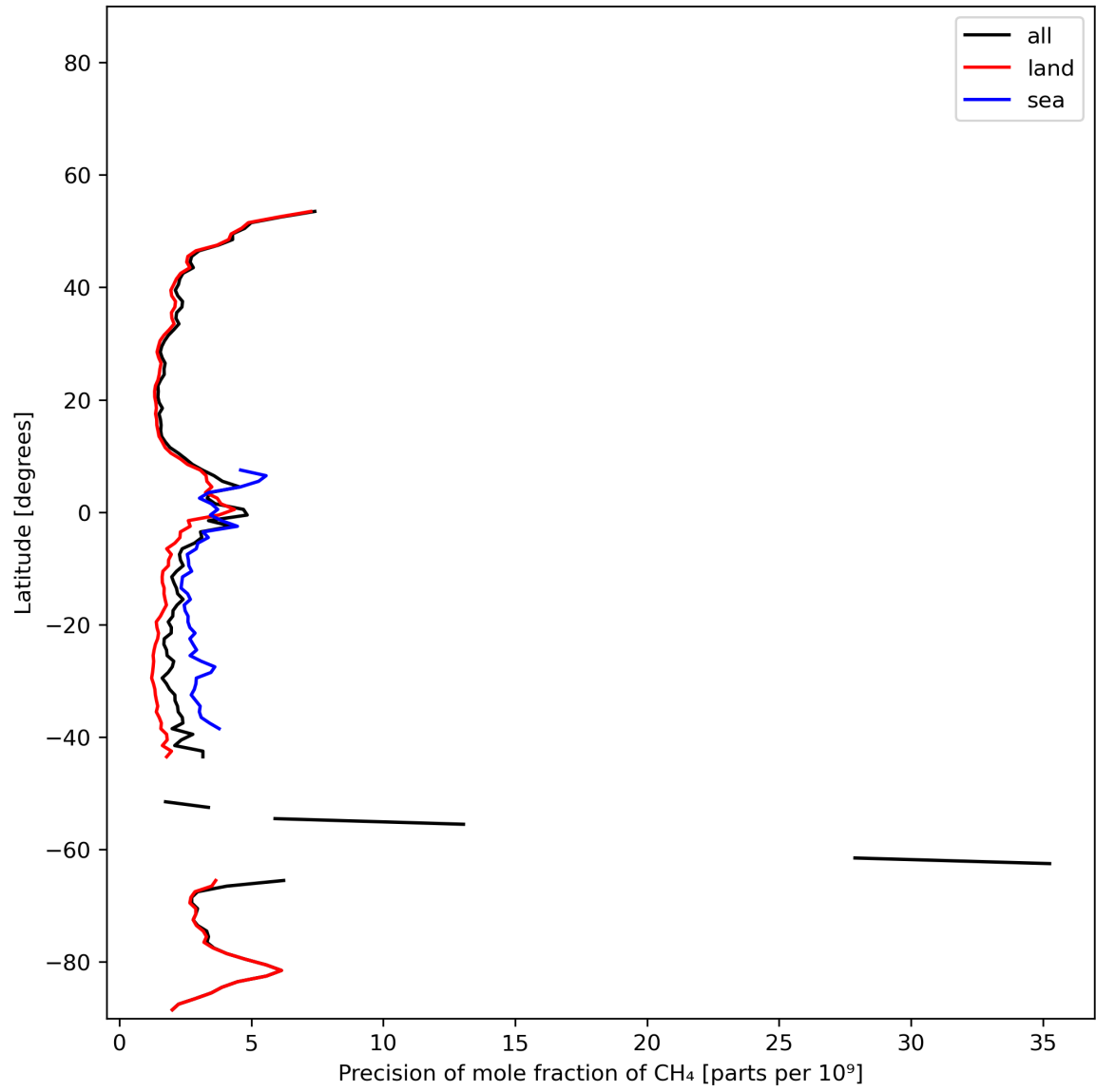
Figure 13: Zonal average of “Precision of mole fraction of CH 4 ” for 2023-11-26 to 2023-11-28.
