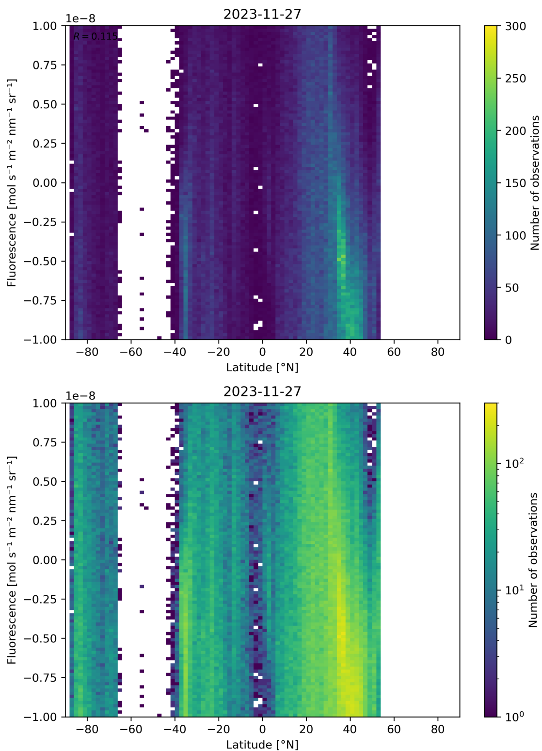
Figure 56: Scatter density plot of “Latitude” against “Fluorescence” for 2023-11-26 to 2023-11-28.
