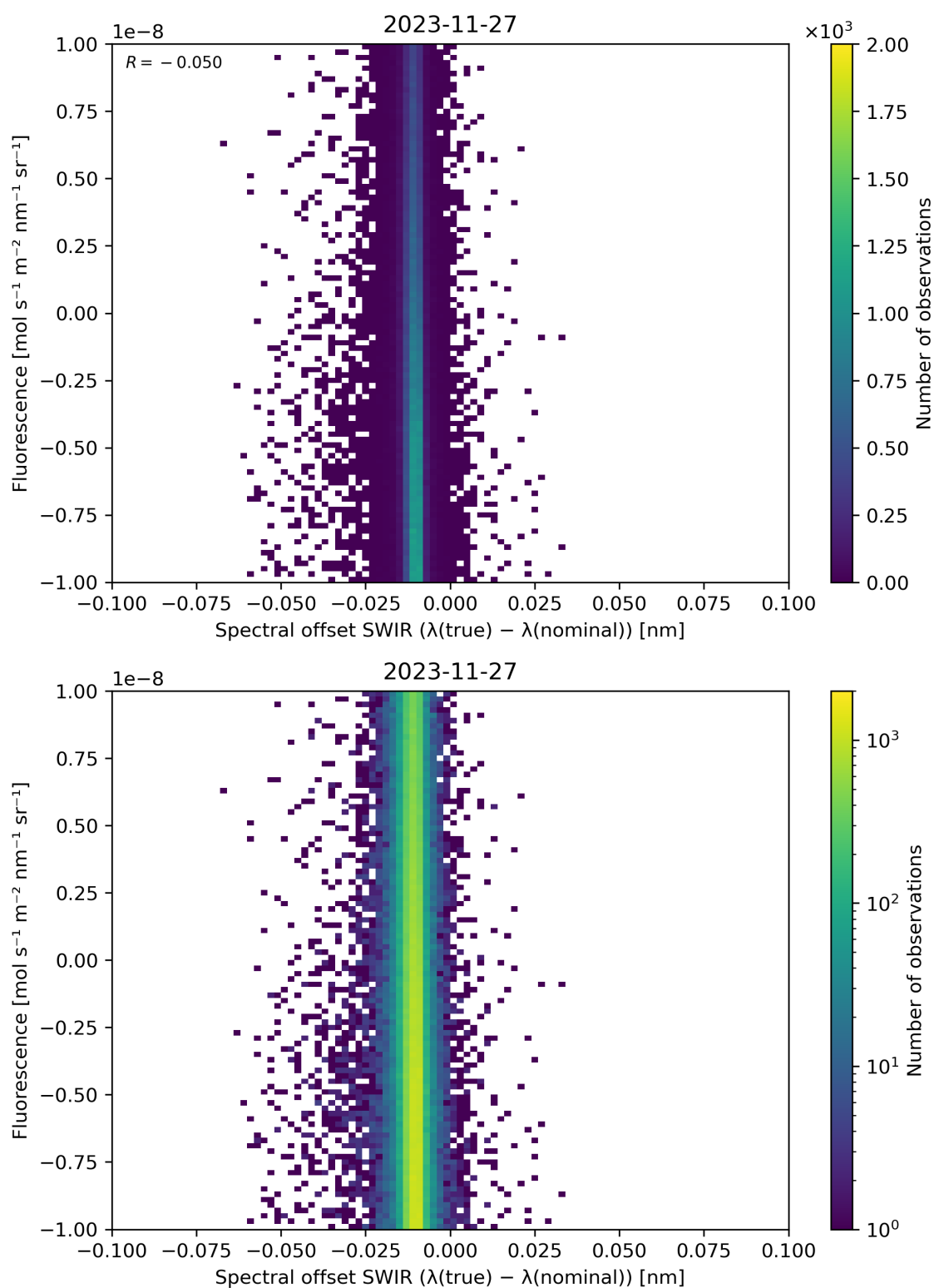
Figure 120: Scatter density plot of “Spectral offset SWIR ( \lambda(\text{true}) - \lambda(\text{nominal}) )” against “Fluorescence” for 2023-11-26 to 2023-11-28.
