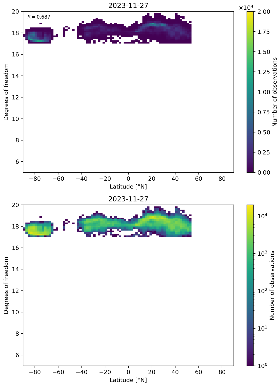
Figure 55: Scatter density plot of “Latitude” against “Degrees of freedom” for 2023-11-26 to 2023-11-28.
