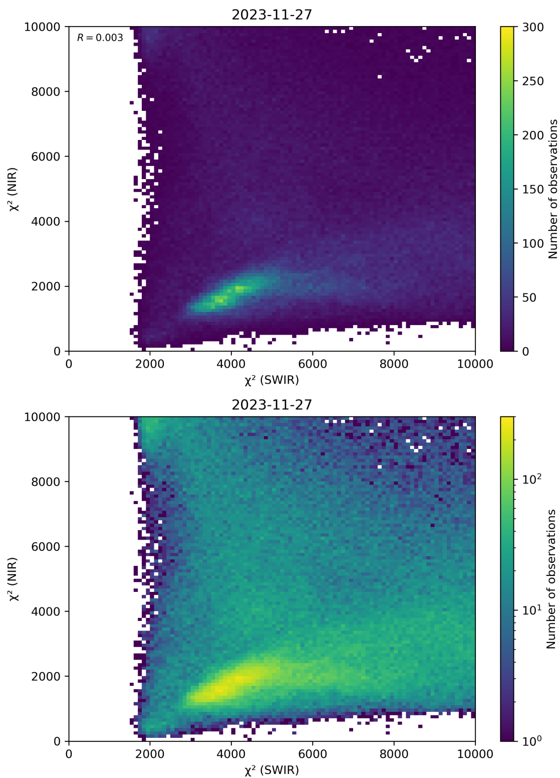
Figure 47: Scatter density plot of “ \chi^2 (SWIR)” against “ \chi^2 (NIR)” for 2023-11-26 to 2023-11-28.
