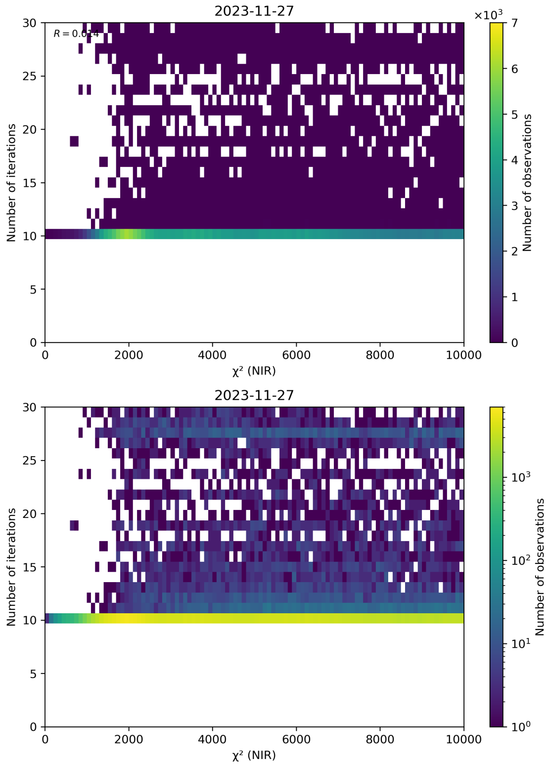
Figure 46: Scatter density plot of “ \chi^2 (NIR)” against “Number of iterations” for 2023-11-26 to 2023-11-28.
