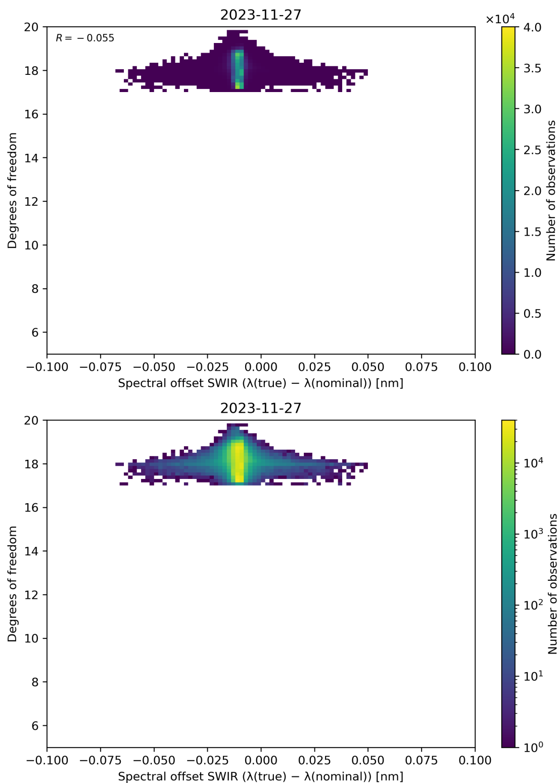
Figure 119: Scatter density plot of “Spectral offset SWIR ( \lambda(\text{true}) - \lambda(\text{nominal}) )” against “Degrees of freedom” for 2023-11-26 to 2023-11-28.
