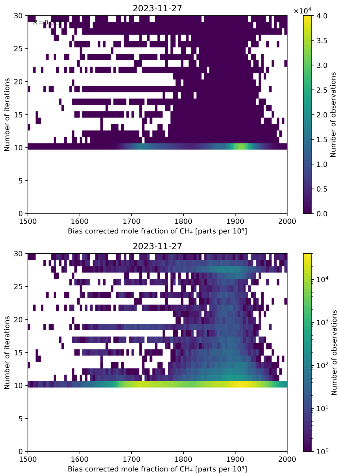
Figure 67: Scatter density plot of “Bias corrected mole fraction of \text{CH}_4 ” against “Number of iterations” for 2023-11-26 to 2023-11-28.
