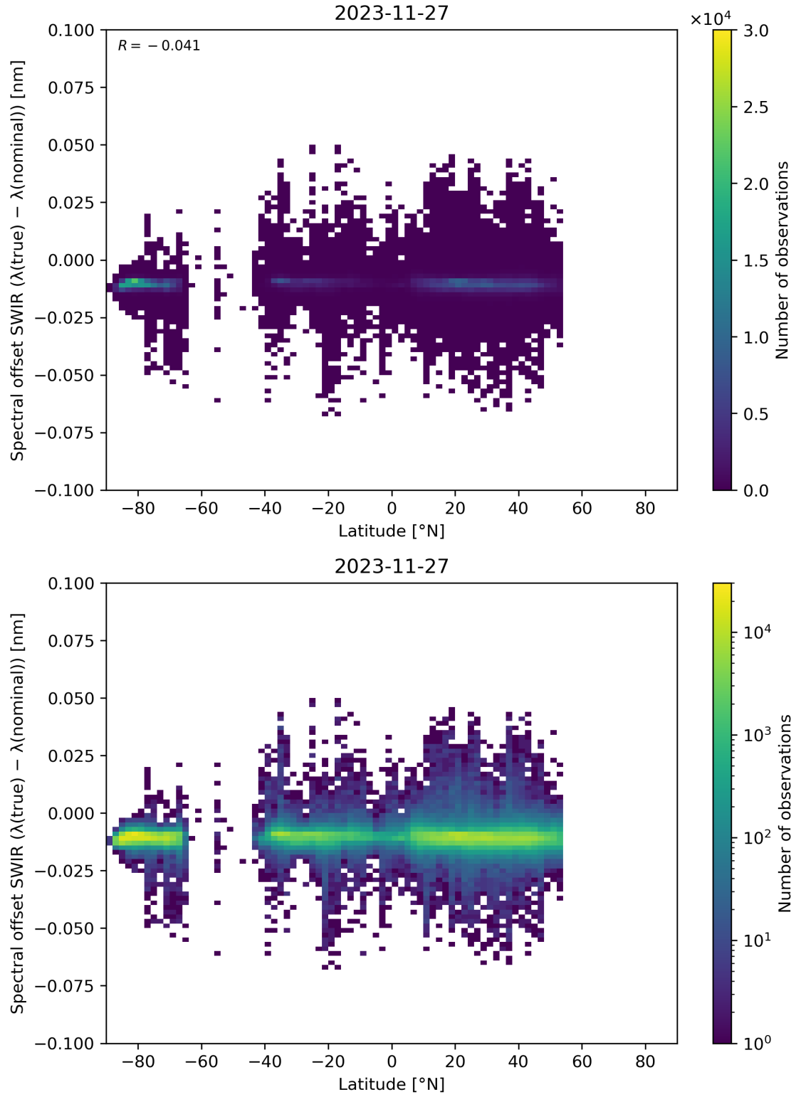
Figure 62: Scatter density plot of “Latitude” against “Spectral offset SWIR ( \lambda(\text{true}) - \lambda(\text{nominal}) )” for 2023-11-26 to 2023-11-28.
