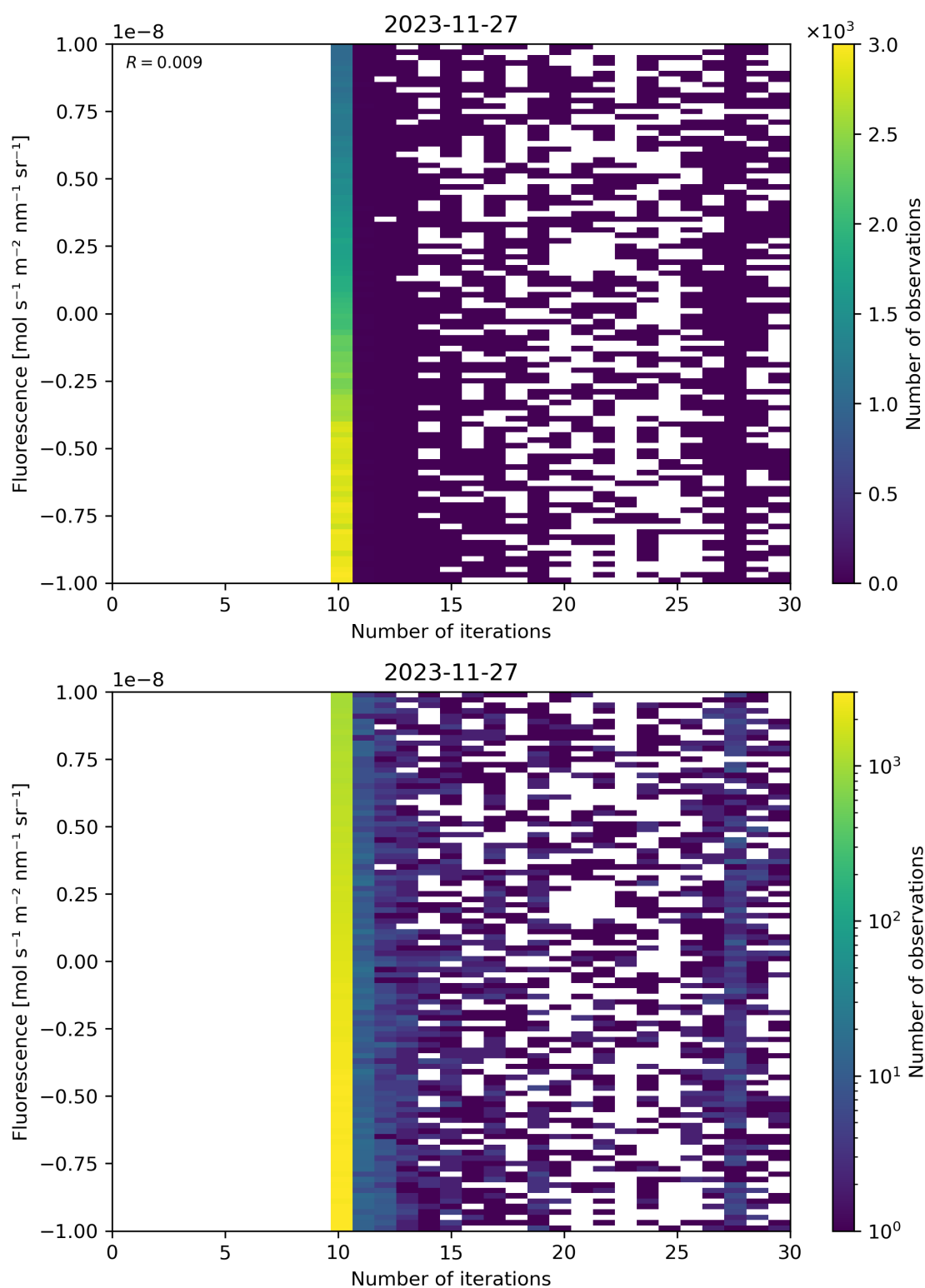
Figure 87: Scatter density plot of “Number of iterations” against “Fluorescence” for 2023-11-26 to 2023-11-28.
