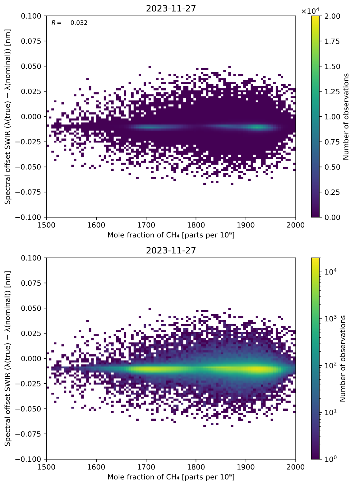
Figure 86: Scatter density plot of “Mole fraction of CH 4 ” against “Spectral offset SWIR ( \lambda(\text{true}) - \lambda(\text{nominal}) )” for 2023-11-26 to 2023-11-28.
