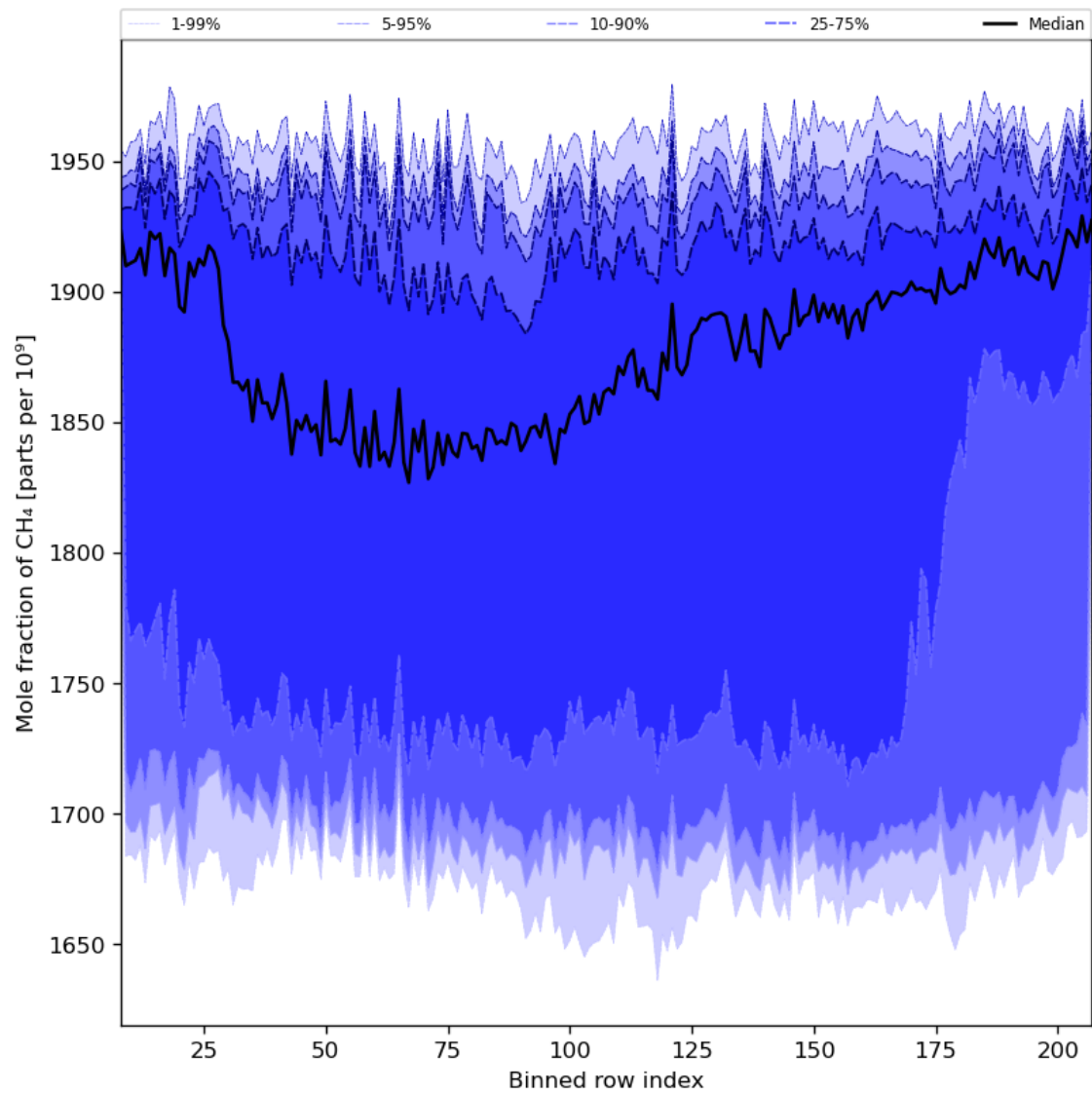
Figure 34: Along track statistics of “Mole fraction of CH 4 ” for 2023-11-26 to 2023-11-28
