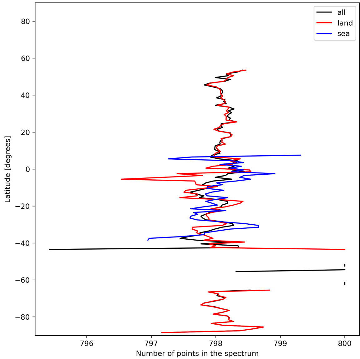
Figure 15: Zonal average of “Number of points in the spectrum” for 2023-11-26 to 2023-11-28.
