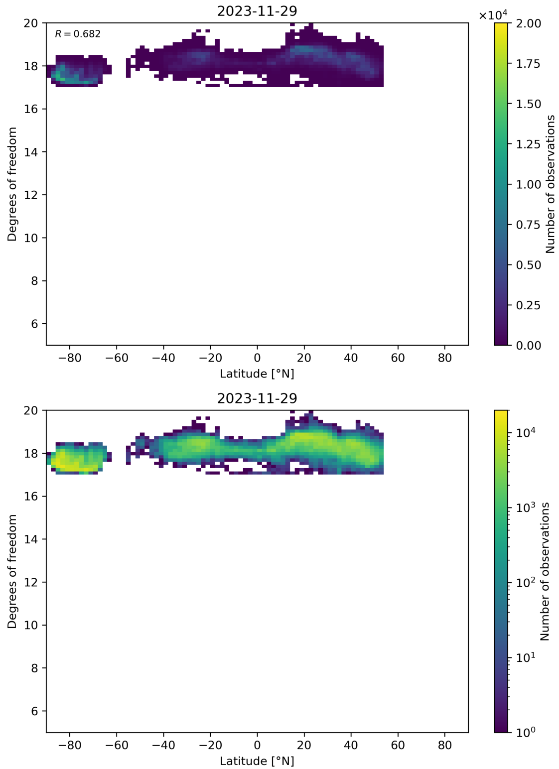
Figure 55: Scatter density plot of “Latitude” against “Degrees of freedom” for 2023-11-28 to 2023-11-30.
