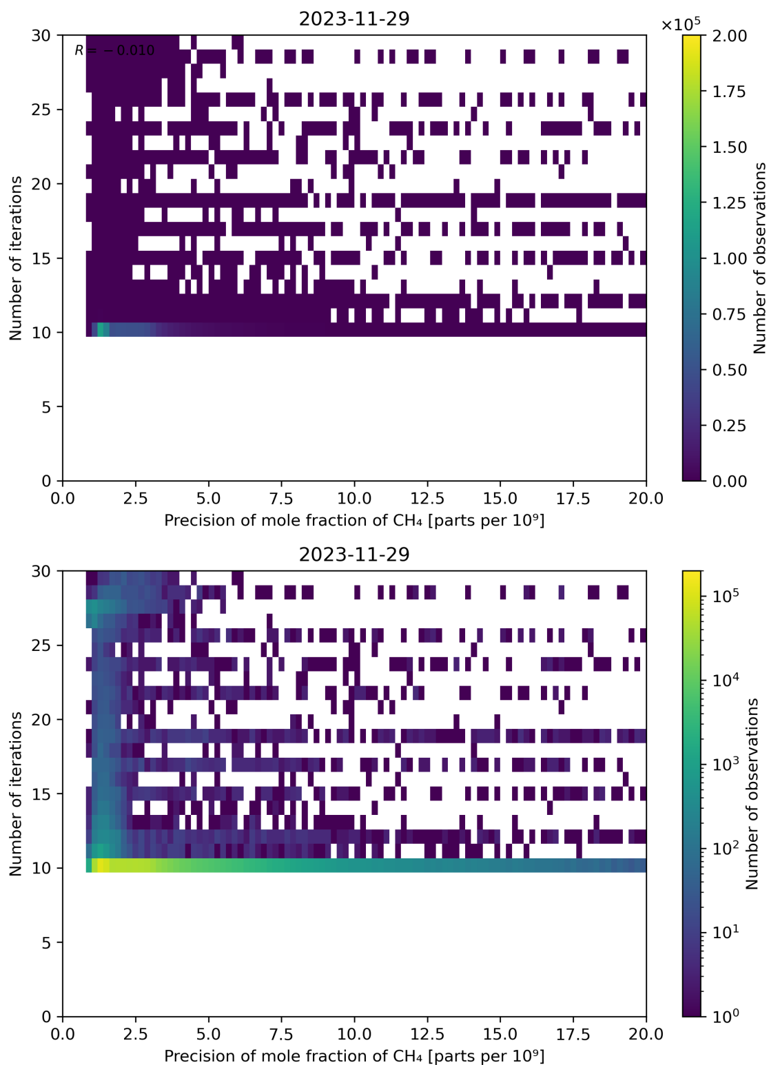
Figure 83: Scatter density plot of “Precision of mole fraction of CH 4 ” against “Number of iterations” for 2023-11-28 to 2023-11-30.
