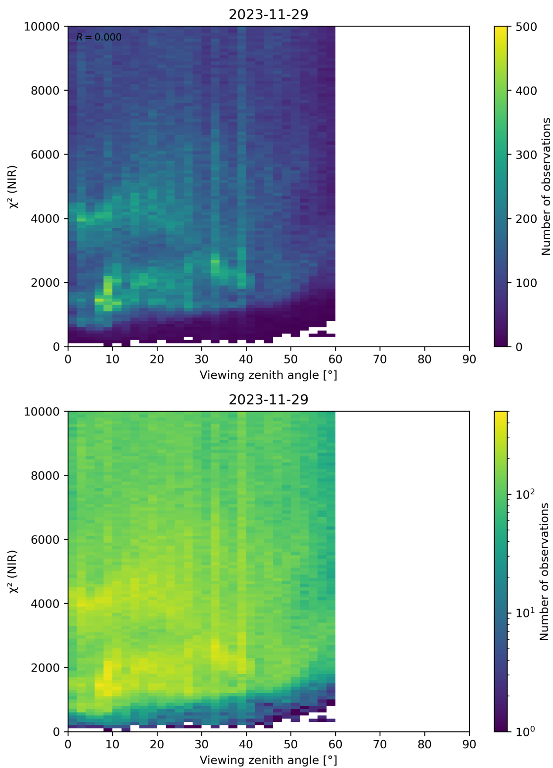
Figure 105: Scatter density plot of “Viewing zenith angle” against “ \chi^2 (NIR)” for 2023-11-28 to 2023-11-30.
