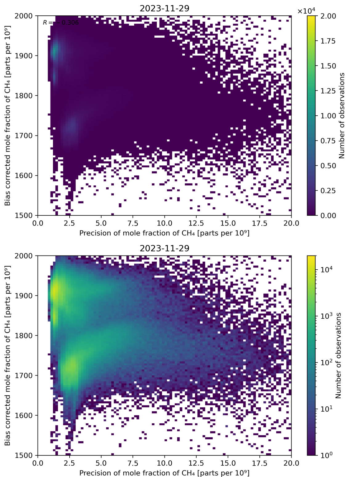
Figure 82: Scatter density plot of “Precision of mole fraction of \text{CH}_4 ” against “Bias corrected mole fraction of \text{CH}_4 ” for 2023-11-28 to 2023-11-30.
