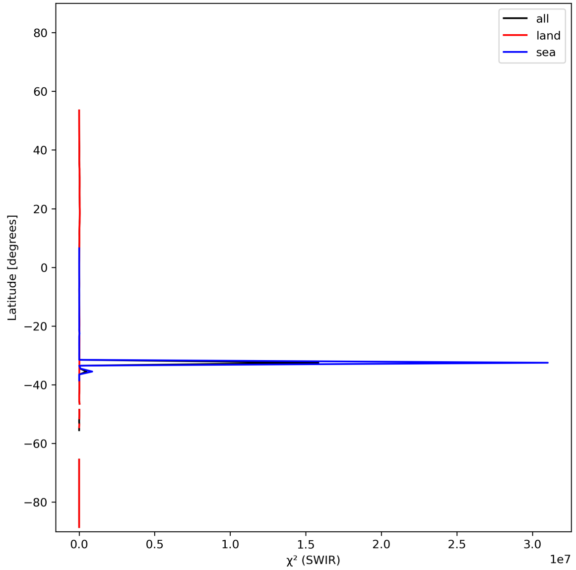
Figure 17: Zonal average of “ \chi^2 (SWIR)” for 2023-11-28 to 2023-11-30.
