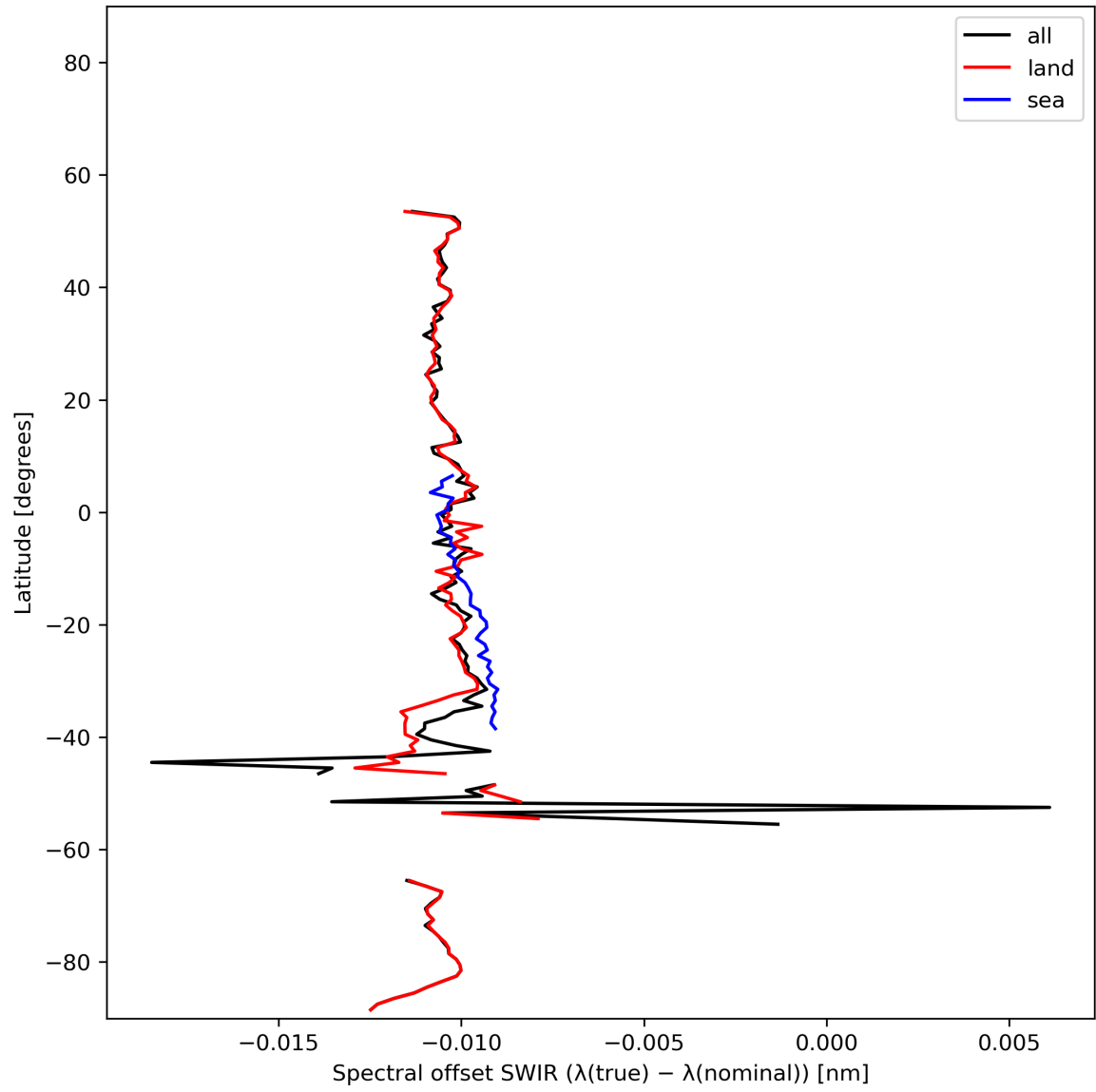
Figure 16: Zonal average of “Spectral offset SWIR ( \lambda(\text{true}) - \lambda(\text{nominal}) )” for 2023-11-28 to 2023-11-30.
