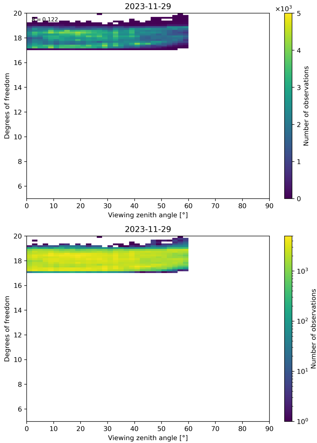
Figure 107: Scatter density plot of “Viewing zenith angle” against “Degrees of freedom” for 2023-11-28 to 2023-11-30.
