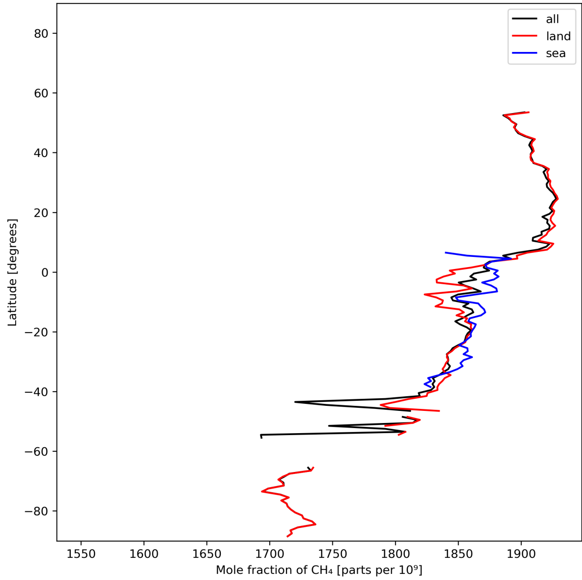
Figure 12: Zonal average of “Mole fraction of CH 4 ” for 2023-11-28 to 2023-11-30.
