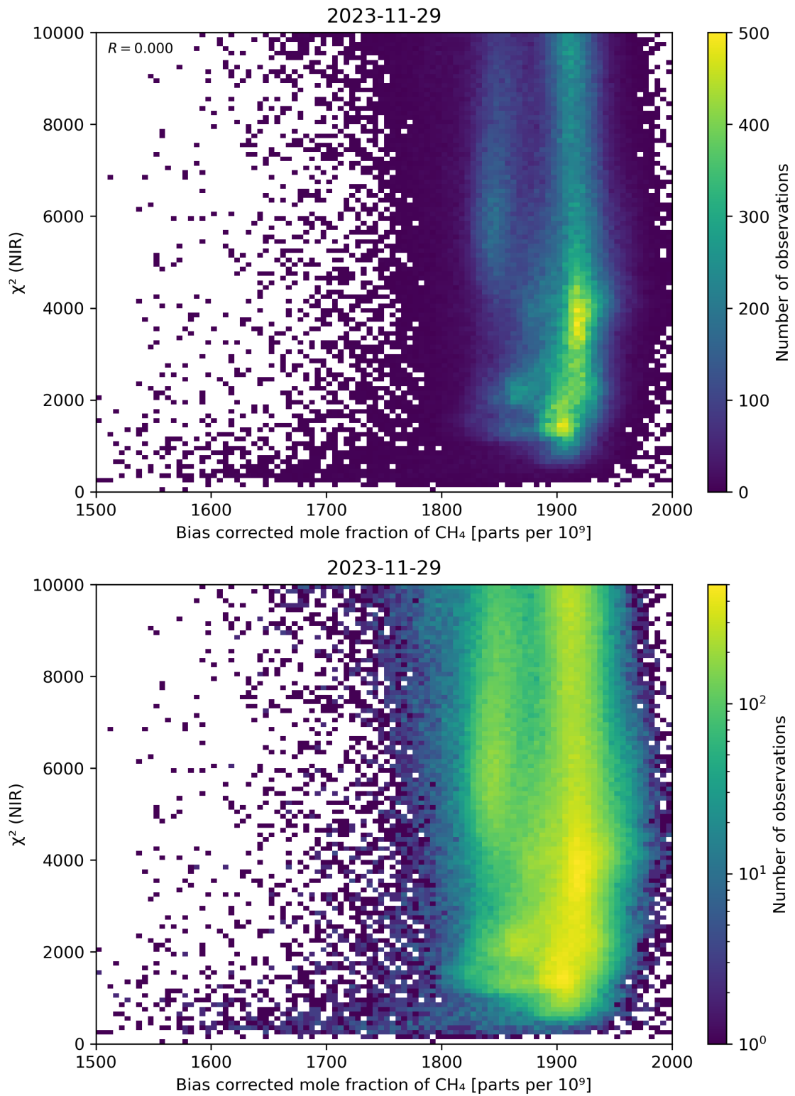
Figure 63: Scatter density plot of “Bias corrected mole fraction of CH 4 ” against “ \chi^2 (NIR)” for 2023-11-28 to 2023-11-30.
