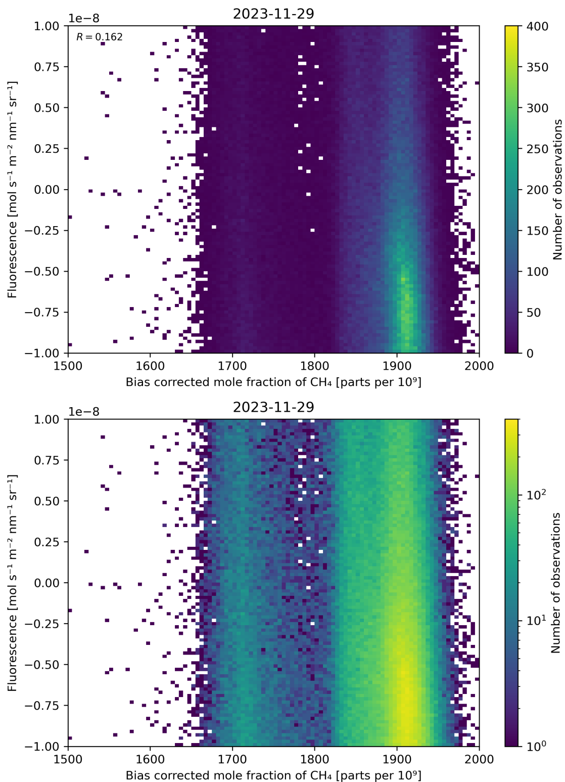
Figure 66: Scatter density plot of “Bias corrected mole fraction of \text{CH}_4 ” against “Fluorescence” for 2023-11-28 to 2023-11-30.
