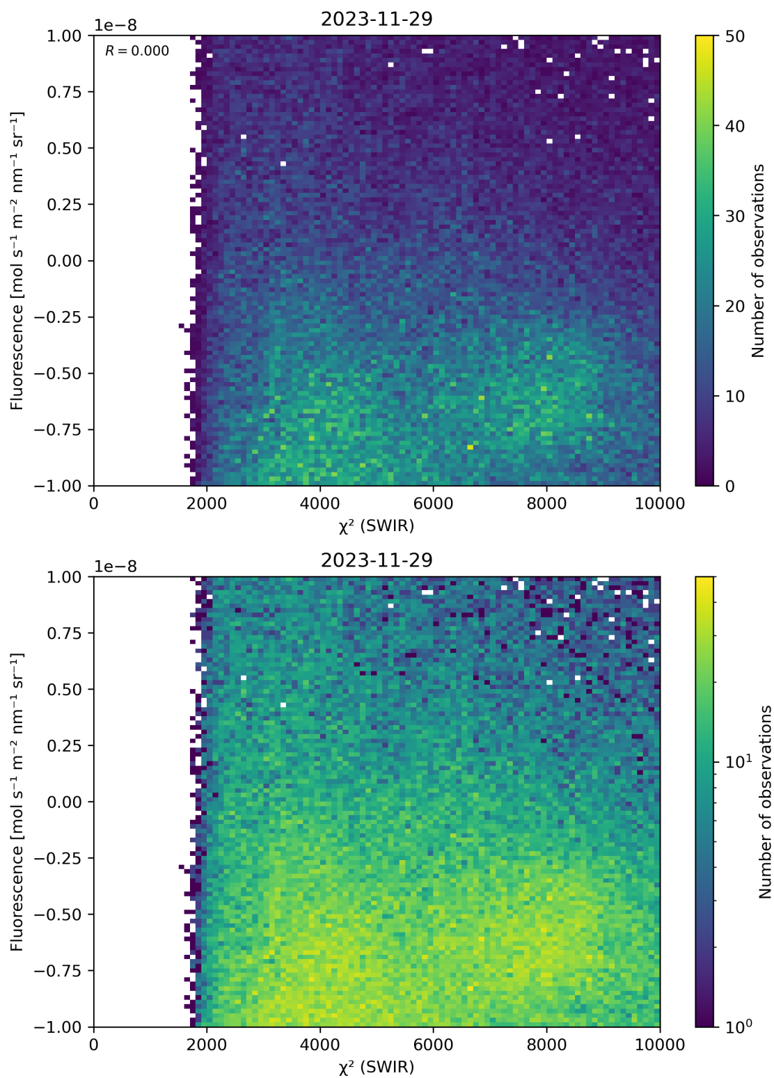
Figure 49: Scatter density plot of “ \chi^2 (SWIR)” against “Fluorescence” for 2023-11-28 to 2023-11-30.
