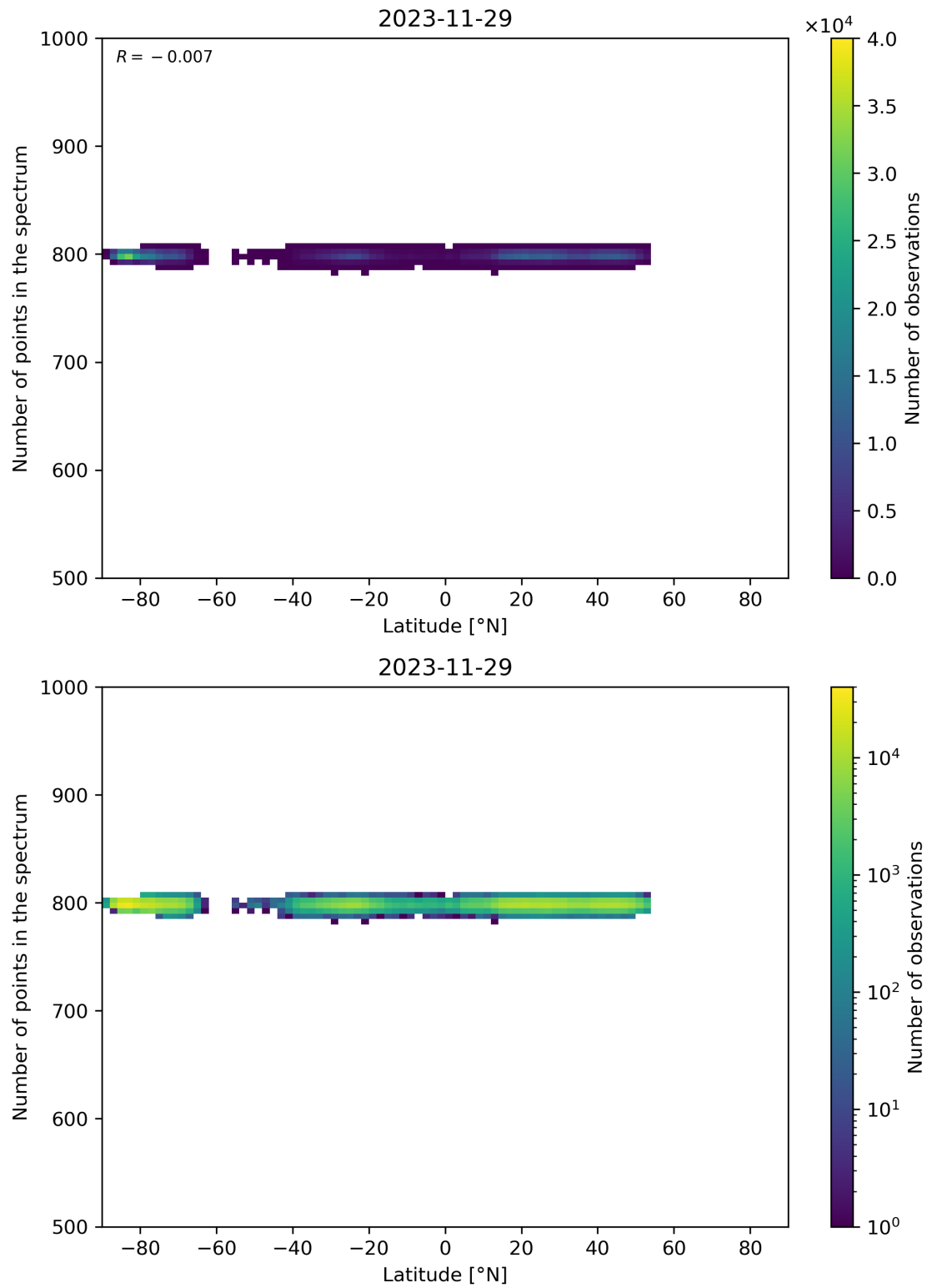
Figure 61: Scatter density plot of “Latitude” against “Number of points in the spectrum” for 2023-11-28 to 2023-11-30.
