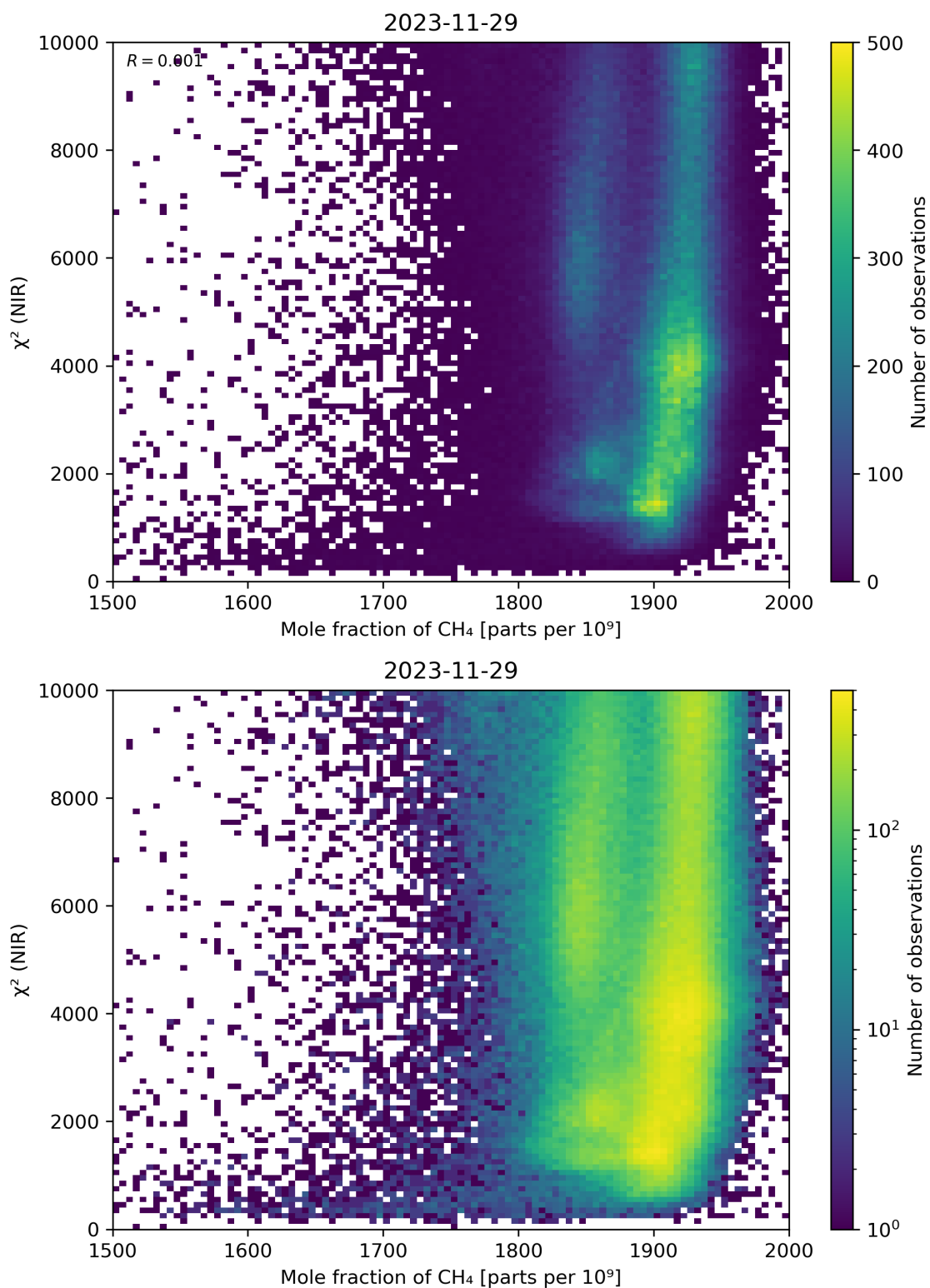
Figure 70: Scatter density plot of “Mole fraction of \text{CH}_4 ” against “ \chi^2 (NIR)” for 2023-11-28 to 2023-11-30.
