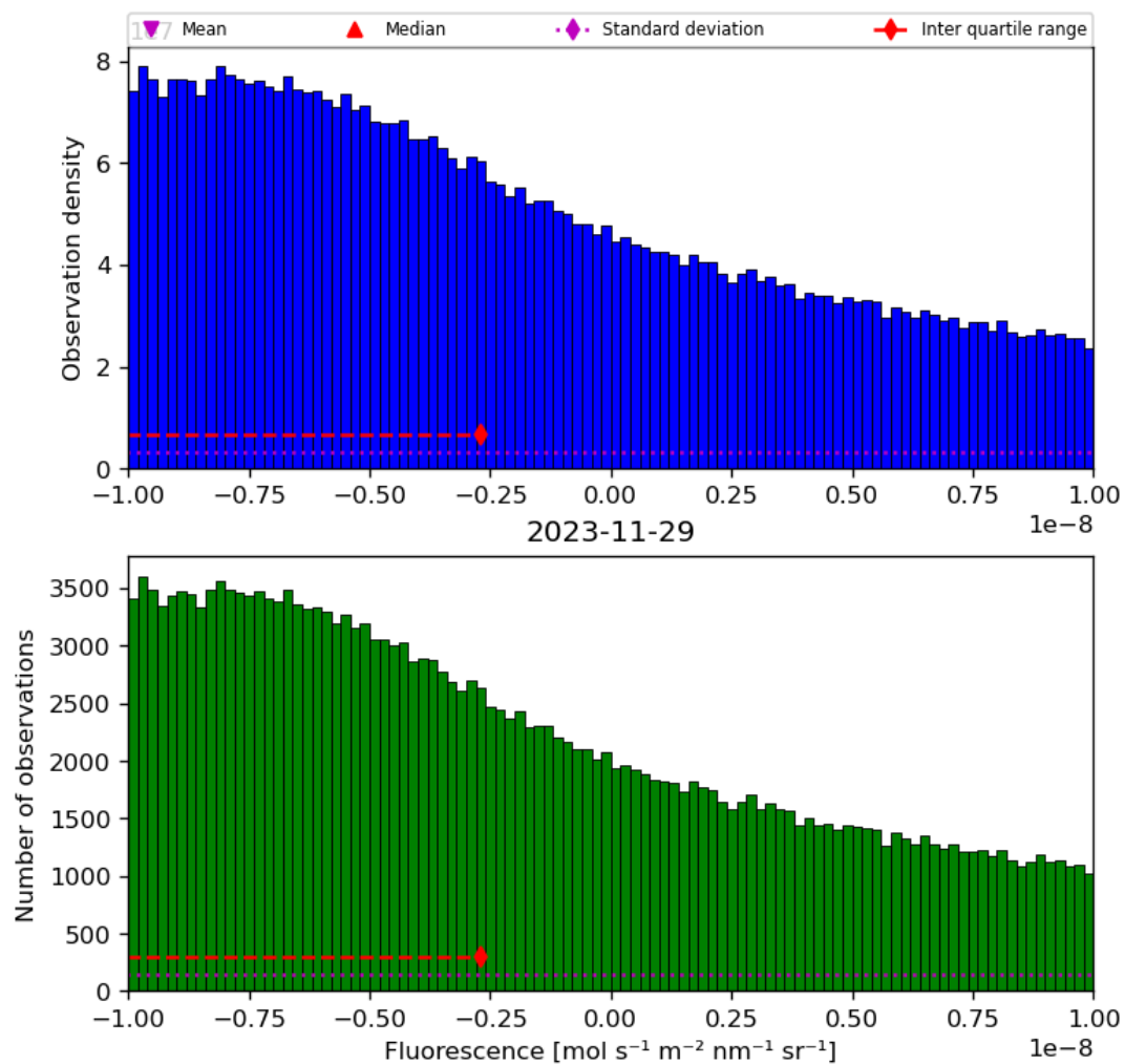
Figure 32: Histogram of “Fluorescence” for 2023-11-28 to 2023-11-30
