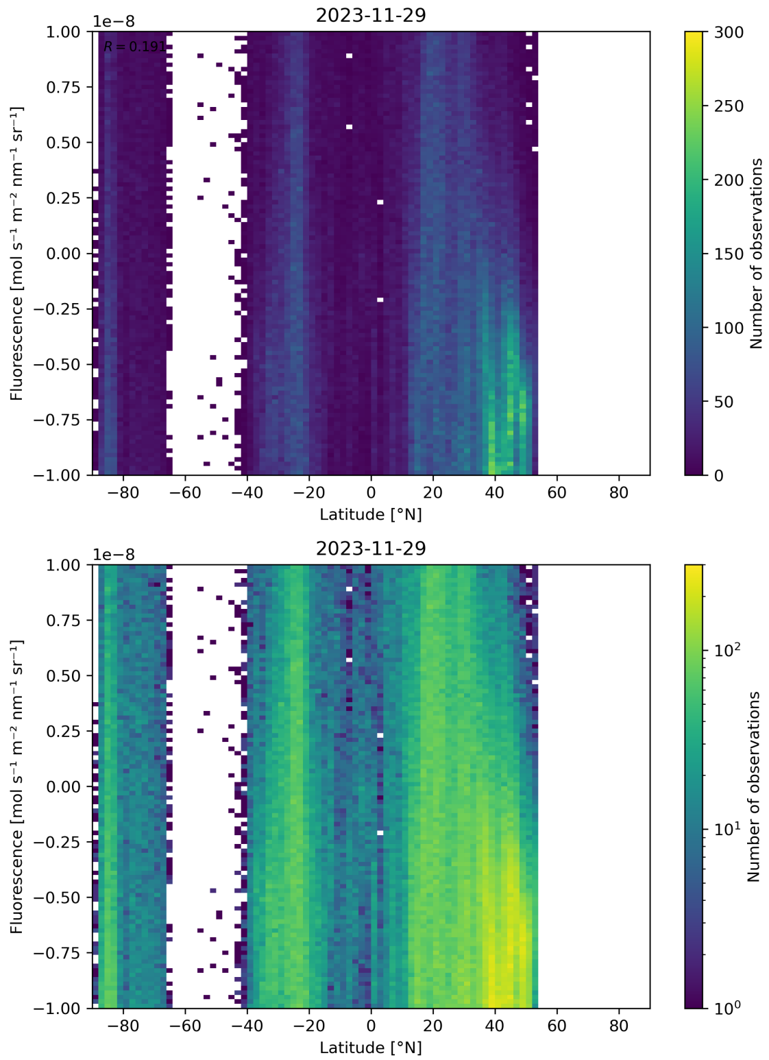
Figure 56: Scatter density plot of “Latitude” against “Fluorescence” for 2023-11-28 to 2023-11-30.
