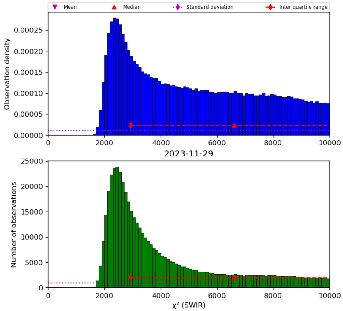
Figure 28: Histogram of “ \chi^2 (SWIR)” for 2023-11-28 to 2023-11-30
