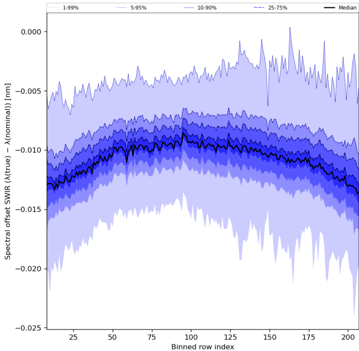
Figure 38: Along track statistics of “Spectral offset SWIR ( \lambda(\text{true}) - \lambda(\text{nominal}) )” for 2023-11-28 to 2023-11-30
