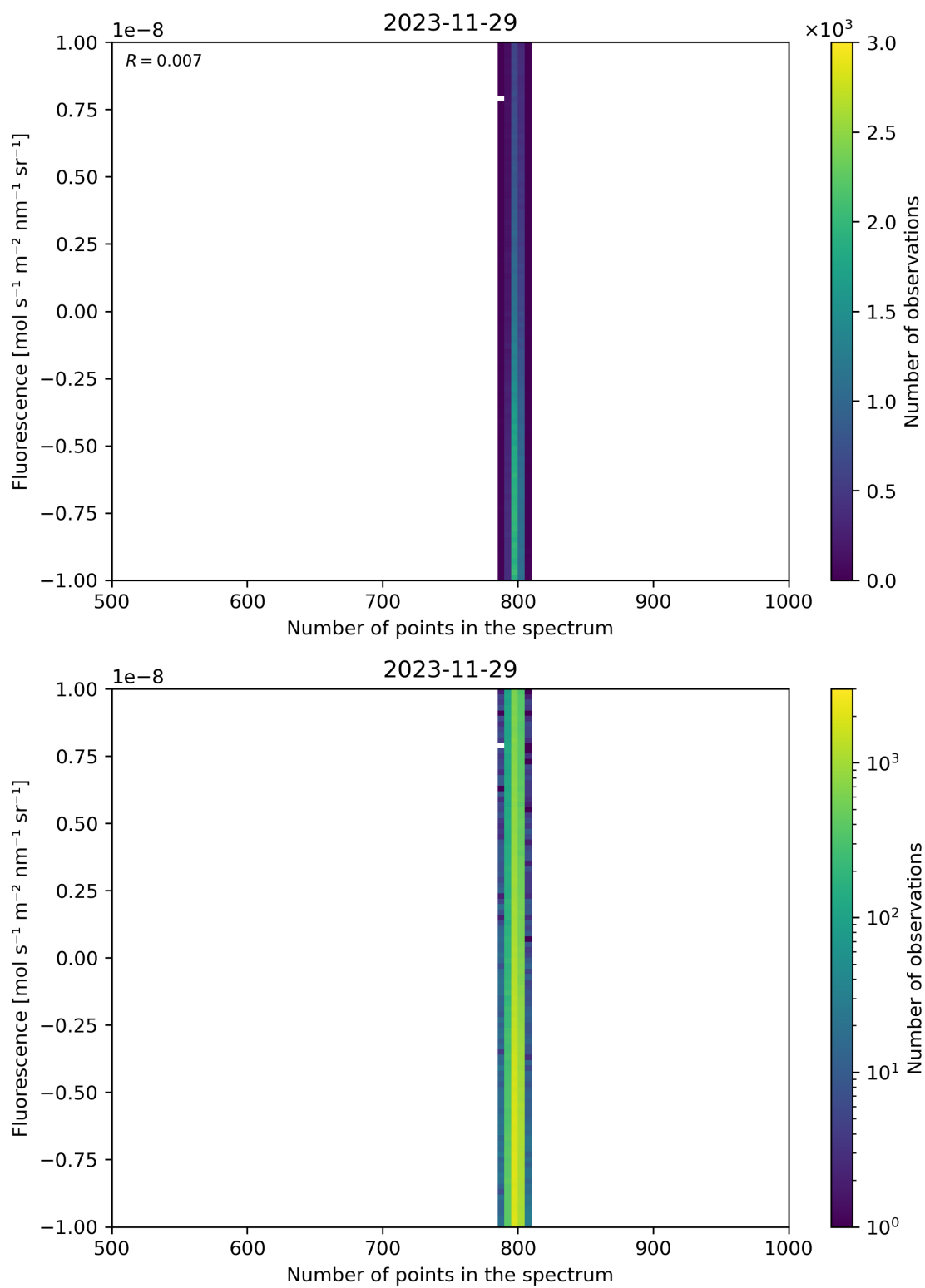
Figure 91: Scatter density plot of “Number of points in the spectrum” against “Fluorescence” for 2023-11-28 to 2023-11-30.
