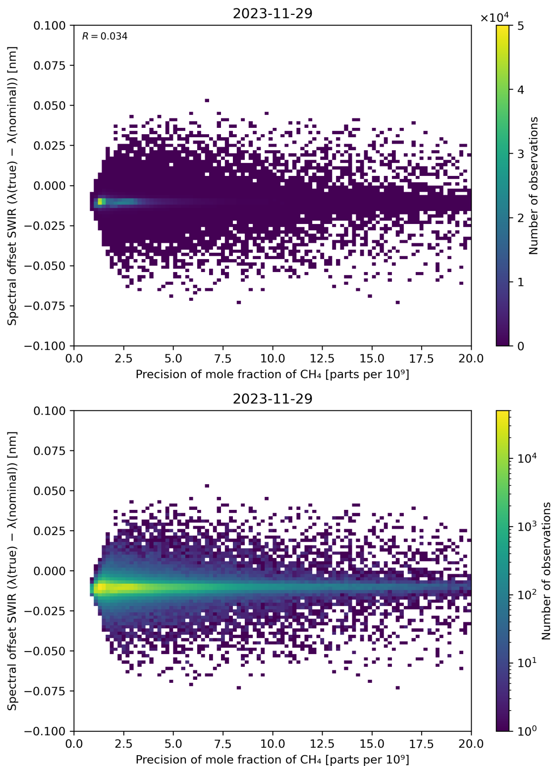
Figure 85: Scatter density plot of “Precision of mole fraction of CH 4 ” against “Spectral offset SWIR ( \lambda(\text{true}) - \lambda(\text{nominal}) )” for 2023-11-28 to 2023-11-30.
