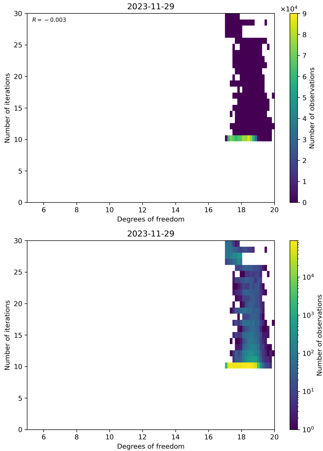
Figure 52: Scatter density plot of “Degrees of freedom” against “Number of iterations” for 2023-11-28 to 2023-11-30.
