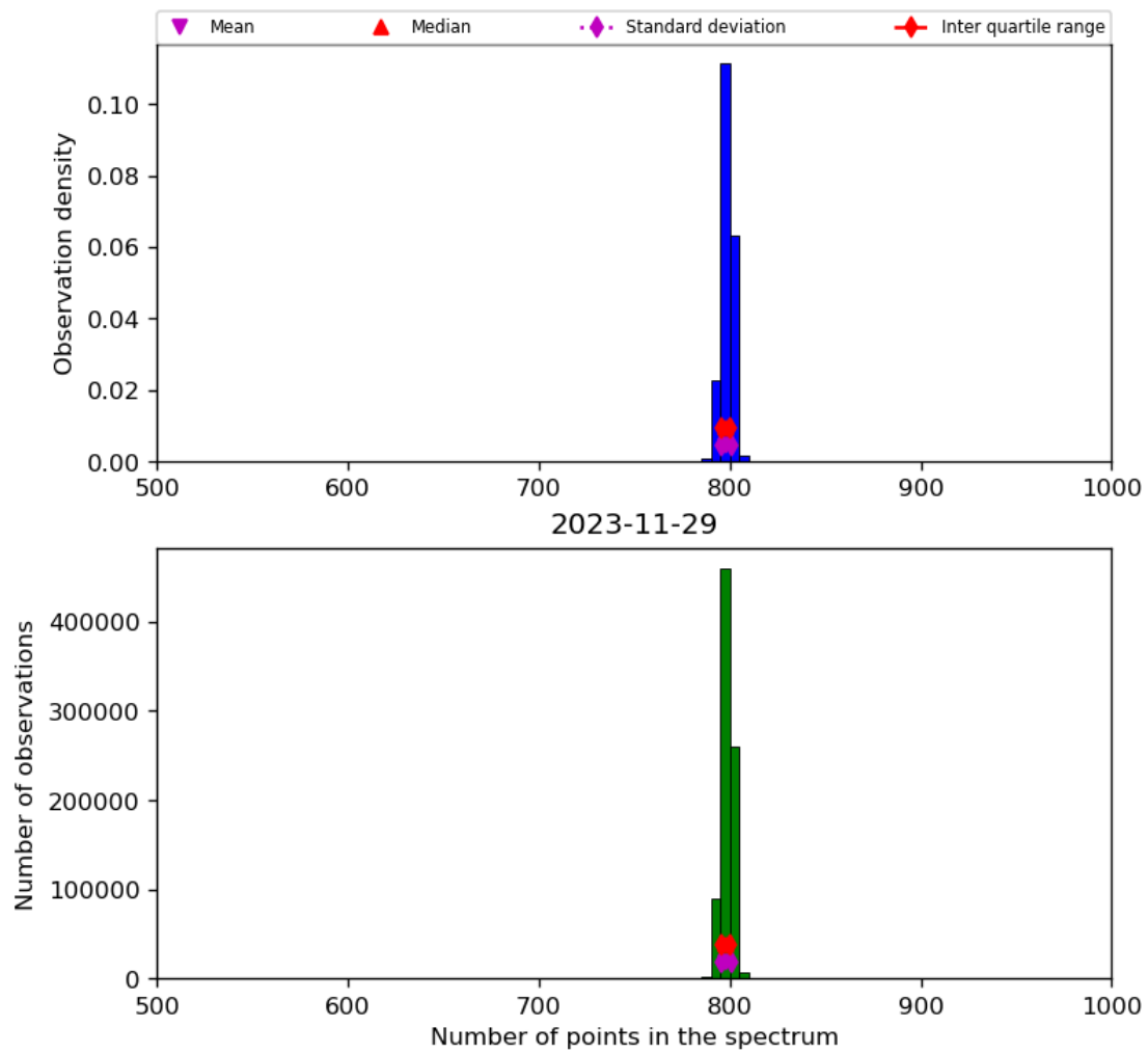
Figure 26: Histogram of “Number of points in the spectrum” for 2023-11-28 to 2023-11-30
