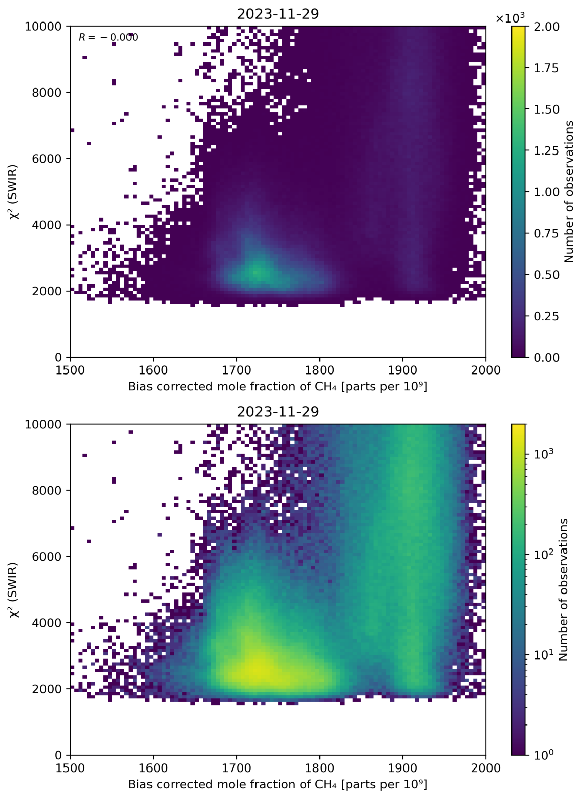
Figure 64: Scatter density plot of “Bias corrected mole fraction of \text{CH}_4 ” against “ \chi^2 (SWIR)” for 2023-11-28 to 2023-11-30.
