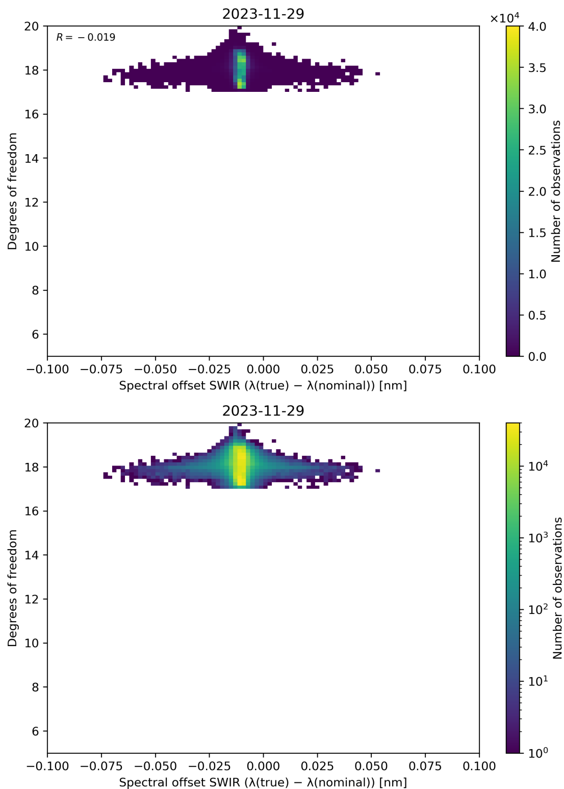
Figure 119: Scatter density plot of “Spectral offset SWIR ( \lambda(\text{true}) - \lambda(\text{nominal}) )” against “Degrees of freedom” for 2023-11-28 to 2023-11-30.
