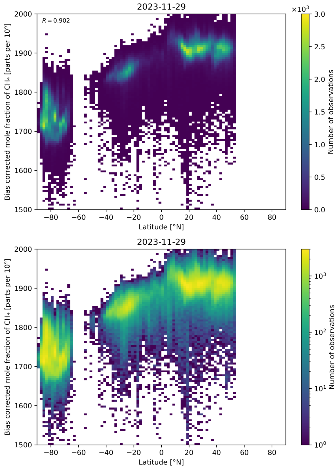
Figure 58: Scatter density plot of “Latitude” against “Bias corrected mole fraction of CH 4 ” for 2023-11-28 to 2023-11-30.
