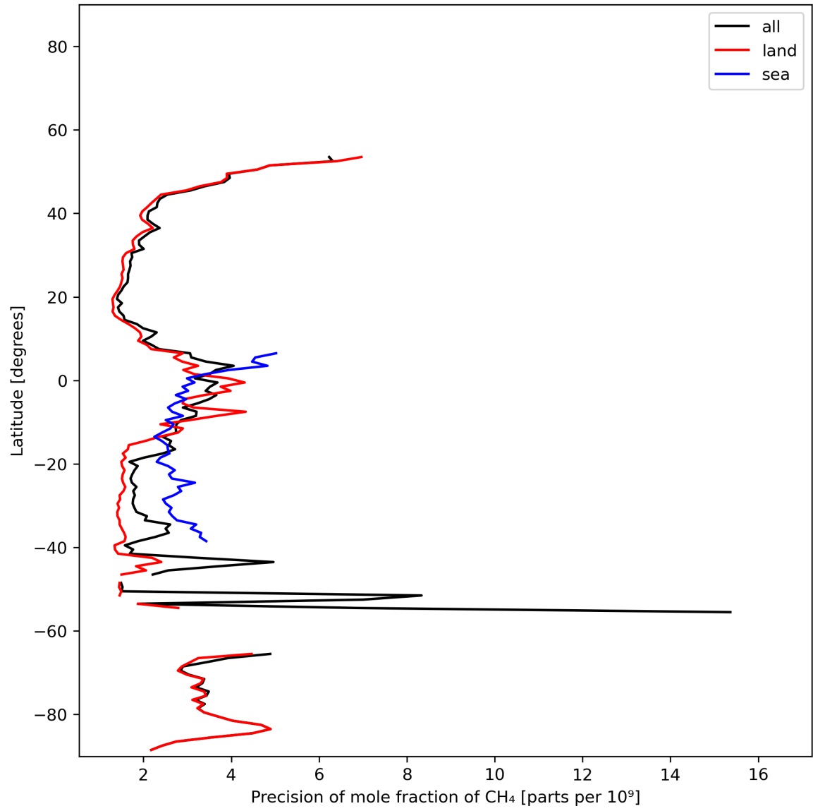
Figure 13: Zonal average of “Precision of mole fraction of CH 4 ” for 2023-11-28 to 2023-11-30.
