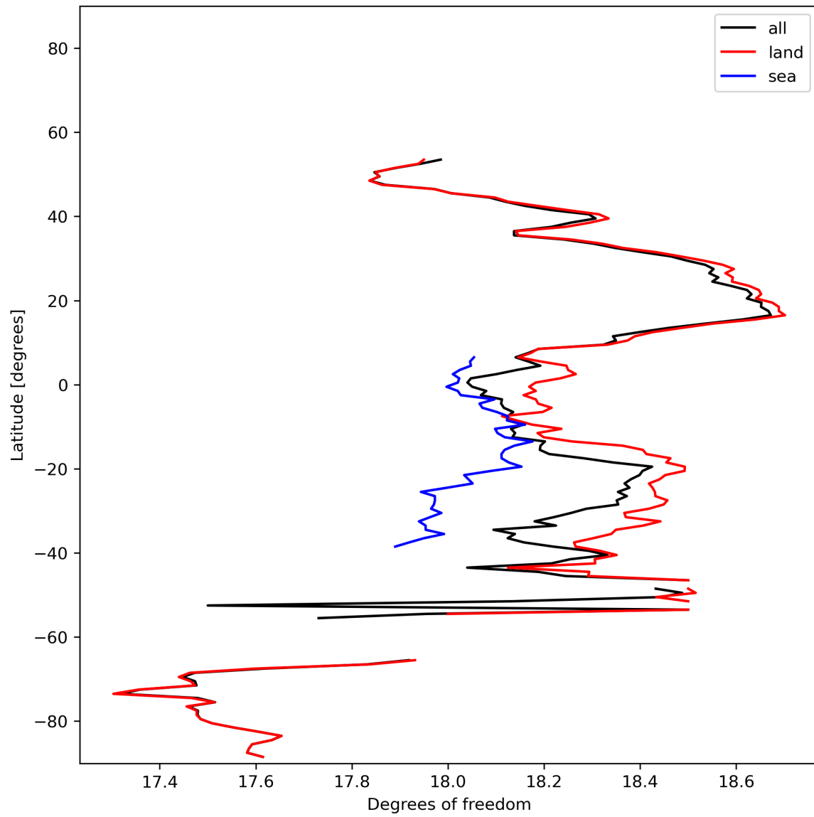
Figure 19: Zonal average of “Degrees of freedom” for 2023-11-28 to 2023-11-30.
