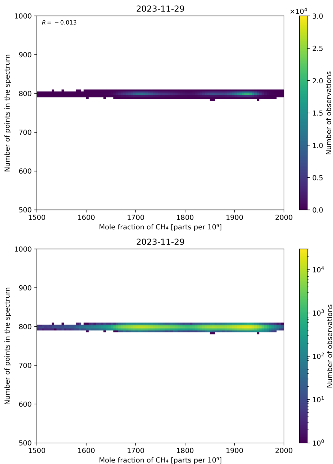
Figure 77: Scatter density plot of “Mole fraction of CH 4 ” against “Number of points in the spectrum” for 2023-11-28 to 2023-11-30.
