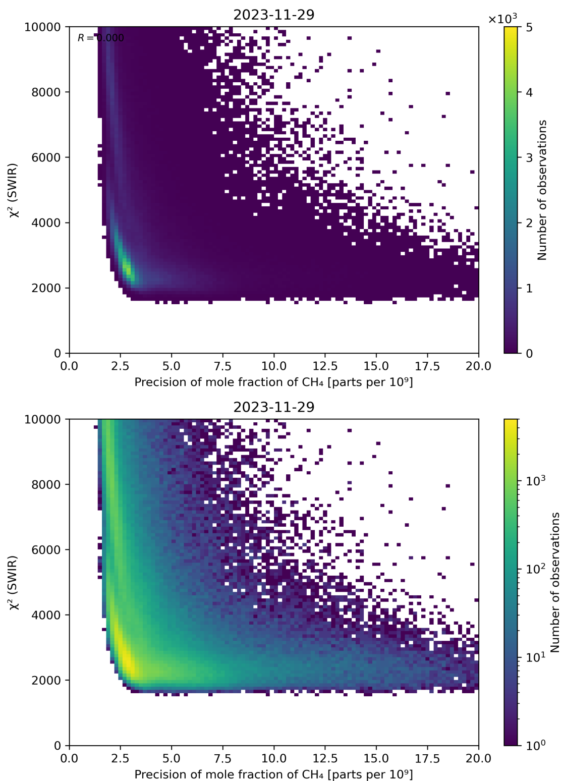
Figure 79: Scatter density plot of “Precision of mole fraction of \text{CH}_4 ” against “ \chi^2 (SWIR)” for 2023-11-28 to 2023-11-30.
