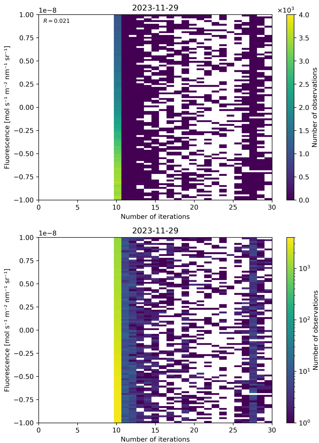
Figure 87: Scatter density plot of “Number of iterations” against “Fluorescence” for 2023-11-28 to 2023-11-30.
