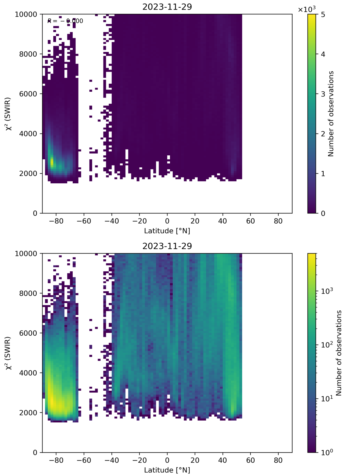
Figure 54: Scatter density plot of “Latitude” against “ \chi^2 (SWIR)” for 2023-11-28 to 2023-11-30.
