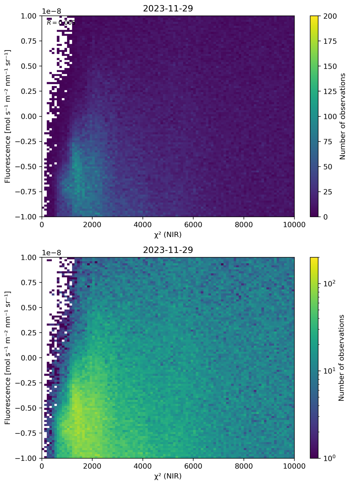
Figure 45: Scatter density plot of “ \chi^2 (NIR)” against “Fluorescence” for 2023-11-28 to 2023-11-30.
