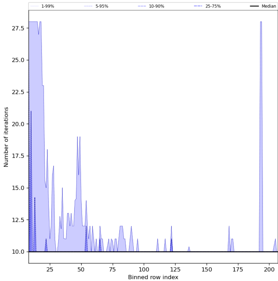
Figure 42: Along track statistics of “Number of iterations” for 2023-11-28 to 2023-11-30
