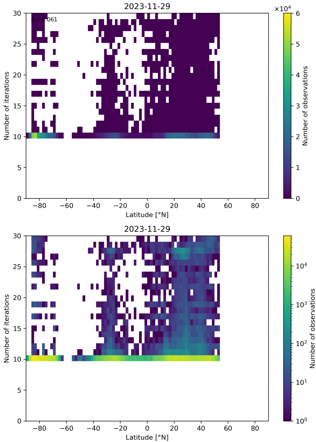
Figure 60: Scatter density plot of “Latitude” against “Number of iterations” for 2023-11-28 to 2023-11-30.
