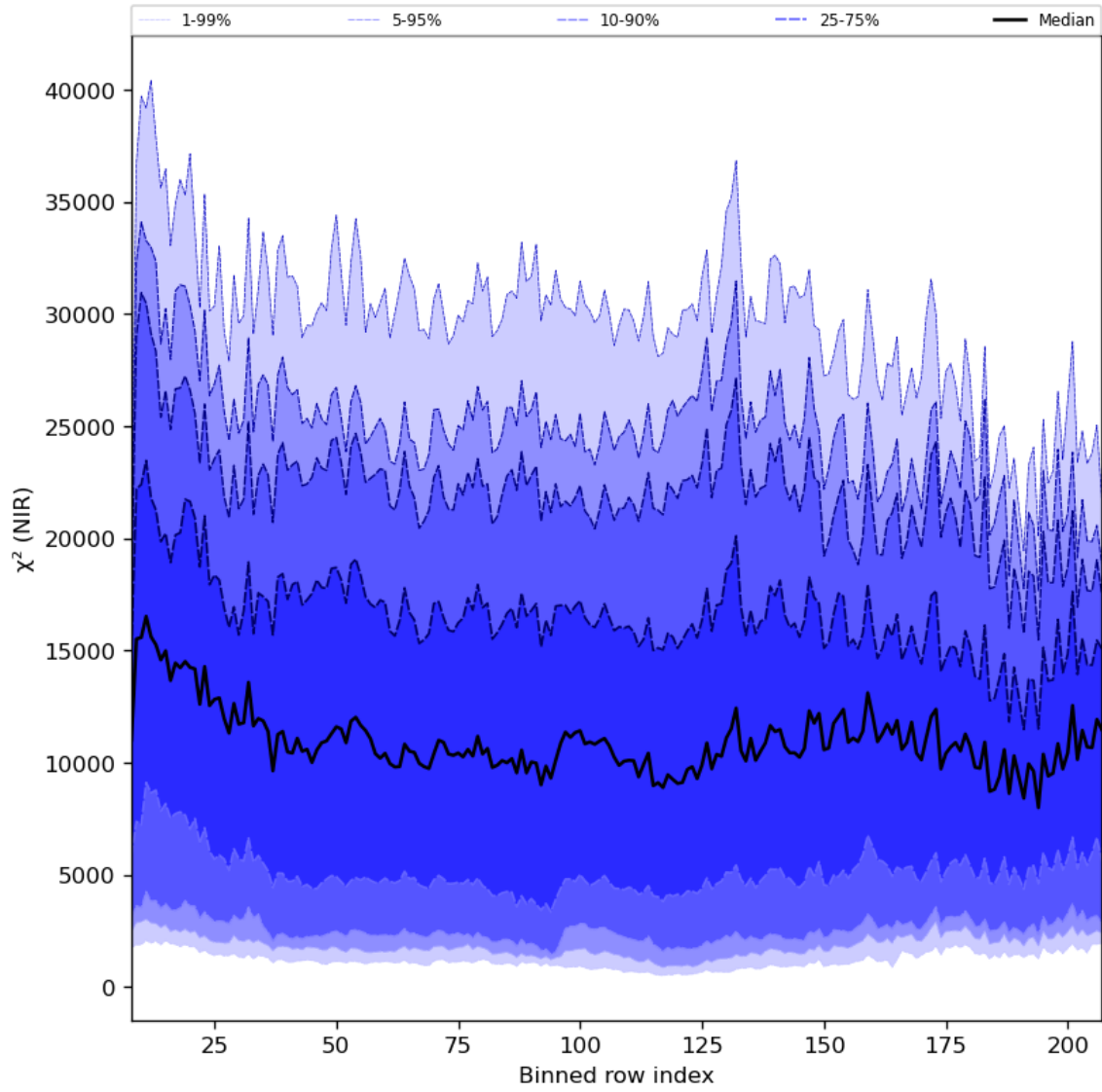
Figure 40: Along track statistics of “ \chi^2 (NIR)” for 2023-11-28 to 2023-11-30
