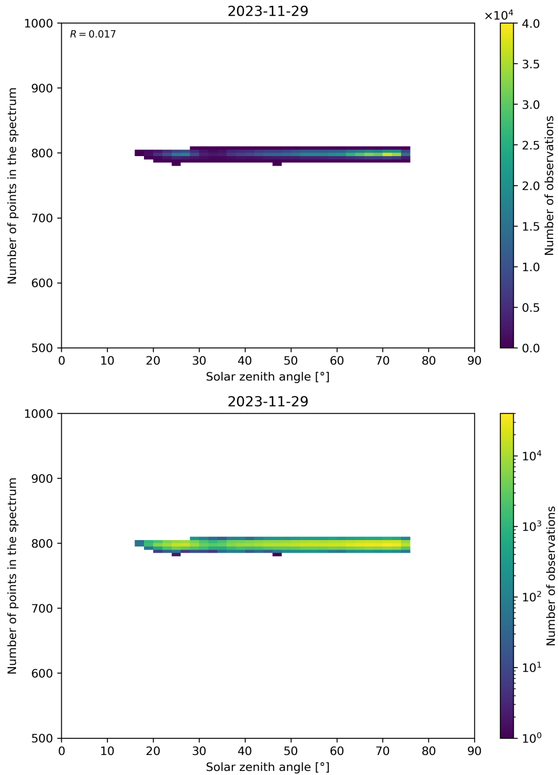
Figure 103: Scatter density plot of “Solar zenith angle” against “Number of points in the spectrum” for 2023-11-28 to 2023-11-30.
