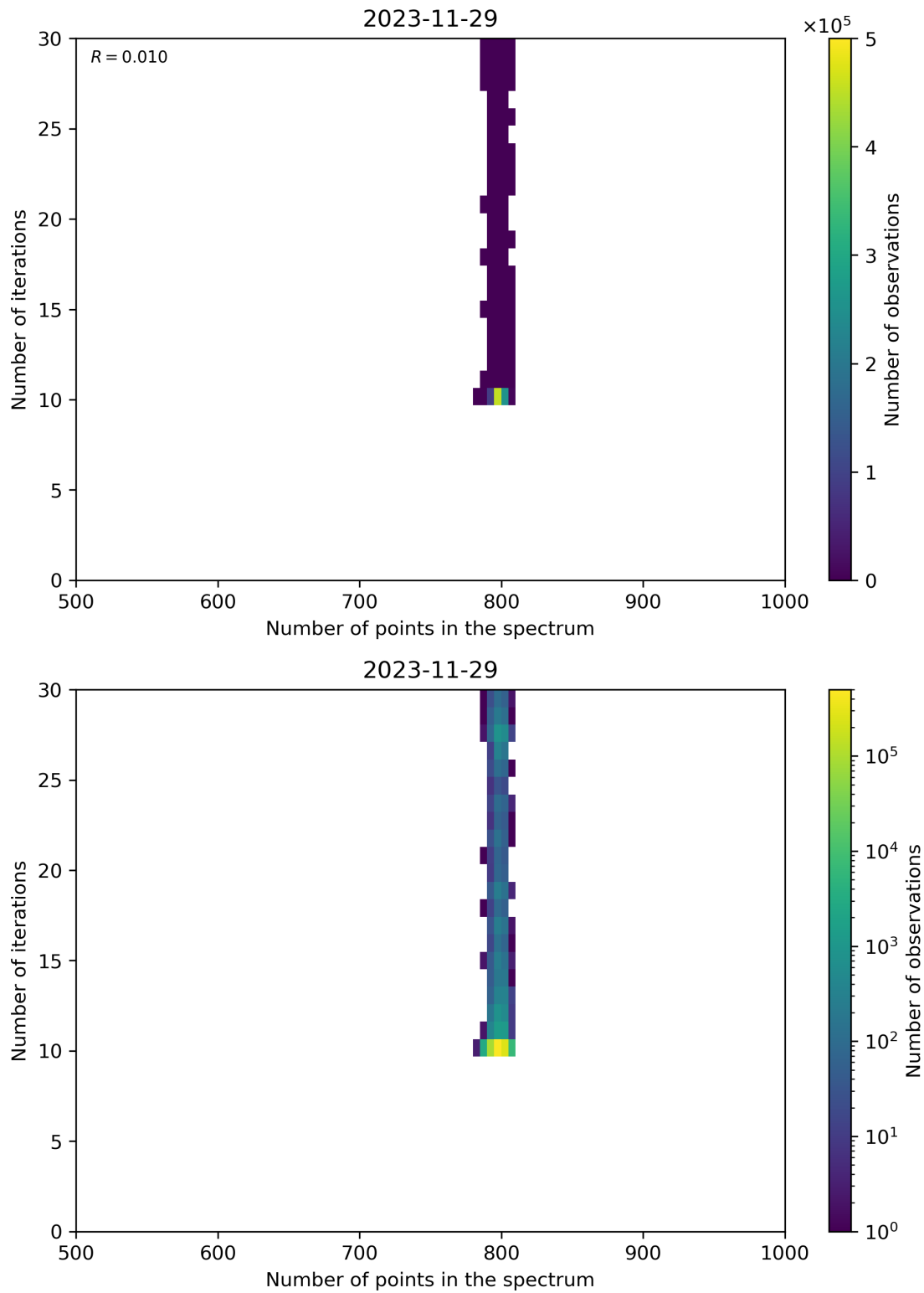
Figure 92: Scatter density plot of “Number of points in the spectrum” against “Number of iterations” for 2023-11-28 to 2023-11-30.
