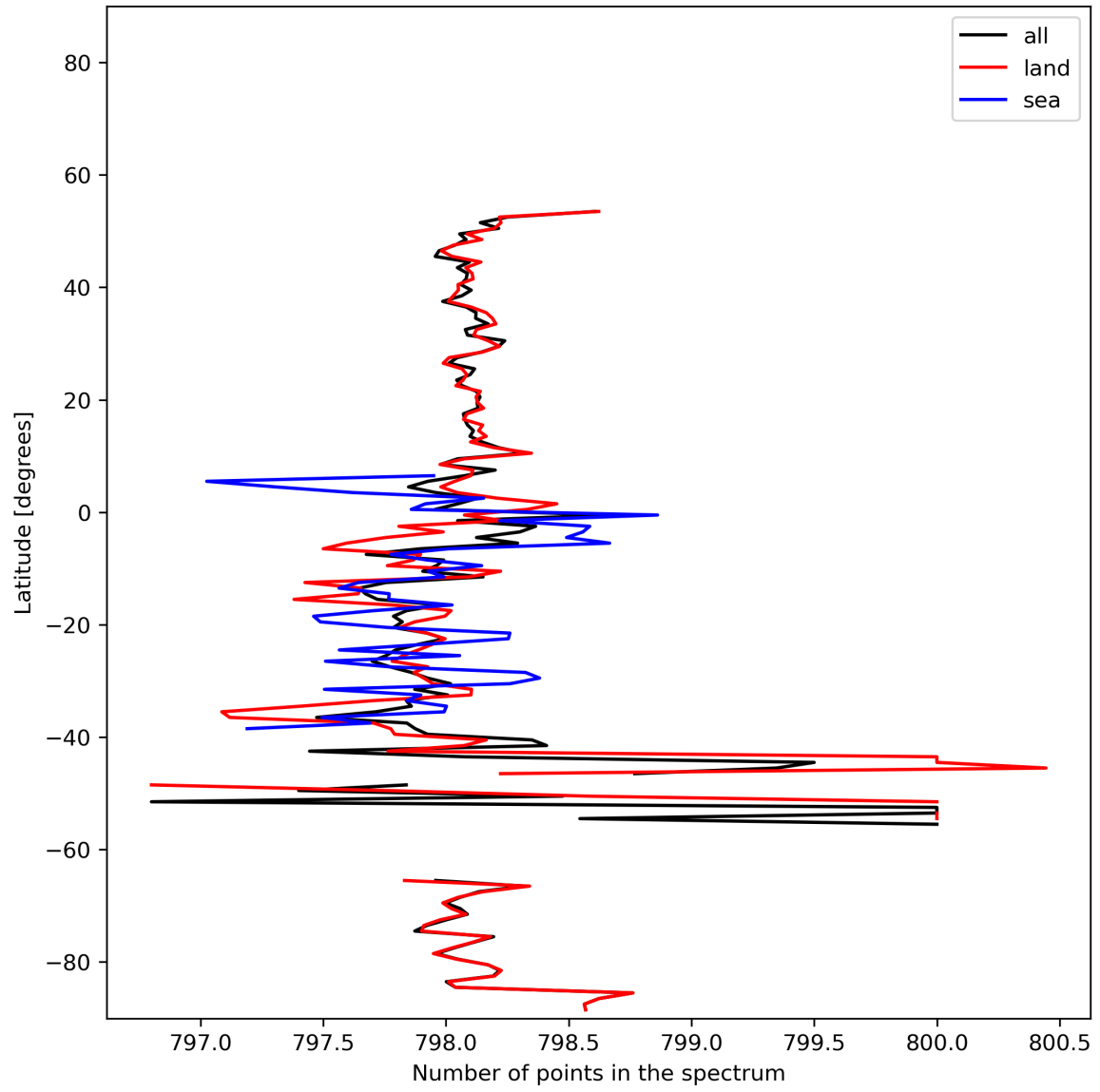
Figure 15: Zonal average of “Number of points in the spectrum” for 2023-11-28 to 2023-11-30.
