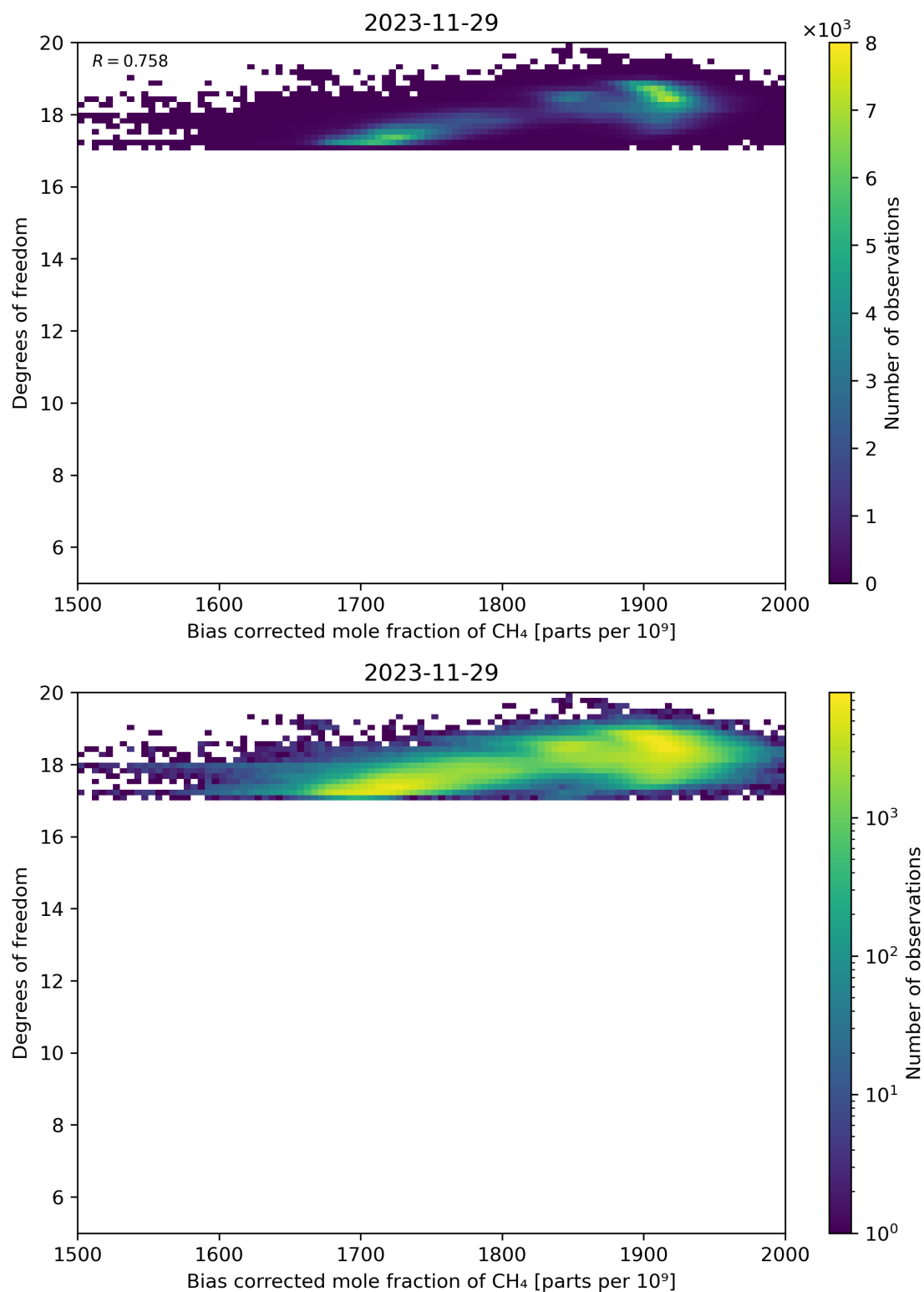
Figure 65: Scatter density plot of “Bias corrected mole fraction of CH 4 ” against “Degrees of freedom” for 2023-11-28 to 2023-11-30.
