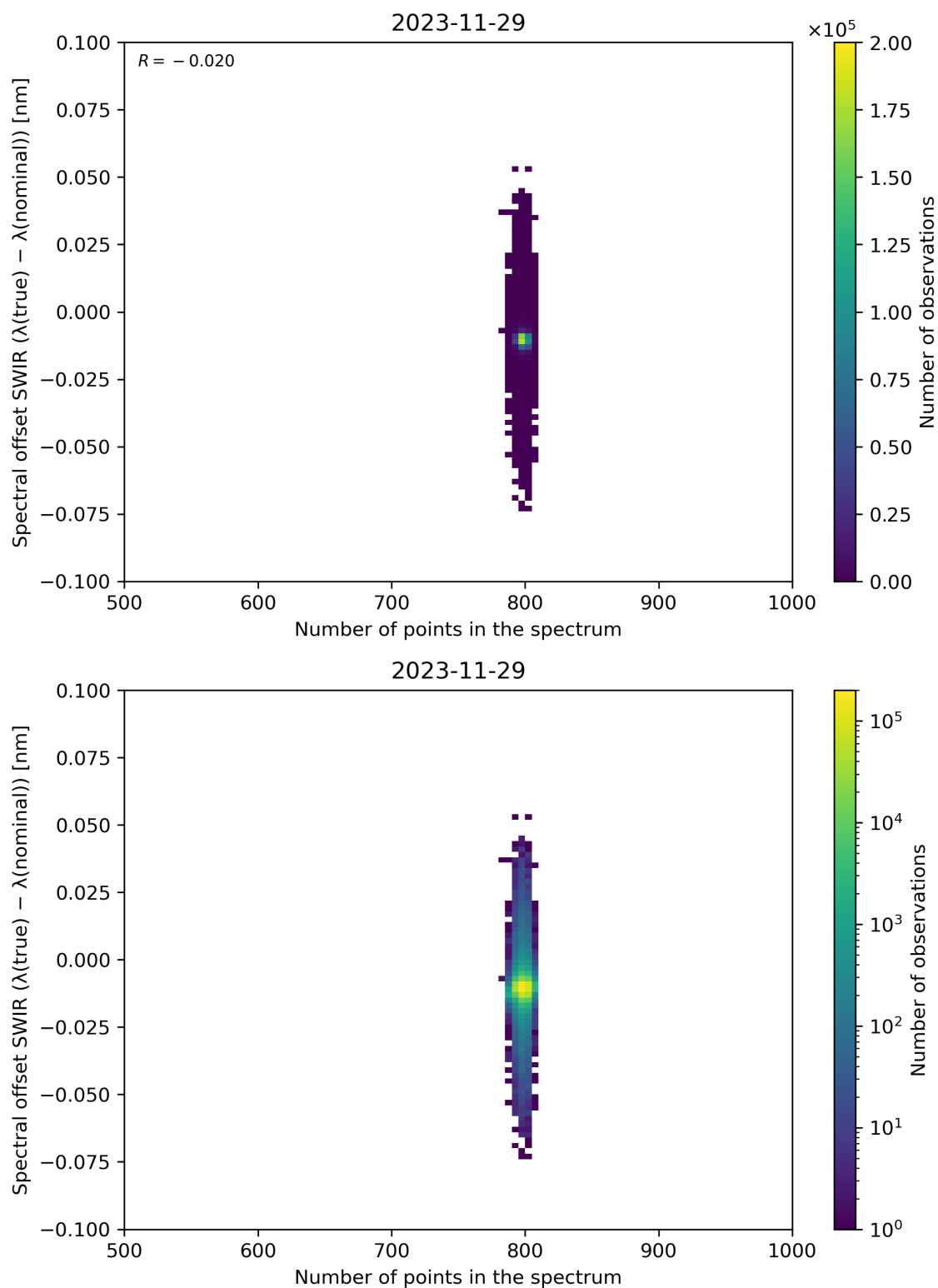
Figure 93: Scatter density plot of “Number of points in the spectrum” against “Spectral offset SWIR ( \lambda(\text{true}) - \lambda(\text{nominal}) )” for 2023-11-28 to 2023-11-30.
