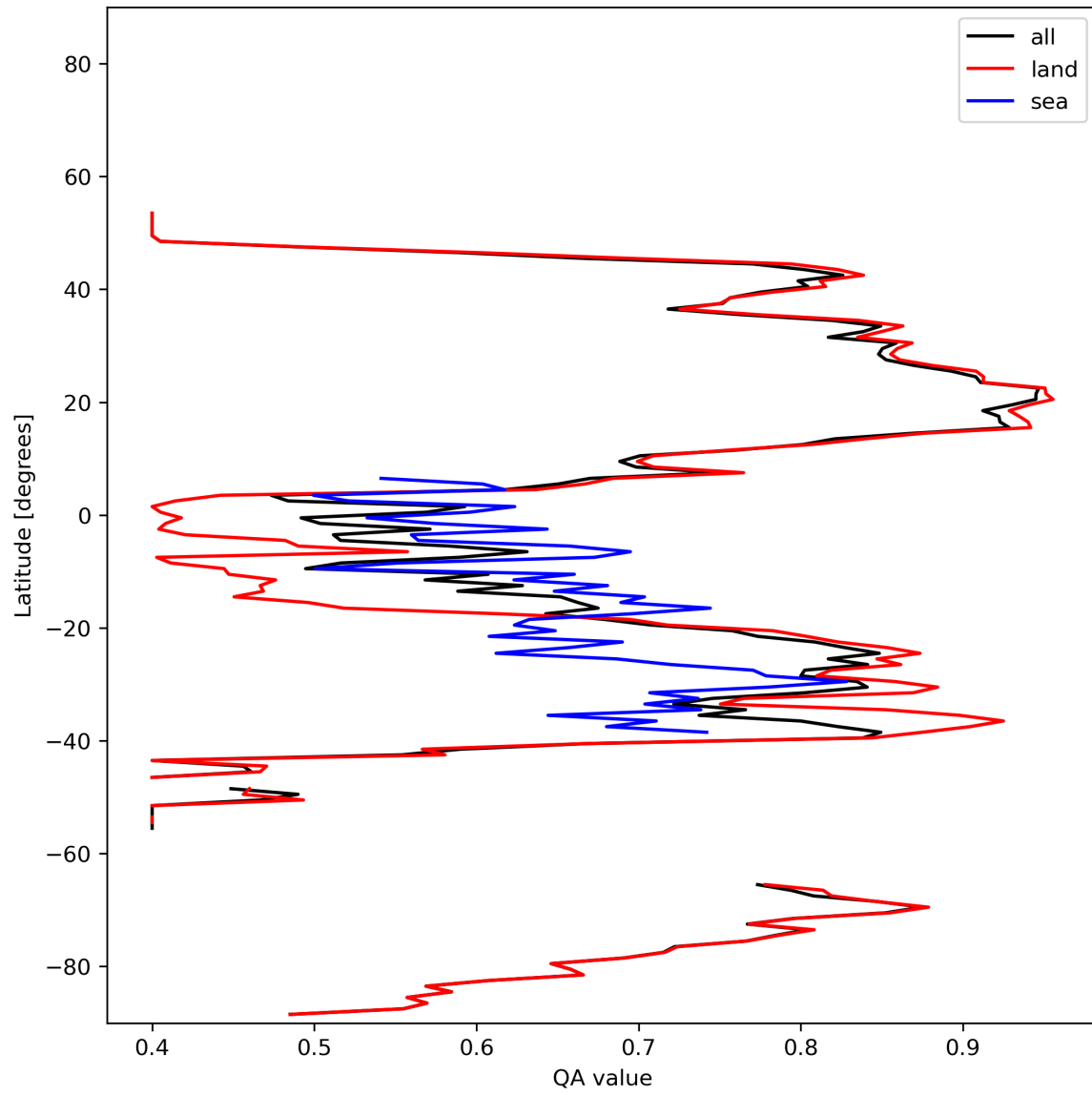
Figure 11: Zonal average of “QA value” for 2023-11-28 to 2023-11-30.
