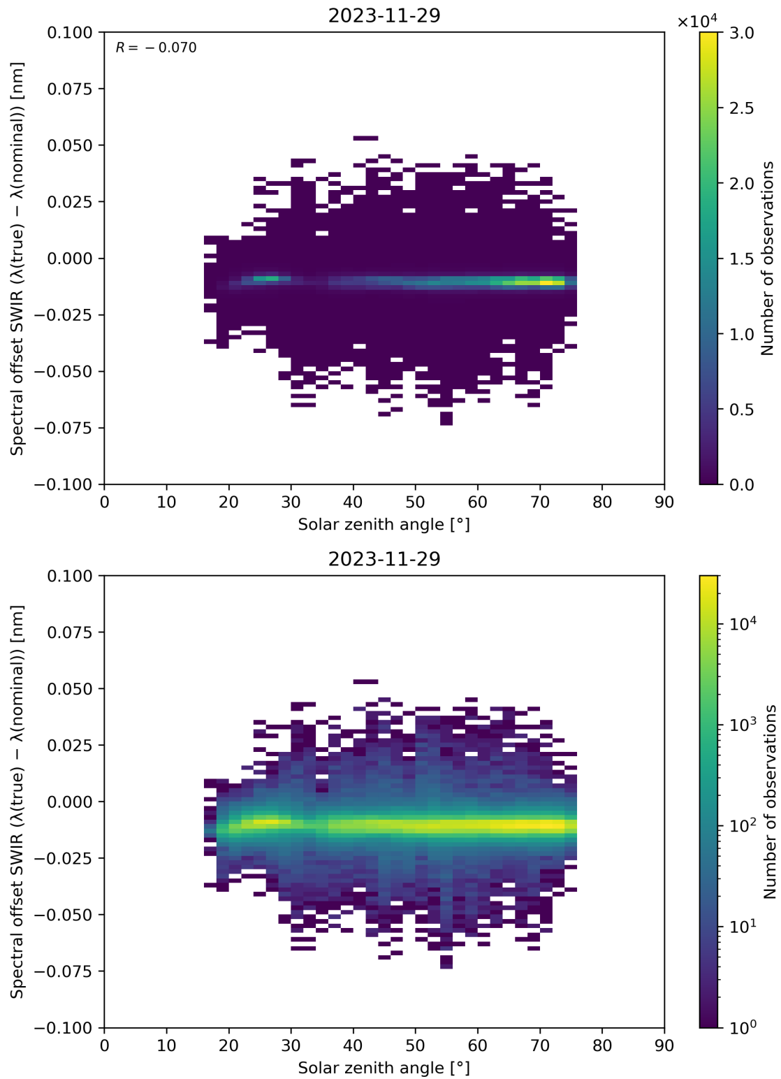
Figure 104: Scatter density plot of “Solar zenith angle” against “Spectral offset SWIR ( \lambda(\text{true}) - \lambda(\text{nominal}) )” for 2023-11-28 to 2023-11-30.
