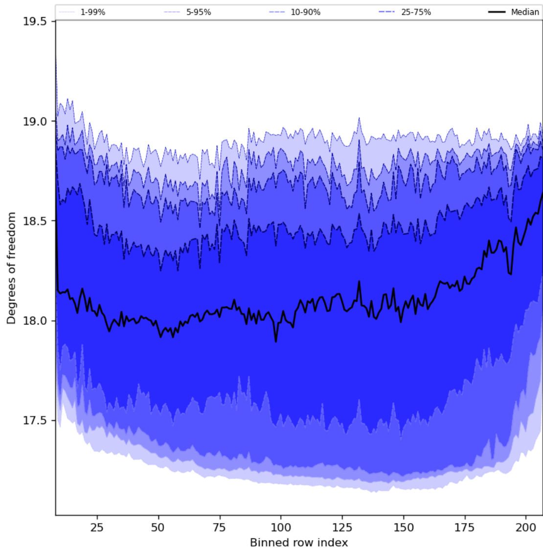
Figure 41: Along track statistics of “Degrees of freedom” for 2023-11-28 to 2023-11-30
