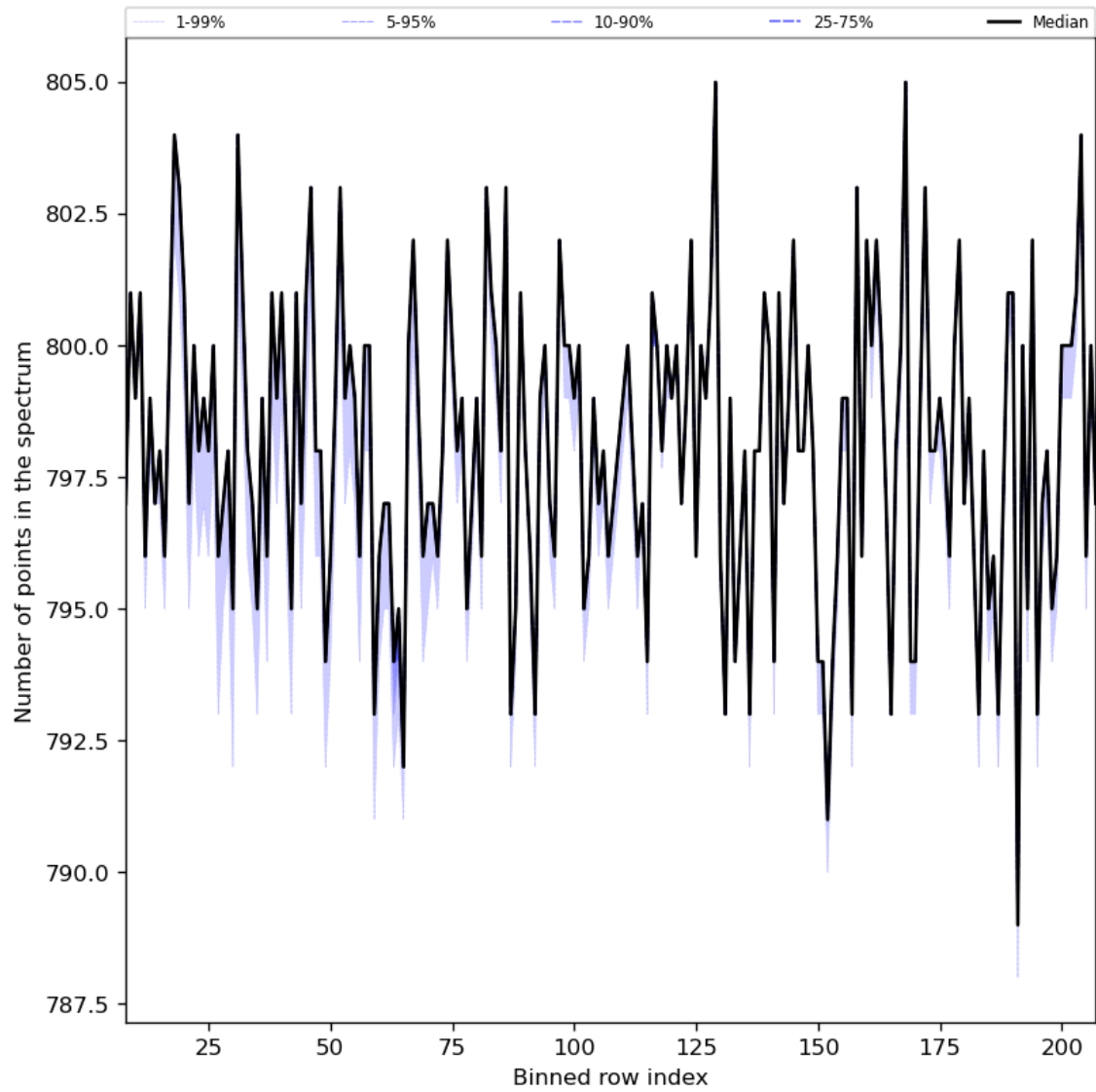
Figure 37: Along track statistics of “Number of points in the spectrum” for 2023-11-28 to 2023-11-30
