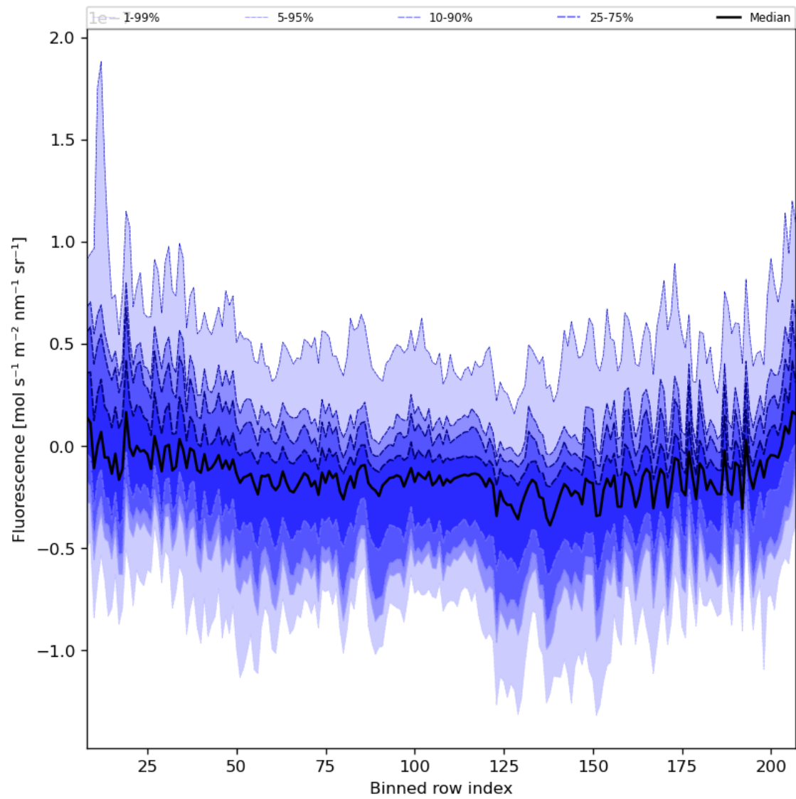
Figure 43: Along track statistics of “Fluorescence” for 2023-11-28 to 2023-11-30
