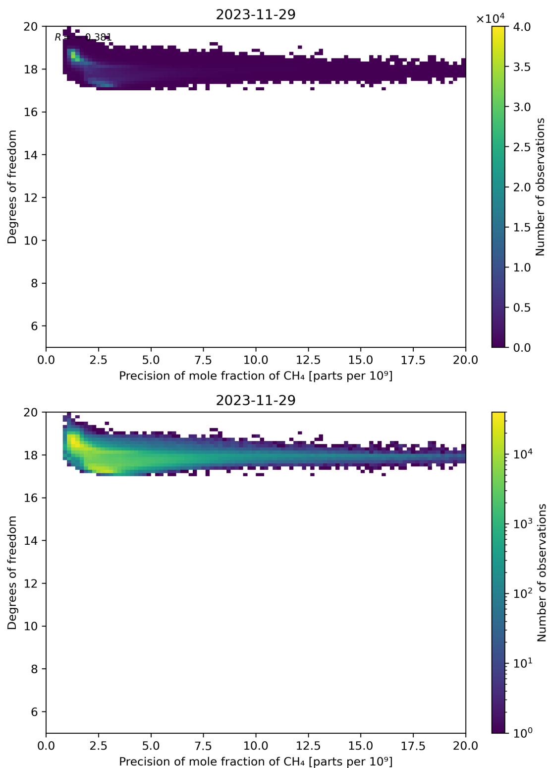
Figure 80: Scatter density plot of “Precision of mole fraction of CH 4 ” against “Degrees of freedom” for 2023-11-28 to 2023-11-30.
