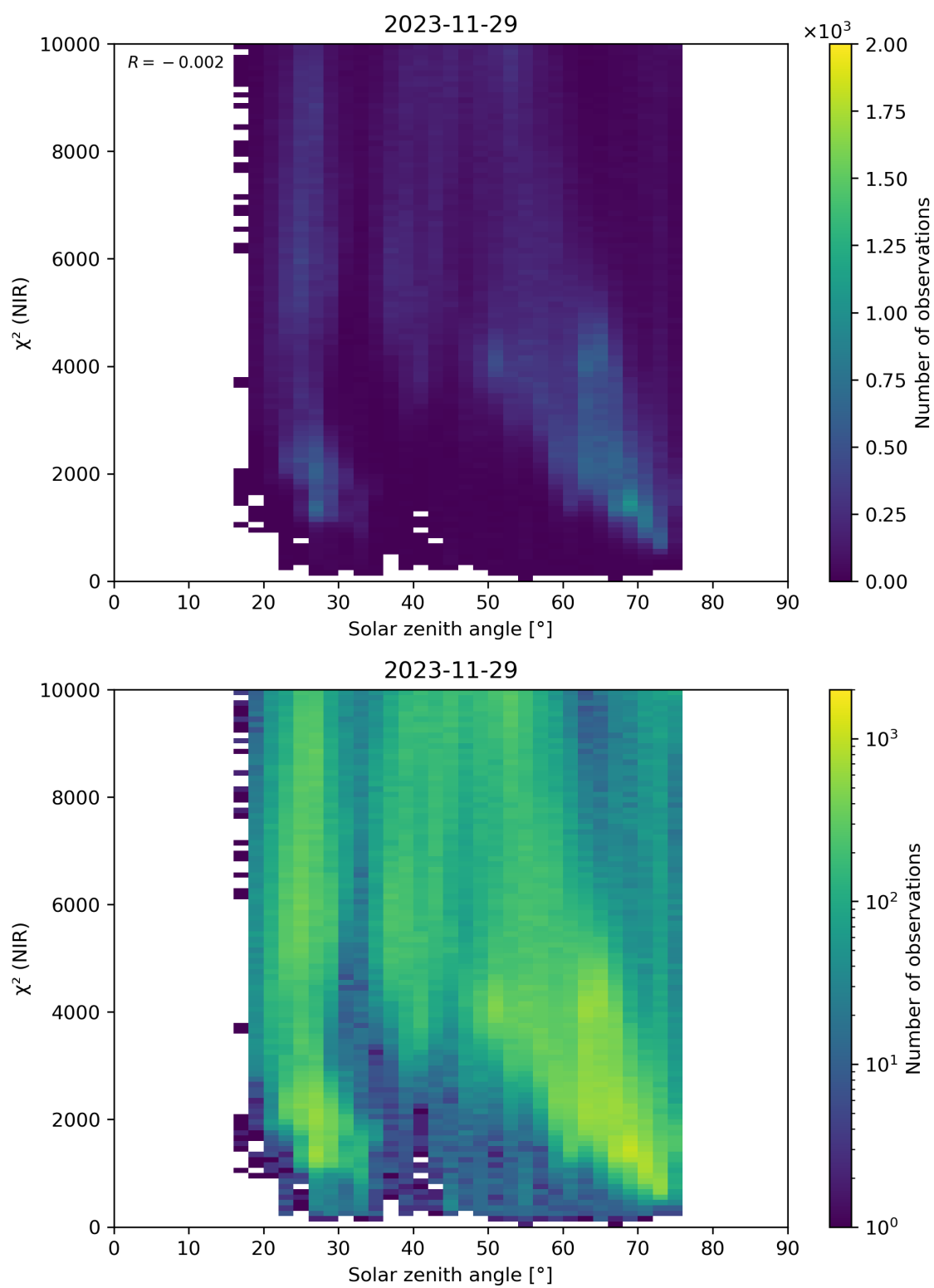
Figure 94: Scatter density plot of “Solar zenith angle” against “ \chi^2 (NIR)” for 2023-11-28 to 2023-11-30.
