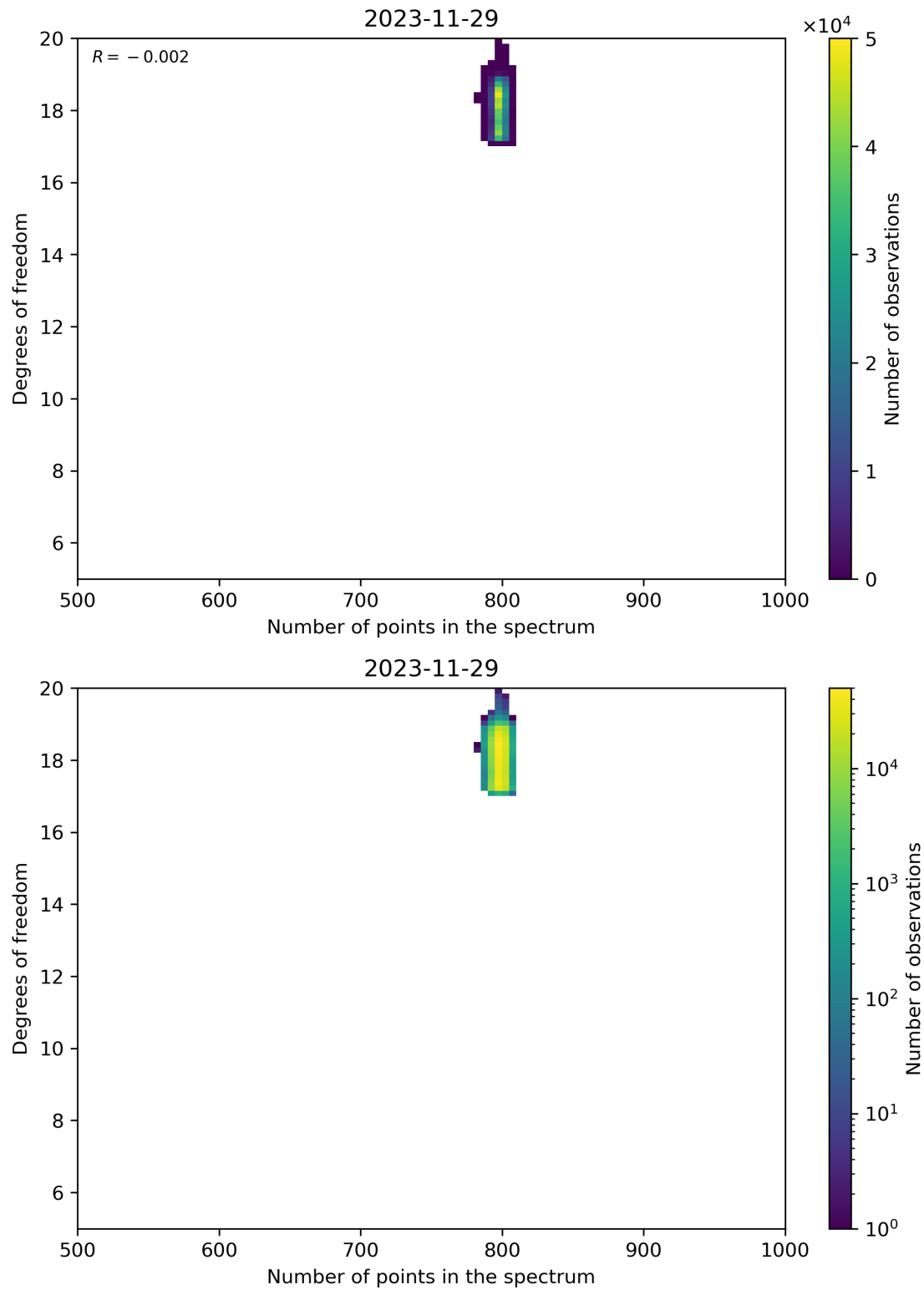
Figure 90: Scatter density plot of “Number of points in the spectrum” against “Degrees of freedom” for 2023-11-28 to 2023-11-30.
