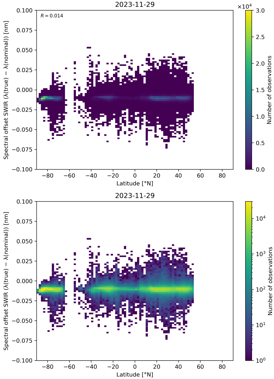
Figure 62: Scatter density plot of “Latitude” against “Spectral offset SWIR ( \lambda(\text{true}) - \lambda(\text{nominal}) )” for 2023-11-28 to 2023-11-30.
