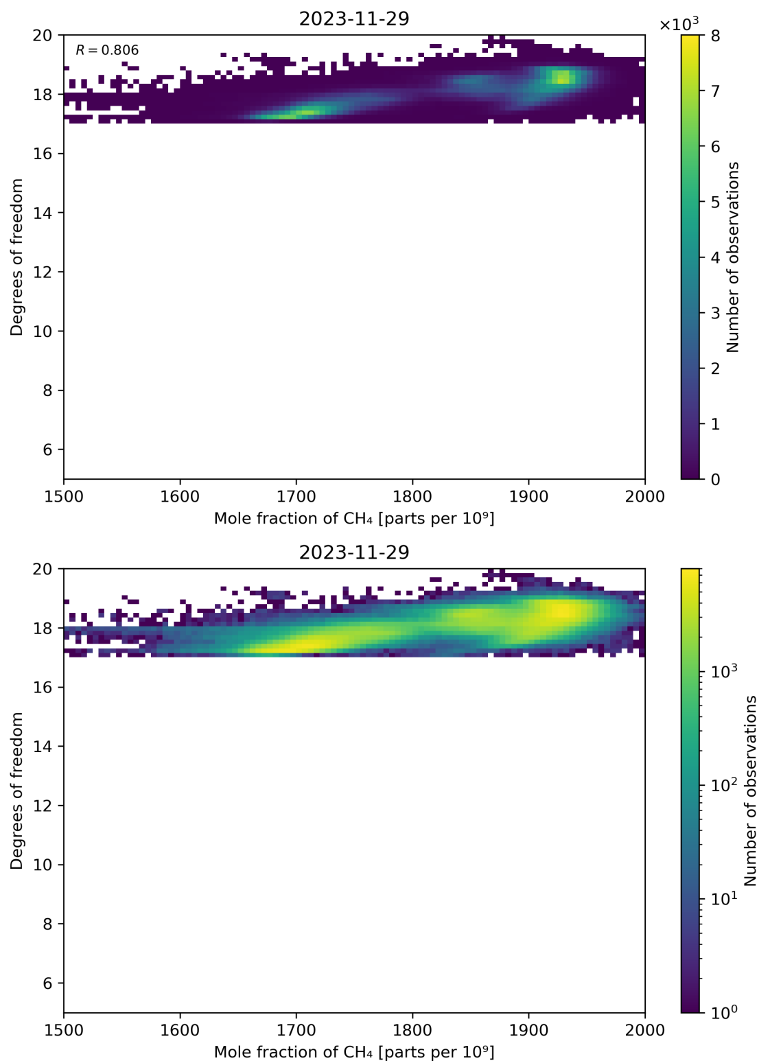
Figure 72: Scatter density plot of “Mole fraction of CH 4 ” against “Degrees of freedom” for 2023-11-28 to 2023-11-30.
