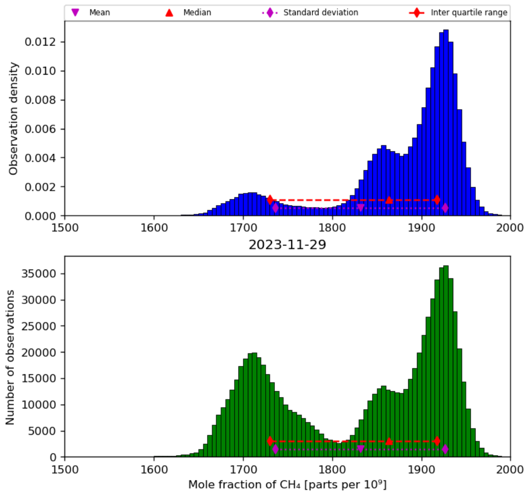
Figure 23: Histogram of “Mole fraction of CH 4 ” for 2023-11-28 to 2023-11-30
