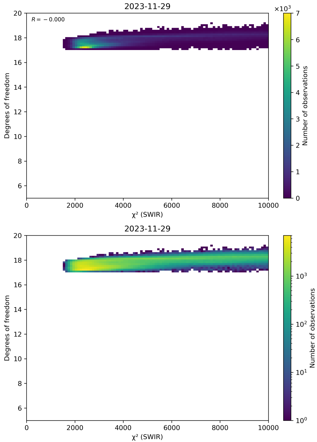
Figure 48: Scatter density plot of “ \chi^2 (SWIR)” against “Degrees of freedom” for 2023-11-28 to 2023-11-30.
