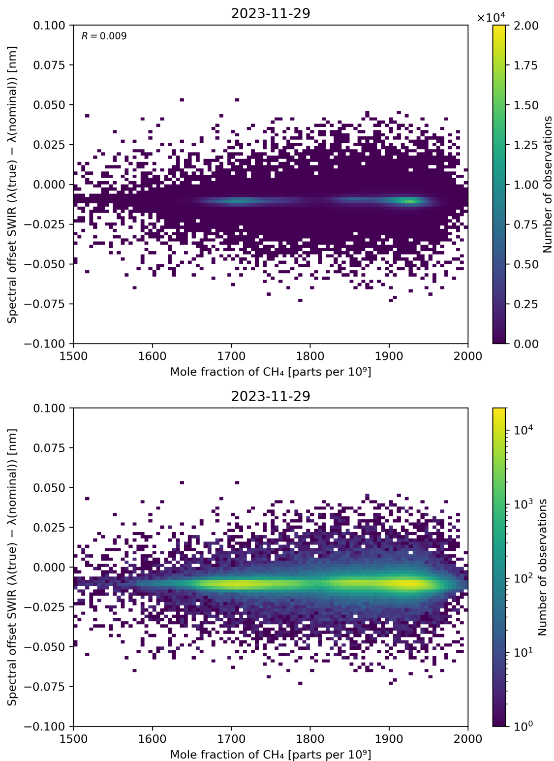
Figure 86: Scatter density plot of “Mole fraction of CH 4 ” against “Spectral offset SWIR ( \lambda(\text{true}) - \lambda(\text{nominal}) )” for 2023-11-28 to 2023-11-30.
