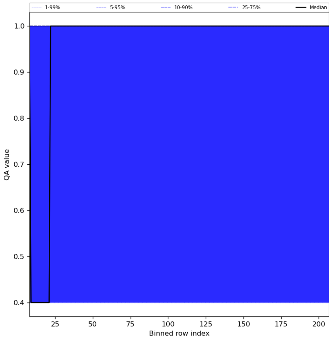
Figure 33: Along track statistics of “QA value” for 2023-11-28 to 2023-11-30
