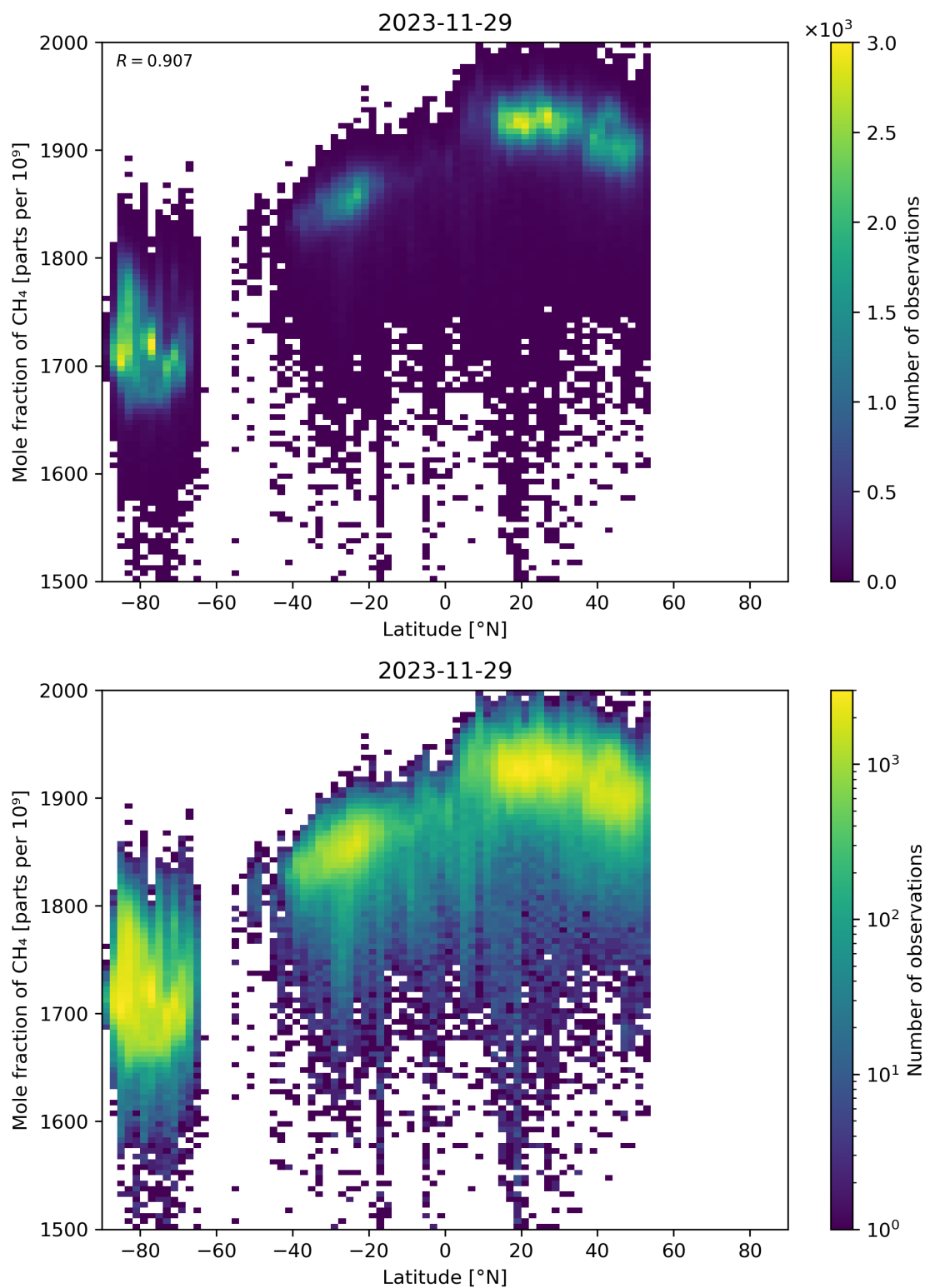
Figure 57: Scatter density plot of “Latitude” against “Mole fraction of \text{CH}_4 ” for 2023-11-28 to 2023-11-30.
