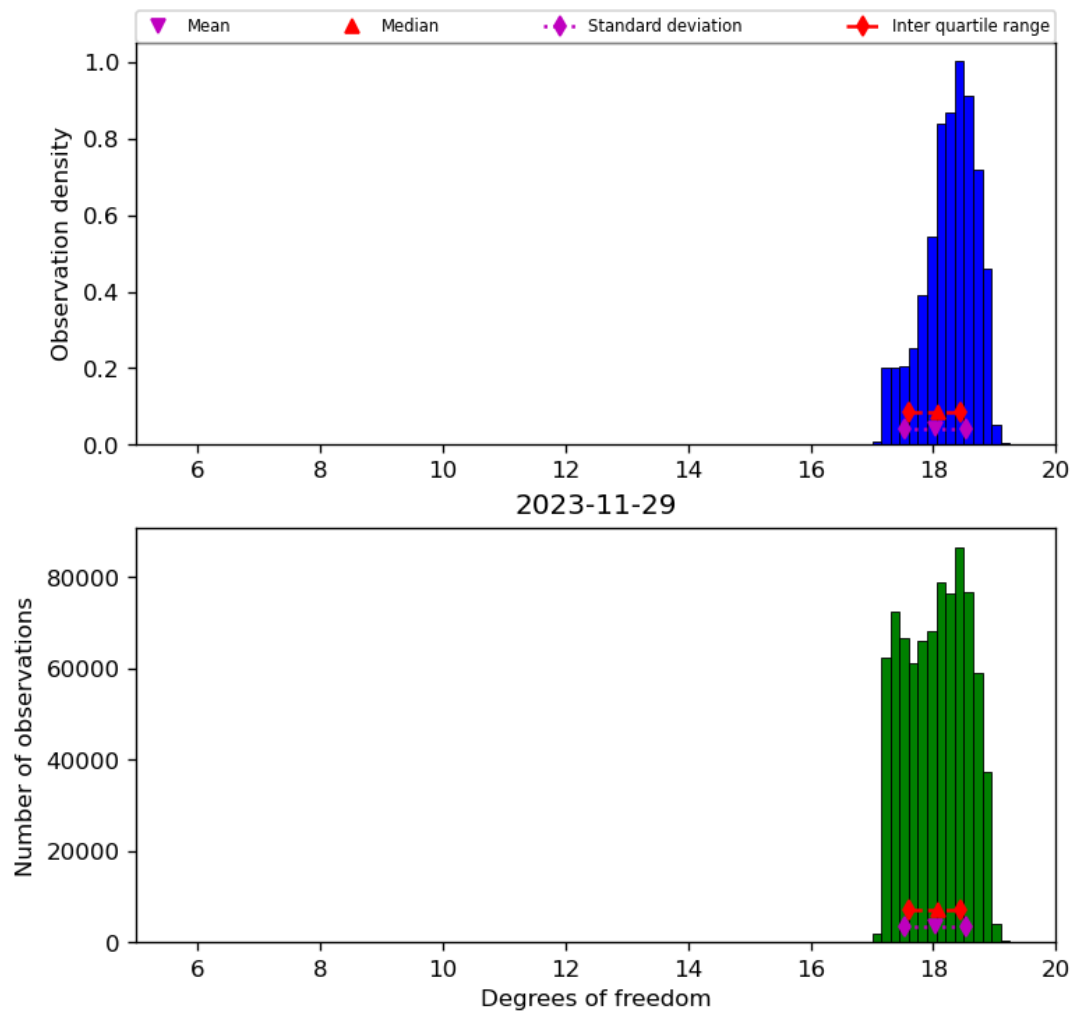
Figure 30: Histogram of “Degrees of freedom” for 2023-11-28 to 2023-11-30
