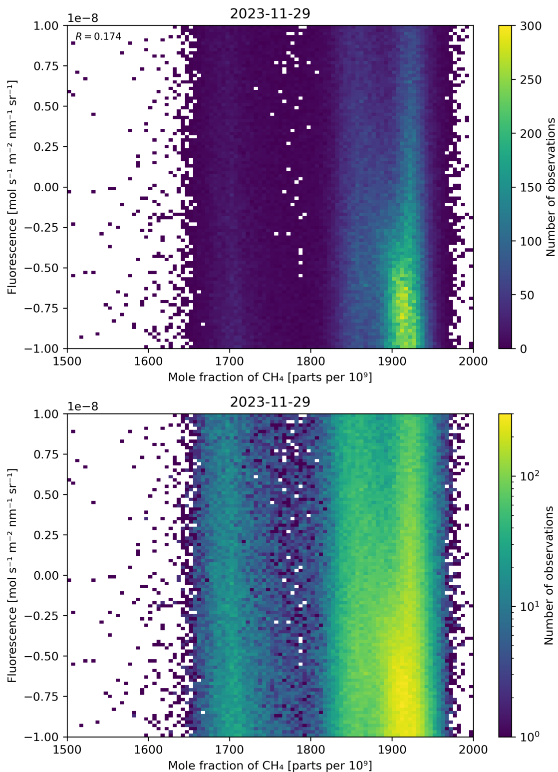
Figure 73: Scatter density plot of “Mole fraction of \text{CH}_4 ” against “Fluorescence” for 2023-11-28 to 2023-11-30.
