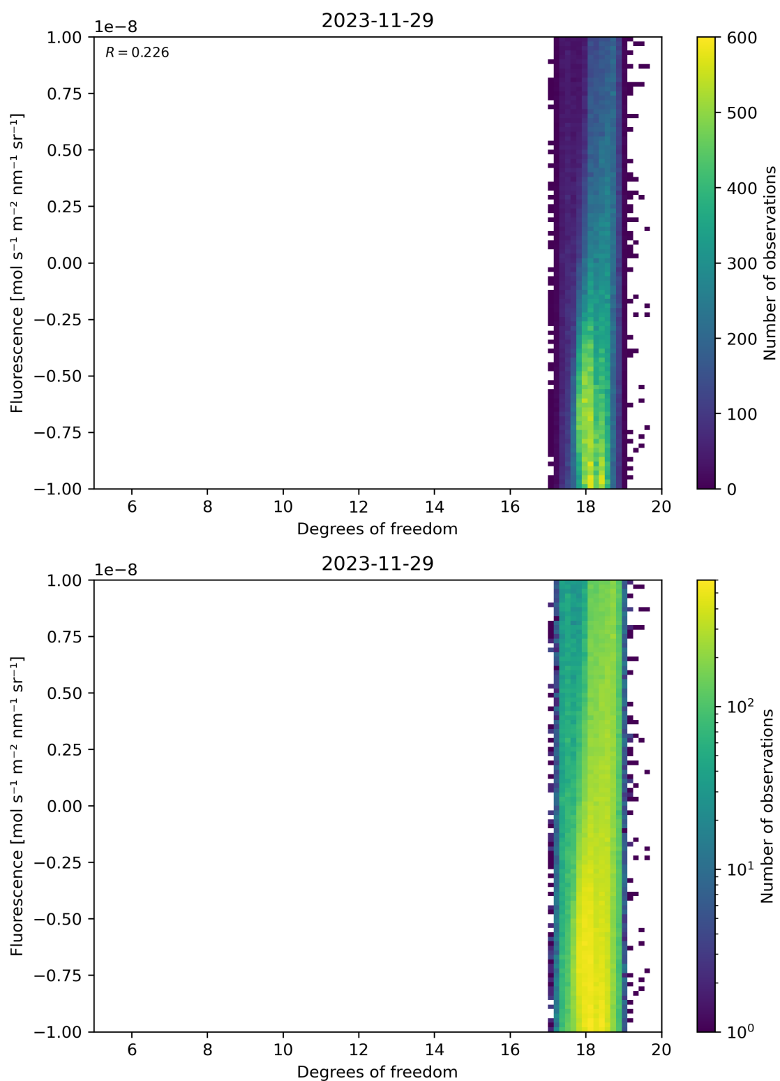
Figure 51: Scatter density plot of “Degrees of freedom” against “Fluorescence” for 2023-11-28 to 2023-11-30.
