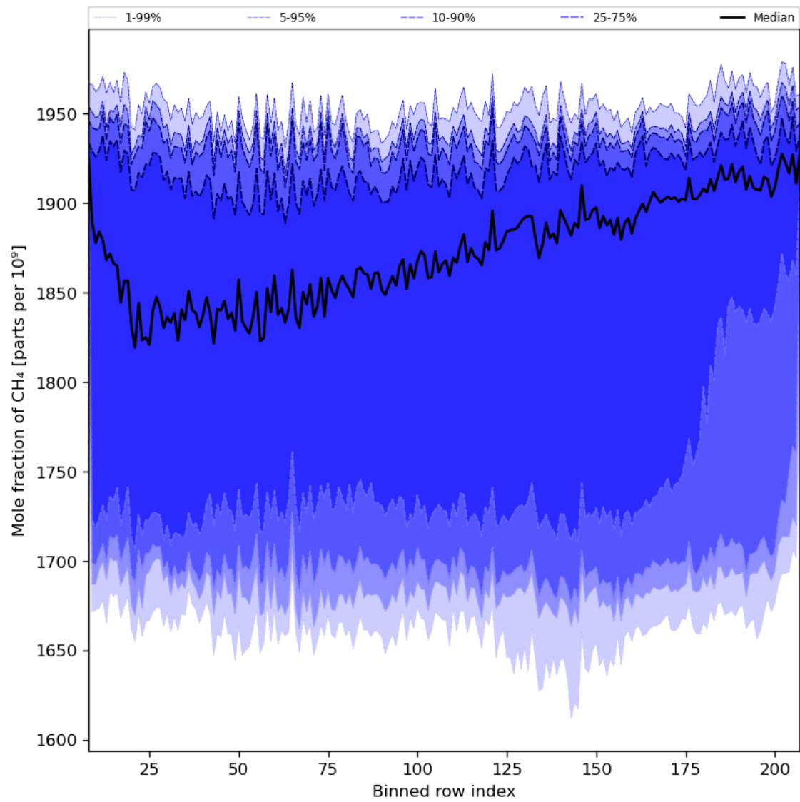
Figure 34: Along track statistics of “Mole fraction of CH 4 ” for 2023-11-28 to 2023-11-30
