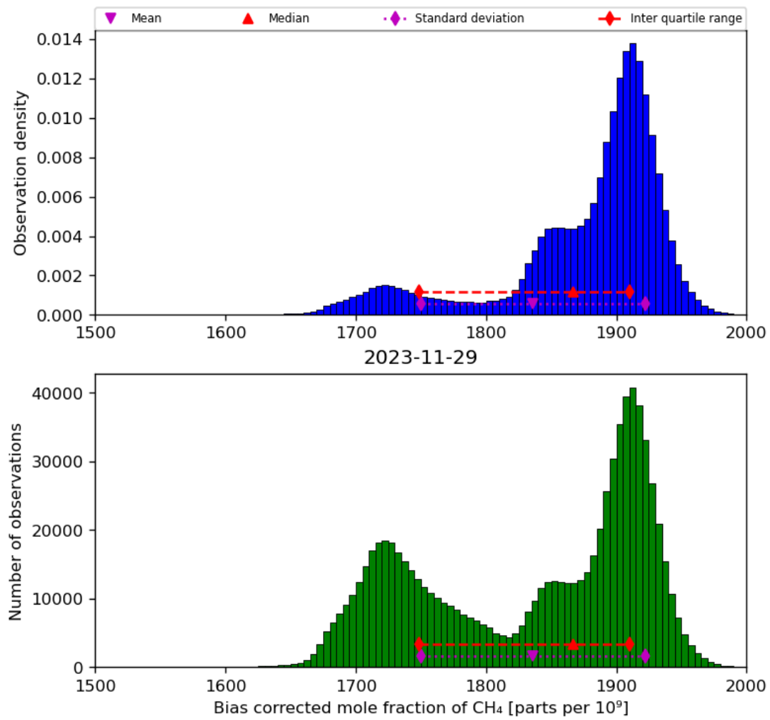
Figure 25: Histogram of “Bias corrected mole fraction of CH 4 ” for 2023-11-28 to 2023-11-30
