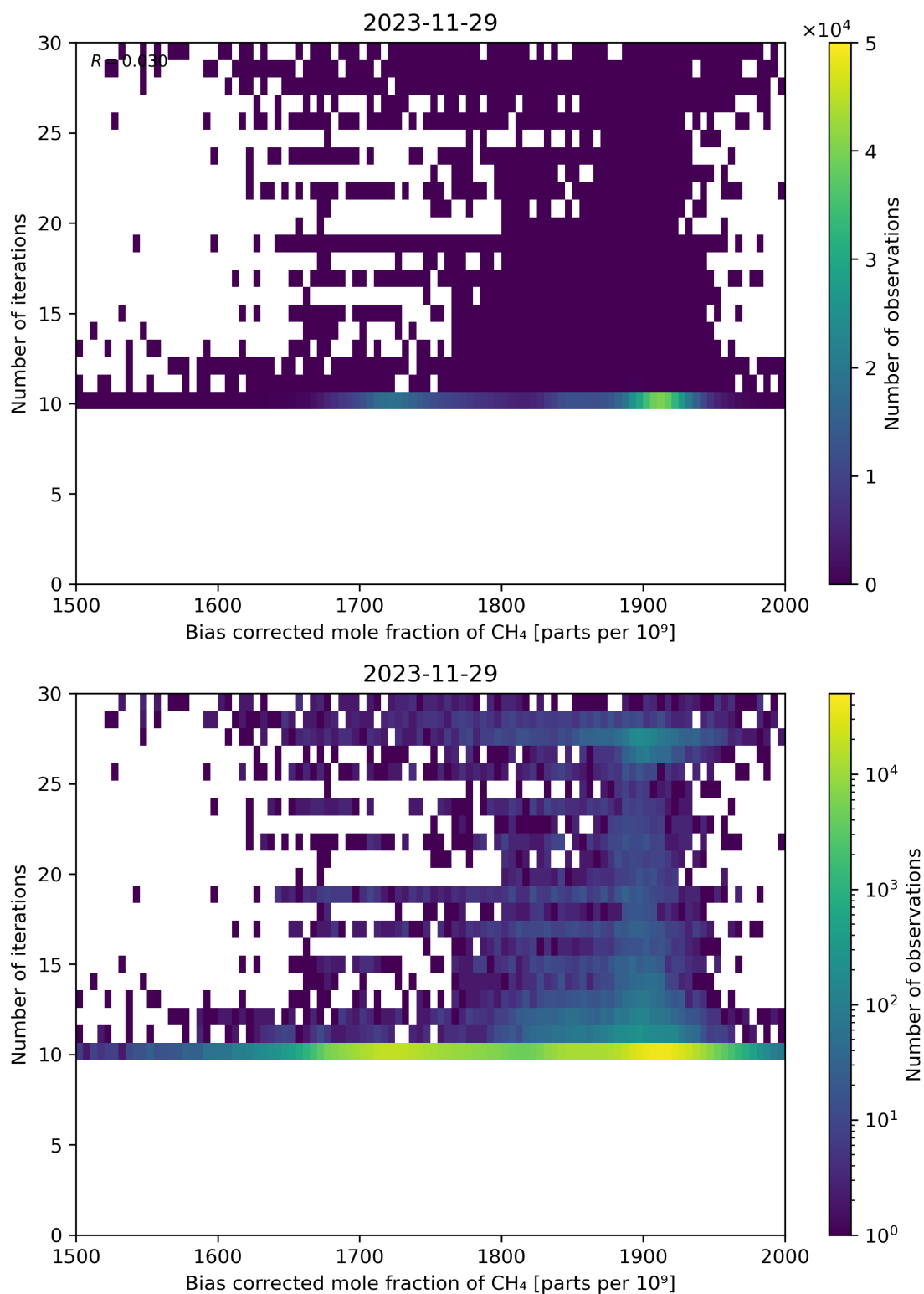
Figure 67: Scatter density plot of “Bias corrected mole fraction of CH 4 ” against “Number of iterations” for 2023-11-28 to 2023-11-30.
