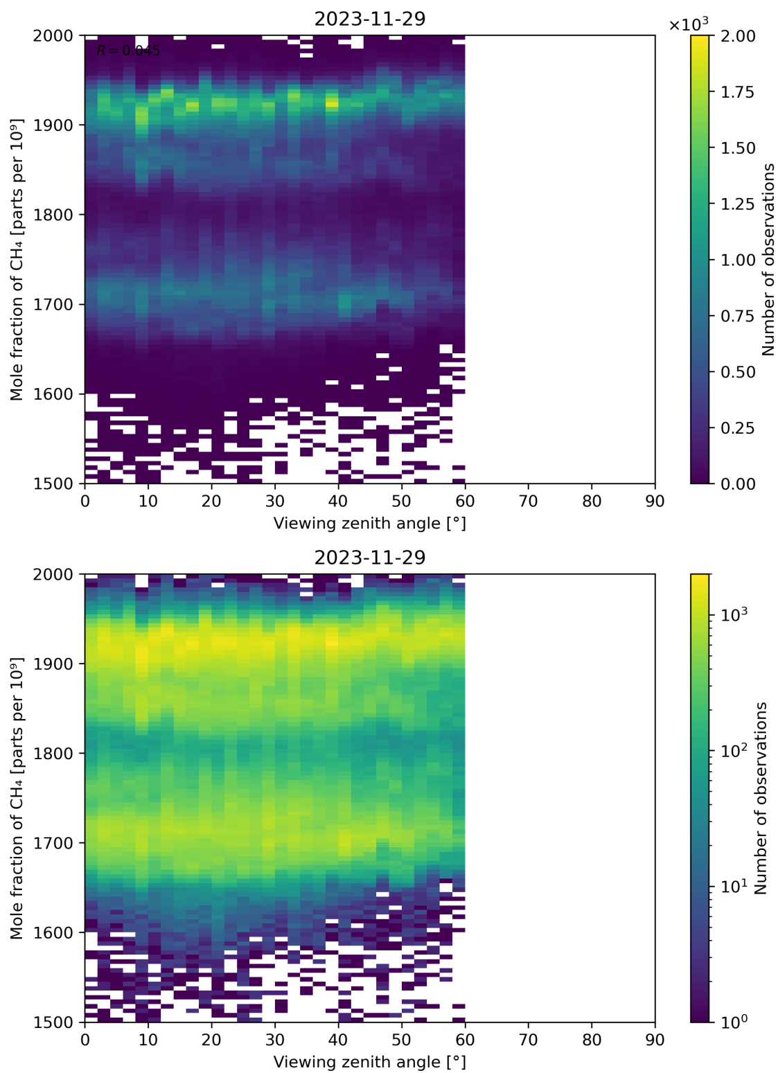
Figure 110: Scatter density plot of “Viewing zenith angle” against “Mole fraction of \text{CH}_4 ” for 2023-11-28 to 2023-11-30.
