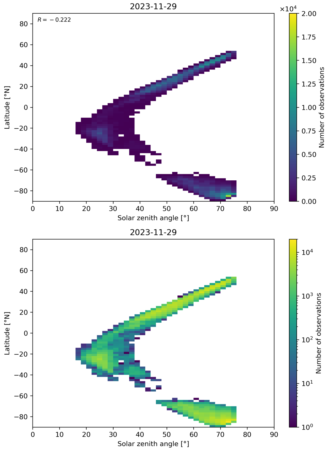
Figure 98: Scatter density plot of “Solar zenith angle” against “Latitude” for 2023-11-28 to 2023-11-30.
