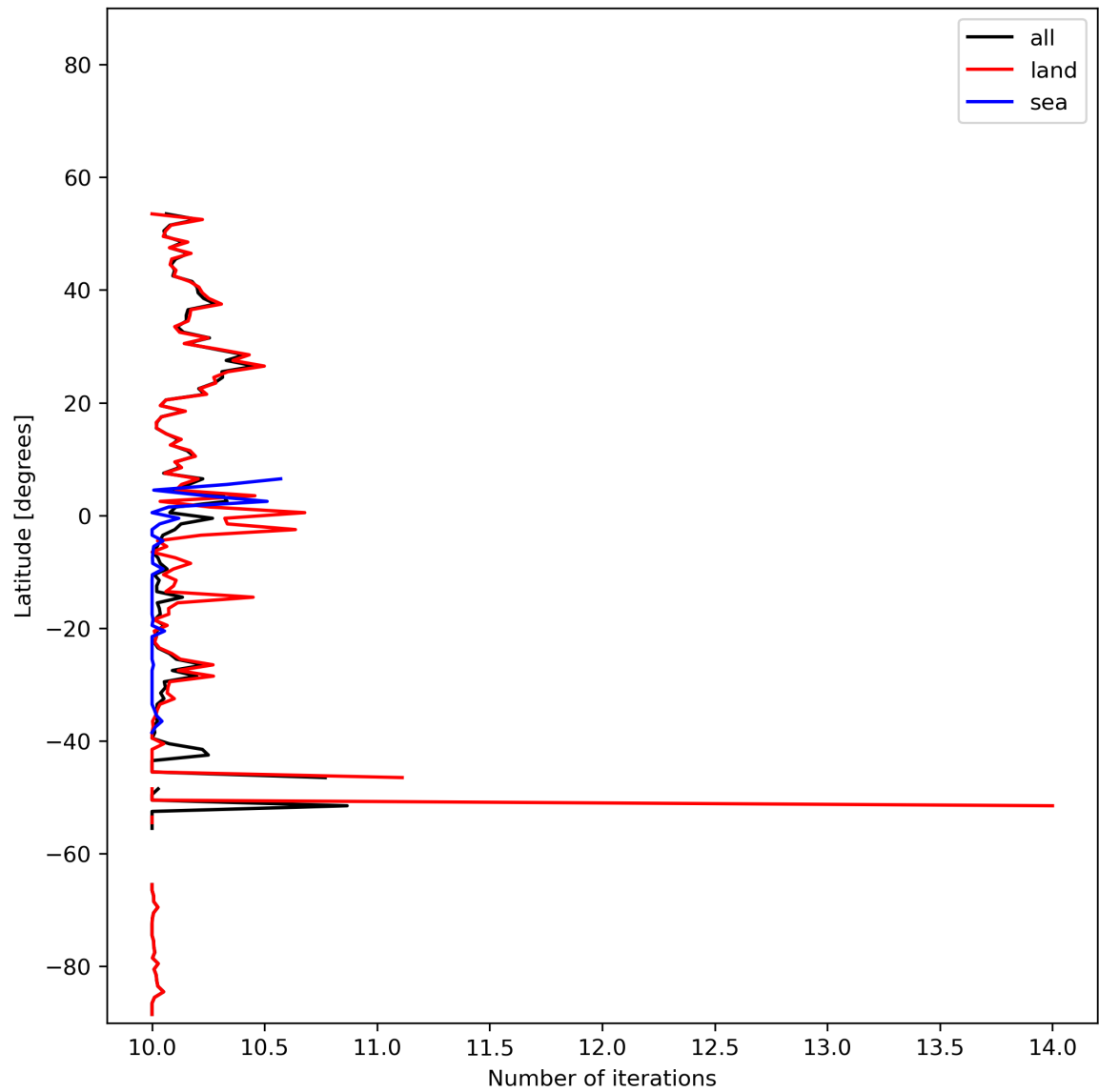
Figure 20: Zonal average of “Number of iterations” for 2023-11-28 to 2023-11-30.
