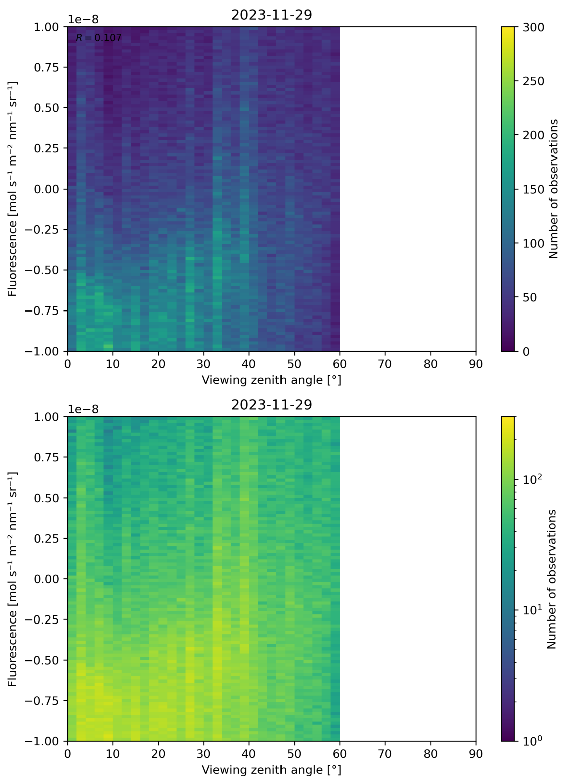
Figure 108: Scatter density plot of “Viewing zenith angle” against “Fluorescence” for 2023-11-28 to 2023-11-30.
