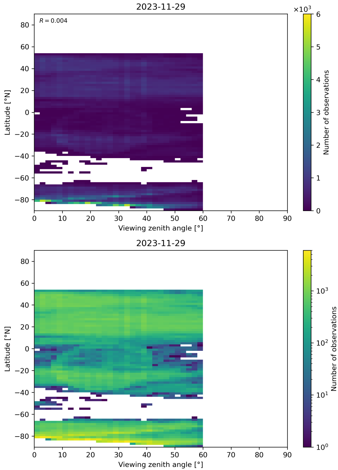
Figure 109: Scatter density plot of “Viewing zenith angle” against “Latitude” for 2023-11-28 to 2023-11-30.
