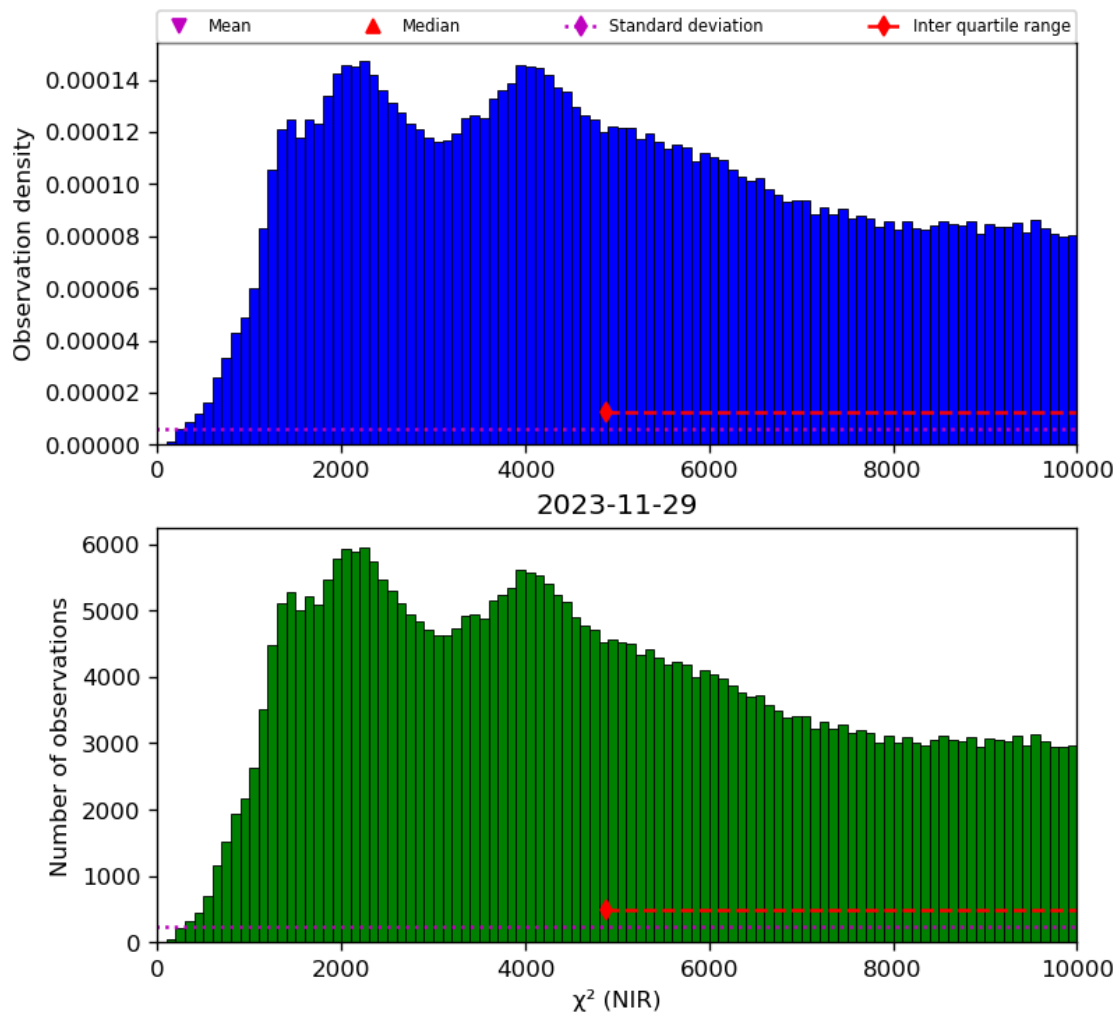
Figure 29: Histogram of “ \chi^2 (NIR)” for 2023-11-28 to 2023-11-30
