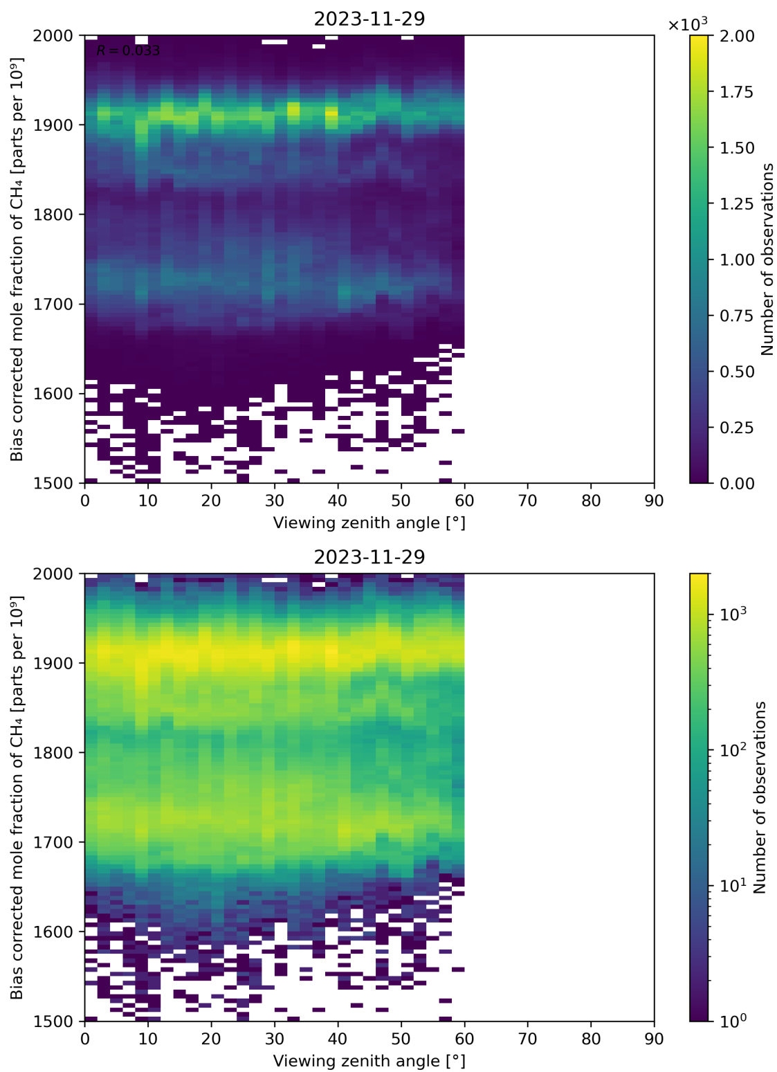
Figure 111: Scatter density plot of “Viewing zenith angle” against “Bias corrected mole fraction of CH 4 ” for 2023-11-28 to 2023-11-30.
