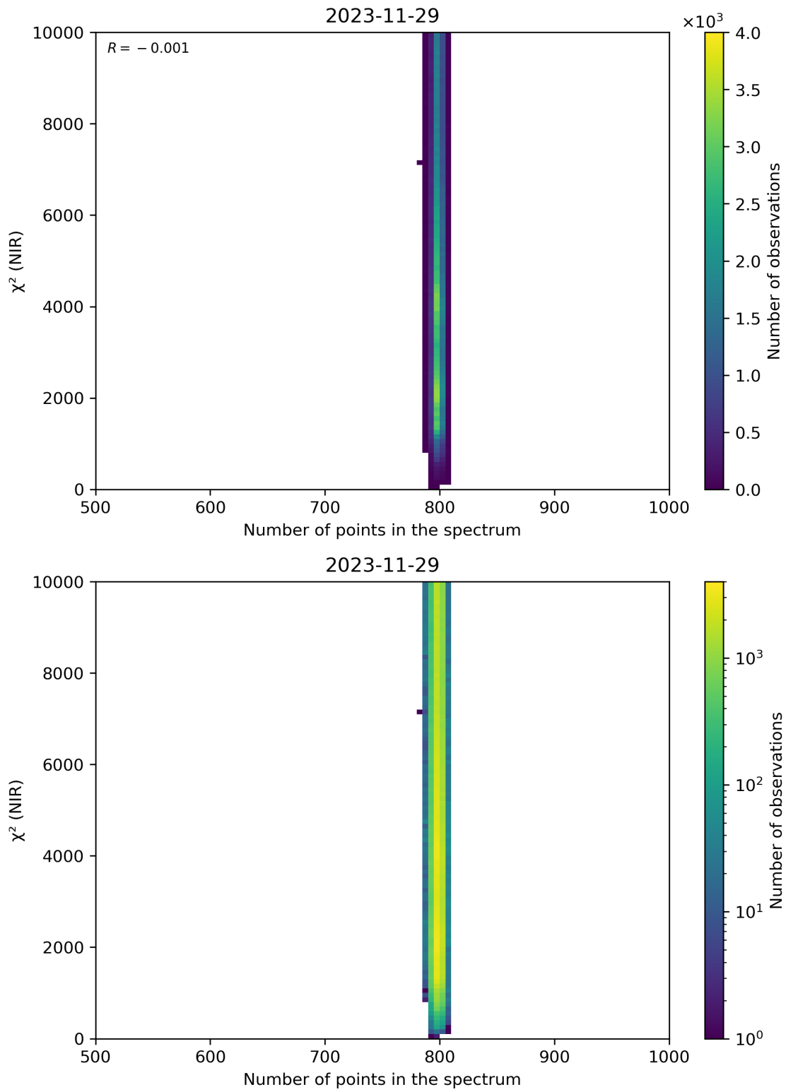
Figure 88: Scatter density plot of “Number of points in the spectrum” against “ \chi^2 (NIR)” for 2023-11-28 to 2023-11-30.
