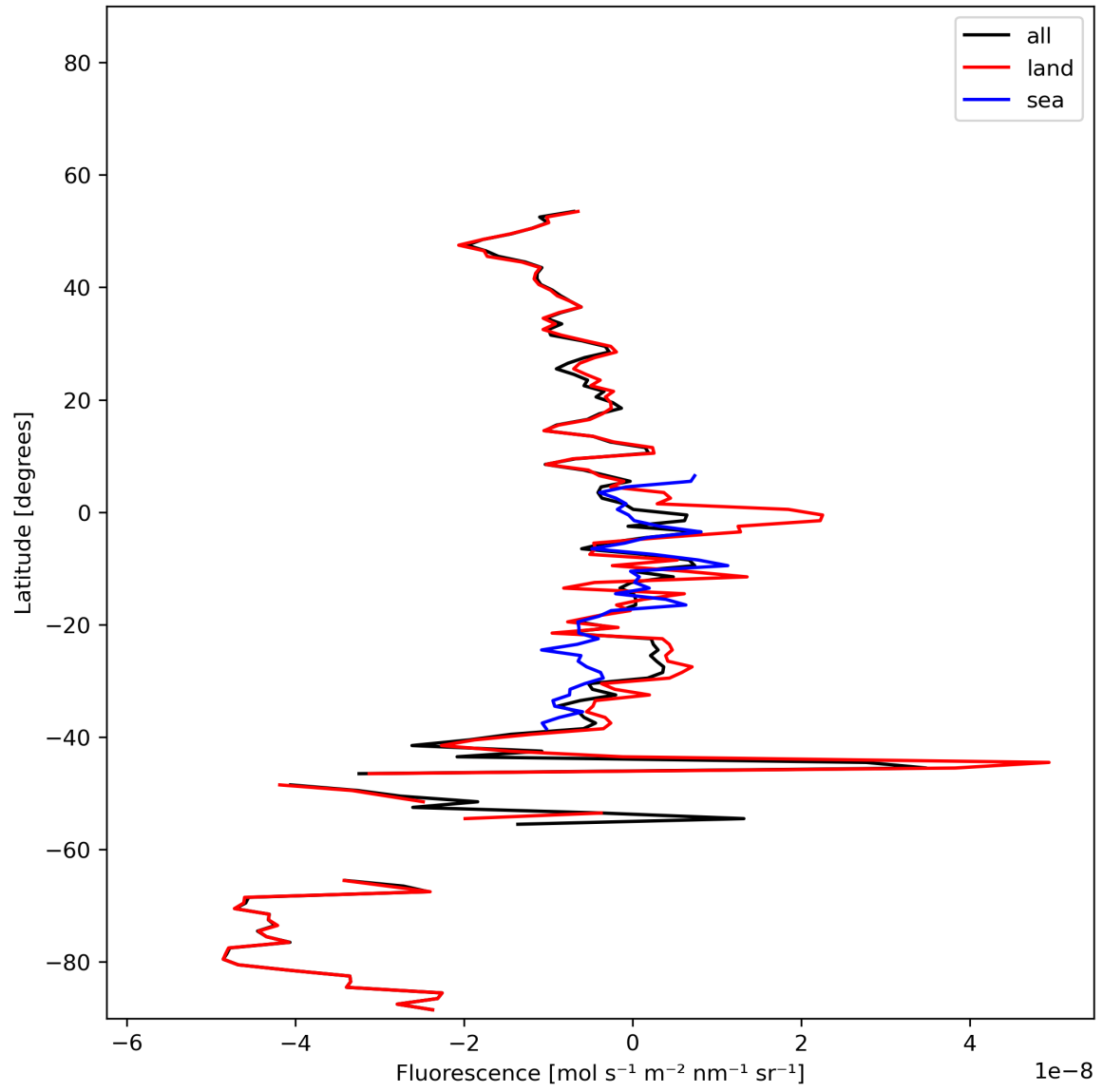
Figure 21: Zonal average of “Fluorescence” for 2023-11-28 to 2023-11-30.
