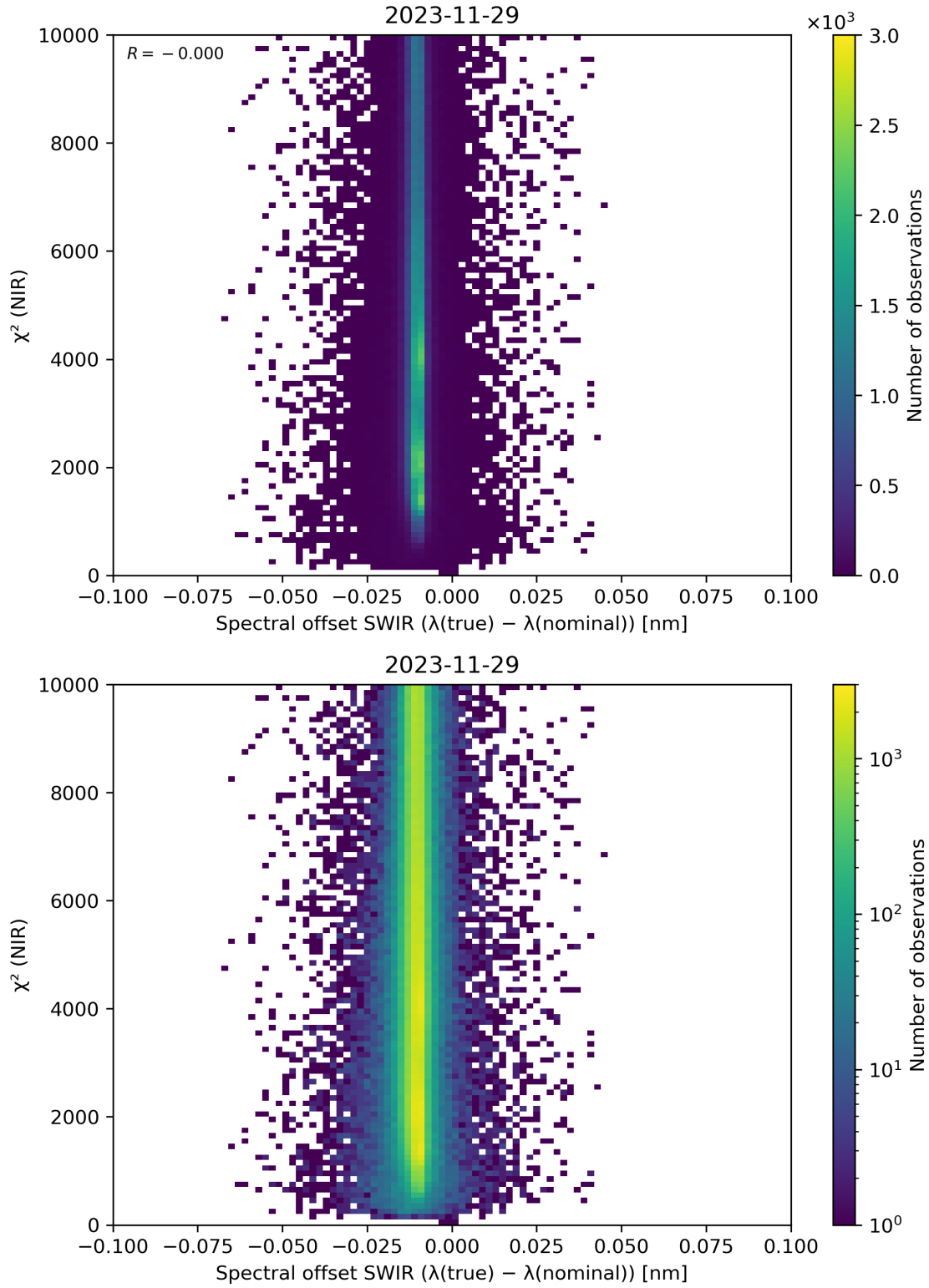
Figure 117: Scatter density plot of “Spectral offset SWIR ( \lambda(\text{true}) - \lambda(\text{nominal}) )” against “ \chi^2 (NIR)” for 2023-11-28 to 2023-11-30.
