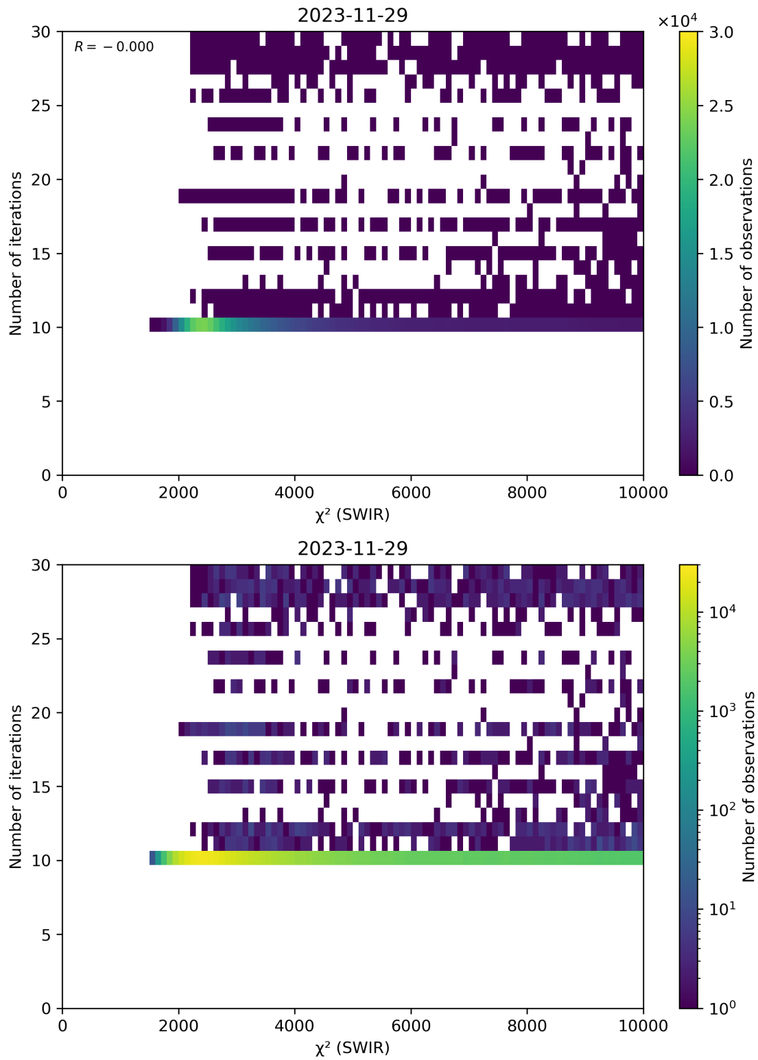
Figure 50: Scatter density plot of “ \chi^2 (SWIR)” against “Number of iterations” for 2023-11-28 to 2023-11-30.
