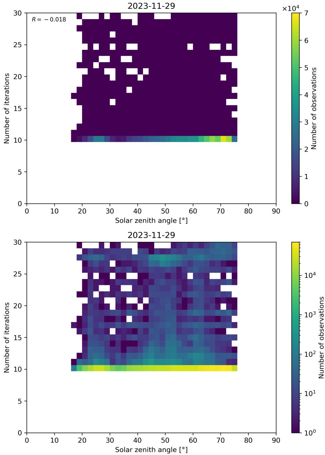
Figure 102: Scatter density plot of “Solar zenith angle” against “Number of iterations” for 2023-11-28 to 2023-11-30.
