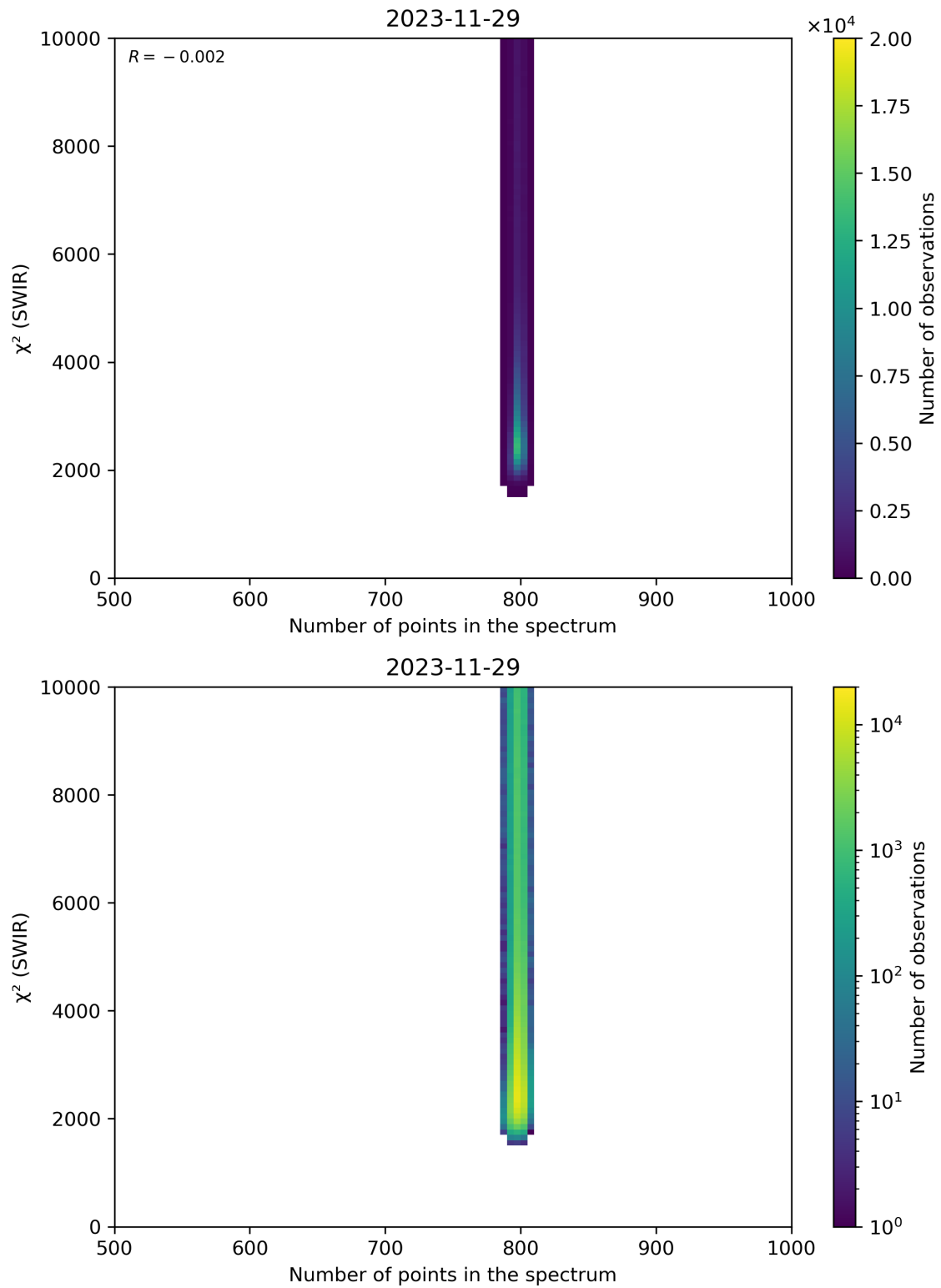
Figure 89: Scatter density plot of “Number of points in the spectrum” against “ \chi^2 (SWIR)” for 2023-11-28 to 2023-11-30.
