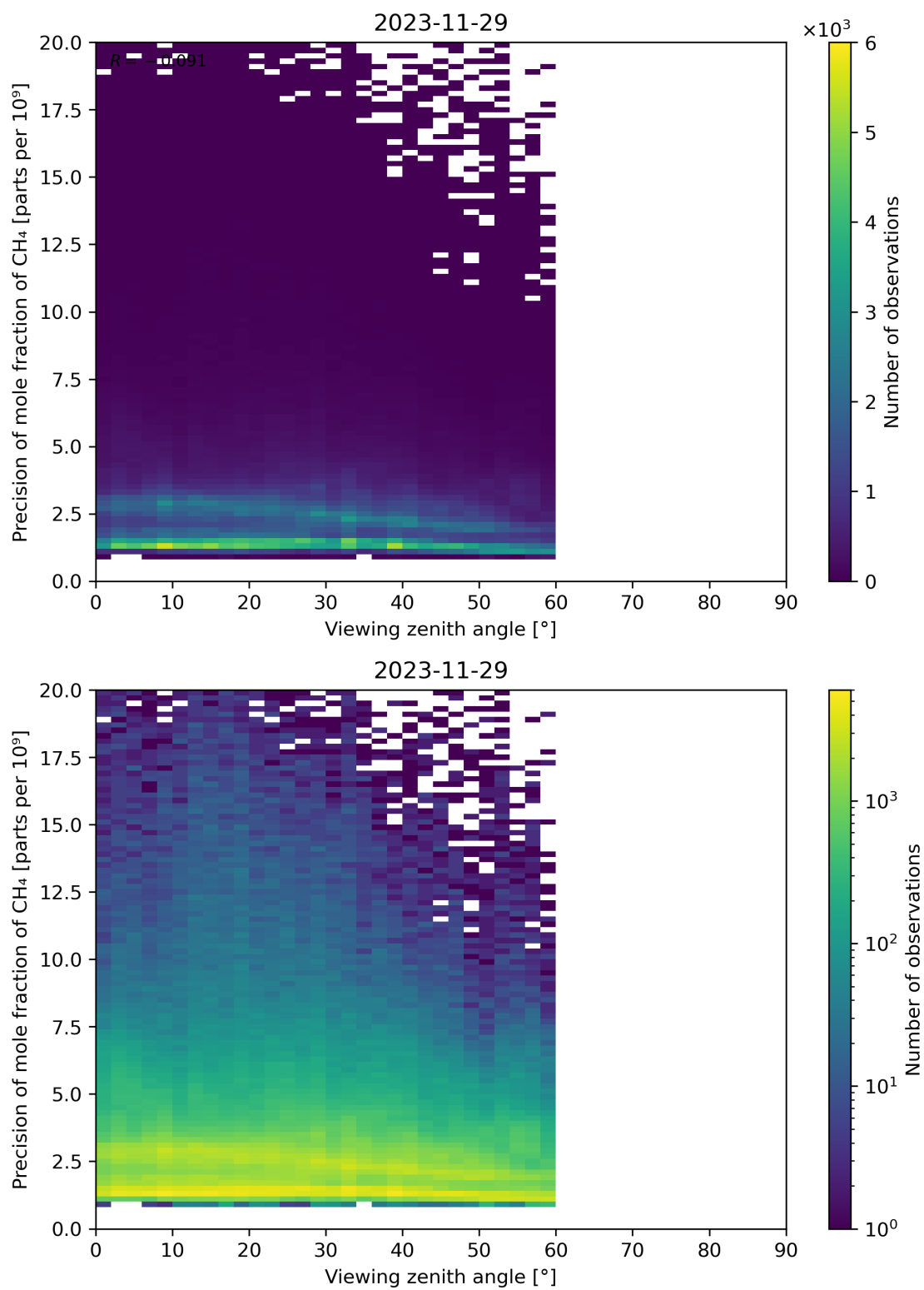
Figure 112: Scatter density plot of “Viewing zenith angle” against “Precision of mole fraction of CH 4 ” for 2023-11-28 to 2023-11-30.
