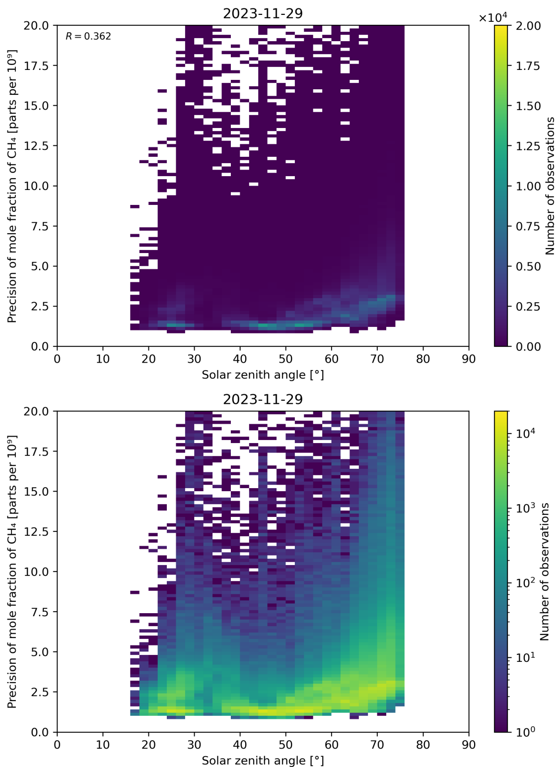
Figure 101: Scatter density plot of “Solar zenith angle” against “Precision of mole fraction of CH 4 ” for 2023-11-28 to 2023-11-30.
