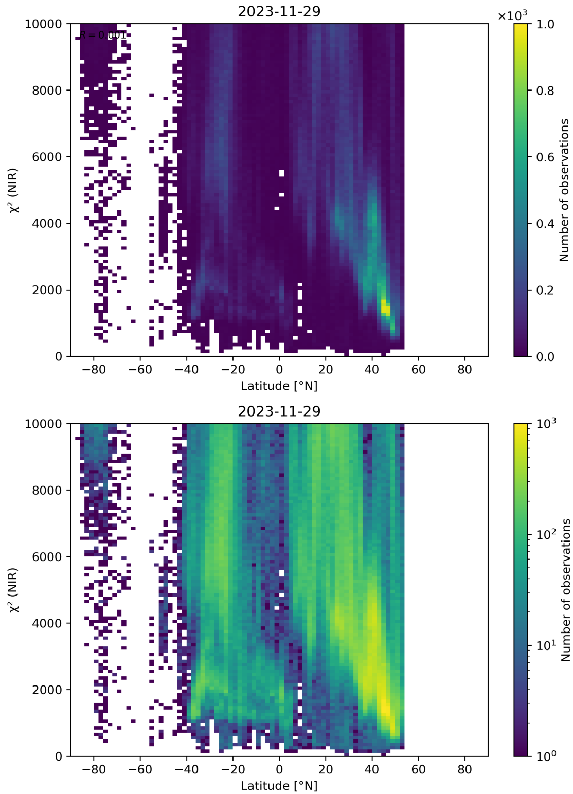
Figure 53: Scatter density plot of “Latitude” against “ \chi^2 (NIR)” for 2023-11-28 to 2023-11-30.
