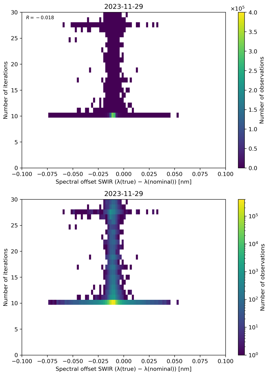
Figure 121: Scatter density plot of “Spectral offset SWIR ( \lambda(\text{true}) - \lambda(\text{nominal}) )” against “Number of iterations” for 2023-11-28 to 2023-11-30.
