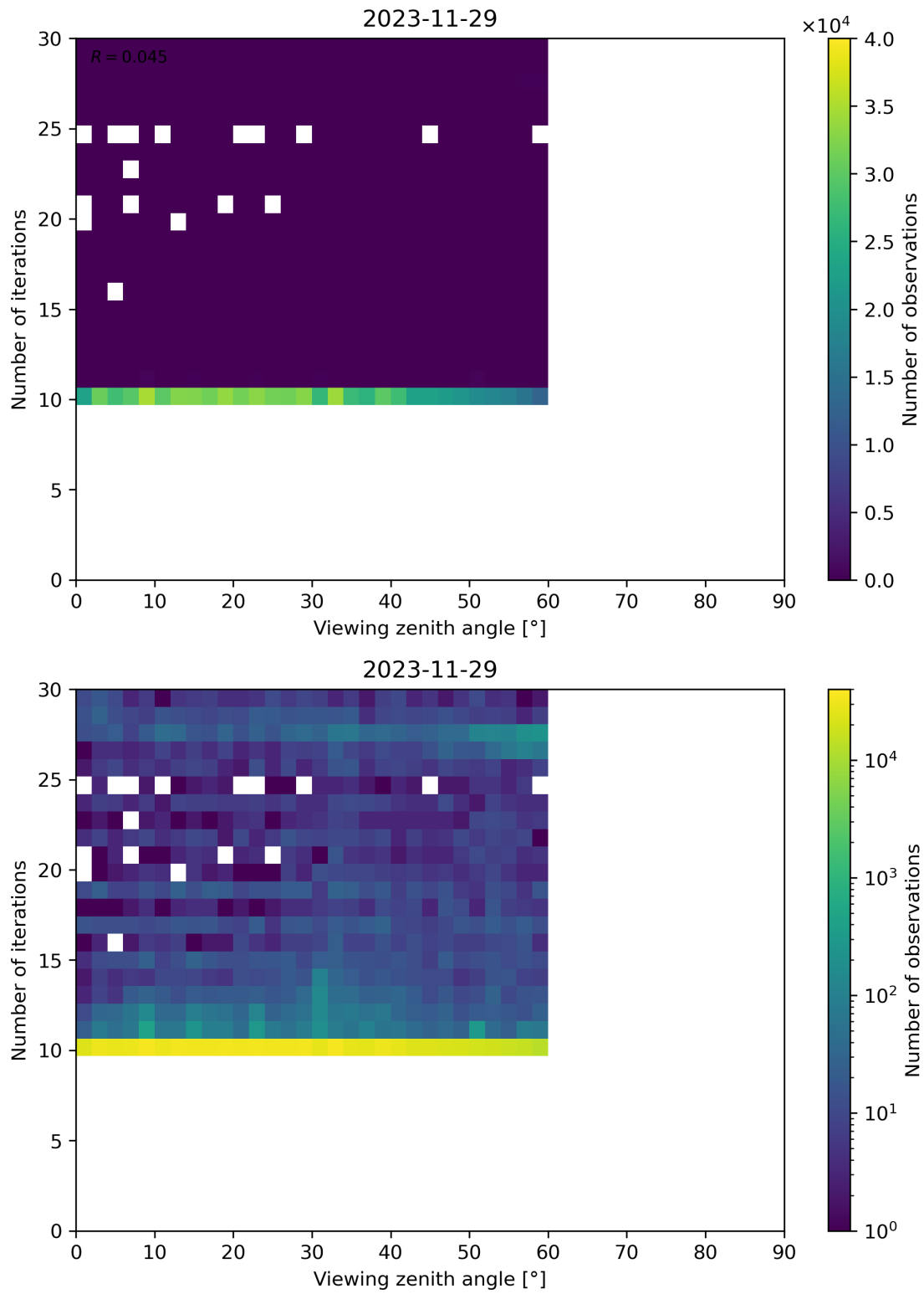
Figure 113: Scatter density plot of “Viewing zenith angle” against “Number of iterations” for 2023-11-28 to 2023-11-30.
