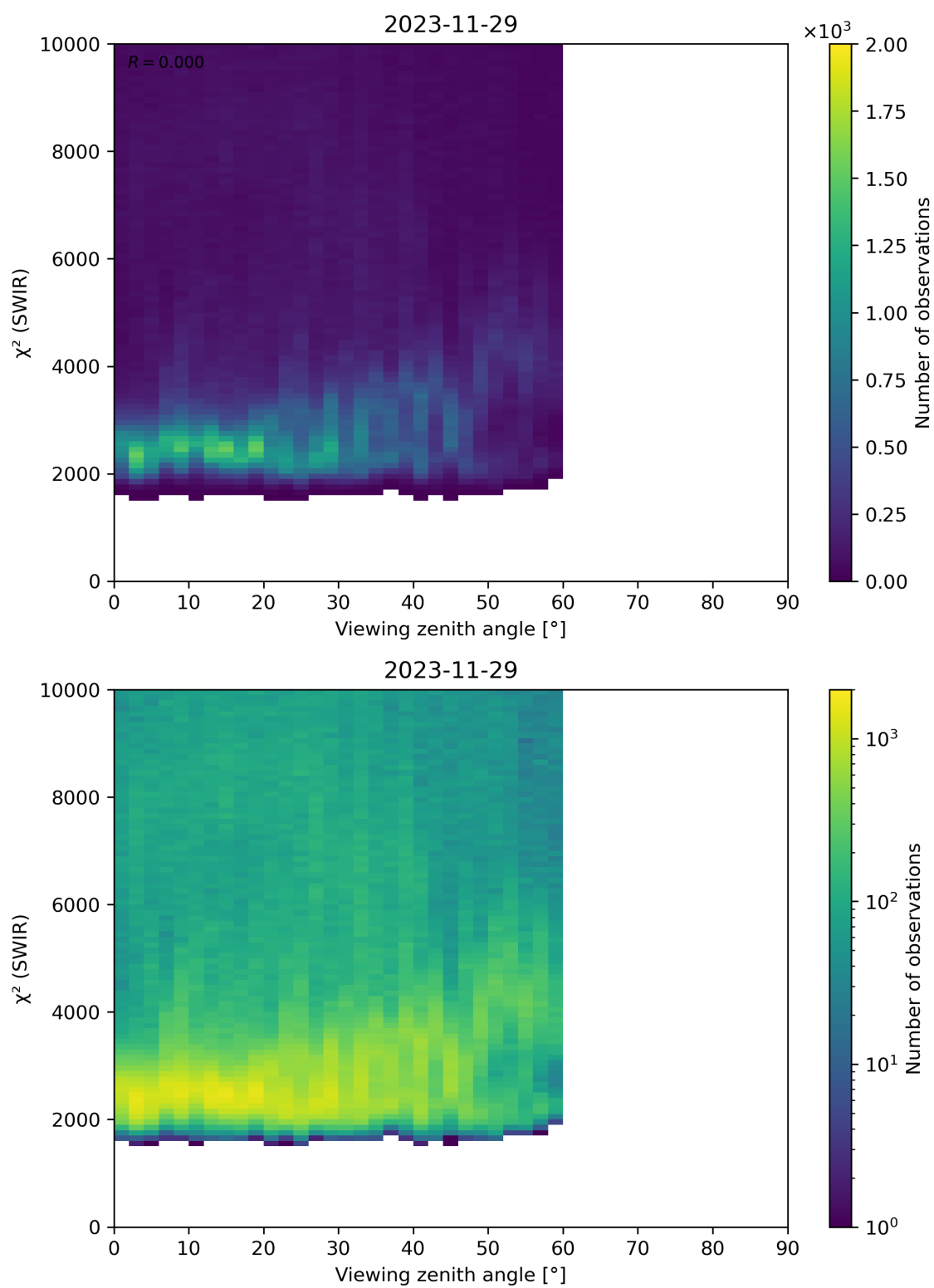
Figure 106: Scatter density plot of “Viewing zenith angle” against “ \chi^2 (SWIR)” for 2023-11-28 to 2023-11-30.
