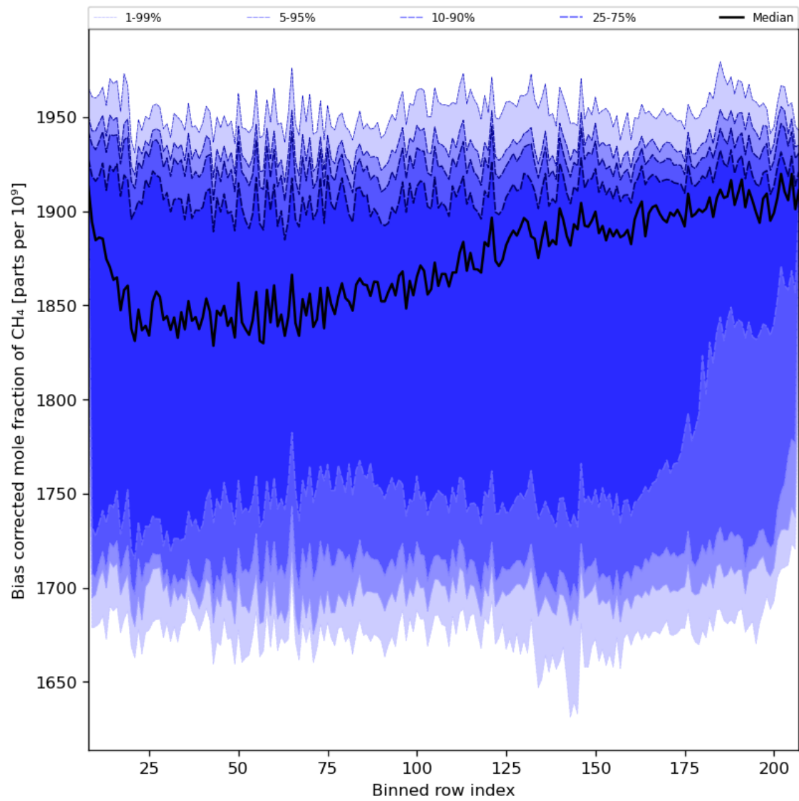
Figure 36: Along track statistics of “Bias corrected mole fraction of CH 4 ” for 2023-11-28 to 2023-11-30
