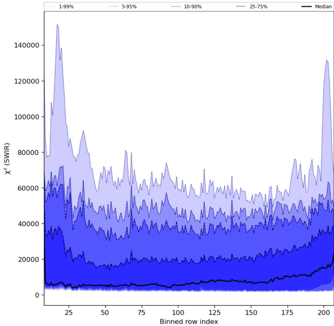
Figure 39: Along track statistics of “ \chi^2 (SWIR)” for 2023-11-28 to 2023-11-30
