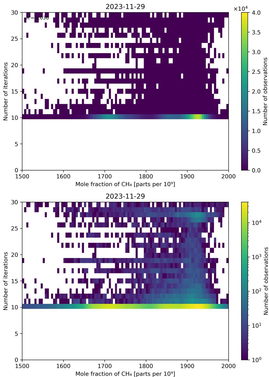
Figure 76: Scatter density plot of “Mole fraction of CH 4 ” against “Number of iterations” for 2023-11-28 to 2023-11-30.
