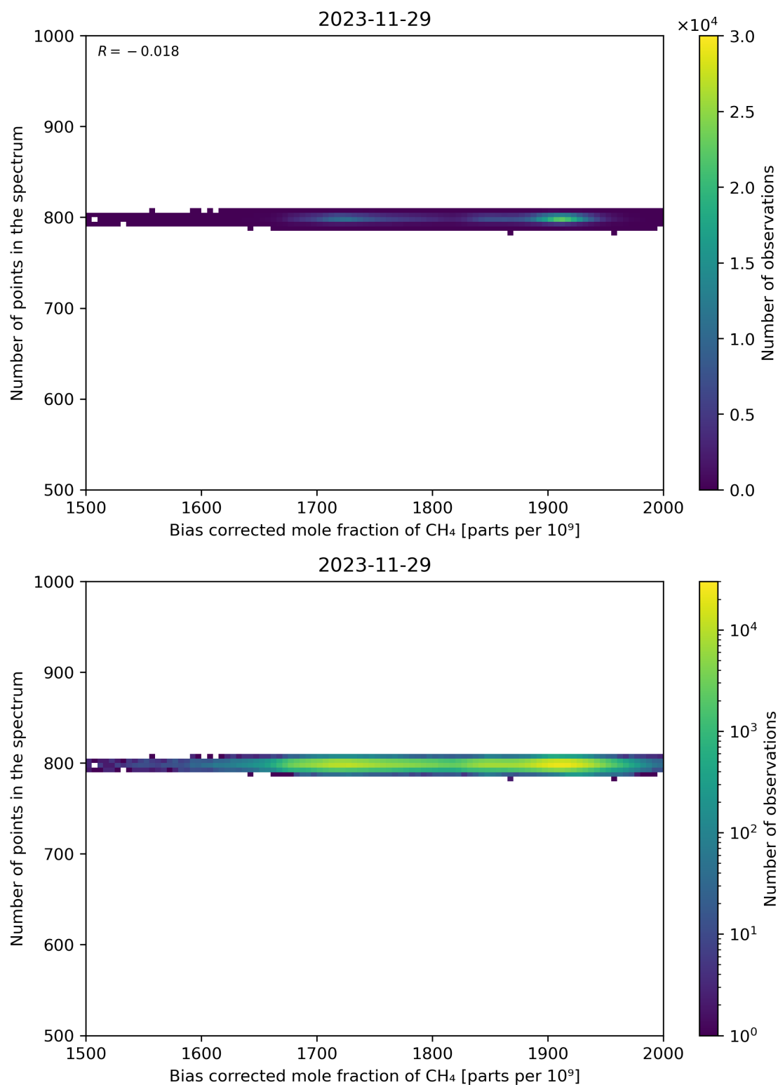
Figure 68: Scatter density plot of “Bias corrected mole fraction of CH 4 ” against “Number of points in the spectrum” for 2023-11-28 to 2023-11-30.
