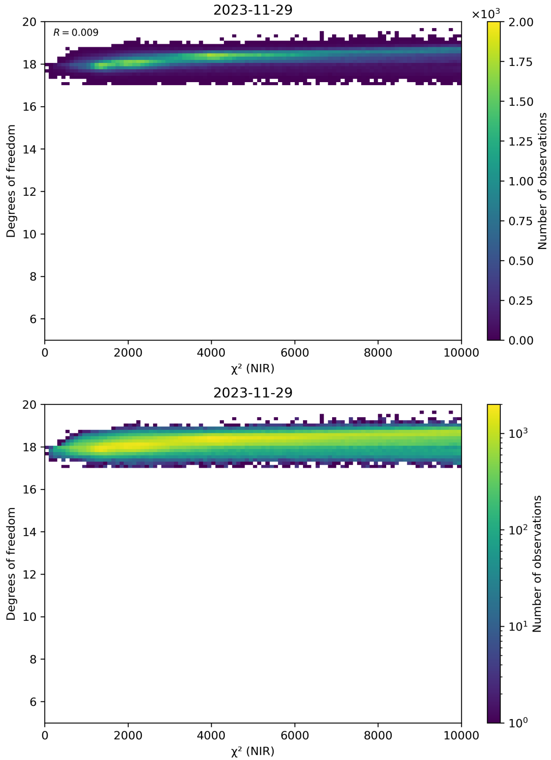
Figure 44: Scatter density plot of “ \chi^2 (NIR)” against “Degrees of freedom” for 2023-11-28 to 2023-11-30.
