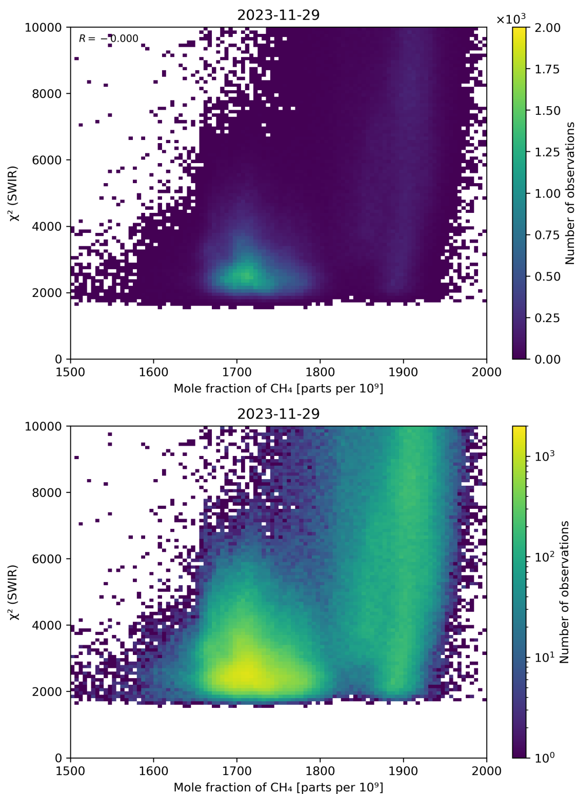
Figure 71: Scatter density plot of “Mole fraction of \text{CH}_4 ” against “ \chi^2 (SWIR)” for 2023-11-28 to 2023-11-30.
