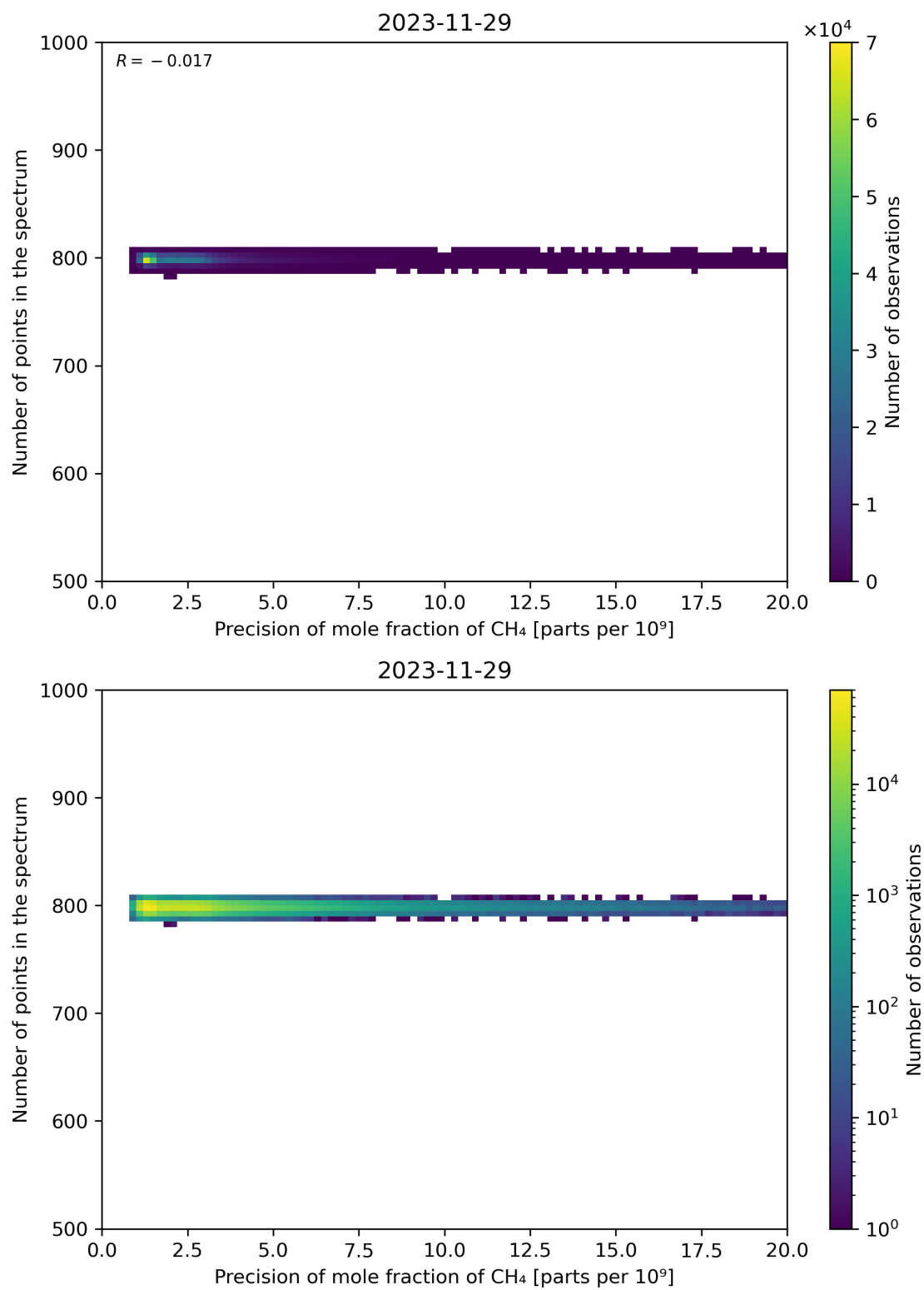
Figure 84: Scatter density plot of “Precision of mole fraction of CH 4 ” against “Number of points in the spectrum” for 2023-11-28 to 2023-11-30.
