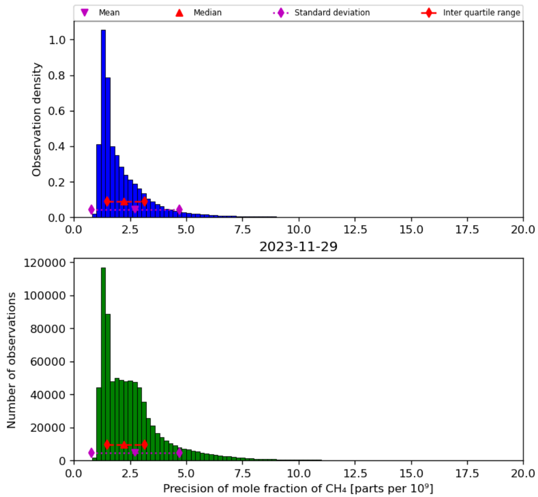
Figure 24: Histogram of “Precision of mole fraction of CH 4 ” for 2023-11-28 to 2023-11-30
