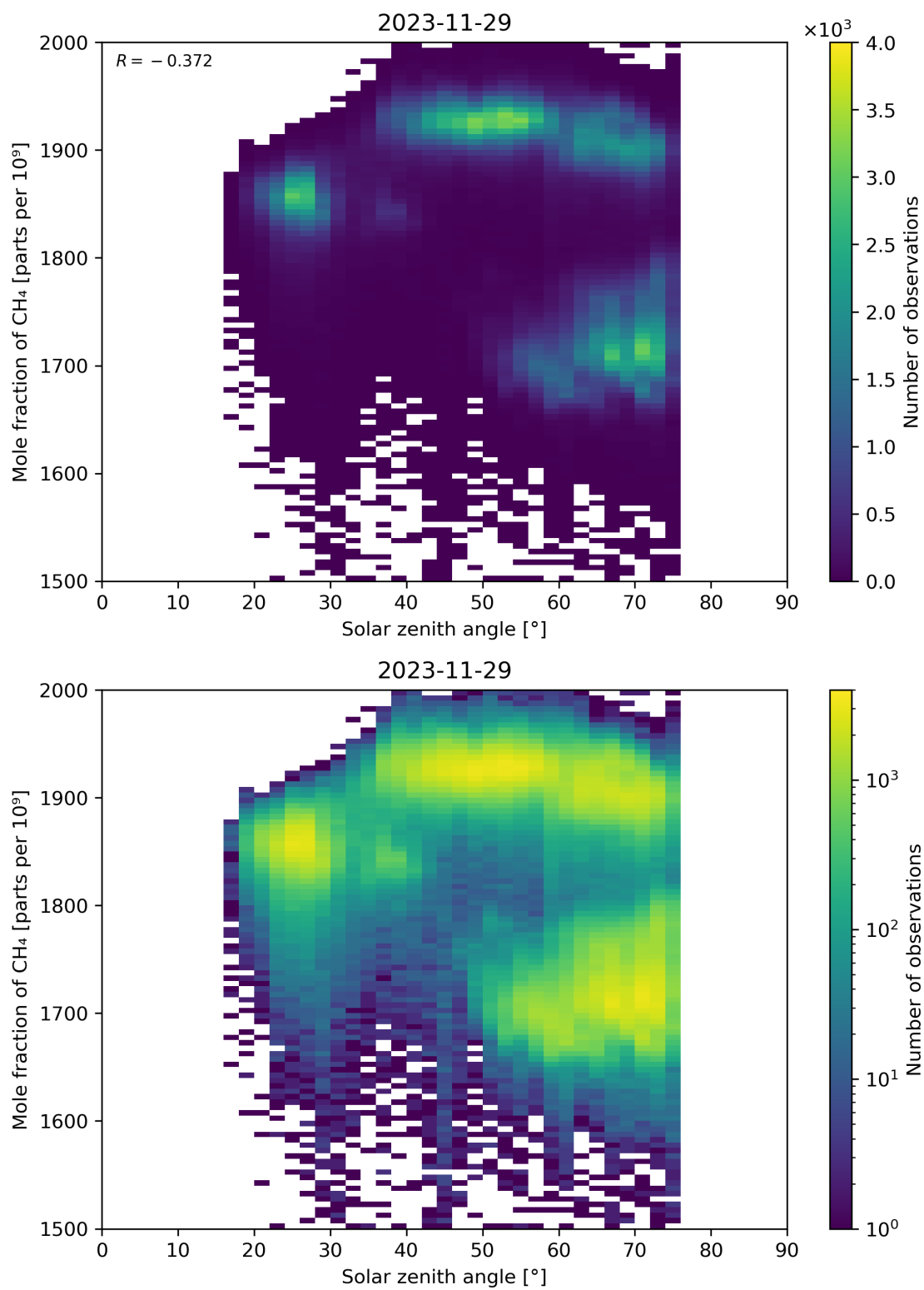
Figure 99: Scatter density plot of “Solar zenith angle” against “Mole fraction of CH 4 ” for 2023-11-28 to 2023-11-30.
