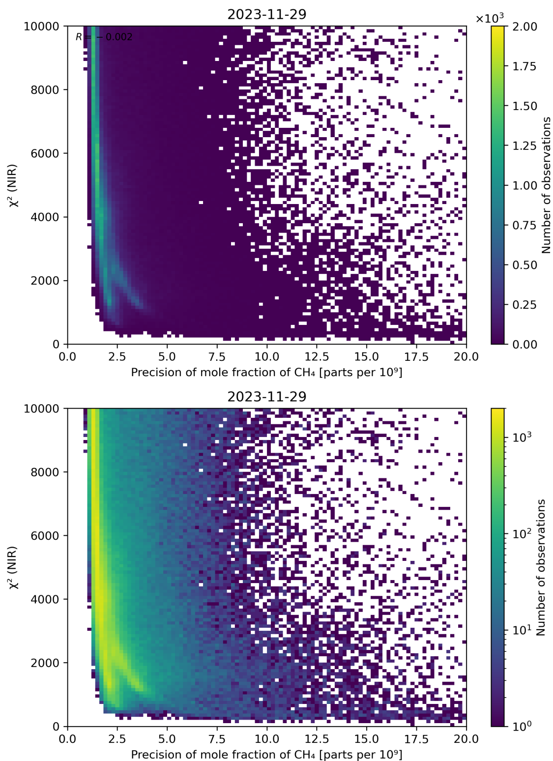
Figure 78: Scatter density plot of “Precision of mole fraction of CH 4 ” against “ \chi^2 (NIR)” for 2023-11-28 to 2023-11-30.
