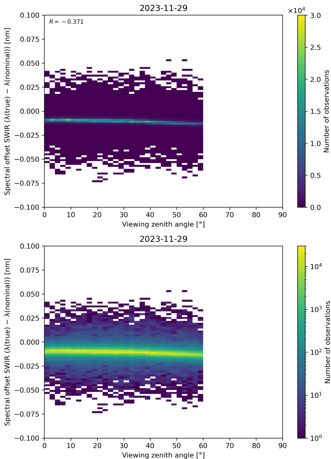
Figure 116: Scatter density plot of “Viewing zenith angle” against “Spectral offset SWIR ( \lambda(\text{true}) - \lambda(\text{nominal}) )” for 2023-11-28 to 2023-11-30.
