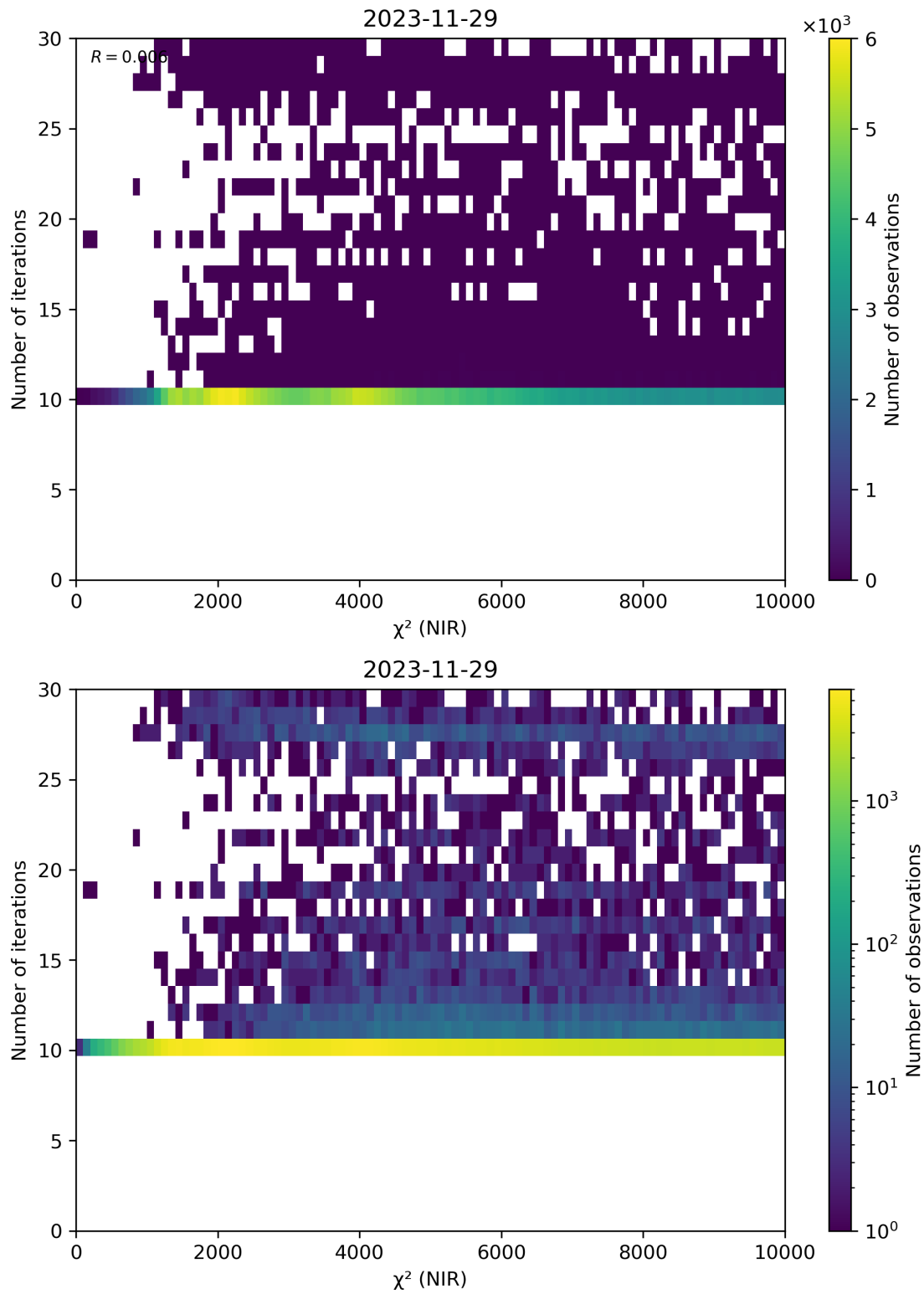
Figure 46: Scatter density plot of “ \chi^2 (NIR)” against “Number of iterations” for 2023-11-28 to 2023-11-30.
