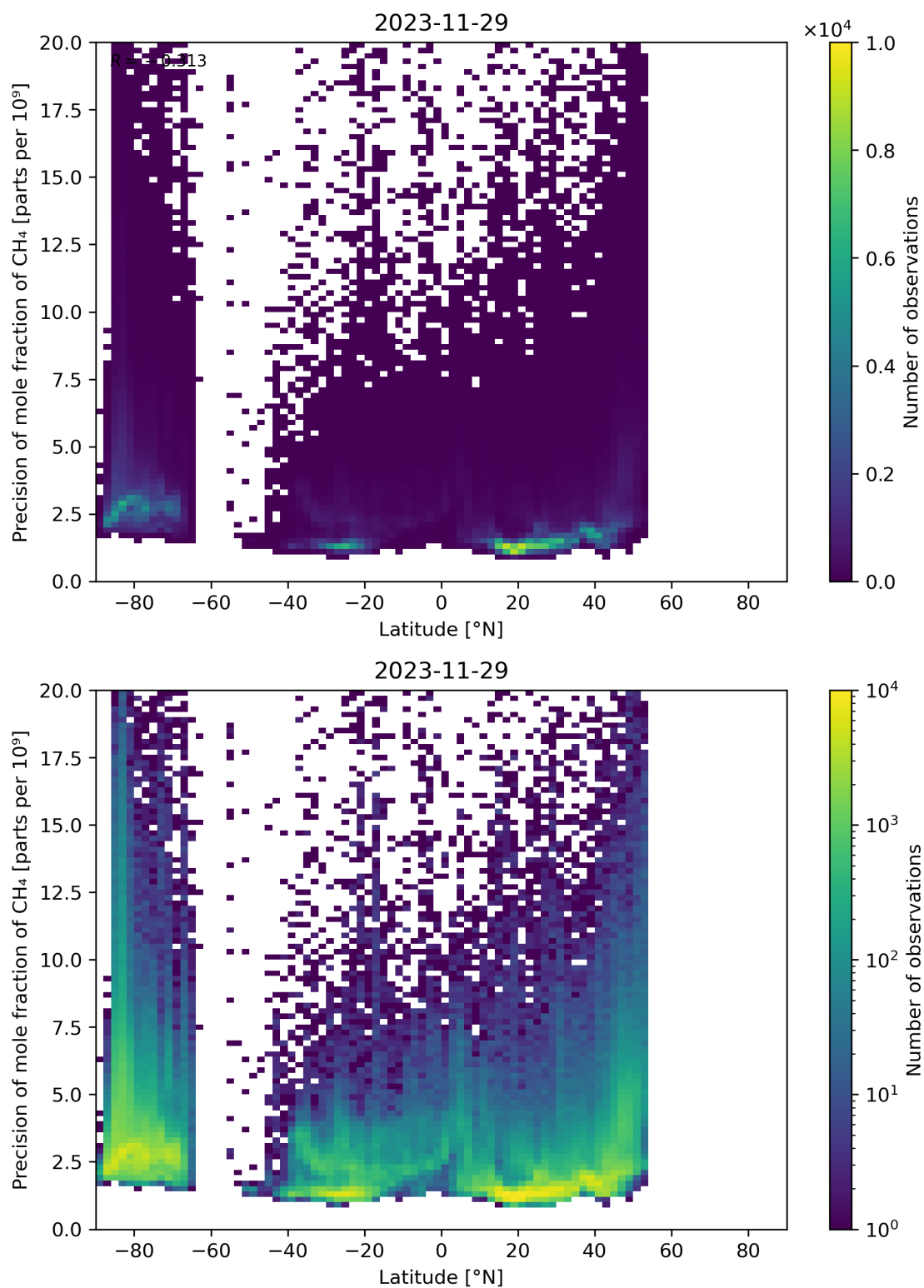
Figure 59: Scatter density plot of “Latitude” against “Precision of mole fraction of CH 4 ” for 2023-11-28 to 2023-11-30.
