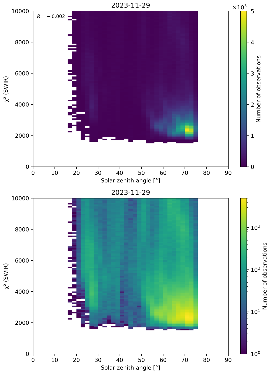
Figure 95: Scatter density plot of “Solar zenith angle” against “ \chi^2 (SWIR)” for 2023-11-28 to 2023-11-30.
