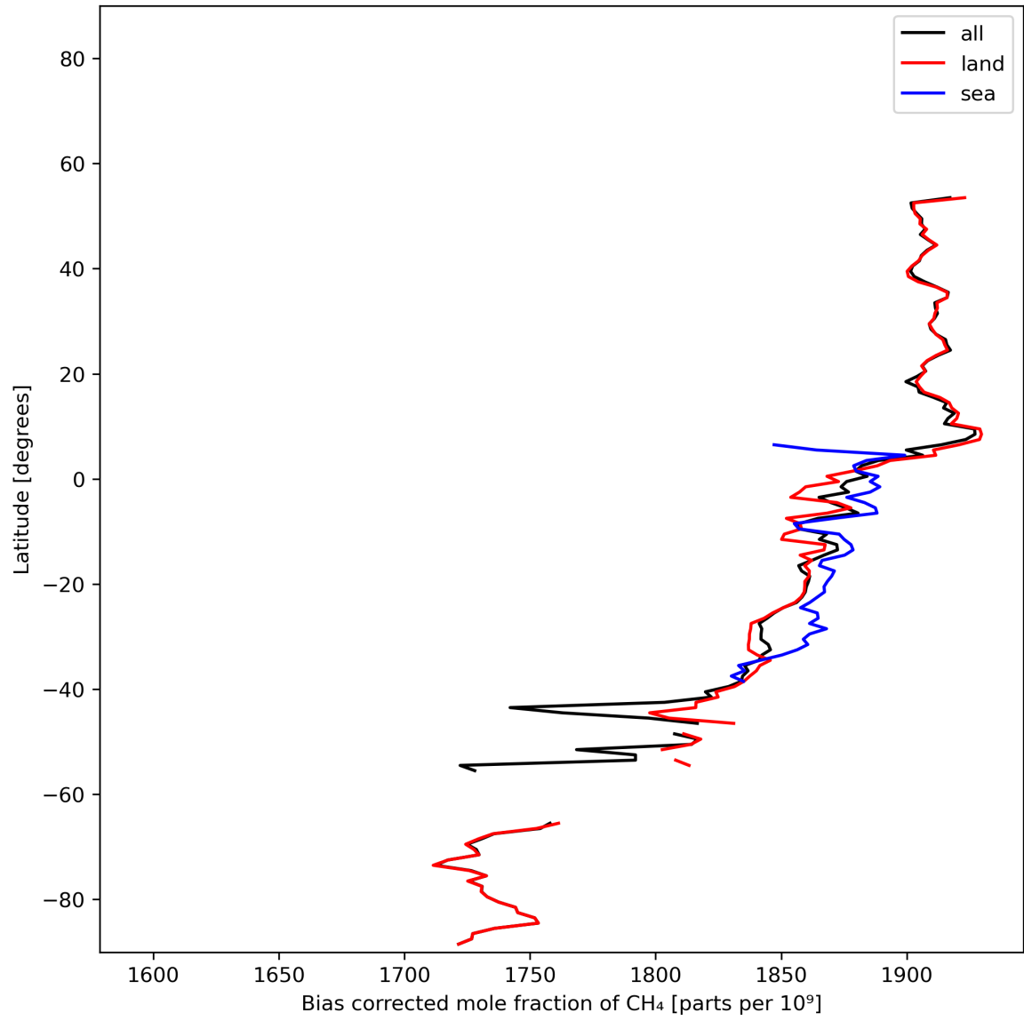
Figure 14: Zonal average of “Bias corrected mole fraction of CH 4 ” for 2023-11-28 to 2023-11-30.
