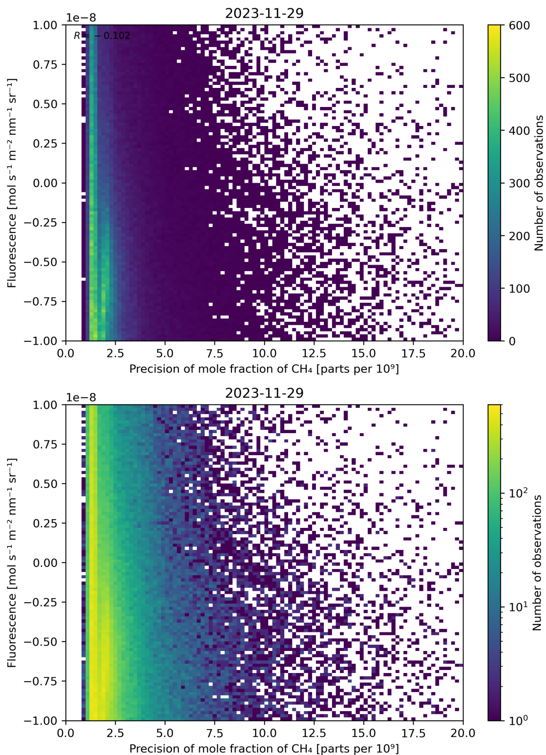
Figure 81: Scatter density plot of “Precision of mole fraction of CH 4 ” against “Fluorescence” for 2023-11-28 to 2023-11-30.
