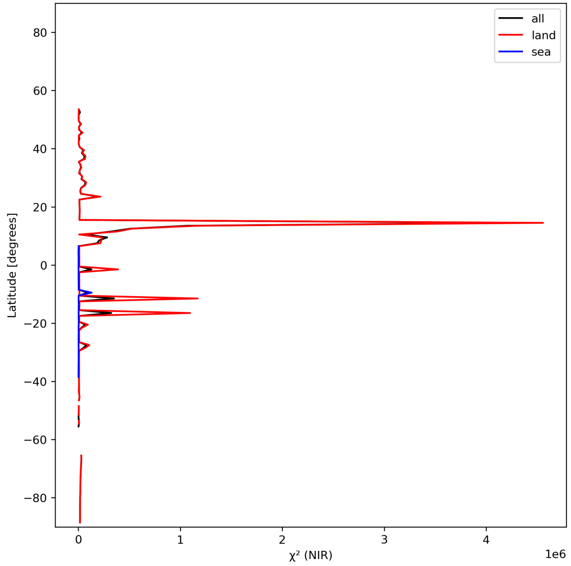
Figure 18: Zonal average of “ \chi^2 (NIR)” for 2023-11-28 to 2023-11-30.
