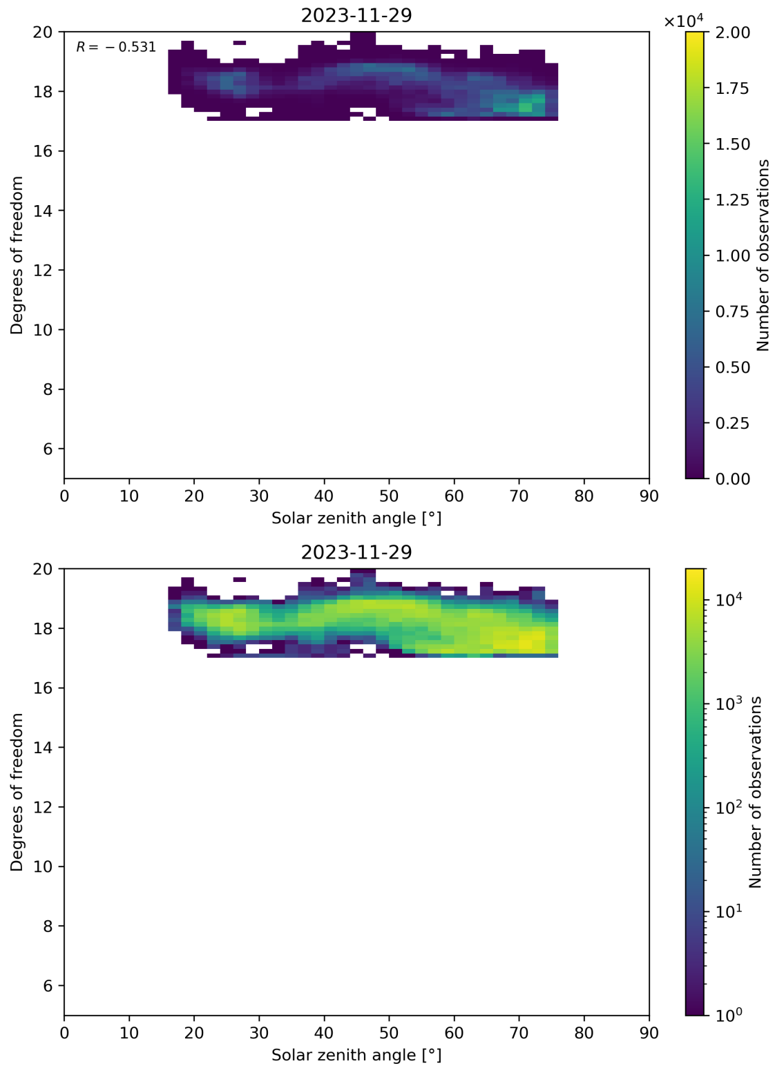
Figure 96: Scatter density plot of “Solar zenith angle” against “Degrees of freedom” for 2023-11-28 to 2023-11-30.
