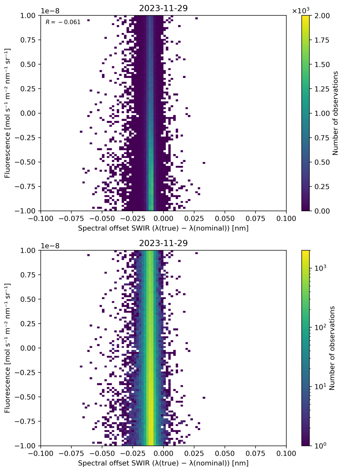
Figure 120: Scatter density plot of “Spectral offset SWIR ( \lambda(\text{true}) - \lambda(\text{nominal}) )” against “Fluorescence” for 2023-11-28 to 2023-11-30.
