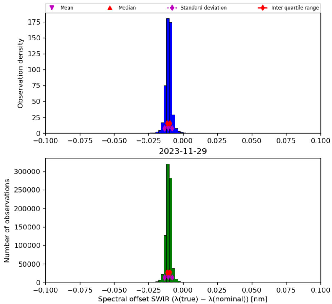
Figure 27: Histogram of “Spectral offset SWIR ( \lambda(\text{true}) - \lambda(\text{nominal}) )” for 2023-11-28 to 2023-11-30
