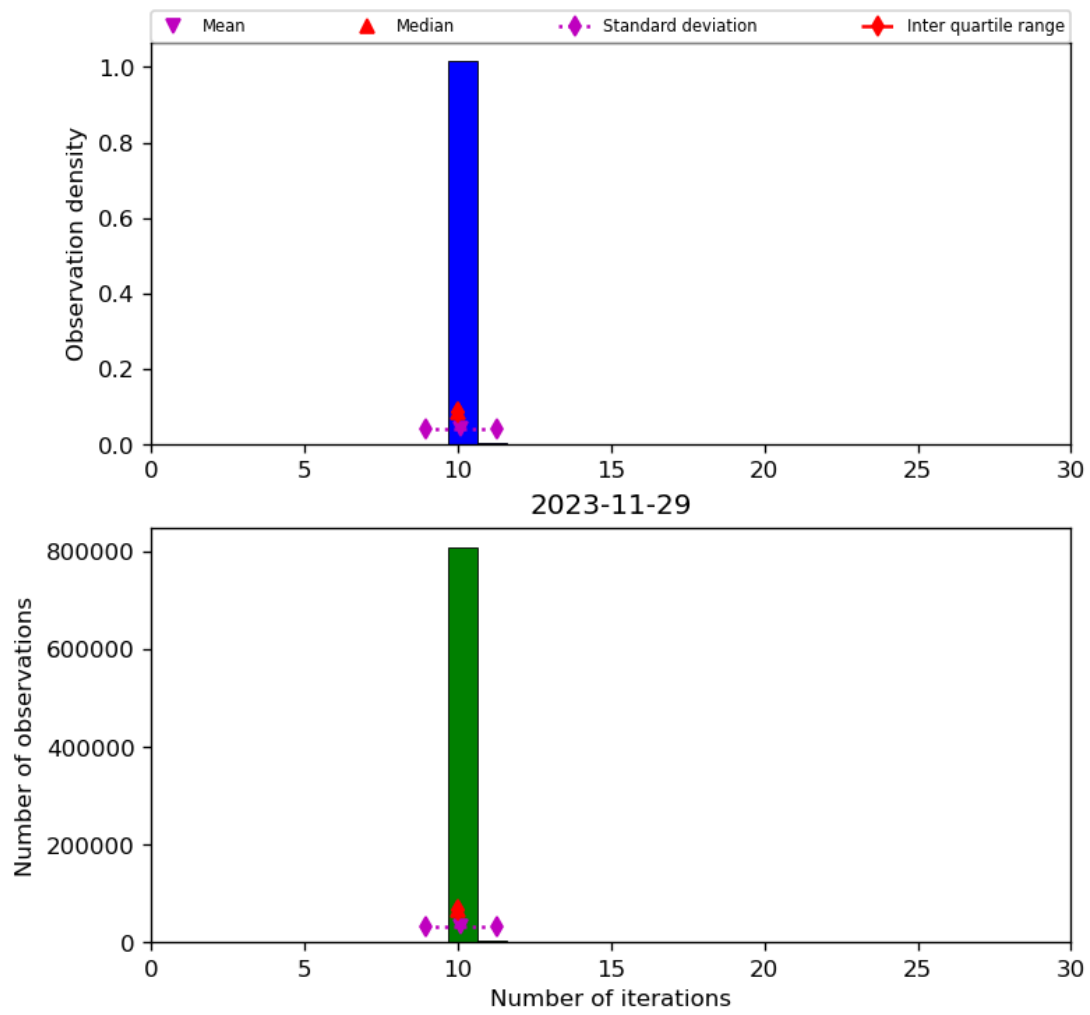
Figure 31: Histogram of “Number of iterations” for 2023-11-28 to 2023-11-30
