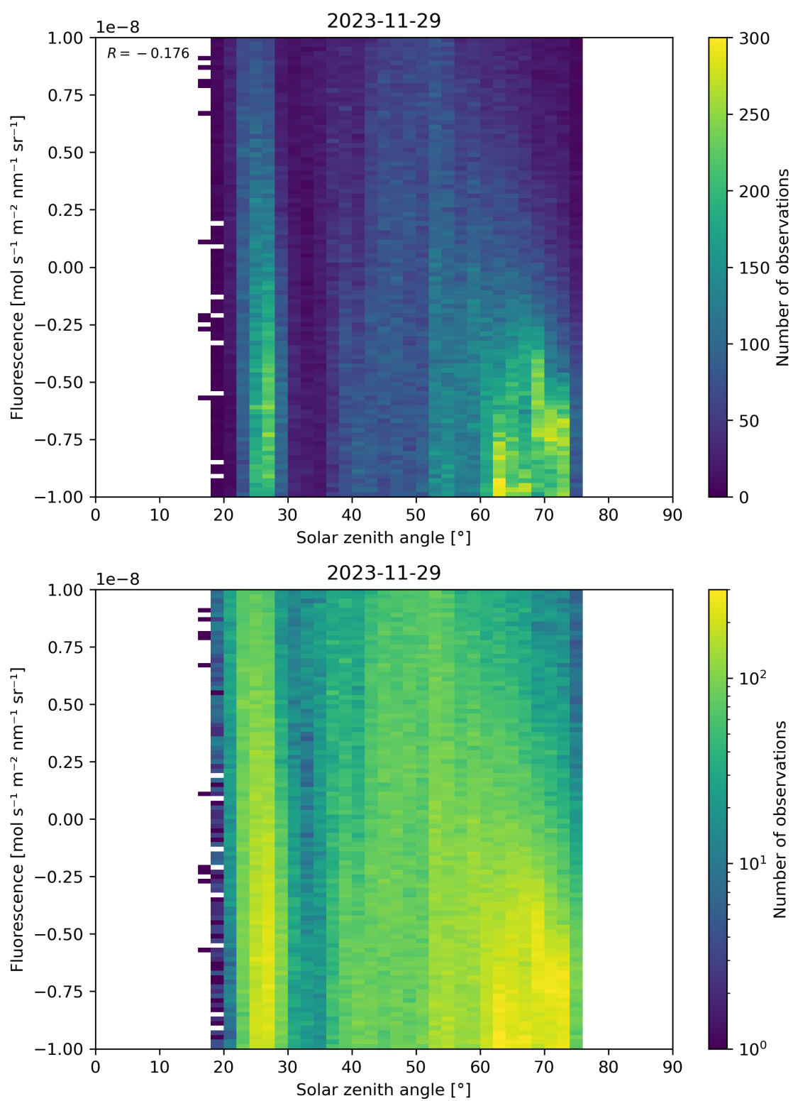
Figure 97: Scatter density plot of “Solar zenith angle” against “Fluorescence” for 2023-11-28 to 2023-11-30.
