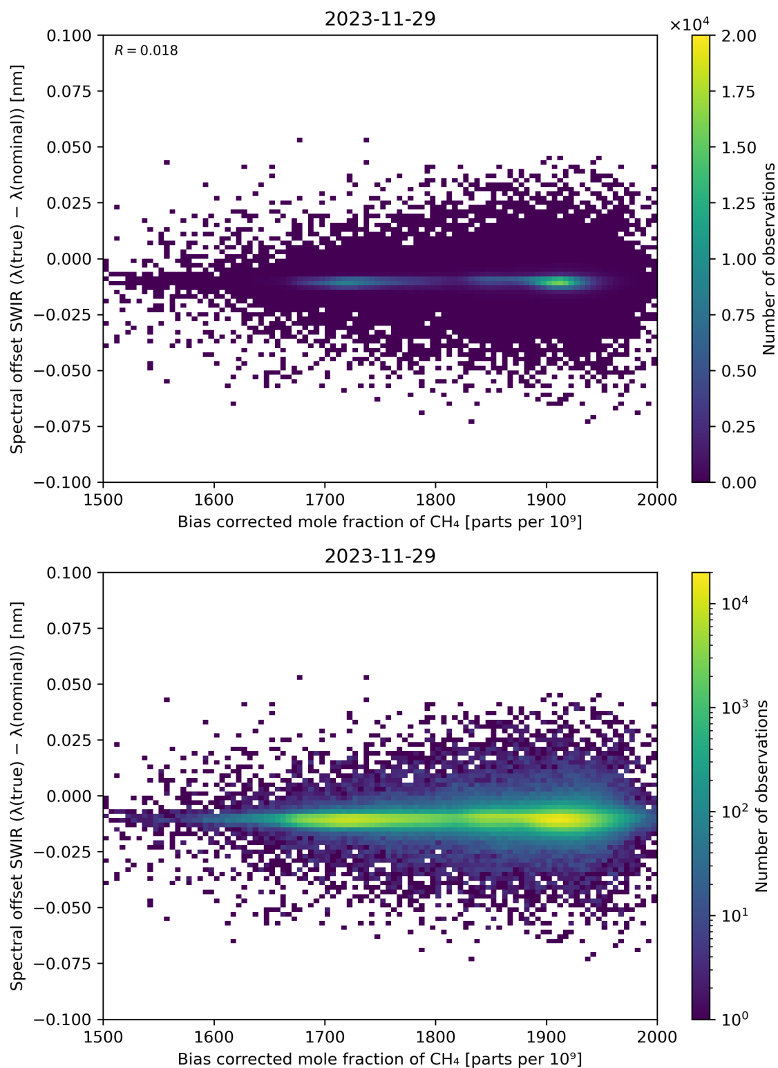
Figure 69: Scatter density plot of “Bias corrected mole fraction of \text{CH}_4 ” against “Spectral offset SWIR ( \lambda(\text{true}) - \lambda(\text{nominal}) )” for 2023-11-28 to 2023-11-30.
