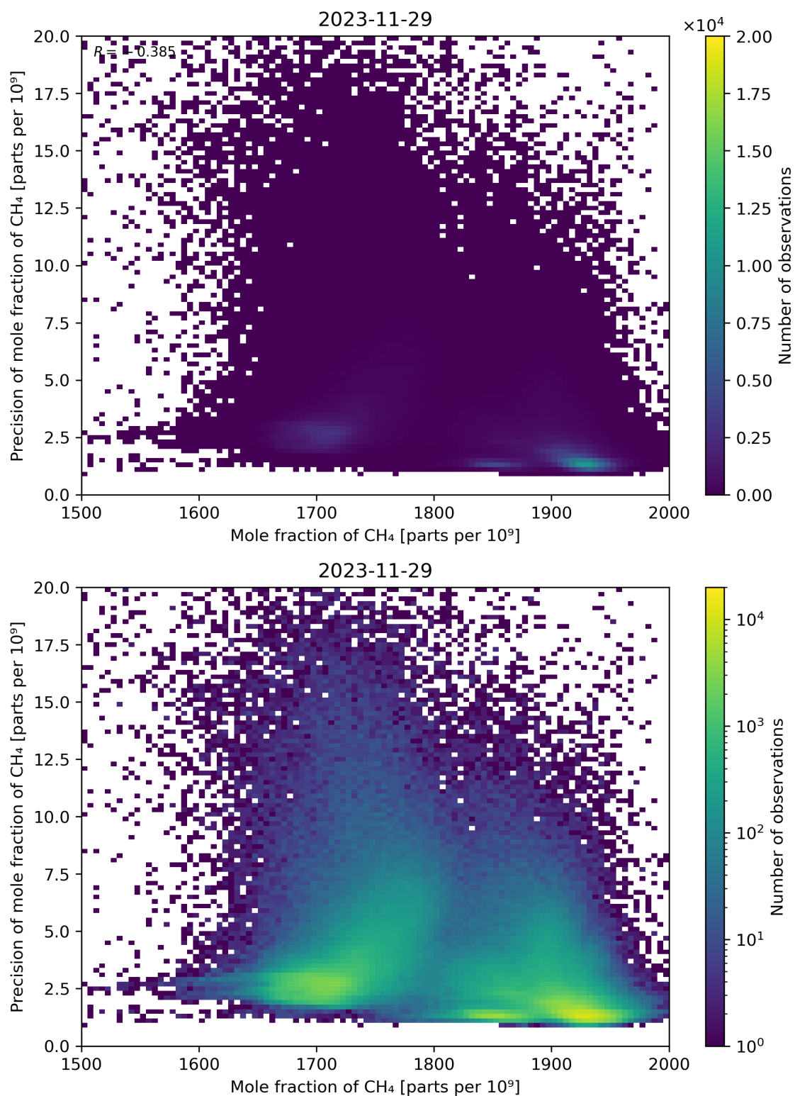
Figure 75: Scatter density plot of “Mole fraction of CH 4 ” against “Precision of mole fraction of CH 4 ” for 2023-11-28 to 2023-11-30.
