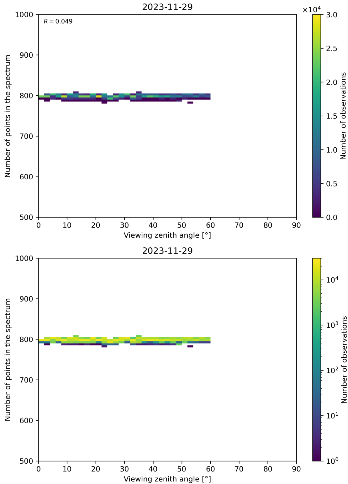
Figure 114: Scatter density plot of “Viewing zenith angle” against “Number of points in the spectrum” for 2023-11-28 to 2023-11-30.
