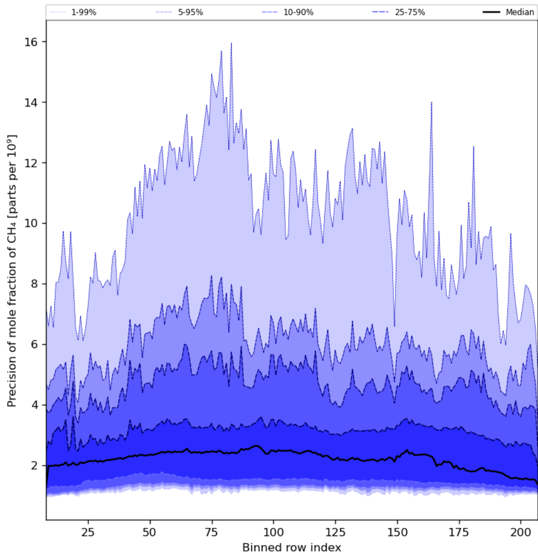
Figure 35: Along track statistics of “Precision of mole fraction of CH 4 ” for 2023-11-28 to 2023-11-30
