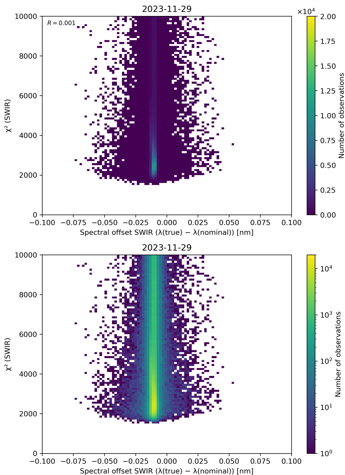
Figure 118: Scatter density plot of “Spectral offset SWIR ( \lambda(\text{true}) - \lambda(\text{nominal}) )” against “ \chi^2 (SWIR)” for 2023-11-28 to 2023-11-30.
