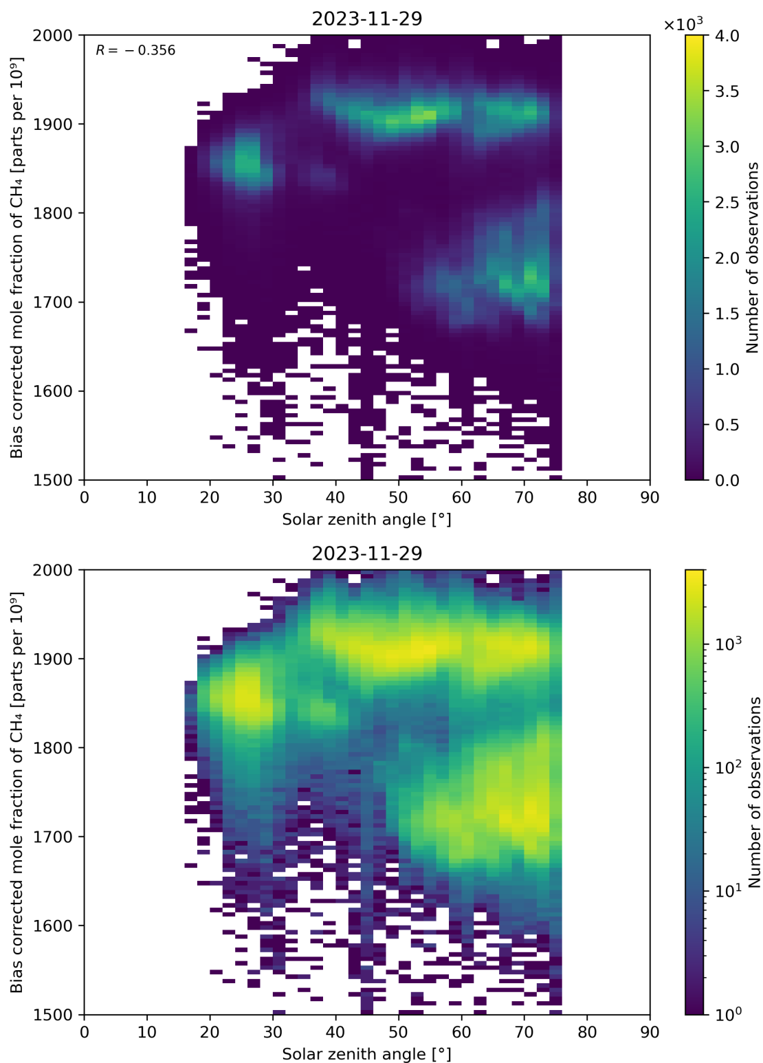
Figure 100: Scatter density plot of “Solar zenith angle” against “Bias corrected mole fraction of \text{CH}_4 ” for 2023-11-28 to 2023-11-30.
