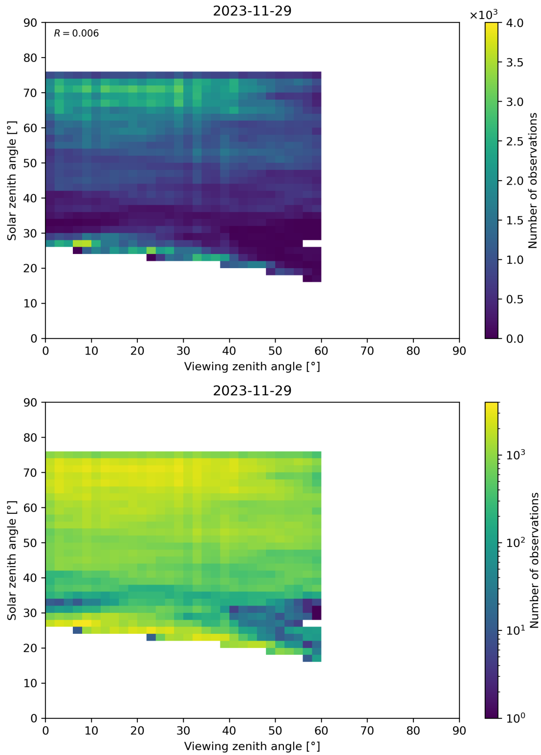
Figure 115: Scatter density plot of “Viewing zenith angle” against “Solar zenith angle” for 2023-11-28 to 2023-11-30.
