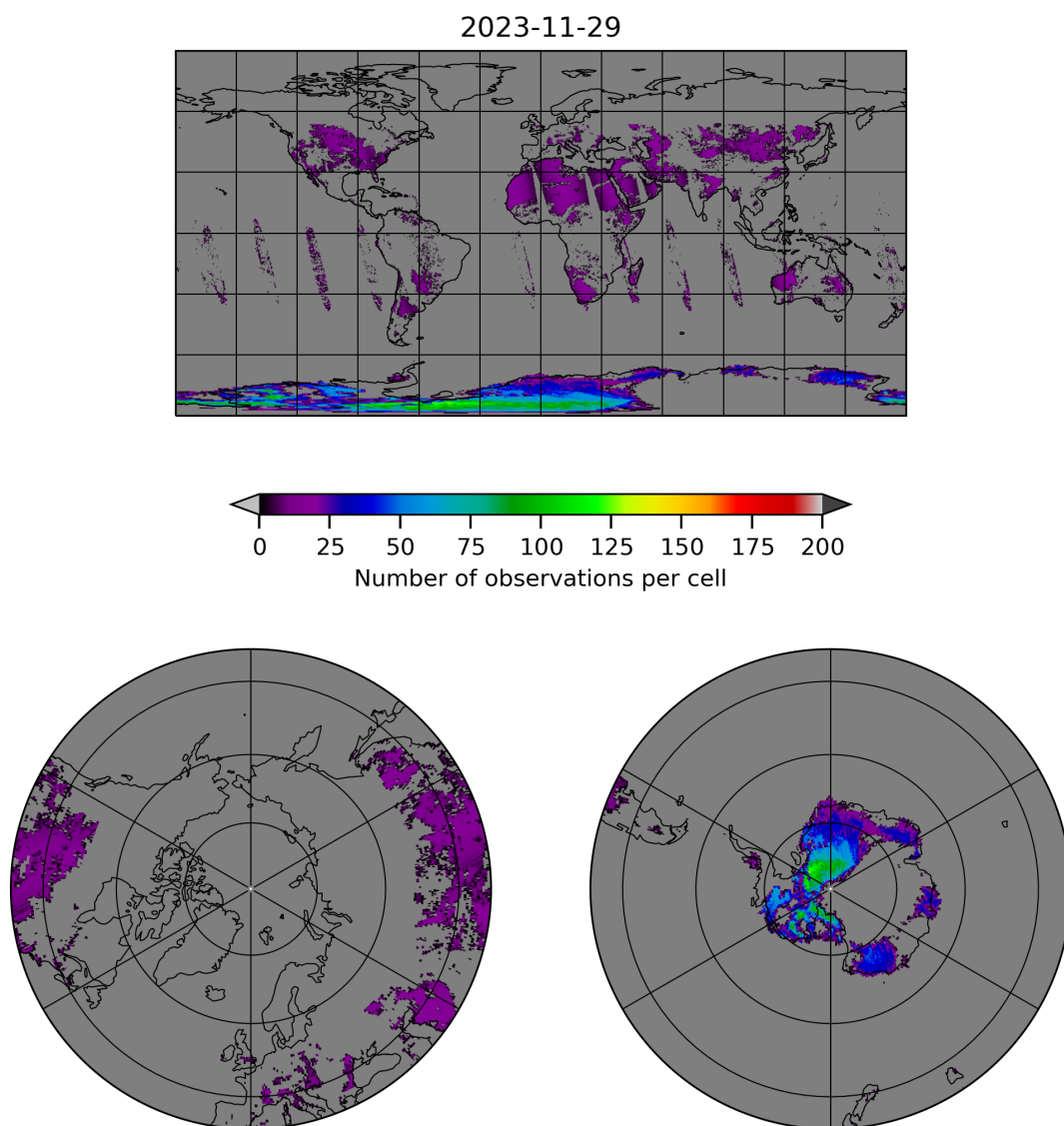
Figure 10: Map of the number of observations for 2023-11-28 to 2023-11-30
