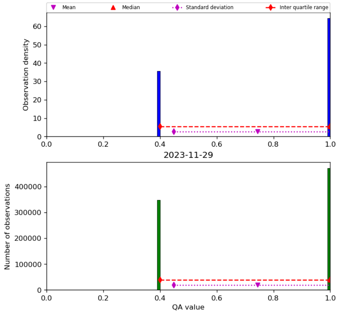
Figure 22: Histogram of “QA value” for 2023-11-28 to 2023-11-30
