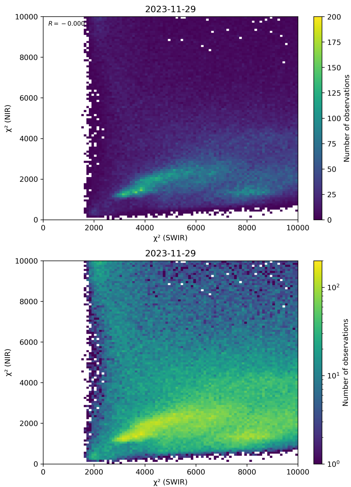
Figure 47: Scatter density plot of “ \chi^2 (SWIR)” against “ \chi^2 (NIR)” for 2023-11-28 to 2023-11-30.
