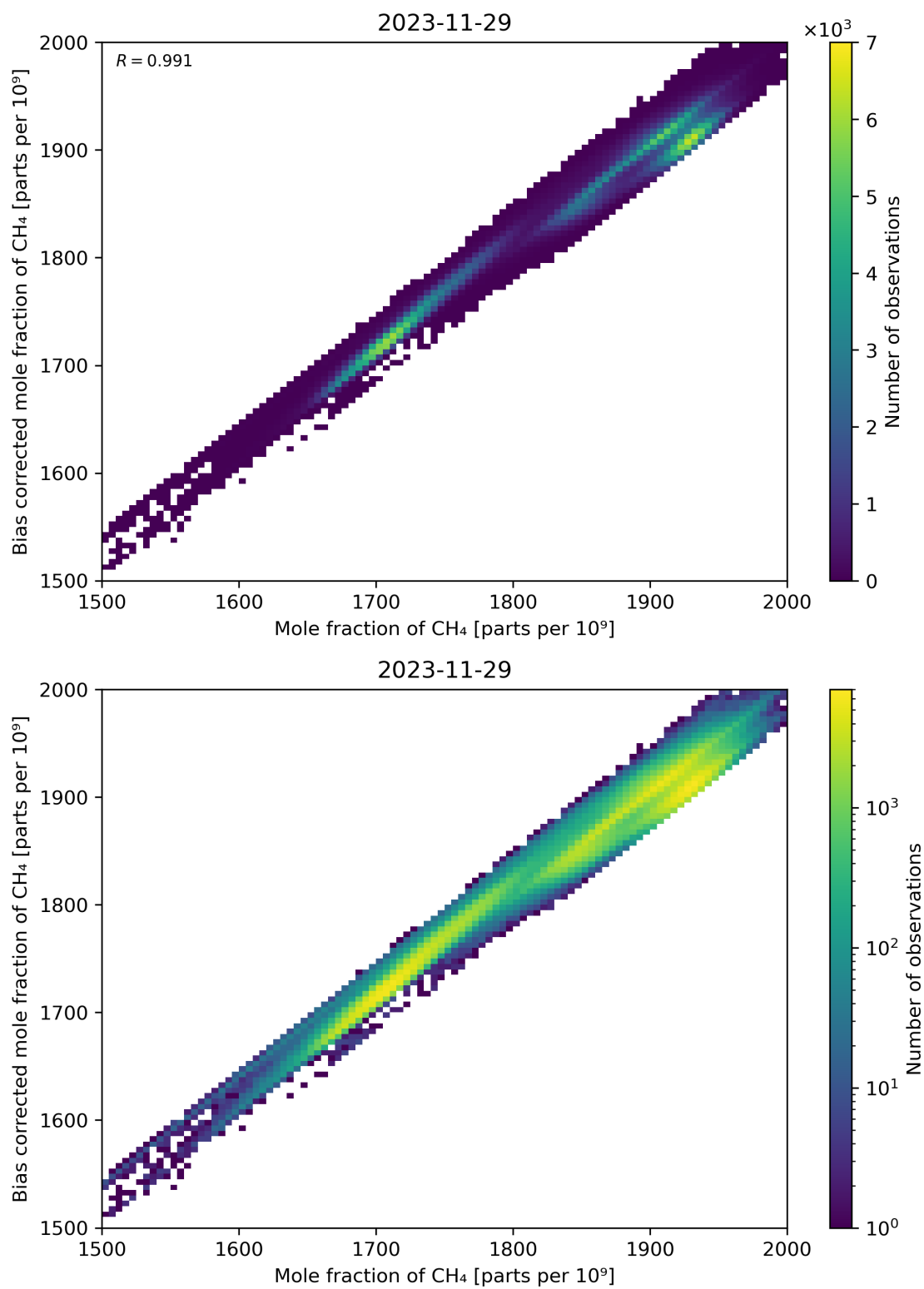
Figure 74: Scatter density plot of “Mole fraction of CH 4 ” against “Bias corrected mole fraction of CH 4 ” for 2023-11-28 to 2023-11-30.
