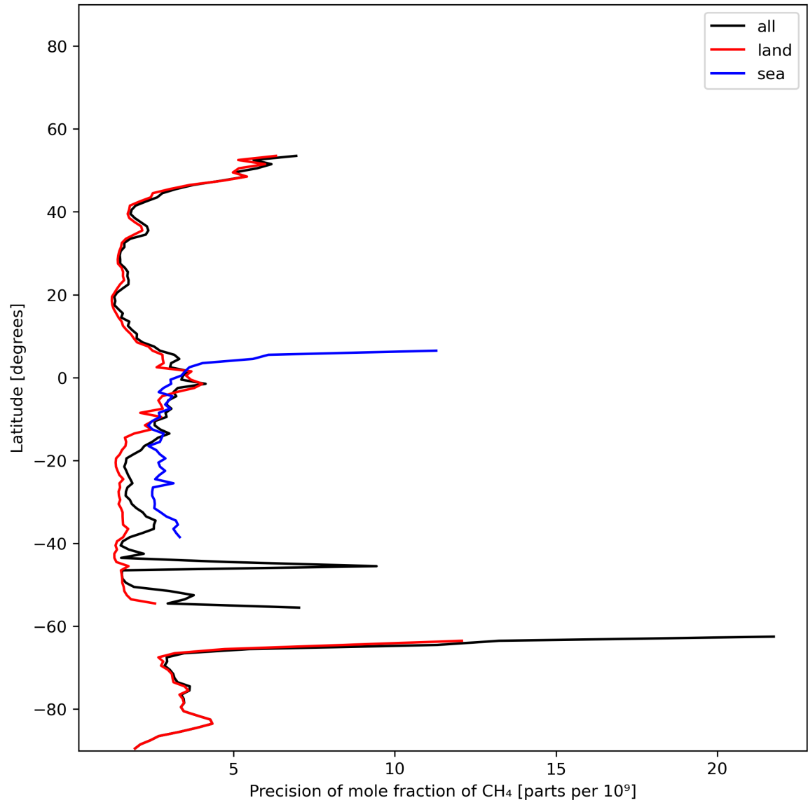
Figure 13: Zonal average of “Precision of mole fraction of CH 4 ” for 2023-11-29 to 2023-12-01.
