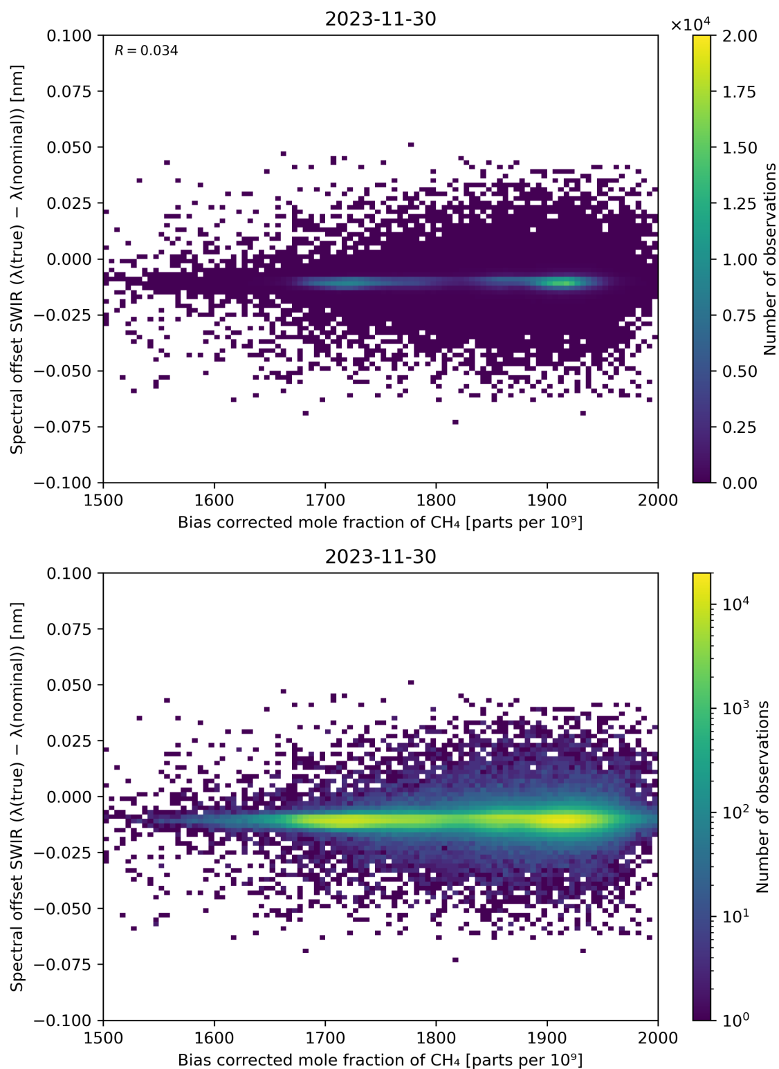
Figure 69: Scatter density plot of “Bias corrected mole fraction of \text{CH}_4 ” against “Spectral offset SWIR ( \lambda(\text{true}) - \lambda(\text{nominal}) )” for 2023-11-29 to 2023-12-01.
