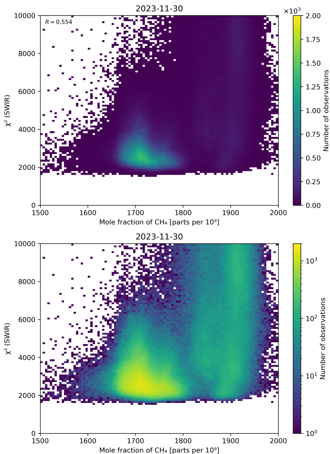
Figure 71: Scatter density plot of “Mole fraction of \text{CH}_4 ” against “ \chi^2 (SWIR)” for 2023-11-29 to 2023-12-01.
