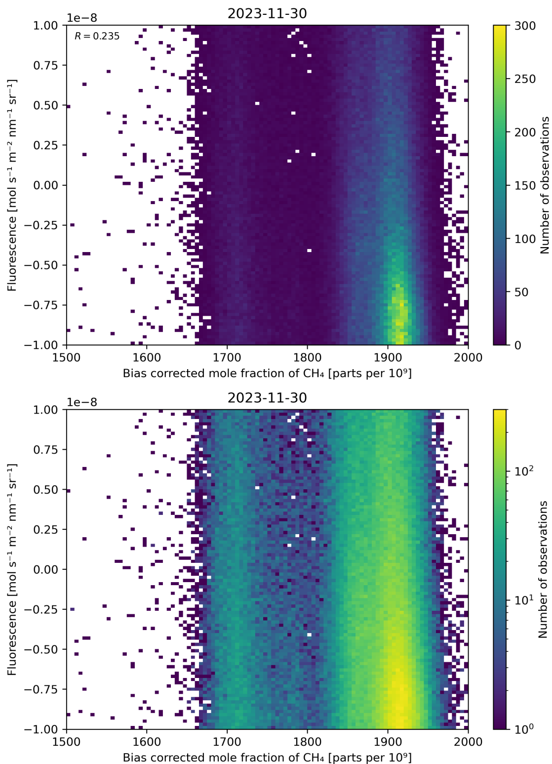
Figure 66: Scatter density plot of “Bias corrected mole fraction of \text{CH}_4 ” against “Fluorescence” for 2023-11-29 to 2023-12-01.
