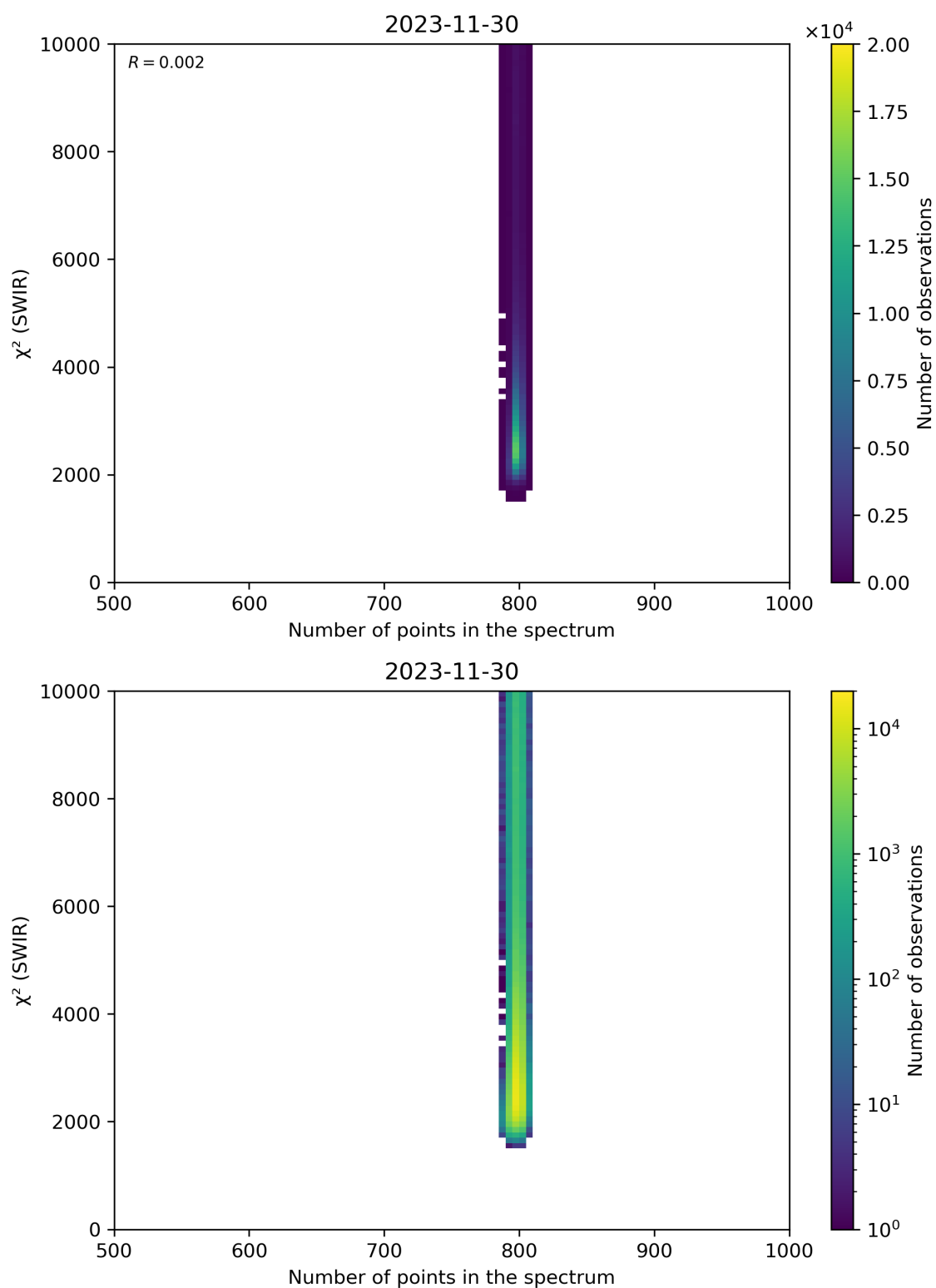
Figure 89: Scatter density plot of “Number of points in the spectrum” against “ \chi^2 (SWIR)” for 2023-11-29 to 2023-12-01.
