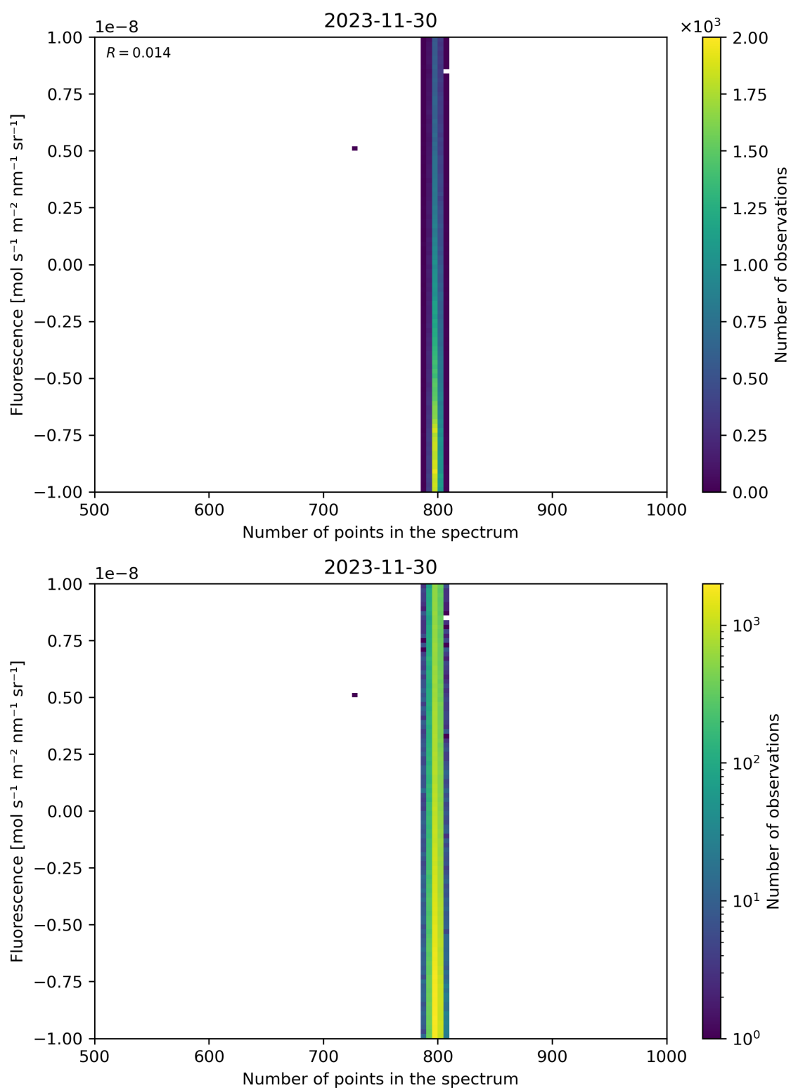
Figure 91: Scatter density plot of “Number of points in the spectrum” against “Fluorescence” for 2023-11-29 to 2023-12-01.
