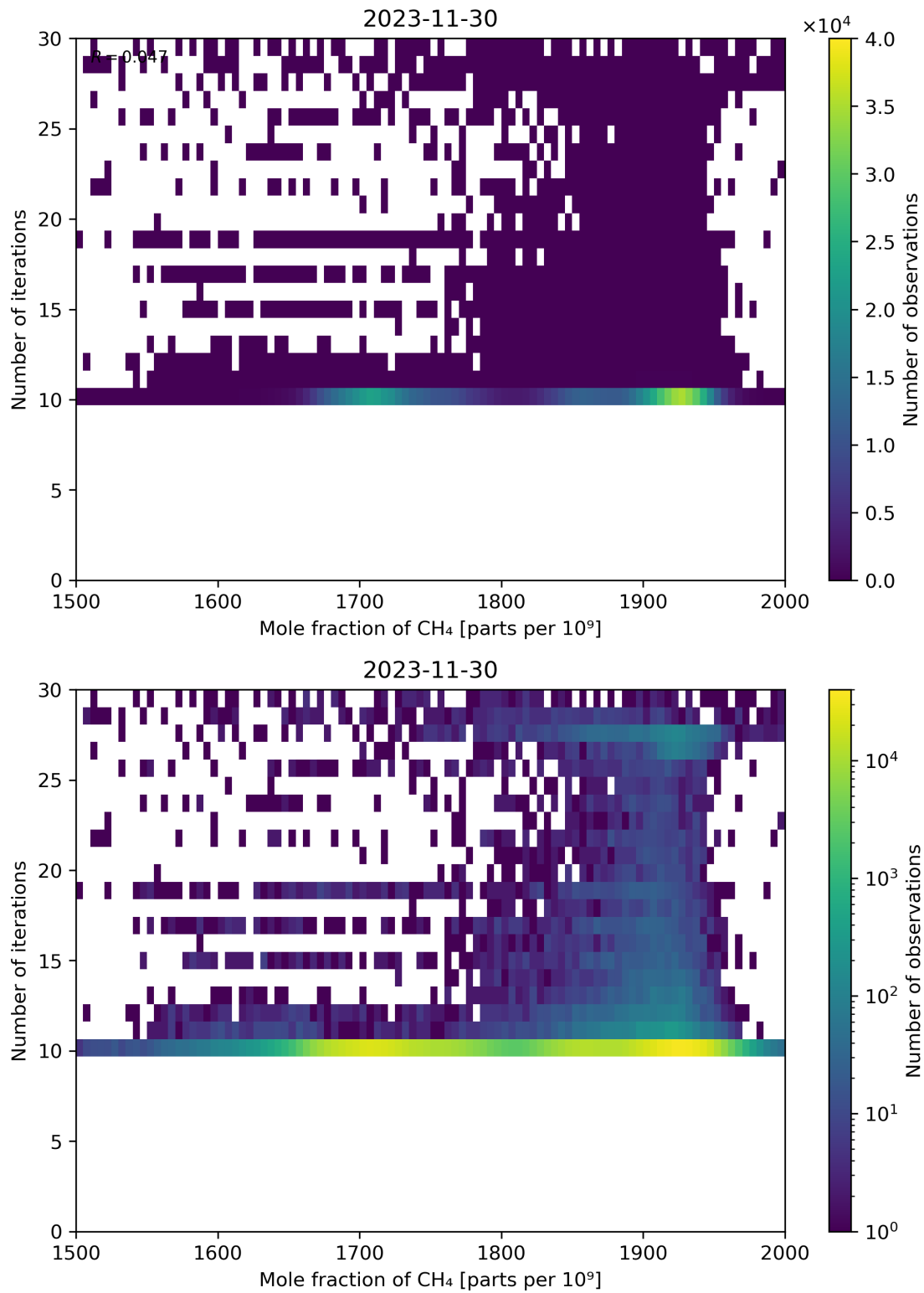
Figure 76: Scatter density plot of “Mole fraction of CH 4 ” against “Number of iterations” for 2023-11-29 to 2023-12-01.
