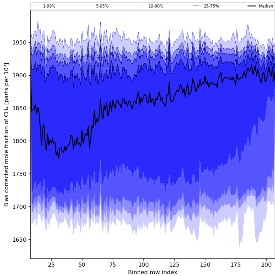
Figure 36: Along track statistics of “Bias corrected mole fraction of CH 4 ” for 2023-11-29 to 2023-12-01
