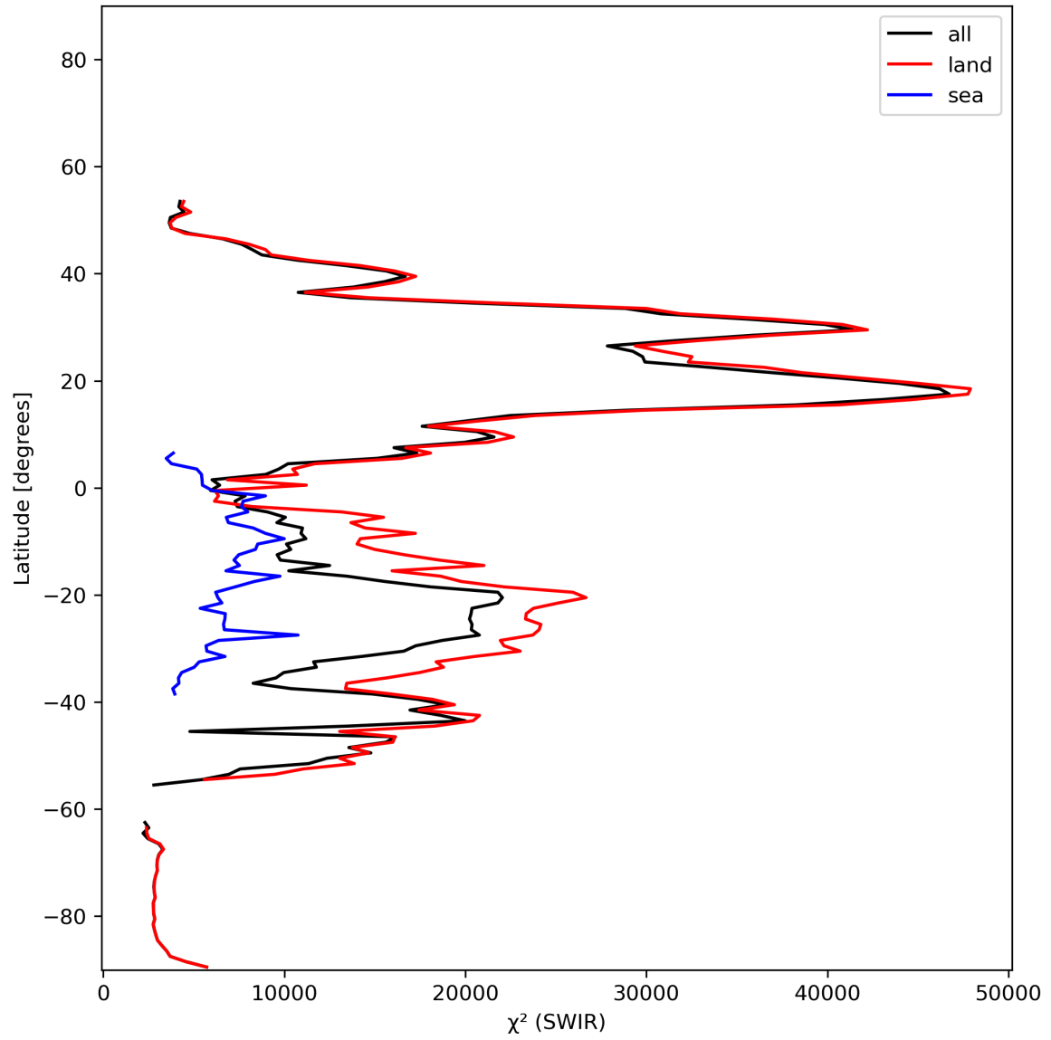
Figure 17: Zonal average of “ \chi^2 (SWIR)” for 2023-11-29 to 2023-12-01.
