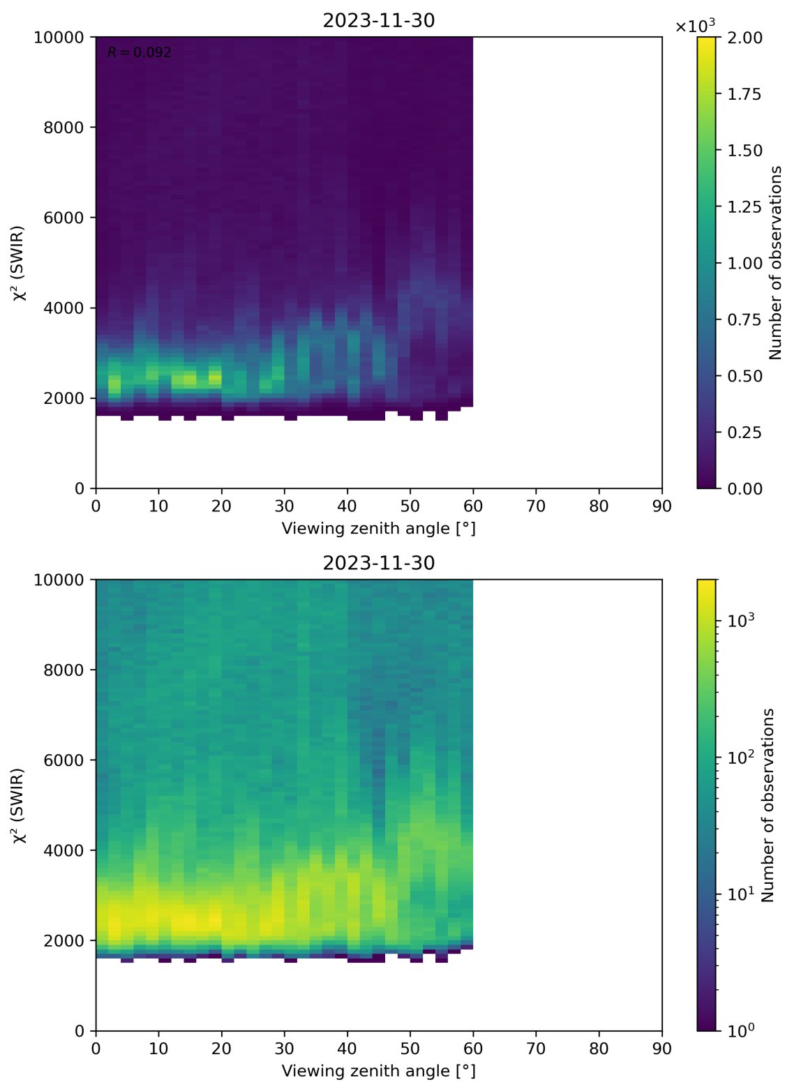
Figure 106: Scatter density plot of “Viewing zenith angle” against “ \chi^2 (SWIR)” for 2023-11-29 to 2023-12-01.
