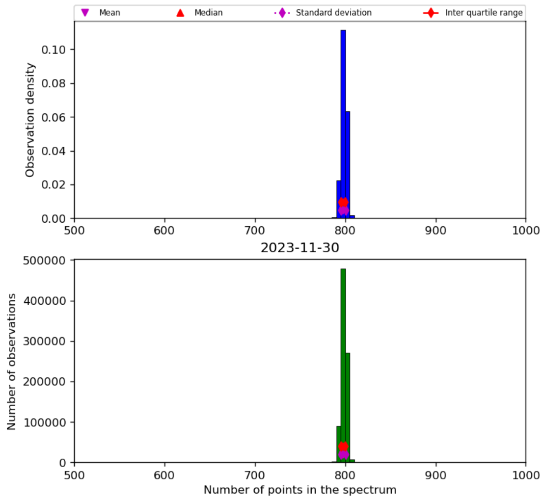
Figure 26: Histogram of “Number of points in the spectrum” for 2023-11-29 to 2023-12-01
