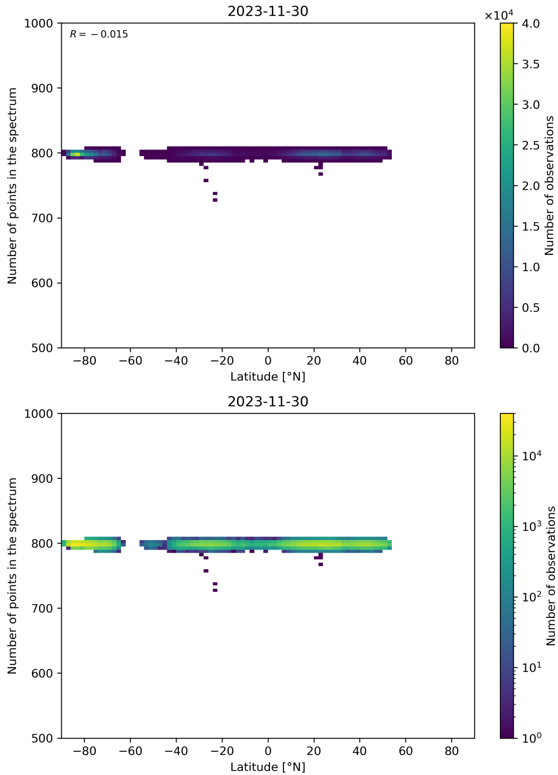
Figure 61: Scatter density plot of “Latitude” against “Number of points in the spectrum” for 2023-11-29 to 2023-12-01.
