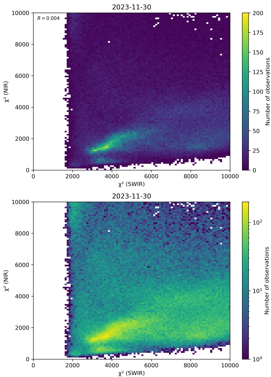
Figure 47: Scatter density plot of “ \chi^2 (SWIR)” against “ \chi^2 (NIR)” for 2023-11-29 to 2023-12-01.
