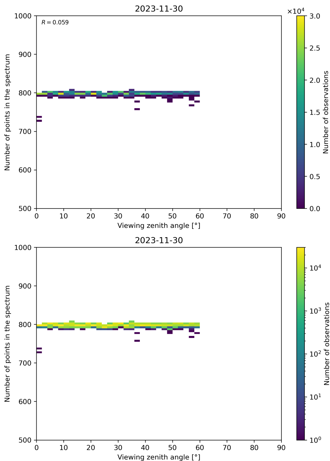
Figure 114: Scatter density plot of “Viewing zenith angle” against “Number of points in the spectrum” for 2023-11-29 to 2023-12-01.
