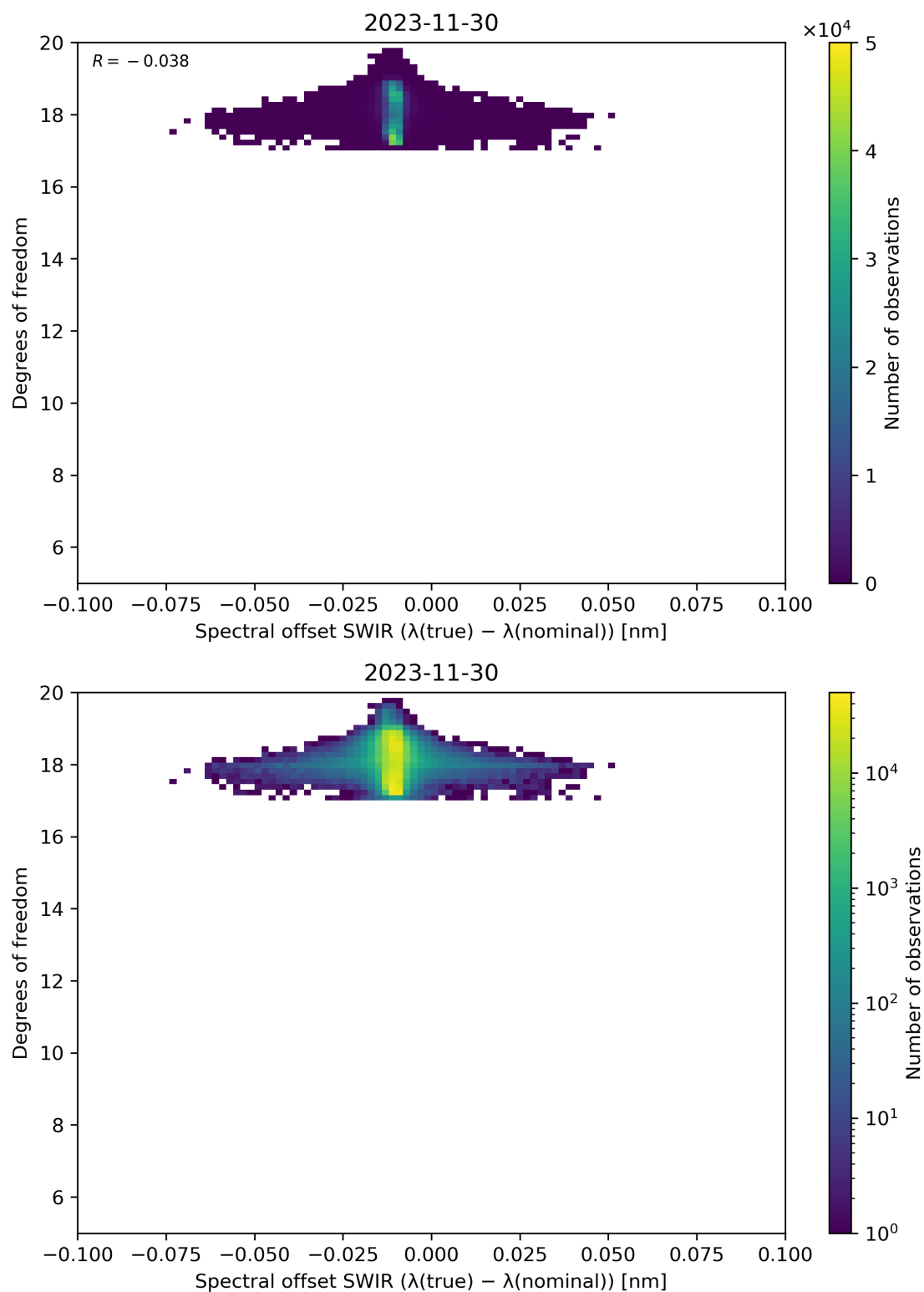
Figure 119: Scatter density plot of “Spectral offset SWIR ( \lambda(\text{true}) - \lambda(\text{nominal}) )” against “Degrees of freedom” for 2023-11-29 to 2023-12-01.
