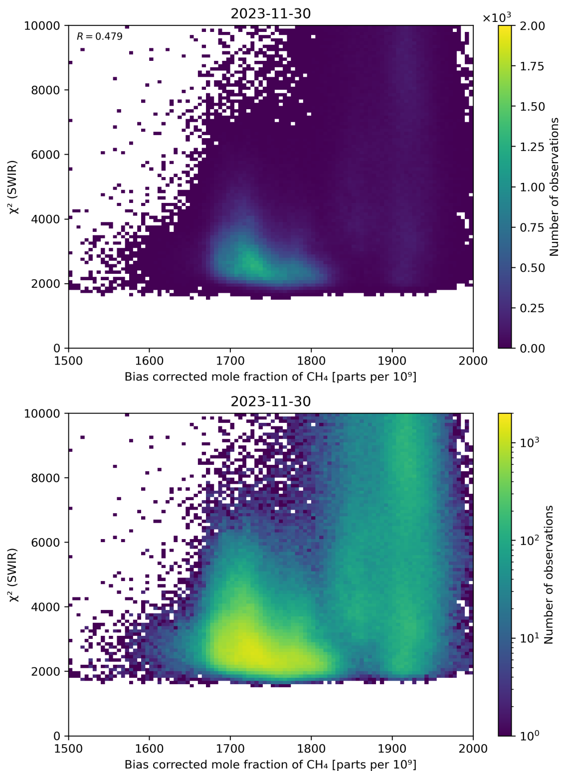
Figure 64: Scatter density plot of “Bias corrected mole fraction of \text{CH}_4 ” against “ \chi^2 (SWIR)” for 2023-11-29 to 2023-12-01.
