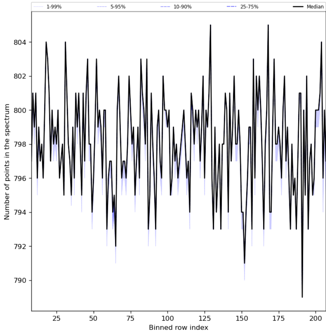
Figure 37: Along track statistics of “Number of points in the spectrum” for 2023-11-29 to 2023-12-01
