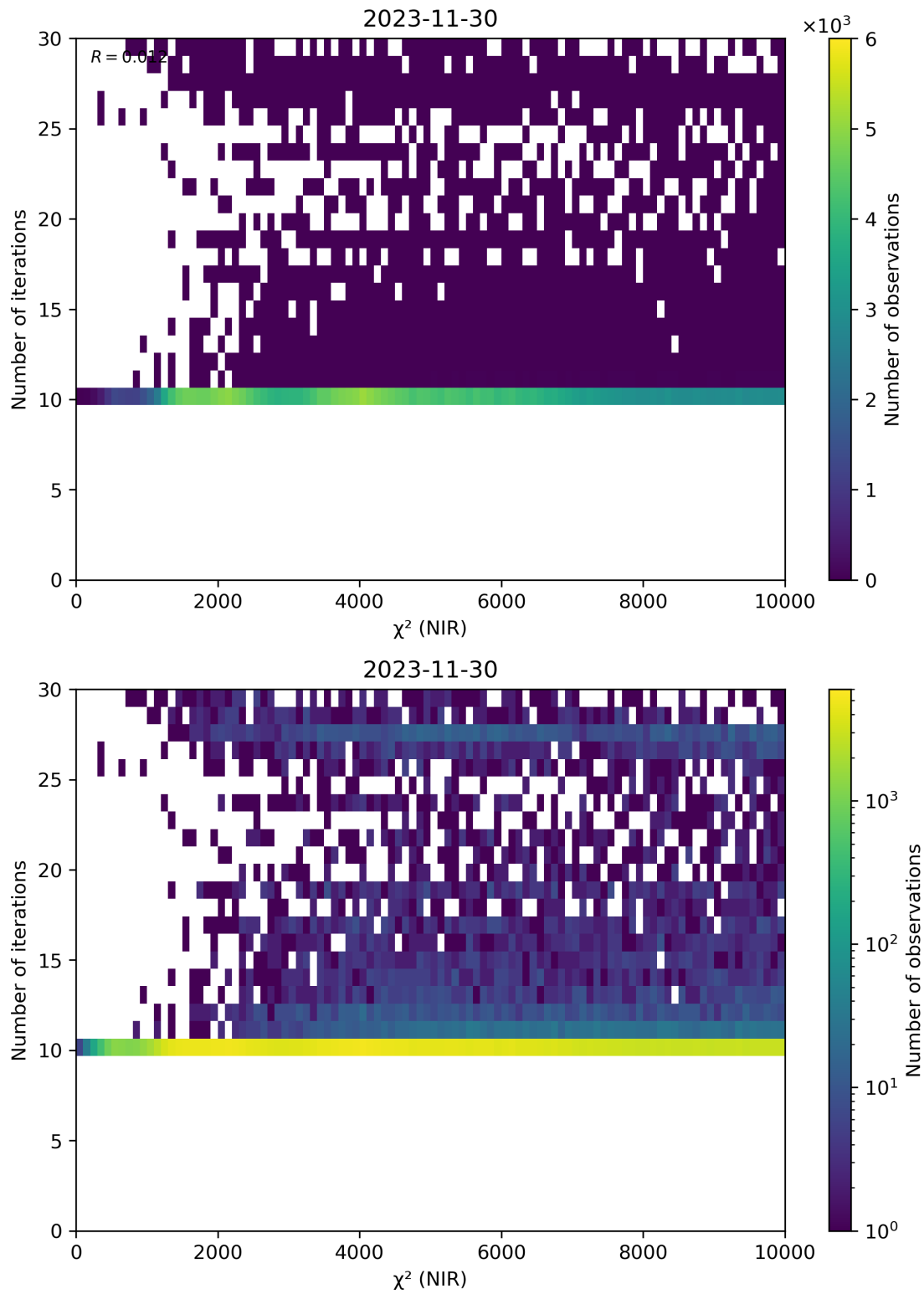
Figure 46: Scatter density plot of “ \chi^2 (NIR)” against “Number of iterations” for 2023-11-29 to 2023-12-01.
