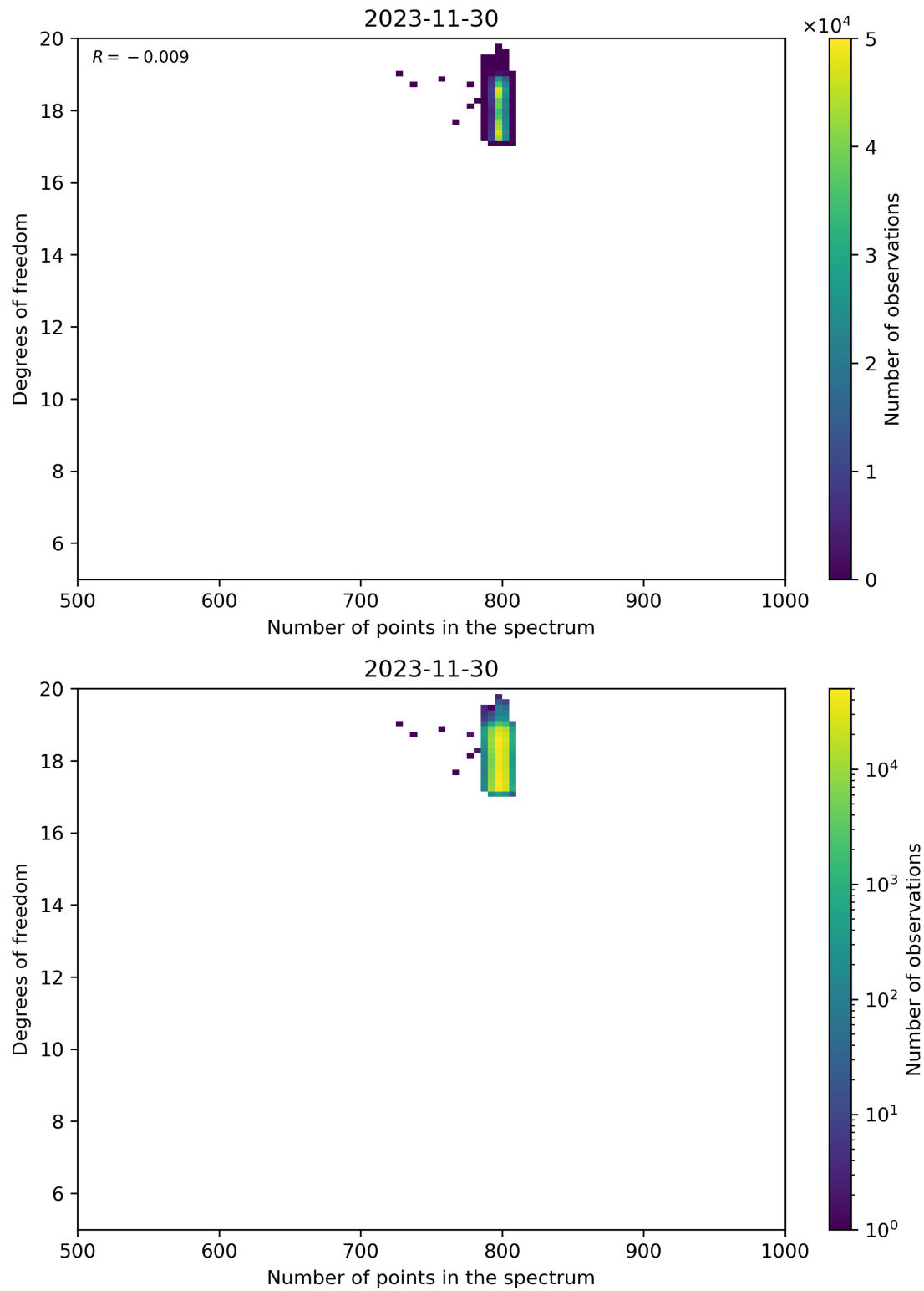
Figure 90: Scatter density plot of “Number of points in the spectrum” against “Degrees of freedom” for 2023-11-29 to 2023-12-01.
