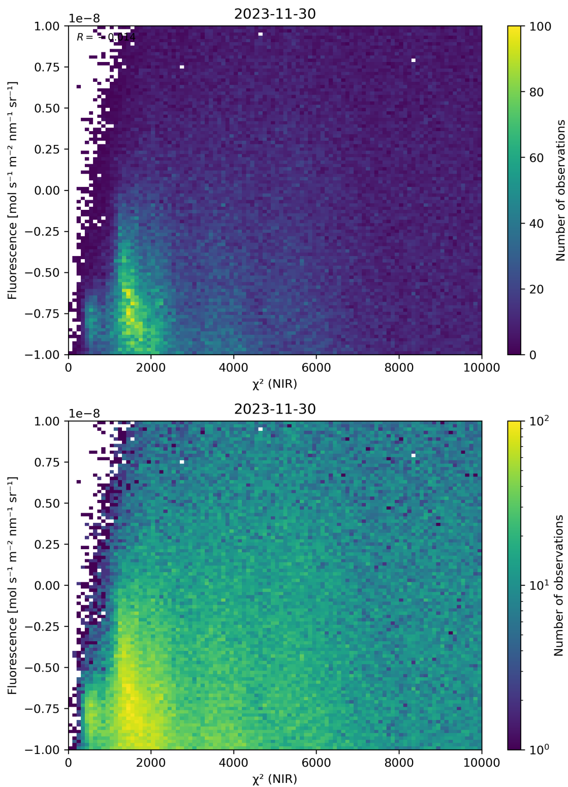
Figure 45: Scatter density plot of “ \chi^2 (NIR)” against “Fluorescence” for 2023-11-29 to 2023-12-01.
