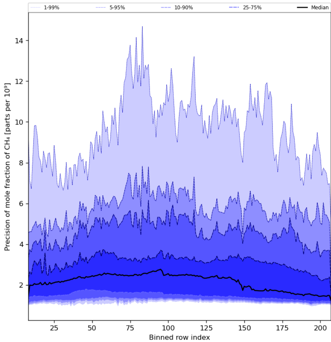
Figure 35: Along track statistics of “Precision of mole fraction of CH 4 ” for 2023-11-29 to 2023-12-01
