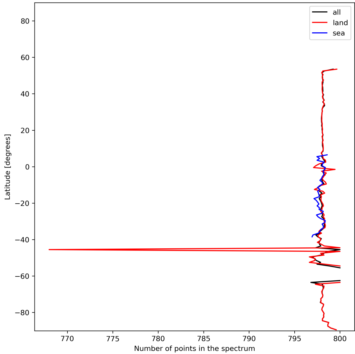
Figure 15: Zonal average of “Number of points in the spectrum” for 2023-11-29 to 2023-12-01.
