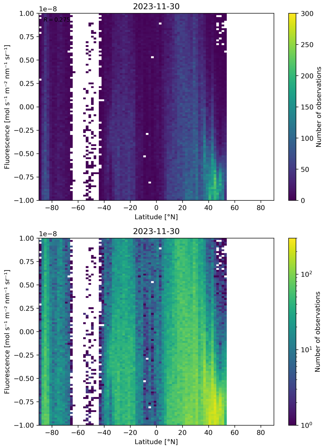
Figure 56: Scatter density plot of “Latitude” against “Fluorescence” for 2023-11-29 to 2023-12-01.
