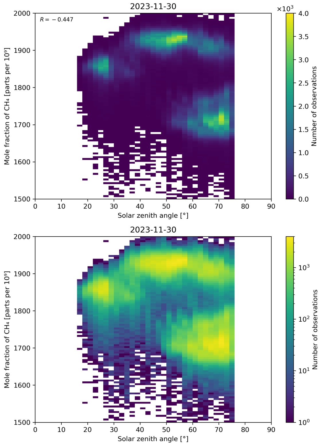
Figure 99: Scatter density plot of “Solar zenith angle” against “Mole fraction of CH 4 ” for 2023-11-29 to 2023-12-01.
