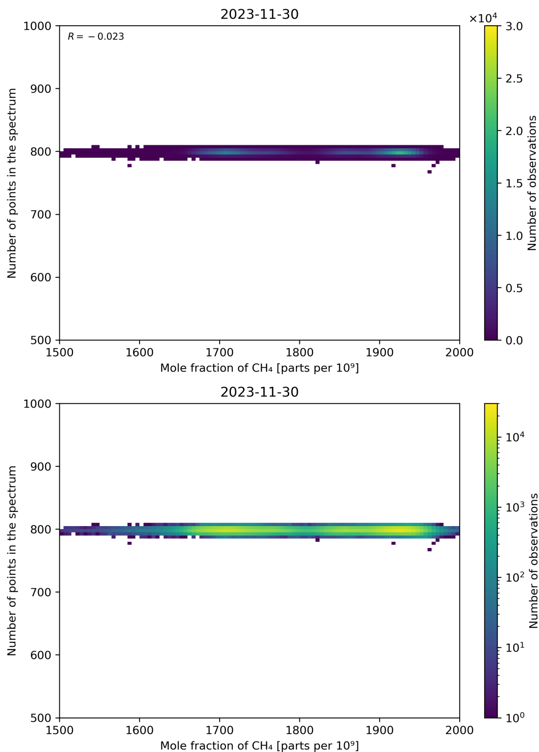
Figure 77: Scatter density plot of “Mole fraction of CH 4 ” against “Number of points in the spectrum” for 2023-11-29 to 2023-12-01.
