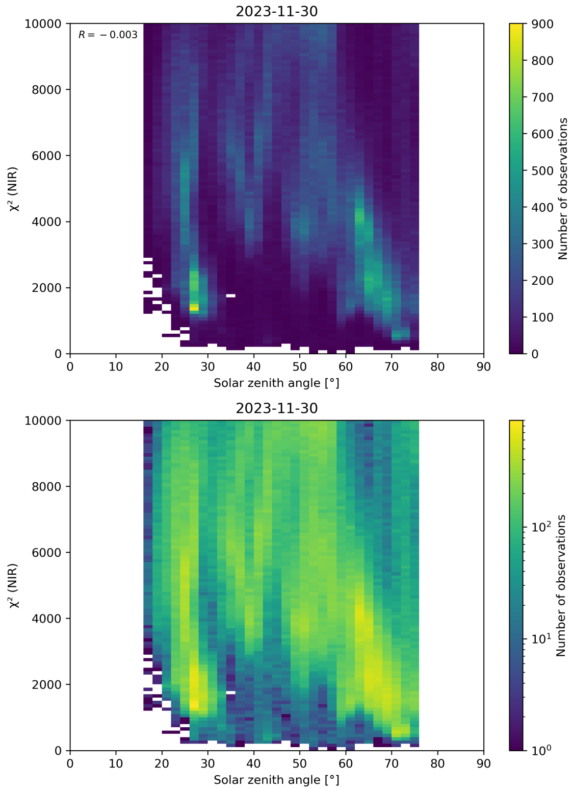
Figure 94: Scatter density plot of “Solar zenith angle” against “ \chi^2 (NIR)” for 2023-11-29 to 2023-12-01.
