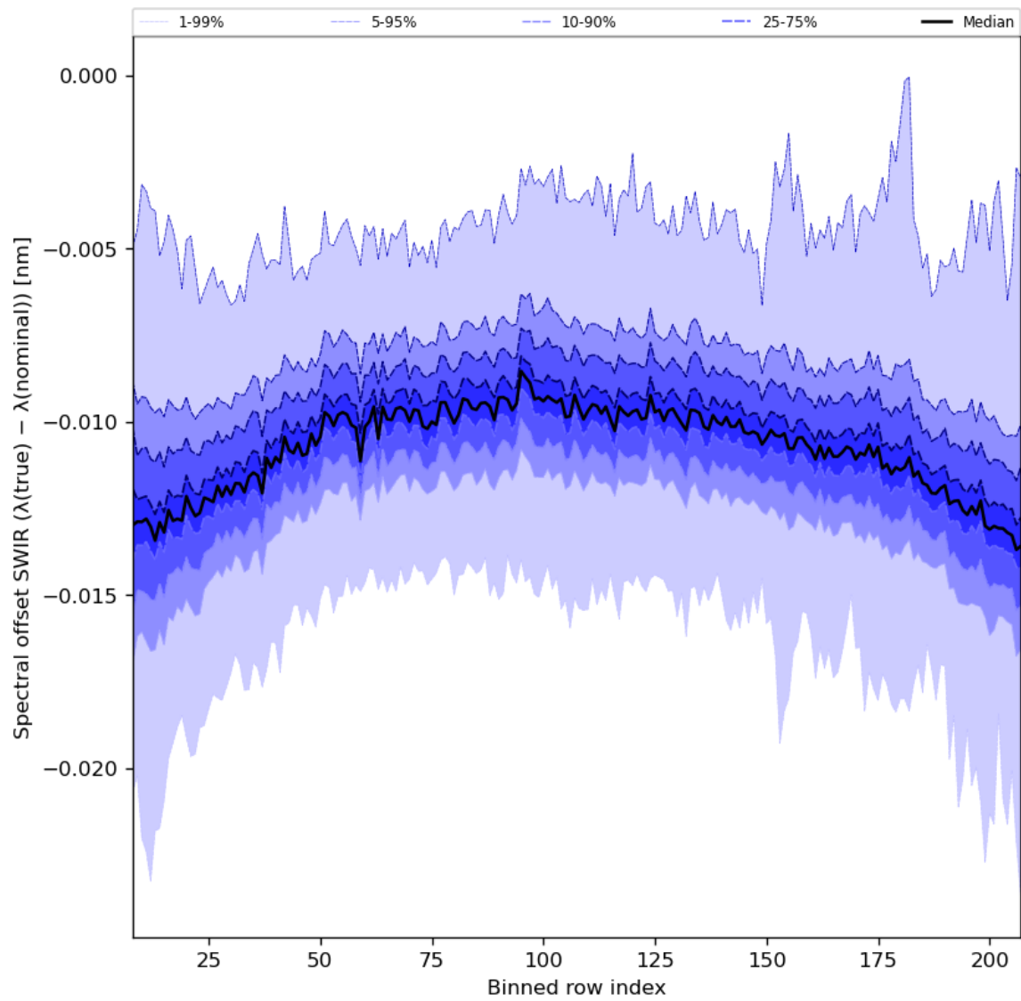
Figure 38: Along track statistics of “Spectral offset SWIR ( \lambda(\text{true}) - \lambda(\text{nominal}) )” for 2023-11-29 to 2023-12-01
