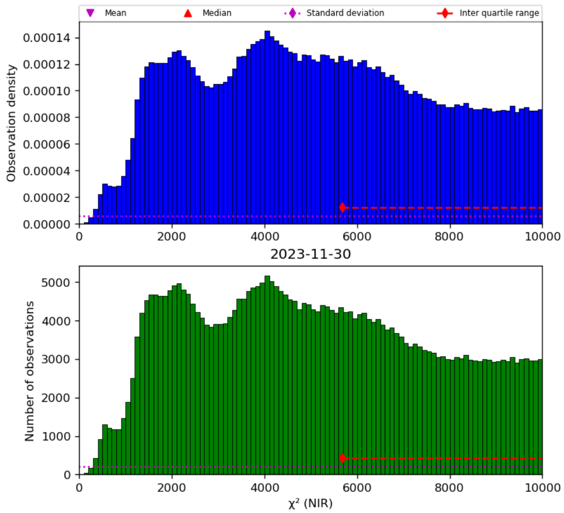
Figure 29: Histogram of “ \chi^2 (NIR)” for 2023-11-29 to 2023-12-01
