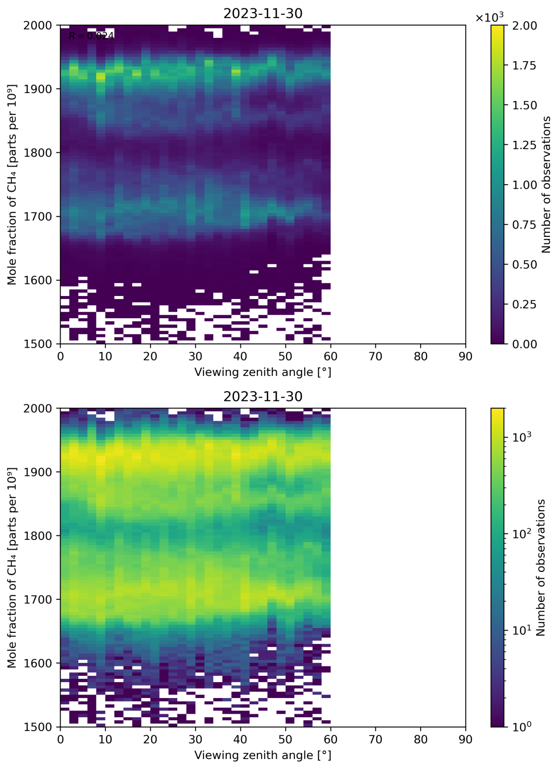
Figure 110: Scatter density plot of “Viewing zenith angle” against “Mole fraction of CH 4 ” for 2023-11-29 to 2023-12-01.
