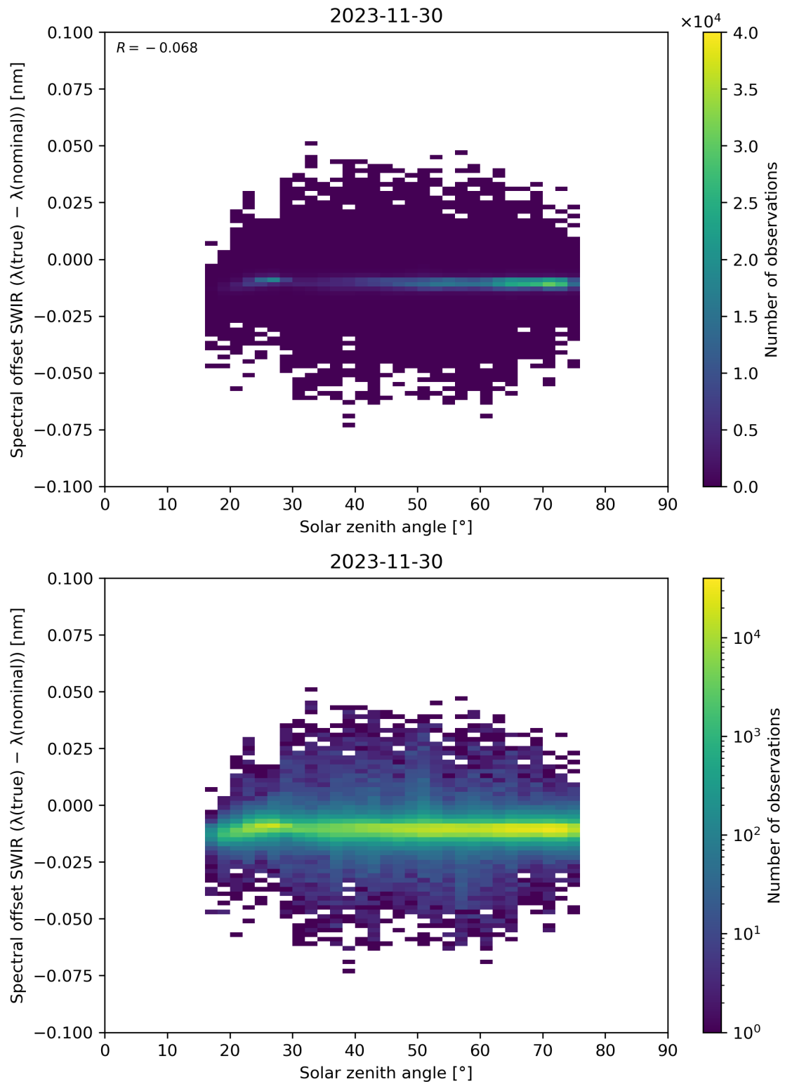
Figure 104: Scatter density plot of “Solar zenith angle” against “Spectral offset SWIR ( \lambda(\text{true}) - \lambda(\text{nominal}) )” for 2023-11-29 to 2023-12-01.
