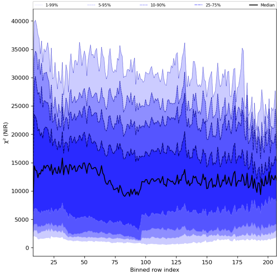
Figure 40: Along track statistics of “ \chi^2 (NIR)” for 2023-11-29 to 2023-12-01
