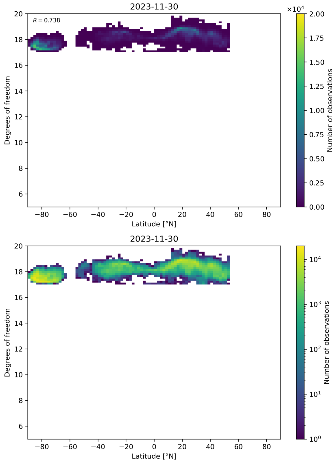
Figure 55: Scatter density plot of “Latitude” against “Degrees of freedom” for 2023-11-29 to 2023-12-01.
