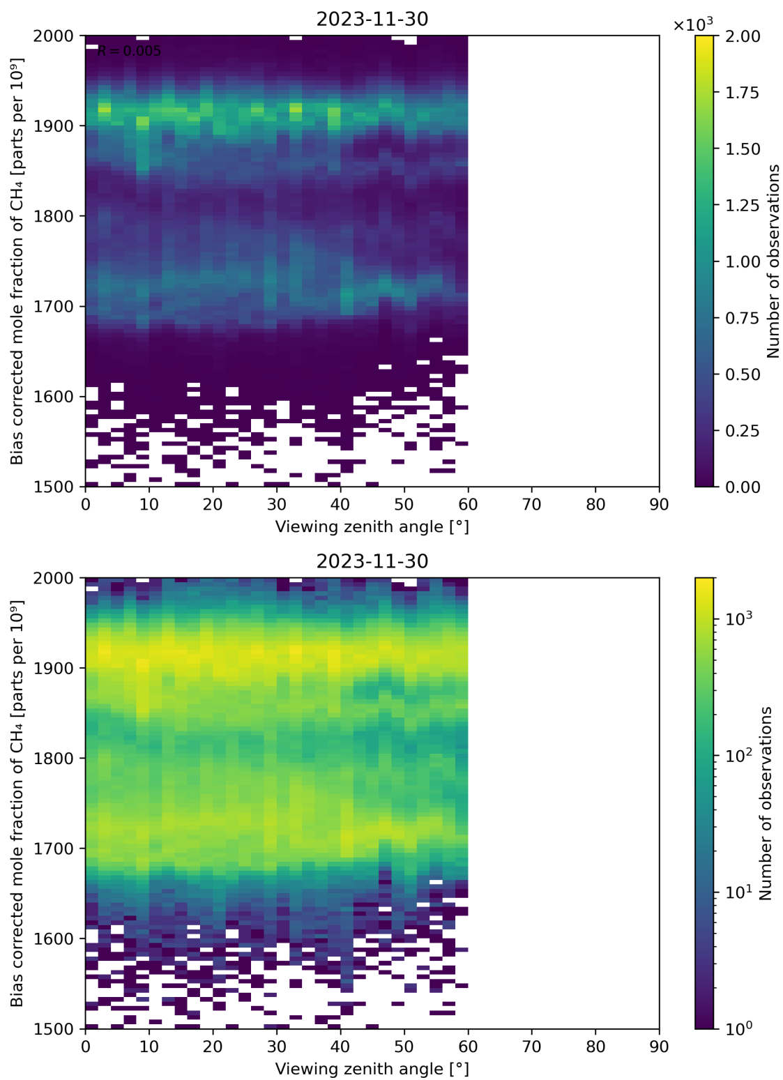
Figure 111: Scatter density plot of “Viewing zenith angle” against “Bias corrected mole fraction of CH 4 ” for 2023-11-29 to 2023-12-01.
