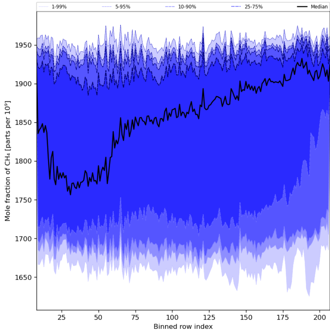
Figure 34: Along track statistics of “Mole fraction of CH 4 ” for 2023-11-29 to 2023-12-01
