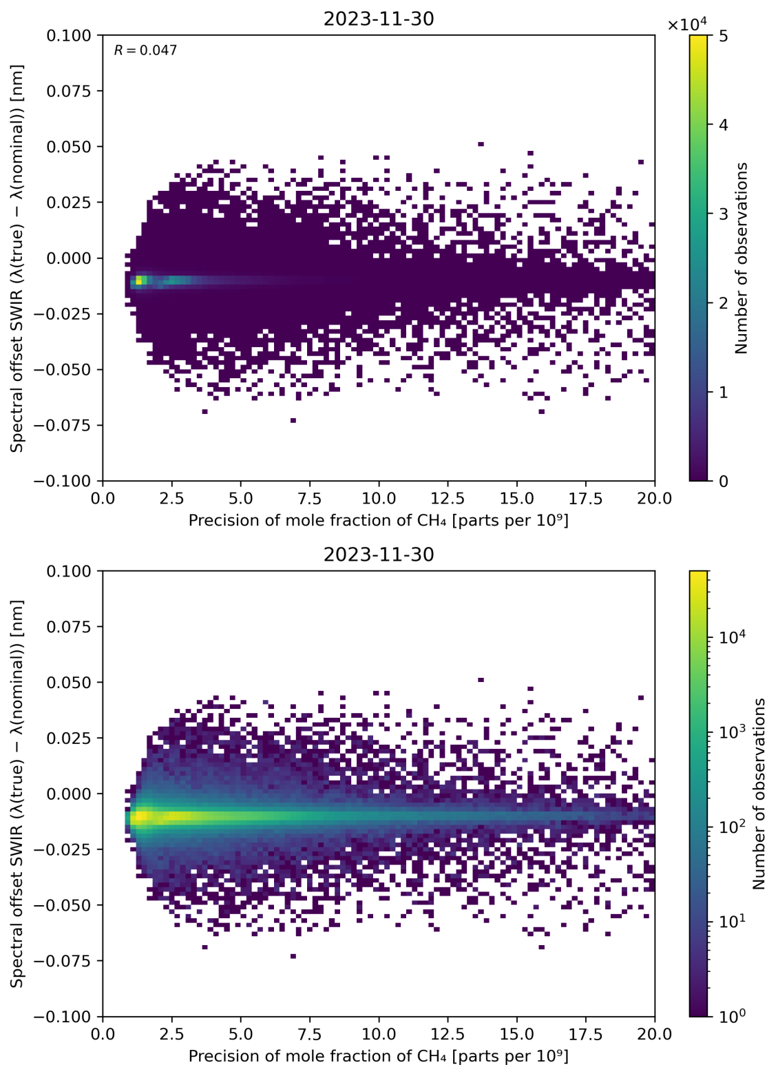
Figure 85: Scatter density plot of “Precision of mole fraction of CH 4 ” against “Spectral offset SWIR ( \lambda(\text{true}) - \lambda(\text{nominal}) )” for 2023-11-29 to 2023-12-01.
