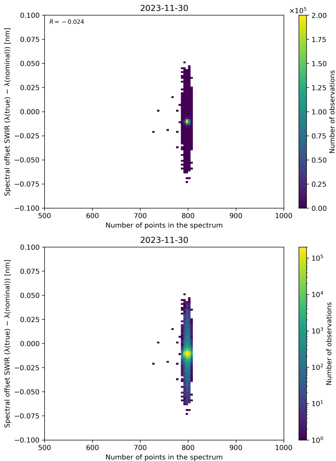
Figure 93: Scatter density plot of “Number of points in the spectrum” against “Spectral offset SWIR ( \lambda(\text{true}) - \lambda(\text{nominal}) )” for 2023-11-29 to 2023-12-01.
