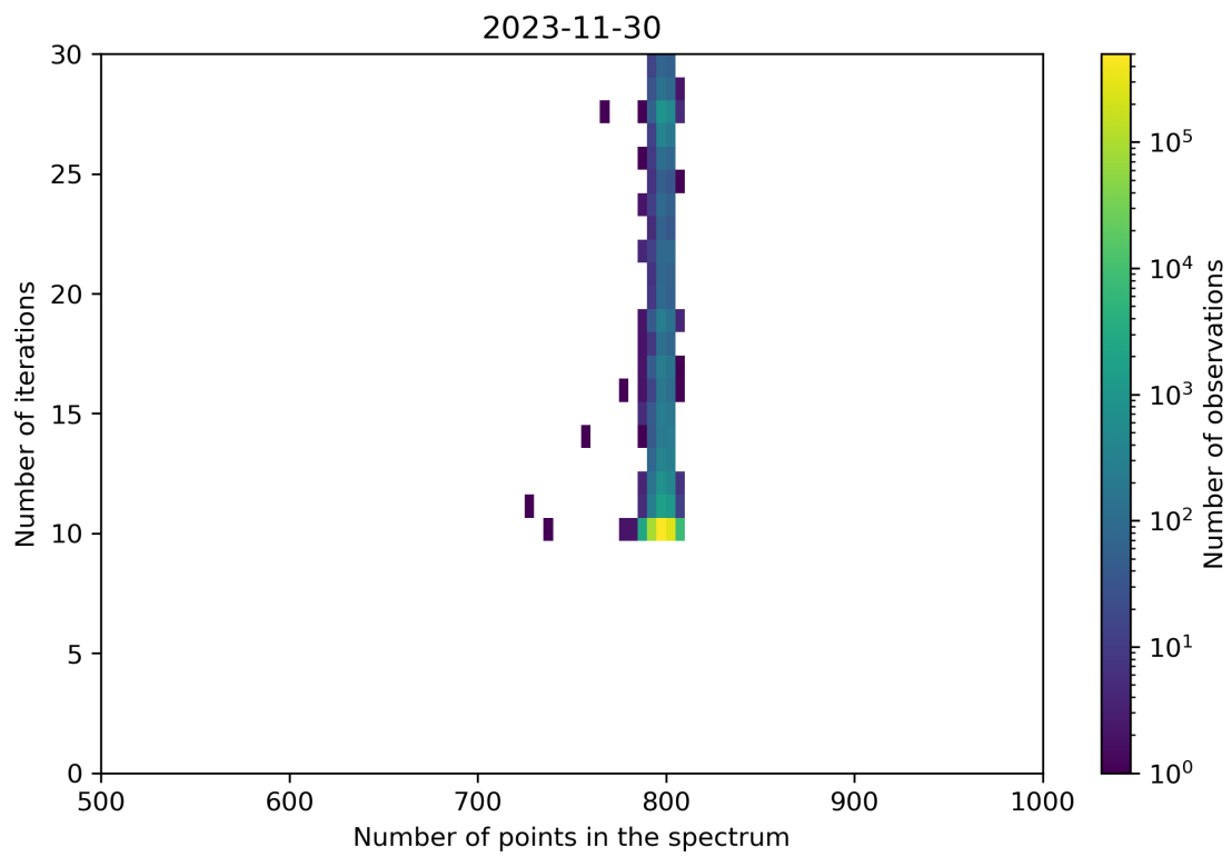
Figure 92: Scatter density plot of “Number of points in the spectrum” against “Number of iterations” for 2023-11-29 to 2023-12-01.
