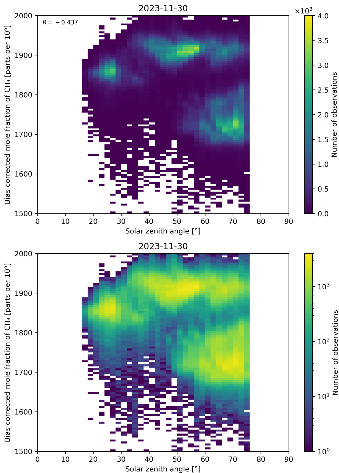
Figure 100: Scatter density plot of “Solar zenith angle” against “Bias corrected mole fraction of CH 4 ” for 2023-11-29 to 2023-12-01.
