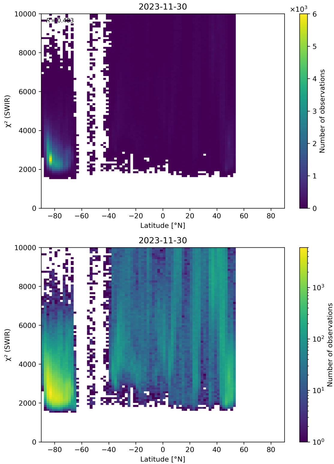
Figure 54: Scatter density plot of “Latitude” against “ \chi^2 (SWIR)” for 2023-11-29 to 2023-12-01.
