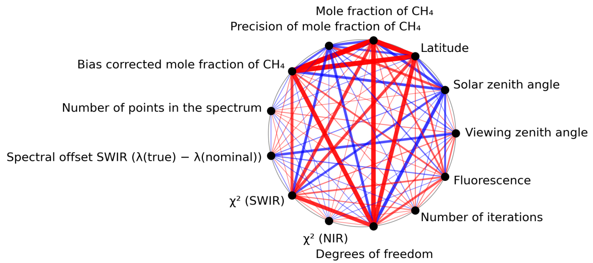
Figure 1: Map of correlation graph for 2023-11-29 to 2023-12-01.
