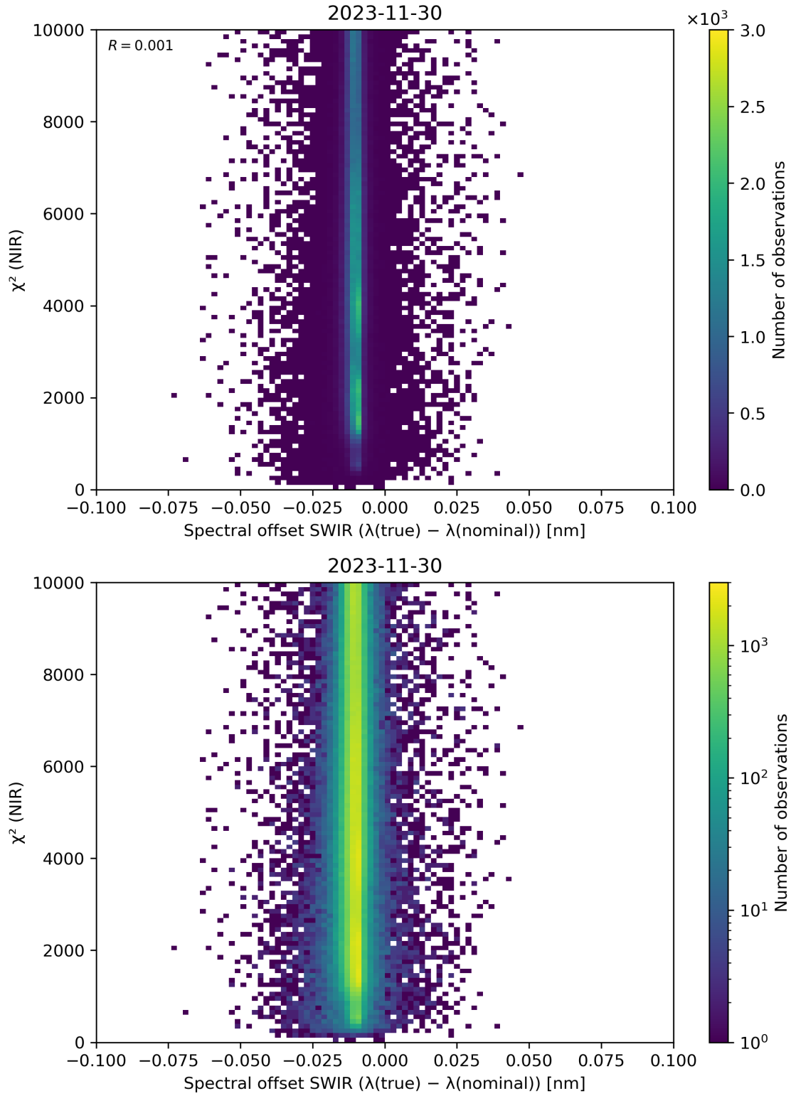
Figure 117: Scatter density plot of “Spectral offset SWIR ( \lambda(\text{true}) - \lambda(\text{nominal}) )” against “ \chi^2 (NIR)” for 2023-11-29 to 2023-12-01.
