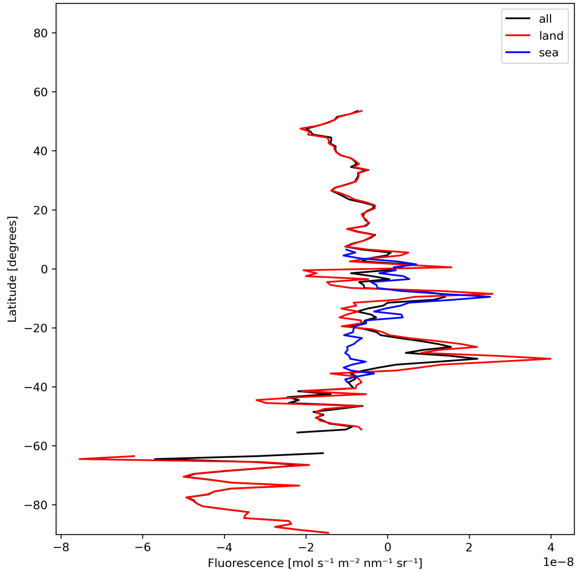
Figure 21: Zonal average of “Fluorescence” for 2023-11-29 to 2023-12-01.
