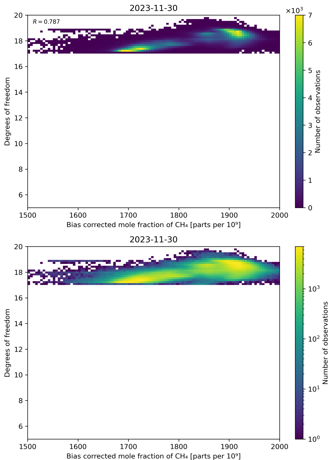
Figure 65: Scatter density plot of “Bias corrected mole fraction of CH 4 ” against “Degrees of freedom” for 2023-11-29 to 2023-12-01.
