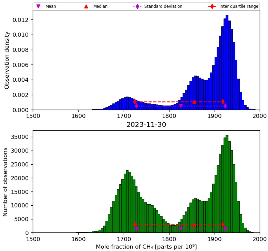
Figure 23: Histogram of “Mole fraction of CH 4 ” for 2023-11-29 to 2023-12-01
