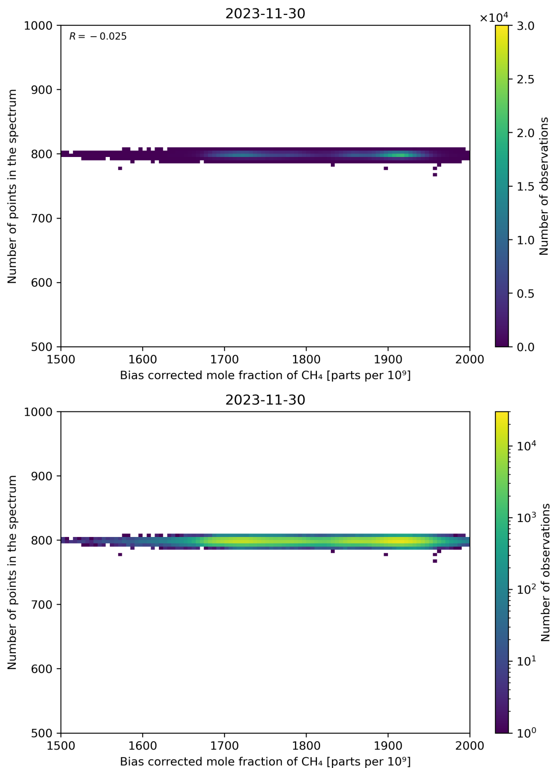
Figure 68: Scatter density plot of “Bias corrected mole fraction of CH 4 ” against “Number of points in the spectrum” for 2023-11-29 to 2023-12-01.
