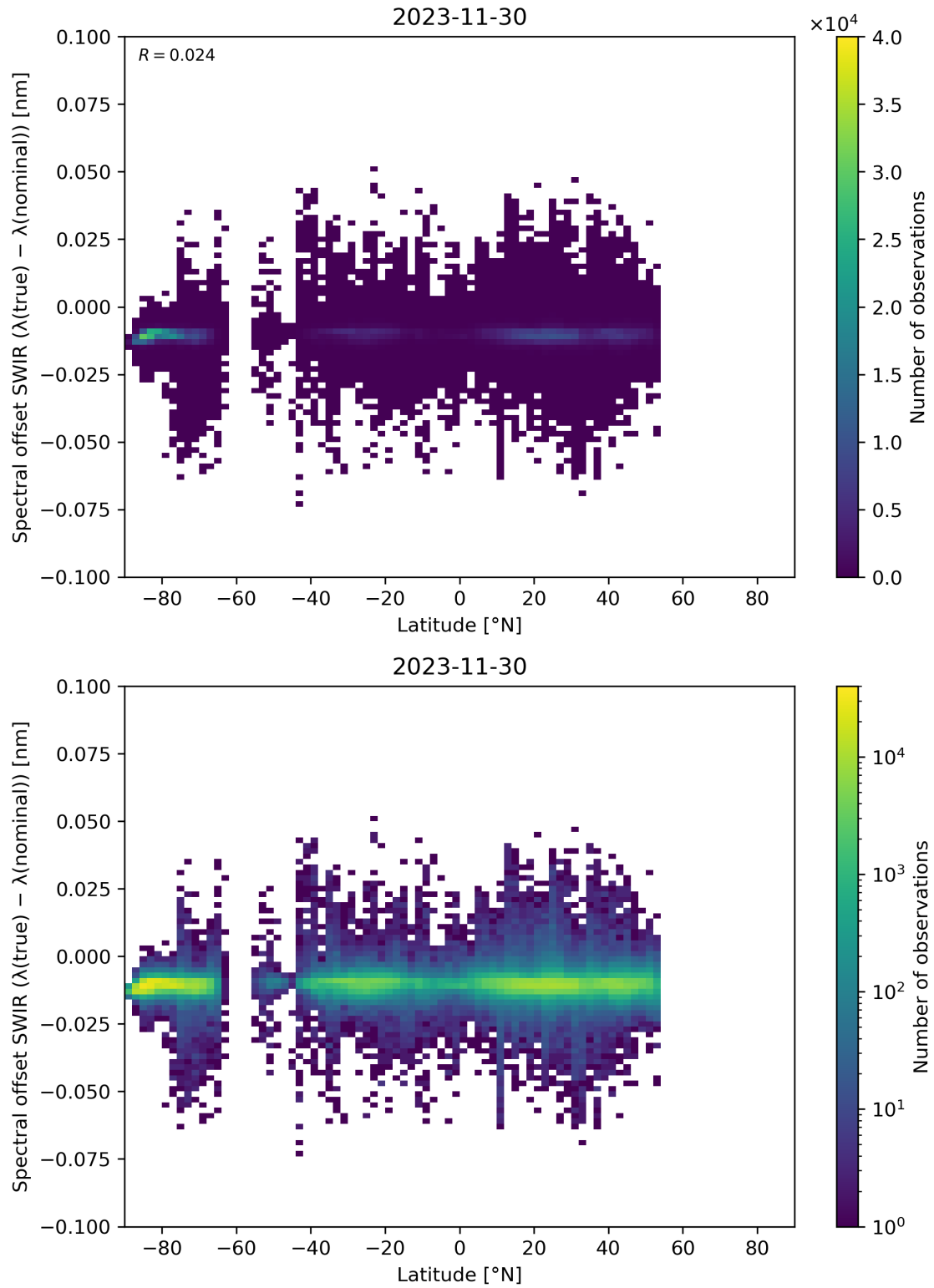
Figure 62: Scatter density plot of “Latitude” against “Spectral offset SWIR ( \lambda(\text{true}) - \lambda(\text{nominal}) )” for 2023-11-29 to 2023-12-01.
