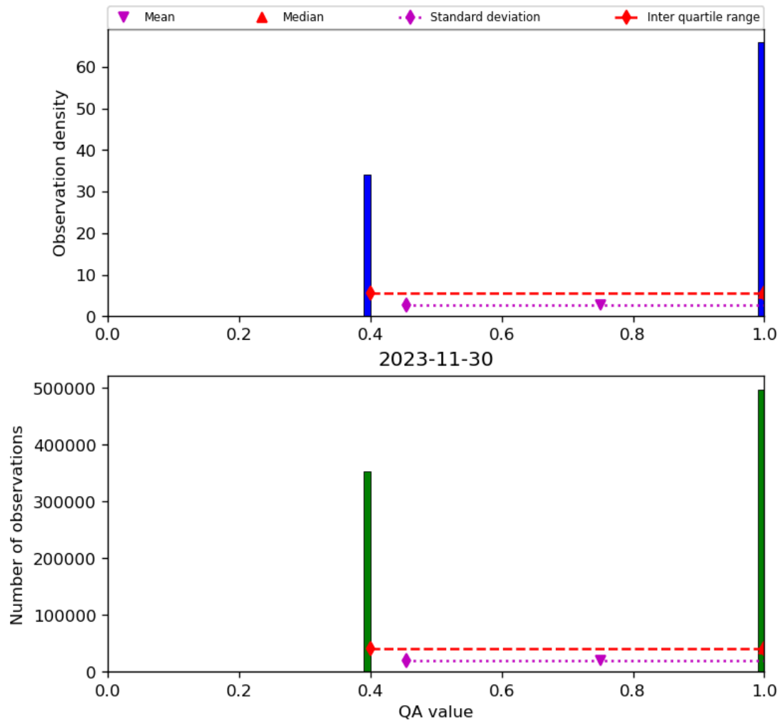
Figure 22: Histogram of “QA value” for 2023-11-29 to 2023-12-01
