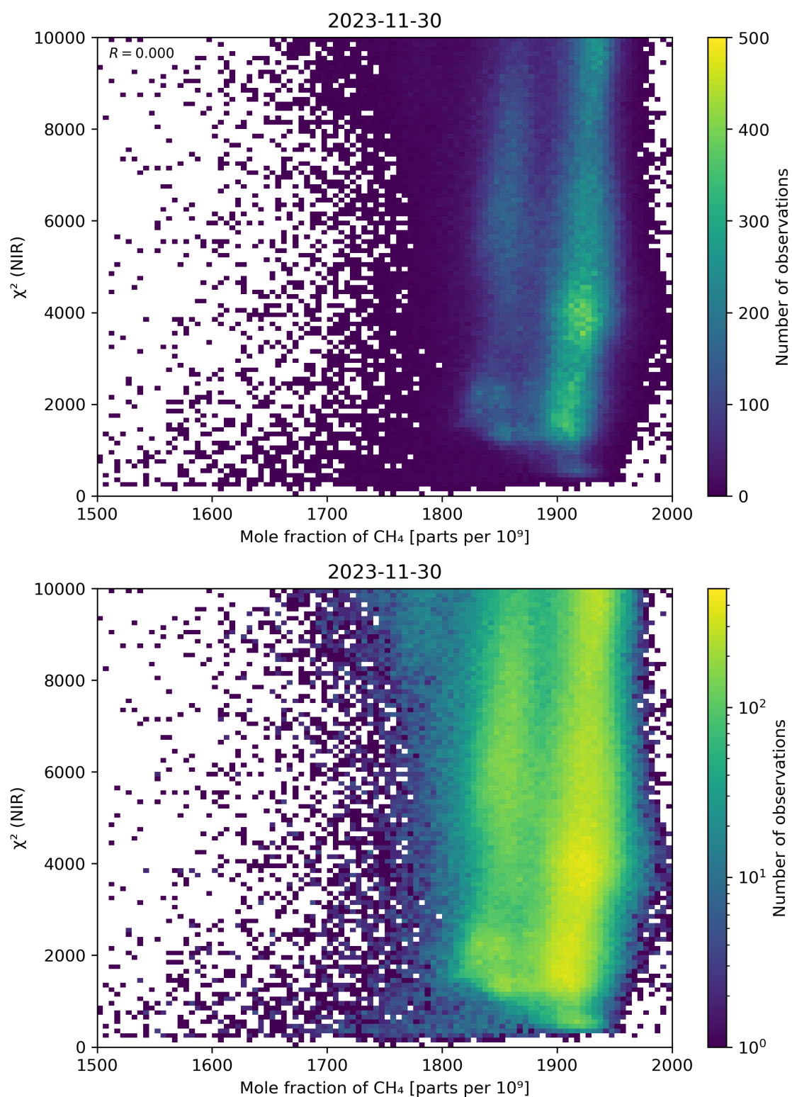
Figure 70: Scatter density plot of “Mole fraction of CH 4 ” against “ \chi^2 (NIR)” for 2023-11-29 to 2023-12-01.
