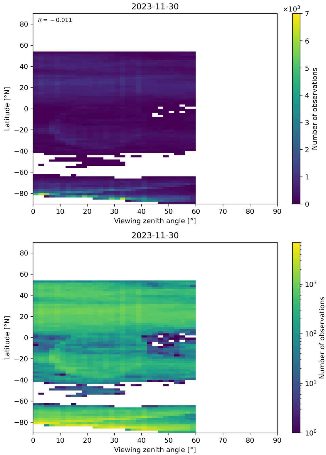
Figure 109: Scatter density plot of “Viewing zenith angle” against “Latitude” for 2023-11-29 to 2023-12-01.
