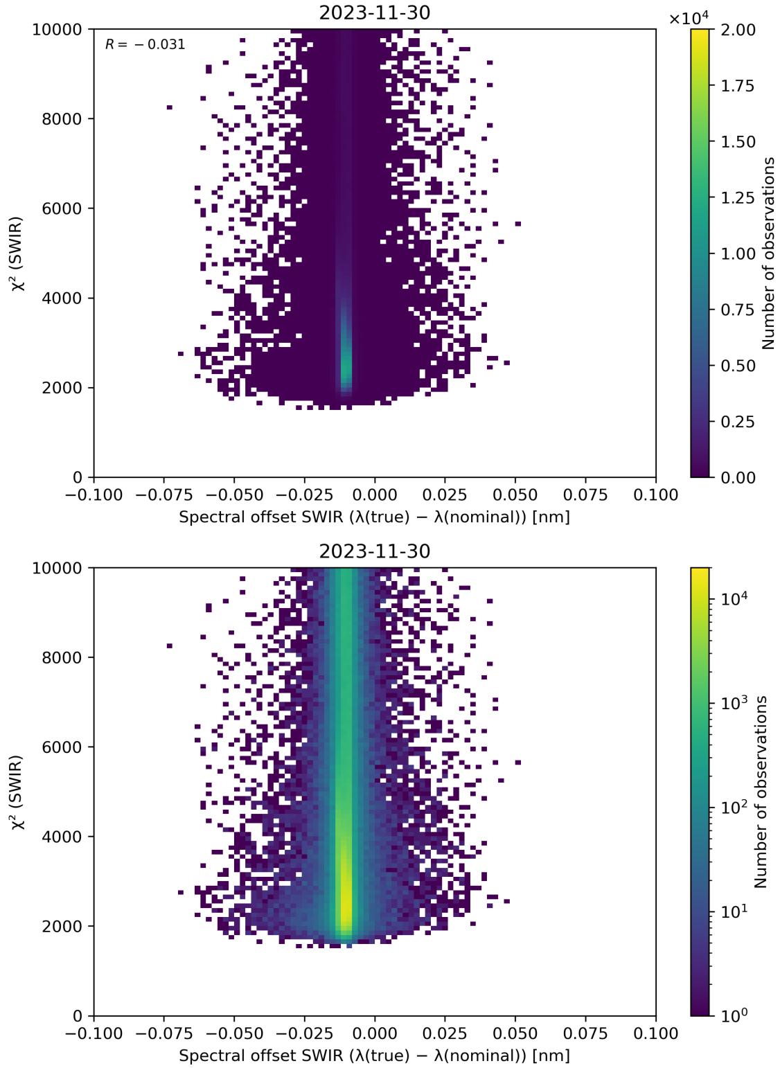
Figure 118: Scatter density plot of “Spectral offset SWIR ( \lambda(\text{true}) - \lambda(\text{nominal}) )” against “ \chi^2 (SWIR)” for 2023-11-29 to 2023-12-01.
