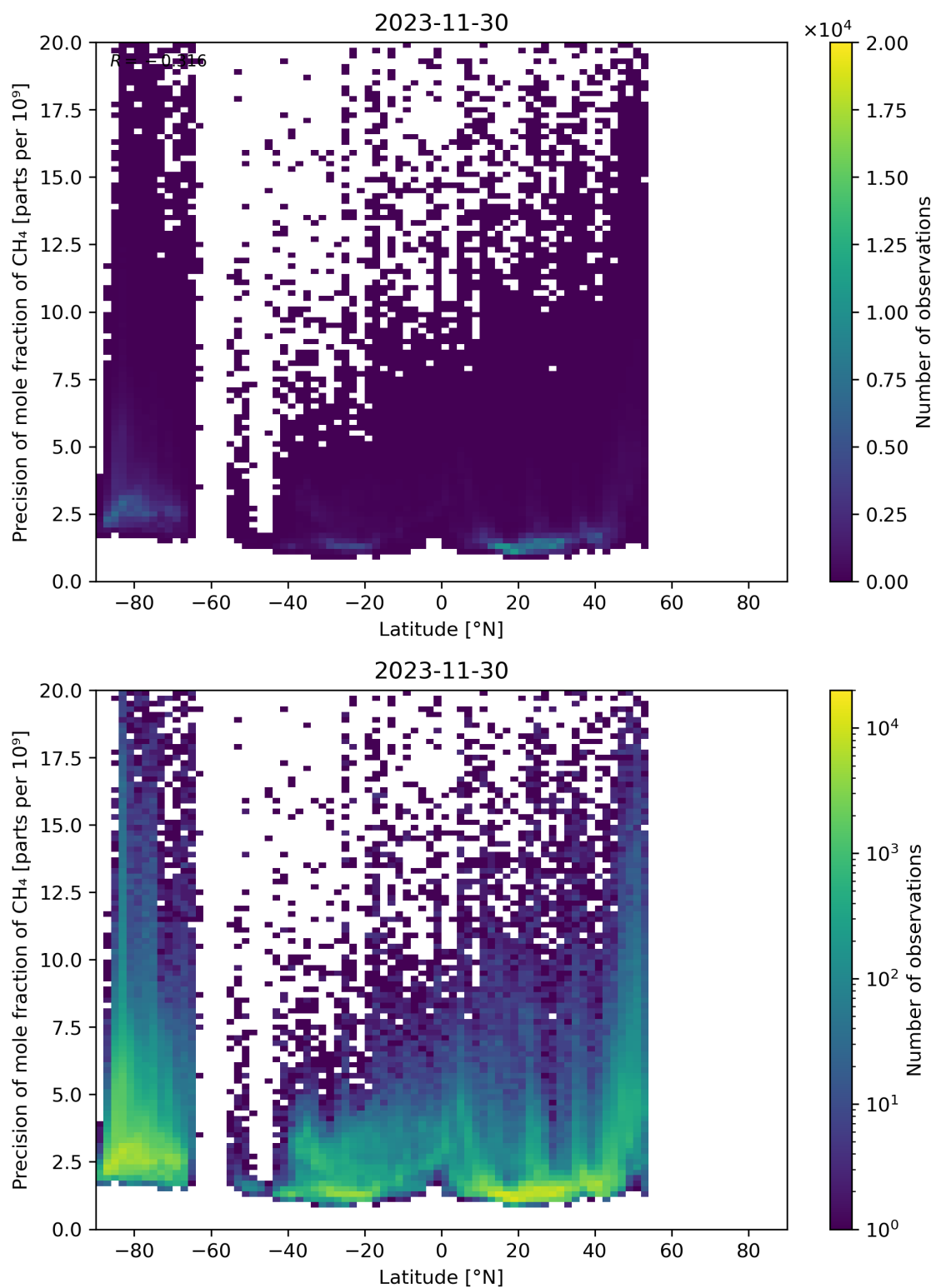
Figure 59: Scatter density plot of “Latitude” against “Precision of mole fraction of CH 4 ” for 2023-11-29 to 2023-12-01.
