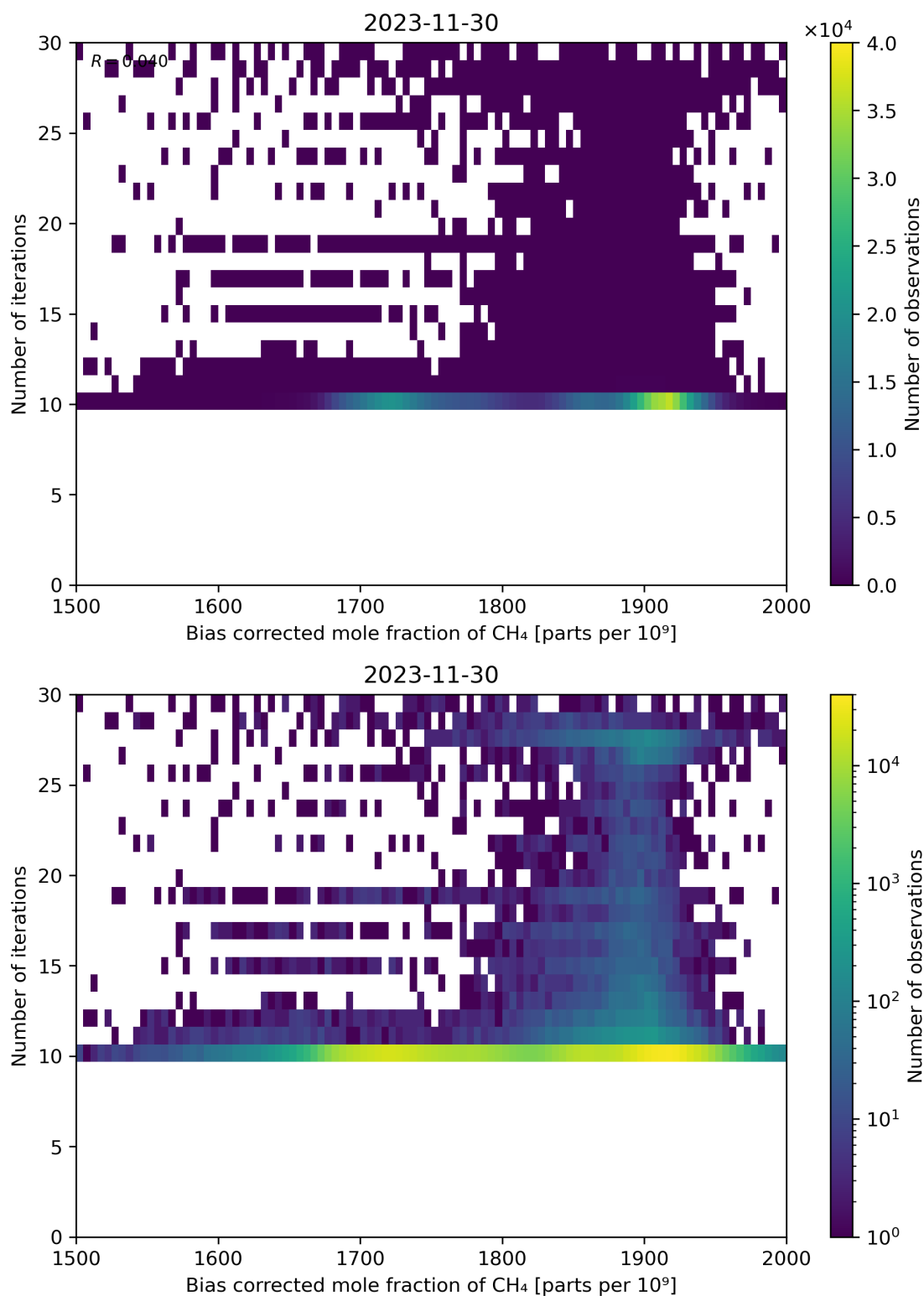
Figure 67: Scatter density plot of “Bias corrected mole fraction of CH 4 ” against “Number of iterations” for 2023-11-29 to 2023-12-01.
