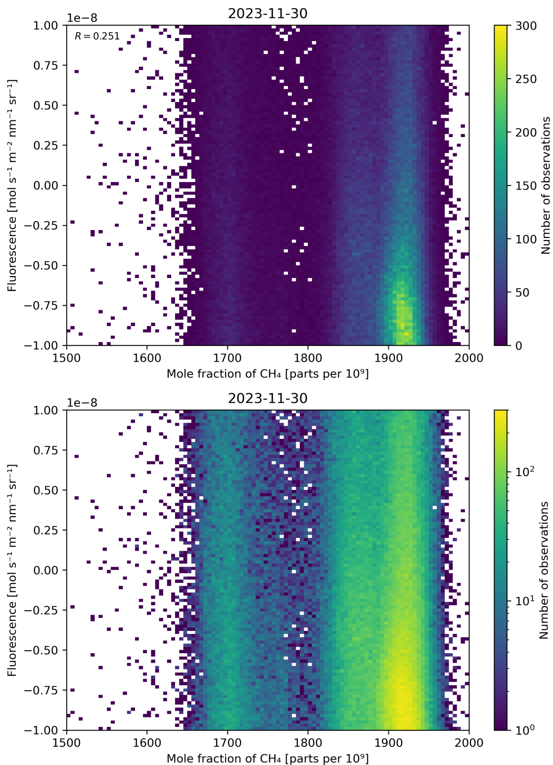
Figure 73: Scatter density plot of “Mole fraction of \text{CH}_4 ” against “Fluorescence” for 2023-11-29 to 2023-12-01.
