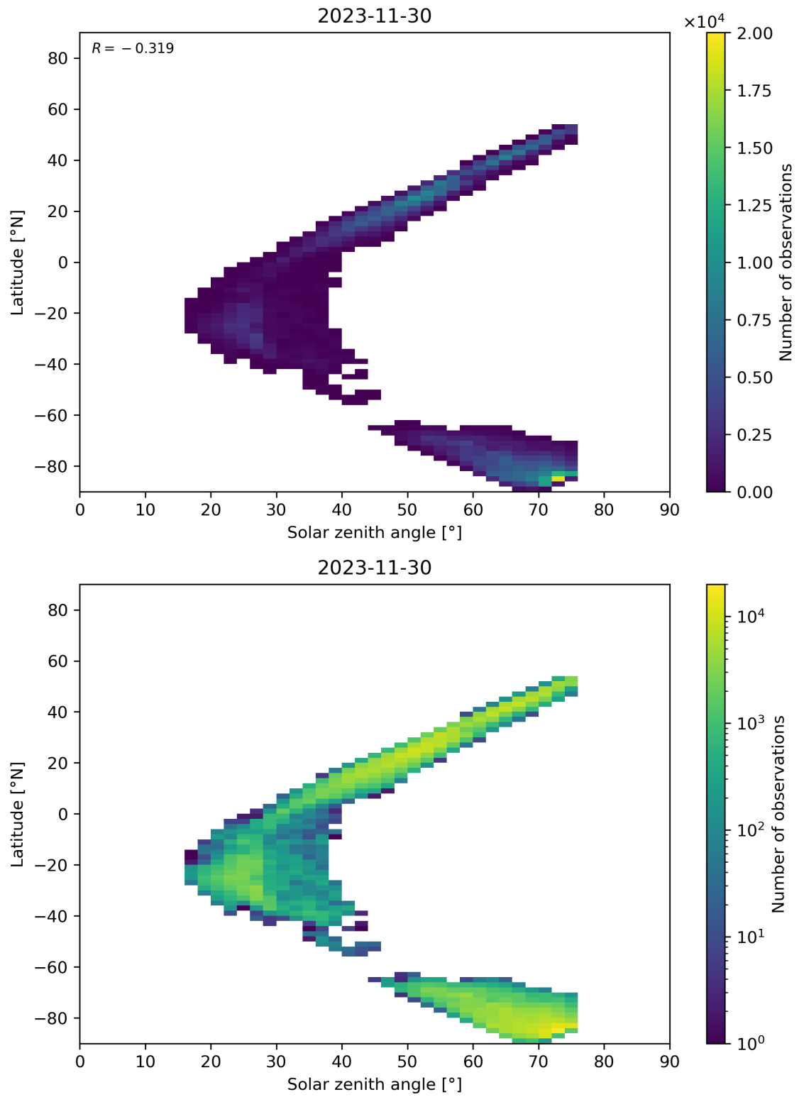
Figure 98: Scatter density plot of “Solar zenith angle” against “Latitude” for 2023-11-29 to 2023-12-01.
