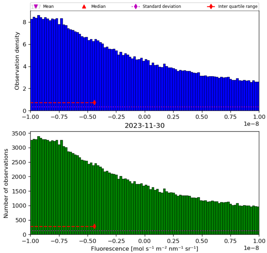
Figure 32: Histogram of “Fluorescence” for 2023-11-29 to 2023-12-01
