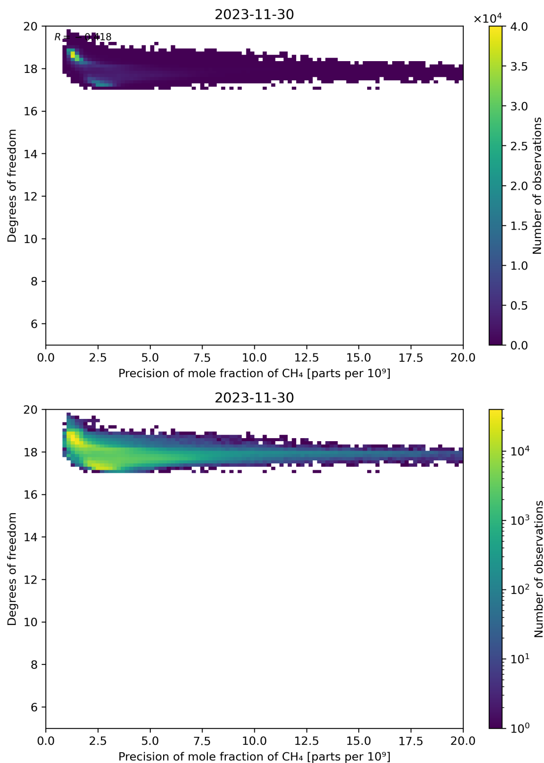
Figure 80: Scatter density plot of “Precision of mole fraction of CH 4 ” against “Degrees of freedom” for 2023-11-29 to 2023-12-01.
