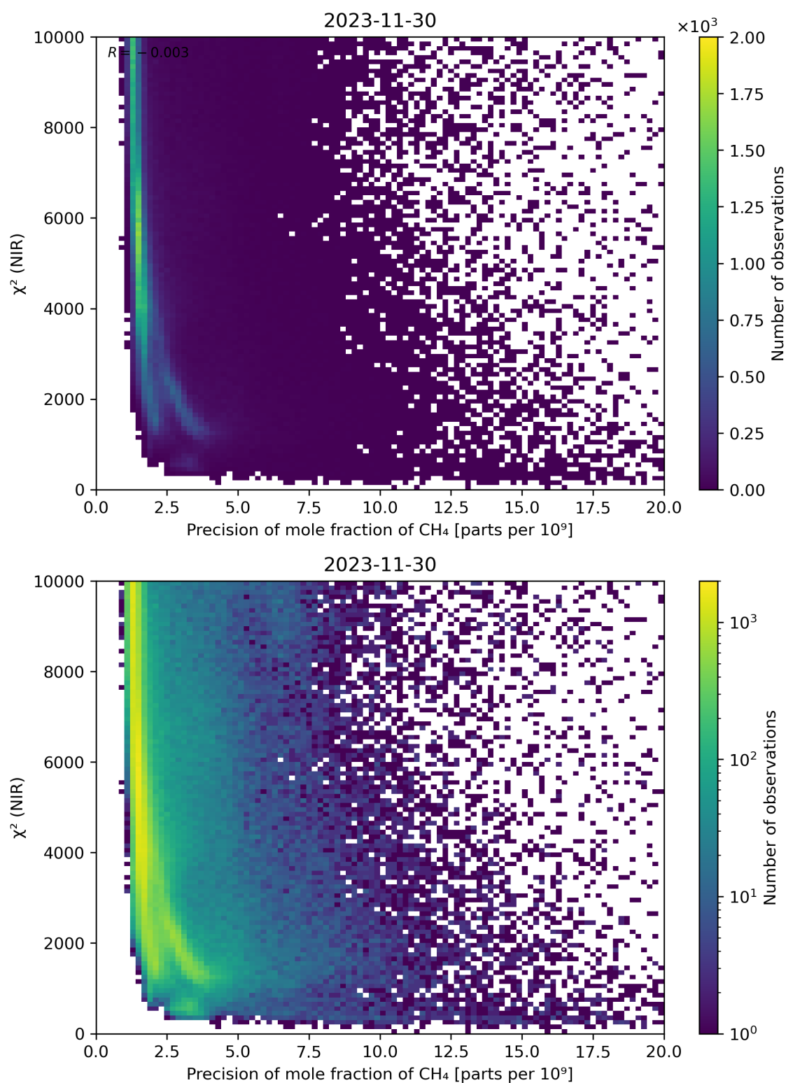
Figure 78: Scatter density plot of “Precision of mole fraction of CH 4 ” against “ \chi^2 (NIR)” for 2023-11-29 to 2023-12-01.
