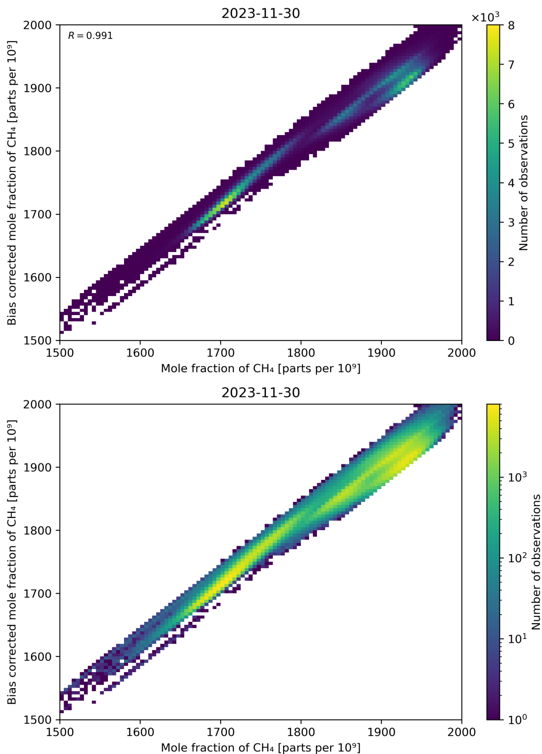
Figure 74: Scatter density plot of “Mole fraction of CH 4 ” against “Bias corrected mole fraction of CH 4 ” for 2023-11-29 to 2023-12-01.
