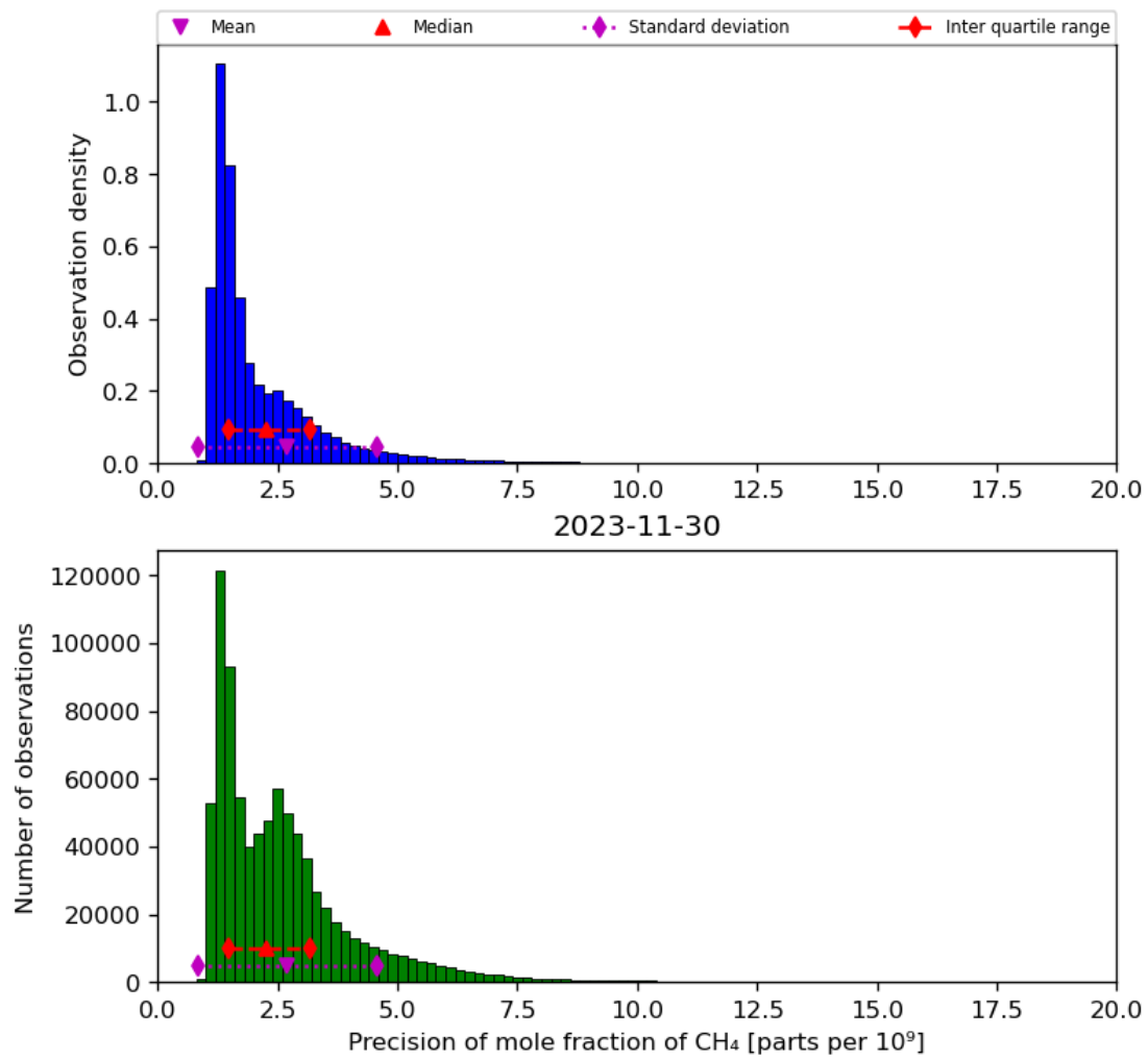
Figure 24: Histogram of “Precision of mole fraction of CH 4 ” for 2023-11-29 to 2023-12-01
