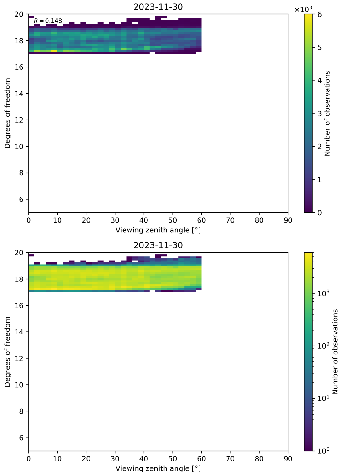
Figure 107: Scatter density plot of “Viewing zenith angle” against “Degrees of freedom” for 2023-11-29 to 2023-12-01.
