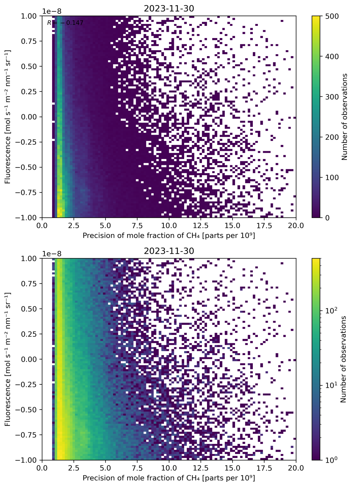
Figure 81: Scatter density plot of “Precision of mole fraction of \text{CH}_4 ” against “Fluorescence” for 2023-11-29 to 2023-12-01.
