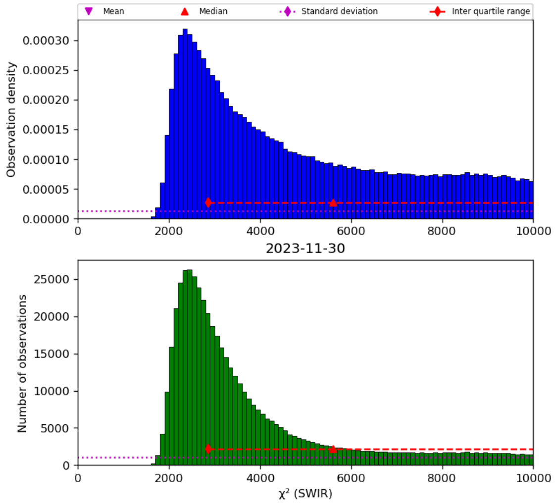
Figure 28: Histogram of “ \chi^2 (SWIR)” for 2023-11-29 to 2023-12-01
