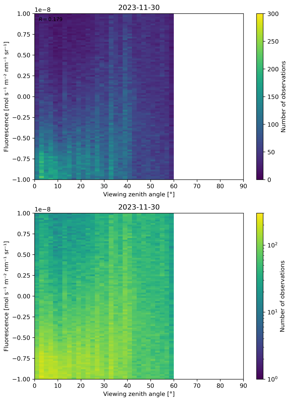
Figure 108: Scatter density plot of “Viewing zenith angle” against “Fluorescence” for 2023-11-29 to 2023-12-01.
