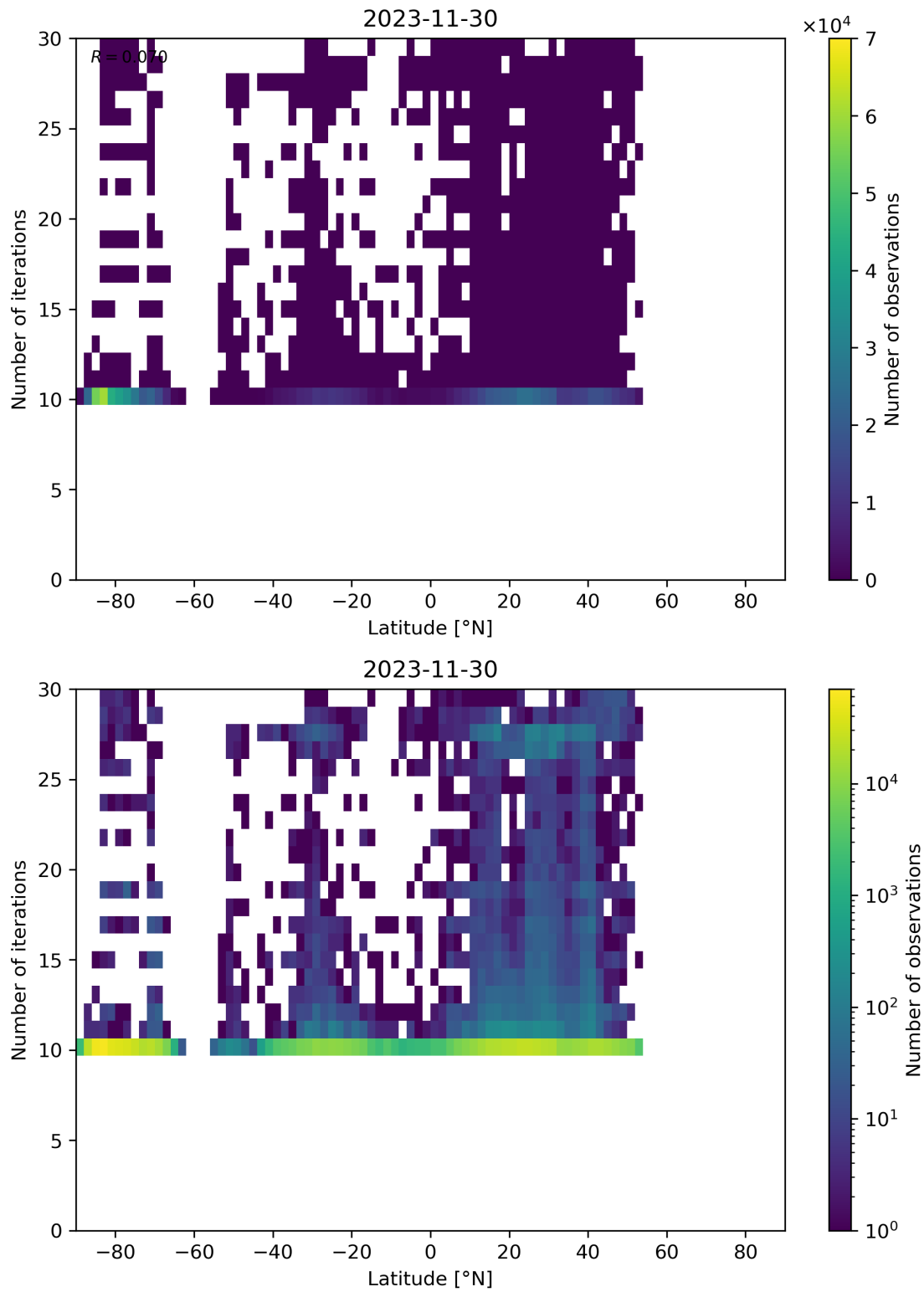
Figure 60: Scatter density plot of “Latitude” against “Number of iterations” for 2023-11-29 to 2023-12-01.
