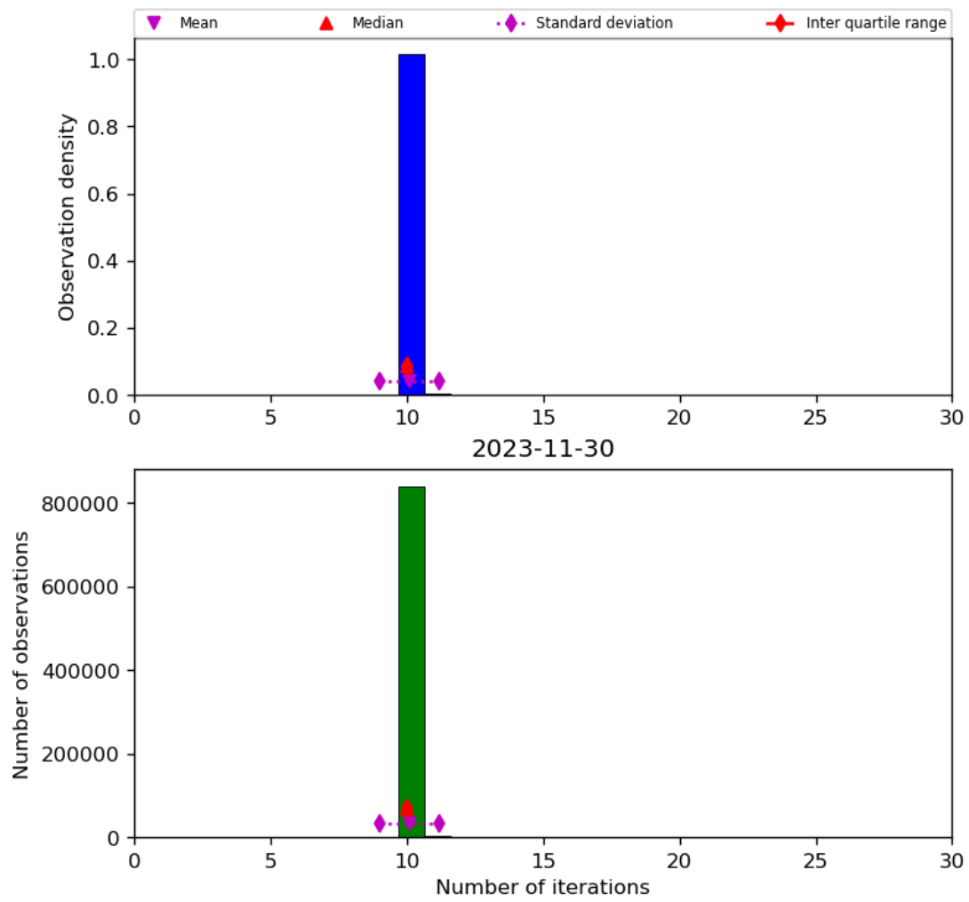
Figure 31: Histogram of “Number of iterations” for 2023-11-29 to 2023-12-01
