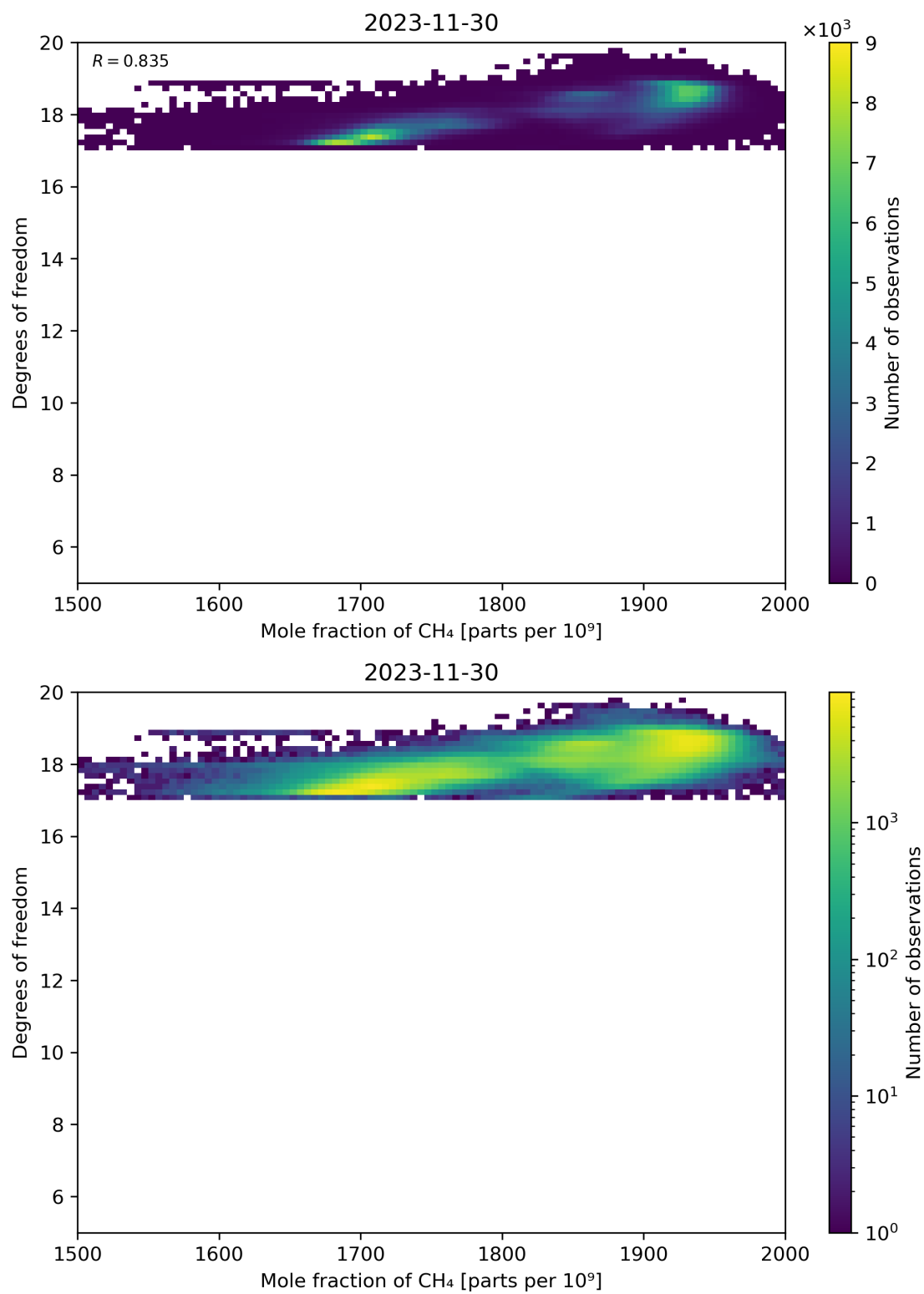
Figure 72: Scatter density plot of “Mole fraction of CH 4 ” against “Degrees of freedom” for 2023-11-29 to 2023-12-01.
