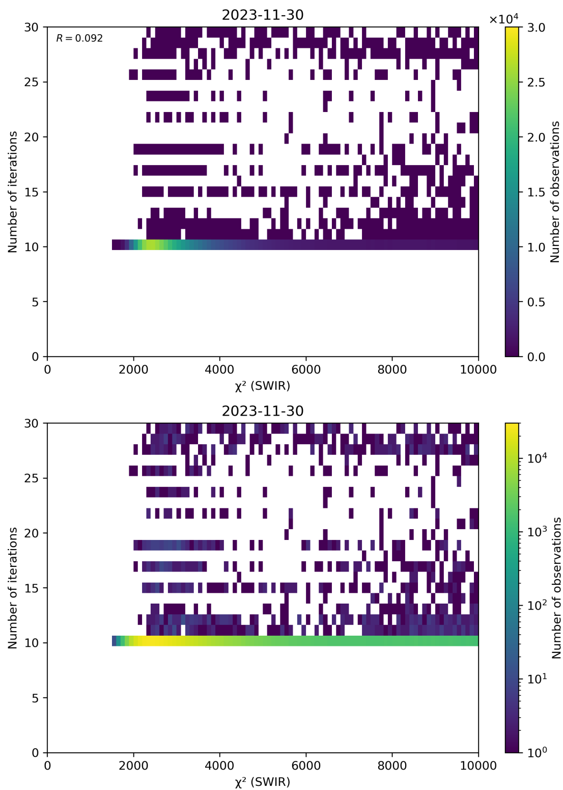
Figure 50: Scatter density plot of “ \chi^2 (SWIR)” against “Number of iterations” for 2023-11-29 to 2023-12-01.
