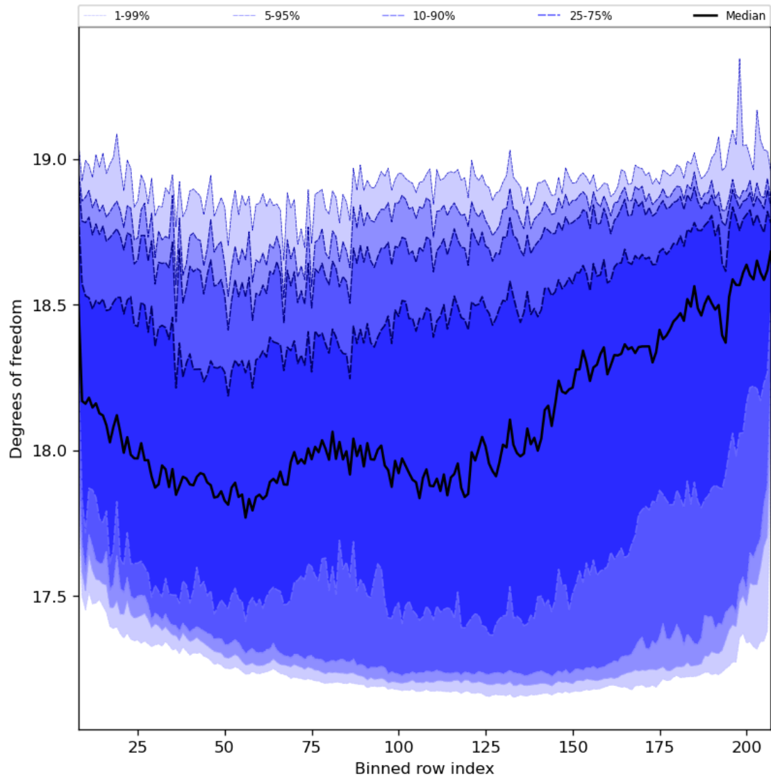
Figure 41: Along track statistics of “Degrees of freedom” for 2023-11-29 to 2023-12-01
