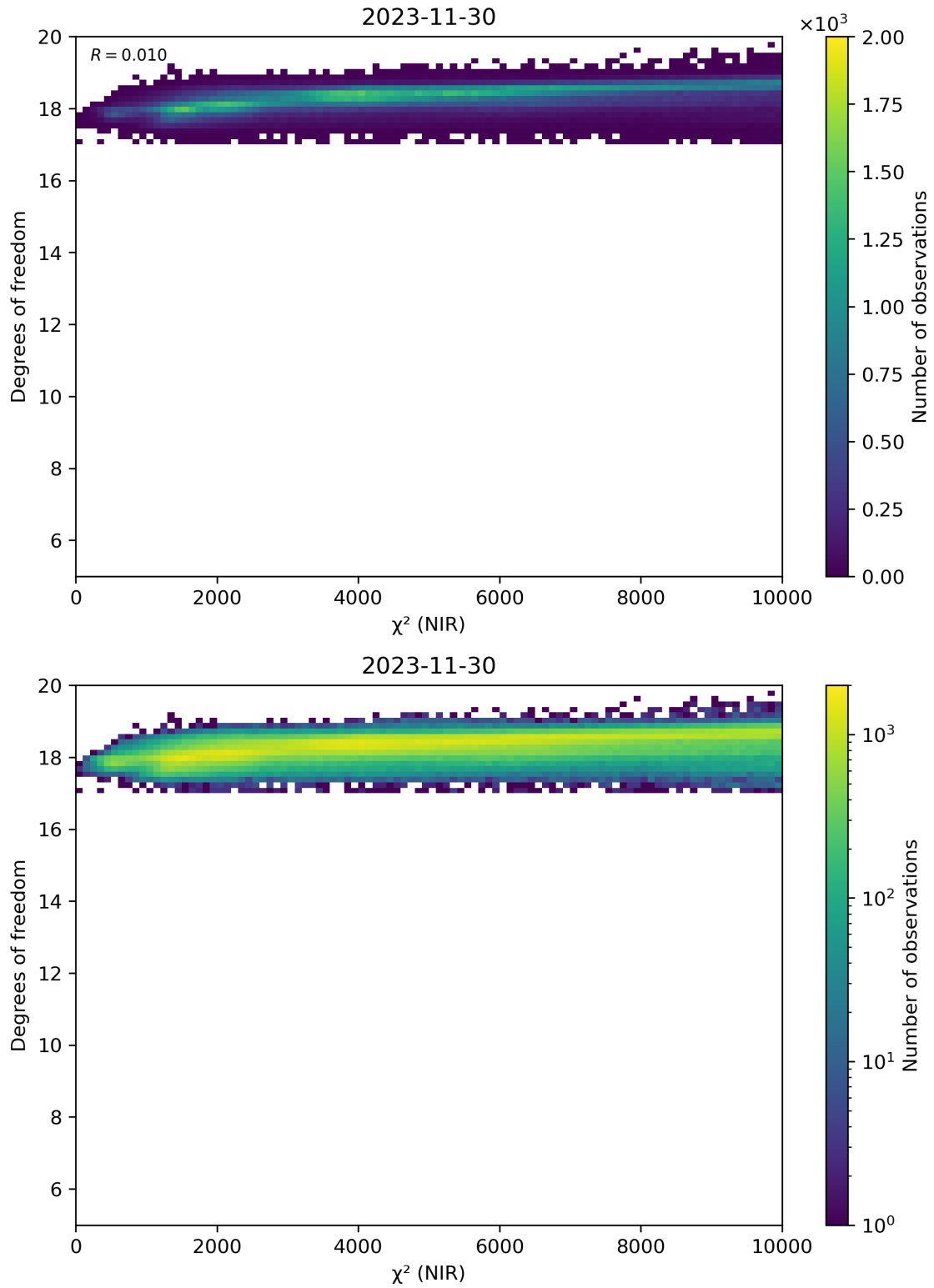
Figure 44: Scatter density plot of “ \chi^2 (NIR)” against “Degrees of freedom” for 2023-11-29 to 2023-12-01.
