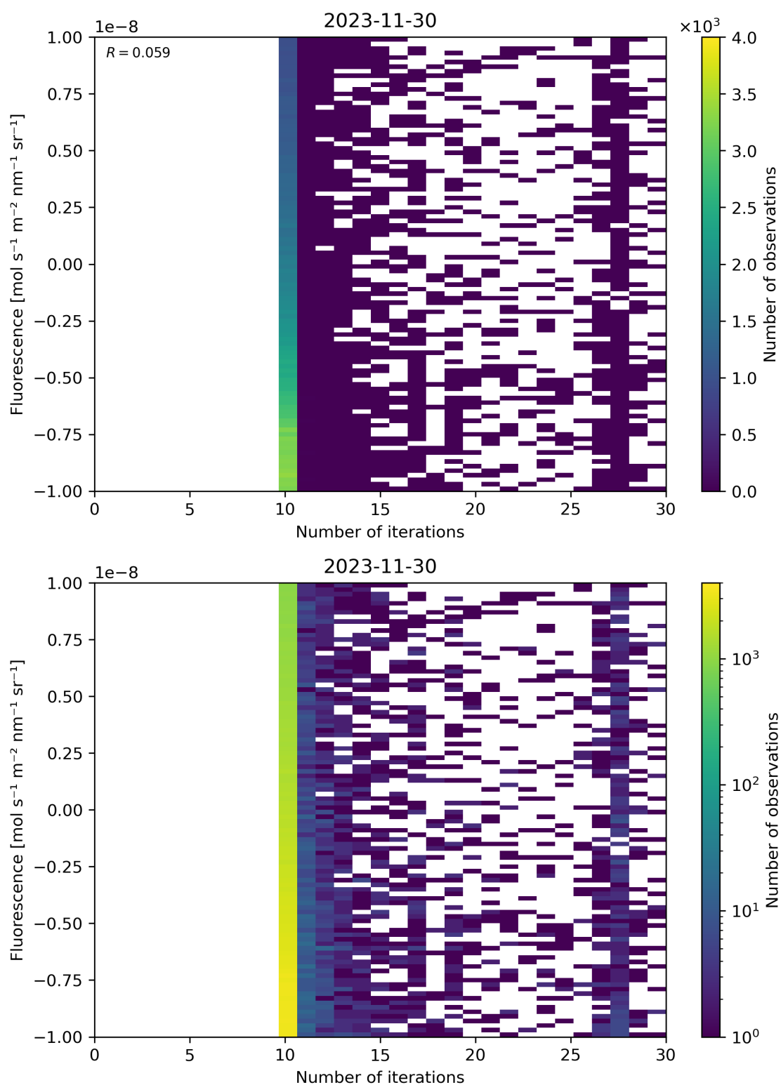
Figure 87: Scatter density plot of “Number of iterations” against “Fluorescence” for 2023-11-29 to 2023-12-01.
