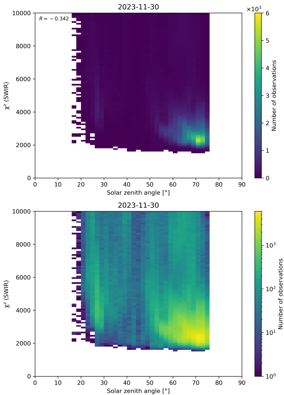
Figure 95: Scatter density plot of “Solar zenith angle” against “ \chi^2 (SWIR)” for 2023-11-29 to 2023-12-01.
