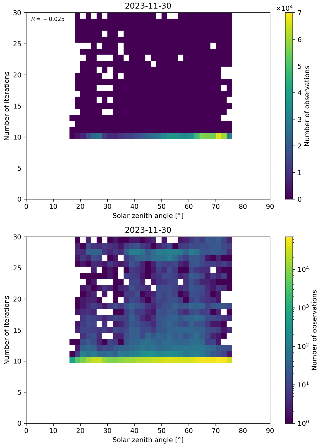
Figure 102: Scatter density plot of “Solar zenith angle” against “Number of iterations” for 2023-11-29 to 2023-12-01.
