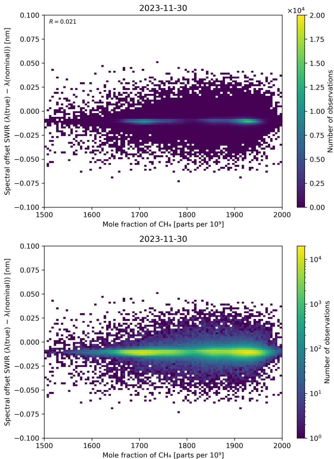
Figure 86: Scatter density plot of “Mole fraction of CH 4 ” against “Spectral offset SWIR ( \lambda(\text{true}) - \lambda(\text{nominal}) )” for 2023-11-29 to 2023-12-01.
