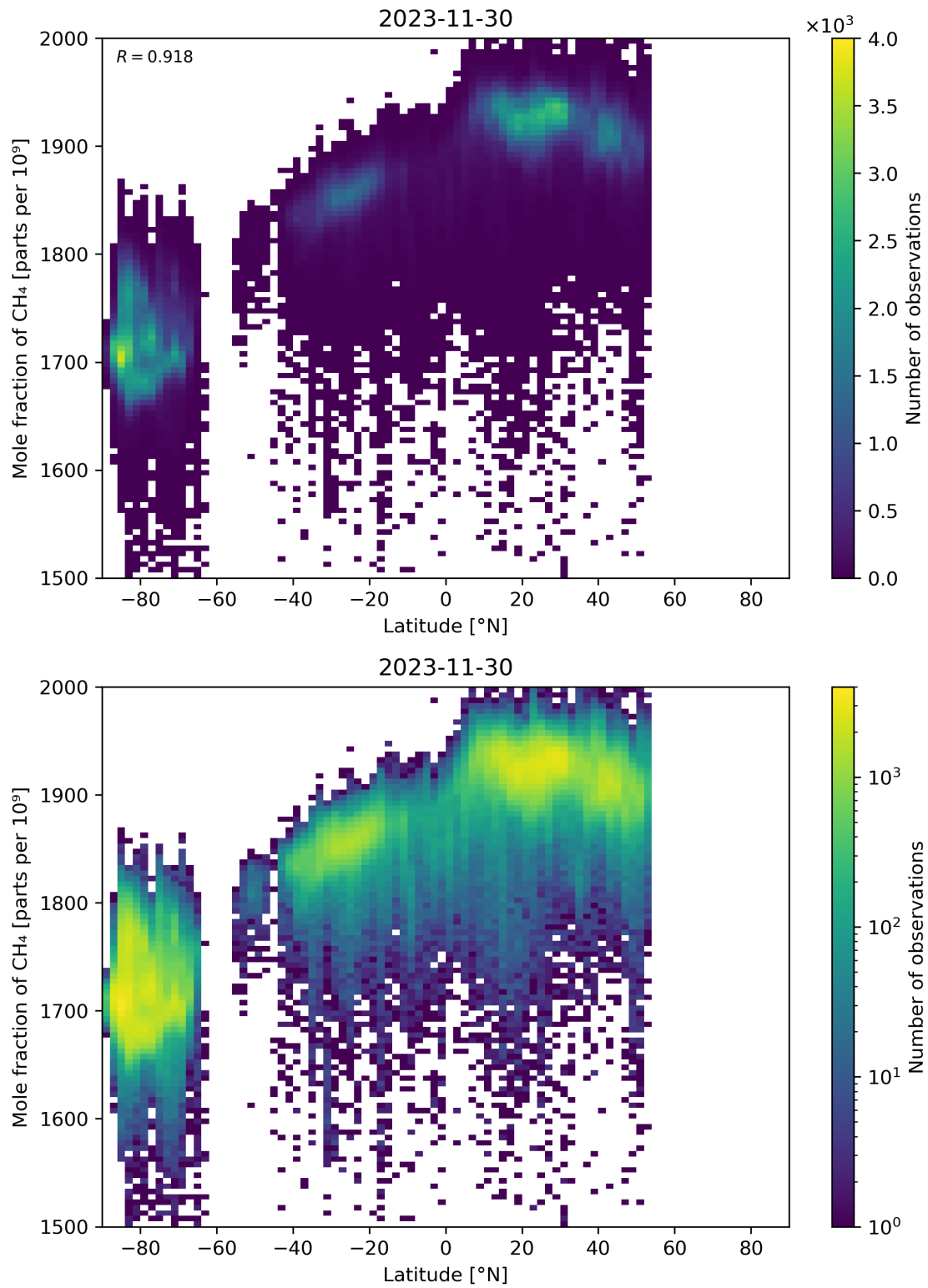
Figure 57: Scatter density plot of “Latitude” against “Mole fraction of CH 4 ” for 2023-11-29 to 2023-12-01.
