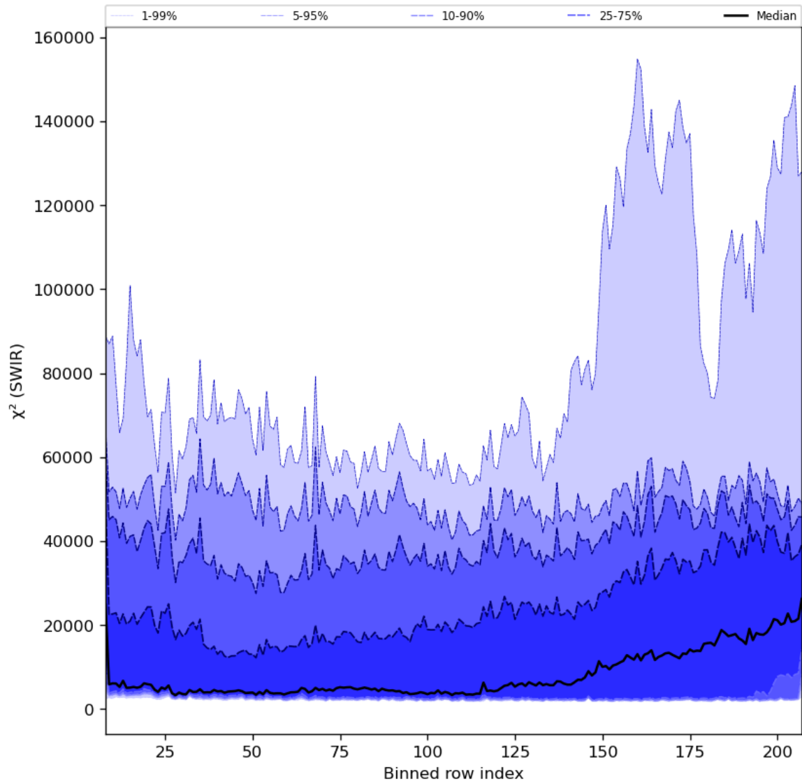
Figure 39: Along track statistics of “ \chi^2 (SWIR)” for 2023-11-29 to 2023-12-01
