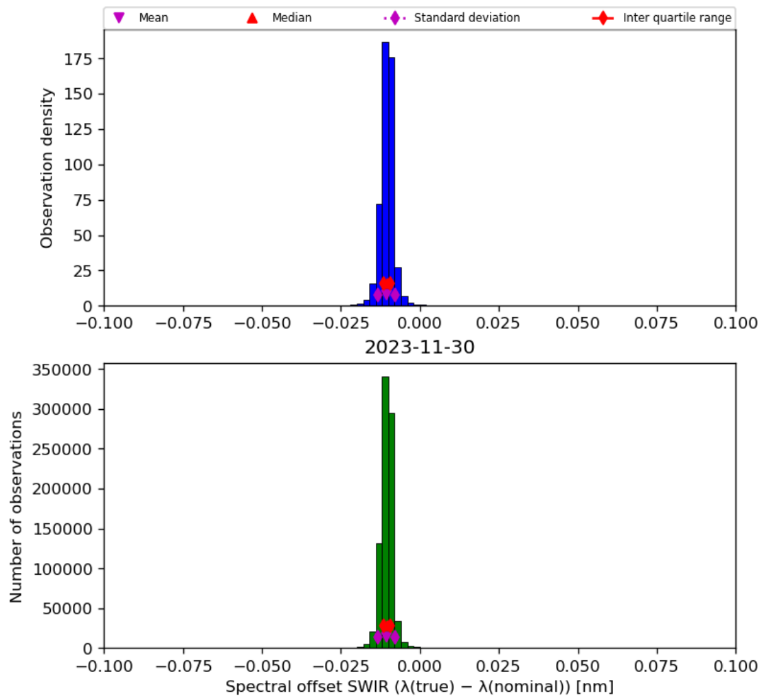
Figure 27: Histogram of “Spectral offset SWIR ( \lambda(\text{true}) - \lambda(\text{nominal}) )” for 2023-11-29 to 2023-12-01
