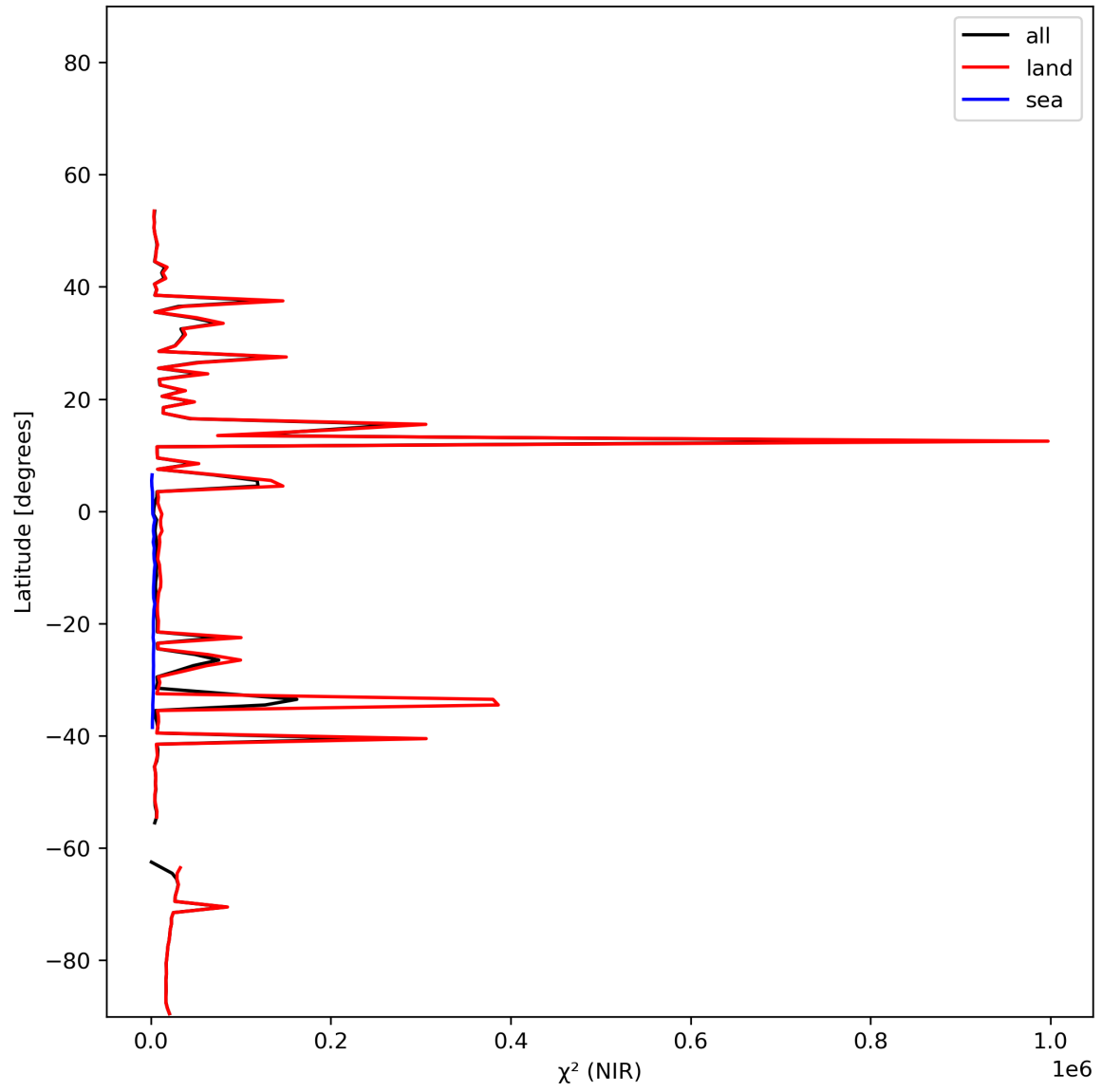
Figure 18: Zonal average of “ \chi^2 (NIR)” for 2023-11-29 to 2023-12-01.
