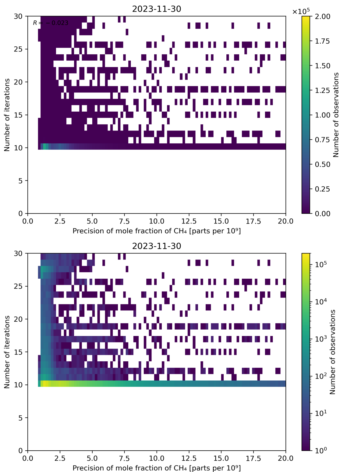
Figure 83: Scatter density plot of “Precision of mole fraction of CH 4 ” against “Number of iterations” for 2023-11-29 to 2023-12-01.
