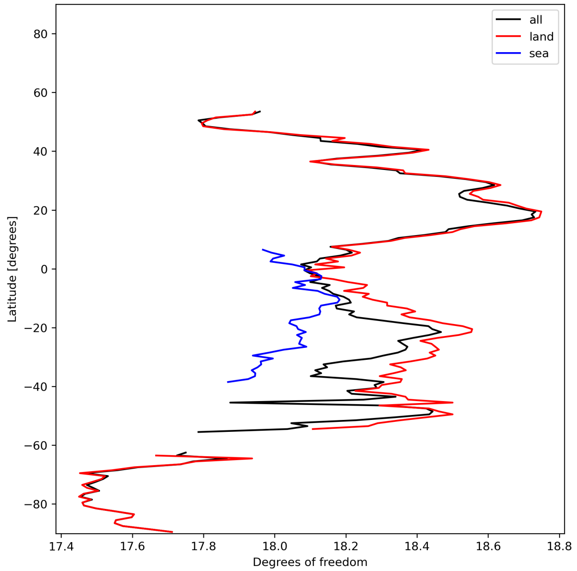
Figure 19: Zonal average of “Degrees of freedom” for 2023-11-29 to 2023-12-01.
