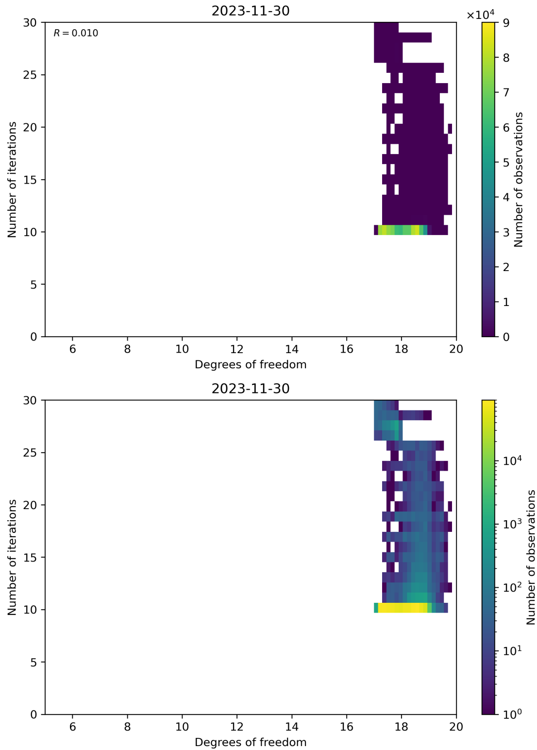
Figure 52: Scatter density plot of “Degrees of freedom” against “Number of iterations” for 2023-11-29 to 2023-12-01.
