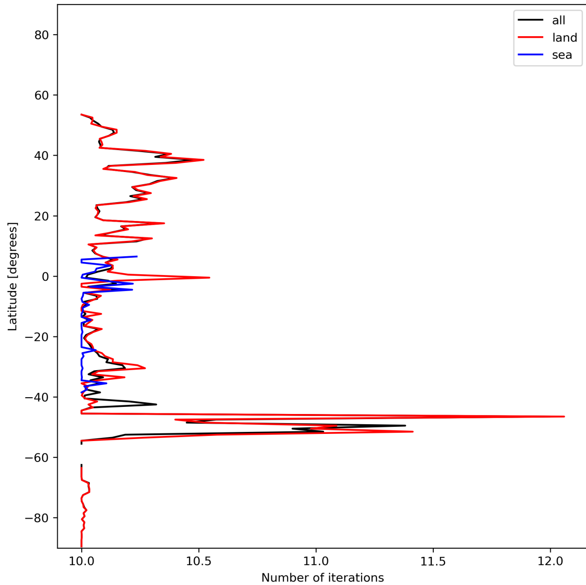
Figure 20: Zonal average of “Number of iterations” for 2023-11-29 to 2023-12-01.
