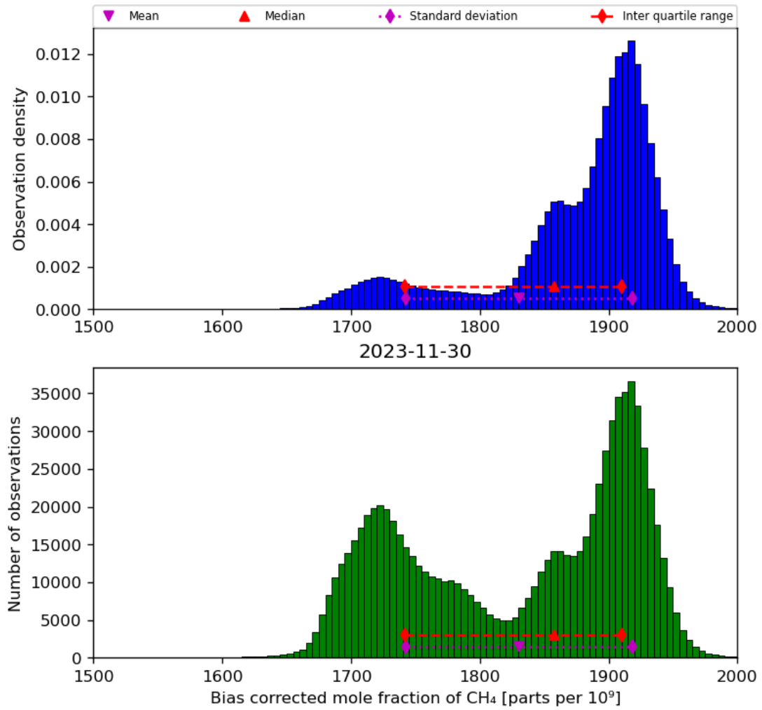
Figure 25: Histogram of “Bias corrected mole fraction of CH 4 ” for 2023-11-29 to 2023-12-01
