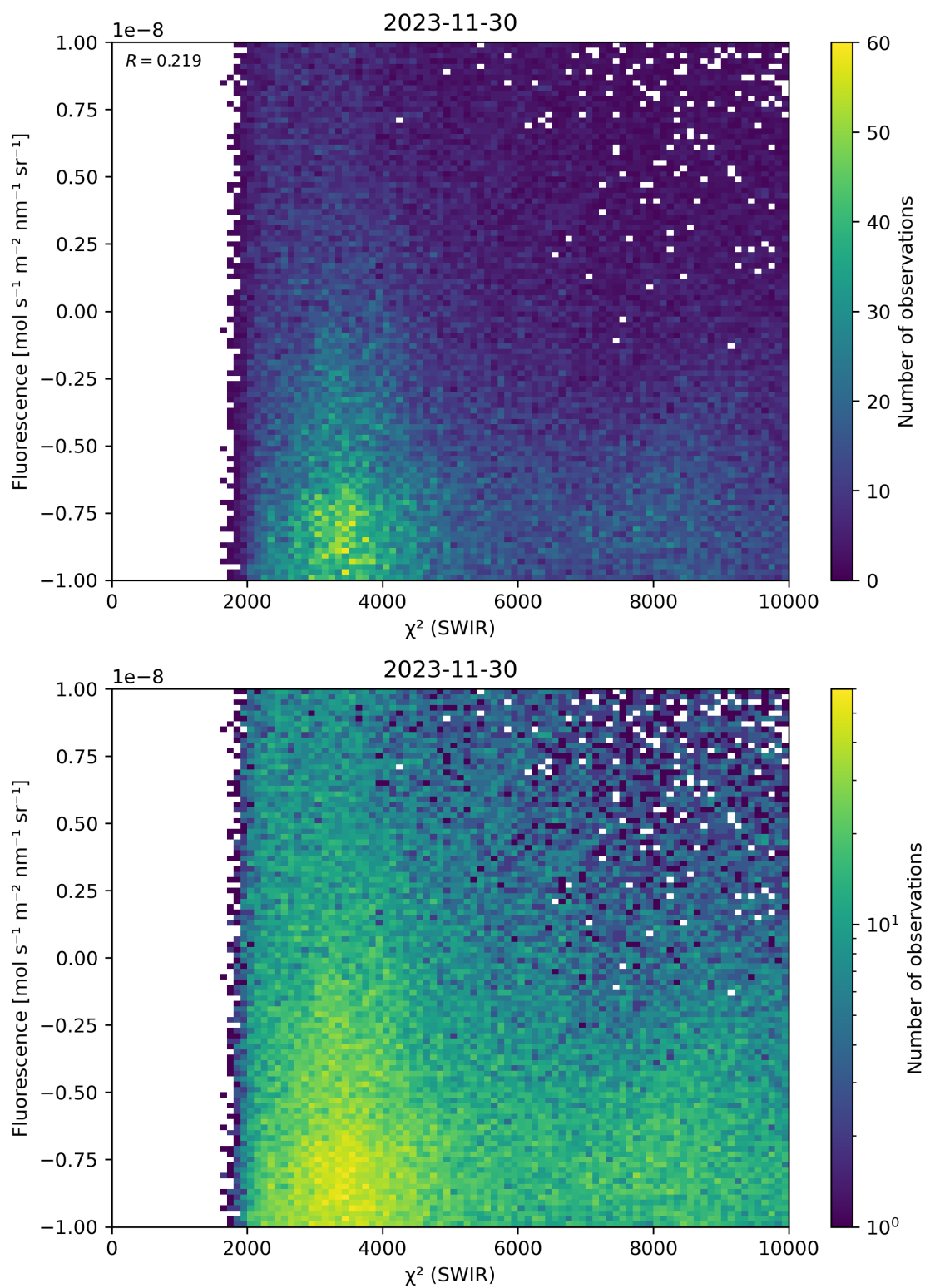
Figure 49: Scatter density plot of “ \chi^2 (SWIR)” against “Fluorescence” for 2023-11-29 to 2023-12-01.
