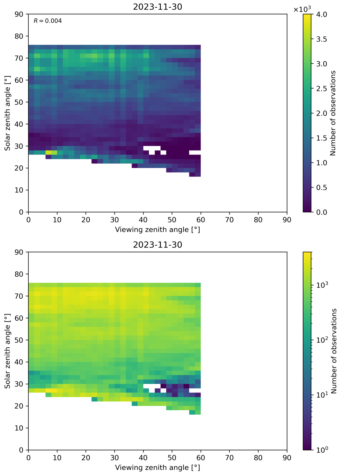
Figure 115: Scatter density plot of “Viewing zenith angle” against “Solar zenith angle” for 2023-11-29 to 2023-12-01.
