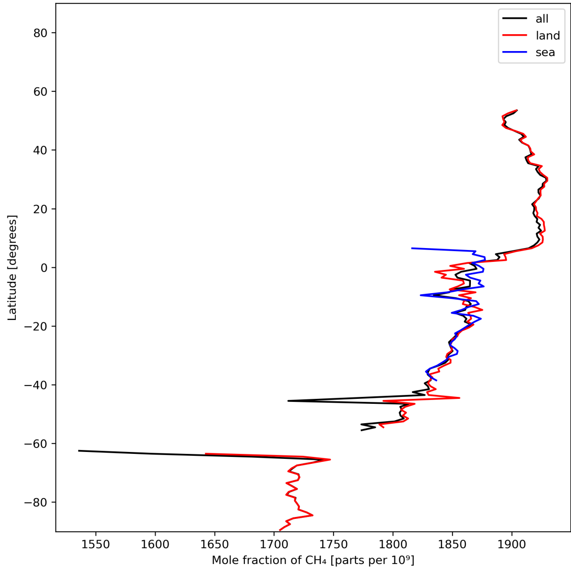
Figure 12: Zonal average of “Mole fraction of \text{CH}_4 ” for 2023-11-29 to 2023-12-01.
