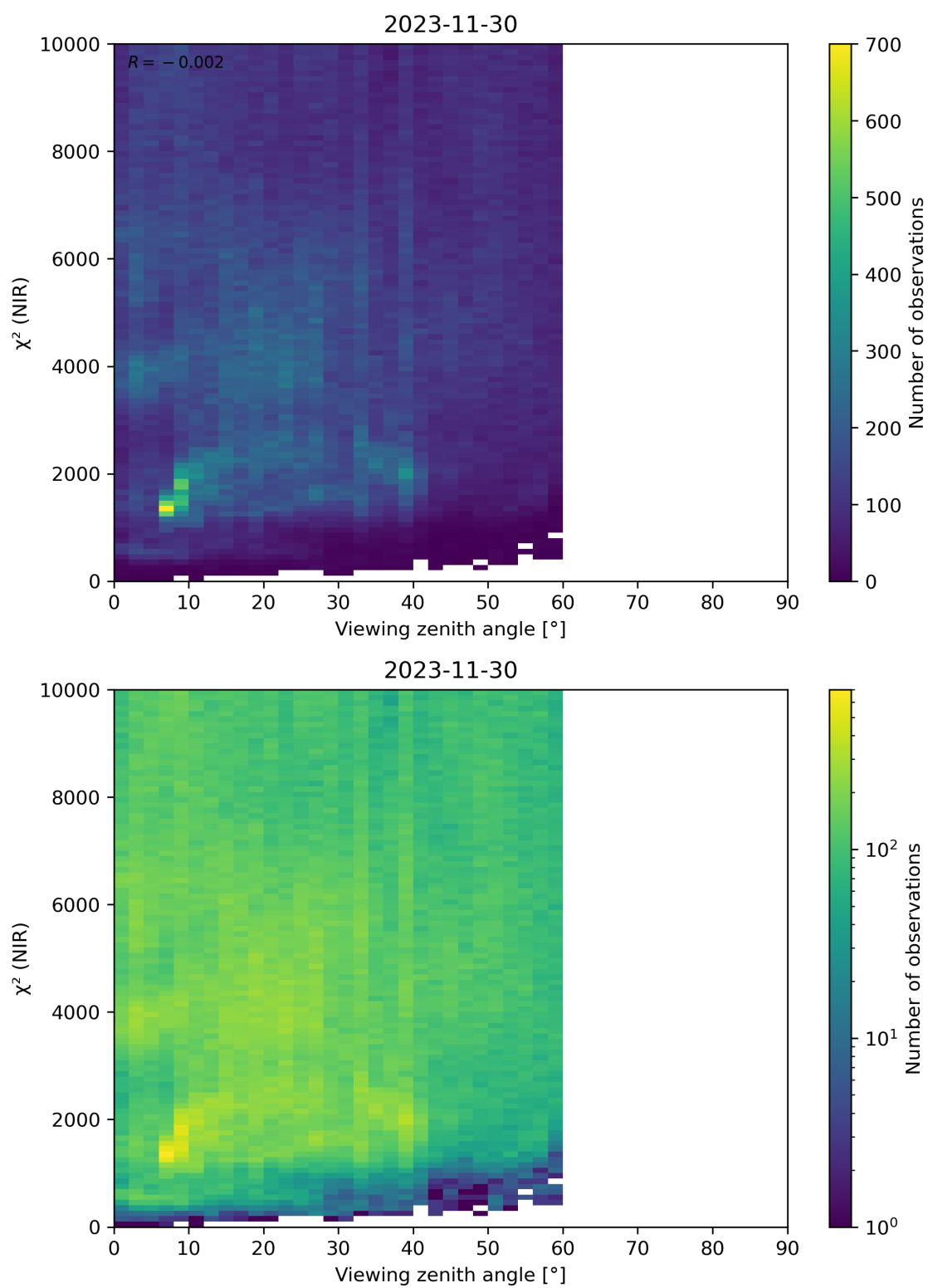
Figure 105: Scatter density plot of “Viewing zenith angle” against “ \chi^2 (NIR)” for 2023-11-29 to 2023-12-01.
