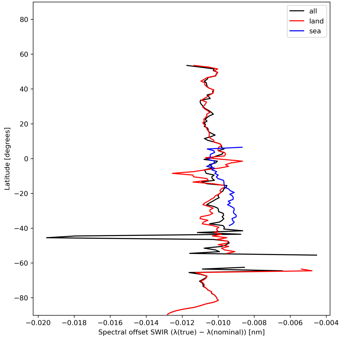
Figure 16: Zonal average of “Spectral offset SWIR ( \lambda(\text{true}) - \lambda(\text{nominal}) )” for 2023-11-29 to 2023-12-01.
