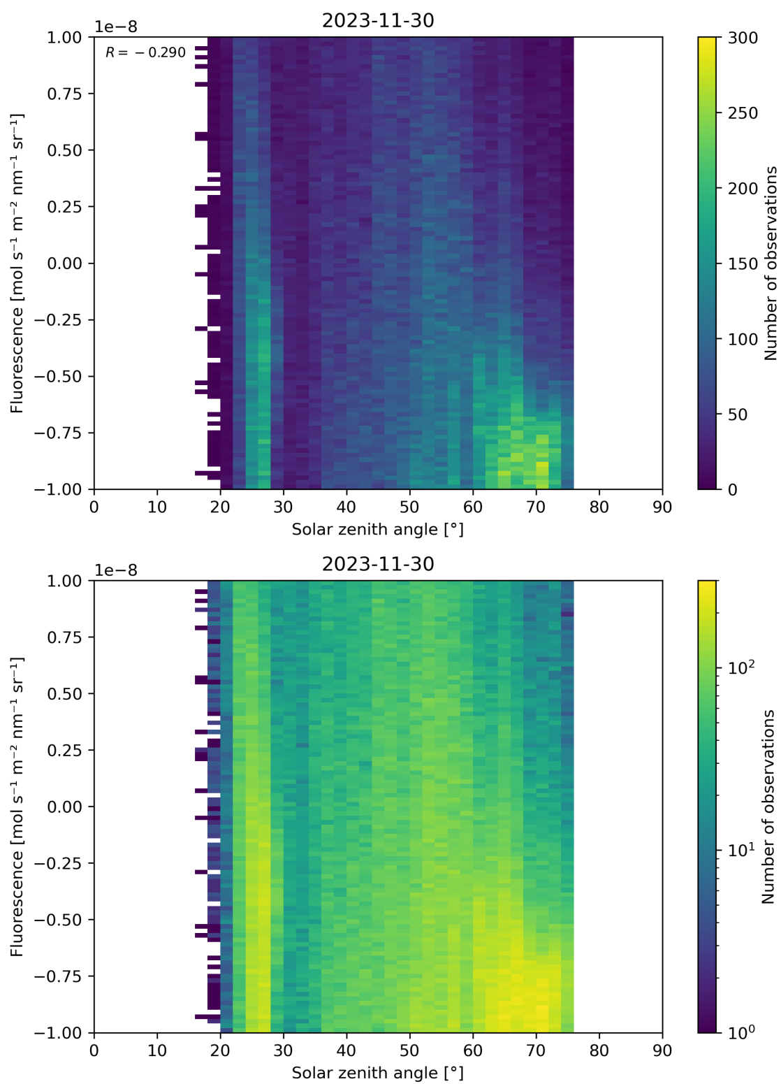
Figure 97: Scatter density plot of “Solar zenith angle” against “Fluorescence” for 2023-11-29 to 2023-12-01.
