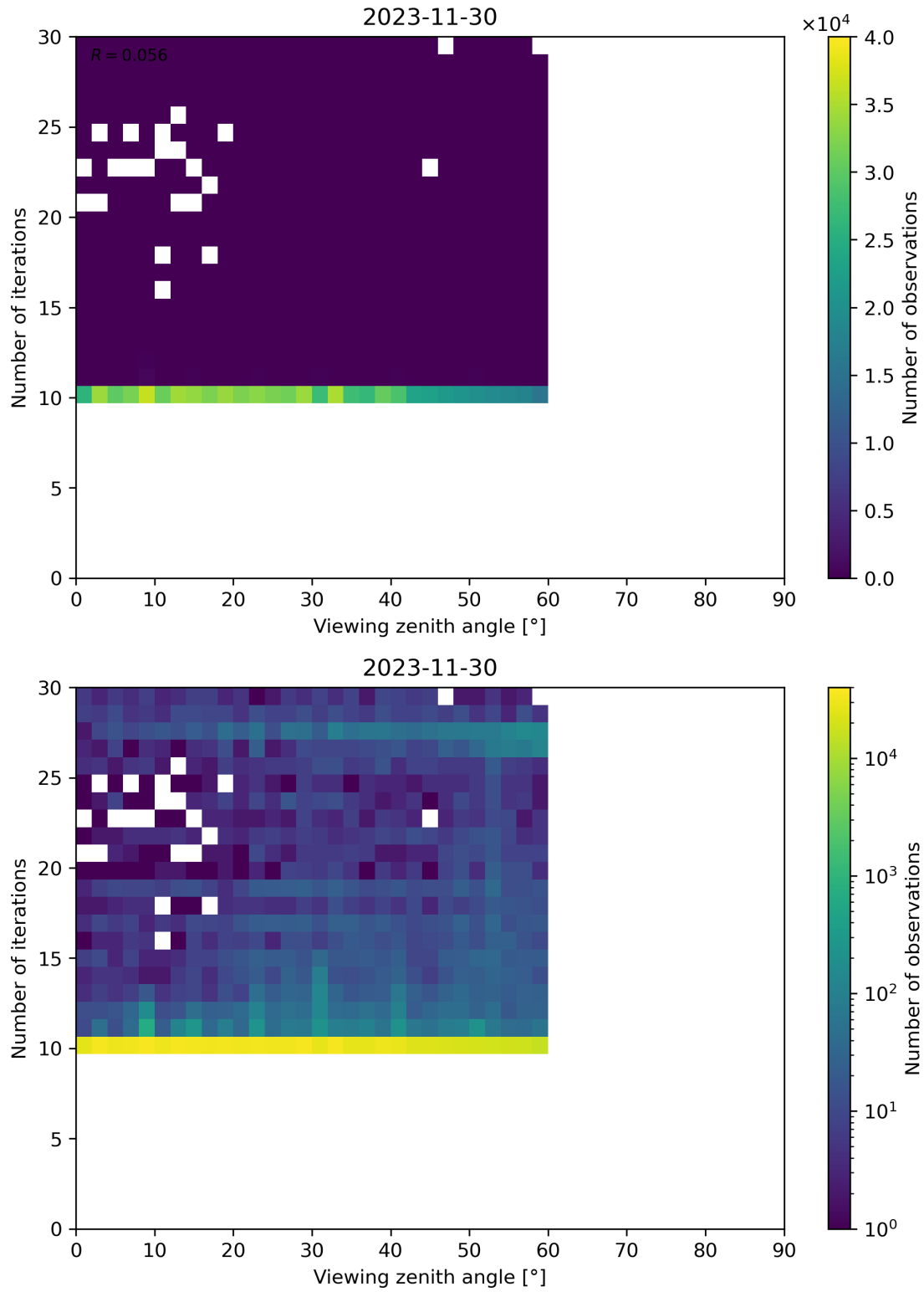
Figure 113: Scatter density plot of “Viewing zenith angle” against “Number of iterations” for 2023-11-29 to 2023-12-01.
