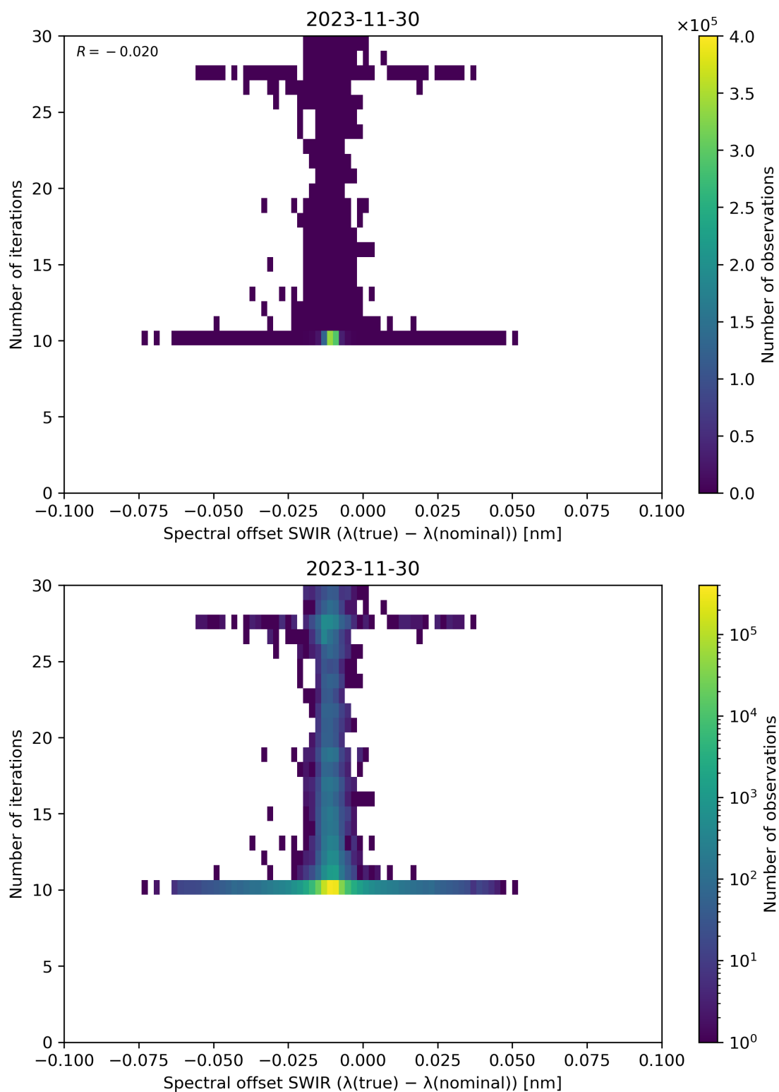
Figure 121: Scatter density plot of “Spectral offset SWIR ( \lambda(\text{true}) - \lambda(\text{nominal}) )” against “Number of iterations” for 2023-11-29 to 2023-12-01.
