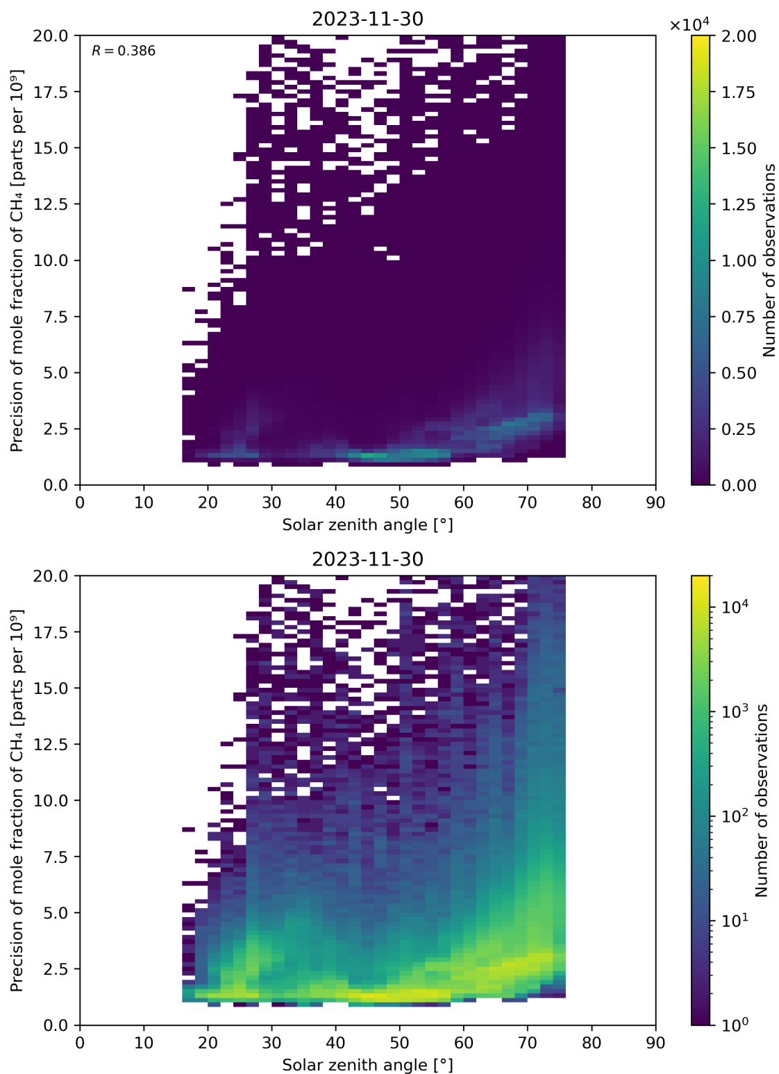
Figure 101: Scatter density plot of “Solar zenith angle” against “Precision of mole fraction of CH 4 ” for 2023-11-29 to 2023-12-01.
