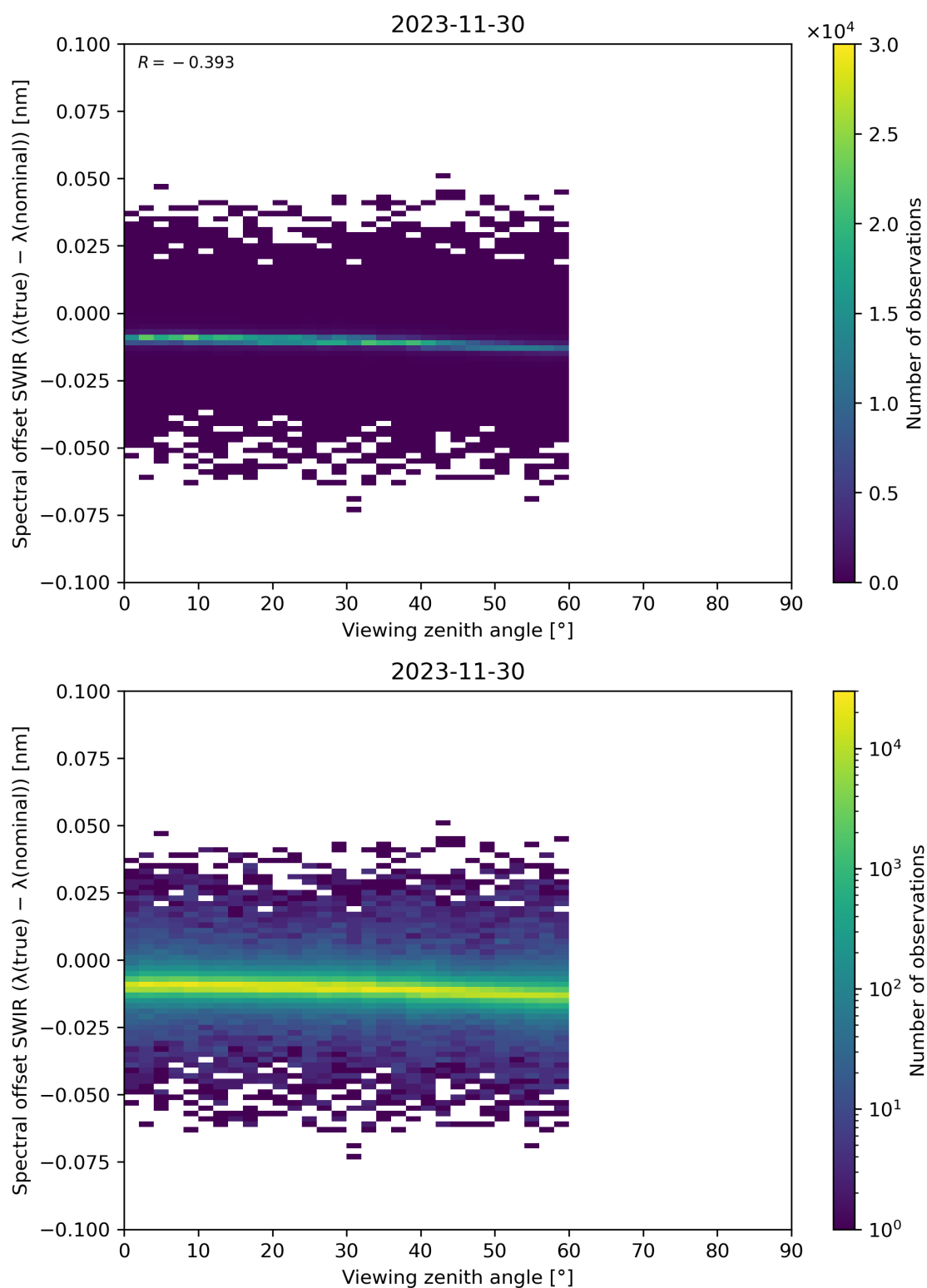
Figure 116: Scatter density plot of “Viewing zenith angle” against “Spectral offset SWIR ( \lambda(\text{true}) - \lambda(\text{nominal}) )” for 2023-11-29 to 2023-12-01.
