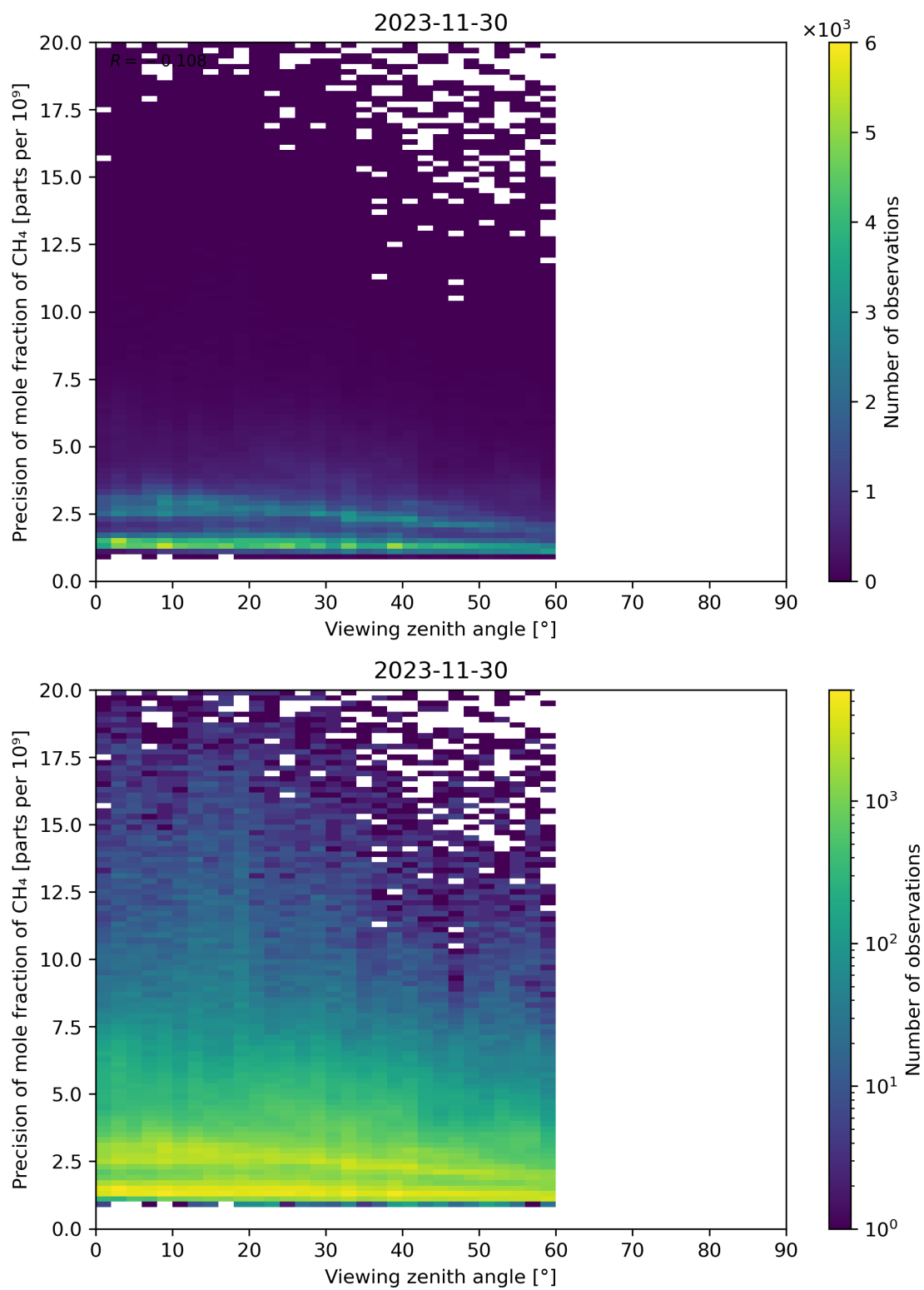
Figure 112: Scatter density plot of “Viewing zenith angle” against “Precision of mole fraction of CH 4 ” for 2023-11-29 to 2023-12-01.
