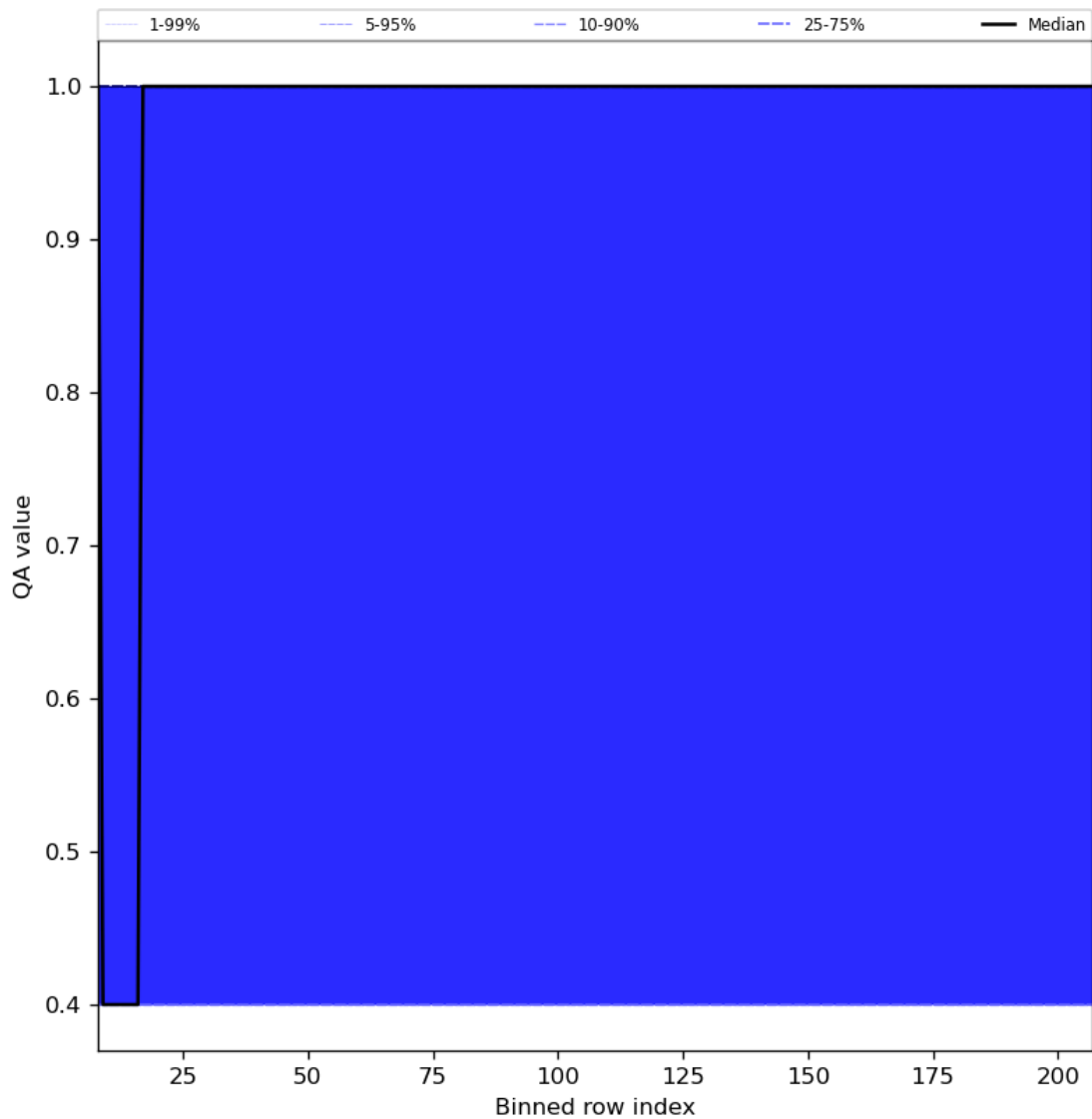
Figure 33: Along track statistics of “QA value” for 2023-11-29 to 2023-12-01
