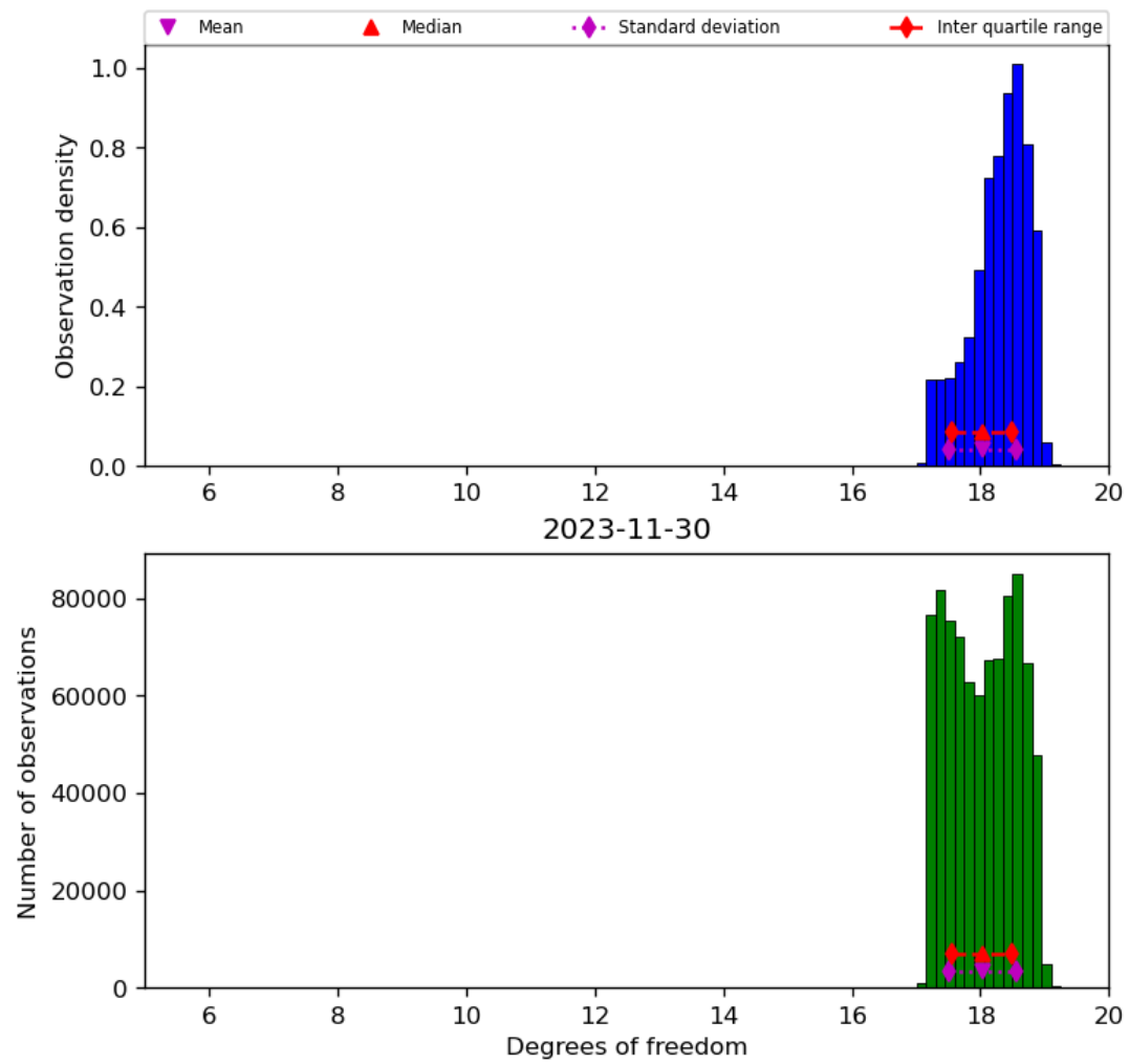
Figure 30: Histogram of “Degrees of freedom” for 2023-11-29 to 2023-12-01
