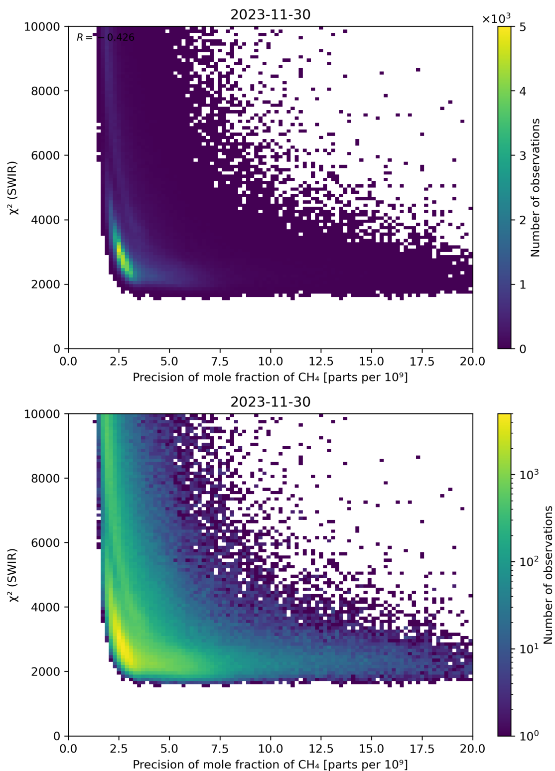
Figure 79: Scatter density plot of “Precision of mole fraction of \text{CH}_4 ” against “ \chi^2 (SWIR)” for 2023-11-29 to 2023-12-01.
