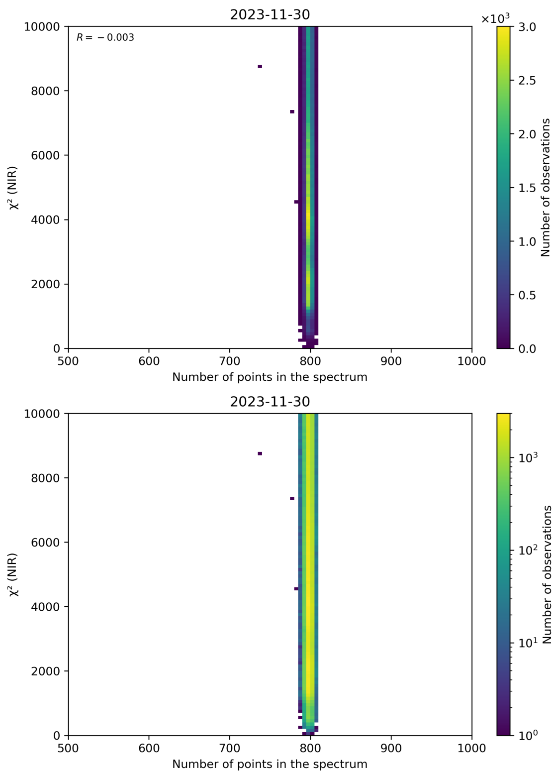
Figure 88: Scatter density plot of “Number of points in the spectrum” against “ \chi^2 (NIR)” for 2023-11-29 to 2023-12-01.
