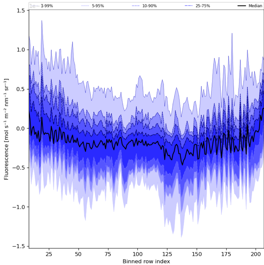
Figure 43: Along track statistics of “Fluorescence” for 2023-11-29 to 2023-12-01
