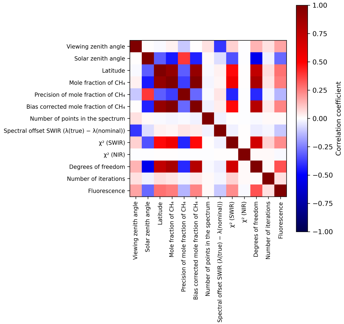
Figure 2: Map of correlation matrix for 2023-11-29 to 2023-12-01.
