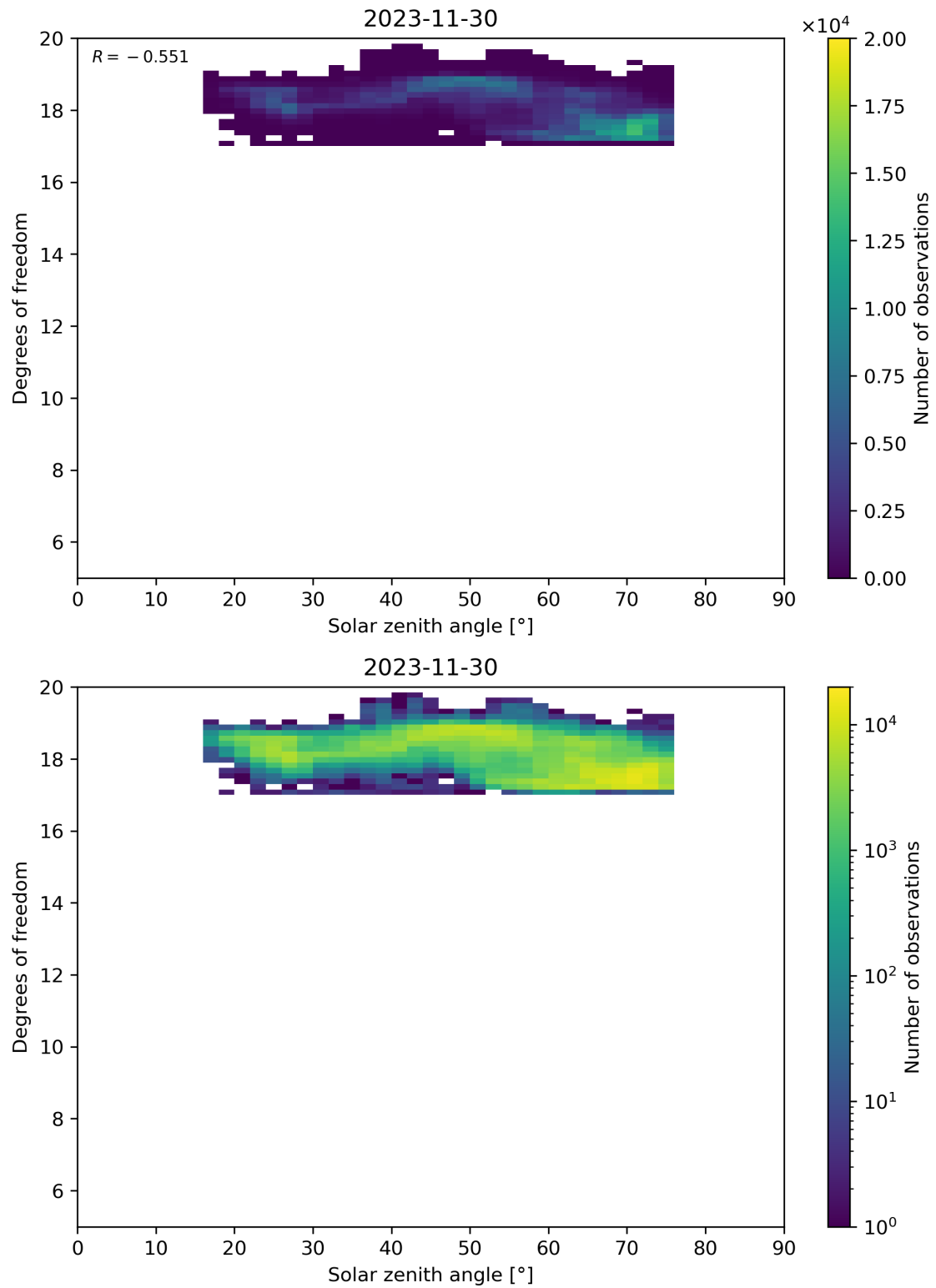
Figure 96: Scatter density plot of “Solar zenith angle” against “Degrees of freedom” for 2023-11-29 to 2023-12-01.
