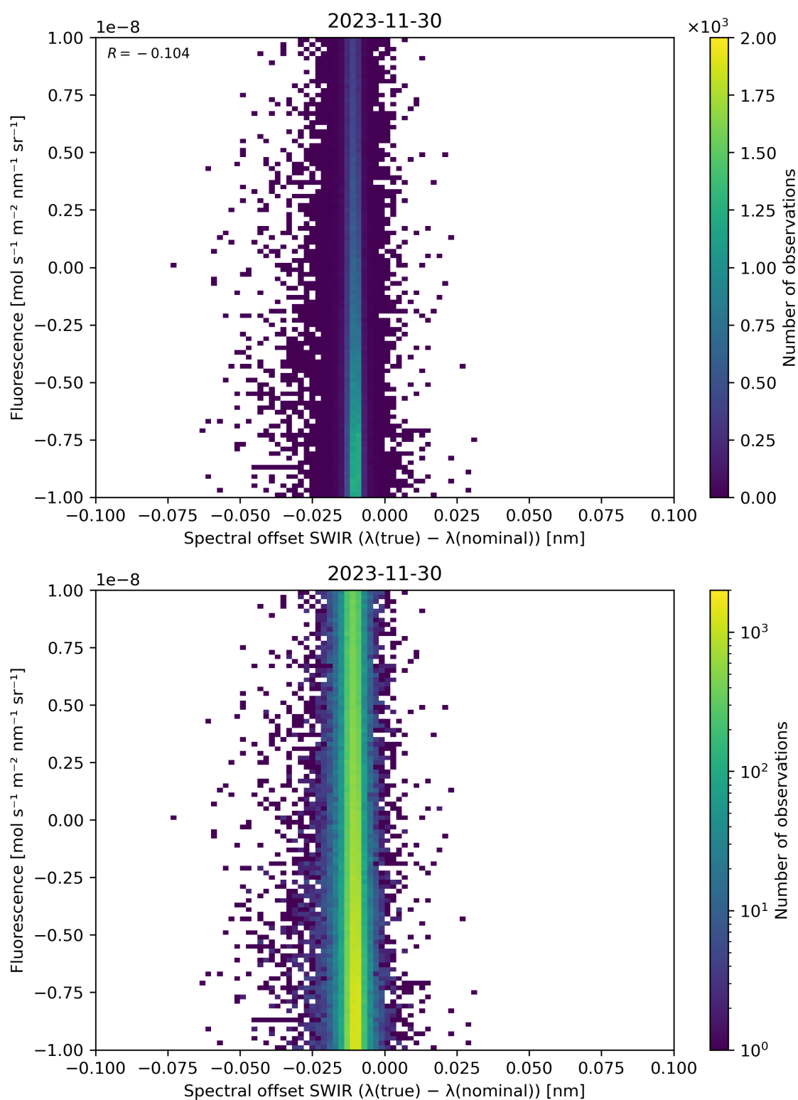
Figure 120: Scatter density plot of “Spectral offset SWIR ( \lambda(\text{true}) - \lambda(\text{nominal}) )” against “Fluorescence” for 2023-11-29 to 2023-12-01.
