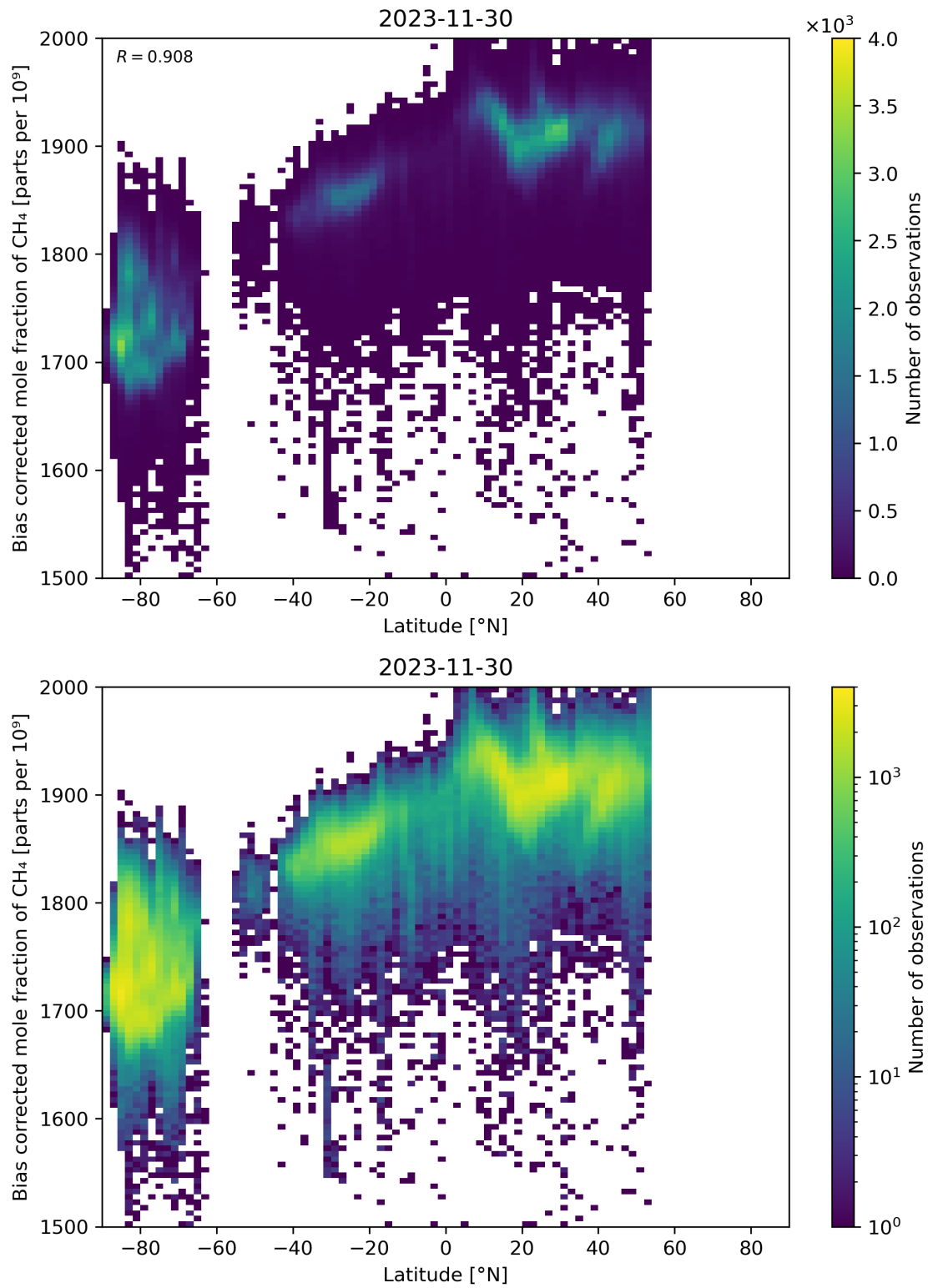
Figure 58: Scatter density plot of “Latitude” against “Bias corrected mole fraction of CH 4 ” for 2023-11-29 to 2023-12-01.
