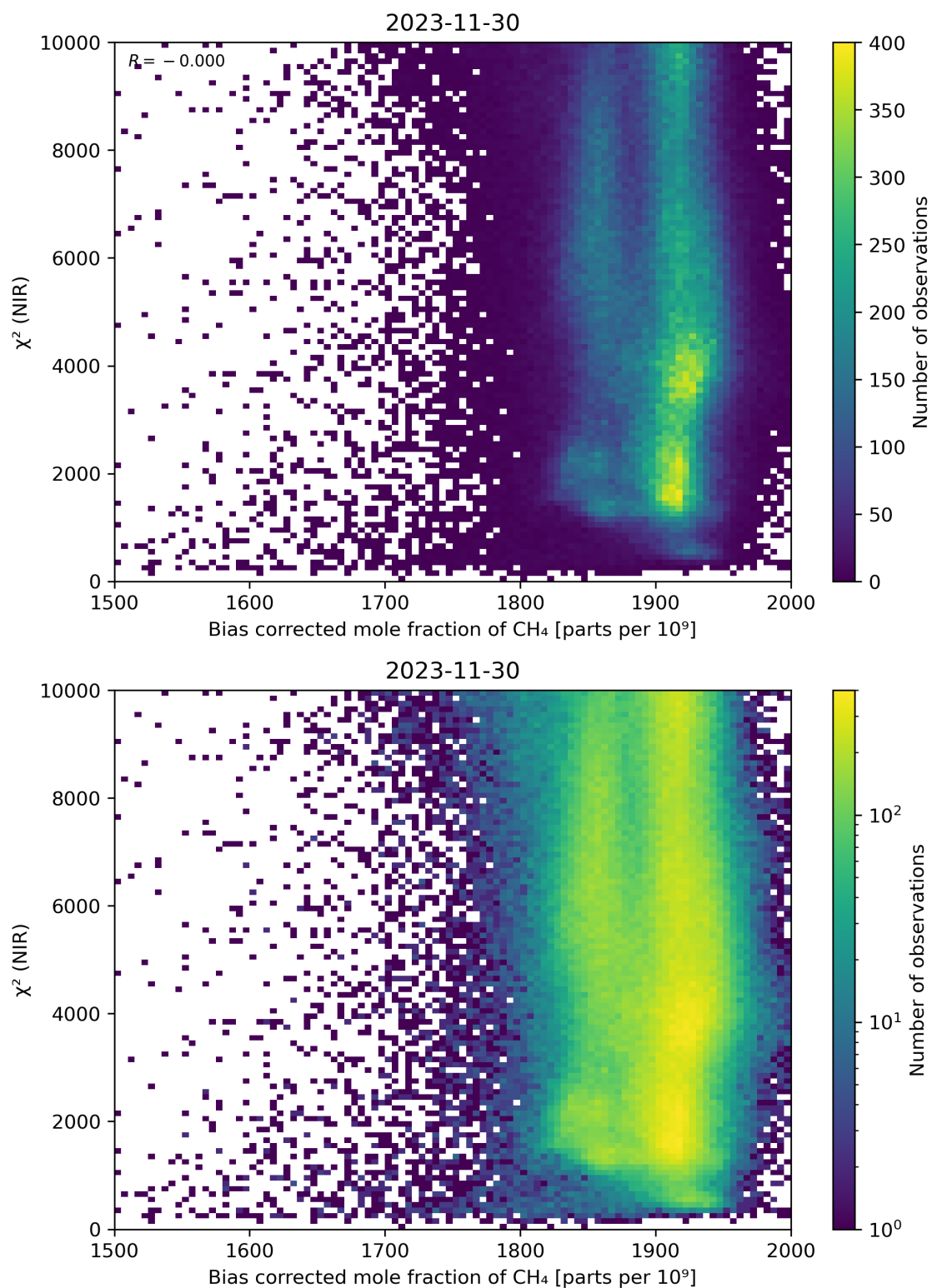
Figure 63: Scatter density plot of “Bias corrected mole fraction of CH 4 ” against “ \chi^2 (NIR)” for 2023-11-29 to 2023-12-01.
