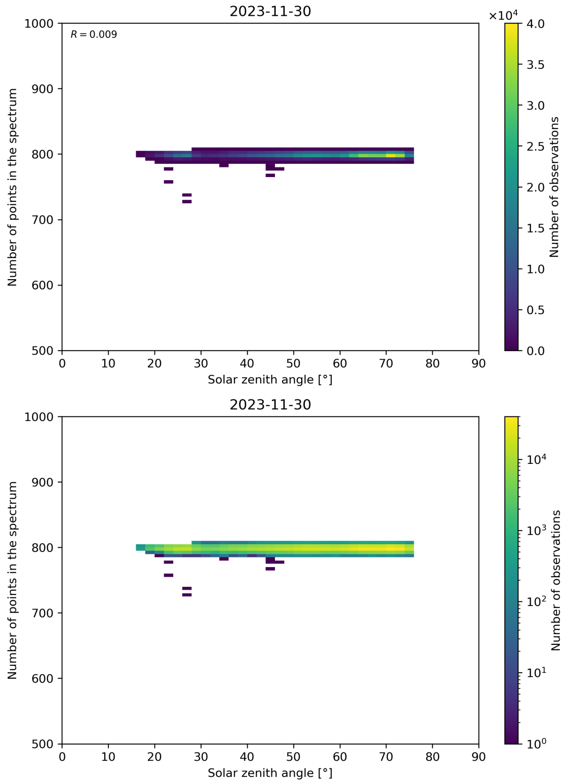
Figure 103: Scatter density plot of “Solar zenith angle” against “Number of points in the spectrum” for 2023-11-29 to 2023-12-01.
