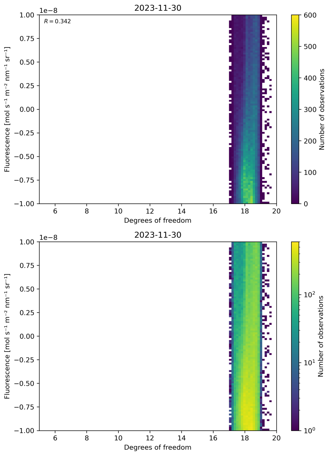
Figure 51: Scatter density plot of “Degrees of freedom” against “Fluorescence” for 2023-11-29 to 2023-12-01.
