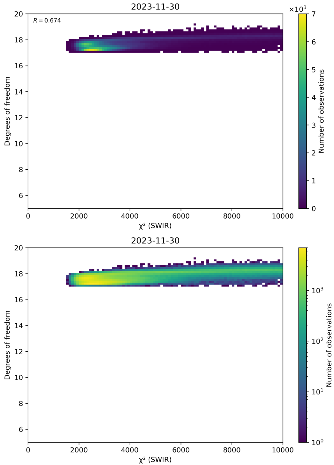
Figure 48: Scatter density plot of " \chi^2 (SWIR)" against "Degrees of freedom" for 2023-11-29 to 2023-12-01.
