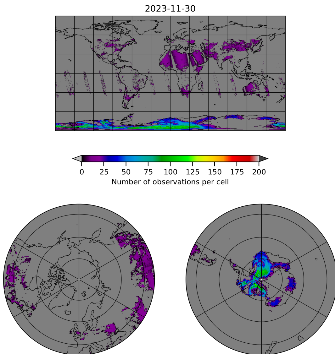
Figure 10: Map of the number of observations for 2023-11-29 to 2023-12-01
