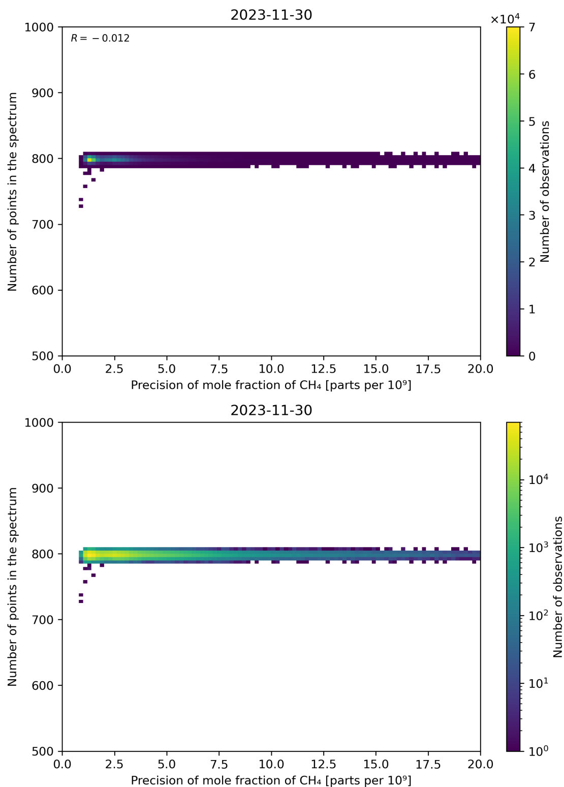
Figure 84: Scatter density plot of “Precision of mole fraction of CH 4 ” against “Number of points in the spectrum” for 2023-11-29 to 2023-12-01.
