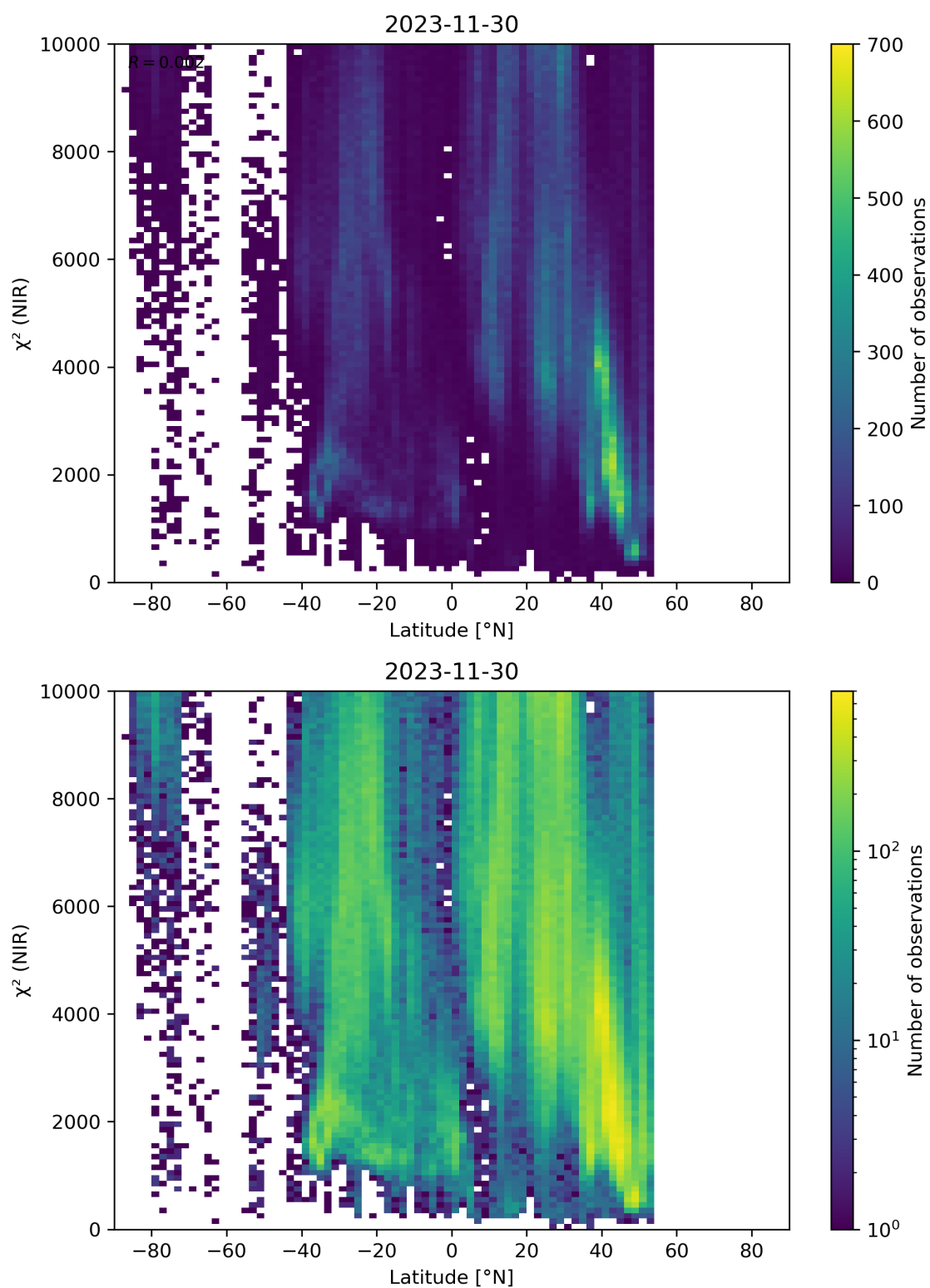
Figure 53: Scatter density plot of “Latitude” against “ \chi^2 (NIR)” for 2023-11-29 to 2023-12-01.
