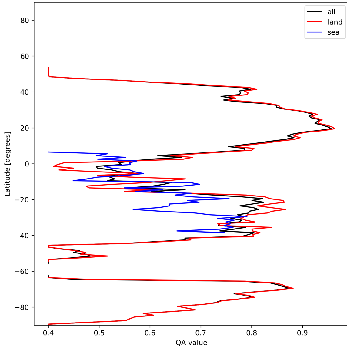
Figure 11: Zonal average of “QA value” for 2023-11-29 to 2023-12-01.
