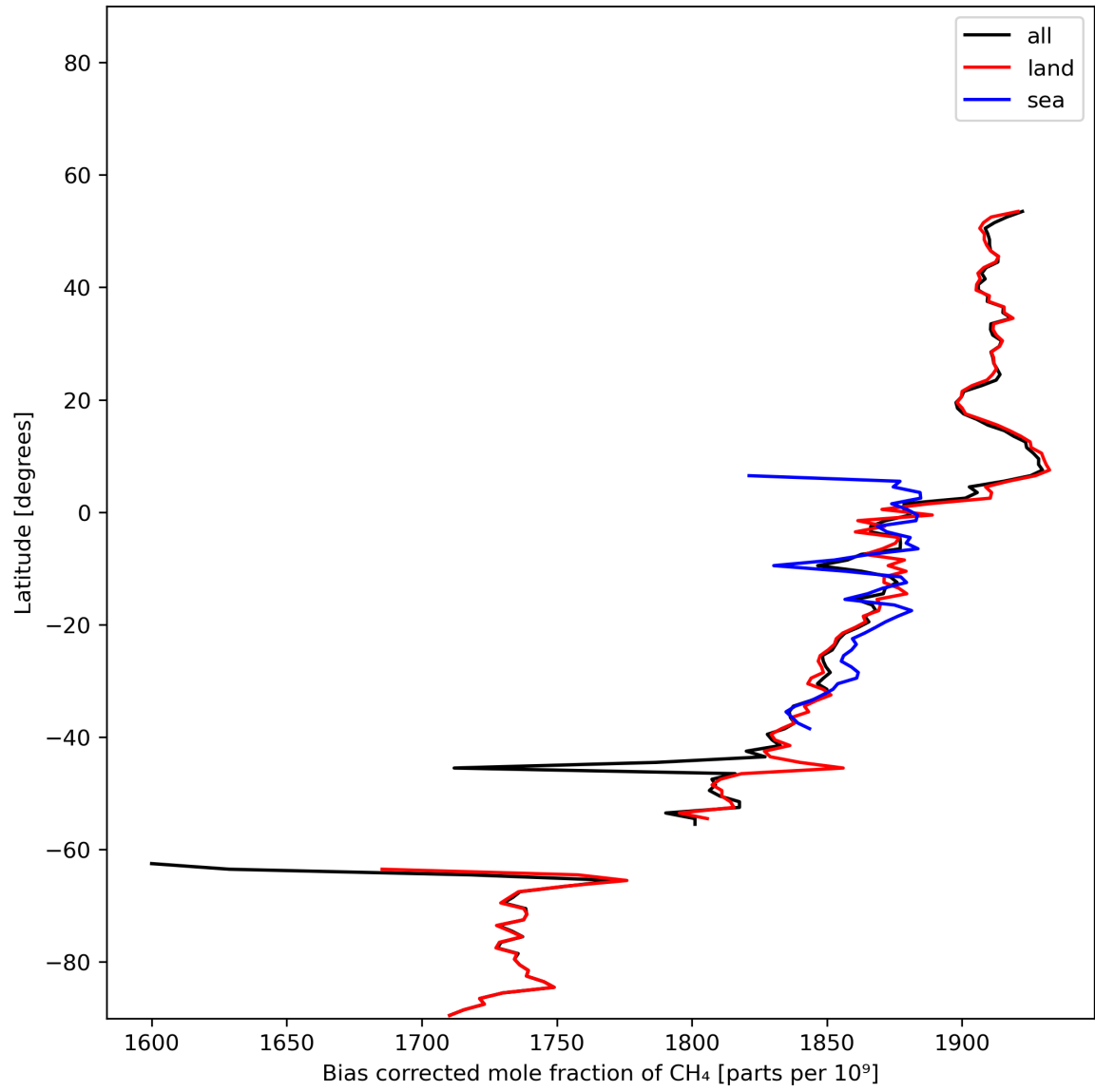
Figure 14: Zonal average of “Bias corrected mole fraction of CH 4 ” for 2023-11-29 to 2023-12-01.
