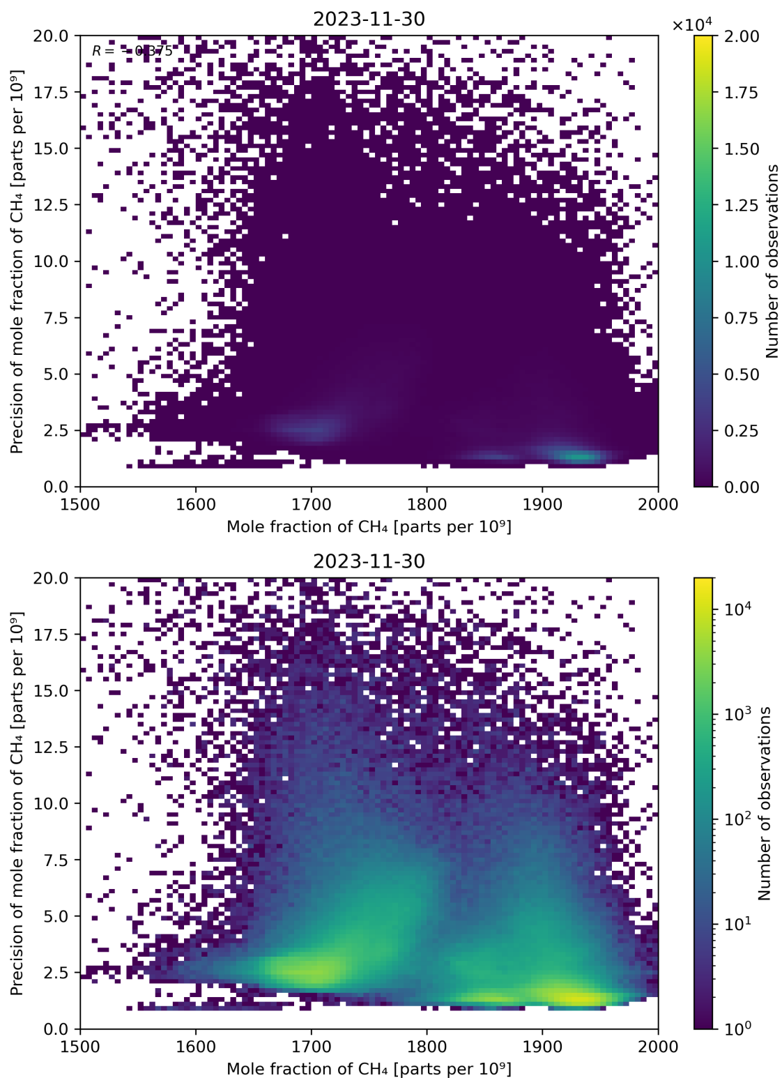
Figure 75: Scatter density plot of “Mole fraction of CH 4 ” against “Precision of mole fraction of CH 4 ” for 2023-11-29 to 2023-12-01.
