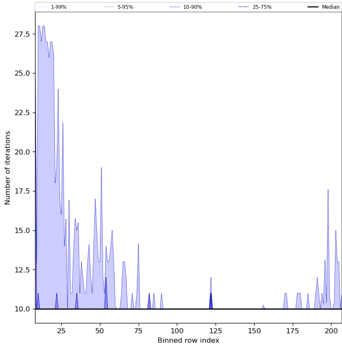
Figure 42: Along track statistics of “Number of iterations” for 2023-11-29 to 2023-12-01
