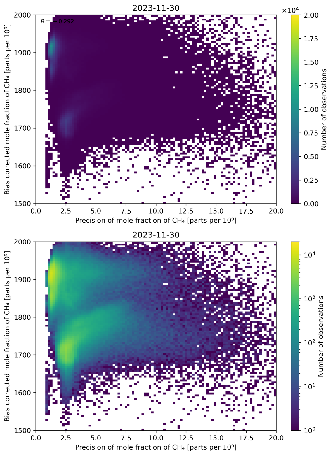
Figure 82: Scatter density plot of “Precision of mole fraction of CH 4 ” against “Bias corrected mole fraction of CH 4 ” for 2023-11-29 to 2023-12-01.
