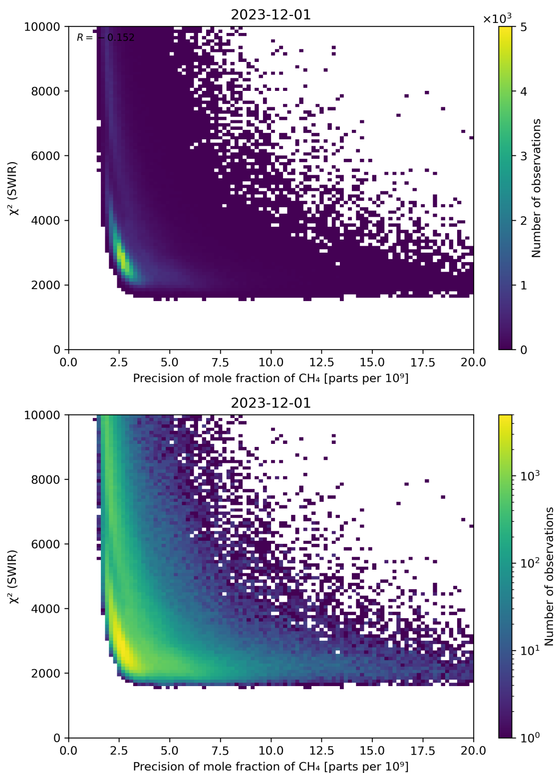
Figure 79: Scatter density plot of “Precision of mole fraction of \text{CH}_4 ” against “ \chi^2 (SWIR)” for 2023-11-30 to 2023-12-02.
