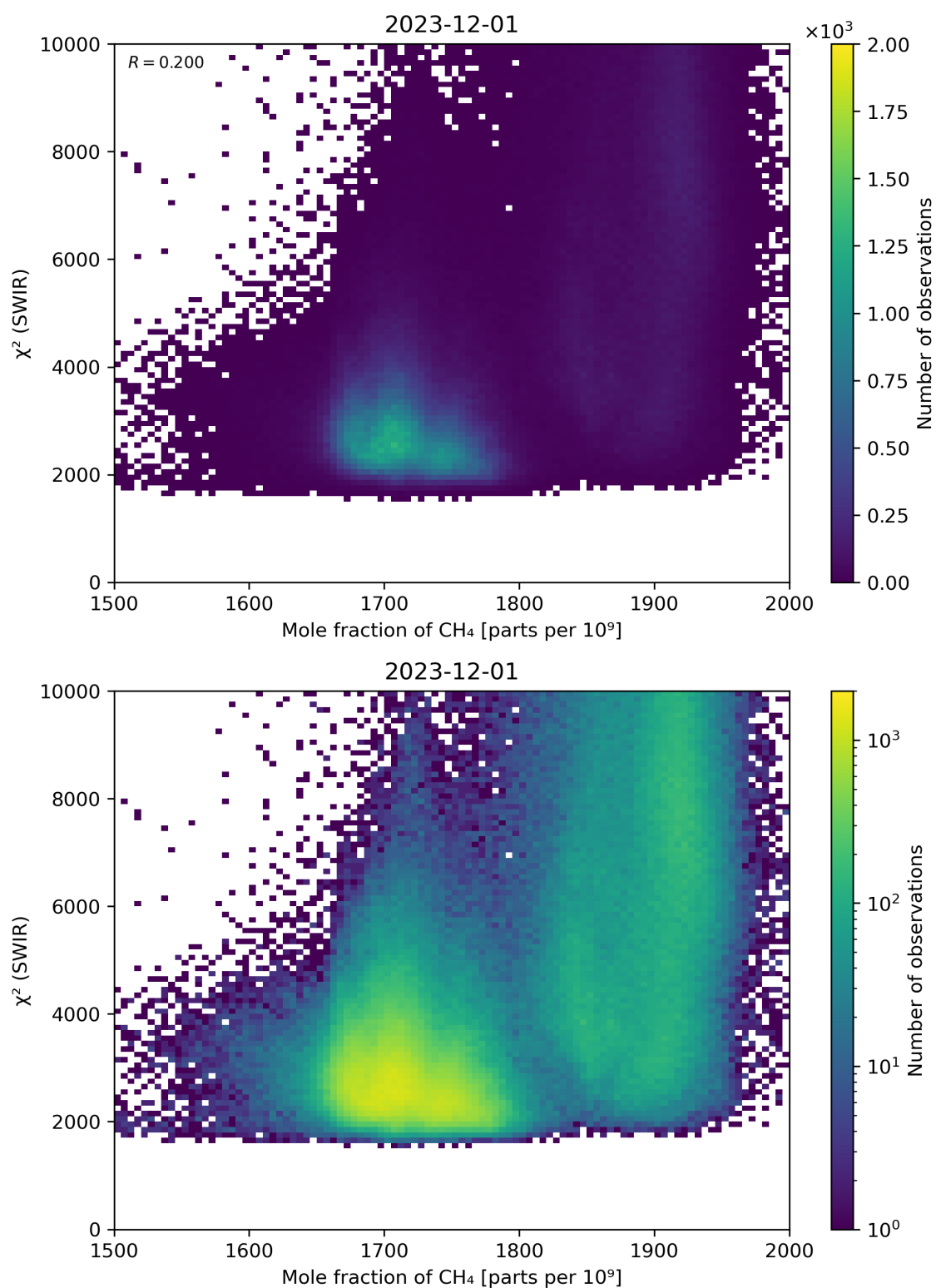
Figure 71: Scatter density plot of “Mole fraction of \text{CH}_4 ” against “ \chi^2 (SWIR)” for 2023-11-30 to 2023-12-02.
