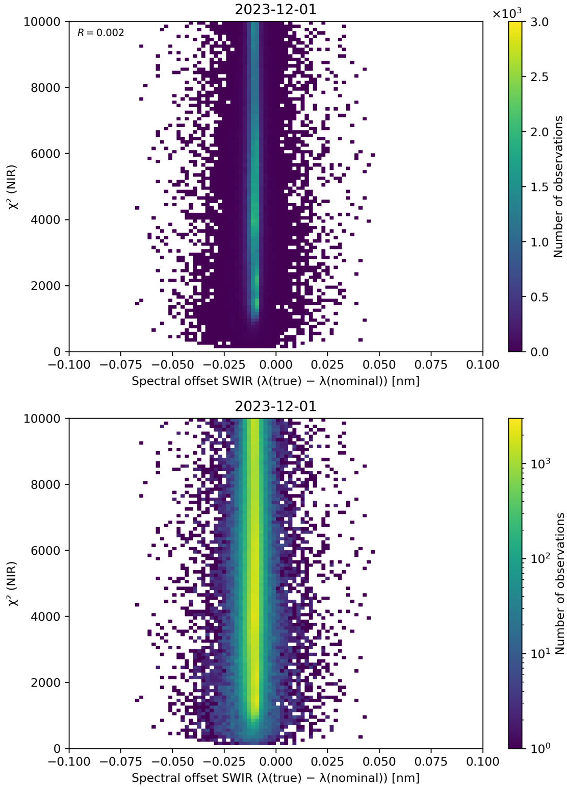
Figure 117: Scatter density plot of “Spectral offset SWIR ( \lambda(\text{true}) - \lambda(\text{nominal}) )” against “ \chi^2 (NIR)” for 2023-11-30 to 2023-12-02.
