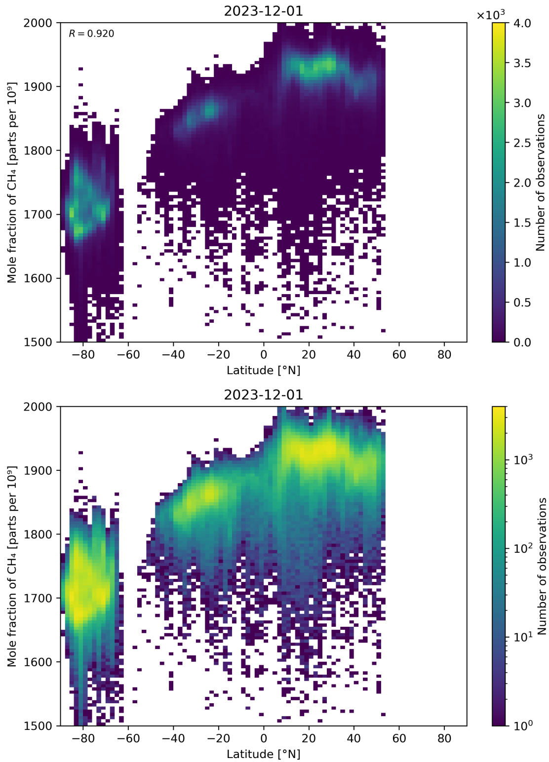
Figure 57: Scatter density plot of “Latitude” against “Mole fraction of CH 4 ” for 2023-11-30 to 2023-12-02.
