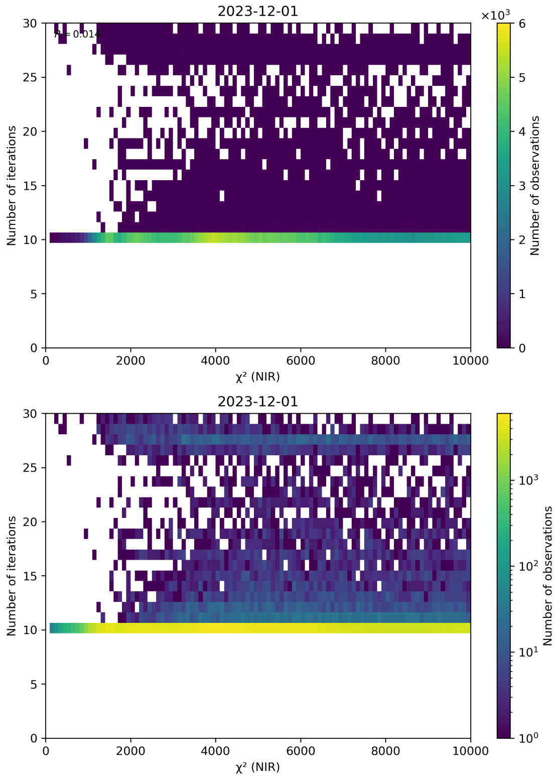
Figure 46: Scatter density plot of “ \chi^2 (NIR)” against “Number of iterations” for 2023-11-30 to 2023-12-02.
