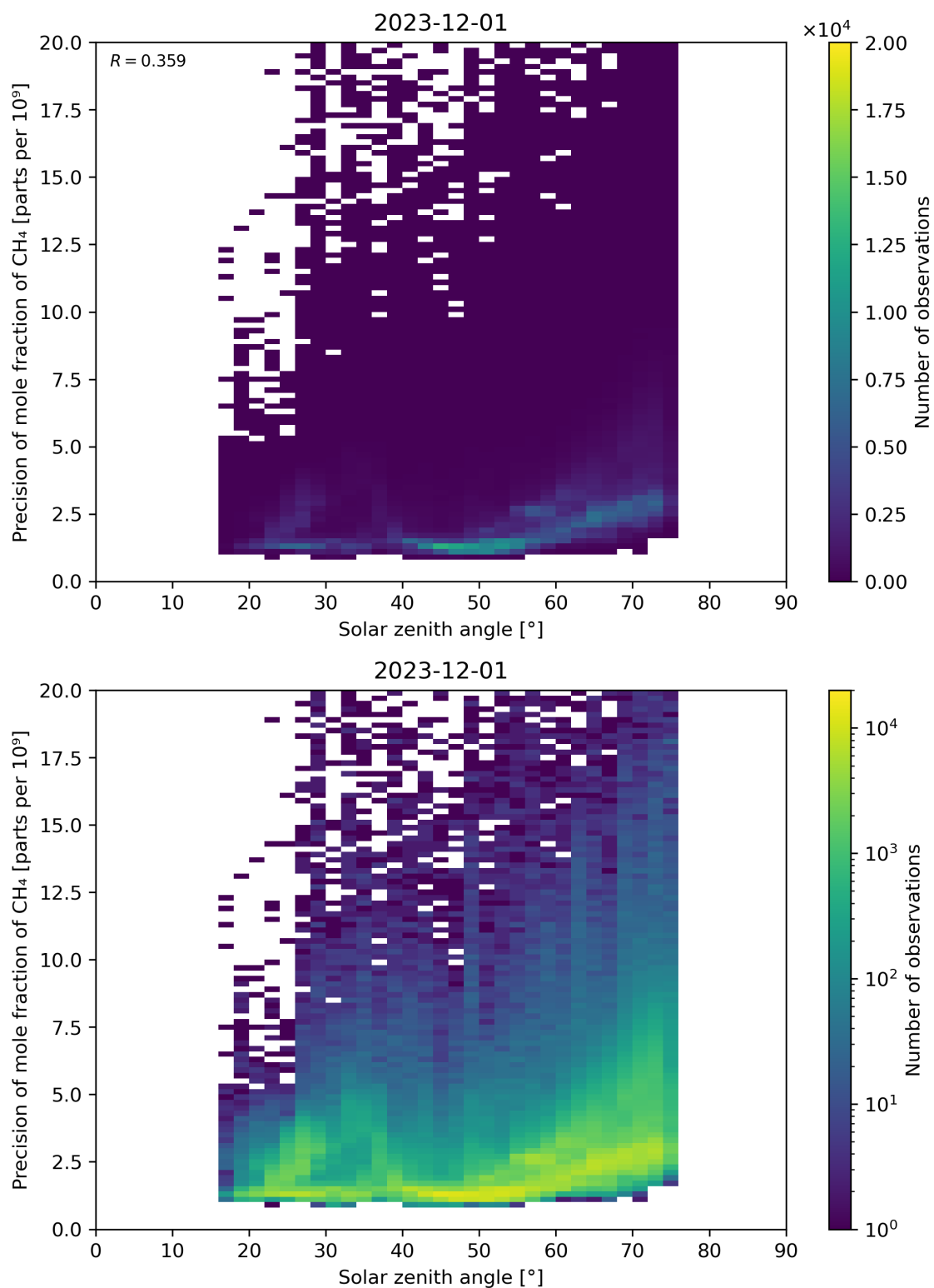
Figure 101: Scatter density plot of “Solar zenith angle” against “Precision of mole fraction of CH 4 ” for 2023-11-30 to 2023-12-02.
