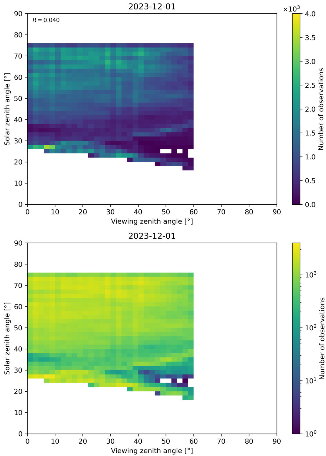
Figure 115: Scatter density plot of “Viewing zenith angle” against “Solar zenith angle” for 2023-11-30 to 2023-12-02.
