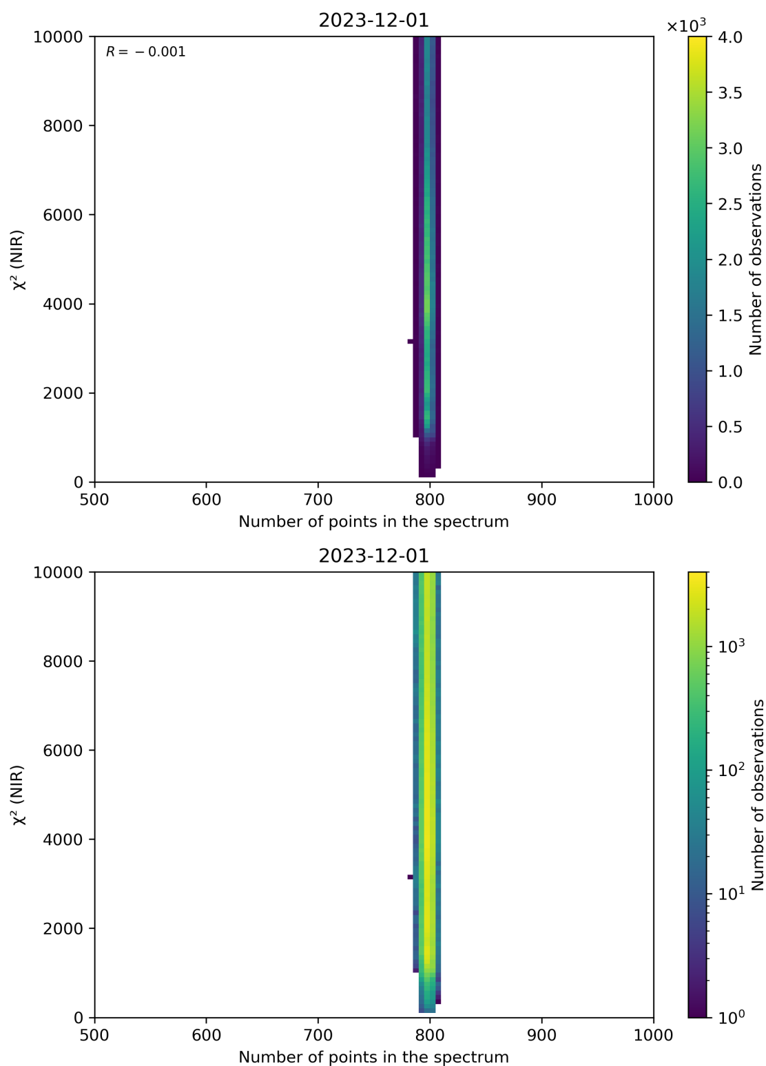
Figure 88: Scatter density plot of “Number of points in the spectrum” against “ \chi^2 (NIR)” for 2023-11-30 to 2023-12-02.
