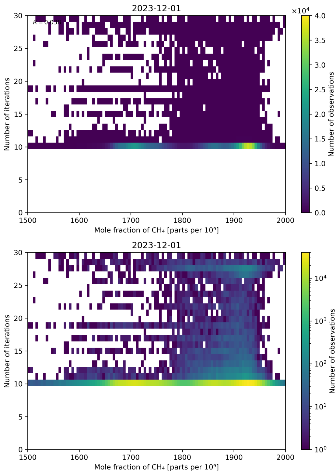
Figure 76: Scatter density plot of “Mole fraction of CH 4 ” against “Number of iterations” for 2023-11-30 to 2023-12-02.
