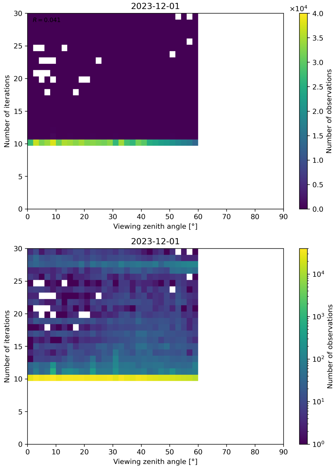
Figure 113: Scatter density plot of “Viewing zenith angle” against “Number of iterations” for 2023-11-30 to 2023-12-02.
