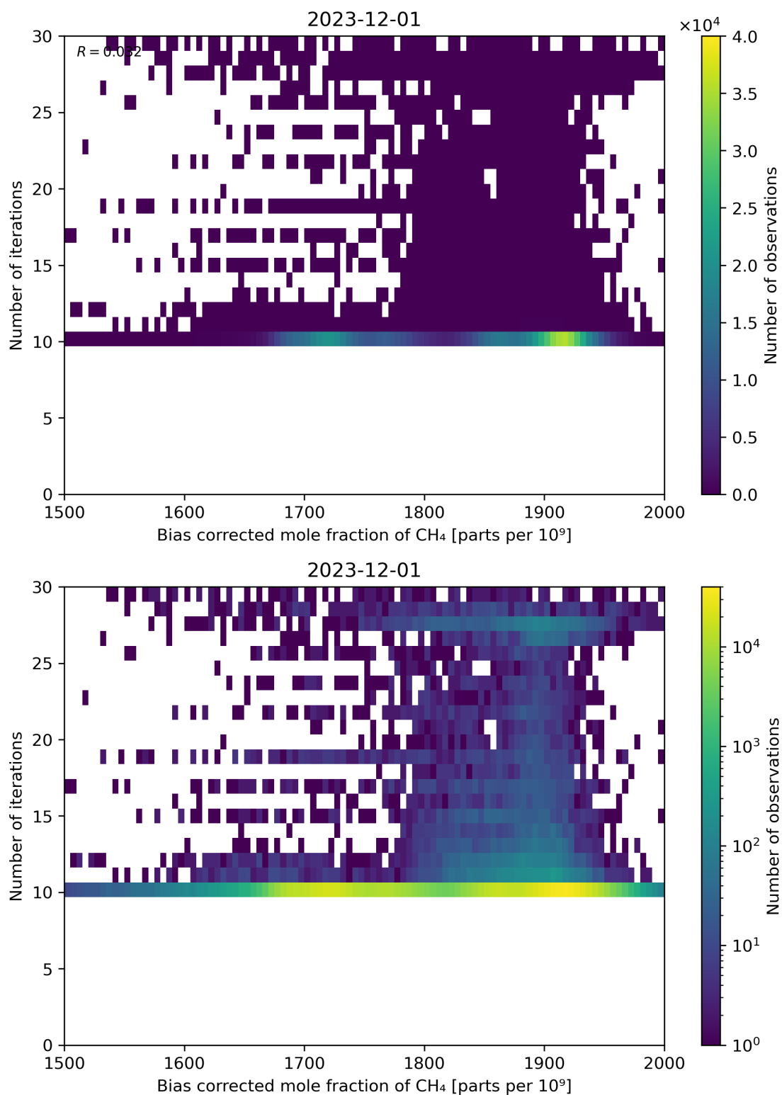
Figure 67: Scatter density plot of “Bias corrected mole fraction of \text{CH}_4 ” against “Number of iterations” for 2023-11-30 to 2023-12-02.
