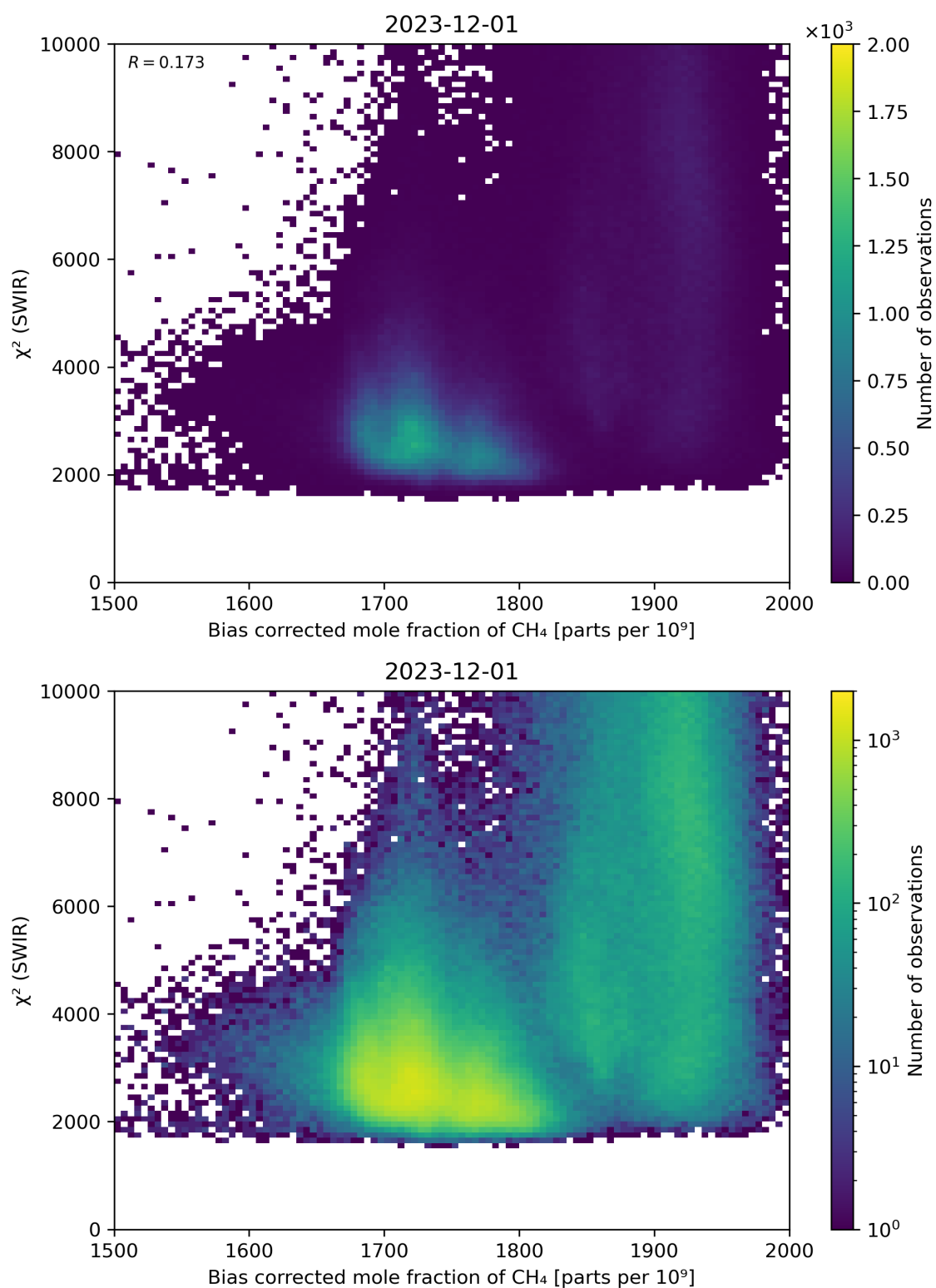
Figure 64: Scatter density plot of “Bias corrected mole fraction of CH 4 ” against “ \chi^2 (SWIR)” for 2023-11-30 to 2023-12-02.
