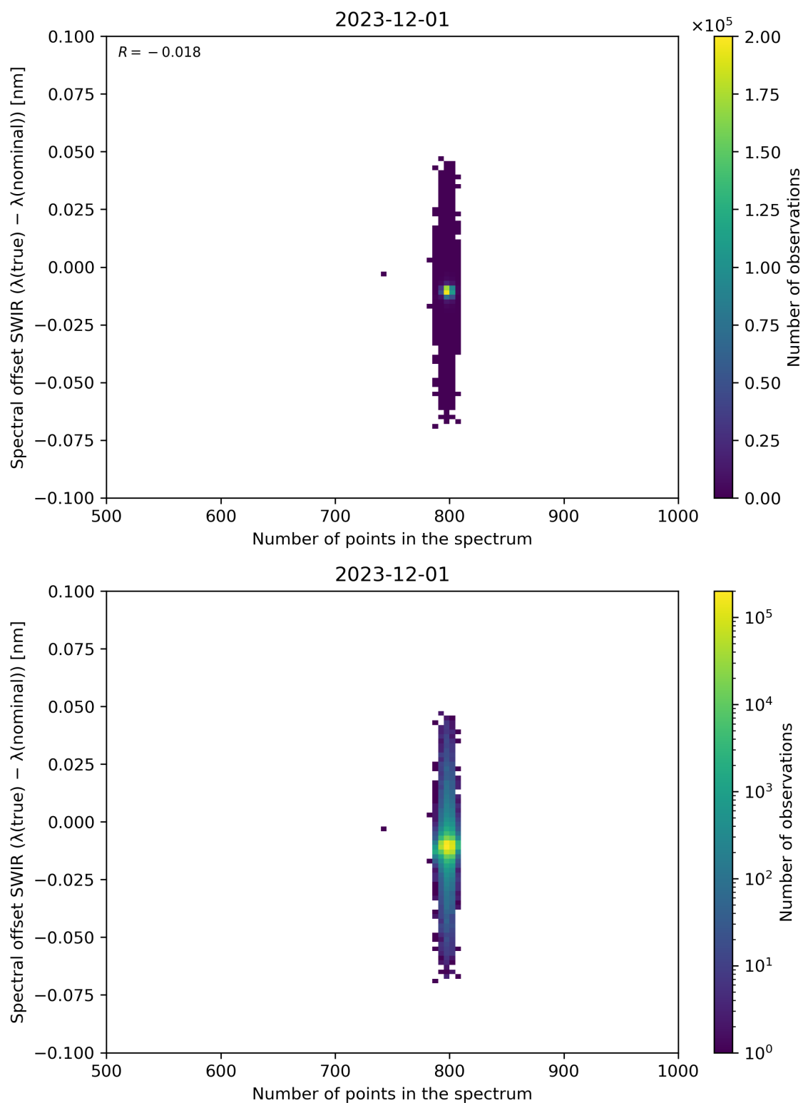
Figure 93: Scatter density plot of “Number of points in the spectrum” against “Spectral offset SWIR ( \lambda(\text{true}) - \lambda(\text{nominal}) )” for 2023-11-30 to 2023-12-02.
