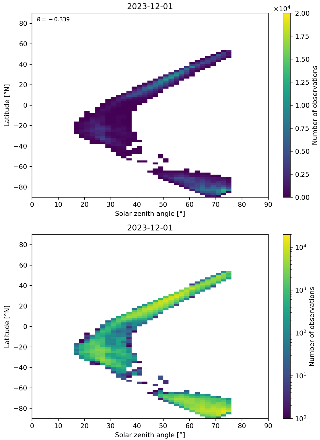
Figure 98: Scatter density plot of “Solar zenith angle” against “Latitude” for 2023-11-30 to 2023-12-02.
