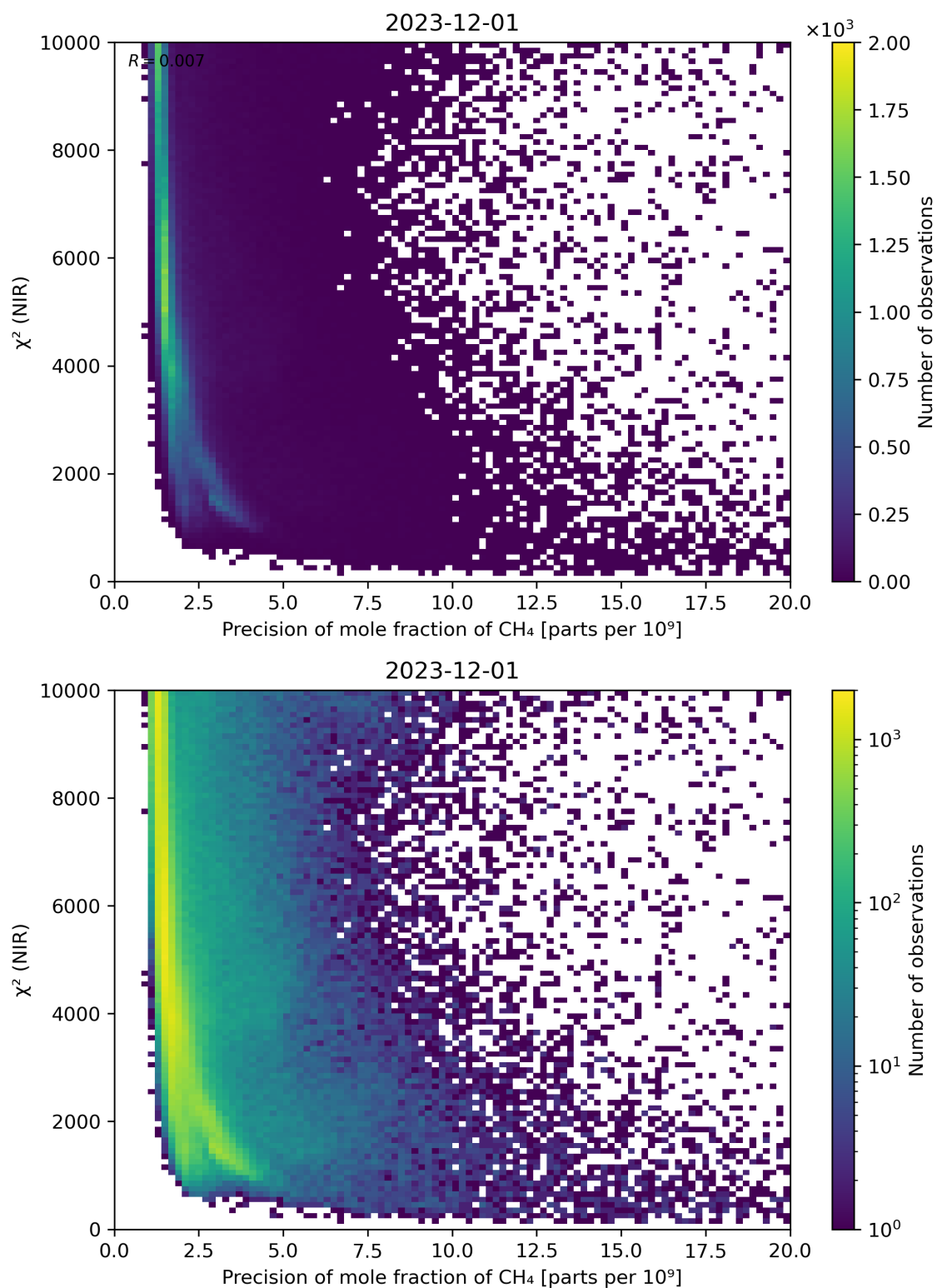
Figure 78: Scatter density plot of “Precision of mole fraction of \text{CH}_4 ” against “ \chi^2 (NIR)” for 2023-11-30 to 2023-12-02.
