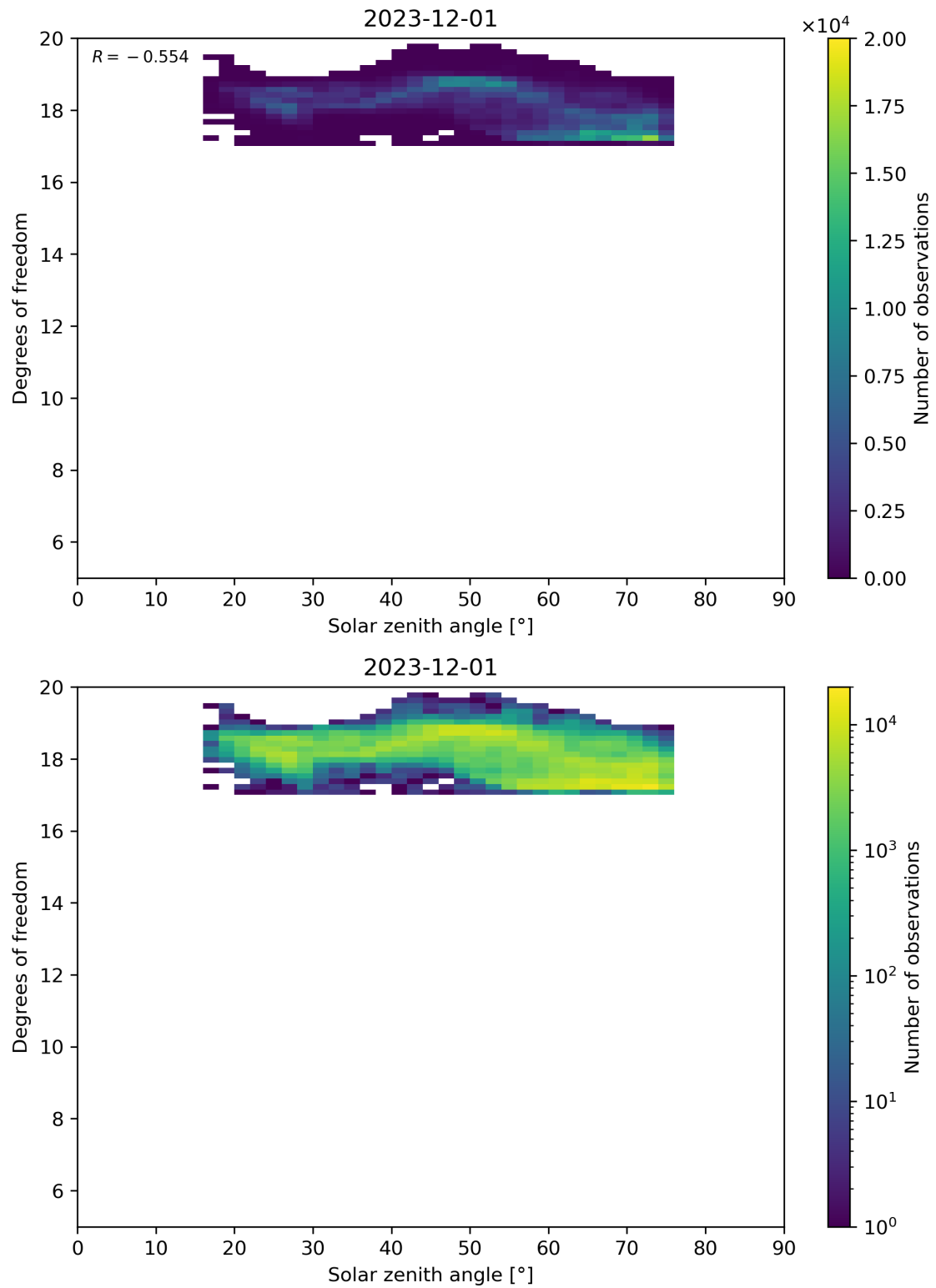
Figure 96: Scatter density plot of “Solar zenith angle” against “Degrees of freedom” for 2023-11-30 to 2023-12-02.
