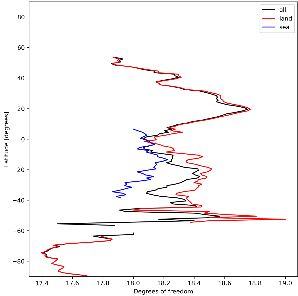
Figure 19: Zonal average of “Degrees of freedom” for 2023-11-30 to 2023-12-02.
