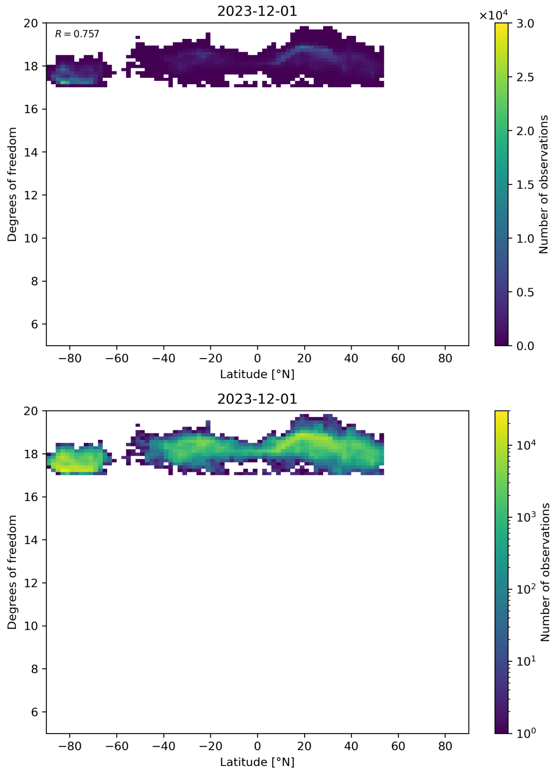
Figure 55: Scatter density plot of “Latitude” against “Degrees of freedom” for 2023-11-30 to 2023-12-02.
