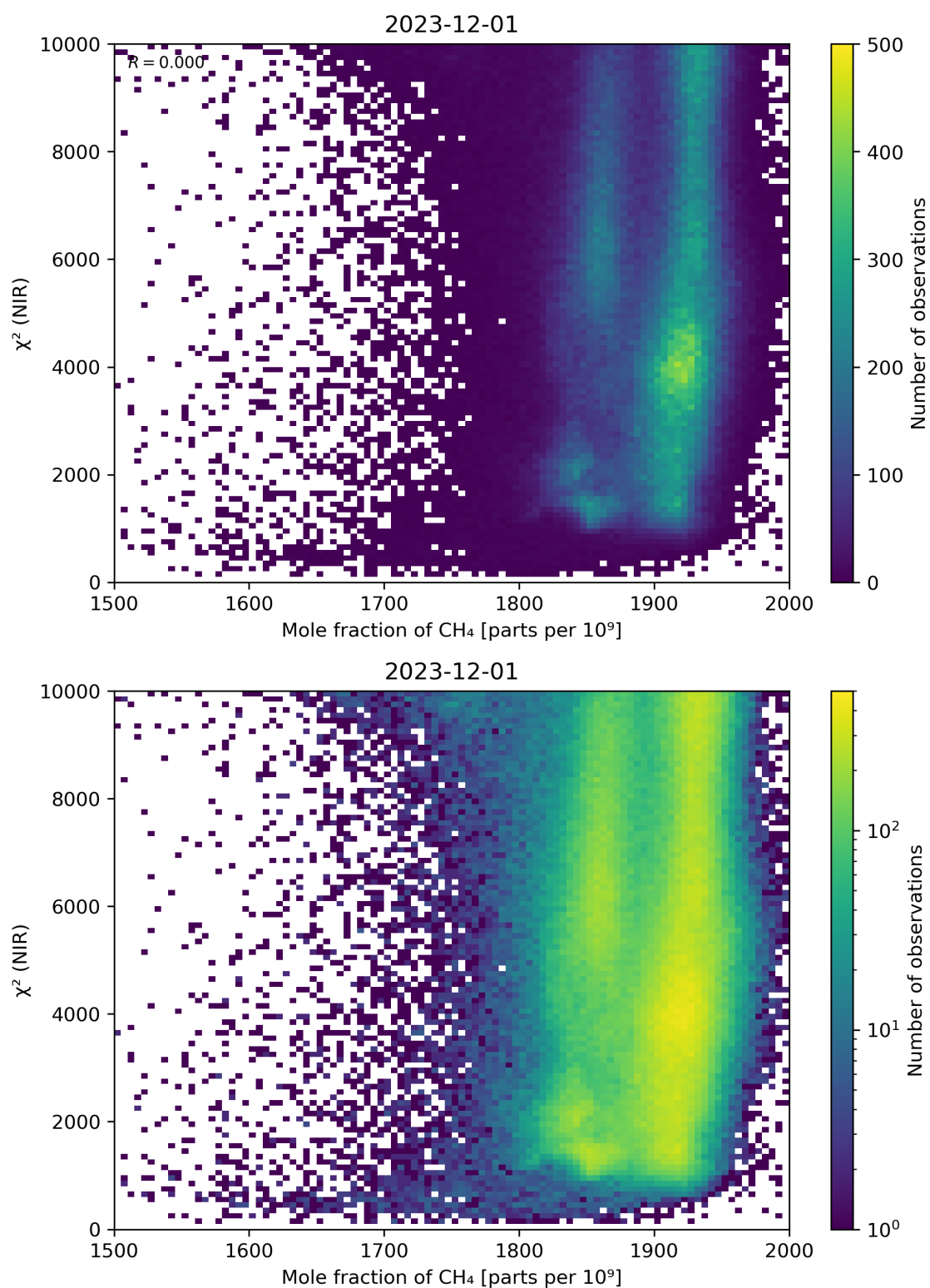
Figure 70: Scatter density plot of “Mole fraction of \text{CH}_4 ” against “ \chi^2 (NIR)” for 2023-11-30 to 2023-12-02.
