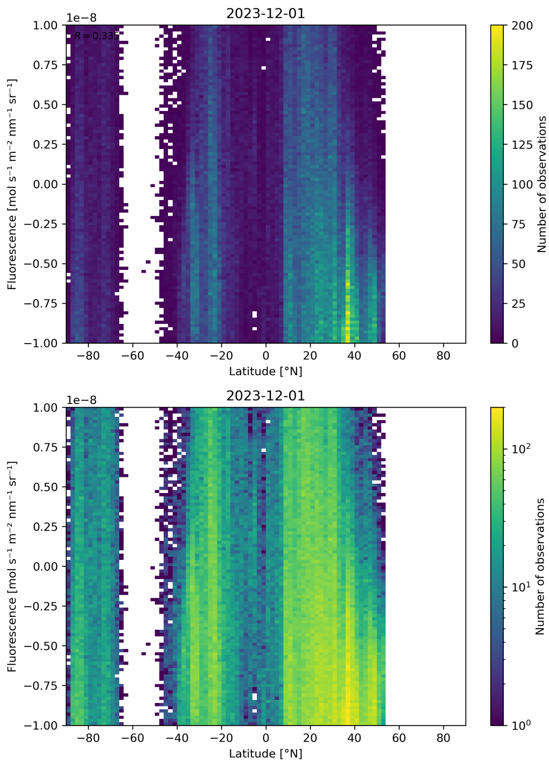
Figure 56: Scatter density plot of “Latitude” against “Fluorescence” for 2023-11-30 to 2023-12-02.
