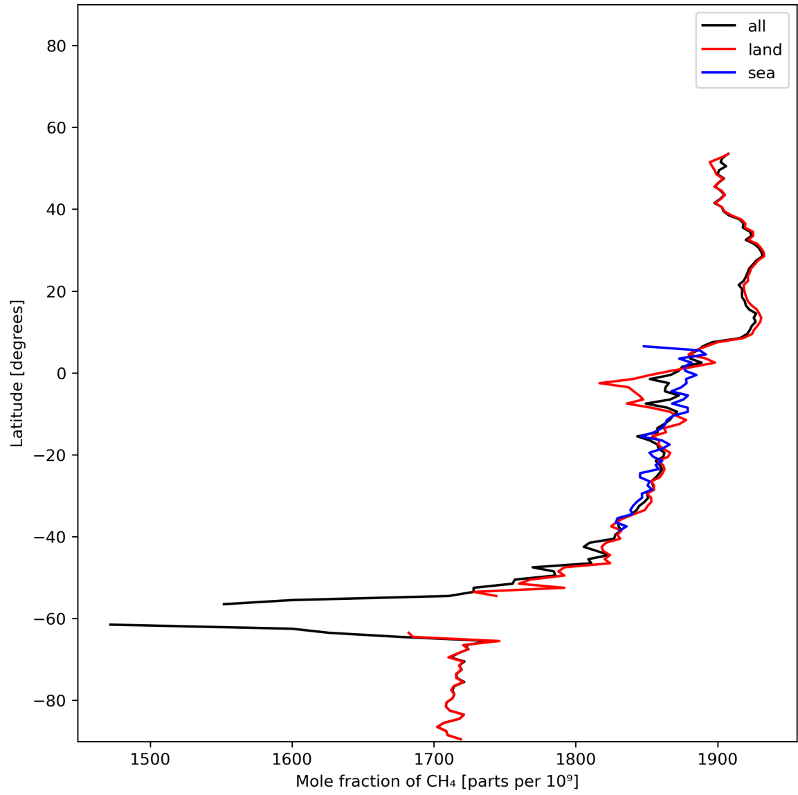
Figure 12: Zonal average of “Mole fraction of CH 4 ” for 2023-11-30 to 2023-12-02.
