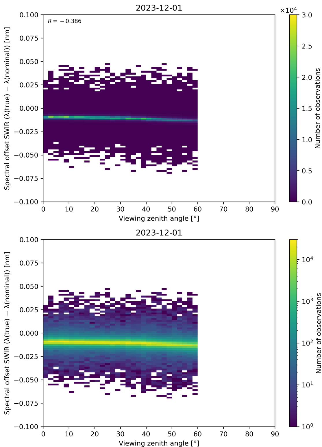
Figure 116: Scatter density plot of “Viewing zenith angle” against “Spectral offset SWIR ( \lambda(\text{true}) - \lambda(\text{nominal}) )” for 2023-11-30 to 2023-12-02.
