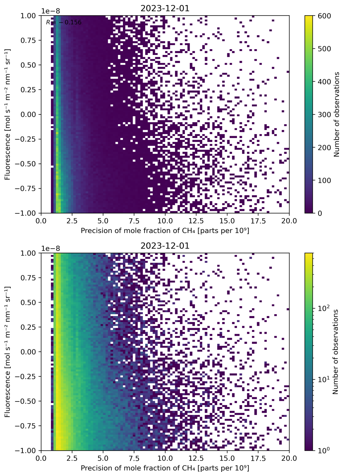
Figure 81: Scatter density plot of “Precision of mole fraction of \text{CH}_4 ” against “Fluorescence” for 2023-11-30 to 2023-12-02.
