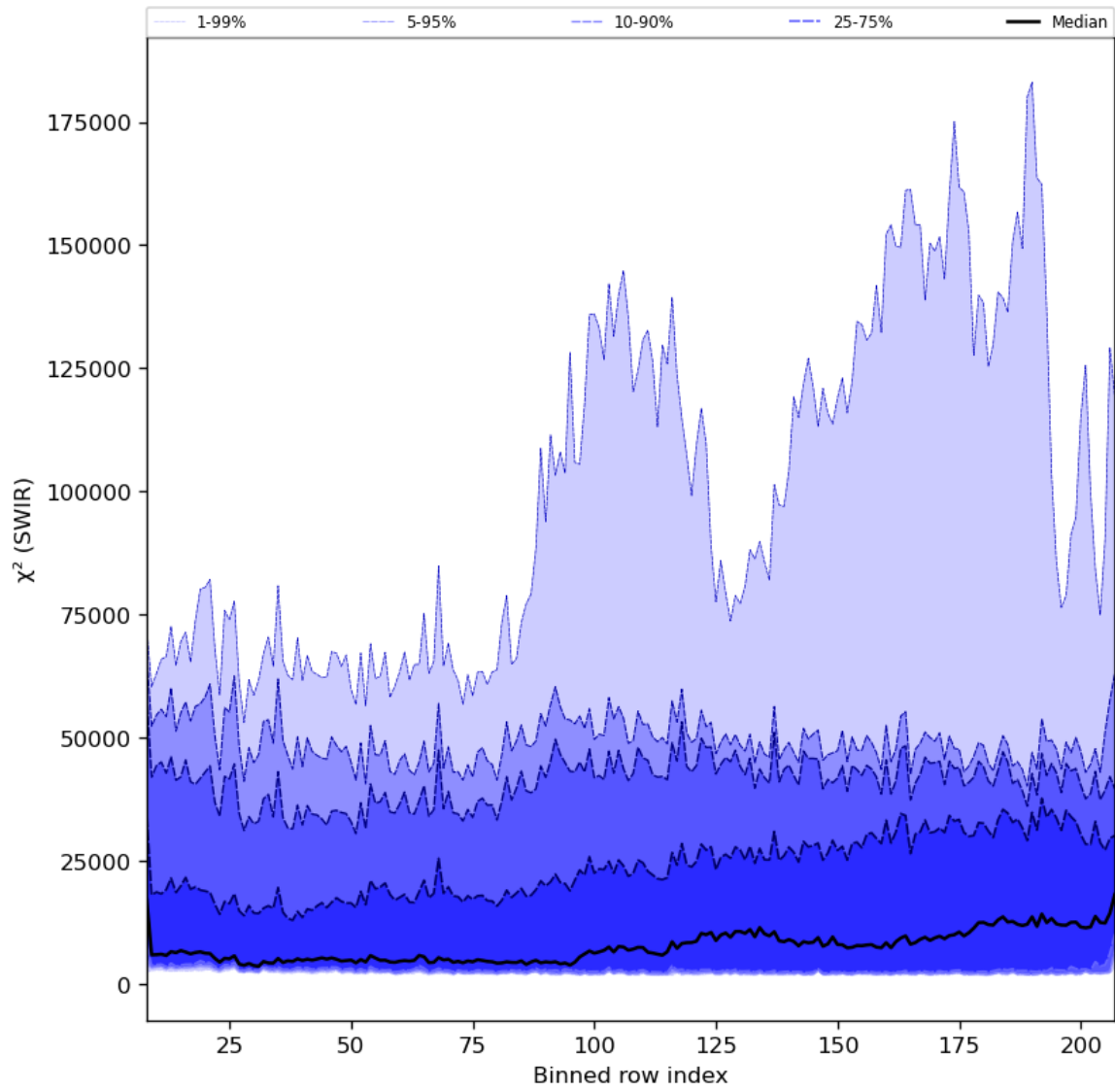
Figure 39: Along track statistics of “ \chi^2 (SWIR)” for 2023-11-30 to 2023-12-02
