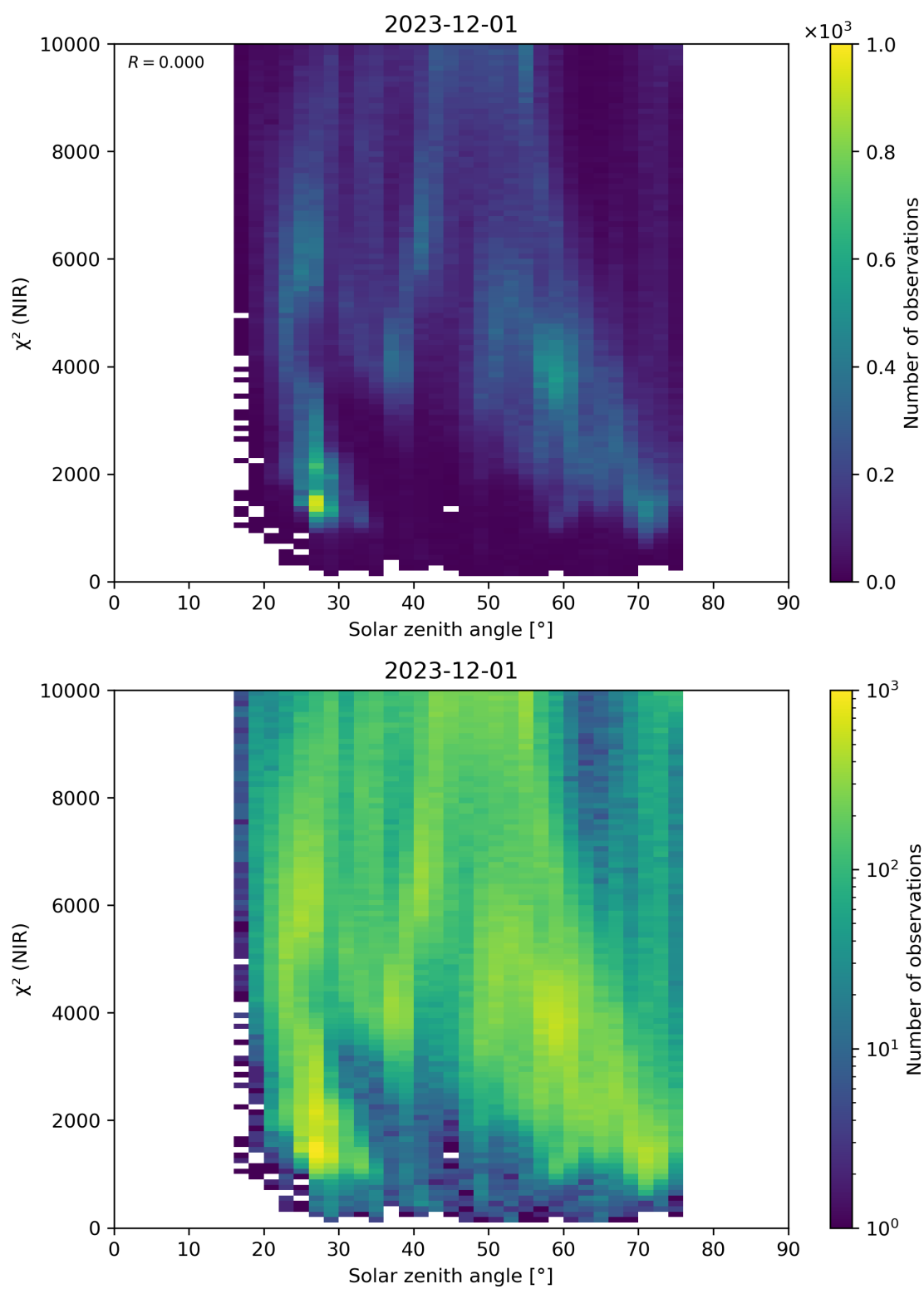
Figure 94: Scatter density plot of “Solar zenith angle” against “ \chi^2 (NIR)” for 2023-11-30 to 2023-12-02.
