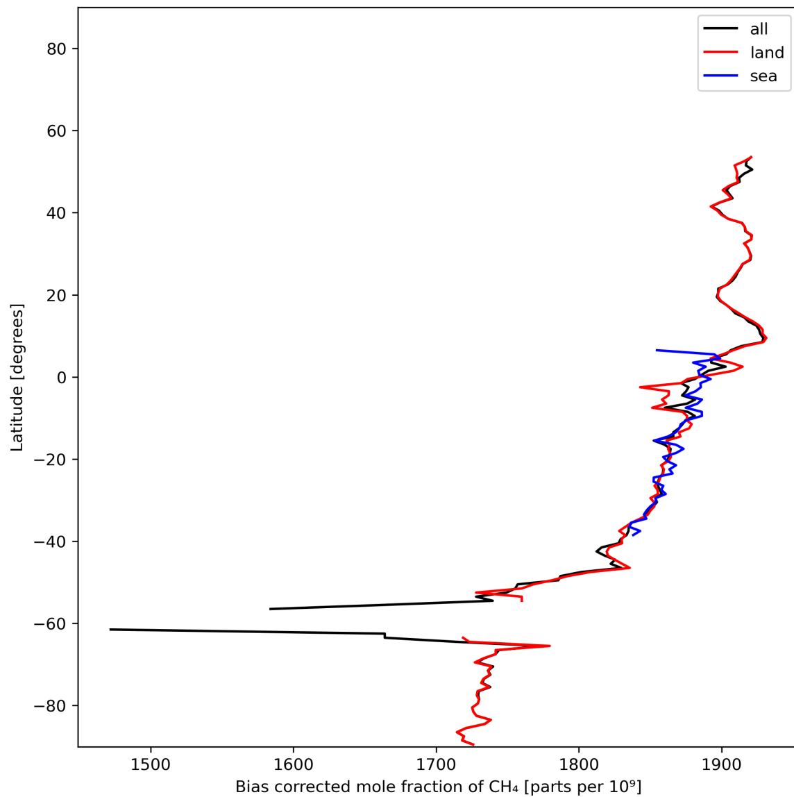
Figure 14: Zonal average of “Bias corrected mole fraction of CH 4 ” for 2023-11-30 to 2023-12-02.
