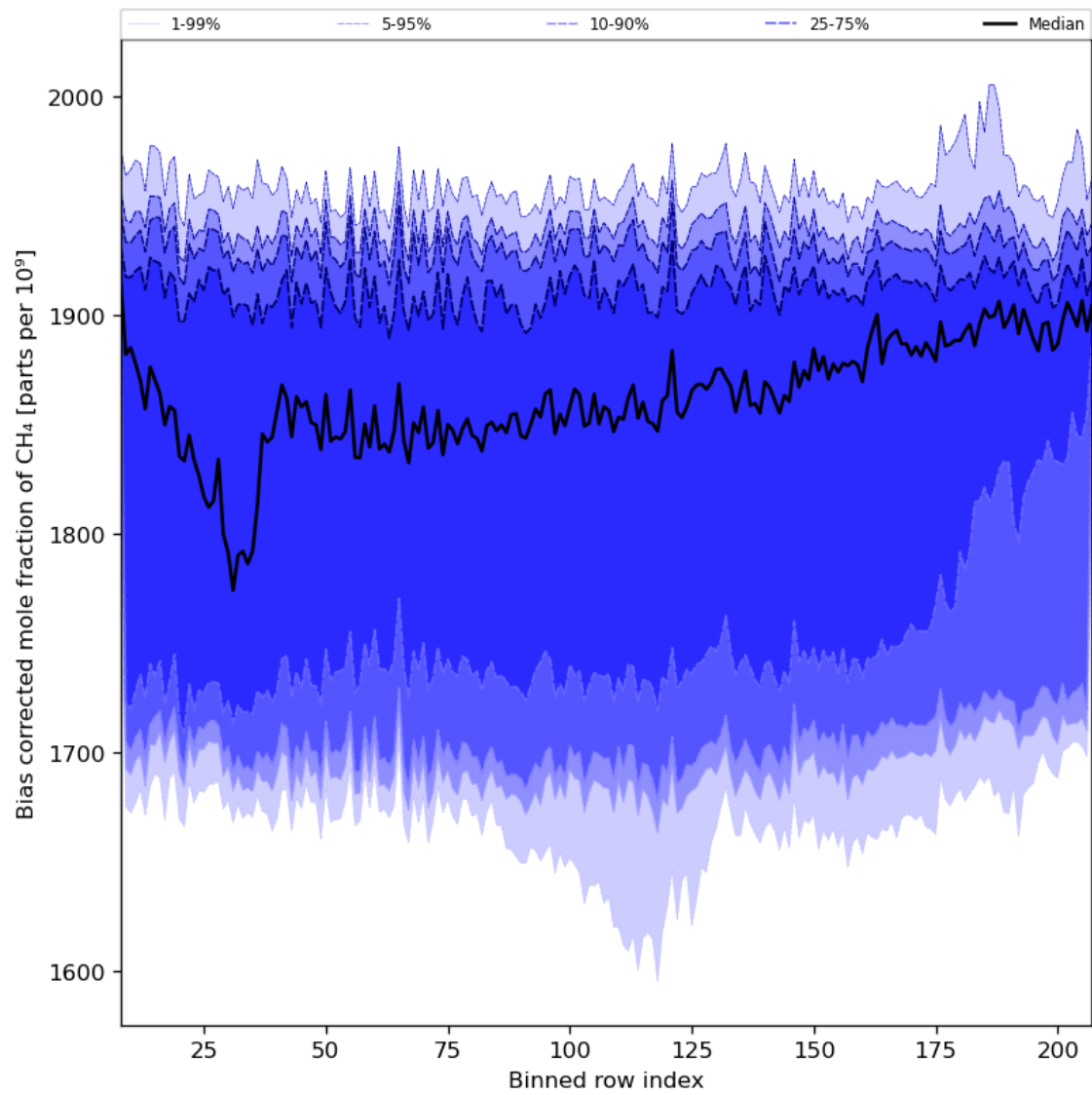
Figure 36: Along track statistics of “Bias corrected mole fraction of CH 4 ” for 2023-11-30 to 2023-12-02
