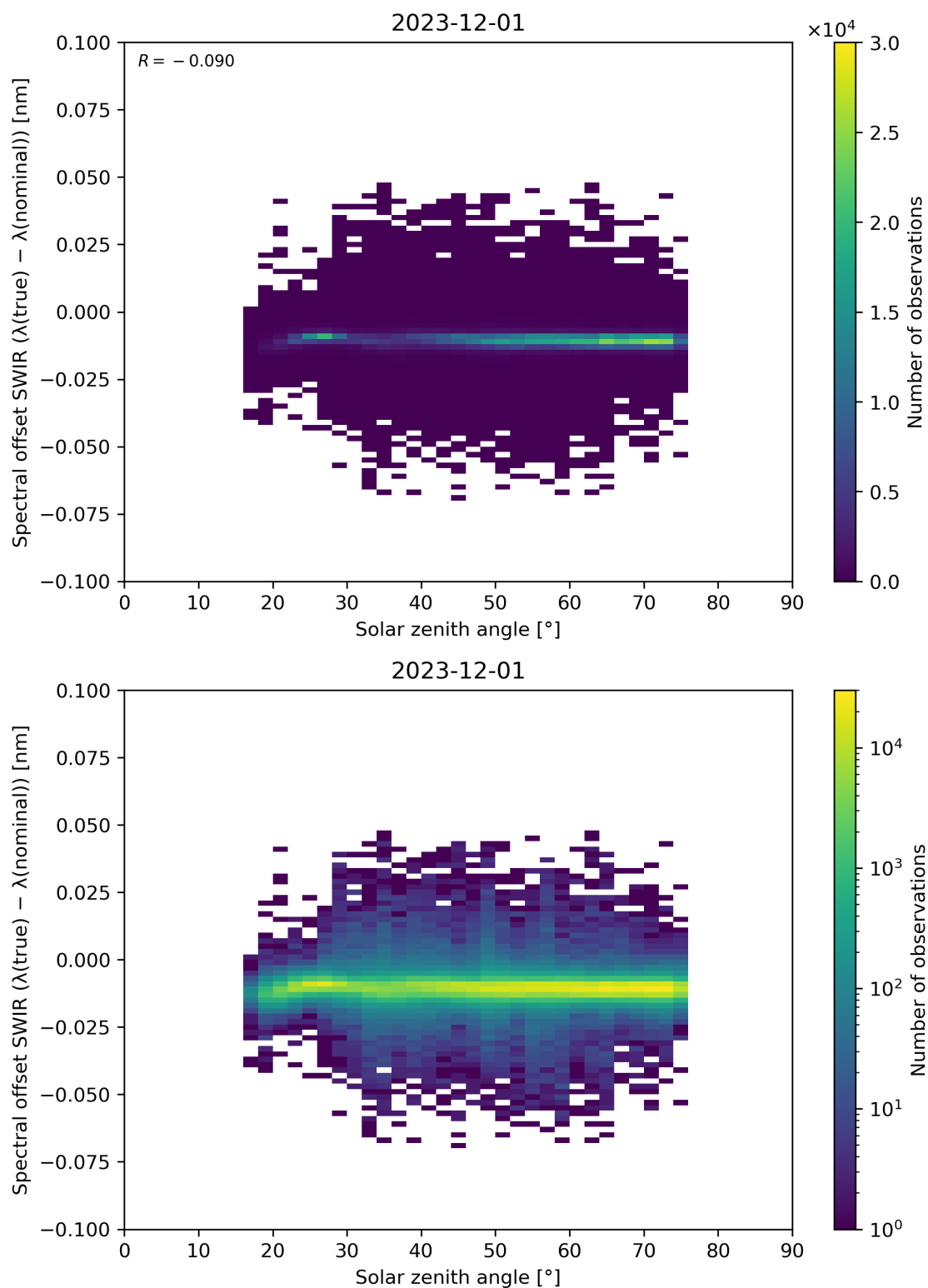
Figure 104: Scatter density plot of “Solar zenith angle” against “Spectral offset SWIR ( \lambda(\text{true}) - \lambda(\text{nominal}) )” for 2023-11-30 to 2023-12-02.
