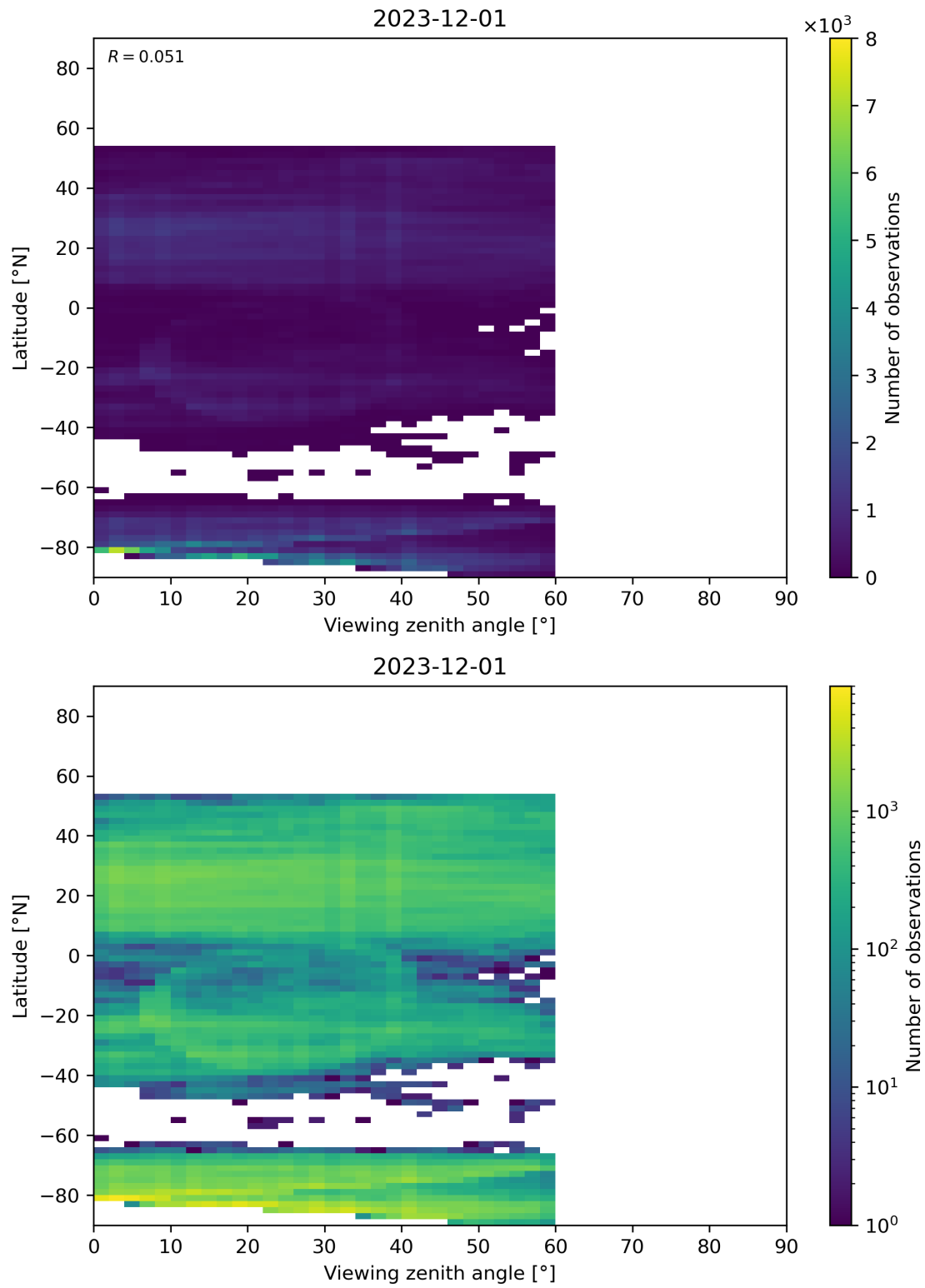
Figure 109: Scatter density plot of “Viewing zenith angle” against “Latitude” for 2023-11-30 to 2023-12-02.
