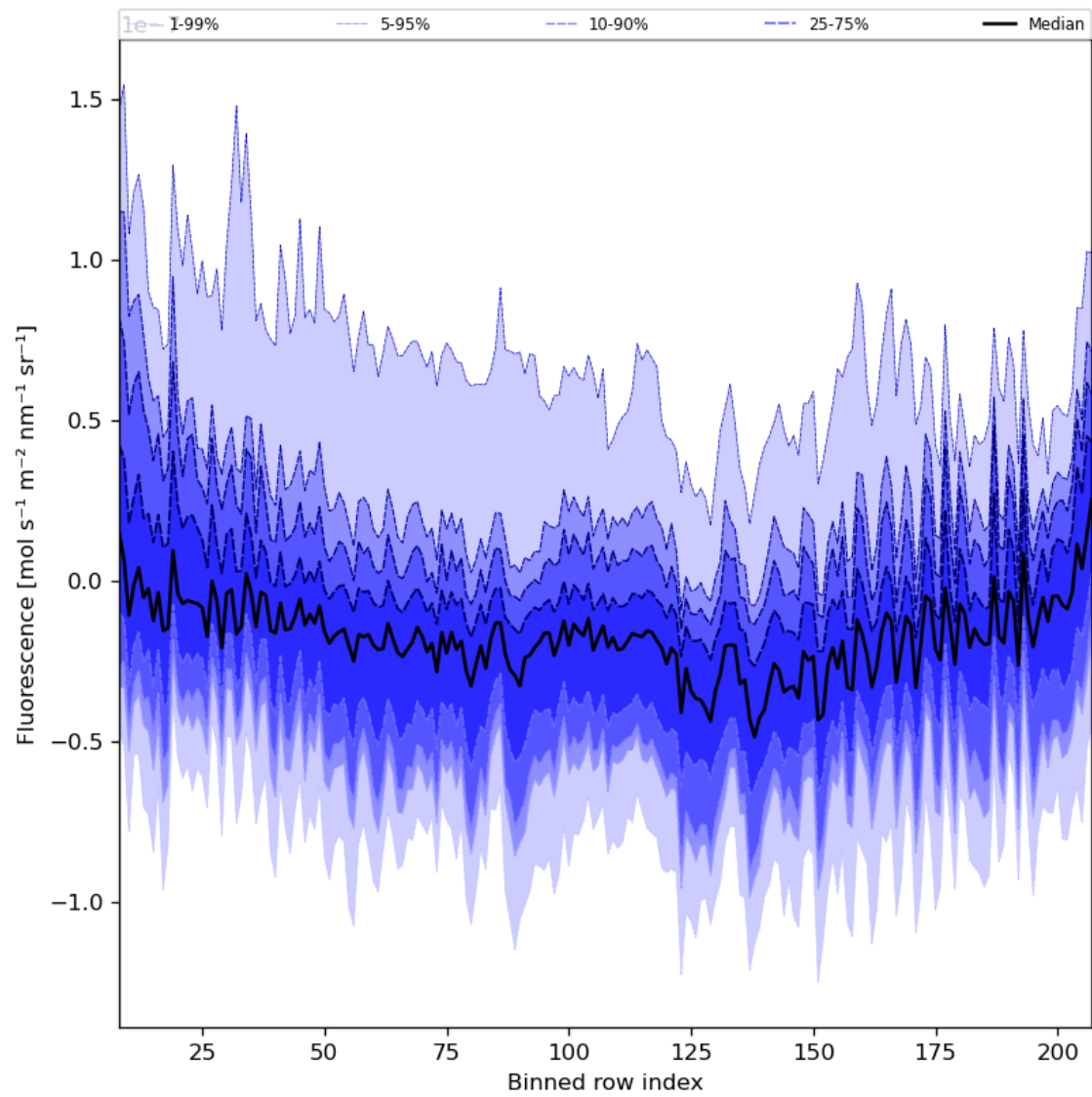
Figure 43: Along track statistics of “Fluorescence” for 2023-11-30 to 2023-12-02
