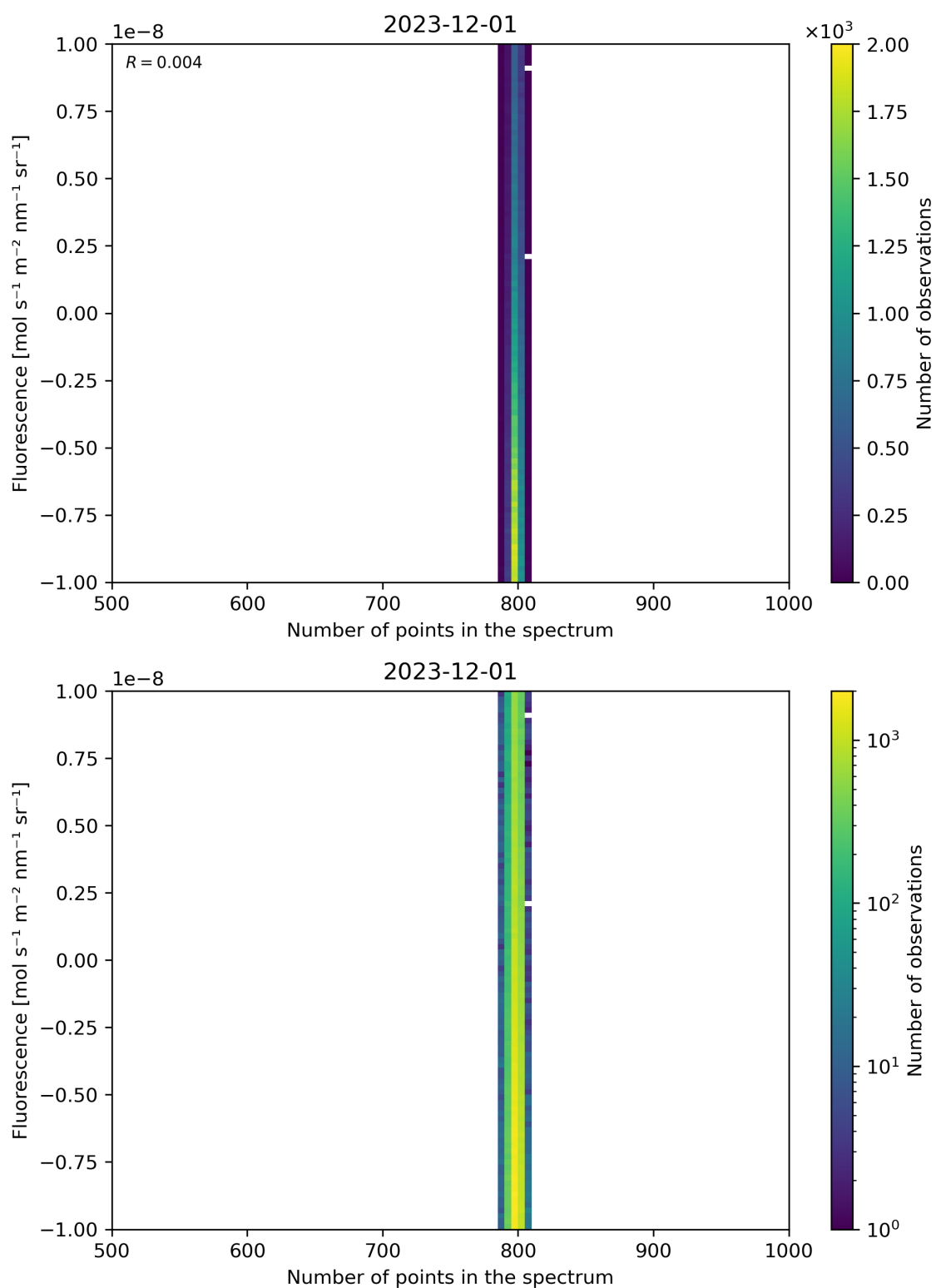
Figure 91: Scatter density plot of “Number of points in the spectrum” against “Fluorescence” for 2023-11-30 to 2023-12-02.
