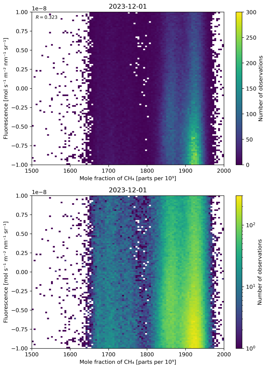
Figure 73: Scatter density plot of “Mole fraction of \text{CH}_4 ” against “Fluorescence” for 2023-11-30 to 2023-12-02.
