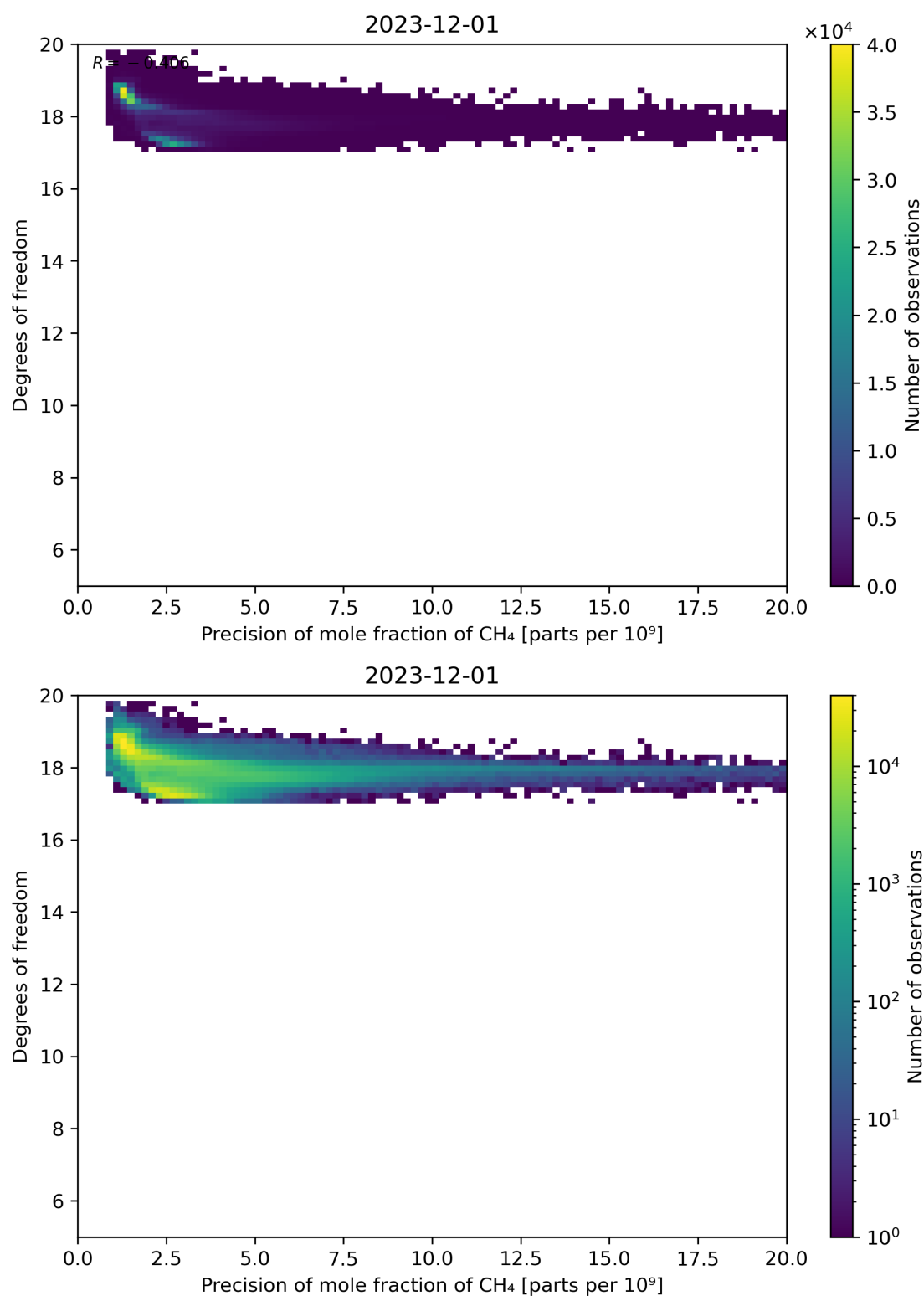
Figure 80: Scatter density plot of “Precision of mole fraction of CH 4 ” against “Degrees of freedom” for 2023-11-30 to 2023-12-02.
