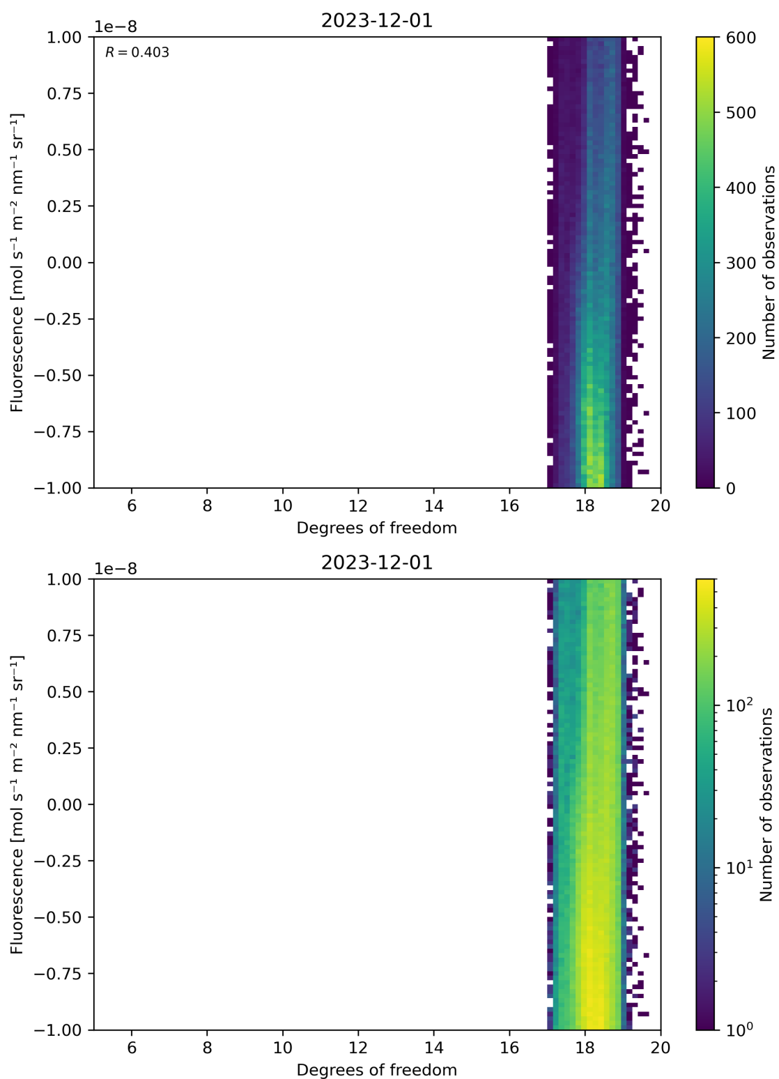
Figure 51: Scatter density plot of “Degrees of freedom” against “Fluorescence” for 2023-11-30 to 2023-12-02.
