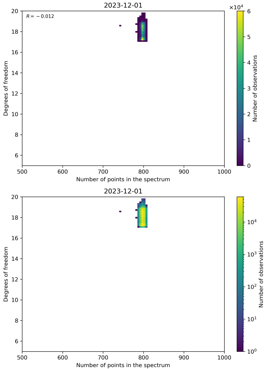
Figure 90: Scatter density plot of “Number of points in the spectrum” against “Degrees of freedom” for 2023-11-30 to 2023-12-02.
