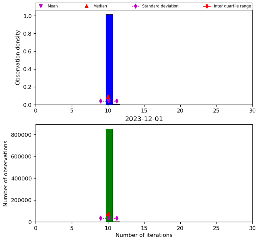
Figure 31: Histogram of “Number of iterations” for 2023-11-30 to 2023-12-02
