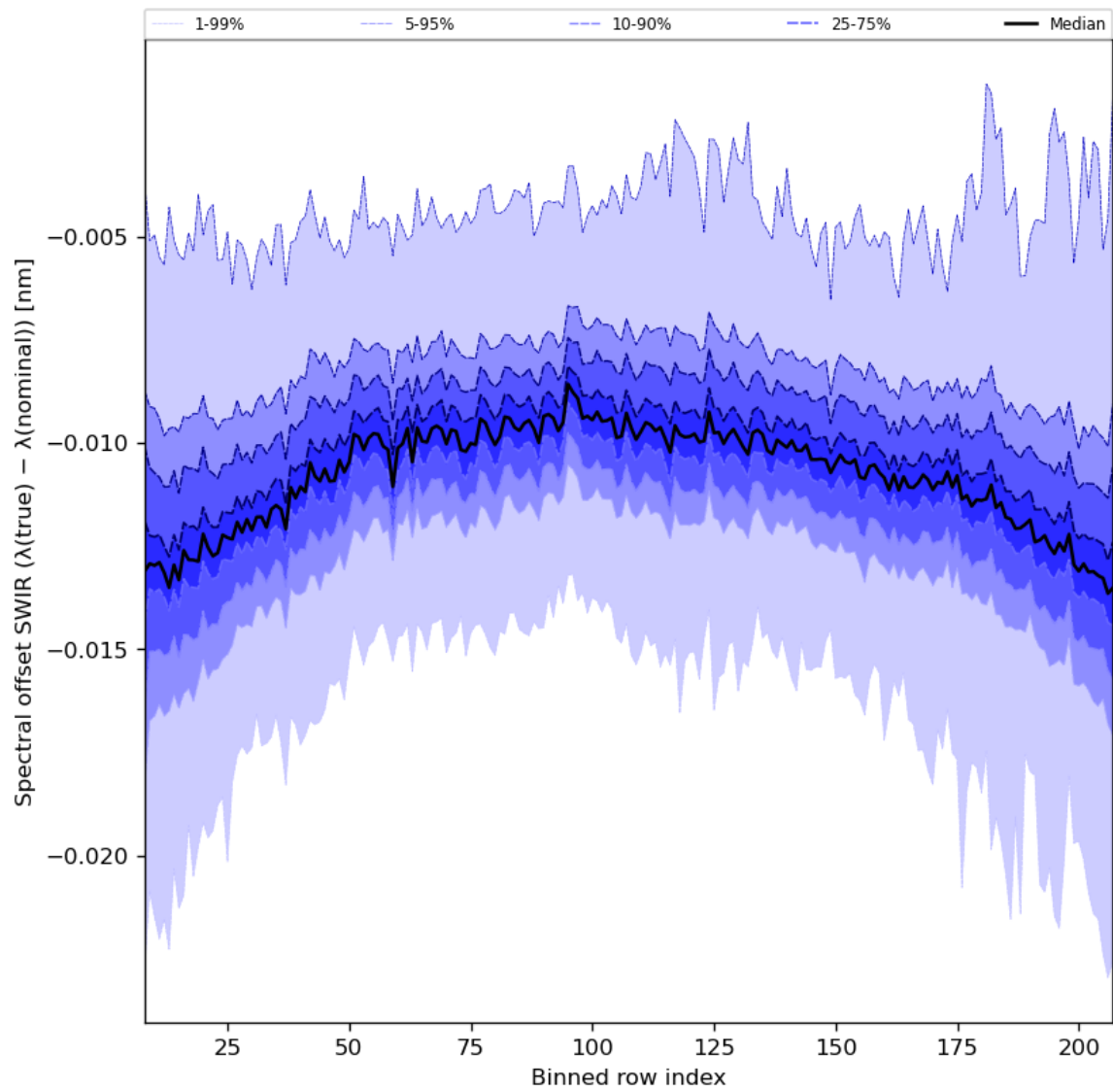
Figure 38: Along track statistics of “Spectral offset SWIR ( \lambda(\text{true}) - \lambda(\text{nominal}) )” for 2023-11-30 to 2023-12-02
