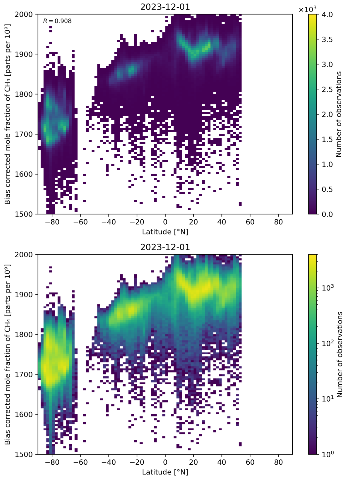
Figure 58: Scatter density plot of “Latitude” against “Bias corrected mole fraction of \text{CH}_4 ” for 2023-11-30 to 2023-12-02.
