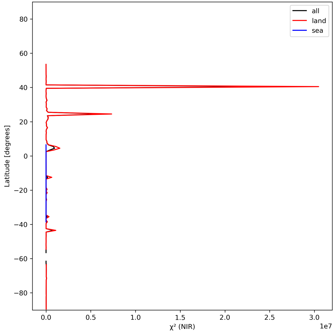
Figure 18: Zonal average of “ \chi^2 (NIR)” for 2023-11-30 to 2023-12-02.
