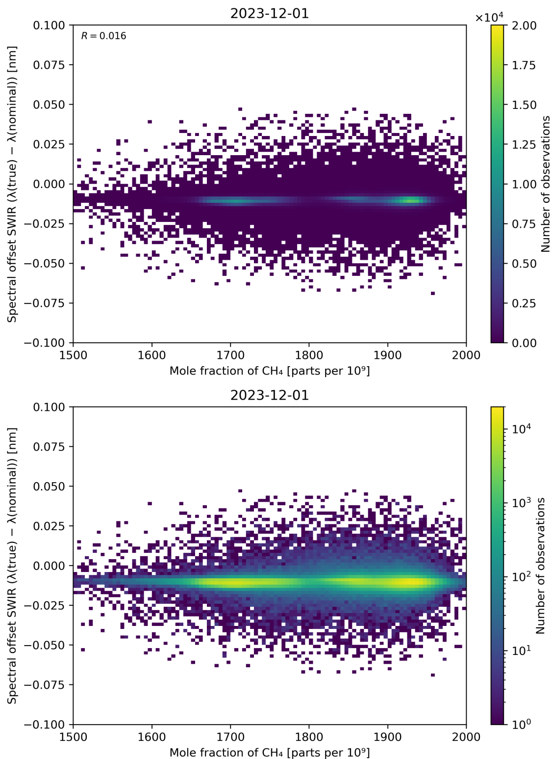
Figure 86: Scatter density plot of “Mole fraction of CH 4 ” against “Spectral offset SWIR ( \lambda(\text{true}) - \lambda(\text{nominal}) )” for 2023-11-30 to 2023-12-02.
