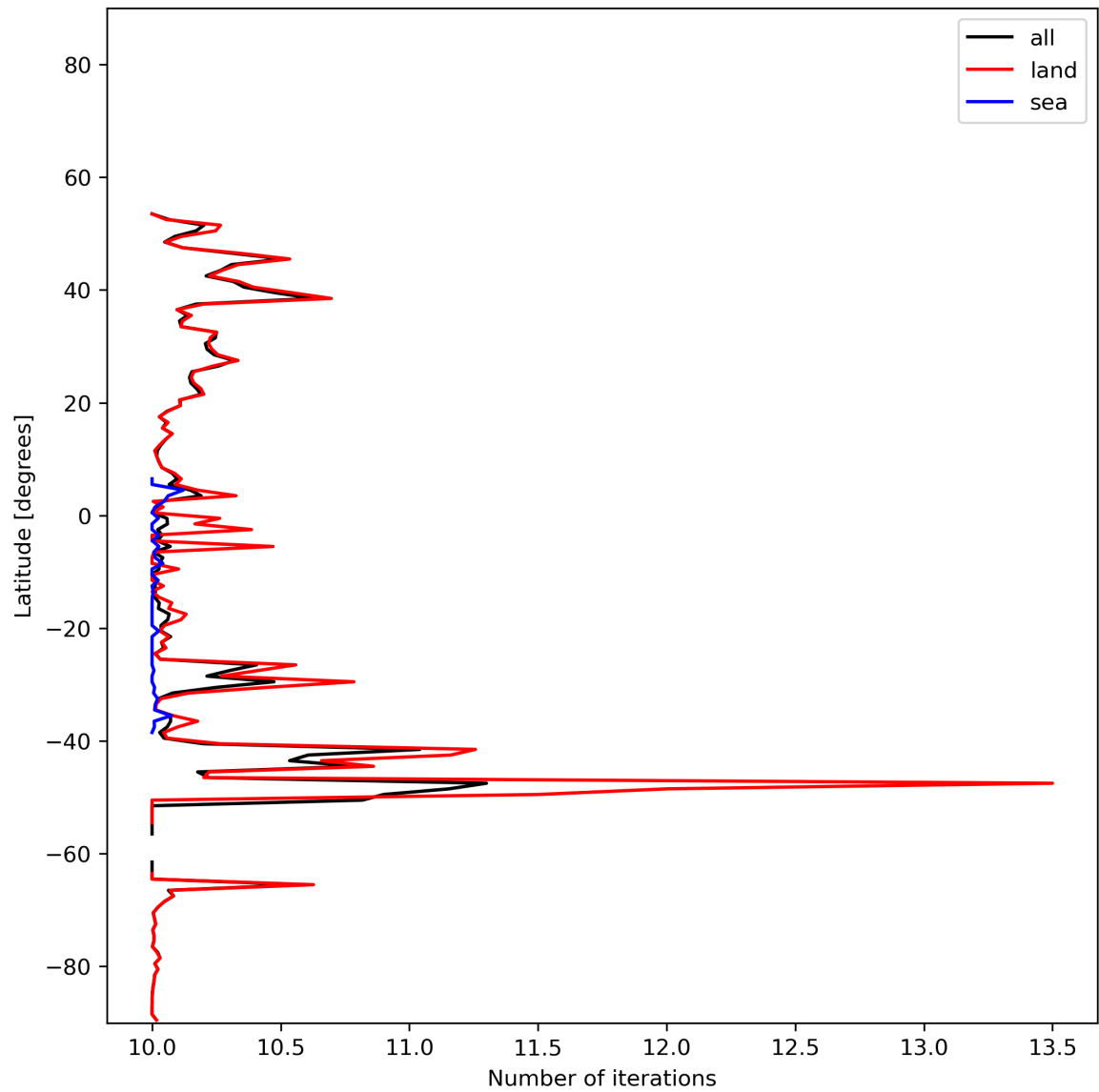
Figure 20: Zonal average of “Number of iterations” for 2023-11-30 to 2023-12-02.
