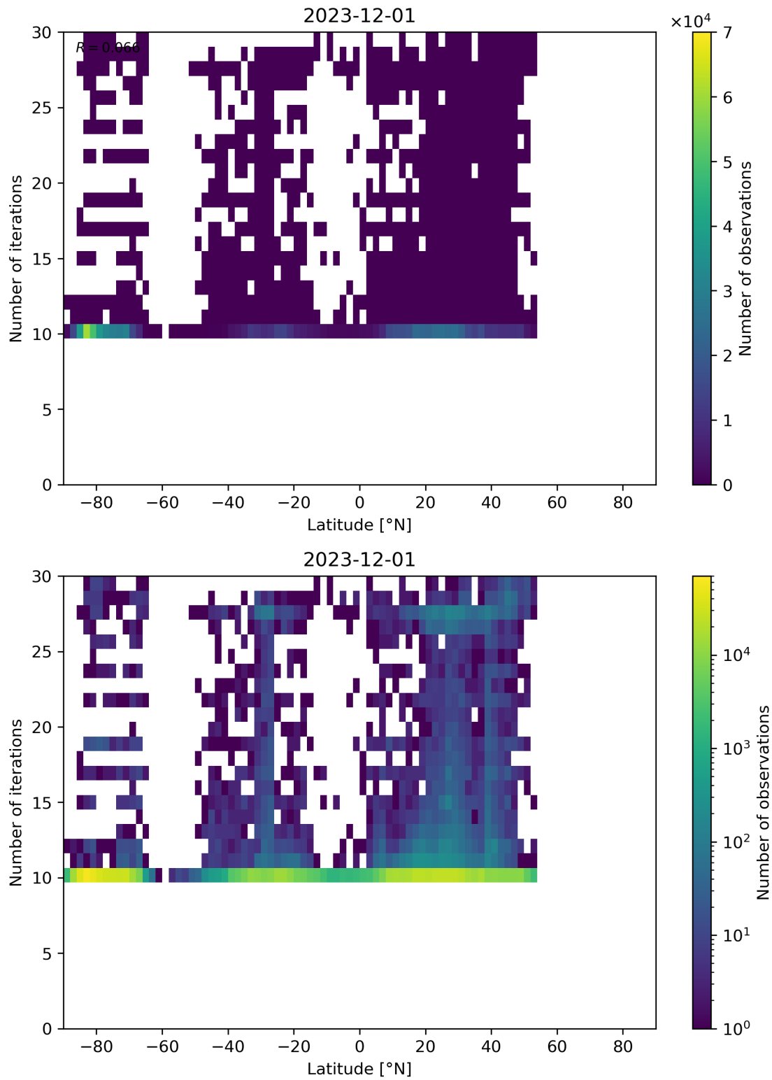
Figure 60: Scatter density plot of “Latitude” against “Number of iterations” for 2023-11-30 to 2023-12-02.
