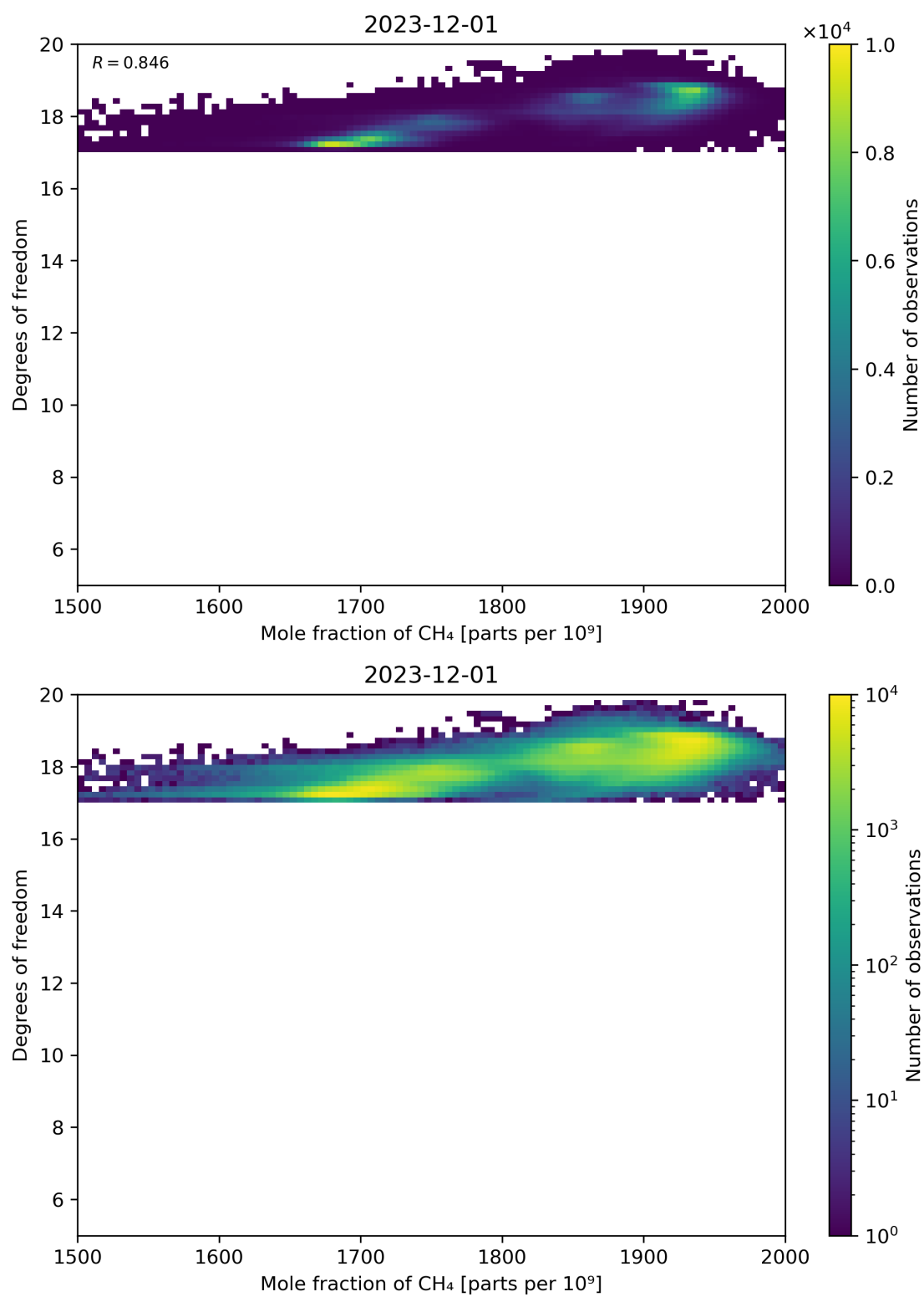
Figure 72: Scatter density plot of “Mole fraction of CH 4 ” against “Degrees of freedom” for 2023-11-30 to 2023-12-02.
