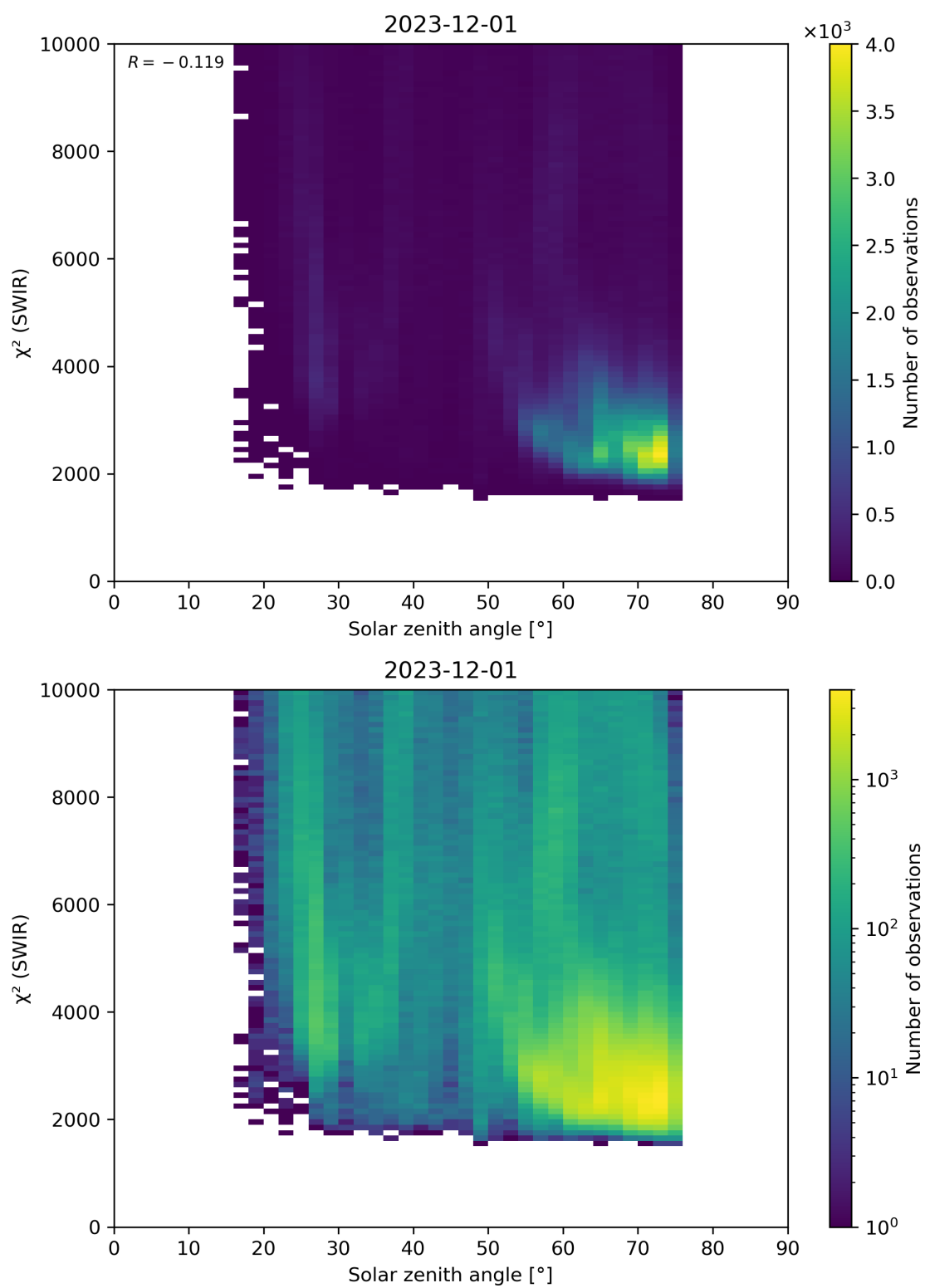
Figure 95: Scatter density plot of “Solar zenith angle” against “ \chi^2 (SWIR)” for 2023-11-30 to 2023-12-02.
