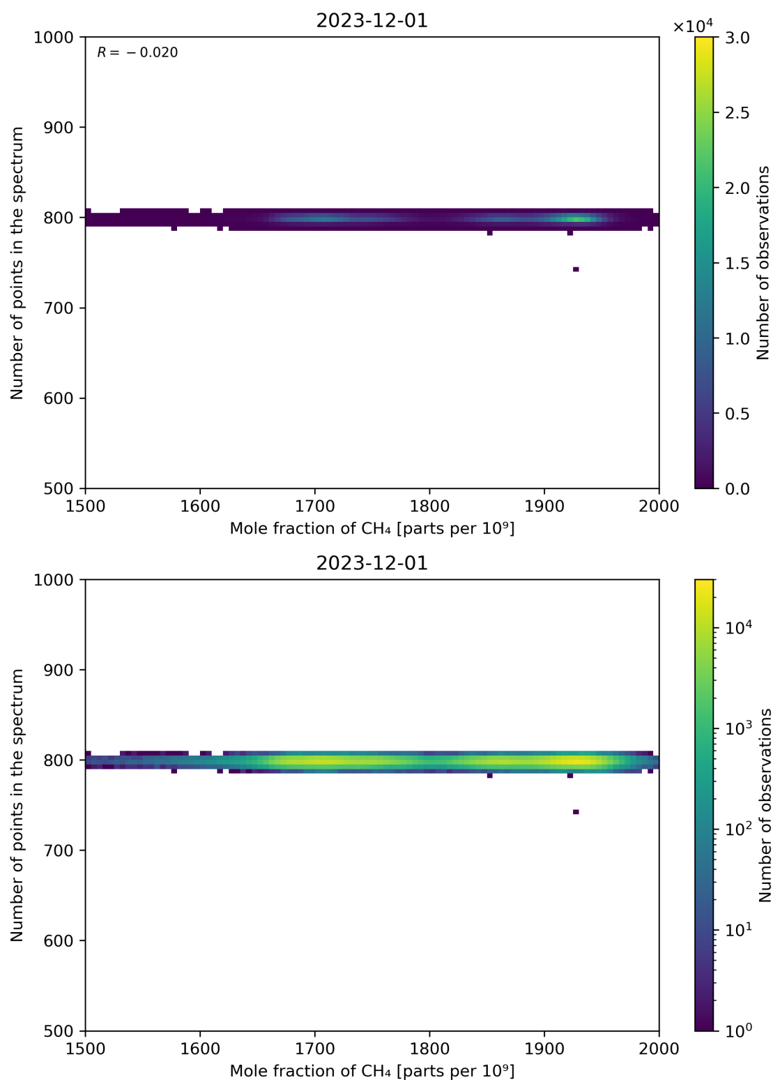
Figure 77: Scatter density plot of “Mole fraction of CH 4 ” against “Number of points in the spectrum” for 2023-11-30 to 2023-12-02.
