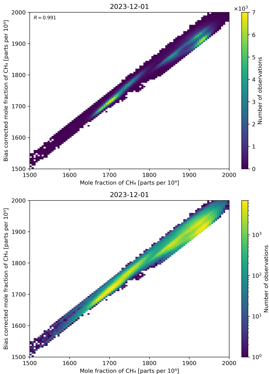
Figure 74: Scatter density plot of “Mole fraction of CH 4 ” against “Bias corrected mole fraction of CH 4 ” for 2023-11-30 to 2023-12-02.
