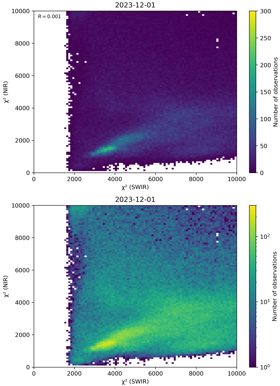
Figure 47: Scatter density plot of “ \chi^2 (SWIR)” against “ \chi^2 (NIR)” for 2023-11-30 to 2023-12-02.
