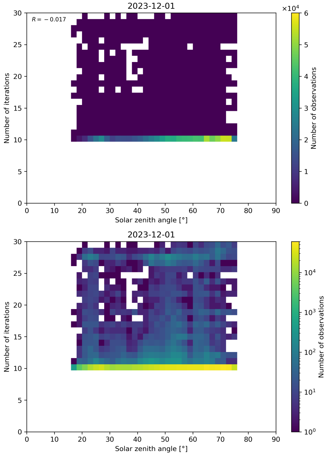
Figure 102: Scatter density plot of “Solar zenith angle” against “Number of iterations” for 2023-11-30 to 2023-12-02.
