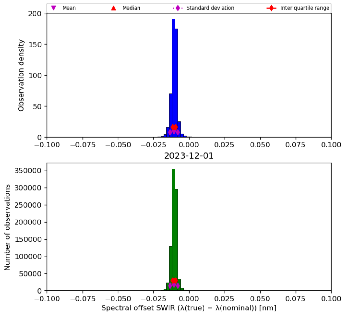
Figure 27: Histogram of “Spectral offset SWIR ( \lambda(\text{true}) - \lambda(\text{nominal}) )” for 2023-11-30 to 2023-12-02
