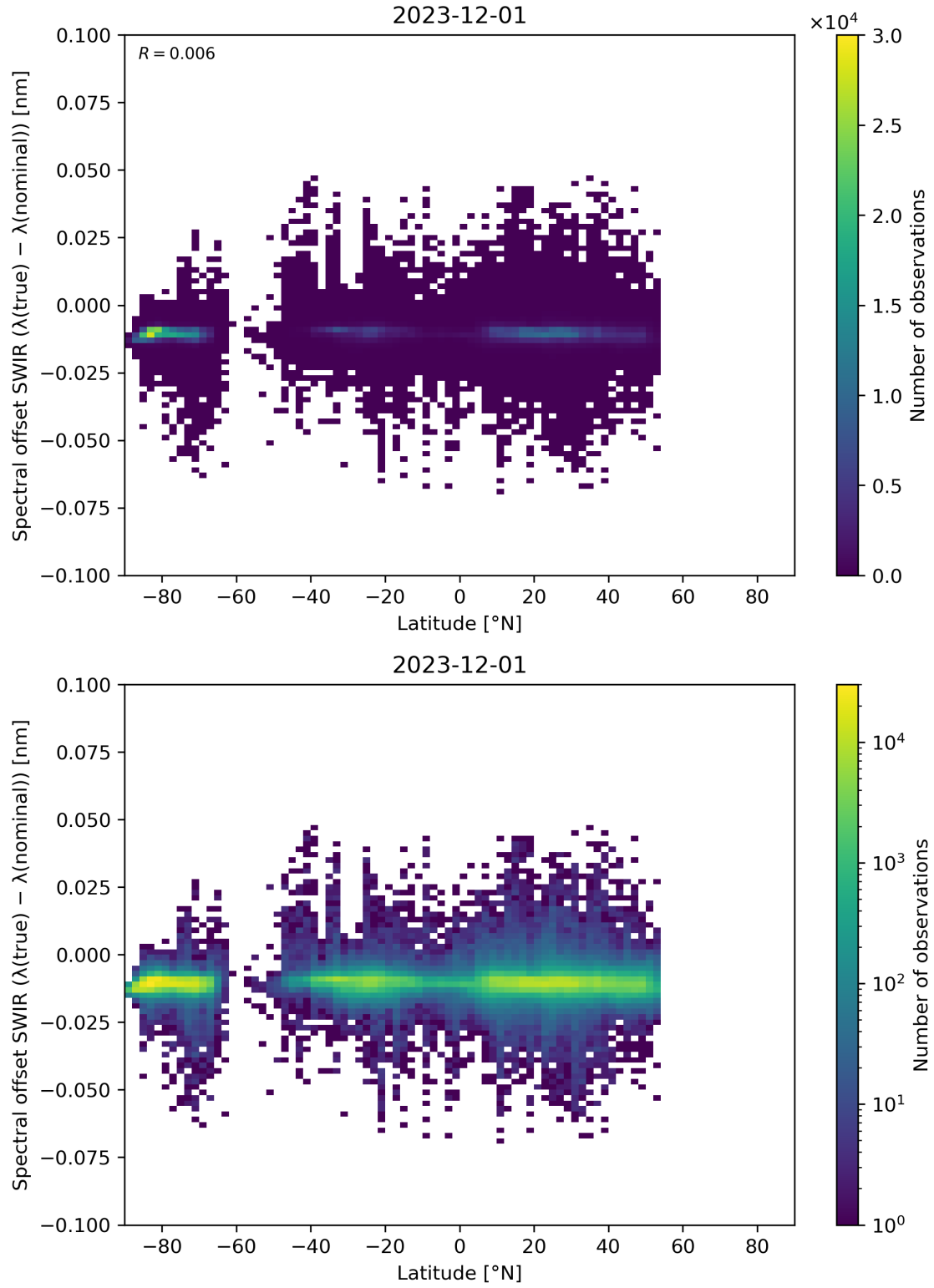
Figure 62: Scatter density plot of “Latitude” against “Spectral offset SWIR ( \lambda(\text{true}) - \lambda(\text{nominal}) )” for 2023-11-30 to 2023-12-02.
