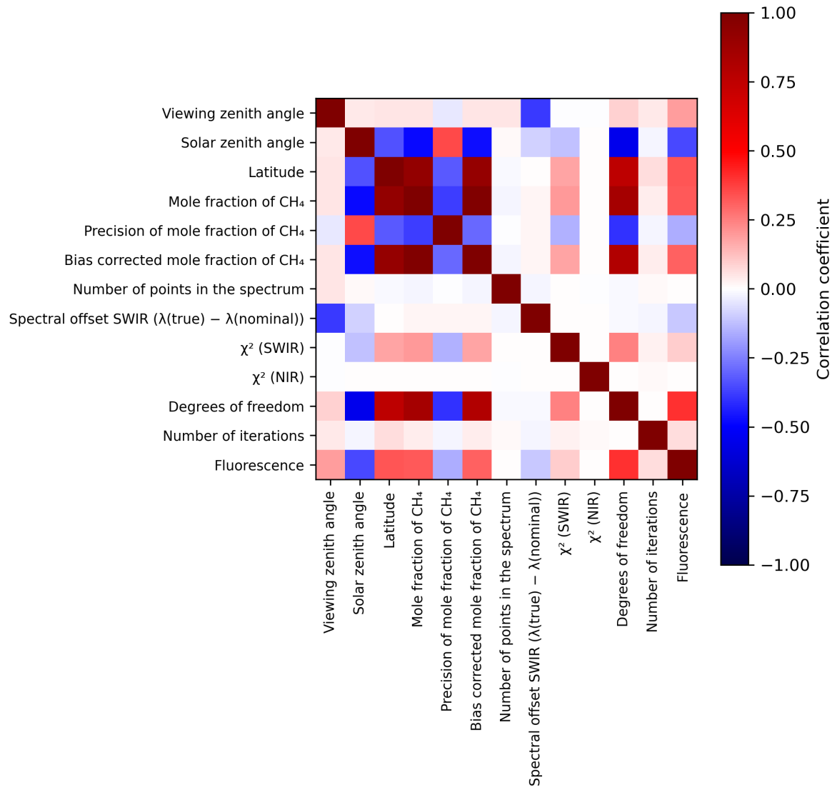
Figure 2: Map of correlation matrix for 2023-11-30 to 2023-12-02.
