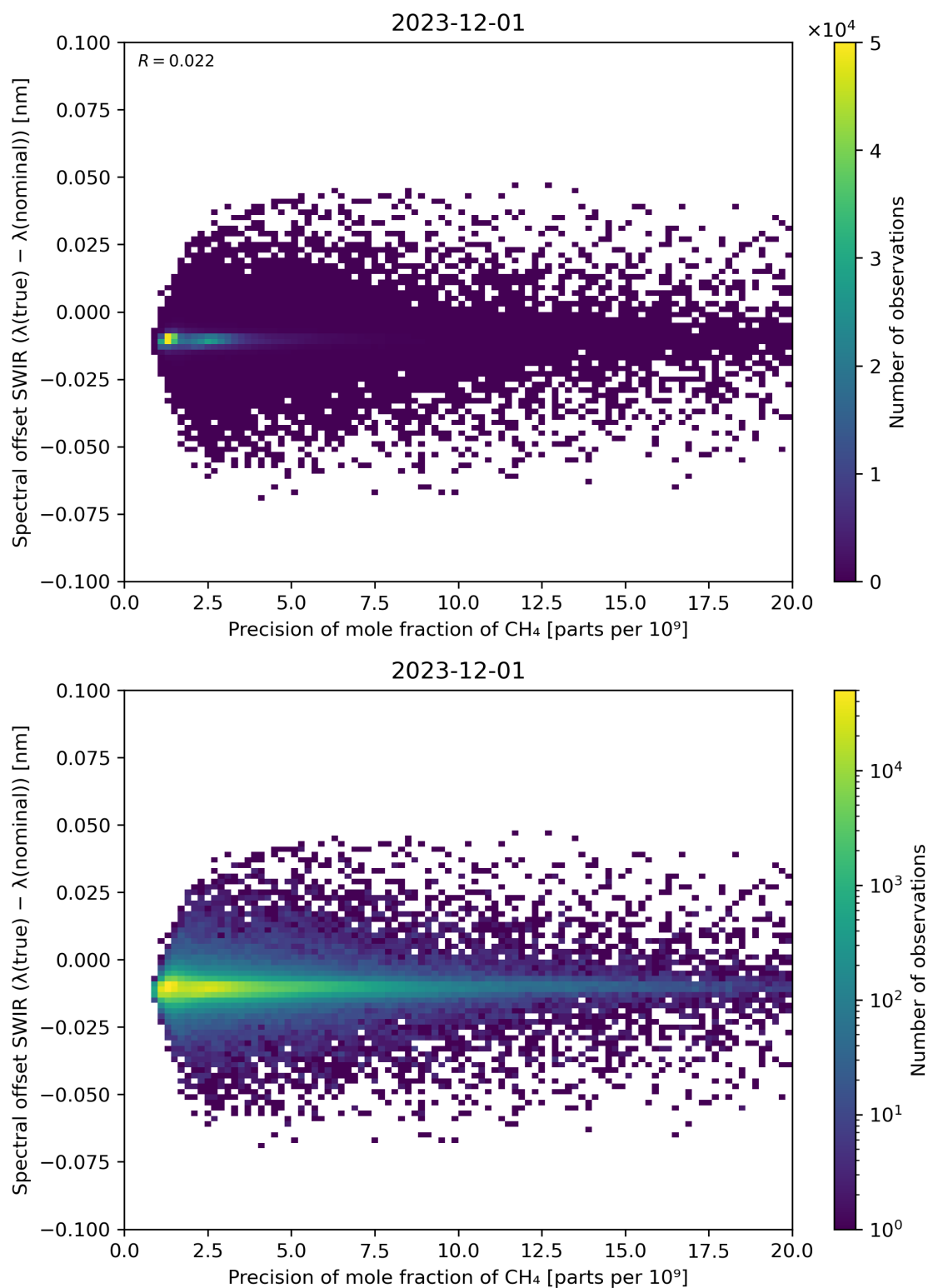
Figure 85: Scatter density plot of “Precision of mole fraction of \text{CH}_4 ” against “Spectral offset SWIR ( \lambda(\text{true}) - \lambda(\text{nominal}) )” for 2023-11-30 to 2023-12-02.
