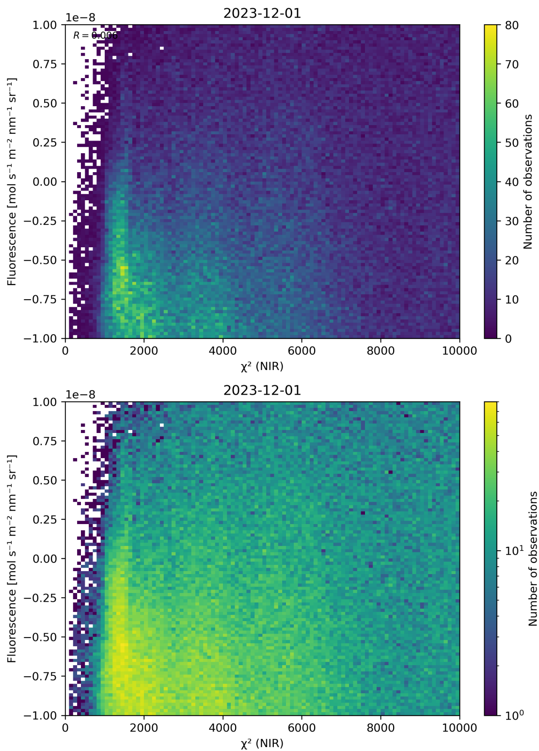
Figure 45: Scatter density plot of “ \chi^2 (NIR)” against “Fluorescence” for 2023-11-30 to 2023-12-02.
