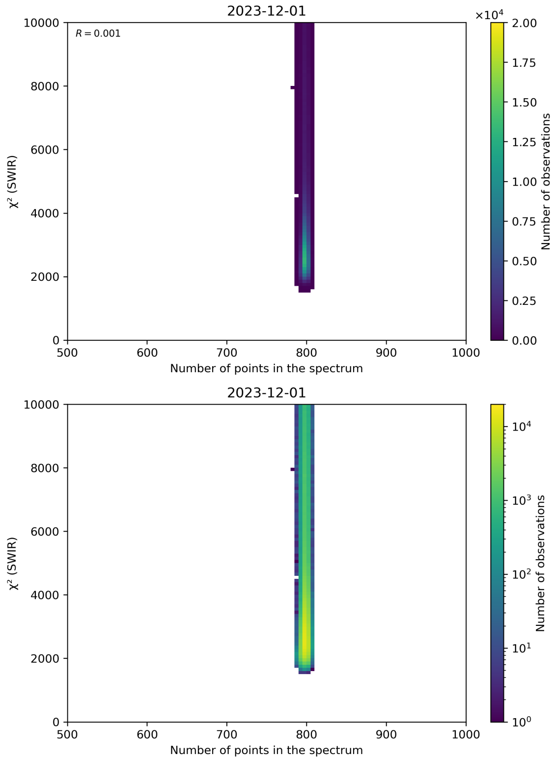
Figure 89: Scatter density plot of “Number of points in the spectrum” against “ \chi^2 (SWIR)” for 2023-11-30 to 2023-12-02.
