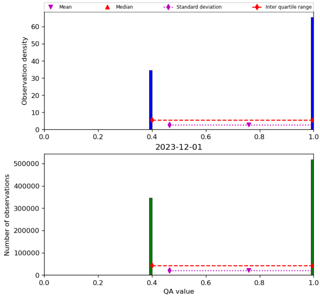
Figure 22: Histogram of “QA value” for 2023-11-30 to 2023-12-02
