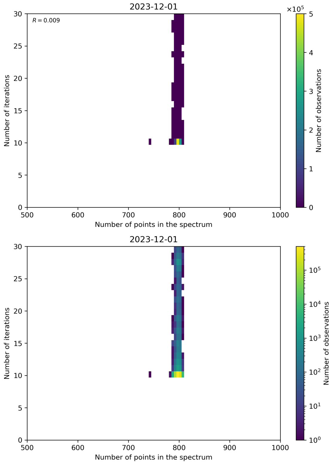
Figure 92: Scatter density plot of “Number of points in the spectrum” against “Number of iterations” for 2023-11-30 to 2023-12-02.
