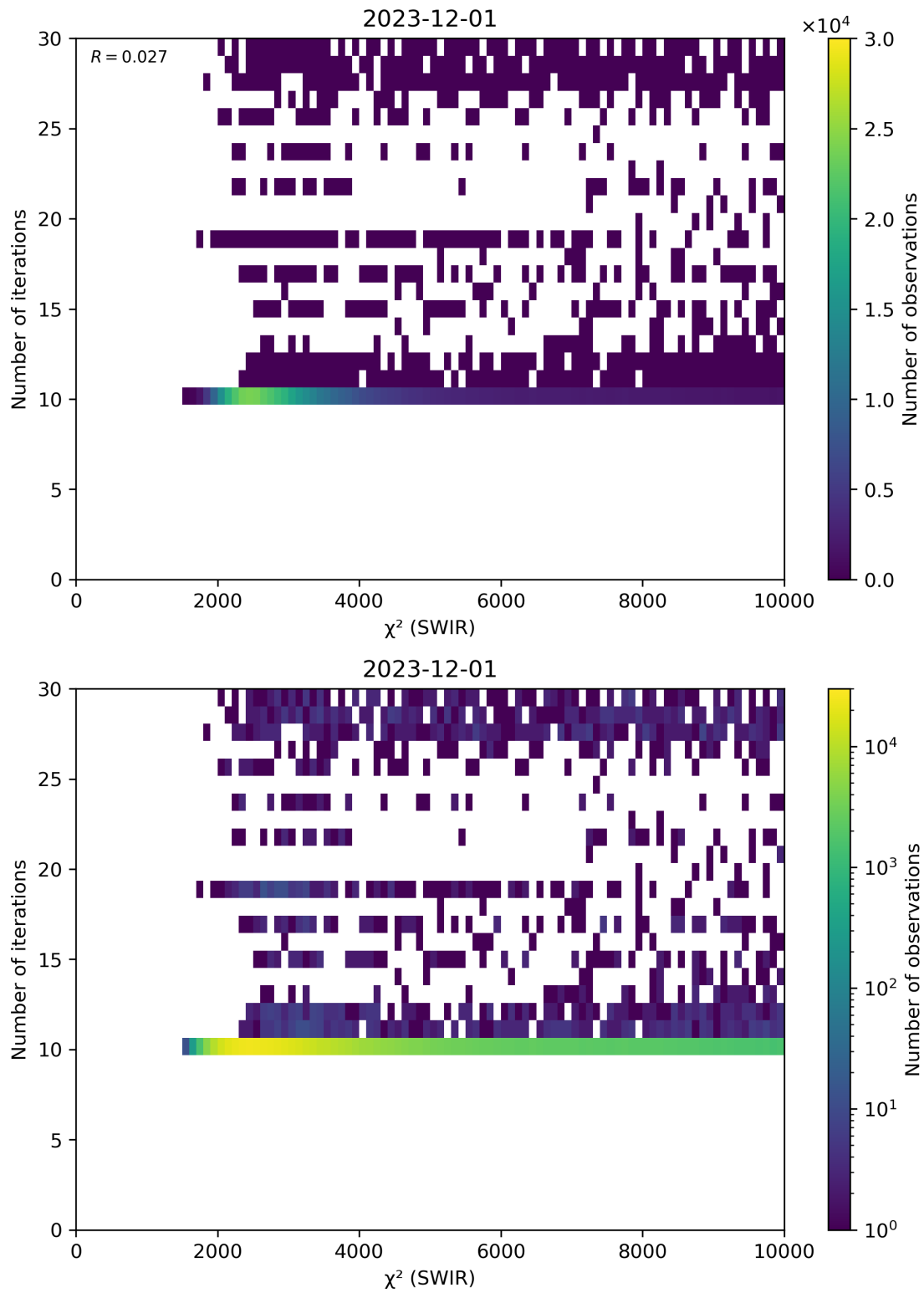
Figure 50: Scatter density plot of " \chi^2 (SWIR)" against "Number of iterations" for 2023-11-30 to 2023-12-02.
