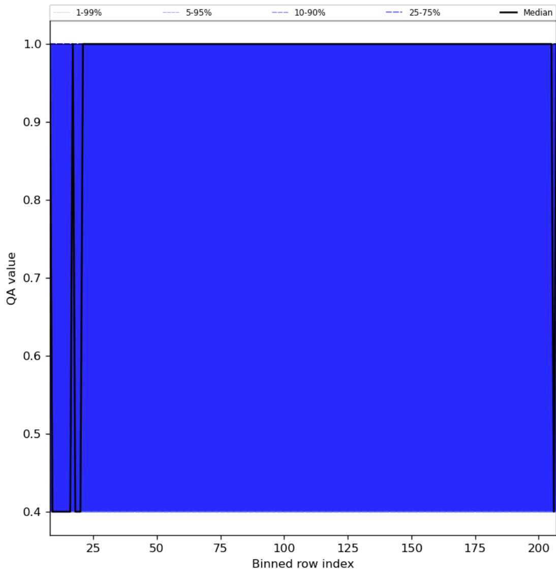
Figure 33: Along track statistics of “QA value” for 2023-11-30 to 2023-12-02
