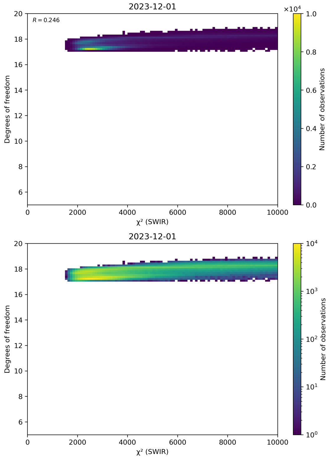
Figure 48: Scatter density plot of “ \chi^2 (SWIR)” against “Degrees of freedom” for 2023-11-30 to 2023-12-02.
