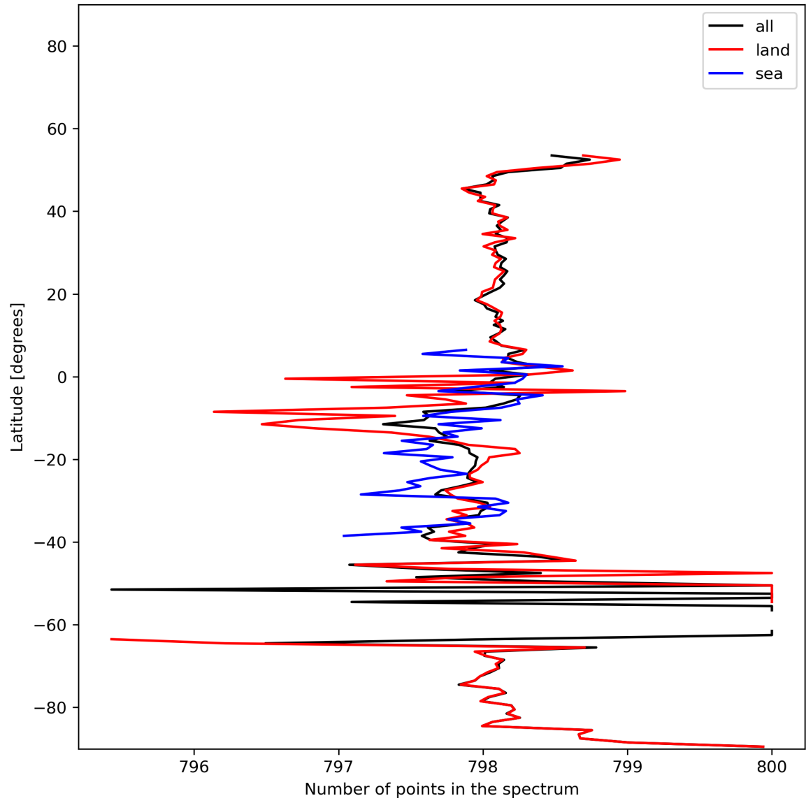
Figure 15: Zonal average of “Number of points in the spectrum” for 2023-11-30 to 2023-12-02.
