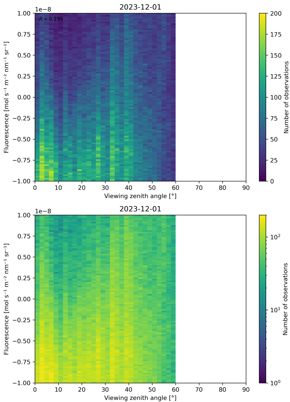
Figure 108: Scatter density plot of “Viewing zenith angle” against “Fluorescence” for 2023-11-30 to 2023-12-02.
