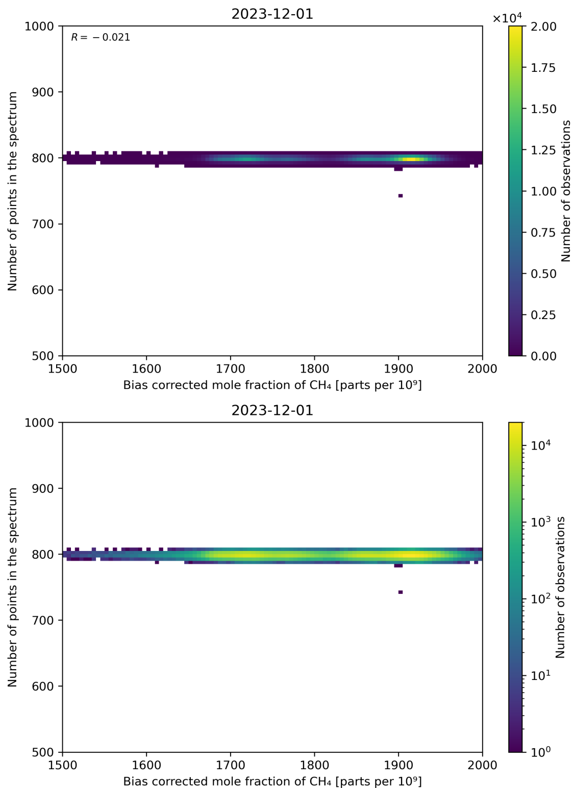
Figure 68: Scatter density plot of “Bias corrected mole fraction of CH 4 ” against “Number of points in the spectrum” for 2023-11-30 to 2023-12-02.
