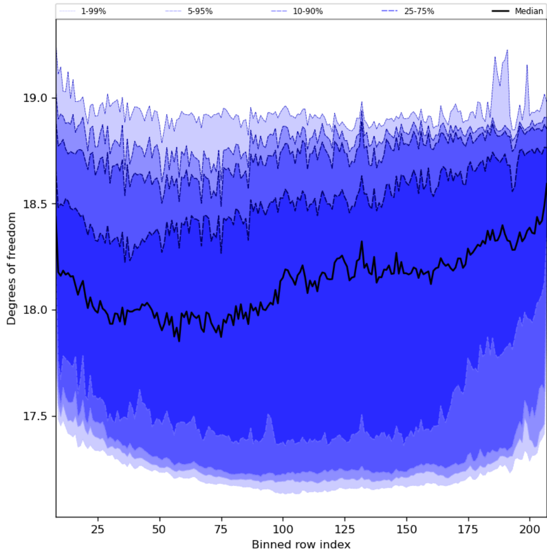
Figure 41: Along track statistics of “Degrees of freedom” for 2023-11-30 to 2023-12-02
