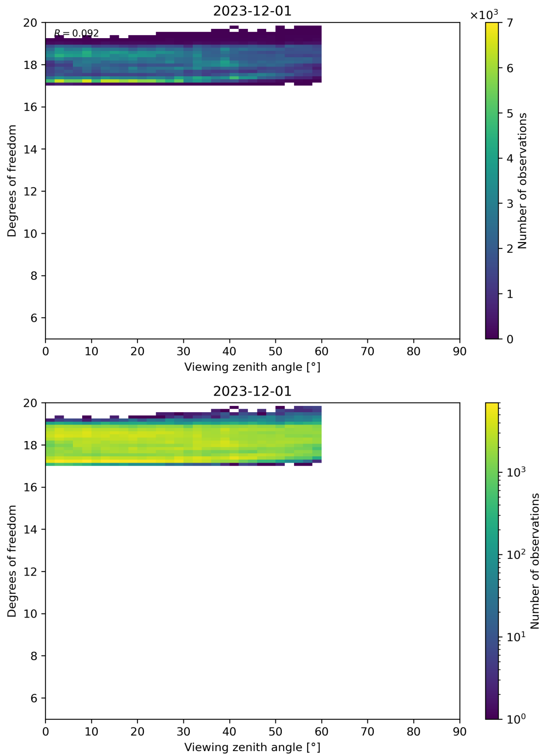
Figure 107: Scatter density plot of “Viewing zenith angle” against “Degrees of freedom” for 2023-11-30 to 2023-12-02.
