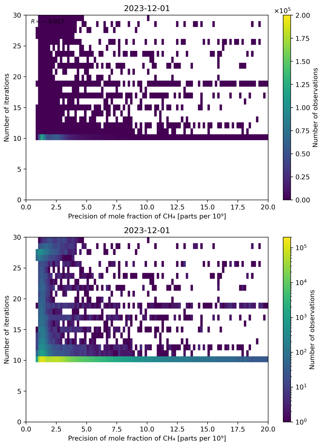
Figure 83: Scatter density plot of “Precision of mole fraction of CH 4 ” against “Number of iterations” for 2023-11-30 to 2023-12-02.
