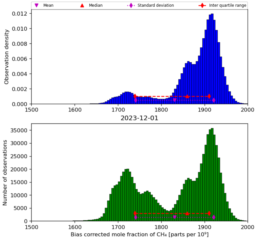
Figure 25: Histogram of “Bias corrected mole fraction of CH 4 ” for 2023-11-30 to 2023-12-02
