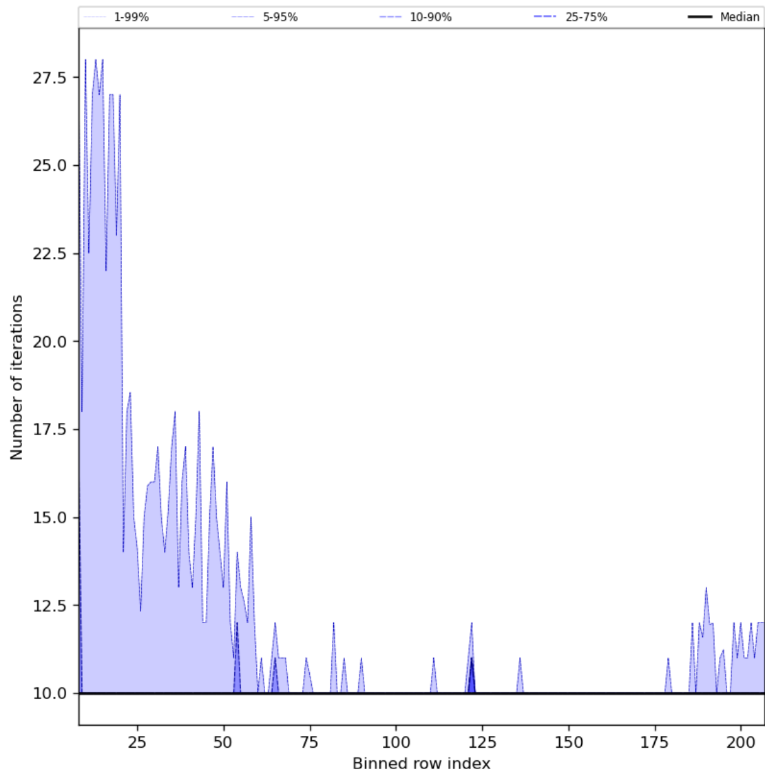
Figure 42: Along track statistics of “Number of iterations” for 2023-11-30 to 2023-12-02
