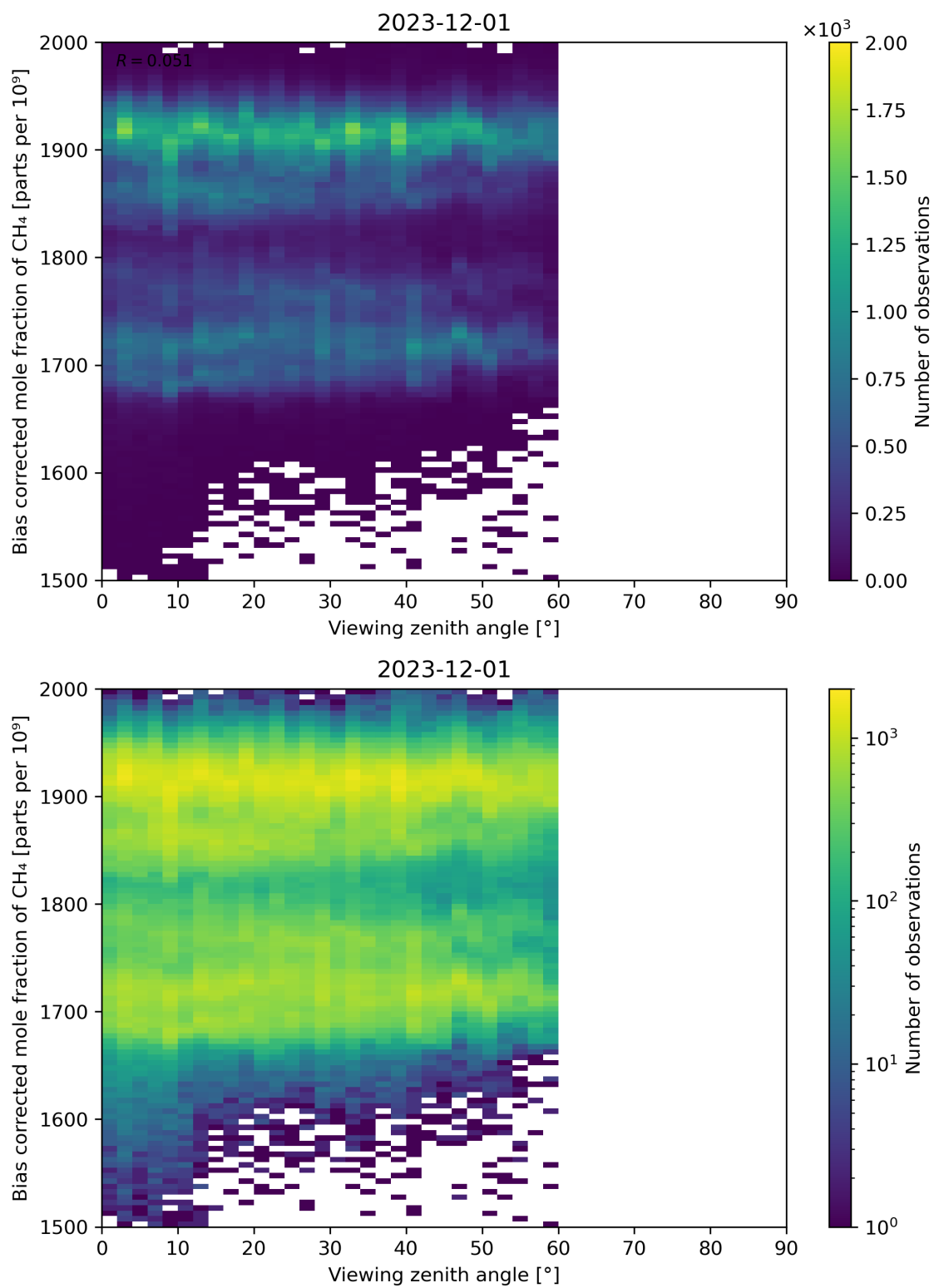
Figure 111: Scatter density plot of “Viewing zenith angle” against “Bias corrected mole fraction of CH 4 ” for 2023-11-30 to 2023-12-02.
