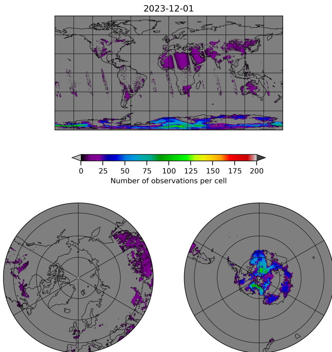
Figure 10: Map of the number of observations for 2023-11-30 to 2023-12-02
