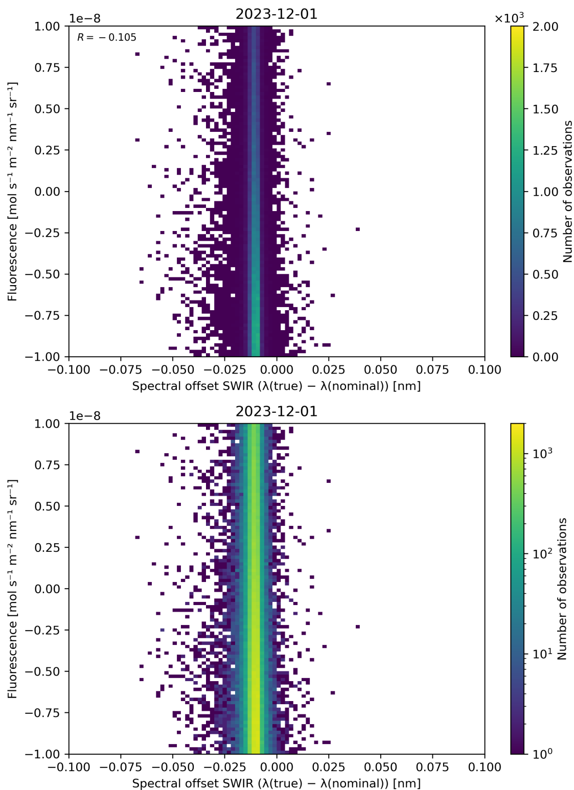
Figure 120: Scatter density plot of “Spectral offset SWIR ( \lambda(\text{true}) - \lambda(\text{nominal}) )” against “Fluorescence” for 2023-11-30 to 2023-12-02.
