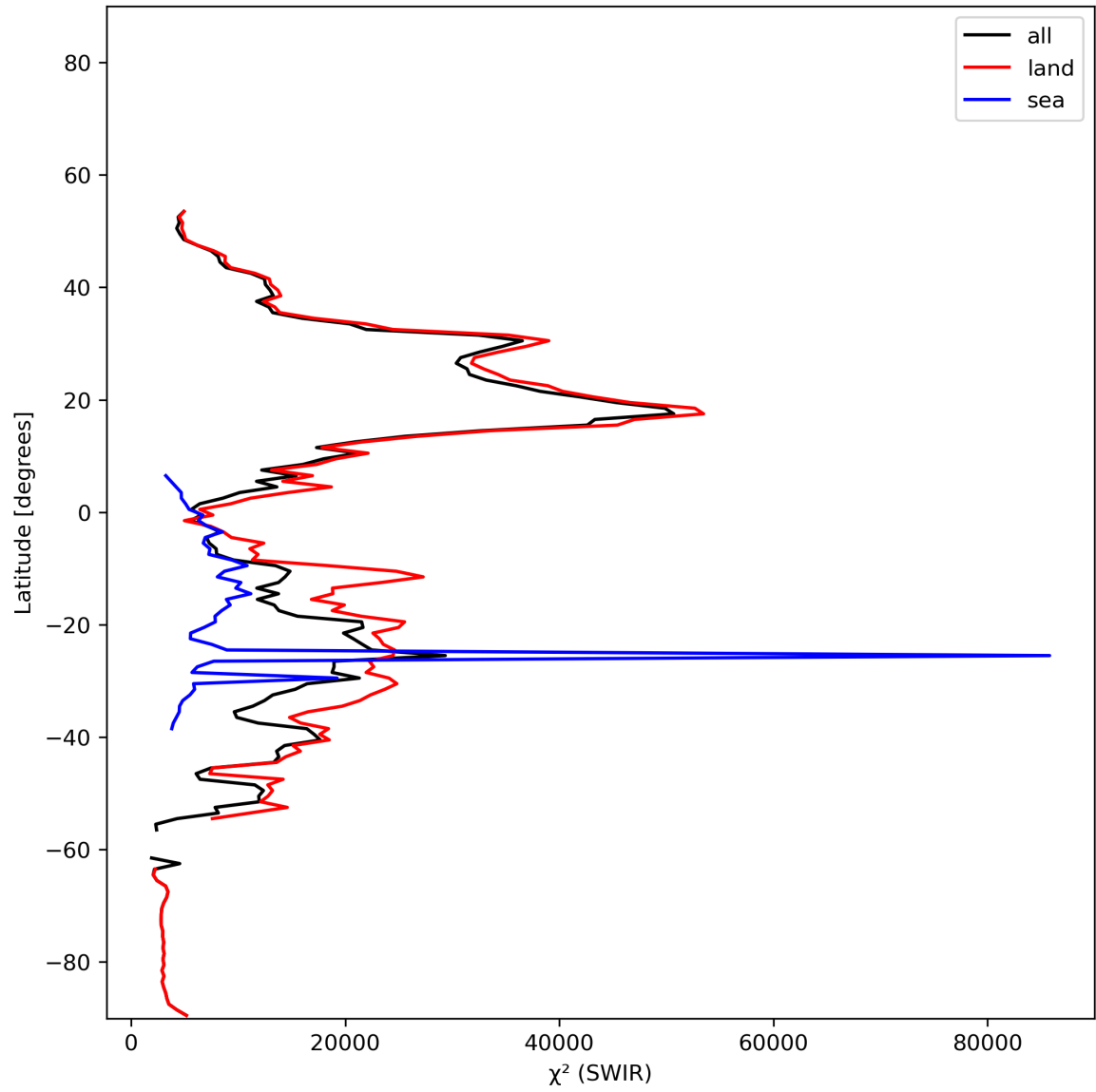
Figure 17: Zonal average of “ \chi^2 (SWIR)” for 2023-11-30 to 2023-12-02.
