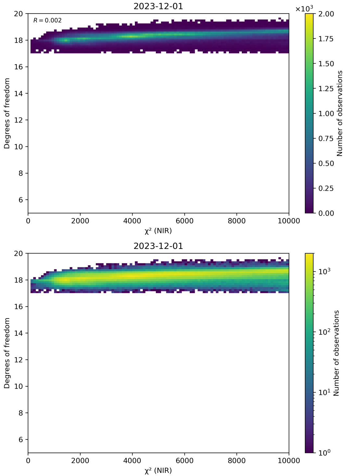
Figure 44: Scatter density plot of “ \chi^2 (NIR)” against “Degrees of freedom” for 2023-11-30 to 2023-12-02.
