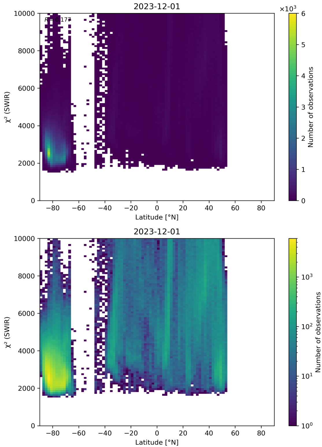
Figure 54: Scatter density plot of “Latitude” against “ \chi^2 (SWIR)” for 2023-11-30 to 2023-12-02.
