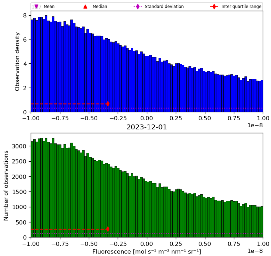
Figure 32: Histogram of “Fluorescence” for 2023-11-30 to 2023-12-02
