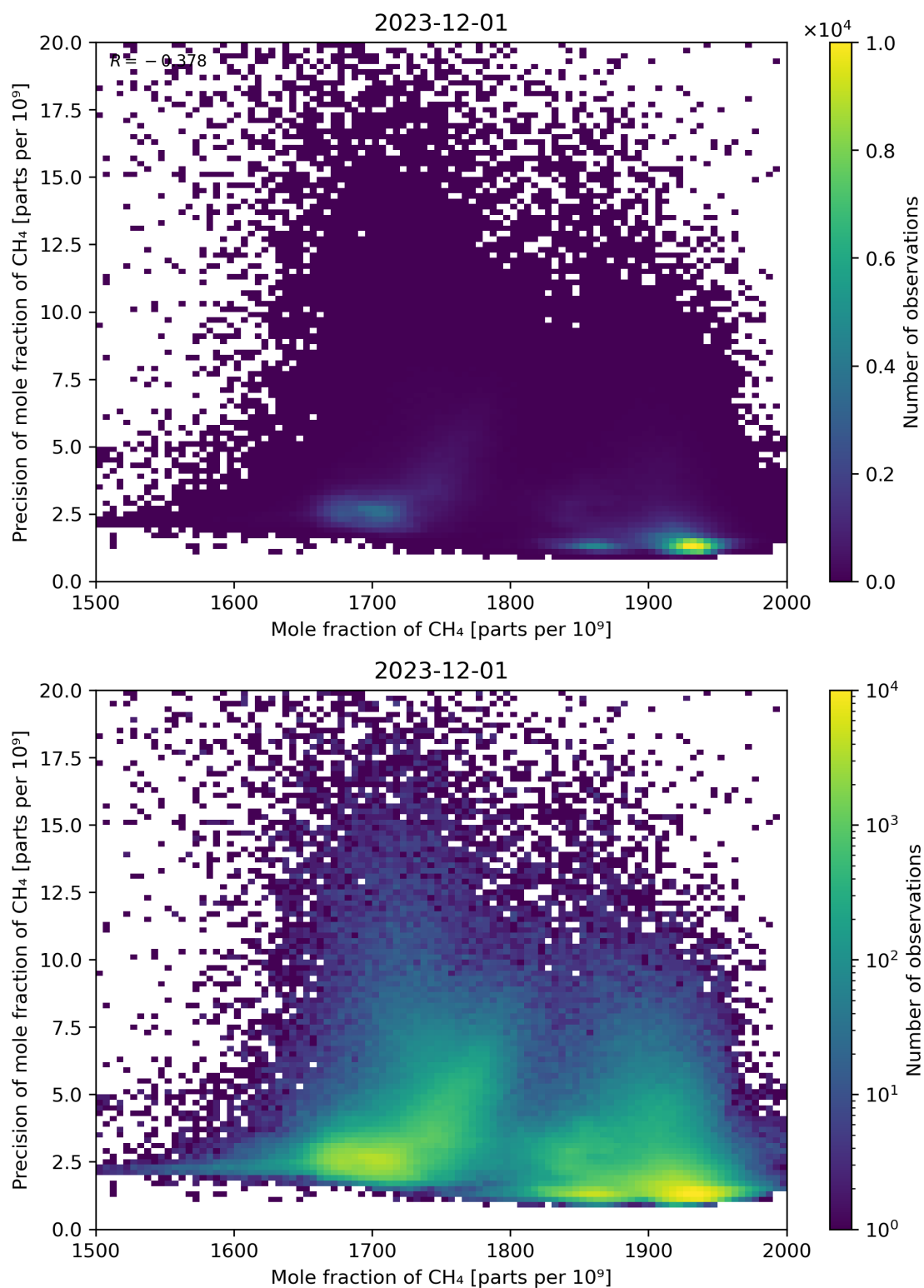
Figure 75: Scatter density plot of “Mole fraction of CH 4 ” against “Precision of mole fraction of CH 4 ” for 2023-11-30 to 2023-12-02.
