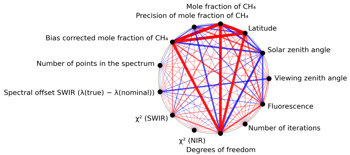
Figure 1: Map of correlation graph for 2023-11-30 to 2023-12-02.
