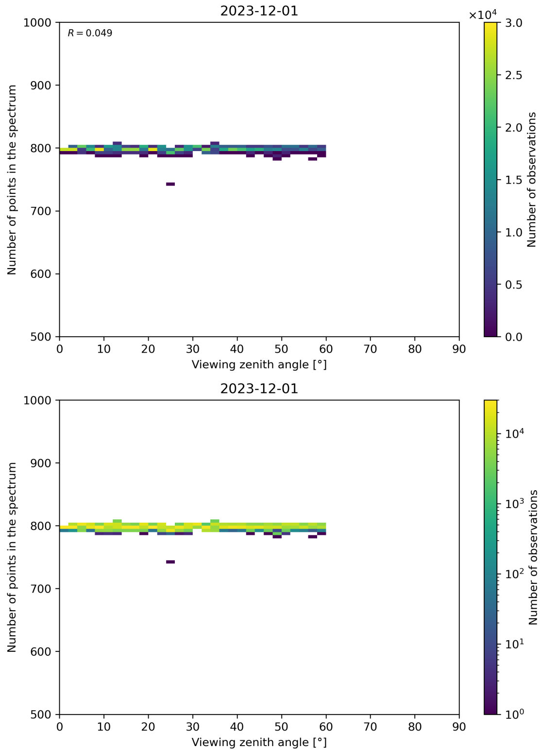
Figure 114: Scatter density plot of “Viewing zenith angle” against “Number of points in the spectrum” for 2023-11-30 to 2023-12-02.
