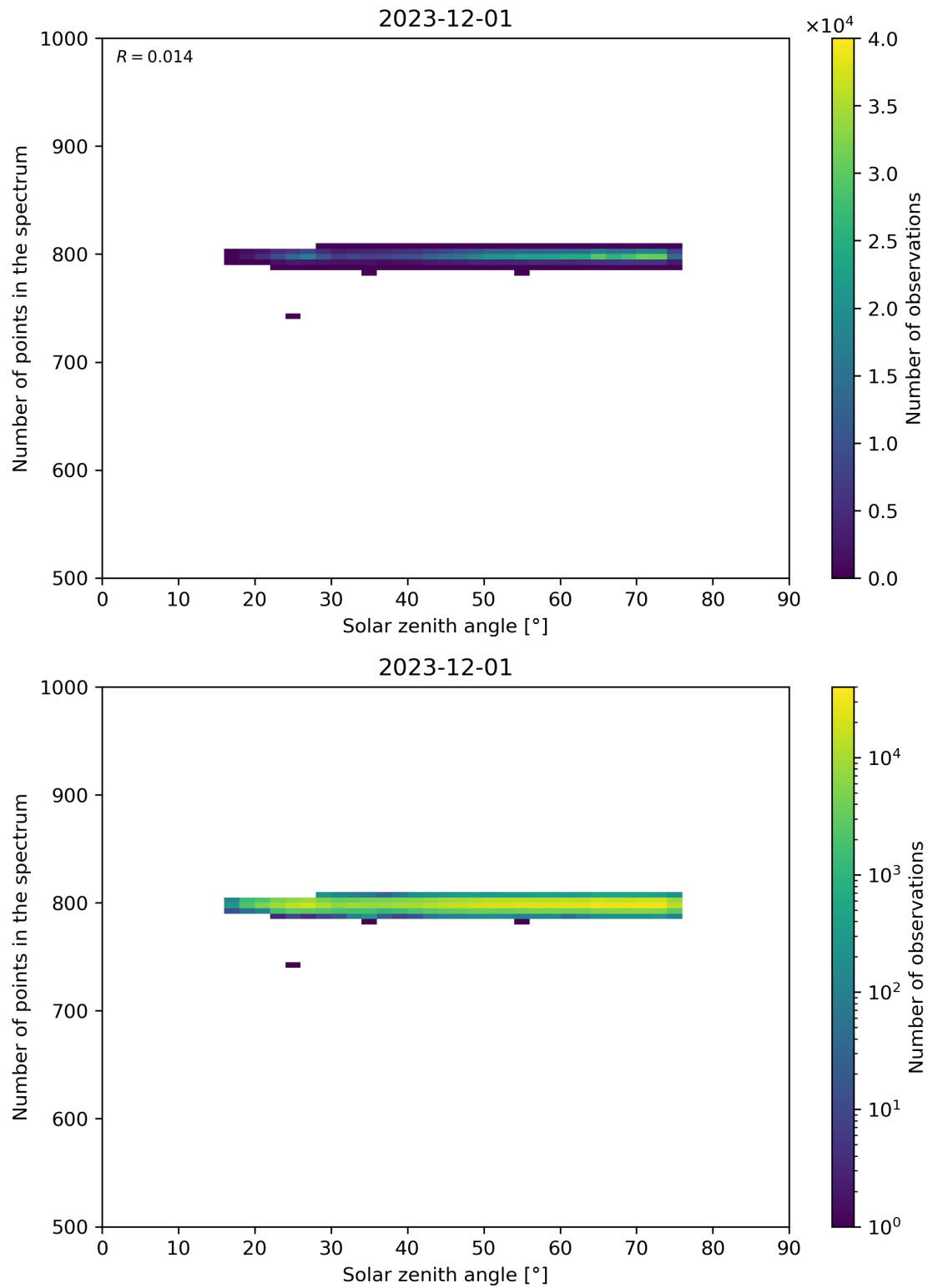
Figure 103: Scatter density plot of “Solar zenith angle” against “Number of points in the spectrum” for 2023-11-30 to 2023-12-02.
