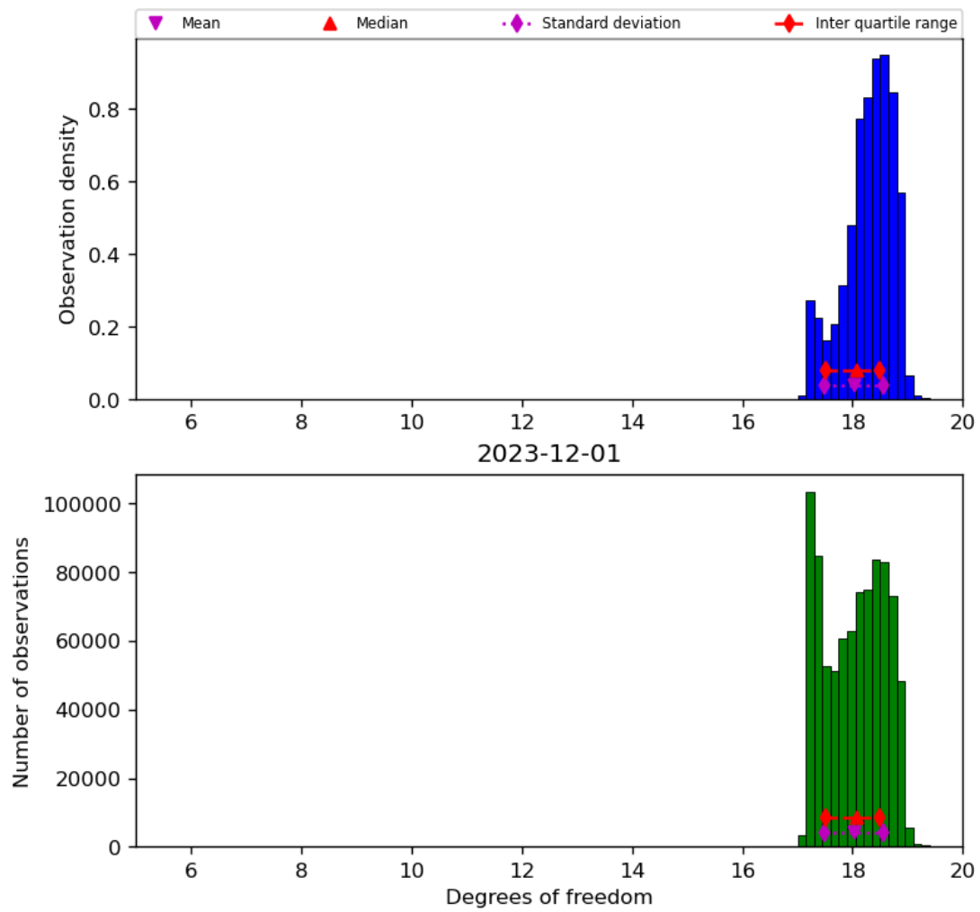
Figure 30: Histogram of “Degrees of freedom” for 2023-11-30 to 2023-12-02
