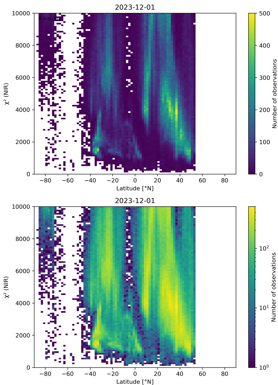
Figure 53: Scatter density plot of “Latitude” against “ \chi^2 (NIR)” for 2023-11-30 to 2023-12-02.
