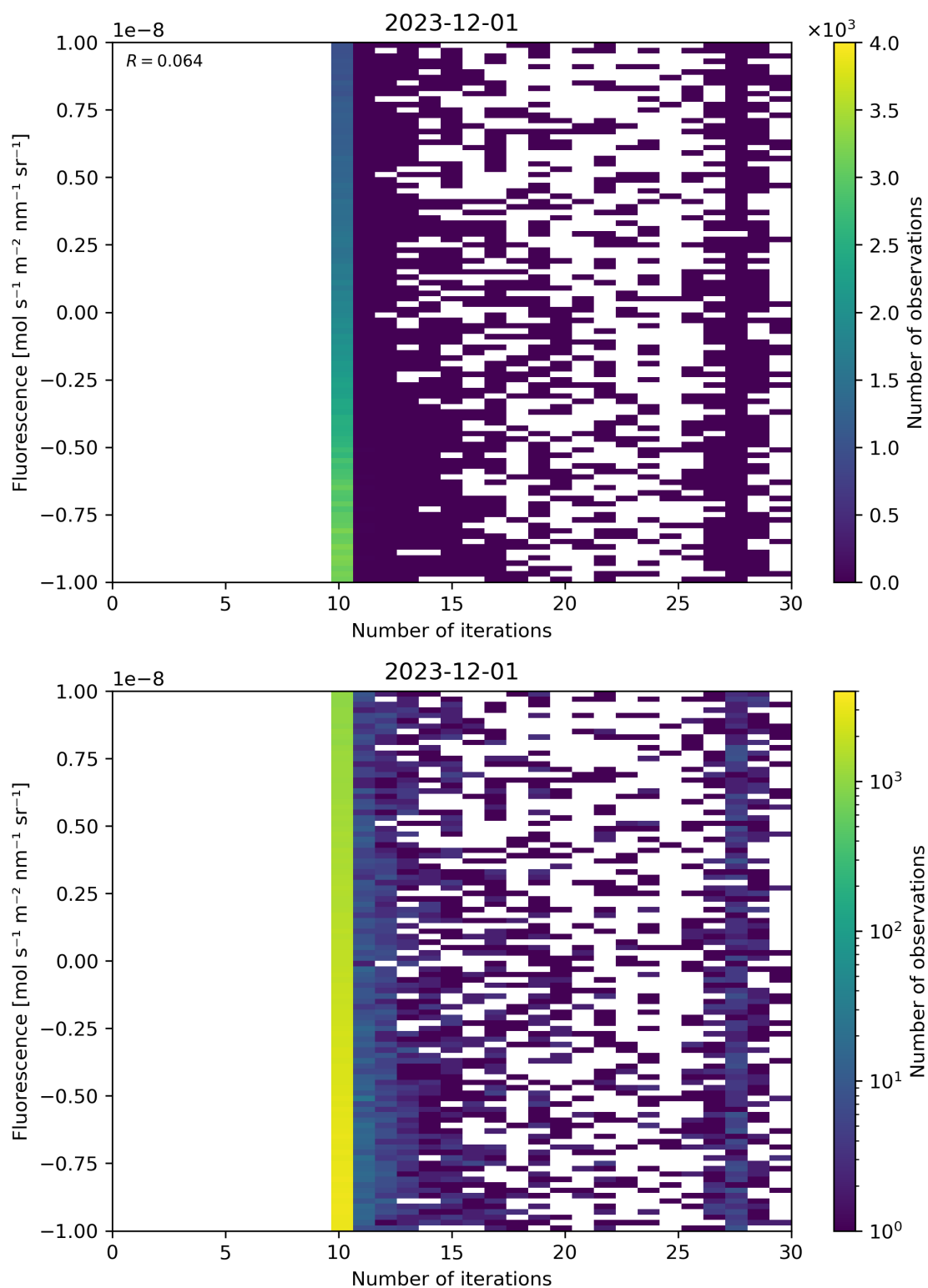
Figure 87: Scatter density plot of “Number of iterations” against “Fluorescence” for 2023-11-30 to 2023-12-02.
