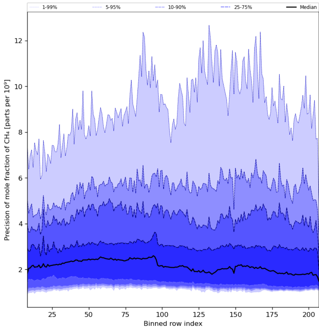
Figure 35: Along track statistics of “Precision of mole fraction of CH 4 ” for 2023-11-30 to 2023-12-02
