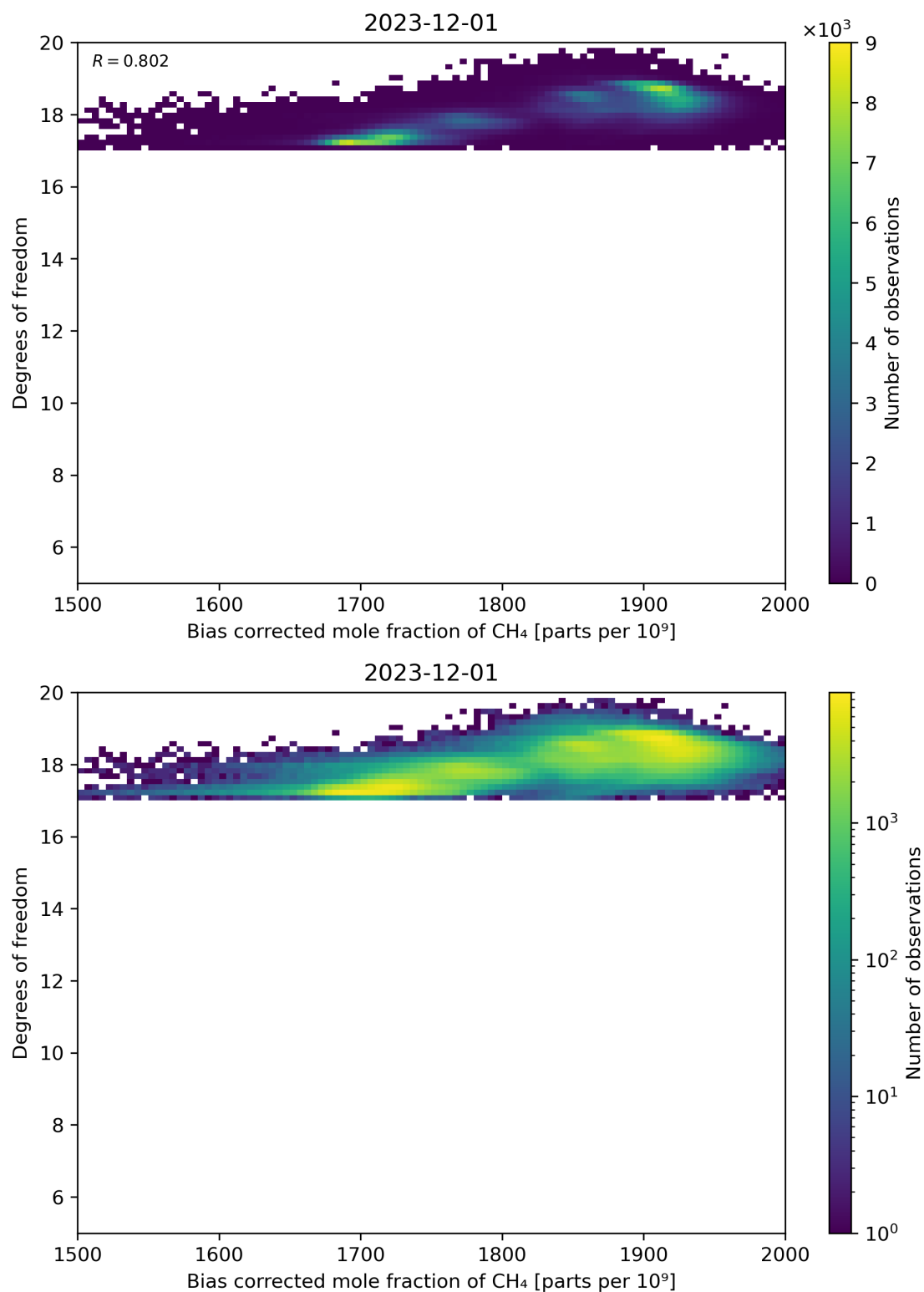
Figure 65: Scatter density plot of “Bias corrected mole fraction of CH 4 ” against “Degrees of freedom” for 2023-11-30 to 2023-12-02.
