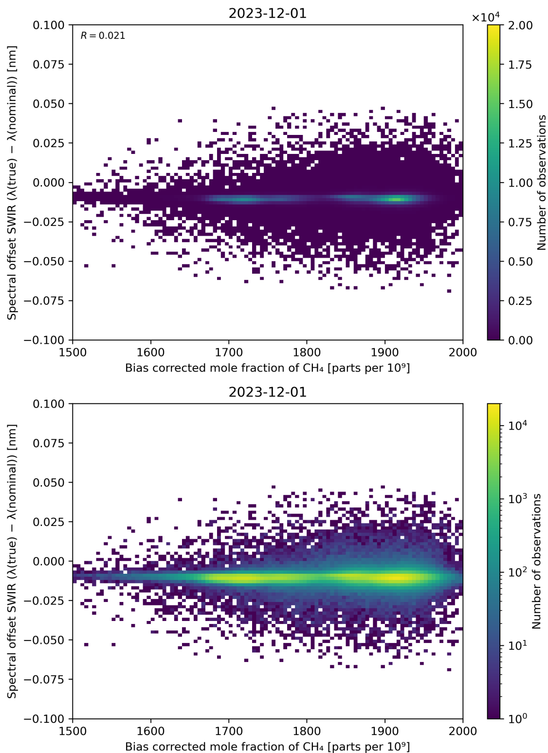
Figure 69: Scatter density plot of “Bias corrected mole fraction of \text{CH}_4 ” against “Spectral offset SWIR ( \lambda(\text{true}) - \lambda(\text{nominal}) )” for 2023-11-30 to 2023-12-02.
