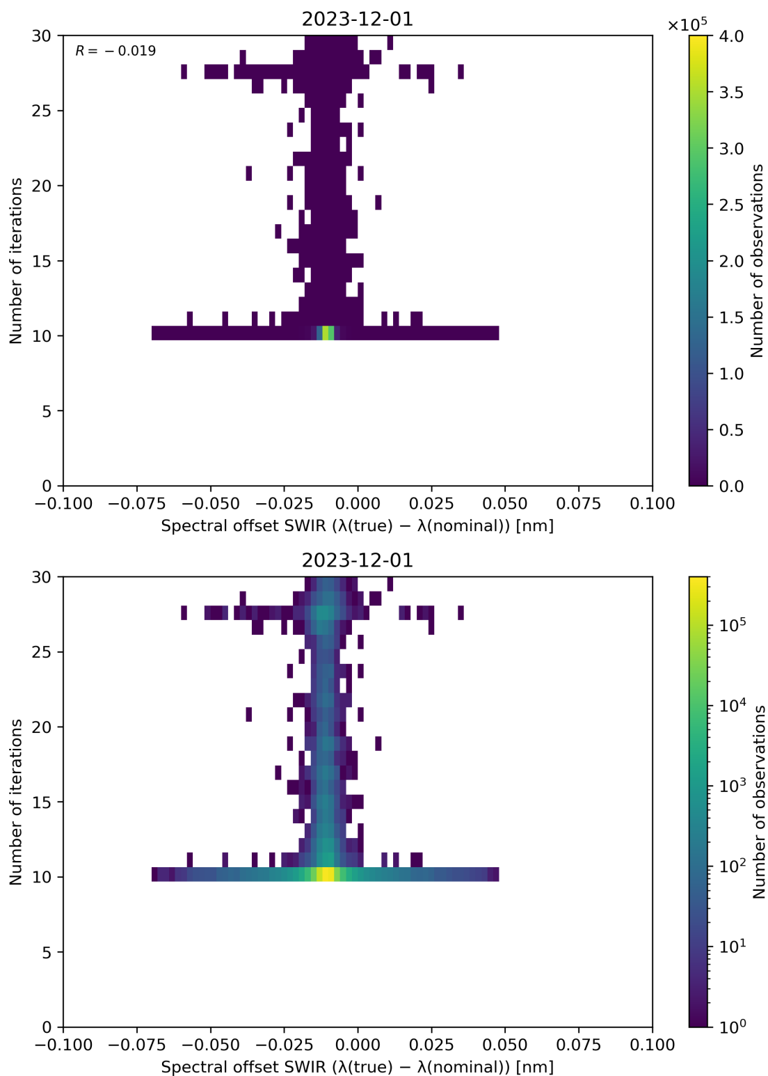
Figure 121: Scatter density plot of “Spectral offset SWIR ( \lambda(\text{true}) - \lambda(\text{nominal}) )” against “Number of iterations” for 2023-11-30 to 2023-12-02.
