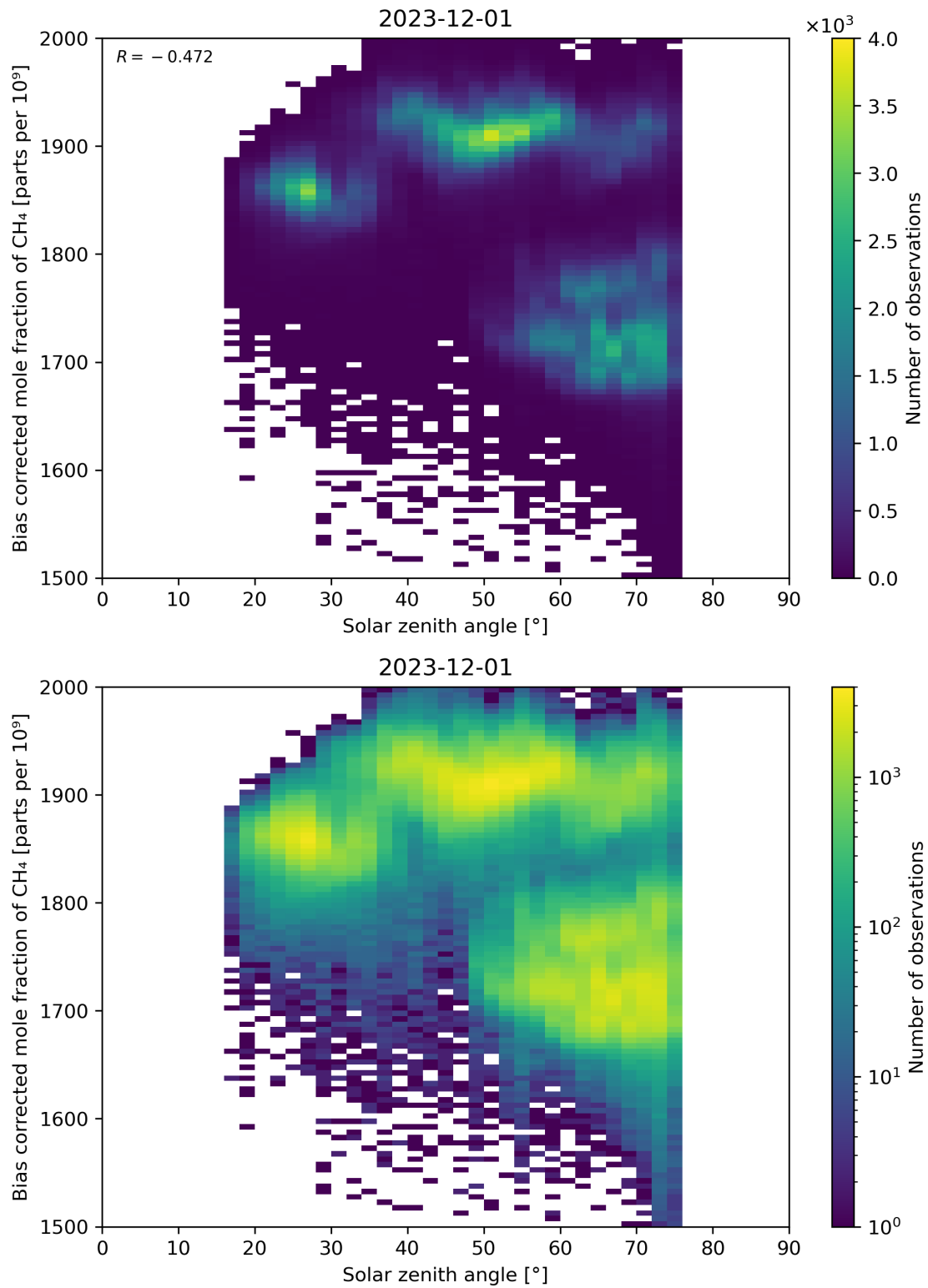
Figure 100: Scatter density plot of “Solar zenith angle” against “Bias corrected mole fraction of \text{CH}_4 ” for 2023-11-30 to 2023-12-02.
