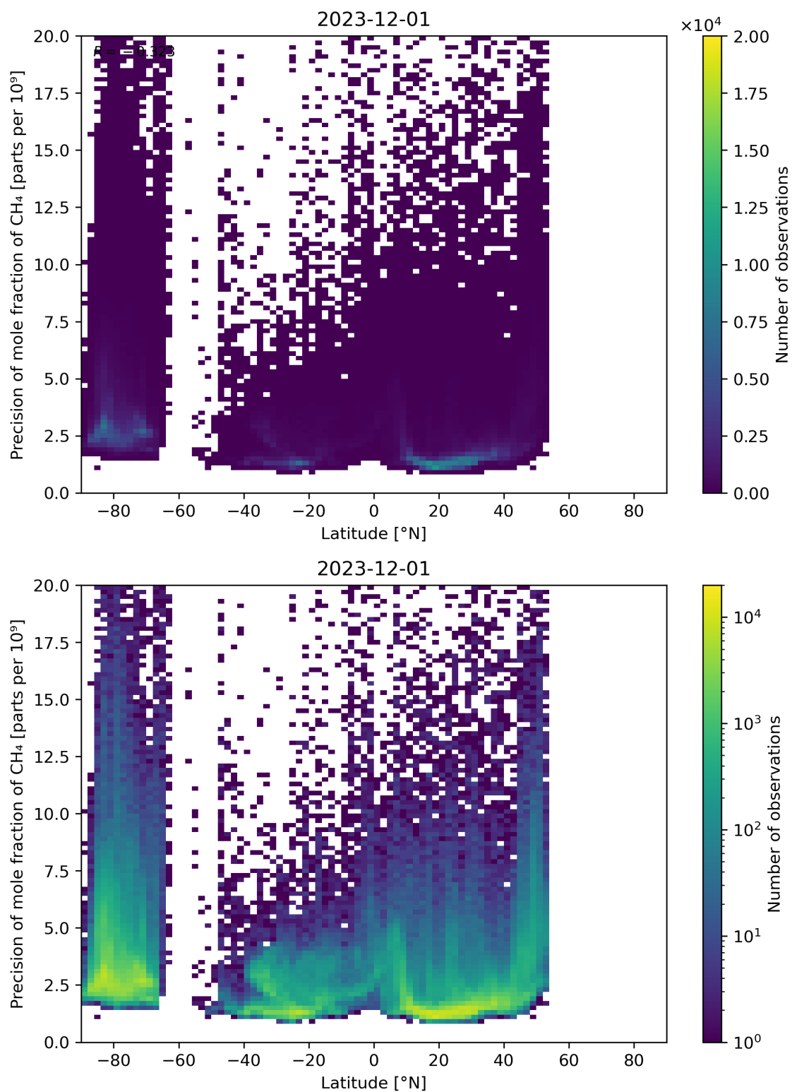
Figure 59: Scatter density plot of “Latitude” against “Precision of mole fraction of CH 4 ” for 2023-11-30 to 2023-12-02.
