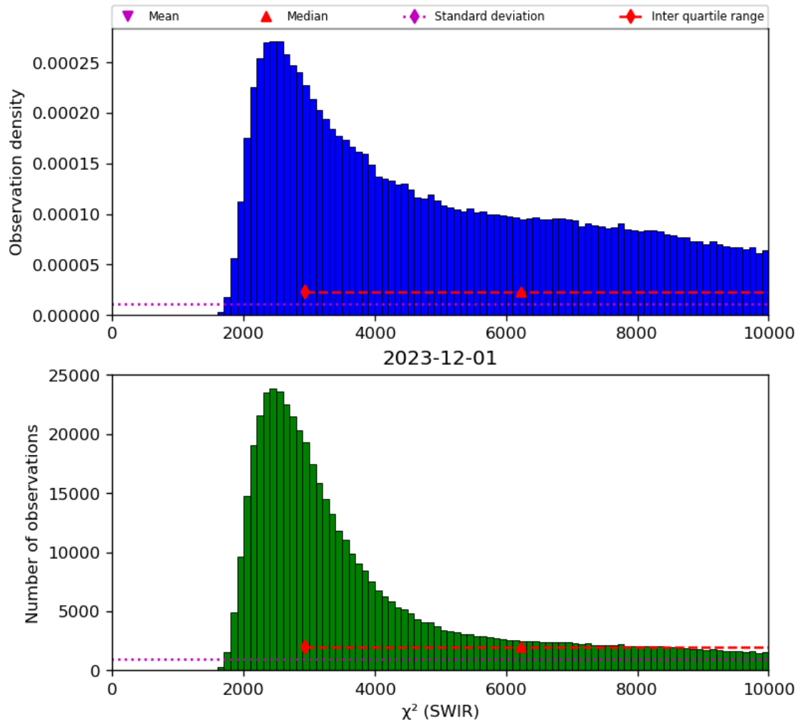
Figure 28: Histogram of “ \chi^2 (SWIR)” for 2023-11-30 to 2023-12-02
