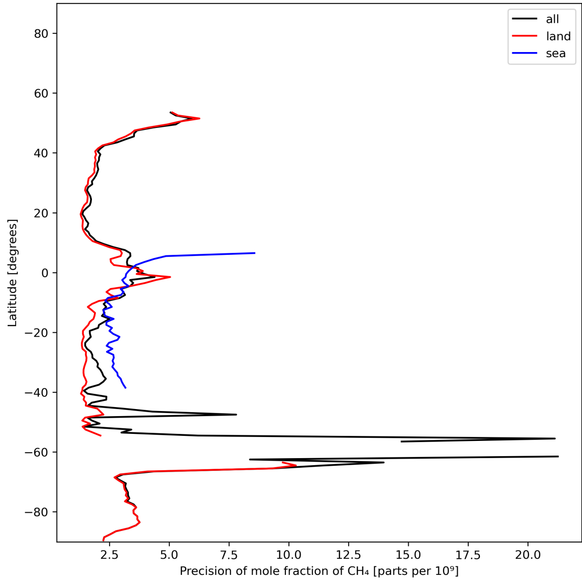
Figure 13: Zonal average of “Precision of mole fraction of CH 4 ” for 2023-11-30 to 2023-12-02.
