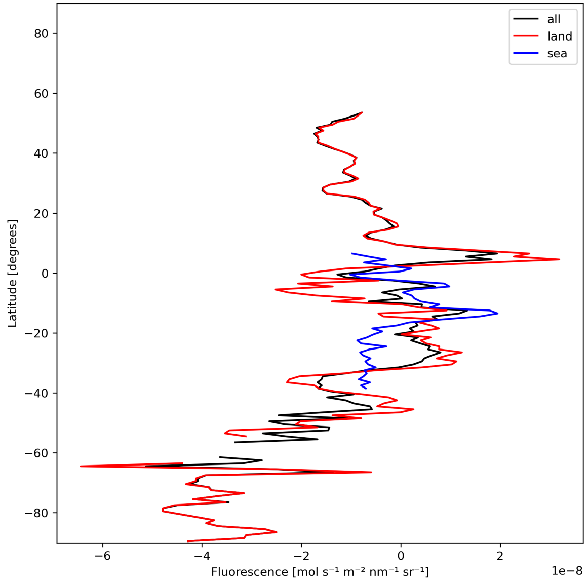
Figure 21: Zonal average of “Fluorescence” for 2023-11-30 to 2023-12-02.
