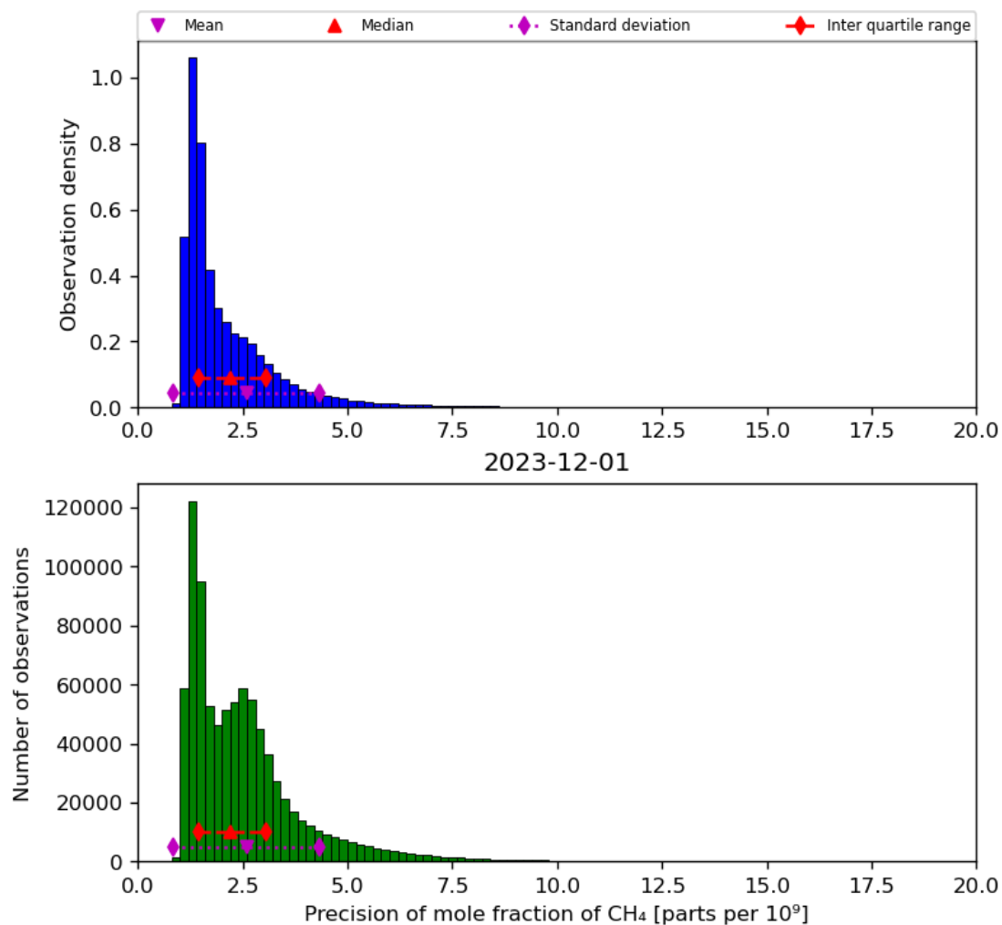
Figure 24: Histogram of “Precision of mole fraction of CH 4 ” for 2023-11-30 to 2023-12-02
