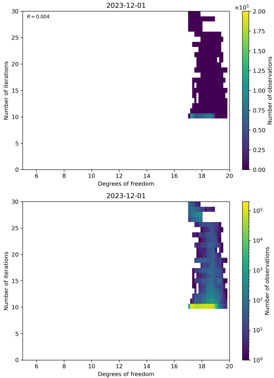
Figure 52: Scatter density plot of “Degrees of freedom” against “Number of iterations” for 2023-11-30 to 2023-12-02.
