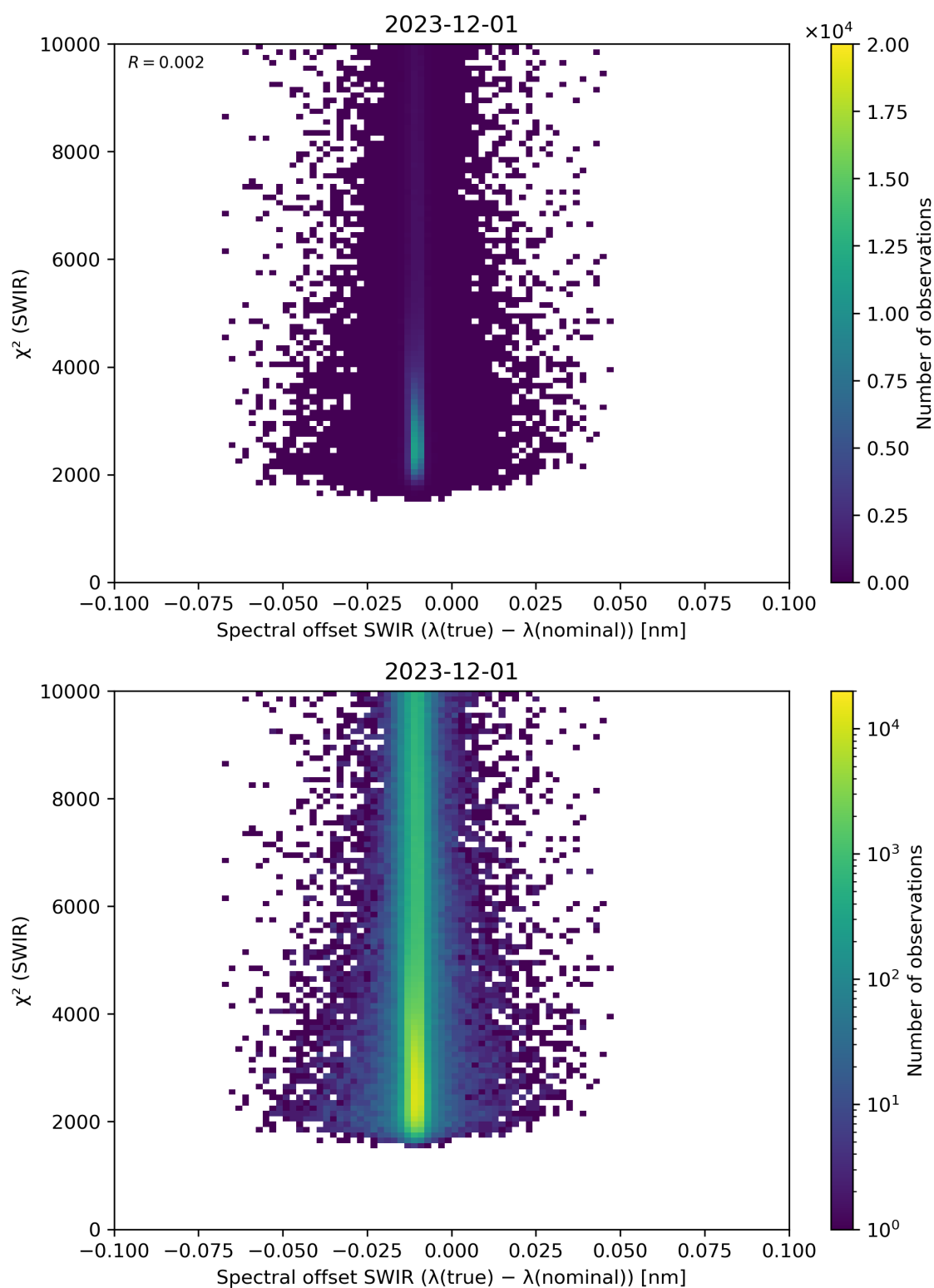
Figure 118: Scatter density plot of “Spectral offset SWIR ( \lambda(\text{true}) - \lambda(\text{nominal}) )” against “ \chi^2 (SWIR)” for 2023-11-30 to 2023-12-02.
