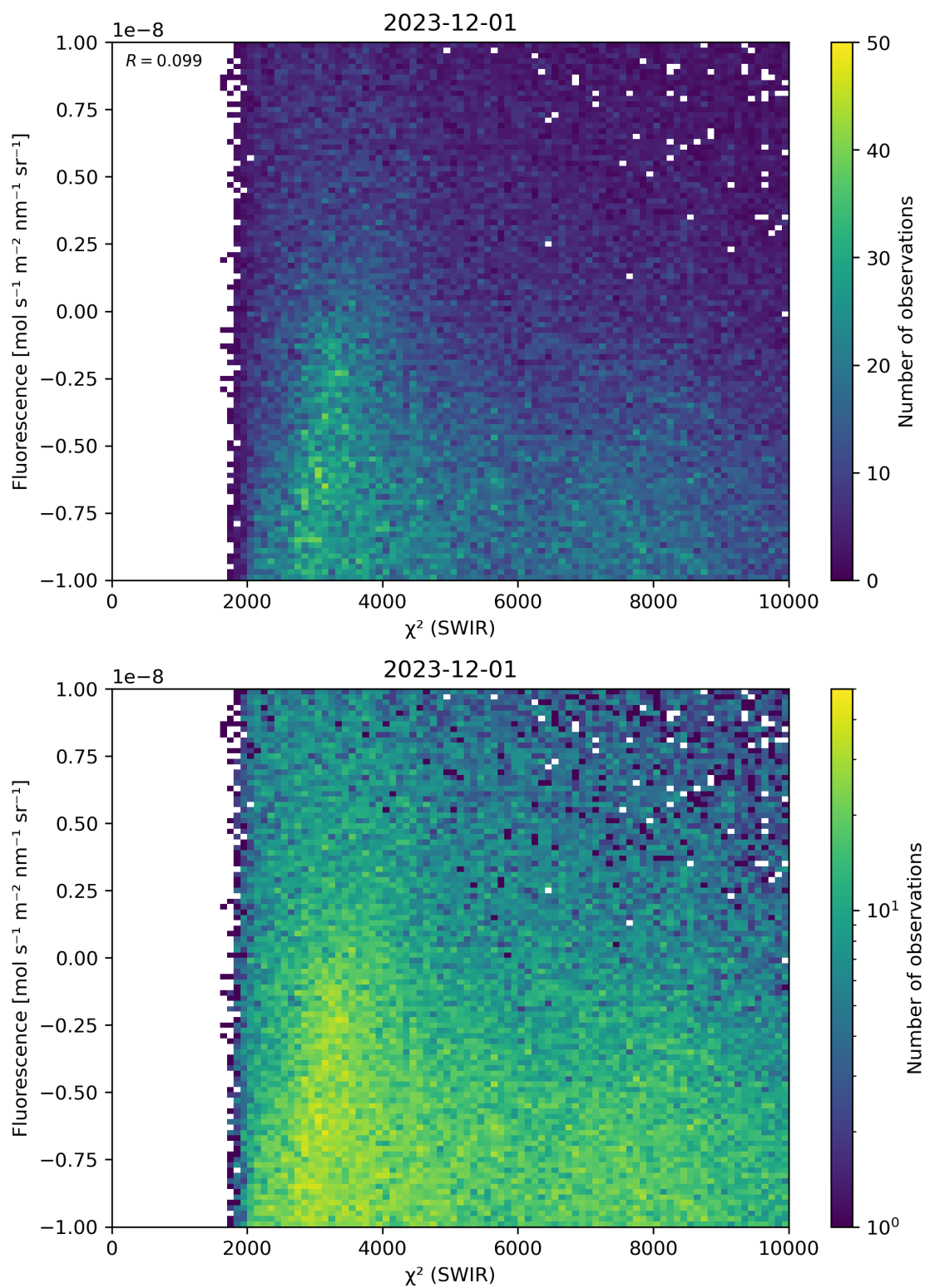
Figure 49: Scatter density plot of “ \chi^2 (SWIR)” against “Fluorescence” for 2023-11-30 to 2023-12-02.
