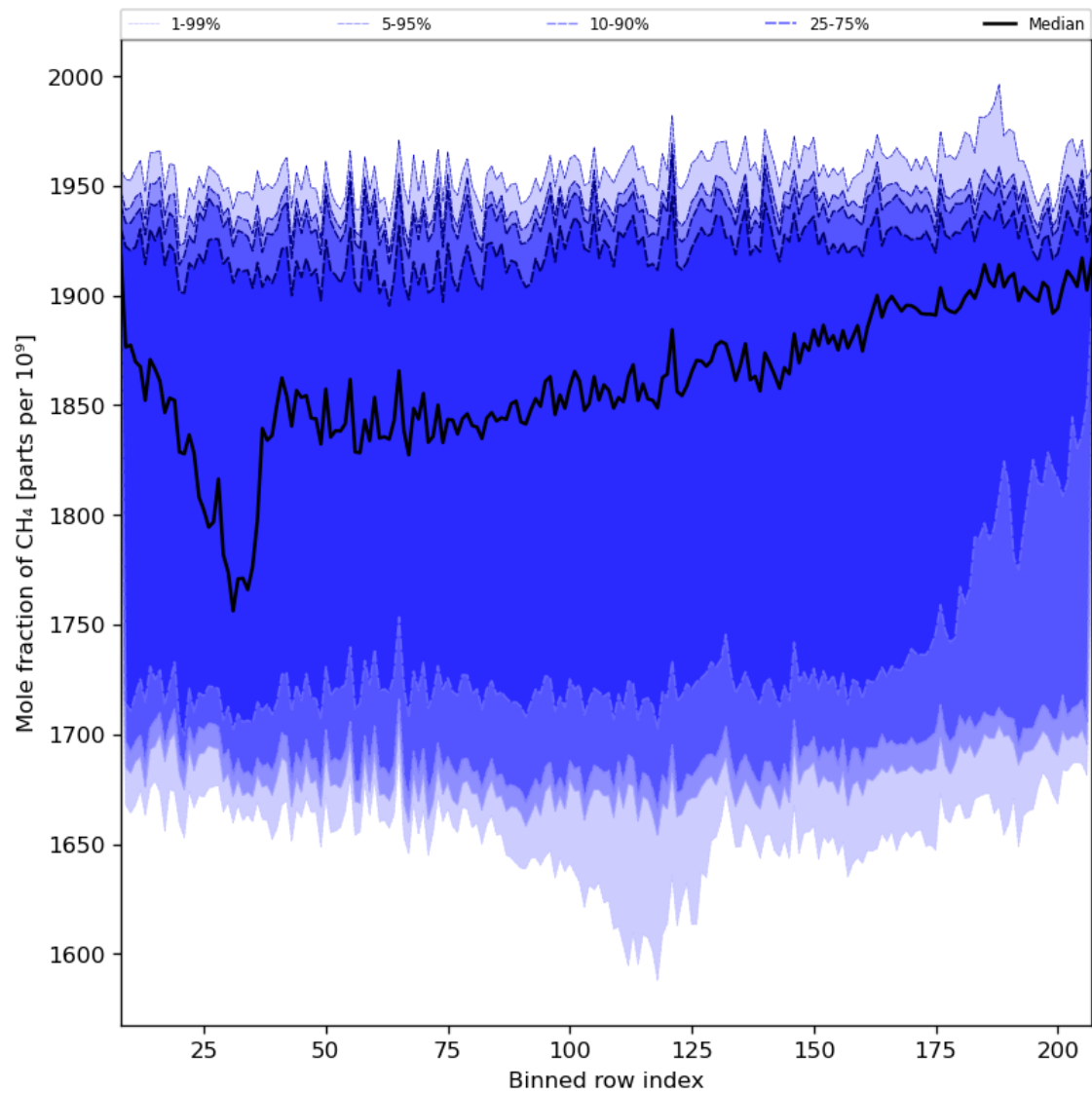
Figure 34: Along track statistics of “Mole fraction of CH 4 ” for 2023-11-30 to 2023-12-02
