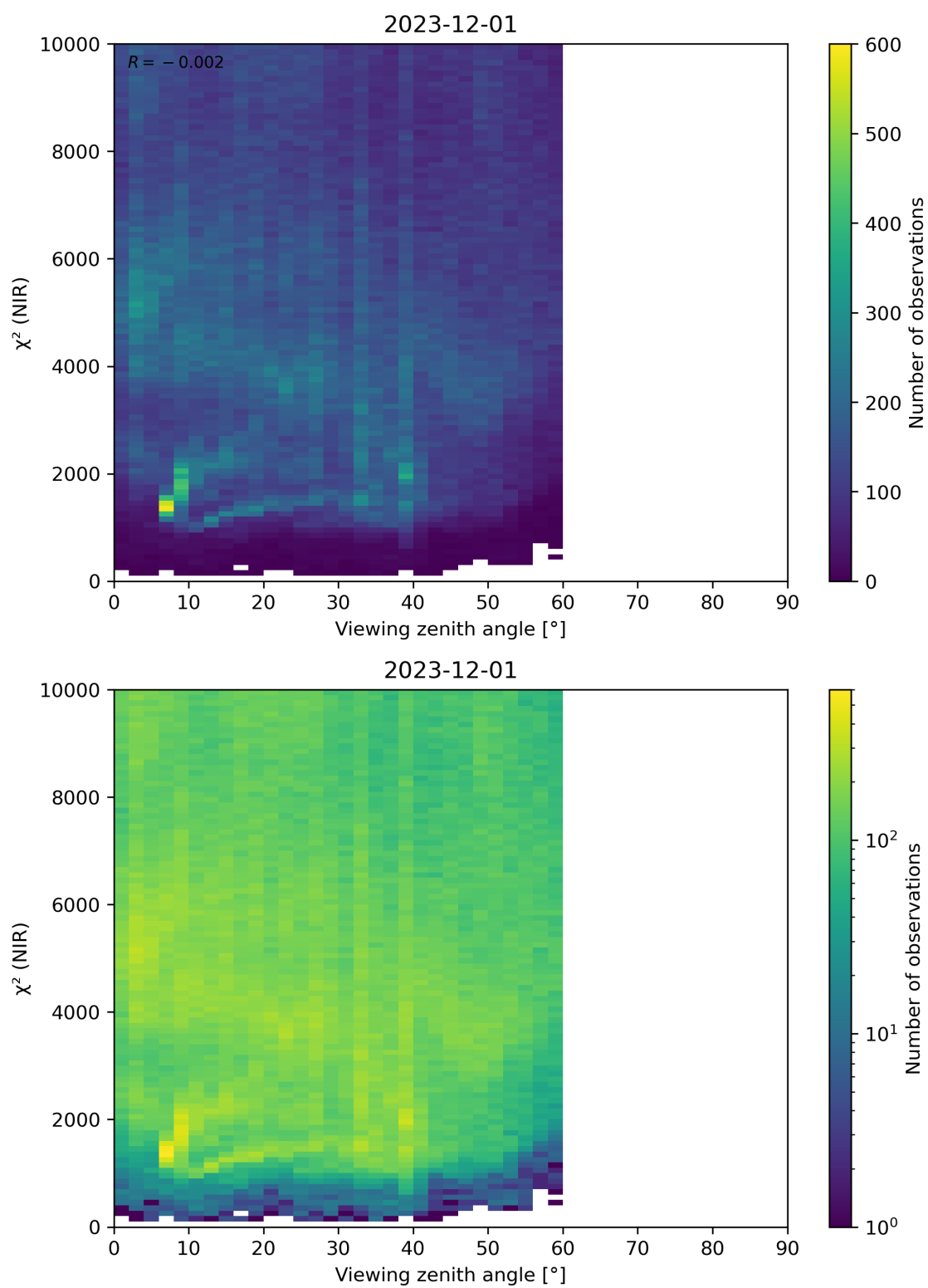
Figure 105: Scatter density plot of “Viewing zenith angle” against “ \chi^2 (NIR)” for 2023-11-30 to 2023-12-02.
