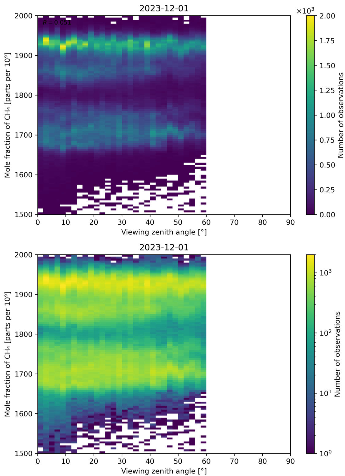
Figure 110: Scatter density plot of “Viewing zenith angle” against “Mole fraction of CH 4 ” for 2023-11-30 to 2023-12-02.
