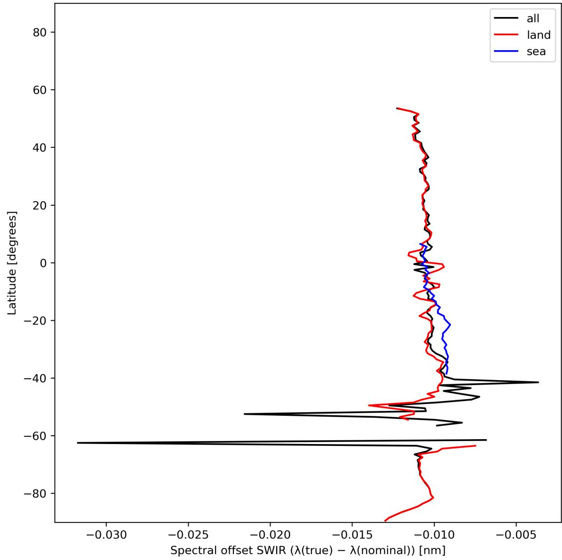
Figure 16: Zonal average of “Spectral offset SWIR ( \lambda(\text{true}) - \lambda(\text{nominal}) )” for 2023-11-30 to 2023-12-02.
