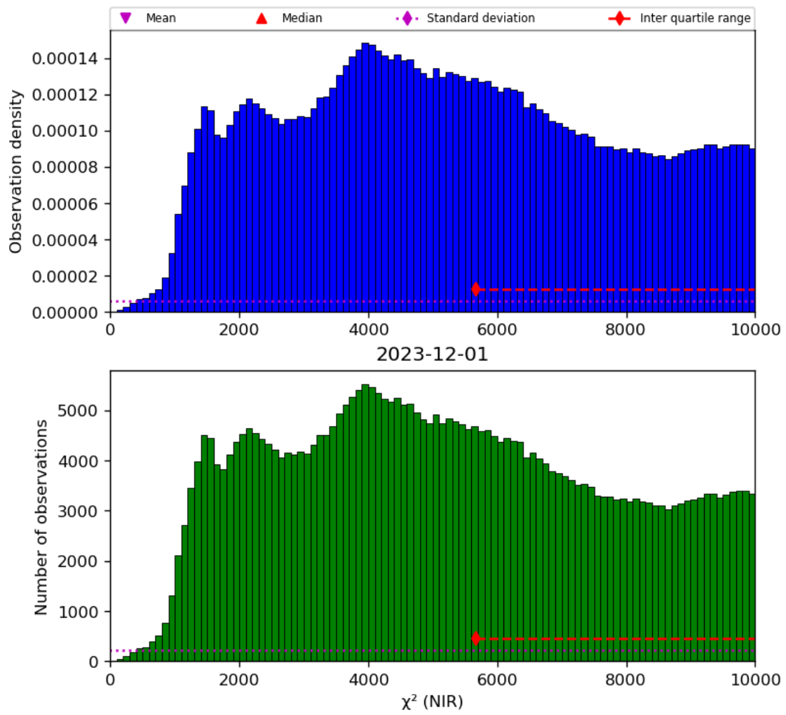
Figure 29: Histogram of “ \chi^2 (NIR)” for 2023-11-30 to 2023-12-02
