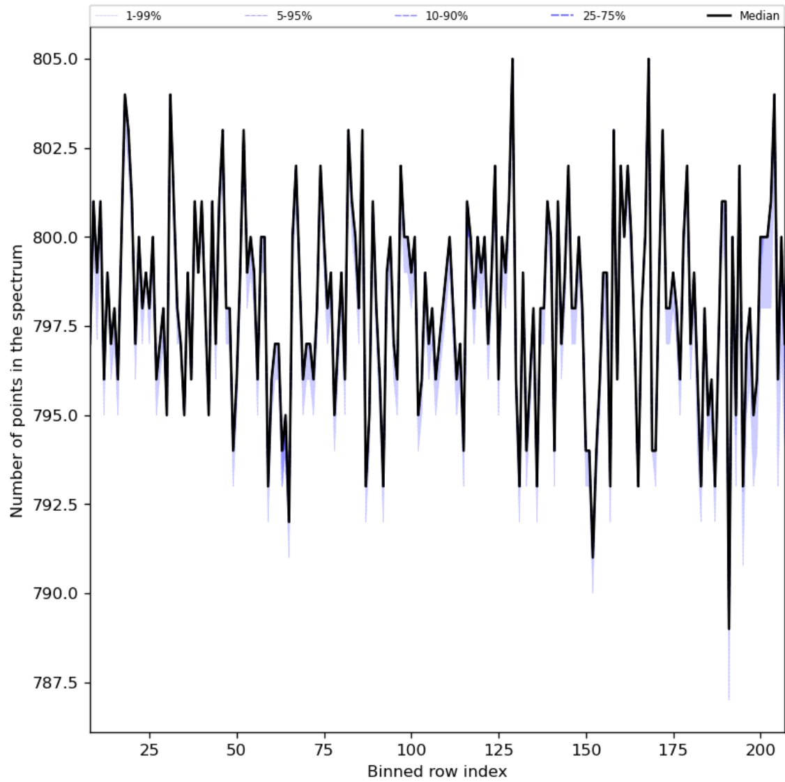
Figure 37: Along track statistics of “Number of points in the spectrum” for 2023-11-30 to 2023-12-02
