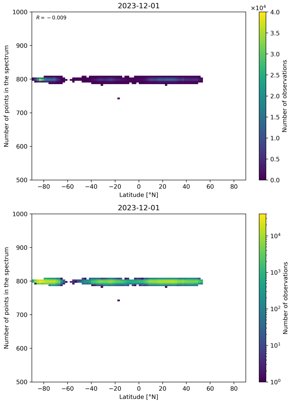
Figure 61: Scatter density plot of “Latitude” against “Number of points in the spectrum” for 2023-11-30 to 2023-12-02.
