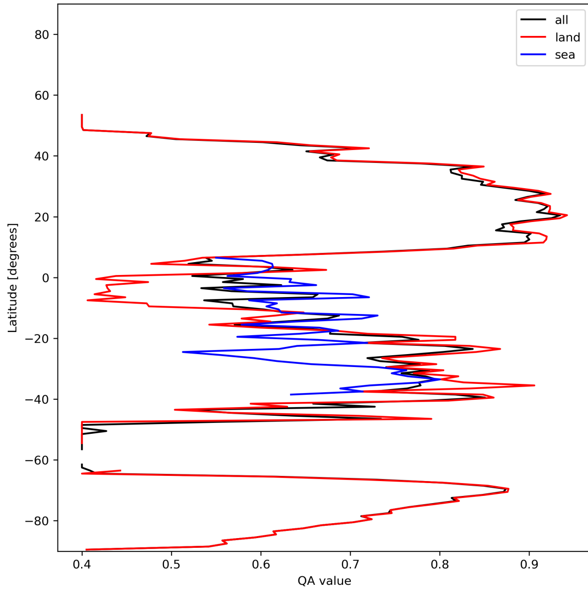
Figure 11: Zonal average of “QA value” for 2023-11-30 to 2023-12-02.
