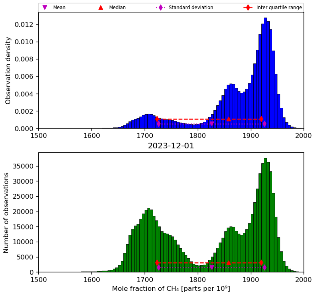
Figure 23: Histogram of “Mole fraction of CH 4 ” for 2023-11-30 to 2023-12-02
