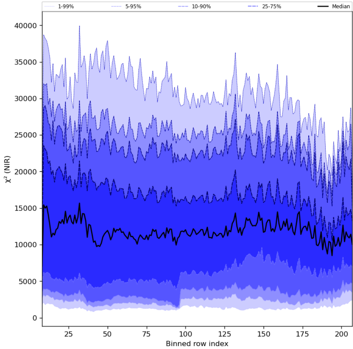
Figure 40: Along track statistics of “ \chi^2 (NIR)” for 2023-11-30 to 2023-12-02
