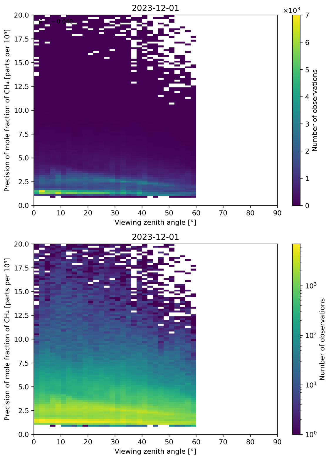
Figure 112: Scatter density plot of “Viewing zenith angle” against “Precision of mole fraction of CH 4 ” for 2023-11-30 to 2023-12-02.
