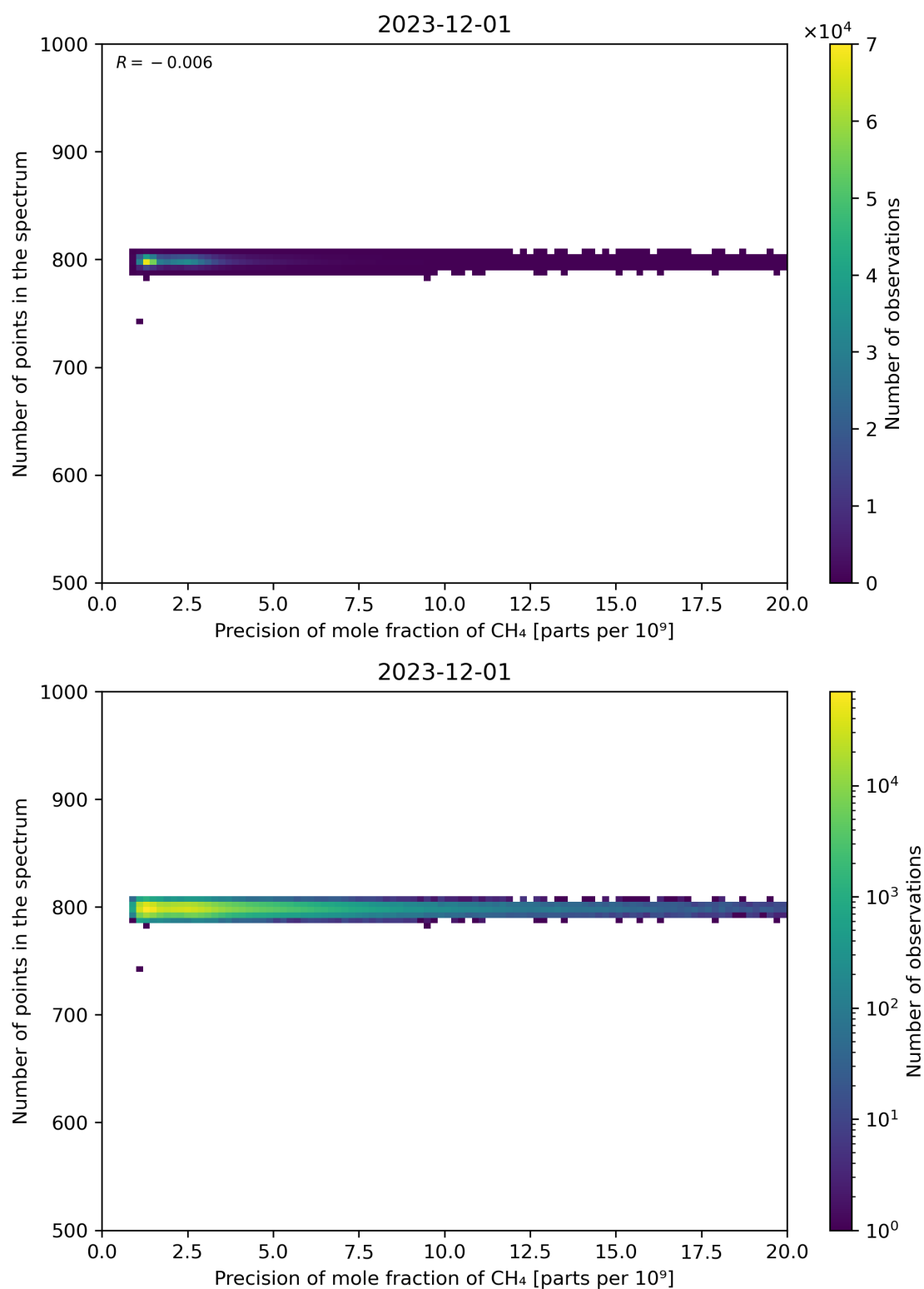
Figure 84: Scatter density plot of “Precision of mole fraction of CH 4 ” against “Number of points in the spectrum” for 2023-11-30 to 2023-12-02.
