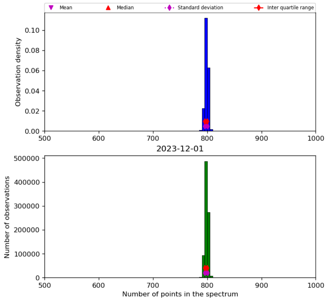
Figure 26: Histogram of “Number of points in the spectrum” for 2023-11-30 to 2023-12-02
