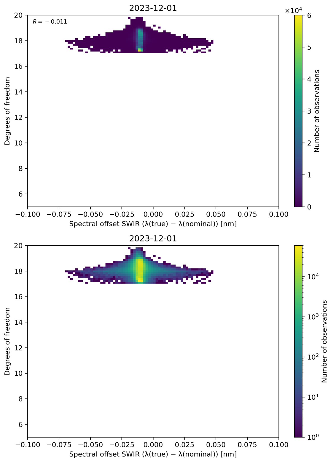
Figure 119: Scatter density plot of “Spectral offset SWIR ( \lambda(\text{true}) - \lambda(\text{nominal}) )” against “Degrees of freedom” for 2023-11-30 to 2023-12-02.
