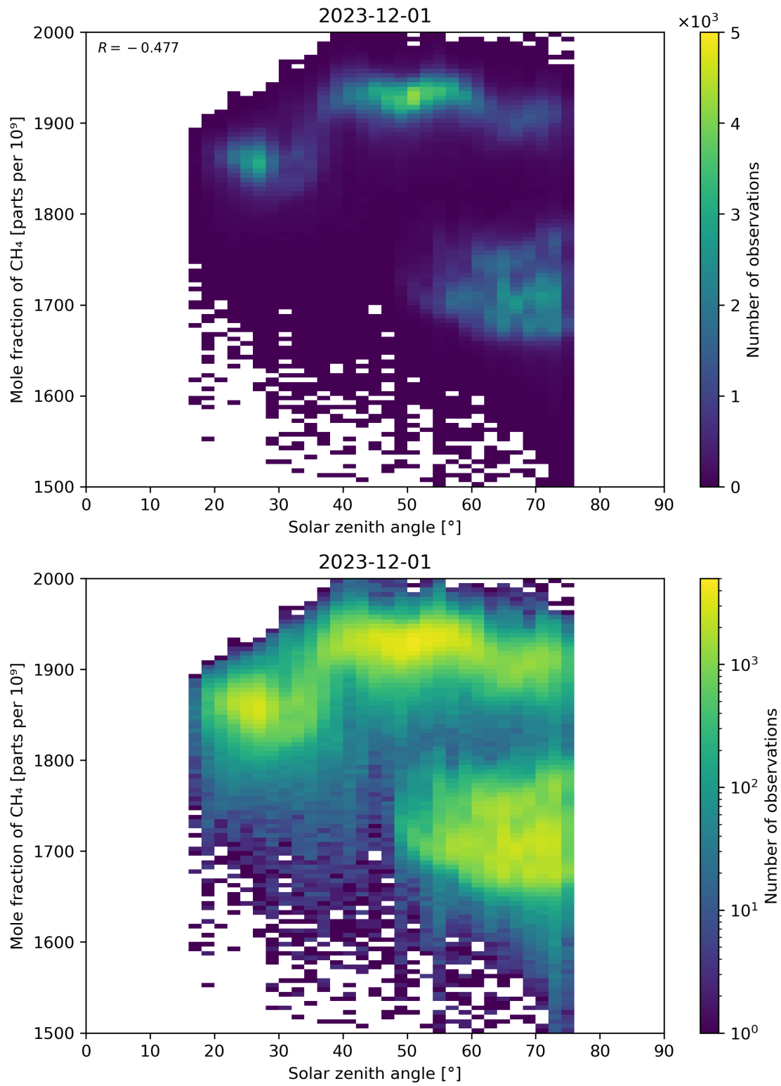
Figure 99: Scatter density plot of “Solar zenith angle” against “Mole fraction of CH 4 ” for 2023-11-30 to 2023-12-02.
