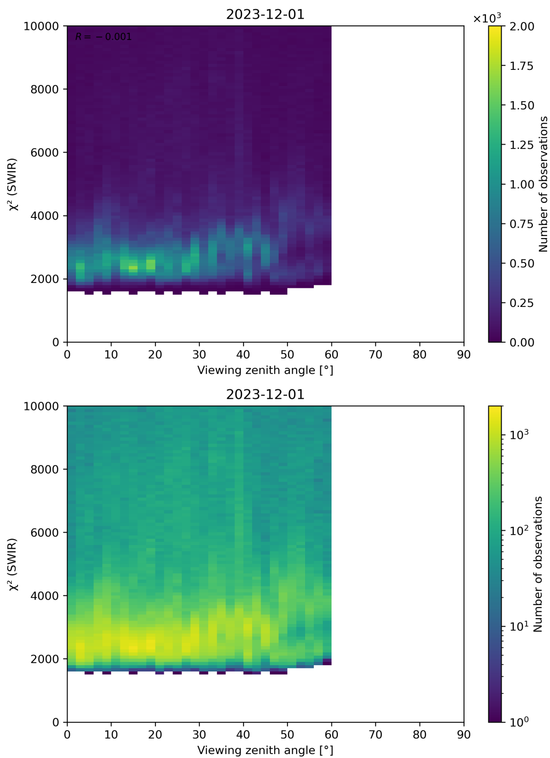
Figure 106: Scatter density plot of “Viewing zenith angle” against “ \chi^2 (SWIR)” for 2023-11-30 to 2023-12-02.
