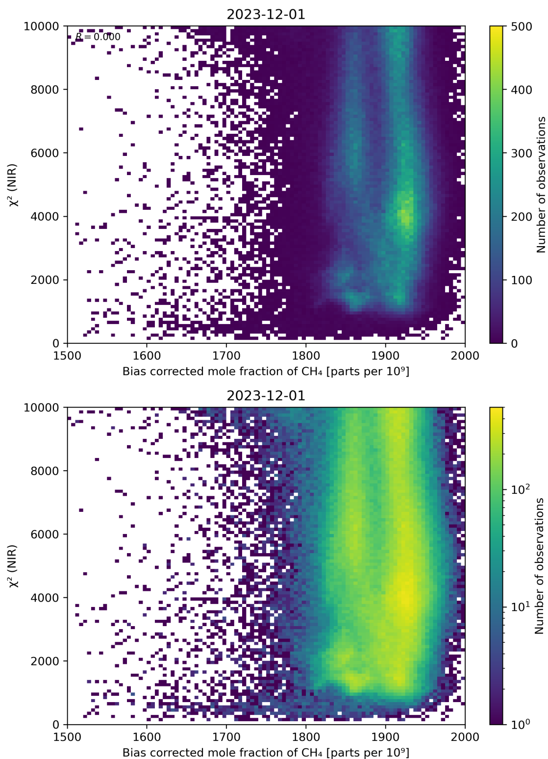
Figure 63: Scatter density plot of “Bias corrected mole fraction of CH 4 ” against “ \chi^2 (NIR)” for 2023-11-30 to 2023-12-02.
