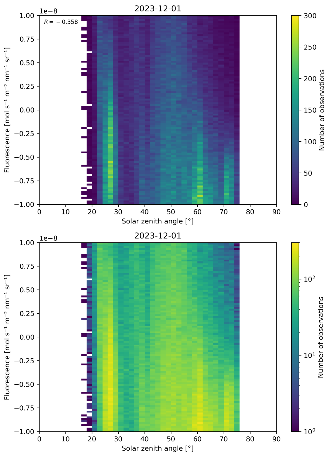
Figure 97: Scatter density plot of “Solar zenith angle” against “Fluorescence” for 2023-11-30 to 2023-12-02.
