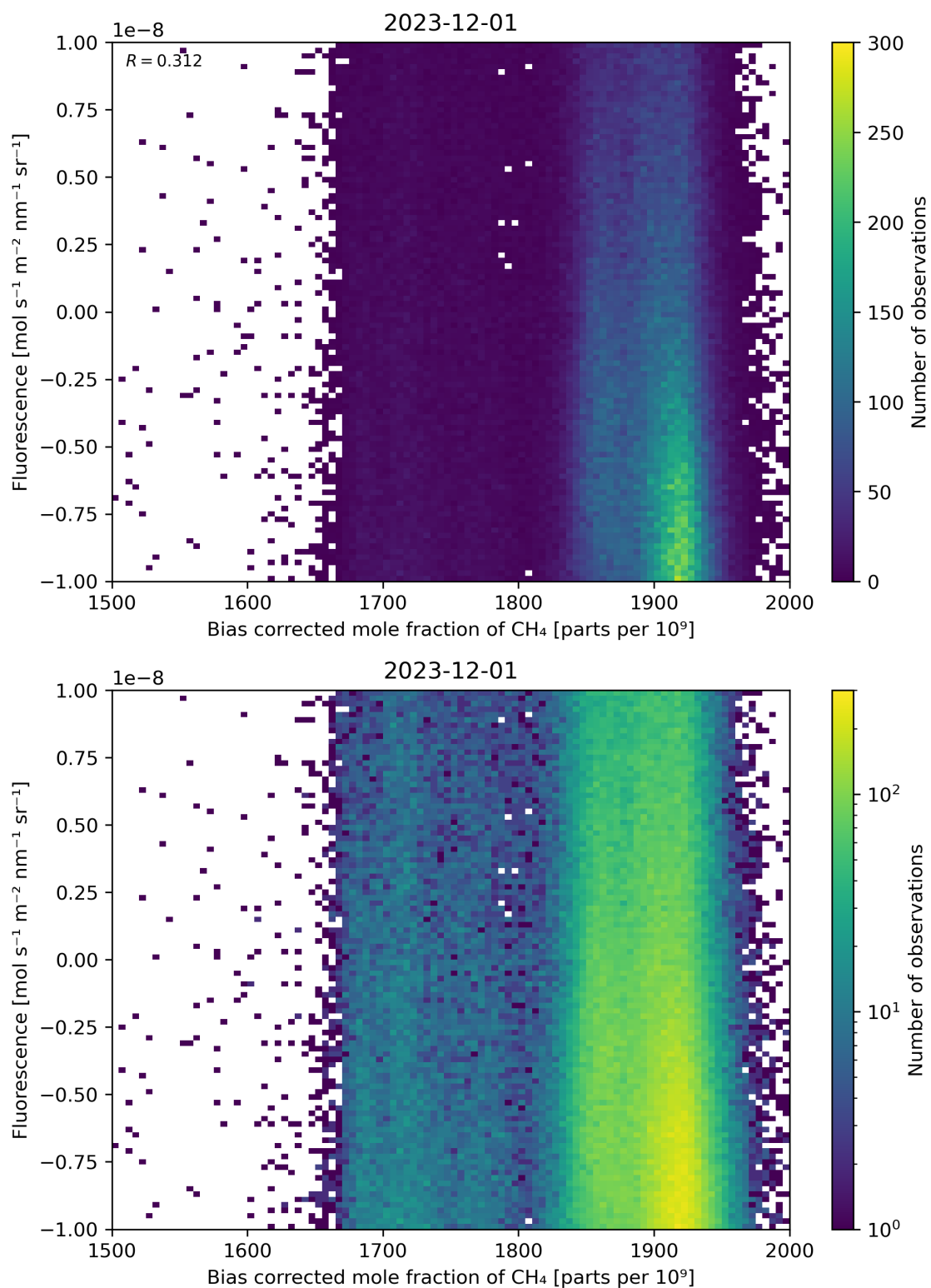
Figure 66: Scatter density plot of “Bias corrected mole fraction of \text{CH}_4 ” against “Fluorescence” for 2023-11-30 to 2023-12-02.
