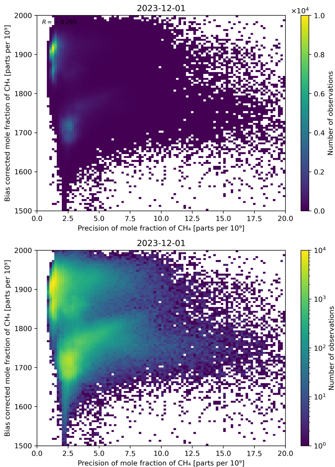
Figure 82: Scatter density plot of “Precision of mole fraction of CH 4 ” against “Bias corrected mole fraction of CH 4 ” for 2023-11-30 to 2023-12-02.
