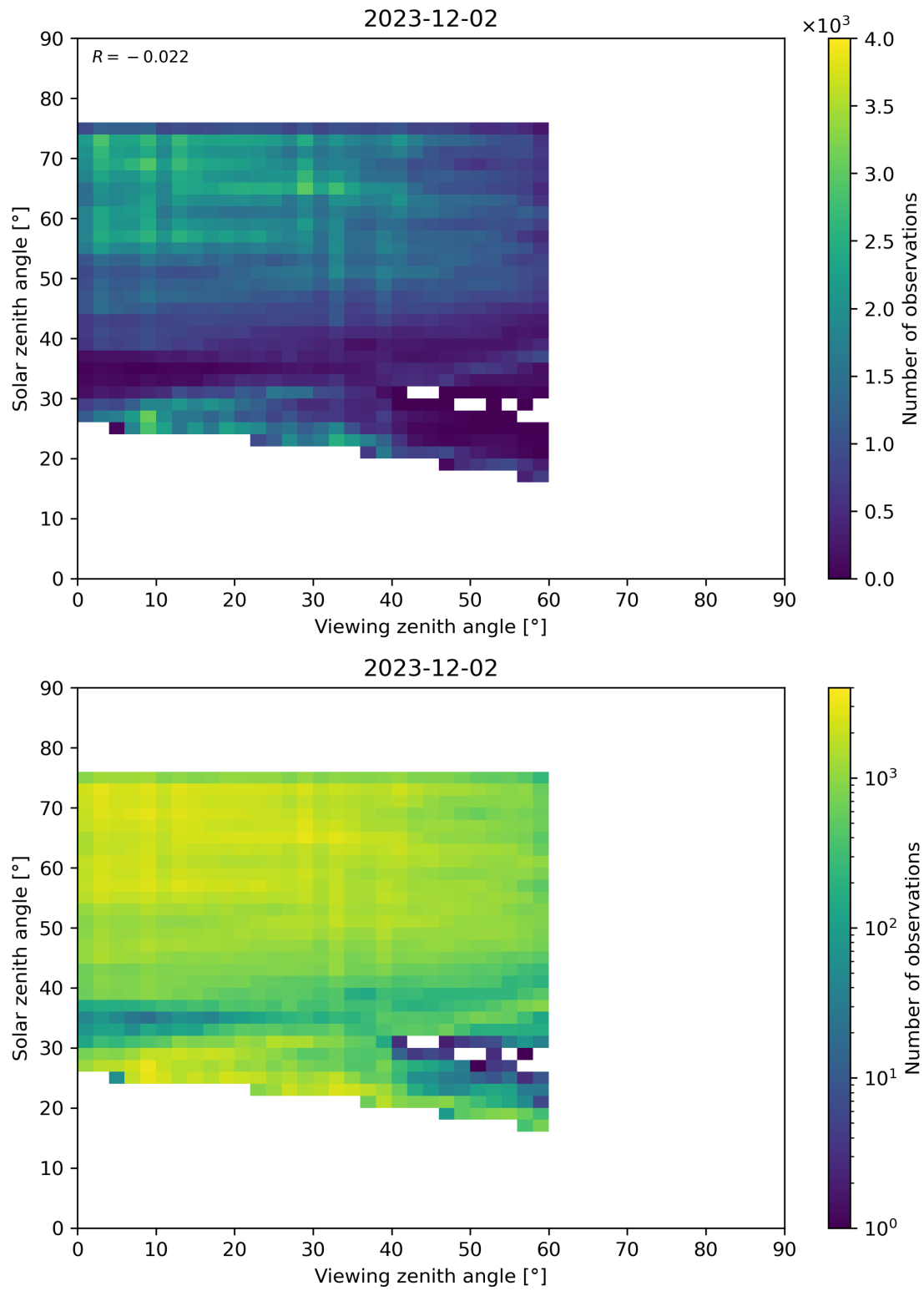
Figure 115: Scatter density plot of “Viewing zenith angle” against “Solar zenith angle” for 2023-12-01 to 2023-12-03.
