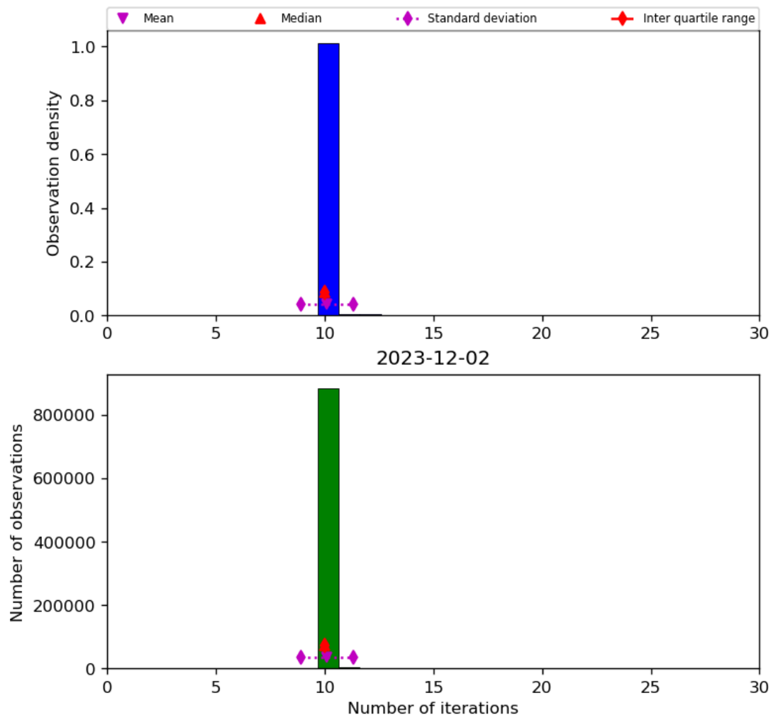
Figure 31: Histogram of “Number of iterations” for 2023-12-01 to 2023-12-03
