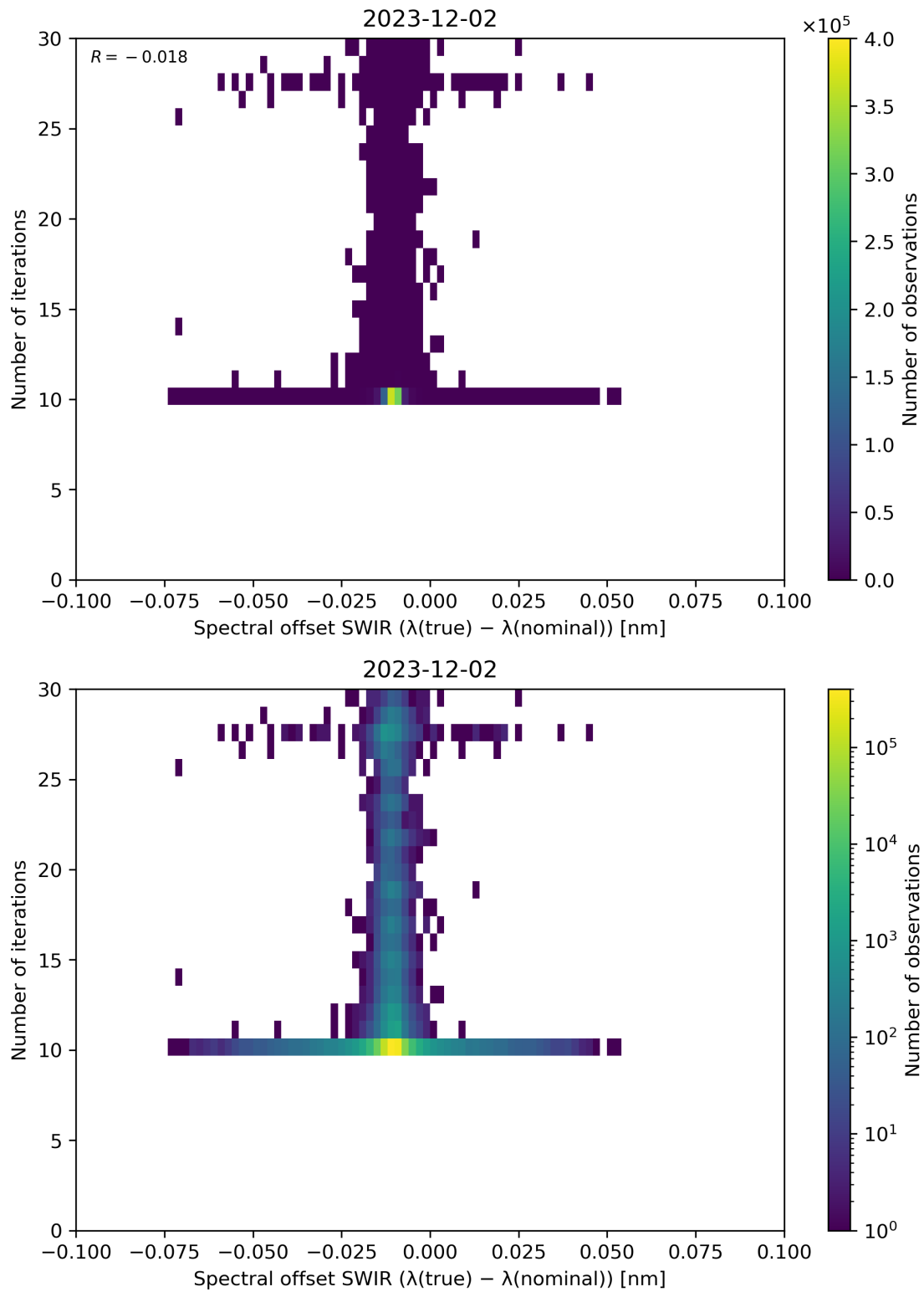
Figure 121: Scatter density plot of “Spectral offset SWIR ( \lambda(\text{true}) - \lambda(\text{nominal}) )” against “Number of iterations” for 2023-12-01 to 2023-12-03.
