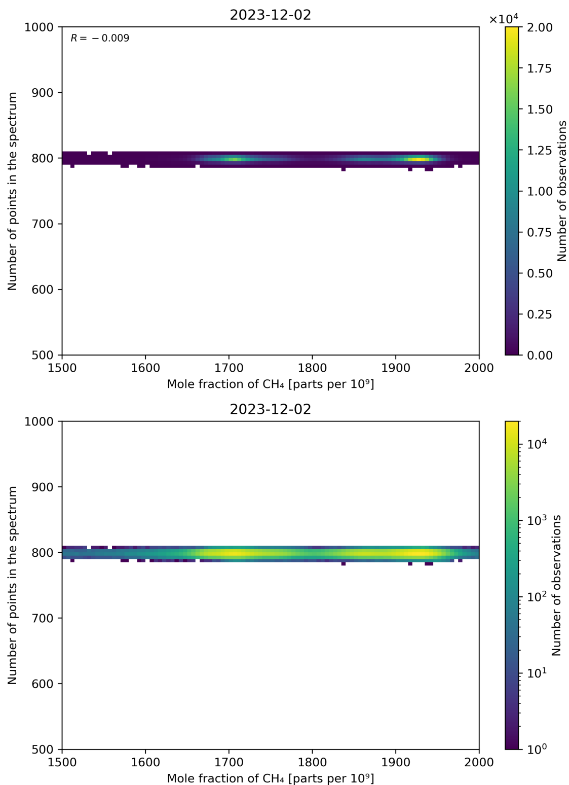
Figure 77: Scatter density plot of “Mole fraction of CH 4 ” against “Number of points in the spectrum” for 2023-12-01 to 2023-12-03.
