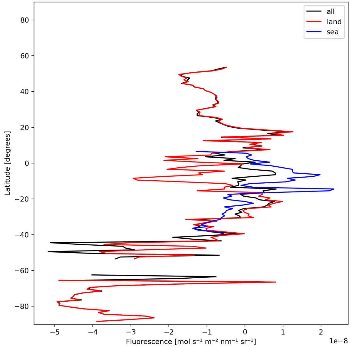
Figure 21: Zonal average of “Fluorescence” for 2023-12-01 to 2023-12-03.
