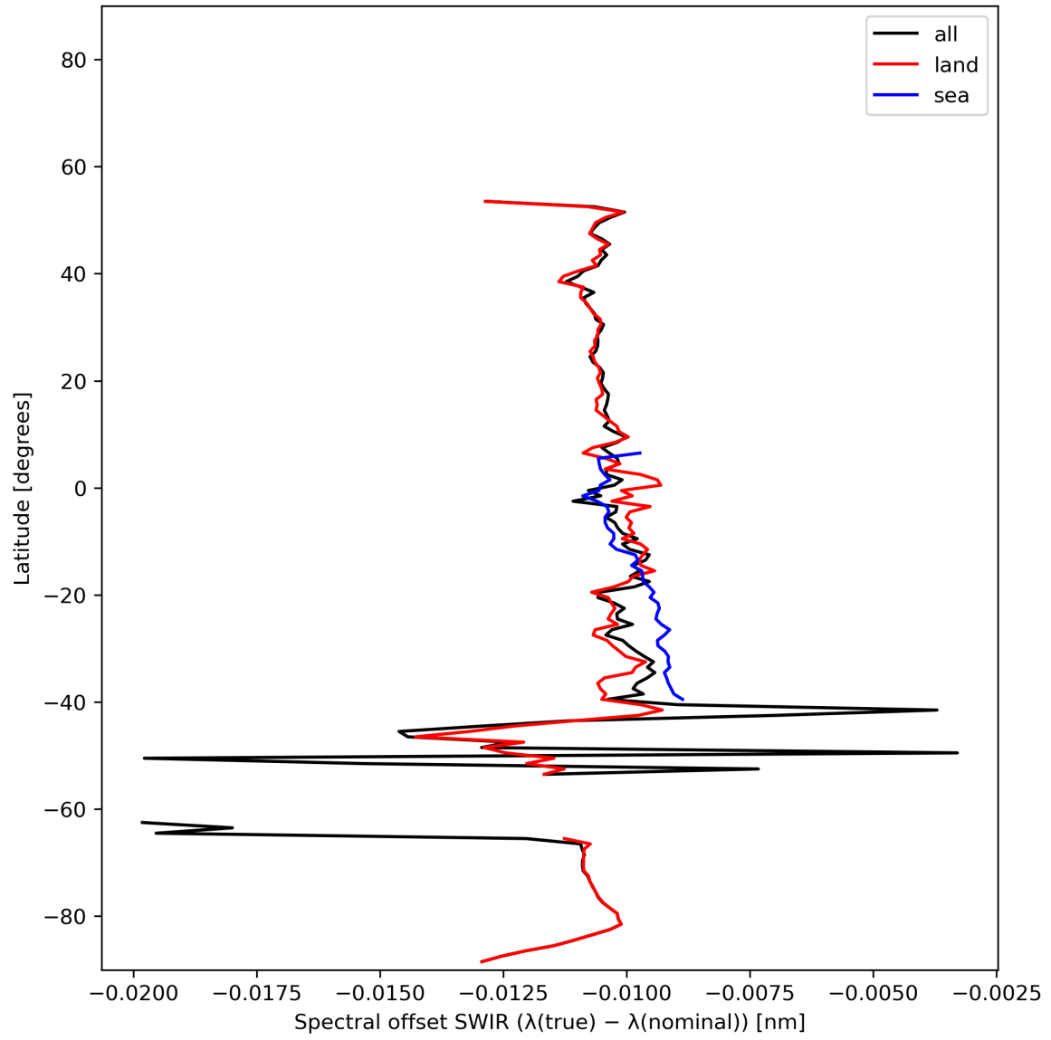
Figure 16: Zonal average of “Spectral offset SWIR ( \lambda(\text{true}) - \lambda(\text{nominal}) )” for 2023-12-01 to 2023-12-03.
