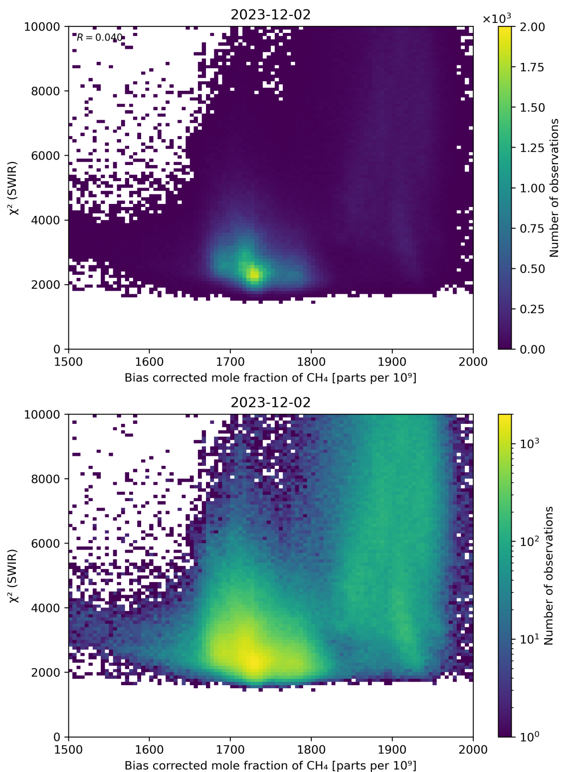
Figure 64: Scatter density plot of “Bias corrected mole fraction of CH 4 ” against “ \chi^2 (SWIR)” for 2023-12-01 to 2023-12-03.
