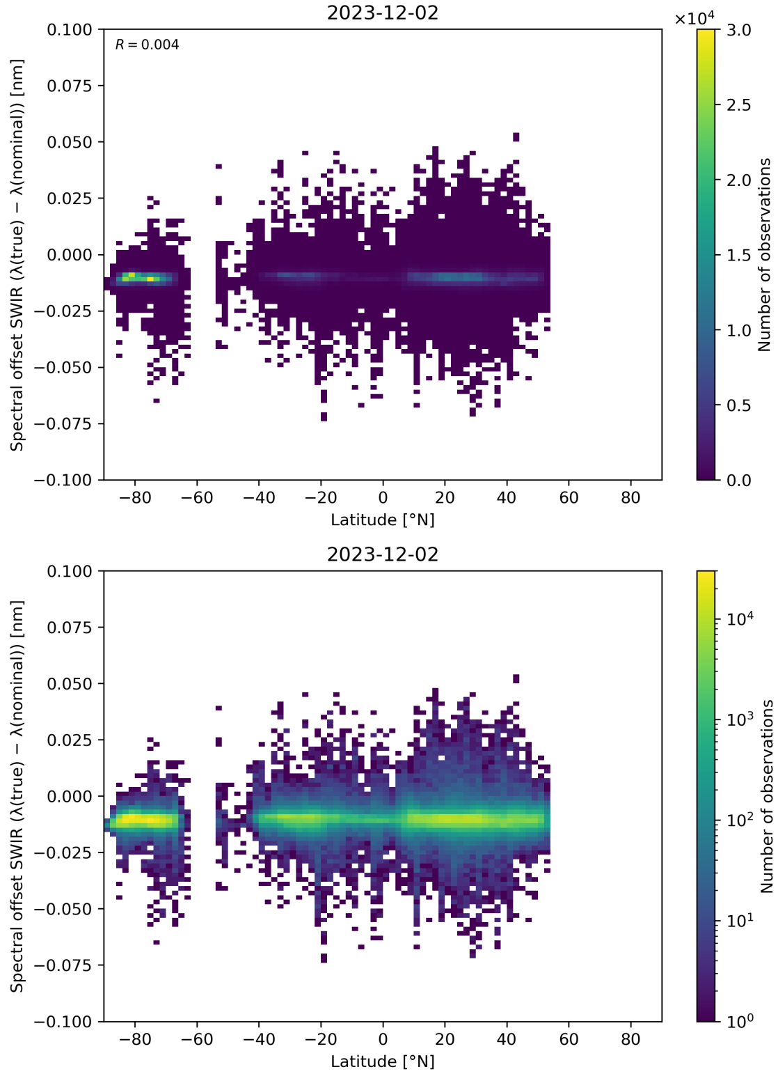
Figure 62: Scatter density plot of “Latitude” against “Spectral offset SWIR ( \lambda(\text{true}) - \lambda(\text{nominal}) )” for 2023-12-01 to 2023-12-03.
