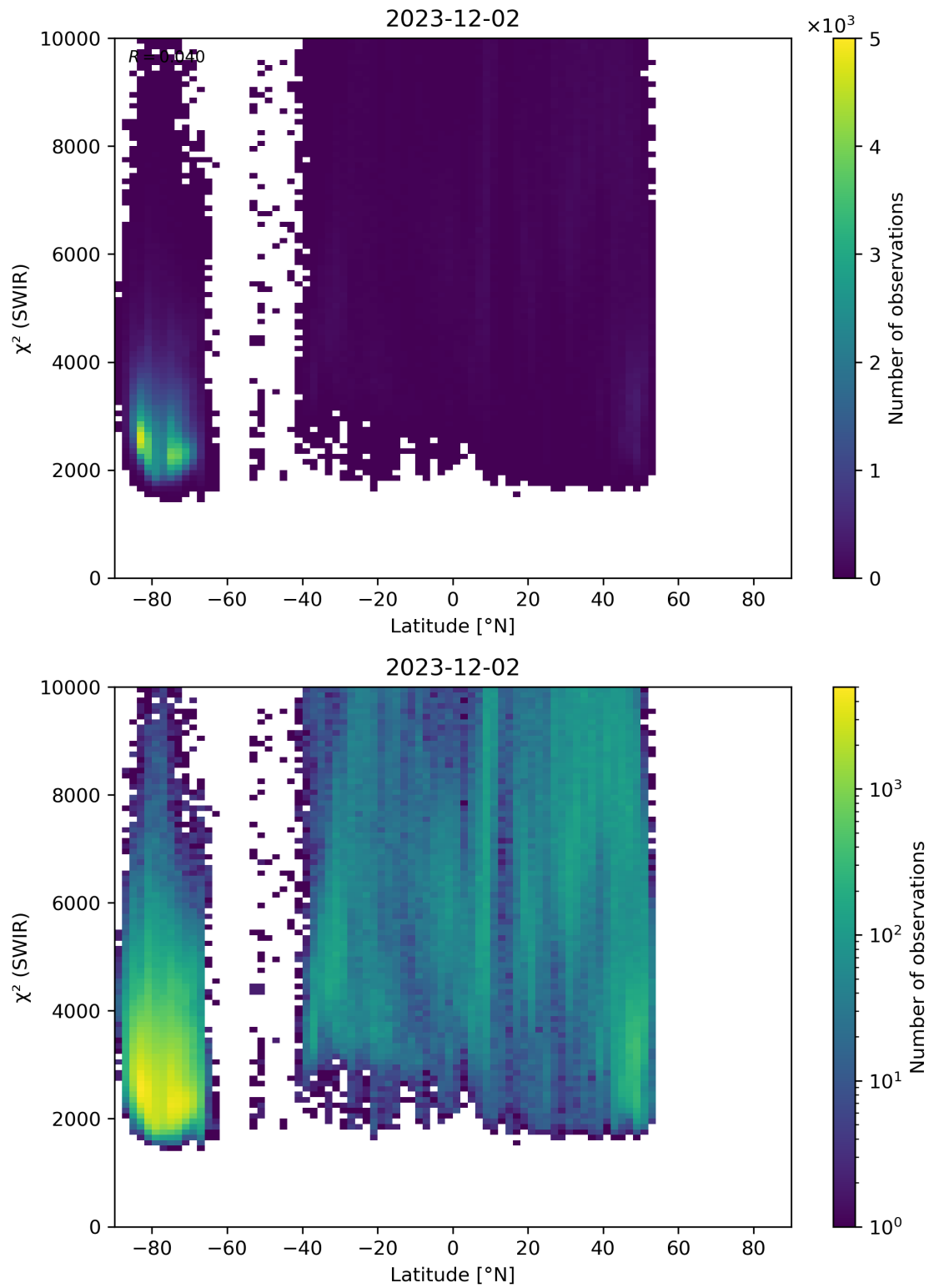
Figure 54: Scatter density plot of “Latitude” against “ \chi^2 (SWIR)” for 2023-12-01 to 2023-12-03.
