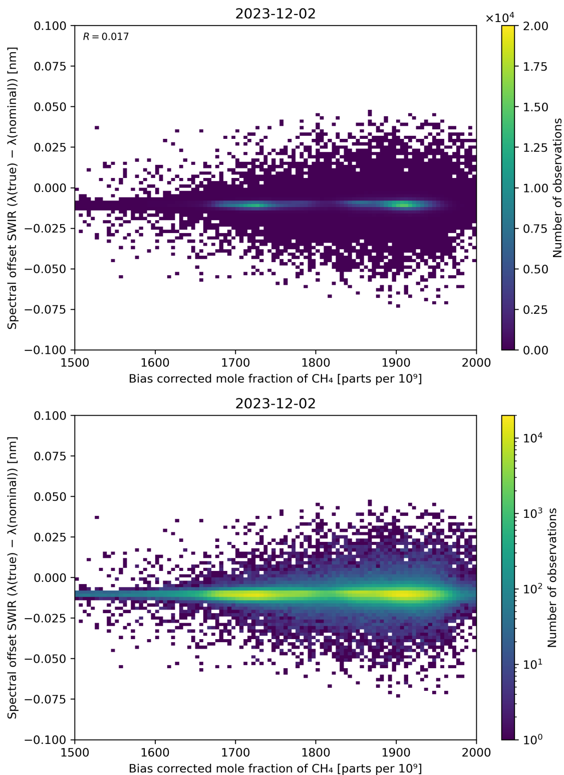
Figure 69: Scatter density plot of “Bias corrected mole fraction of \text{CH}_4 ” against “Spectral offset SWIR ( \lambda(\text{true}) - \lambda(\text{nominal}) )” for 2023-12-01 to 2023-12-03.
