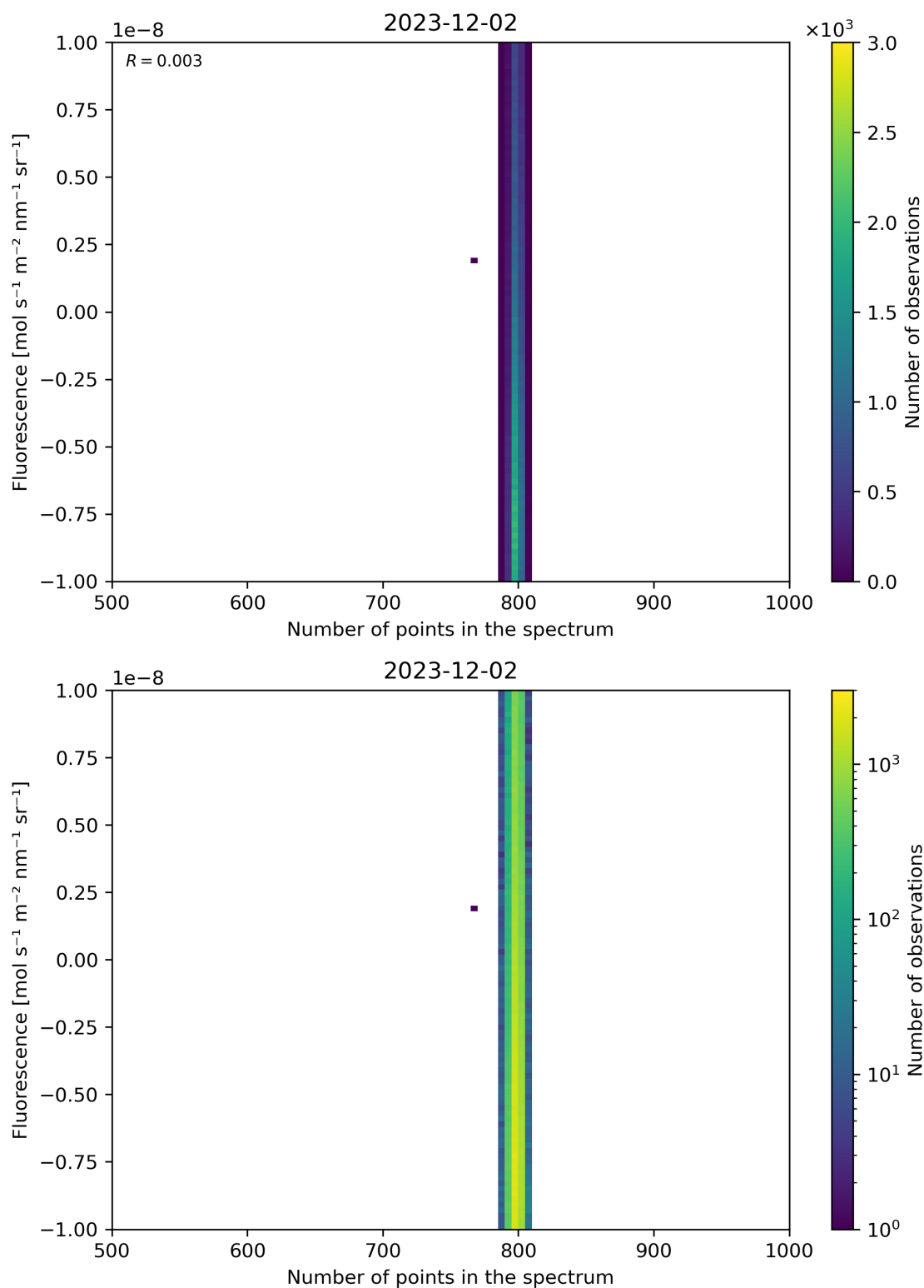
Figure 91: Scatter density plot of “Number of points in the spectrum” against “Fluorescence” for 2023-12-01 to 2023-12-03.
