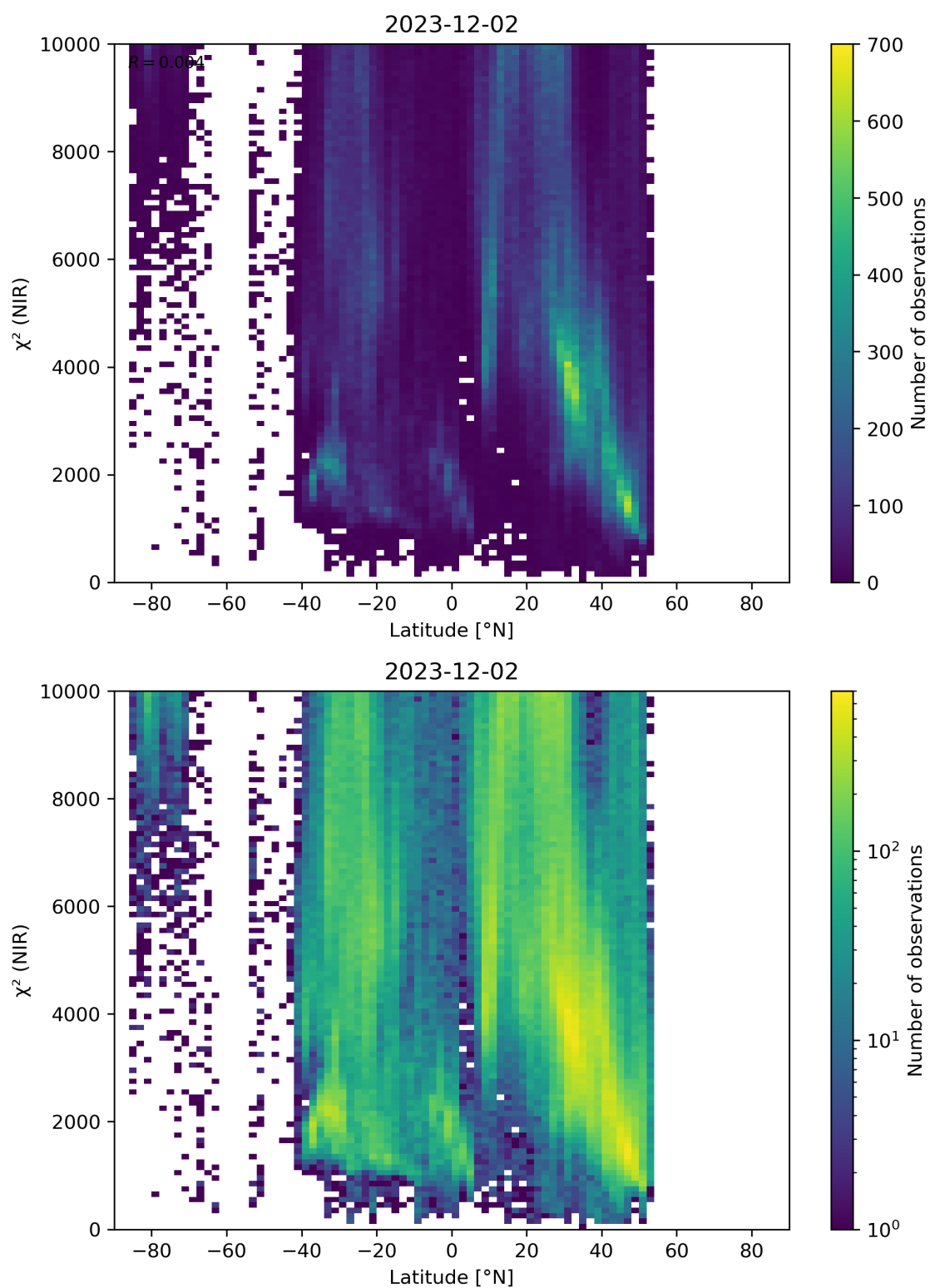
Figure 53: Scatter density plot of “Latitude” against “ \chi^2 (NIR)” for 2023-12-01 to 2023-12-03.
