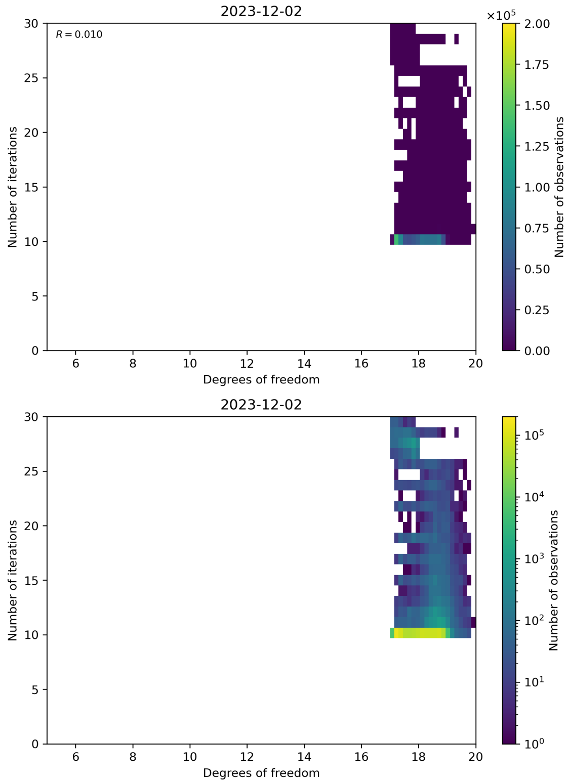
Figure 52: Scatter density plot of “Degrees of freedom” against “Number of iterations” for 2023-12-01 to 2023-12-03.
