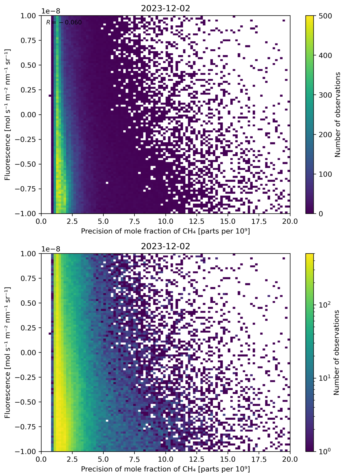
Figure 81: Scatter density plot of “Precision of mole fraction of \text{CH}_4 ” against “Fluorescence” for 2023-12-01 to 2023-12-03.
