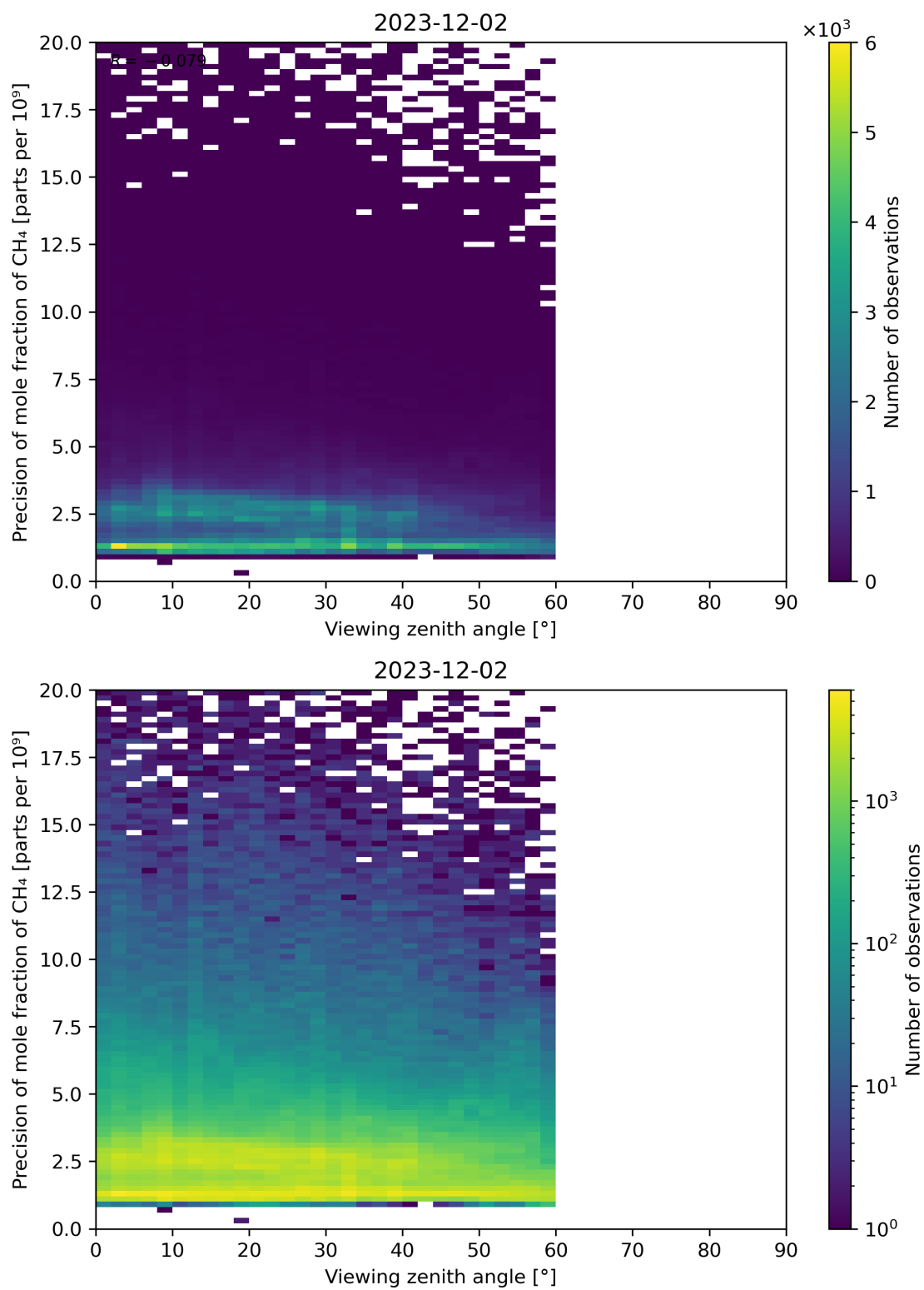
Figure 112: Scatter density plot of “Viewing zenith angle” against “Precision of mole fraction of CH 4 ” for 2023-12-01 to 2023-12-03.
