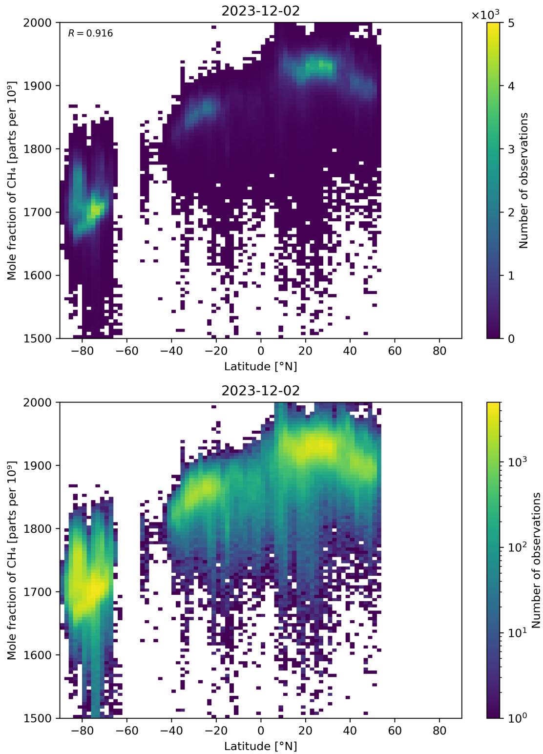
Figure 57: Scatter density plot of “Latitude” against “Mole fraction of CH 4 ” for 2023-12-01 to 2023-12-03.
