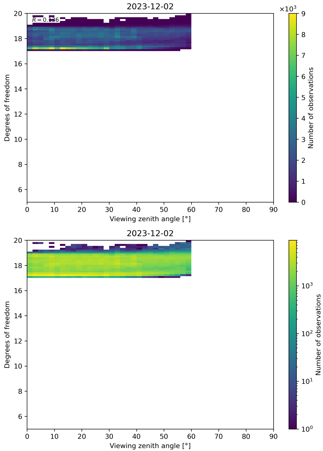
Figure 107: Scatter density plot of “Viewing zenith angle” against “Degrees of freedom” for 2023-12-01 to 2023-12-03.
