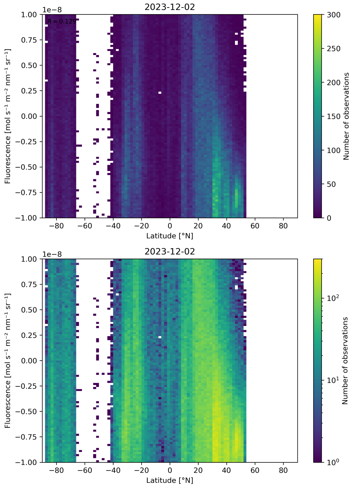
Figure 56: Scatter density plot of “Latitude” against “Fluorescence” for 2023-12-01 to 2023-12-03.
