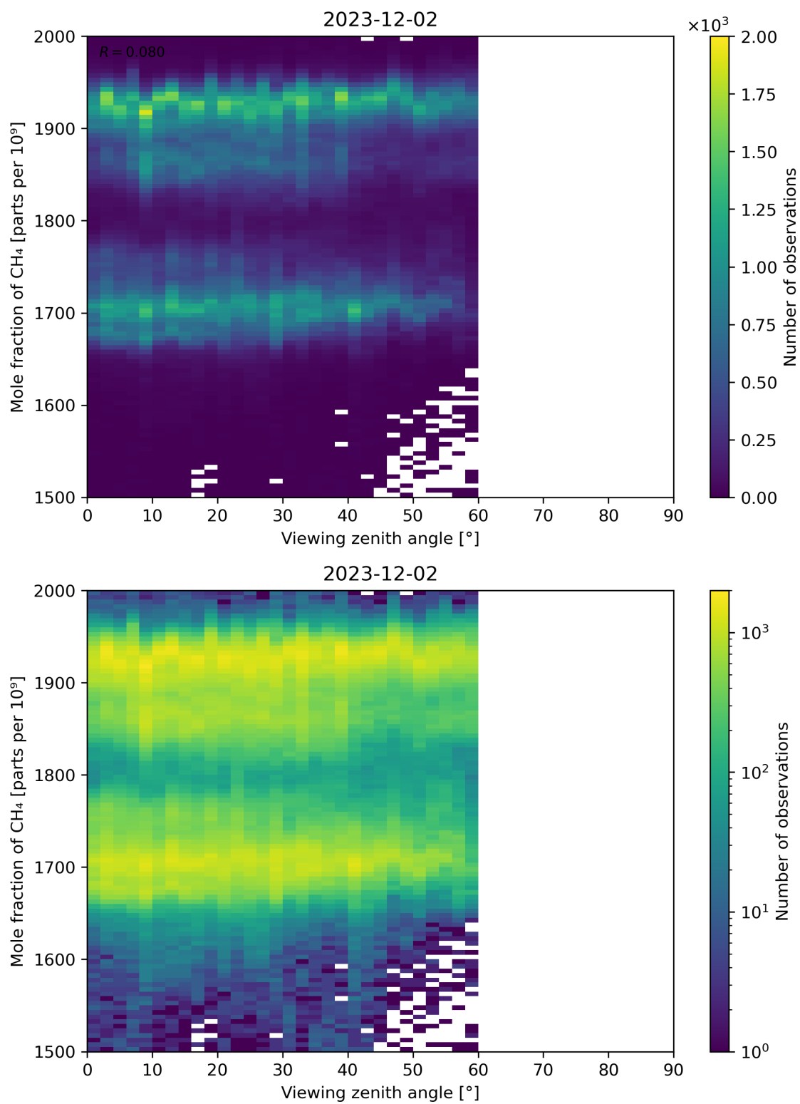
Figure 110: Scatter density plot of “Viewing zenith angle” against “Mole fraction of CH 4 ” for 2023-12-01 to 2023-12-03.
