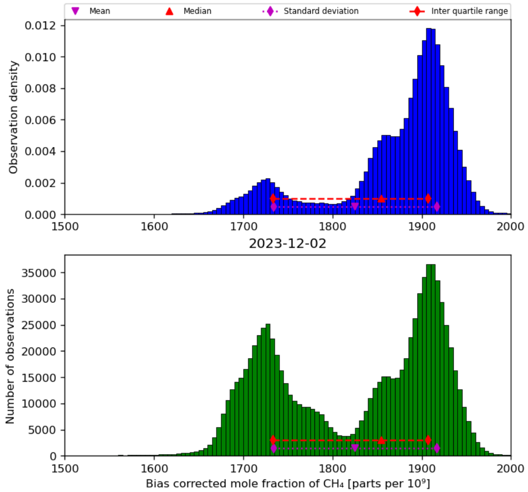
Figure 25: Histogram of “Bias corrected mole fraction of CH 4 ” for 2023-12-01 to 2023-12-03
