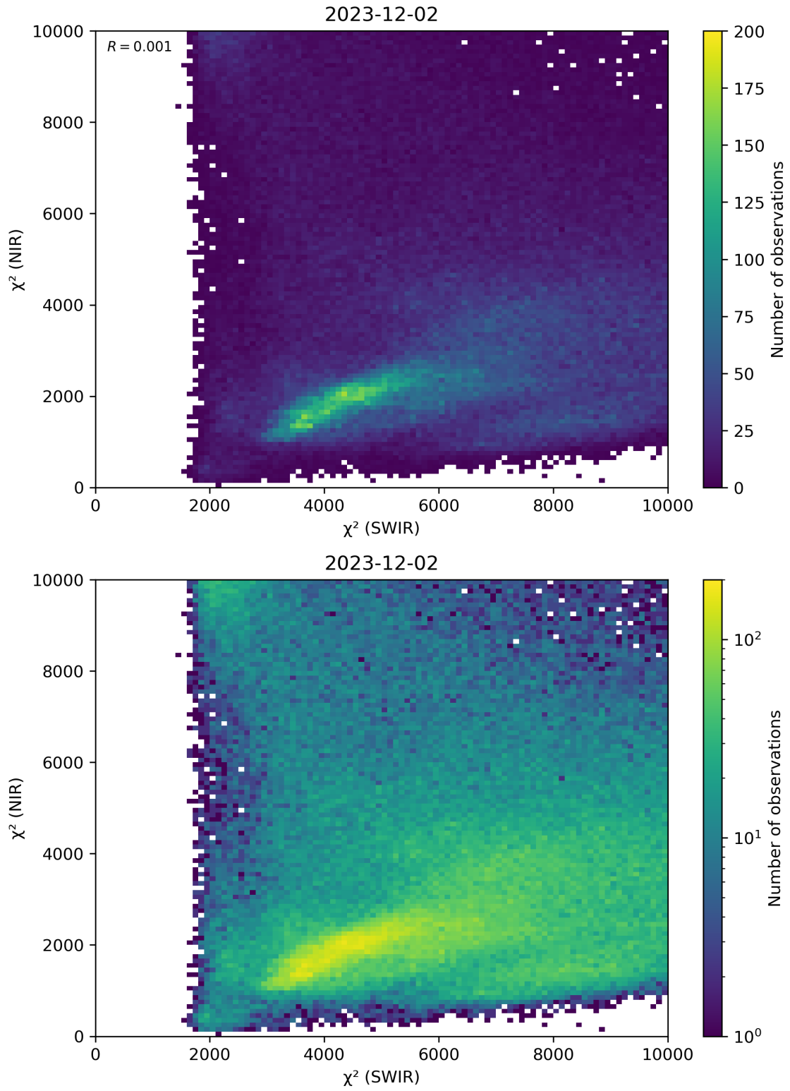
Figure 47: Scatter density plot of “ \chi^2 (SWIR)” against “ \chi^2 (NIR)” for 2023-12-01 to 2023-12-03.
