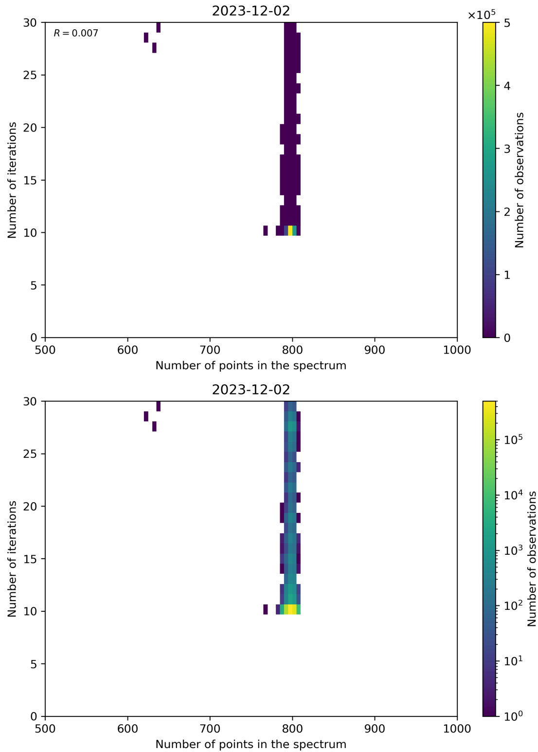
Figure 92: Scatter density plot of “Number of points in the spectrum” against “Number of iterations” for 2023-12-01 to 2023-12-03.
