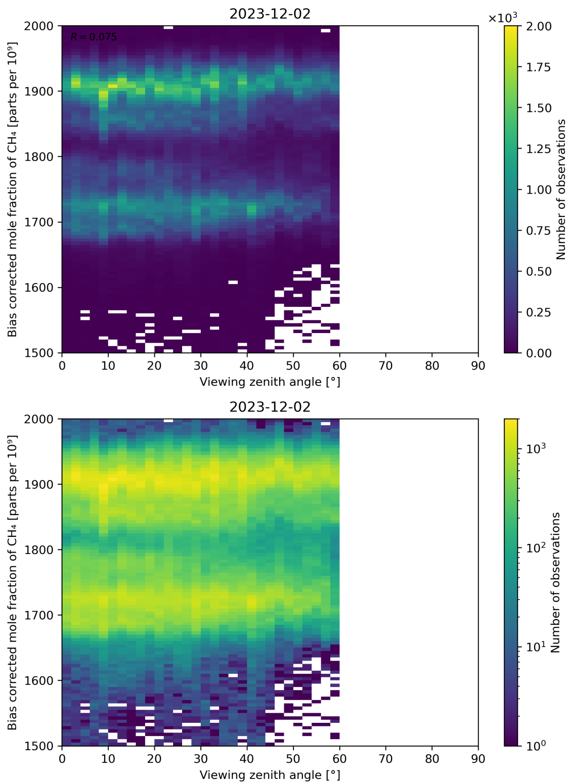
Figure 111: Scatter density plot of “Viewing zenith angle” against “Bias corrected mole fraction of CH 4 ” for 2023-12-01 to 2023-12-03.
