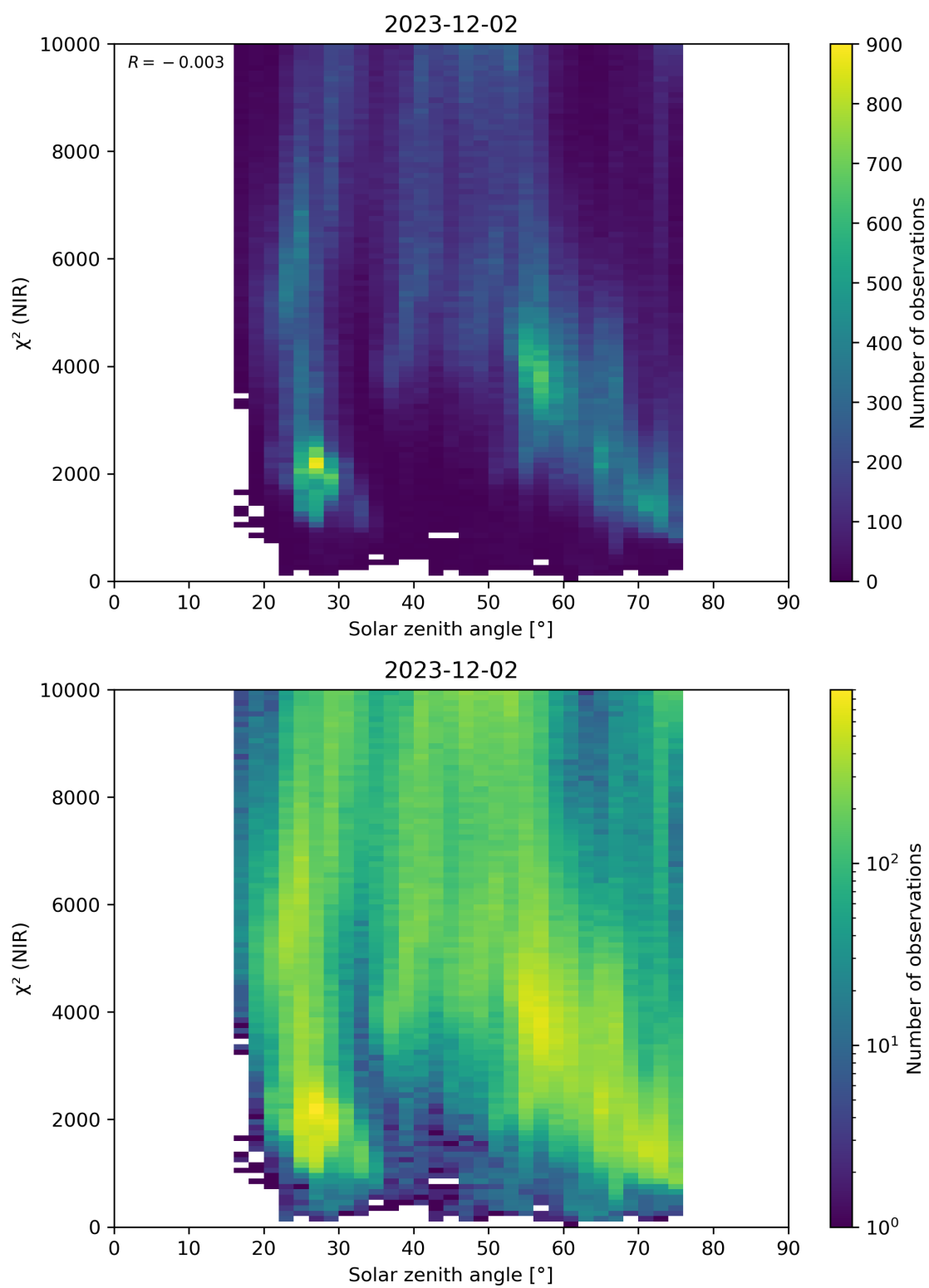
Figure 94: Scatter density plot of “Solar zenith angle” against “ \chi^2 (NIR)” for 2023-12-01 to 2023-12-03.
