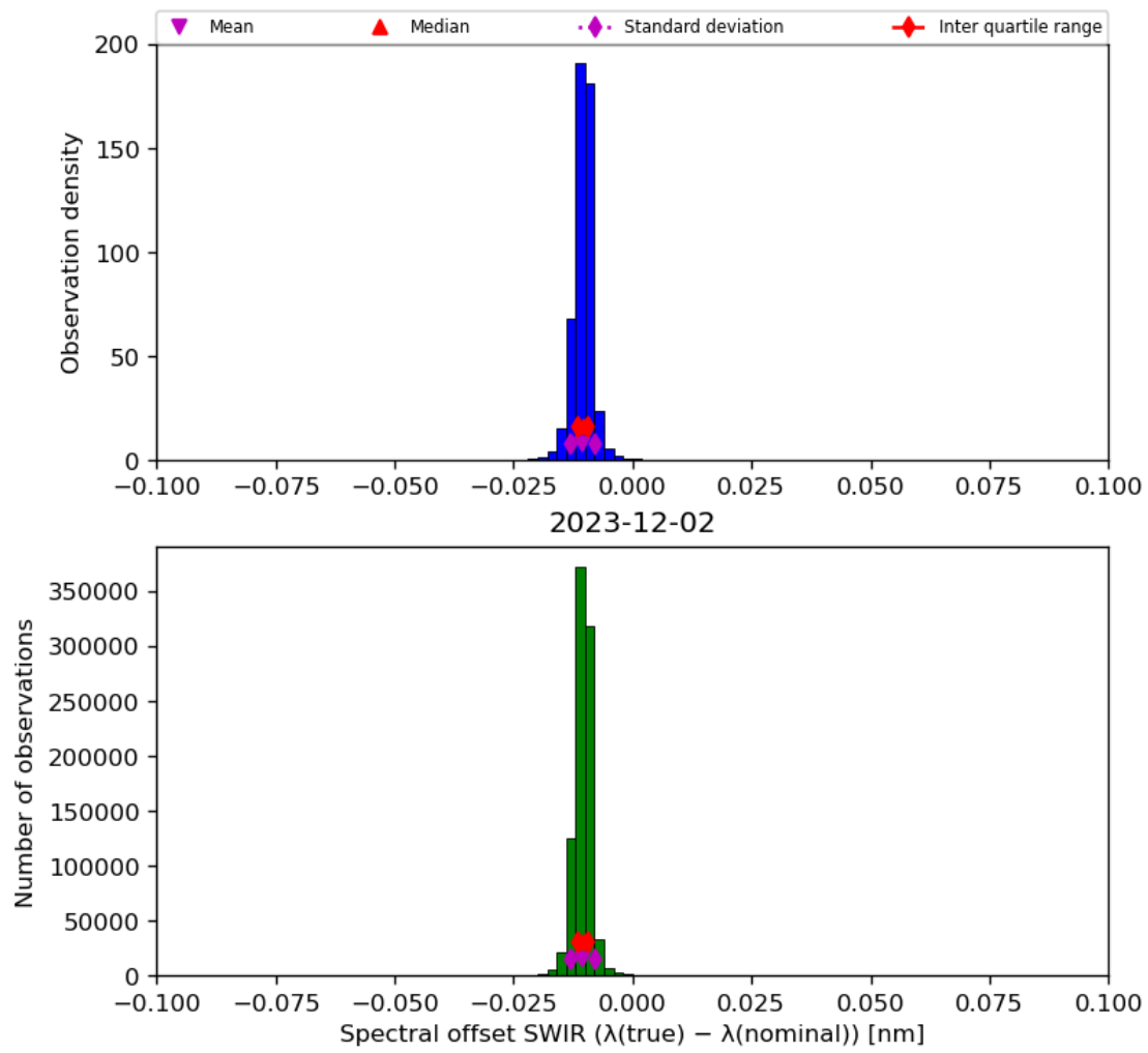
Figure 27: Histogram of “Spectral offset SWIR ( \lambda(\text{true}) - \lambda(\text{nominal}) )” for 2023-12-01 to 2023-12-03
