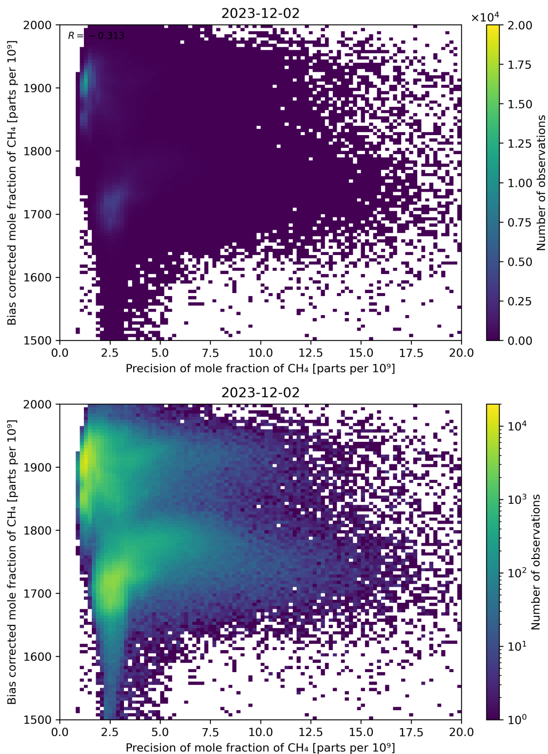
Figure 82: Scatter density plot of “Precision of mole fraction of CH 4 ” against “Bias corrected mole fraction of CH 4 ” for 2023-12-01 to 2023-12-03.
