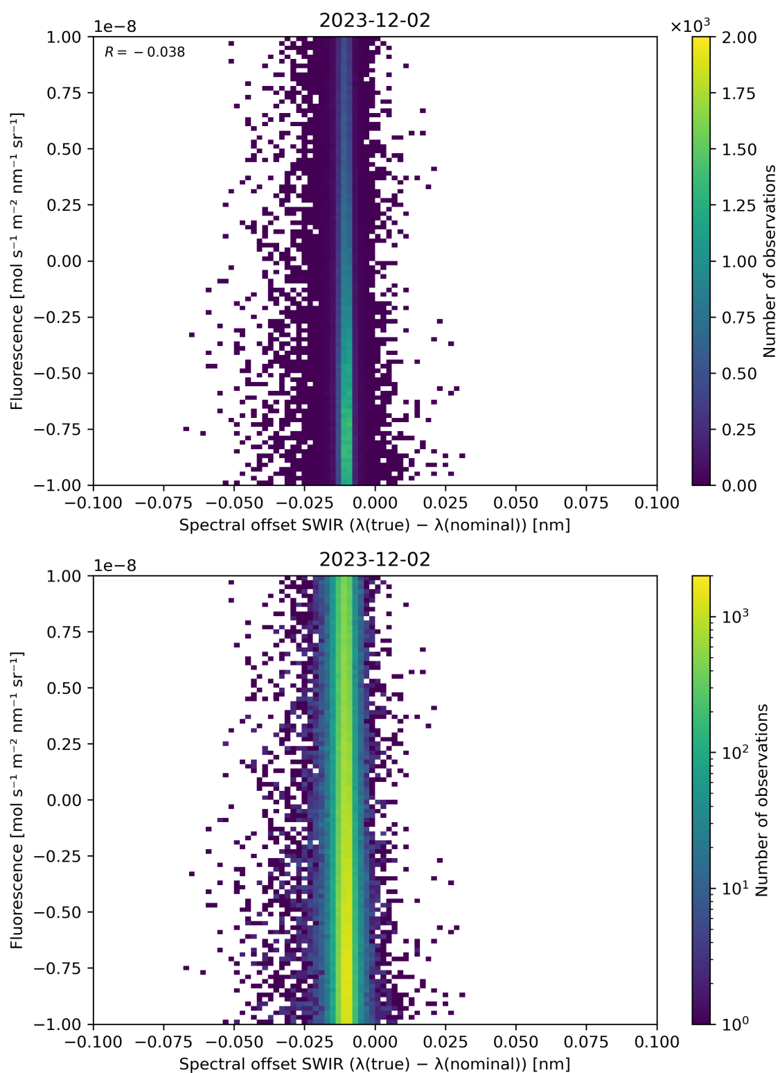
Figure 120: Scatter density plot of “Spectral offset SWIR ( \lambda(\text{true}) - \lambda(\text{nominal}) )” against “Fluorescence” for 2023-12-01 to 2023-12-03.
