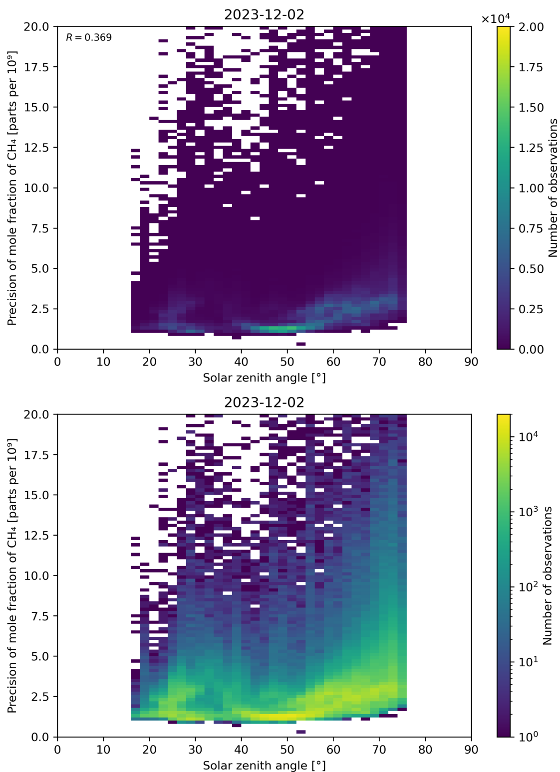
Figure 101: Scatter density plot of “Solar zenith angle” against “Precision of mole fraction of CH 4 ” for 2023-12-01 to 2023-12-03.
