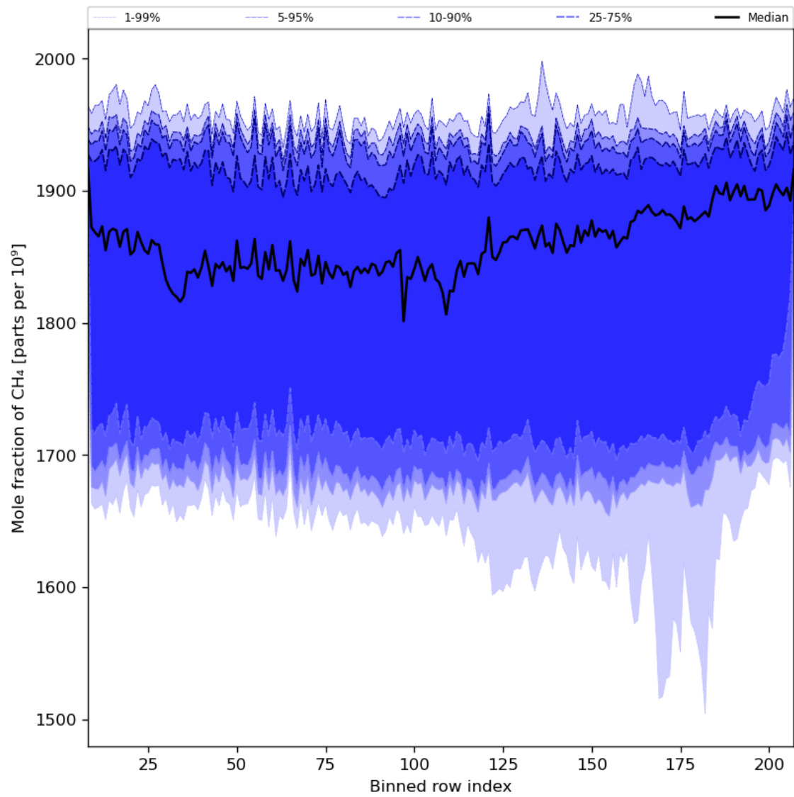
Figure 34: Along track statistics of “Mole fraction of CH 4 ” for 2023-12-01 to 2023-12-03
