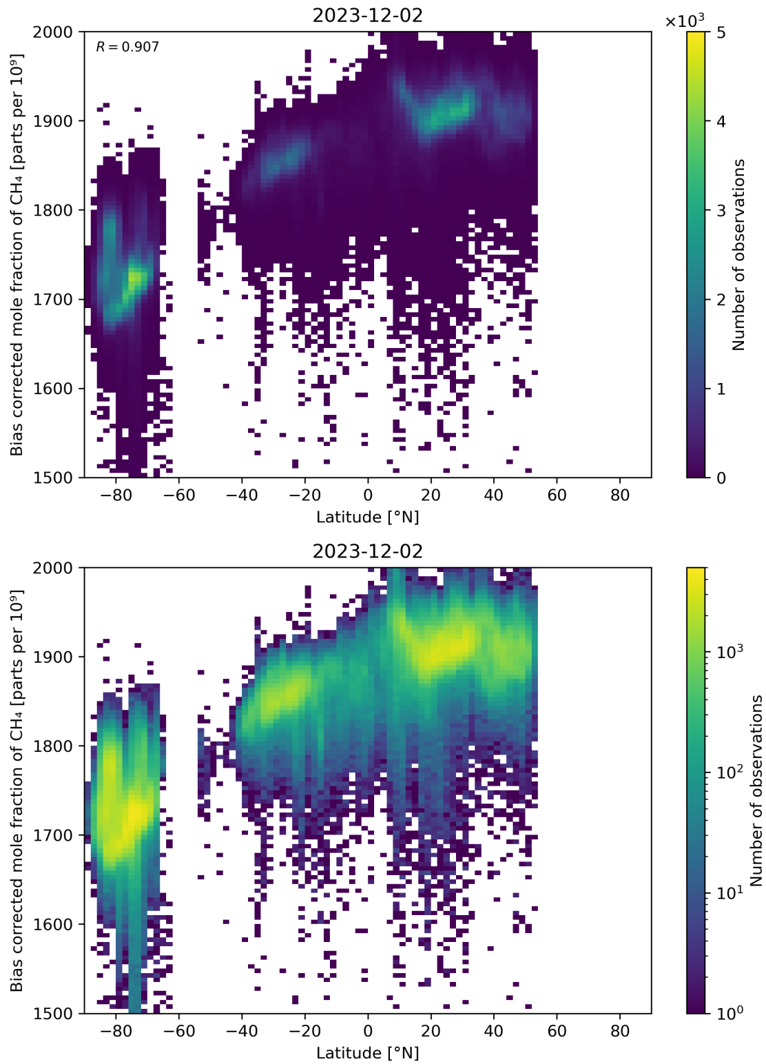
Figure 58: Scatter density plot of “Latitude” against “Bias corrected mole fraction of \text{CH}_4 ” for 2023-12-01 to 2023-12-03.
