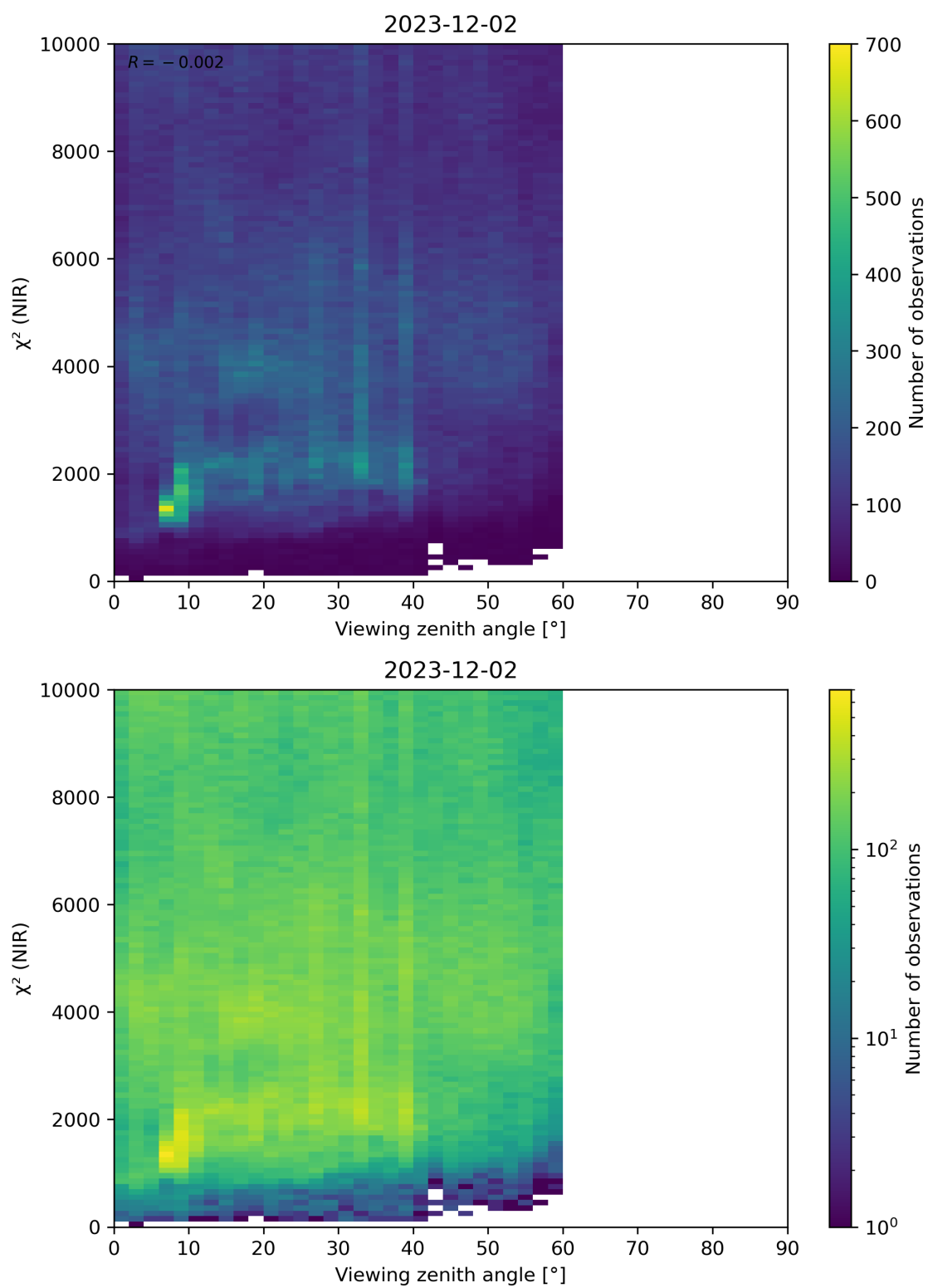
Figure 105: Scatter density plot of “Viewing zenith angle” against “ \chi^2 (NIR)” for 2023-12-01 to 2023-12-03.
