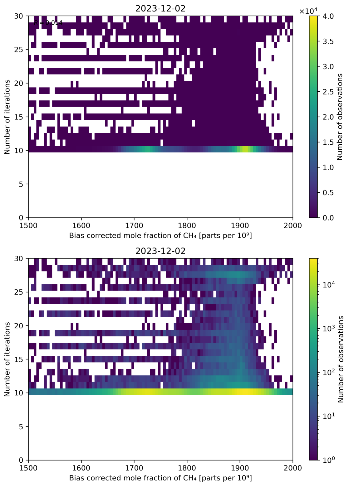
Figure 67: Scatter density plot of “Bias corrected mole fraction of \text{CH}_4 ” against “Number of iterations” for 2023-12-01 to 2023-12-03.
