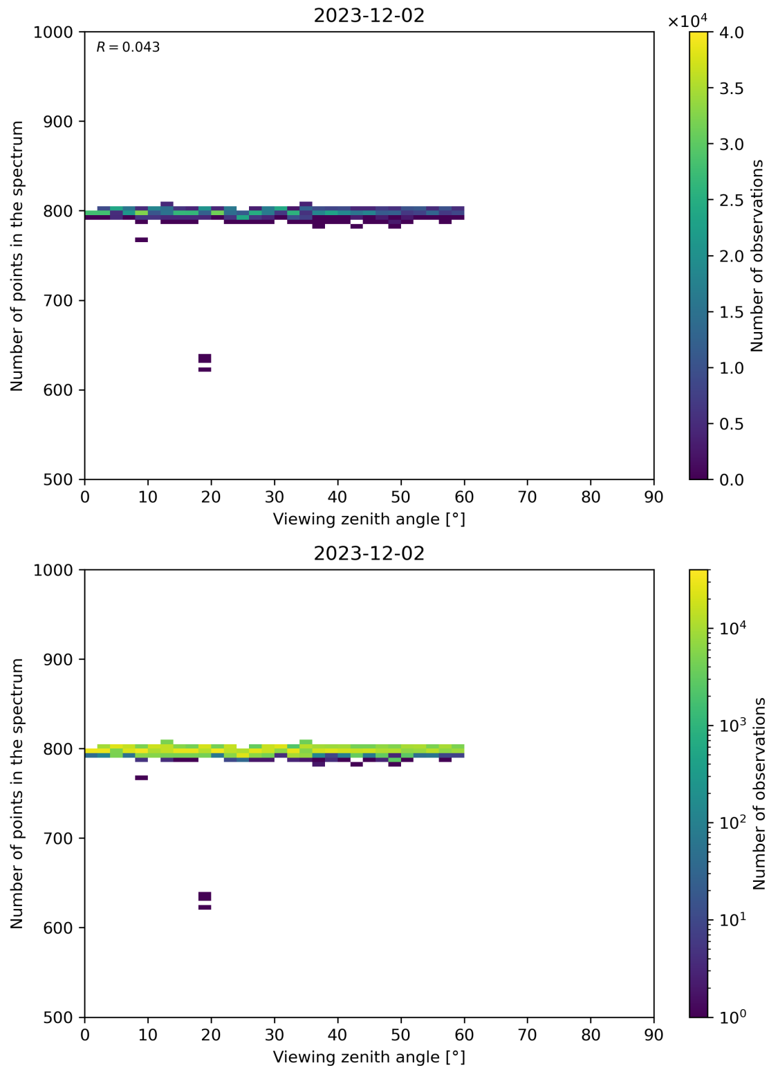
Figure 114: Scatter density plot of “Viewing zenith angle” against “Number of points in the spectrum” for 2023-12-01 to 2023-12-03.
