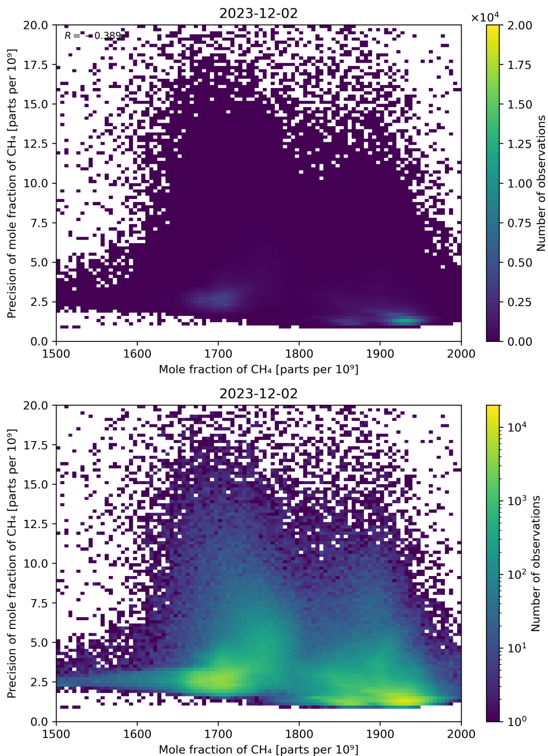
Figure 75: Scatter density plot of “Mole fraction of CH 4 ” against “Precision of mole fraction of CH 4 ” for 2023-12-01 to 2023-12-03.
