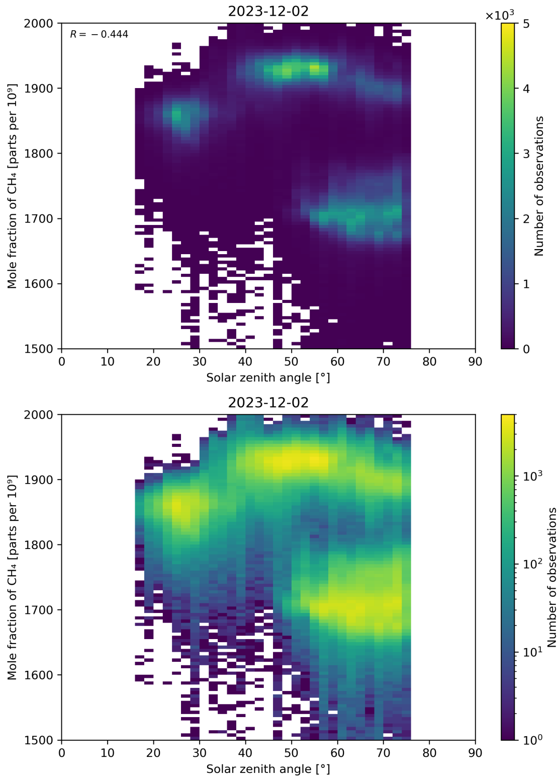
Figure 99: Scatter density plot of “Solar zenith angle” against “Mole fraction of CH 4 ” for 2023-12-01 to 2023-12-03.
