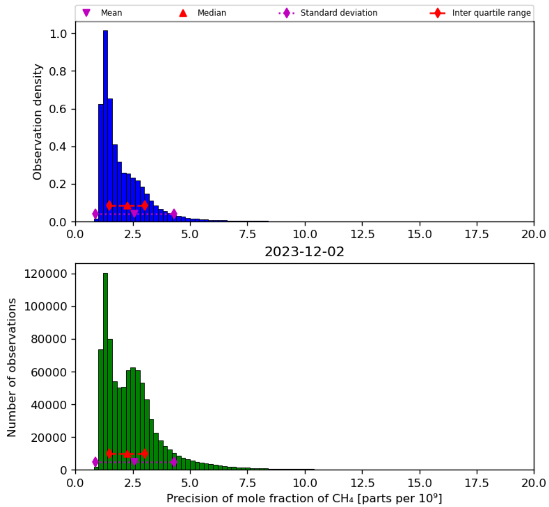
Figure 24: Histogram of “Precision of mole fraction of CH 4 ” for 2023-12-01 to 2023-12-03
