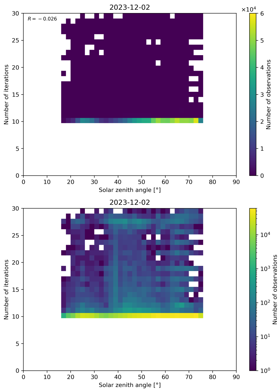
Figure 102: Scatter density plot of “Solar zenith angle” against “Number of iterations” for 2023-12-01 to 2023-12-03.
