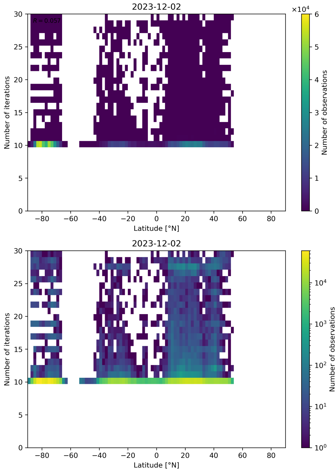
Figure 60: Scatter density plot of “Latitude” against “Number of iterations” for 2023-12-01 to 2023-12-03.
