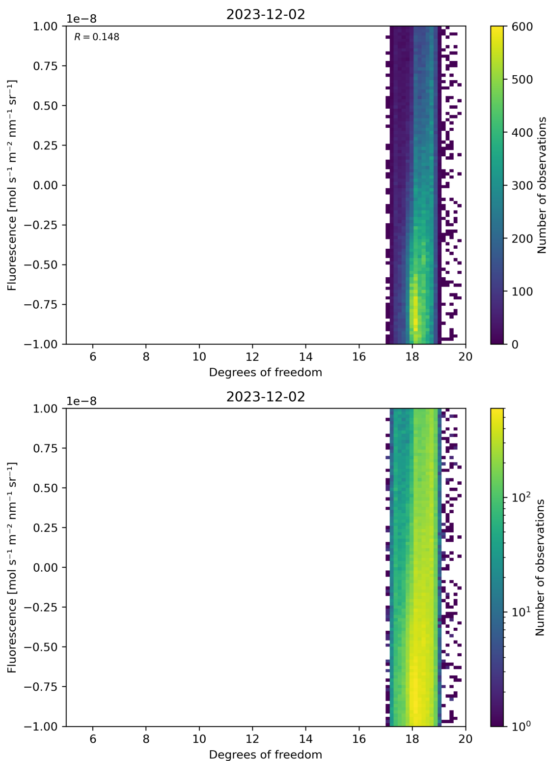
Figure 51: Scatter density plot of “Degrees of freedom” against “Fluorescence” for 2023-12-01 to 2023-12-03.
