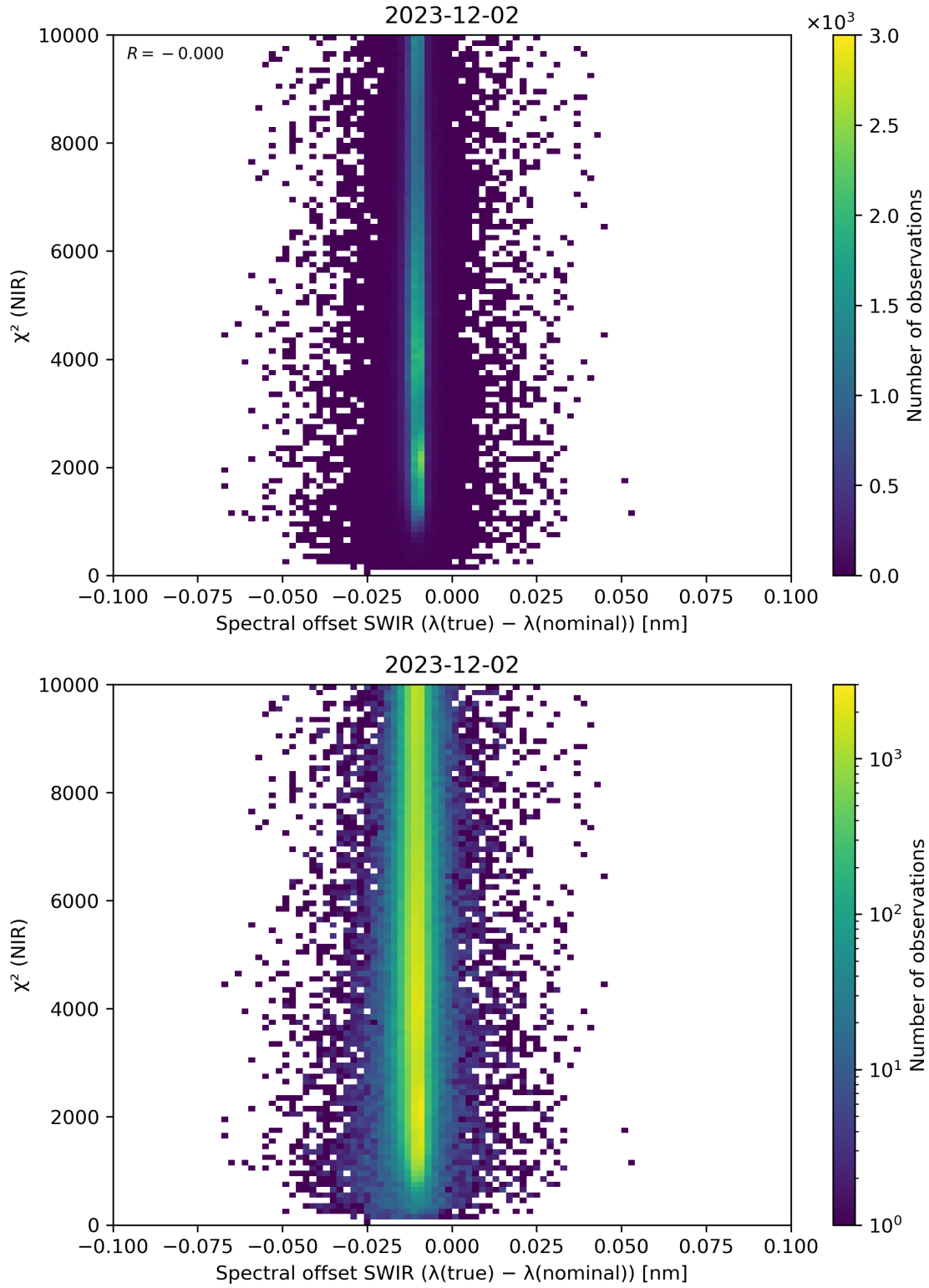
Figure 117: Scatter density plot of “Spectral offset SWIR ( \lambda(\text{true}) - \lambda(\text{nominal}) )” against “ \chi^2 (NIR)” for 2023-12-01 to 2023-12-03.
