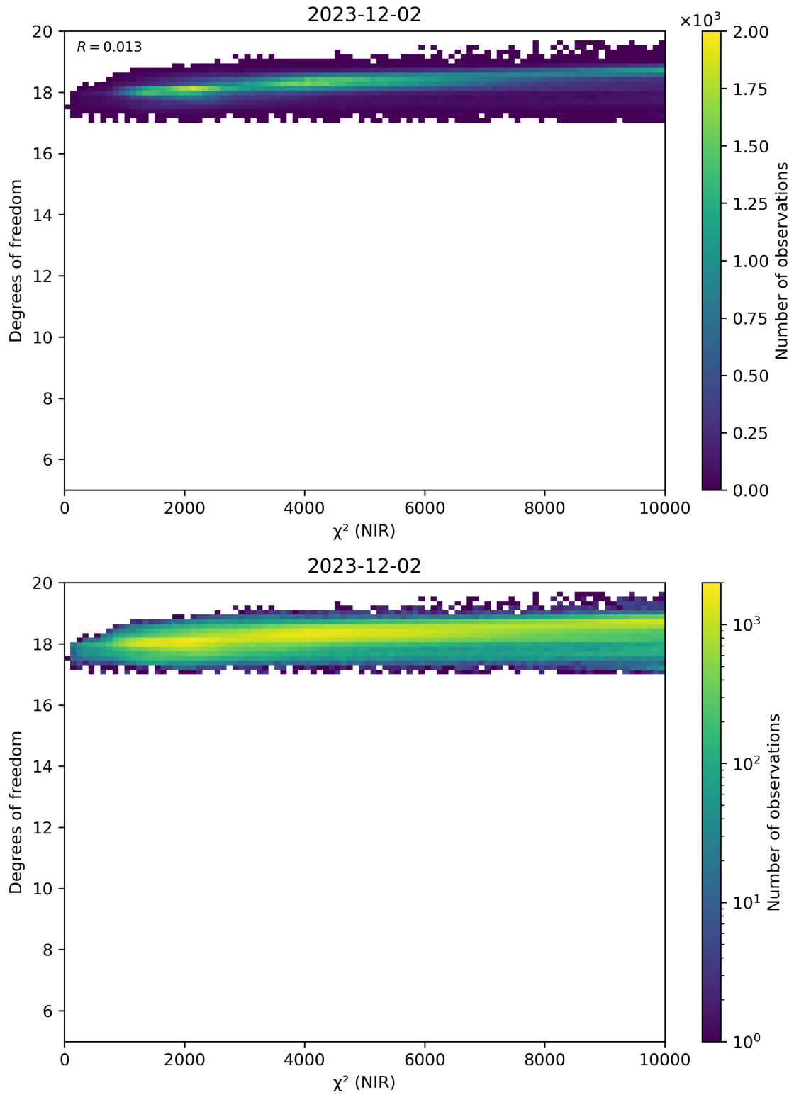
Figure 44: Scatter density plot of “ \chi^2 (NIR)” against “Degrees of freedom” for 2023-12-01 to 2023-12-03.
