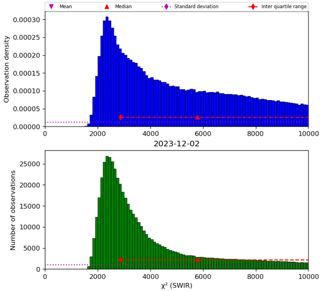
Figure 28: Histogram of “ \chi^2 (SWIR)” for 2023-12-01 to 2023-12-03
