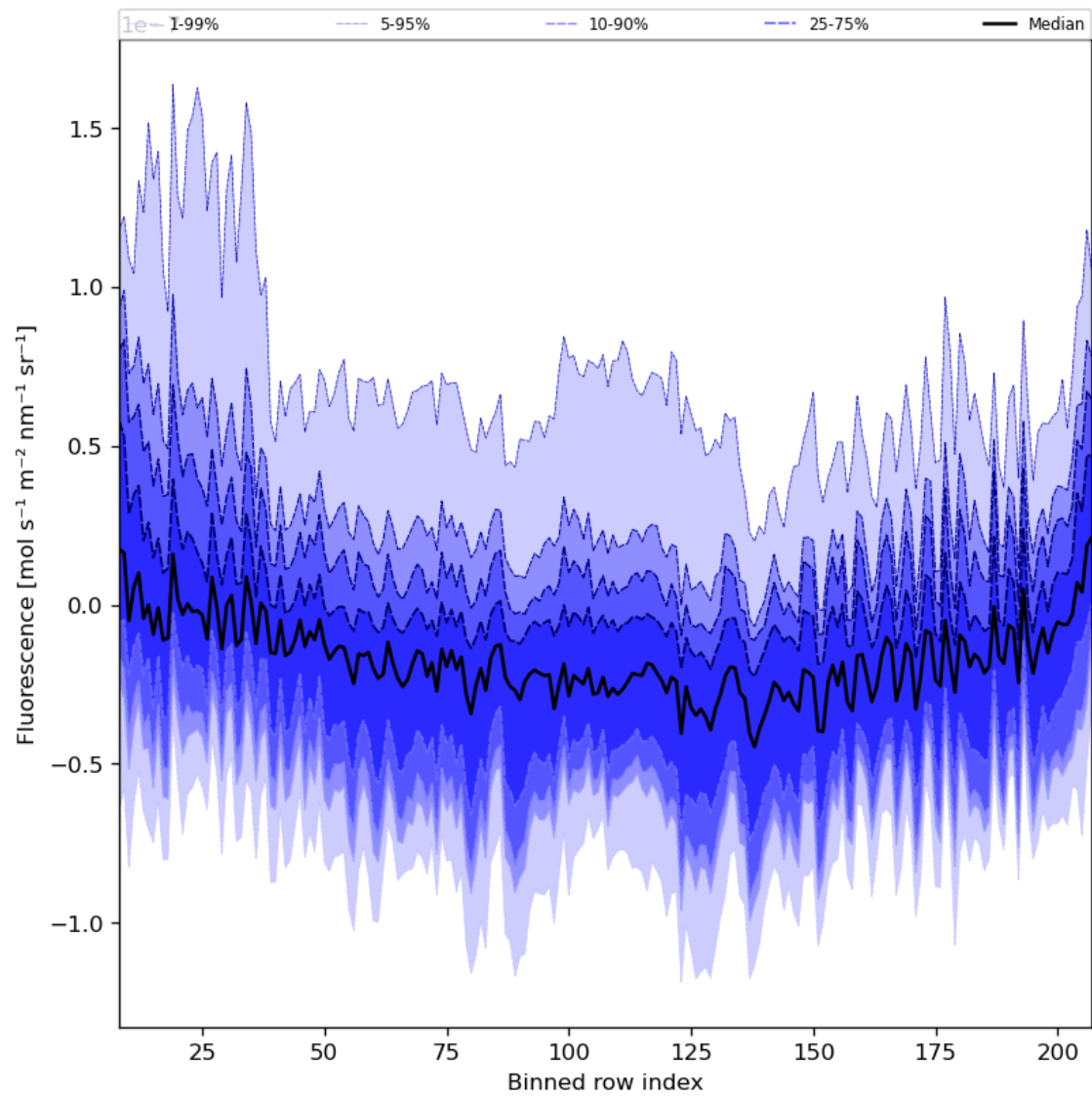
Figure 43: Along track statistics of “Fluorescence” for 2023-12-01 to 2023-12-03
