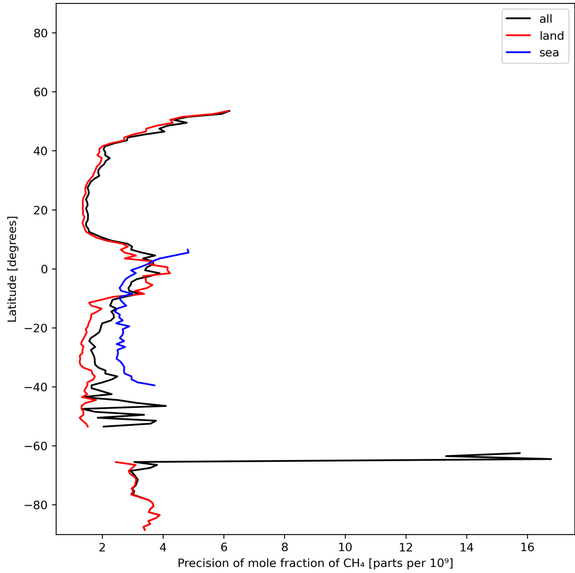
Figure 13: Zonal average of “Precision of mole fraction of CH 4 ” for 2023-12-01 to 2023-12-03.
