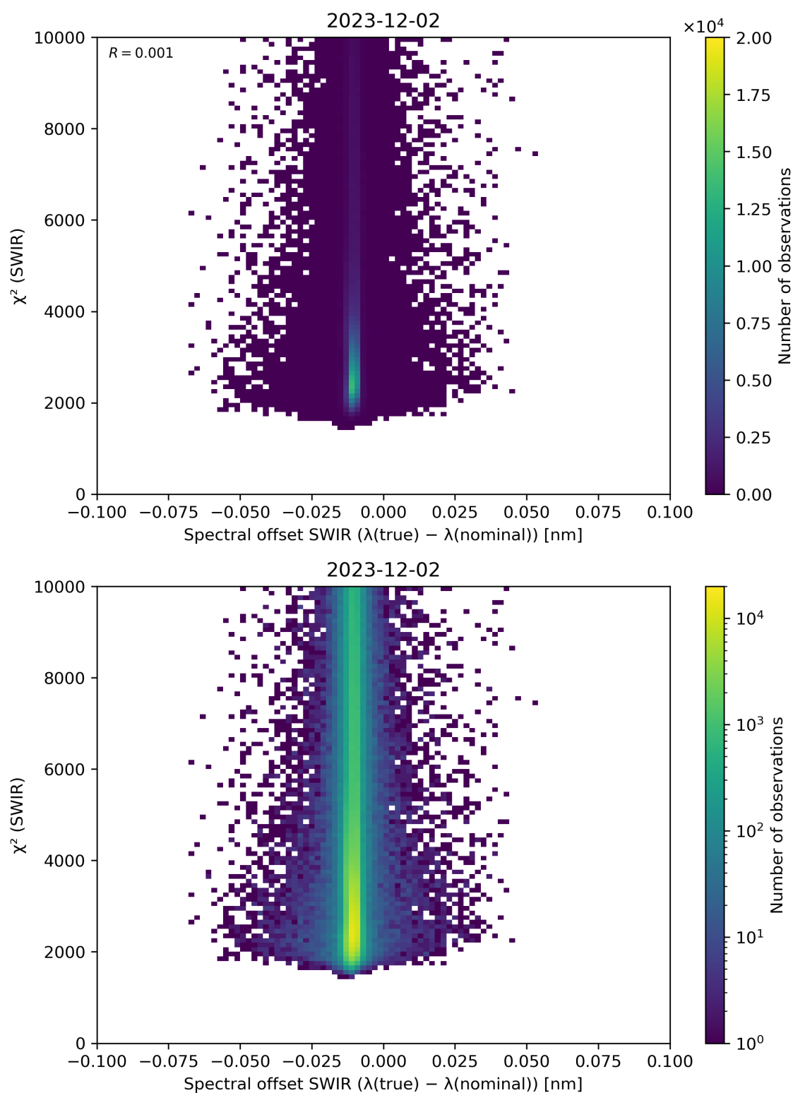
Figure 118: Scatter density plot of “Spectral offset SWIR ( \lambda(\text{true}) - \lambda(\text{nominal}) )” against “ \chi^2 (SWIR)” for 2023-12-01 to 2023-12-03.
