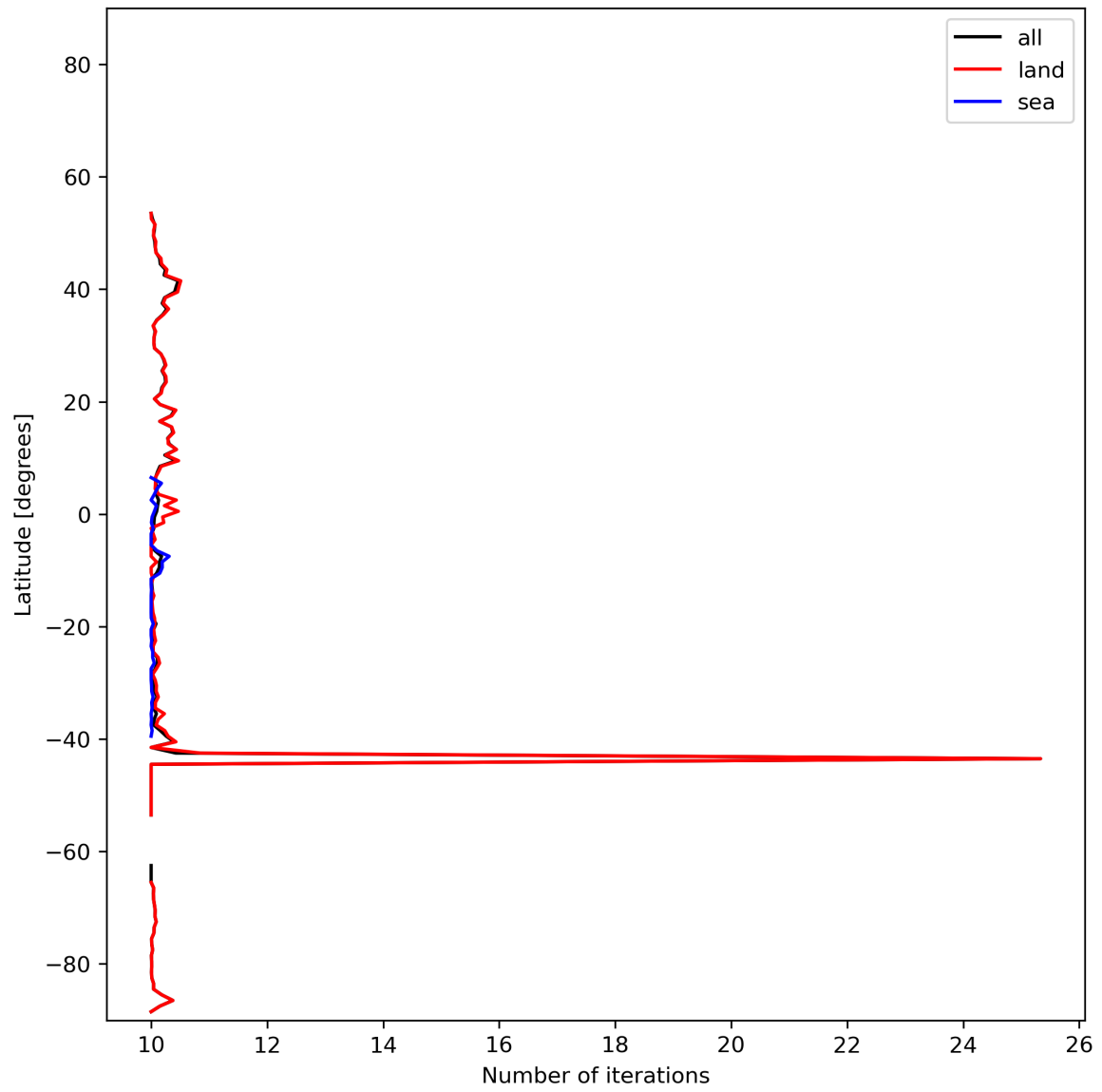
Figure 20: Zonal average of “Number of iterations” for 2023-12-01 to 2023-12-03.
