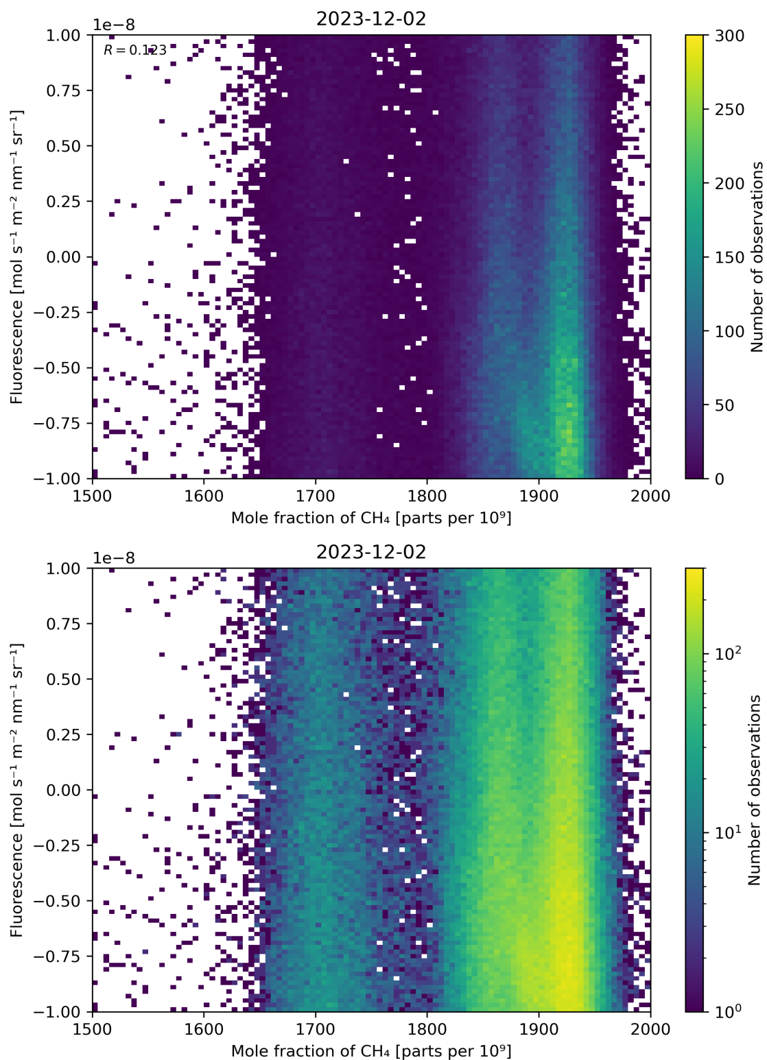
Figure 73: Scatter density plot of “Mole fraction of \text{CH}_4 ” against “Fluorescence” for 2023-12-01 to 2023-12-03.
