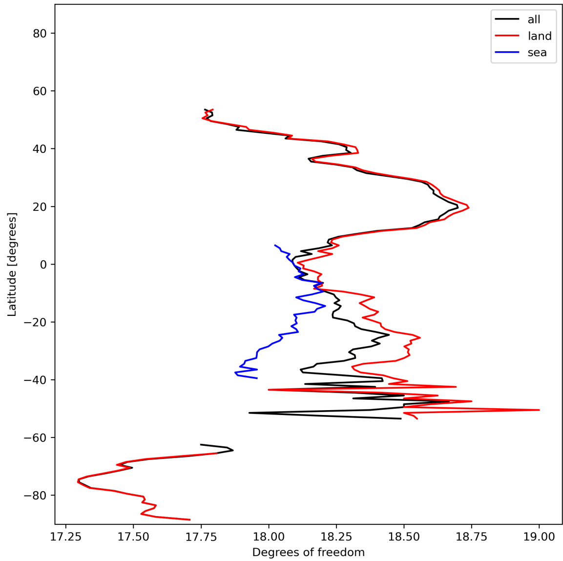
Figure 19: Zonal average of “Degrees of freedom” for 2023-12-01 to 2023-12-03.
