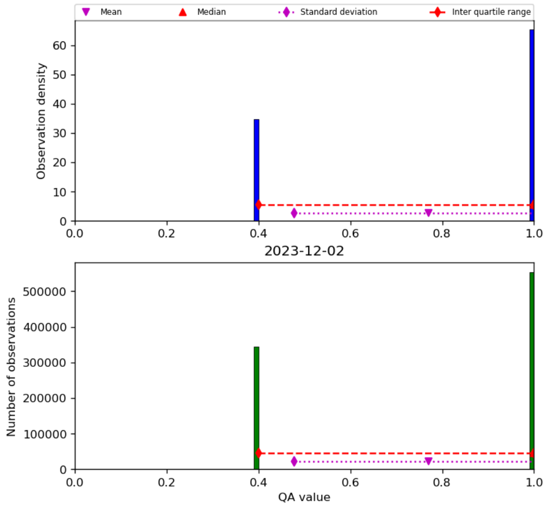
Figure 22: Histogram of “QA value” for 2023-12-01 to 2023-12-03
