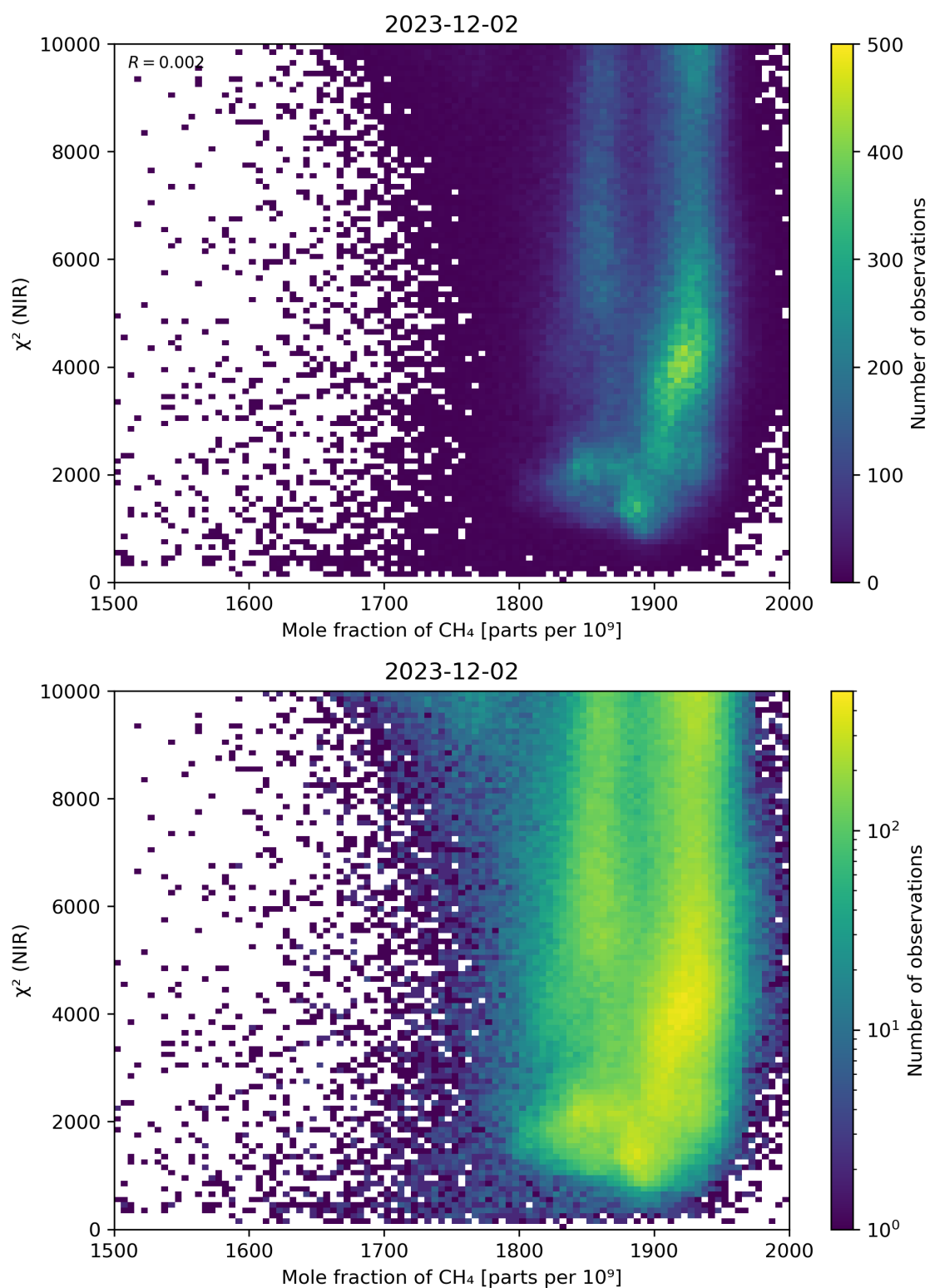
Figure 70: Scatter density plot of “Mole fraction of \text{CH}_4 ” against “ \chi^2 (NIR)” for 2023-12-01 to 2023-12-03.
