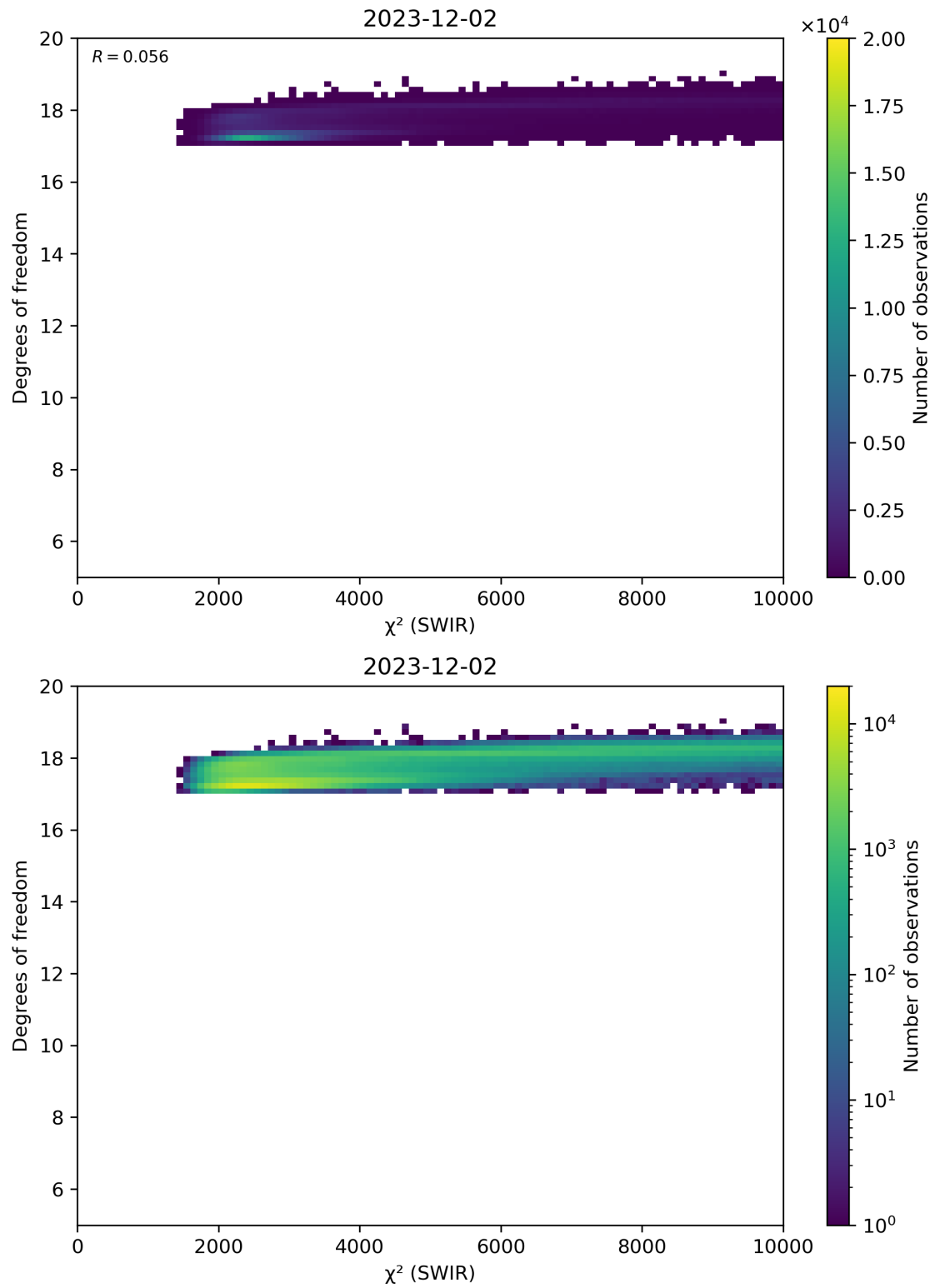
Figure 48: Scatter density plot of “ \chi^2 (SWIR)” against “Degrees of freedom” for 2023-12-01 to 2023-12-03.
