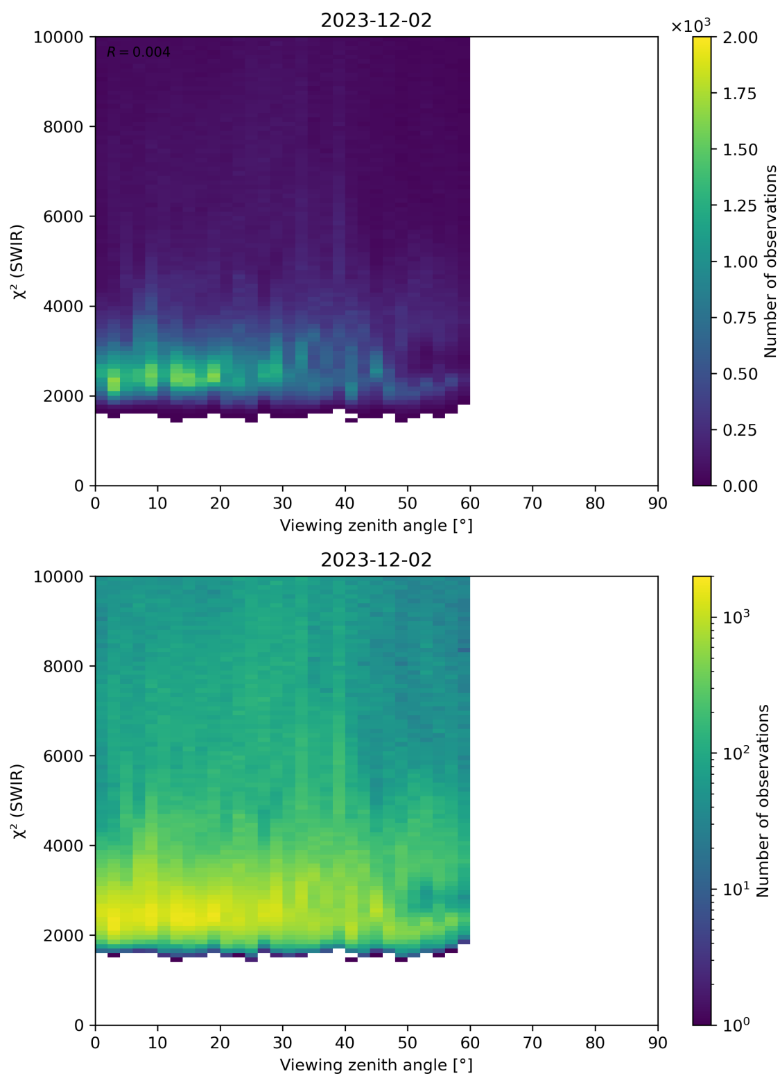
Figure 106: Scatter density plot of “Viewing zenith angle” against “ \chi^2 (SWIR)” for 2023-12-01 to 2023-12-03.
