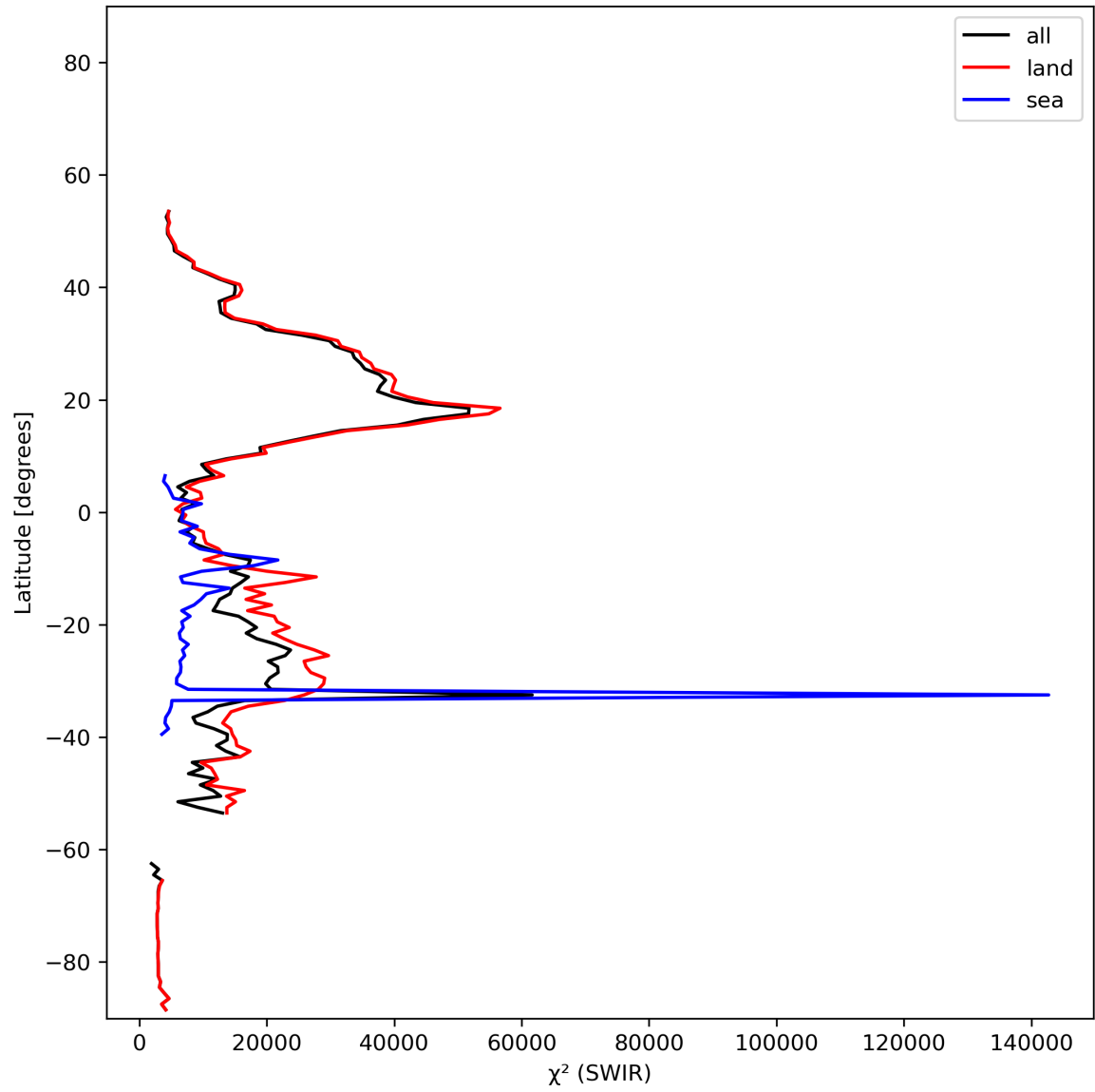
Figure 17: Zonal average of “ \chi^2 (SWIR)” for 2023-12-01 to 2023-12-03.
