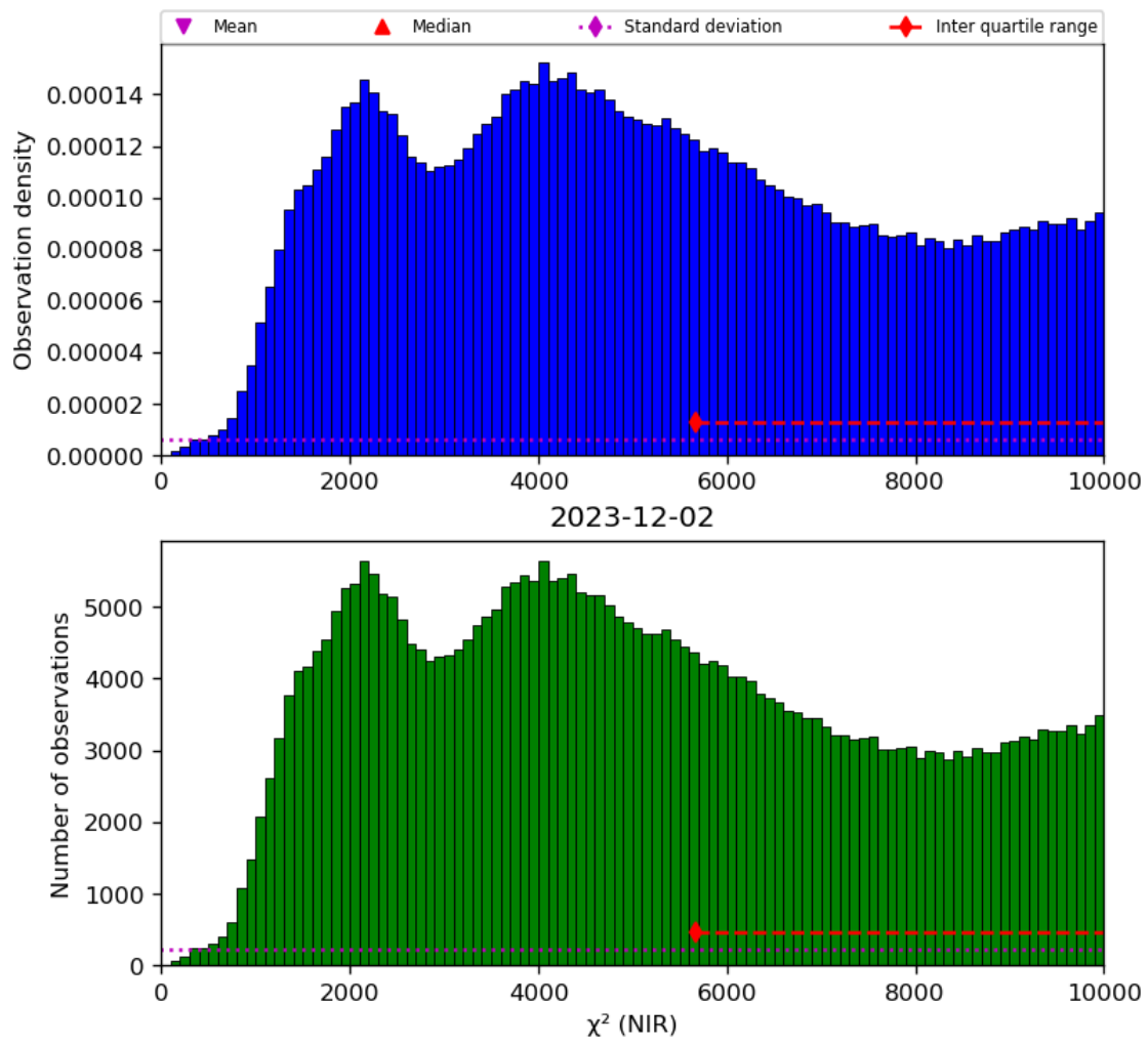
Figure 29: Histogram of “ \chi^2 (NIR)” for 2023-12-01 to 2023-12-03
