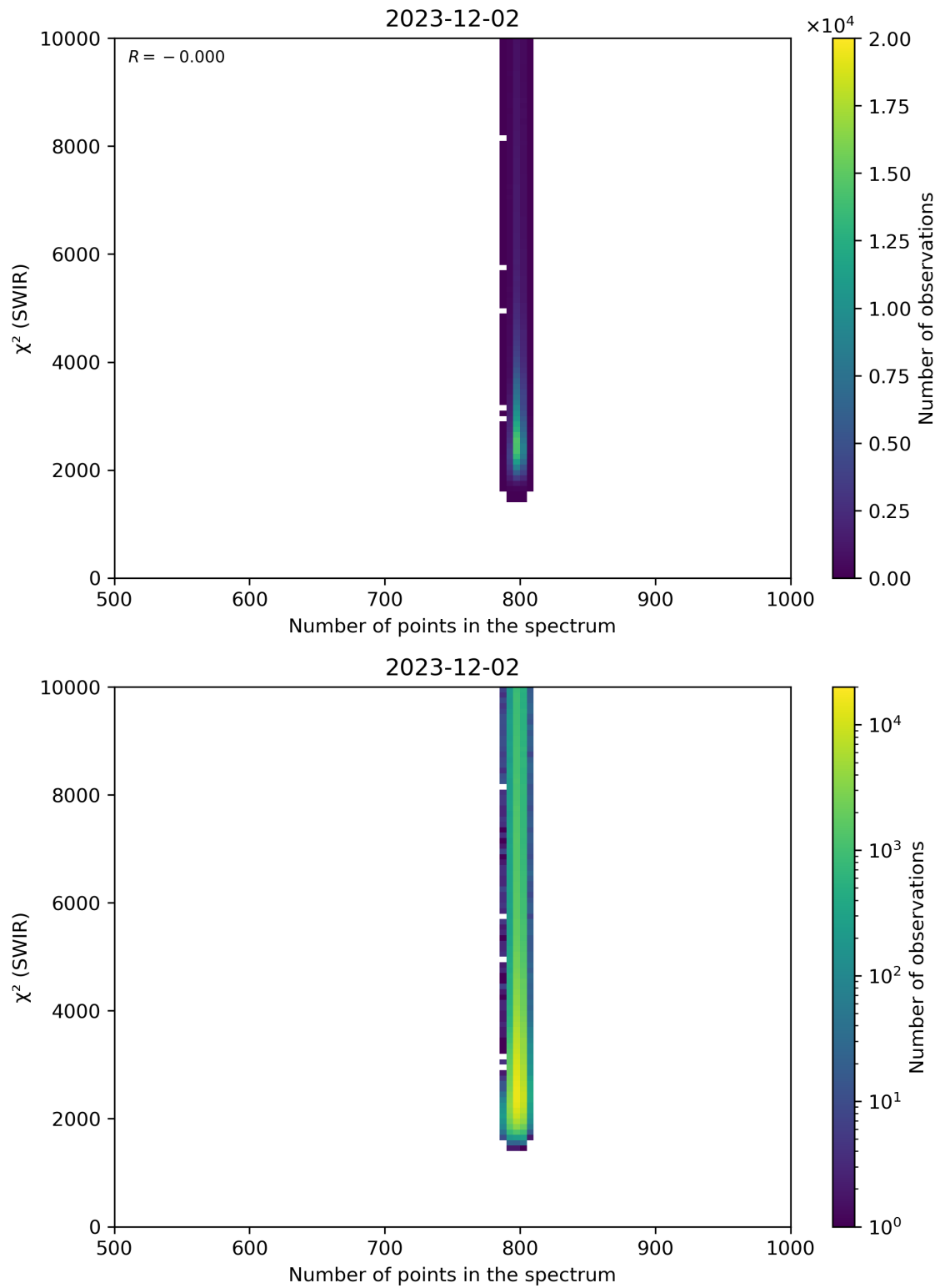
Figure 89: Scatter density plot of “Number of points in the spectrum” against “ \chi^2 (SWIR)” for 2023-12-01 to 2023-12-03.
