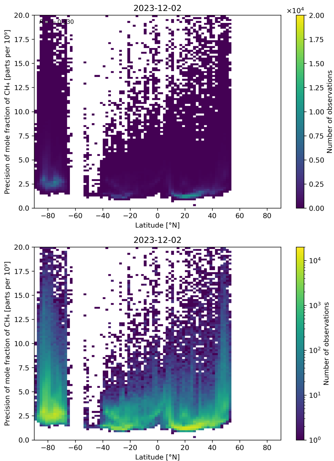
Figure 59: Scatter density plot of “Latitude” against “Precision of mole fraction of CH 4 ” for 2023-12-01 to 2023-12-03.
