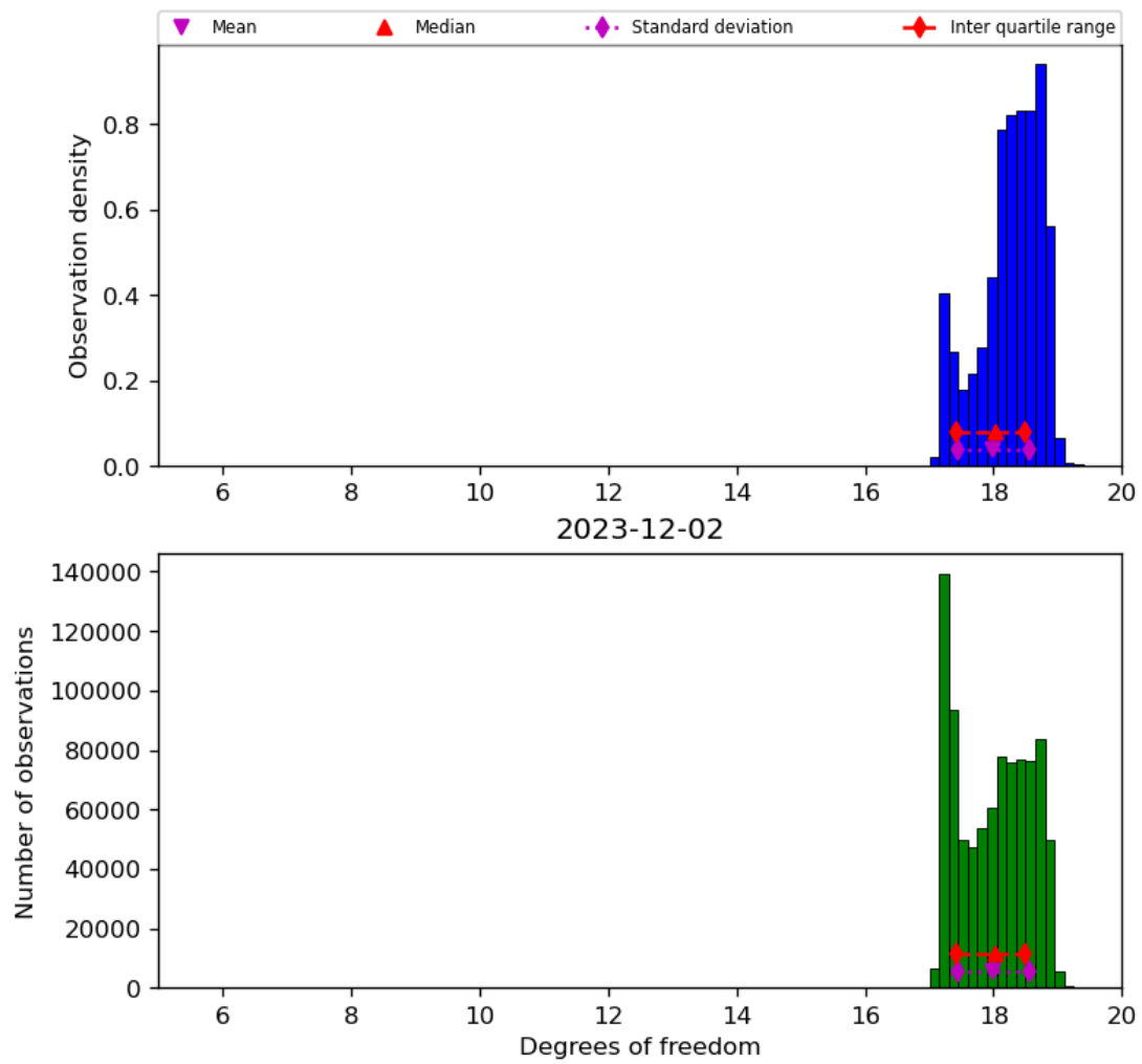
Figure 30: Histogram of “Degrees of freedom” for 2023-12-01 to 2023-12-03
