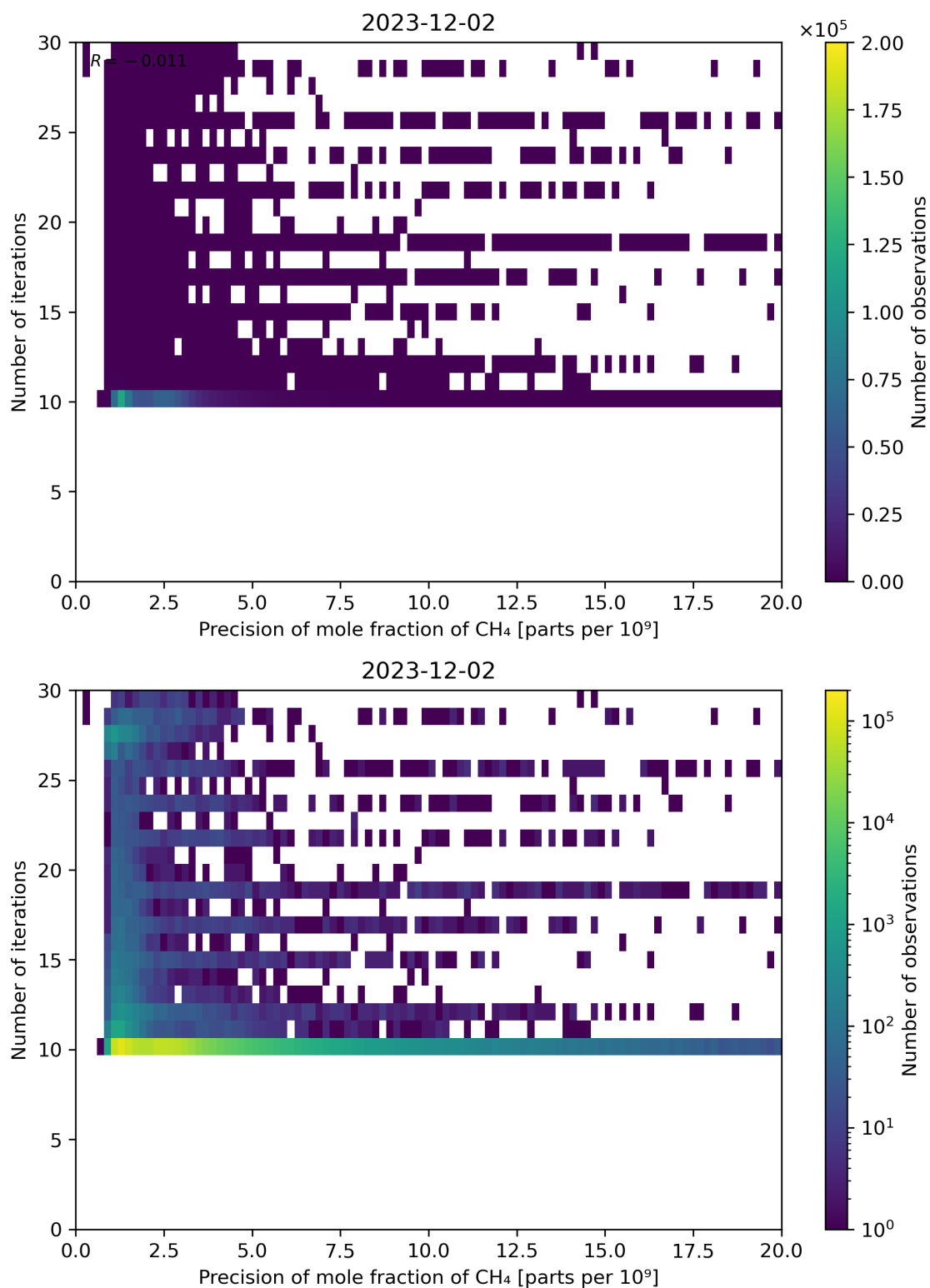
Figure 83: Scatter density plot of “Precision of mole fraction of CH 4 ” against “Number of iterations” for 2023-12-01 to 2023-12-03.
