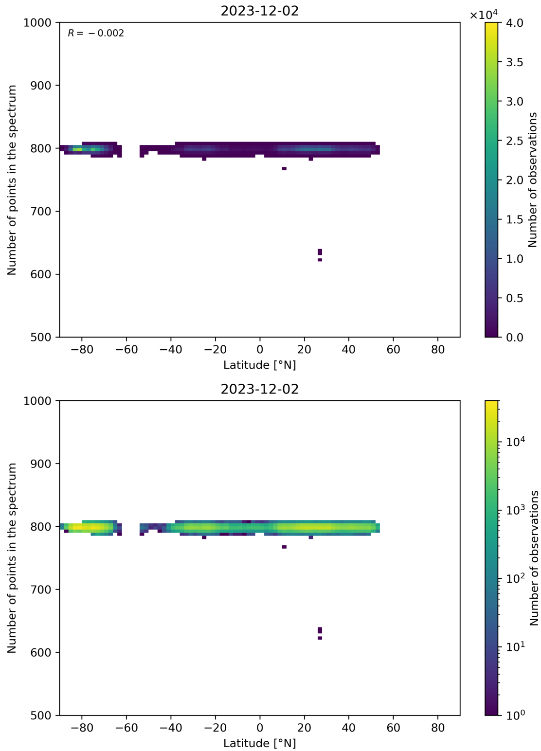
Figure 61: Scatter density plot of “Latitude” against “Number of points in the spectrum” for 2023-12-01 to 2023-12-03.
