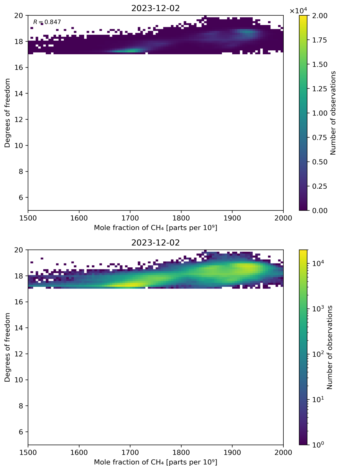
Figure 72: Scatter density plot of “Mole fraction of CH 4 ” against “Degrees of freedom” for 2023-12-01 to 2023-12-03.
