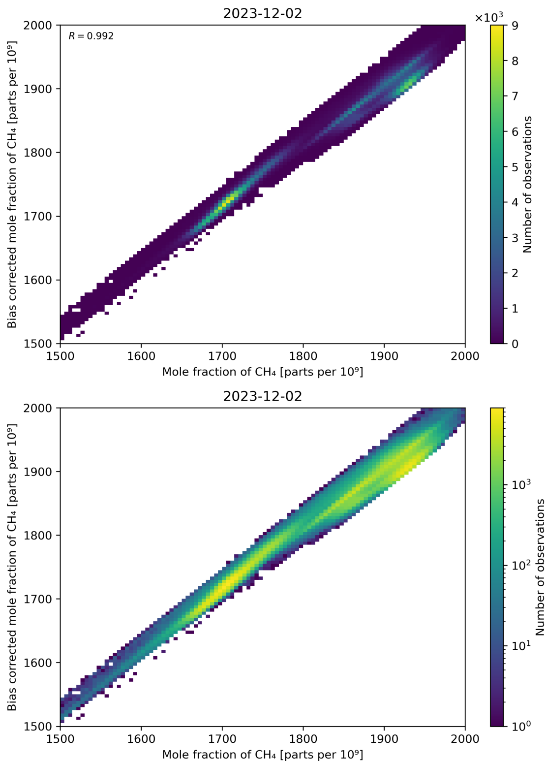
Figure 74: Scatter density plot of “Mole fraction of CH 4 ” against “Bias corrected mole fraction of CH 4 ” for 2023-12-01 to 2023-12-03.
