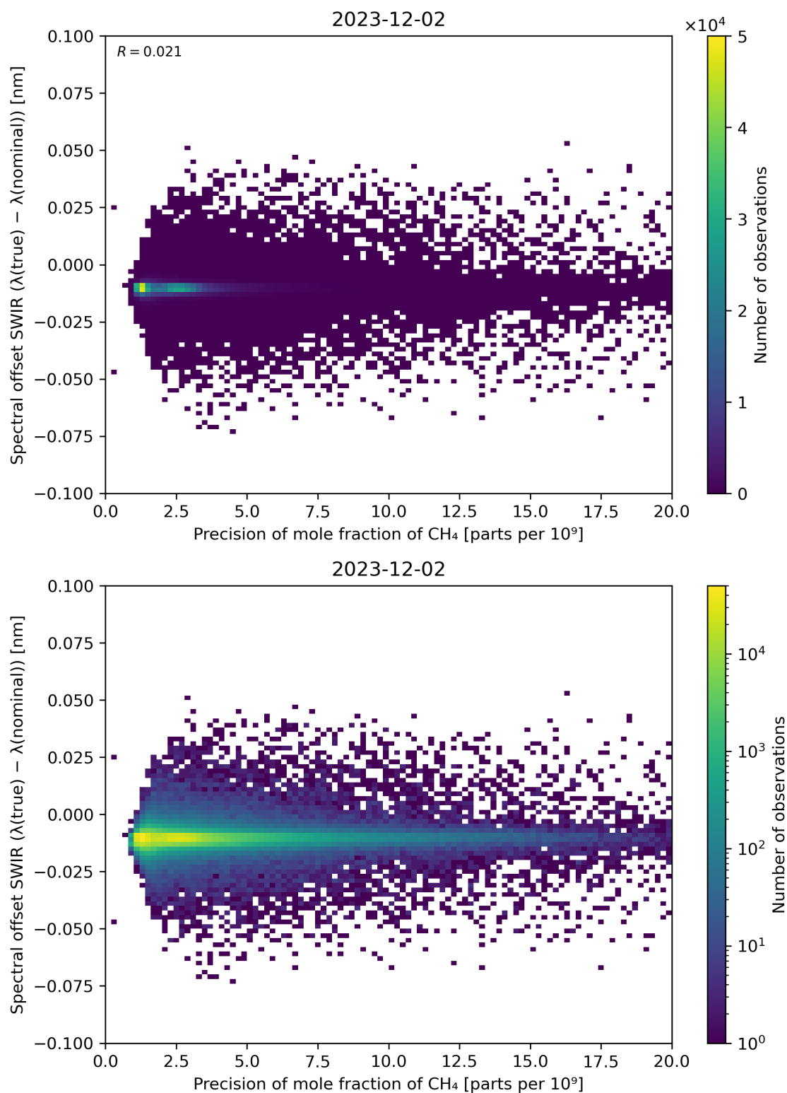
Figure 85: Scatter density plot of “Precision of mole fraction of CH 4 ” against “Spectral offset SWIR ( \lambda(\text{true}) - \lambda(\text{nominal}) )” for 2023-12-01 to 2023-12-03.
