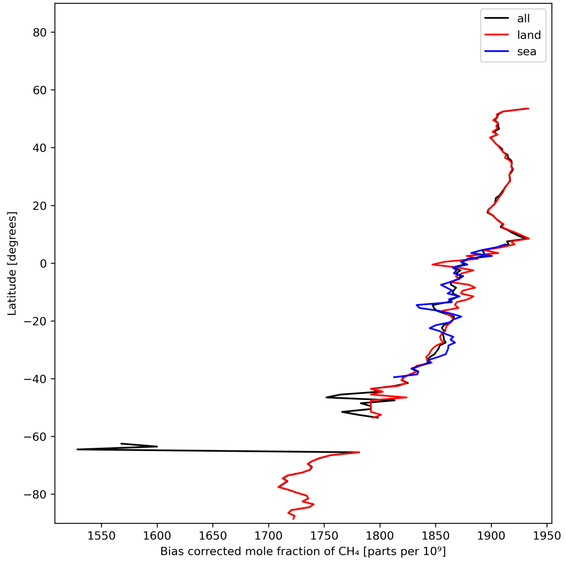
Figure 14: Zonal average of “Bias corrected mole fraction of CH 4 ” for 2023-12-01 to 2023-12-03.
