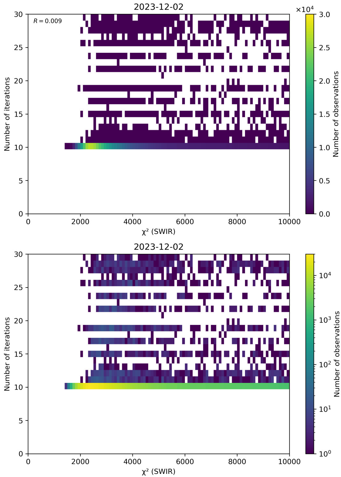
Figure 50: Scatter density plot of “ \chi^2 (SWIR)” against “Number of iterations” for 2023-12-01 to 2023-12-03.
