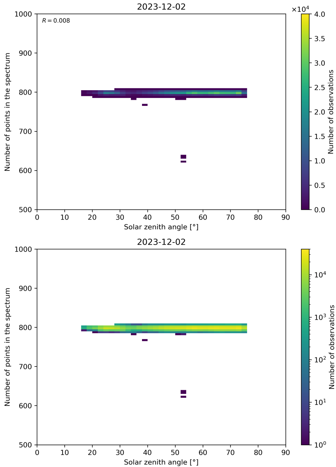
Figure 103: Scatter density plot of “Solar zenith angle” against “Number of points in the spectrum” for 2023-12-01 to 2023-12-03.
