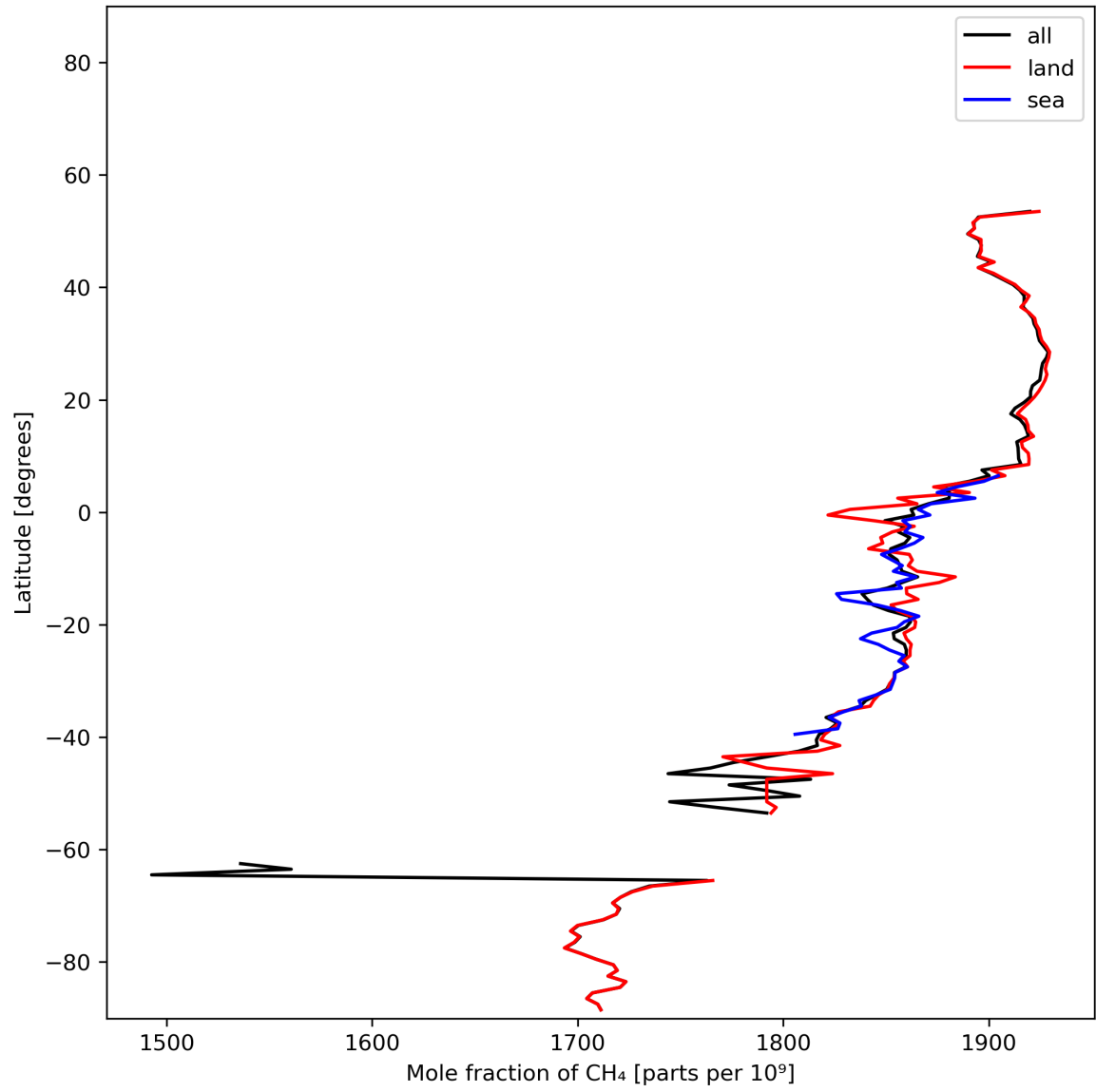
Figure 12: Zonal average of “Mole fraction of \text{CH}_4 ” for 2023-12-01 to 2023-12-03.
