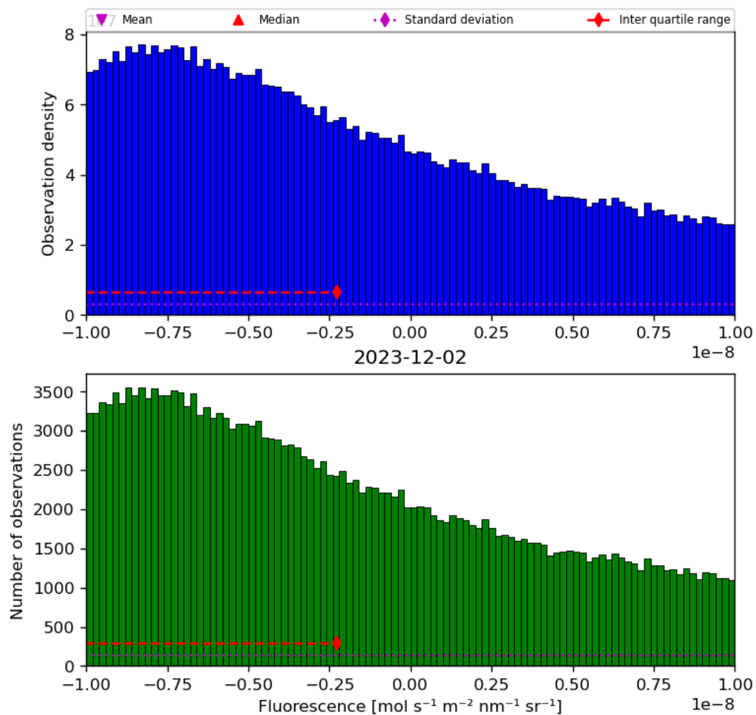
Figure 32: Histogram of “Fluorescence” for 2023-12-01 to 2023-12-03
