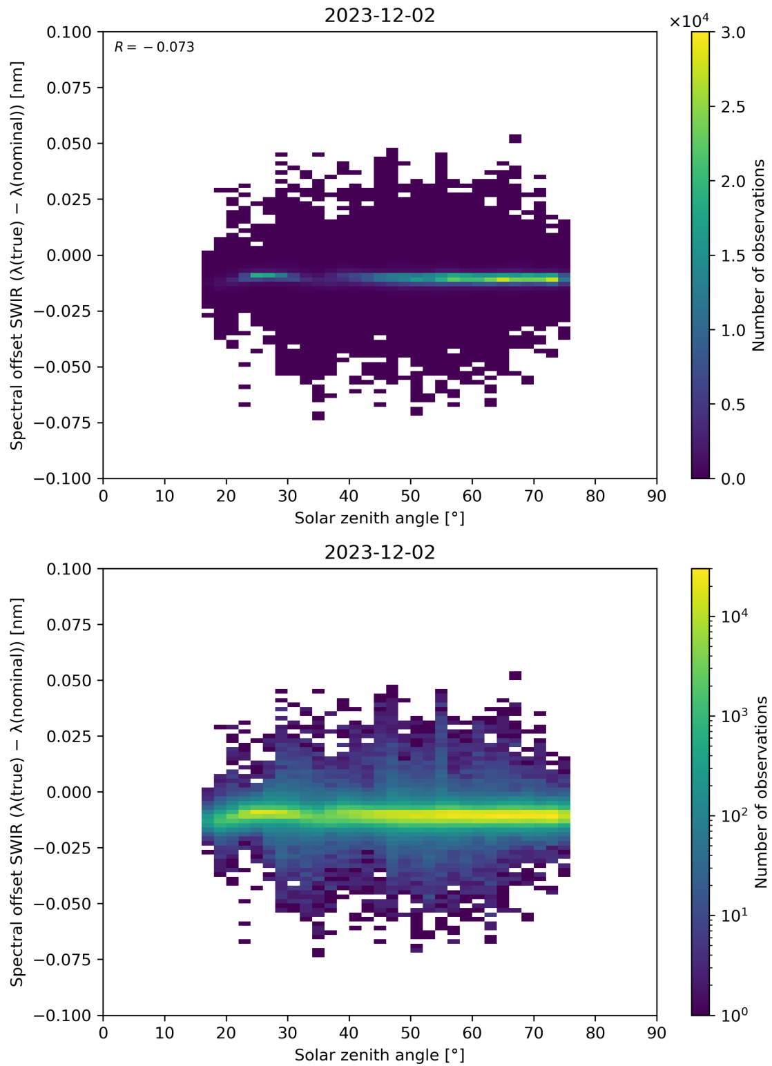
Figure 104: Scatter density plot of “Solar zenith angle” against “Spectral offset SWIR ( \lambda(\text{true}) - \lambda(\text{nominal}) )” for 2023-12-01 to 2023-12-03.
