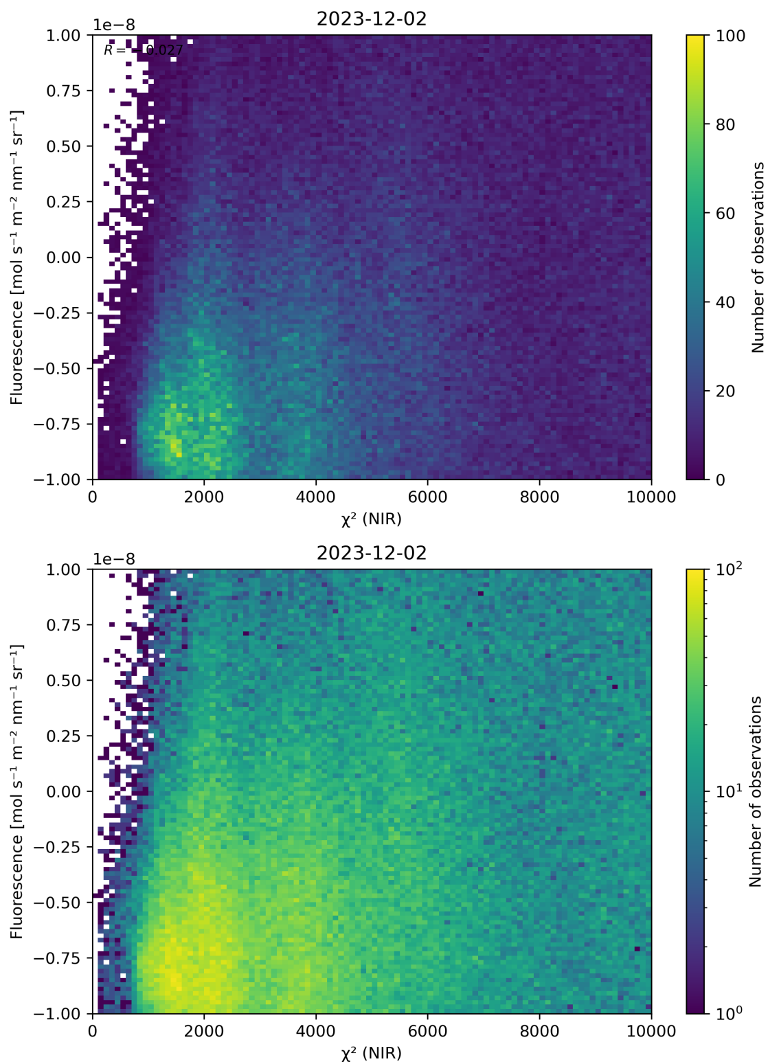
Figure 45: Scatter density plot of “ \chi^2 (NIR)” against “Fluorescence” for 2023-12-01 to 2023-12-03.
