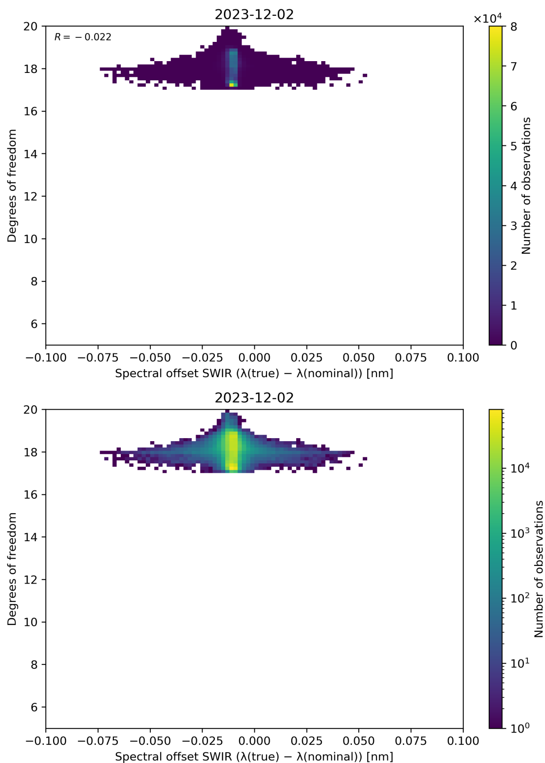
Figure 119: Scatter density plot of “Spectral offset SWIR ( \lambda(\text{true}) - \lambda(\text{nominal}) )” against “Degrees of freedom” for 2023-12-01 to 2023-12-03.
