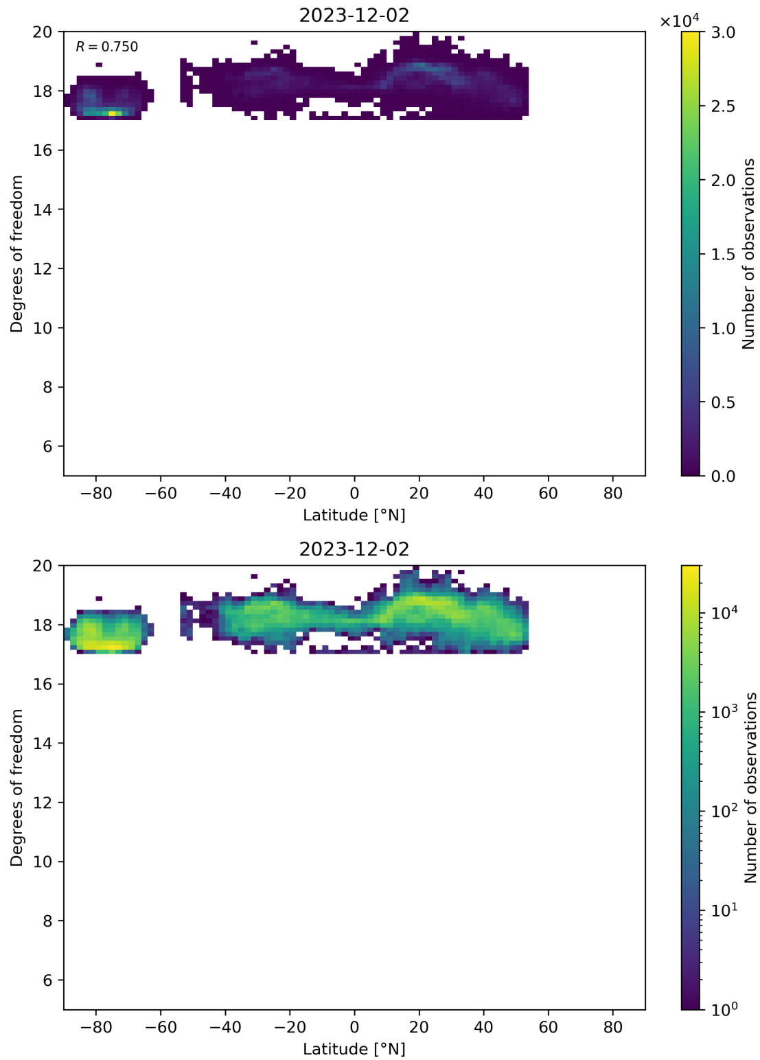
Figure 55: Scatter density plot of “Latitude” against “Degrees of freedom” for 2023-12-01 to 2023-12-03.
