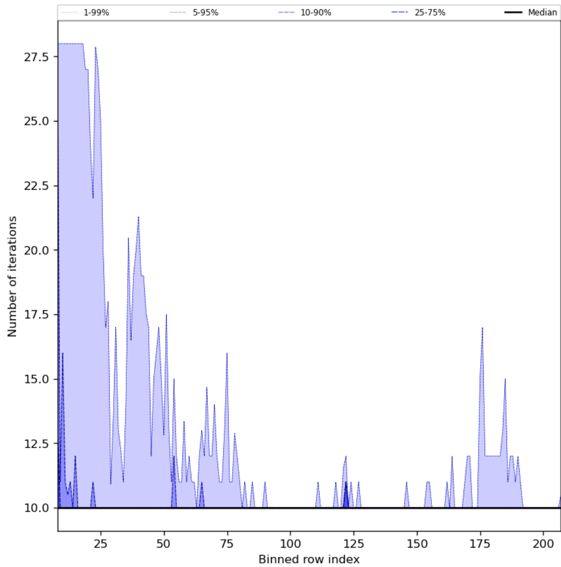
Figure 42: Along track statistics of “Number of iterations” for 2023-12-01 to 2023-12-03
