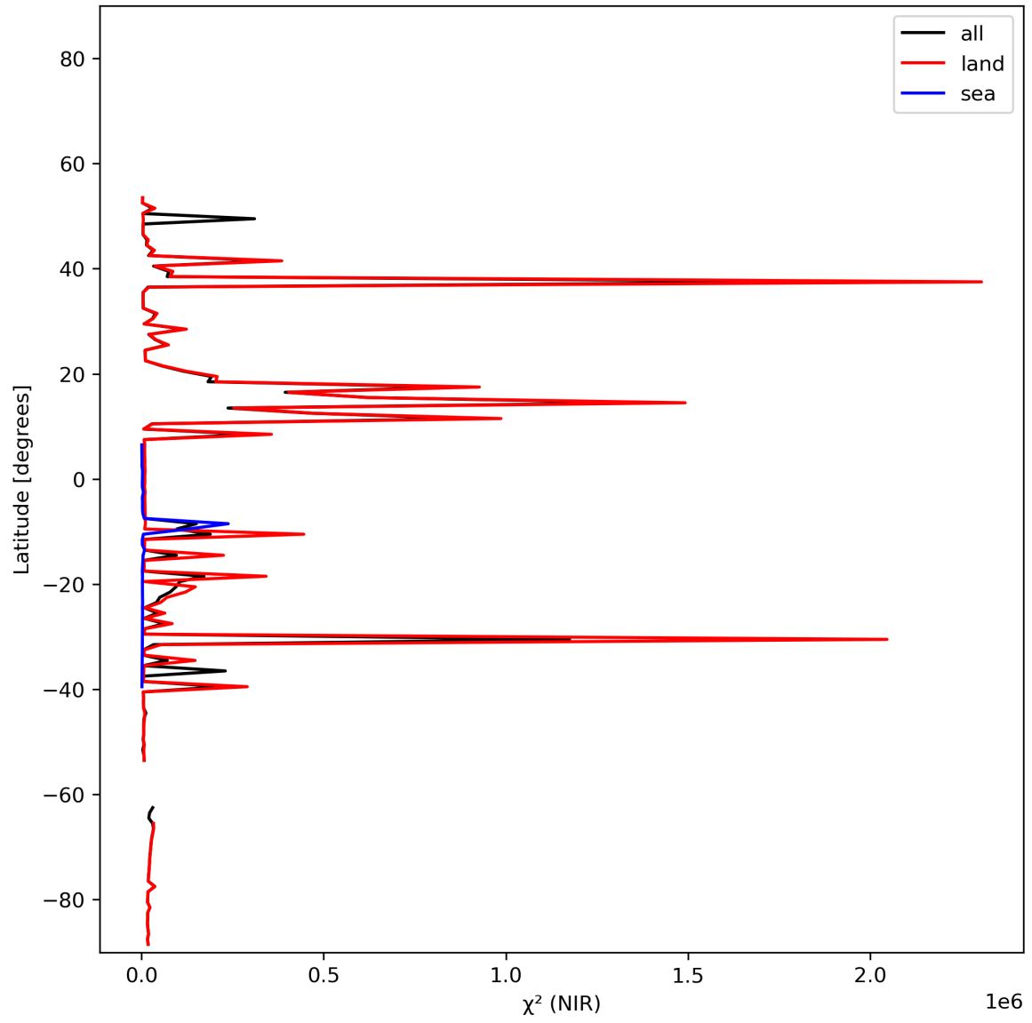
Figure 18: Zonal average of “ \chi^2 (NIR)” for 2023-12-01 to 2023-12-03.
