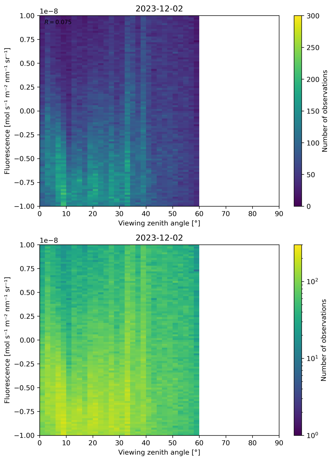
Figure 108: Scatter density plot of “Viewing zenith angle” against “Fluorescence” for 2023-12-01 to 2023-12-03.
