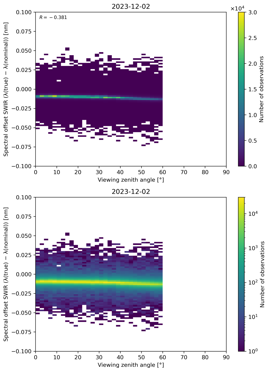
Figure 116: Scatter density plot of “Viewing zenith angle” against “Spectral offset SWIR ( \lambda(\text{true}) - \lambda(\text{nominal}) )” for 2023-12-01 to 2023-12-03.
