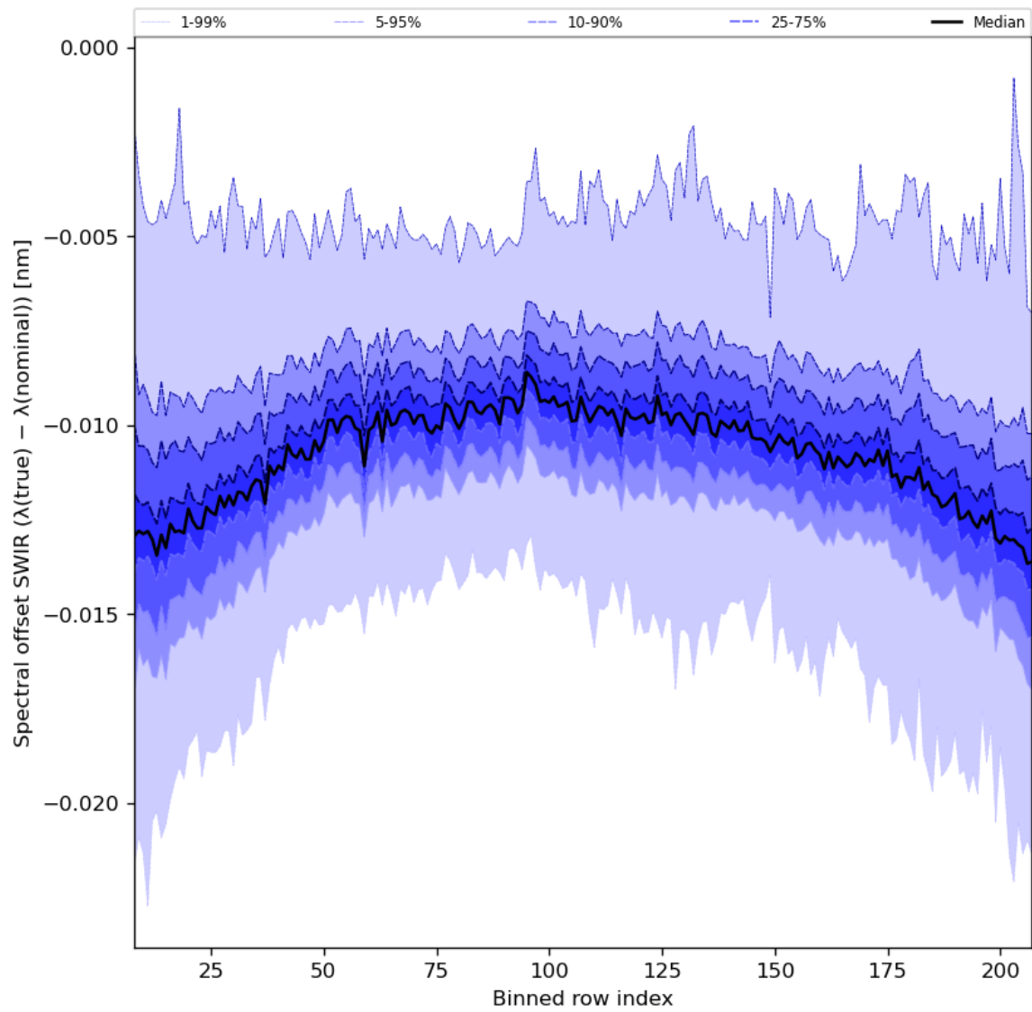
Figure 38: Along track statistics of “Spectral offset SWIR ( \lambda(\text{true}) - \lambda(\text{nominal}) )” for 2023-12-01 to 2023-12-03
