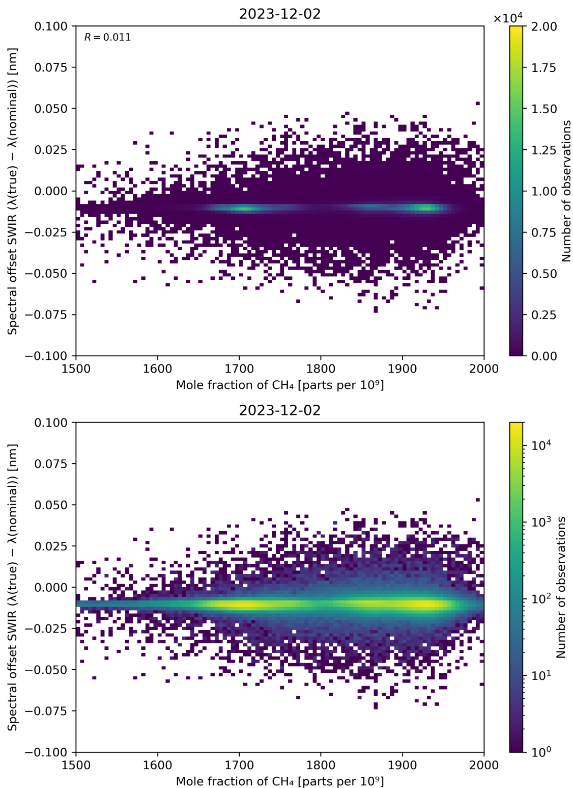
Figure 86: Scatter density plot of “Mole fraction of CH 4 ” against “Spectral offset SWIR ( \lambda(\text{true}) - \lambda(\text{nominal}) )” for 2023-12-01 to 2023-12-03.
