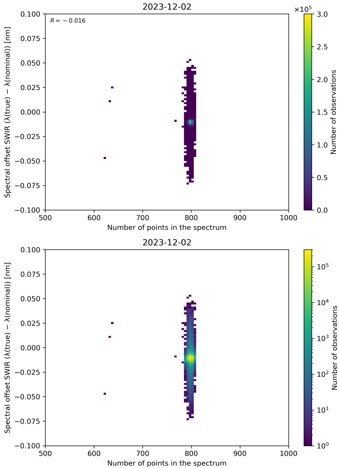
Figure 93: Scatter density plot of “Number of points in the spectrum” against “Spectral offset SWIR ( \lambda(\text{true}) - \lambda(\text{nominal}) )” for 2023-12-01 to 2023-12-03.
