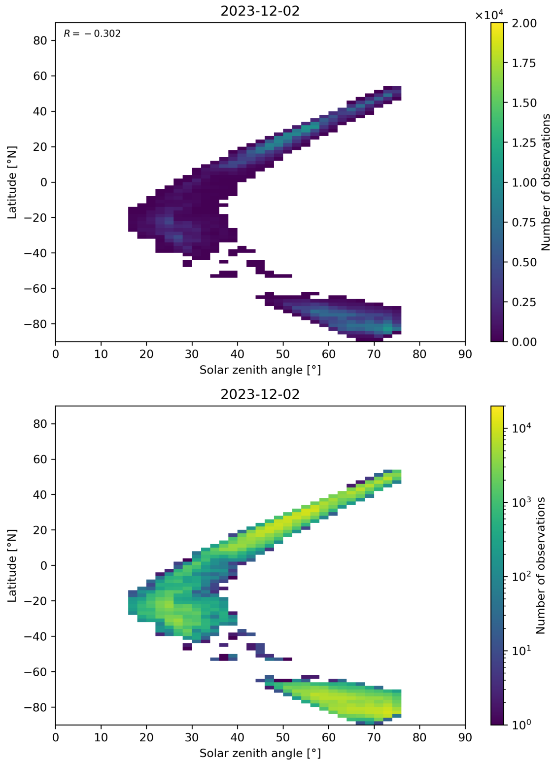
Figure 98: Scatter density plot of “Solar zenith angle” against “Latitude” for 2023-12-01 to 2023-12-03.
