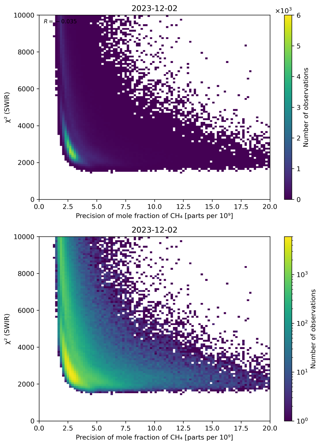
Figure 79: Scatter density plot of “Precision of mole fraction of \text{CH}_4 ” against “ \chi^2 (SWIR)” for 2023-12-01 to 2023-12-03.
