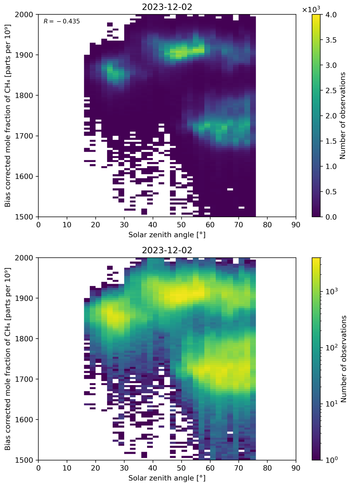
Figure 100: Scatter density plot of “Solar zenith angle” against “Bias corrected mole fraction of CH 4 ” for 2023-12-01 to 2023-12-03.
