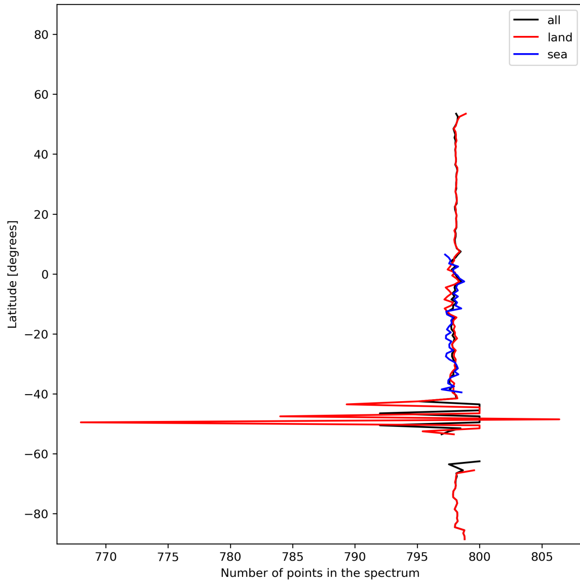
Figure 15: Zonal average of “Number of points in the spectrum” for 2023-12-01 to 2023-12-03.
