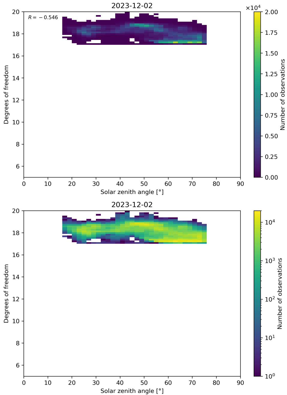
Figure 96: Scatter density plot of “Solar zenith angle” against “Degrees of freedom” for 2023-12-01 to 2023-12-03.
