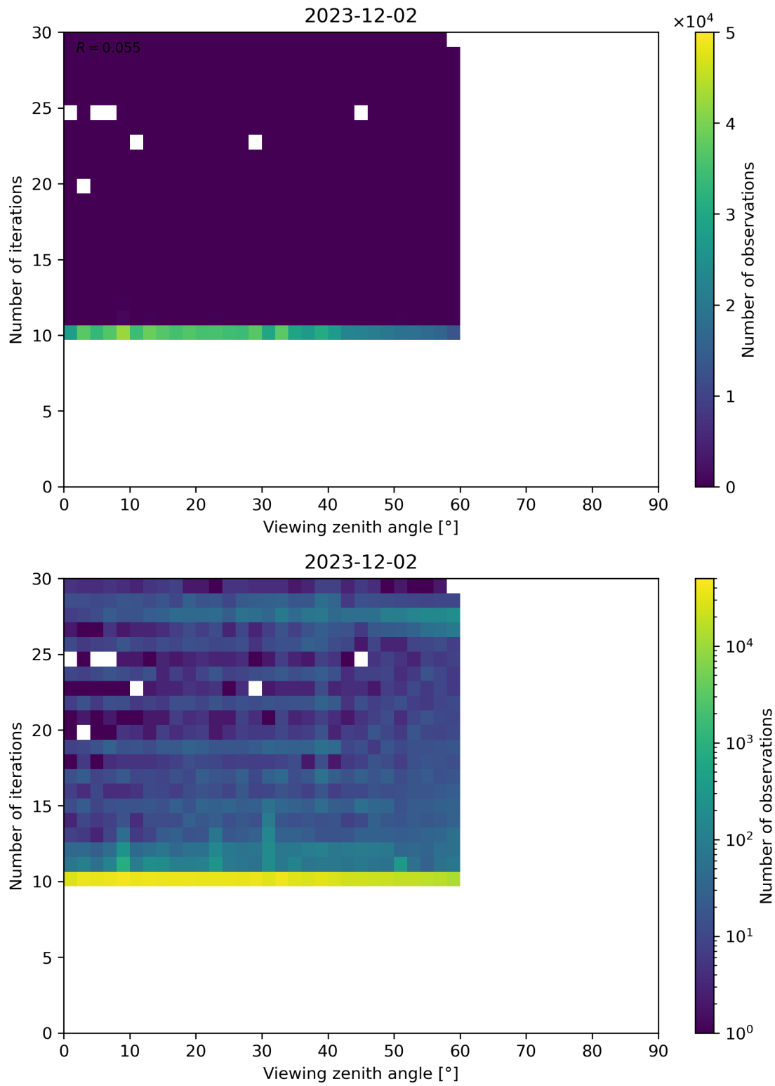
Figure 113: Scatter density plot of “Viewing zenith angle” against “Number of iterations” for 2023-12-01 to 2023-12-03.
