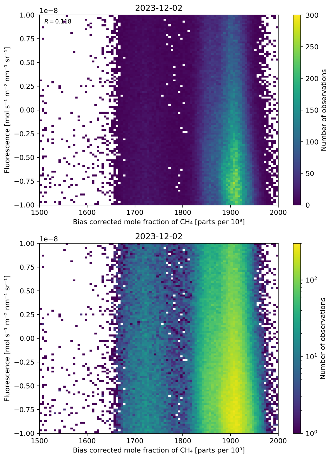
Figure 66: Scatter density plot of “Bias corrected mole fraction of \text{CH}_4 ” against “Fluorescence” for 2023-12-01 to 2023-12-03.
