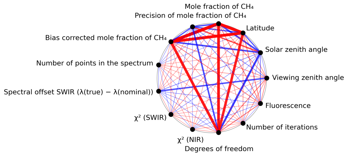
Figure 1: Map of correlation graph for 2023-12-01 to 2023-12-03.
