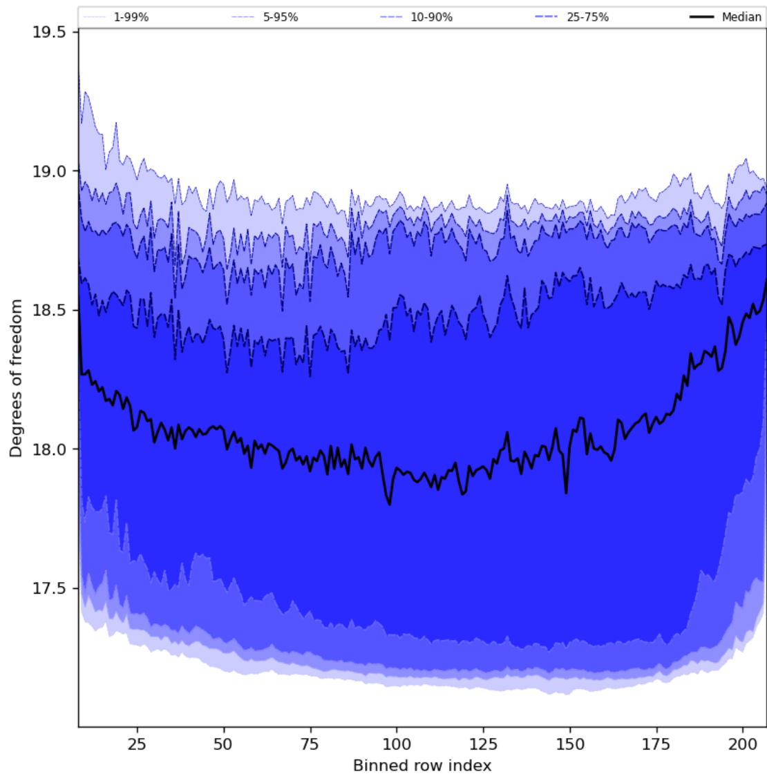
Figure 41: Along track statistics of “Degrees of freedom” for 2023-12-01 to 2023-12-03
