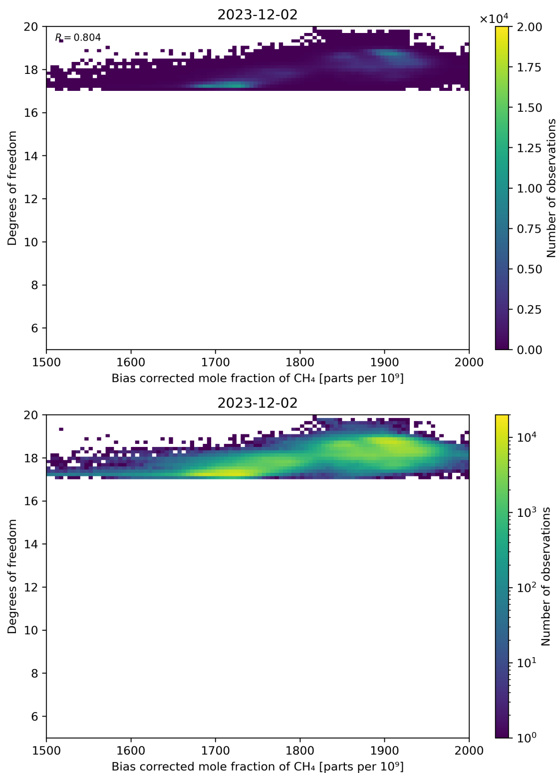
Figure 65: Scatter density plot of “Bias corrected mole fraction of CH 4 ” against “Degrees of freedom” for 2023-12-01 to 2023-12-03.
