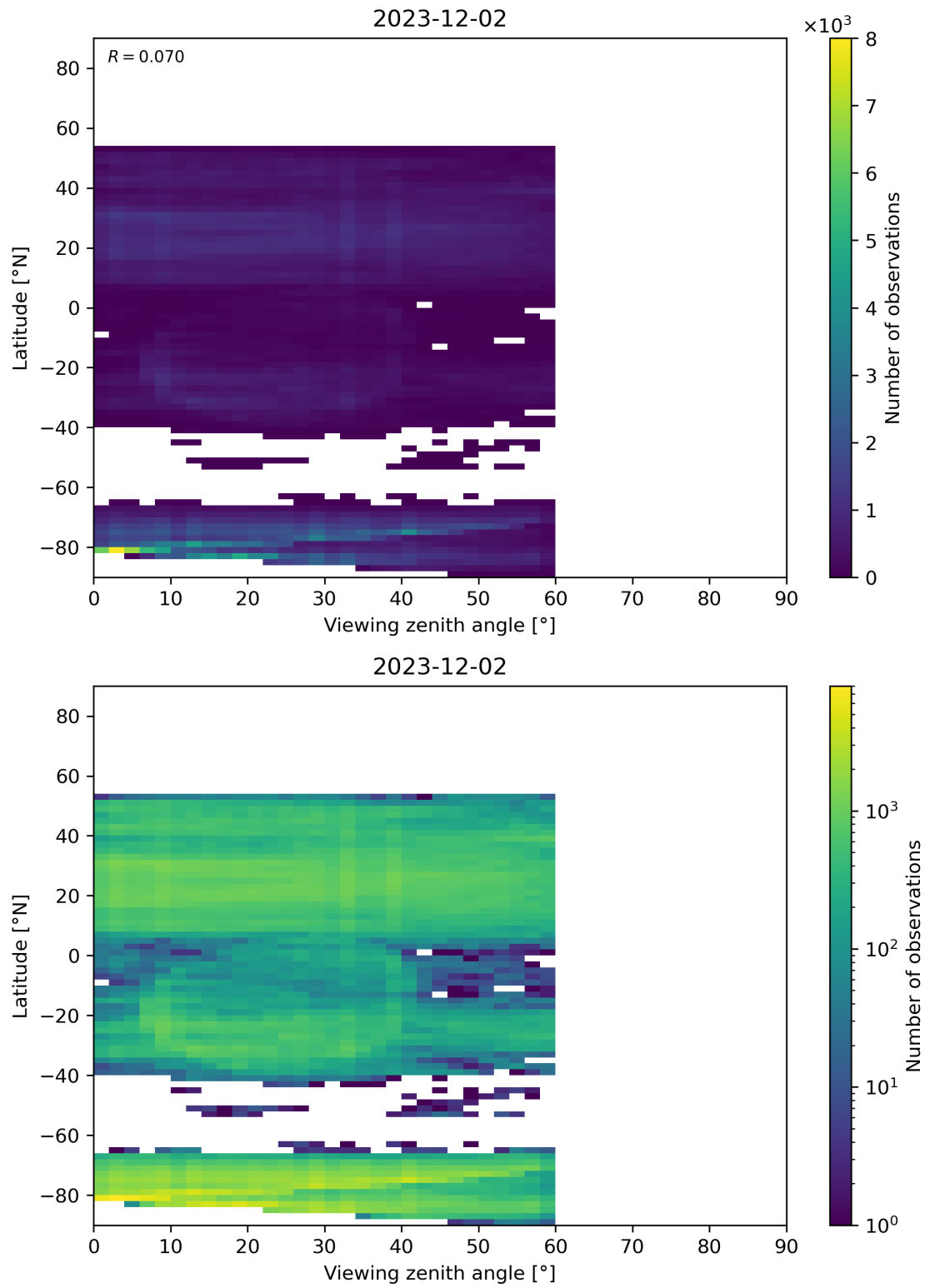
Figure 109: Scatter density plot of “Viewing zenith angle” against “Latitude” for 2023-12-01 to 2023-12-03.
