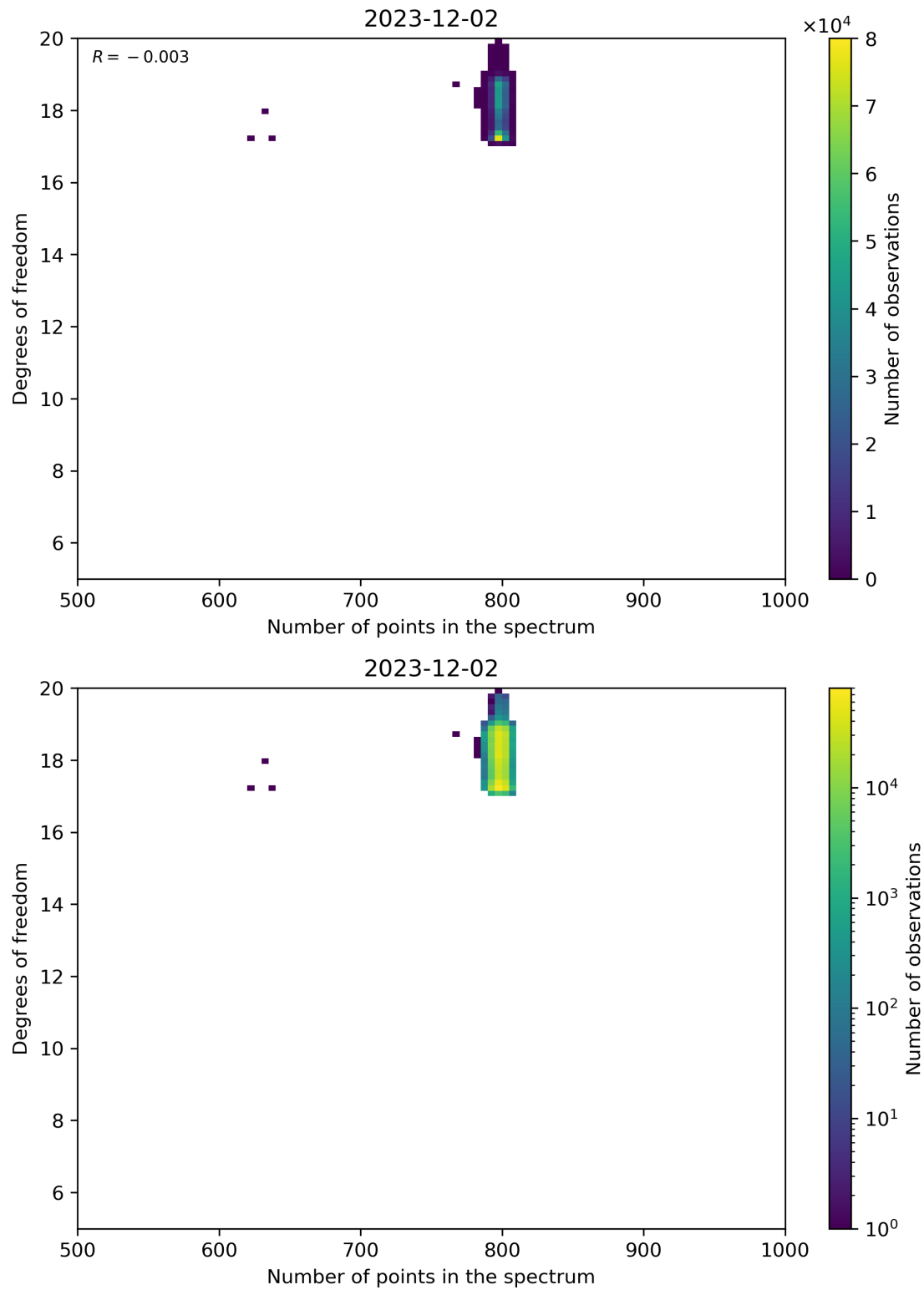
Figure 90: Scatter density plot of “Number of points in the spectrum” against “Degrees of freedom” for 2023-12-01 to 2023-12-03.
