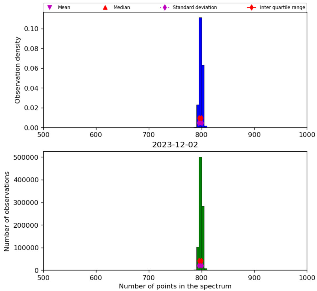
Figure 26: Histogram of “Number of points in the spectrum” for 2023-12-01 to 2023-12-03
