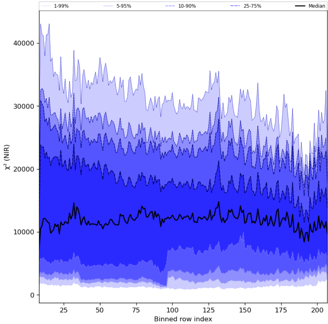
Figure 40: Along track statistics of “ \chi^2 (NIR)” for 2023-12-01 to 2023-12-03
