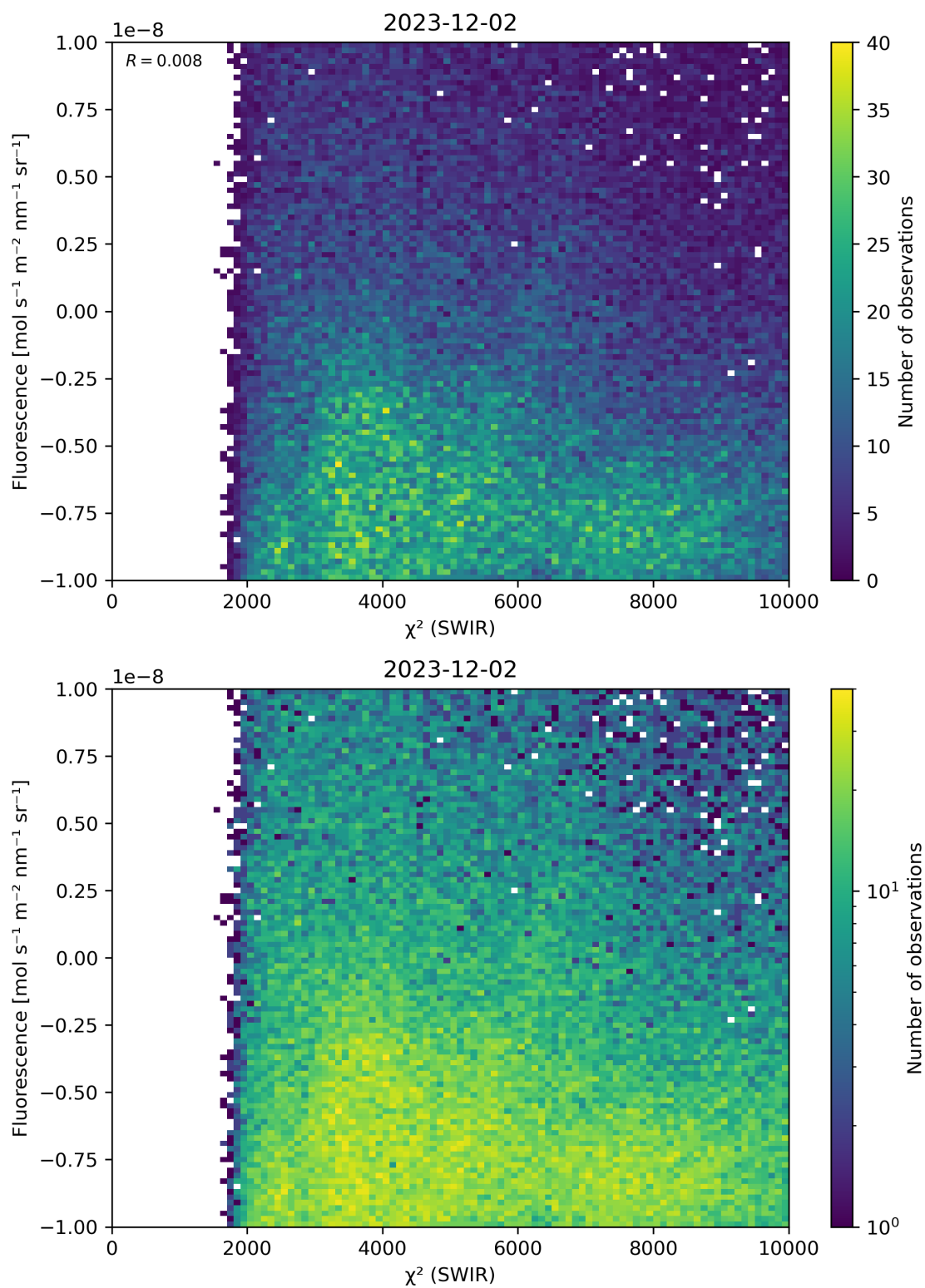
Figure 49: Scatter density plot of “ \chi^2 (SWIR)” against “Fluorescence” for 2023-12-01 to 2023-12-03.
