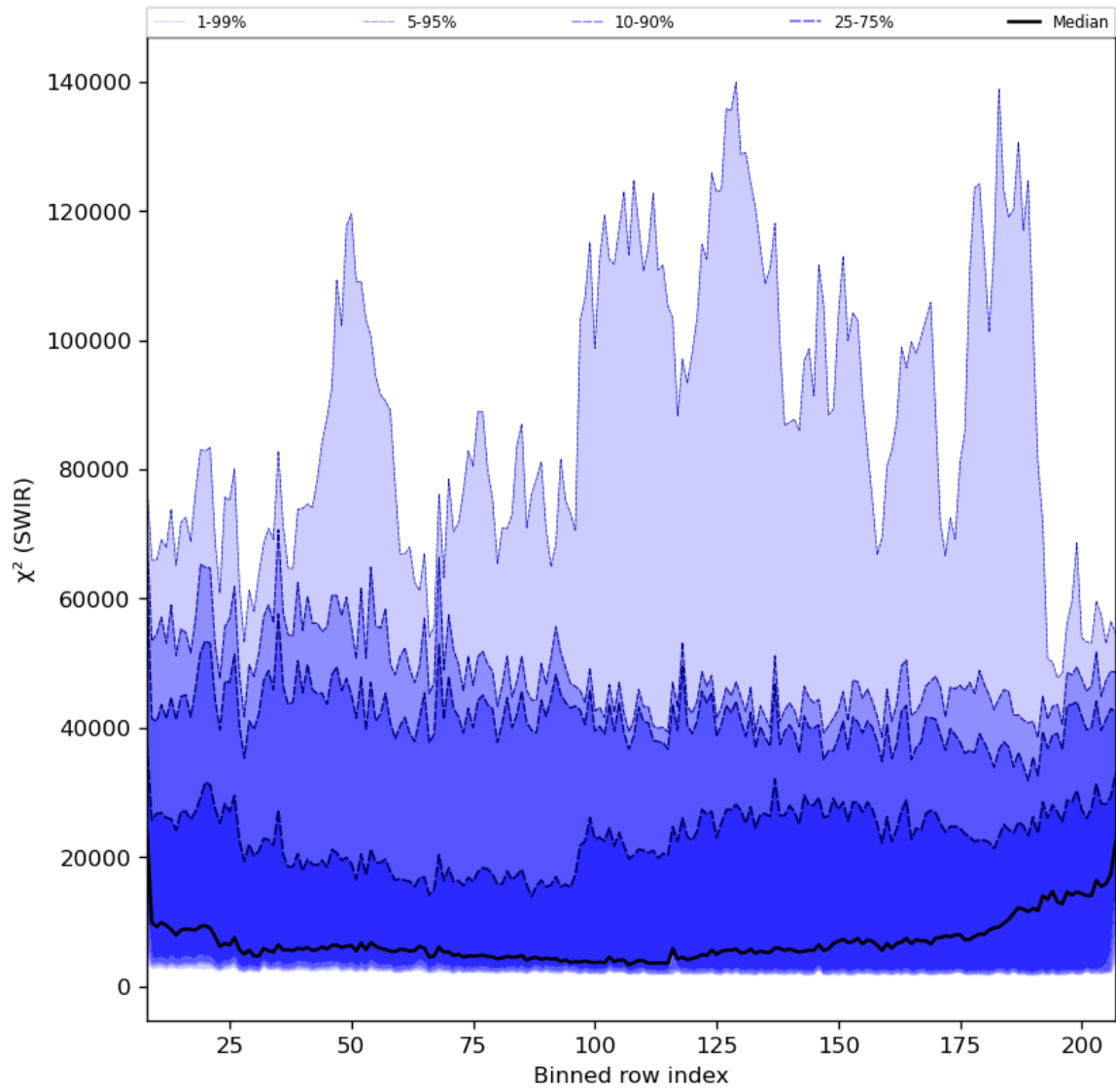
Figure 39: Along track statistics of " \chi^2 (SWIR)" for 2023-12-01 to 2023-12-03
