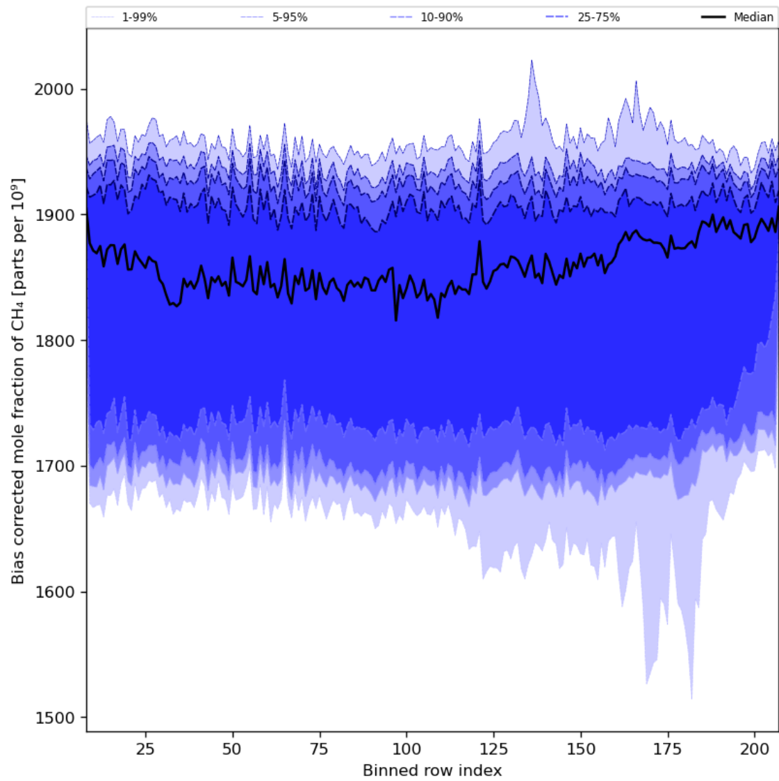
Figure 36: Along track statistics of “Bias corrected mole fraction of CH 4 ” for 2023-12-01 to 2023-12-03
