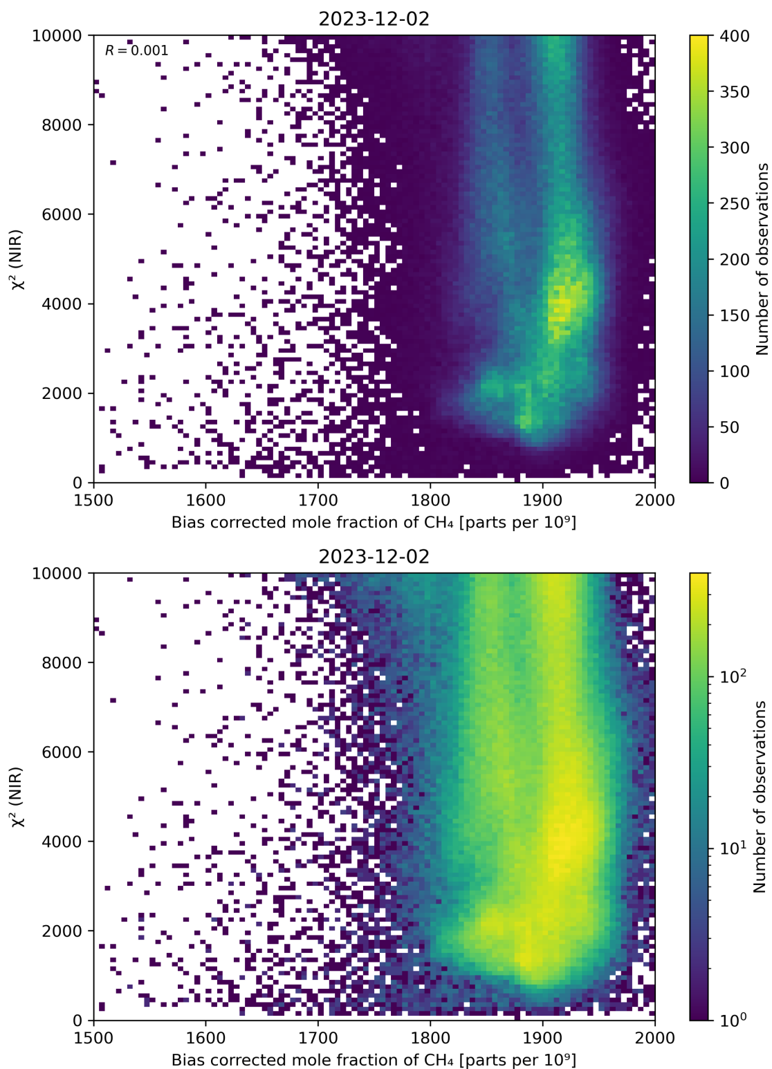
Figure 63: Scatter density plot of “Bias corrected mole fraction of CH 4 ” against “ \chi^2 (NIR)” for 2023-12-01 to 2023-12-03.
