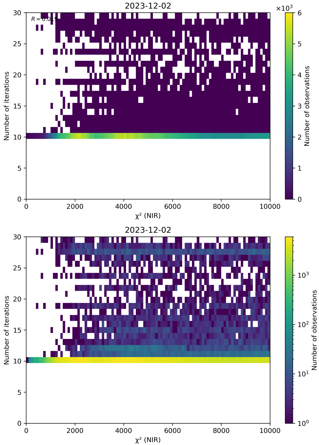
Figure 46: Scatter density plot of “ \chi^2 (NIR)” against “Number of iterations” for 2023-12-01 to 2023-12-03.
