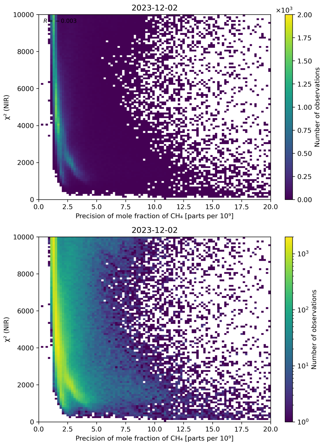
Figure 78: Scatter density plot of “Precision of mole fraction of CH 4 ” against “ \chi^2 (NIR)” for 2023-12-01 to 2023-12-03.
