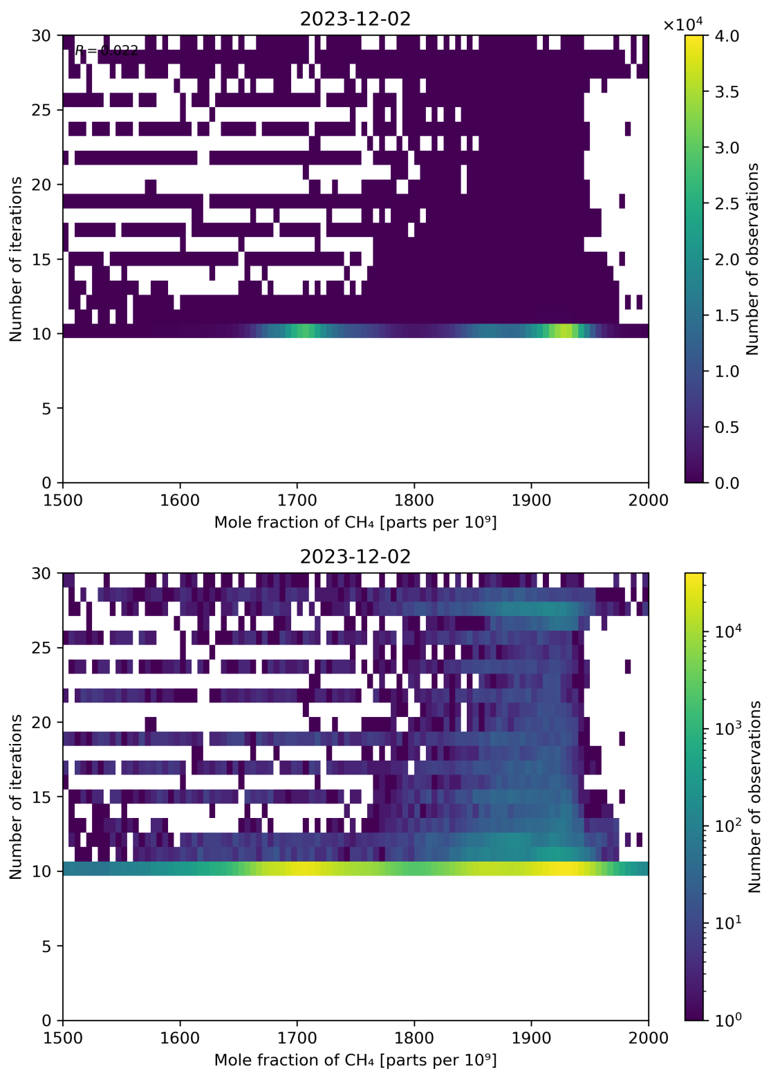
Figure 76: Scatter density plot of “Mole fraction of CH 4 ” against “Number of iterations” for 2023-12-01 to 2023-12-03.
