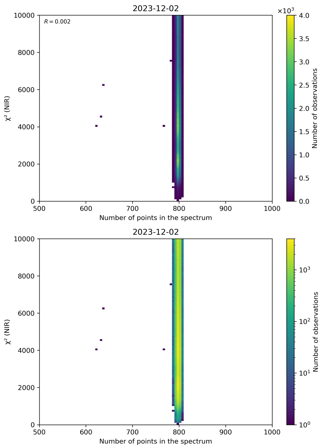
Figure 88: Scatter density plot of “Number of points in the spectrum” against “ \chi^2 (NIR)” for 2023-12-01 to 2023-12-03.
