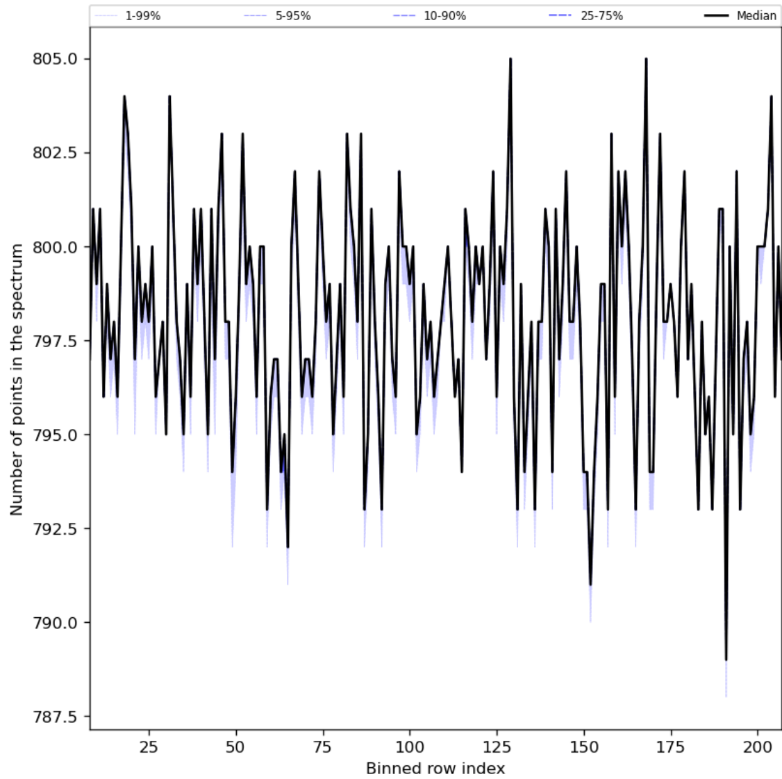
Figure 37: Along track statistics of “Number of points in the spectrum” for 2023-12-01 to 2023-12-03
