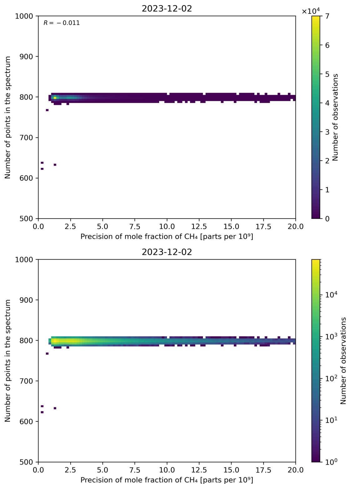
Figure 84: Scatter density plot of “Precision of mole fraction of CH 4 ” against “Number of points in the spectrum” for 2023-12-01 to 2023-12-03.
