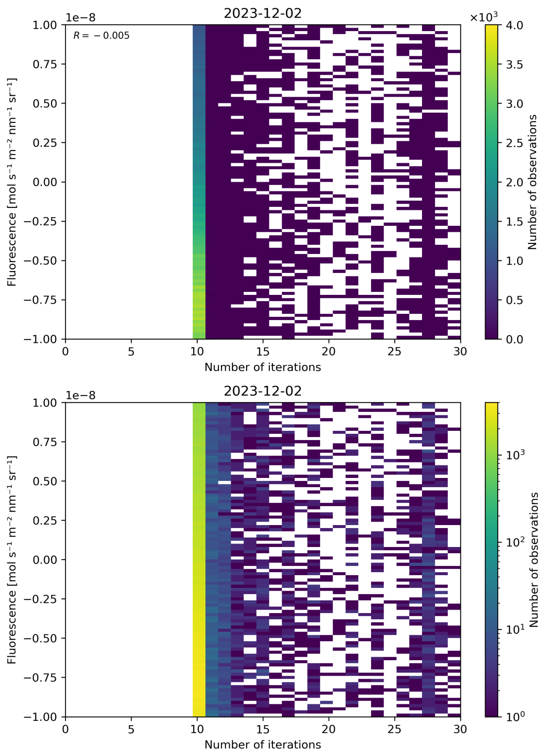
Figure 87: Scatter density plot of “Number of iterations” against “Fluorescence” for 2023-12-01 to 2023-12-03.
