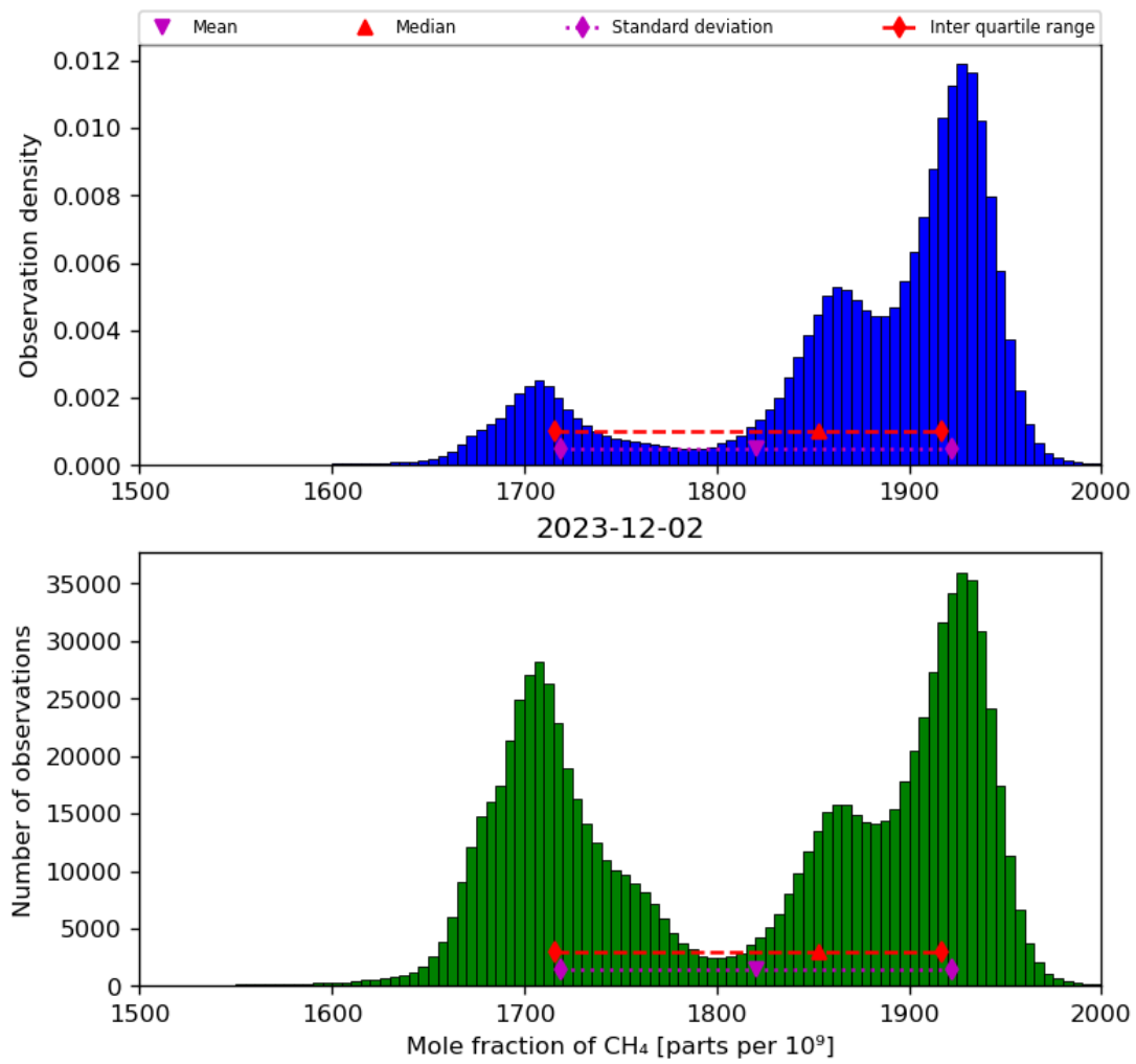
Figure 23: Histogram of “Mole fraction of CH 4 ” for 2023-12-01 to 2023-12-03
