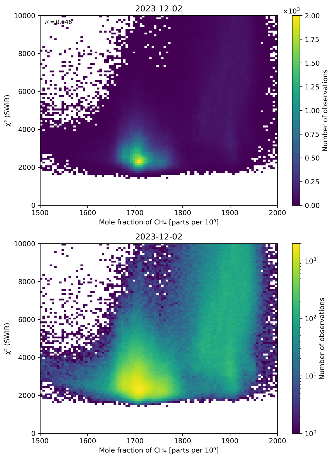
Figure 71: Scatter density plot of “Mole fraction of CH 4 ” against “ \chi^2 (SWIR)” for 2023-12-01 to 2023-12-03.
