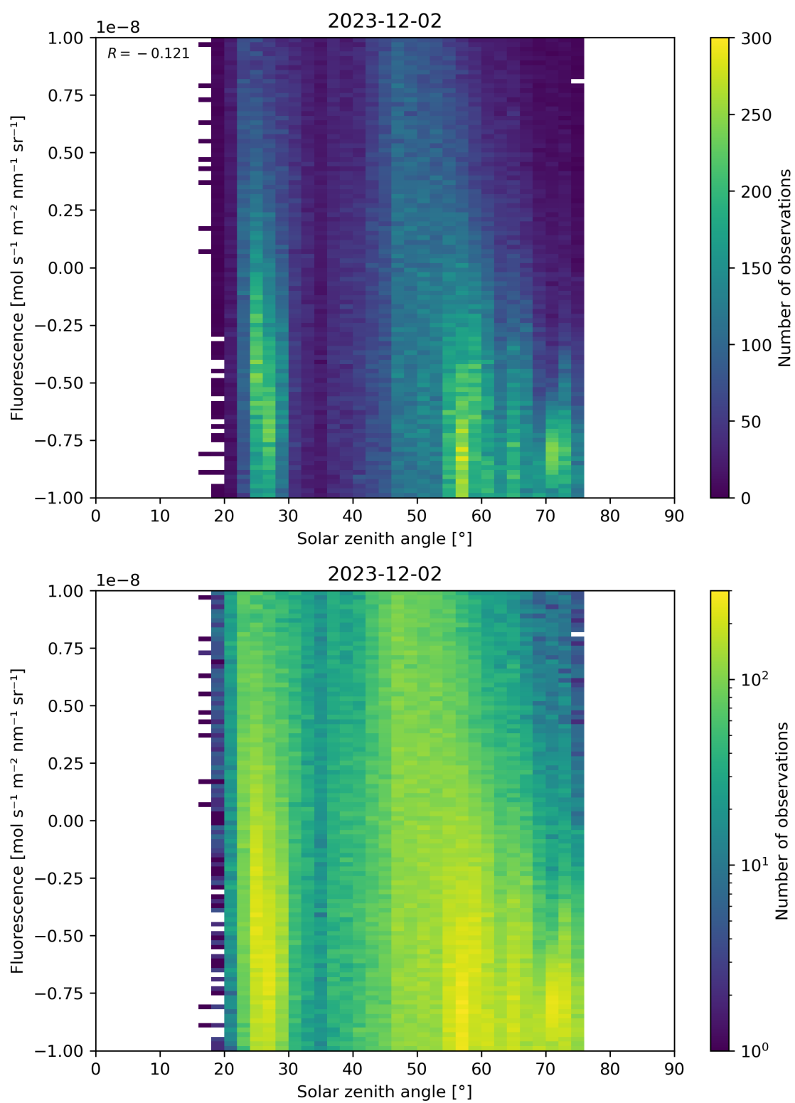
Figure 97: Scatter density plot of “Solar zenith angle” against “Fluorescence” for 2023-12-01 to 2023-12-03.
