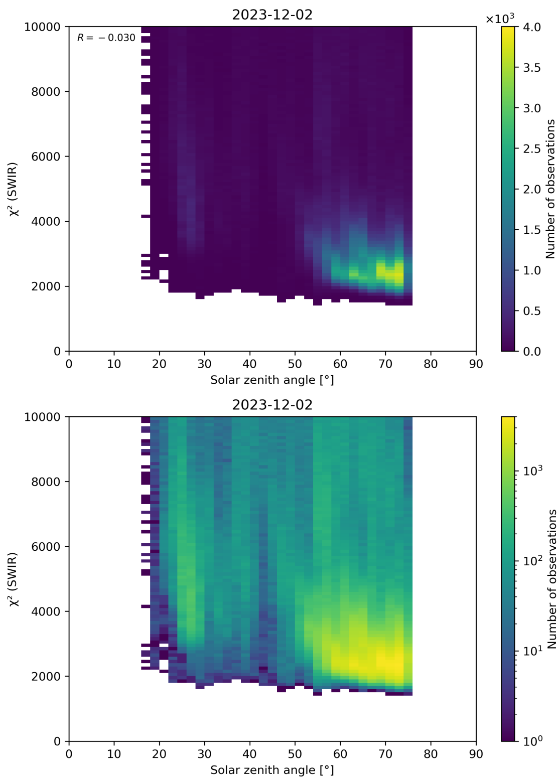
Figure 95: Scatter density plot of “Solar zenith angle” against “ \chi^2 (SWIR)” for 2023-12-01 to 2023-12-03.
