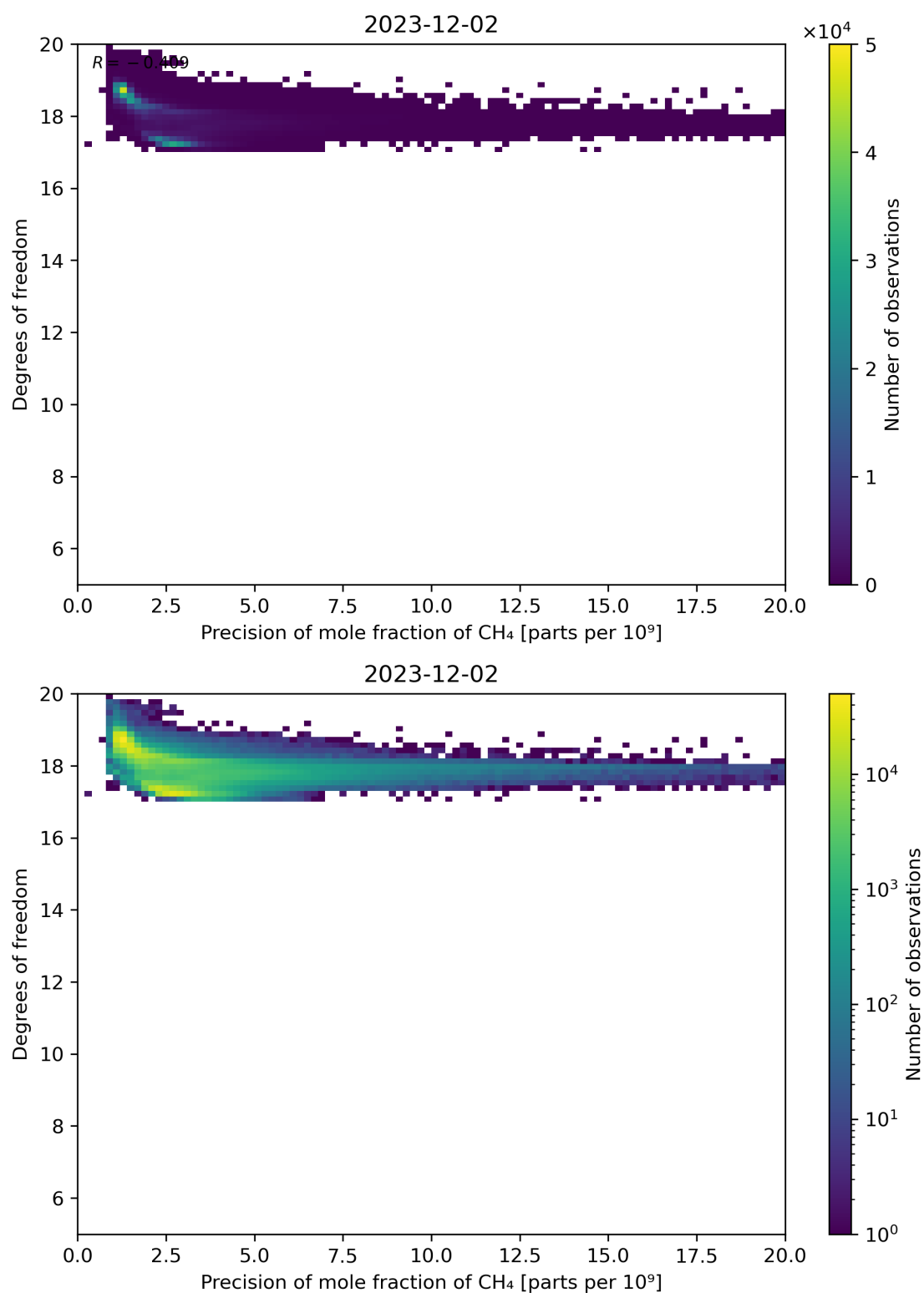
Figure 80: Scatter density plot of “Precision of mole fraction of CH 4 ” against “Degrees of freedom” for 2023-12-01 to 2023-12-03.
