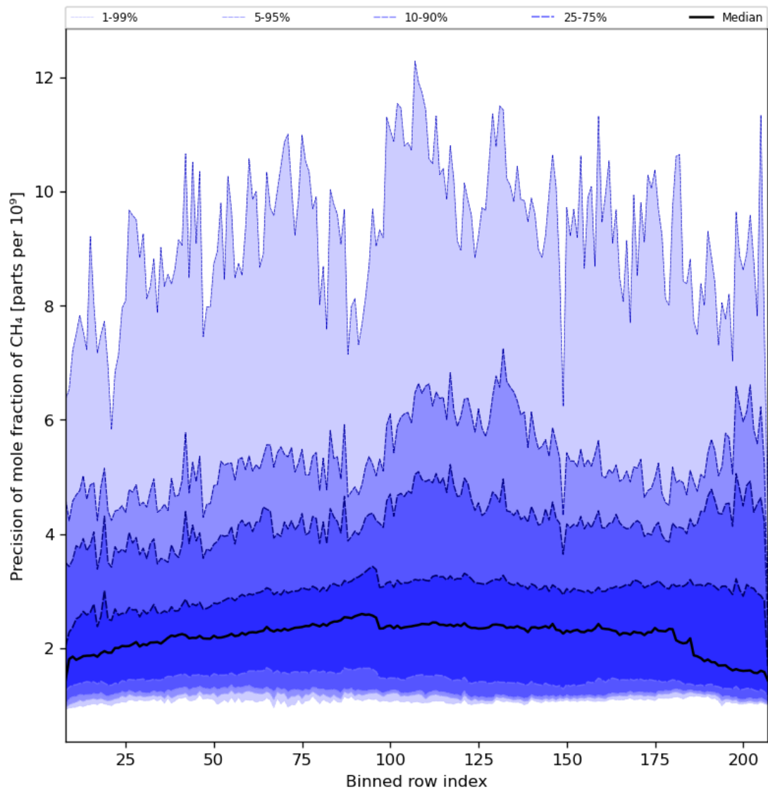
Figure 35: Along track statistics of “Precision of mole fraction of CH 4 ” for 2023-12-01 to 2023-12-03
