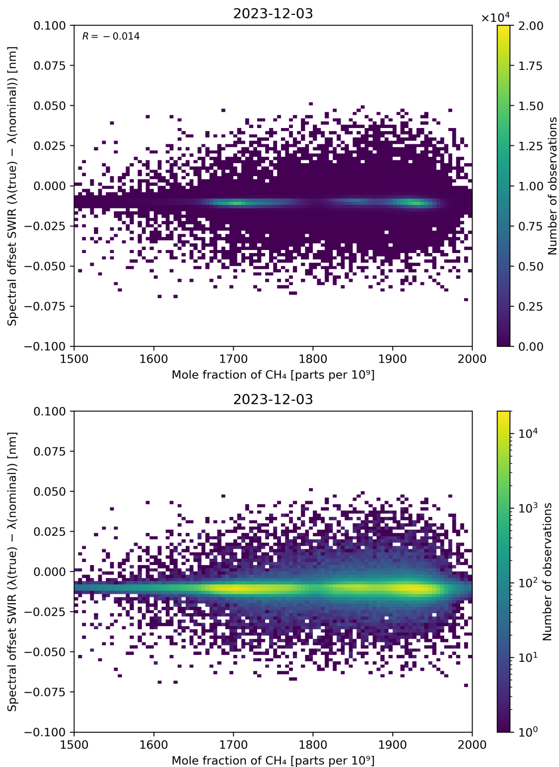
Figure 86: Scatter density plot of “Mole fraction of CH 4 ” against “Spectral offset SWIR ( \lambda(\text{true}) - \lambda(\text{nominal}) )” for 2023-12-02 to 2023-12-04.
