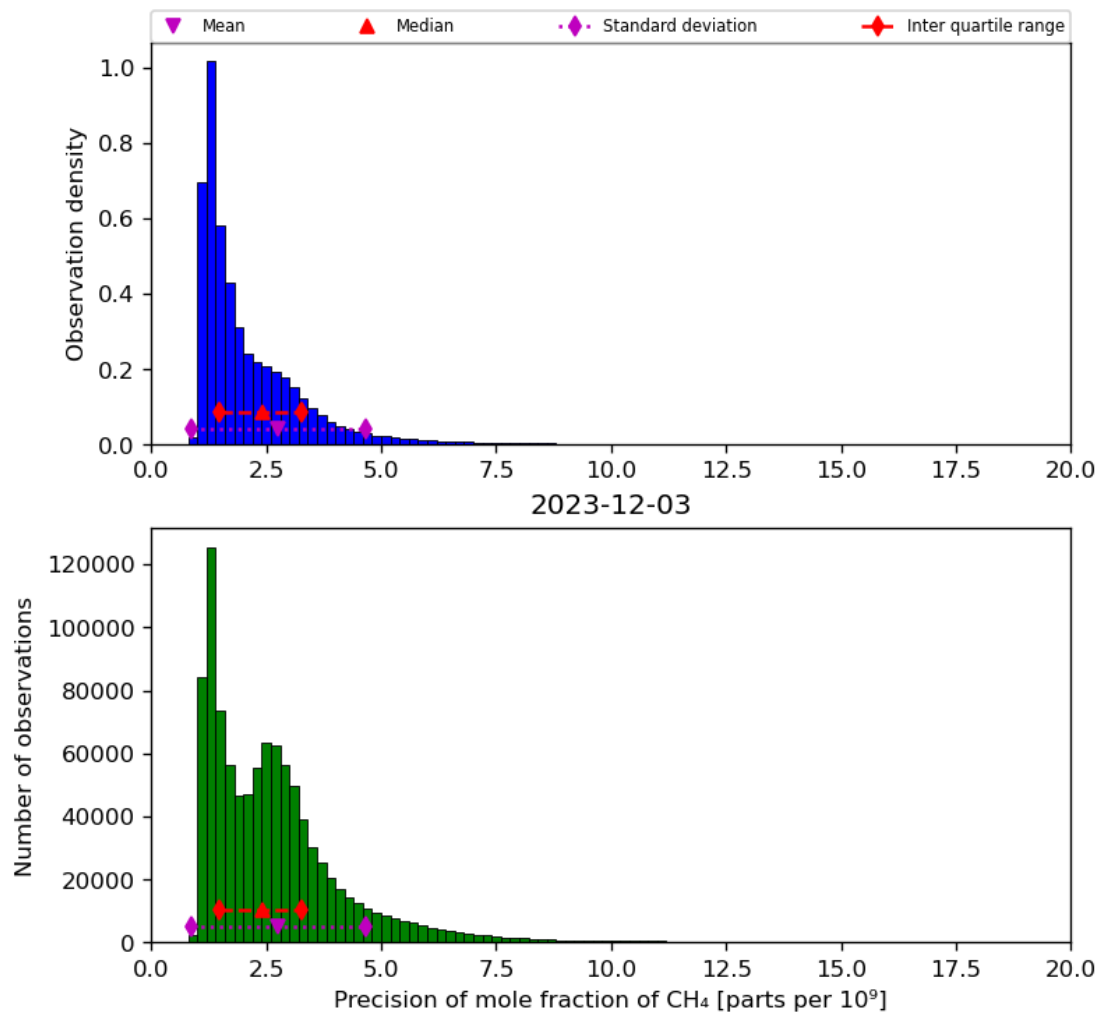
Figure 24: Histogram of “Precision of mole fraction of CH 4 ” for 2023-12-02 to 2023-12-04
