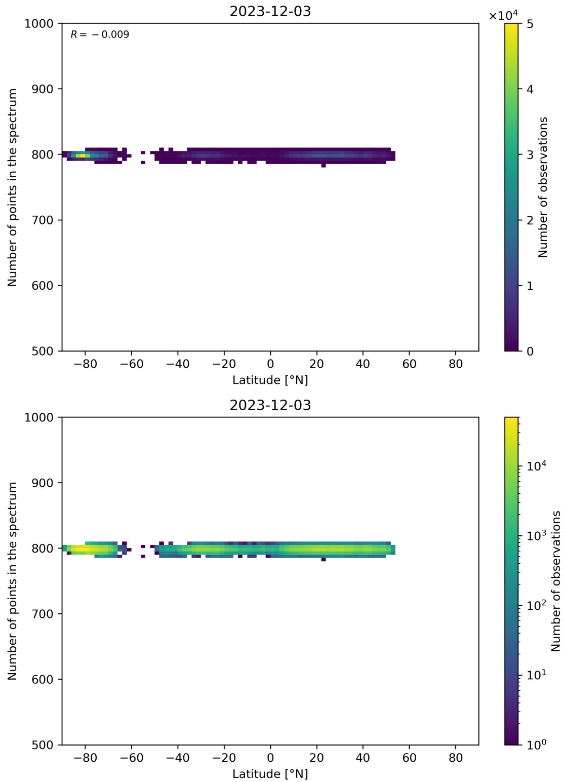
Figure 61: Scatter density plot of “Latitude” against “Number of points in the spectrum” for 2023-12-02 to 2023-12-04.
