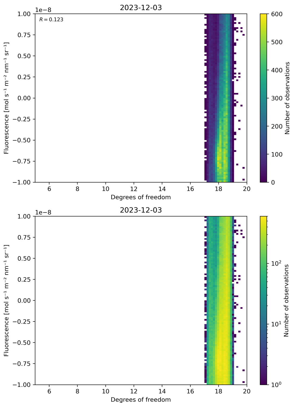
Figure 51: Scatter density plot of “Degrees of freedom” against “Fluorescence” for 2023-12-02 to 2023-12-04.
