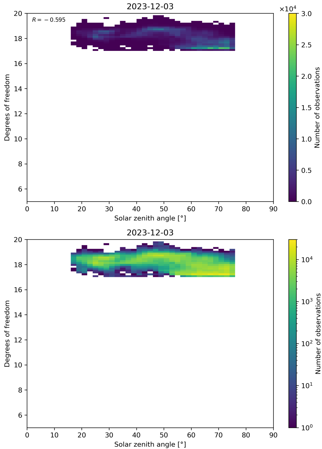
Figure 96: Scatter density plot of “Solar zenith angle” against “Degrees of freedom” for 2023-12-02 to 2023-12-04.
