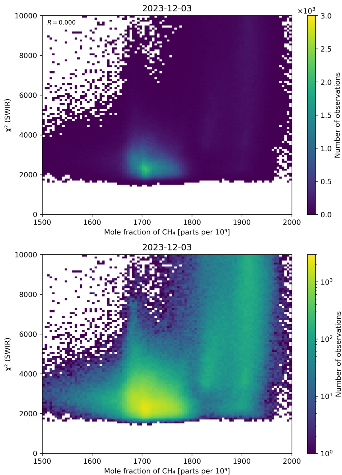
Figure 71: Scatter density plot of “Mole fraction of \text{CH}_4 ” against “ \chi^2 (SWIR)” for 2023-12-02 to 2023-12-04.
