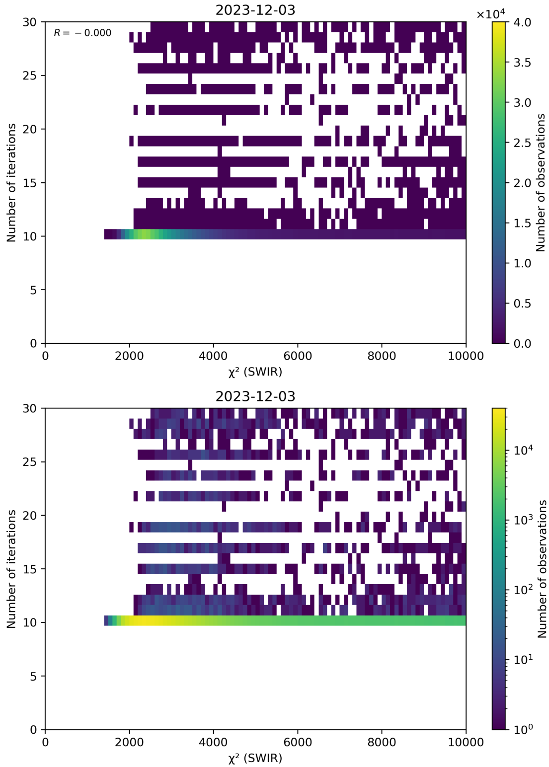
Figure 50: Scatter density plot of “ \chi^2 (SWIR)” against “Number of iterations” for 2023-12-02 to 2023-12-04.
