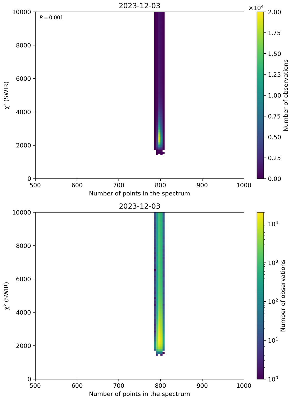
Figure 89: Scatter density plot of “Number of points in the spectrum” against “ \chi^2 (SWIR)” for 2023-12-02 to 2023-12-04.
