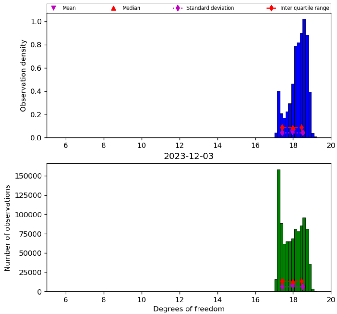
Figure 30: Histogram of “Degrees of freedom” for 2023-12-02 to 2023-12-04
