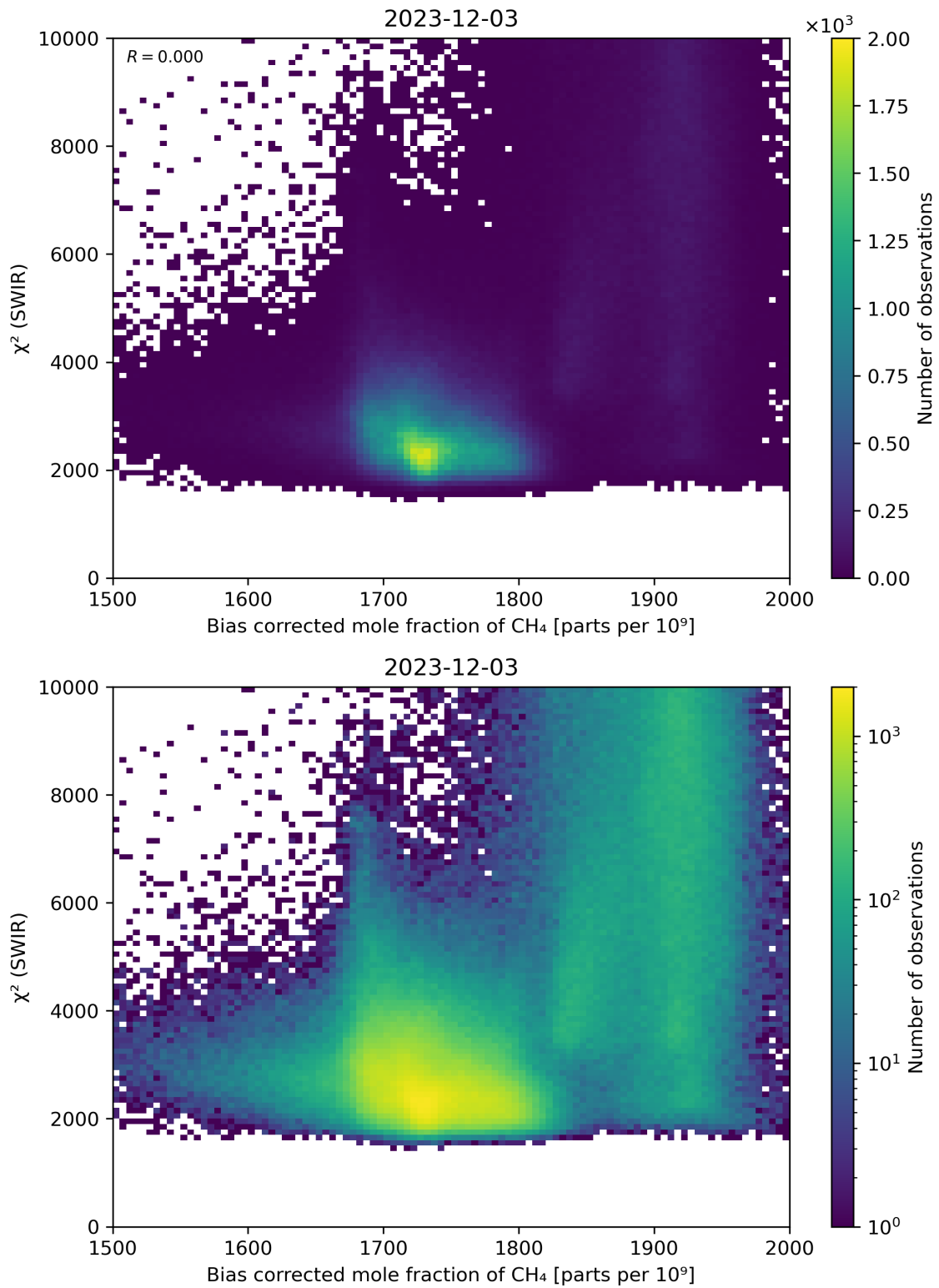
Figure 64: Scatter density plot of “Bias corrected mole fraction of \text{CH}_4 ” against “ \chi^2 (SWIR)” for 2023-12-02 to 2023-12-04.
