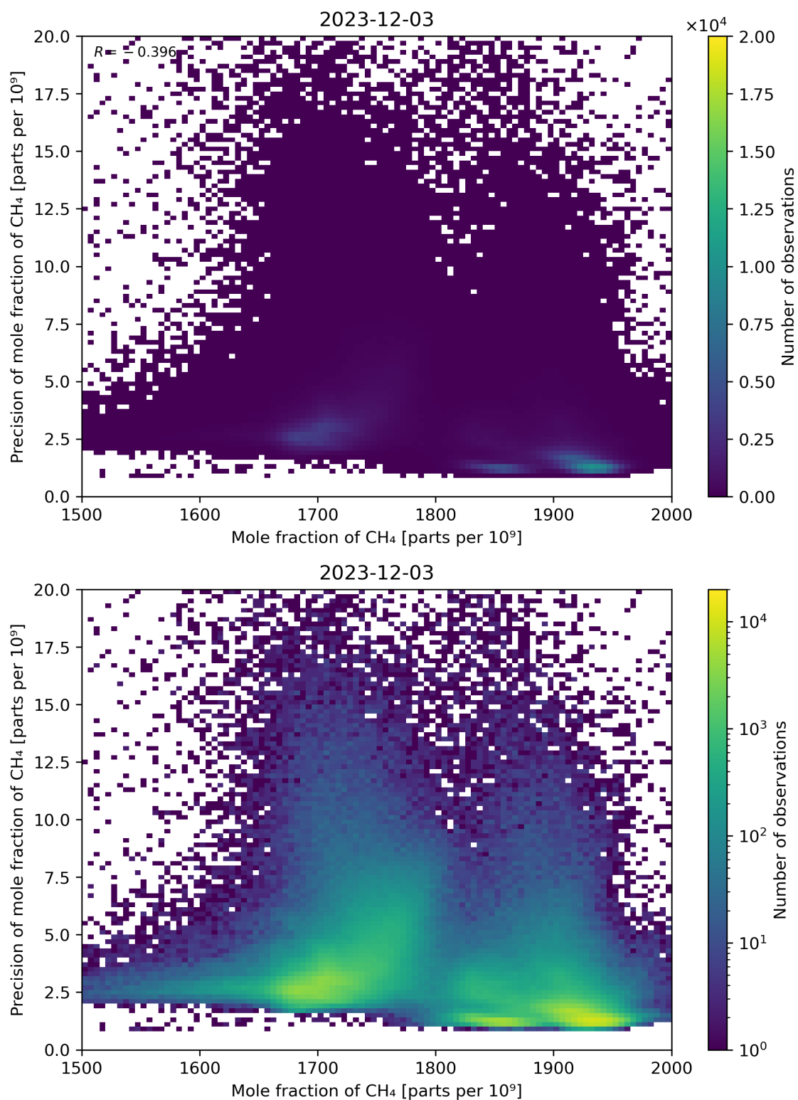
Figure 75: Scatter density plot of “Mole fraction of CH 4 ” against “Precision of mole fraction of CH 4 ” for 2023-12-02 to 2023-12-04.
