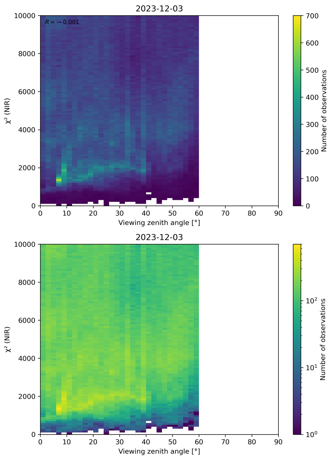
Figure 105: Scatter density plot of “Viewing zenith angle” against “ \chi^2 (NIR)” for 2023-12-02 to 2023-12-04.
