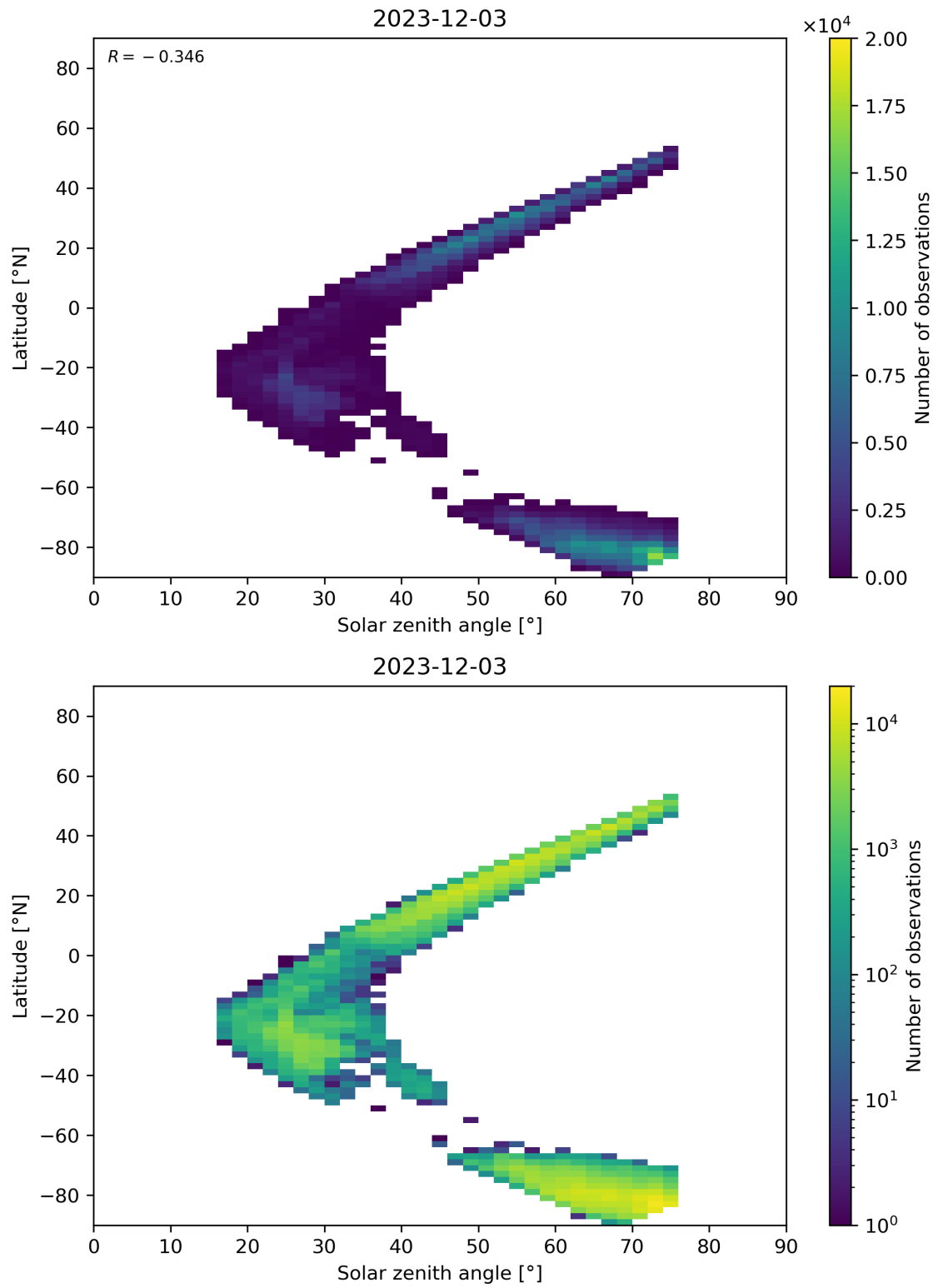
Figure 98: Scatter density plot of “Solar zenith angle” against “Latitude” for 2023-12-02 to 2023-12-04.
