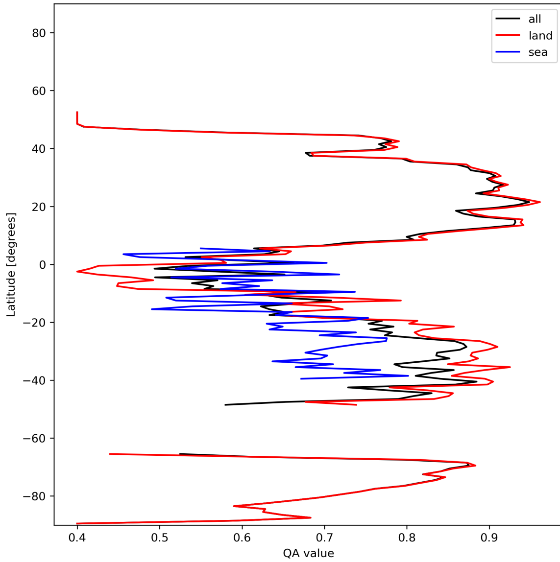
Figure 11: Zonal average of “QA value” for 2023-12-02 to 2023-12-04.
