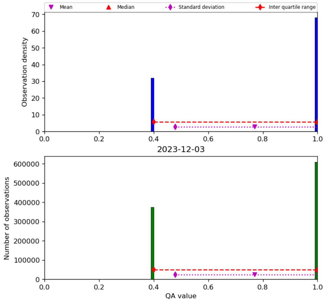
Figure 22: Histogram of “QA value” for 2023-12-02 to 2023-12-04
