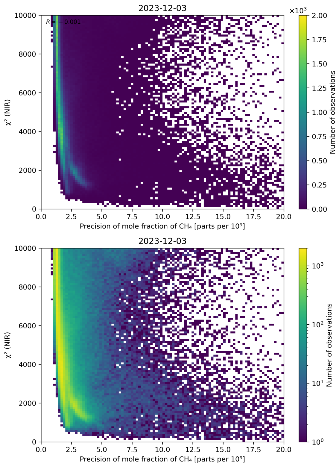
Figure 78: Scatter density plot of “Precision of mole fraction of CH 4 ” against “ \chi^2 (NIR)” for 2023-12-02 to 2023-12-04.
