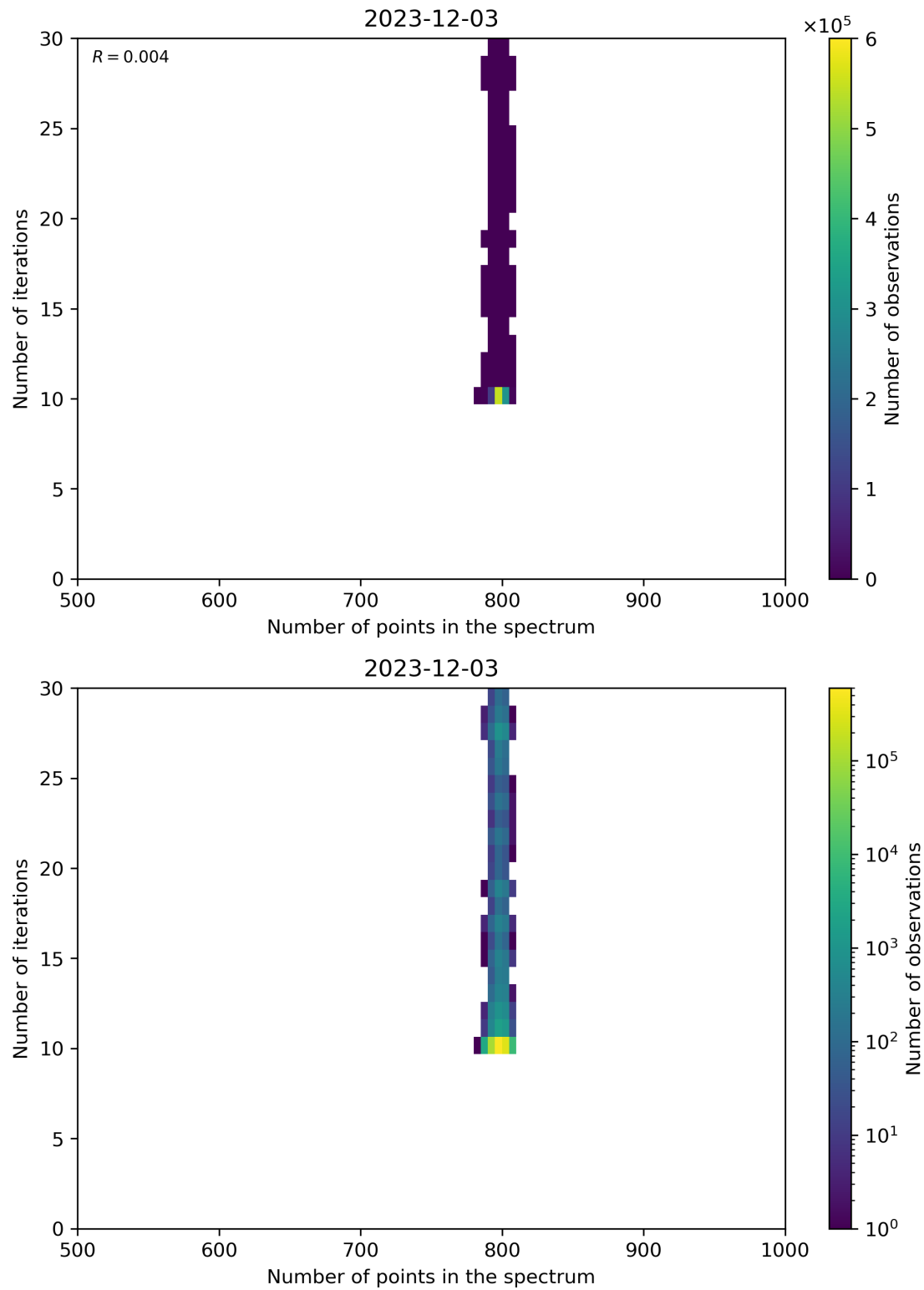
Figure 92: Scatter density plot of “Number of points in the spectrum” against “Number of iterations” for 2023-12-02 to 2023-12-04.
