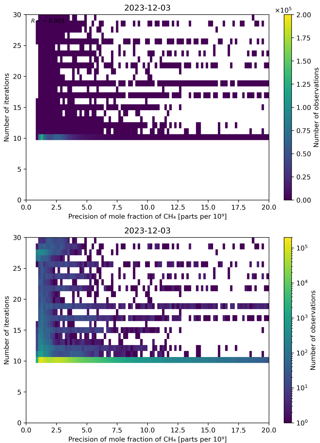
Figure 83: Scatter density plot of “Precision of mole fraction of CH 4 ” against “Number of iterations” for 2023-12-02 to 2023-12-04.
