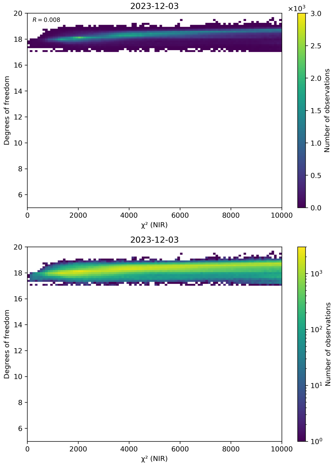
Figure 44: Scatter density plot of “ \chi^2 (NIR)” against “Degrees of freedom” for 2023-12-02 to 2023-12-04.
