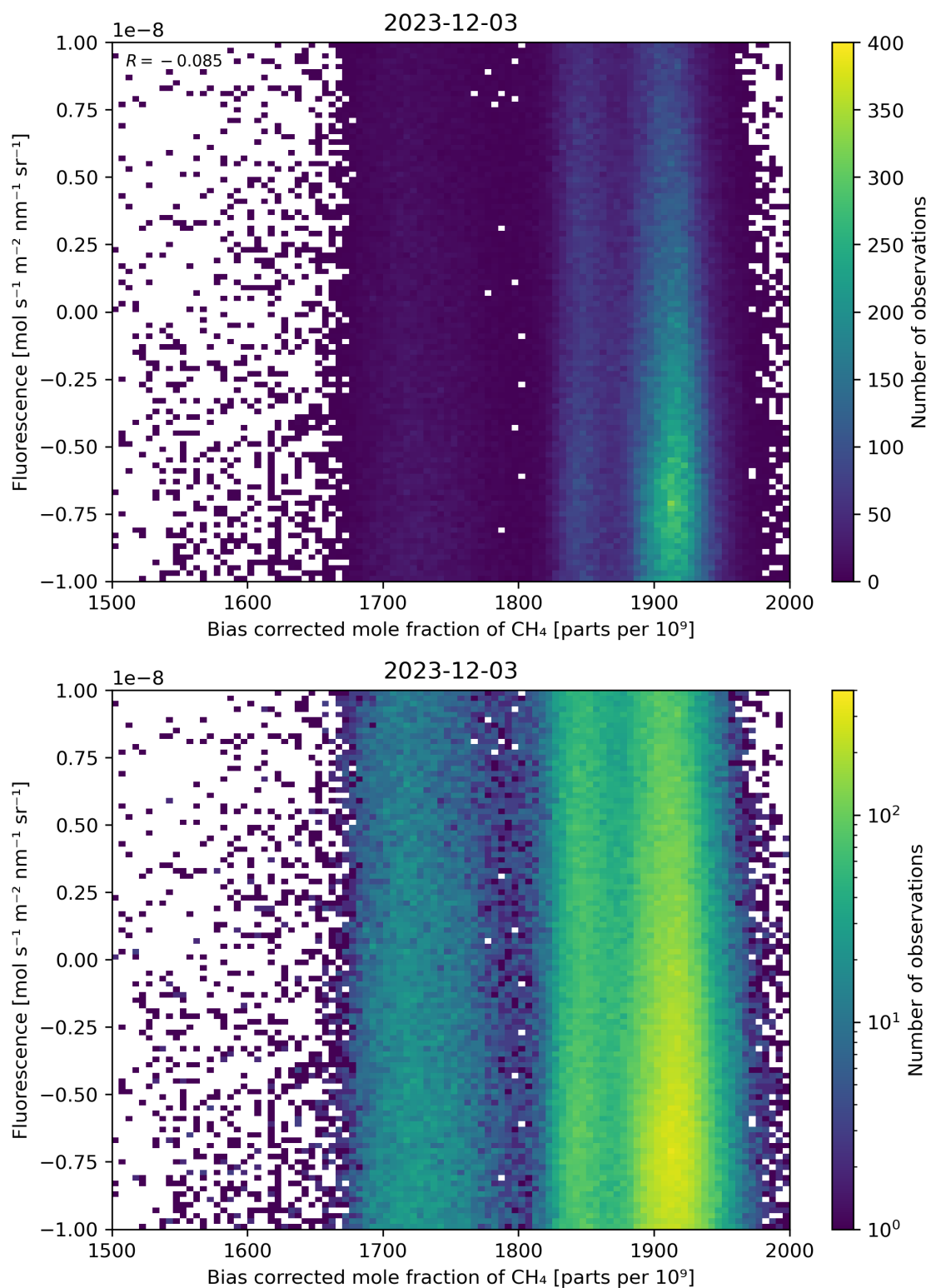
Figure 66: Scatter density plot of “Bias corrected mole fraction of \text{CH}_4 ” against “Fluorescence” for 2023-12-02 to 2023-12-04.
