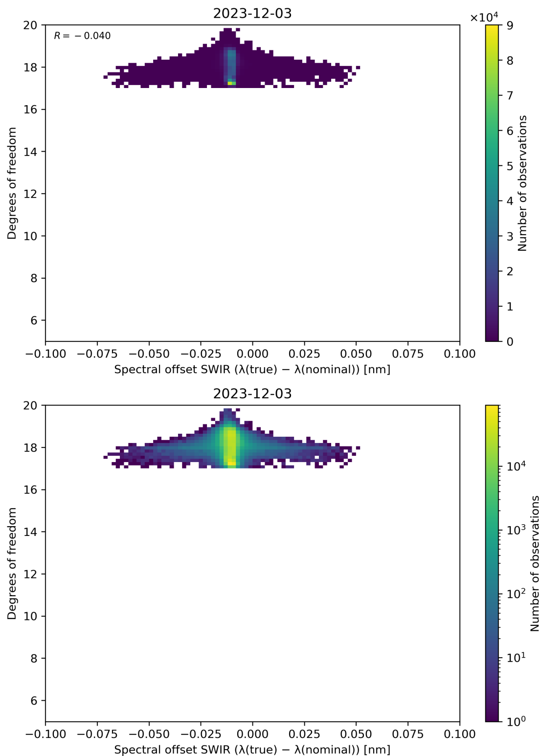
Figure 119: Scatter density plot of “Spectral offset SWIR ( \lambda(\text{true}) - \lambda(\text{nominal}) )” against “Degrees of freedom” for 2023-12-02 to 2023-12-04.
