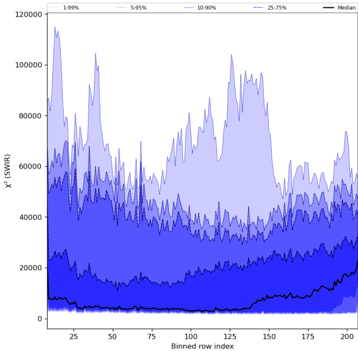
Figure 39: Along track statistics of “ \chi^2 (SWIR)” for 2023-12-02 to 2023-12-04
