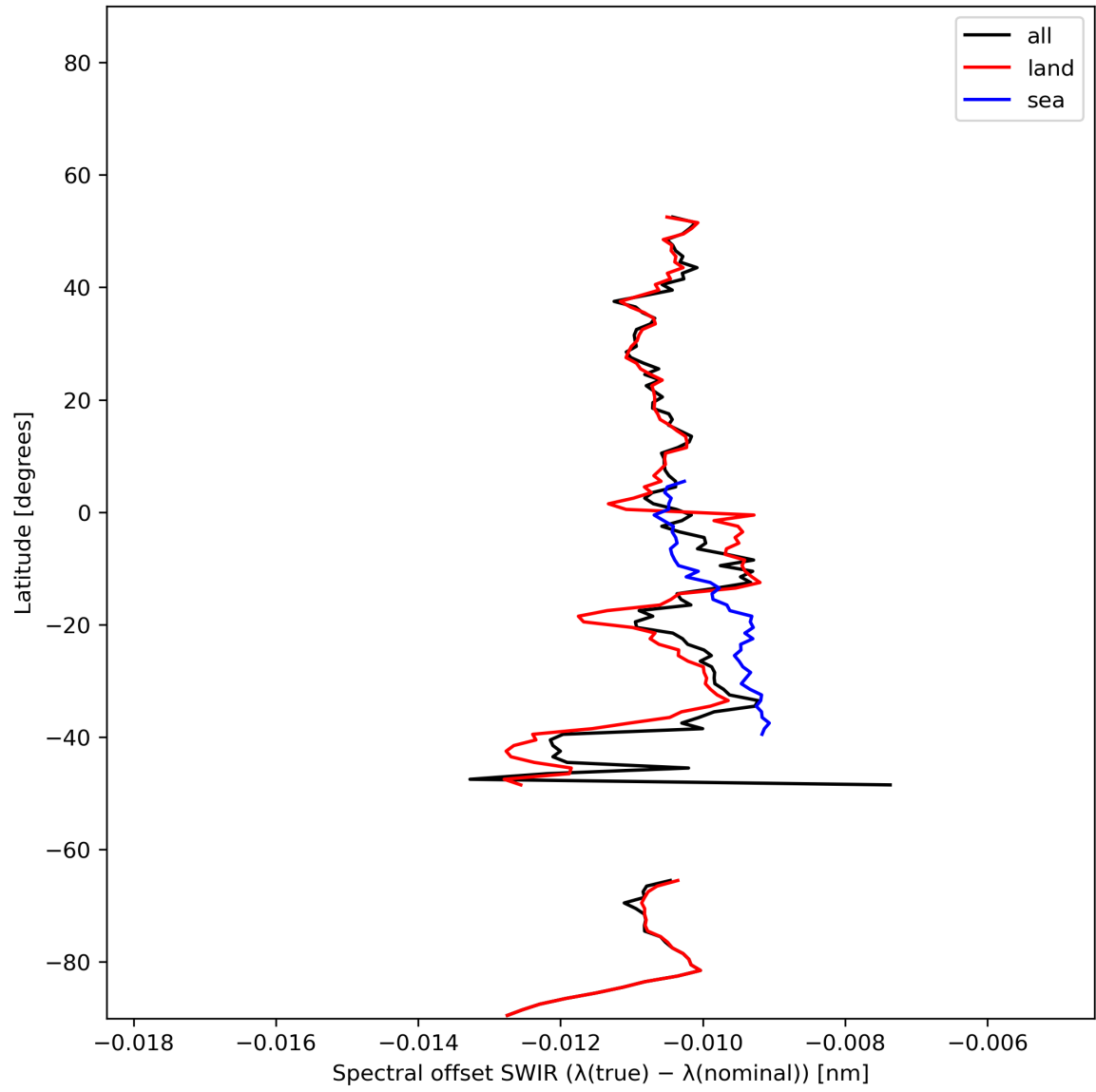
Figure 16: Zonal average of “Spectral offset SWIR ( \lambda(\text{true}) - \lambda(\text{nominal}) )” for 2023-12-02 to 2023-12-04.
