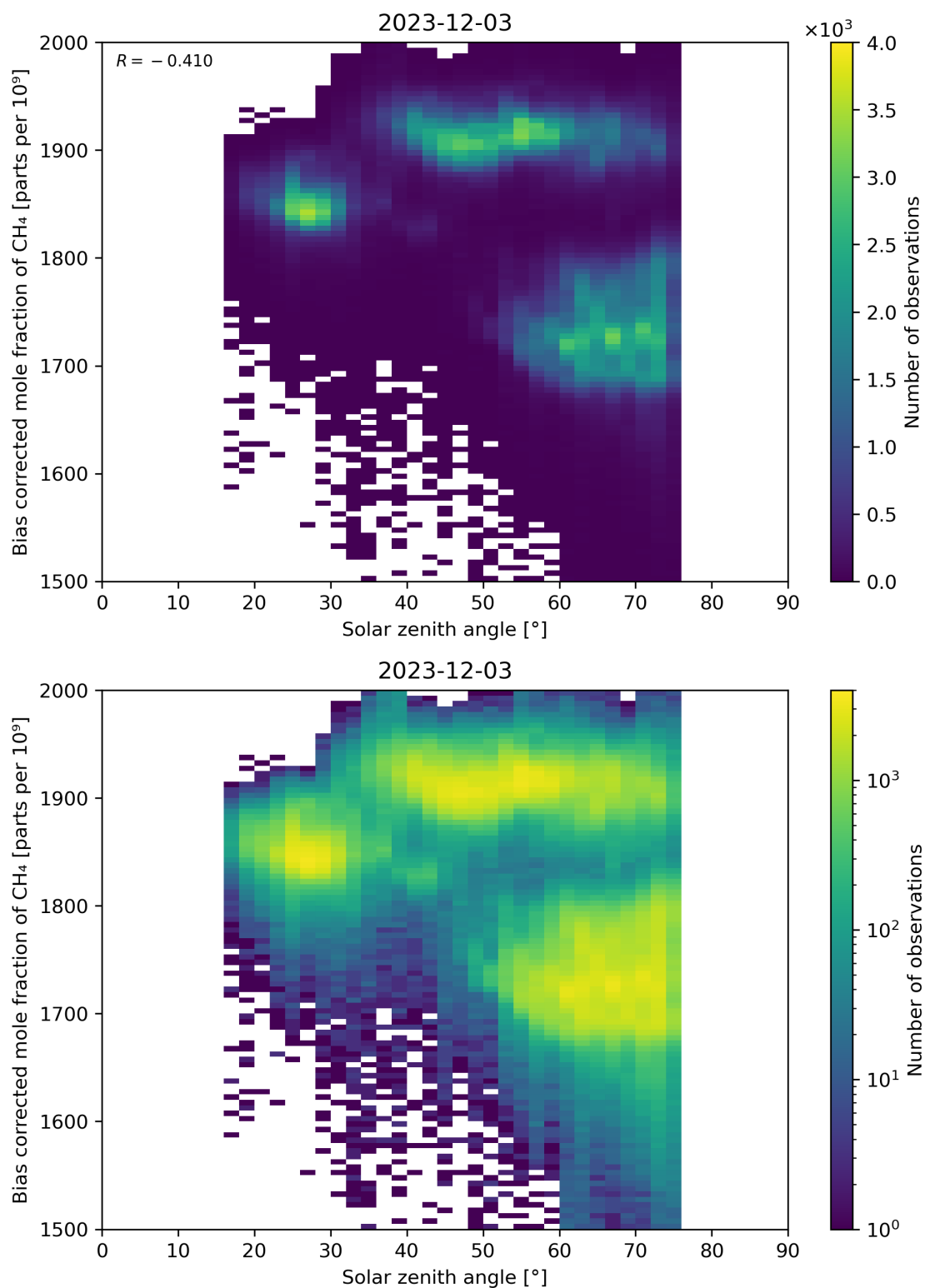
Figure 100: Scatter density plot of “Solar zenith angle” against “Bias corrected mole fraction of \text{CH}_4 ” for 2023-12-02 to 2023-12-04.
