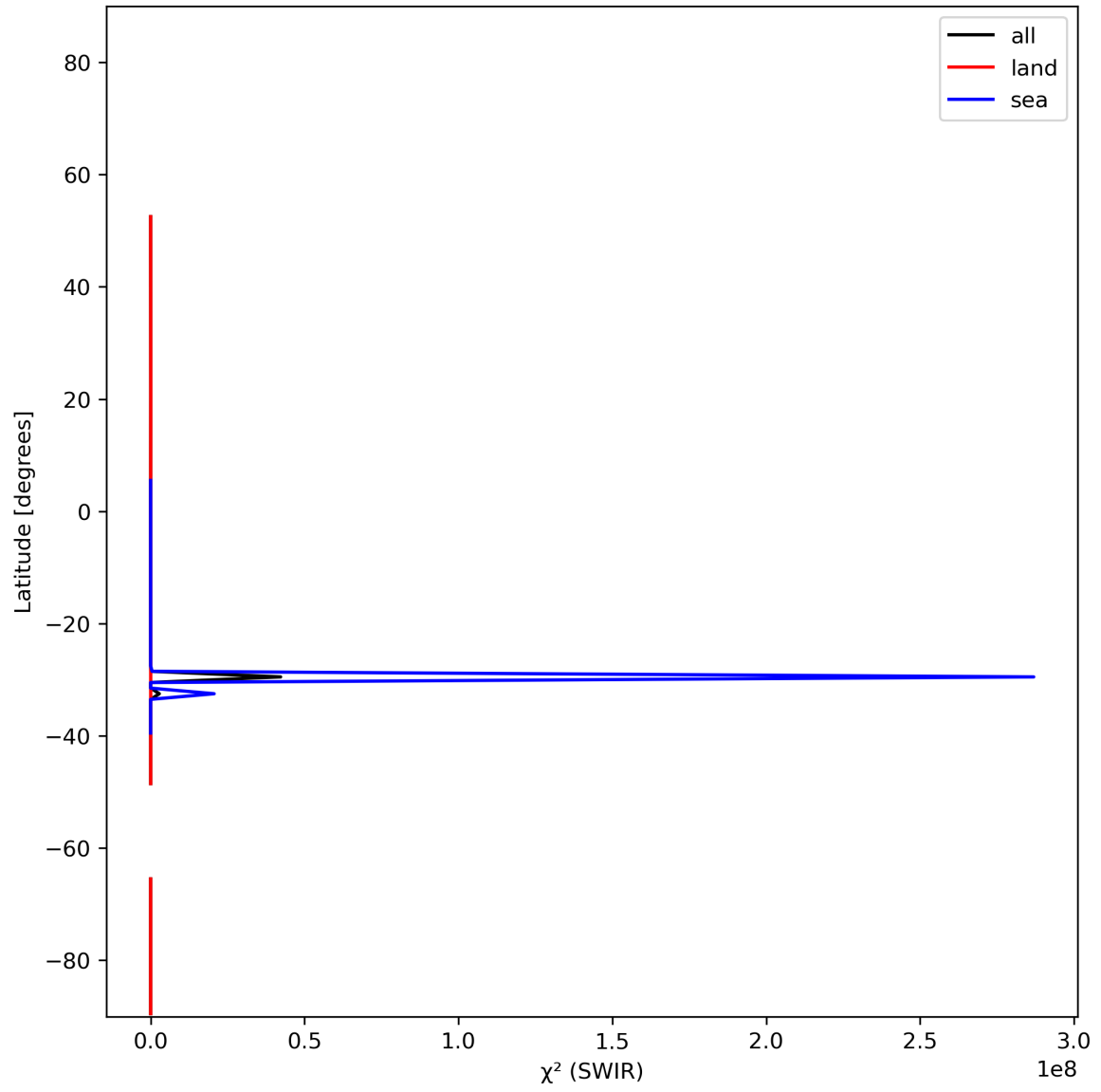
Figure 17: Zonal average of “ \chi^2 (SWIR)” for 2023-12-02 to 2023-12-04.
