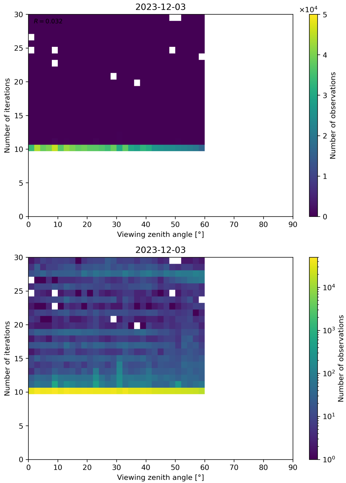
Figure 113: Scatter density plot of “Viewing zenith angle” against “Number of iterations” for 2023-12-02 to 2023-12-04.
