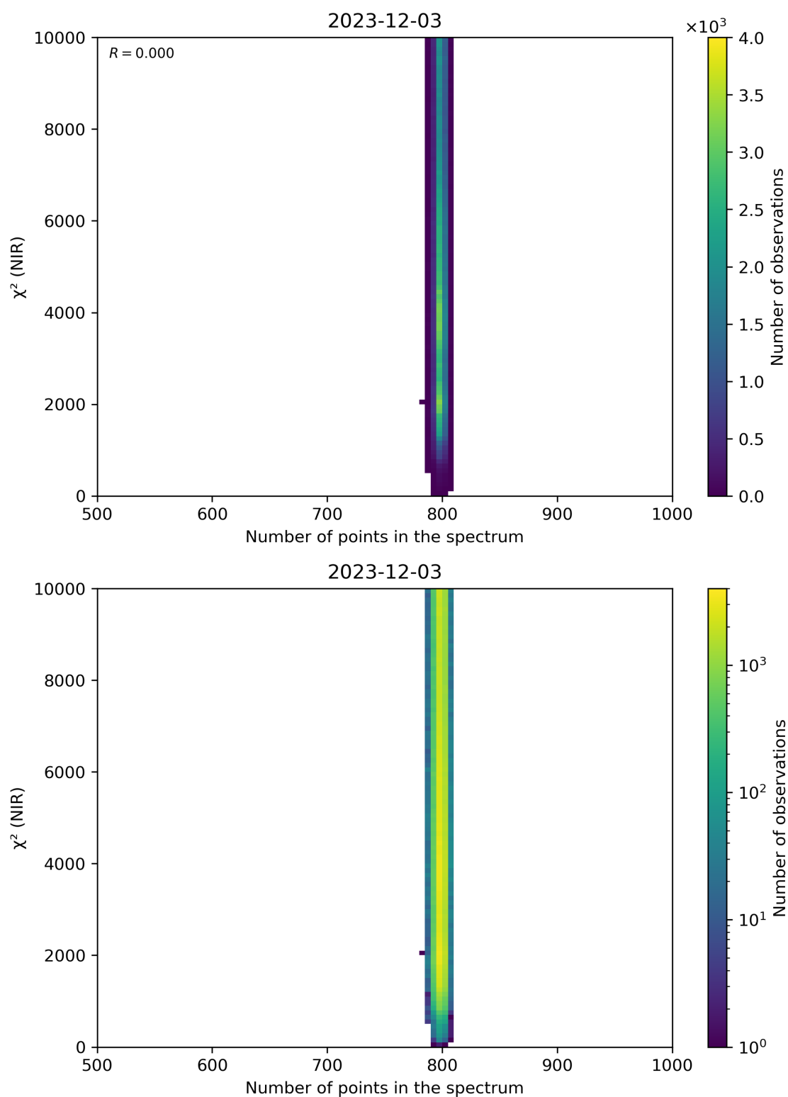
Figure 88: Scatter density plot of “Number of points in the spectrum” against “ \chi^2 (NIR)” for 2023-12-02 to 2023-12-04.
