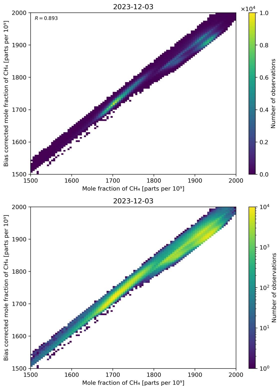
Figure 74: Scatter density plot of “Mole fraction of CH 4 ” against “Bias corrected mole fraction of CH 4 ” for 2023-12-02 to 2023-12-04.
