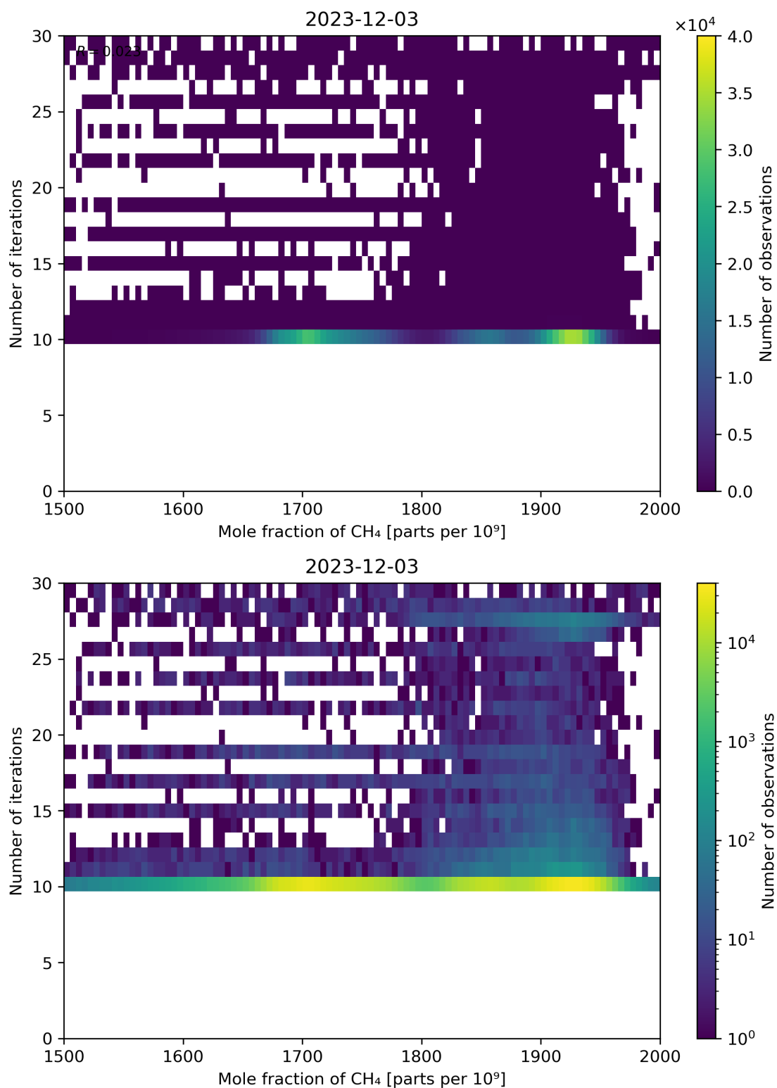
Figure 76: Scatter density plot of “Mole fraction of CH 4 ” against “Number of iterations” for 2023-12-02 to 2023-12-04.
