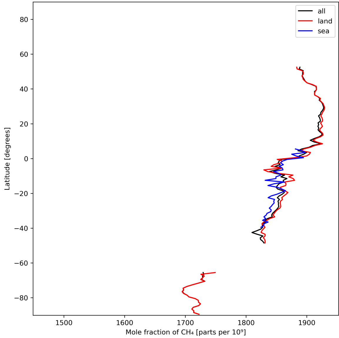
Figure 12: Zonal average of “Mole fraction of CH 4 ” for 2023-12-02 to 2023-12-04.
