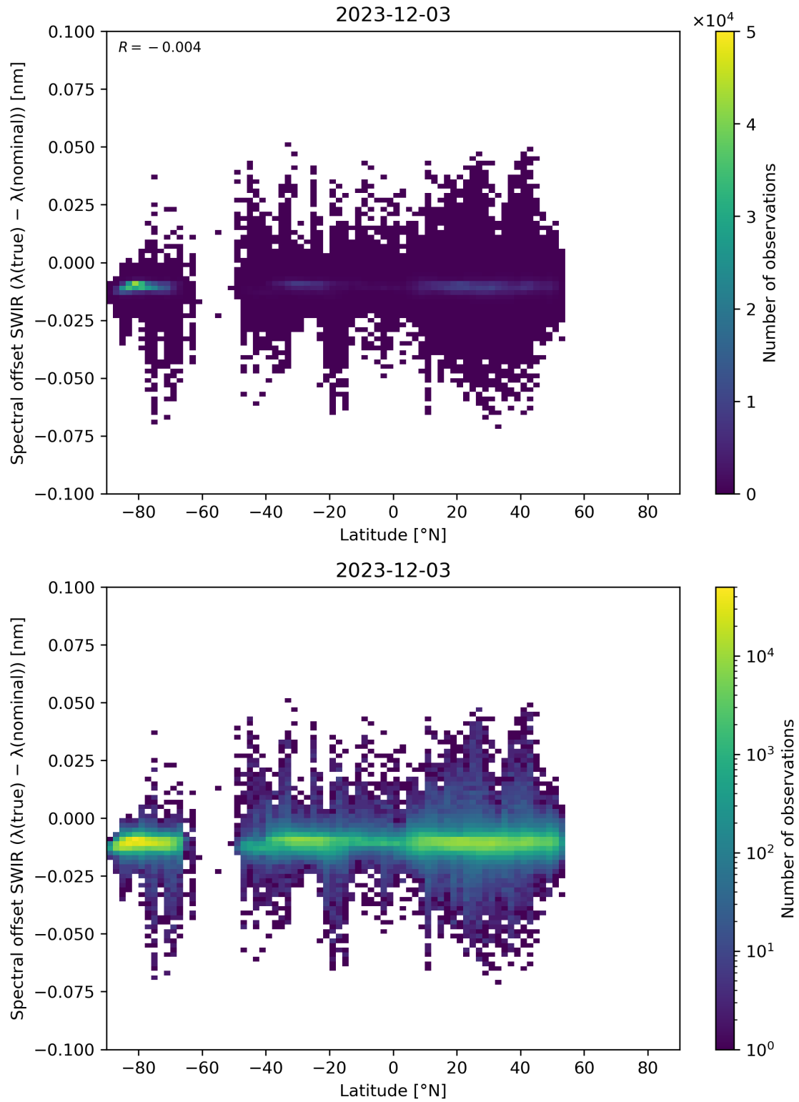
Figure 62: Scatter density plot of “Latitude” against “Spectral offset SWIR ( \lambda(\text{true}) - \lambda(\text{nominal}) )” for 2023-12-02 to 2023-12-04.
