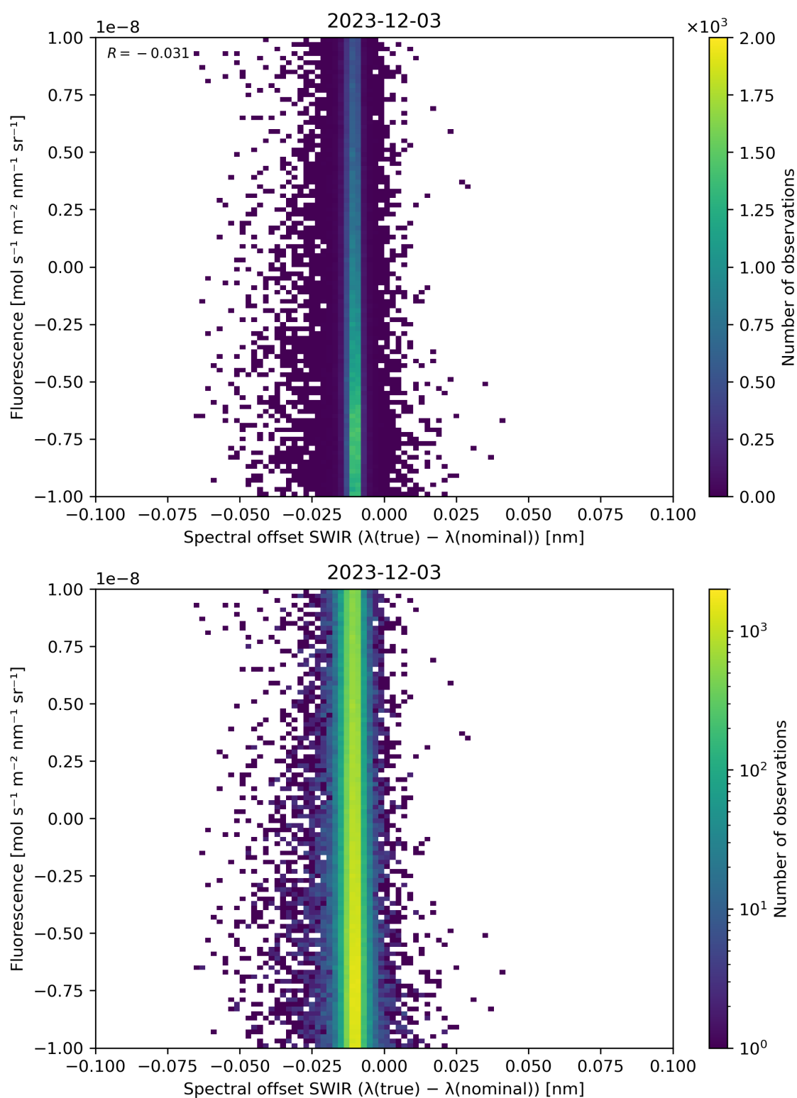
Figure 120: Scatter density plot of “Spectral offset SWIR ( \lambda(\text{true}) - \lambda(\text{nominal}) )” against “Fluorescence” for 2023-12-02 to 2023-12-04.
