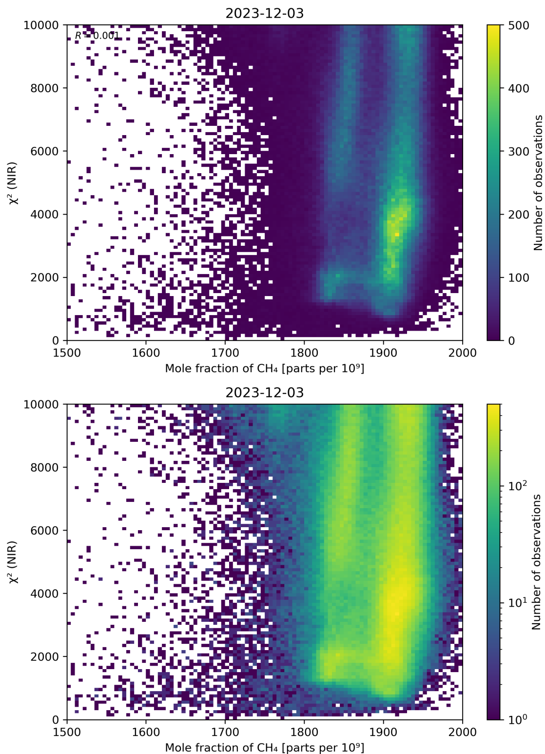
Figure 70: Scatter density plot of “Mole fraction of \text{CH}_4 ” against “ \chi^2 (NIR)” for 2023-12-02 to 2023-12-04.
