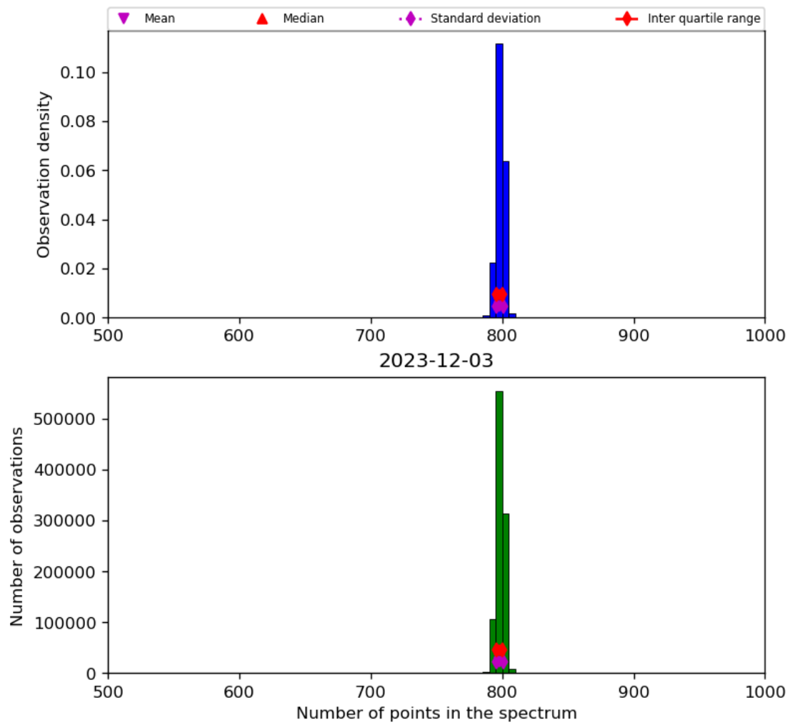
Figure 26: Histogram of “Number of points in the spectrum” for 2023-12-02 to 2023-12-04
