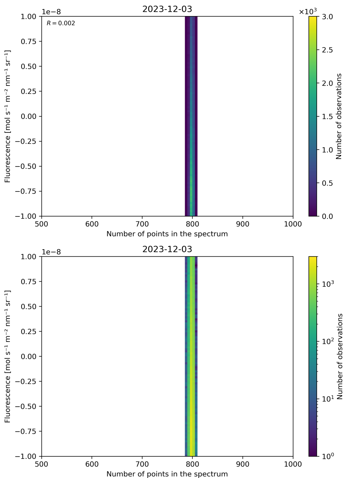
Figure 91: Scatter density plot of “Number of points in the spectrum” against “Fluorescence” for 2023-12-02 to 2023-12-04.
