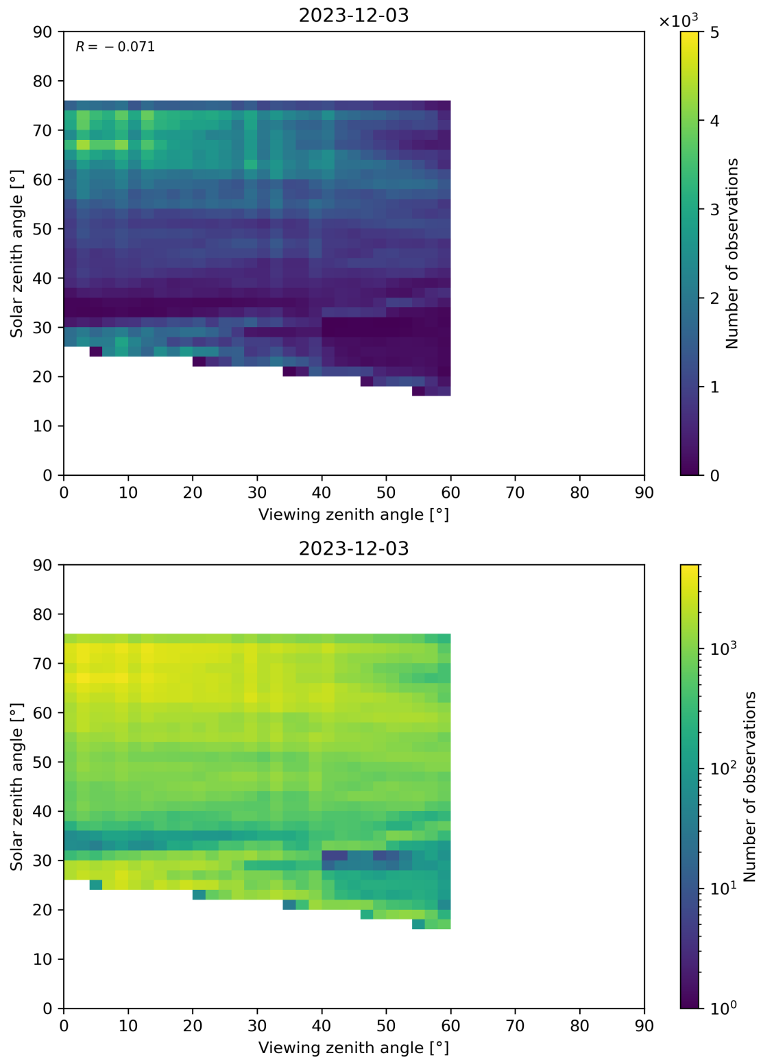
Figure 115: Scatter density plot of “Viewing zenith angle” against “Solar zenith angle” for 2023-12-02 to 2023-12-04.
