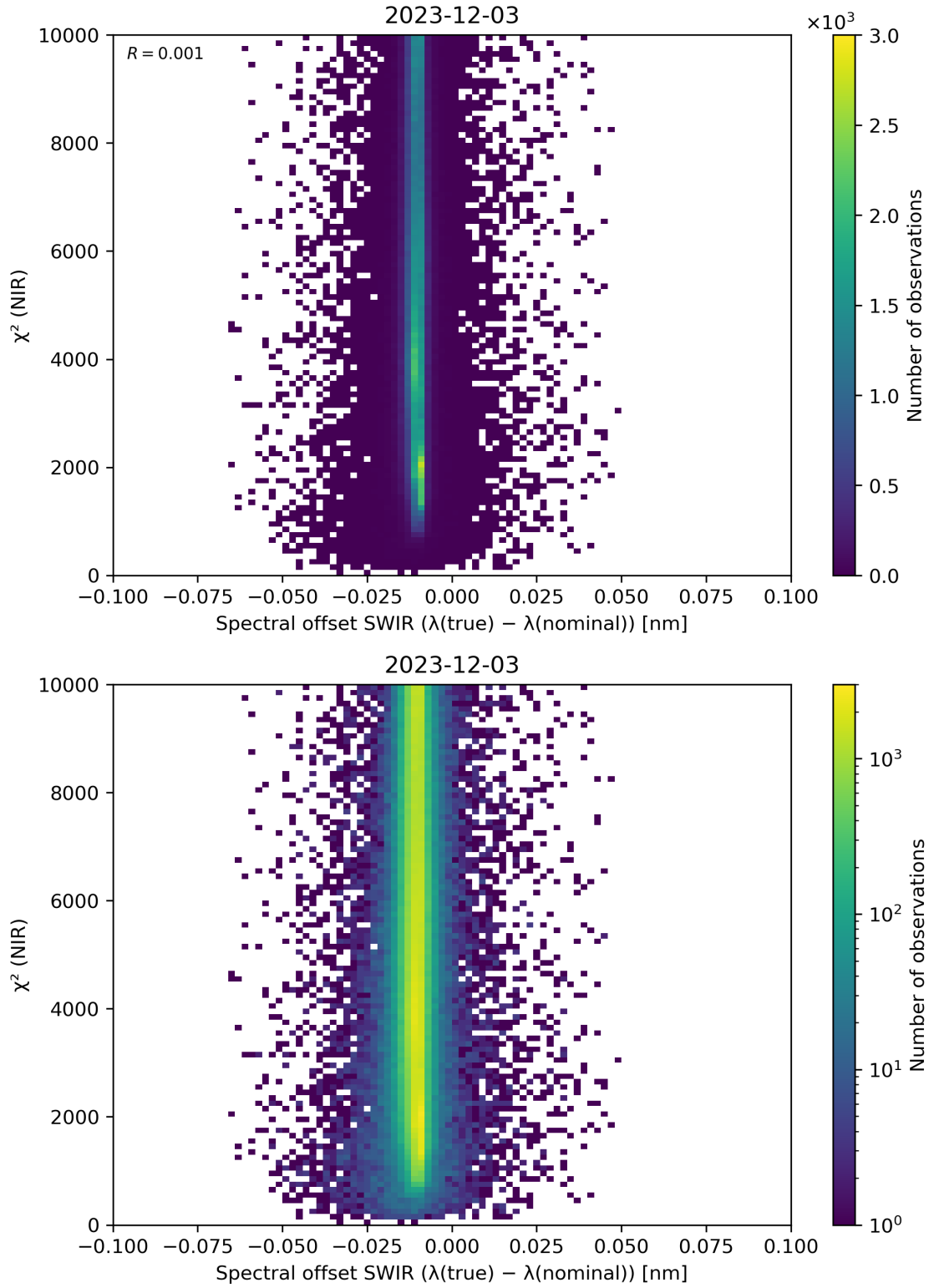
Figure 117: Scatter density plot of “Spectral offset SWIR ( \lambda(\text{true}) - \lambda(\text{nominal}) )” against “ \chi^2 (NIR)” for 2023-12-02 to 2023-12-04.
