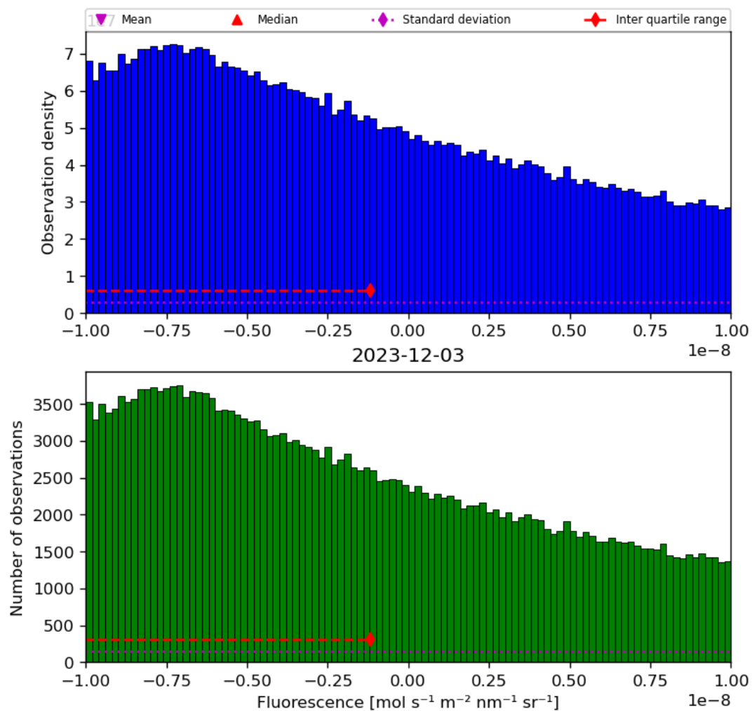
Figure 32: Histogram of “Fluorescence” for 2023-12-02 to 2023-12-04
