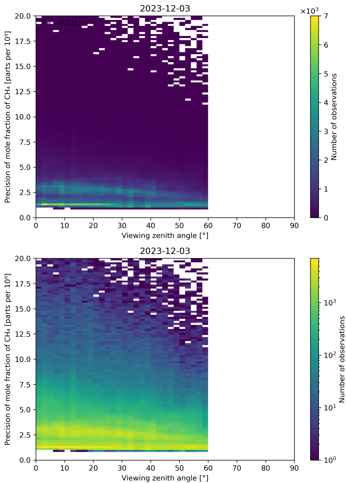
Figure 112: Scatter density plot of “Viewing zenith angle” against “Precision of mole fraction of CH 4 ” for 2023-12-02 to 2023-12-04.
