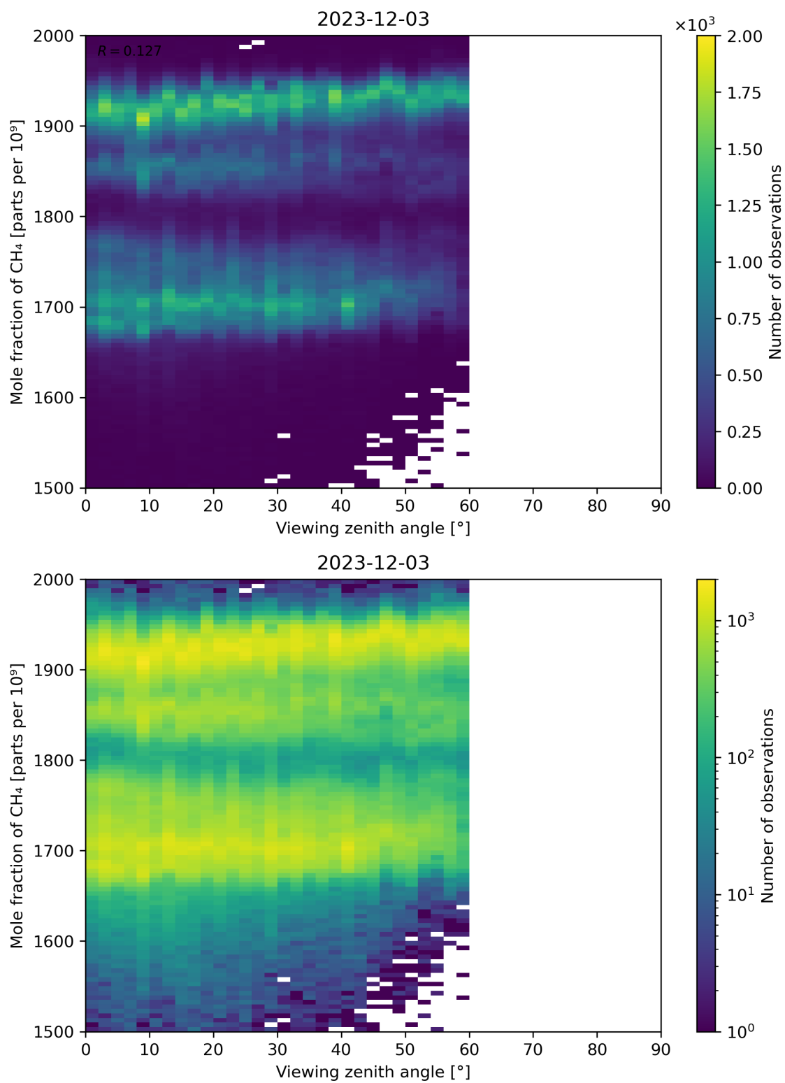
Figure 110: Scatter density plot of “Viewing zenith angle” against “Mole fraction of CH 4 ” for 2023-12-02 to 2023-12-04.
