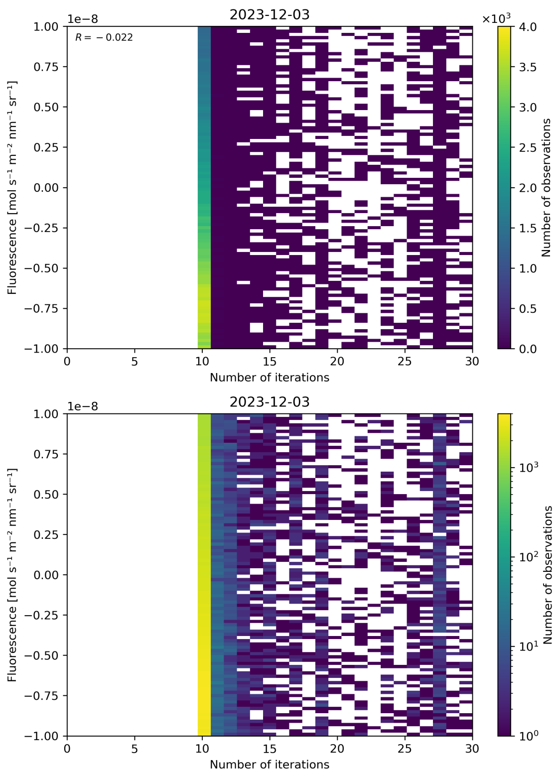
Figure 87: Scatter density plot of “Number of iterations” against “Fluorescence” for 2023-12-02 to 2023-12-04.
