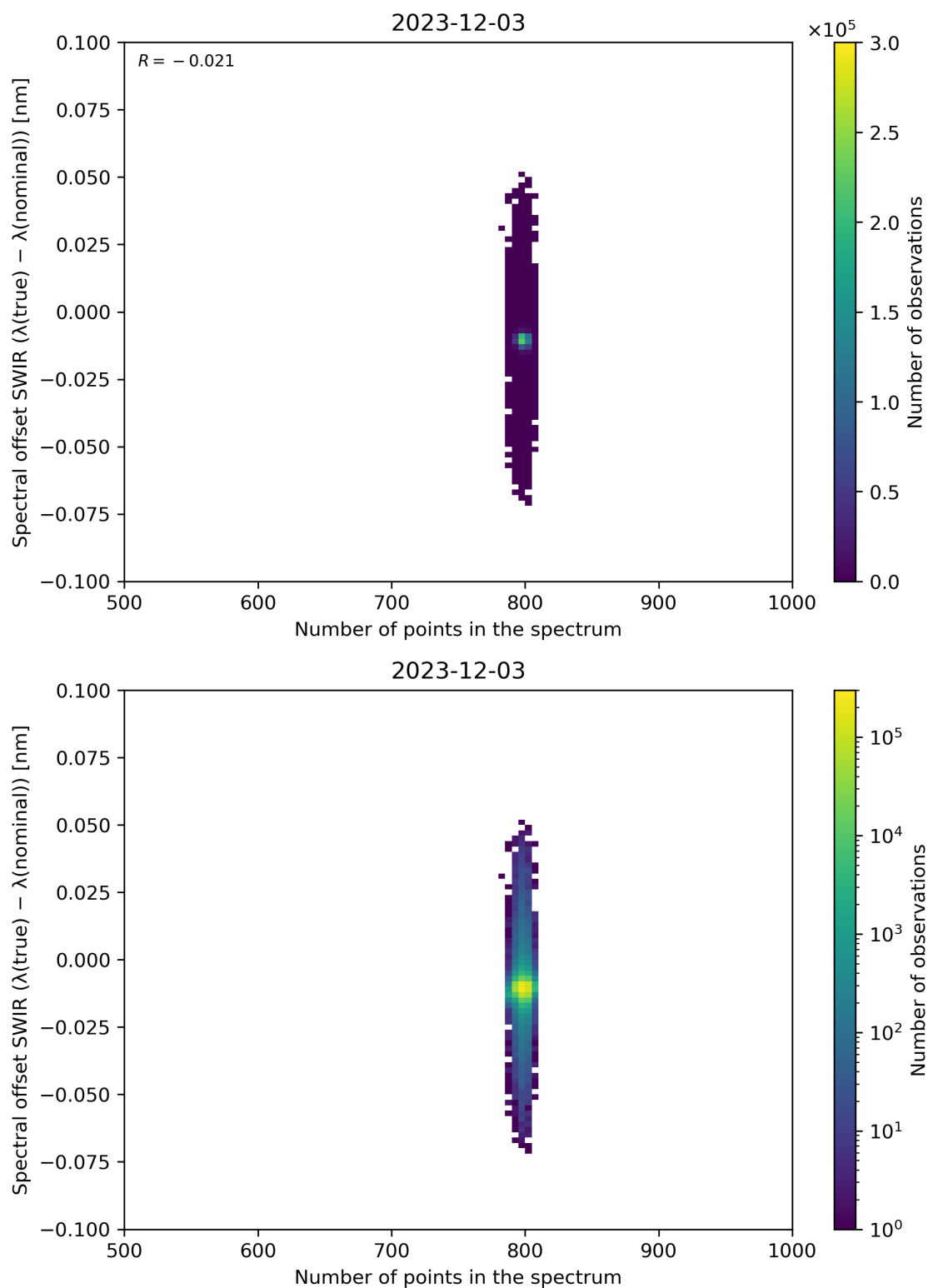
Figure 93: Scatter density plot of “Number of points in the spectrum” against “Spectral offset SWIR ( \lambda(\text{true}) - \lambda(\text{nominal}) )” for 2023-12-02 to 2023-12-04.
