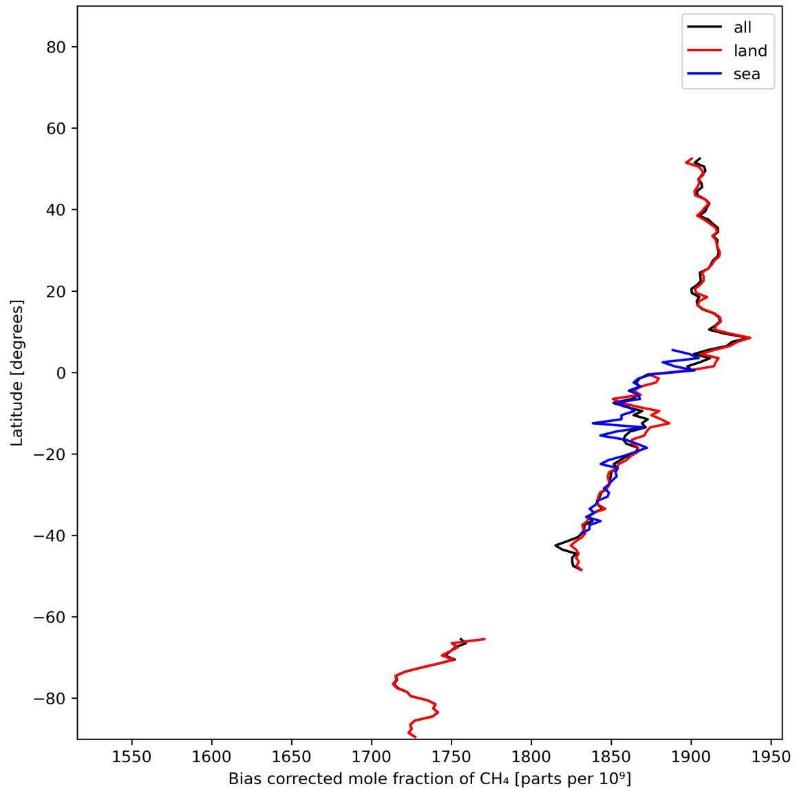
Figure 14: Zonal average of “Bias corrected mole fraction of CH 4 ” for 2023-12-02 to 2023-12-04.
