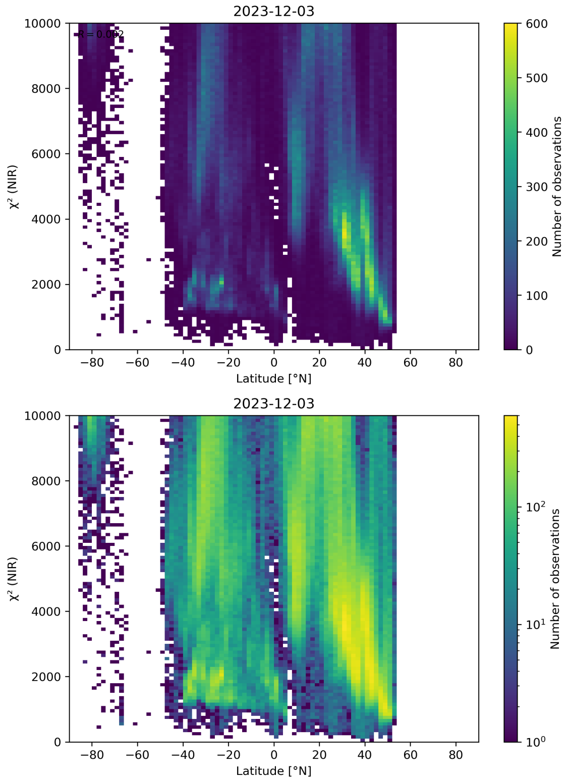
Figure 53: Scatter density plot of “Latitude” against “ \chi^2 (NIR)” for 2023-12-02 to 2023-12-04.
