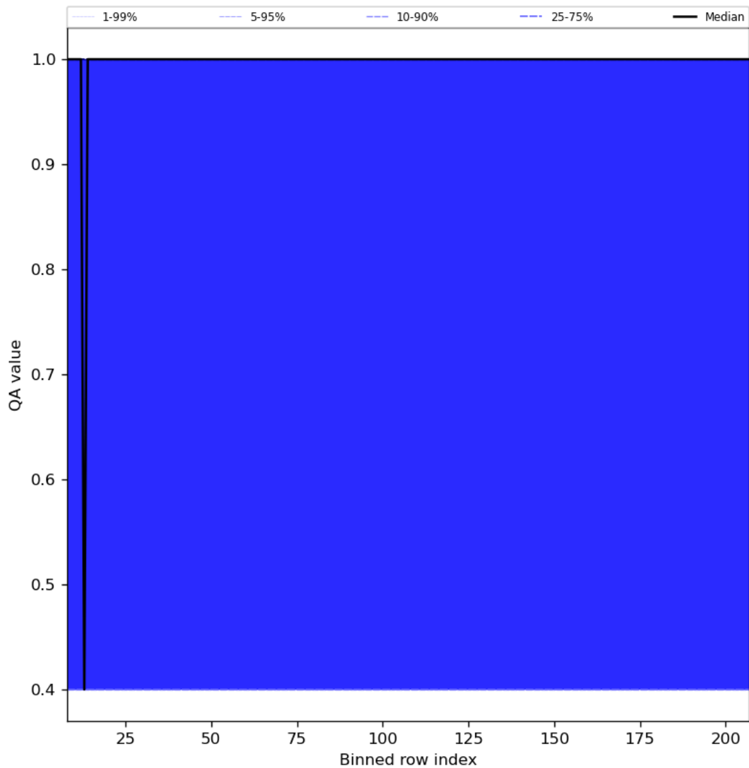
Figure 33: Along track statistics of “QA value” for 2023-12-02 to 2023-12-04
