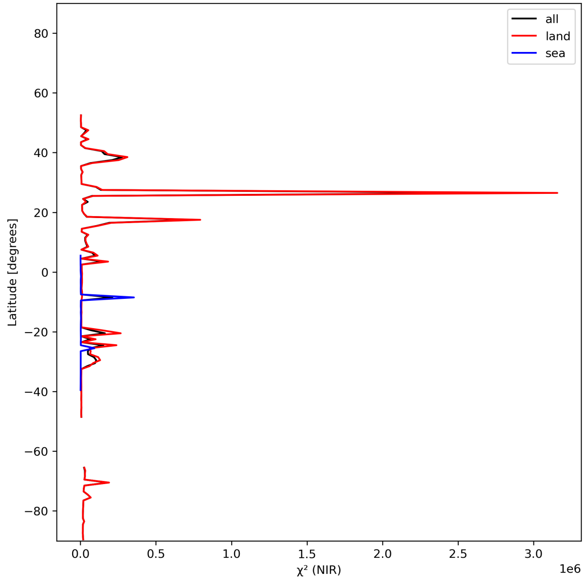
Figure 18: Zonal average of “ \chi^2 (NIR)” for 2023-12-02 to 2023-12-04.
