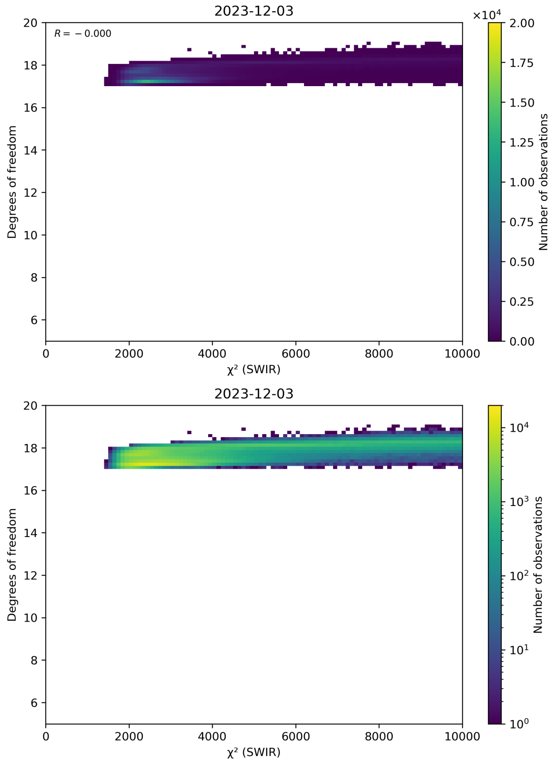
Figure 48: Scatter density plot of “ \chi^2 (SWIR)” against “Degrees of freedom” for 2023-12-02 to 2023-12-04.
