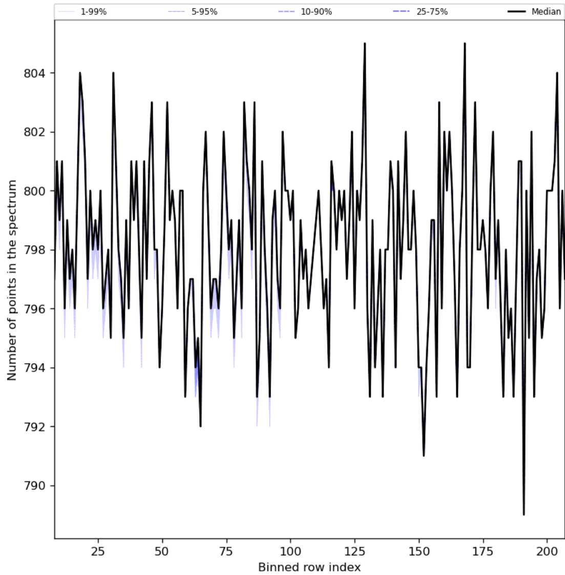
Figure 37: Along track statistics of “Number of points in the spectrum” for 2023-12-02 to 2023-12-04
