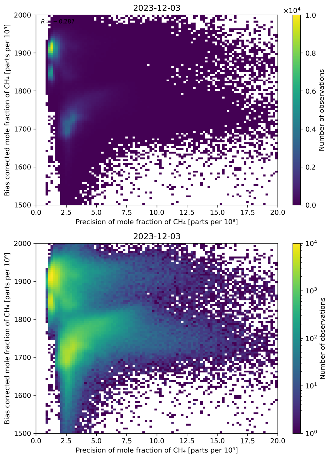
Figure 82: Scatter density plot of “Precision of mole fraction of CH 4 ” against “Bias corrected mole fraction of CH 4 ” for 2023-12-02 to 2023-12-04.
