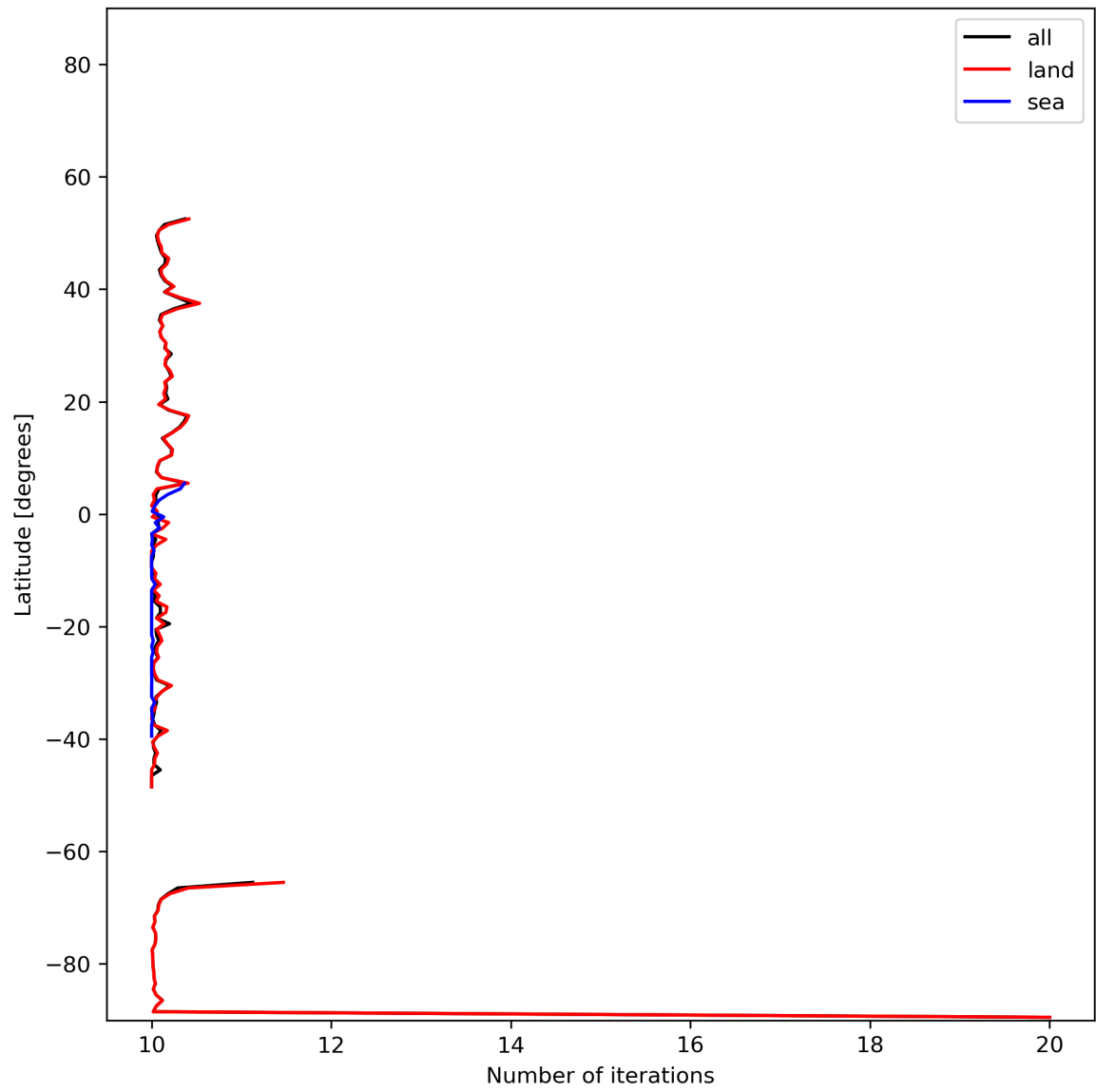
Figure 20: Zonal average of “Number of iterations” for 2023-12-02 to 2023-12-04.
