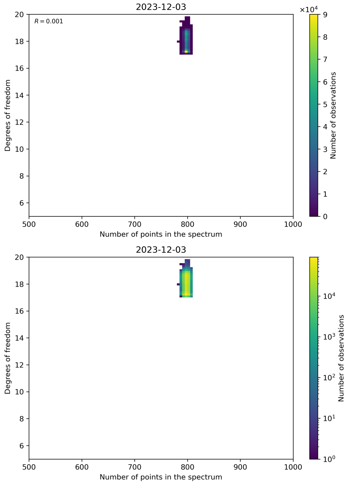
Figure 90: Scatter density plot of “Number of points in the spectrum” against “Degrees of freedom” for 2023-12-02 to 2023-12-04.
