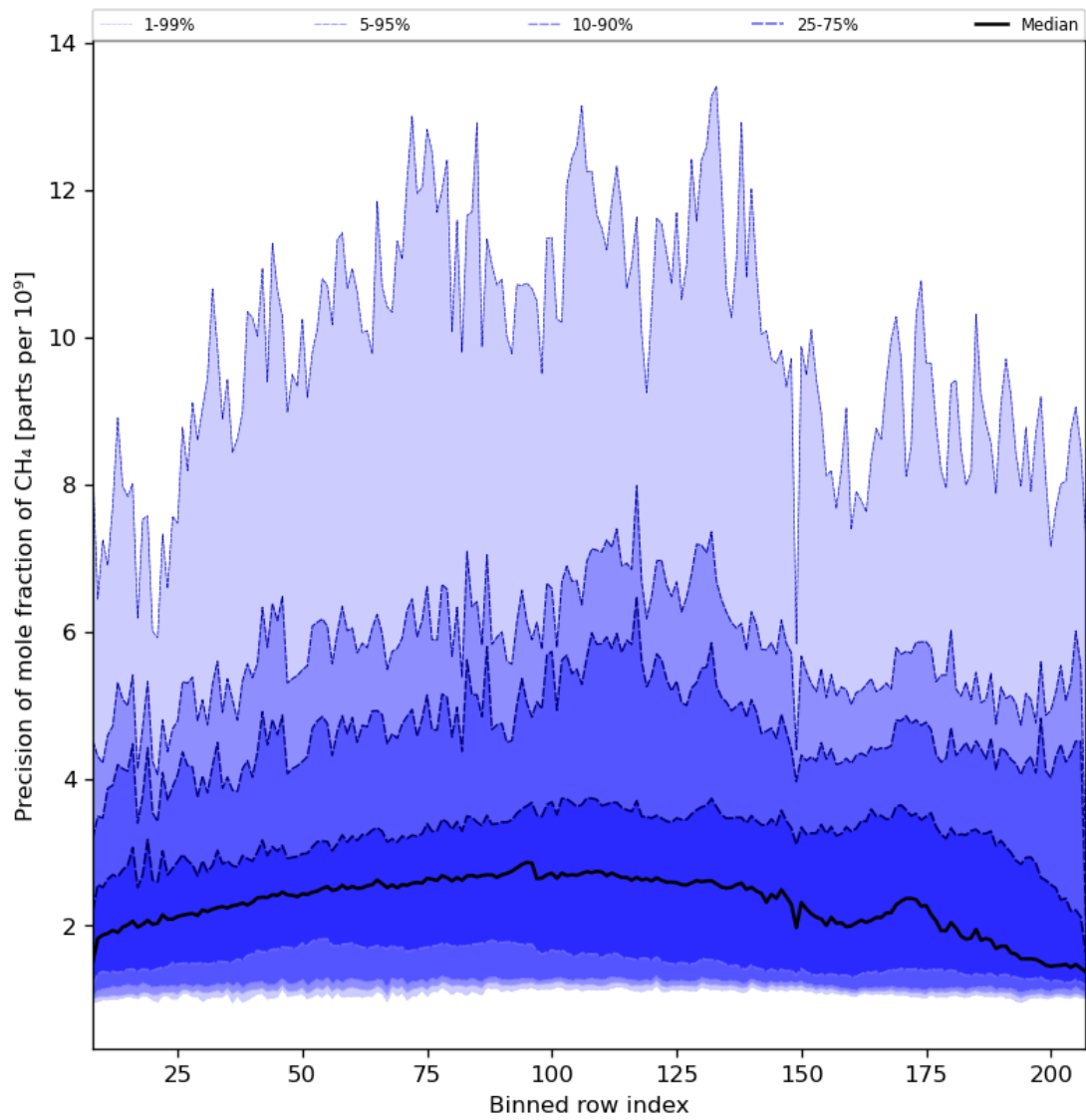
Figure 35: Along track statistics of “Precision of mole fraction of CH 4 ” for 2023-12-02 to 2023-12-04
