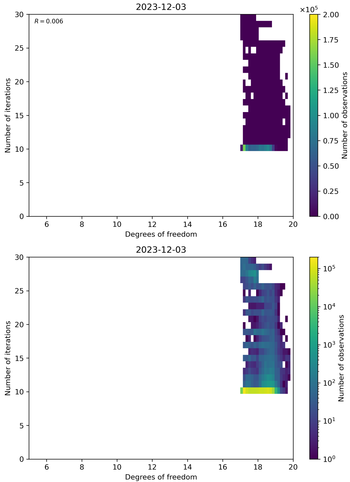
Figure 52: Scatter density plot of “Degrees of freedom” against “Number of iterations” for 2023-12-02 to 2023-12-04.
