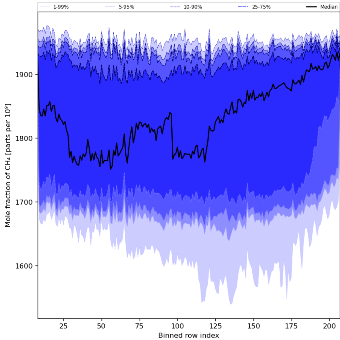
Figure 34: Along track statistics of “Mole fraction of CH 4 ” for 2023-12-02 to 2023-12-04
