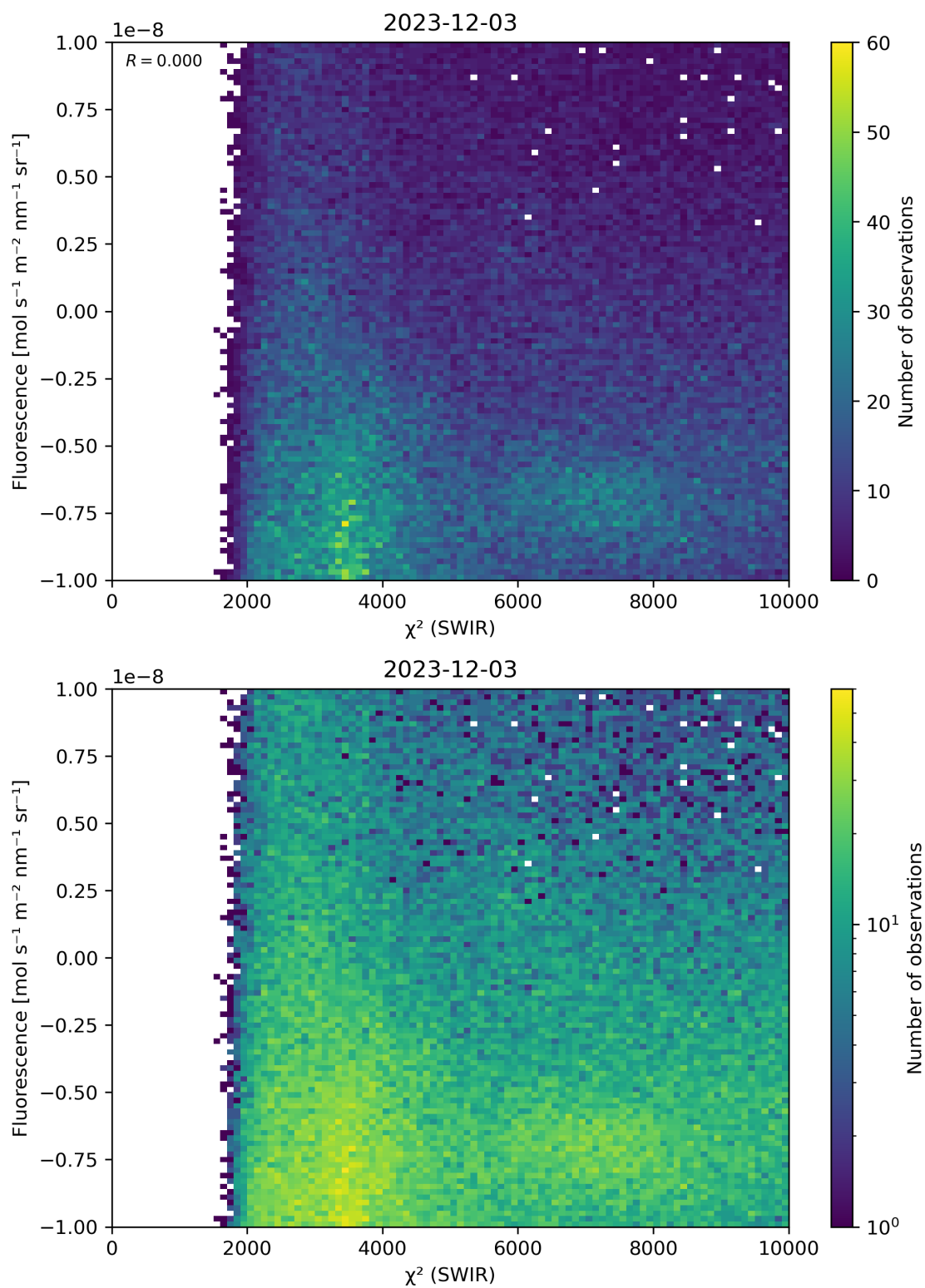
Figure 49: Scatter density plot of “ \chi^2 (SWIR)” against “Fluorescence” for 2023-12-02 to 2023-12-04.
