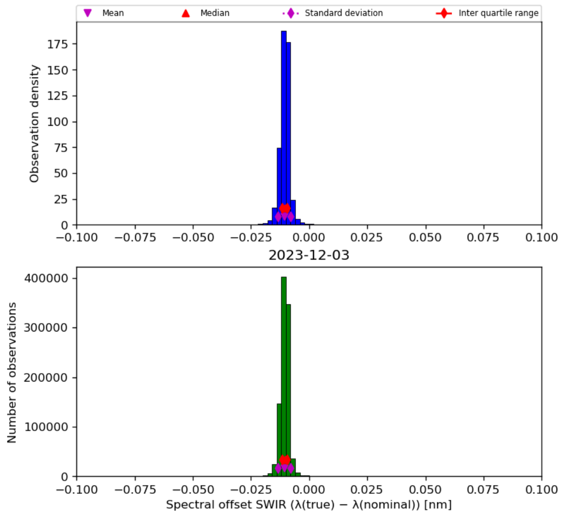
Figure 27: Histogram of “Spectral offset SWIR ( \lambda(\text{true}) - \lambda(\text{nominal}) )” for 2023-12-02 to 2023-12-04
