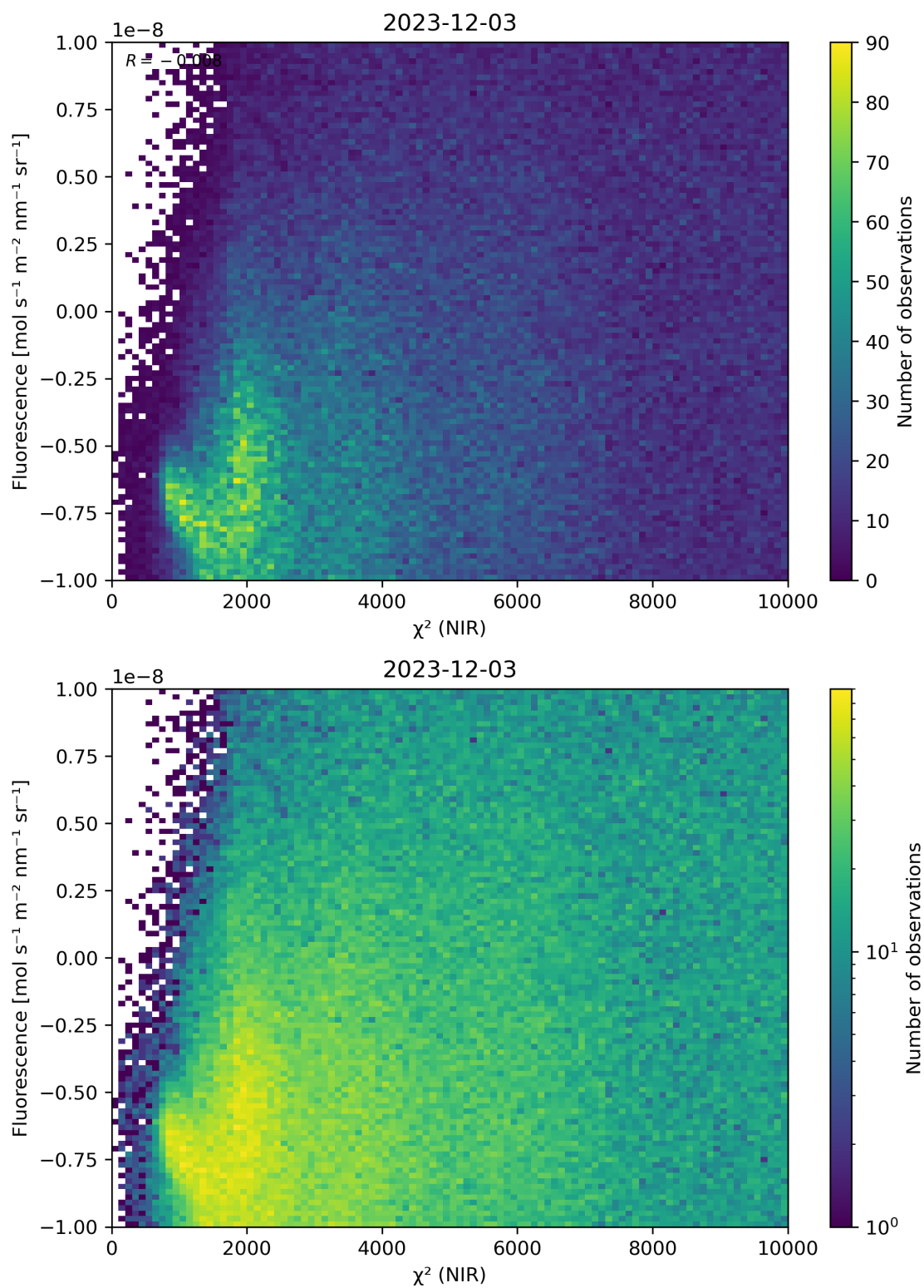
Figure 45: Scatter density plot of “ \chi^2 (NIR)” against “Fluorescence” for 2023-12-02 to 2023-12-04.
