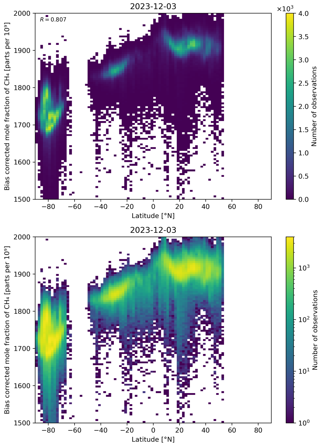
Figure 58: Scatter density plot of “Latitude” against “Bias corrected mole fraction of CH 4 ” for 2023-12-02 to 2023-12-04.
