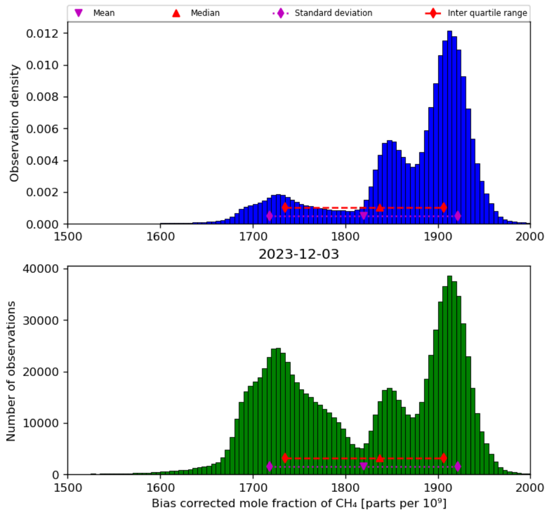
Figure 25: Histogram of “Bias corrected mole fraction of CH 4 ” for 2023-12-02 to 2023-12-04
