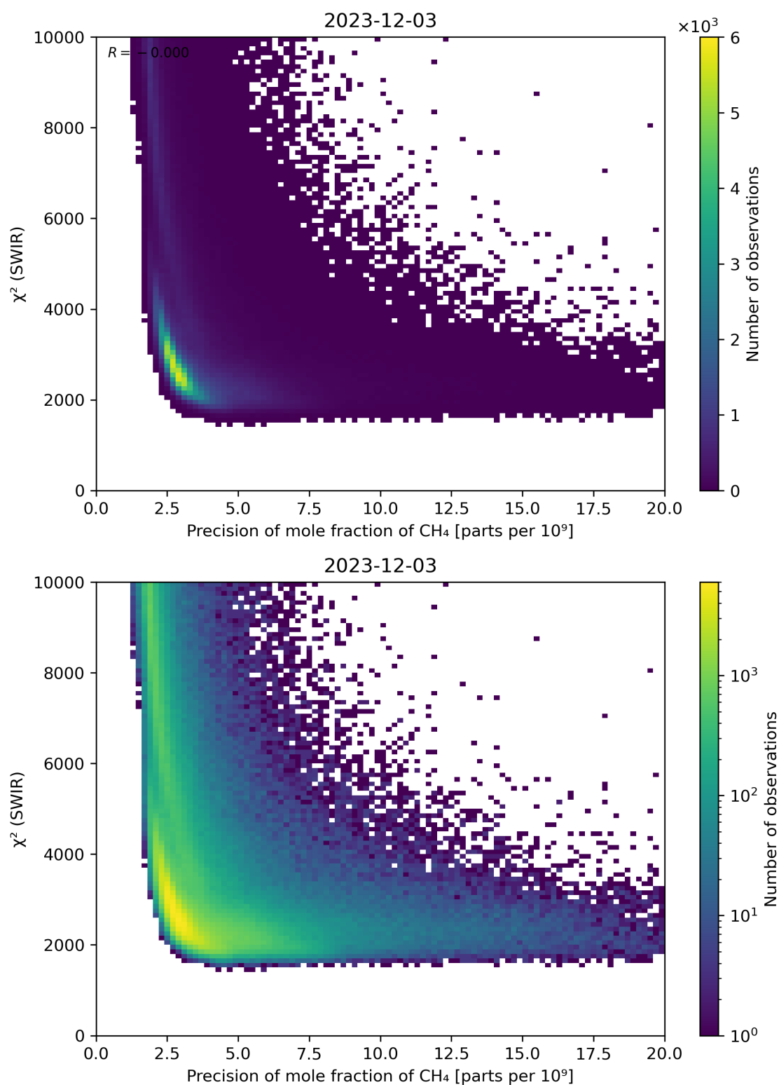
Figure 79: Scatter density plot of “Precision of mole fraction of \text{CH}_4 ” against “ \chi^2 (SWIR)” for 2023-12-02 to 2023-12-04.
