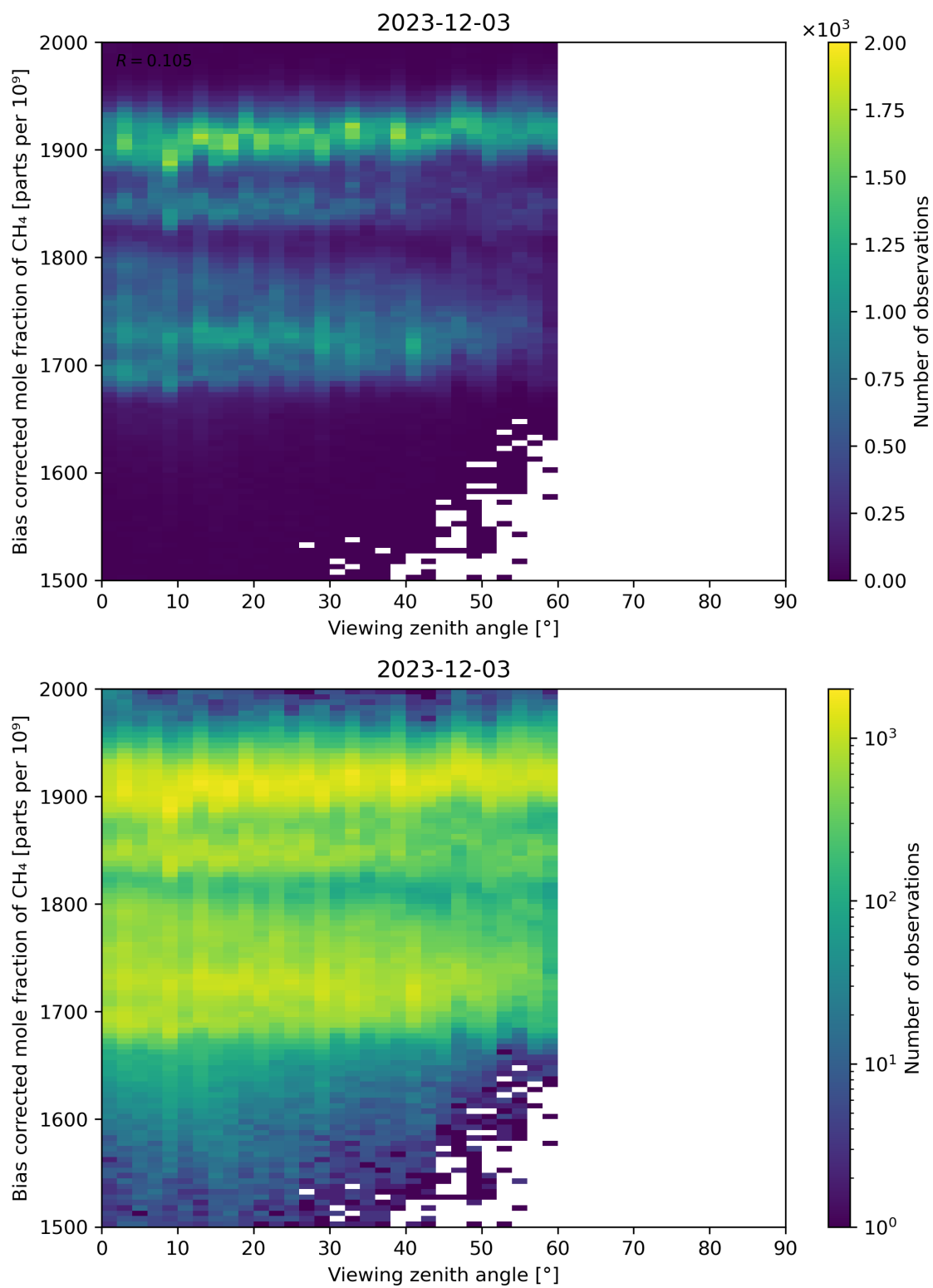
Figure 111: Scatter density plot of “Viewing zenith angle” against “Bias corrected mole fraction of CH 4 ” for 2023-12-02 to 2023-12-04.
