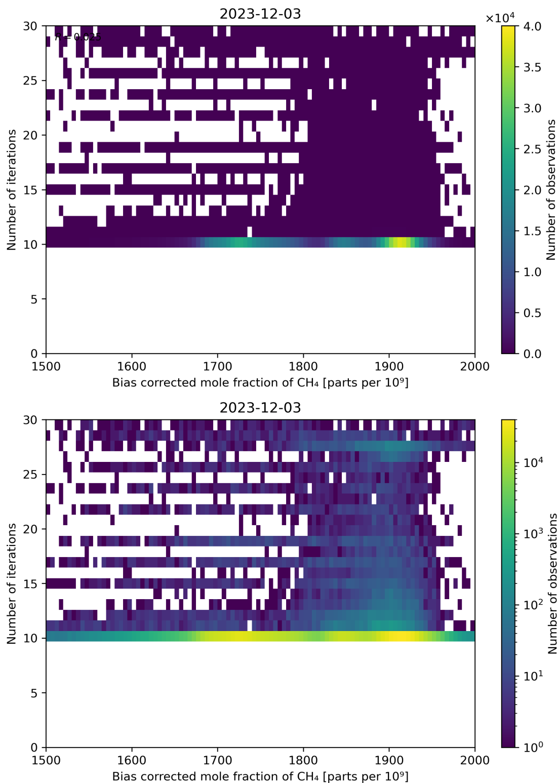
Figure 67: Scatter density plot of “Bias corrected mole fraction of \text{CH}_4 ” against “Number of iterations” for 2023-12-02 to 2023-12-04.
