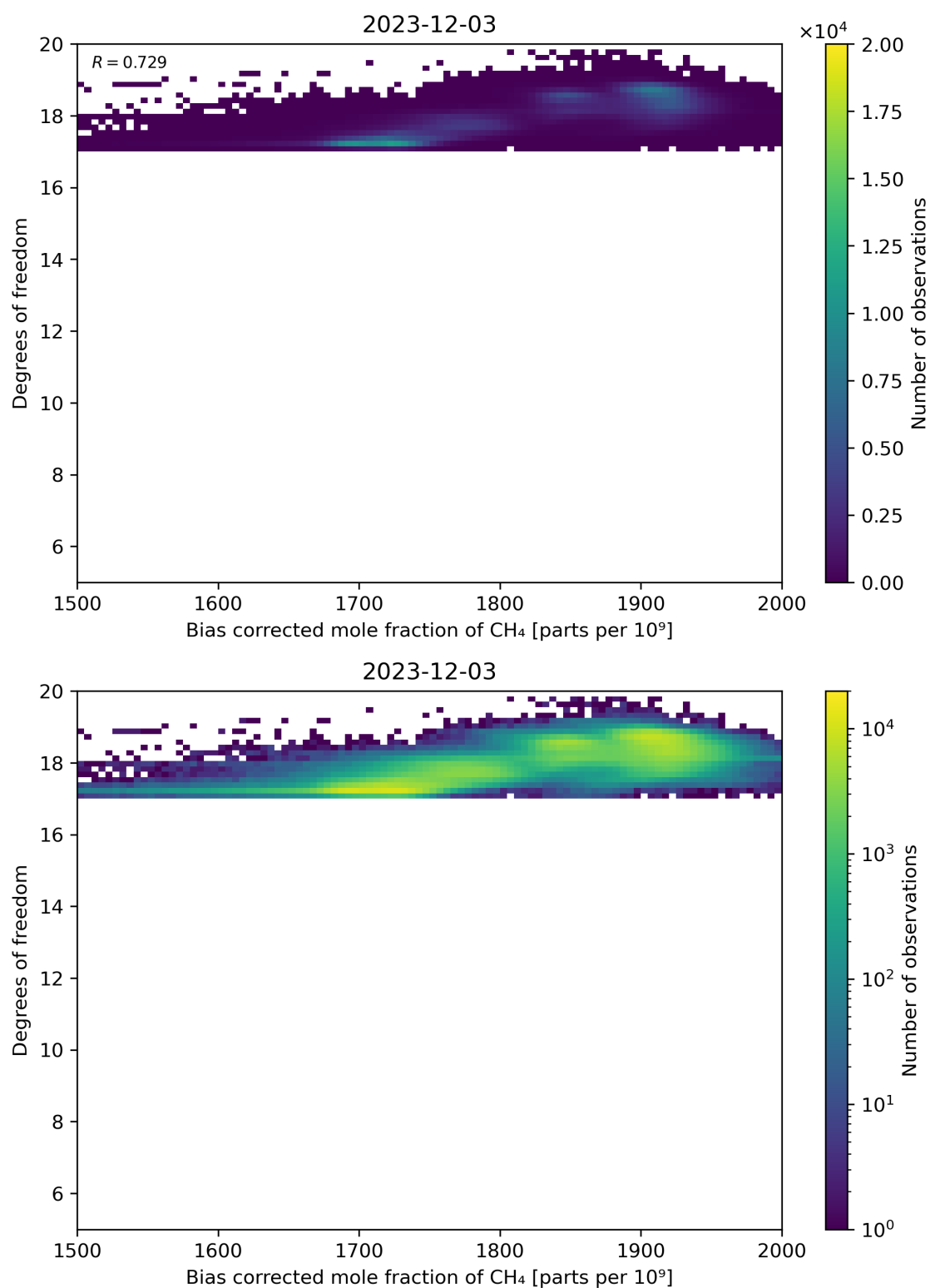
Figure 65: Scatter density plot of “Bias corrected mole fraction of CH 4 ” against “Degrees of freedom” for 2023-12-02 to 2023-12-04.
