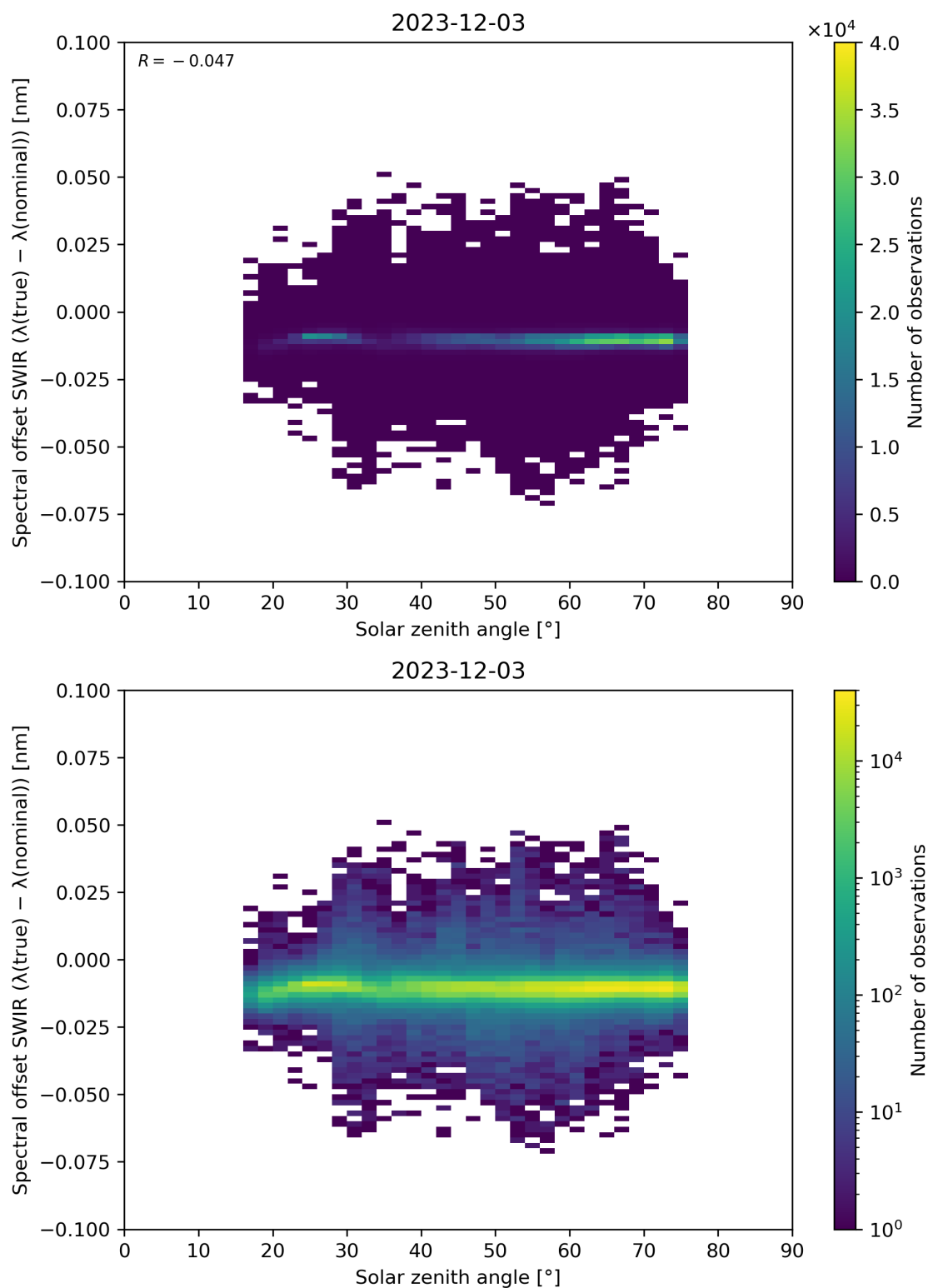
Figure 104: Scatter density plot of “Solar zenith angle” against “Spectral offset SWIR ( \lambda(\text{true}) - \lambda(\text{nominal}) )” for 2023-12-02 to 2023-12-04.
