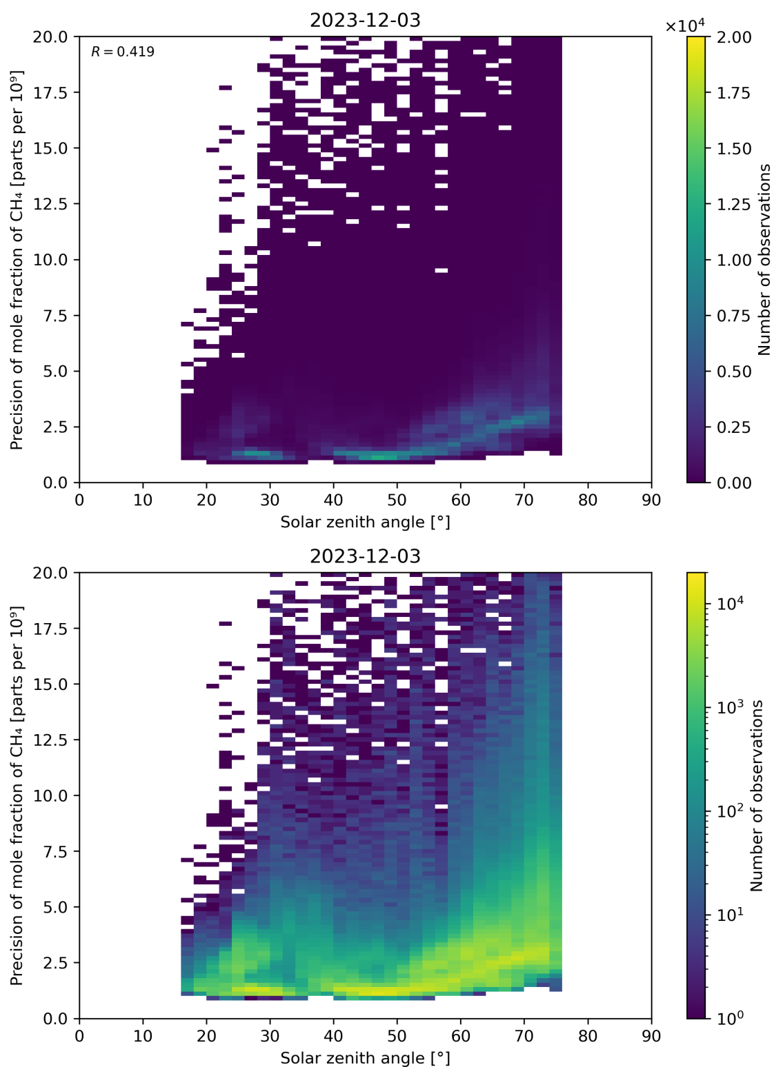
Figure 101: Scatter density plot of “Solar zenith angle” against “Precision of mole fraction of \text{CH}_4 ” for 2023-12-02 to 2023-12-04.
