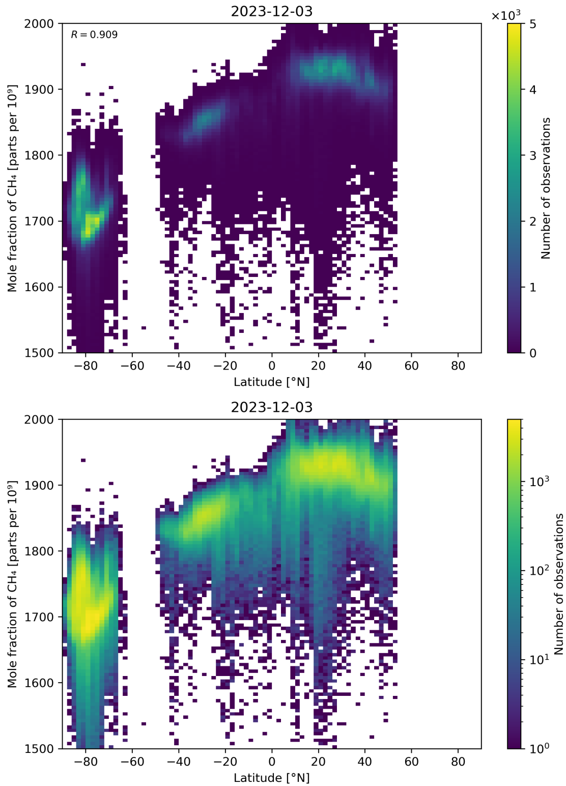
Figure 57: Scatter density plot of “Latitude” against “Mole fraction of CH 4 ” for 2023-12-02 to 2023-12-04.
