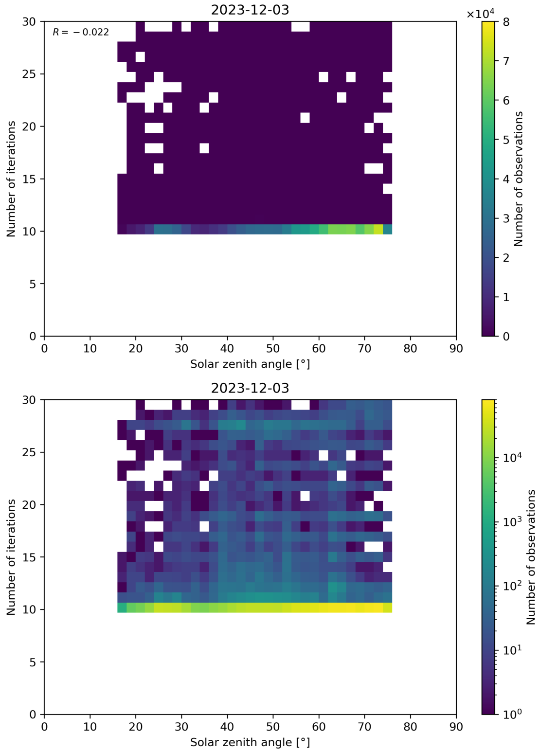
Figure 102: Scatter density plot of “Solar zenith angle” against “Number of iterations” for 2023-12-02 to 2023-12-04.
