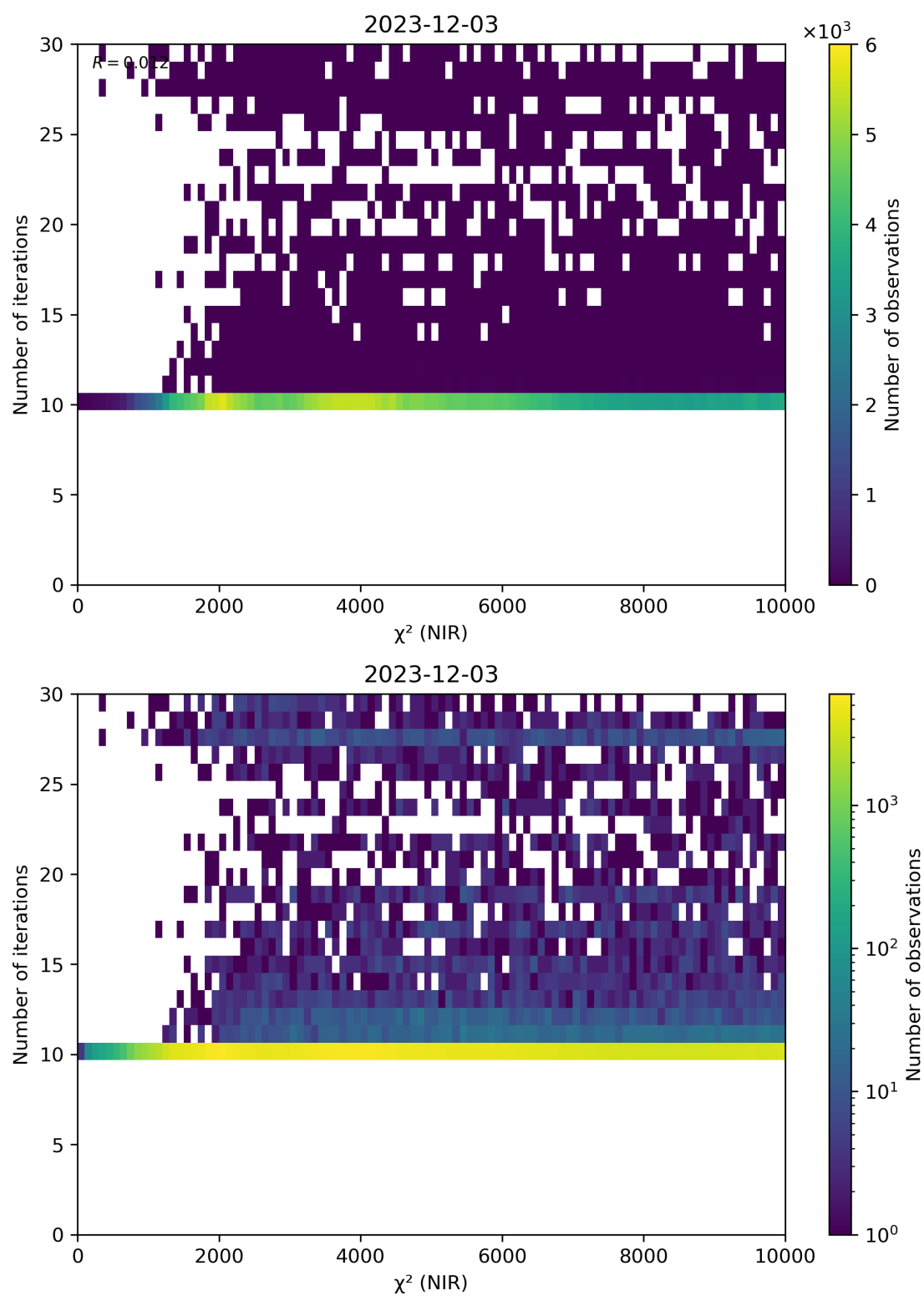
Figure 46: Scatter density plot of “ \chi^2 (NIR)” against “Number of iterations” for 2023-12-02 to 2023-12-04.
