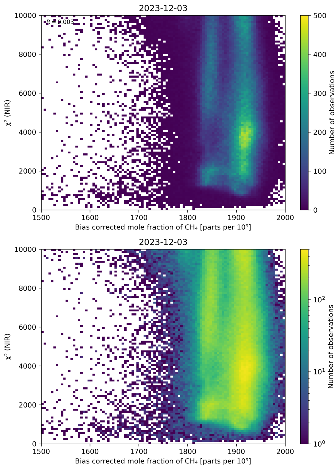
Figure 63: Scatter density plot of “Bias corrected mole fraction of CH 4 ” against “ \chi^2 (NIR)” for 2023-12-02 to 2023-12-04.
