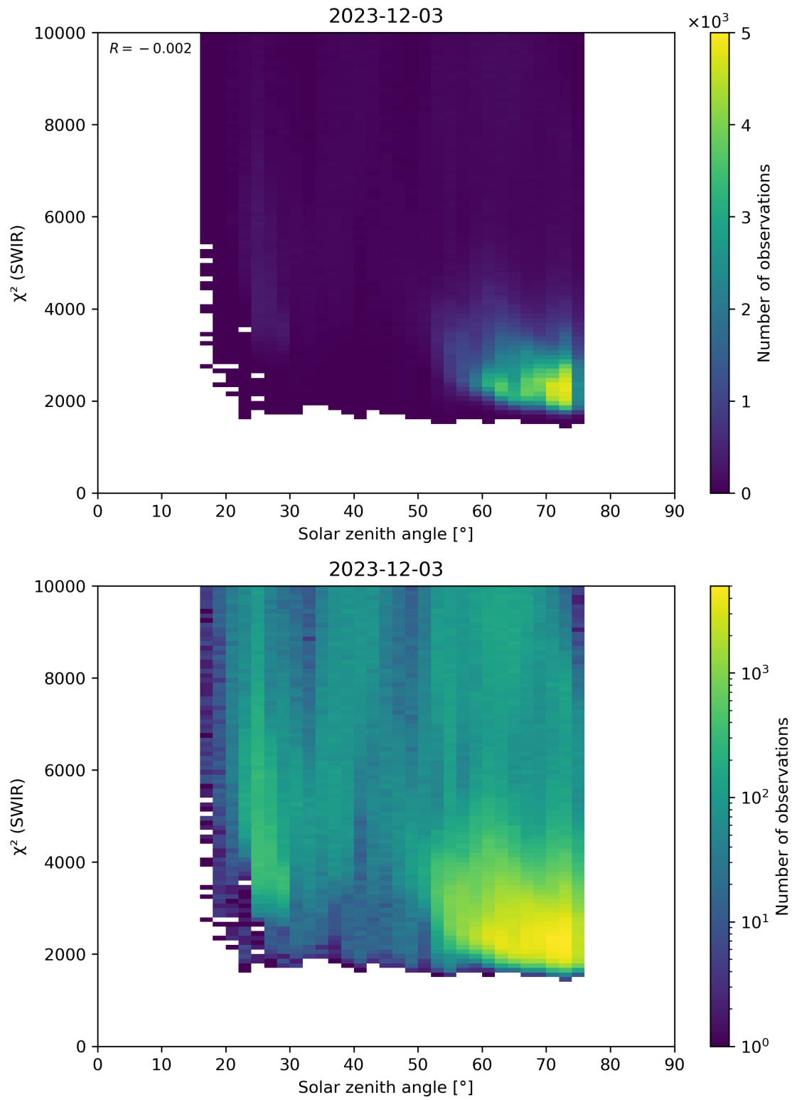
Figure 95: Scatter density plot of “Solar zenith angle” against “ \chi^2 (SWIR)” for 2023-12-02 to 2023-12-04.
