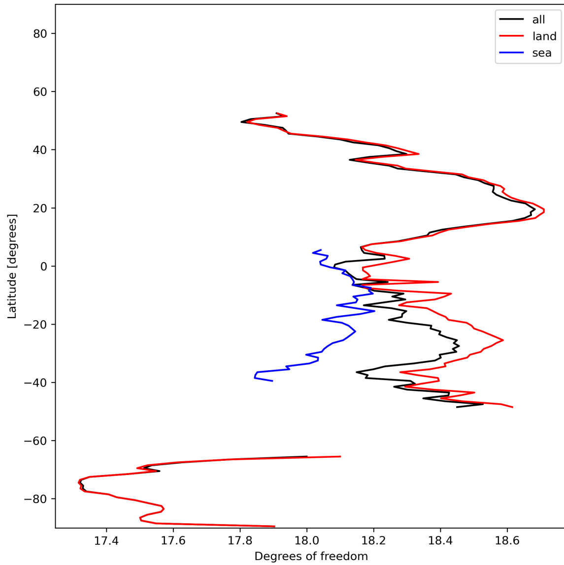
Figure 19: Zonal average of “Degrees of freedom” for 2023-12-02 to 2023-12-04.
