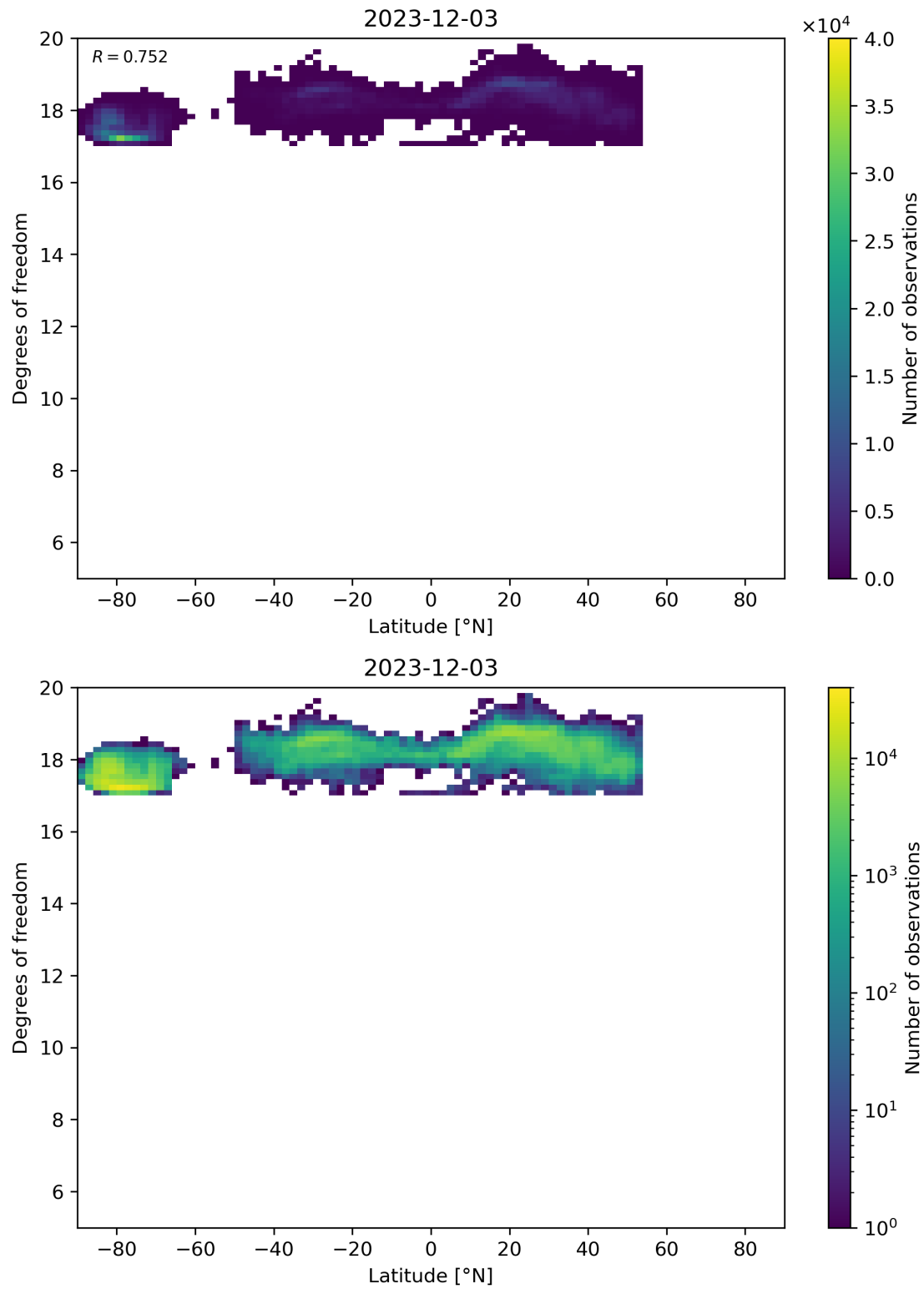
Figure 55: Scatter density plot of “Latitude” against “Degrees of freedom” for 2023-12-02 to 2023-12-04.
