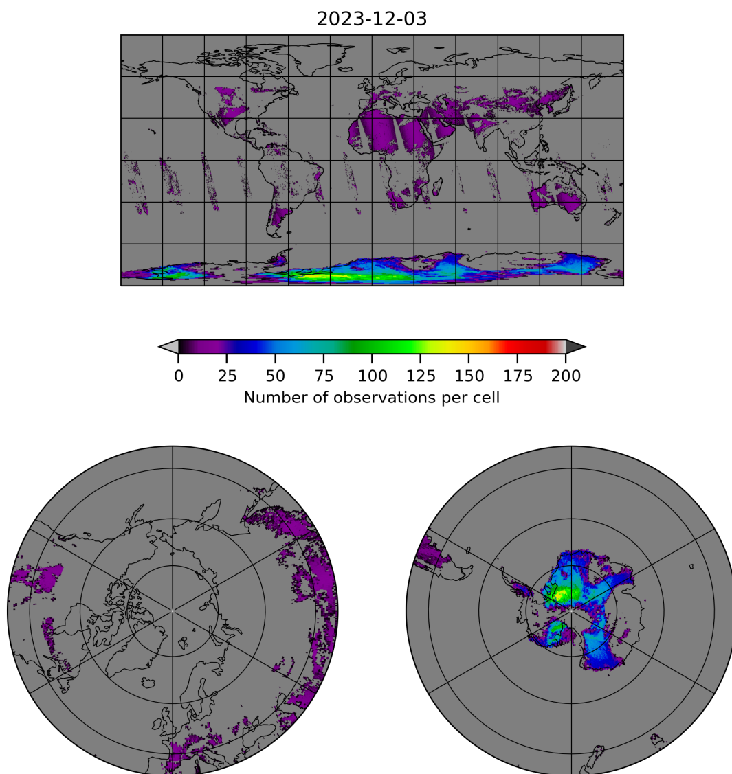
Figure 10: Map of the number of observations for 2023-12-02 to 2023-12-04
