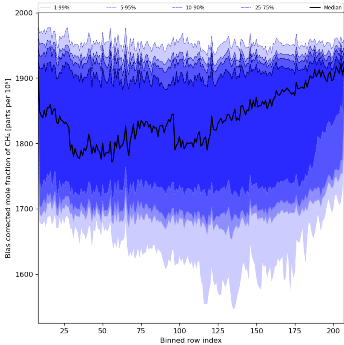
Figure 36: Along track statistics of “Bias corrected mole fraction of CH 4 ” for 2023-12-02 to 2023-12-04
