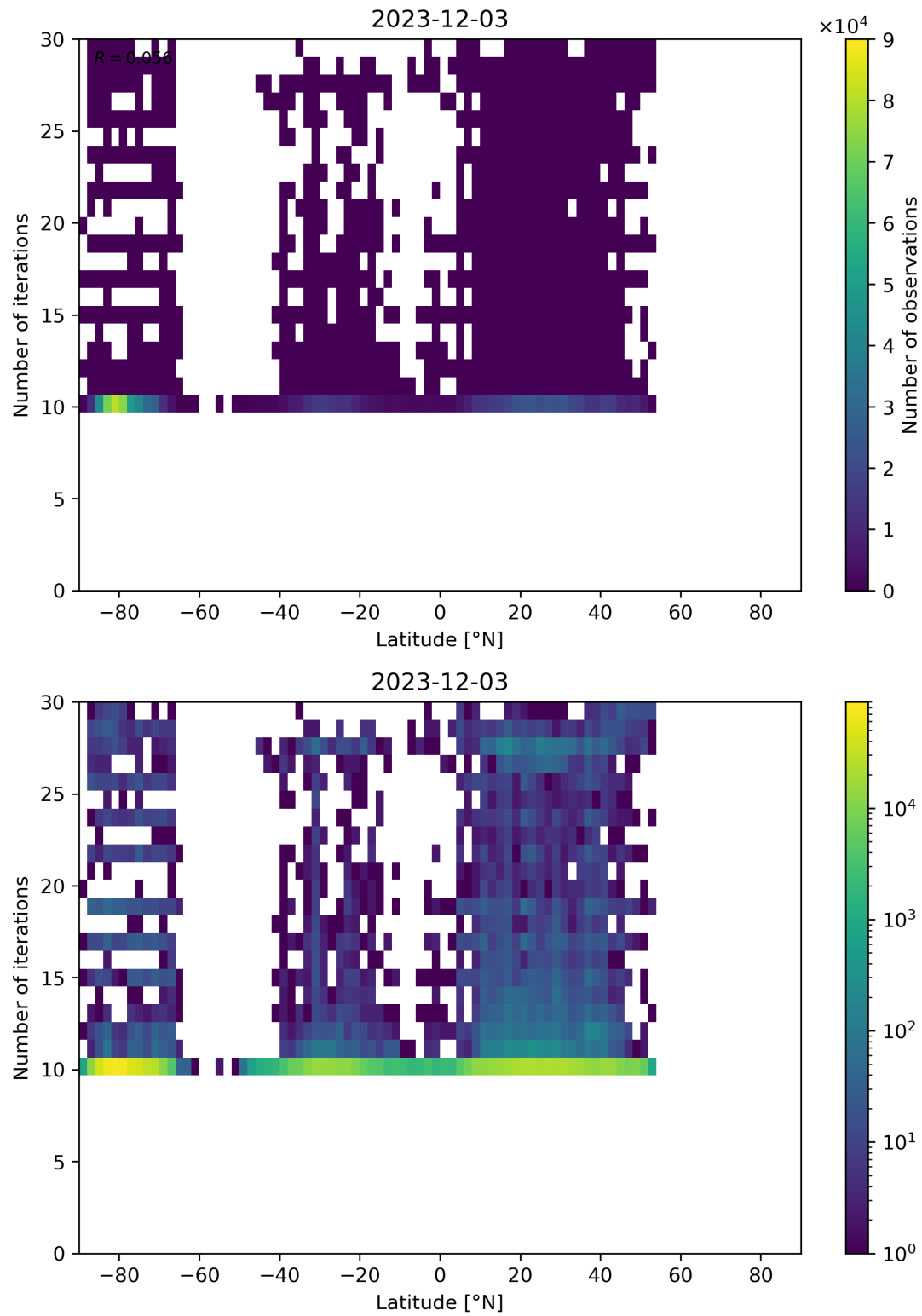
Figure 60: Scatter density plot of “Latitude” against “Number of iterations” for 2023-12-02 to 2023-12-04.
