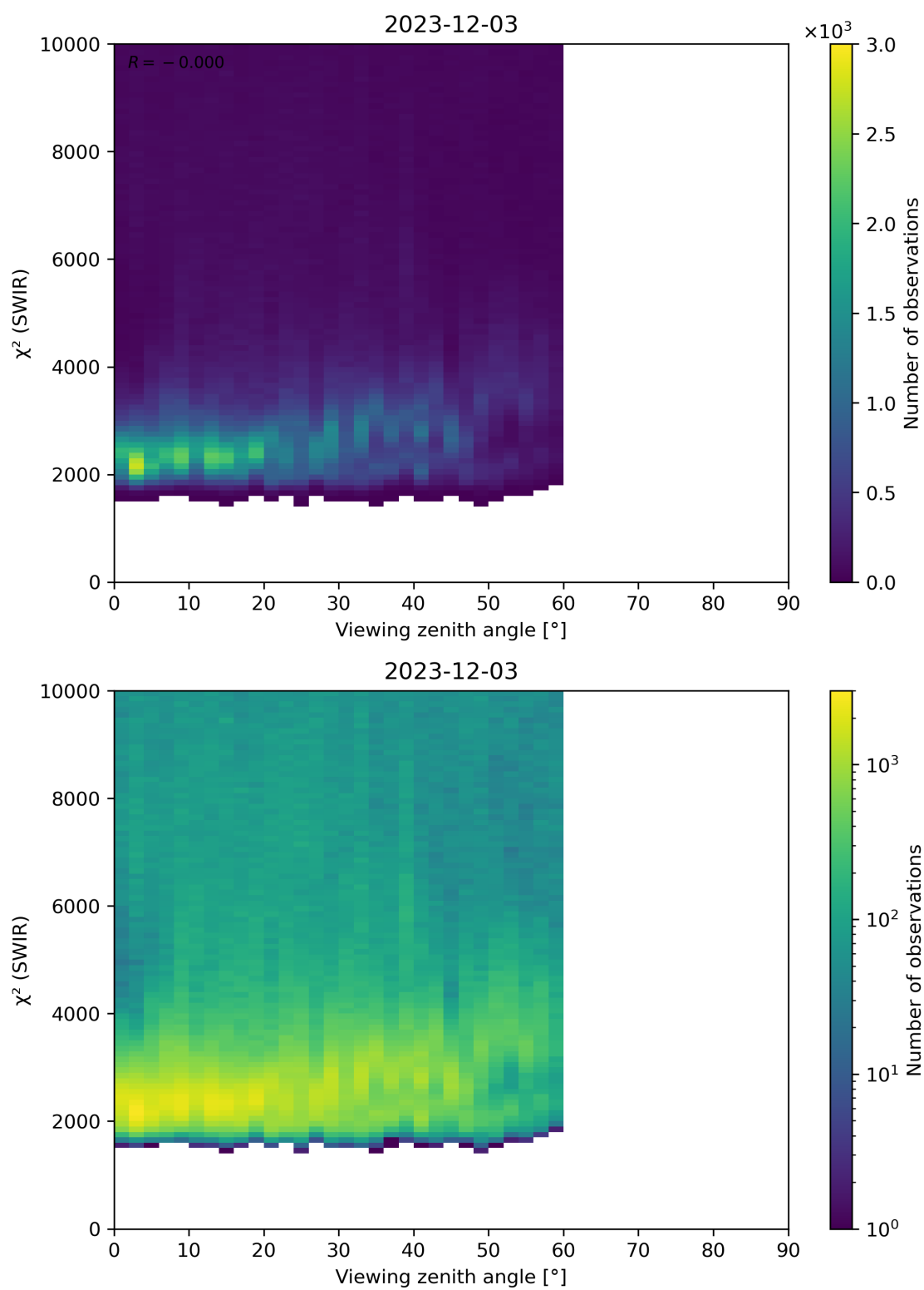
Figure 106: Scatter density plot of “Viewing zenith angle” against “ \chi^2 (SWIR)” for 2023-12-02 to 2023-12-04.
