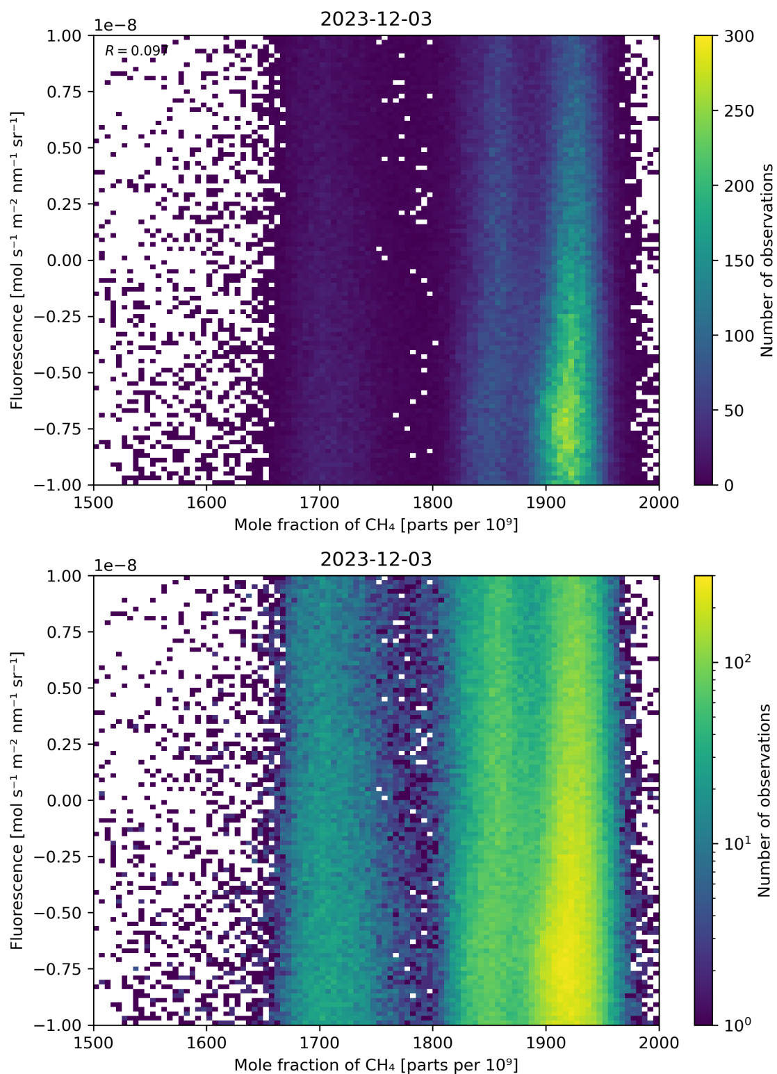
Figure 73: Scatter density plot of “Mole fraction of \text{CH}_4 ” against “Fluorescence” for 2023-12-02 to 2023-12-04.
