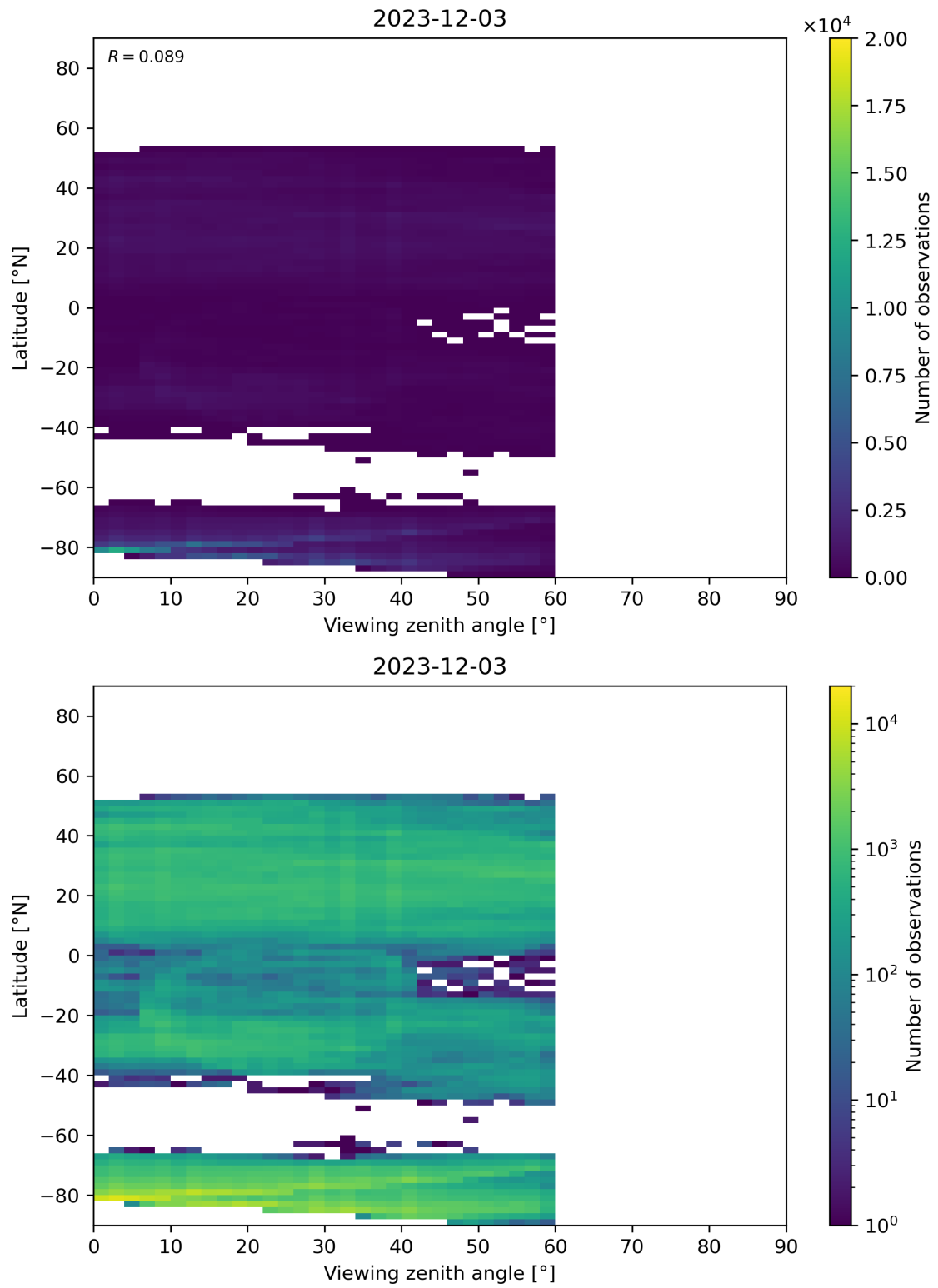
Figure 109: Scatter density plot of “Viewing zenith angle” against “Latitude” for 2023-12-02 to 2023-12-04.
