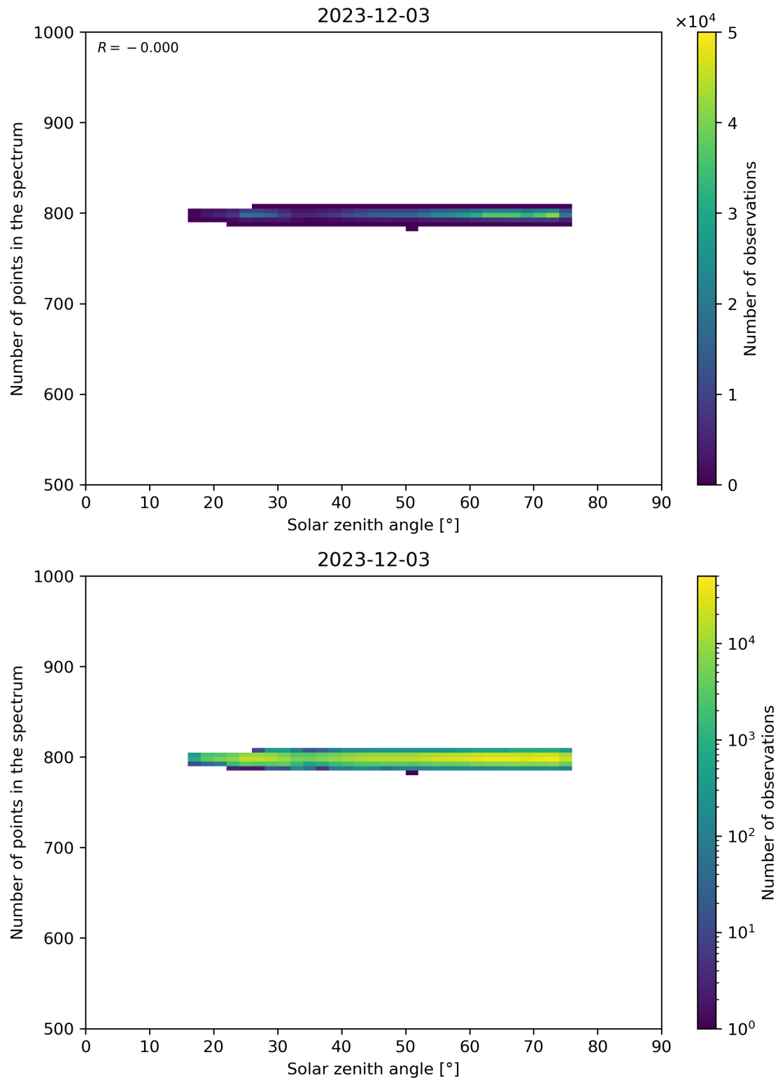
Figure 103: Scatter density plot of “Solar zenith angle” against “Number of points in the spectrum” for 2023-12-02 to 2023-12-04.
