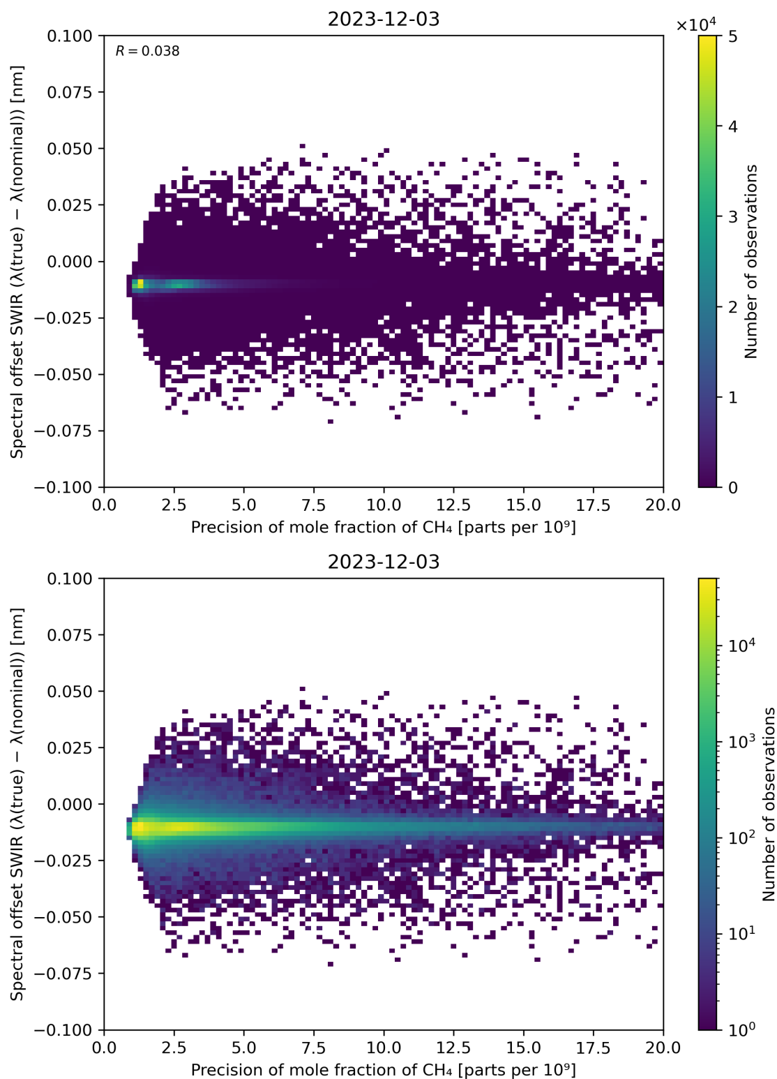
Figure 85: Scatter density plot of “Precision of mole fraction of CH 4 ” against “Spectral offset SWIR ( \lambda(\text{true}) - \lambda(\text{nominal}) )” for 2023-12-02 to 2023-12-04.
