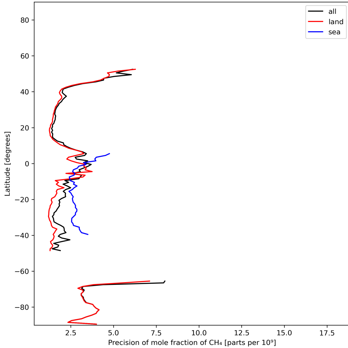
Figure 13: Zonal average of “Precision of mole fraction of CH 4 ” for 2023-12-02 to 2023-12-04.
