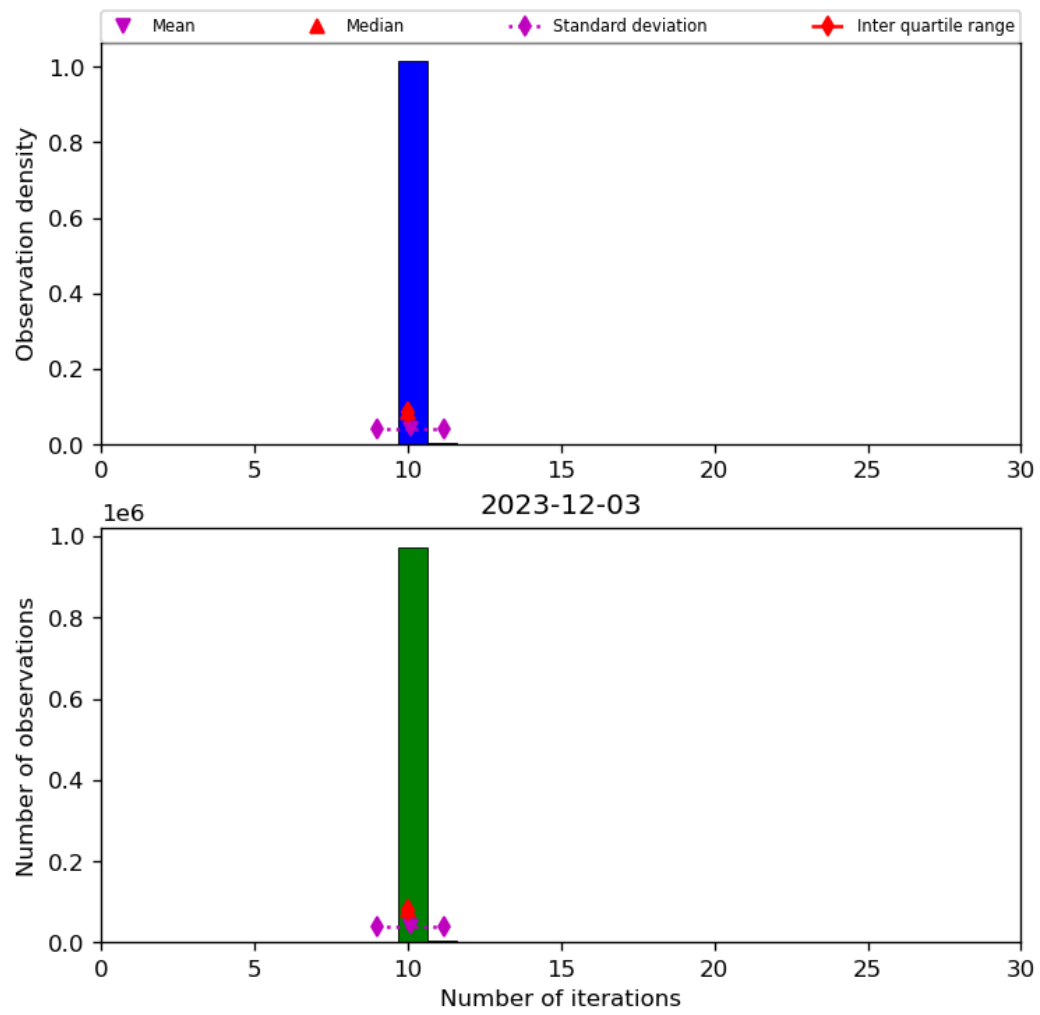
Figure 31: Histogram of “Number of iterations” for 2023-12-02 to 2023-12-04
