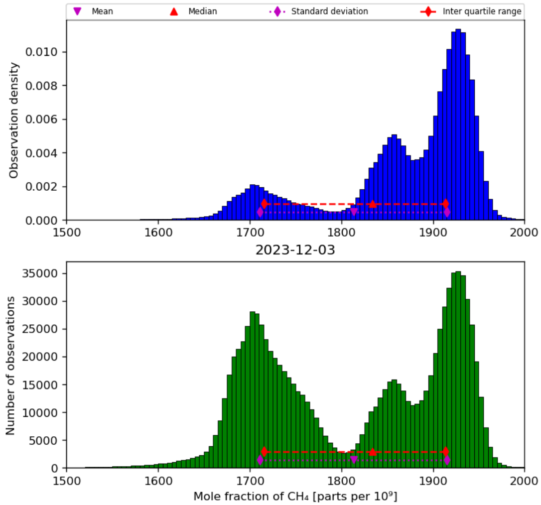
Figure 23: Histogram of “Mole fraction of CH 4 ” for 2023-12-02 to 2023-12-04
