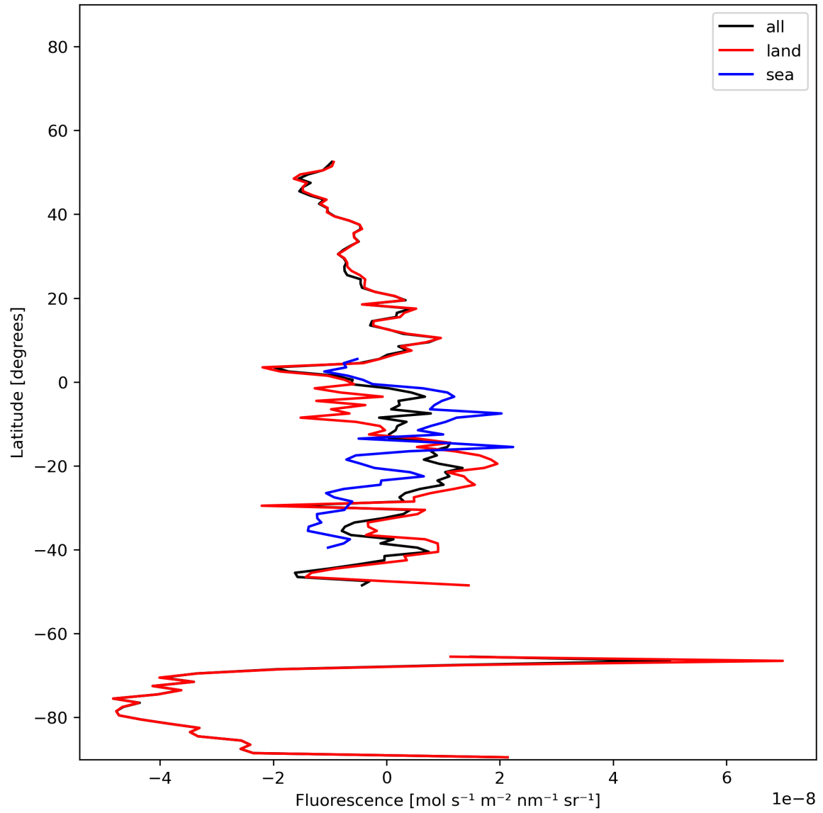
Figure 21: Zonal average of “Fluorescence” for 2023-12-02 to 2023-12-04.
