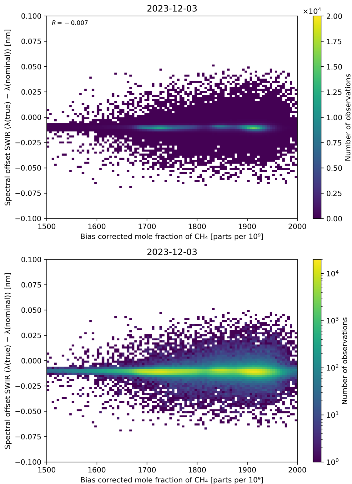
Figure 69: Scatter density plot of “Bias corrected mole fraction of \text{CH}_4 ” against “Spectral offset SWIR ( \lambda(\text{true}) - \lambda(\text{nominal}) )” for 2023-12-02 to 2023-12-04.
