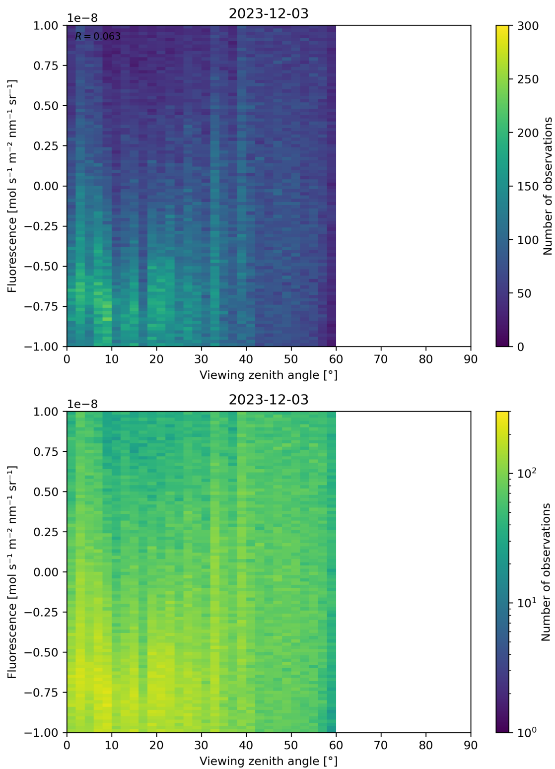
Figure 108: Scatter density plot of “Viewing zenith angle” against “Fluorescence” for 2023-12-02 to 2023-12-04.
