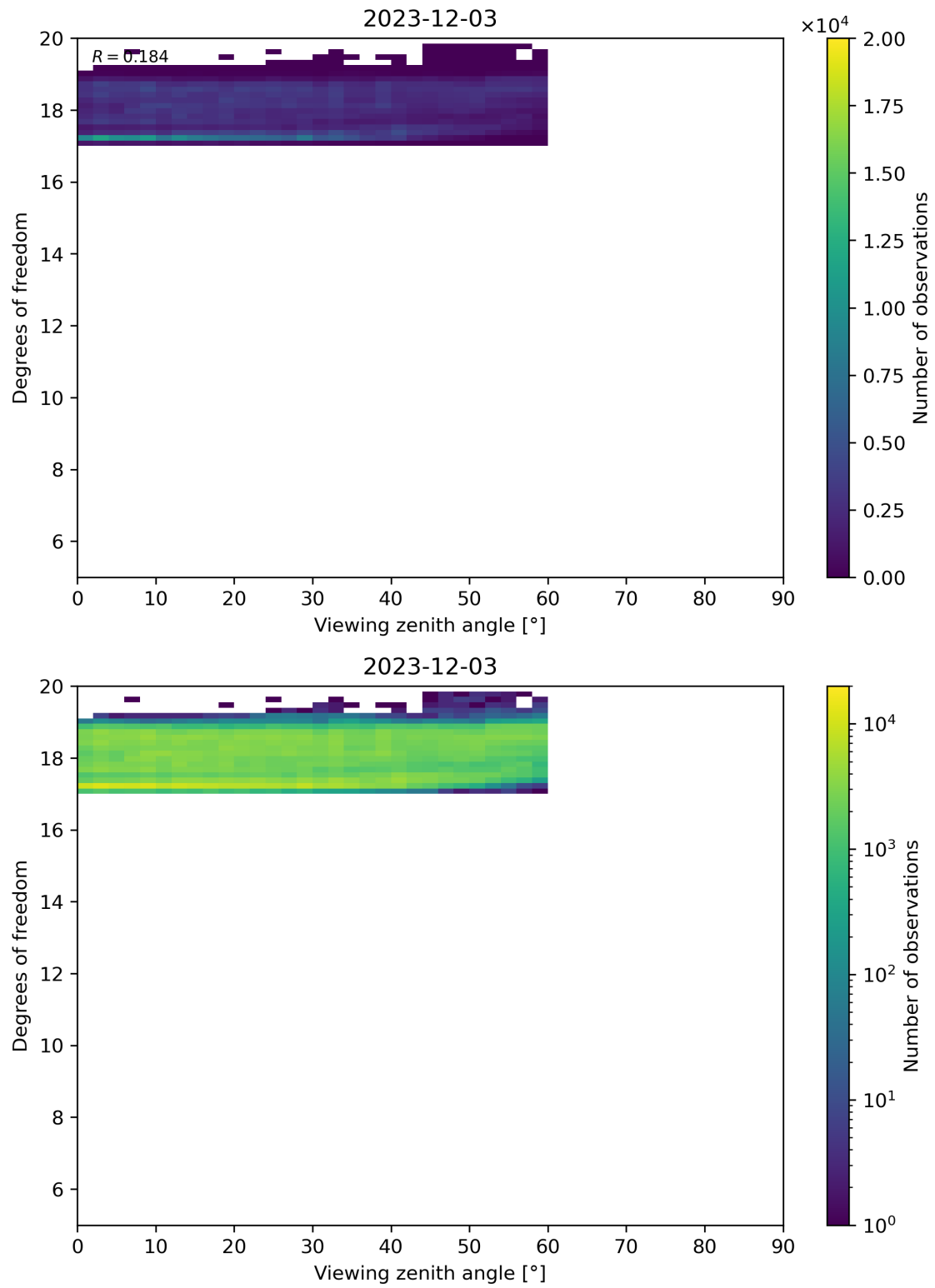
Figure 107: Scatter density plot of “Viewing zenith angle” against “Degrees of freedom” for 2023-12-02 to 2023-12-04.
