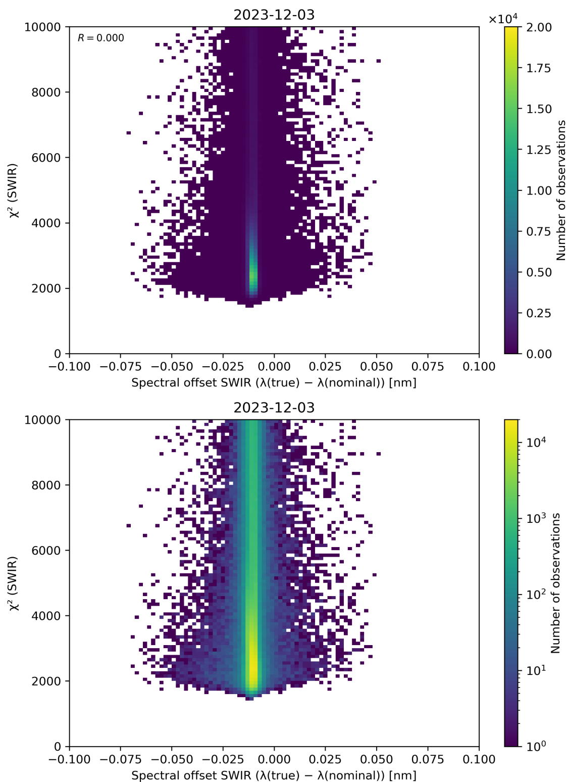
Figure 118: Scatter density plot of “Spectral offset SWIR ( \lambda(\text{true}) - \lambda(\text{nominal}) )” against “ \chi^2 (SWIR)” for 2023-12-02 to 2023-12-04.
