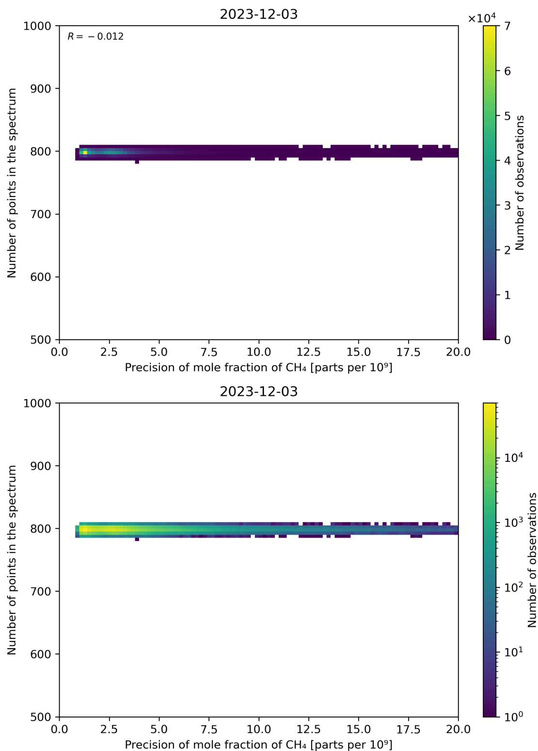
Figure 84: Scatter density plot of “Precision of mole fraction of CH 4 ” against “Number of points in the spectrum” for 2023-12-02 to 2023-12-04.
