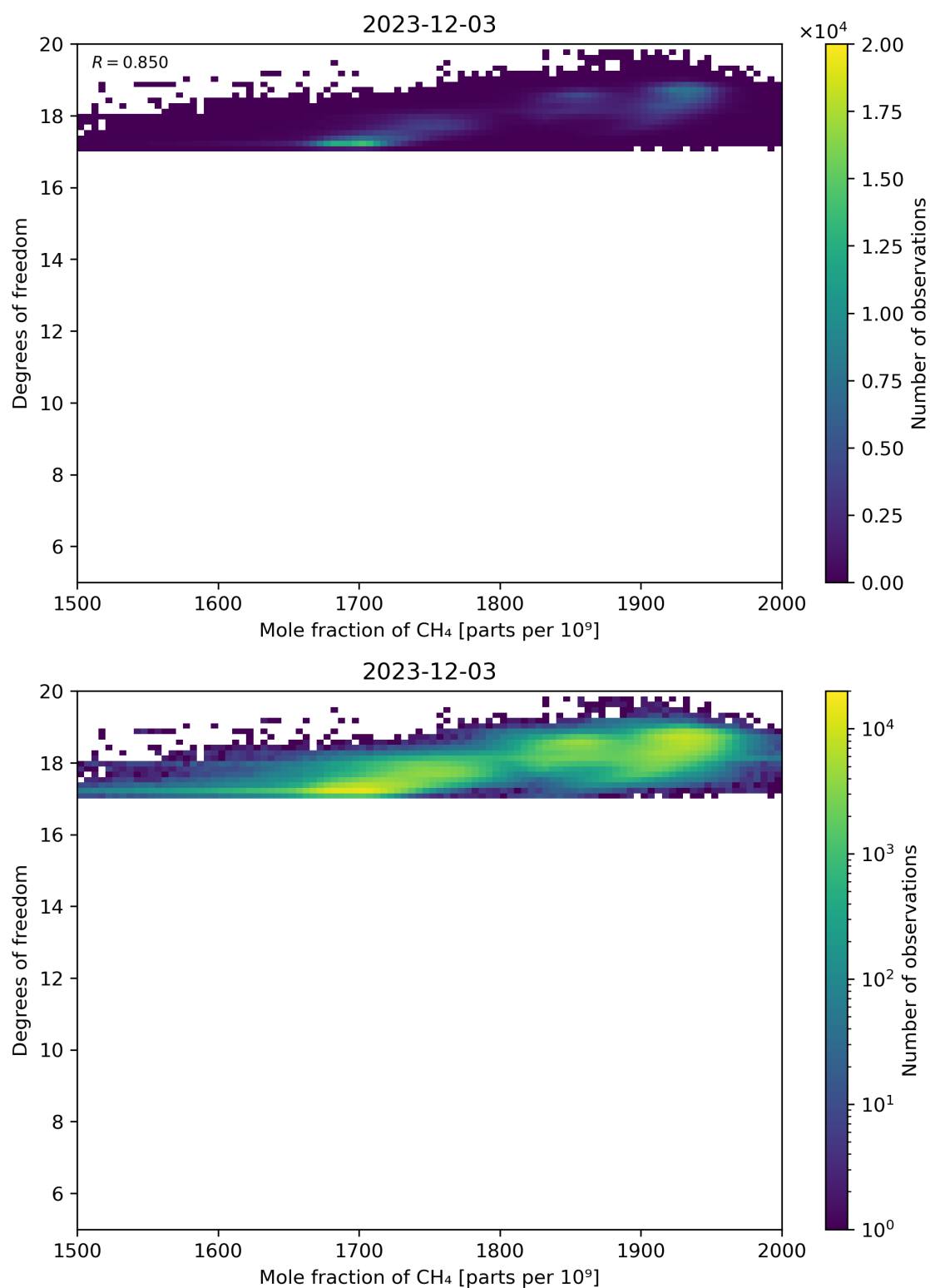
Figure 72: Scatter density plot of “Mole fraction of CH 4 ” against “Degrees of freedom” for 2023-12-02 to 2023-12-04.
