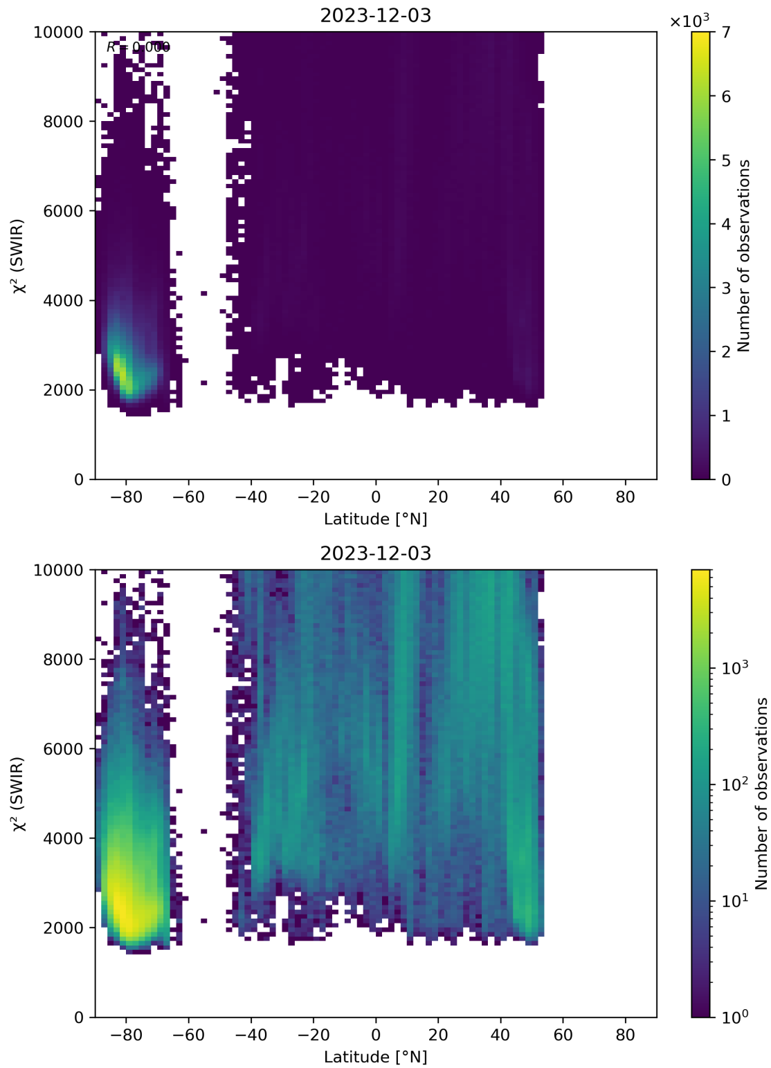
Figure 54: Scatter density plot of “Latitude” against “ \chi^2 (SWIR)” for 2023-12-02 to 2023-12-04.
