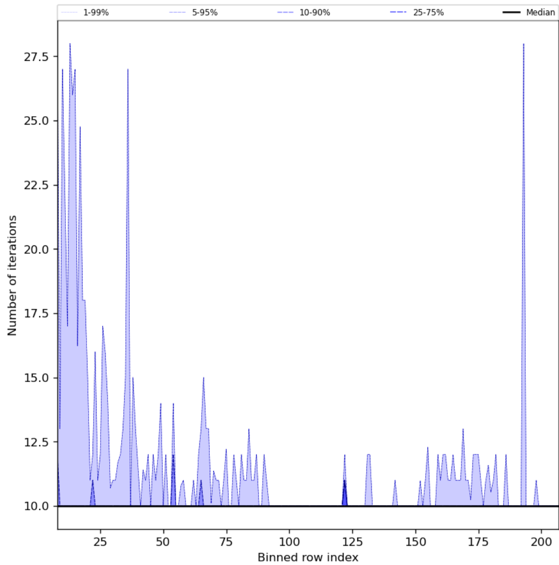
Figure 42: Along track statistics of “Number of iterations” for 2023-12-02 to 2023-12-04
