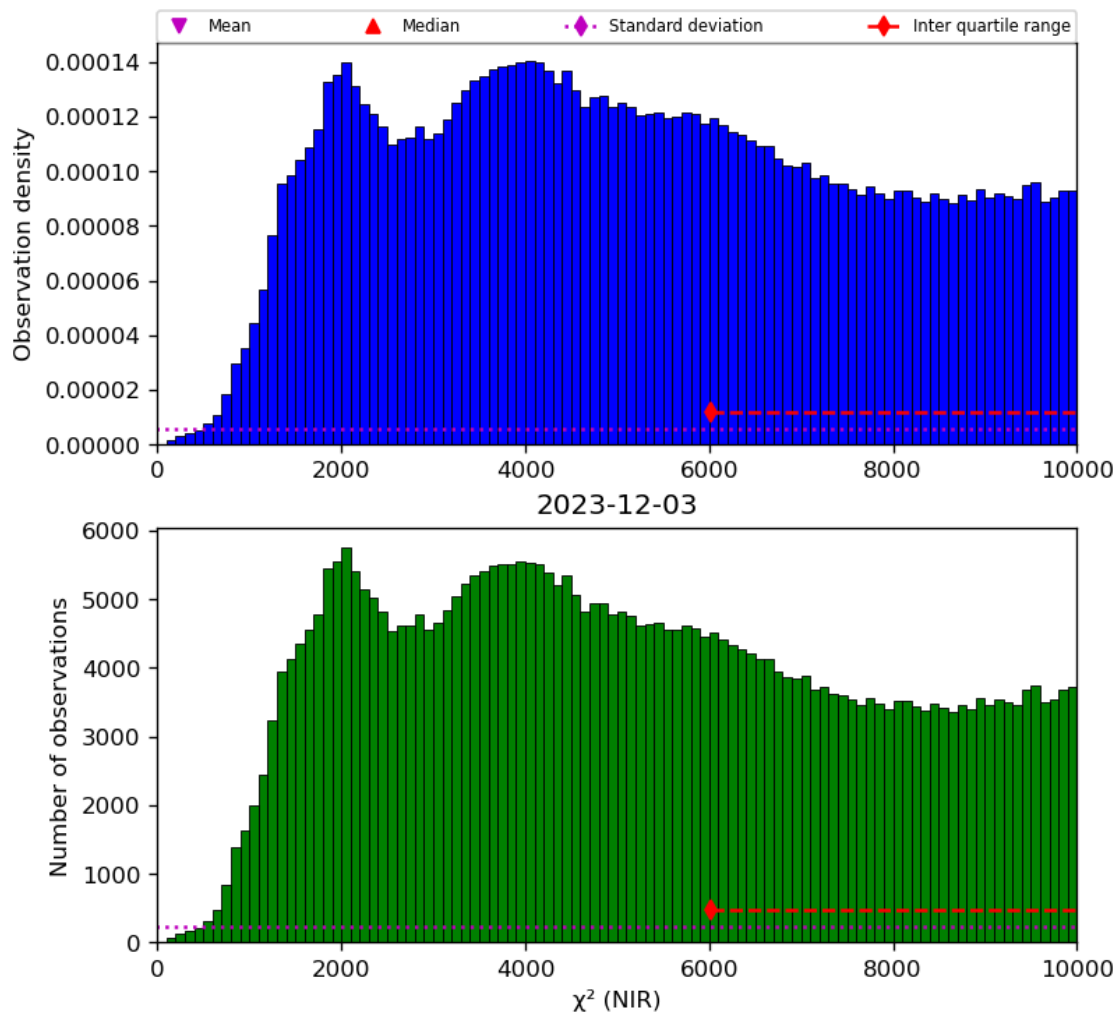
Figure 29: Histogram of “ \chi^2 (NIR)” for 2023-12-02 to 2023-12-04
