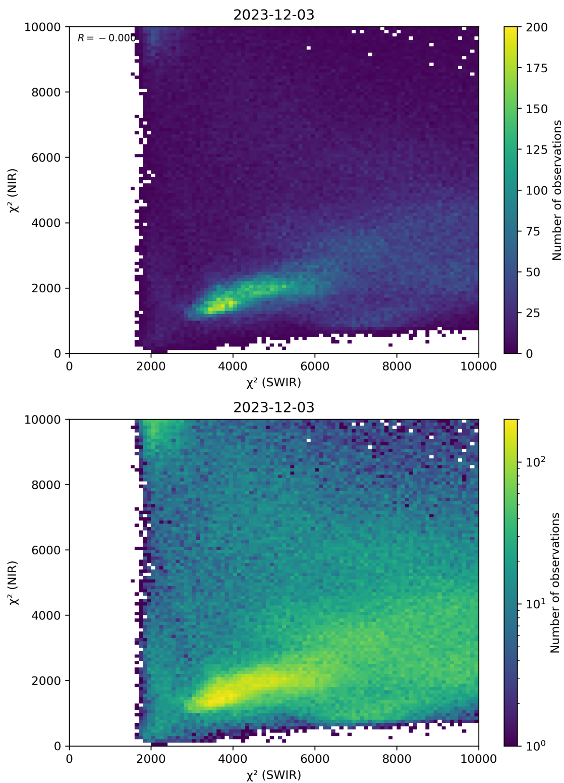
Figure 47: Scatter density plot of “ \chi^2 (SWIR)” against “ \chi^2 (NIR)” for 2023-12-02 to 2023-12-04.
