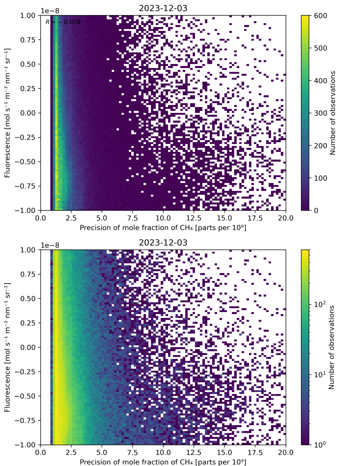
Figure 81: Scatter density plot of “Precision of mole fraction of \text{CH}_4 ” against “Fluorescence” for 2023-12-02 to 2023-12-04.
