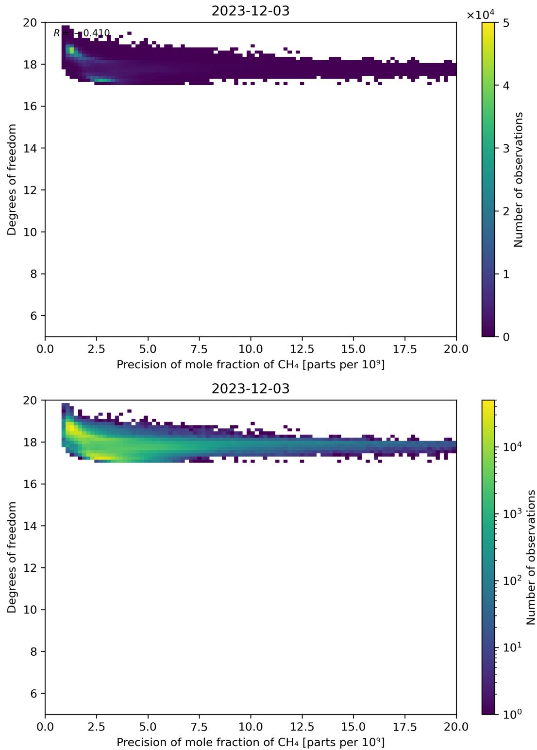
Figure 80: Scatter density plot of “Precision of mole fraction of CH 4 ” against “Degrees of freedom” for 2023-12-02 to 2023-12-04.
