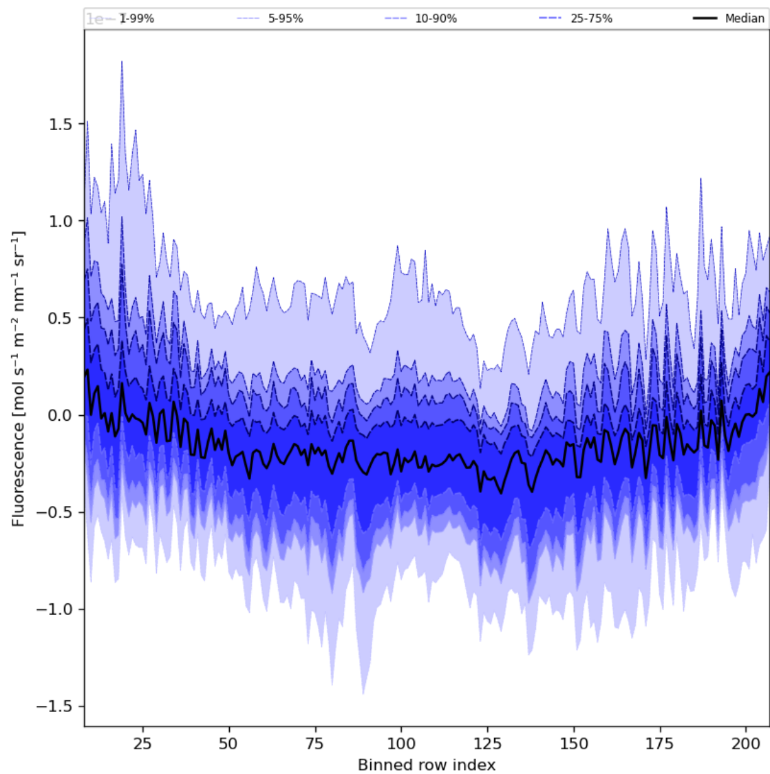
Figure 43: Along track statistics of “Fluorescence” for 2023-12-02 to 2023-12-04
