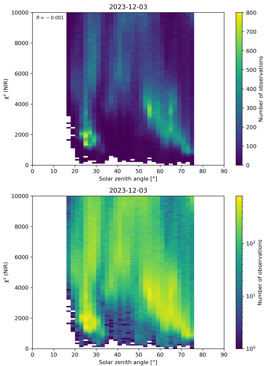
Figure 94: Scatter density plot of “Solar zenith angle” against “ \chi^2 (NIR)” for 2023-12-02 to 2023-12-04.
