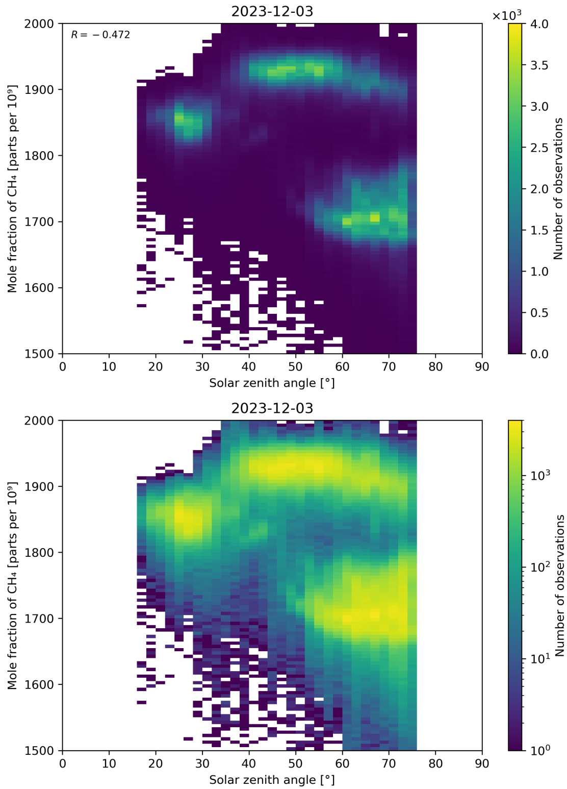
Figure 99: Scatter density plot of “Solar zenith angle” against “Mole fraction of CH 4 ” for 2023-12-02 to 2023-12-04.
