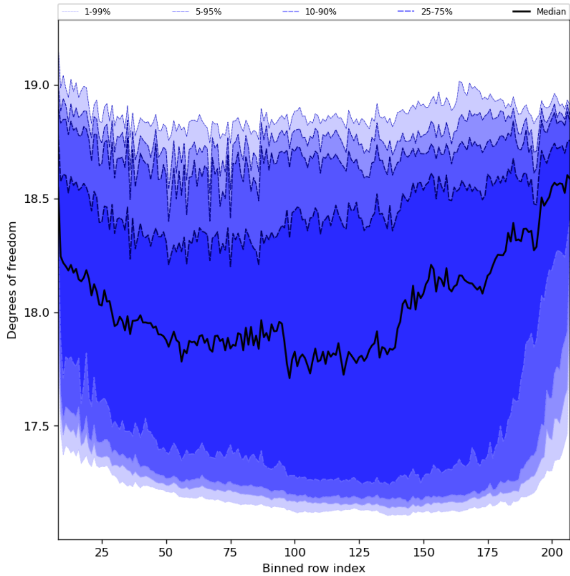
Figure 41: Along track statistics of “Degrees of freedom” for 2023-12-02 to 2023-12-04
