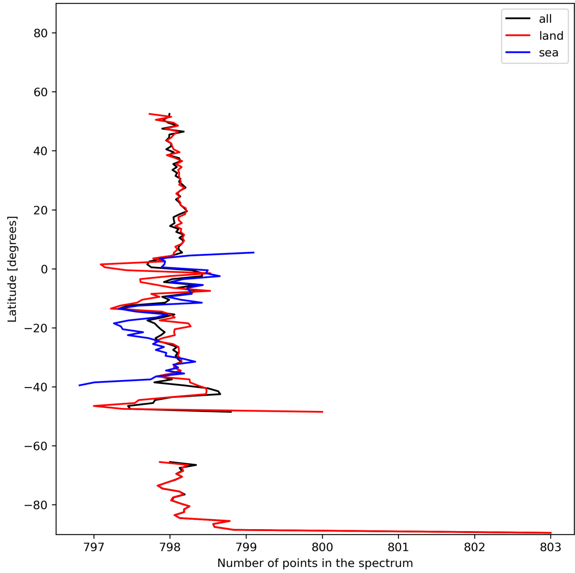
Figure 15: Zonal average of “Number of points in the spectrum” for 2023-12-02 to 2023-12-04.
