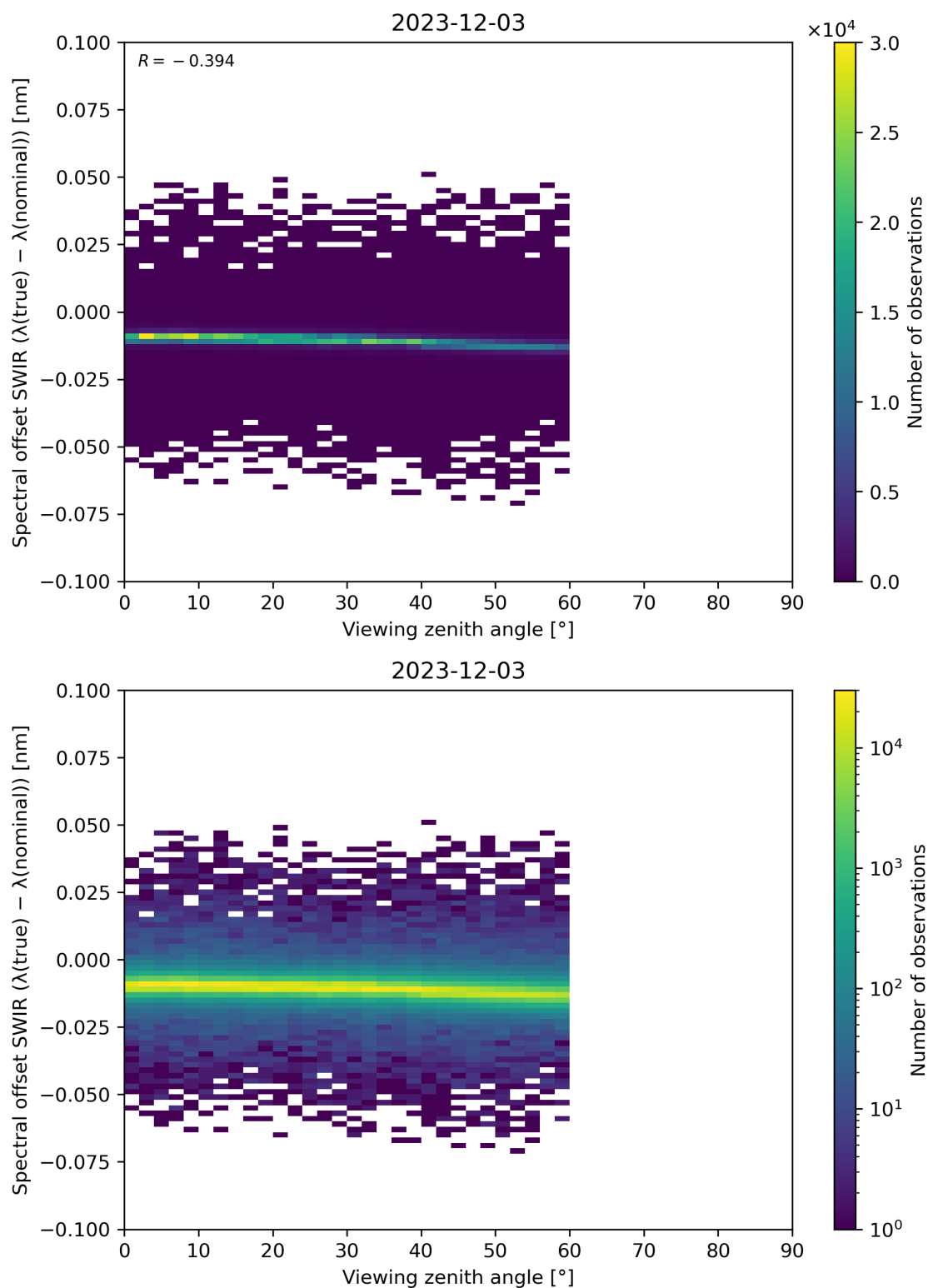
Figure 116: Scatter density plot of “Viewing zenith angle” against “Spectral offset SWIR ( \lambda(\text{true}) - \lambda(\text{nominal}) )” for 2023-12-02 to 2023-12-04.
