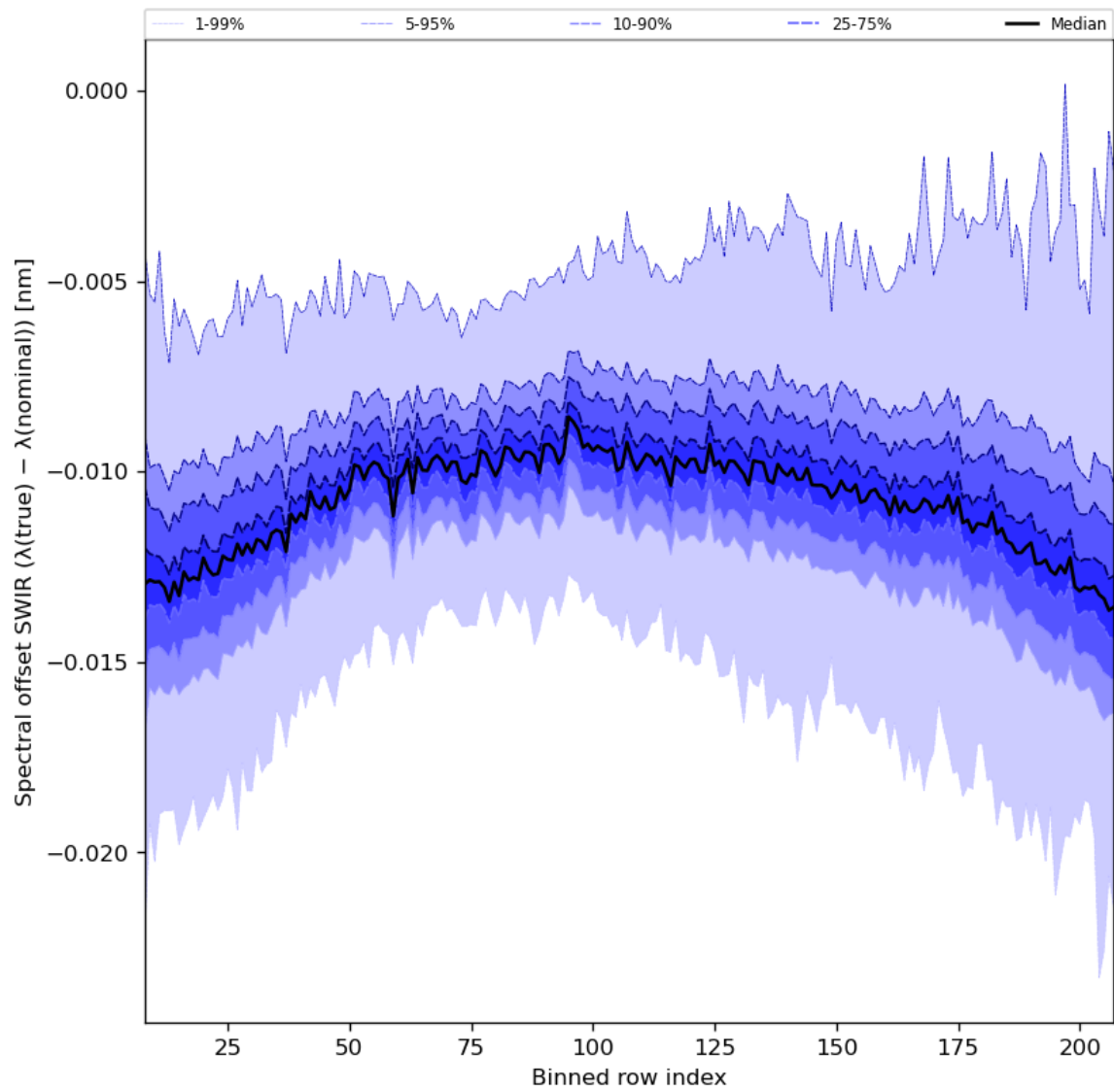
Figure 38: Along track statistics of “Spectral offset SWIR ( \lambda(\text{true}) - \lambda(\text{nominal}) )” for 2023-12-02 to 2023-12-04
