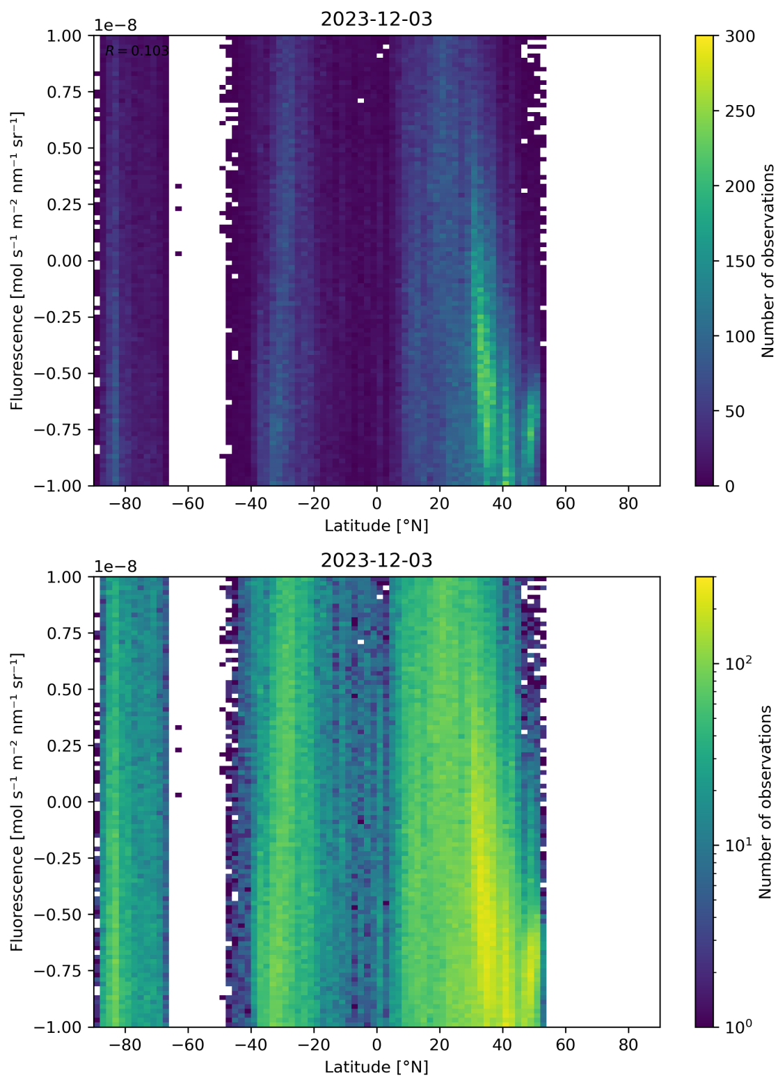
Figure 56: Scatter density plot of “Latitude” against “Fluorescence” for 2023-12-02 to 2023-12-04.
