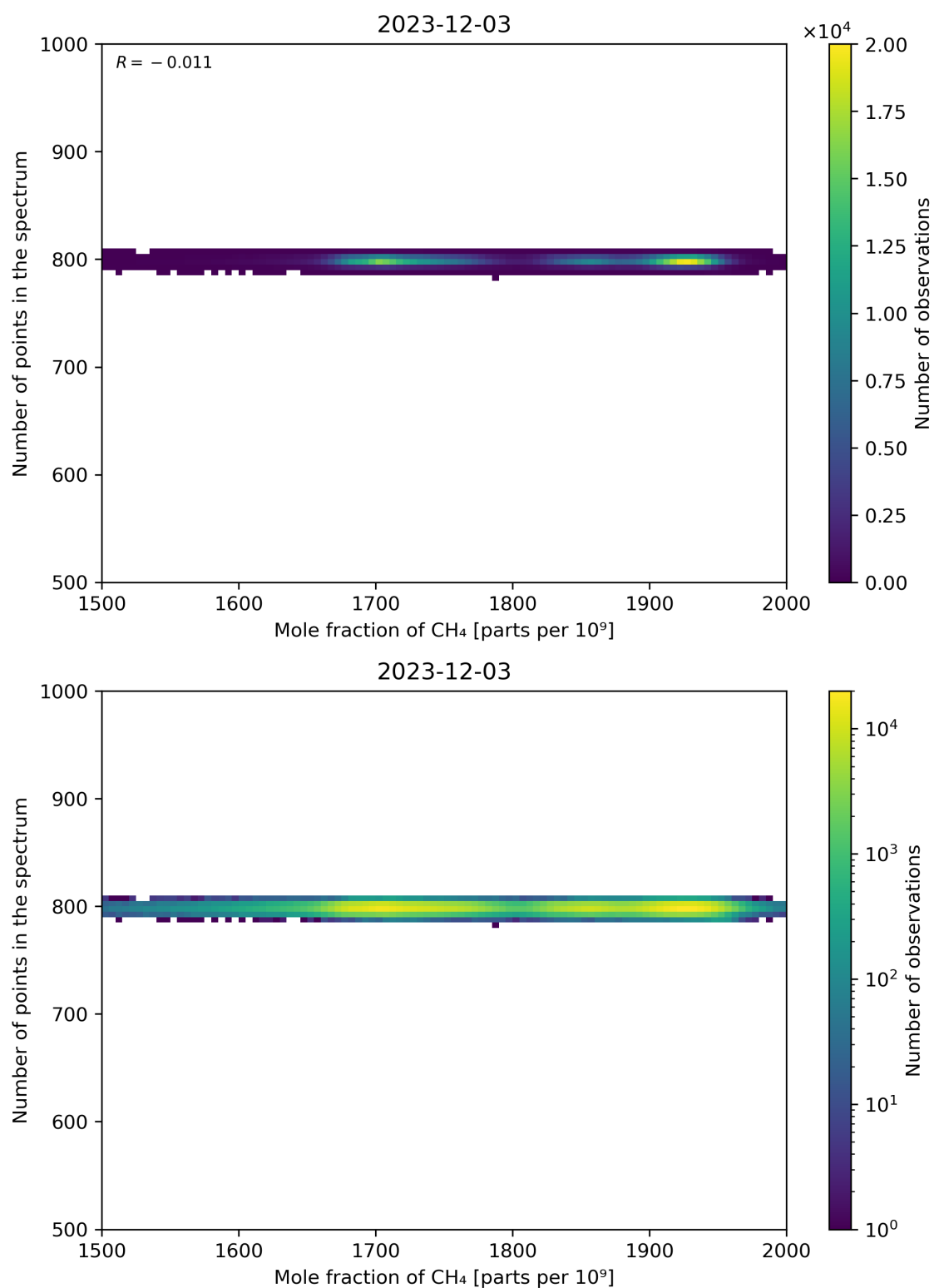
Figure 77: Scatter density plot of “Mole fraction of CH 4 ” against “Number of points in the spectrum” for 2023-12-02 to 2023-12-04.
