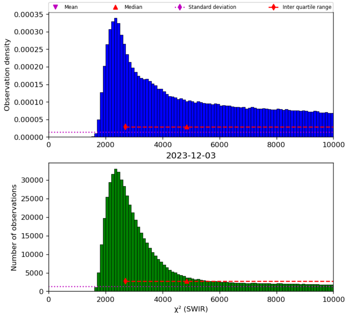
Figure 28: Histogram of “ \chi^2 (SWIR)” for 2023-12-02 to 2023-12-04
