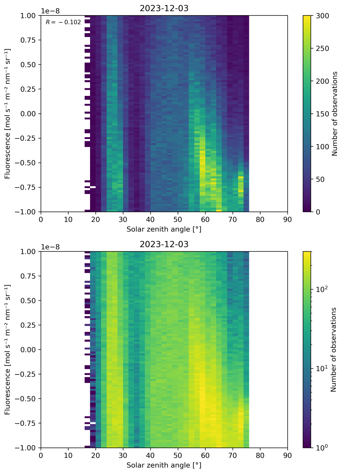
Figure 97: Scatter density plot of “Solar zenith angle” against “Fluorescence” for 2023-12-02 to 2023-12-04.
