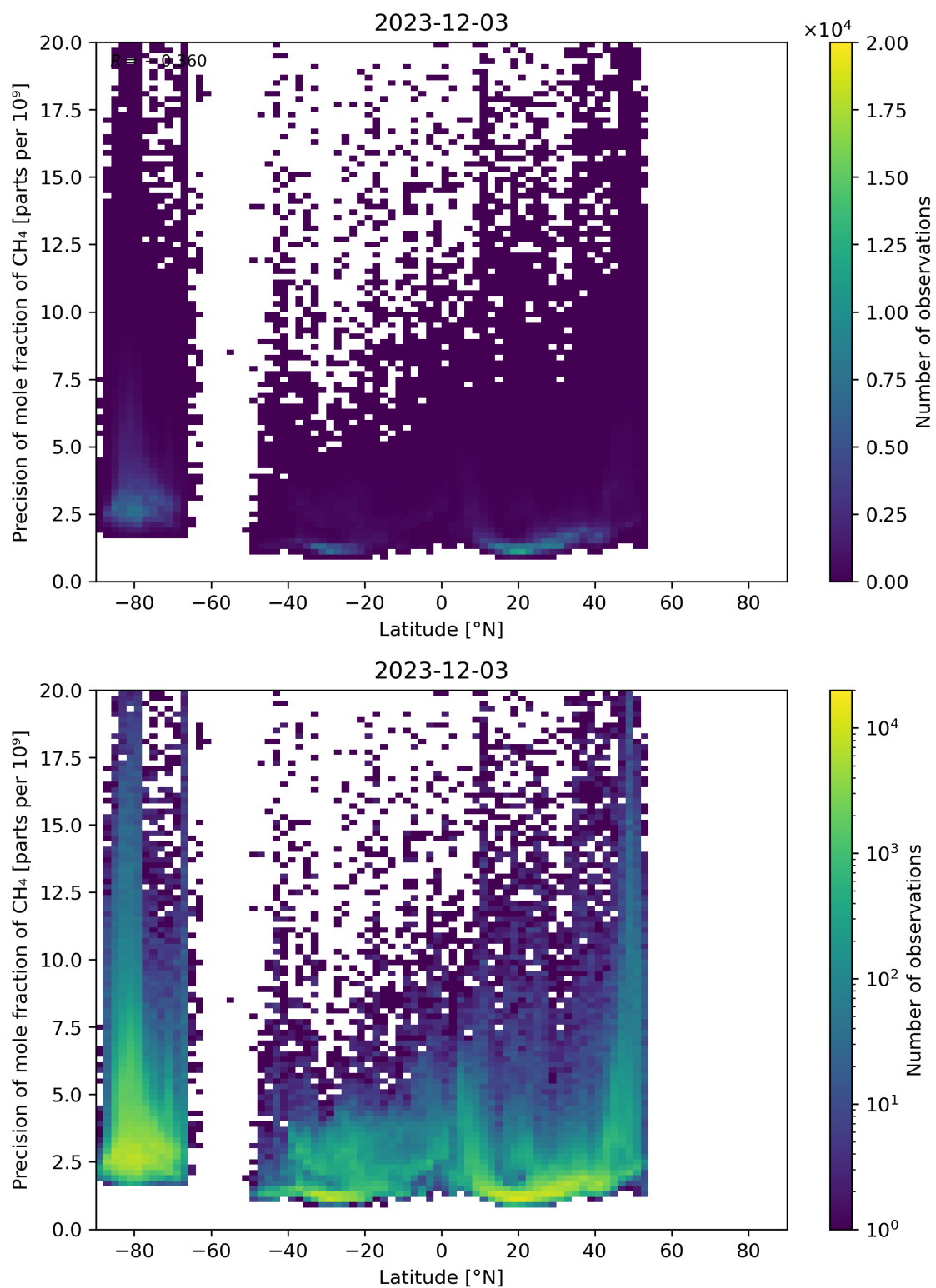
Figure 59: Scatter density plot of “Latitude” against “Precision of mole fraction of CH 4 ” for 2023-12-02 to 2023-12-04.
