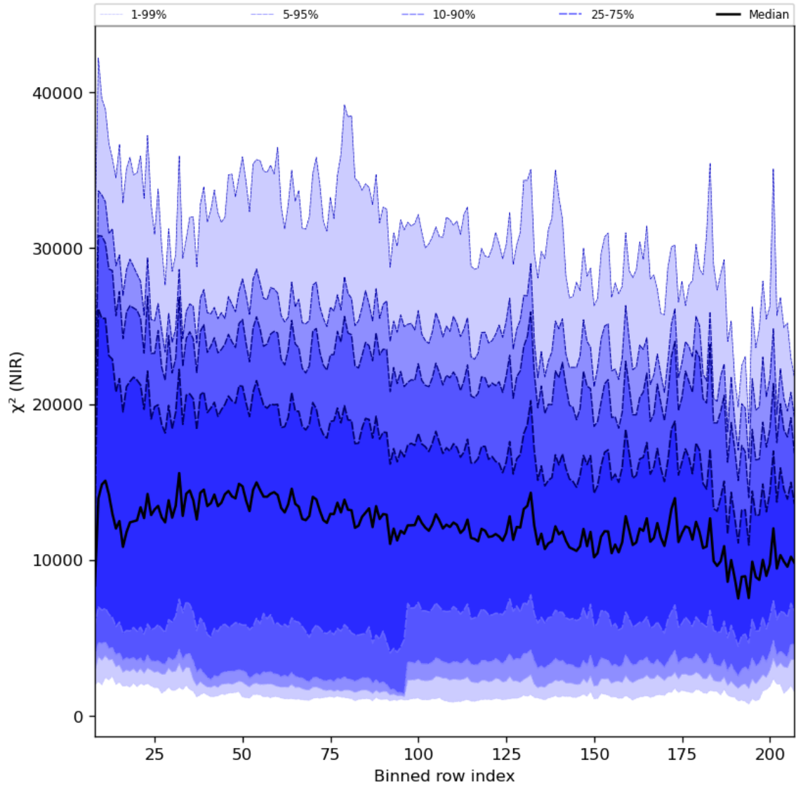
Figure 40: Along track statistics of “ \chi^2 (NIR)” for 2023-12-02 to 2023-12-04
