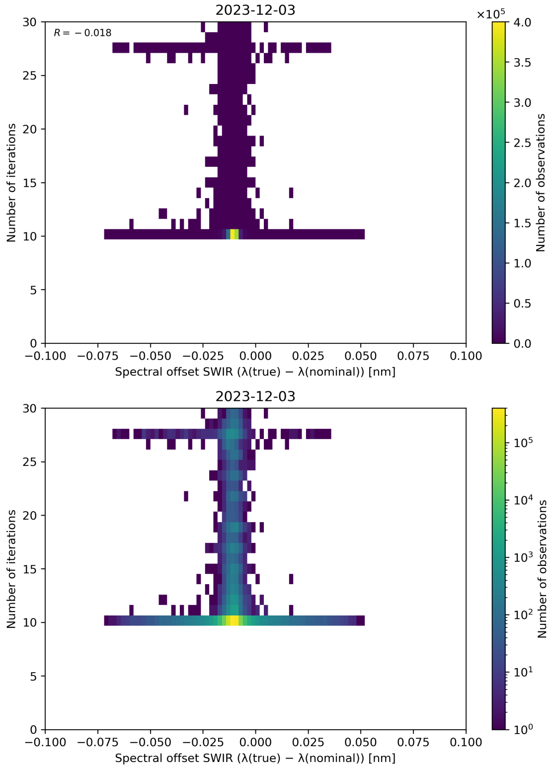
Figure 121: Scatter density plot of “Spectral offset SWIR ( \lambda(\text{true}) - \lambda(\text{nominal}) )” against “Number of iterations” for 2023-12-02 to 2023-12-04.
