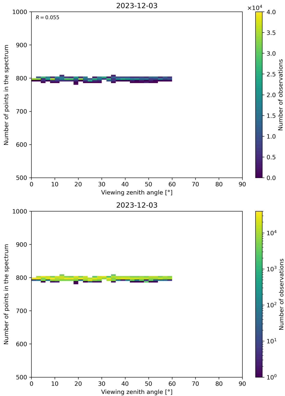
Figure 114: Scatter density plot of “Viewing zenith angle” against “Number of points in the spectrum” for 2023-12-02 to 2023-12-04.
