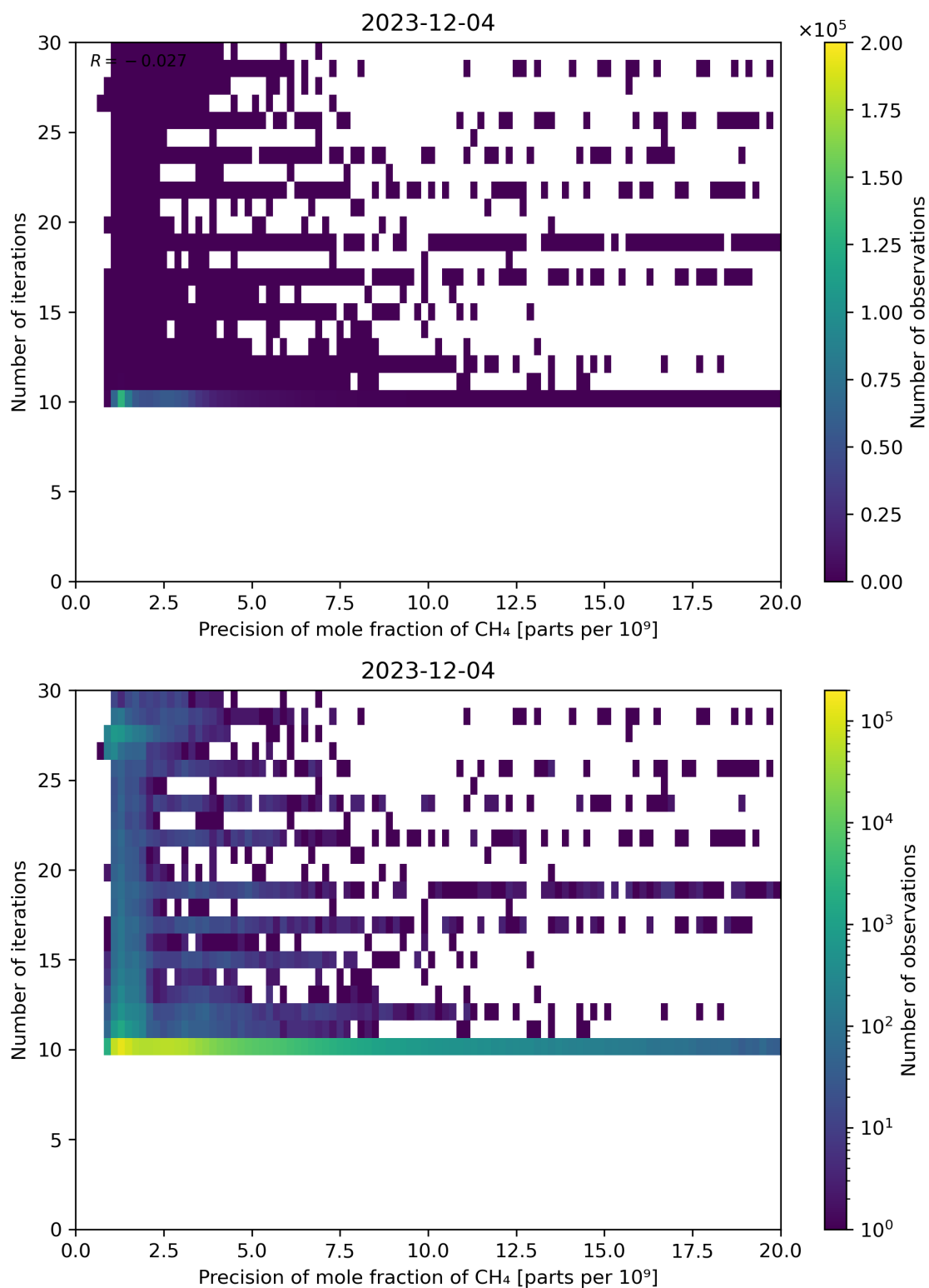
Figure 83: Scatter density plot of “Precision of mole fraction of CH 4 ” against “Number of iterations” for 2023-12-04 to 2023-12-05.
