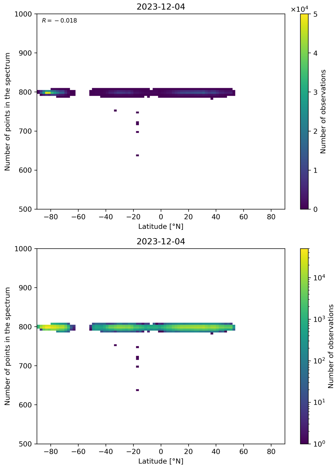
Figure 61: Scatter density plot of “Latitude” against “Number of points in the spectrum” for 2023-12-04 to 2023-12-05.
