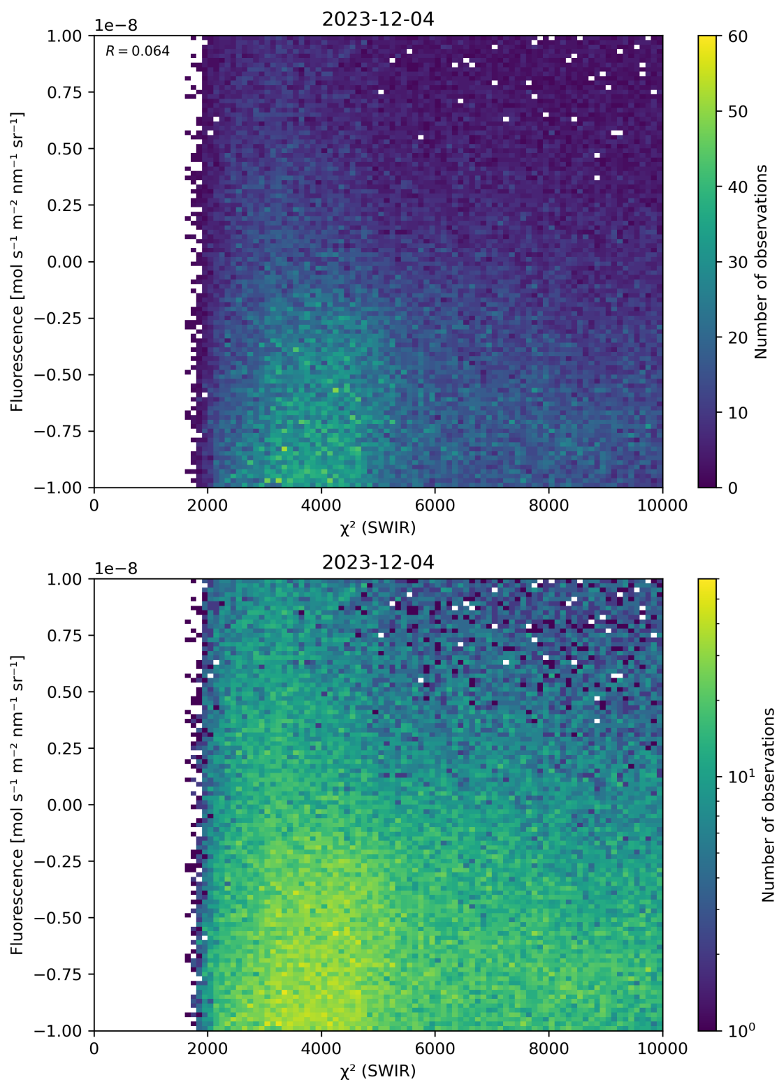
Figure 49: Scatter density plot of “ \chi^2 (SWIR)” against “Fluorescence” for 2023-12-04 to 2023-12-05.
