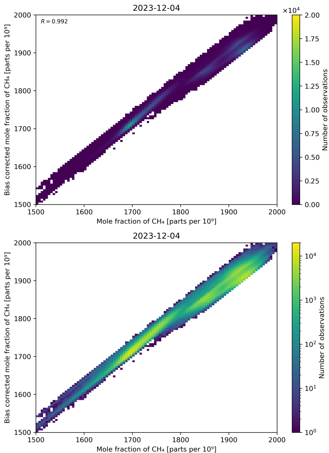
Figure 74: Scatter density plot of “Mole fraction of CH 4 ” against “Bias corrected mole fraction of CH 4 ” for 2023-12-04 to 2023-12-05.
