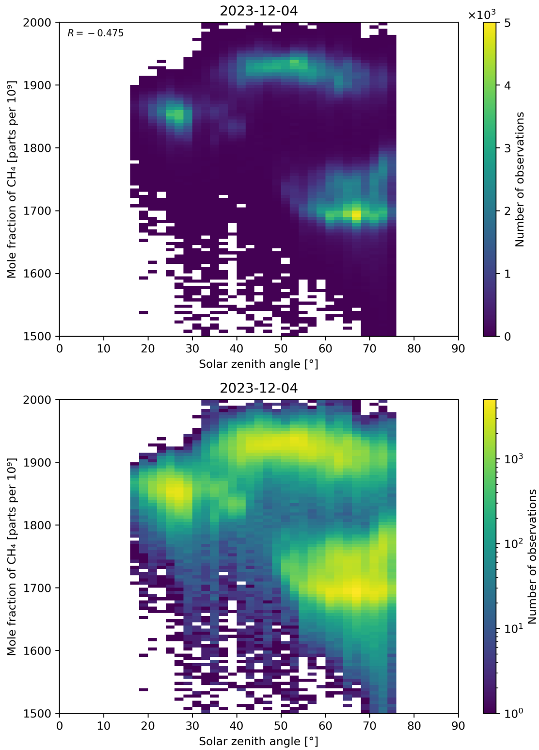
Figure 99: Scatter density plot of “Solar zenith angle” against “Mole fraction of CH 4 ” for 2023-12-04 to 2023-12-05.
