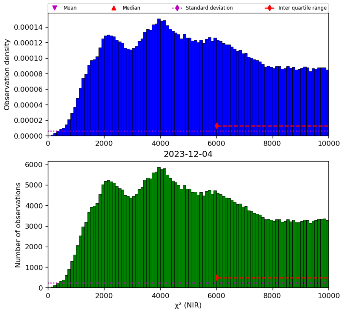
Figure 29: Histogram of “ \chi^2 (NIR)” for 2023-12-04 to 2023-12-05
