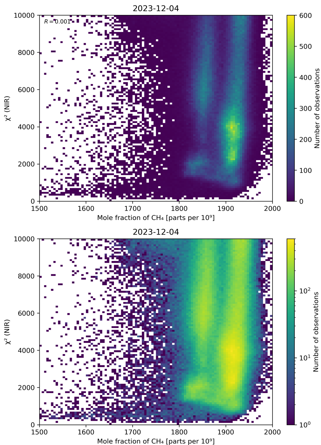
Figure 70: Scatter density plot of “Mole fraction of \text{CH}_4 ” against “ \chi^2 (NIR)” for 2023-12-04 to 2023-12-05.
