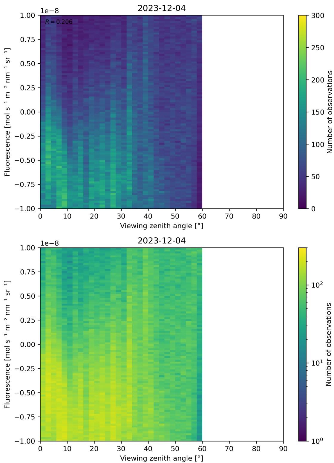
Figure 108: Scatter density plot of “Viewing zenith angle” against “Fluorescence” for 2023-12-04 to 2023-12-05.
