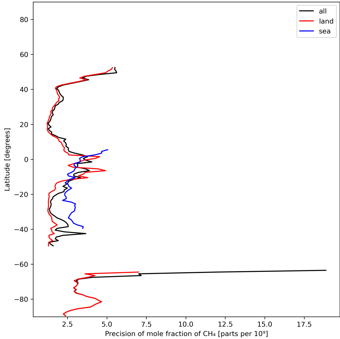
Figure 13: Zonal average of “Precision of mole fraction of CH 4 ” for 2023-12-04 to 2023-12-05.
