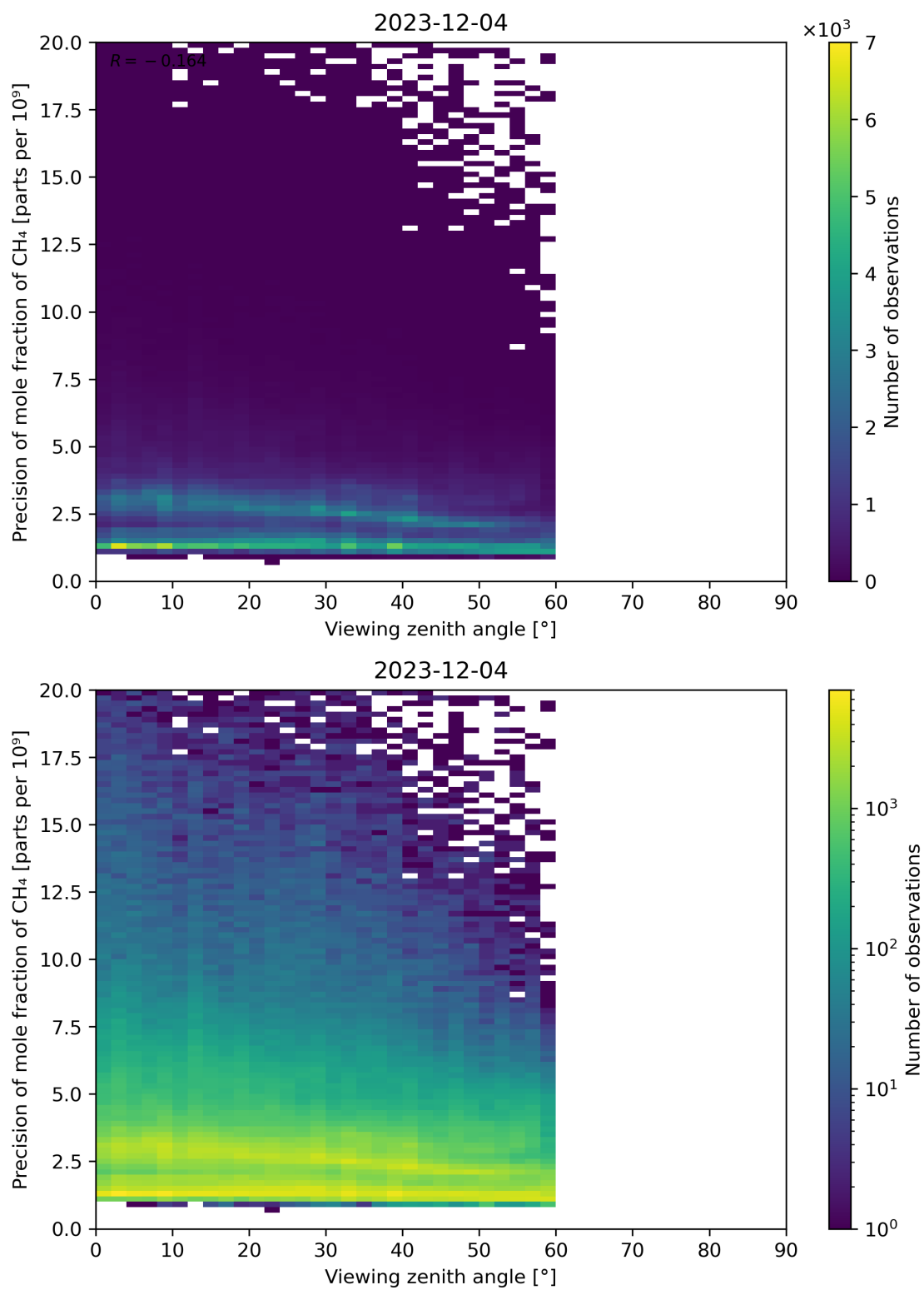
Figure 112: Scatter density plot of “Viewing zenith angle” against “Precision of mole fraction of CH 4 ” for 2023-12-04 to 2023-12-05.
