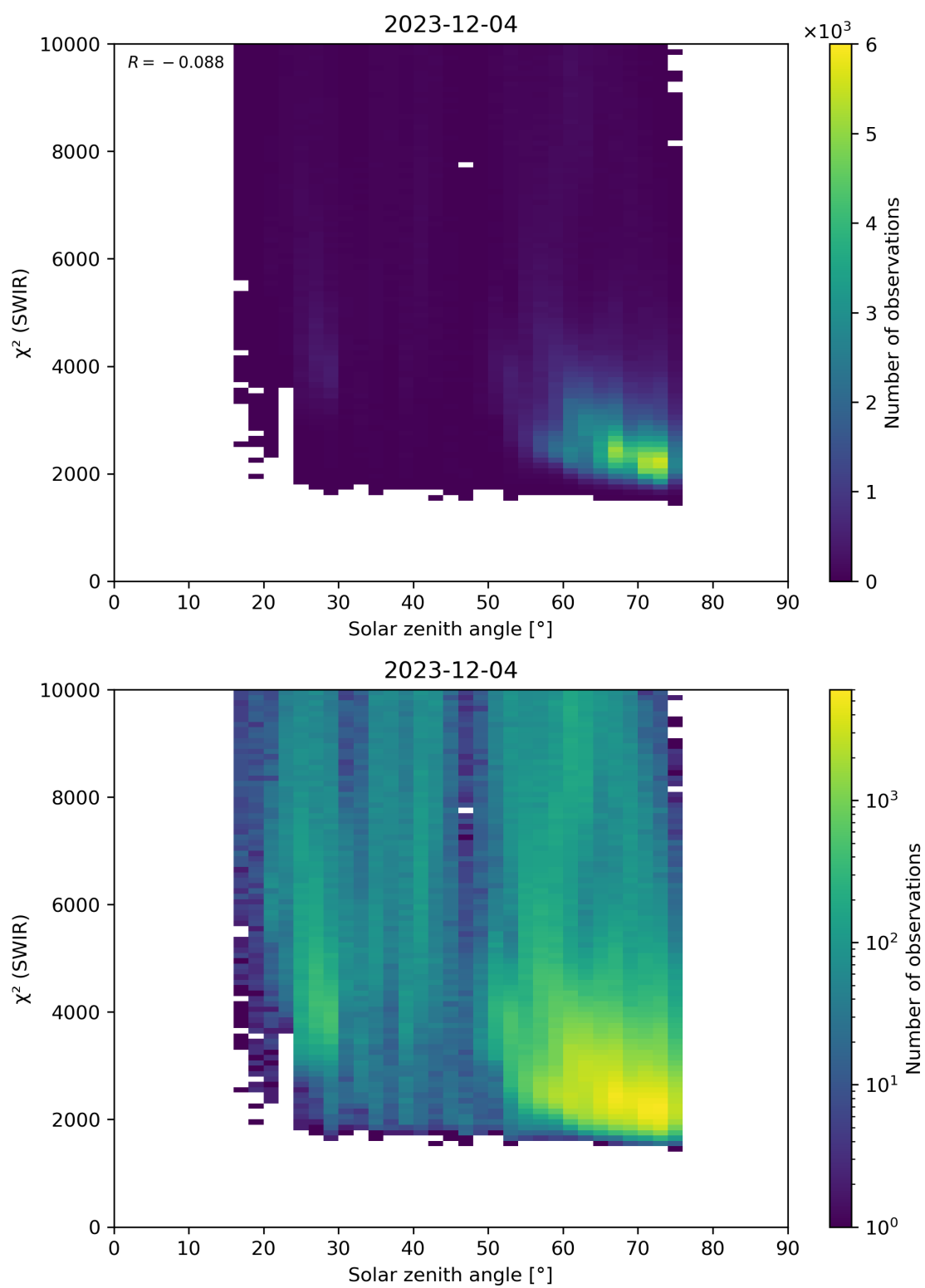
Figure 95: Scatter density plot of “Solar zenith angle” against “ \chi^2 (SWIR)” for 2023-12-04 to 2023-12-05.
