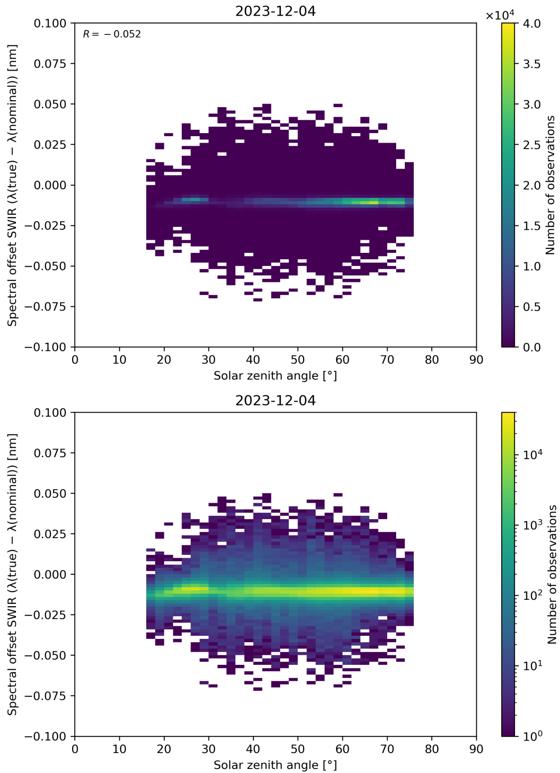
Figure 104: Scatter density plot of “Solar zenith angle” against “Spectral offset SWIR ( \lambda(\text{true}) - \lambda(\text{nominal}) )” for 2023-12-04 to 2023-12-05.
