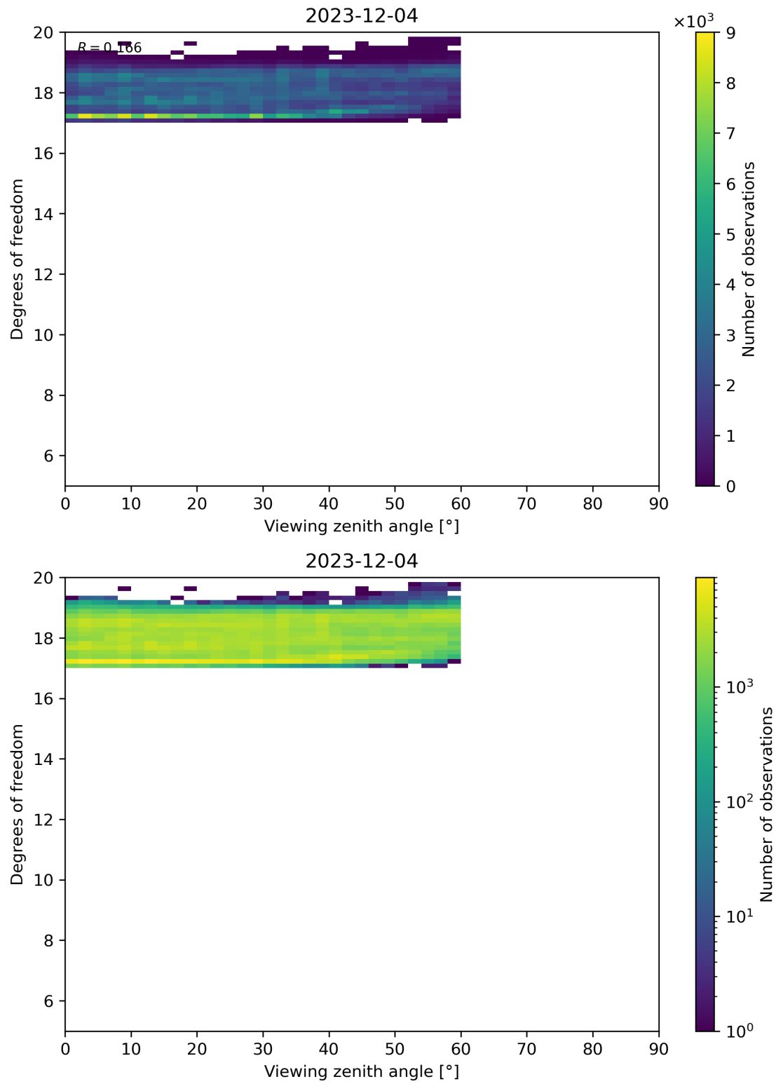
Figure 107: Scatter density plot of “Viewing zenith angle” against “Degrees of freedom” for 2023-12-04 to 2023-12-05.
