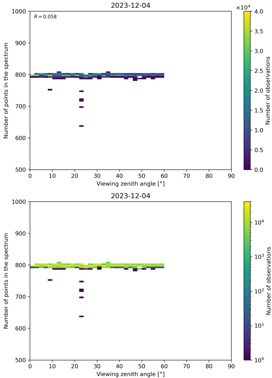
Figure 114: Scatter density plot of “Viewing zenith angle” against “Number of points in the spectrum” for 2023-12-04 to 2023-12-05.
