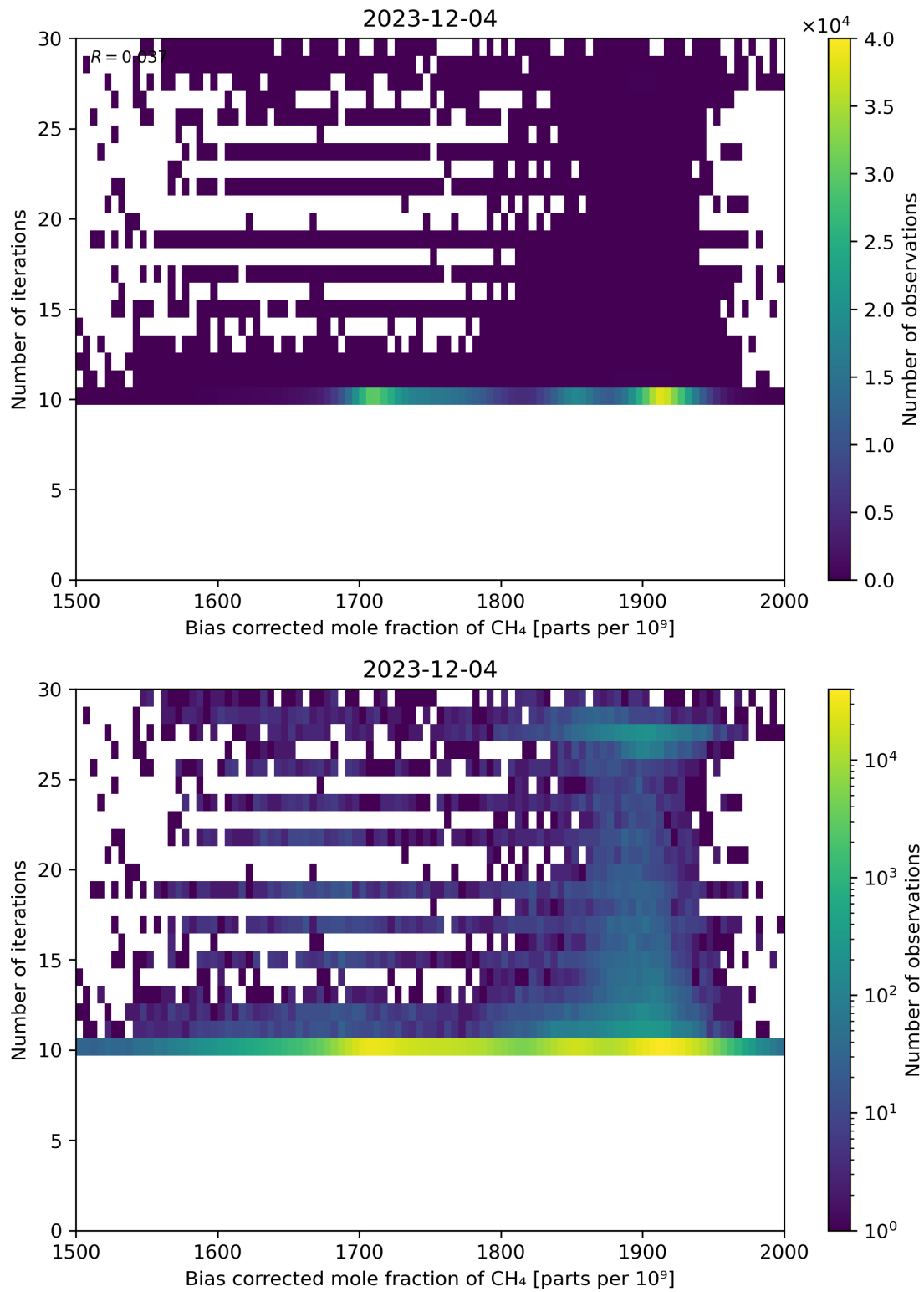
Figure 67: Scatter density plot of “Bias corrected mole fraction of \text{CH}_4 ” against “Number of iterations” for 2023-12-04 to 2023-12-05.
