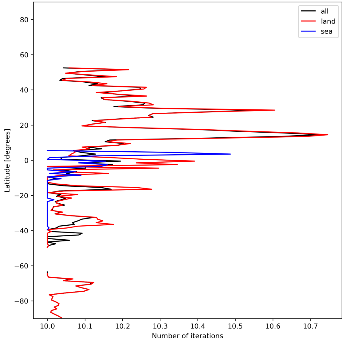
Figure 20: Zonal average of “Number of iterations” for 2023-12-04 to 2023-12-05.
