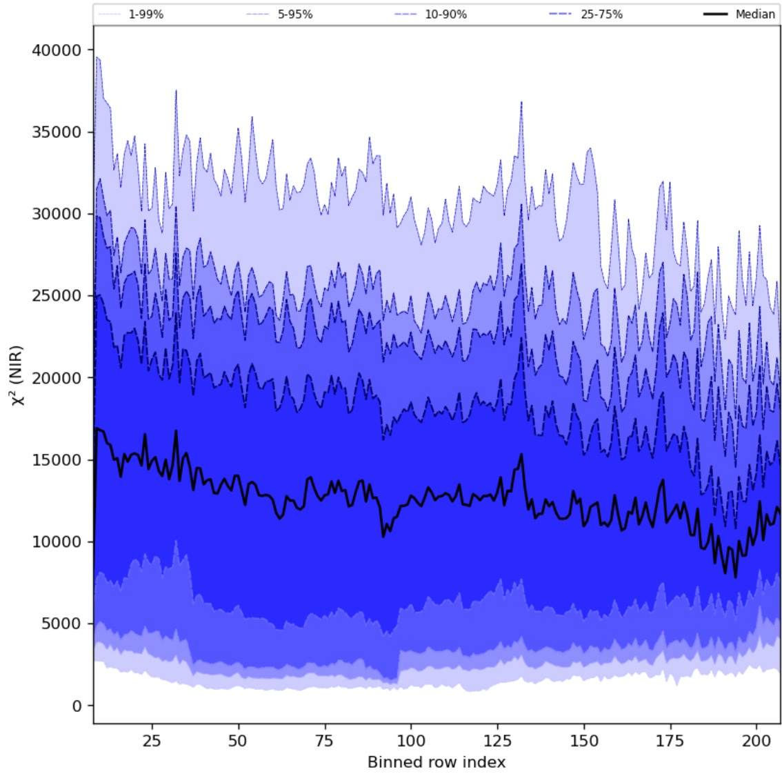
Figure 40: Along track statistics of “ \chi^2 (NIR)” for 2023-12-04 to 2023-12-05
