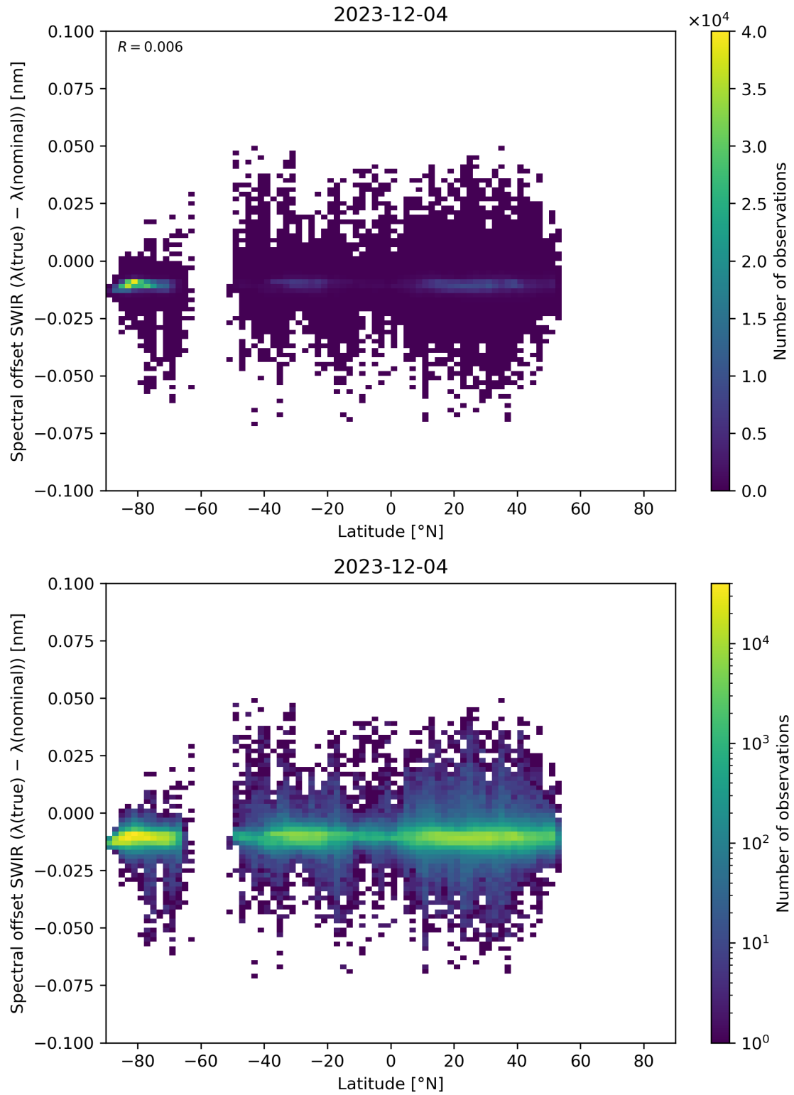
Figure 62: Scatter density plot of “Latitude” against “Spectral offset SWIR ( \lambda(\text{true}) - \lambda(\text{nominal}) )” for 2023-12-04 to 2023-12-05.
