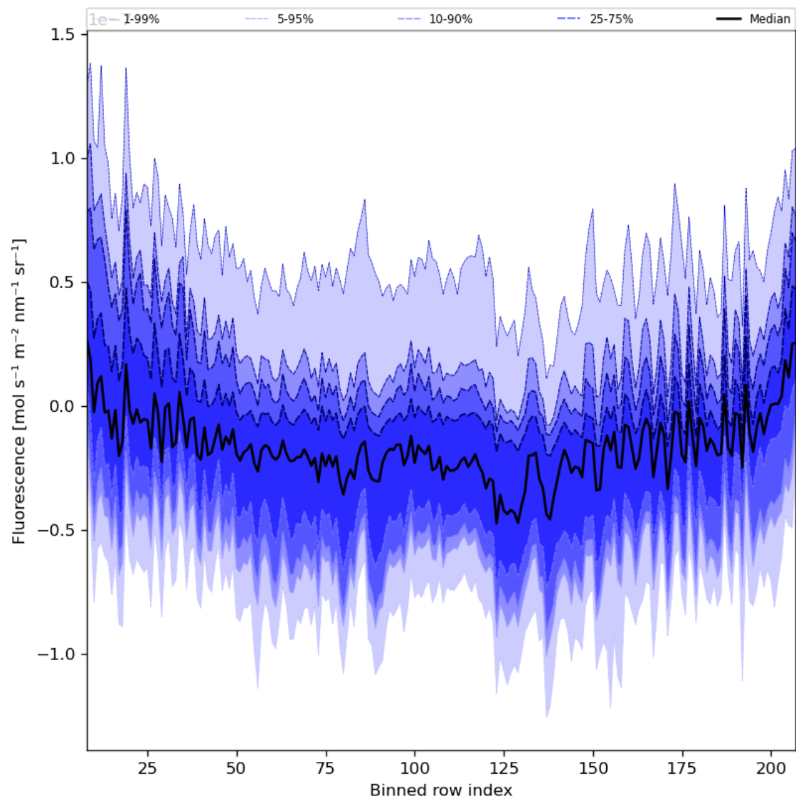
Figure 43: Along track statistics of “Fluorescence” for 2023-12-04 to 2023-12-05
