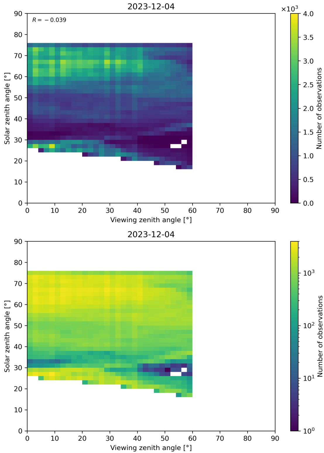
Figure 115: Scatter density plot of “Viewing zenith angle” against “Solar zenith angle” for 2023-12-04 to 2023-12-05.
