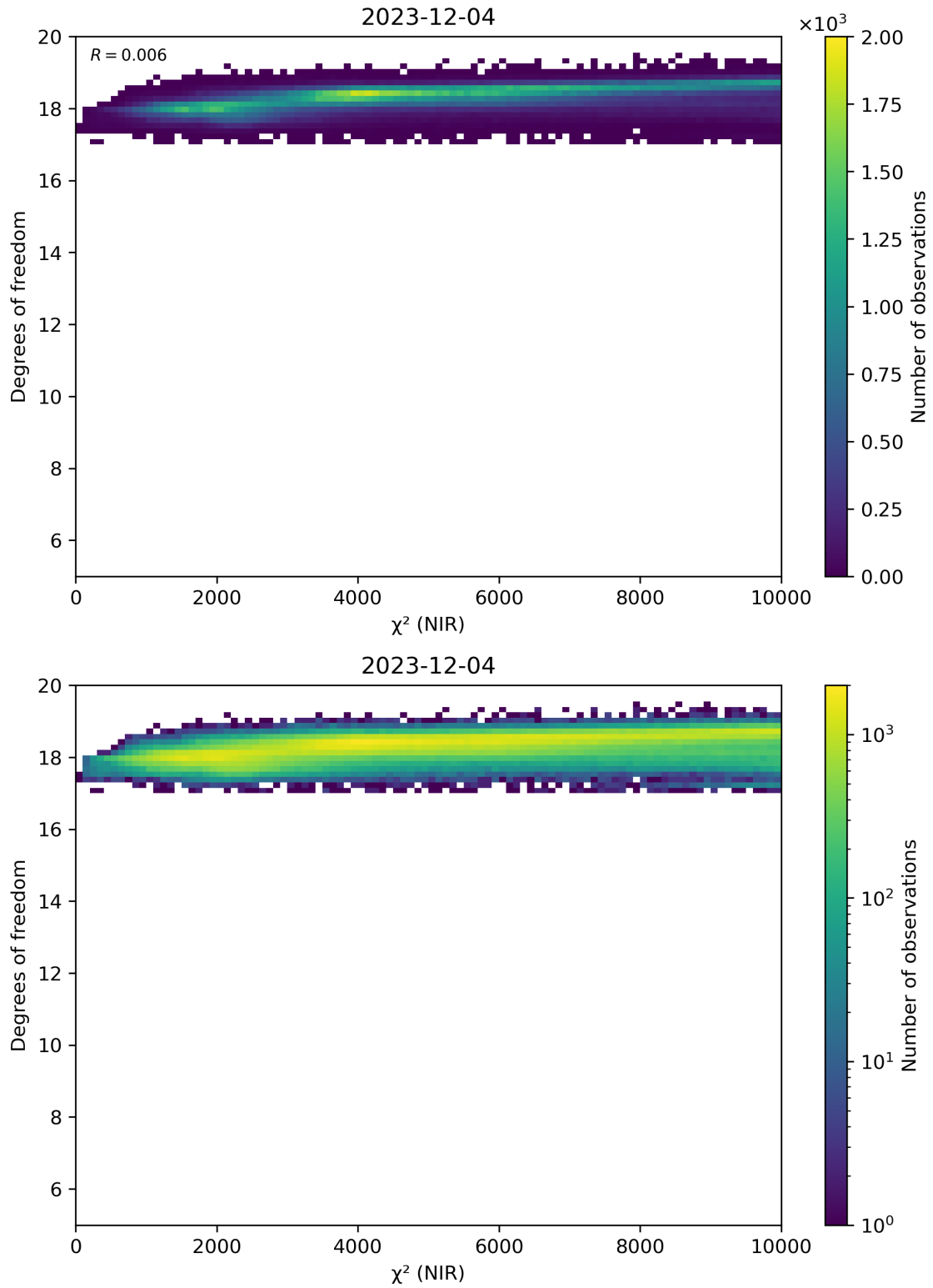
Figure 44: Scatter density plot of “ \chi^2 (NIR)” against “Degrees of freedom” for 2023-12-04 to 2023-12-05.
