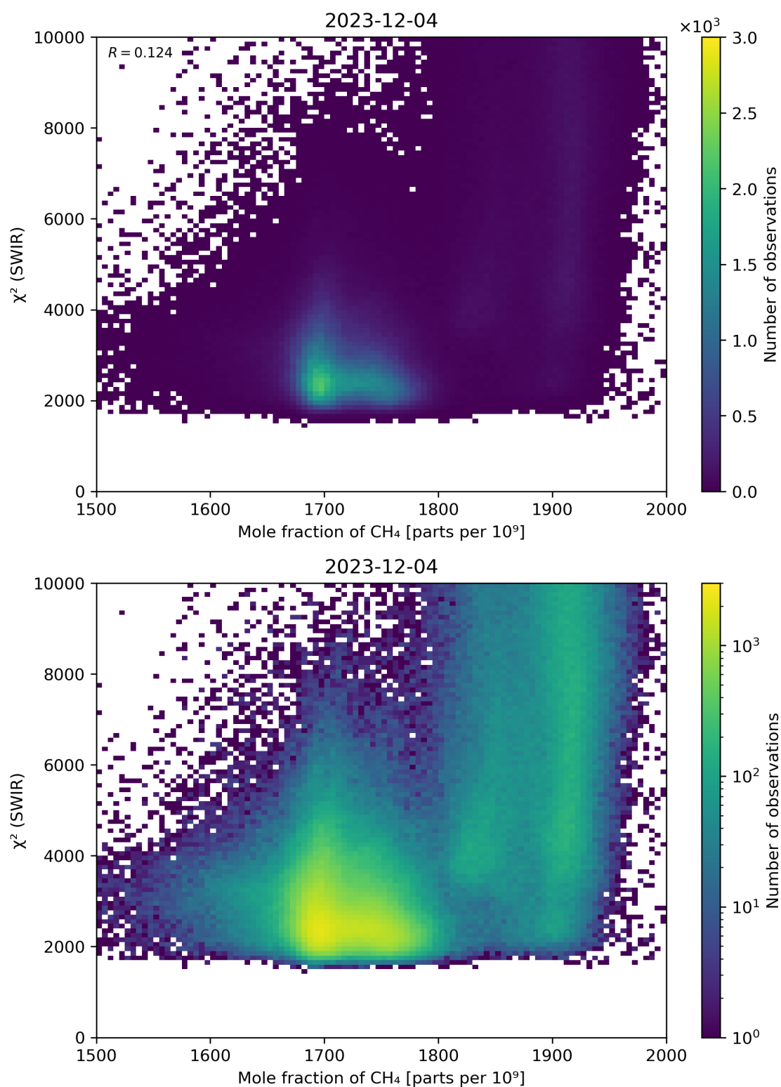
Figure 71: Scatter density plot of “Mole fraction of \text{CH}_4 ” against “ \chi^2 (SWIR)” for 2023-12-04 to 2023-12-05.
