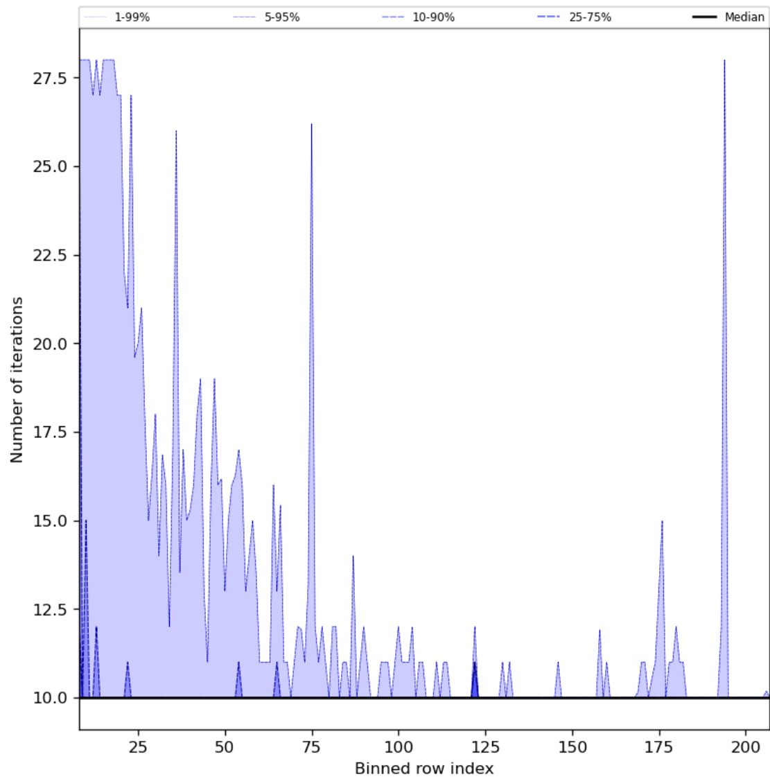
Figure 42: Along track statistics of “Number of iterations” for 2023-12-04 to 2023-12-05
