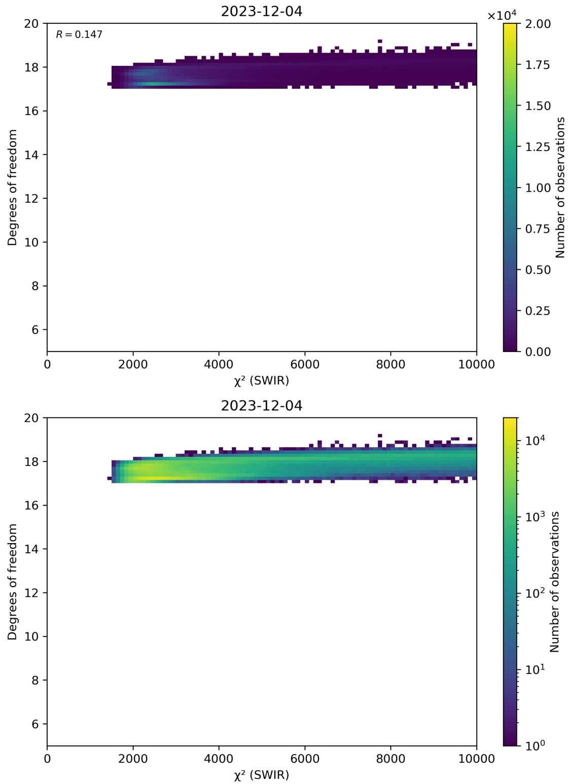
Figure 48: Scatter density plot of “ \chi^2 (SWIR)” against “Degrees of freedom” for 2023-12-04 to 2023-12-05.
