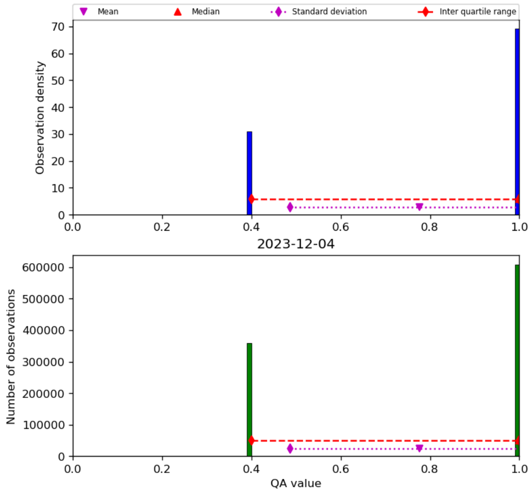
Figure 22: Histogram of “QA value” for 2023-12-04 to 2023-12-05
