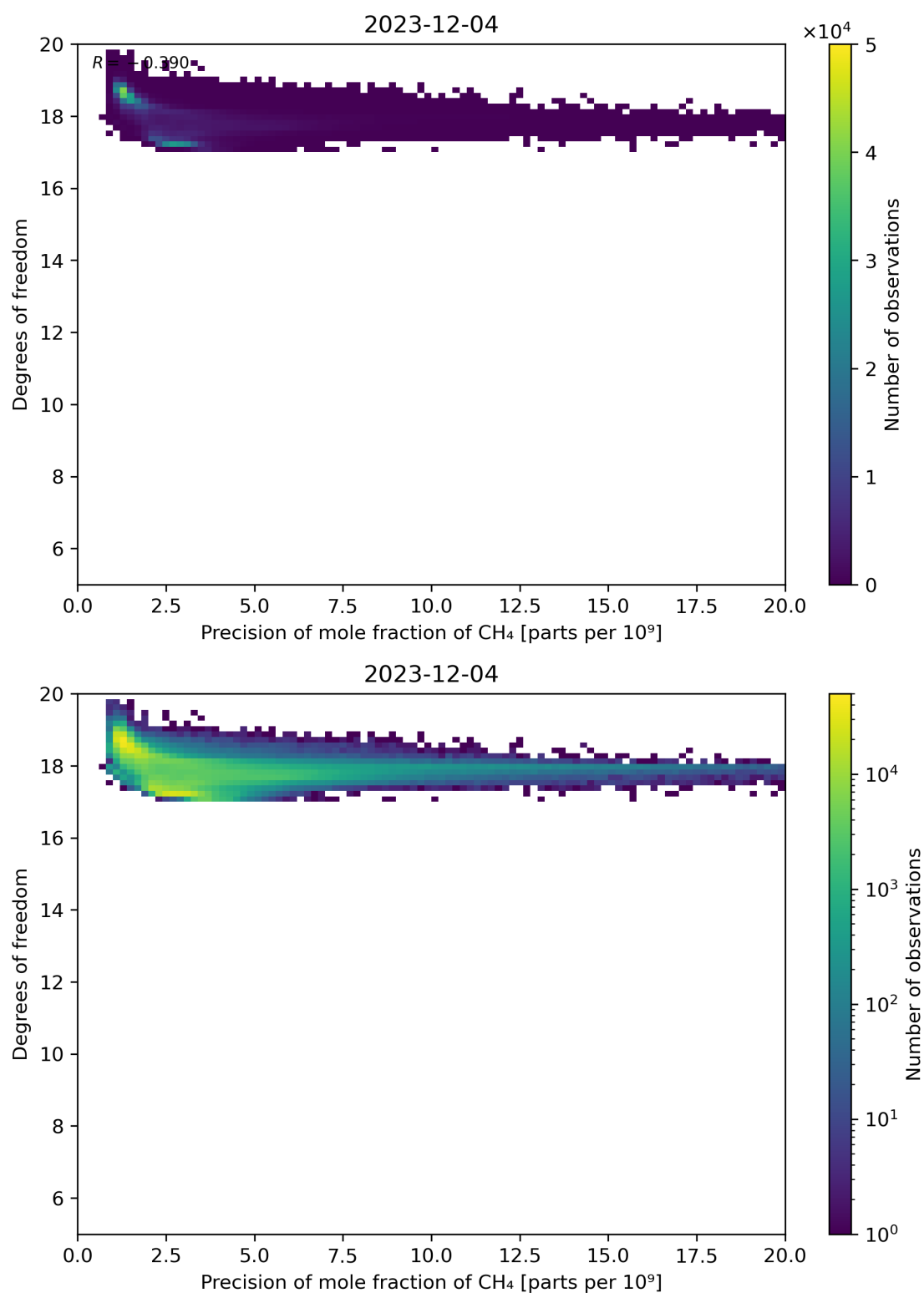
Figure 80: Scatter density plot of “Precision of mole fraction of CH 4 ” against “Degrees of freedom” for 2023-12-04 to 2023-12-05.
