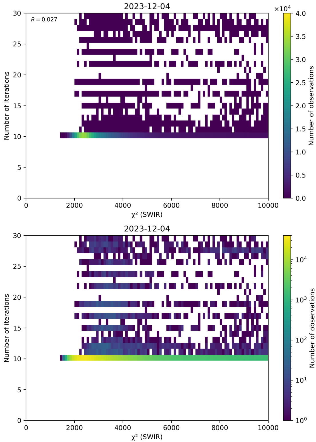
Figure 50: Scatter density plot of “ \chi^2 (SWIR)” against “Number of iterations” for 2023-12-04 to 2023-12-05.
