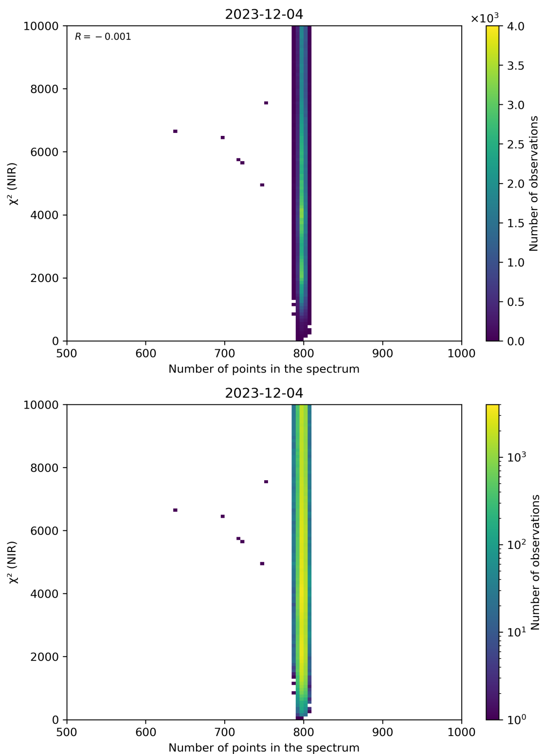
Figure 88: Scatter density plot of “Number of points in the spectrum” against “ \chi^2 (NIR)” for 2023-12-04 to 2023-12-05.
