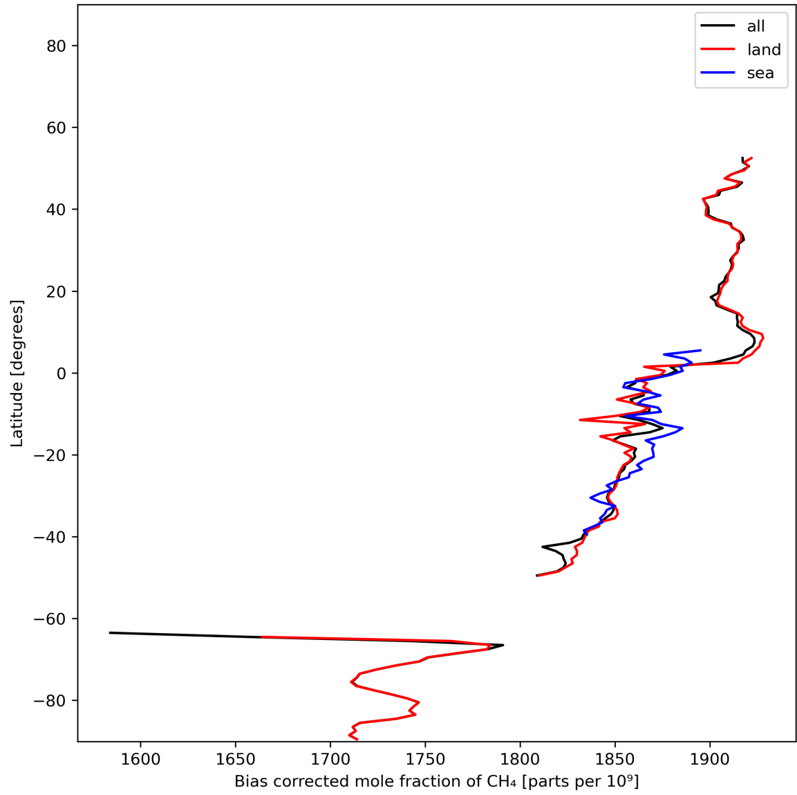
Figure 14: Zonal average of “Bias corrected mole fraction of \text{CH}_4 ” for 2023-12-04 to 2023-12-05.
