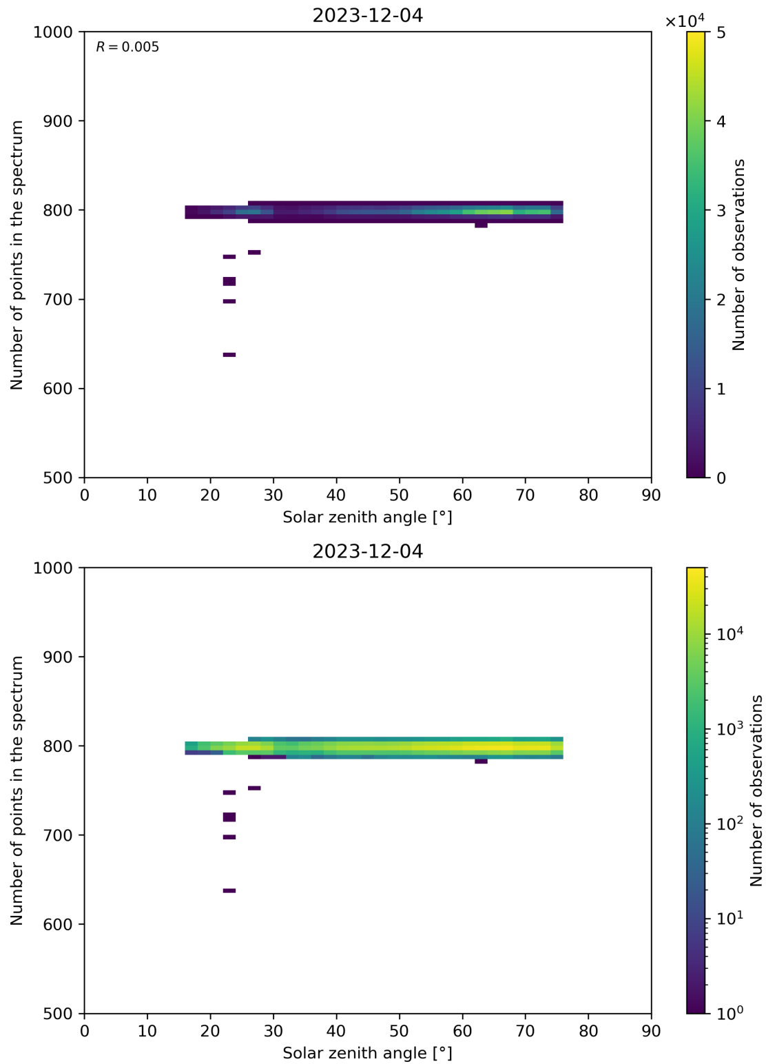
Figure 103: Scatter density plot of “Solar zenith angle” against “Number of points in the spectrum” for 2023-12-04 to 2023-12-05.
