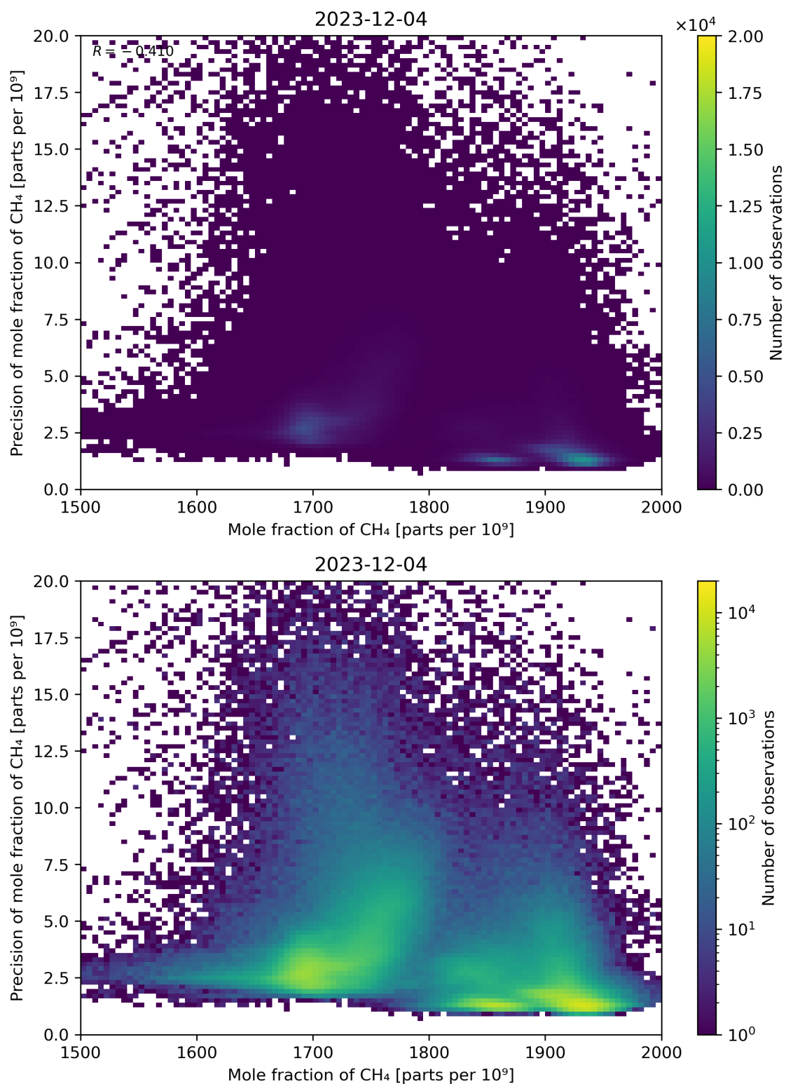
Figure 75: Scatter density plot of “Mole fraction of CH 4 ” against “Precision of mole fraction of CH 4 ” for 2023-12-04 to 2023-12-05.
