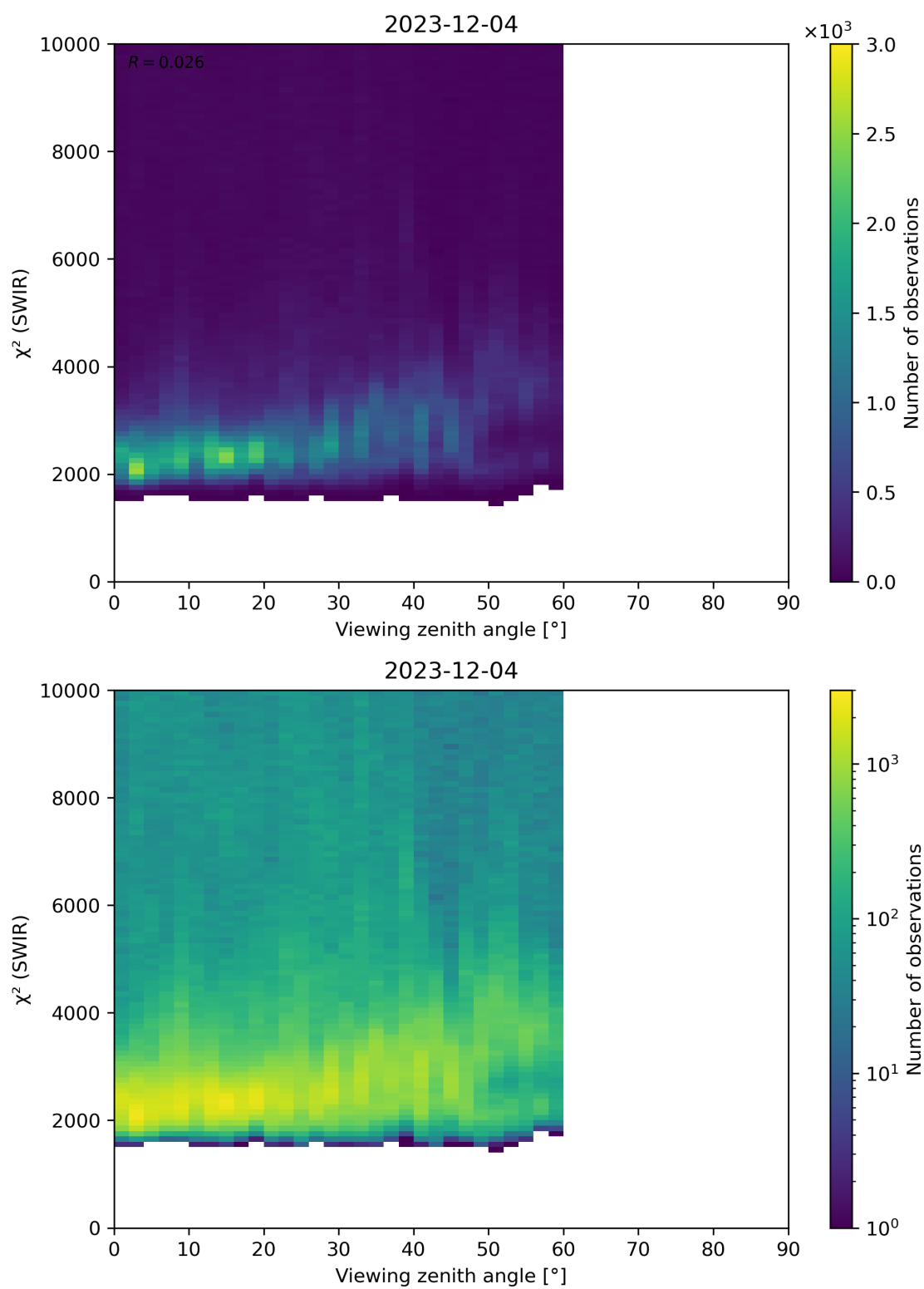
Figure 106: Scatter density plot of “Viewing zenith angle” against “ \chi^2 (SWIR)” for 2023-12-04 to 2023-12-05.
