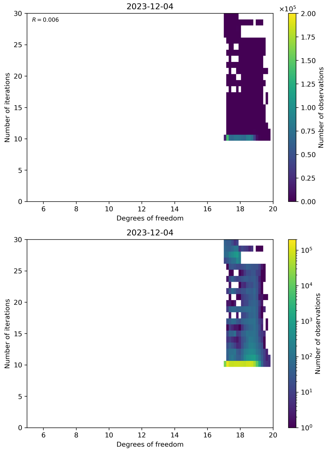
Figure 52: Scatter density plot of “Degrees of freedom” against “Number of iterations” for 2023-12-04 to 2023-12-05.
