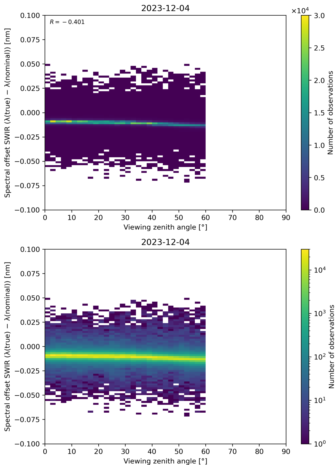
Figure 116: Scatter density plot of “Viewing zenith angle” against “Spectral offset SWIR ( \lambda(\text{true}) - \lambda(\text{nominal}) )” for 2023-12-04 to 2023-12-05.
