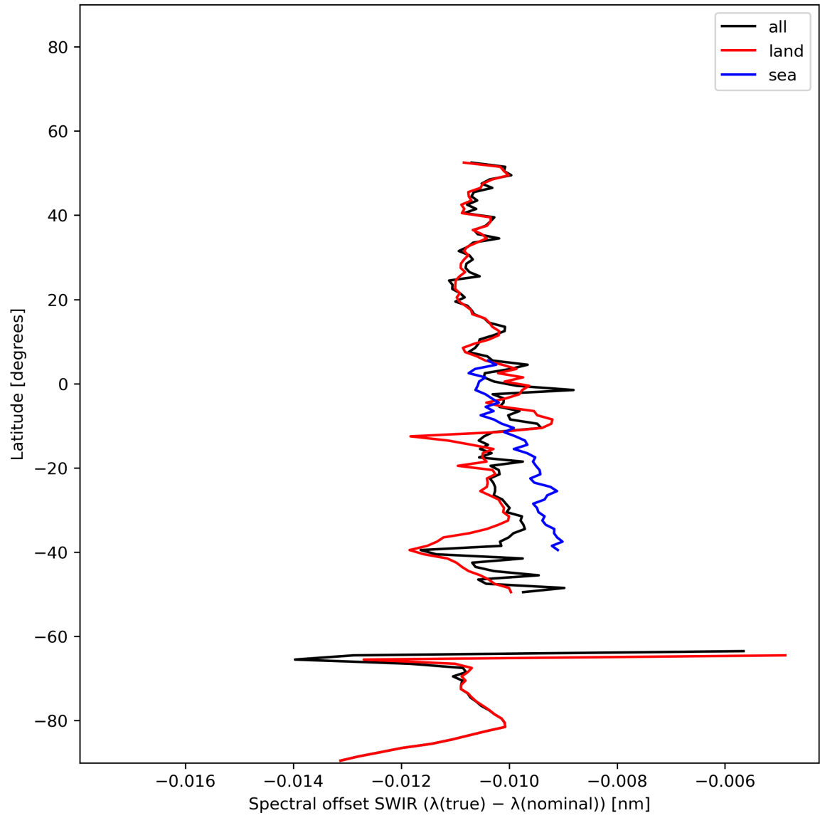
Figure 16: Zonal average of “Spectral offset SWIR ( \lambda(\text{true}) - \lambda(\text{nominal}) )” for 2023-12-04 to 2023-12-05.
