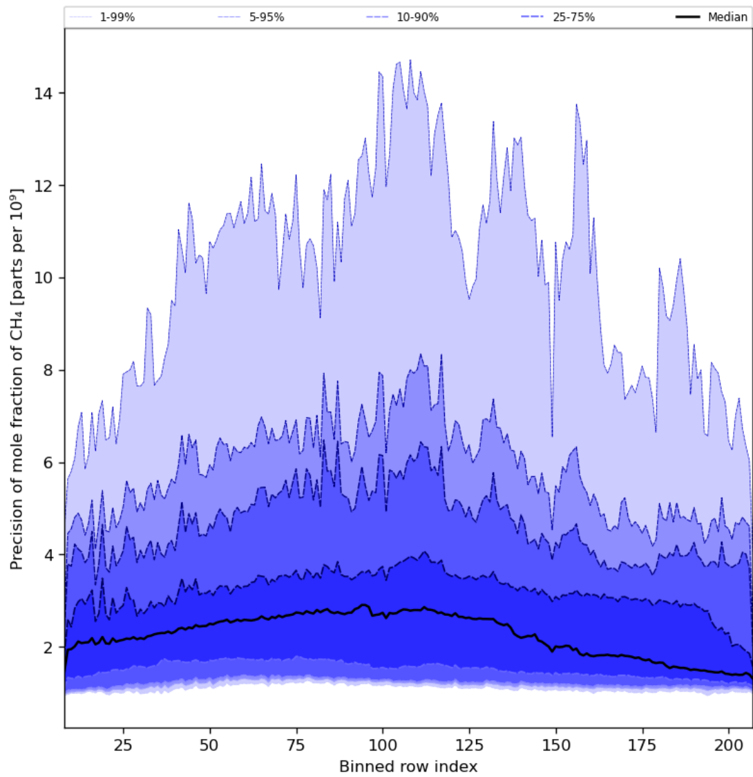
Figure 35: Along track statistics of “Precision of mole fraction of \text{CH}_4 ” for 2023-12-04 to 2023-12-05
