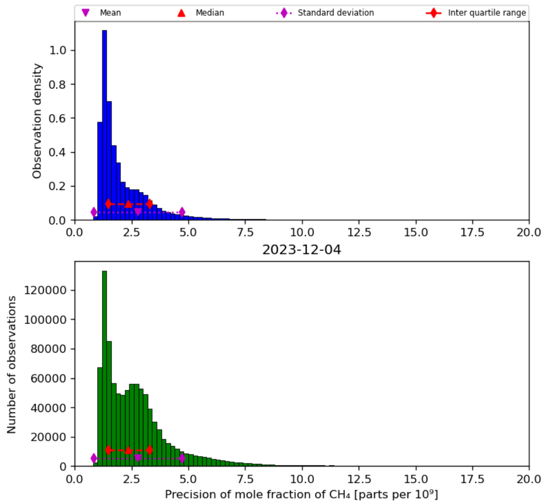
Figure 24: Histogram of “Precision of mole fraction of CH 4 ” for 2023-12-04 to 2023-12-05
