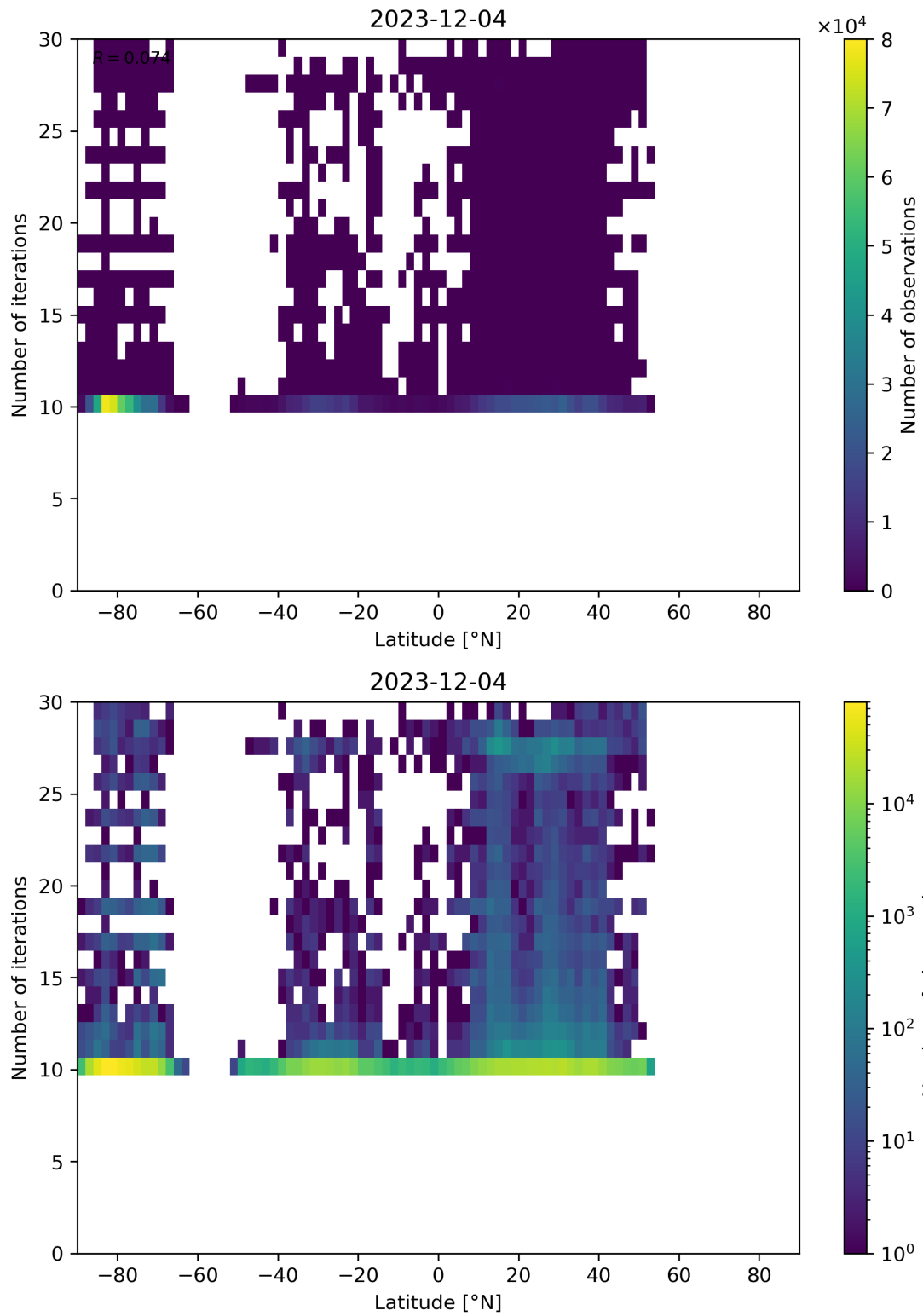
Figure 60: Scatter density plot of “Latitude” against “Number of iterations” for 2023-12-04 to 2023-12-05.
