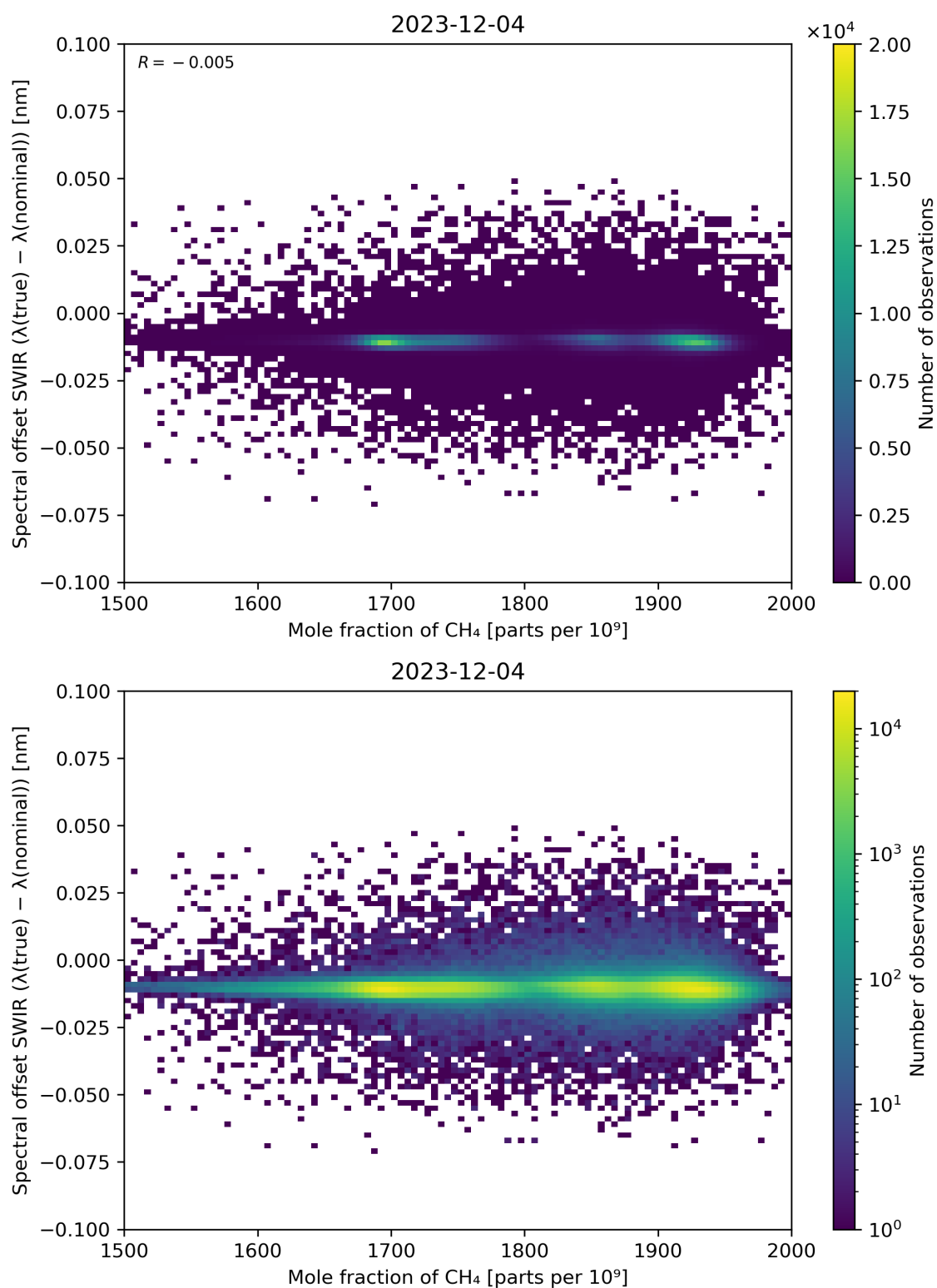
Figure 86: Scatter density plot of “Mole fraction of CH 4 ” against “Spectral offset SWIR ( \lambda(\text{true}) - \lambda(\text{nominal}) )” for 2023-12-04 to 2023-12-05.
