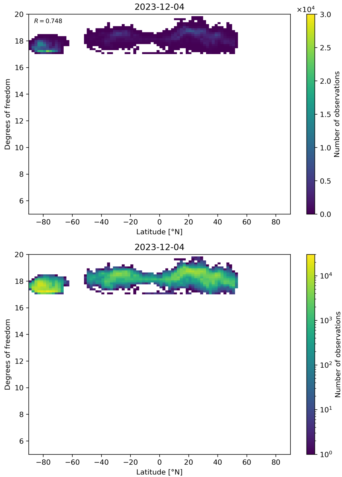
Figure 55: Scatter density plot of “Latitude” against “Degrees of freedom” for 2023-12-04 to 2023-12-05.
