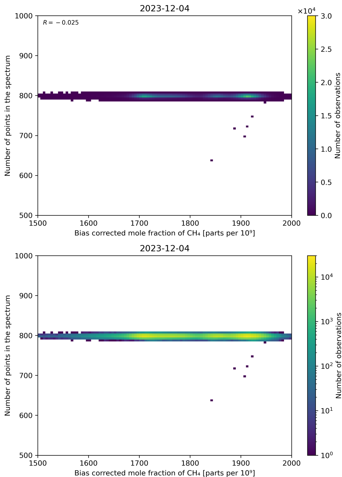
Figure 68: Scatter density plot of “Bias corrected mole fraction of CH 4 ” against “Number of points in the spectrum” for 2023-12-04 to 2023-12-05.
