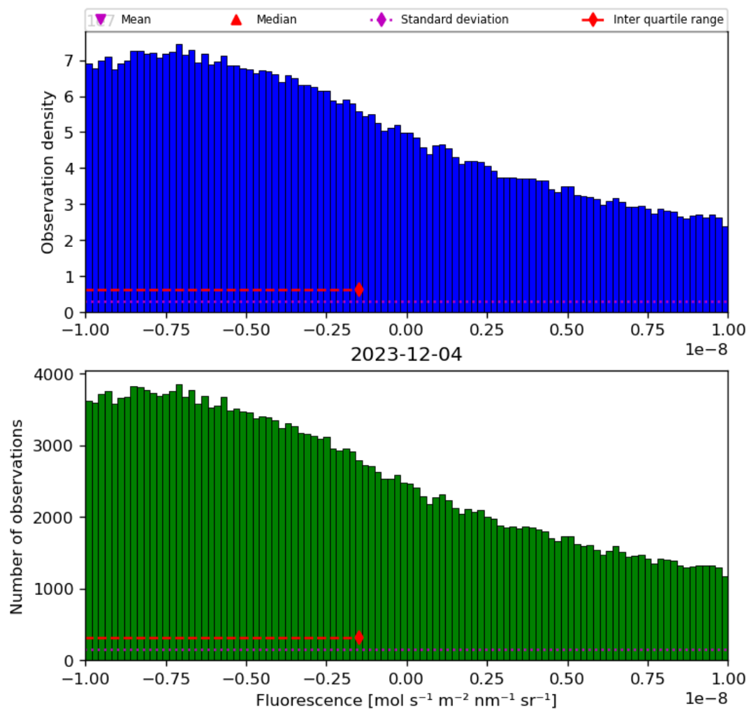
Figure 32: Histogram of “Fluorescence” for 2023-12-04 to 2023-12-05
