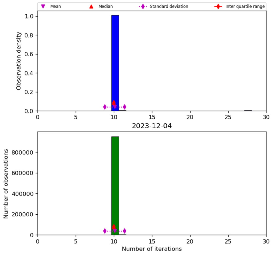
Figure 31: Histogram of “Number of iterations” for 2023-12-04 to 2023-12-05
