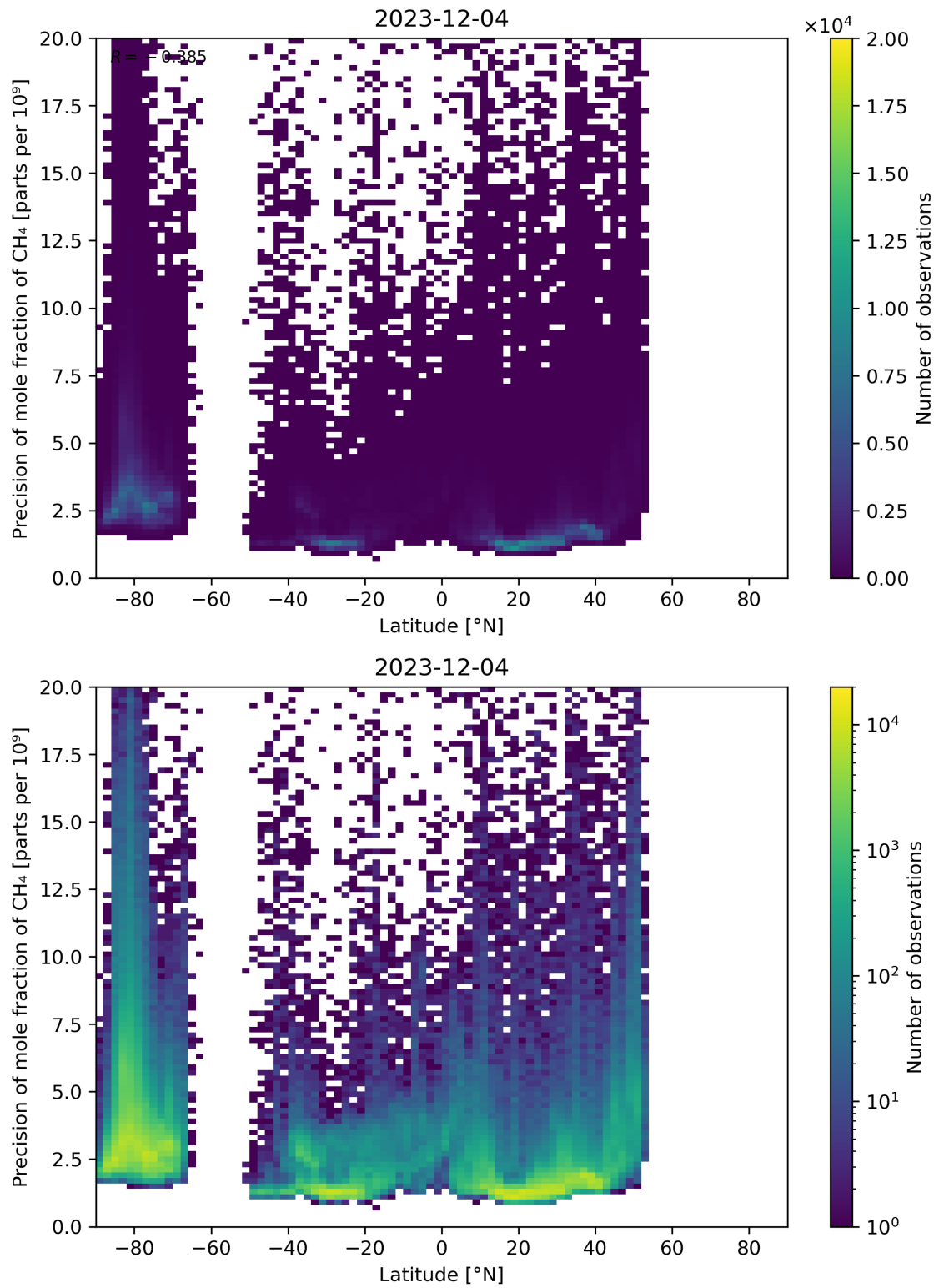
Figure 59: Scatter density plot of “Latitude” against “Precision of mole fraction of CH 4 ” for 2023-12-04 to 2023-12-05.
