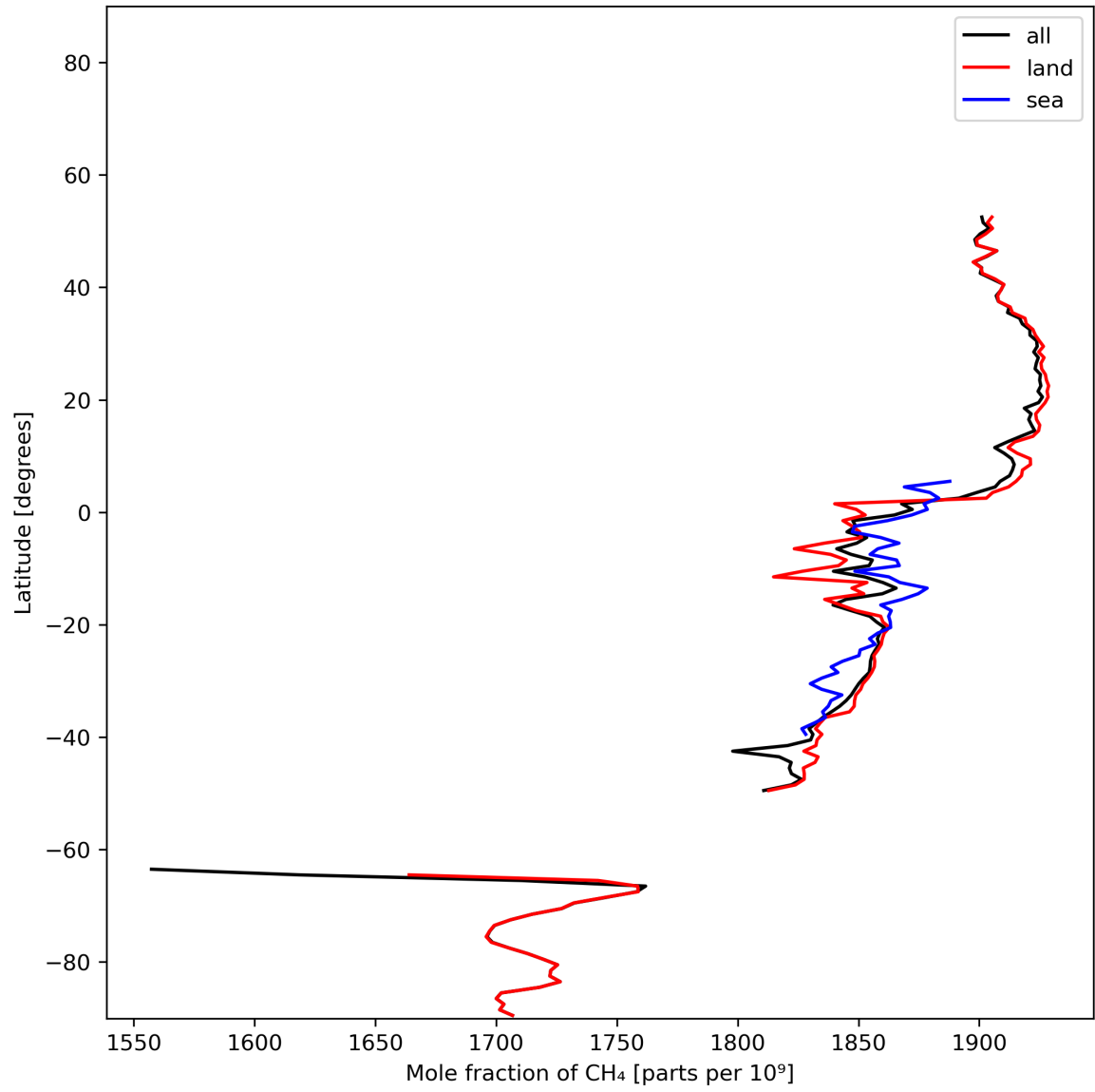
Figure 12: Zonal average of “Mole fraction of \text{CH}_4 ” for 2023-12-04 to 2023-12-05.
