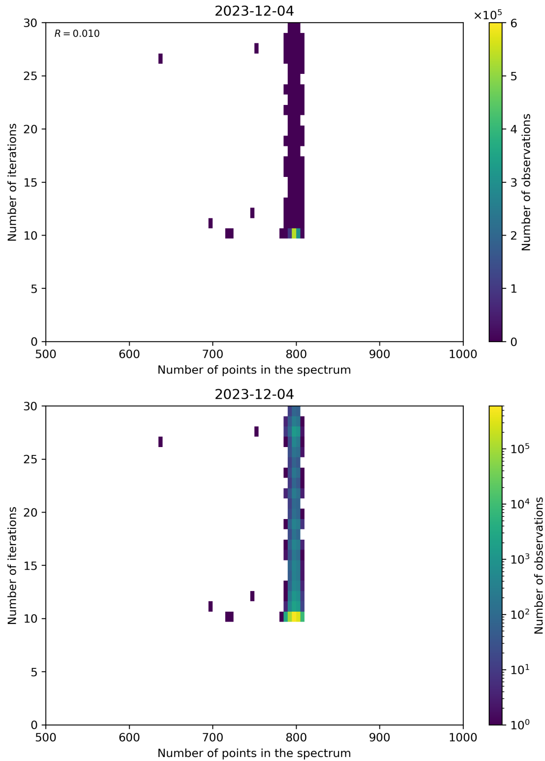
Figure 92: Scatter density plot of “Number of points in the spectrum” against “Number of iterations” for 2023-12-04 to 2023-12-05.
