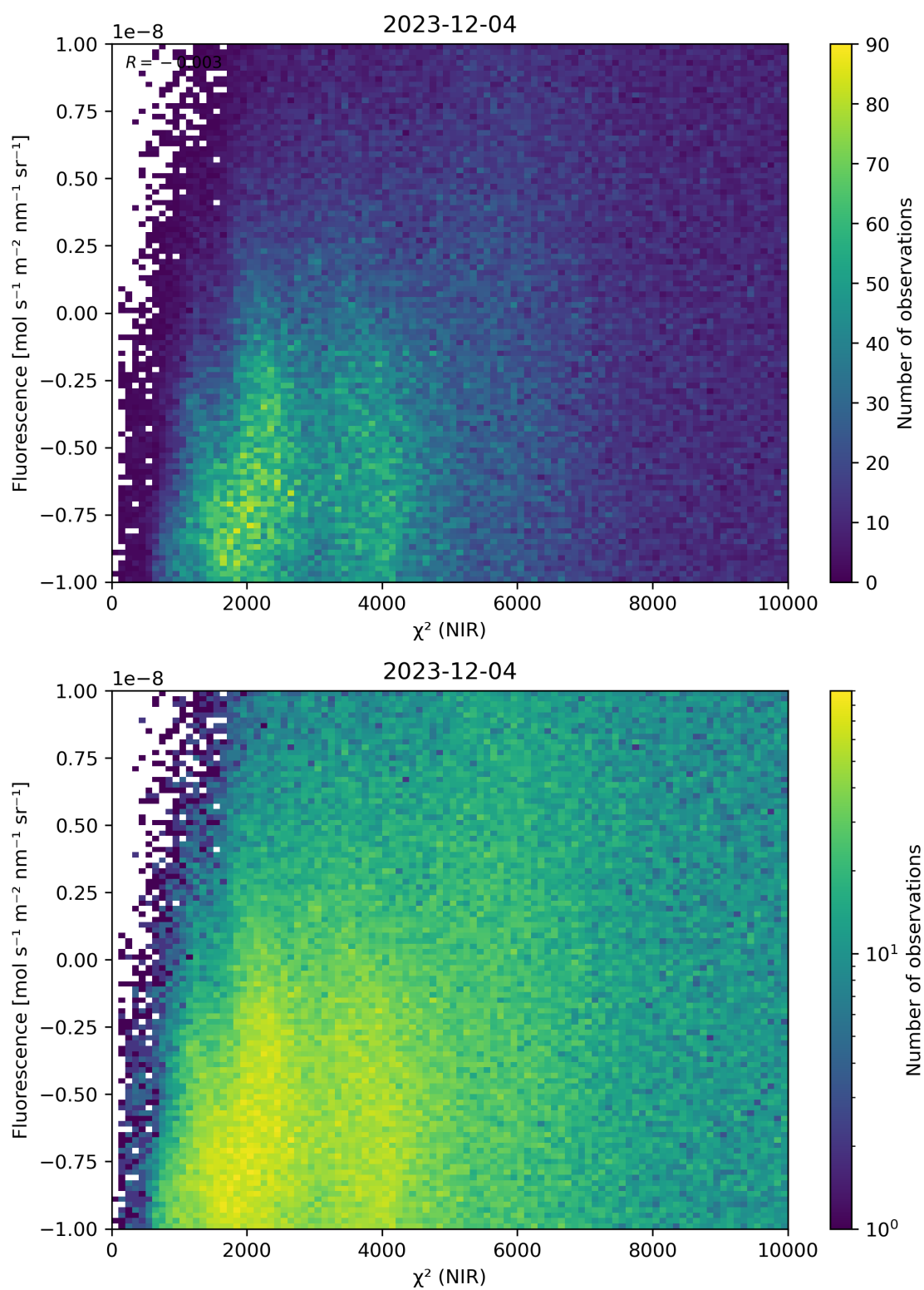
Figure 45: Scatter density plot of “ \chi^2 (NIR)” against “Fluorescence” for 2023-12-04 to 2023-12-05.
