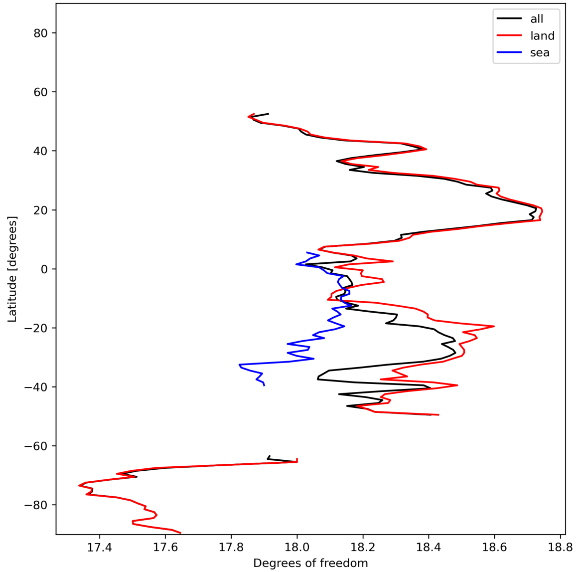
Figure 19: Zonal average of “Degrees of freedom” for 2023-12-04 to 2023-12-05.
