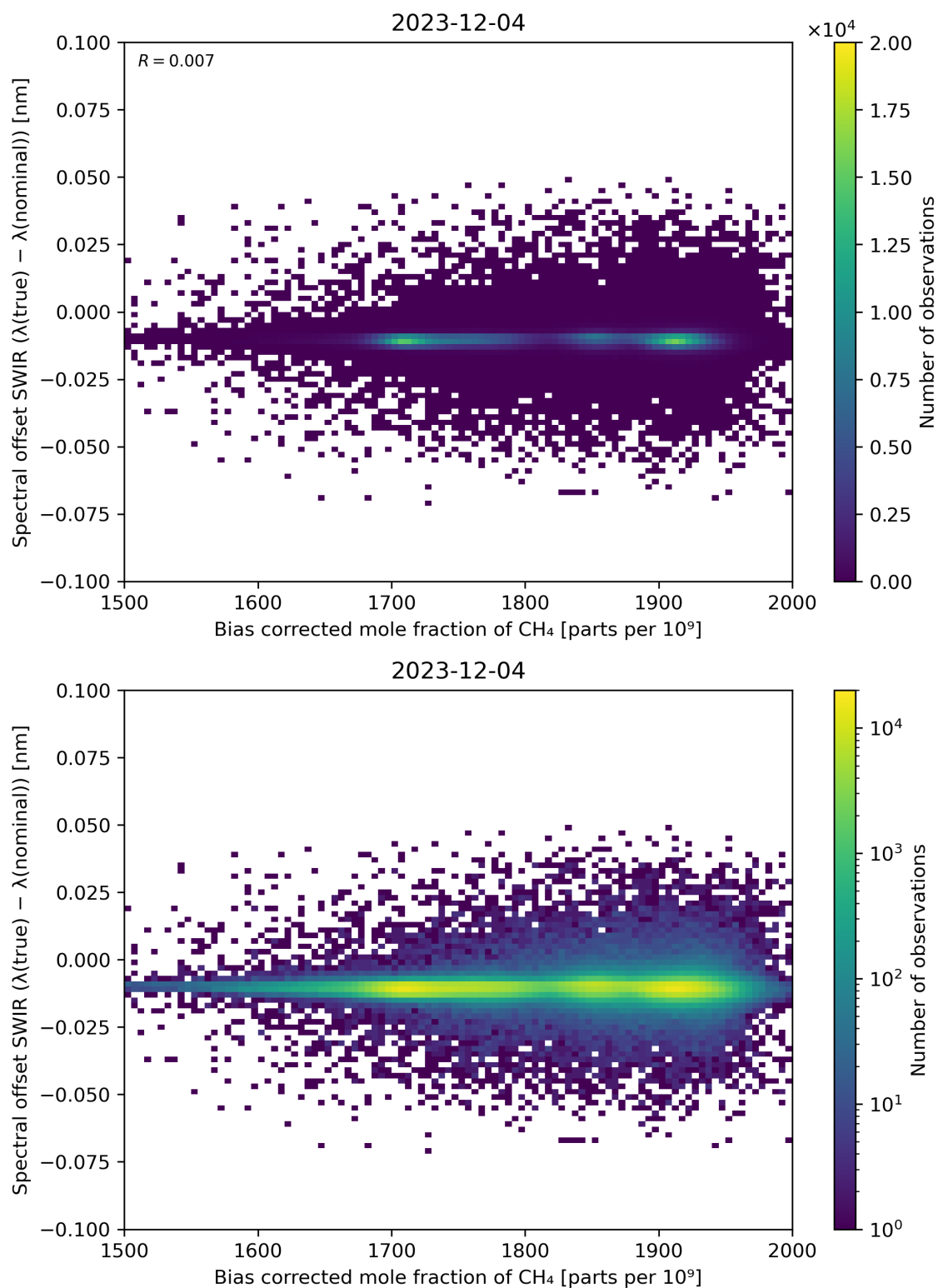
Figure 69: Scatter density plot of “Bias corrected mole fraction of \text{CH}_4 ” against “Spectral offset SWIR ( \lambda(\text{true}) - \lambda(\text{nominal}) )” for 2023-12-04 to 2023-12-05.
