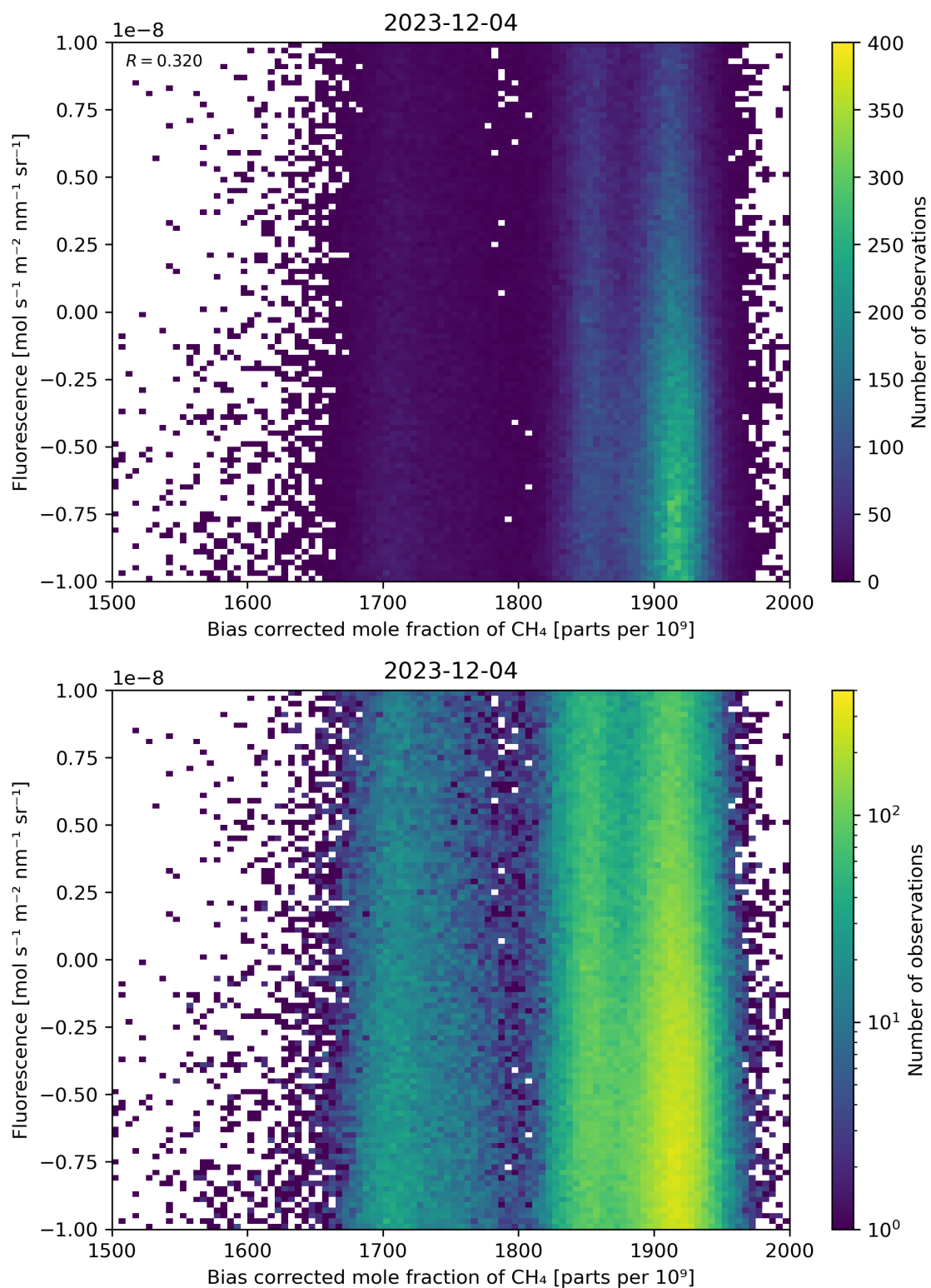
Figure 66: Scatter density plot of “Bias corrected mole fraction of \text{CH}_4 ” against “Fluorescence” for 2023-12-04 to 2023-12-05.
