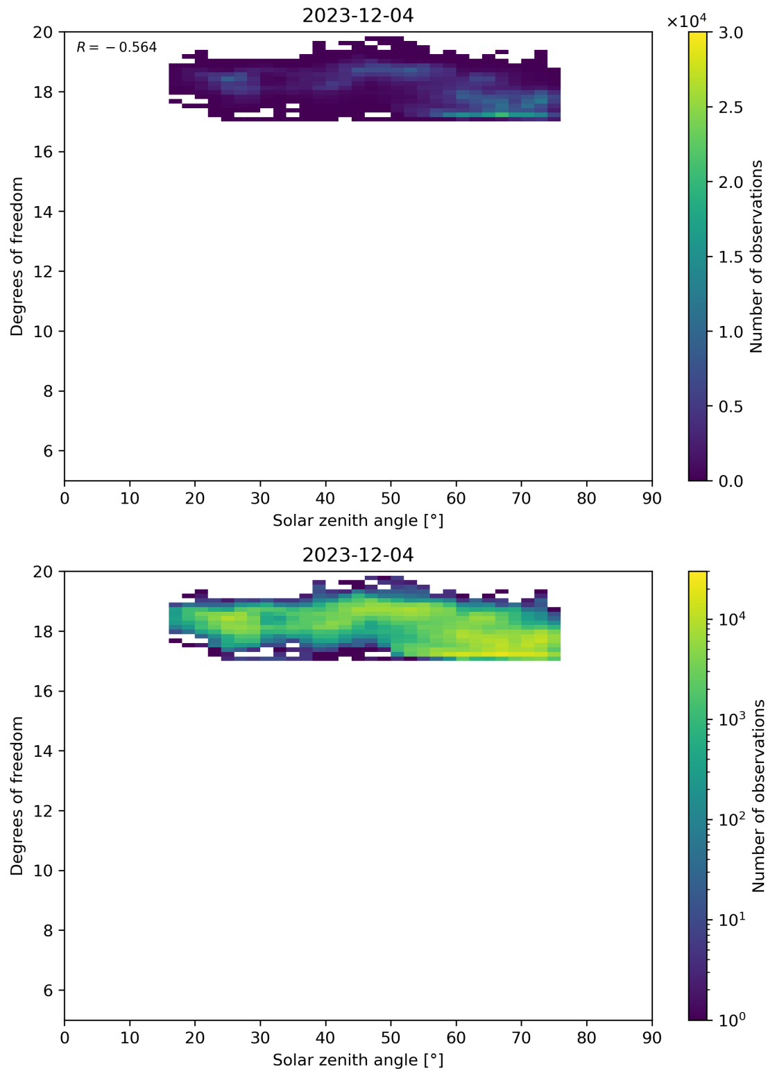
Figure 96: Scatter density plot of “Solar zenith angle” against “Degrees of freedom” for 2023-12-04 to 2023-12-05.
