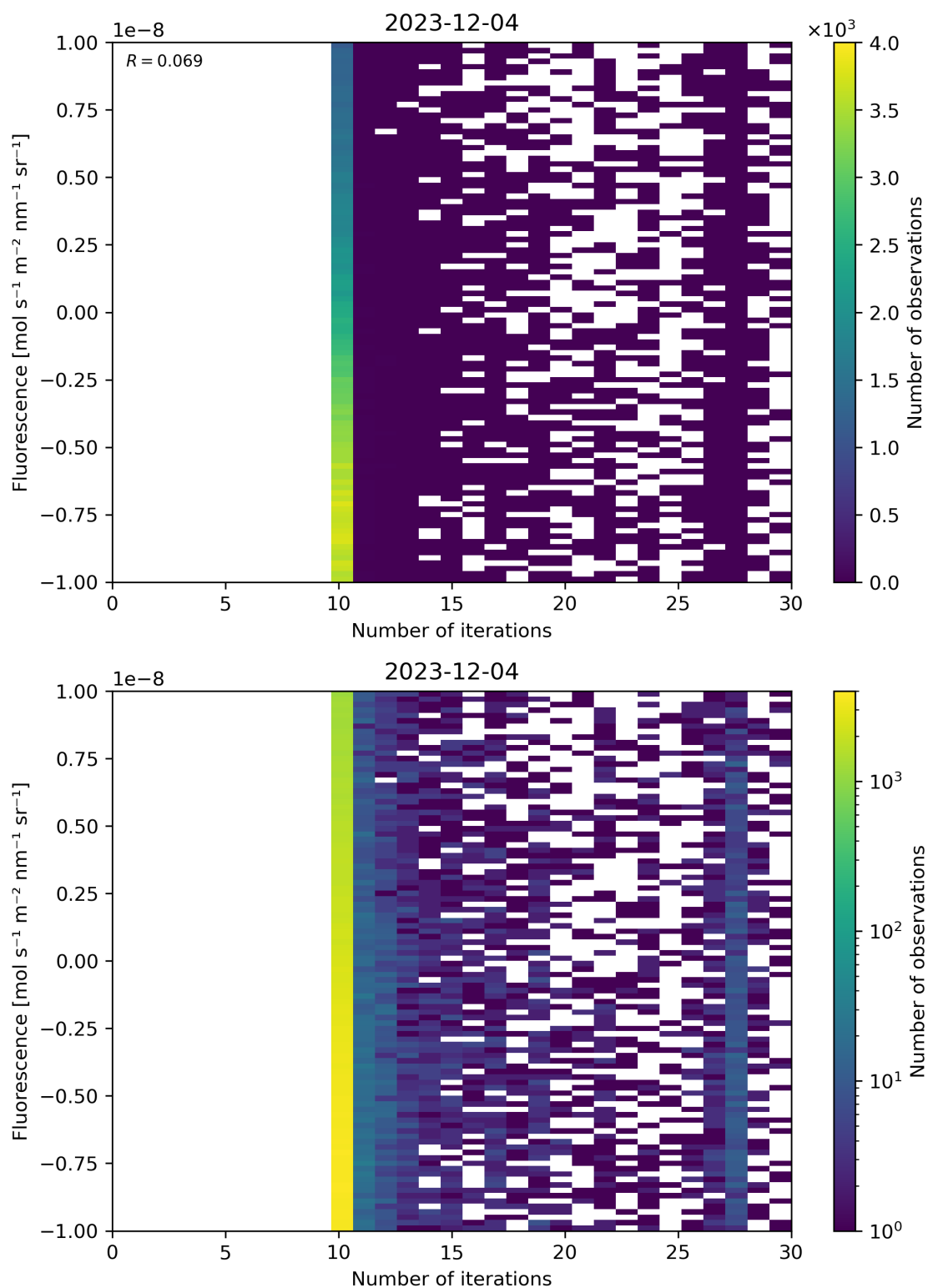
Figure 87: Scatter density plot of “Number of iterations” against “Fluorescence” for 2023-12-04 to 2023-12-05.
