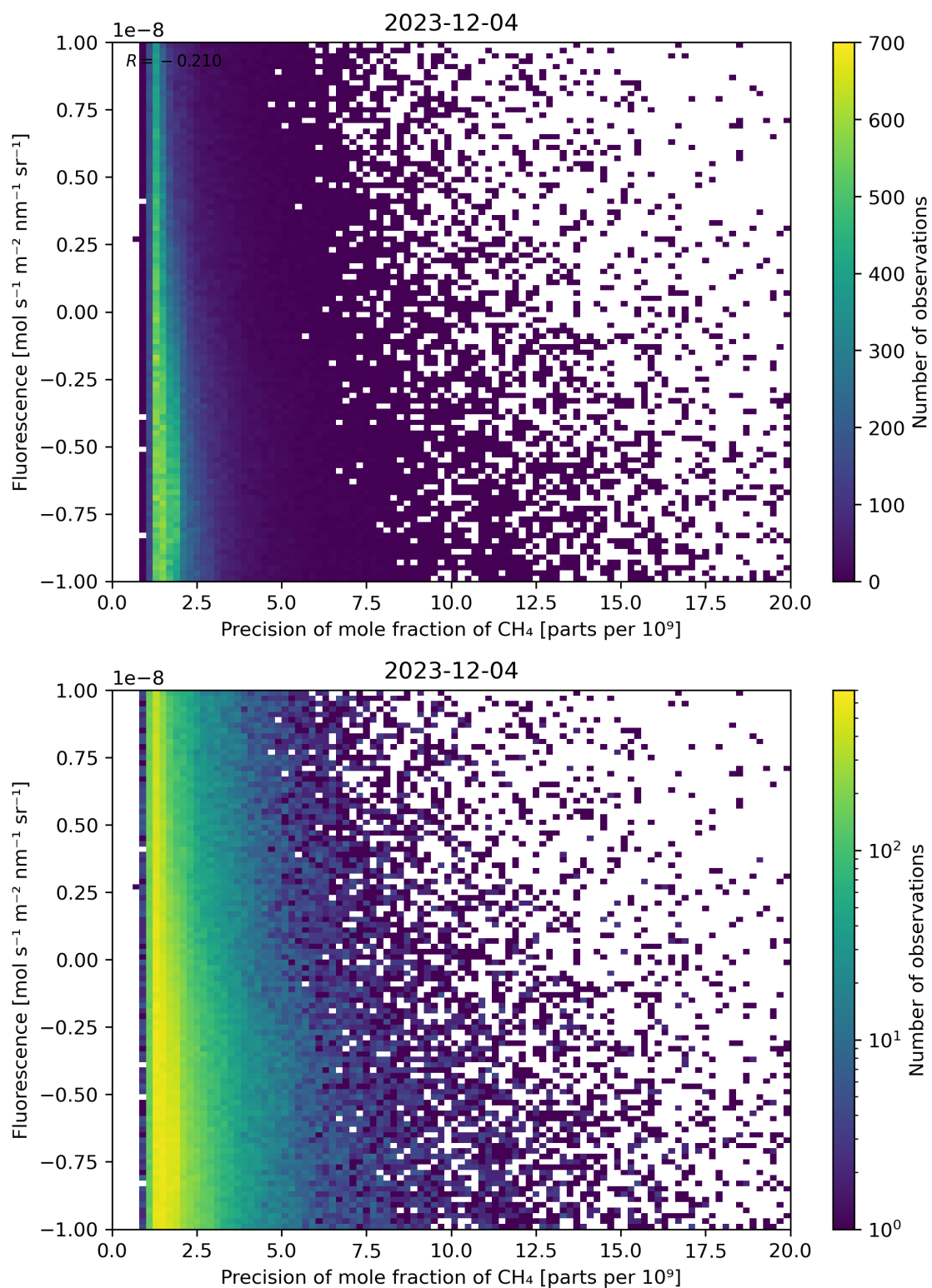
Figure 81: Scatter density plot of “Precision of mole fraction of \text{CH}_4 ” against “Fluorescence” for 2023-12-04 to 2023-12-05.
