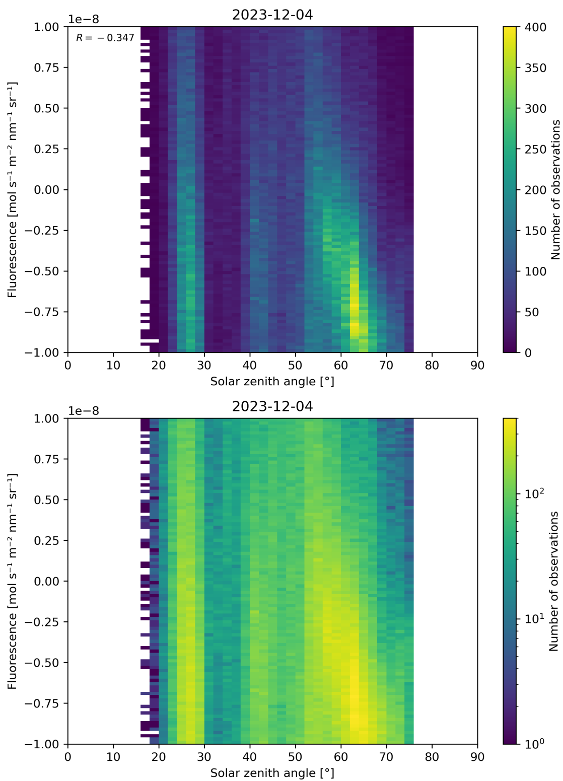
Figure 97: Scatter density plot of “Solar zenith angle” against “Fluorescence” for 2023-12-04 to 2023-12-05.
