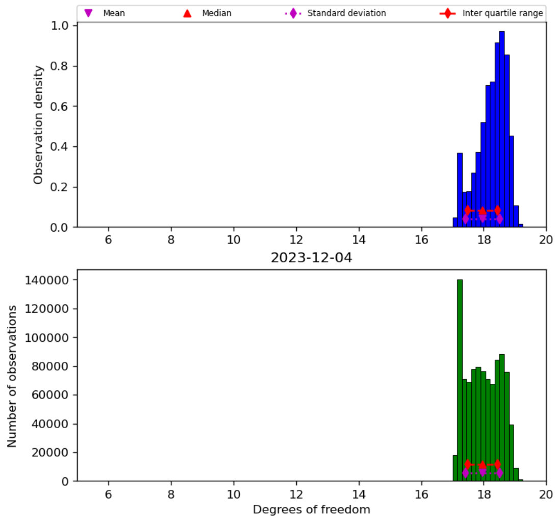
Figure 30: Histogram of “Degrees of freedom” for 2023-12-04 to 2023-12-05
