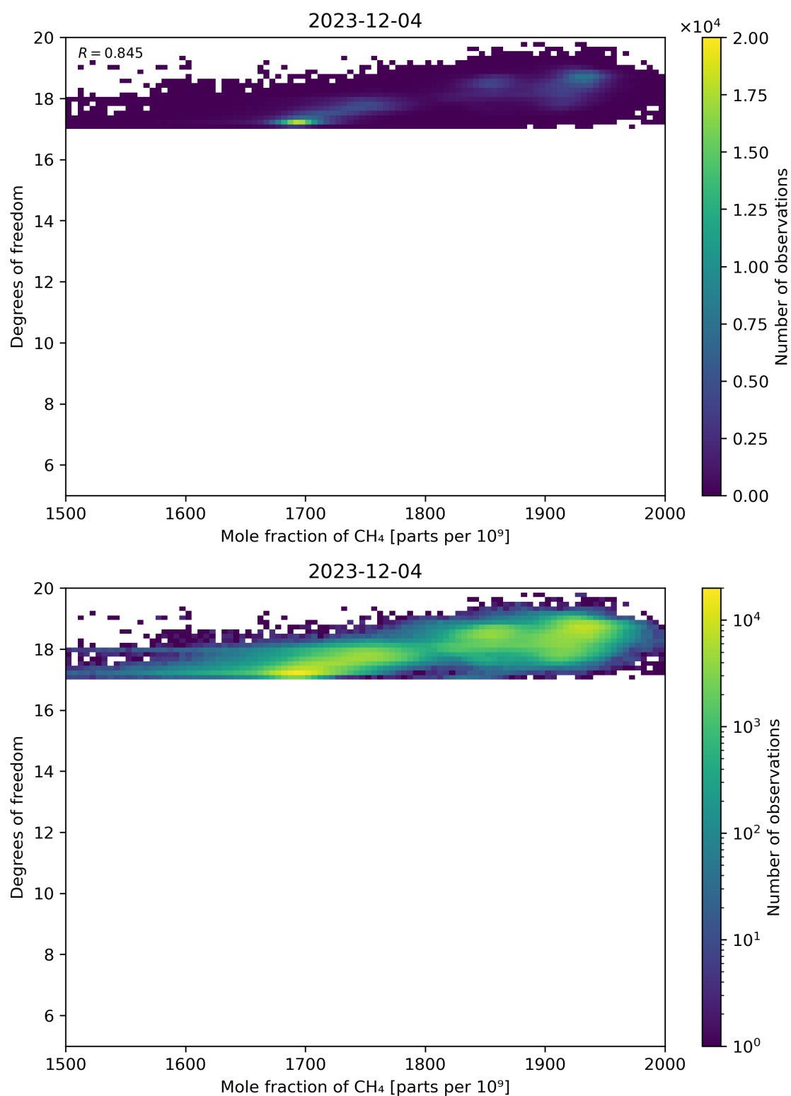
Figure 72: Scatter density plot of “Mole fraction of CH 4 ” against “Degrees of freedom” for 2023-12-04 to 2023-12-05.
