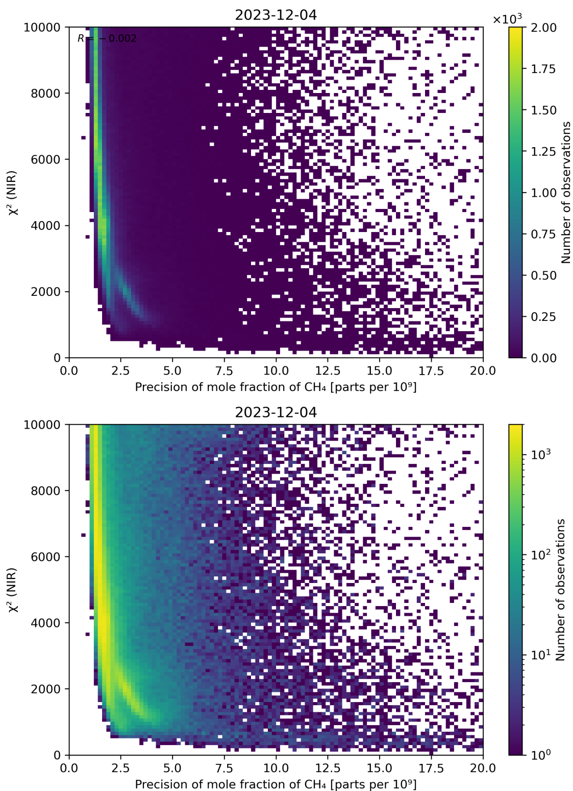
Figure 78: Scatter density plot of “Precision of mole fraction of CH 4 ” against “ \chi^2 (NIR)” for 2023-12-04 to 2023-12-05.
