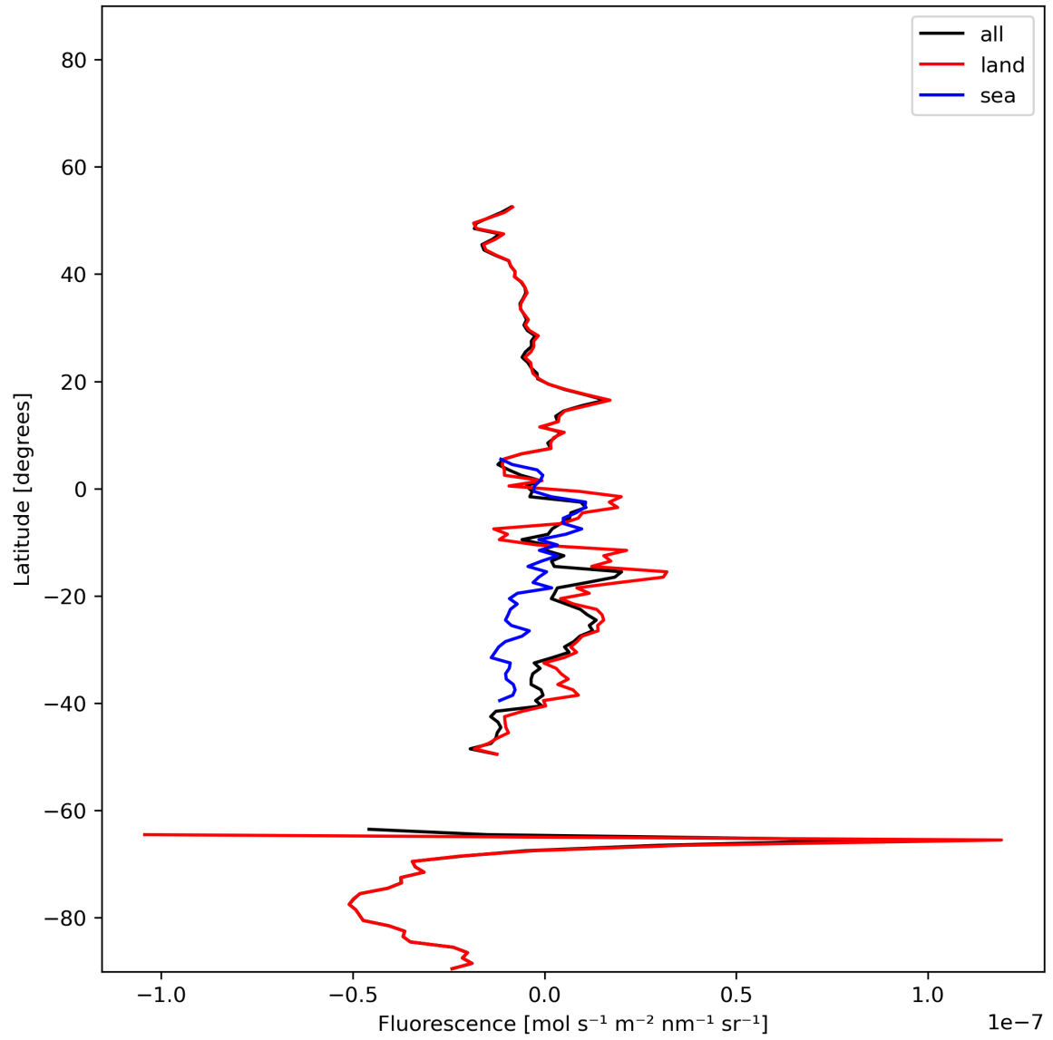
Figure 21: Zonal average of “Fluorescence” for 2023-12-04 to 2023-12-05.
