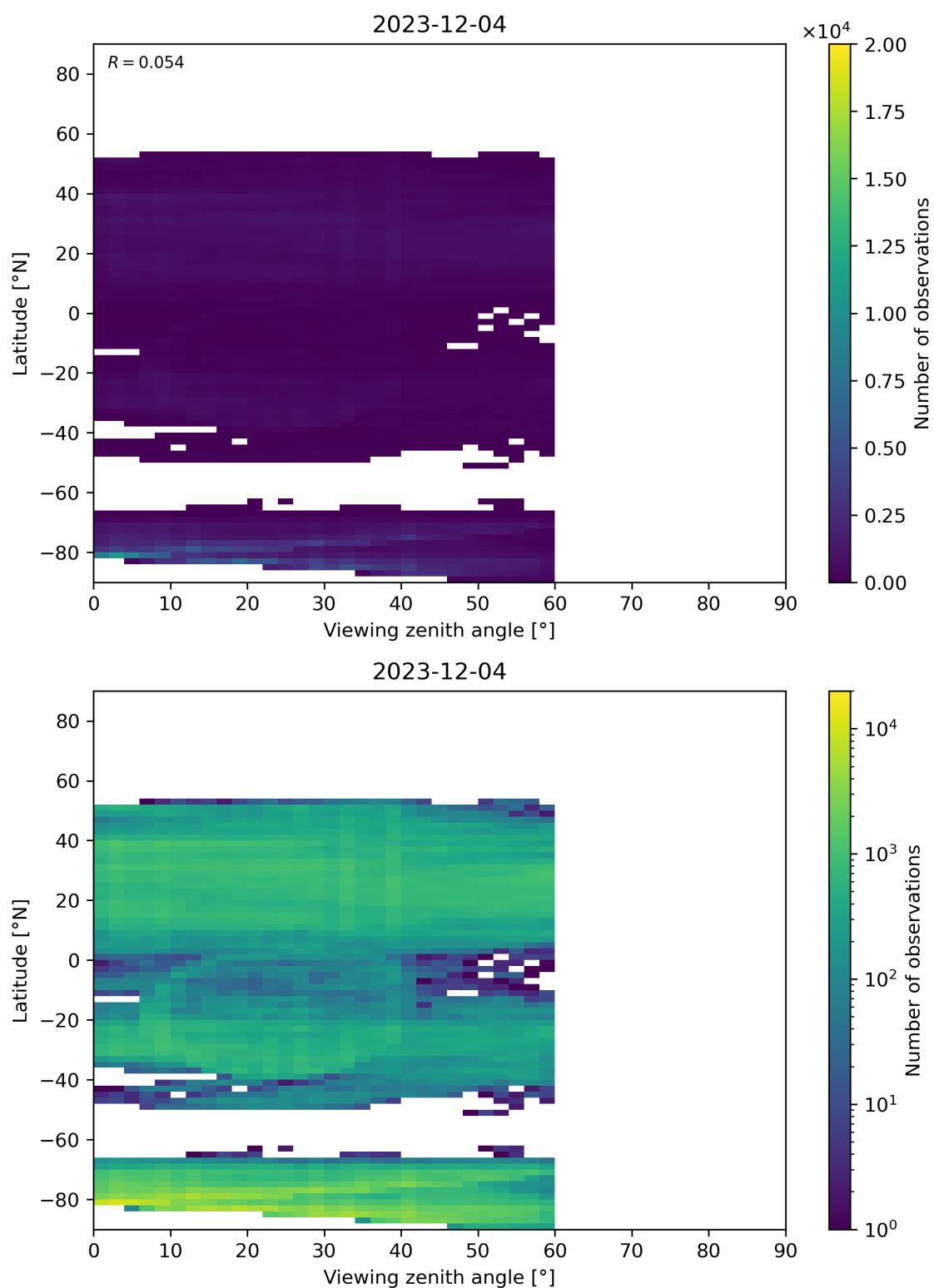
Figure 109: Scatter density plot of “Viewing zenith angle” against “Latitude” for 2023-12-04 to 2023-12-05.
