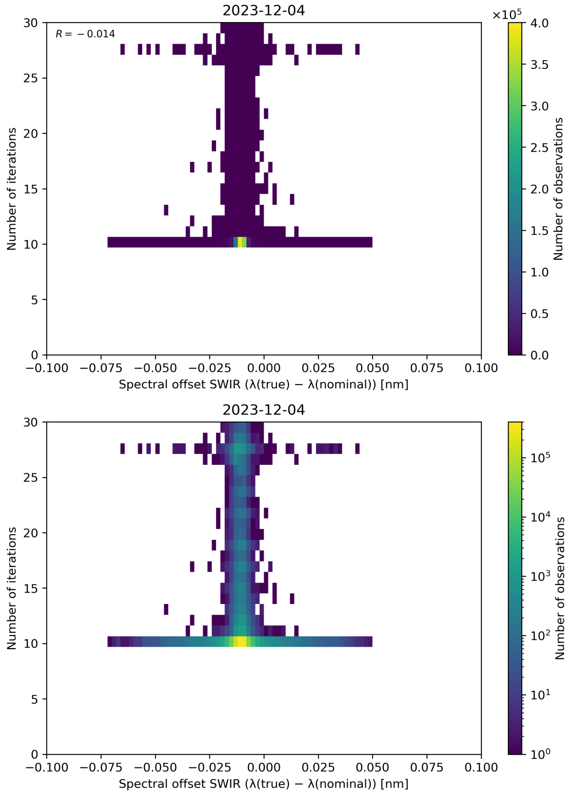
Figure 121: Scatter density plot of “Spectral offset SWIR ( \lambda(\text{true}) - \lambda(\text{nominal}) )” against “Number of iterations” for 2023-12-04 to 2023-12-05.
