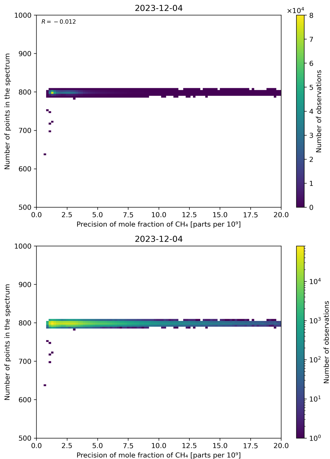
Figure 84: Scatter density plot of “Precision of mole fraction of CH 4 ” against “Number of points in the spectrum” for 2023-12-04 to 2023-12-05.
