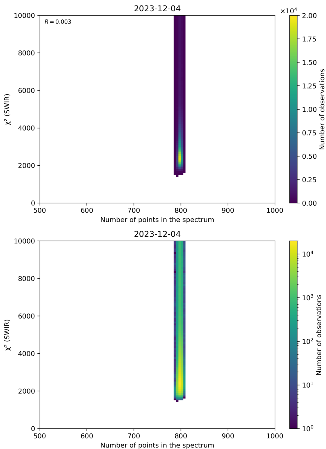
Figure 89: Scatter density plot of “Number of points in the spectrum” against “ \chi^2 (SWIR)” for 2023-12-04 to 2023-12-05.
