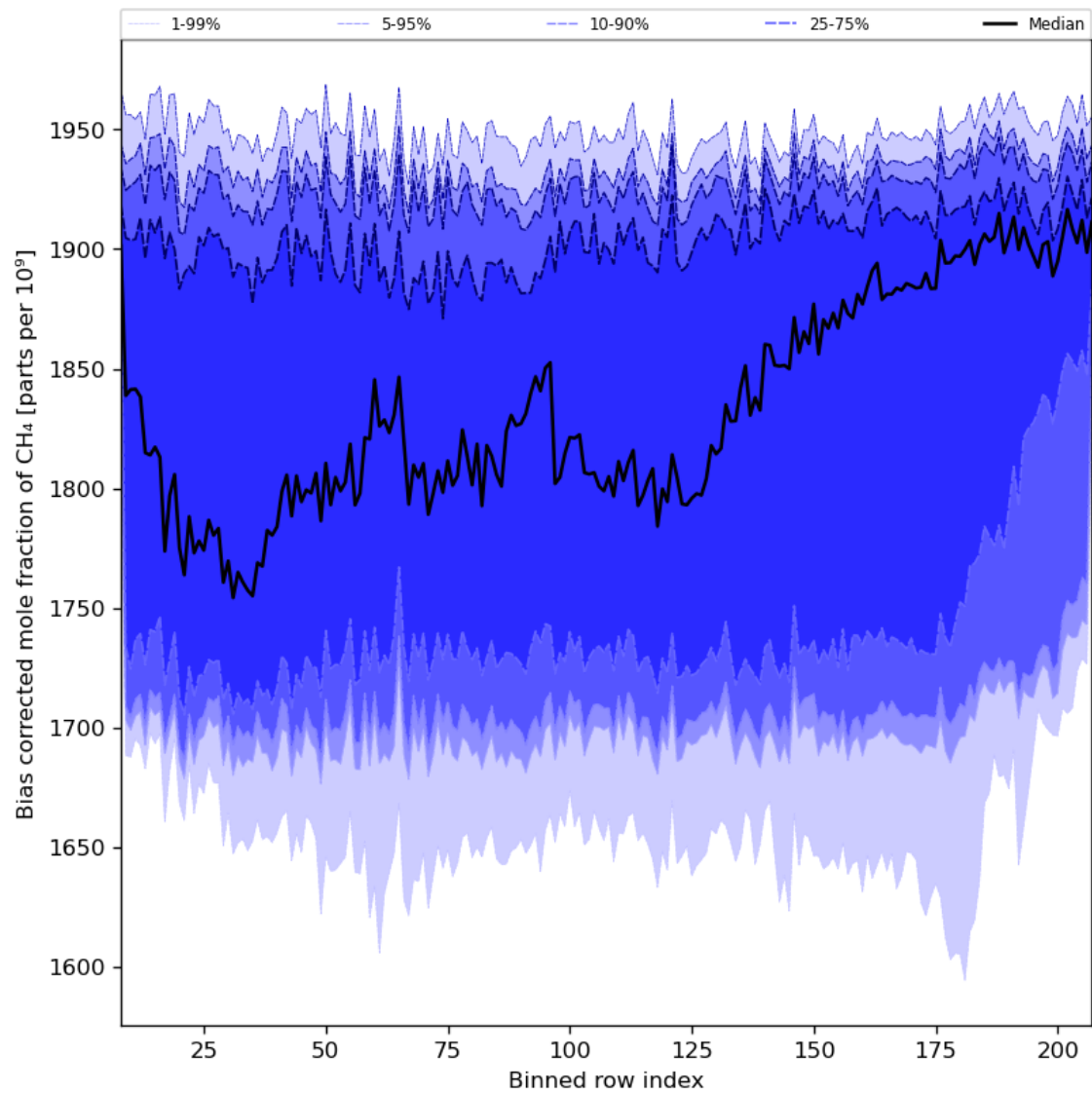
Figure 36: Along track statistics of “Bias corrected mole fraction of CH 4 ” for 2023-12-04 to 2023-12-05
