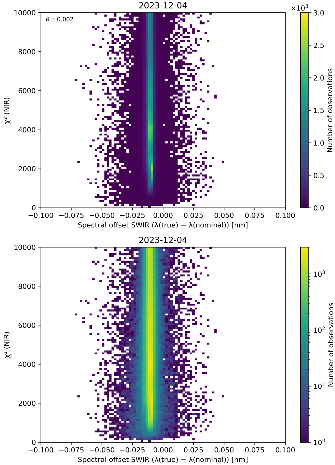
Figure 117: Scatter density plot of “Spectral offset SWIR ( \lambda(\text{true}) - \lambda(\text{nominal}) )” against “ \chi^2 (NIR)” for 2023-12-04 to 2023-12-05.
