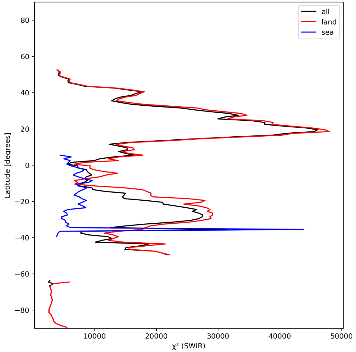
Figure 17: Zonal average of “ \chi^2 (SWIR)” for 2023-12-04 to 2023-12-05.
