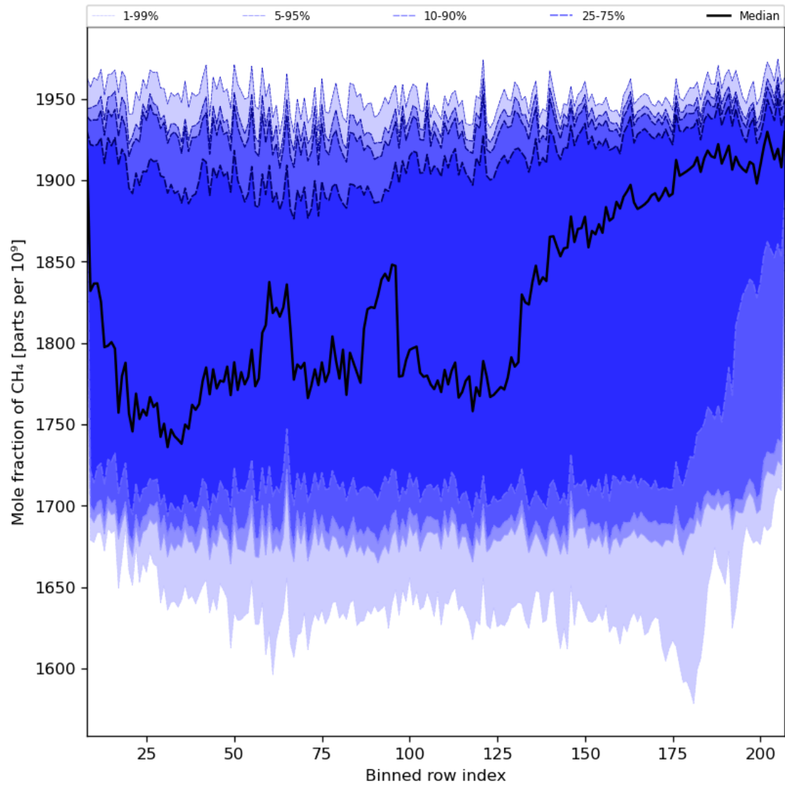
Figure 34: Along track statistics of “Mole fraction of CH 4 ” for 2023-12-04 to 2023-12-05
