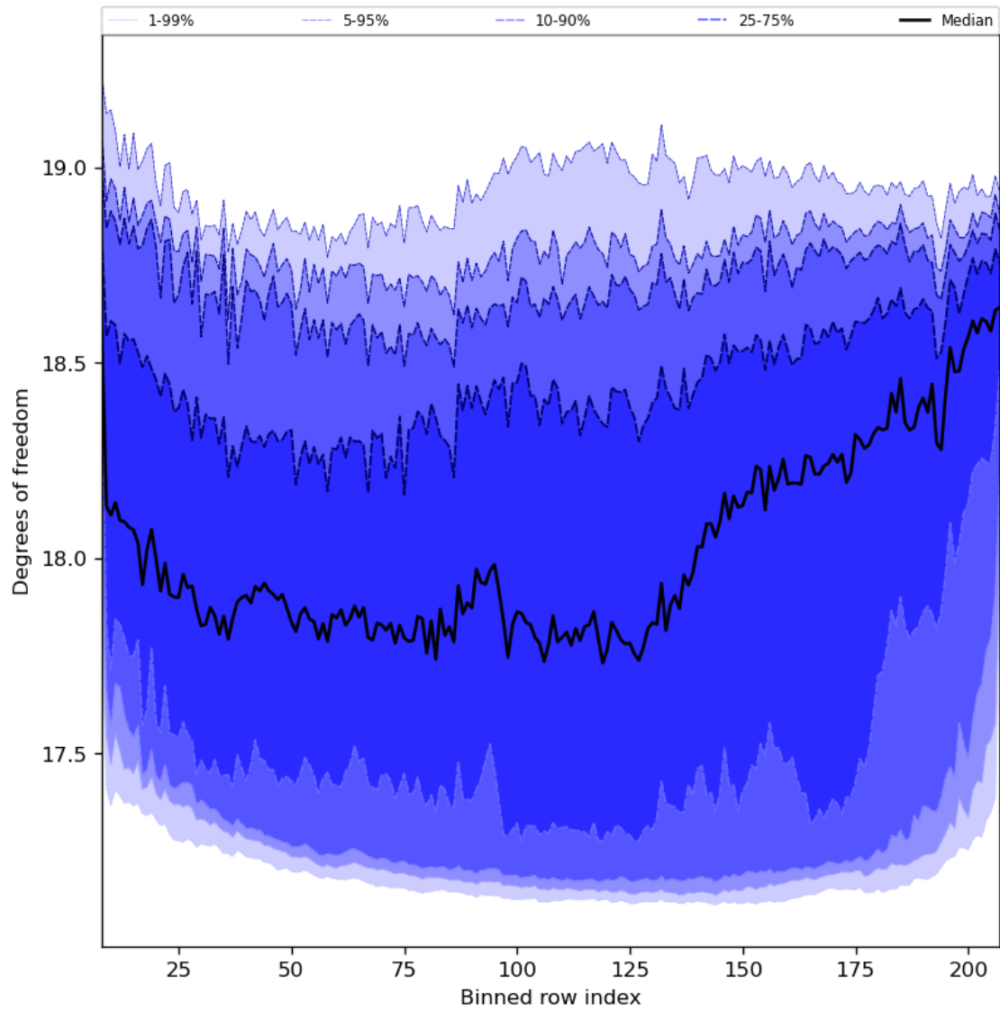
Figure 41: Along track statistics of “Degrees of freedom” for 2023-12-04 to 2023-12-05
