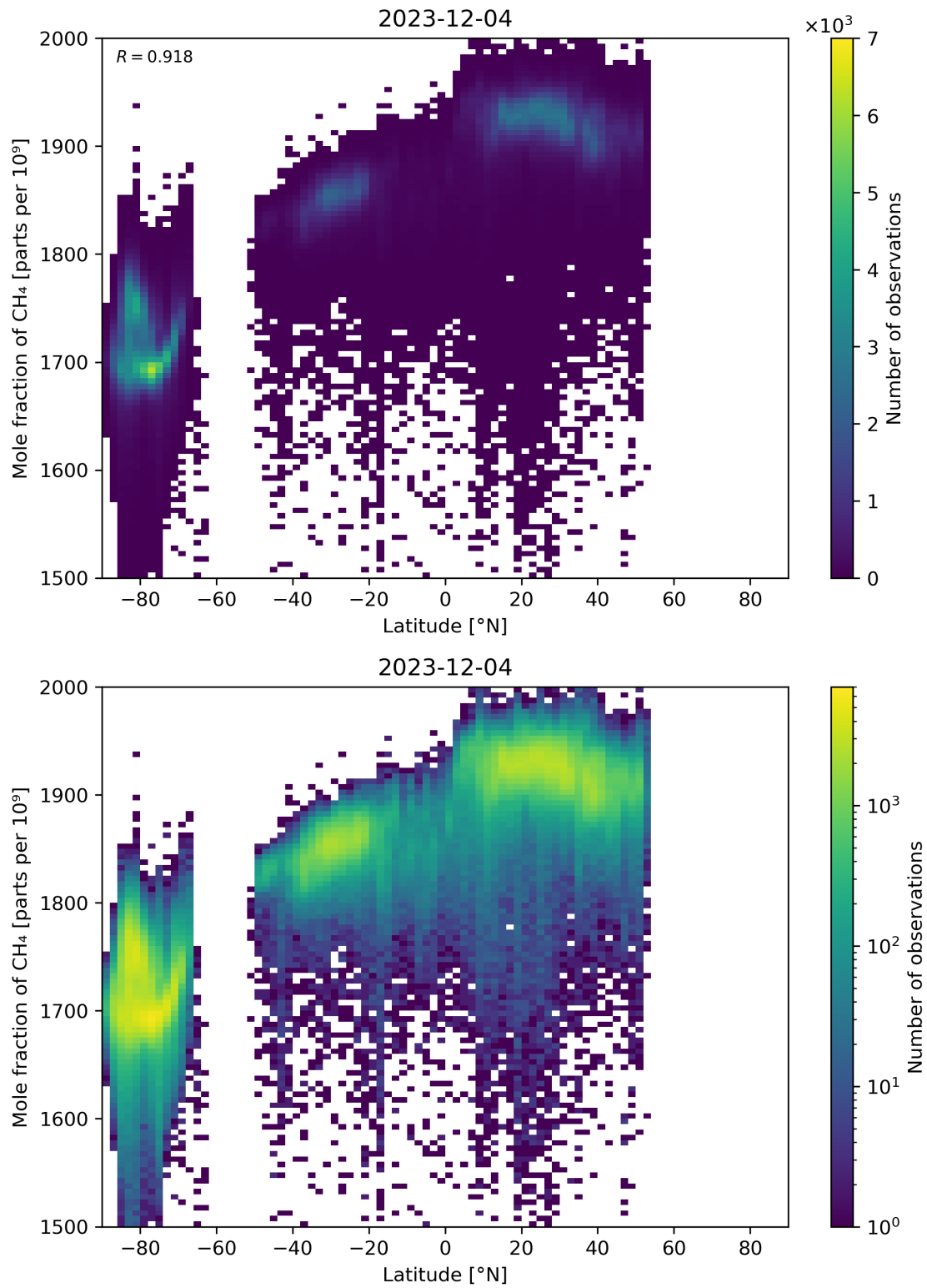
Figure 57: Scatter density plot of “Latitude” against “Mole fraction of CH 4 ” for 2023-12-04 to 2023-12-05.
