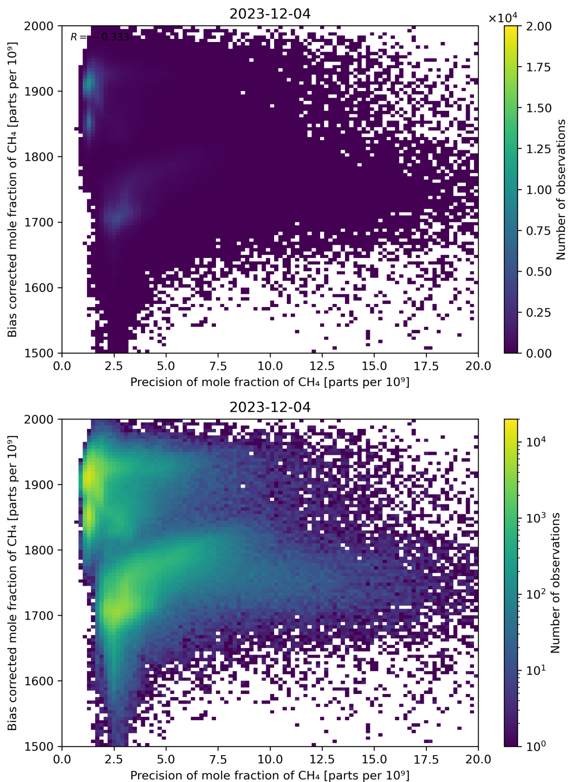
Figure 82: Scatter density plot of “Precision of mole fraction of CH 4 ” against “Bias corrected mole fraction of CH 4 ” for 2023-12-04 to 2023-12-05.
