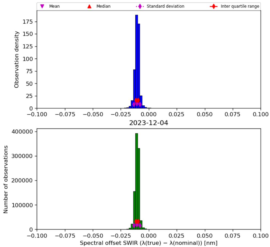
Figure 27: Histogram of “Spectral offset SWIR ( \lambda(\text{true}) - \lambda(\text{nominal}) )” for 2023-12-04 to 2023-12-05
