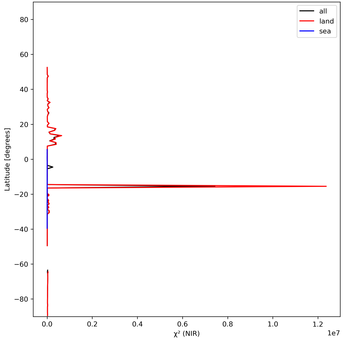
Figure 18: Zonal average of “ \chi^2 (NIR)” for 2023-12-04 to 2023-12-05.
