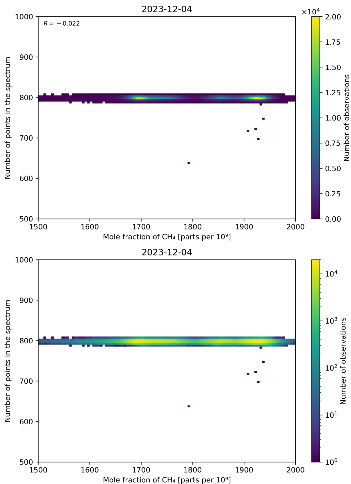
Figure 77: Scatter density plot of “Mole fraction of CH 4 ” against “Number of points in the spectrum” for 2023-12-04 to 2023-12-05.
