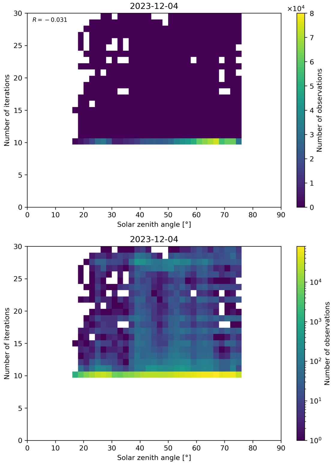
Figure 102: Scatter density plot of “Solar zenith angle” against “Number of iterations” for 2023-12-04 to 2023-12-05.
