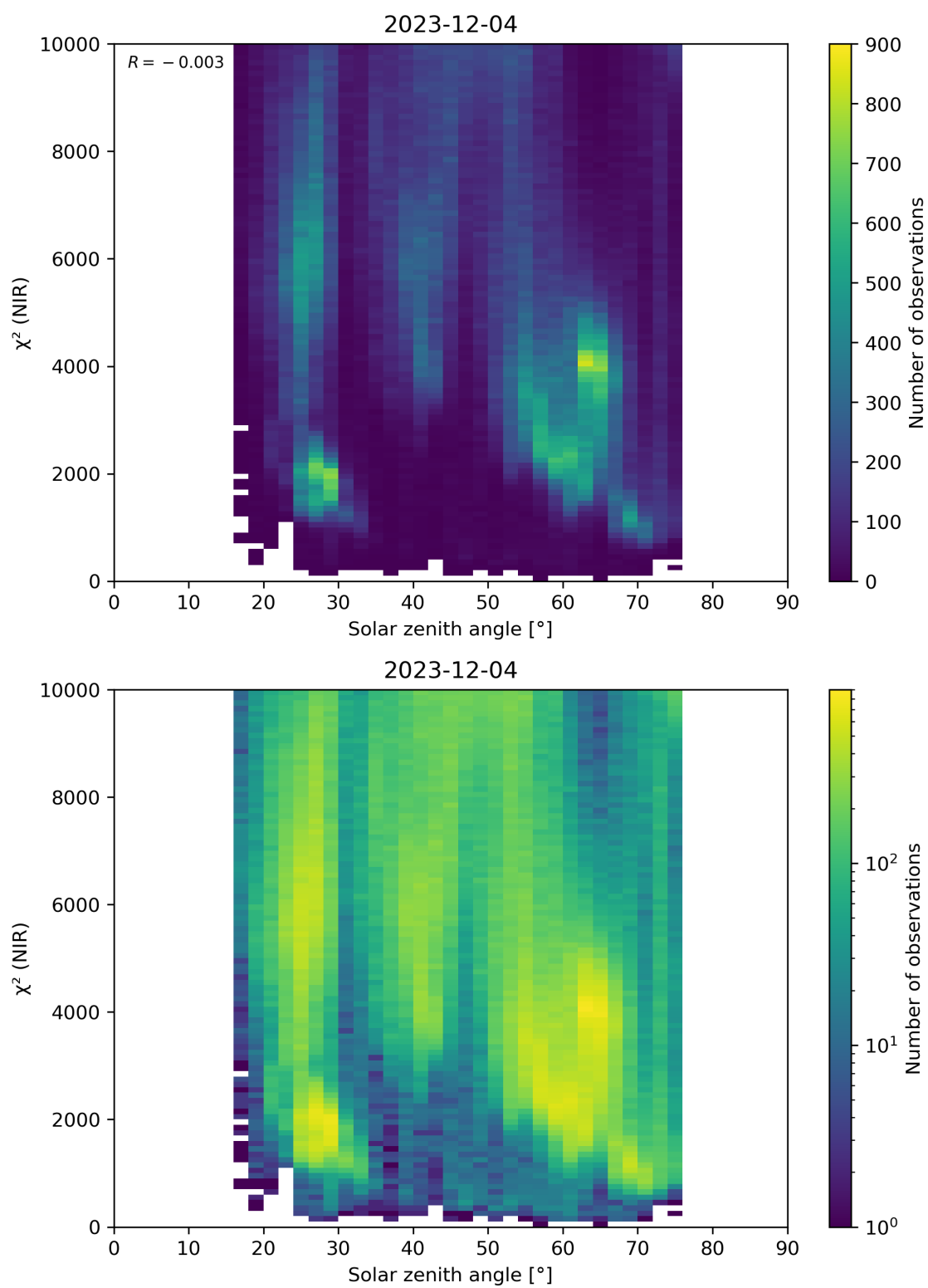
Figure 94: Scatter density plot of “Solar zenith angle” against “ \chi^2 (NIR)” for 2023-12-04 to 2023-12-05.
