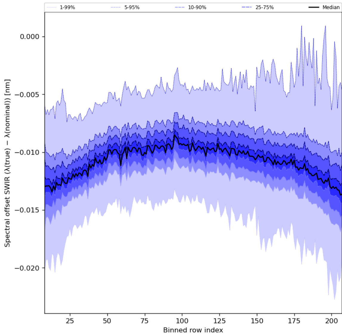
Figure 38: Along track statistics of “Spectral offset SWIR ( \lambda(\text{true}) - \lambda(\text{nominal}) )” for 2023-12-04 to 2023-12-05
