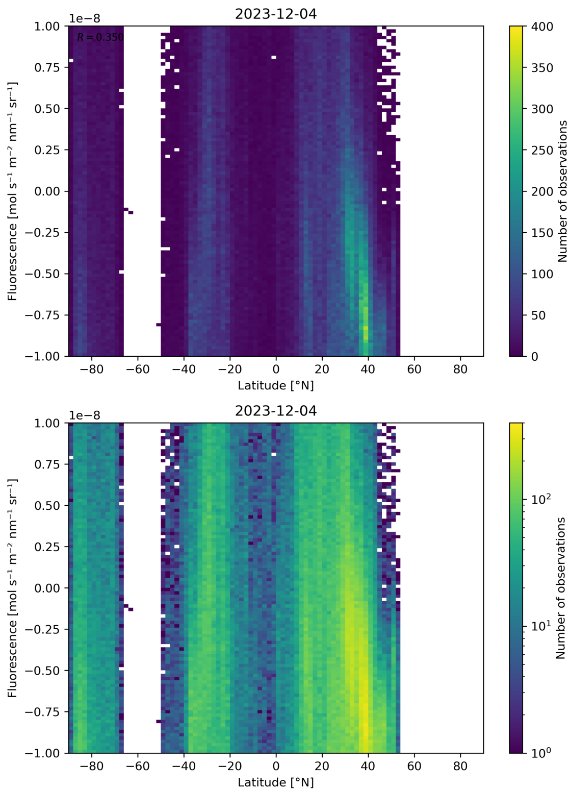
Figure 56: Scatter density plot of “Latitude” against “Fluorescence” for 2023-12-04 to 2023-12-05.
