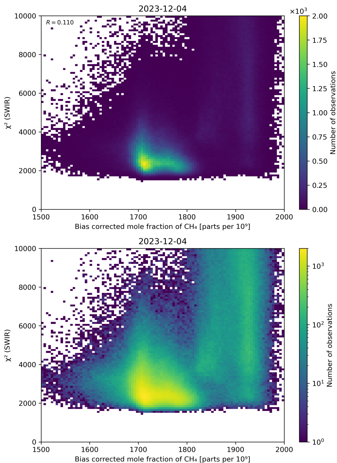
Figure 64: Scatter density plot of “Bias corrected mole fraction of \text{CH}_4 ” against “ \chi^2 (SWIR)” for 2023-12-04 to 2023-12-05.
