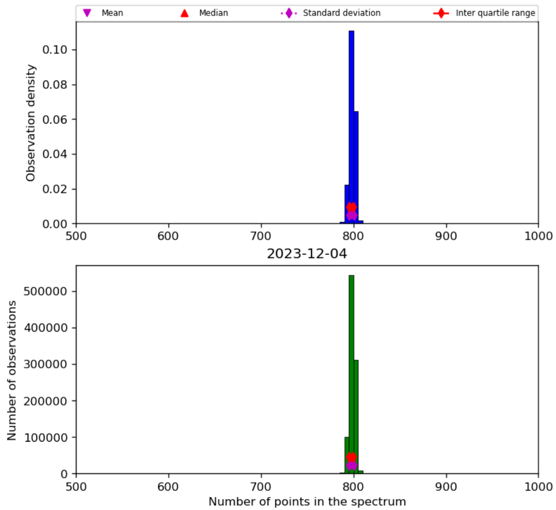
Figure 26: Histogram of “Number of points in the spectrum” for 2023-12-04 to 2023-12-05
