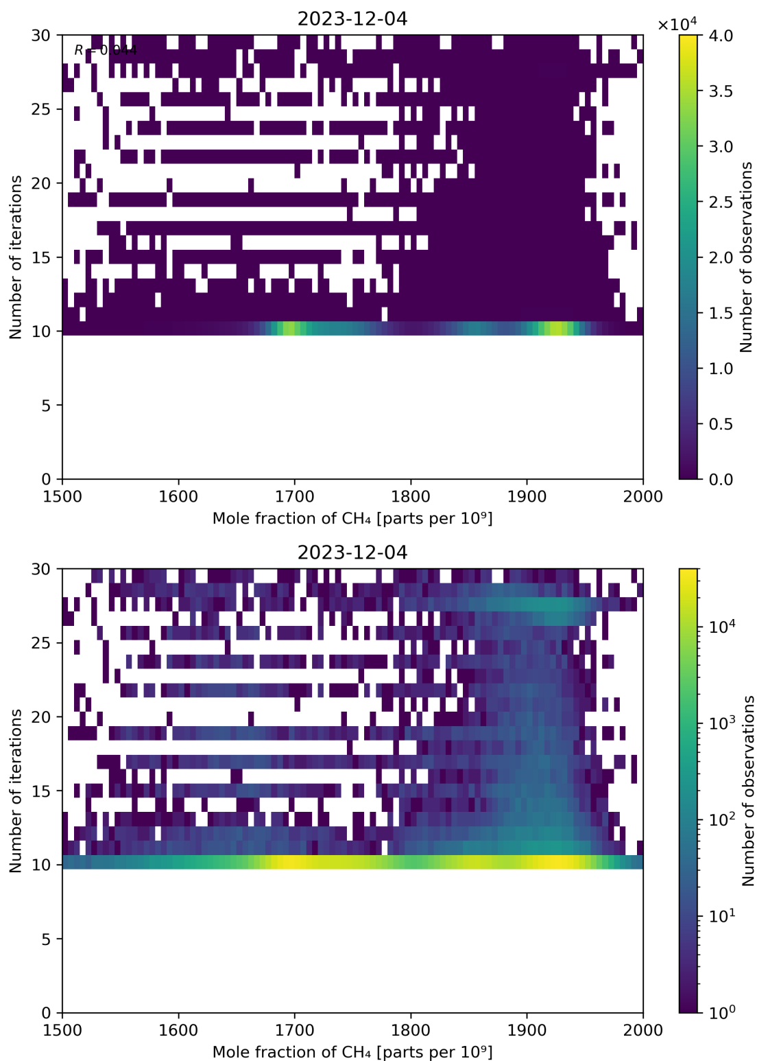
Figure 76: Scatter density plot of “Mole fraction of CH 4 ” against “Number of iterations” for 2023-12-04 to 2023-12-05.
