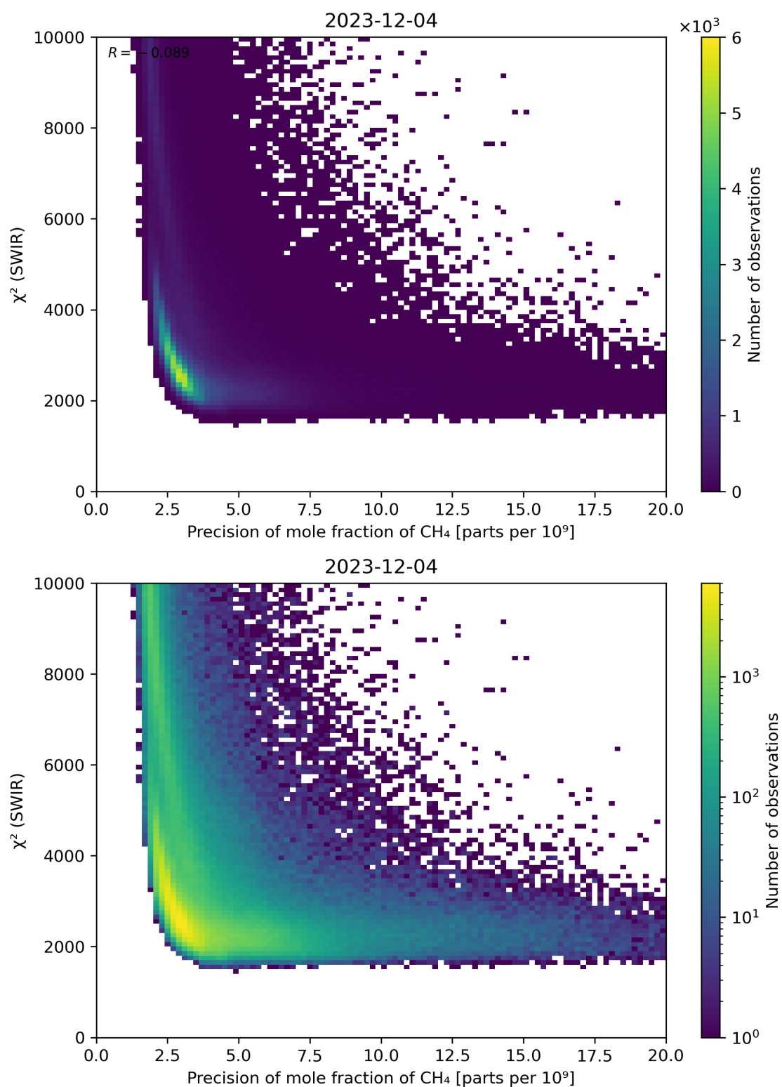
Figure 79: Scatter density plot of “Precision of mole fraction of \text{CH}_4 ” against “ \chi^2 (SWIR)” for 2023-12-04 to 2023-12-05.
