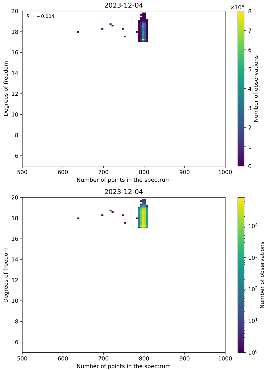
Figure 90: Scatter density plot of “Number of points in the spectrum” against “Degrees of freedom” for 2023-12-04 to 2023-12-05.
