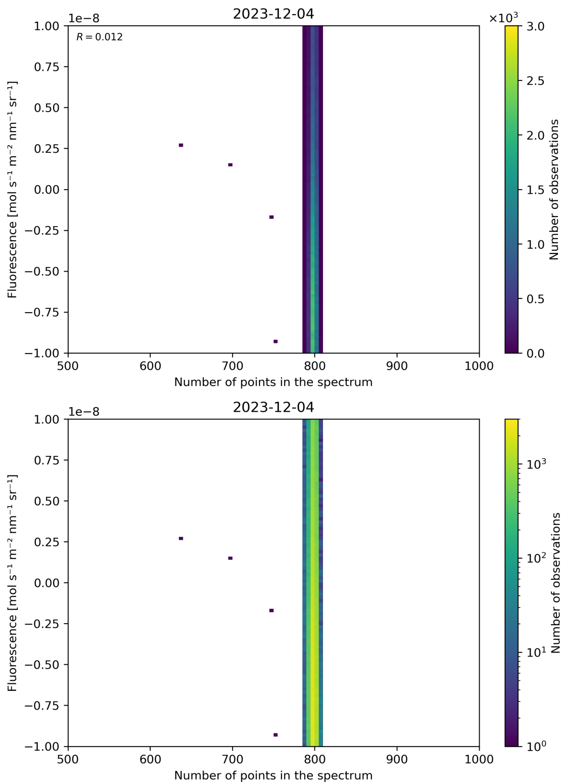
Figure 91: Scatter density plot of “Number of points in the spectrum” against “Fluorescence” for 2023-12-04 to 2023-12-05.
