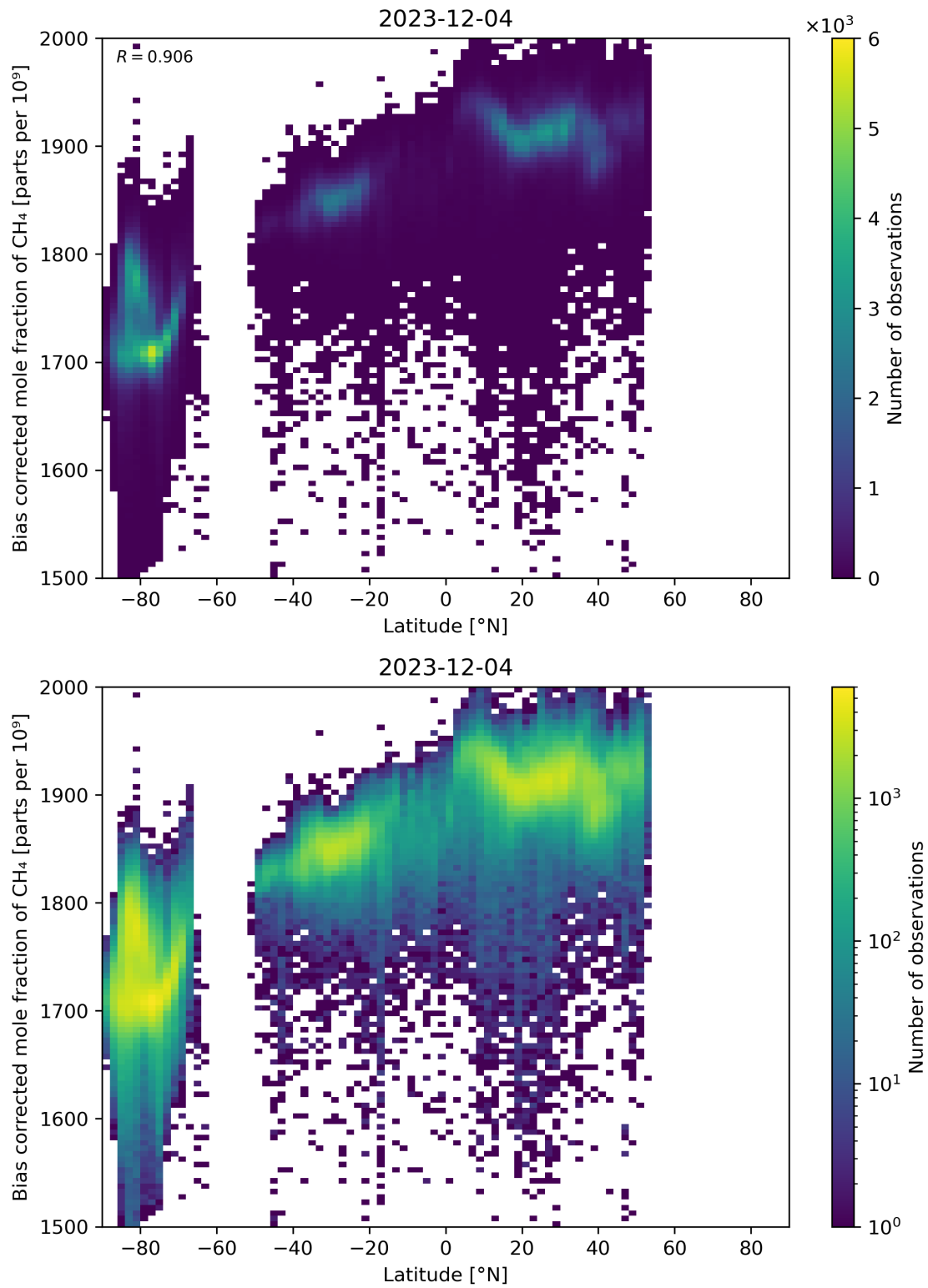
Figure 58: Scatter density plot of “Latitude” against “Bias corrected mole fraction of CH 4 ” for 2023-12-04 to 2023-12-05.
