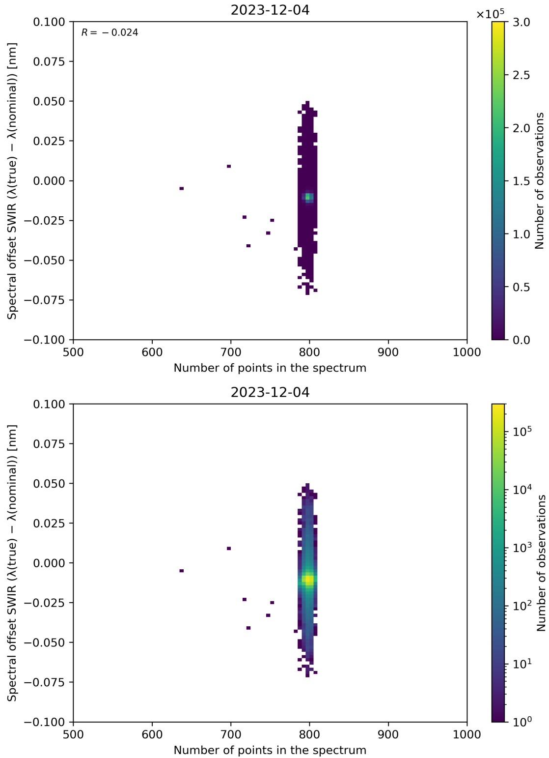
Figure 93: Scatter density plot of “Number of points in the spectrum” against “Spectral offset SWIR ( \lambda(\text{true}) - \lambda(\text{nominal}) )” for 2023-12-04 to 2023-12-05.
