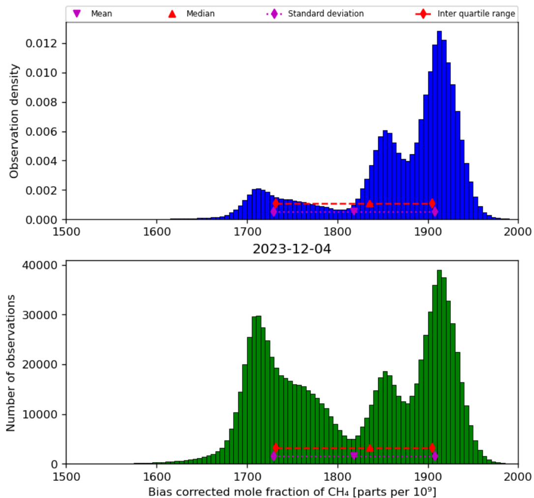
Figure 25: Histogram of “Bias corrected mole fraction of CH 4 ” for 2023-12-04 to 2023-12-05
