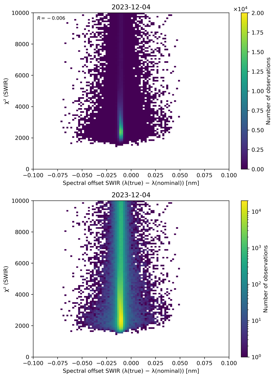
Figure 118: Scatter density plot of “Spectral offset SWIR ( \lambda(\text{true}) - \lambda(\text{nominal}) )” against “ \chi^2 (SWIR)” for 2023-12-04 to 2023-12-05.
