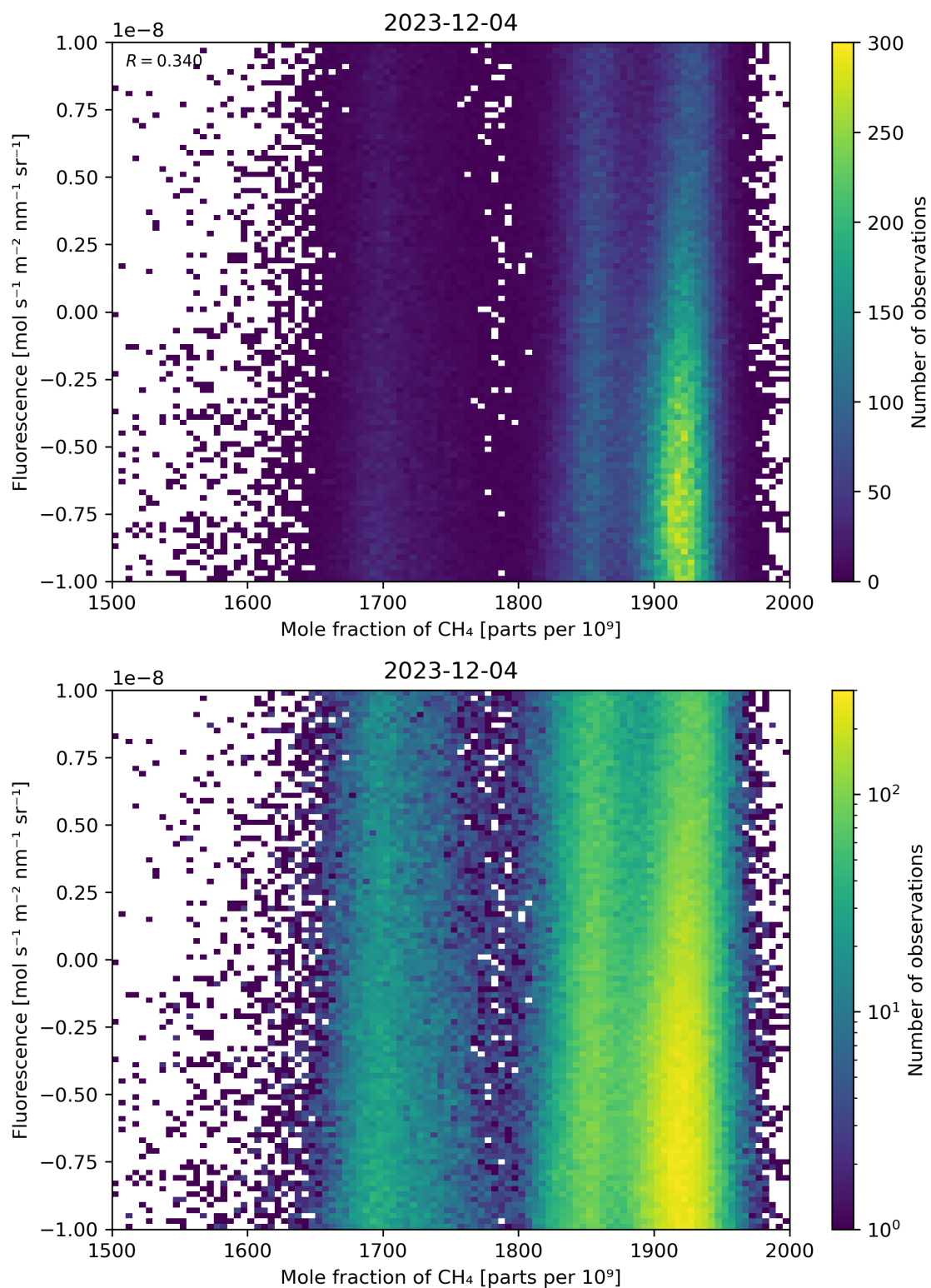
Figure 73: Scatter density plot of “Mole fraction of \text{CH}_4 ” against “Fluorescence” for 2023-12-04 to 2023-12-05.
