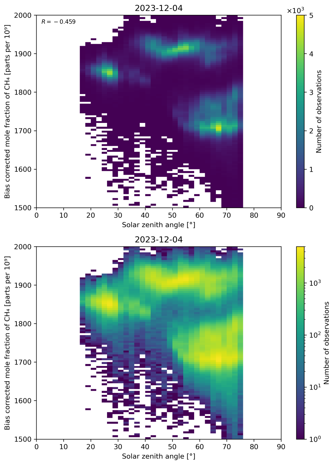
Figure 100: Scatter density plot of “Solar zenith angle” against “Bias corrected mole fraction of CH 4 ” for 2023-12-04 to 2023-12-05.
