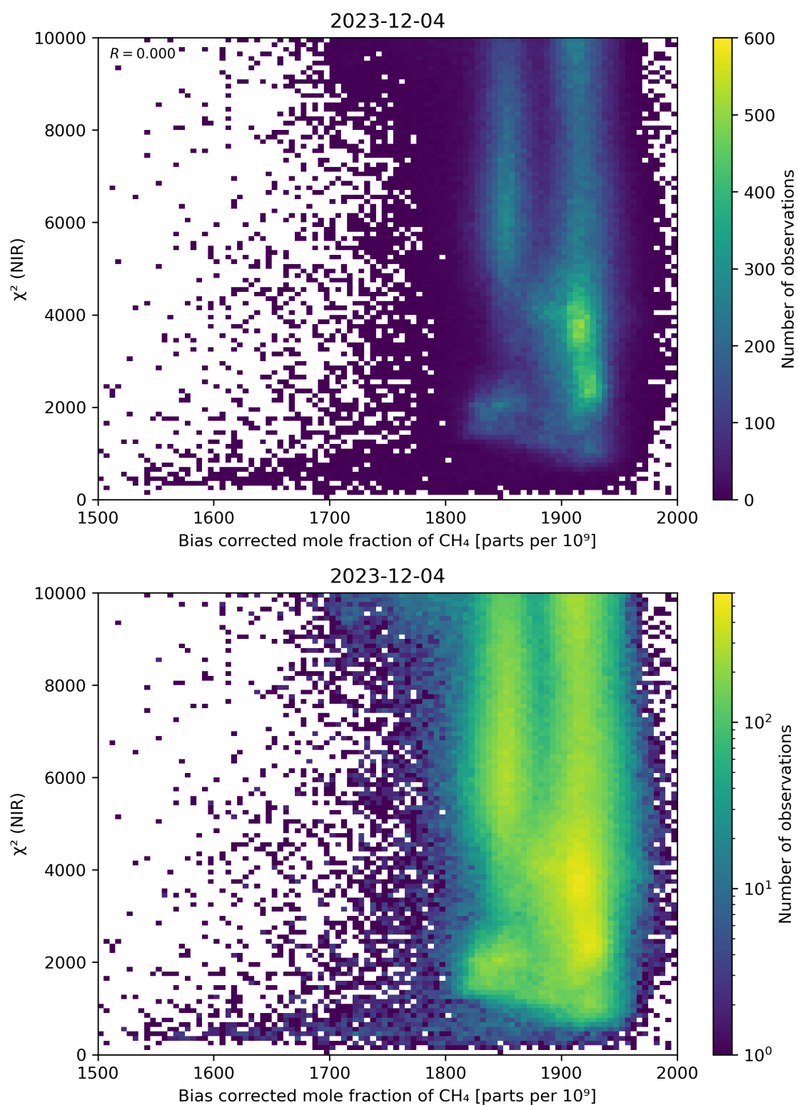
Figure 63: Scatter density plot of “Bias corrected mole fraction of CH 4 ” against “ \chi^2 (NIR)” for 2023-12-04 to 2023-12-05.
