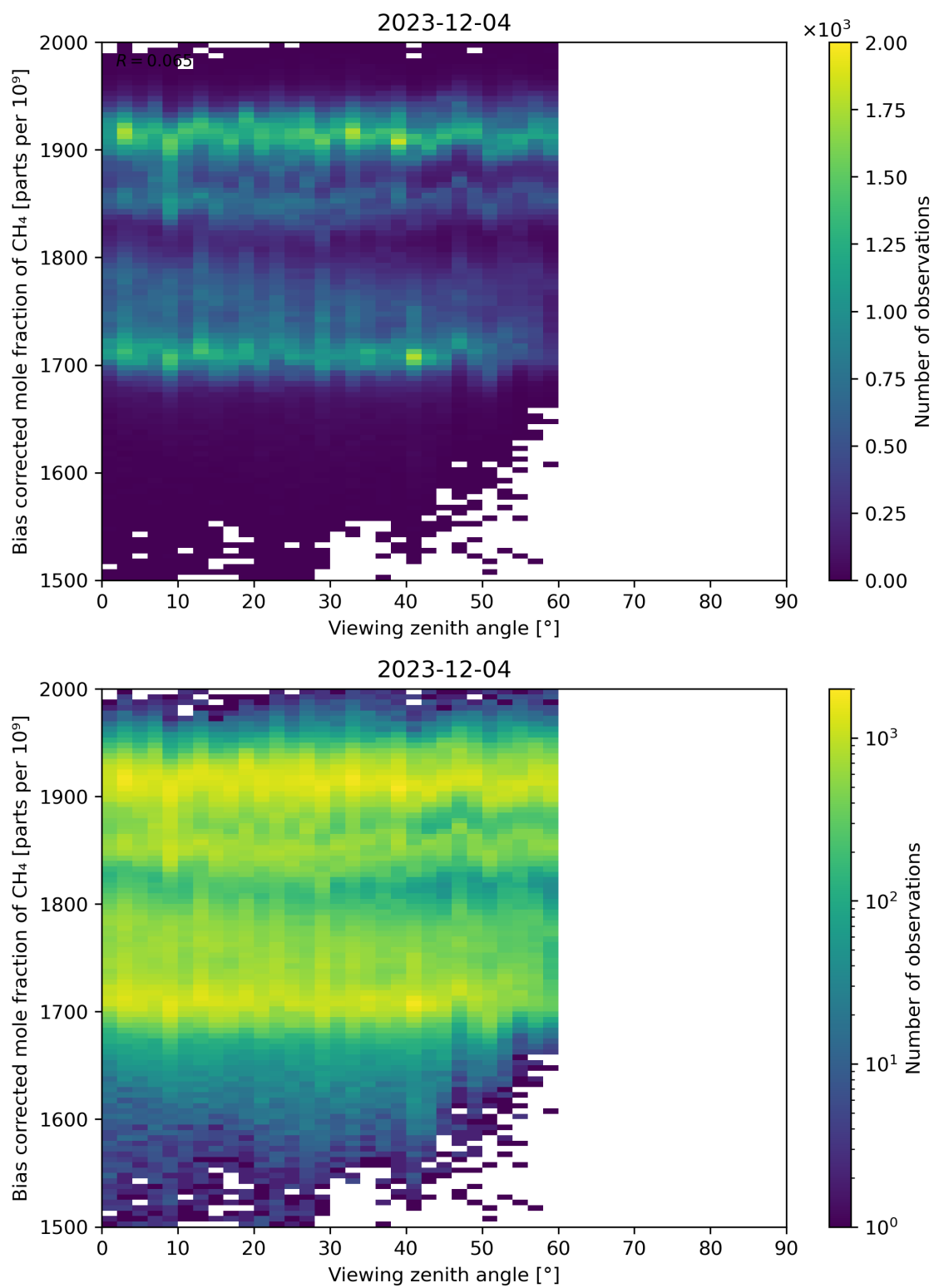
Figure 111: Scatter density plot of “Viewing zenith angle” against “Bias corrected mole fraction of CH 4 ” for 2023-12-04 to 2023-12-05.
