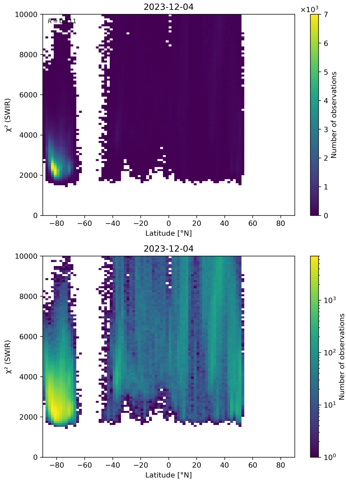
Figure 54: Scatter density plot of “Latitude” against “ \chi^2 (SWIR)” for 2023-12-04 to 2023-12-05.
