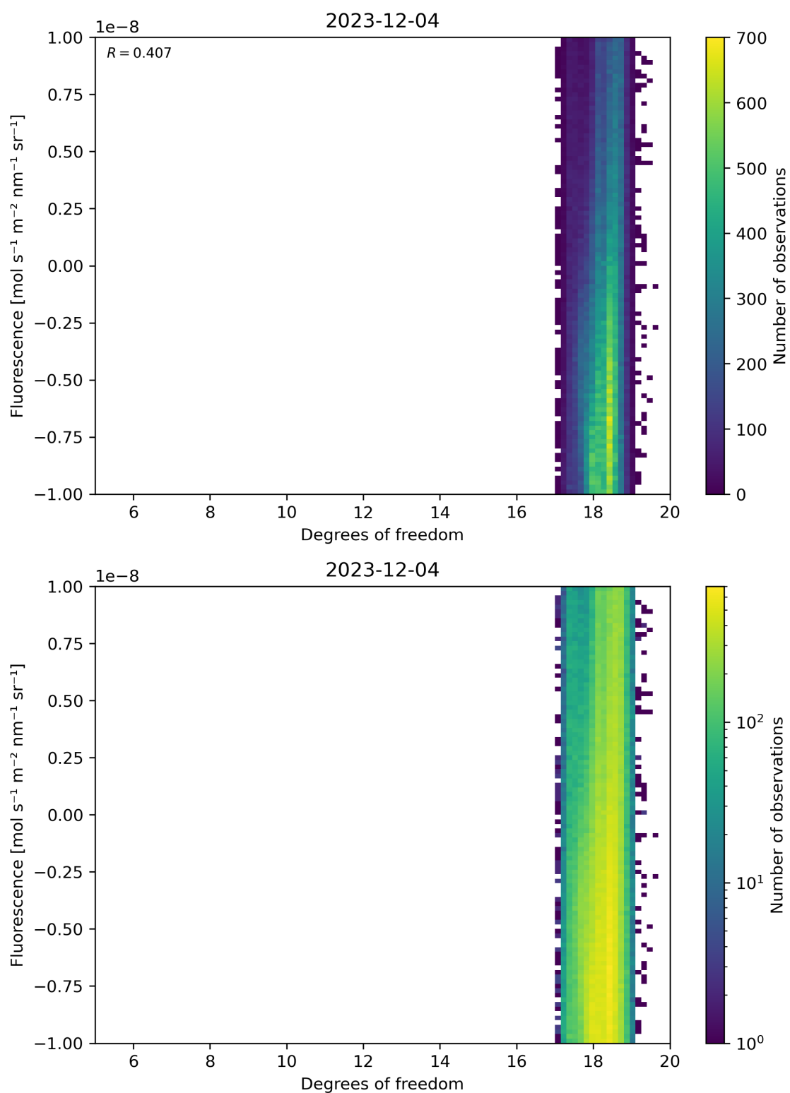
Figure 51: Scatter density plot of “Degrees of freedom” against “Fluorescence” for 2023-12-04 to 2023-12-05.
