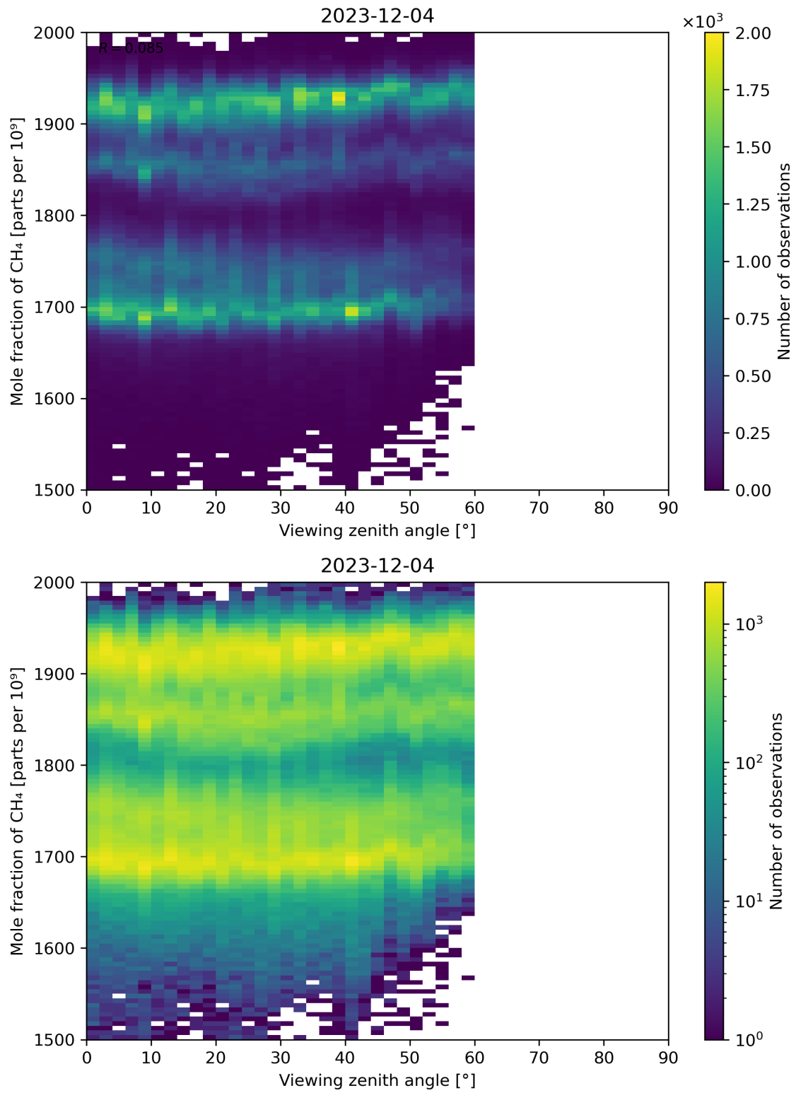
Figure 110: Scatter density plot of “Viewing zenith angle” against “Mole fraction of CH 4 ” for 2023-12-04 to 2023-12-05.
