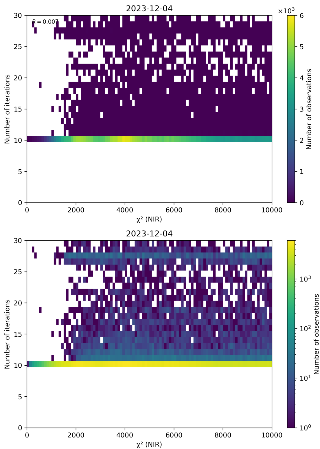
Figure 46: Scatter density plot of “ \chi^2 (NIR)” against “Number of iterations” for 2023-12-04 to 2023-12-05.
