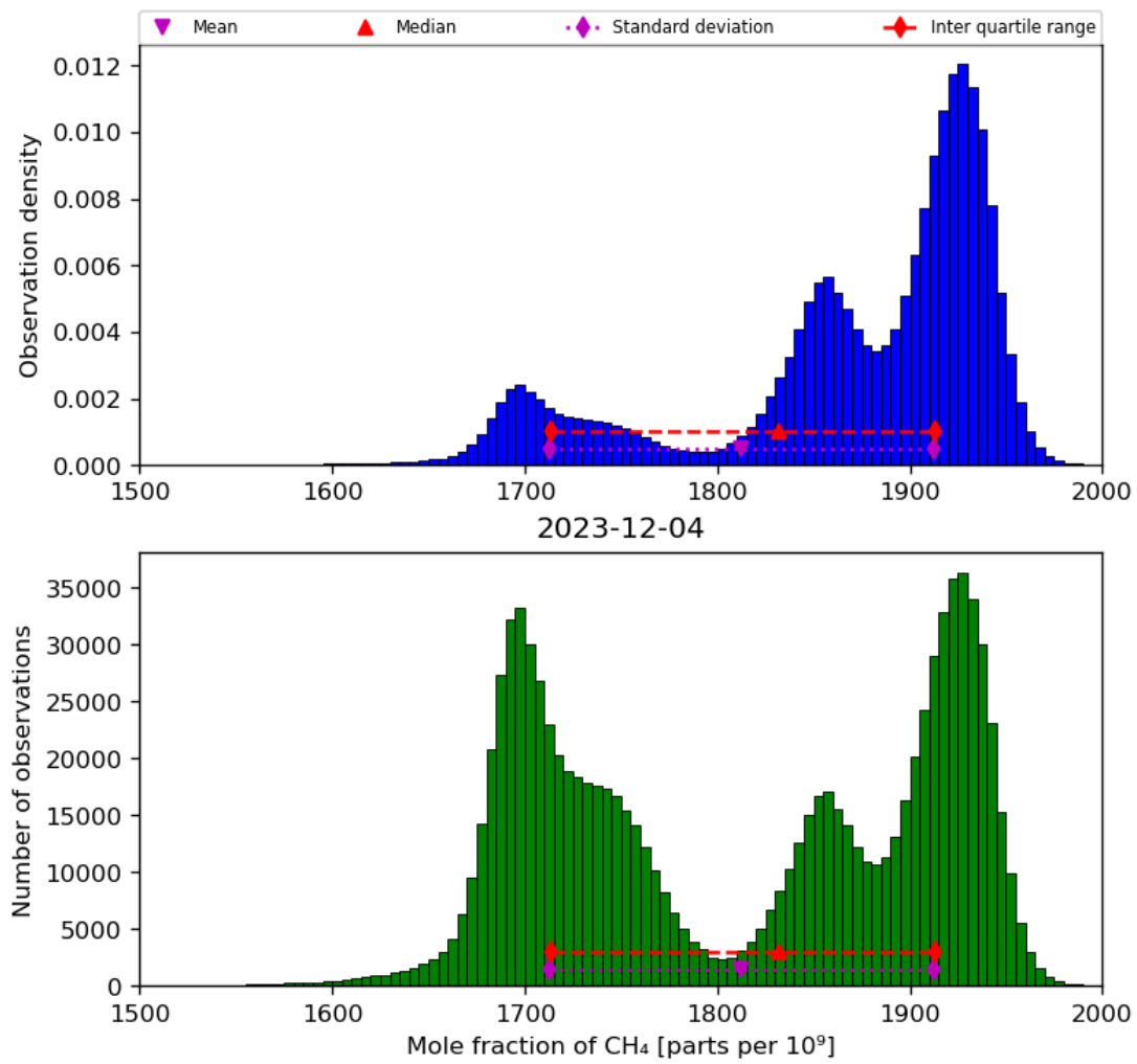
Figure 23: Histogram of “Mole fraction of CH 4 ” for 2023-12-04 to 2023-12-05
