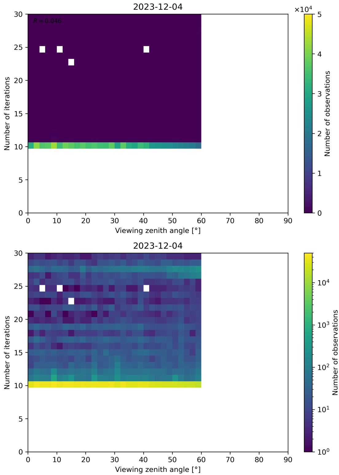
Figure 113: Scatter density plot of “Viewing zenith angle” against “Number of iterations” for 2023-12-04 to 2023-12-05.
