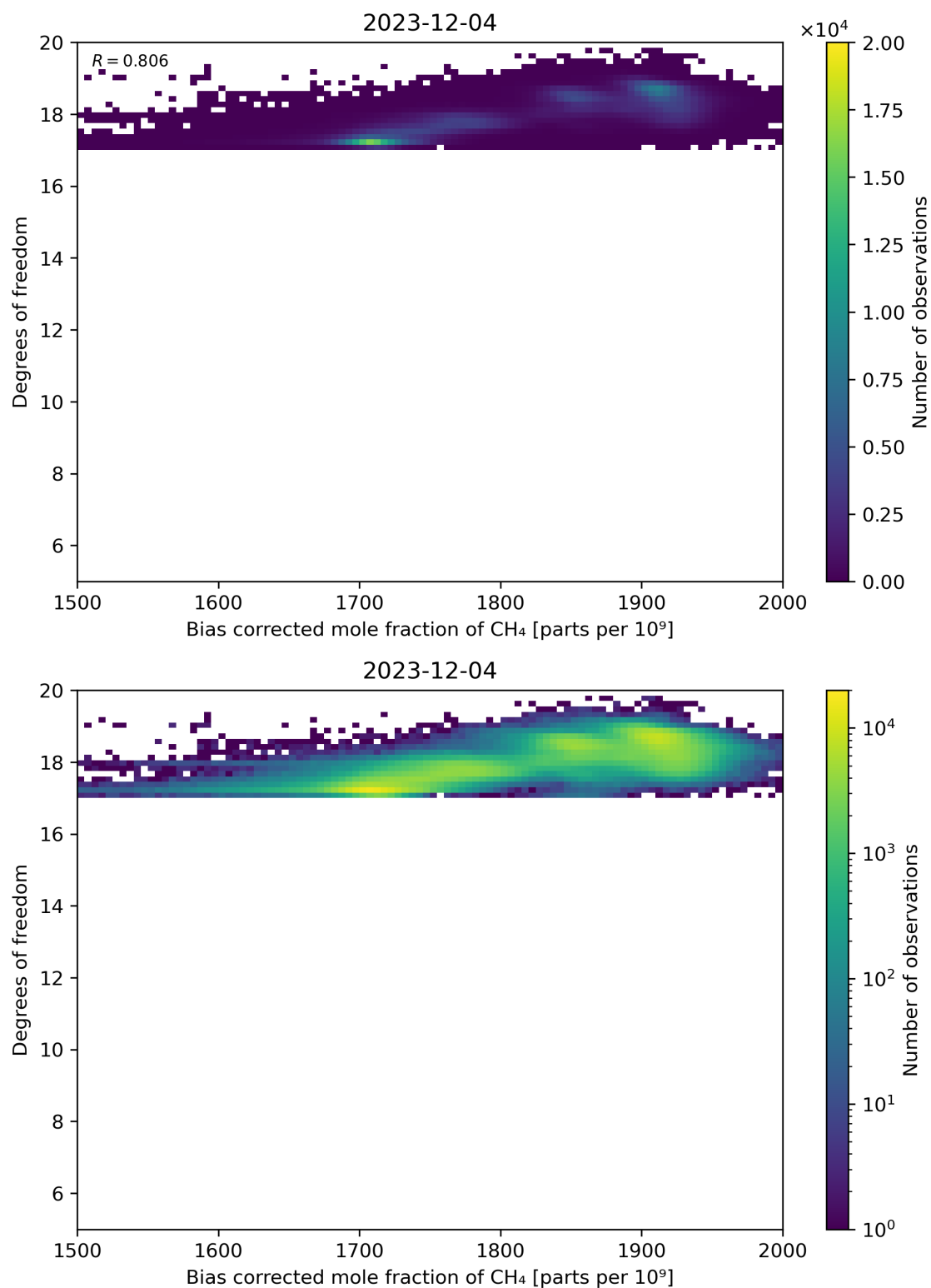
Figure 65: Scatter density plot of “Bias corrected mole fraction of CH 4 ” against “Degrees of freedom” for 2023-12-04 to 2023-12-05.
