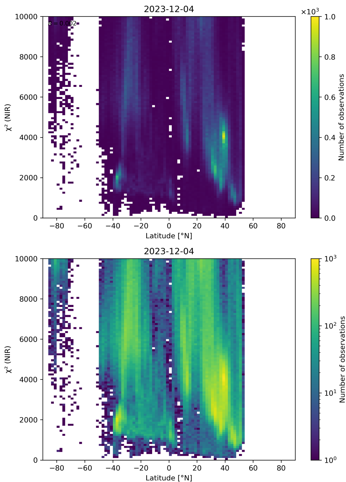
Figure 53: Scatter density plot of “Latitude” against “ \chi^2 (NIR)” for 2023-12-04 to 2023-12-05.
