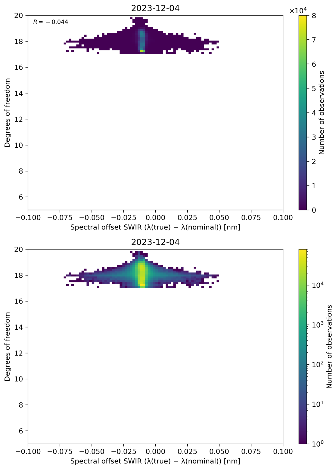
Figure 119: Scatter density plot of “Spectral offset SWIR ( \lambda(\text{true}) - \lambda(\text{nominal}) )” against “Degrees of freedom” for 2023-12-04 to 2023-12-05.
