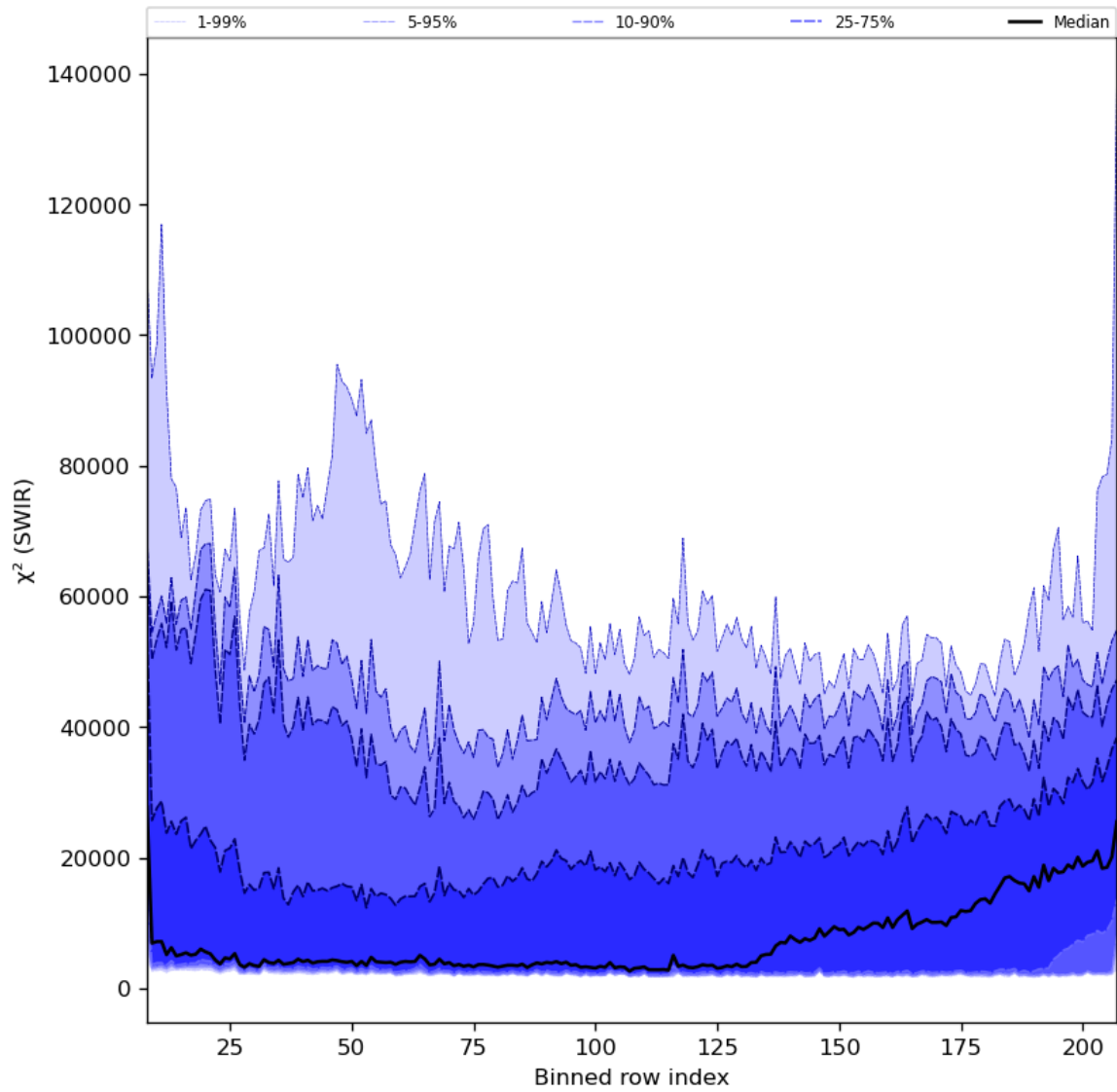
Figure 39: Along track statistics of “ \chi^2 (SWIR)” for 2023-12-04 to 2023-12-05
