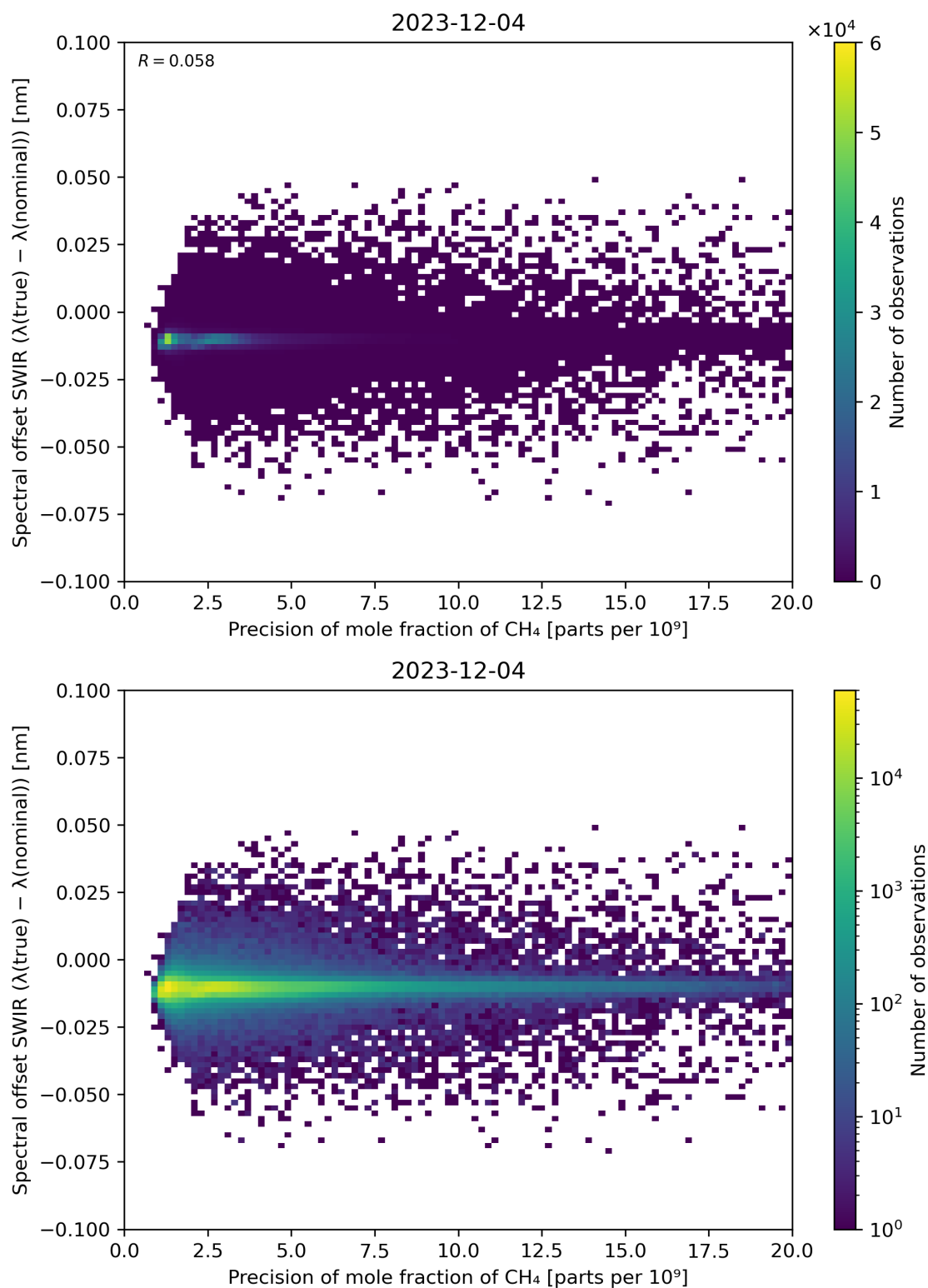
Figure 85: Scatter density plot of “Precision of mole fraction of \text{CH}_4 ” against “Spectral offset SWIR ( \lambda(\text{true}) - \lambda(\text{nominal}) )” for 2023-12-04 to 2023-12-05.
