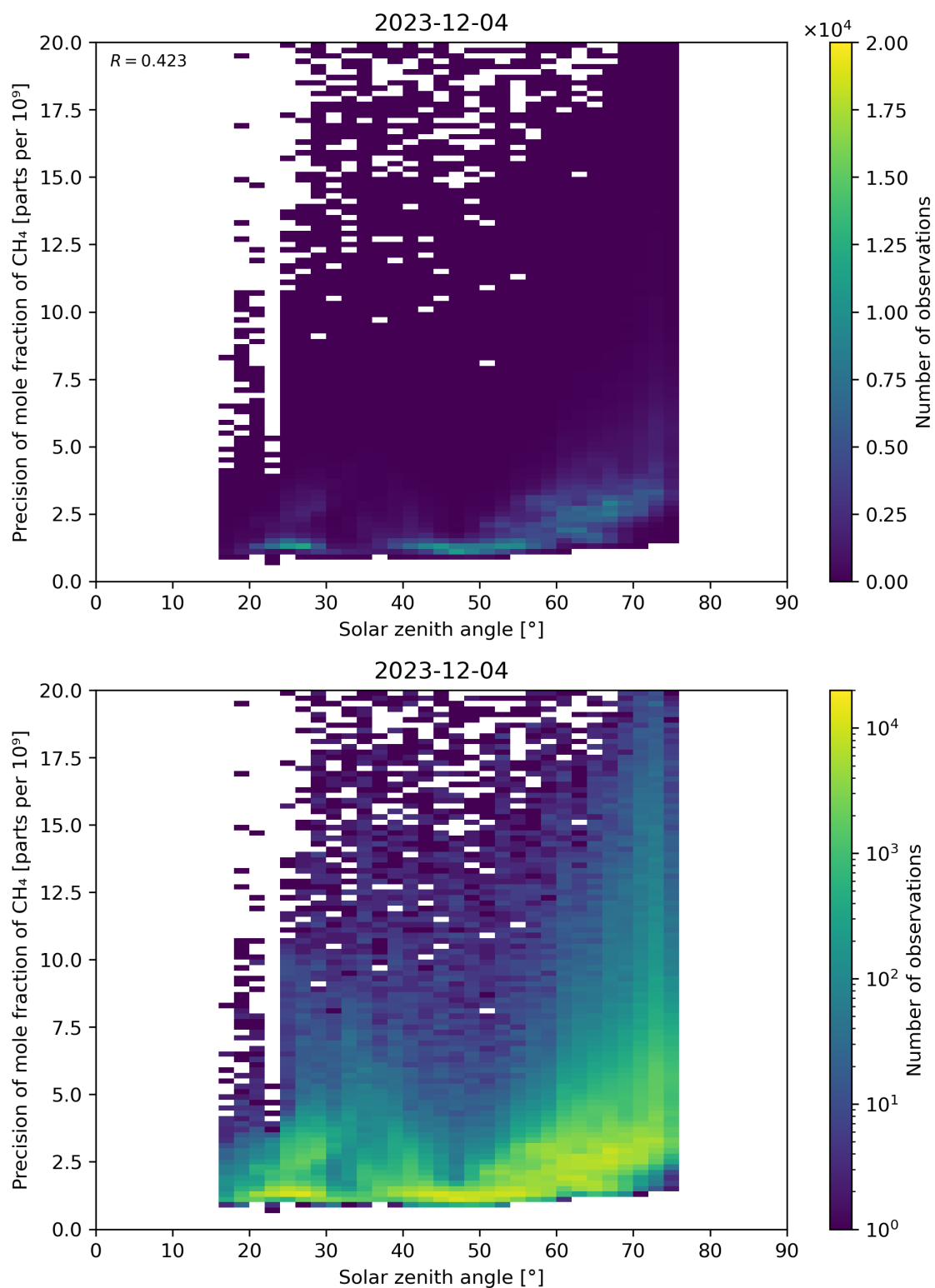
Figure 101: Scatter density plot of “Solar zenith angle” against “Precision of mole fraction of CH 4 ” for 2023-12-04 to 2023-12-05.
