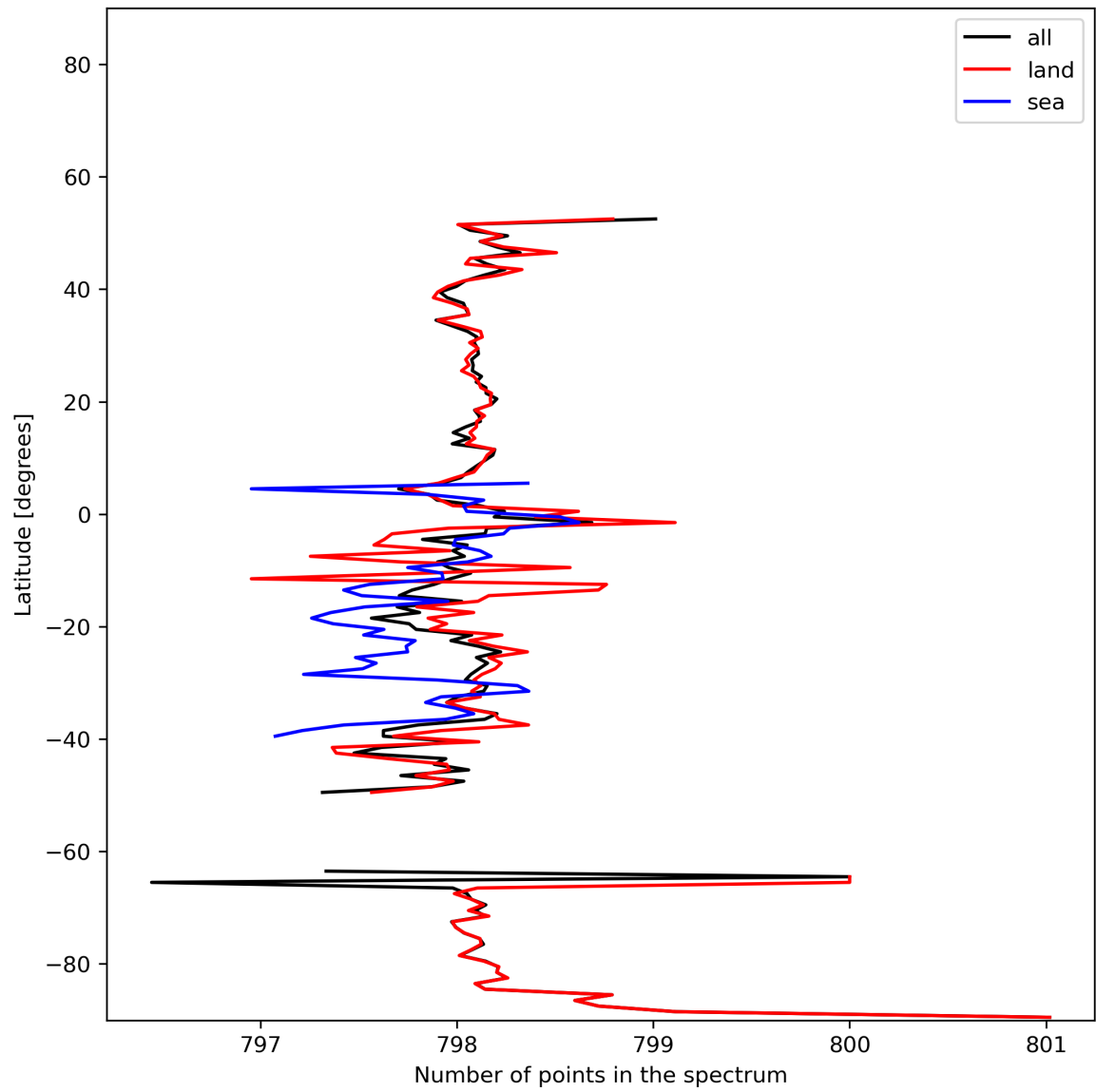
Figure 15: Zonal average of “Number of points in the spectrum” for 2023-12-04 to 2023-12-05.
