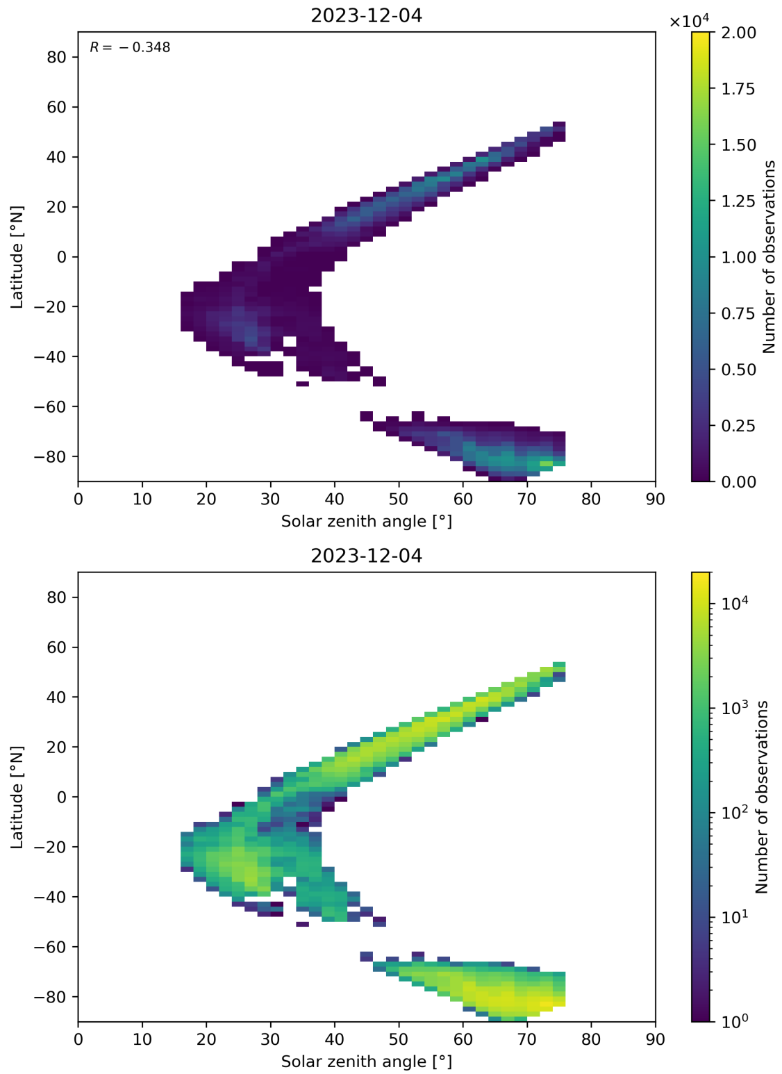
Figure 98: Scatter density plot of “Solar zenith angle” against “Latitude” for 2023-12-04 to 2023-12-05.
