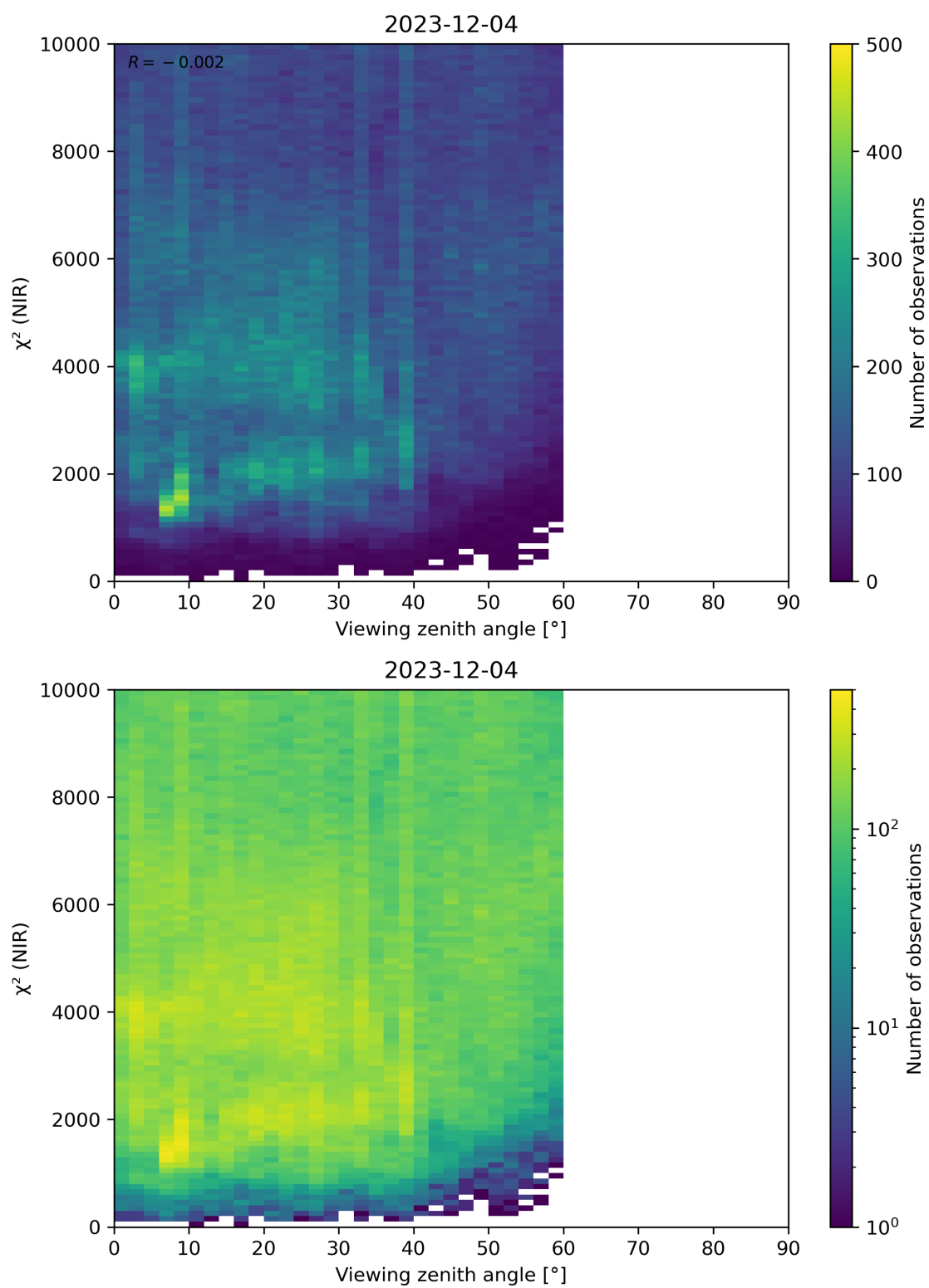
Figure 105: Scatter density plot of “Viewing zenith angle” against “ \chi^2 (NIR)” for 2023-12-04 to 2023-12-05.
