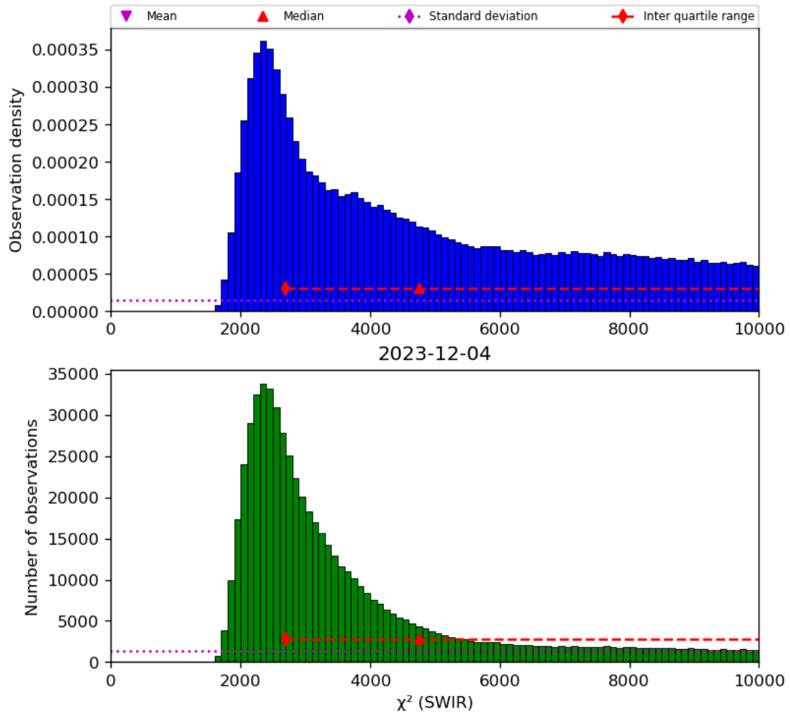
Figure 28: Histogram of “ \chi^2 (SWIR)” for 2023-12-04 to 2023-12-05
