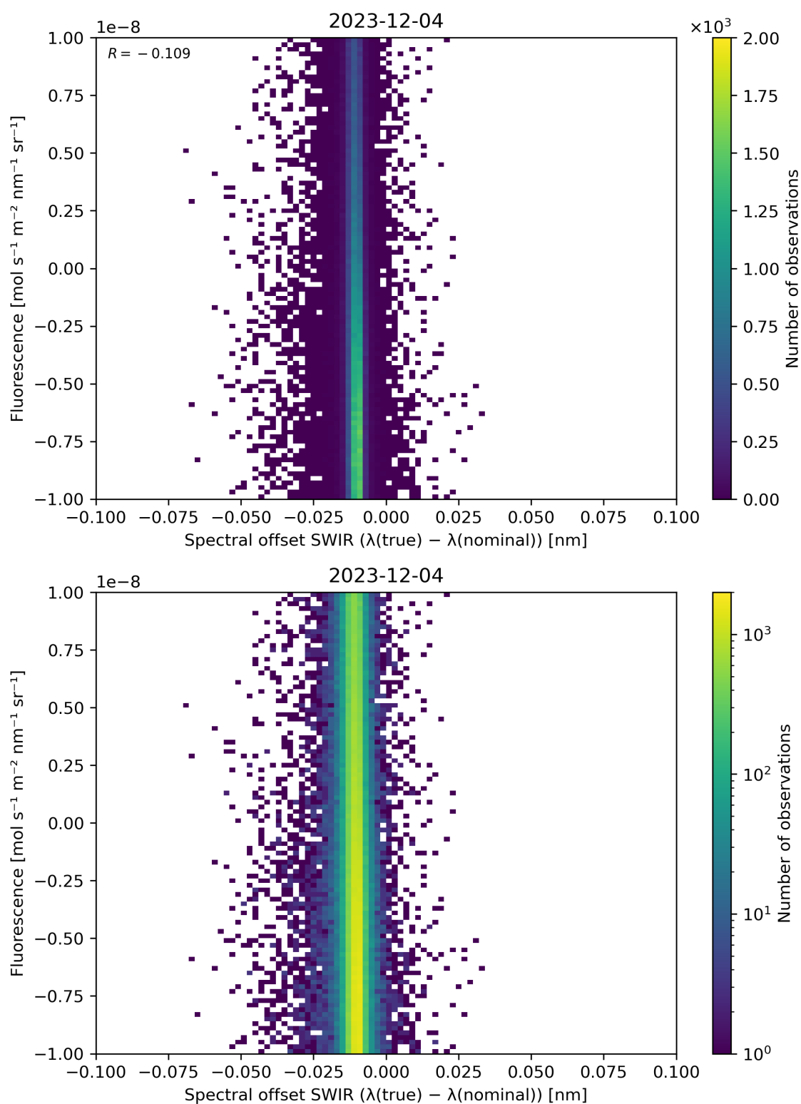
Figure 120: Scatter density plot of “Spectral offset SWIR ( \lambda(\text{true}) - \lambda(\text{nominal}) )” against “Fluorescence” for 2023-12-04 to 2023-12-05.
