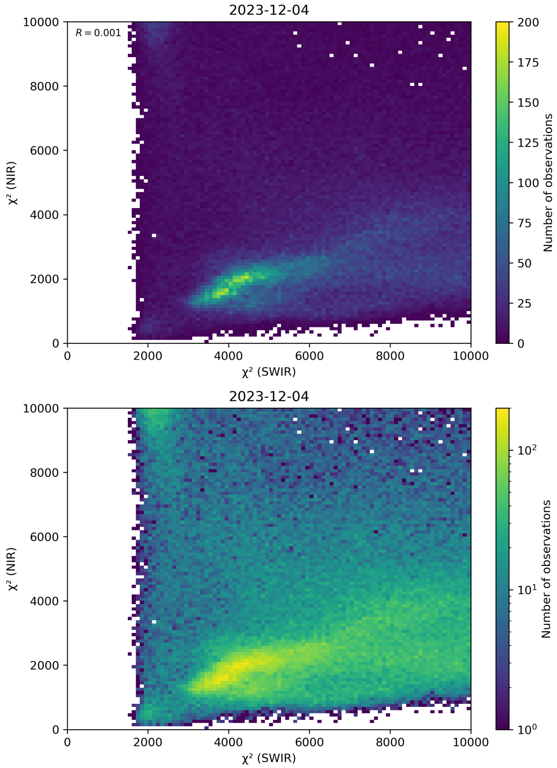
Figure 47: Scatter density plot of “ \chi^2 (SWIR)” against “ \chi^2 (NIR)” for 2023-12-04 to 2023-12-05.
