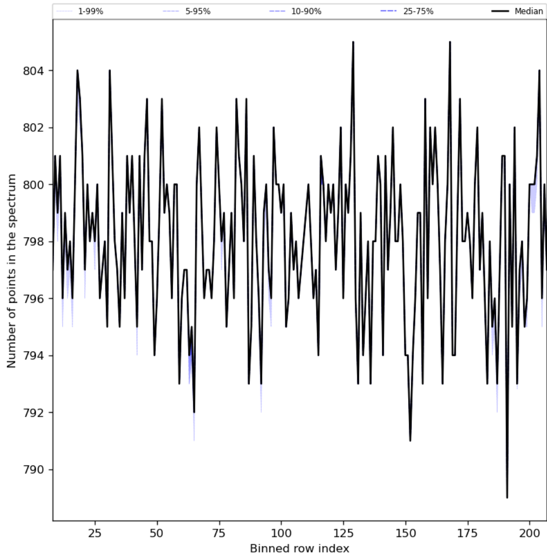
Figure 37: Along track statistics of “Number of points in the spectrum” for 2023-12-04 to 2023-12-05
