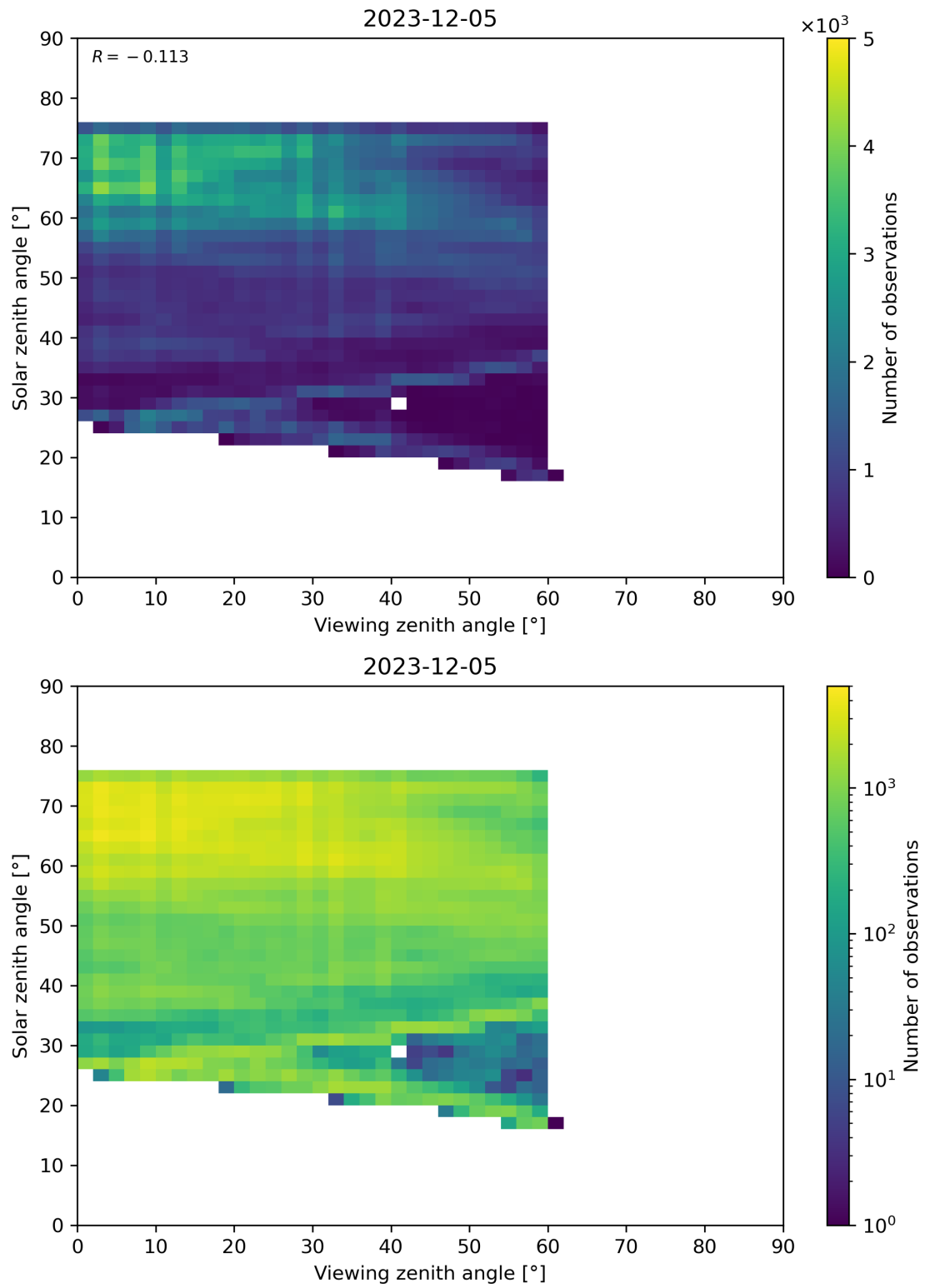
Figure 115: Scatter density plot of “Viewing zenith angle” against “Solar zenith angle” for 2023-12-04 to 2023-12-06.
