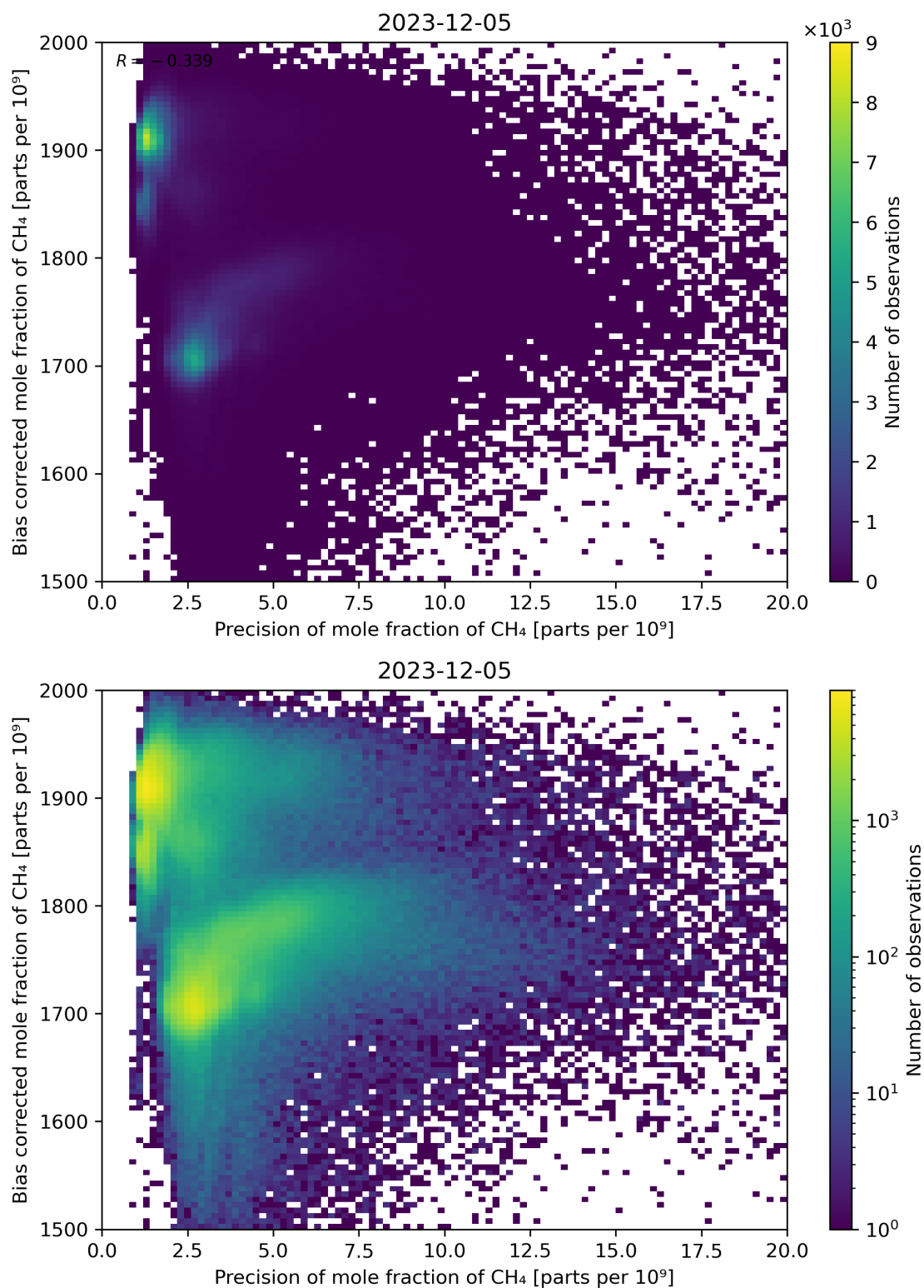
Figure 82: Scatter density plot of “Precision of mole fraction of CH 4 ” against “Bias corrected mole fraction of CH 4 ” for 2023-12-04 to 2023-12-06.
