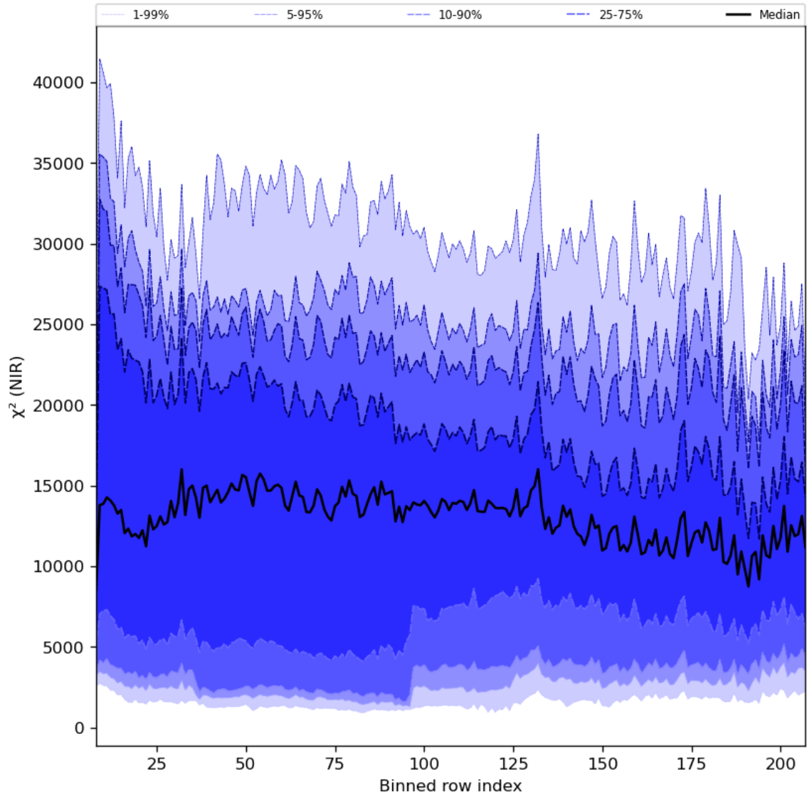
Figure 40: Along track statistics of " \chi^2 (NIR)" for 2023-12-04 to 2023-12-06
