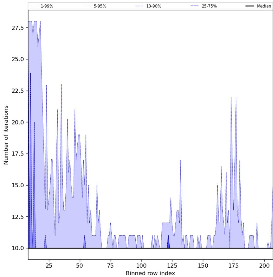
Figure 42: Along track statistics of “Number of iterations” for 2023-12-04 to 2023-12-06
