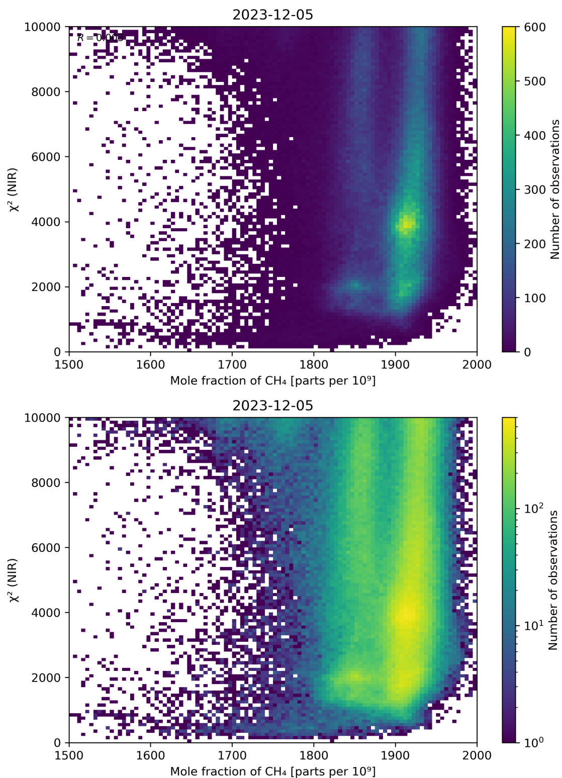
Figure 70: Scatter density plot of “Mole fraction of \text{CH}_4 ” against “ \chi^2 (NIR)” for 2023-12-04 to 2023-12-06.
