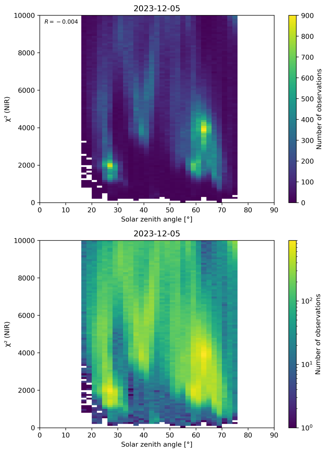
Figure 94: Scatter density plot of “Solar zenith angle” against “ \chi^2 (NIR)” for 2023-12-04 to 2023-12-06.
