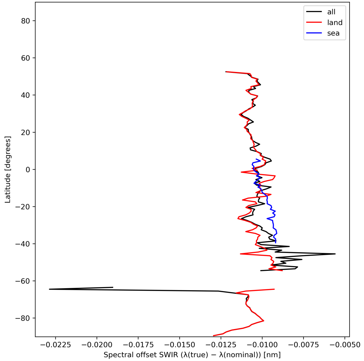
Figure 16: Zonal average of “Spectral offset SWIR ( \lambda(\text{true}) - \lambda(\text{nominal}) )” for 2023-12-04 to 2023-12-06.
