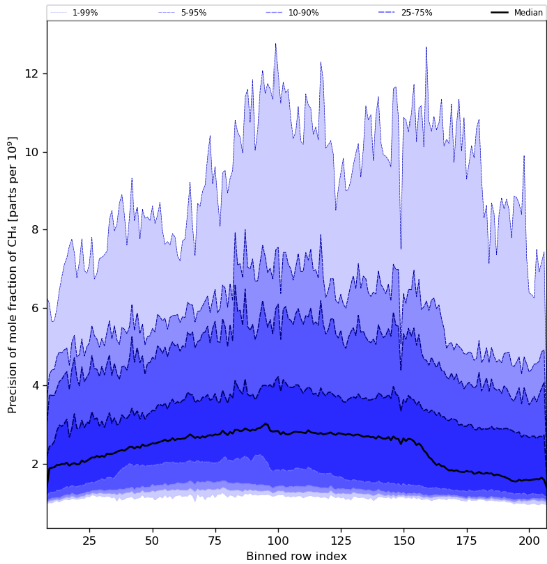
Figure 35: Along track statistics of “Precision of mole fraction of CH 4 ” for 2023-12-04 to 2023-12-06
