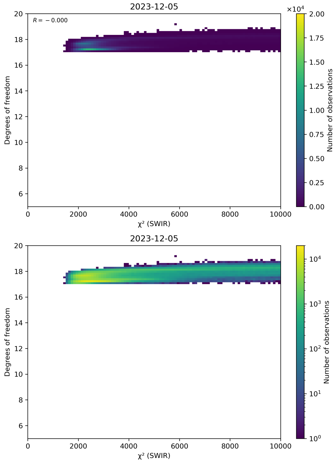
Figure 48: Scatter density plot of “ \chi^2 (SWIR)” against “Degrees of freedom” for 2023-12-04 to 2023-12-06.
