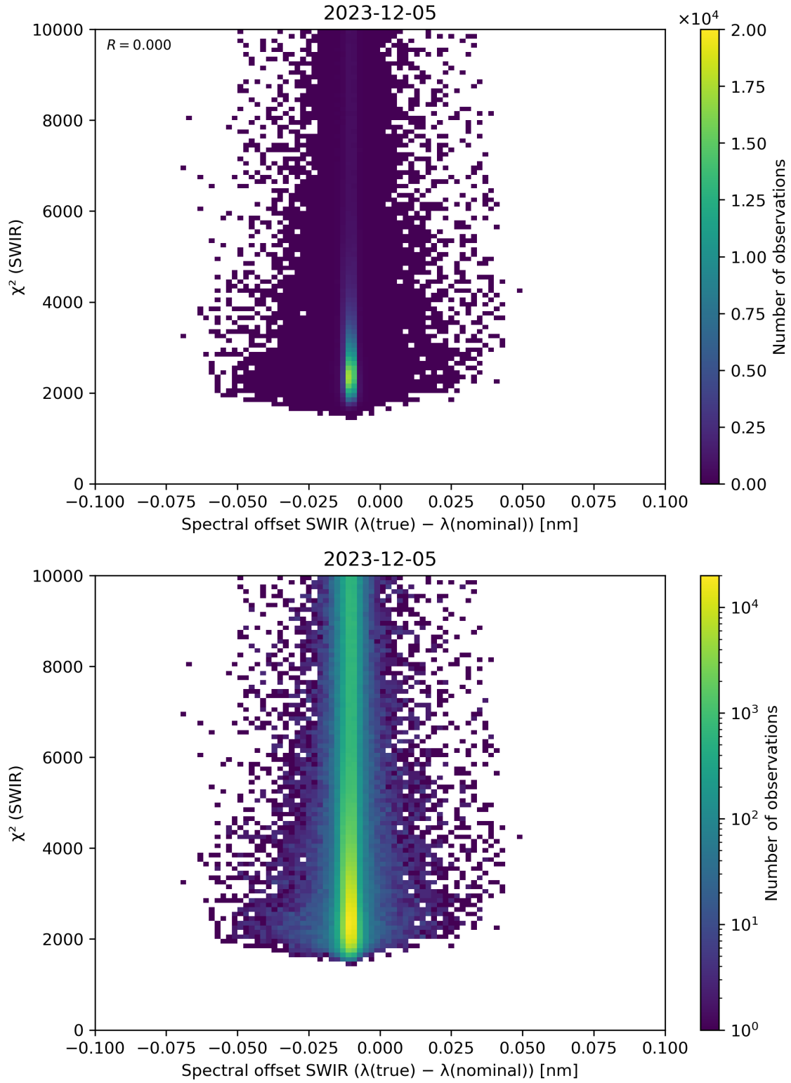
Figure 118: Scatter density plot of “Spectral offset SWIR ( \lambda(\text{true}) - \lambda(\text{nominal}) )” against “ \chi^2 (SWIR)” for 2023-12-04 to 2023-12-06.
