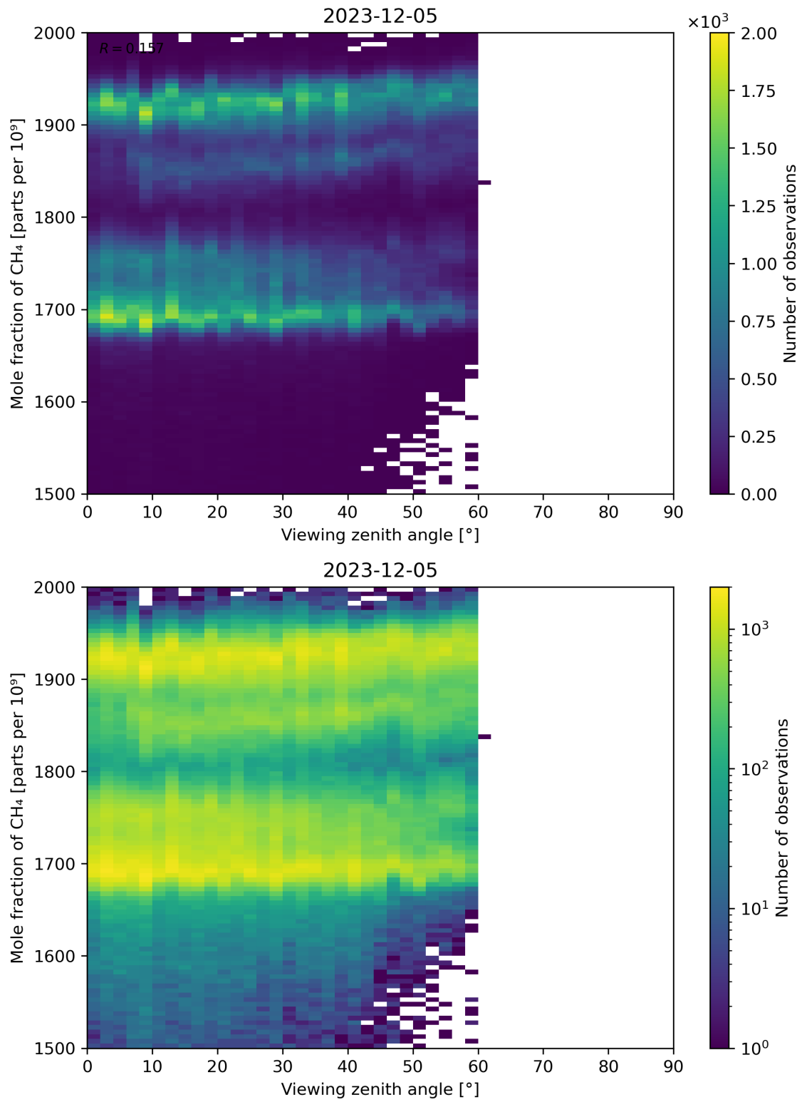
Figure 110: Scatter density plot of “Viewing zenith angle” against “Mole fraction of CH 4 ” for 2023-12-04 to 2023-12-06.
