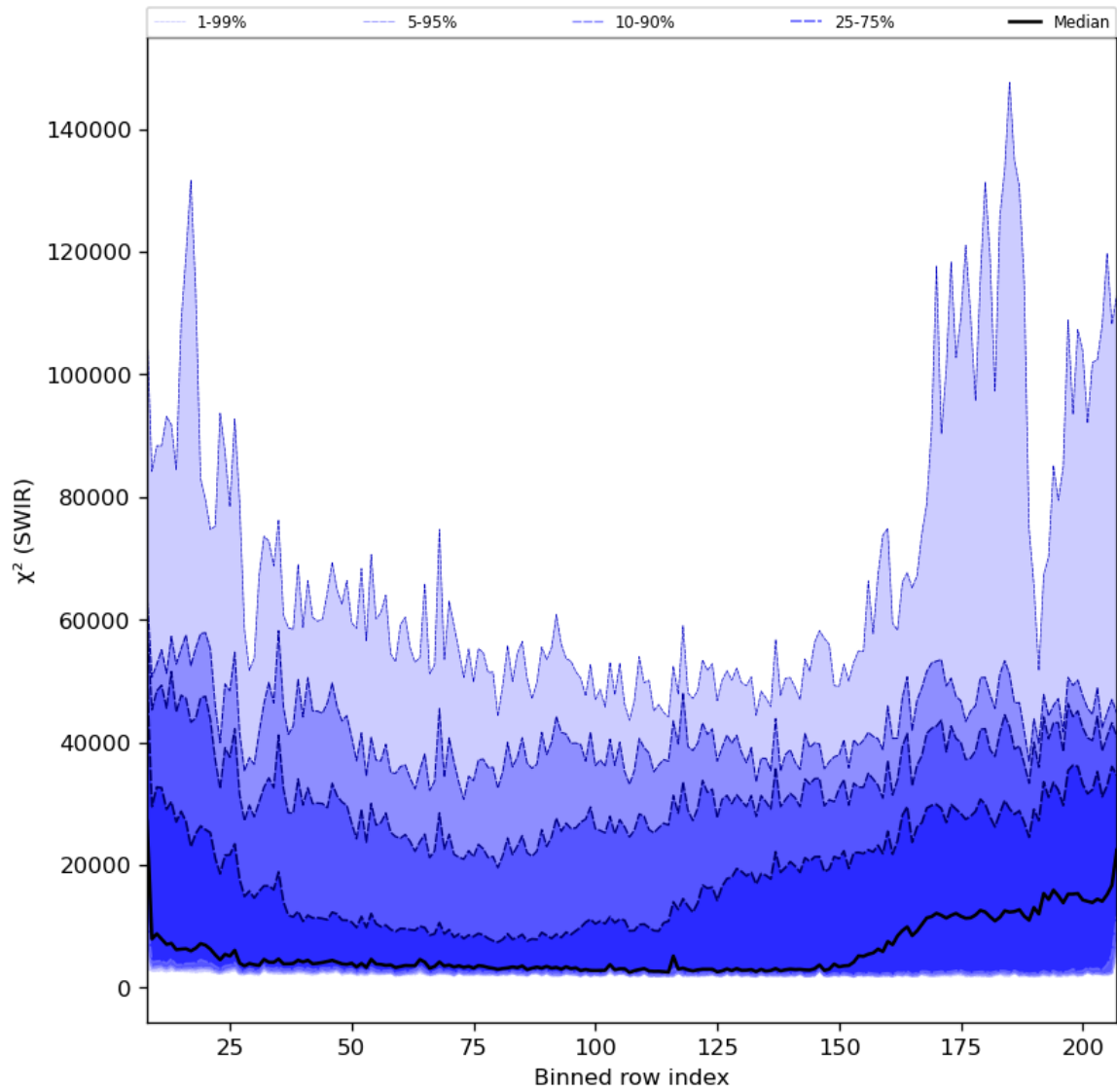
Figure 39: Along track statistics of “ \chi^2 (SWIR)” for 2023-12-04 to 2023-12-06
