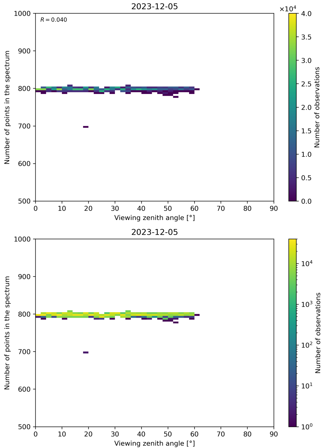
Figure 114: Scatter density plot of “Viewing zenith angle” against “Number of points in the spectrum” for 2023-12-04 to 2023-12-06.
