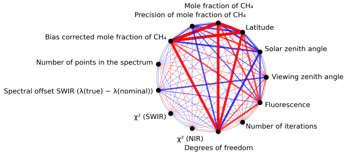
Figure 1: Map of correlation graph for 2023-12-04 to 2023-12-06.
