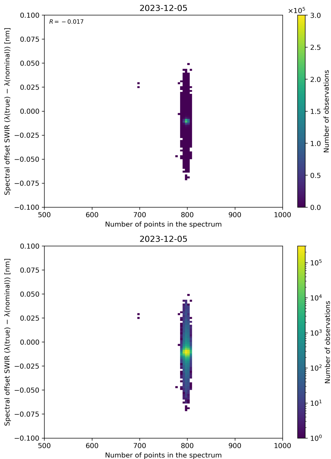
Figure 93: Scatter density plot of “Number of points in the spectrum” against “Spectral offset SWIR ( \lambda(\text{true}) - \lambda(\text{nominal}) )” for 2023-12-04 to 2023-12-06.
