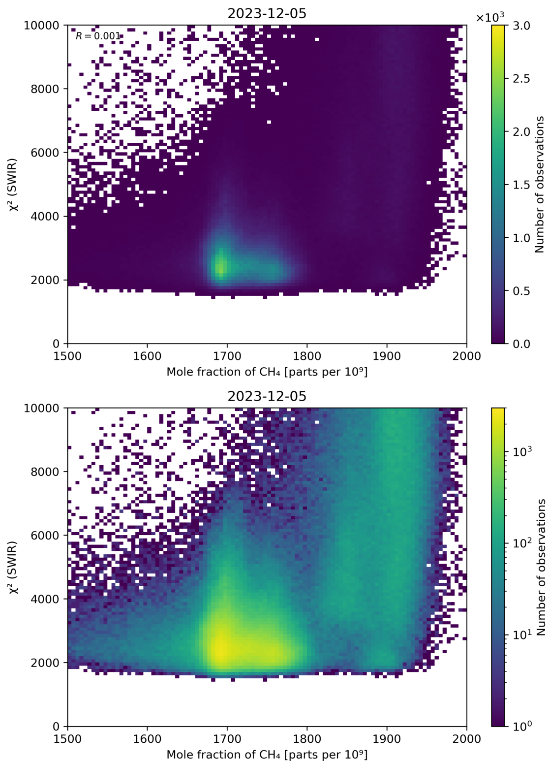
Figure 71: Scatter density plot of “Mole fraction of \text{CH}_4 ” against “ \chi^2 (SWIR)” for 2023-12-04 to 2023-12-06.
