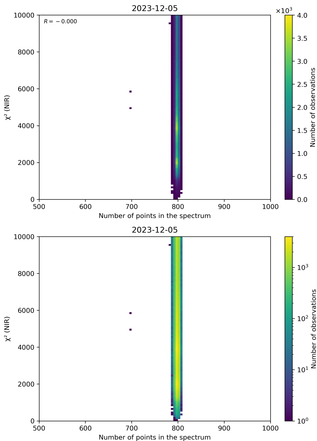
Figure 88: Scatter density plot of “Number of points in the spectrum” against “ \chi^2 (NIR)” for 2023-12-04 to 2023-12-06.
