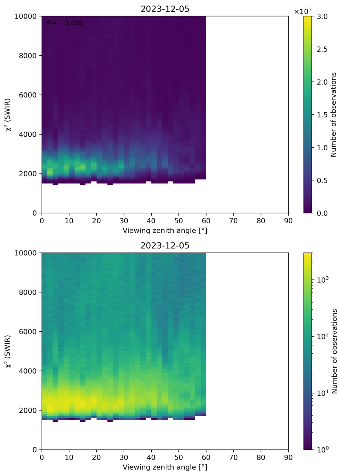
Figure 106: Scatter density plot of “Viewing zenith angle” against “ \chi^2 (SWIR)” for 2023-12-04 to 2023-12-06.
