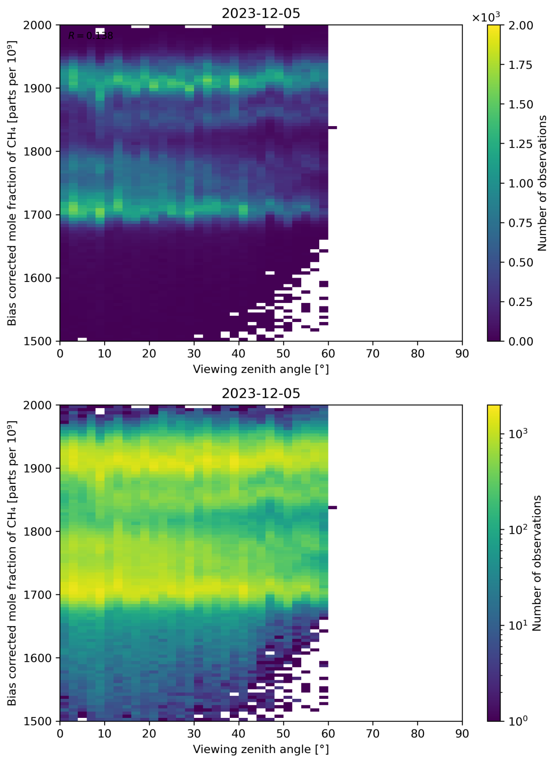
Figure 111: Scatter density plot of “Viewing zenith angle” against “Bias corrected mole fraction of CH 4 ” for 2023-12-04 to 2023-12-06.
