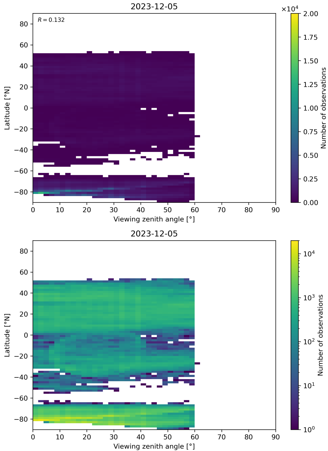
Figure 109: Scatter density plot of “Viewing zenith angle” against “Latitude” for 2023-12-04 to 2023-12-06.
