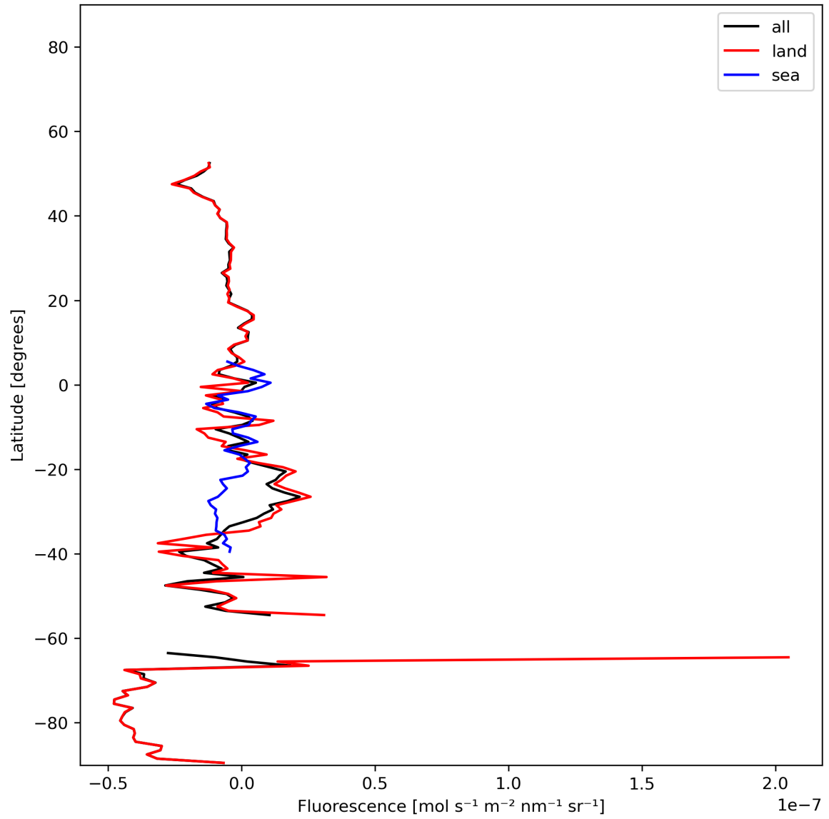
Figure 21: Zonal average of “Fluorescence” for 2023-12-04 to 2023-12-06.
