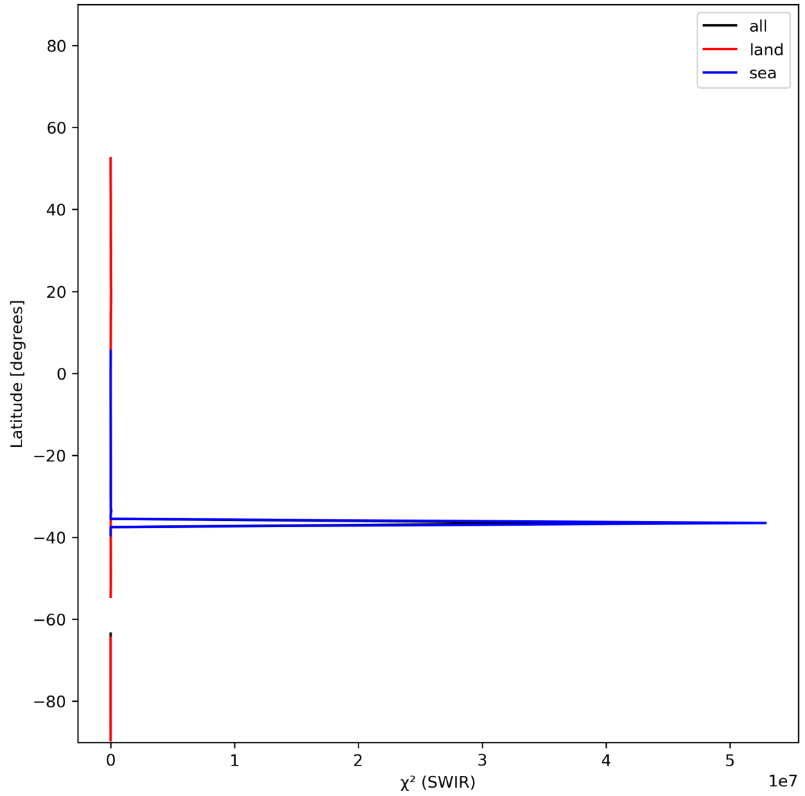
Figure 17: Zonal average of “ \chi^2 (SWIR)” for 2023-12-04 to 2023-12-06.
