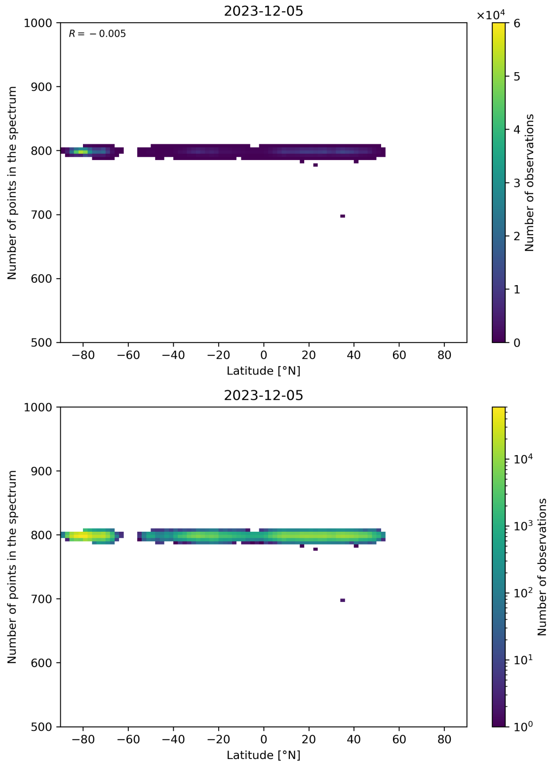
Figure 61: Scatter density plot of “Latitude” against “Number of points in the spectrum” for 2023-12-04 to 2023-12-06.
