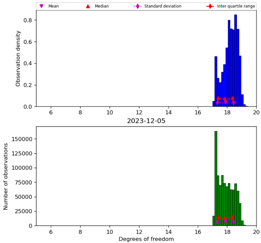
Figure 30: Histogram of “Degrees of freedom” for 2023-12-04 to 2023-12-06
