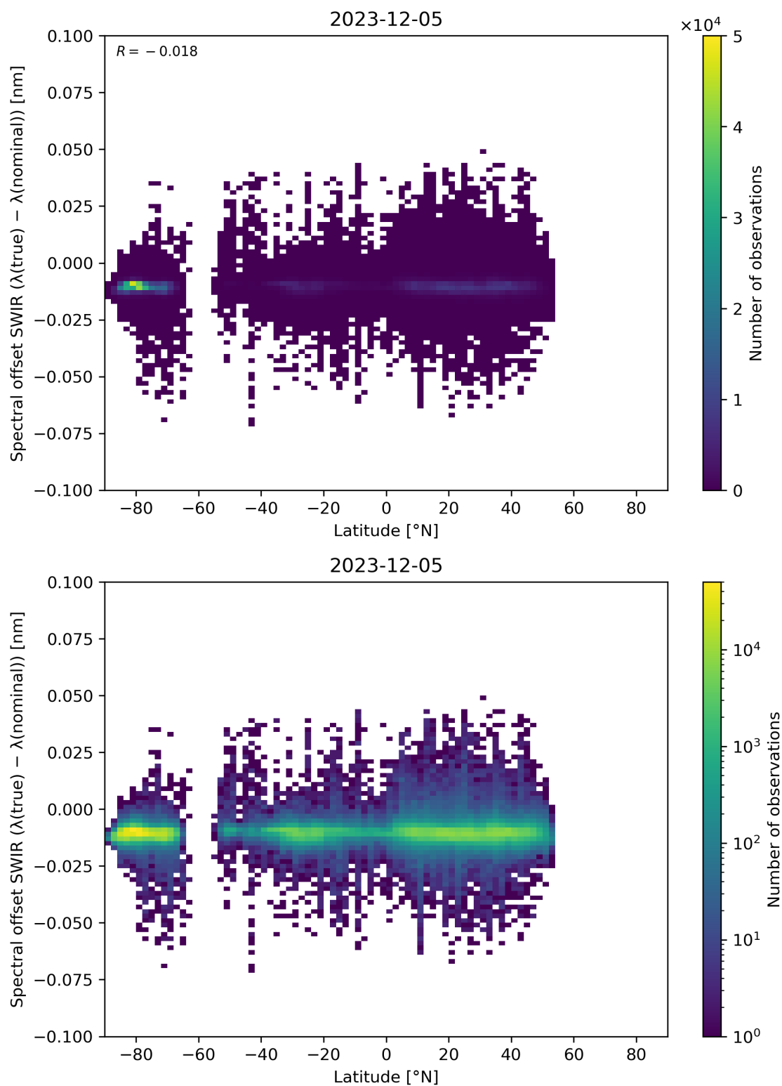
Figure 62: Scatter density plot of “Latitude” against “Spectral offset SWIR ( \lambda(\text{true}) - \lambda(\text{nominal}) )” for 2023-12-04 to 2023-12-06.
