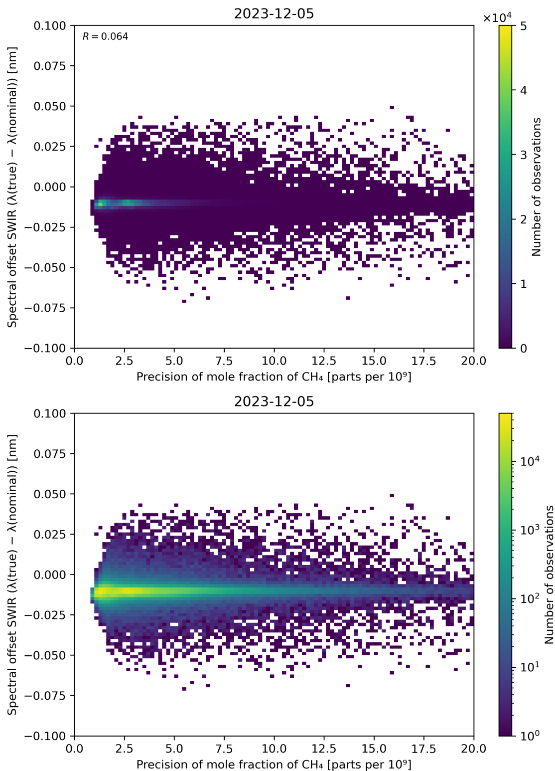
Figure 85: Scatter density plot of “Precision of mole fraction of CH 4 ” against “Spectral offset SWIR ( \lambda(\text{true}) - \lambda(\text{nominal}) )” for 2023-12-04 to 2023-12-06.
