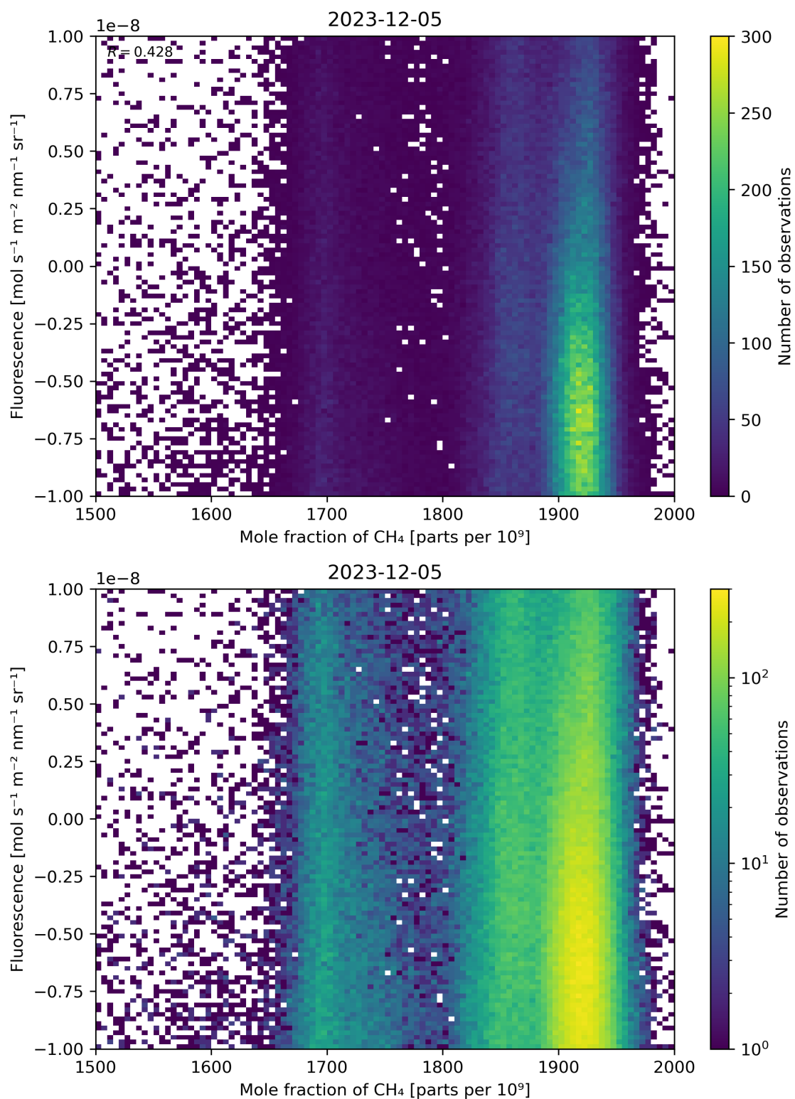
Figure 73: Scatter density plot of “Mole fraction of CH 4 ” against “Fluorescence” for 2023-12-04 to 2023-12-06.
