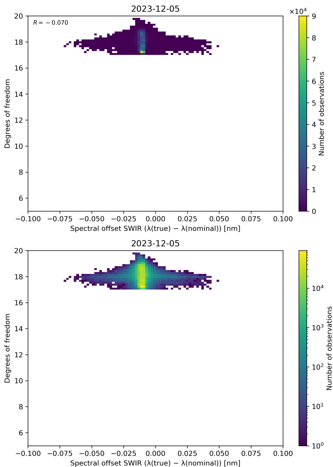
Figure 119: Scatter density plot of “Spectral offset SWIR ( \lambda(\text{true}) - \lambda(\text{nominal}) )” against “Degrees of freedom” for 2023-12-04 to 2023-12-06.
