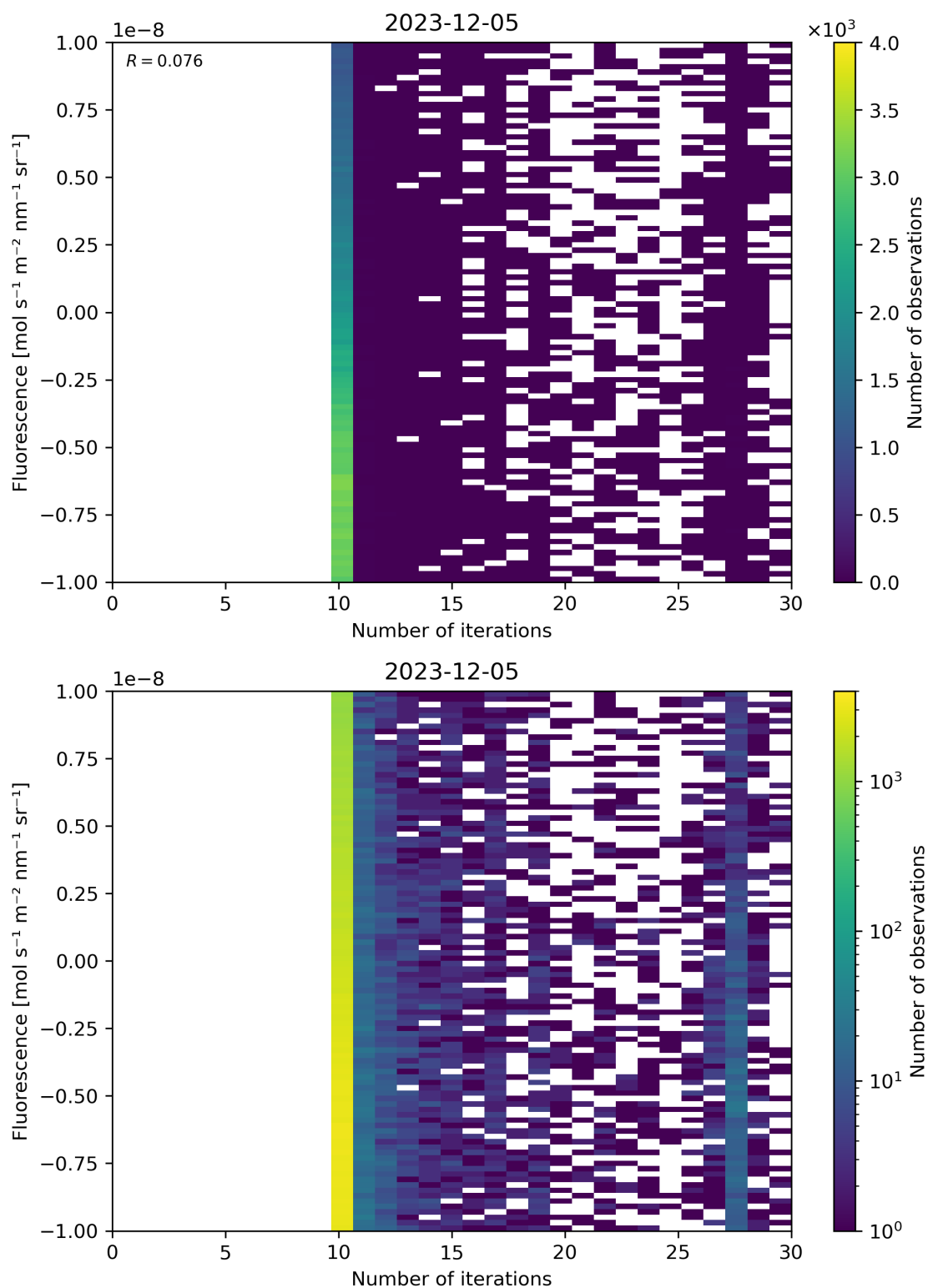
Figure 87: Scatter density plot of “Number of iterations” against “Fluorescence” for 2023-12-04 to 2023-12-06.
