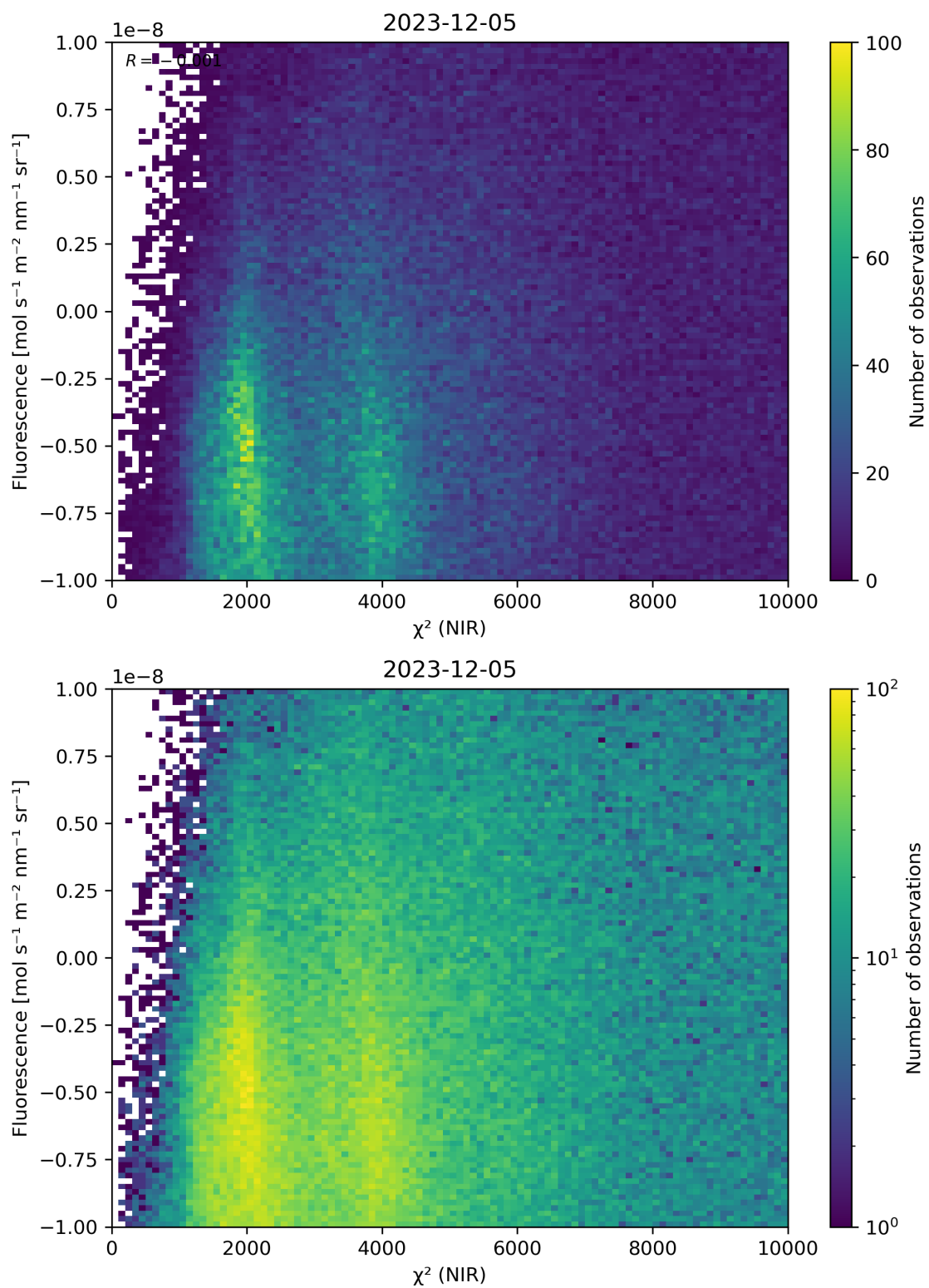
Figure 45: Scatter density plot of “ \chi^2 (NIR)” against “Fluorescence” for 2023-12-04 to 2023-12-06.
