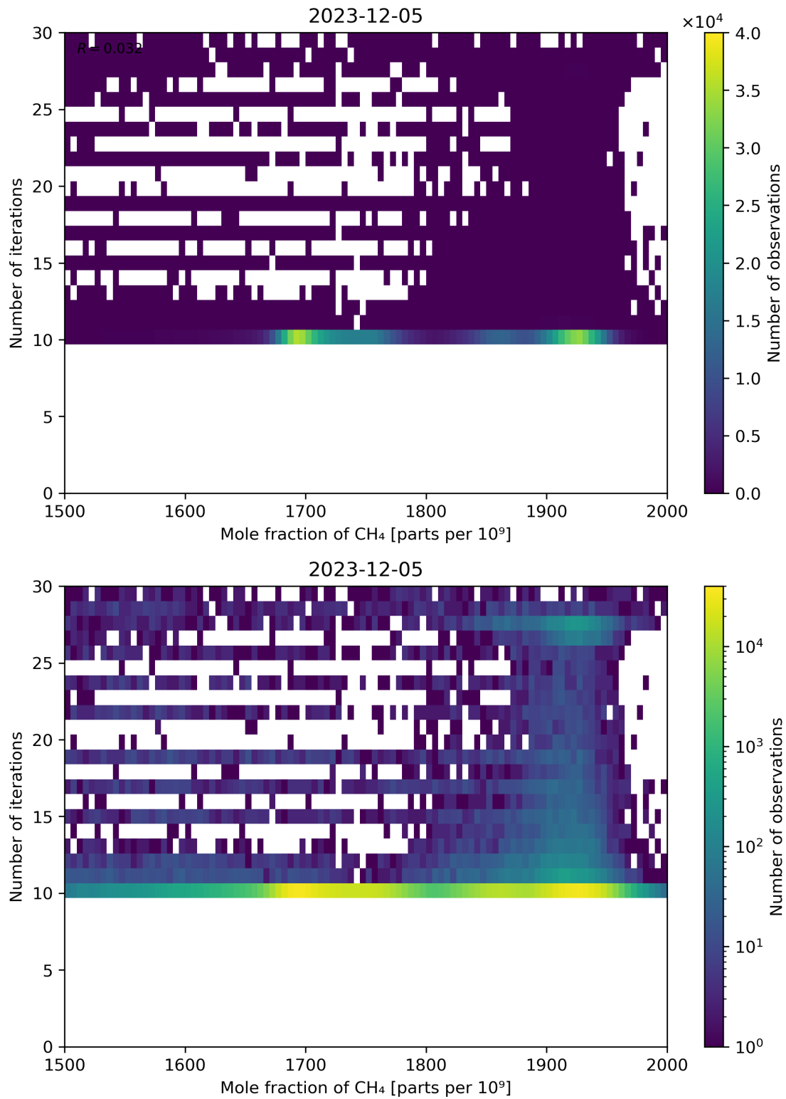
Figure 76: Scatter density plot of “Mole fraction of CH 4 ” against “Number of iterations” for 2023-12-04 to 2023-12-06.
