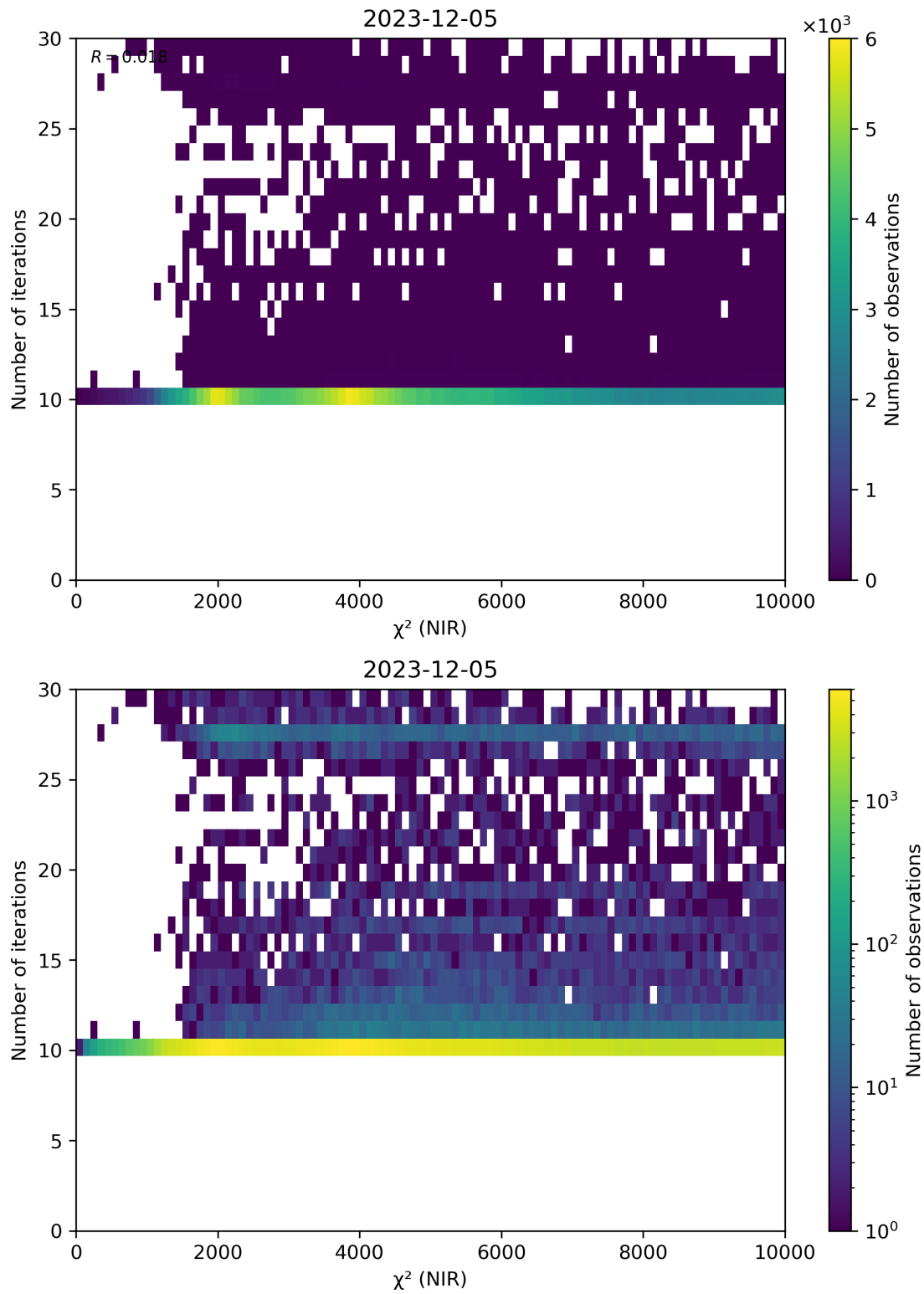
Figure 46: Scatter density plot of “ \chi^2 (NIR)” against “Number of iterations” for 2023-12-04 to 2023-12-06.
