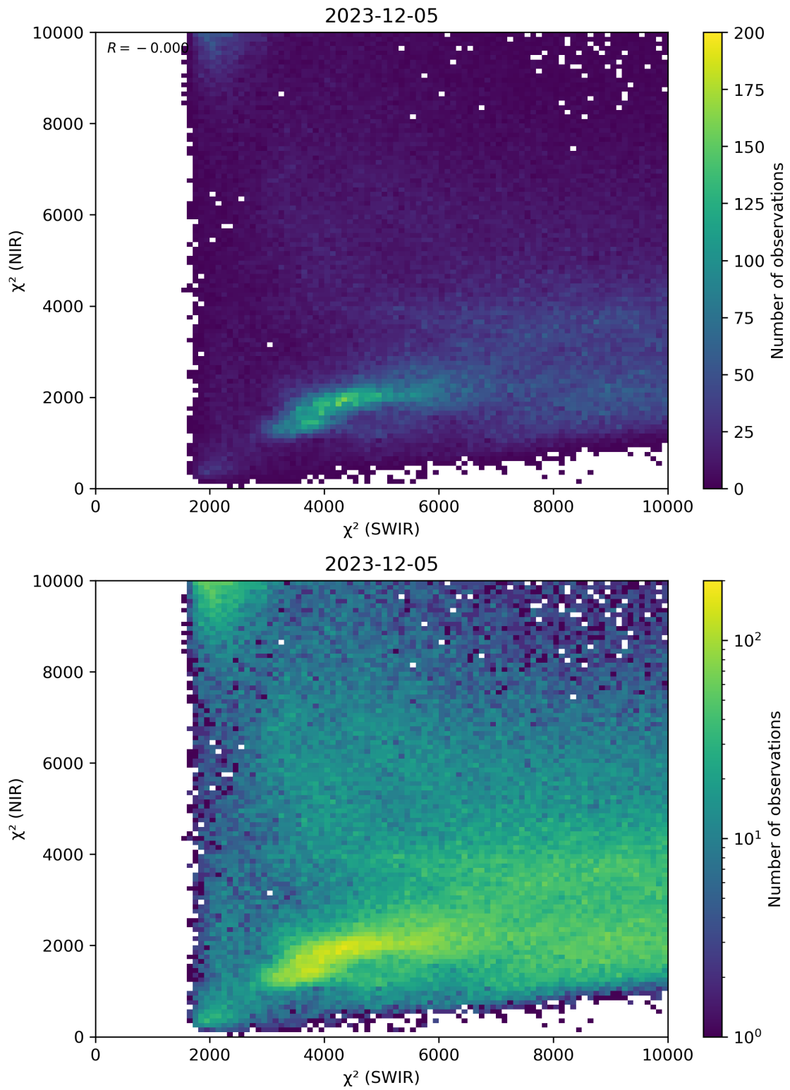
Figure 47: Scatter density plot of “ \chi^2 (SWIR)” against “ \chi^2 (NIR)” for 2023-12-04 to 2023-12-06.
