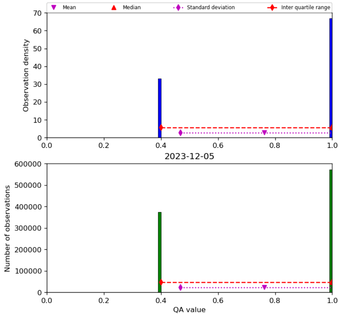
Figure 22: Histogram of “QA value” for 2023-12-04 to 2023-12-06
