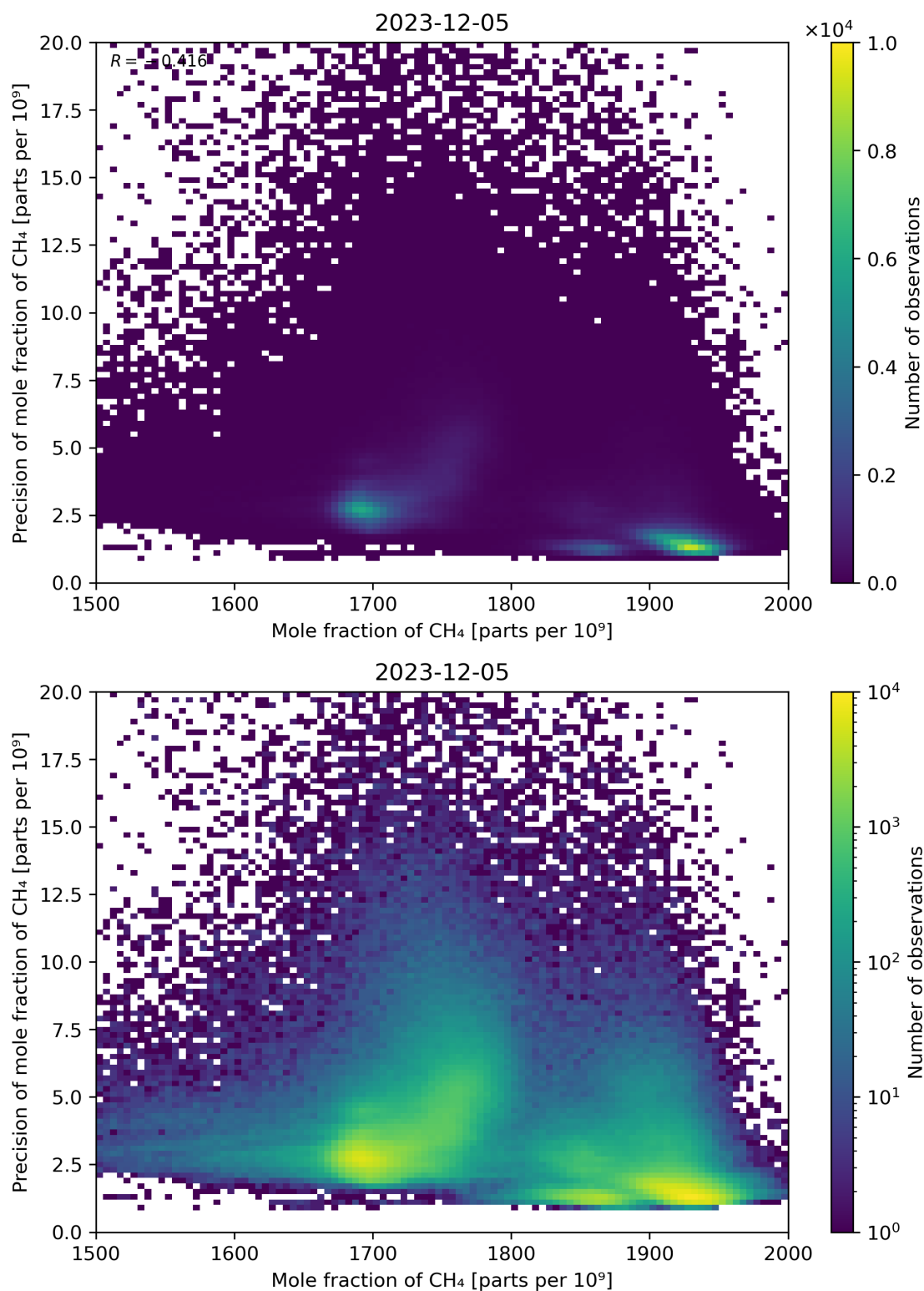
Figure 75: Scatter density plot of “Mole fraction of CH 4 ” against “Precision of mole fraction of CH 4 ” for 2023-12-04 to 2023-12-06.
