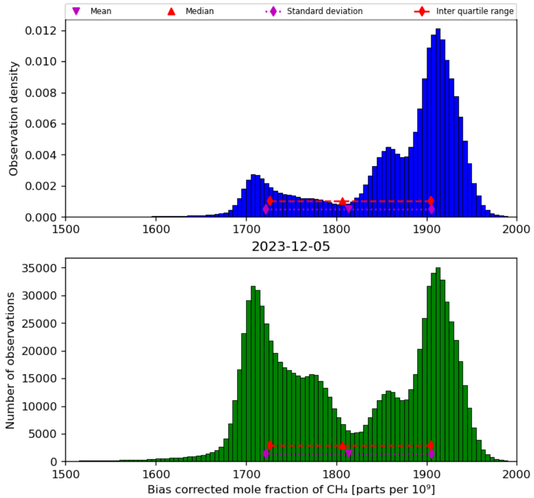
Figure 25: Histogram of “Bias corrected mole fraction of CH 4 ” for 2023-12-04 to 2023-12-06
