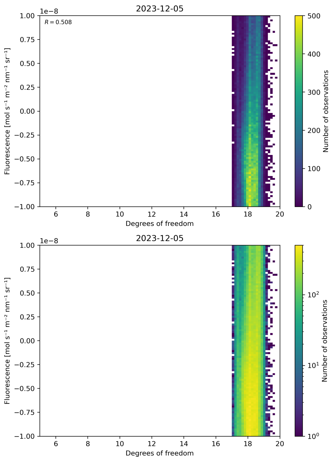
Figure 51: Scatter density plot of “Degrees of freedom” against “Fluorescence” for 2023-12-04 to 2023-12-06.
