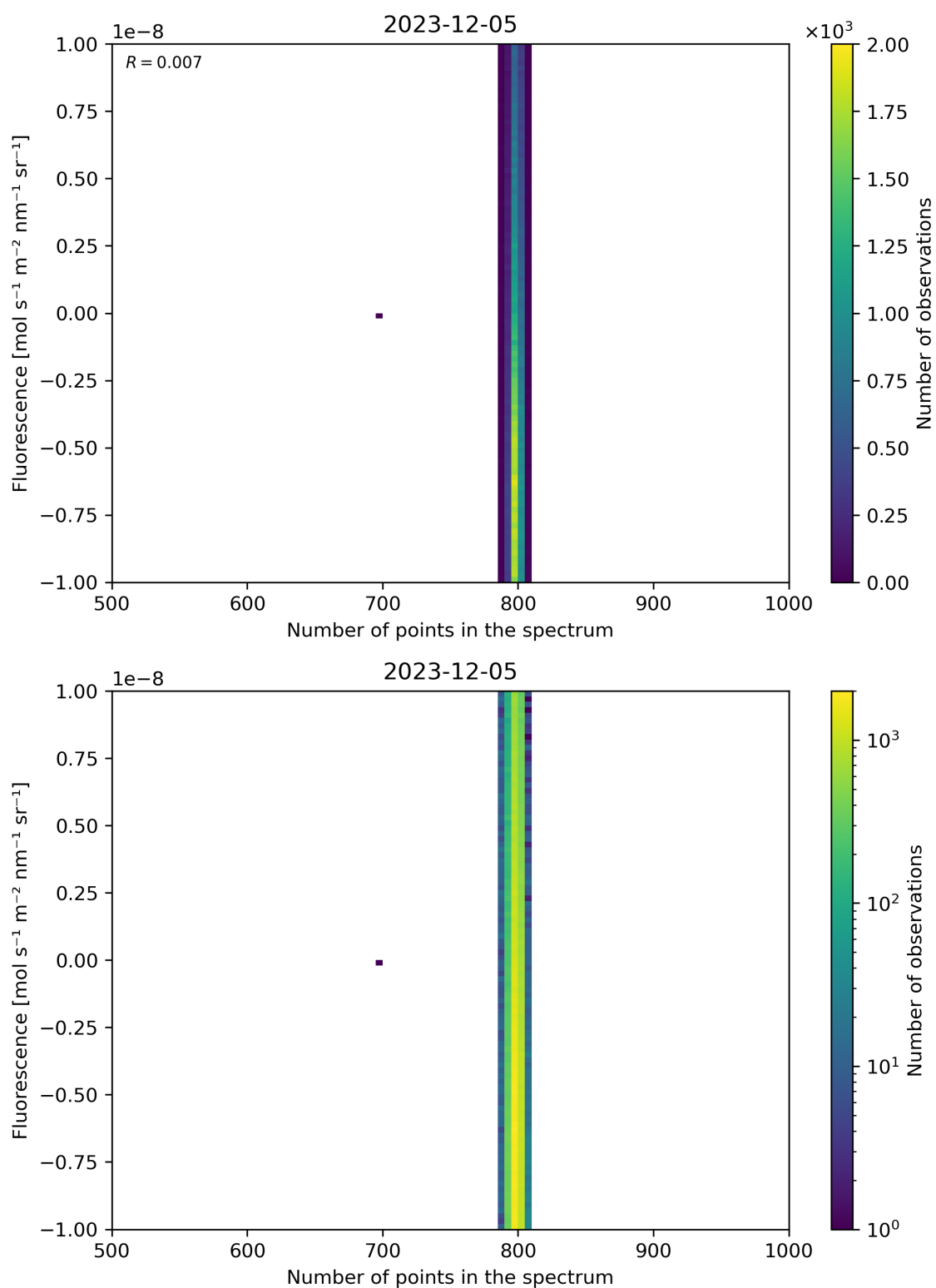
Figure 91: Scatter density plot of “Number of points in the spectrum” against “Fluorescence” for 2023-12-04 to 2023-12-06.
