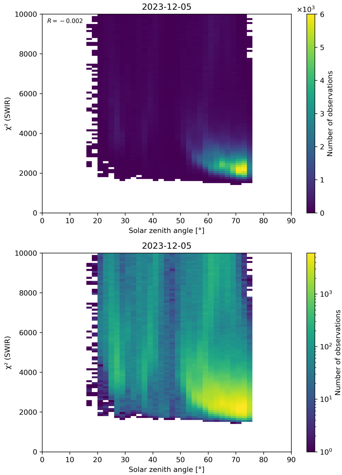
Figure 95: Scatter density plot of “Solar zenith angle” against “ \chi^2 (SWIR)” for 2023-12-04 to 2023-12-06.
