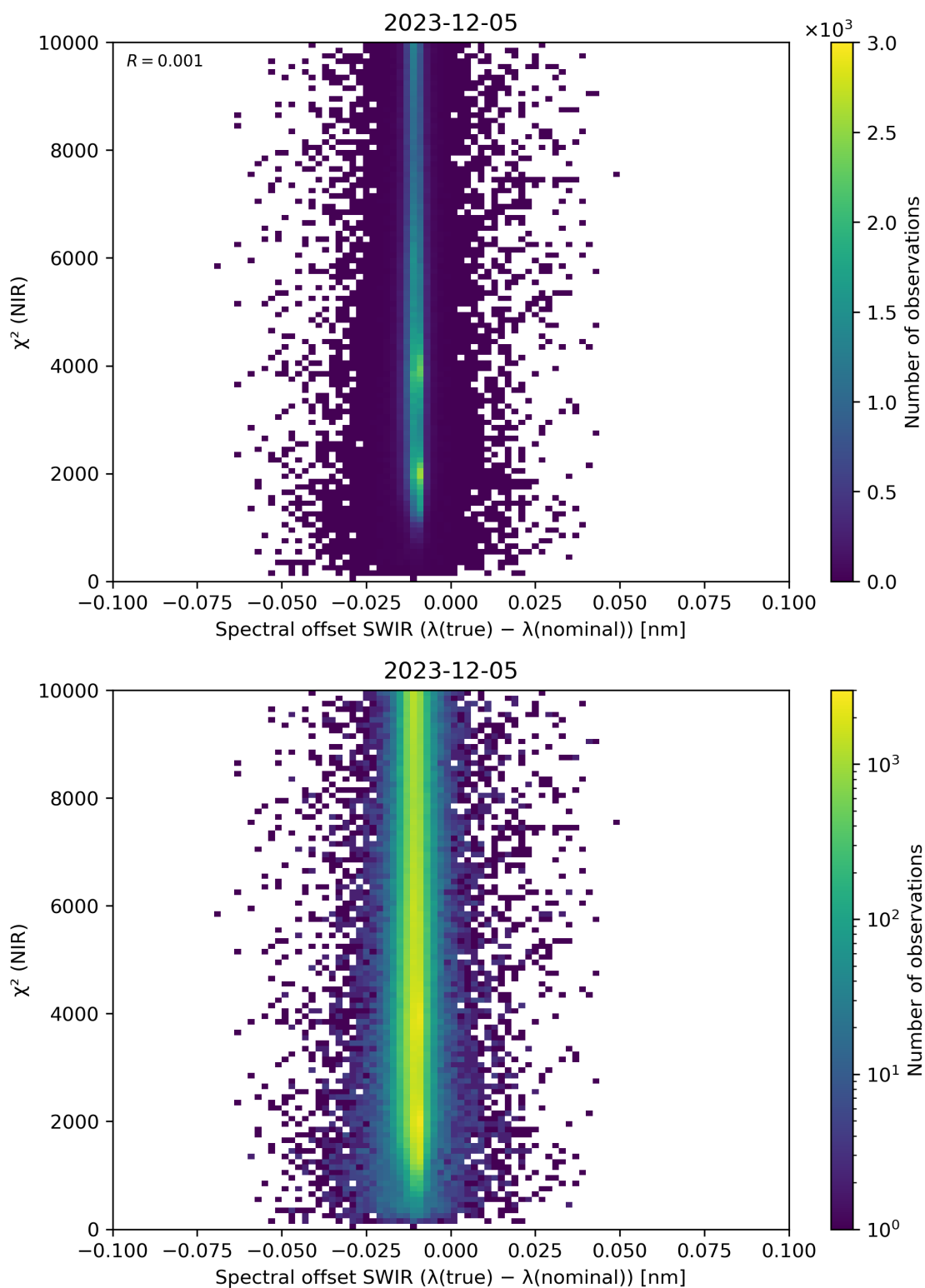
Figure 117: Scatter density plot of “Spectral offset SWIR ( \lambda(\text{true}) - \lambda(\text{nominal}) )” against “ \chi^2 (NIR)” for 2023-12-04 to 2023-12-06.
