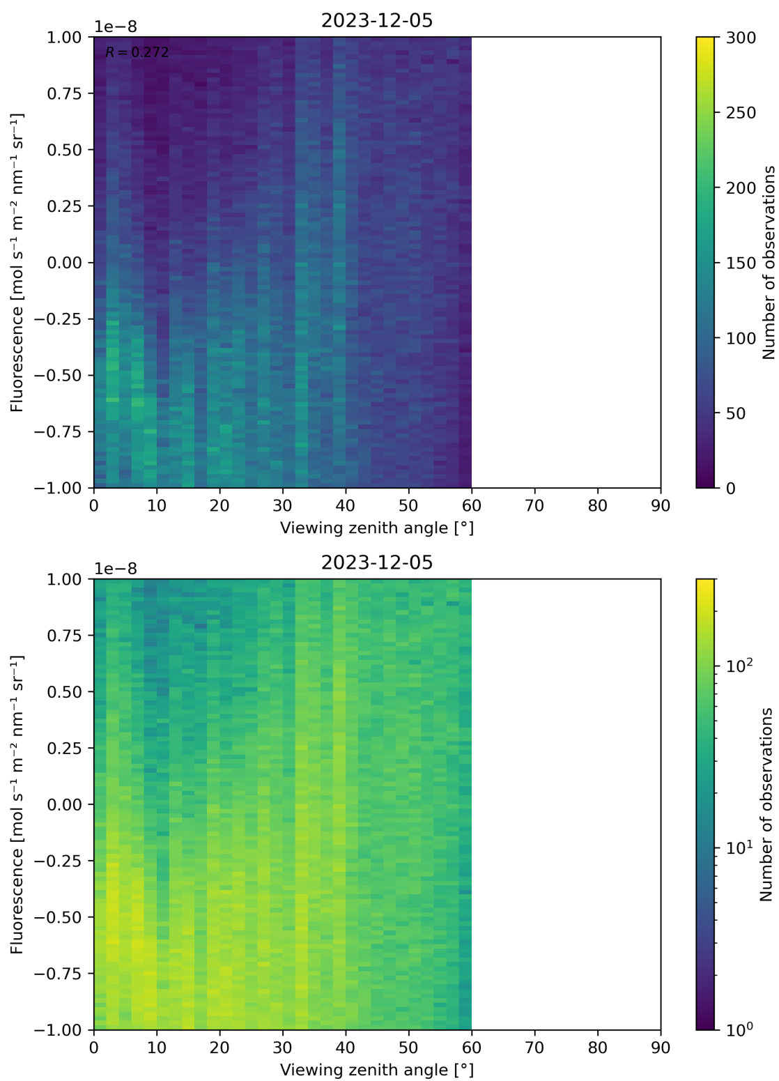
Figure 108: Scatter density plot of “Viewing zenith angle” against “Fluorescence” for 2023-12-04 to 2023-12-06.
