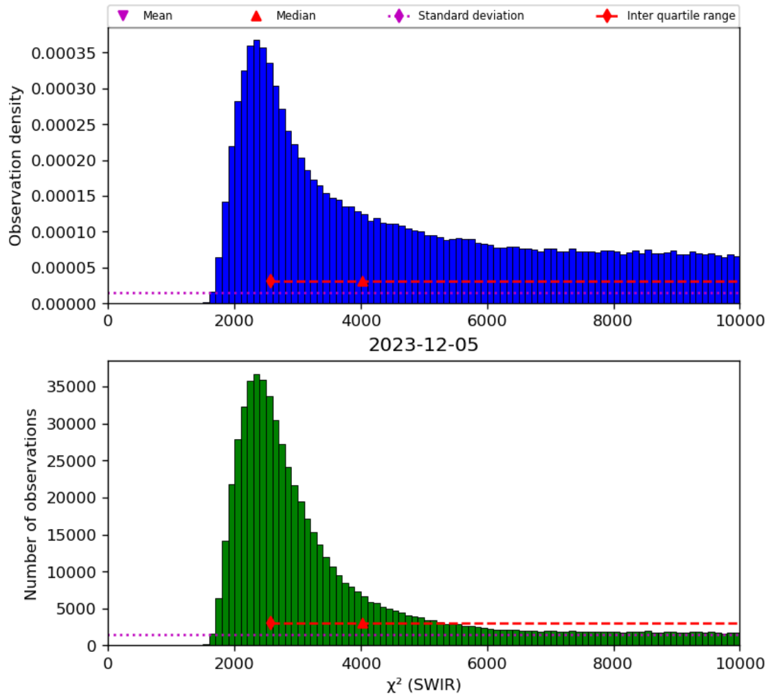
Figure 28: Histogram of “ \chi^2 (SWIR)” for 2023-12-04 to 2023-12-06
