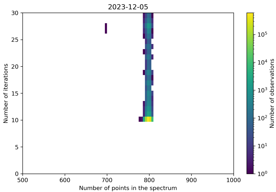
Figure 92: Scatter density plot of “Number of points in the spectrum” against “Number of iterations” for 2023-12-04 to 2023-12-06.
