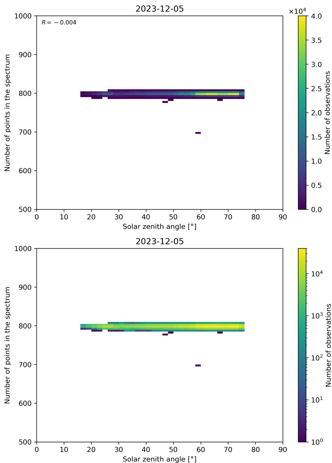
Figure 103: Scatter density plot of “Solar zenith angle” against “Number of points in the spectrum” for 2023-12-04 to 2023-12-06.
