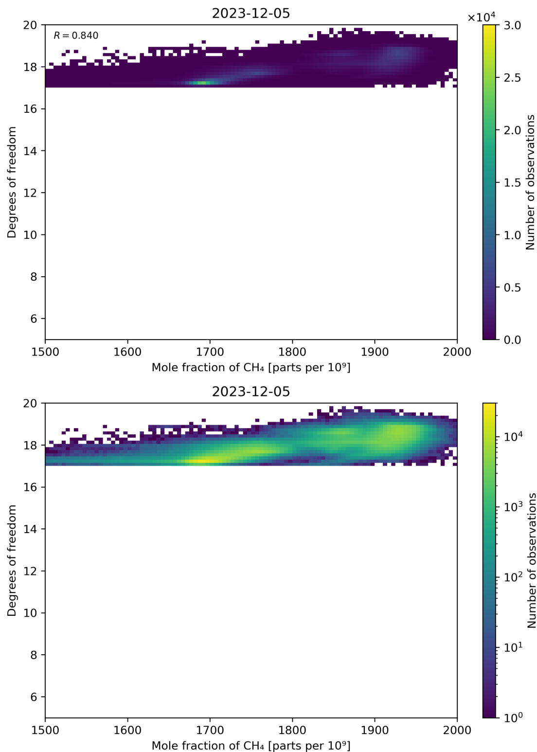
Figure 72: Scatter density plot of “Mole fraction of CH 4 ” against “Degrees of freedom” for 2023-12-04 to 2023-12-06.
