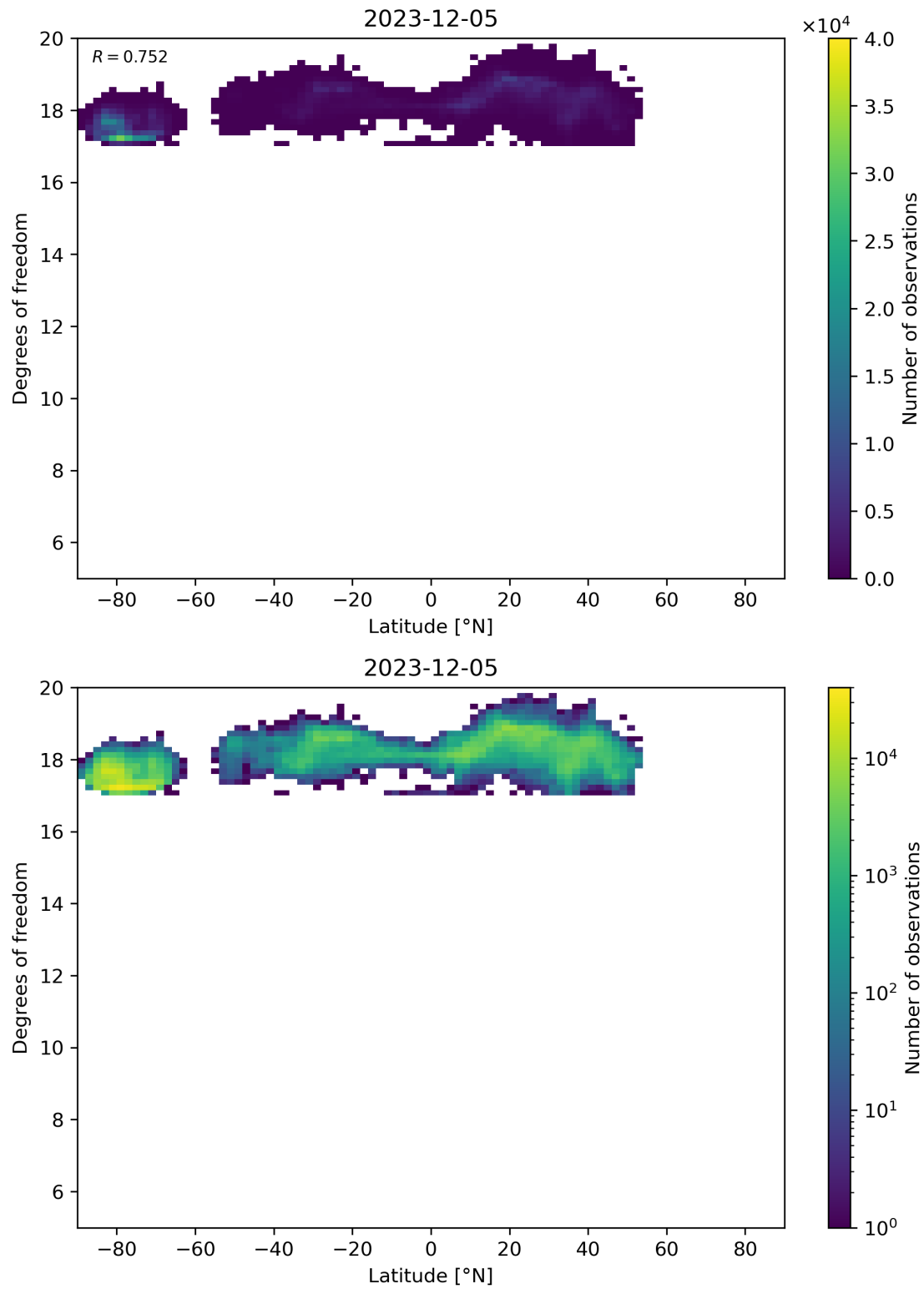
Figure 55: Scatter density plot of “Latitude” against “Degrees of freedom” for 2023-12-04 to 2023-12-06.
