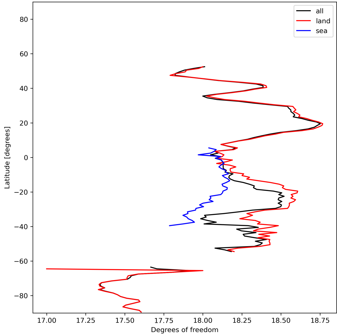
Figure 19: Zonal average of “Degrees of freedom” for 2023-12-04 to 2023-12-06.
