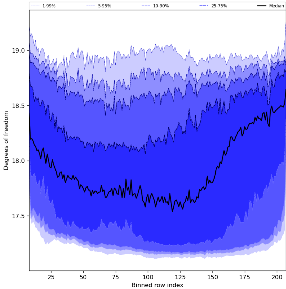
Figure 41: Along track statistics of “Degrees of freedom” for 2023-12-04 to 2023-12-06
