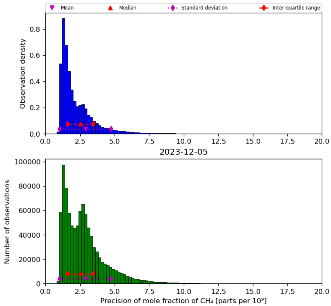
Figure 24: Histogram of “Precision of mole fraction of CH 4 ” for 2023-12-04 to 2023-12-06
