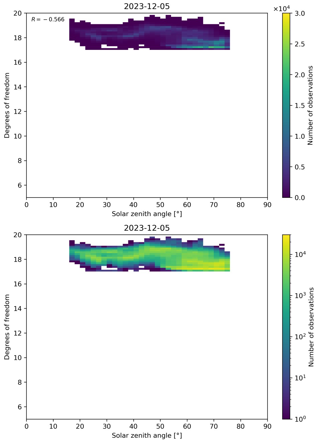
Figure 96: Scatter density plot of “Solar zenith angle” against “Degrees of freedom” for 2023-12-04 to 2023-12-06.
