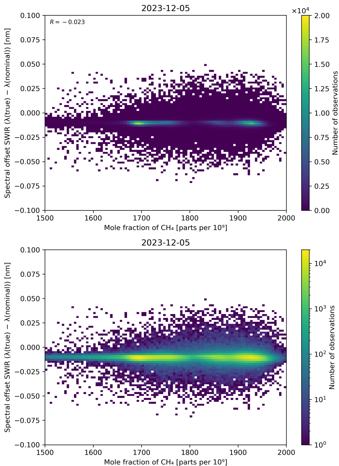
Figure 86: Scatter density plot of “Mole fraction of \text{CH}_4 ” against “Spectral offset SWIR ( \lambda(\text{true}) - \lambda(\text{nominal}) )” for 2023-12-04 to 2023-12-06.
