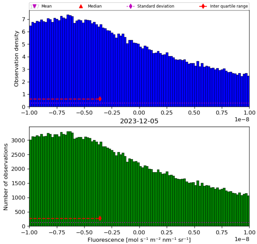
Figure 32: Histogram of “Fluorescence” for 2023-12-04 to 2023-12-06
