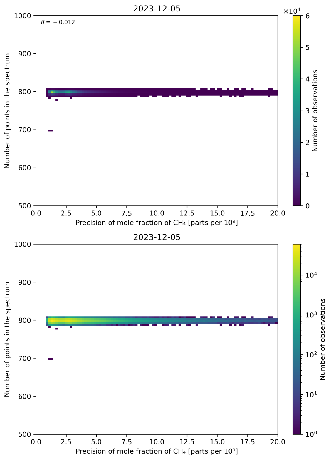
Figure 84: Scatter density plot of “Precision of mole fraction of CH 4 ” against “Number of points in the spectrum” for 2023-12-04 to 2023-12-06.
