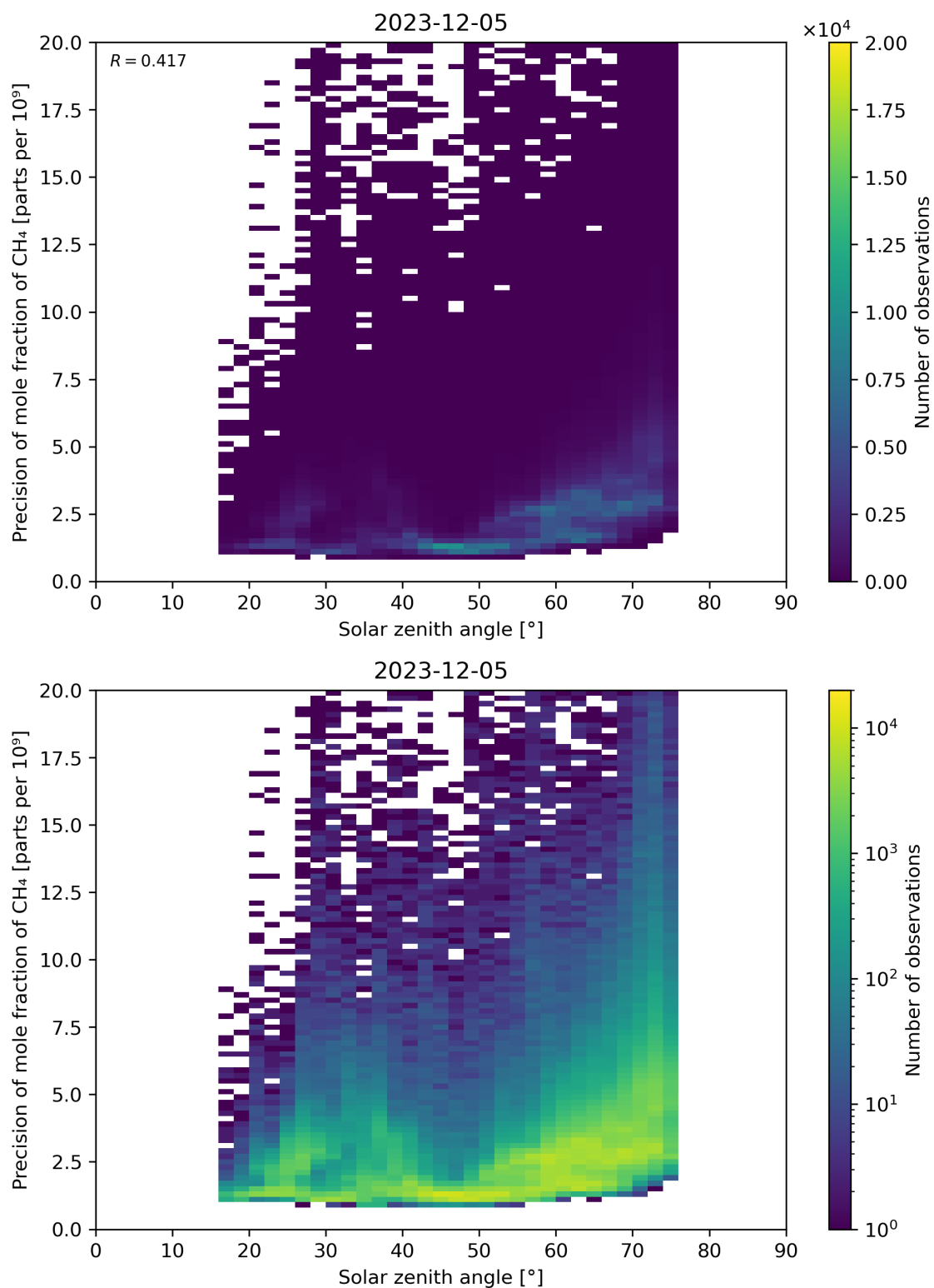
Figure 101: Scatter density plot of “Solar zenith angle” against “Precision of mole fraction of CH 4 ” for 2023-12-04 to 2023-12-06.
