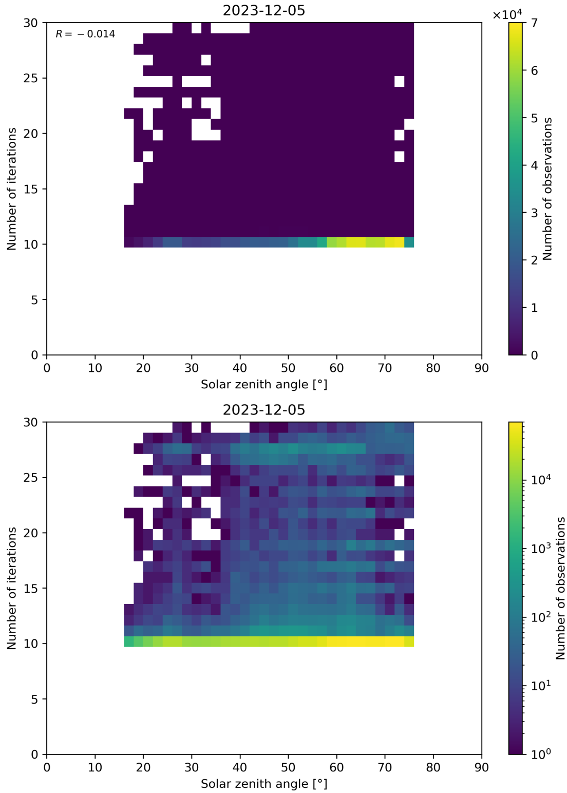
Figure 102: Scatter density plot of “Solar zenith angle” against “Number of iterations” for 2023-12-04 to 2023-12-06.
