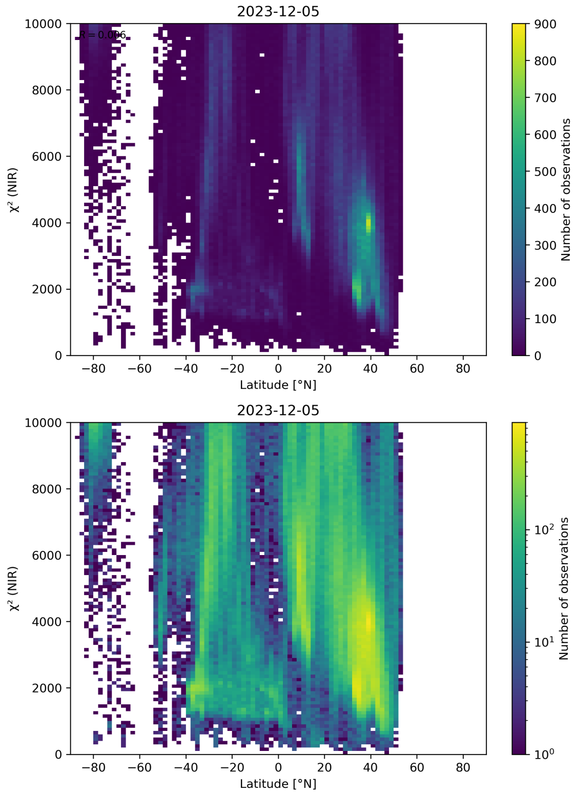
Figure 53: Scatter density plot of “Latitude” against “ \chi^2 (NIR)” for 2023-12-04 to 2023-12-06.
