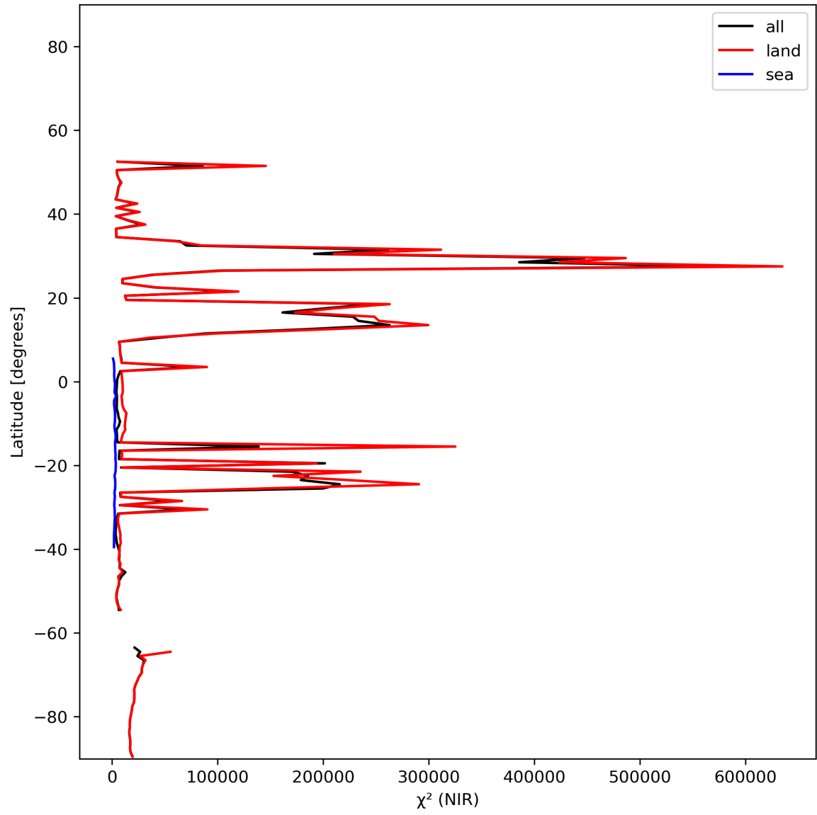
Figure 18: Zonal average of “ \chi^2 (NIR)” for 2023-12-04 to 2023-12-06.
