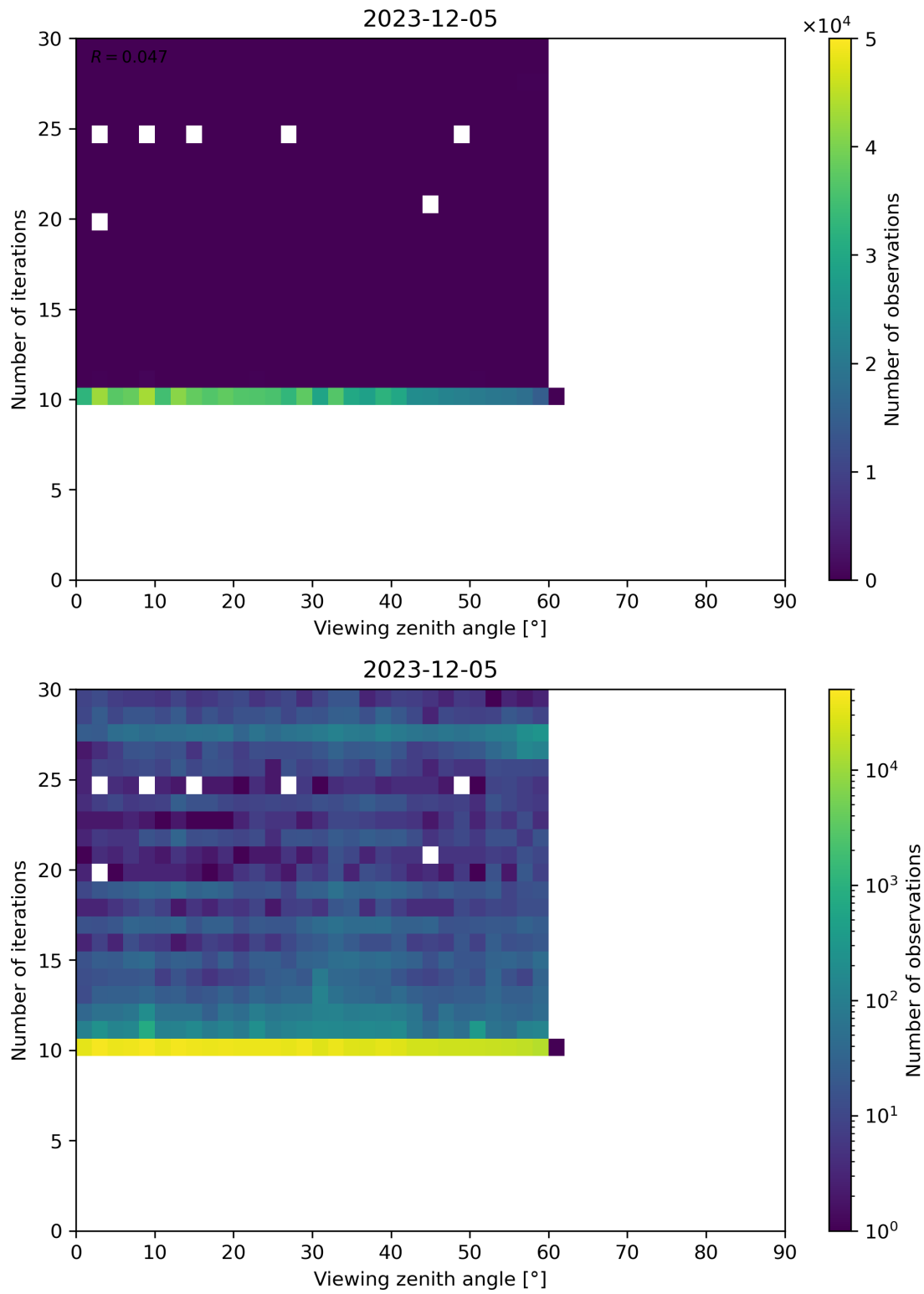
Figure 113: Scatter density plot of “Viewing zenith angle” against “Number of iterations” for 2023-12-04 to 2023-12-06.
