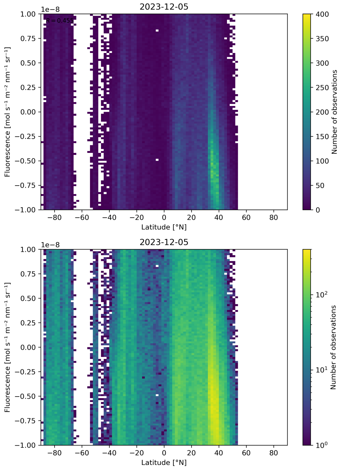
Figure 56: Scatter density plot of “Latitude” against “Fluorescence” for 2023-12-04 to 2023-12-06.
