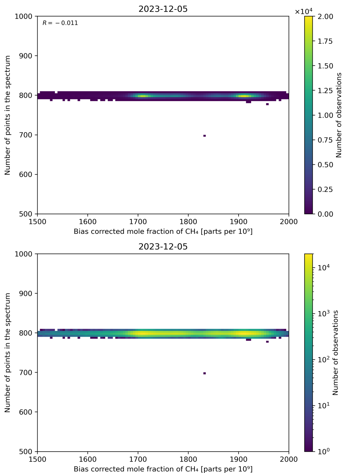
Figure 68: Scatter density plot of “Bias corrected mole fraction of CH 4 ” against “Number of points in the spectrum” for 2023-12-04 to 2023-12-06.
