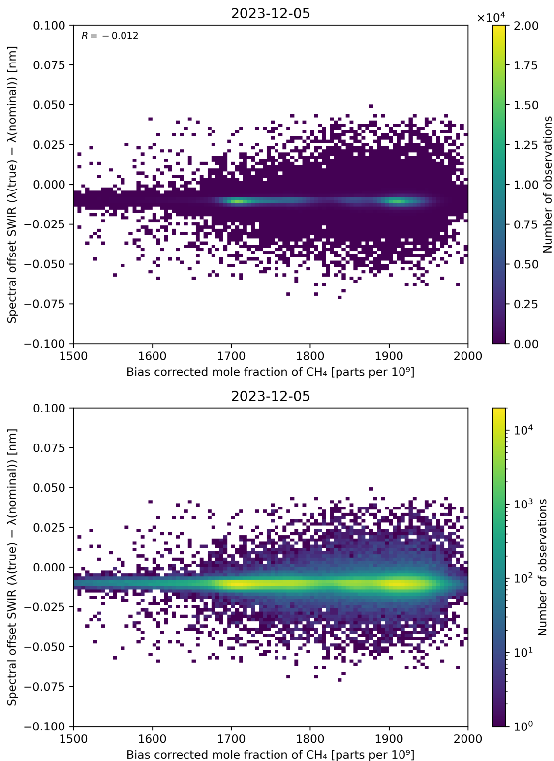
Figure 69: Scatter density plot of “Bias corrected mole fraction of \text{CH}_4 ” against “Spectral offset SWIR ( \lambda(\text{true}) - \lambda(\text{nominal}) )” for 2023-12-04 to 2023-12-06.
