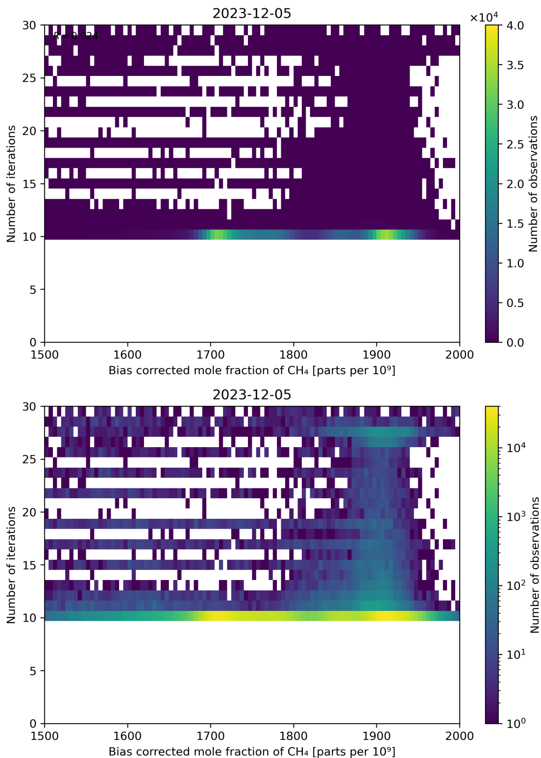
Figure 67: Scatter density plot of “Bias corrected mole fraction of CH 4 ” against “Number of iterations” for 2023-12-04 to 2023-12-06.
