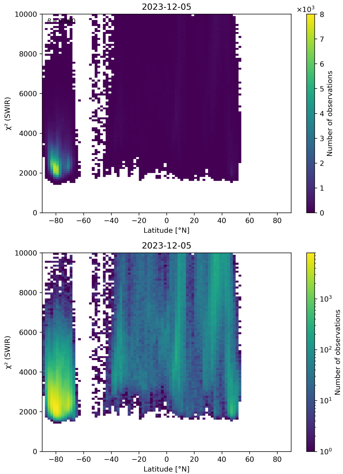
Figure 54: Scatter density plot of “Latitude” against “ \chi^2 (SWIR)” for 2023-12-04 to 2023-12-06.
