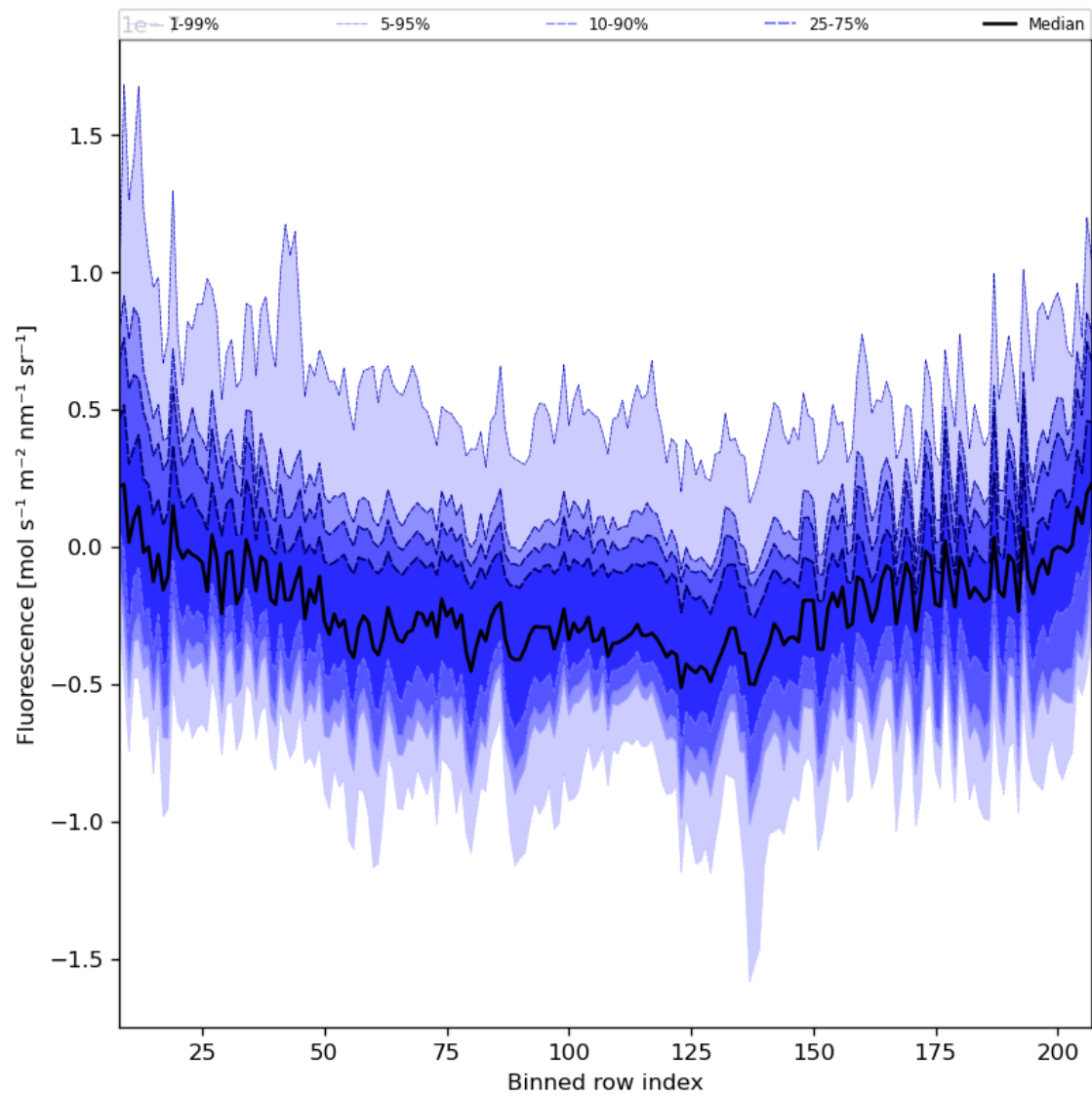
Figure 43: Along track statistics of “Fluorescence” for 2023-12-04 to 2023-12-06
