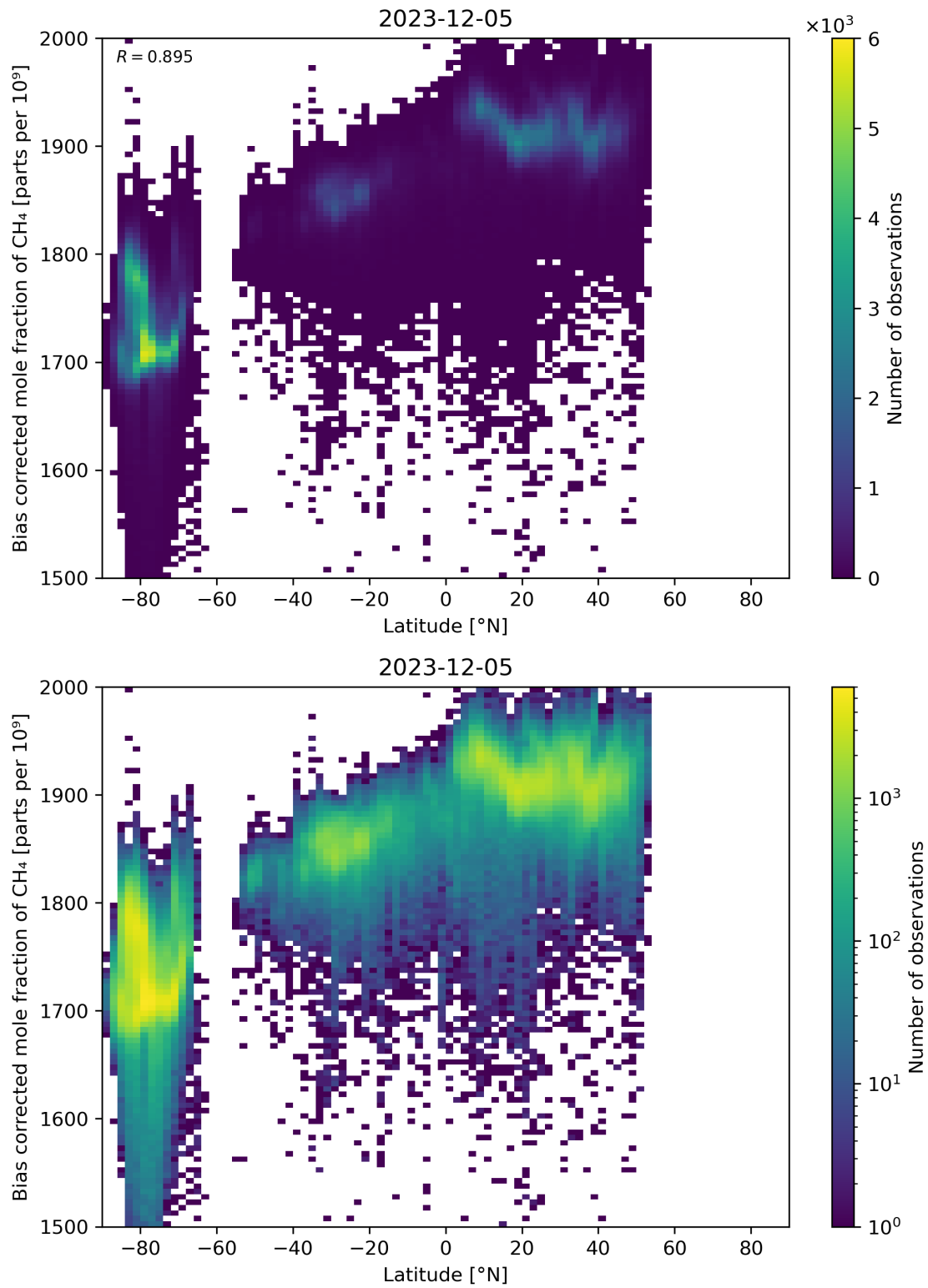
Figure 58: Scatter density plot of “Latitude” against “Bias corrected mole fraction of CH 4 ” for 2023-12-04 to 2023-12-06.
