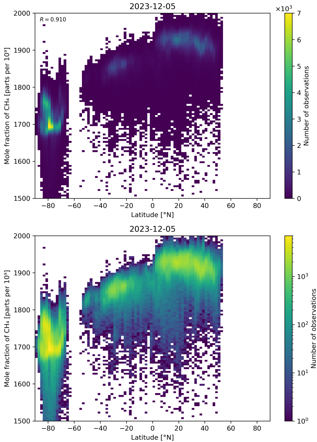
Figure 57: Scatter density plot of “Latitude” against “Mole fraction of CH 4 ” for 2023-12-04 to 2023-12-06.
