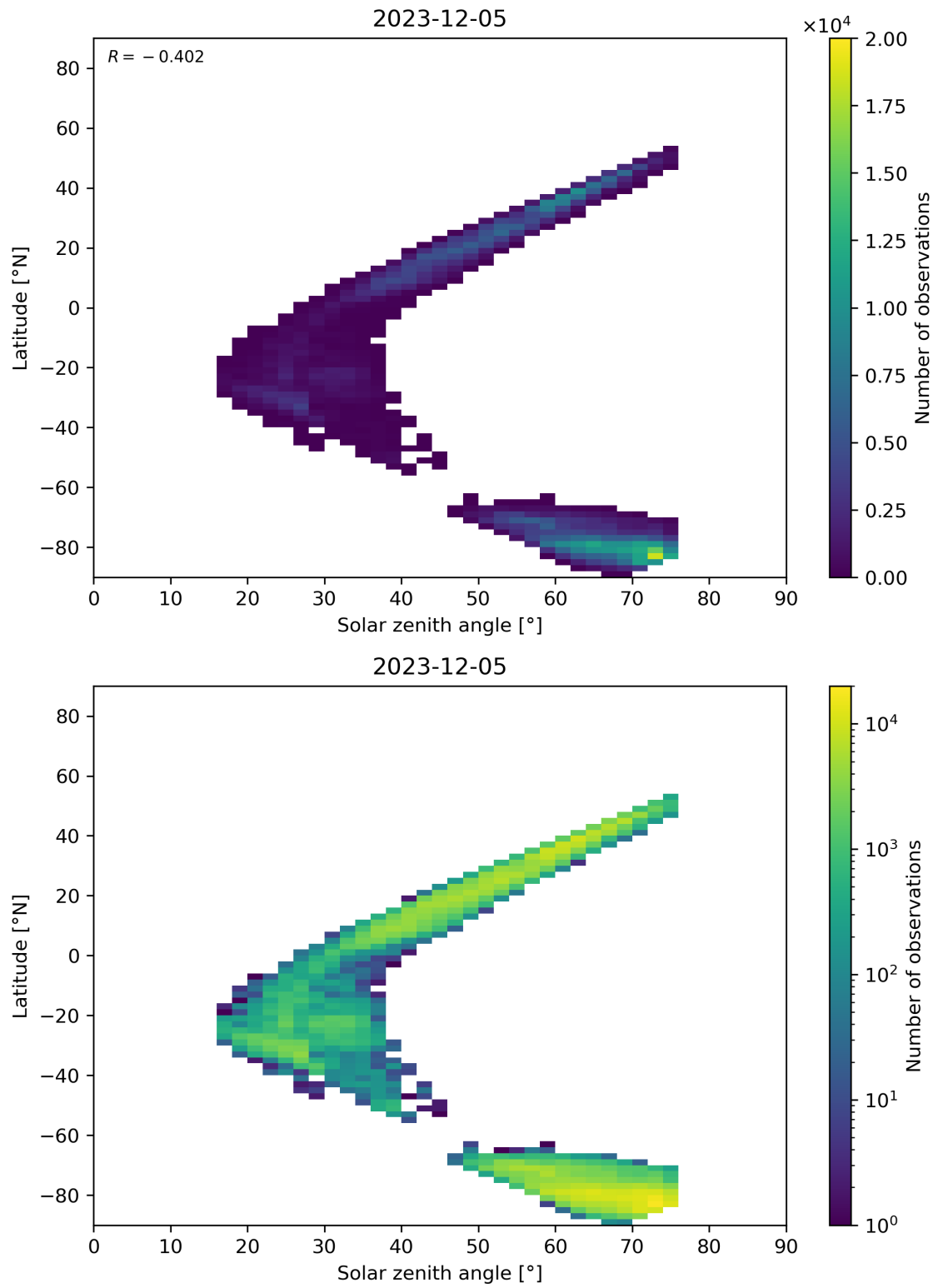
Figure 98: Scatter density plot of “Solar zenith angle” against “Latitude” for 2023-12-04 to 2023-12-06.
