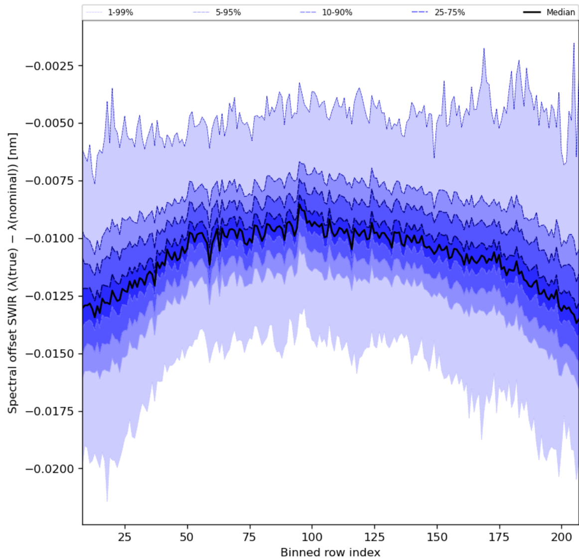
Figure 38: Along track statistics of “Spectral offset SWIR ( \lambda(\text{true}) - \lambda(\text{nominal}) )” for 2023-12-04 to 2023-12-06
