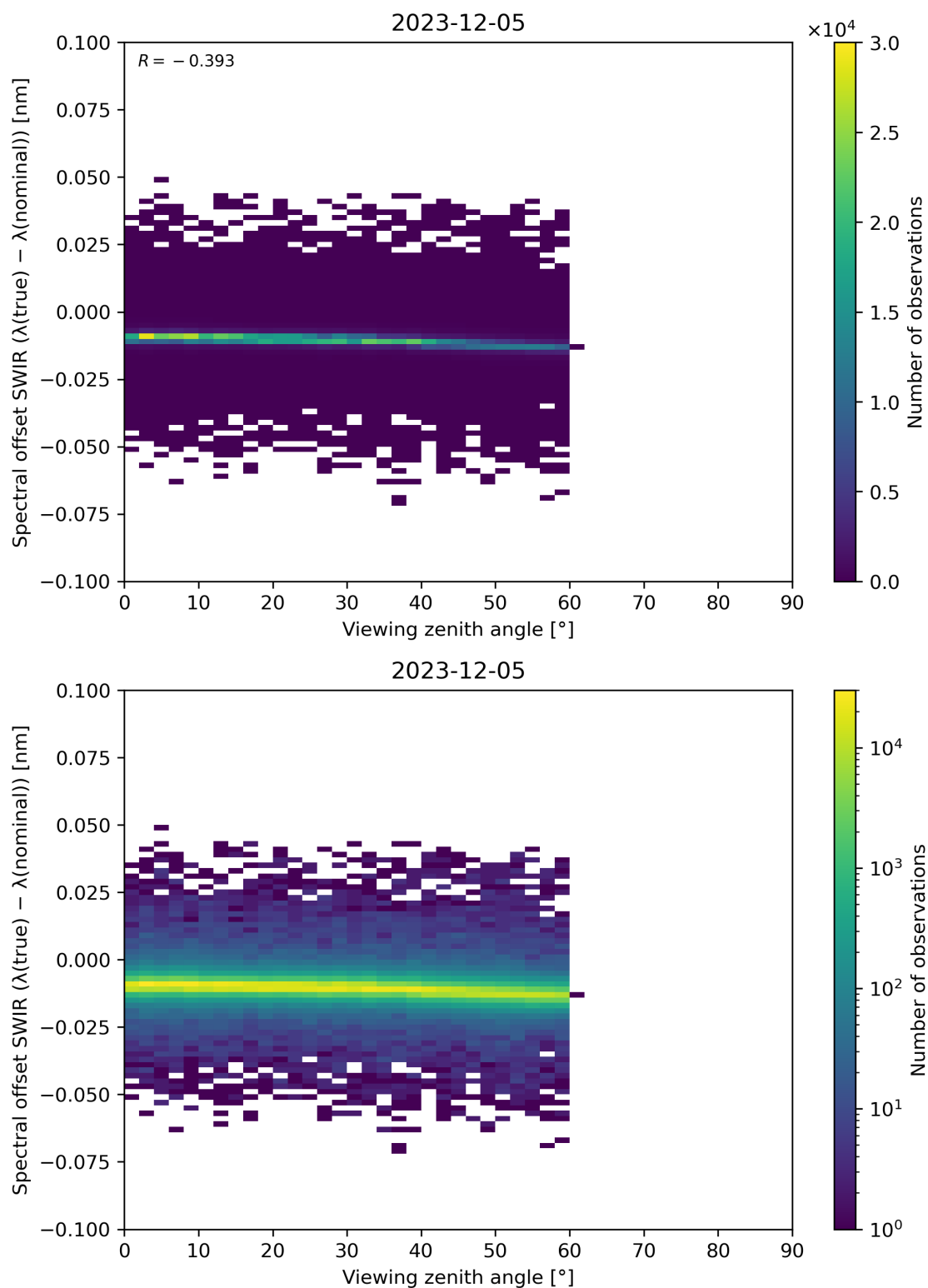
Figure 116: Scatter density plot of “Viewing zenith angle” against “Spectral offset SWIR ( \lambda(\text{true}) - \lambda(\text{nominal}) )” for 2023-12-04 to 2023-12-06.
