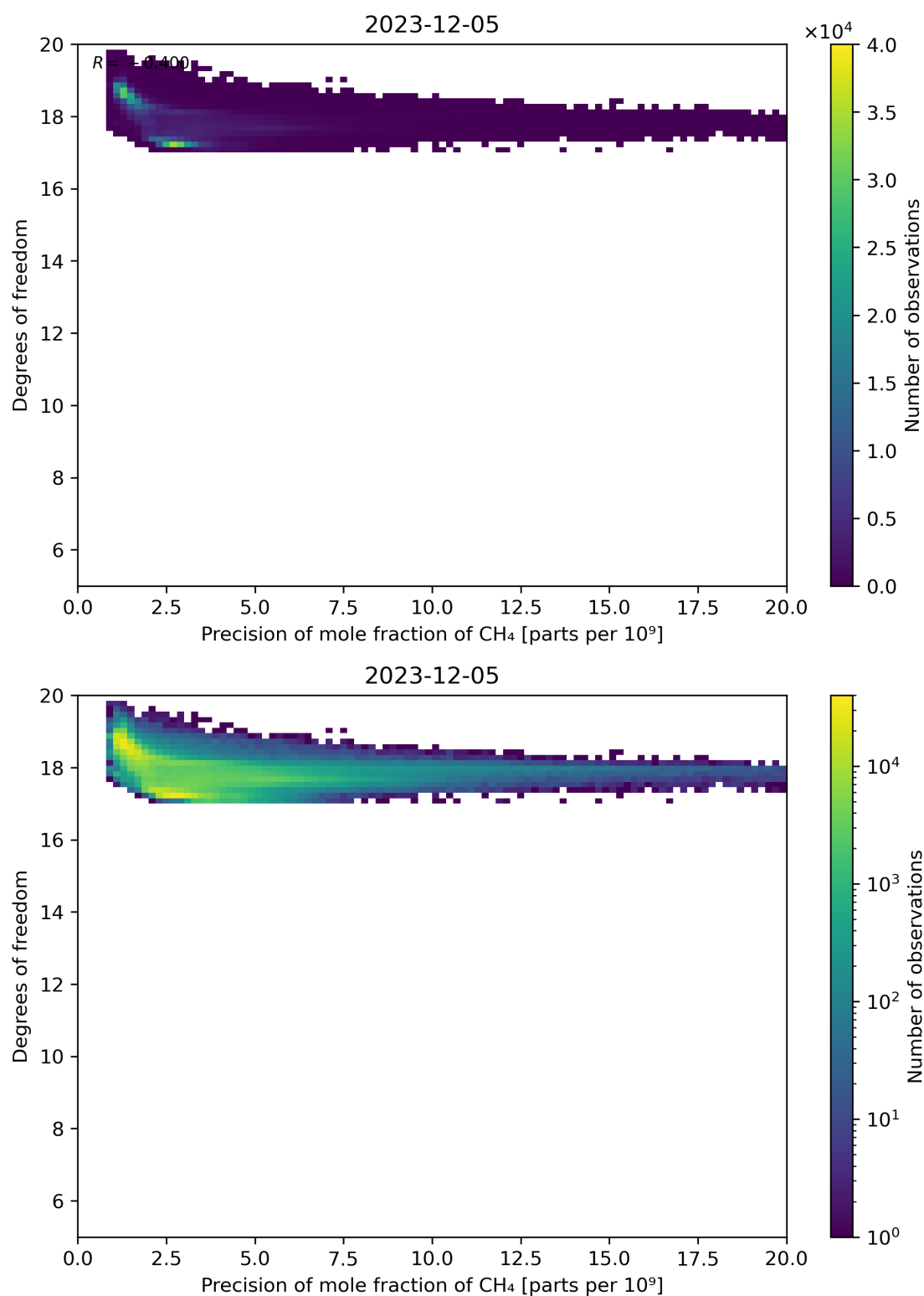
Figure 80: Scatter density plot of “Precision of mole fraction of CH 4 ” against “Degrees of freedom” for 2023-12-04 to 2023-12-06.
