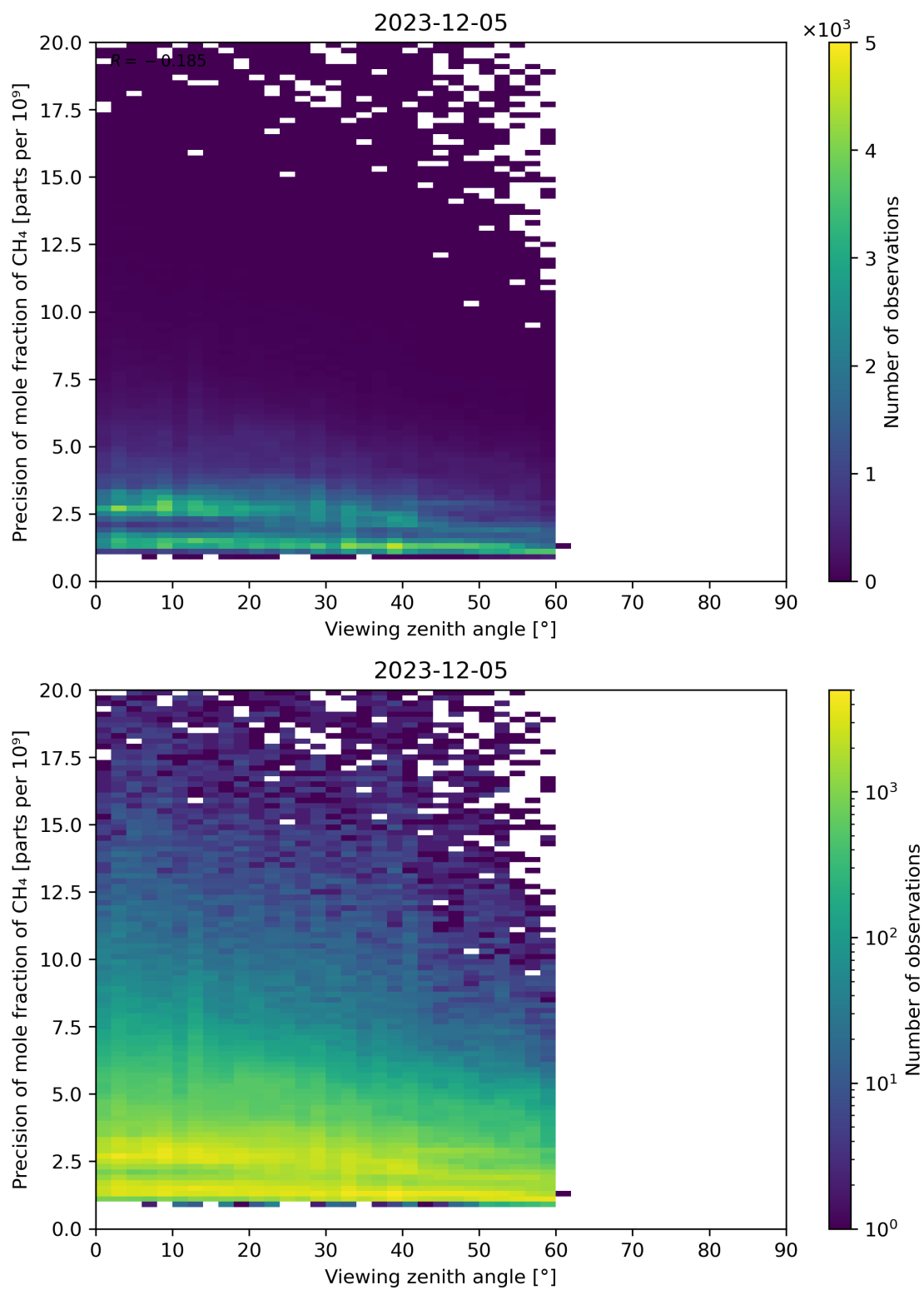
Figure 112: Scatter density plot of “Viewing zenith angle” against “Precision of mole fraction of CH 4 ” for 2023-12-04 to 2023-12-06.
