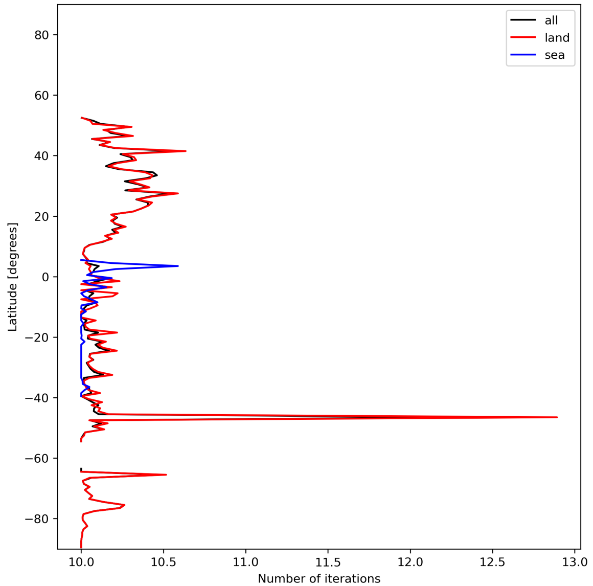
Figure 20: Zonal average of “Number of iterations” for 2023-12-04 to 2023-12-06.
