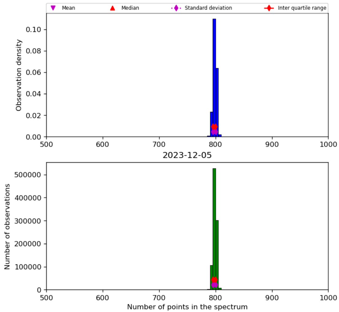
Figure 26: Histogram of “Number of points in the spectrum” for 2023-12-04 to 2023-12-06
