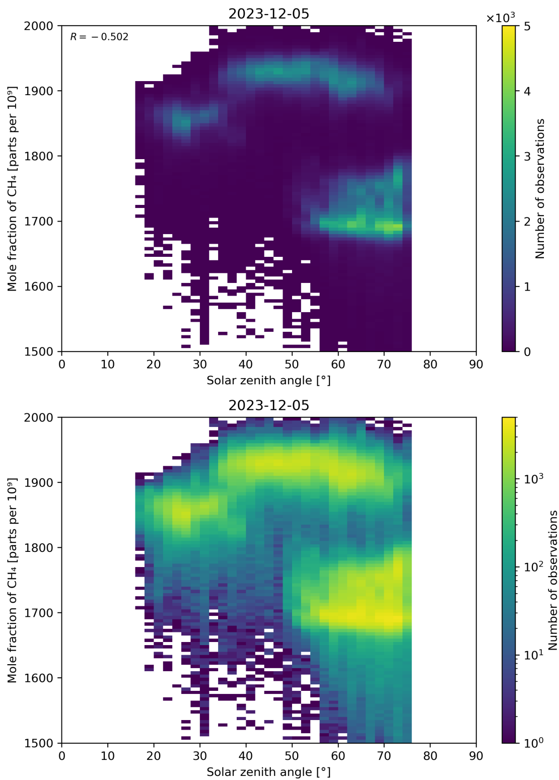
Figure 99: Scatter density plot of “Solar zenith angle” against “Mole fraction of CH 4 ” for 2023-12-04 to 2023-12-06.
