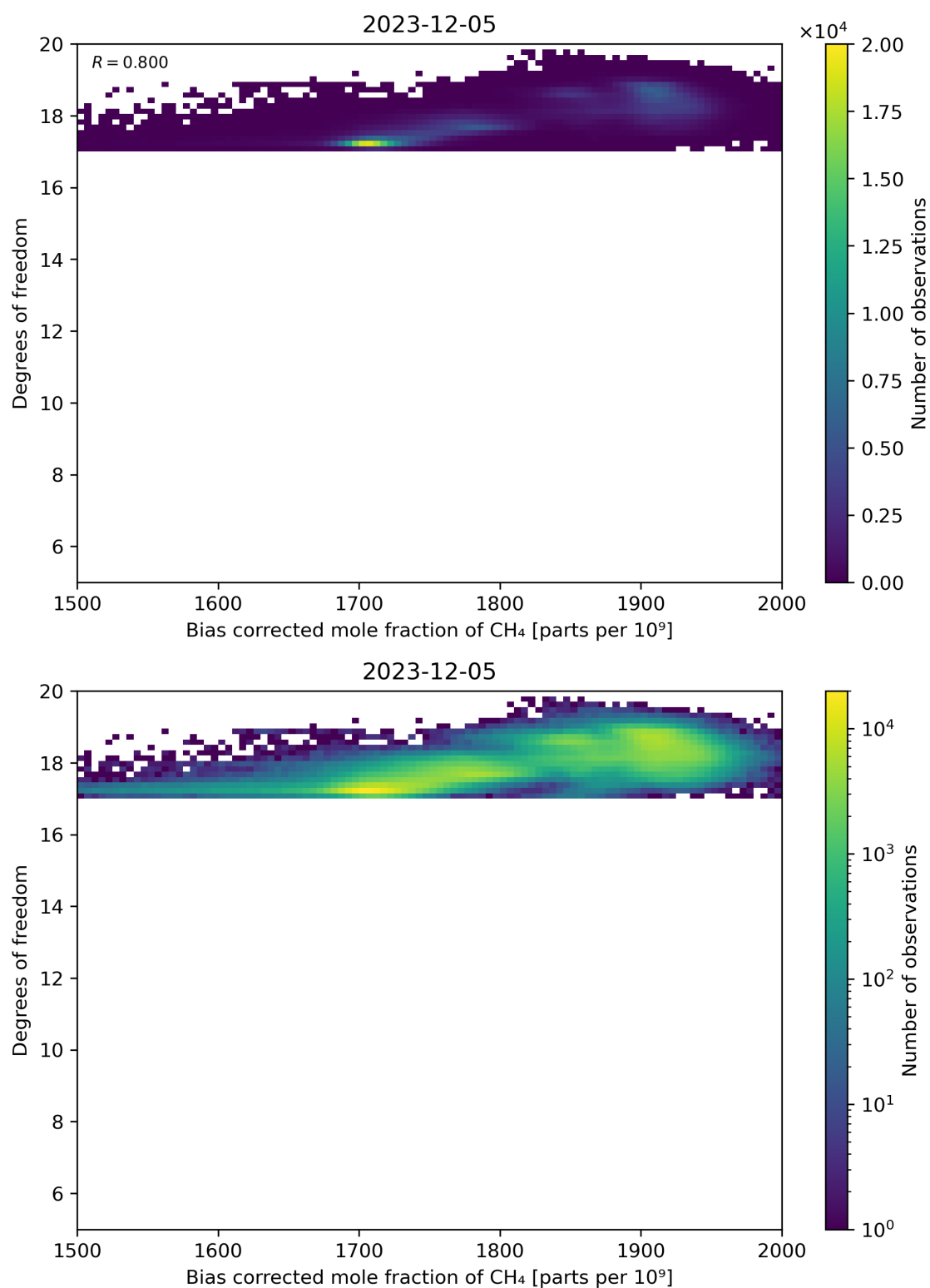
Figure 65: Scatter density plot of “Bias corrected mole fraction of CH 4 ” against “Degrees of freedom” for 2023-12-04 to 2023-12-06.
