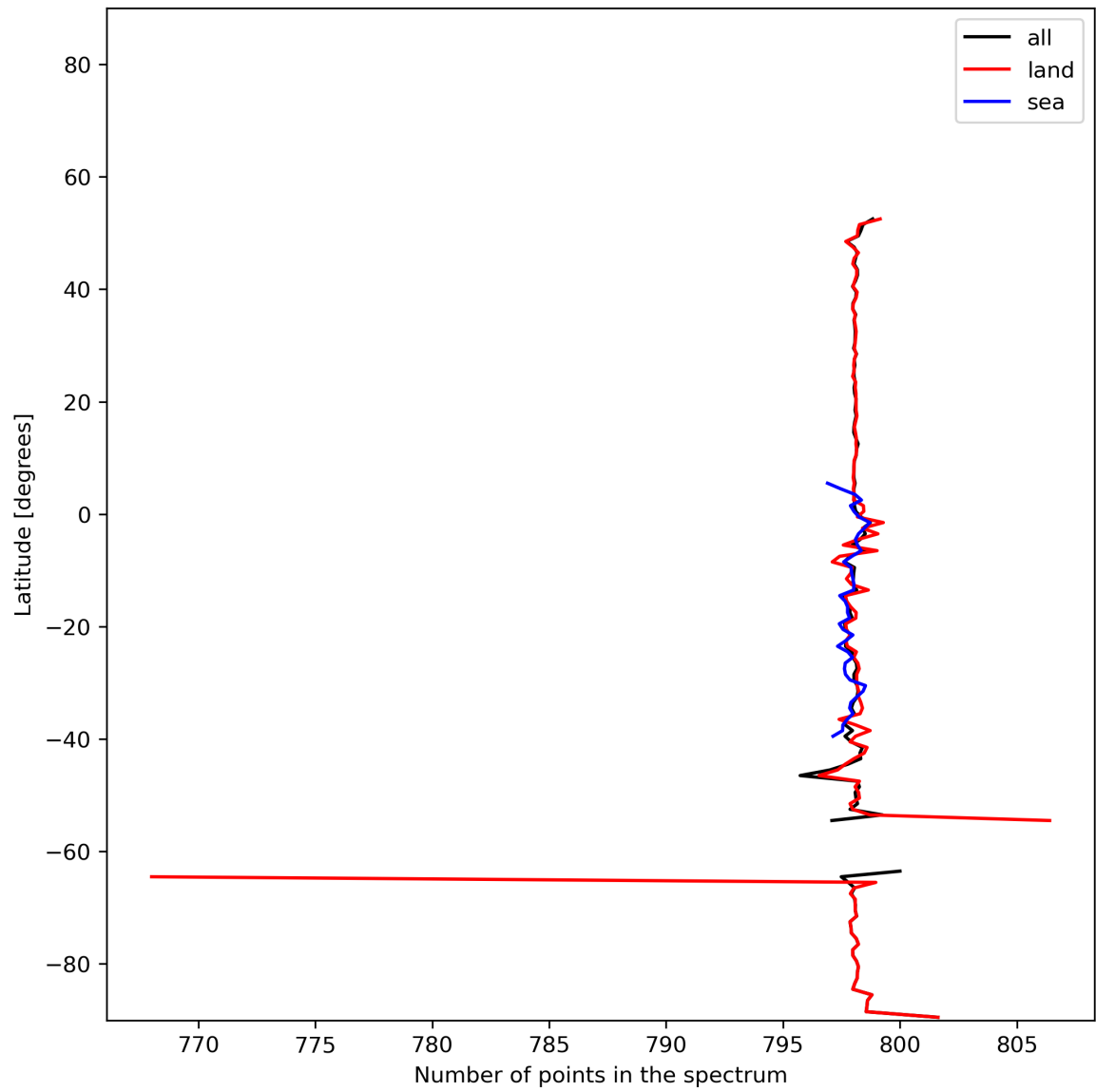
Figure 15: Zonal average of “Number of points in the spectrum” for 2023-12-04 to 2023-12-06.
