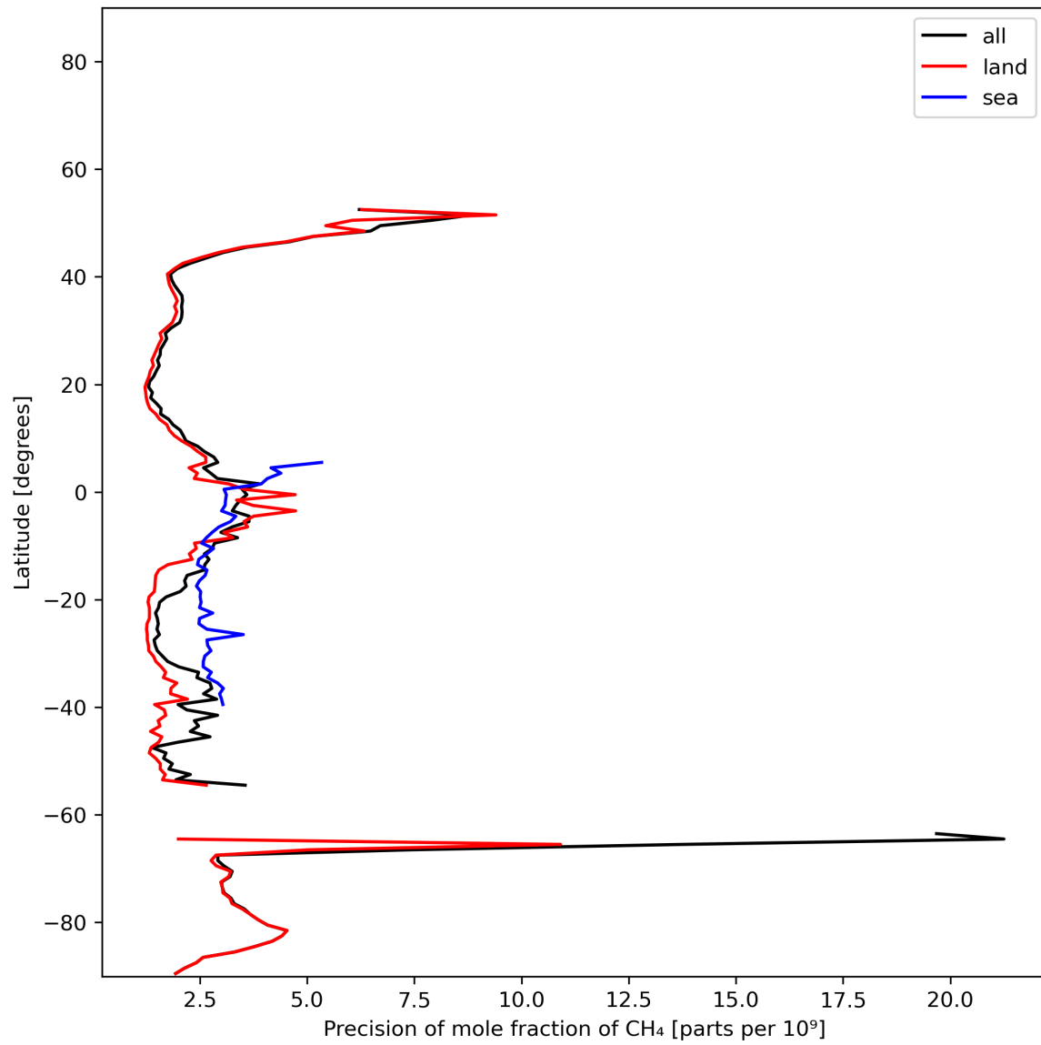
Figure 13: Zonal average of “Precision of mole fraction of CH 4 ” for 2023-12-04 to 2023-12-06.
