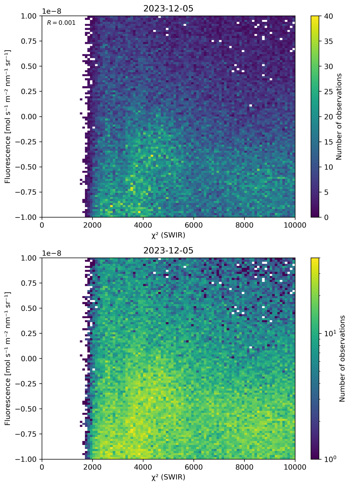
Figure 49: Scatter density plot of “ \chi^2 (SWIR)” against “Fluorescence” for 2023-12-04 to 2023-12-06.
