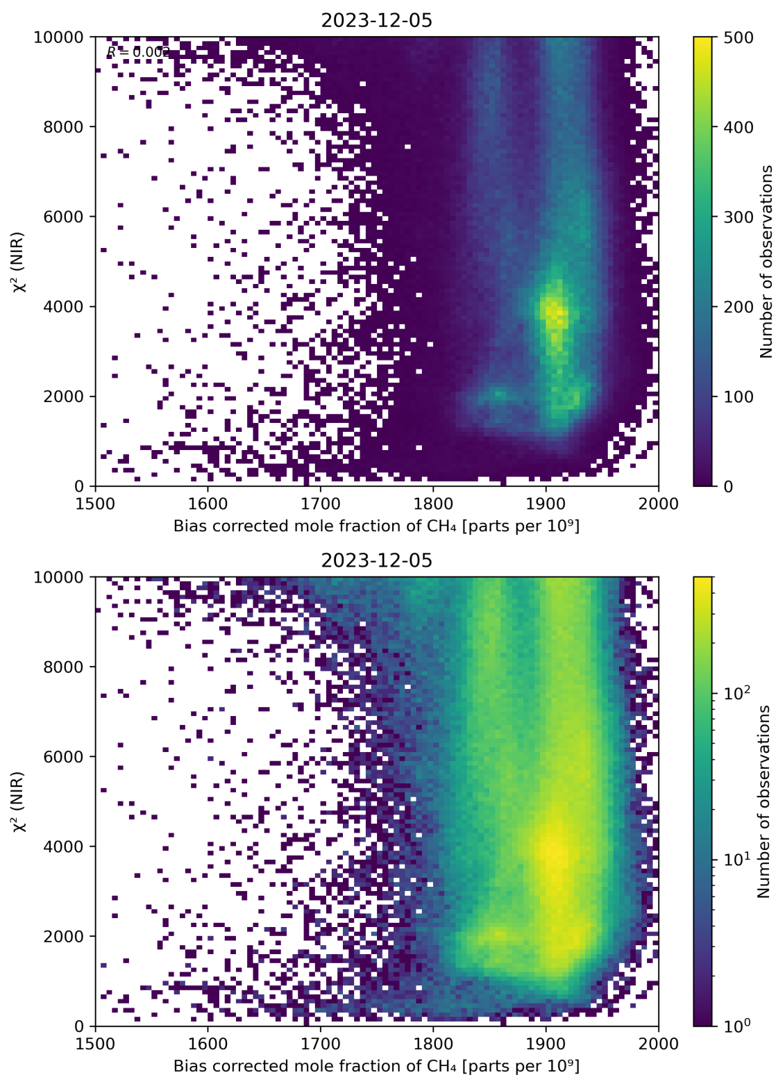
Figure 63: Scatter density plot of “Bias corrected mole fraction of \text{CH}_4 ” against “ \chi^2 (NIR)” for 2023-12-04 to 2023-12-06.
