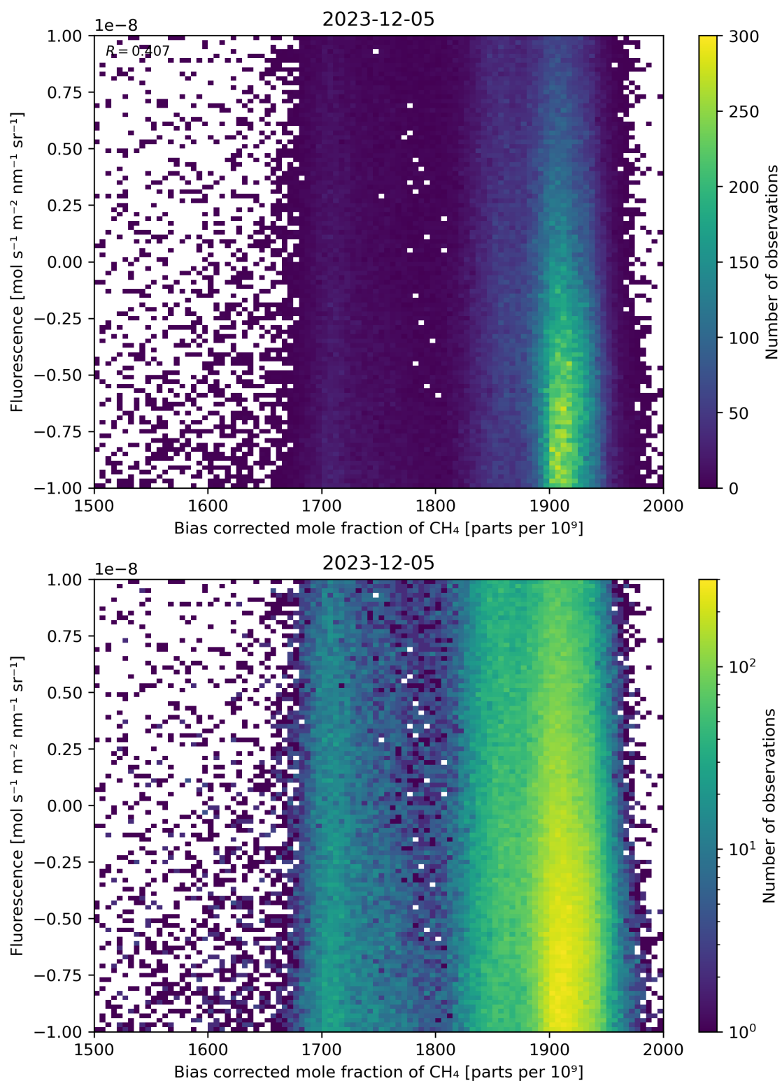
Figure 66: Scatter density plot of “Bias corrected mole fraction of \text{CH}_4 ” against “Fluorescence” for 2023-12-04 to 2023-12-06.
