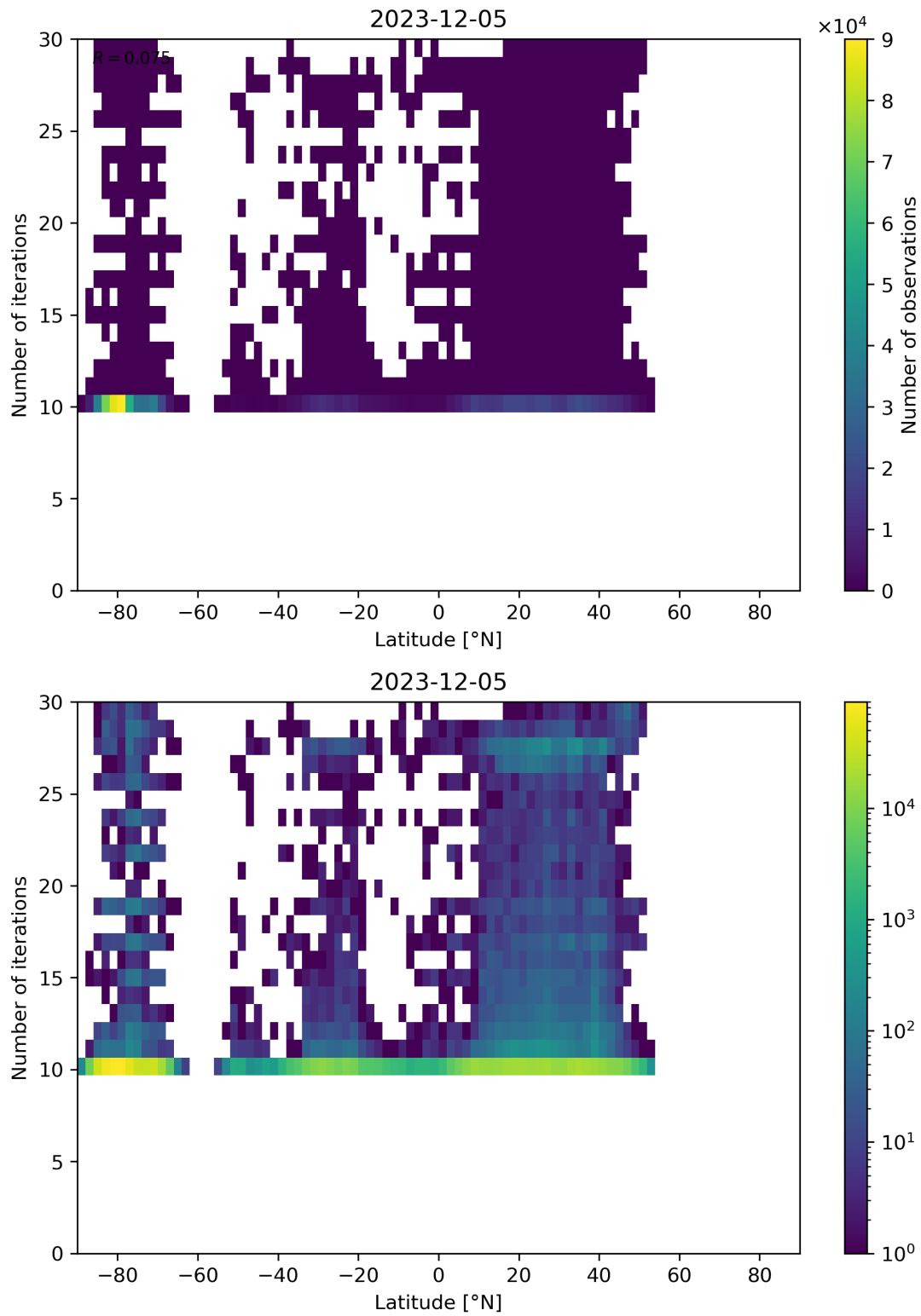
Figure 60: Scatter density plot of “Latitude” against “Number of iterations” for 2023-12-04 to 2023-12-06.
