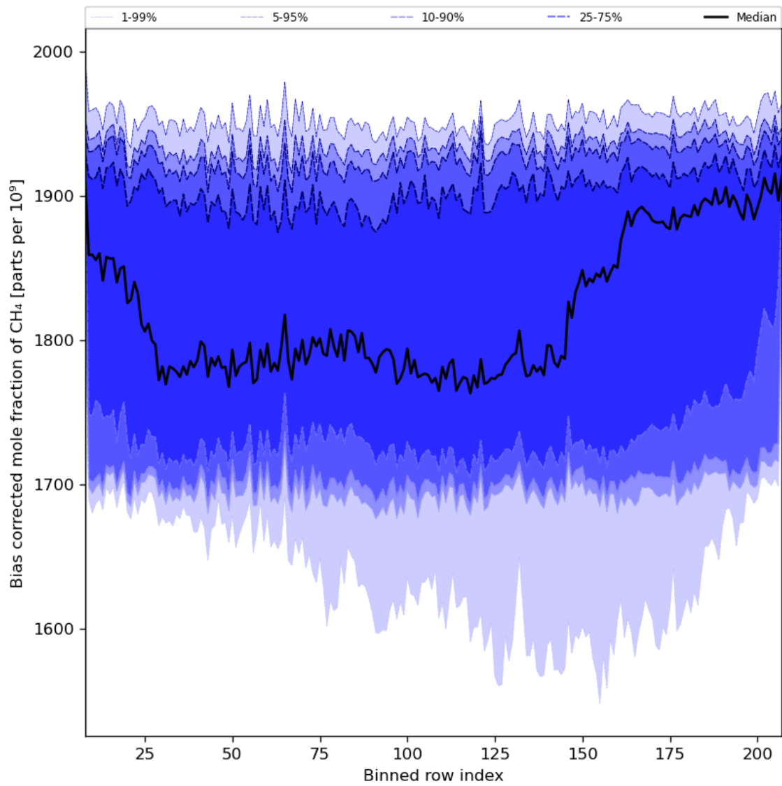
Figure 36: Along track statistics of “Bias corrected mole fraction of CH 4 ” for 2023-12-04 to 2023-12-06
