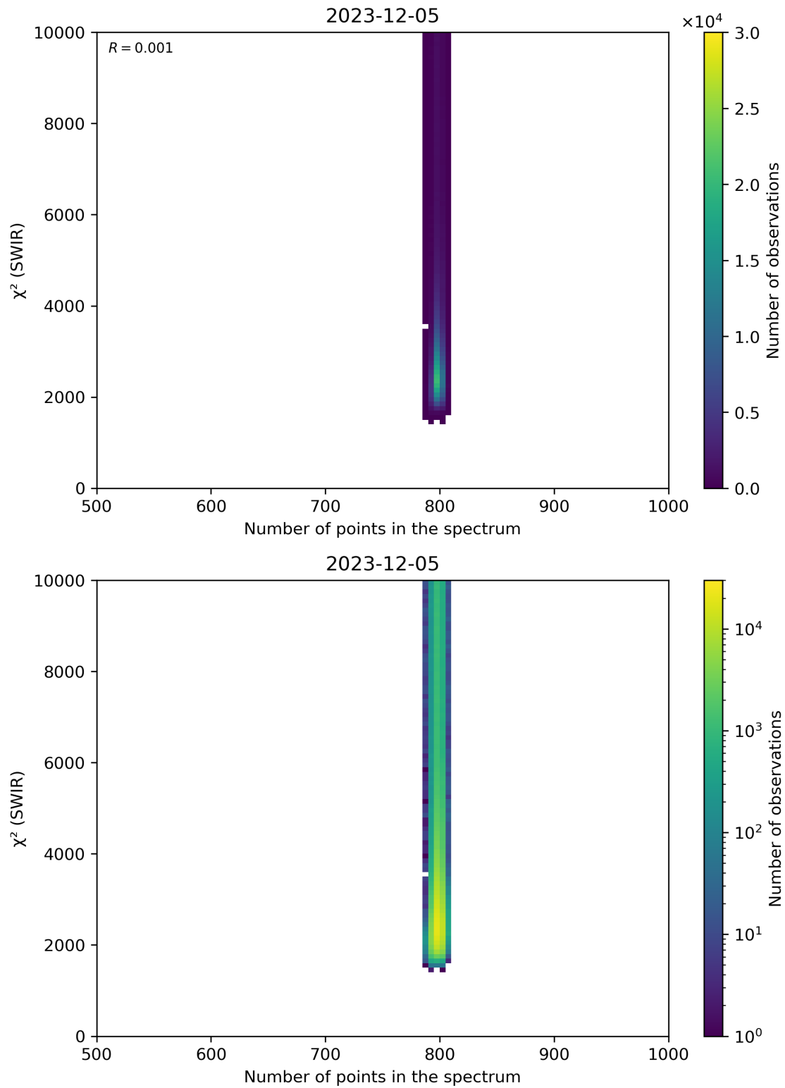
Figure 89: Scatter density plot of “Number of points in the spectrum” against “ \chi^2 (SWIR)” for 2023-12-04 to 2023-12-06.
