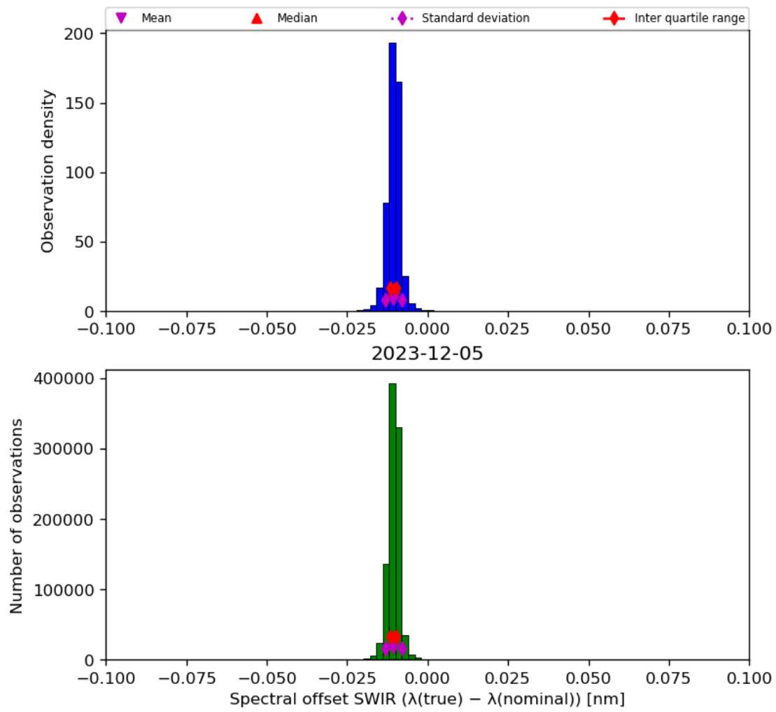
Figure 27: Histogram of “Spectral offset SWIR ( \lambda(\text{true}) - \lambda(\text{nominal}) )” for 2023-12-04 to 2023-12-06
