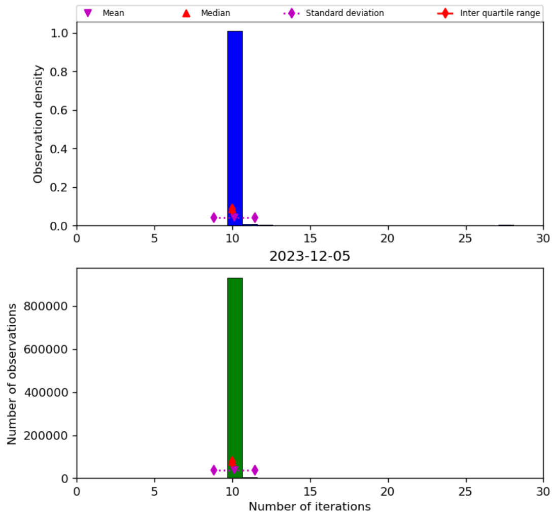
Figure 31: Histogram of “Number of iterations” for 2023-12-04 to 2023-12-06
