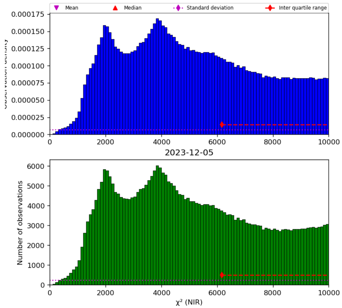
Figure 29: Histogram of “ \chi^2 (NIR)” for 2023-12-04 to 2023-12-06
