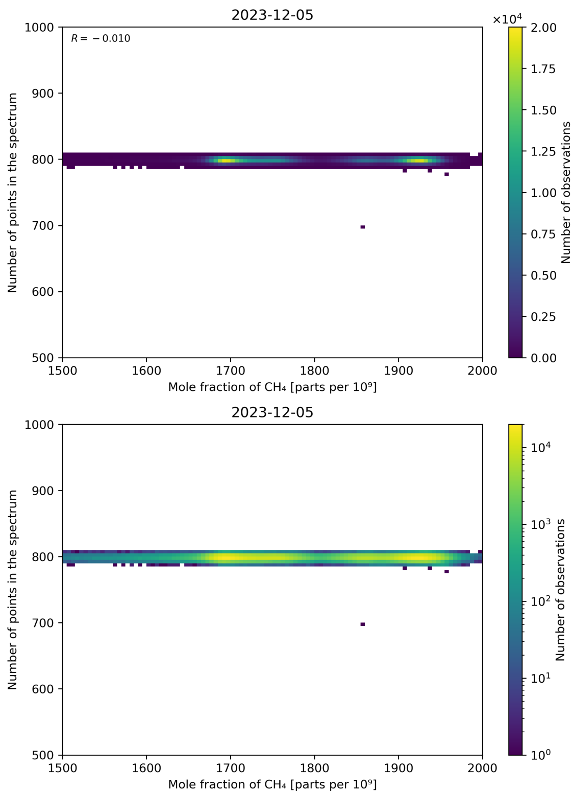
Figure 77: Scatter density plot of “Mole fraction of CH 4 ” against “Number of points in the spectrum” for 2023-12-04 to 2023-12-06.
