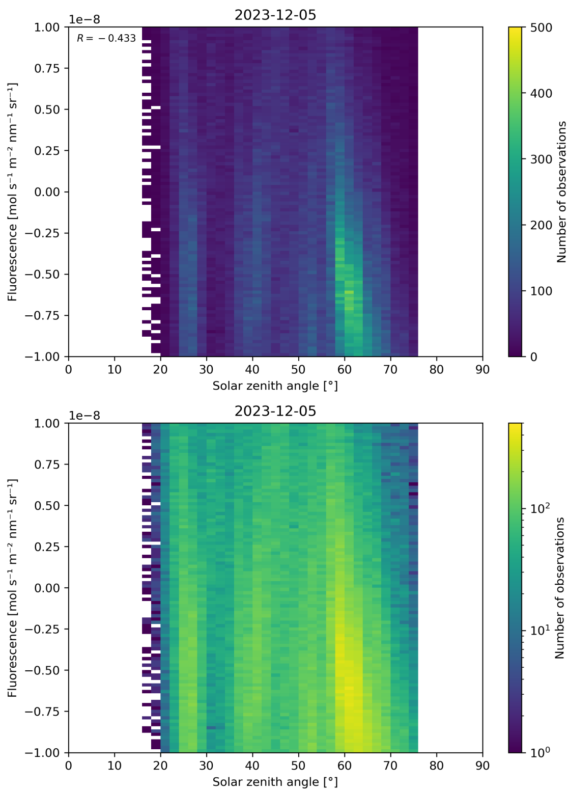
Figure 97: Scatter density plot of “Solar zenith angle” against “Fluorescence” for 2023-12-04 to 2023-12-06.
