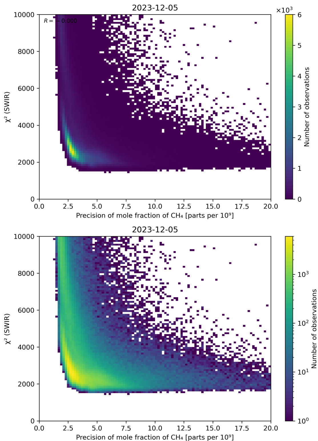
Figure 79: Scatter density plot of “Precision of mole fraction of CH 4 ” against “ \chi^2 (SWIR)” for 2023-12-04 to 2023-12-06.
