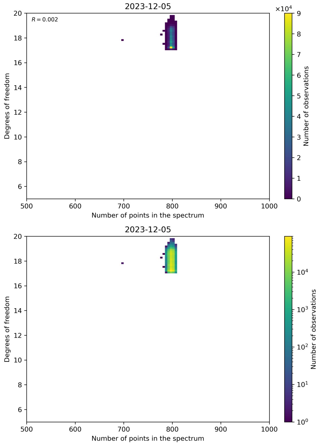
Figure 90: Scatter density plot of “Number of points in the spectrum” against “Degrees of freedom” for 2023-12-04 to 2023-12-06.
