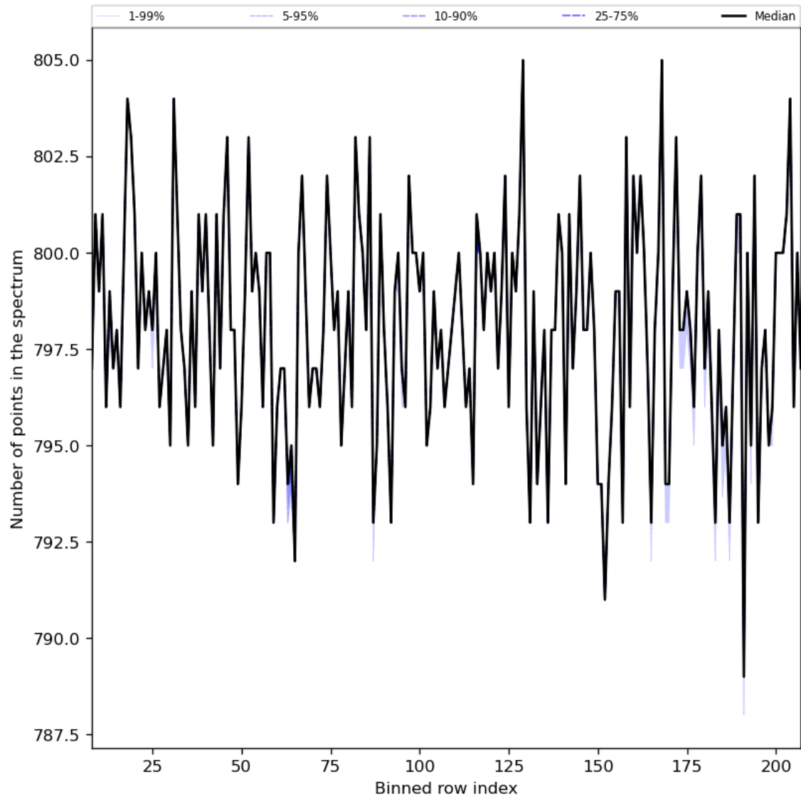
Figure 37: Along track statistics of “Number of points in the spectrum” for 2023-12-04 to 2023-12-06
