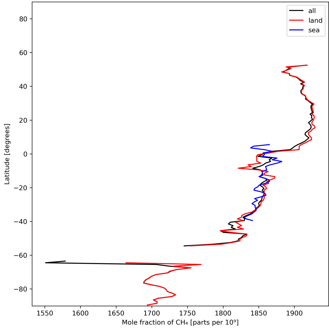
Figure 12: Zonal average of “Mole fraction of CH 4 ” for 2023-12-04 to 2023-12-06.
