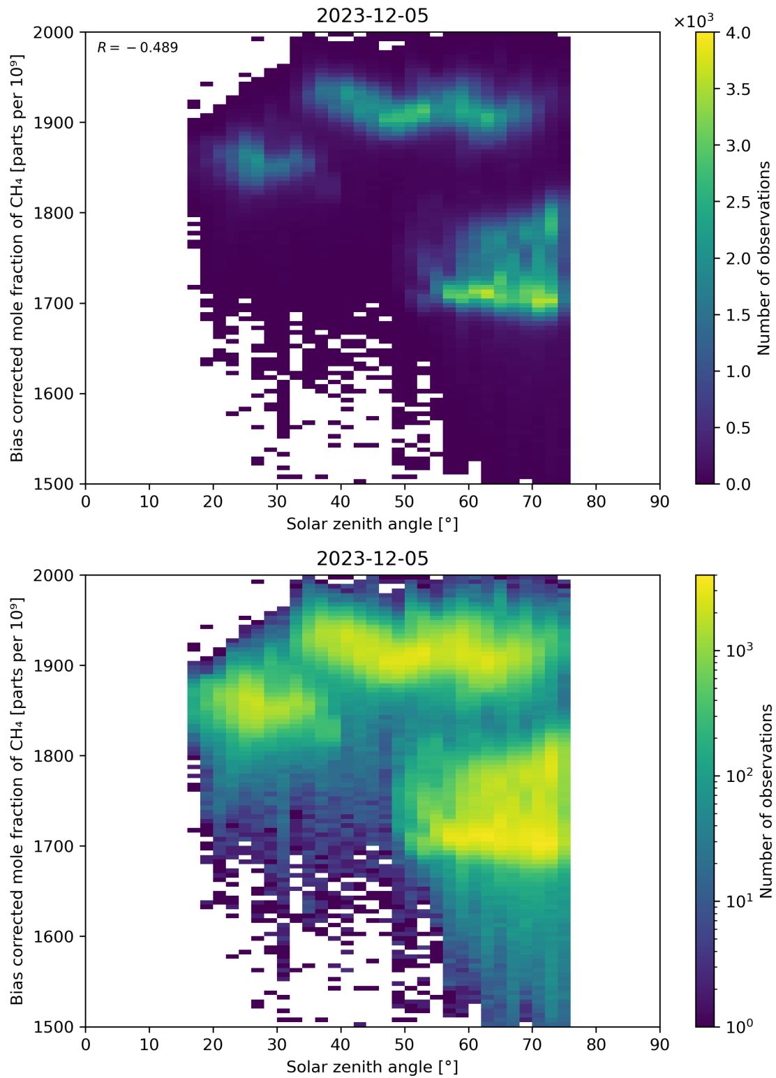
Figure 100: Scatter density plot of “Solar zenith angle” against “Bias corrected mole fraction of \text{CH}_4 ” for 2023-12-04 to 2023-12-06.
