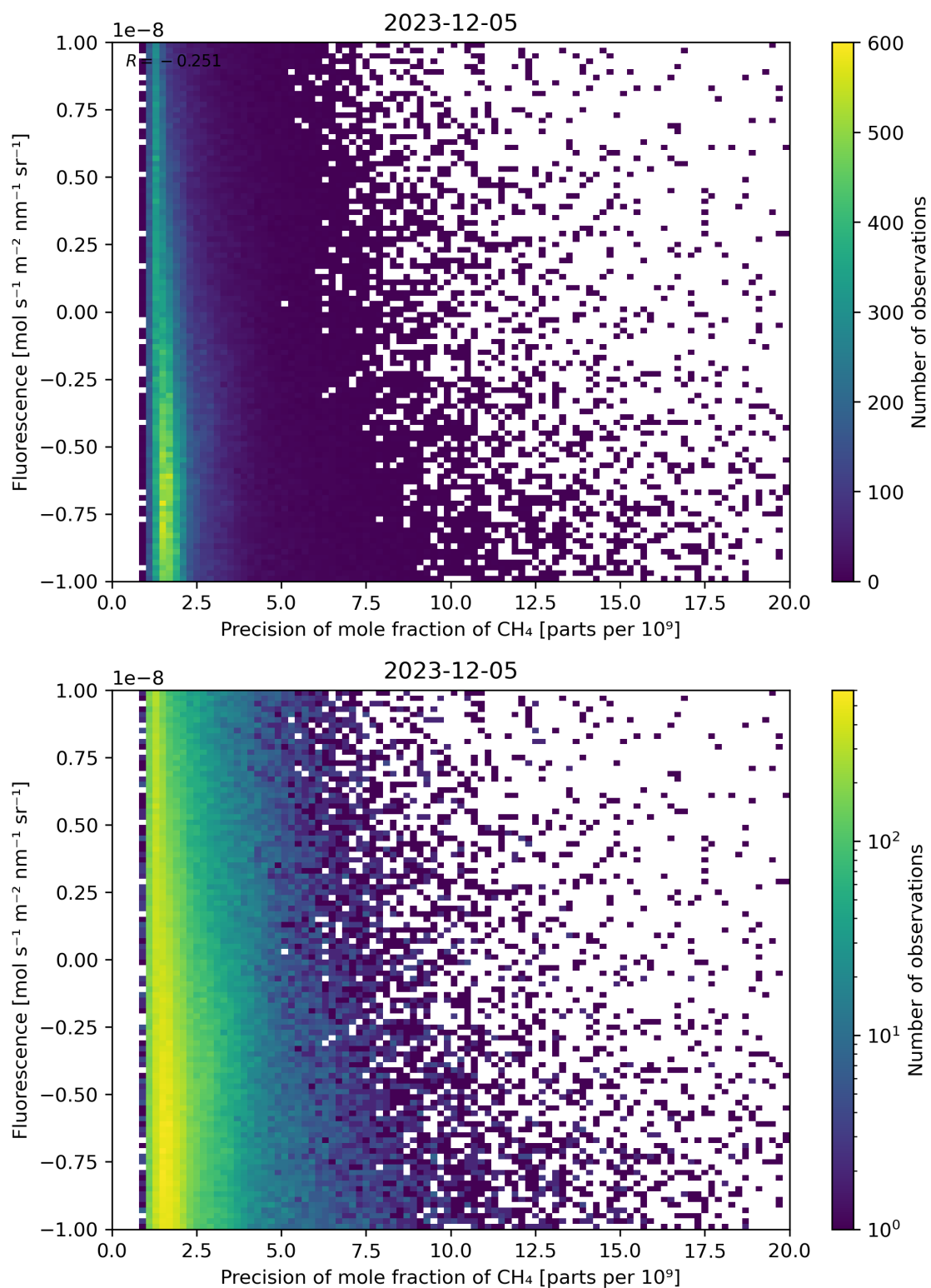
Figure 81: Scatter density plot of “Precision of mole fraction of \text{CH}_4 ” against “Fluorescence” for 2023-12-04 to 2023-12-06.
