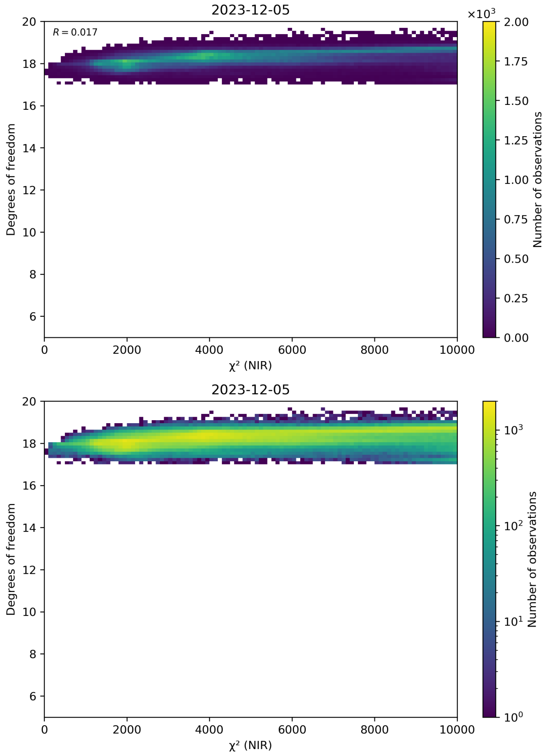
Figure 44: Scatter density plot of “ \chi^2 (NIR)” against “Degrees of freedom” for 2023-12-04 to 2023-12-06.
