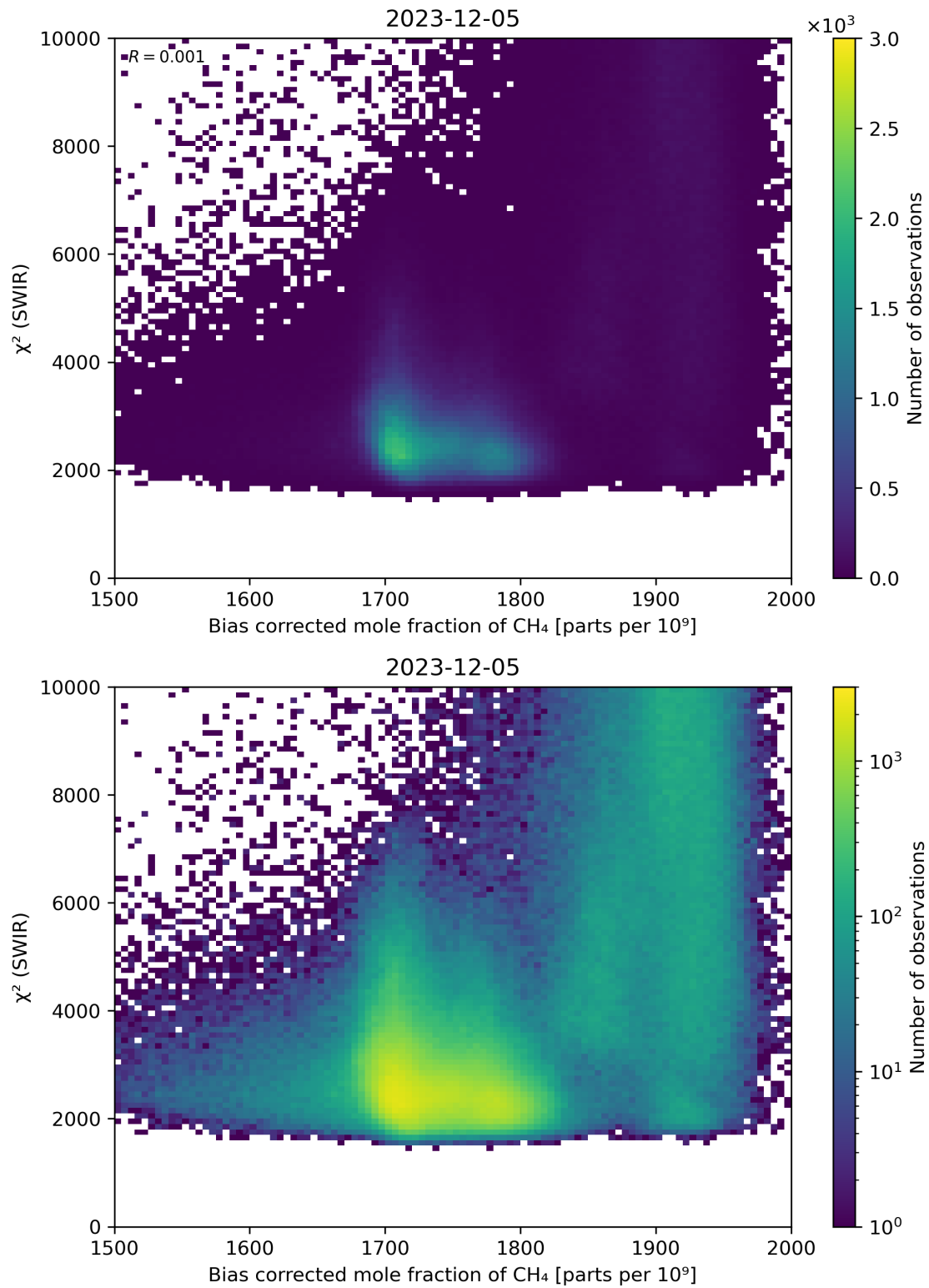
Figure 64: Scatter density plot of “Bias corrected mole fraction of CH 4 ” against “ \chi^2 (SWIR)” for 2023-12-04 to 2023-12-06.
