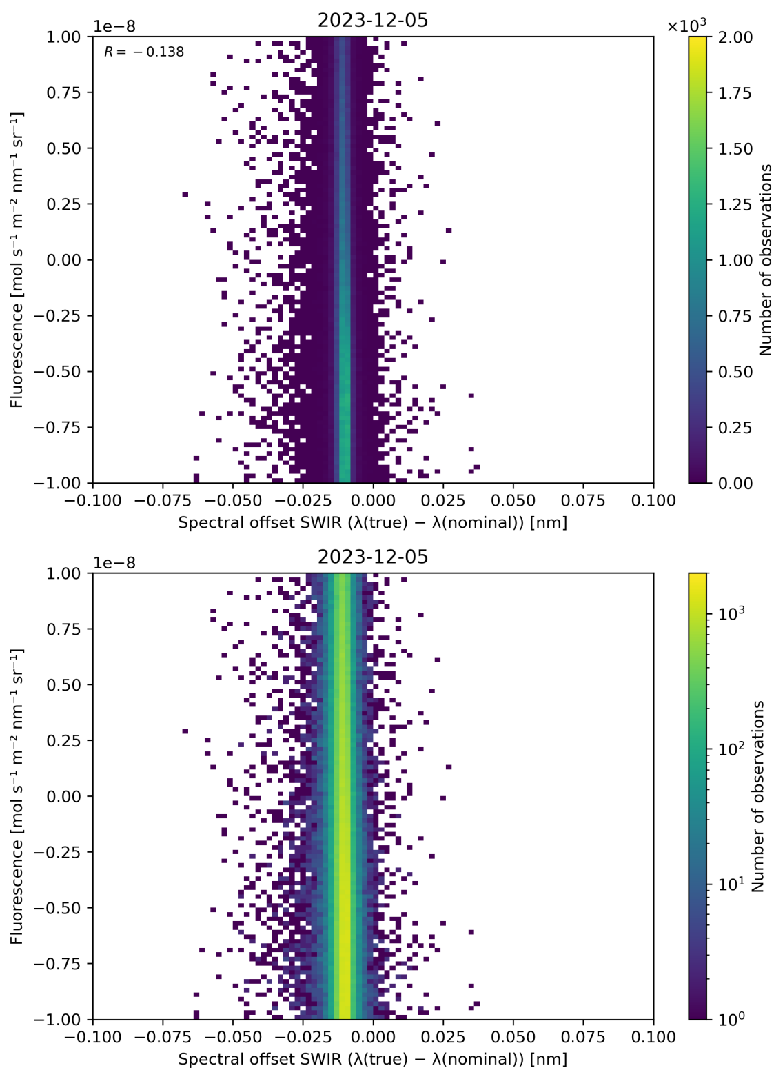
Figure 120: Scatter density plot of “Spectral offset SWIR ( \lambda(\text{true}) - \lambda(\text{nominal}) )” against “Fluorescence” for 2023-12-04 to 2023-12-06.
