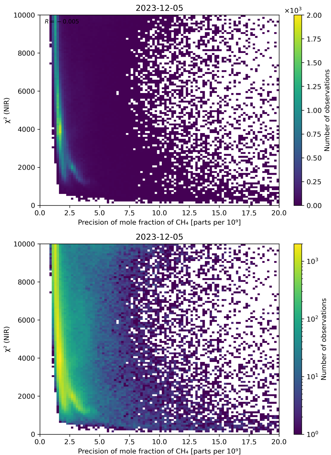
Figure 78: Scatter density plot of “Precision of mole fraction of CH 4 ” against “ \chi^2 (NIR)” for 2023-12-04 to 2023-12-06.
