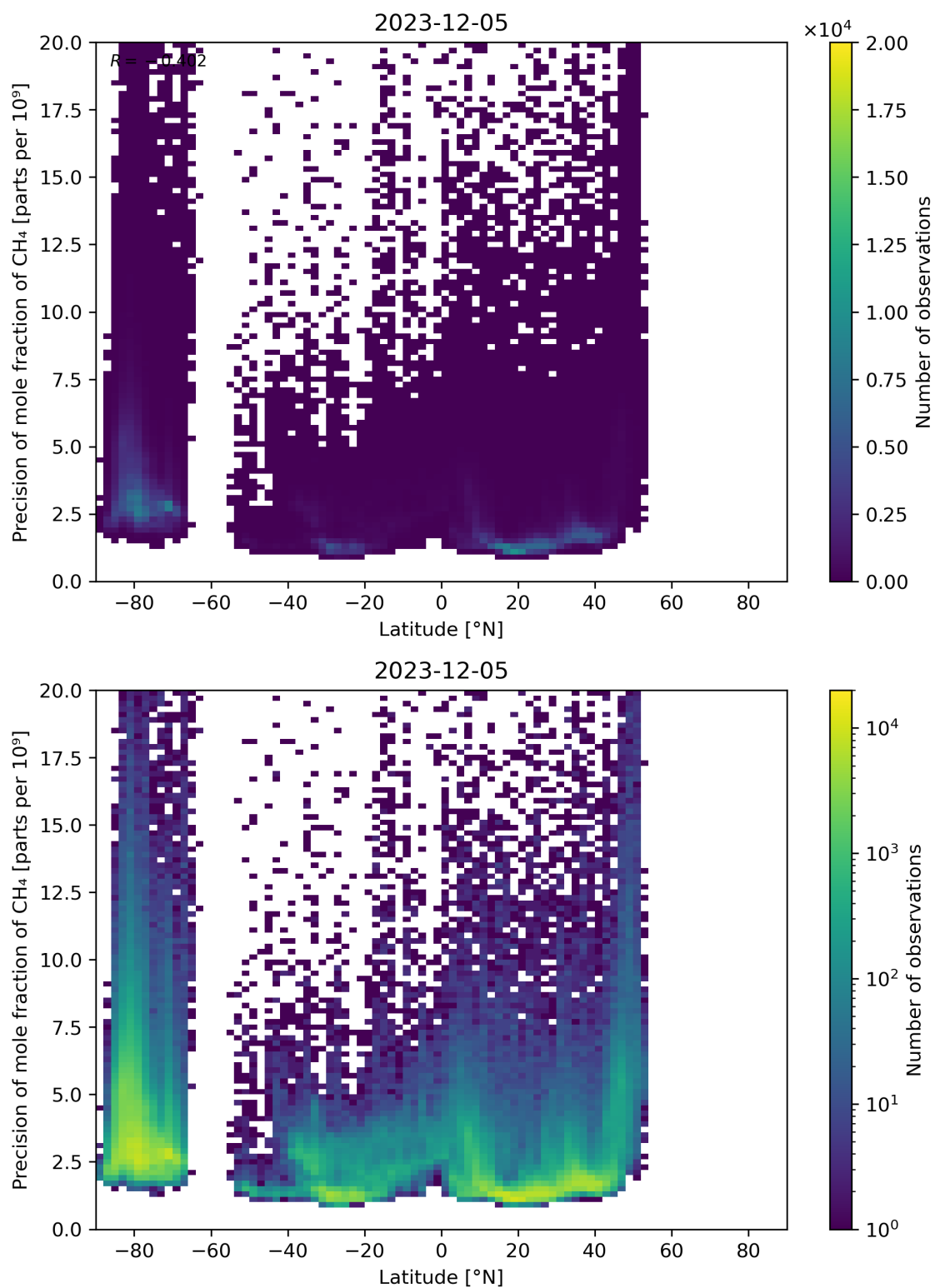
Figure 59: Scatter density plot of “Latitude” against “Precision of mole fraction of CH 4 ” for 2023-12-04 to 2023-12-06.
