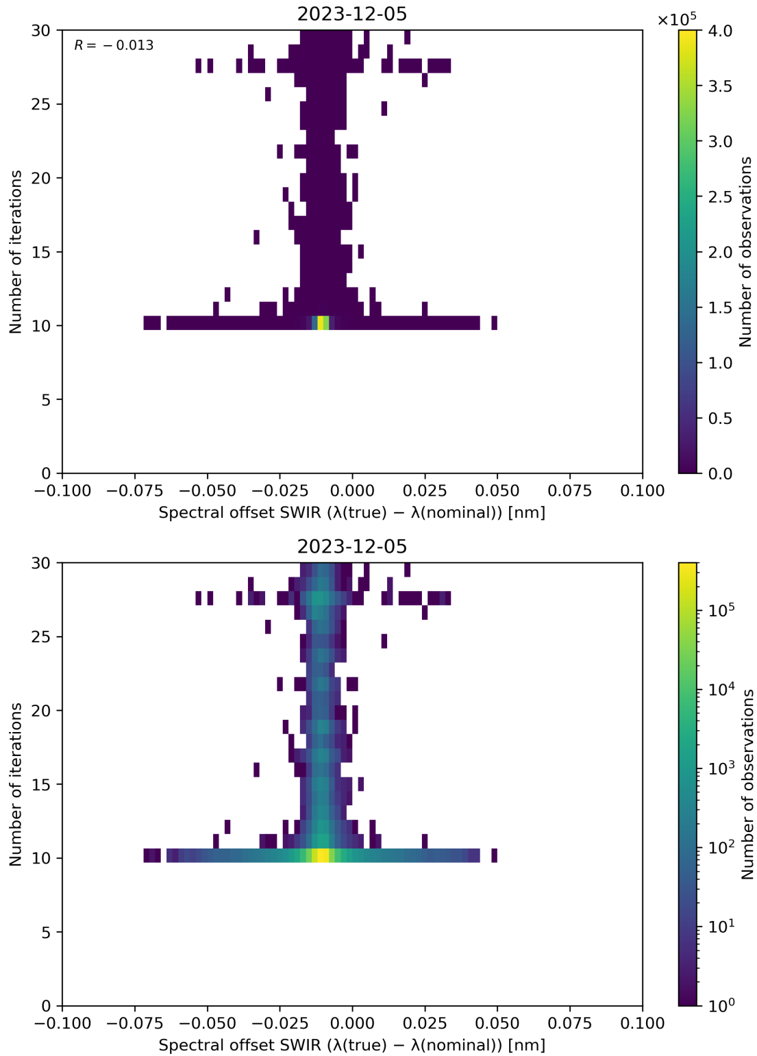
Figure 121: Scatter density plot of “Spectral offset SWIR ( \lambda(\text{true}) - \lambda(\text{nominal}) )” against “Number of iterations” for 2023-12-04 to 2023-12-06.
