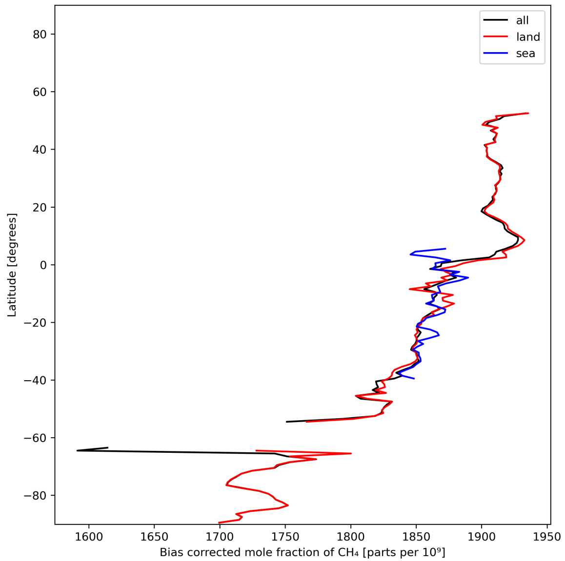
Figure 14: Zonal average of “Bias corrected mole fraction of CH 4 ” for 2023-12-04 to 2023-12-06.
