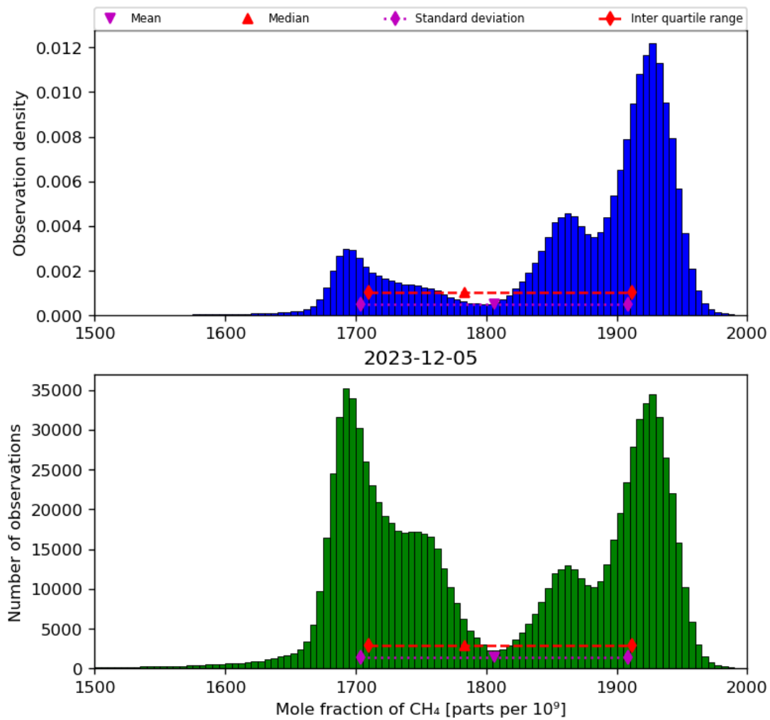
Figure 23: Histogram of “Mole fraction of CH 4 ” for 2023-12-04 to 2023-12-06
