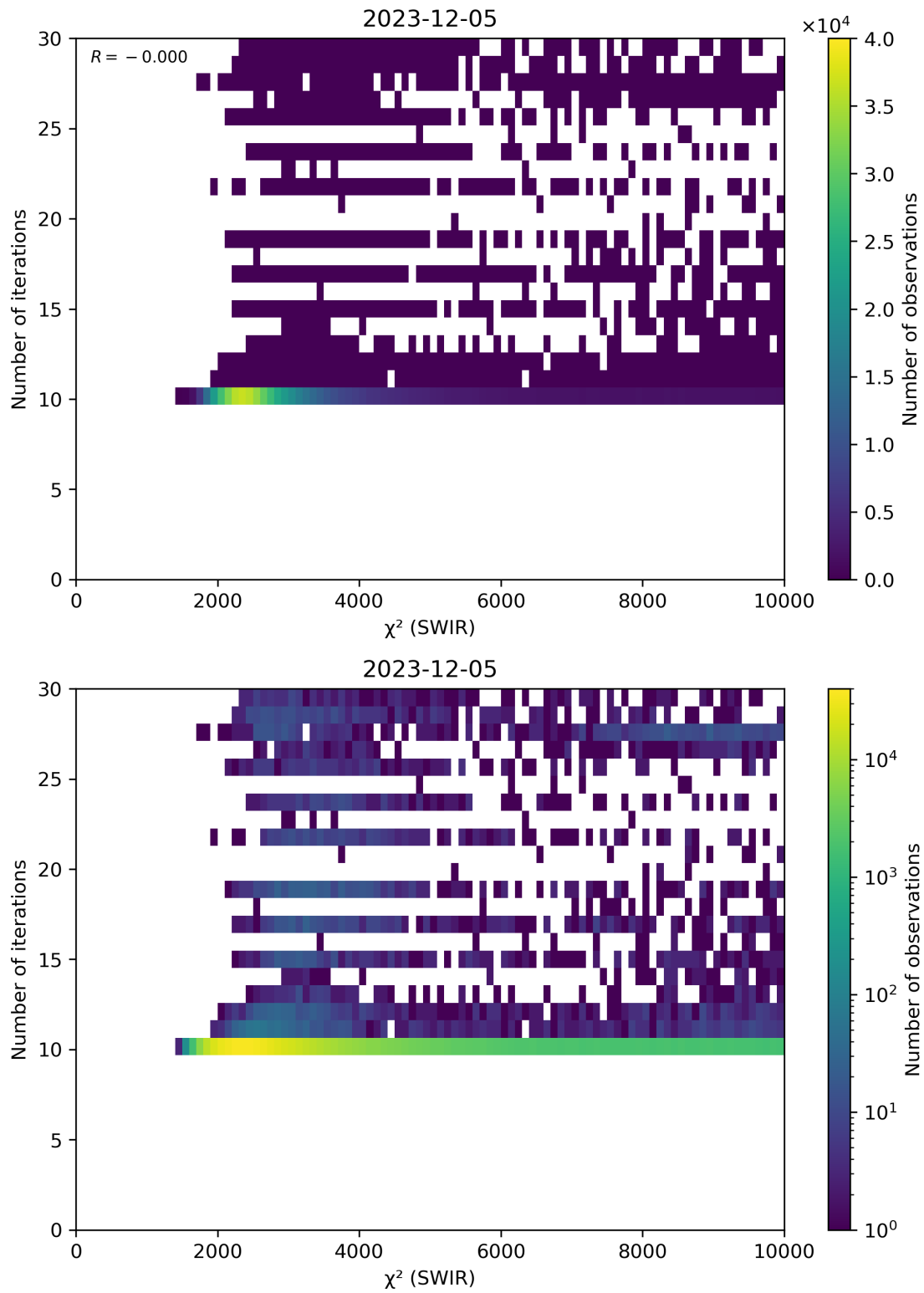
Figure 50: Scatter density plot of “ \chi^2 (SWIR)” against “Number of iterations” for 2023-12-04 to 2023-12-06.
