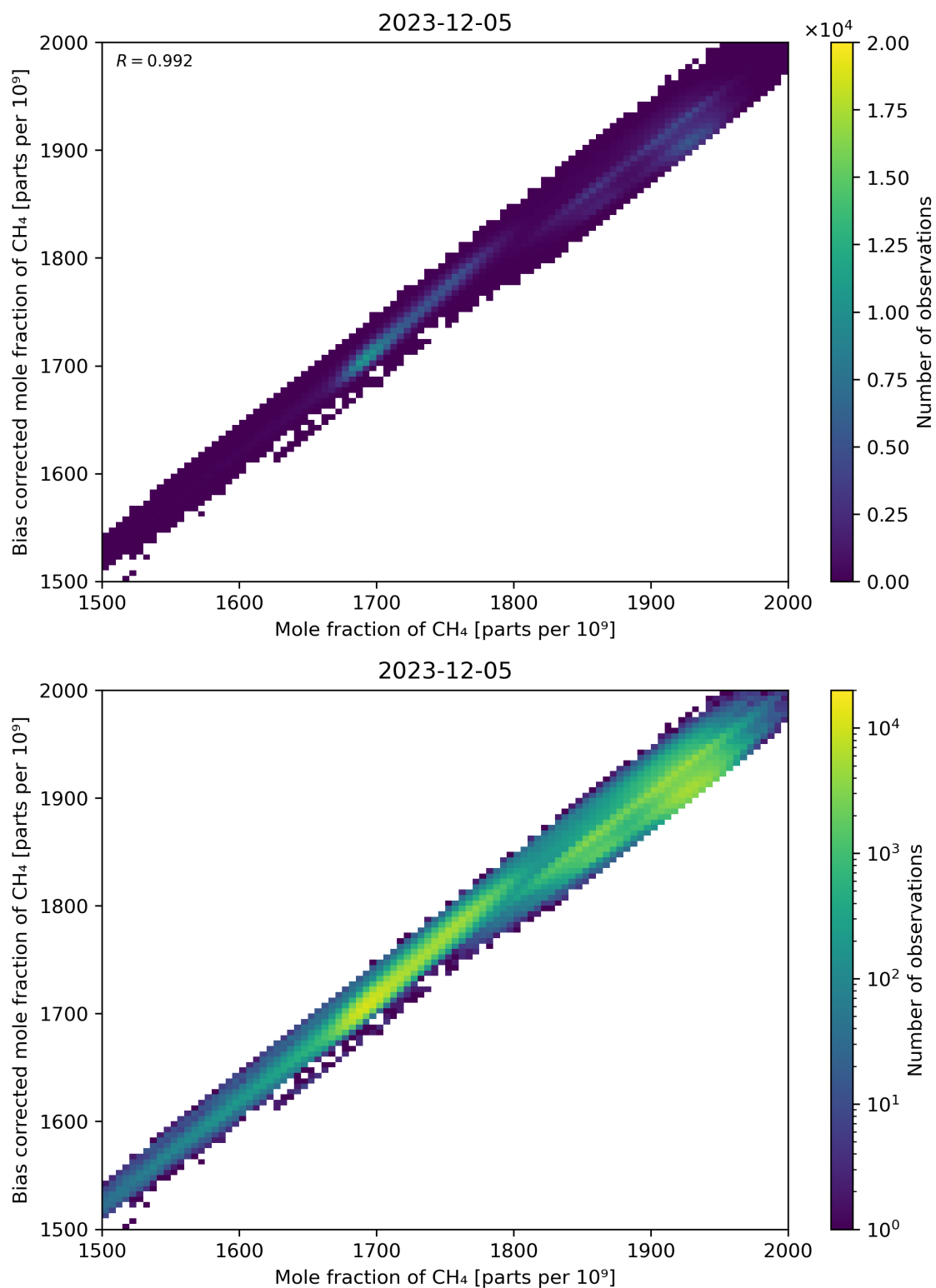
Figure 74: Scatter density plot of “Mole fraction of CH 4 ” against “Bias corrected mole fraction of CH 4 ” for 2023-12-04 to 2023-12-06.
