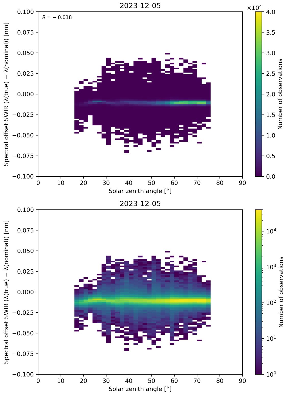
Figure 104: Scatter density plot of “Solar zenith angle” against “Spectral offset SWIR ( \lambda(\text{true}) - \lambda(\text{nominal}) )” for 2023-12-04 to 2023-12-06.
