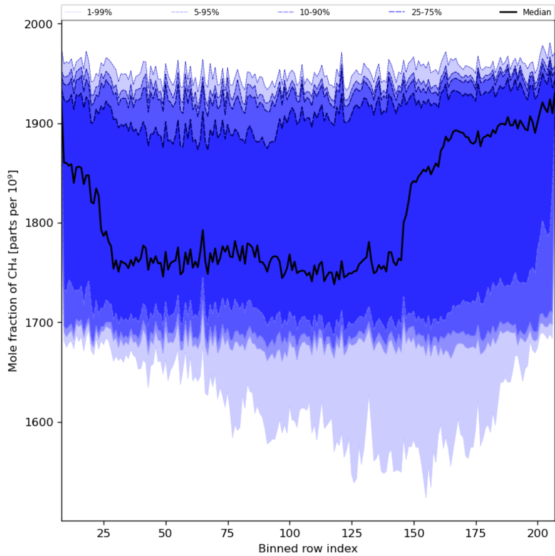
Figure 34: Along track statistics of “Mole fraction of CH 4 ” for 2023-12-04 to 2023-12-06
