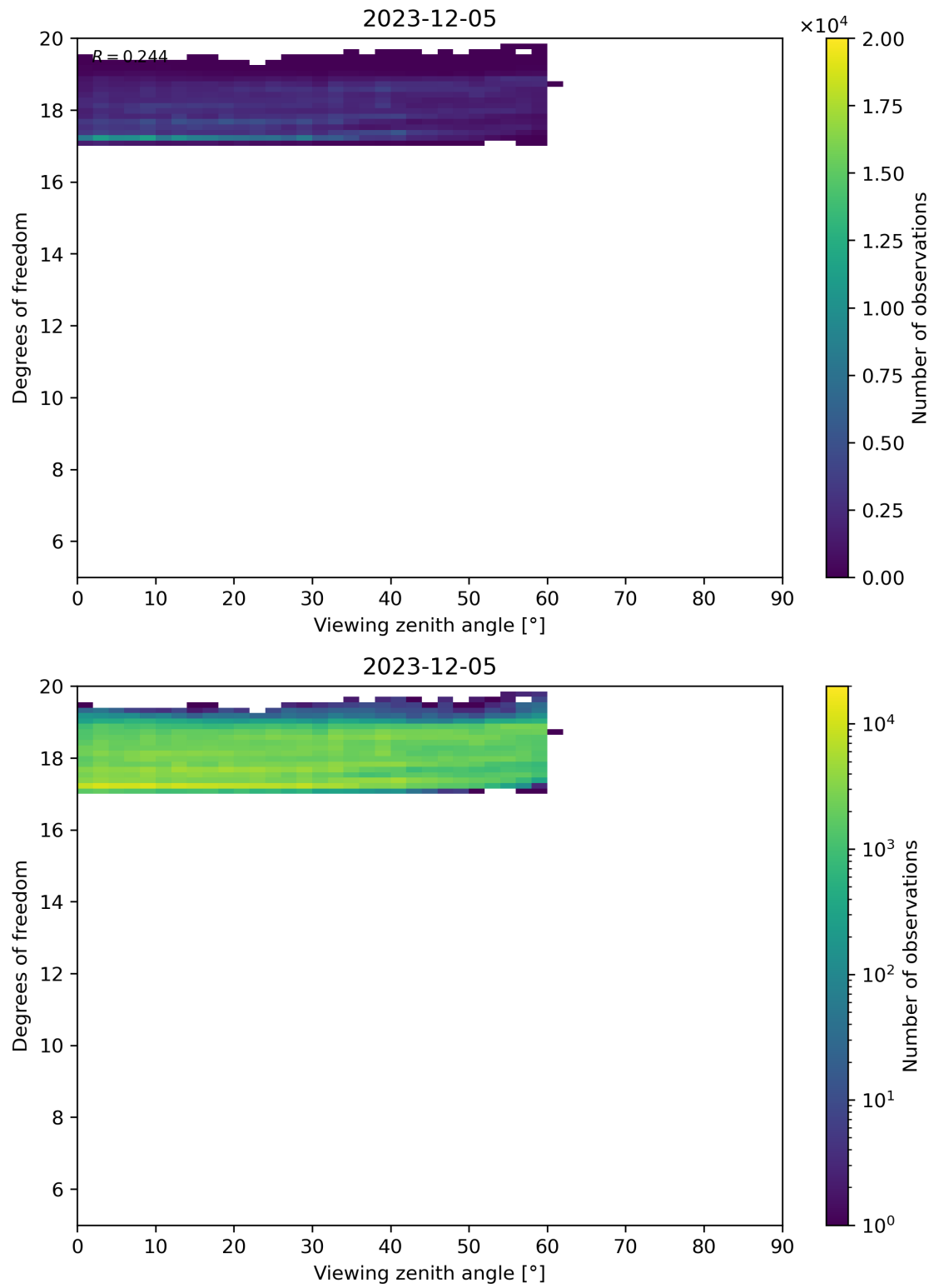
Figure 107: Scatter density plot of “Viewing zenith angle” against “Degrees of freedom” for 2023-12-04 to 2023-12-06.
