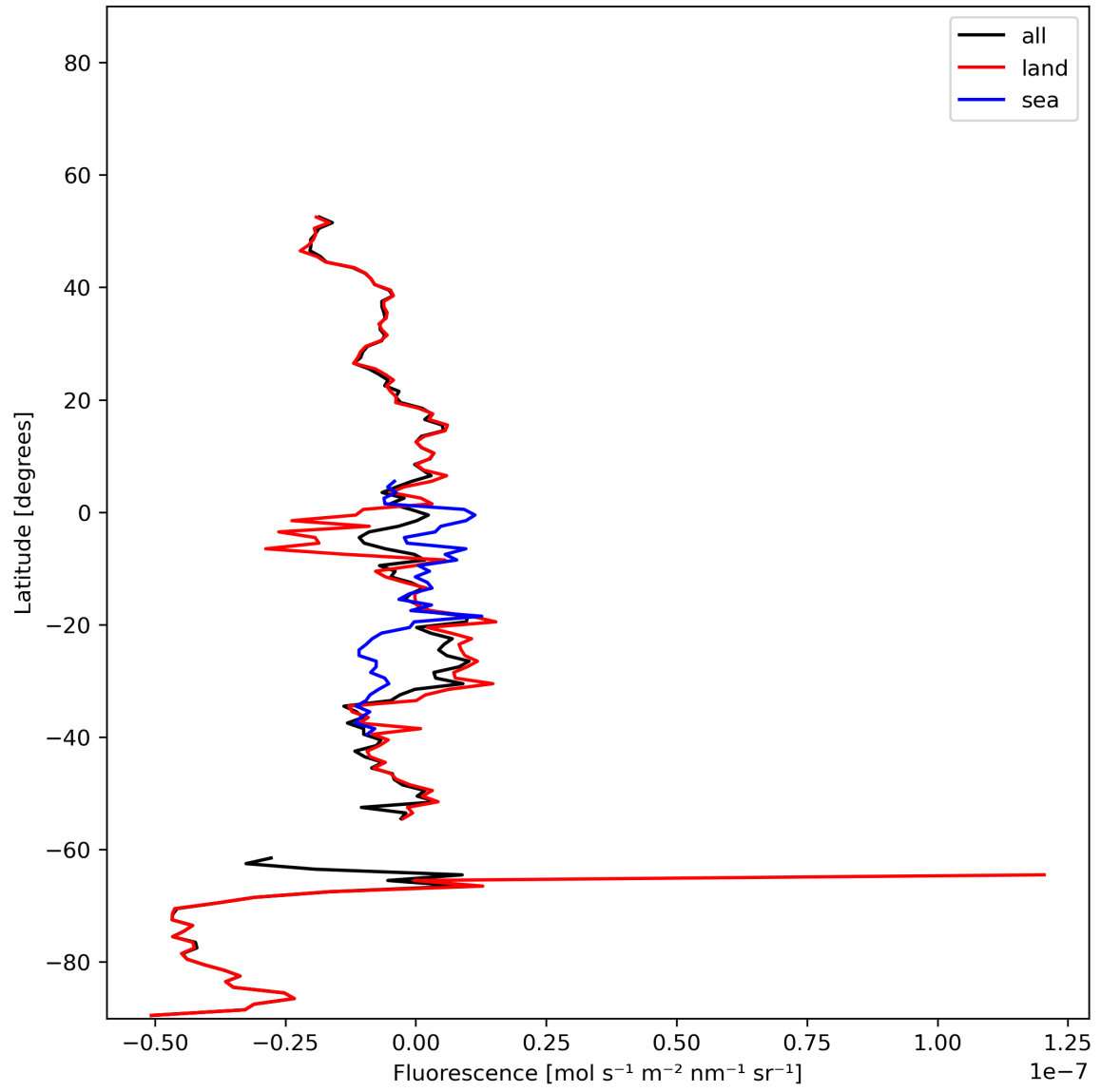
Figure 21: Zonal average of “Fluorescence” for 2023-12-05 to 2023-12-07.
