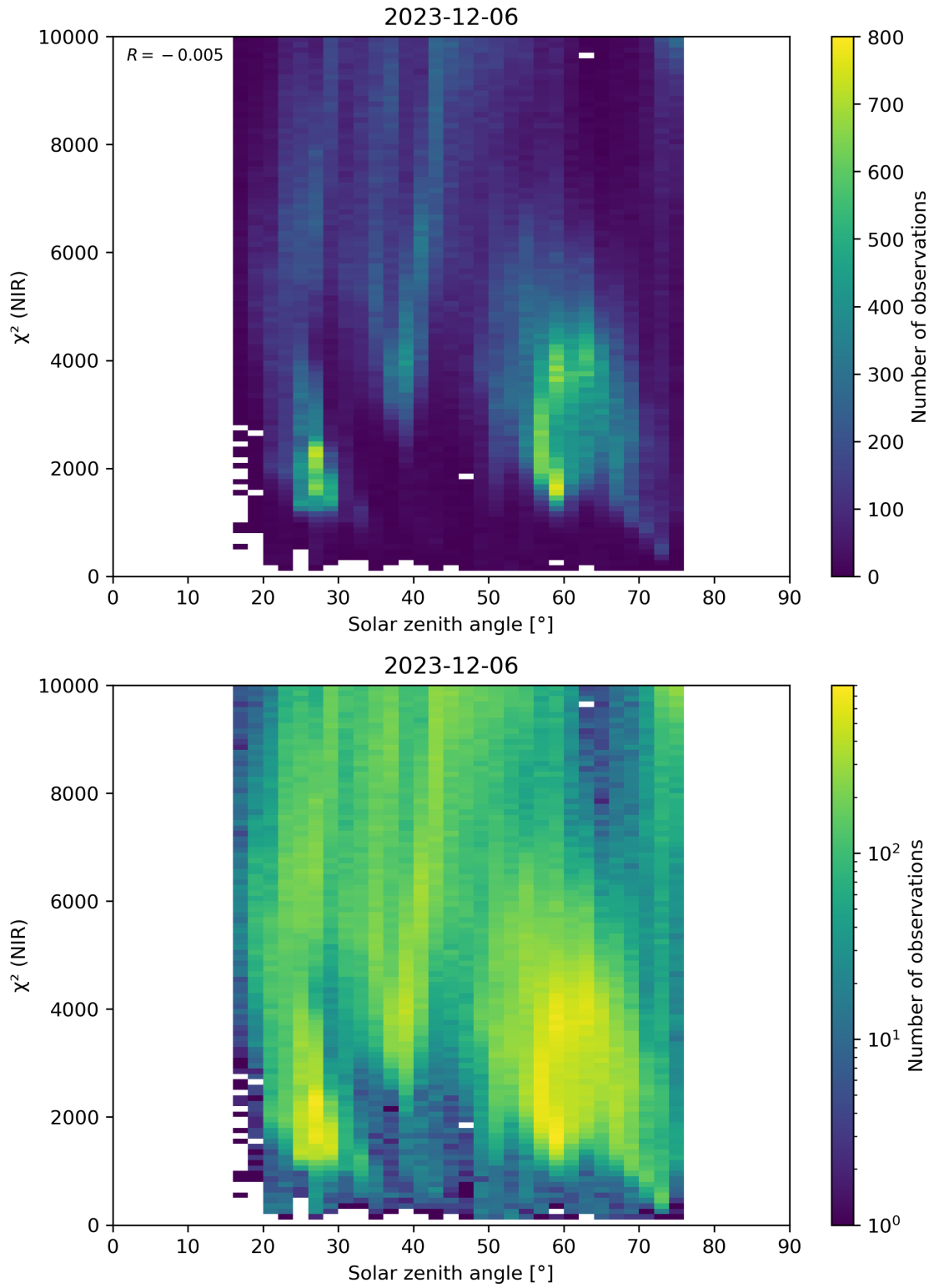
Figure 94: Scatter density plot of “Solar zenith angle” against “ \chi^2 (NIR)” for 2023-12-05 to 2023-12-07.
