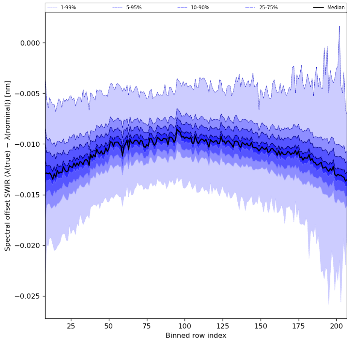
Figure 38: Along track statistics of “Spectral offset SWIR ( \lambda(\text{true}) - \lambda(\text{nominal}) )” for 2023-12-05 to 2023-12-07
