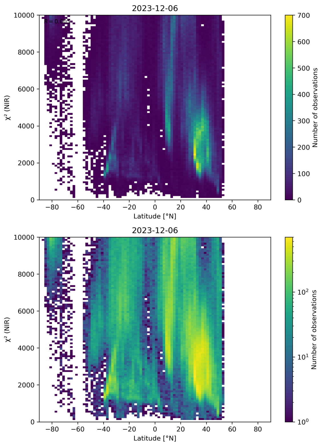
Figure 53: Scatter density plot of “Latitude” against “ \chi^2 (NIR)” for 2023-12-05 to 2023-12-07.
