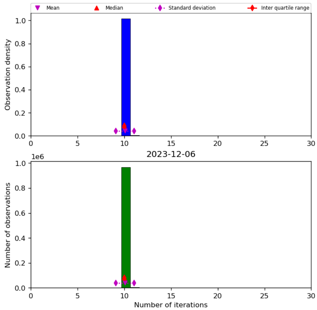
Figure 31: Histogram of “Number of iterations” for 2023-12-05 to 2023-12-07
