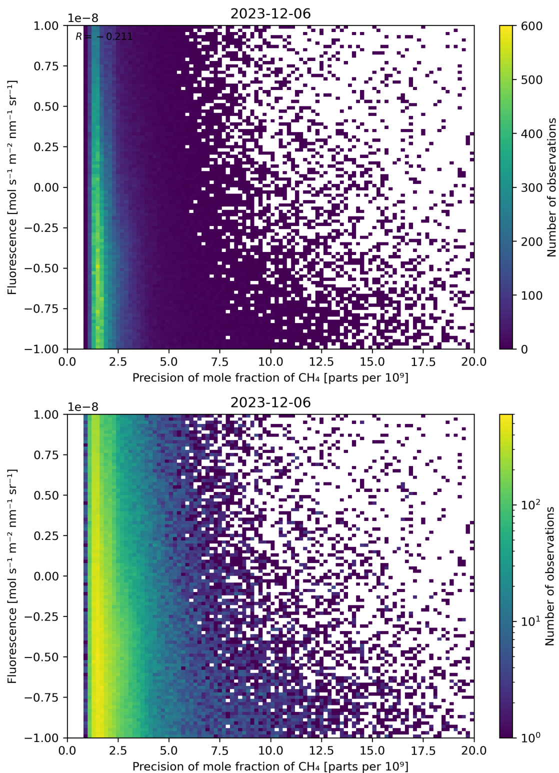
Figure 81: Scatter density plot of “Precision of mole fraction of \text{CH}_4 ” against “Fluorescence” for 2023-12-05 to 2023-12-07.
