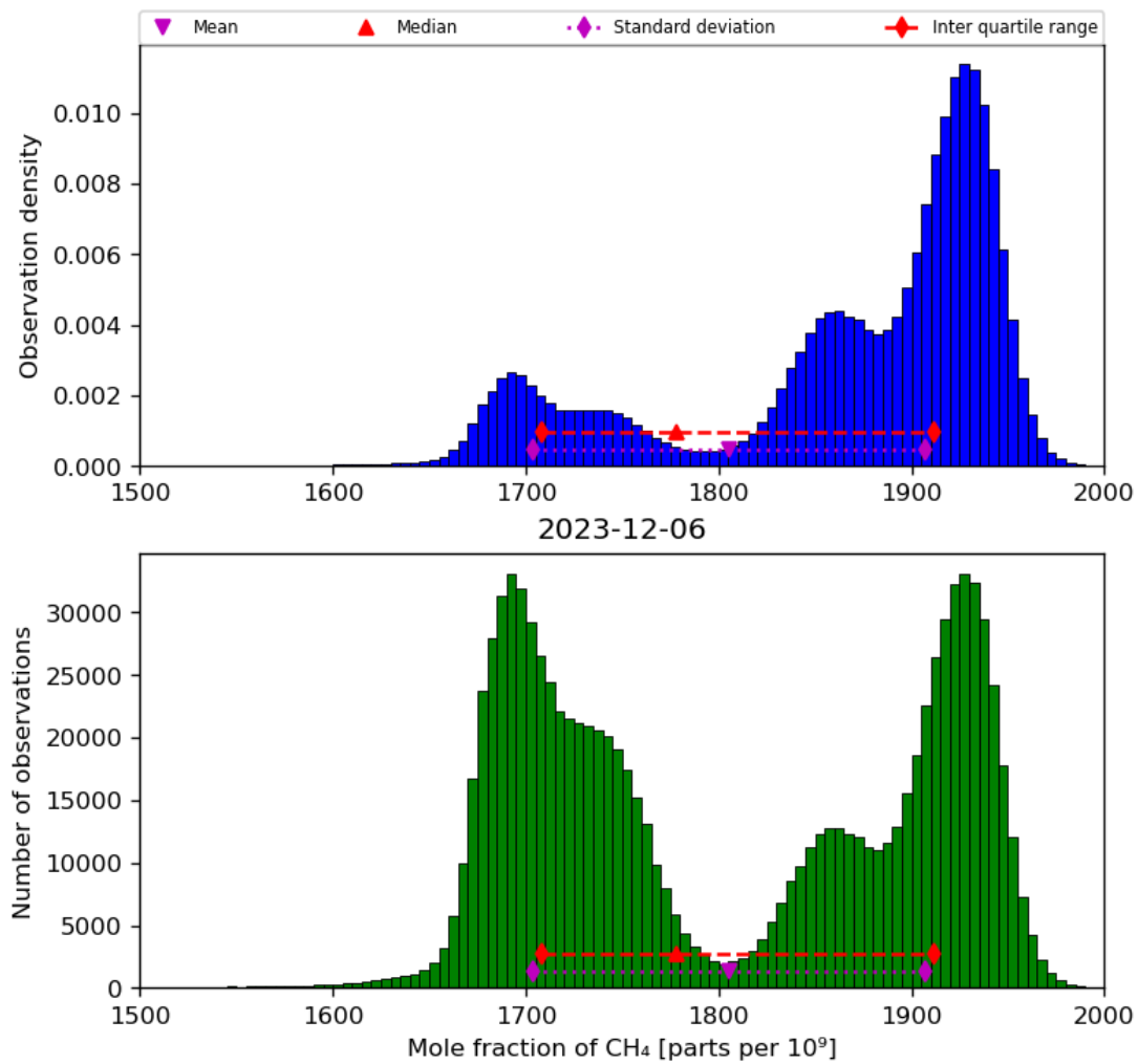
Figure 23: Histogram of “Mole fraction of CH 4 ” for 2023-12-05 to 2023-12-07
