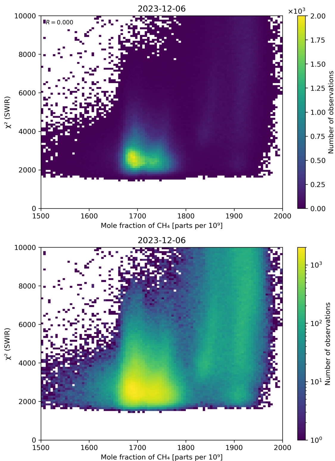
Figure 71: Scatter density plot of “Mole fraction of \text{CH}_4 ” against “ \chi^2 (SWIR)” for 2023-12-05 to 2023-12-07.
