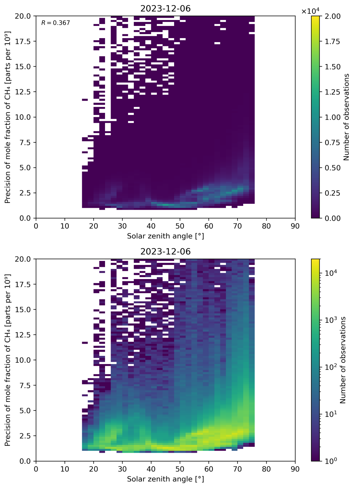
Figure 101: Scatter density plot of “Solar zenith angle” against “Precision of mole fraction of CH 4 ” for 2023-12-05 to 2023-12-07.
