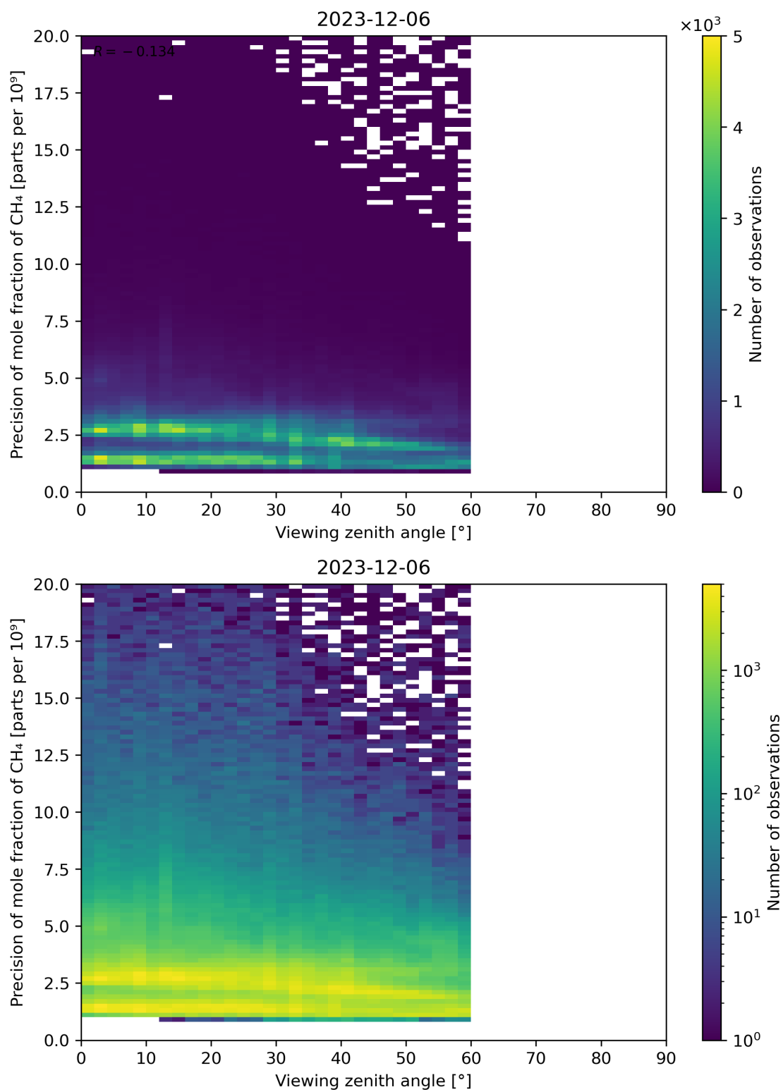
Figure 112: Scatter density plot of “Viewing zenith angle” against “Precision of mole fraction of CH 4 ” for 2023-12-05 to 2023-12-07.
