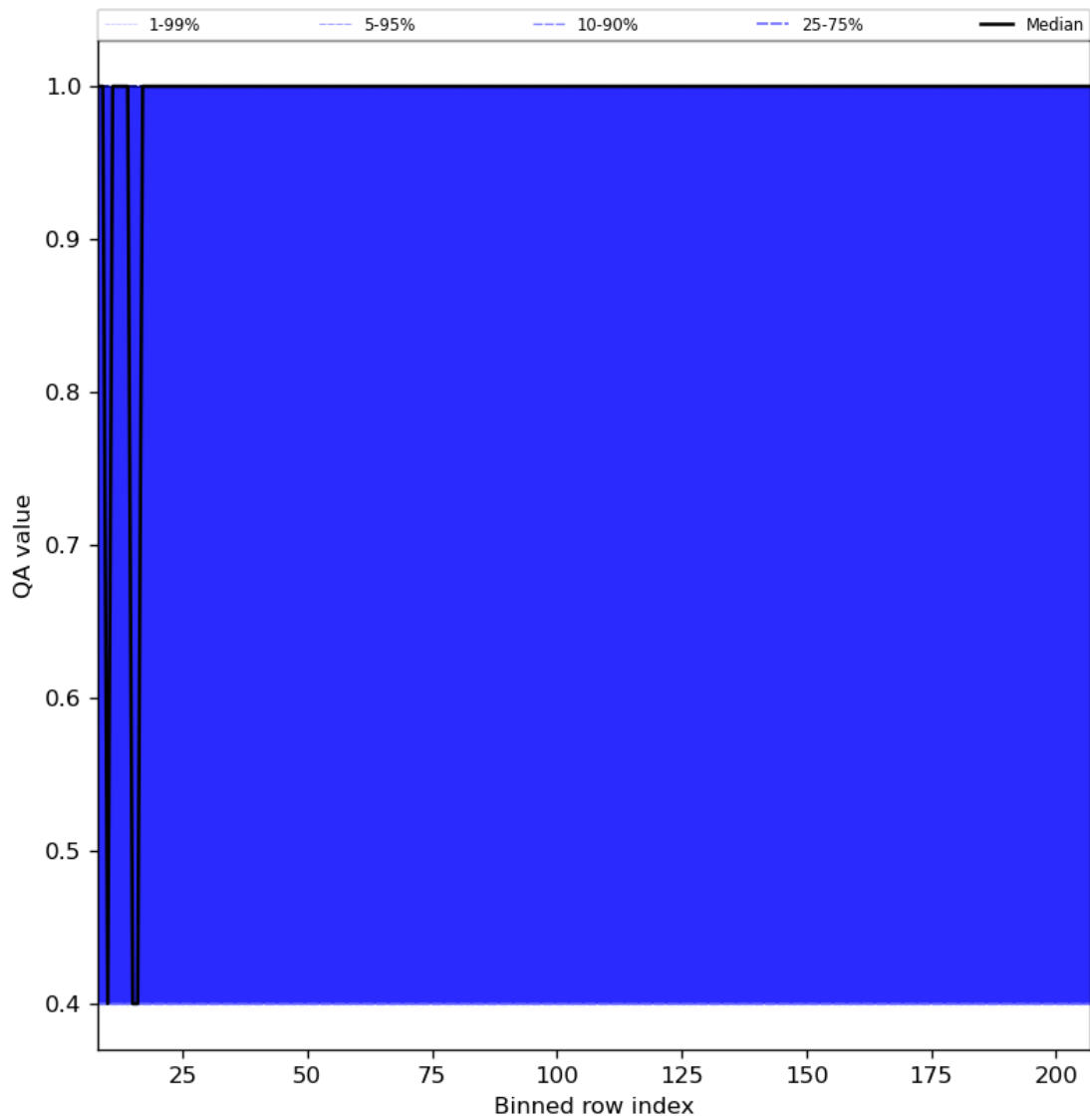
Figure 33: Along track statistics of “QA value” for 2023-12-05 to 2023-12-07
