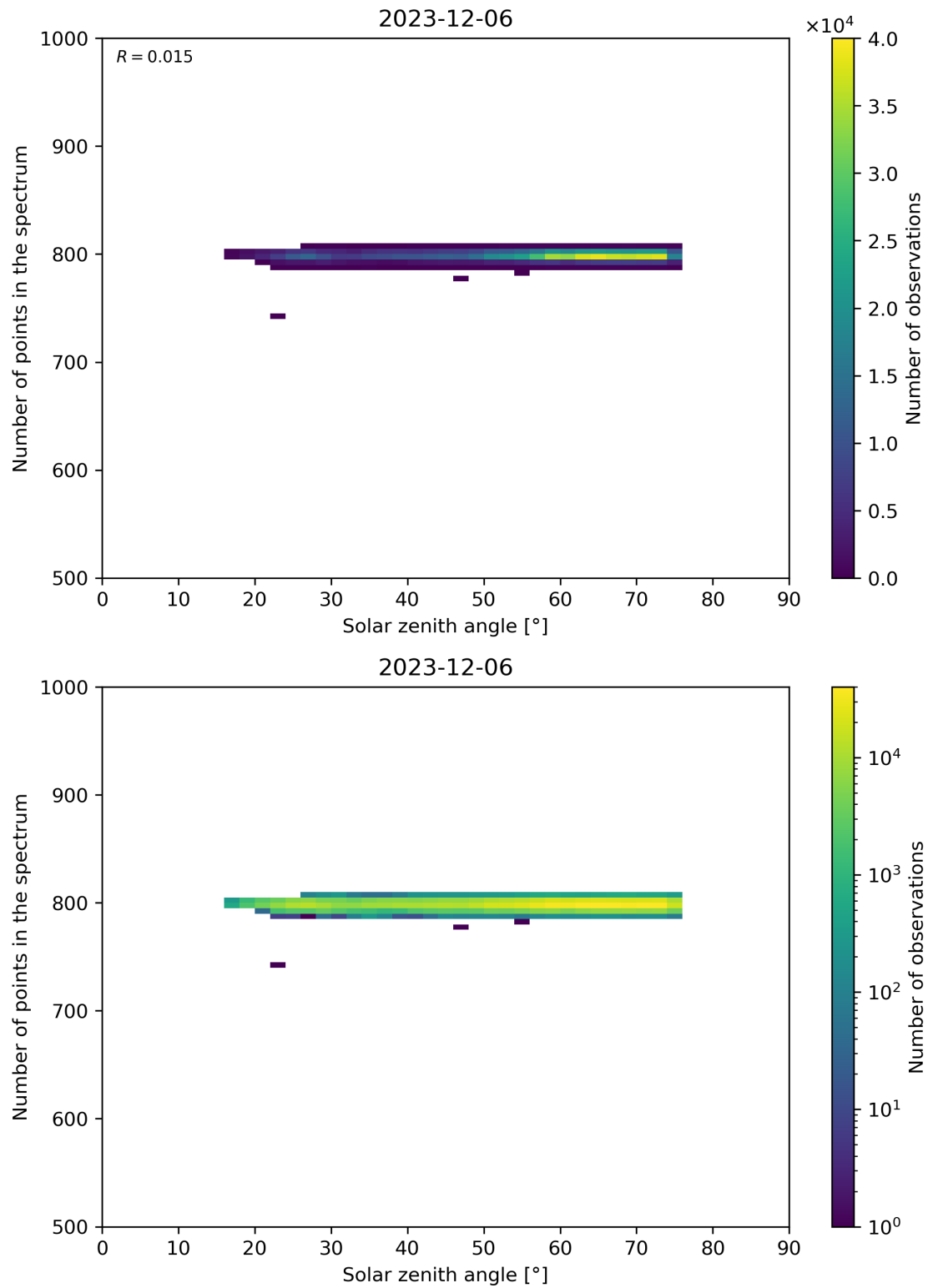
Figure 103: Scatter density plot of “Solar zenith angle” against “Number of points in the spectrum” for 2023-12-05 to 2023-12-07.
