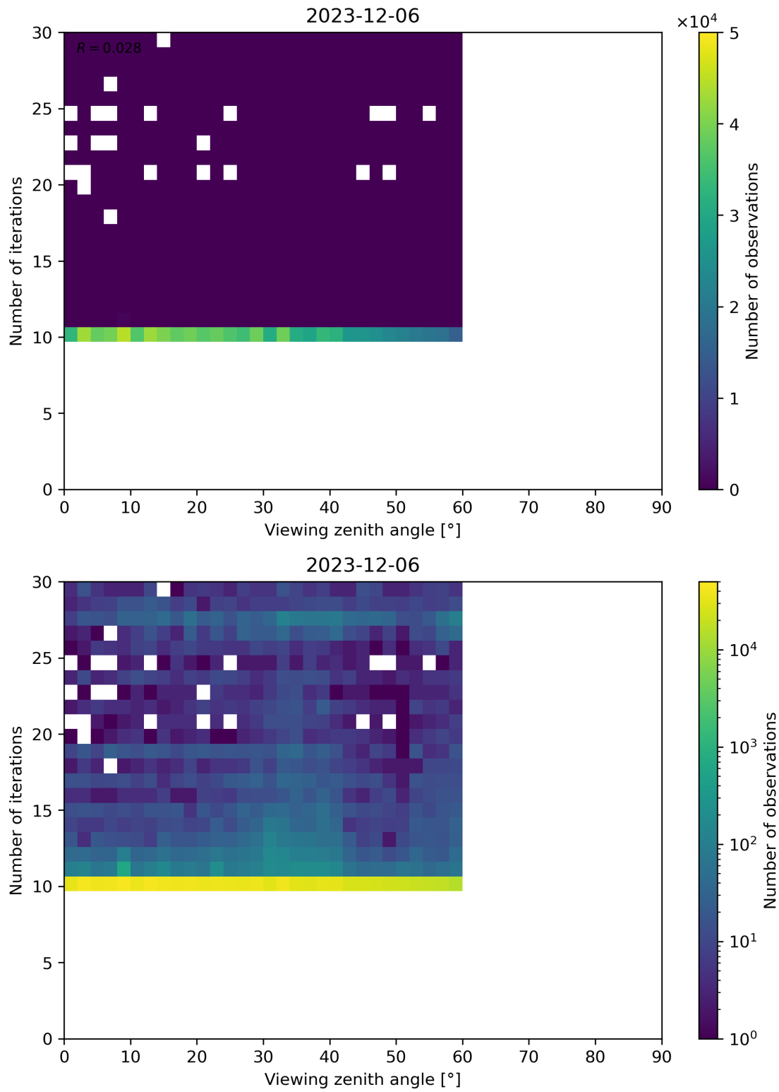
Figure 113: Scatter density plot of “Viewing zenith angle” against “Number of iterations” for 2023-12-05 to 2023-12-07.
