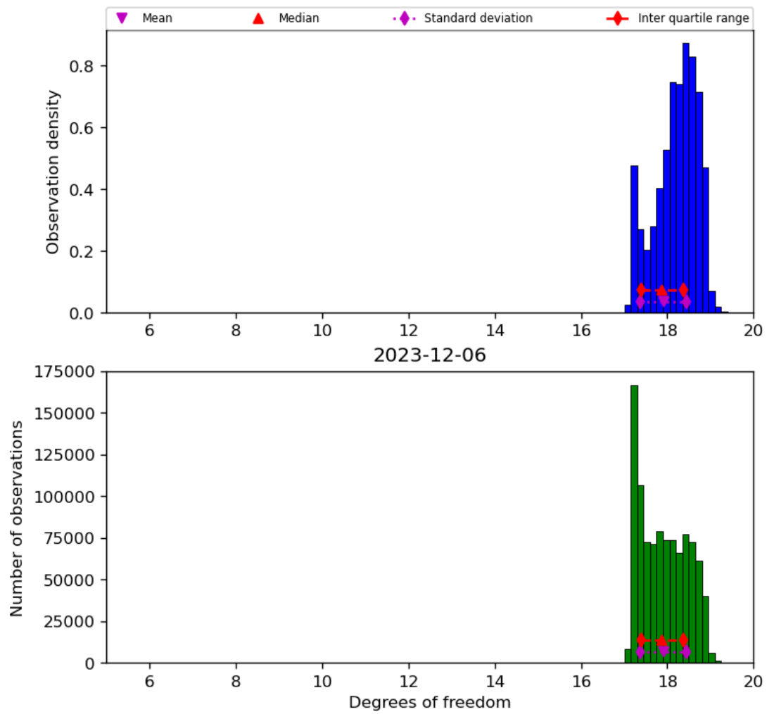
Figure 30: Histogram of “Degrees of freedom” for 2023-12-05 to 2023-12-07
