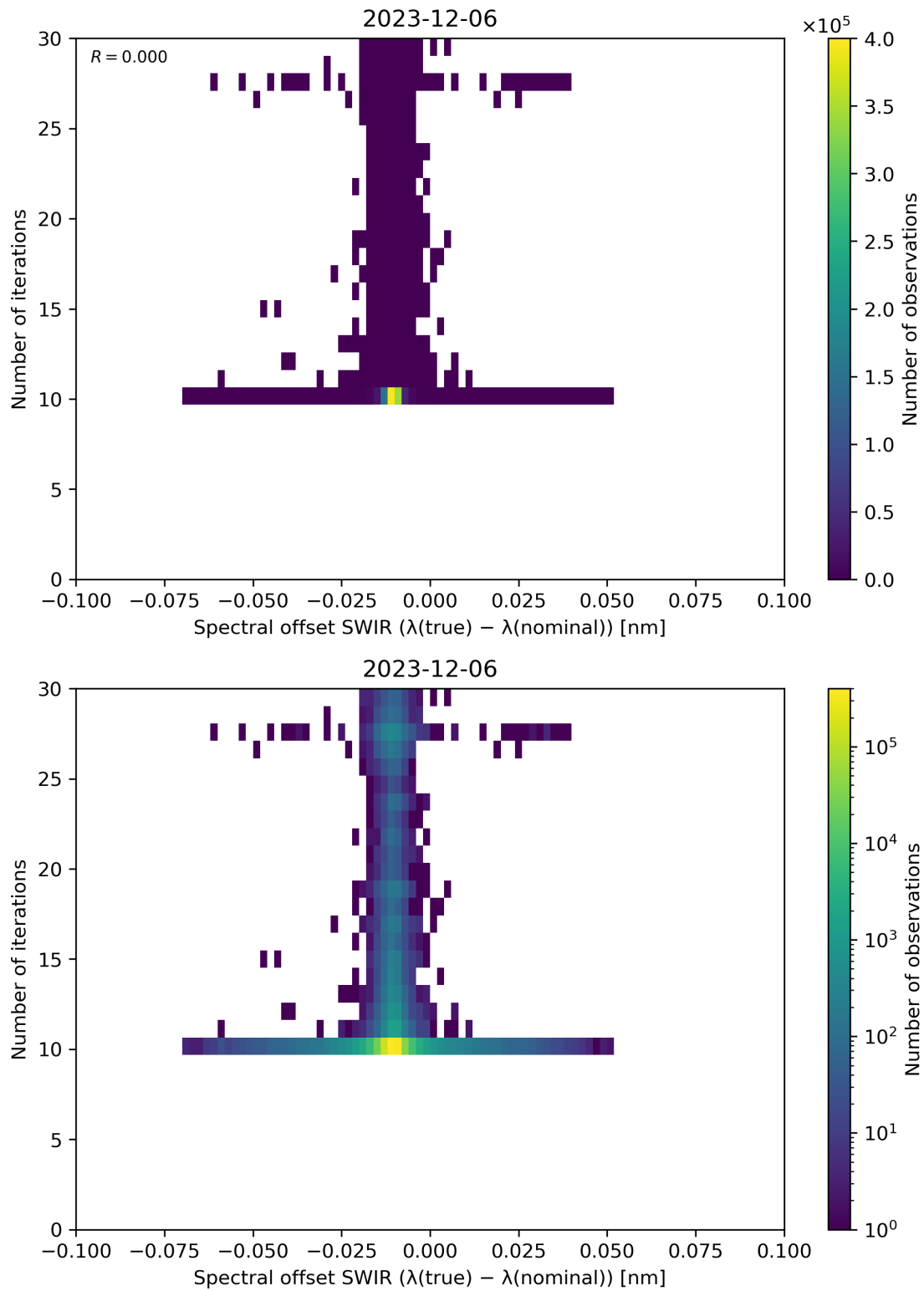
Figure 121: Scatter density plot of “Spectral offset SWIR ( \lambda(\text{true}) - \lambda(\text{nominal}) )” against “Number of iterations” for 2023-12-05 to 2023-12-07.
