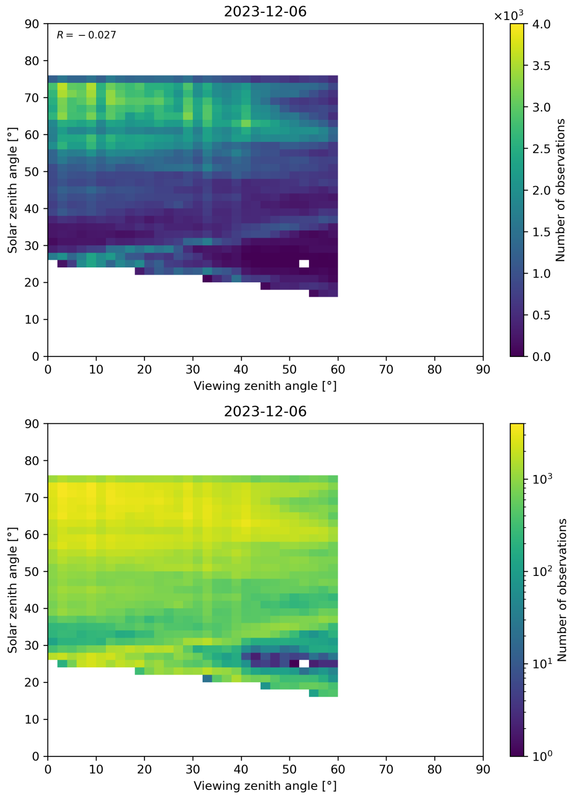
Figure 115: Scatter density plot of “Viewing zenith angle” against “Solar zenith angle” for 2023-12-05 to 2023-12-07.
