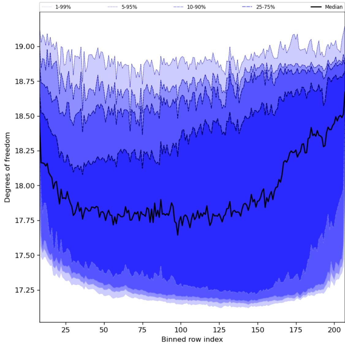
Figure 41: Along track statistics of “Degrees of freedom” for 2023-12-05 to 2023-12-07
