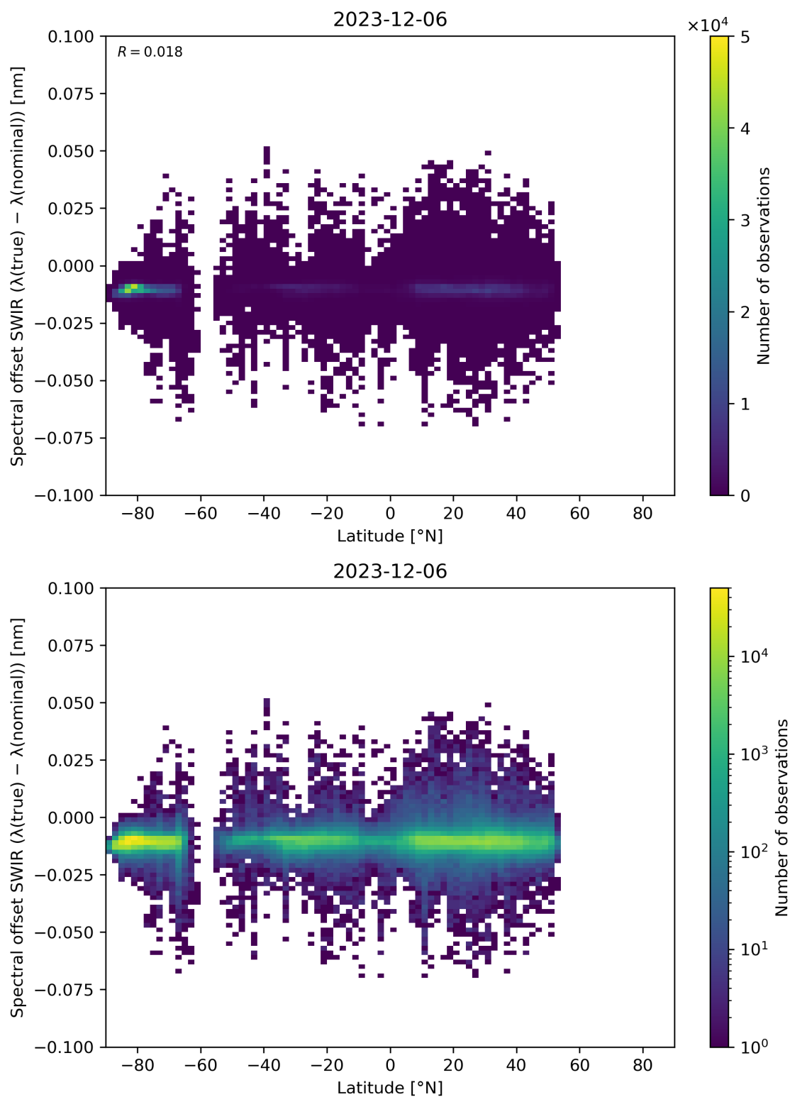
Figure 62: Scatter density plot of “Latitude” against “Spectral offset SWIR ( \lambda(\text{true}) - \lambda(\text{nominal}) )” for 2023-12-05 to 2023-12-07.
