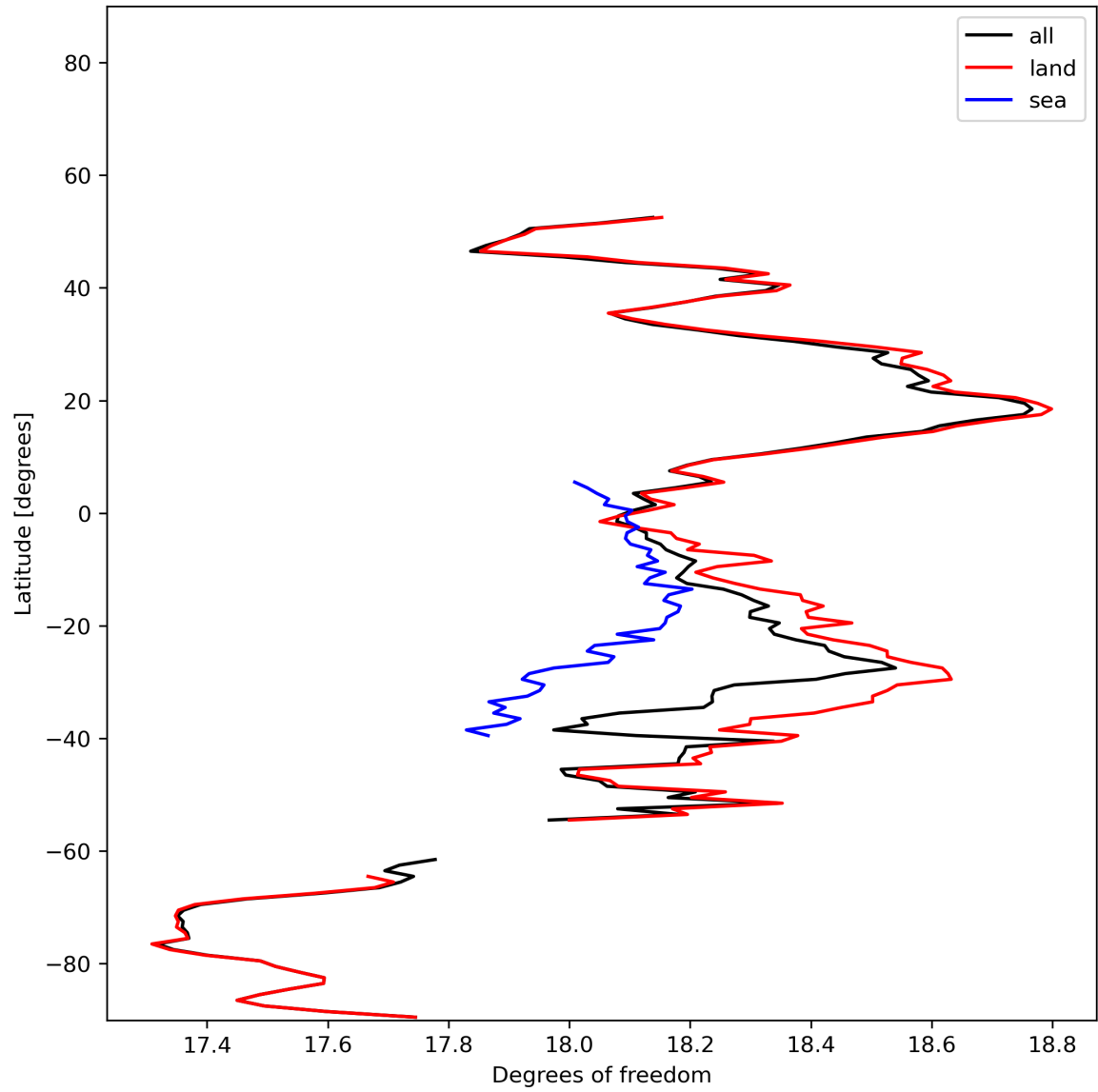
Figure 19: Zonal average of “Degrees of freedom” for 2023-12-05 to 2023-12-07.
