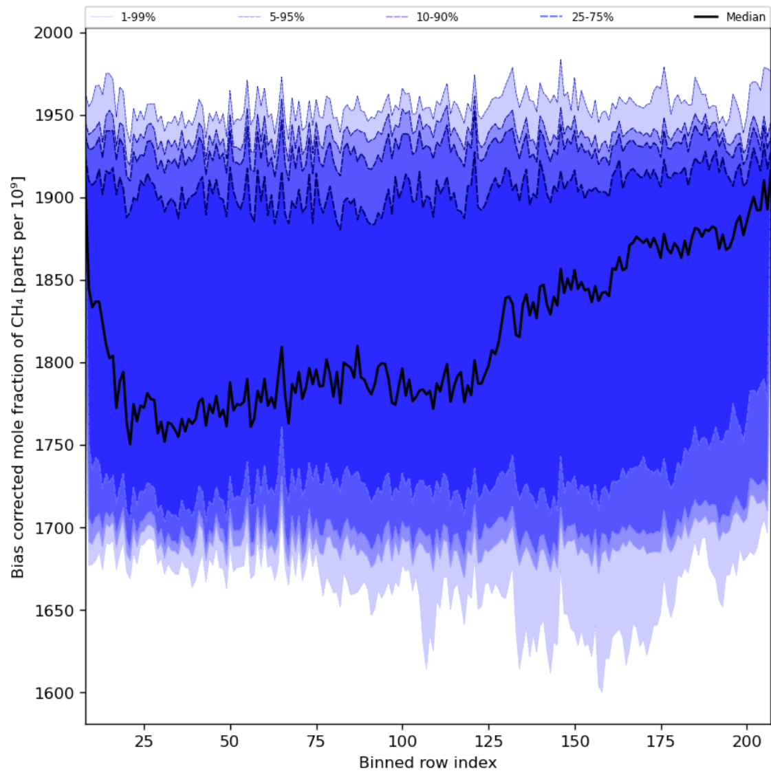
Figure 36: Along track statistics of “Bias corrected mole fraction of CH 4 ” for 2023-12-05 to 2023-12-07
