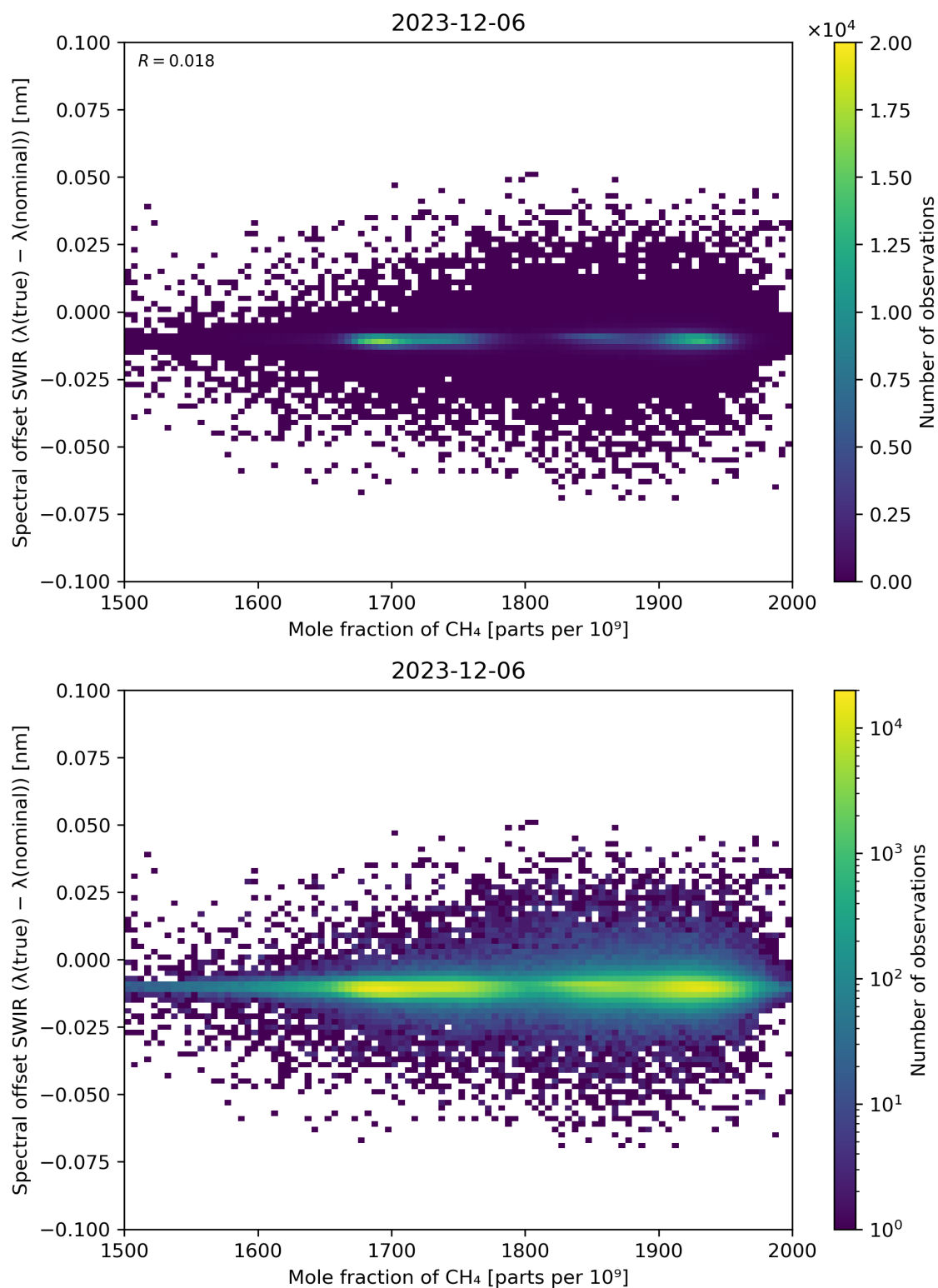
Figure 86: Scatter density plot of “Mole fraction of CH 4 ” against “Spectral offset SWIR ( \lambda(\text{true}) - \lambda(\text{nominal}) )” for 2023-12-05 to 2023-12-07.
