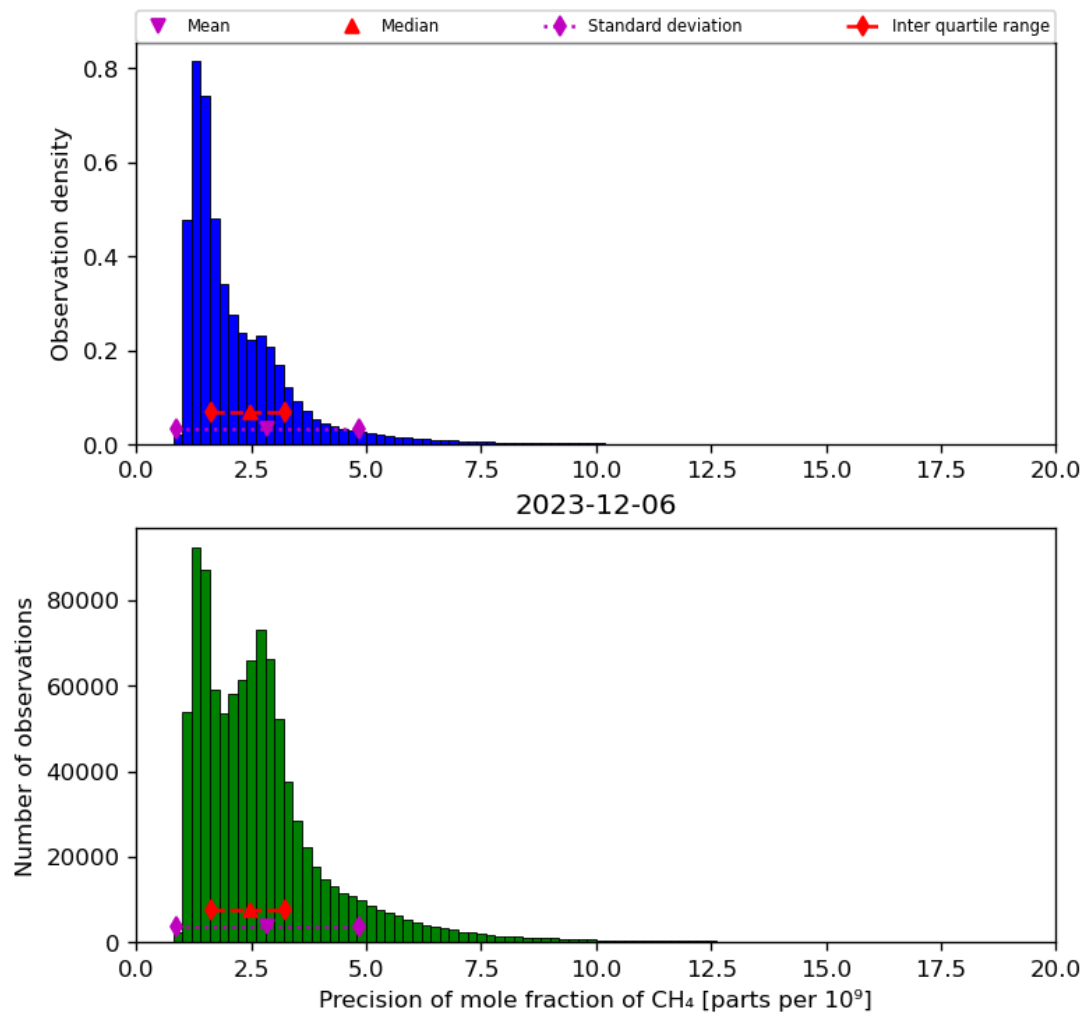
Figure 24: Histogram of “Precision of mole fraction of CH 4 ” for 2023-12-05 to 2023-12-07
