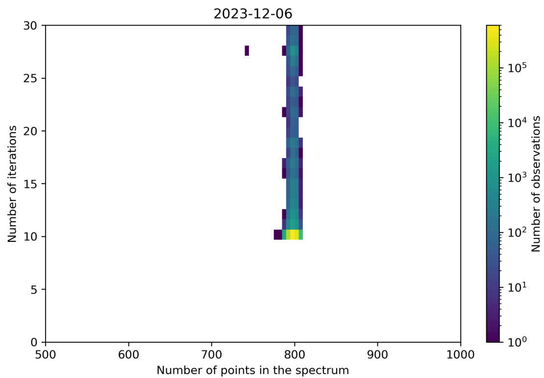
Figure 92: Scatter density plot of “Number of points in the spectrum” against “Number of iterations” for 2023-12-05 to 2023-12-07.
