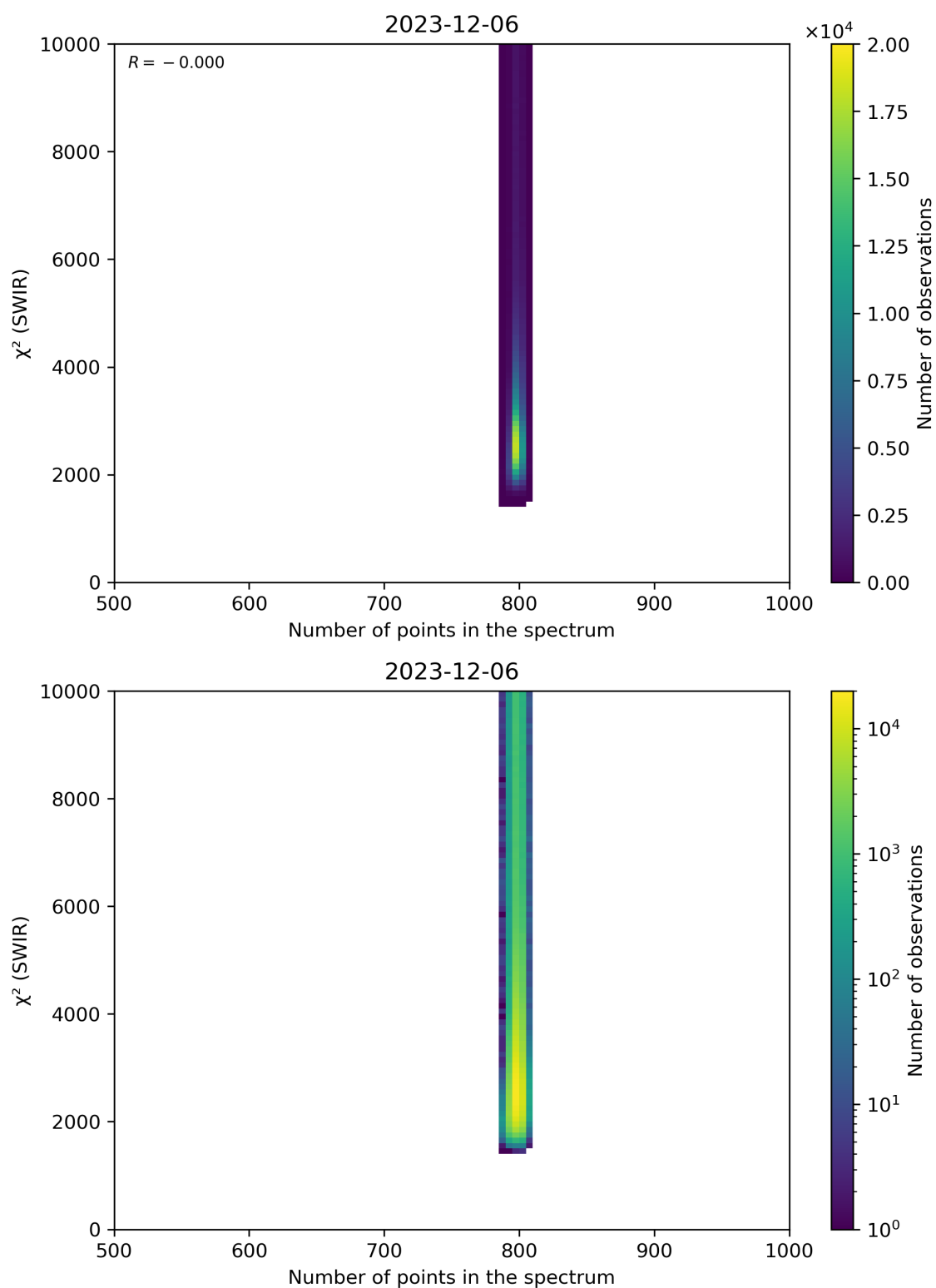
Figure 89: Scatter density plot of “Number of points in the spectrum” against “ \chi^2 (SWIR)” for 2023-12-05 to 2023-12-07.
