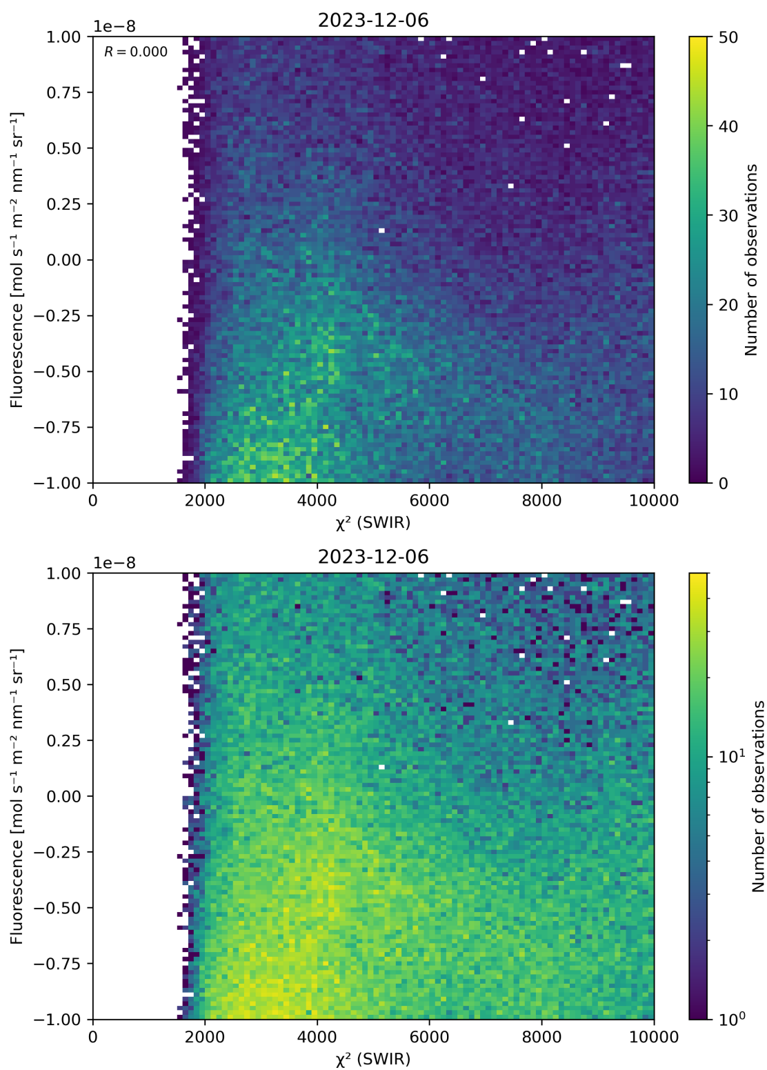
Figure 49: Scatter density plot of “ \chi^2 (SWIR)” against “Fluorescence” for 2023-12-05 to 2023-12-07.
