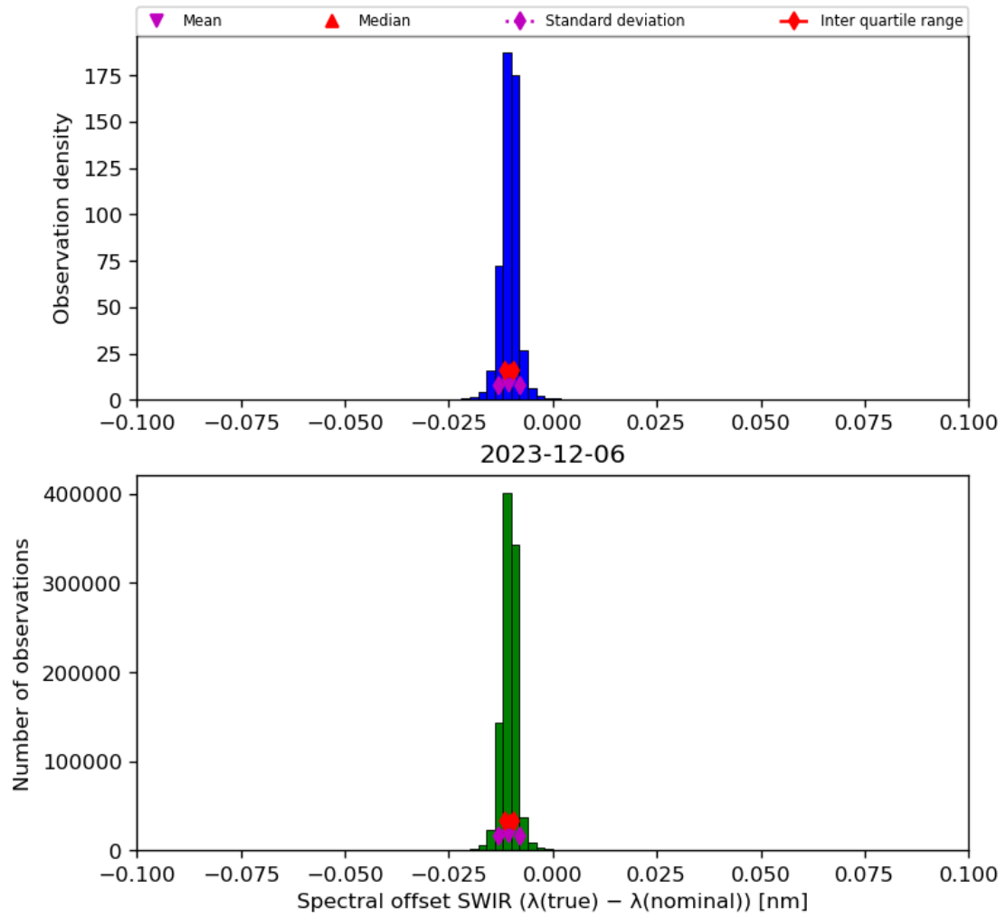
Figure 27: Histogram of “Spectral offset SWIR ( \lambda(\text{true}) - \lambda(\text{nominal}) )” for 2023-12-05 to 2023-12-07
