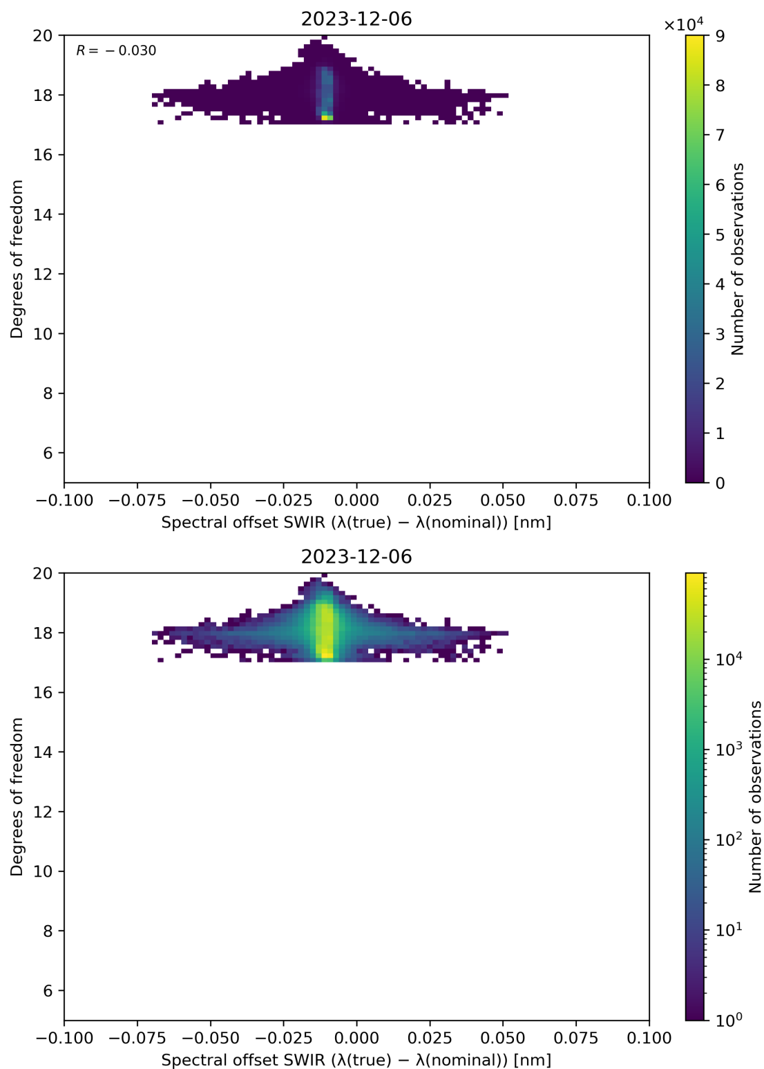
Figure 119: Scatter density plot of “Spectral offset SWIR ( \lambda(\text{true}) - \lambda(\text{nominal}) )” against “Degrees of freedom” for 2023-12-05 to 2023-12-07.
