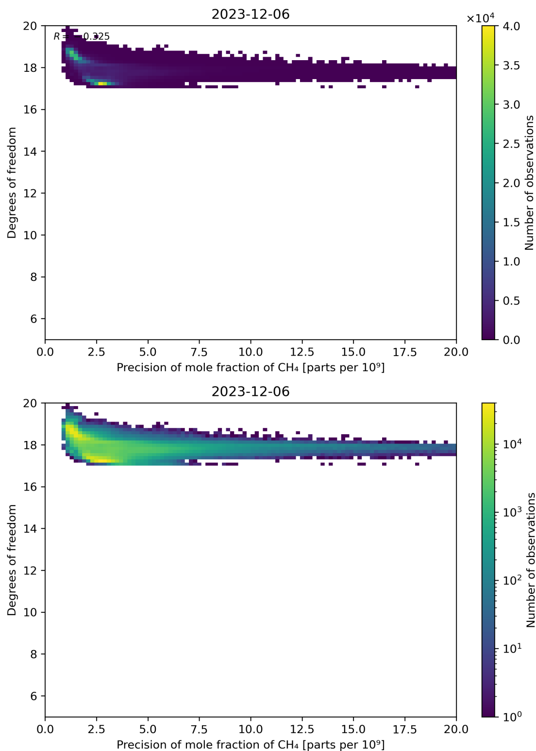
Figure 80: Scatter density plot of “Precision of mole fraction of CH 4 ” against “Degrees of freedom” for 2023-12-05 to 2023-12-07.
