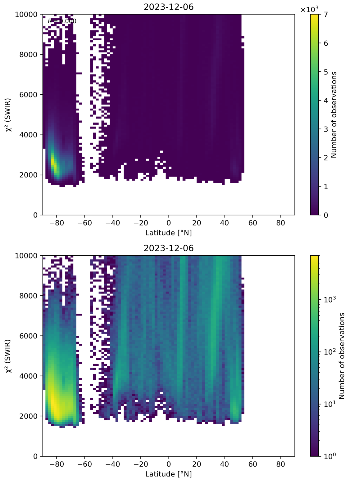
Figure 54: Scatter density plot of “Latitude” against “ \chi^2 (SWIR)” for 2023-12-05 to 2023-12-07.
