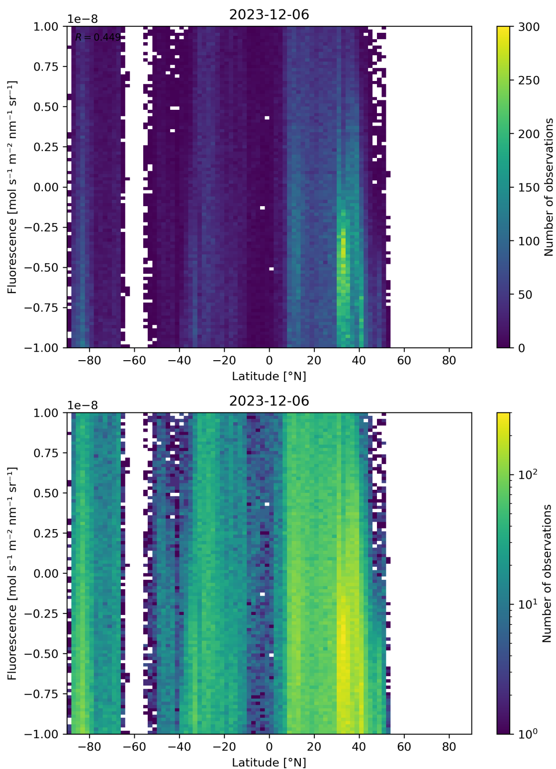
Figure 56: Scatter density plot of “Latitude” against “Fluorescence” for 2023-12-05 to 2023-12-07.
