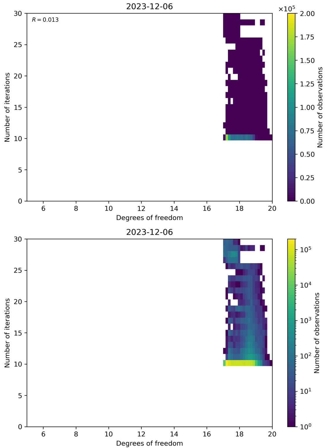
Figure 52: Scatter density plot of “Degrees of freedom” against “Number of iterations” for 2023-12-05 to 2023-12-07.
