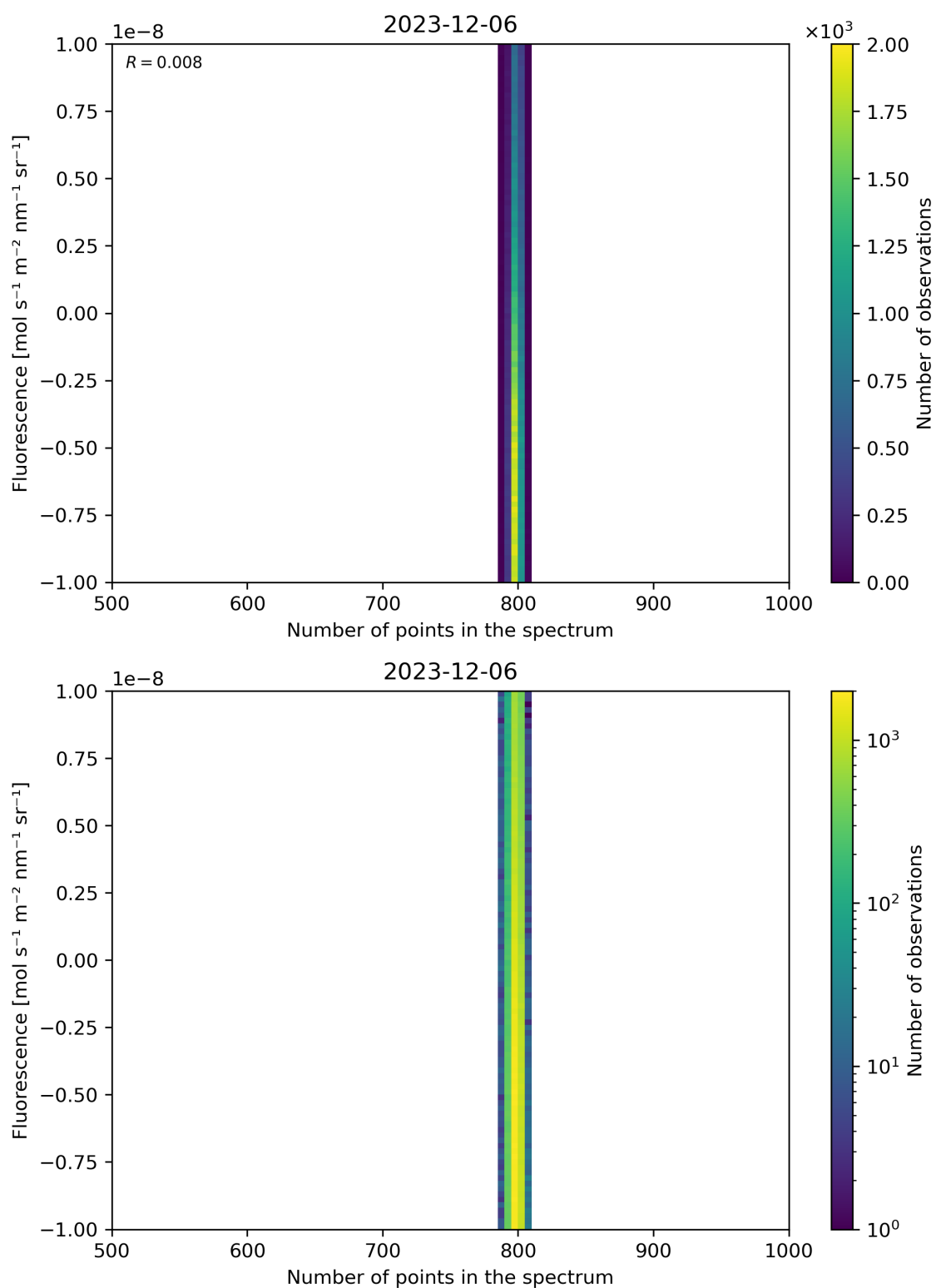
Figure 91: Scatter density plot of “Number of points in the spectrum” against “Fluorescence” for 2023-12-05 to 2023-12-07.
