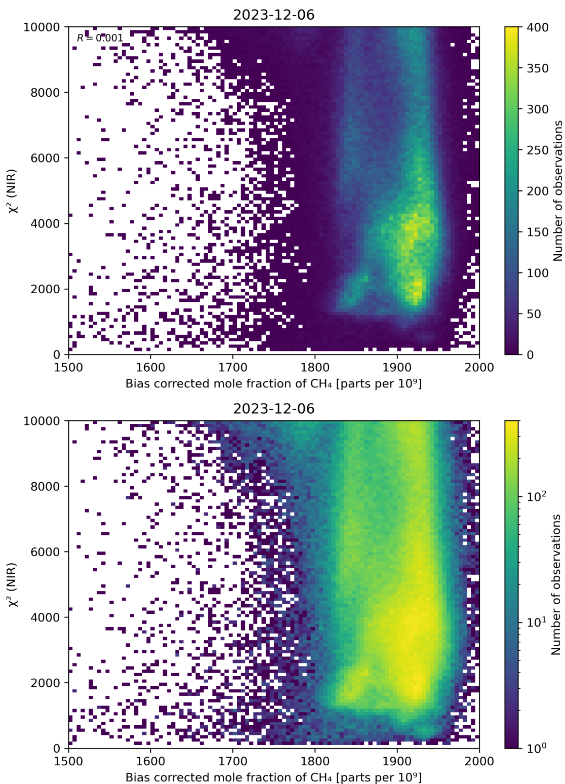
Figure 63: Scatter density plot of “Bias corrected mole fraction of CH 4 ” against “ \chi^2 (NIR)” for 2023-12-05 to 2023-12-07.
