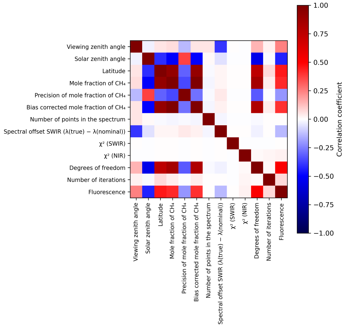
Figure 2: Map of correlation matrix for 2023-12-05 to 2023-12-07.
