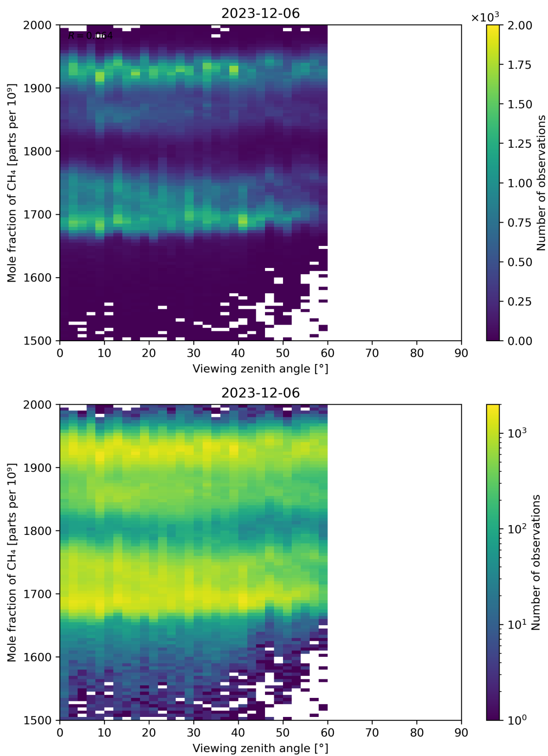
Figure 110: Scatter density plot of “Viewing zenith angle” against “Mole fraction of CH 4 ” for 2023-12-05 to 2023-12-07.
