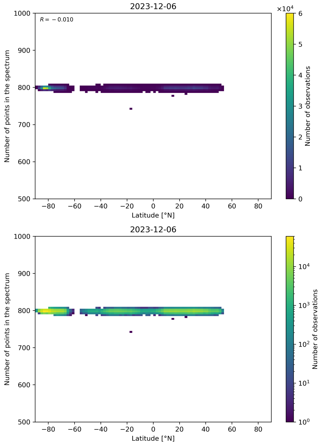
Figure 61: Scatter density plot of “Latitude” against “Number of points in the spectrum” for 2023-12-05 to 2023-12-07.
