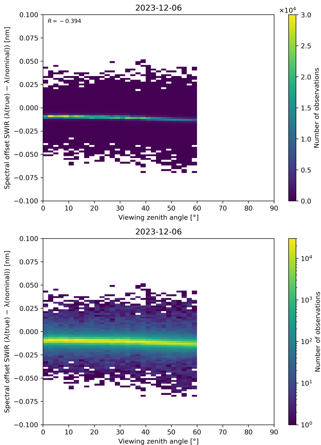
Figure 116: Scatter density plot of “Viewing zenith angle” against “Spectral offset SWIR ( \lambda(\text{true}) - \lambda(\text{nominal}) )” for 2023-12-05 to 2023-12-07.
