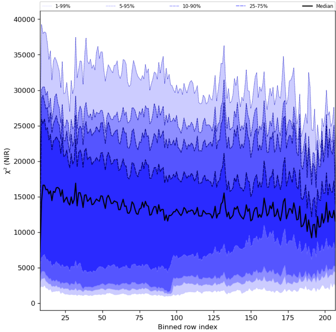
Figure 40: Along track statistics of “ \chi^2 (NIR)” for 2023-12-05 to 2023-12-07
