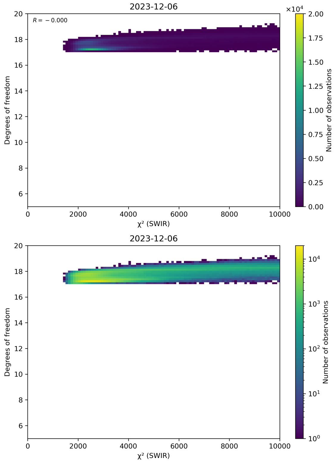
Figure 48: Scatter density plot of “ \chi^2 (SWIR)” against “Degrees of freedom” for 2023-12-05 to 2023-12-07.
