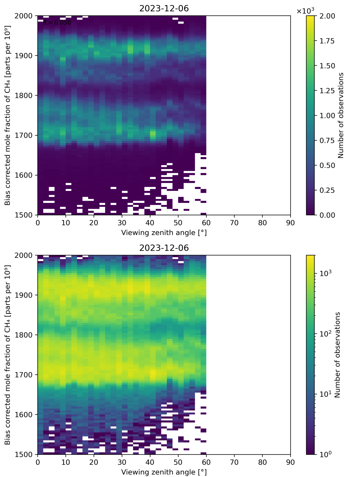
Figure 111: Scatter density plot of “Viewing zenith angle” against “Bias corrected mole fraction of CH 4 ” for 2023-12-05 to 2023-12-07.
