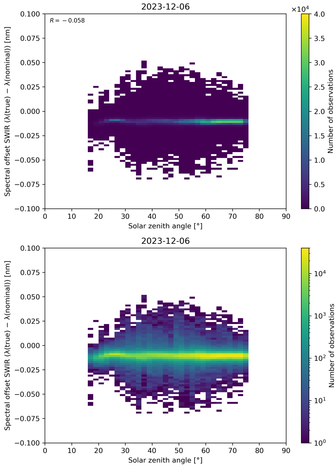
Figure 104: Scatter density plot of “Solar zenith angle” against “Spectral offset SWIR ( \lambda(\text{true}) - \lambda(\text{nominal}) )” for 2023-12-05 to 2023-12-07.
