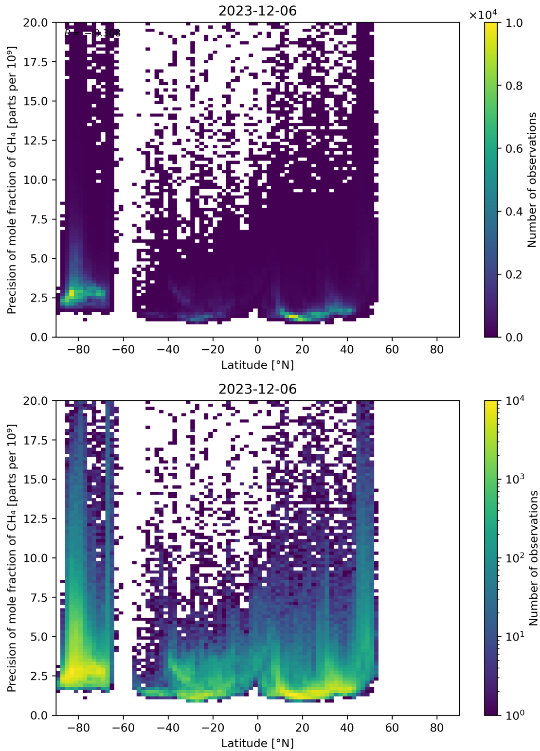
Figure 59: Scatter density plot of “Latitude” against “Precision of mole fraction of CH 4 ” for 2023-12-05 to 2023-12-07.
