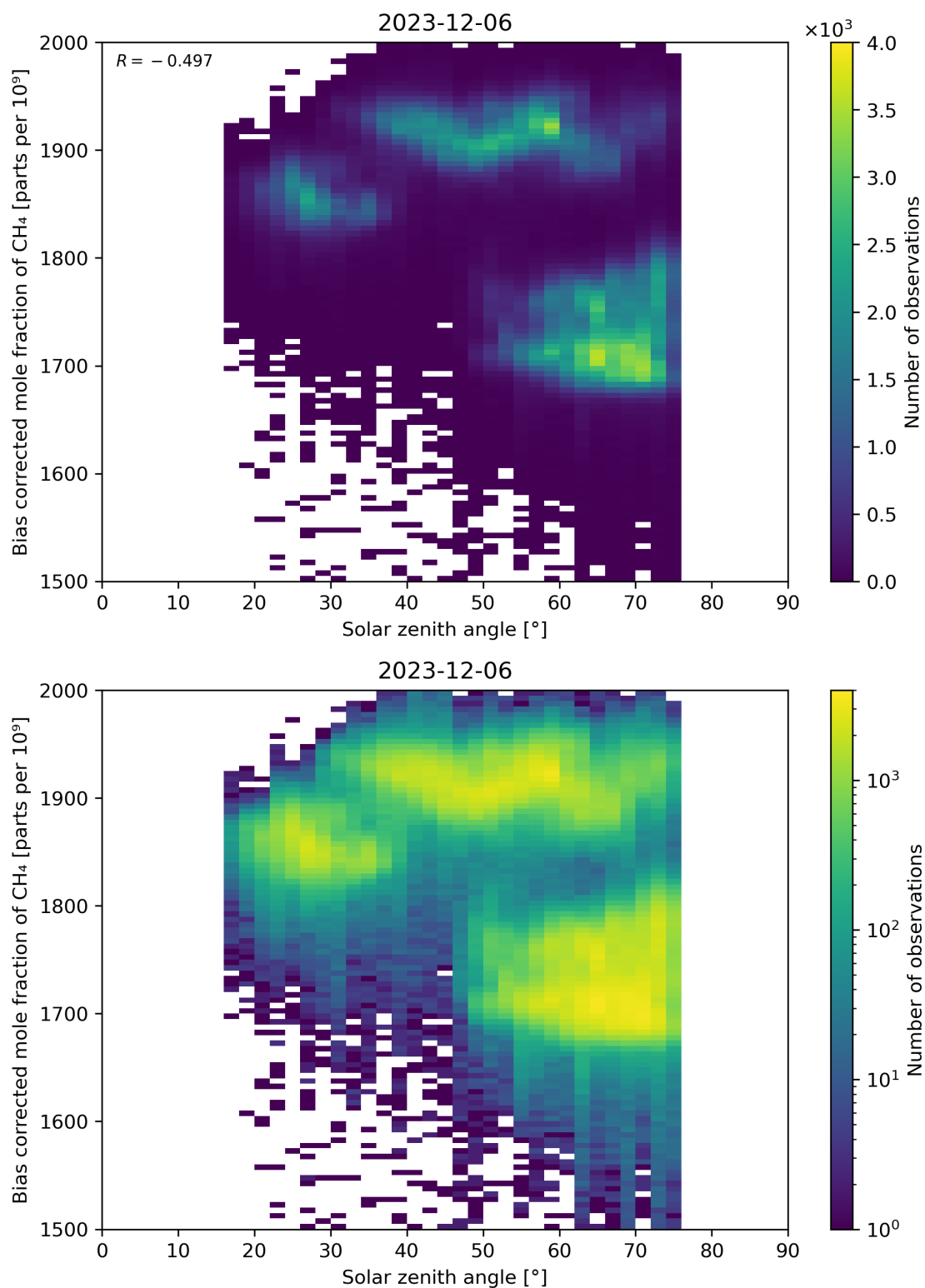
Figure 100: Scatter density plot of “Solar zenith angle” against “Bias corrected mole fraction of CH 4 ” for 2023-12-05 to 2023-12-07.
