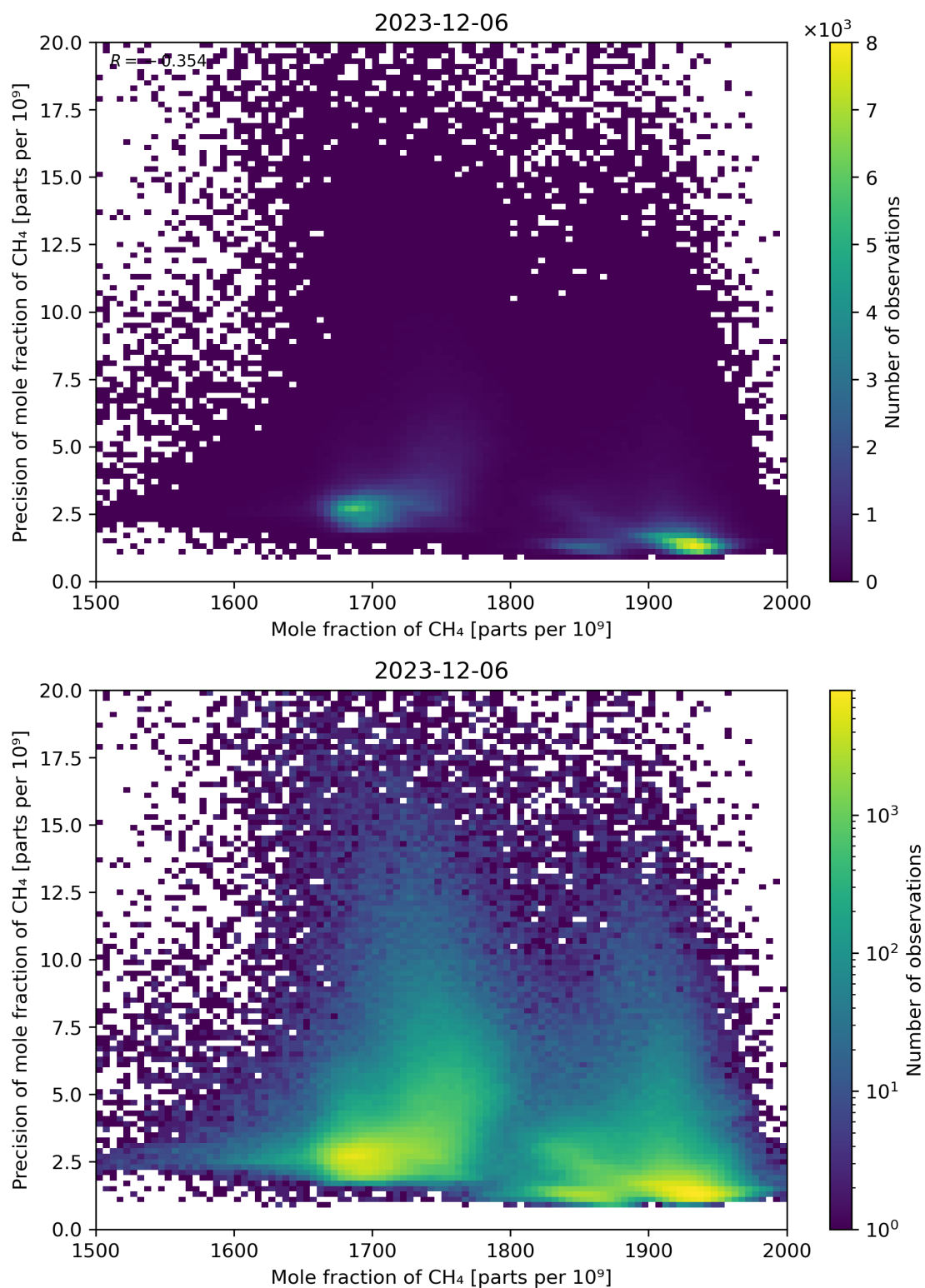
Figure 75: Scatter density plot of “Mole fraction of CH 4 ” against “Precision of mole fraction of CH 4 ” for 2023-12-05 to 2023-12-07.
