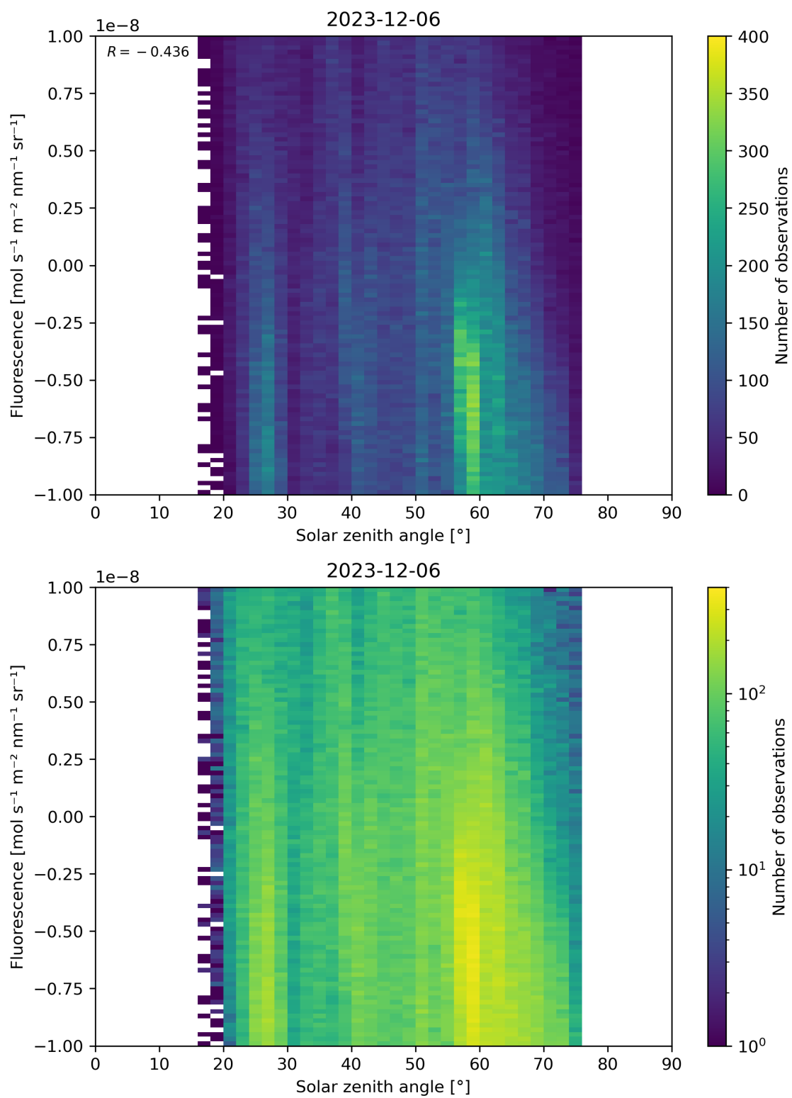
Figure 97: Scatter density plot of “Solar zenith angle” against “Fluorescence” for 2023-12-05 to 2023-12-07.
