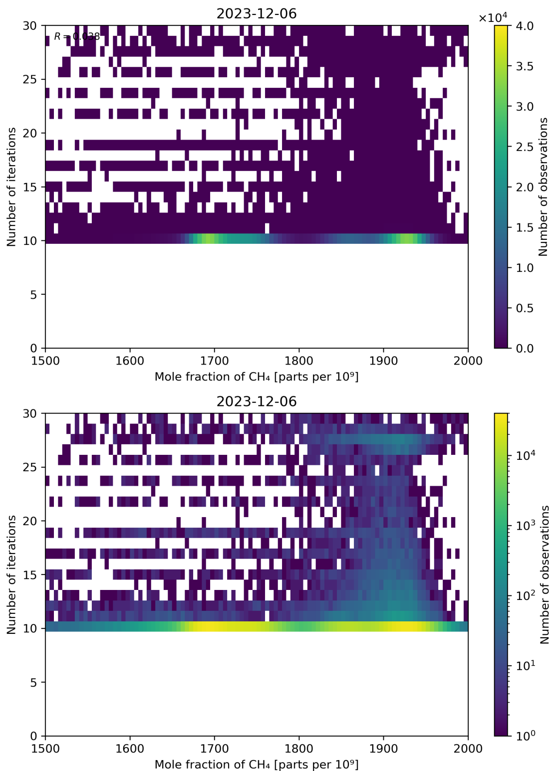
Figure 76: Scatter density plot of “Mole fraction of CH 4 ” against “Number of iterations” for 2023-12-05 to 2023-12-07.
