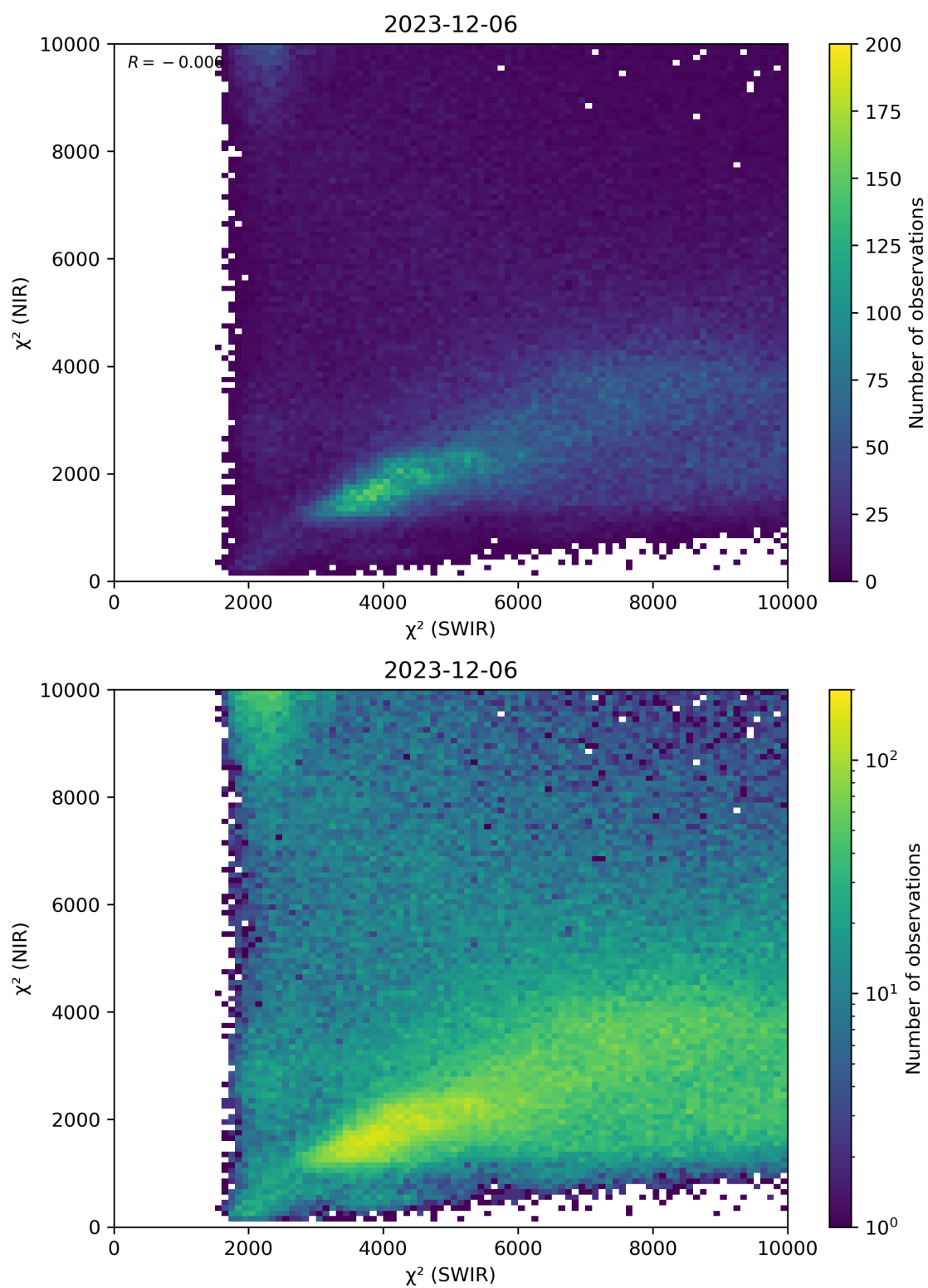
Figure 47: Scatter density plot of “ \chi^2 (SWIR)” against “ \chi^2 (NIR)” for 2023-12-05 to 2023-12-07.
