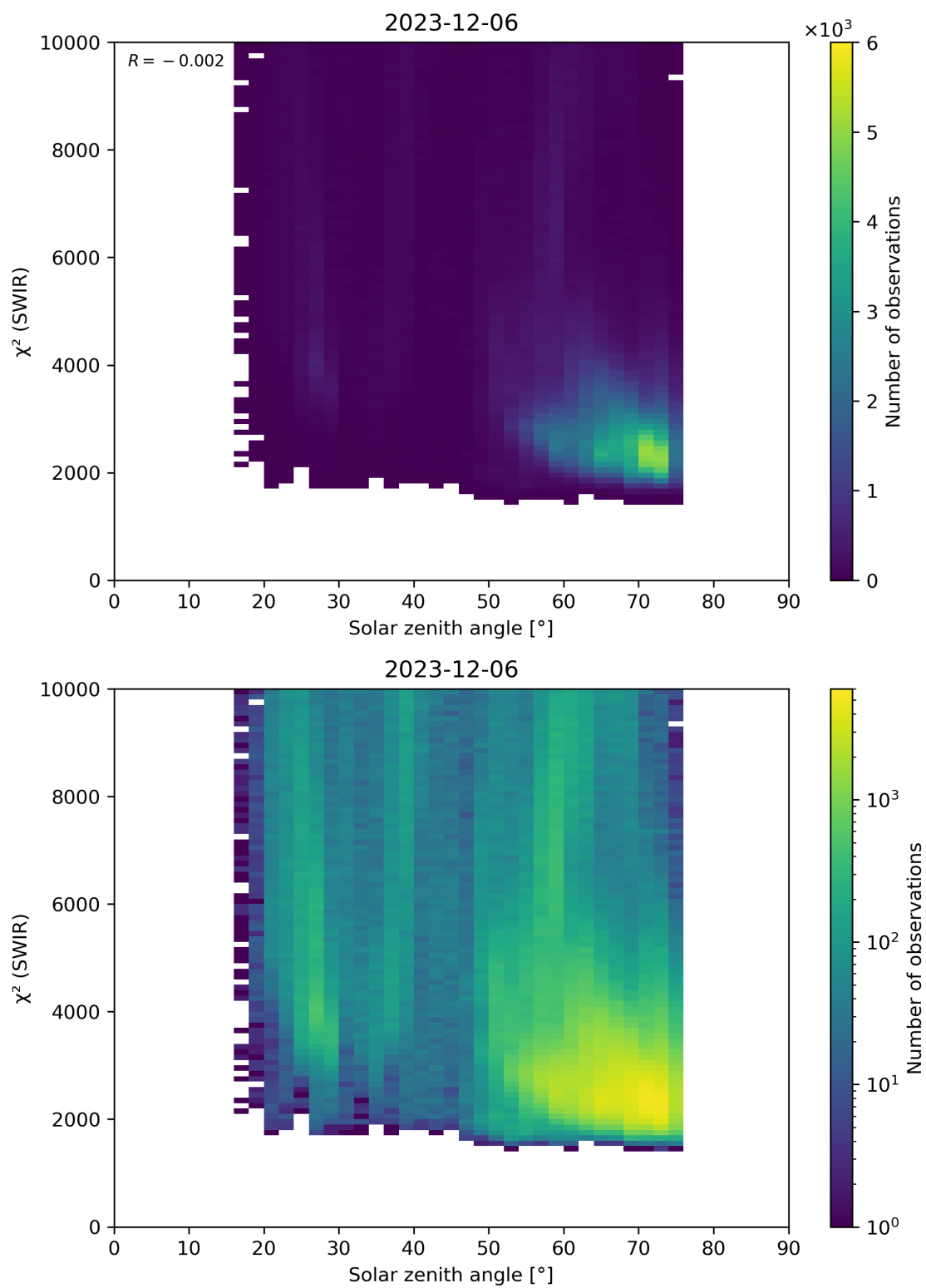
Figure 95: Scatter density plot of “Solar zenith angle” against “ \chi^2 (SWIR)” for 2023-12-05 to 2023-12-07.
