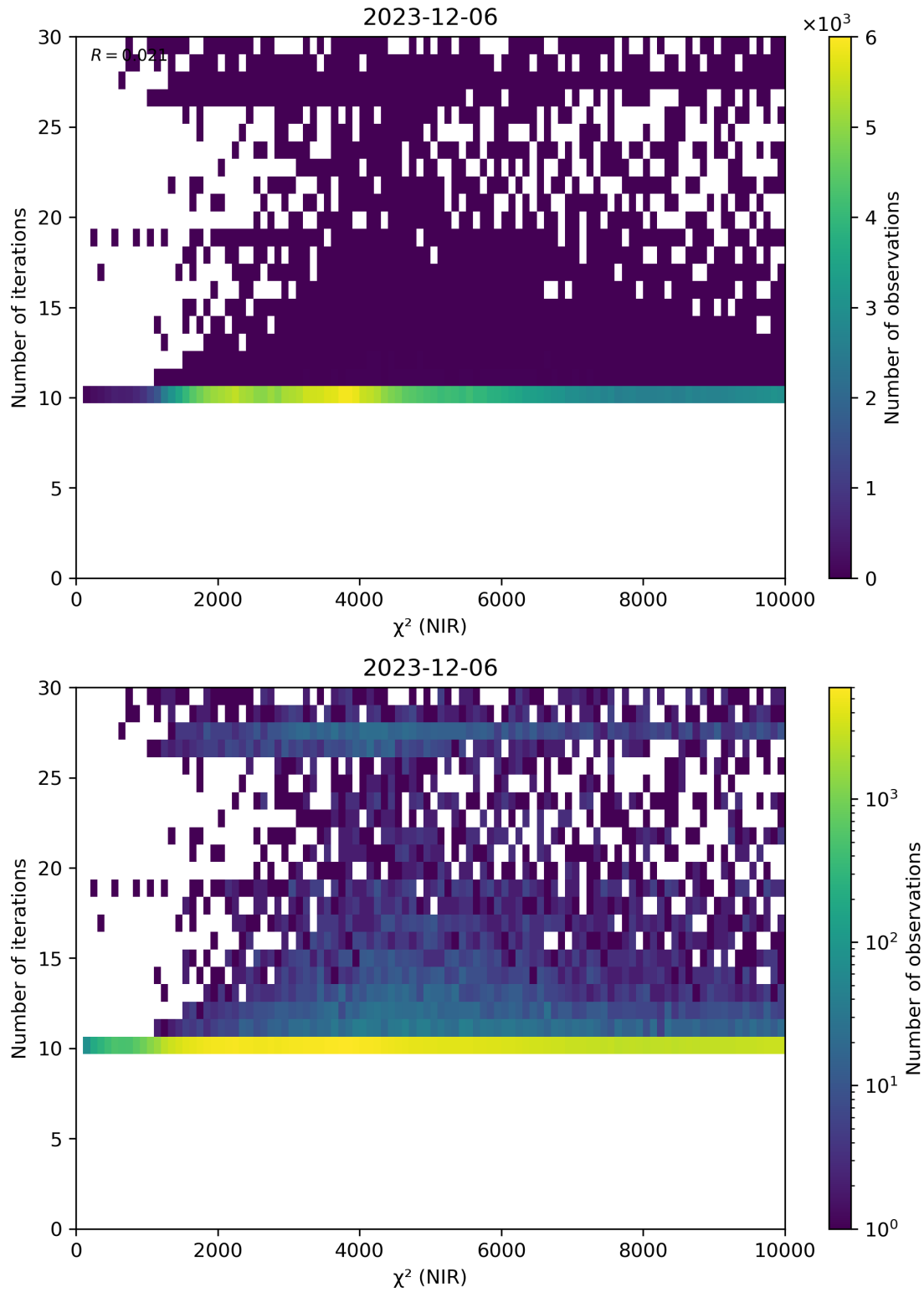
Figure 46: Scatter density plot of “ \chi^2 (NIR)” against “Number of iterations” for 2023-12-05 to 2023-12-07.
