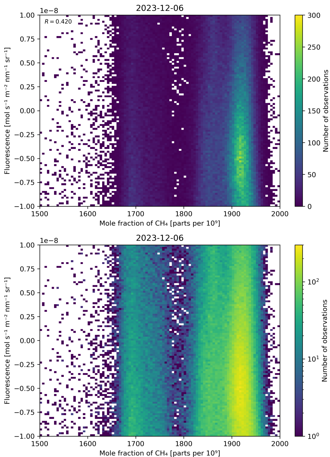
Figure 73: Scatter density plot of “Mole fraction of \text{CH}_4 ” against “Fluorescence” for 2023-12-05 to 2023-12-07.
