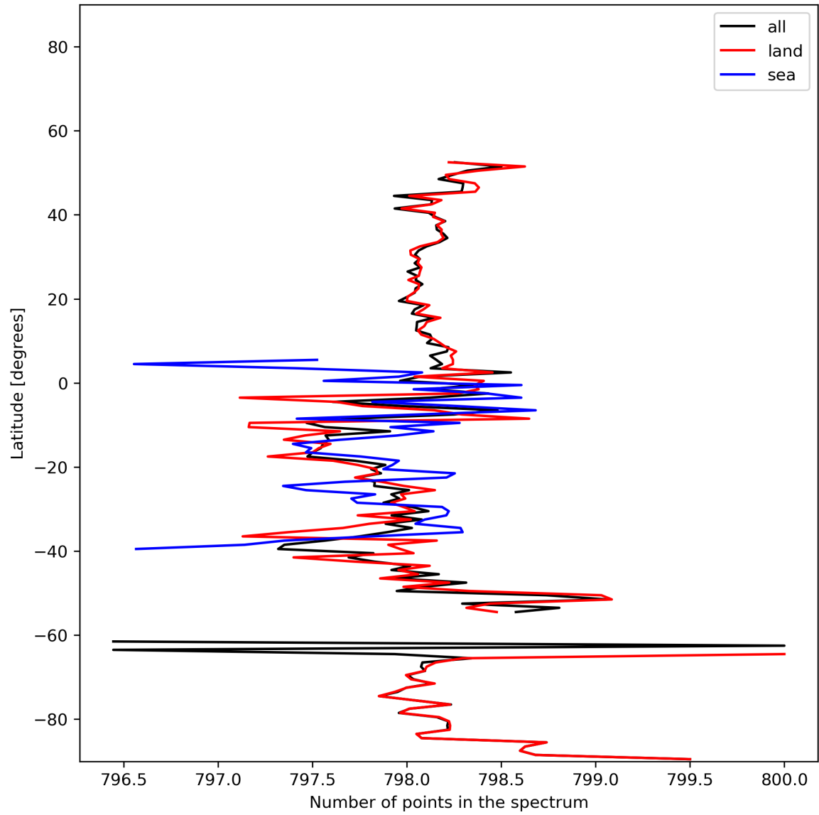
Figure 15: Zonal average of “Number of points in the spectrum” for 2023-12-05 to 2023-12-07.
