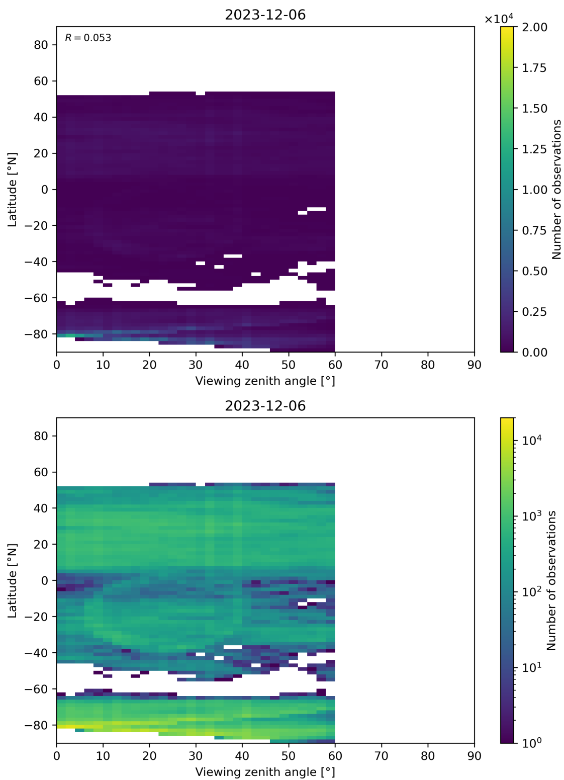
Figure 109: Scatter density plot of “Viewing zenith angle” against “Latitude” for 2023-12-05 to 2023-12-07.
