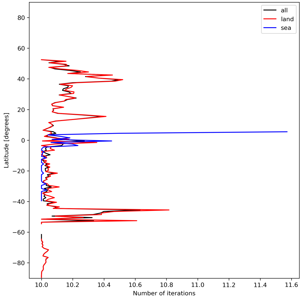
Figure 20: Zonal average of “Number of iterations” for 2023-12-05 to 2023-12-07.
