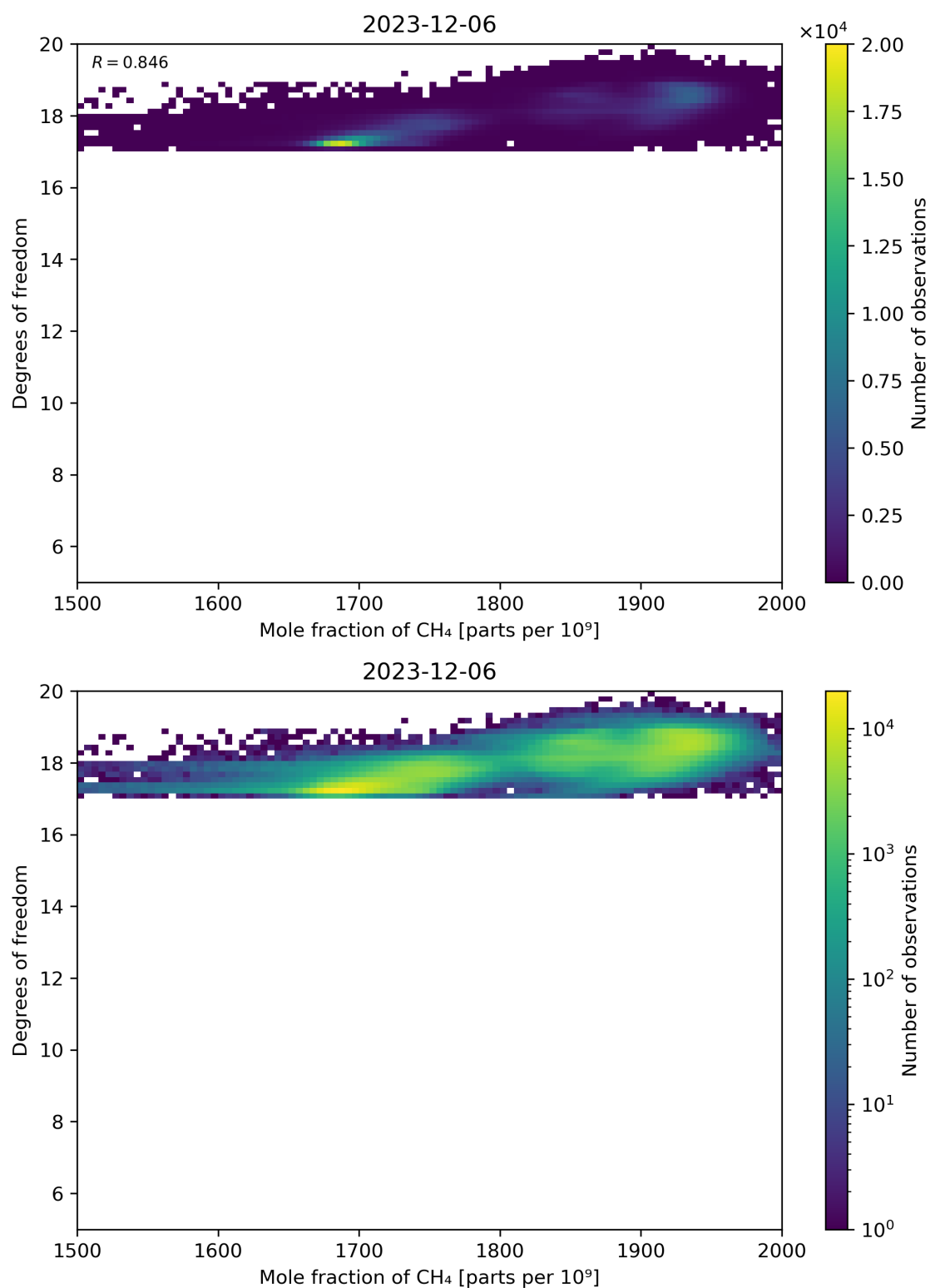
Figure 72: Scatter density plot of “Mole fraction of CH 4 ” against “Degrees of freedom” for 2023-12-05 to 2023-12-07.
