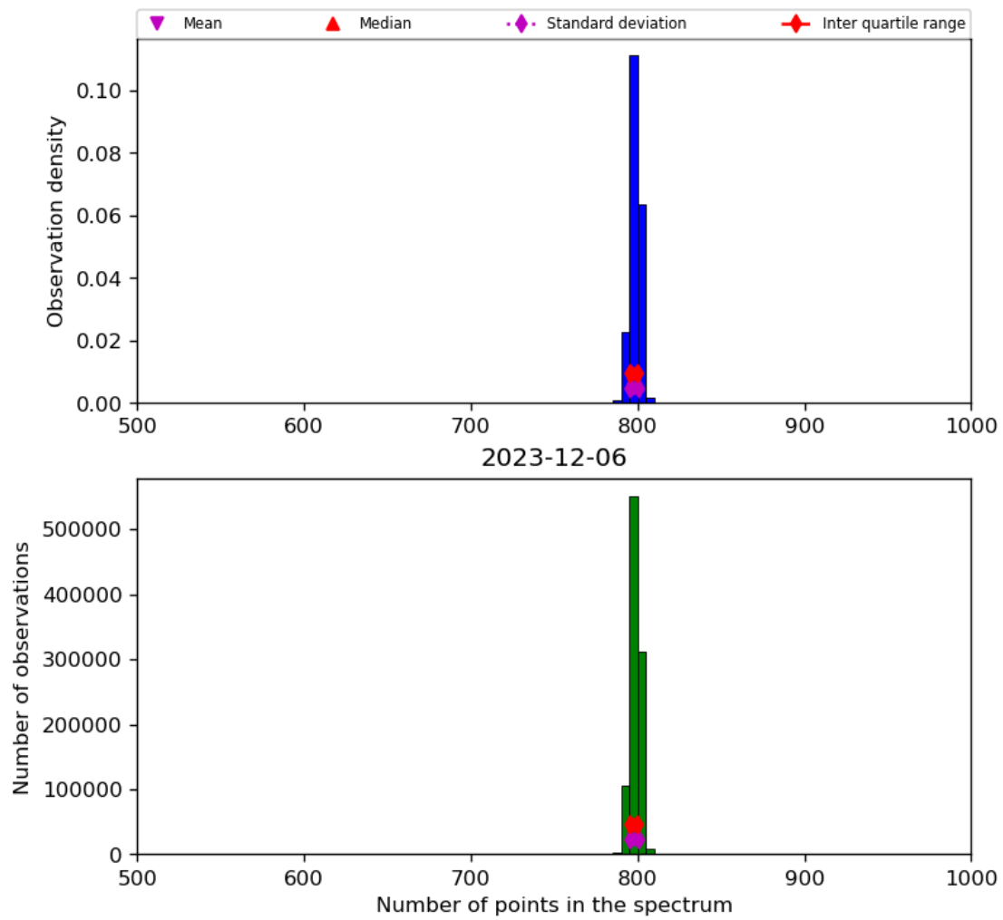
Figure 26: Histogram of “Number of points in the spectrum” for 2023-12-05 to 2023-12-07
