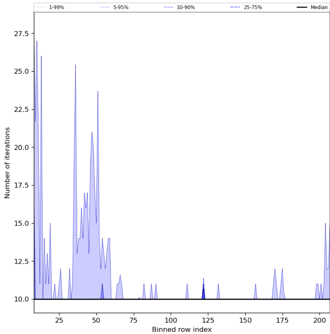
Figure 42: Along track statistics of “Number of iterations” for 2023-12-05 to 2023-12-07
