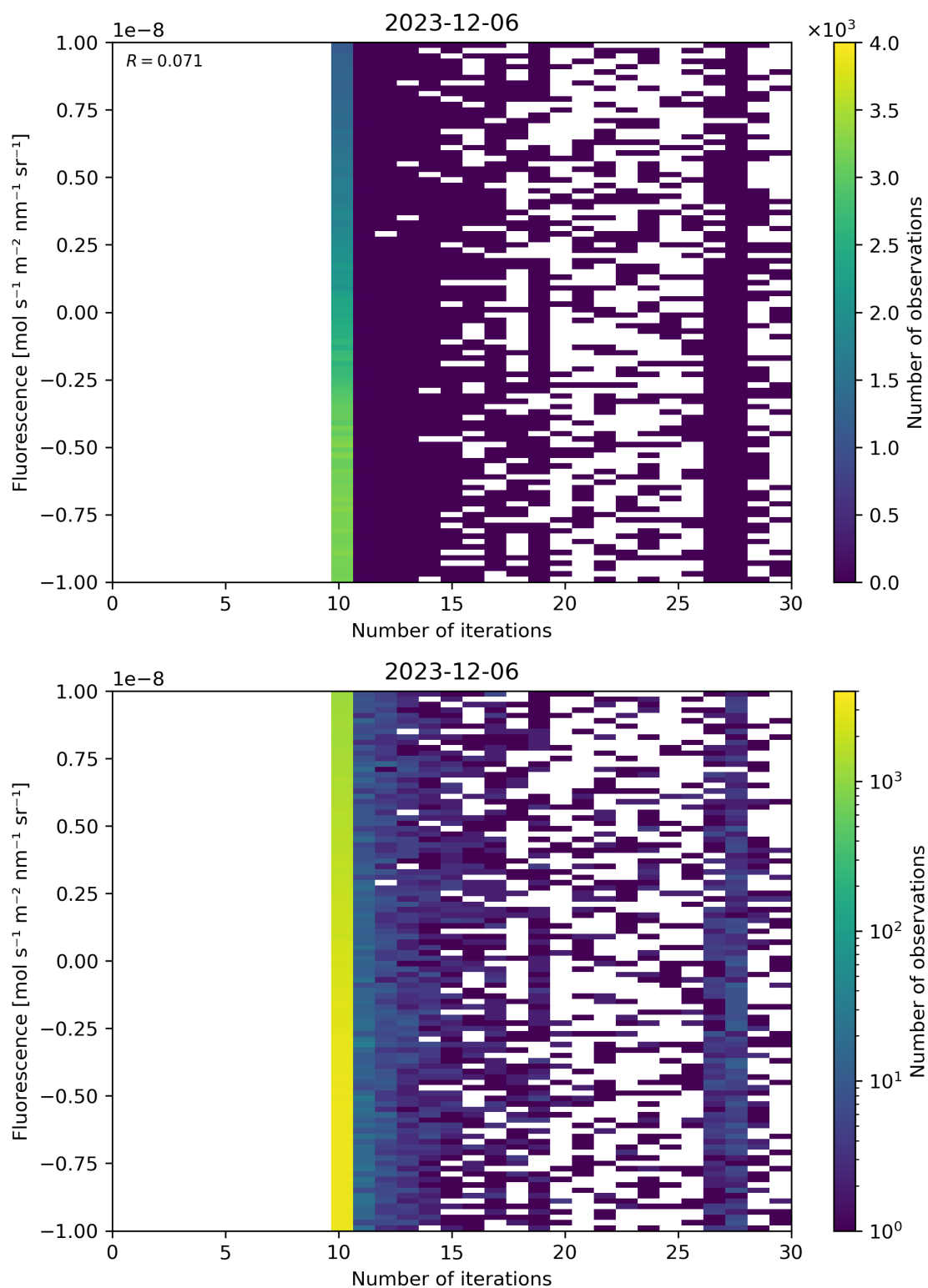
Figure 87: Scatter density plot of “Number of iterations” against “Fluorescence” for 2023-12-05 to 2023-12-07.
