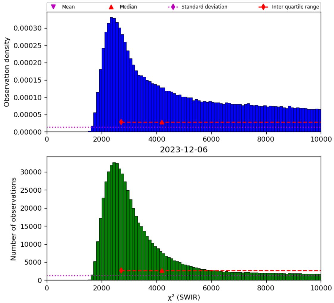
Figure 28: Histogram of “ \chi^2 (SWIR)” for 2023-12-05 to 2023-12-07
