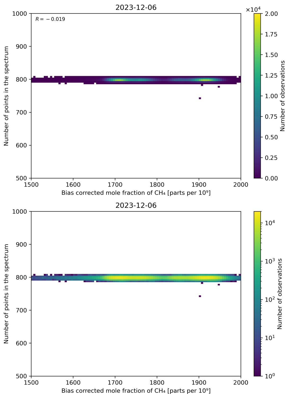
Figure 68: Scatter density plot of “Bias corrected mole fraction of CH 4 ” against “Number of points in the spectrum” for 2023-12-05 to 2023-12-07.
