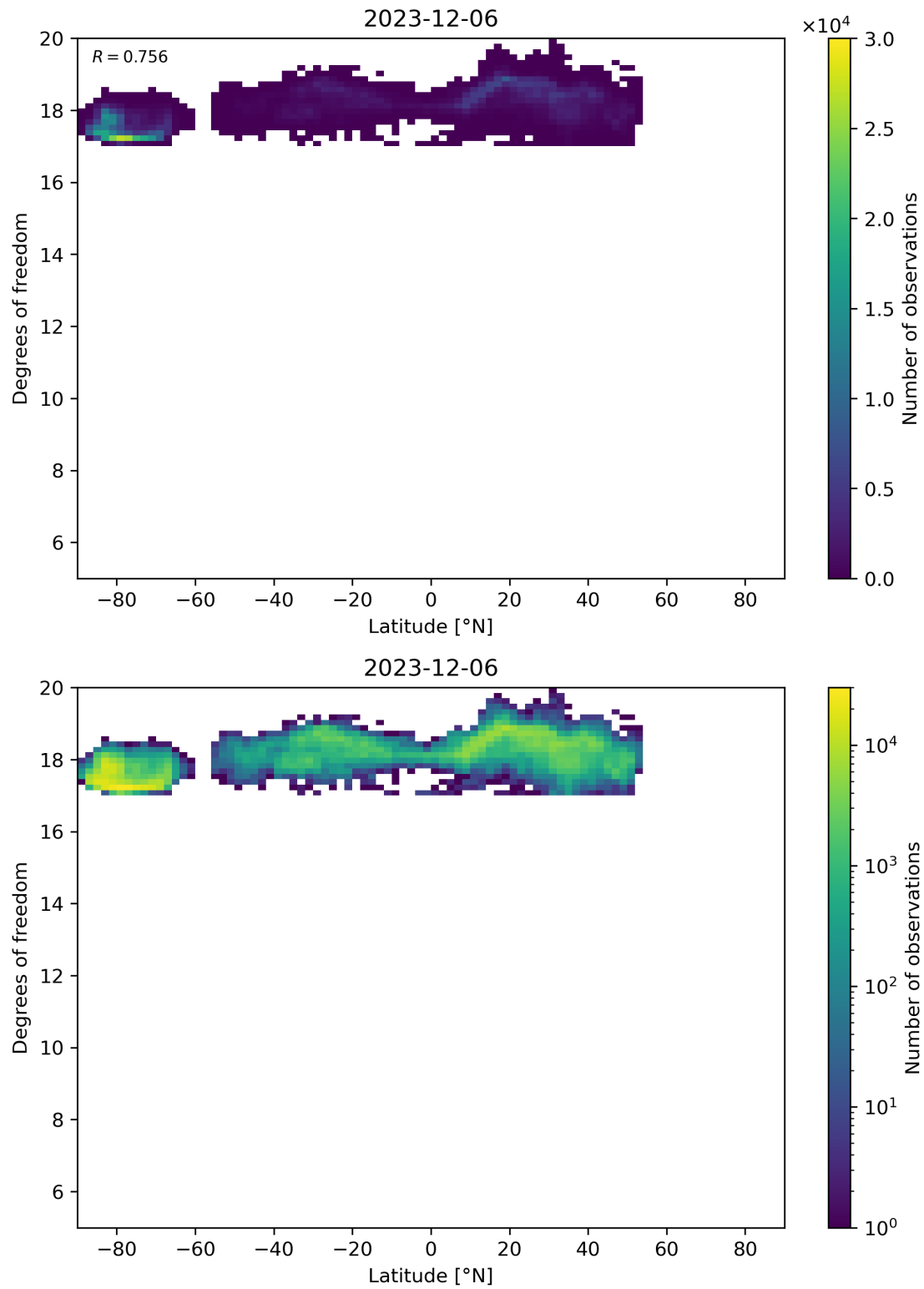
Figure 55: Scatter density plot of “Latitude” against “Degrees of freedom” for 2023-12-05 to 2023-12-07.
