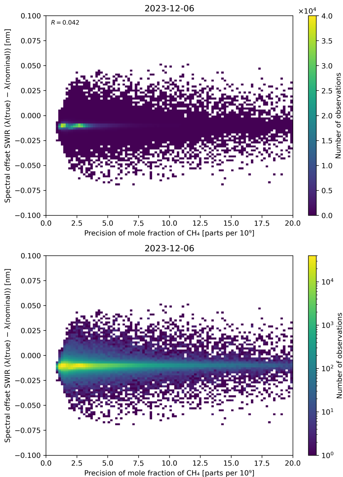
Figure 85: Scatter density plot of “Precision of mole fraction of CH 4 ” against “Spectral offset SWIR ( \lambda(\text{true}) - \lambda(\text{nominal}) )” for 2023-12-05 to 2023-12-07.
