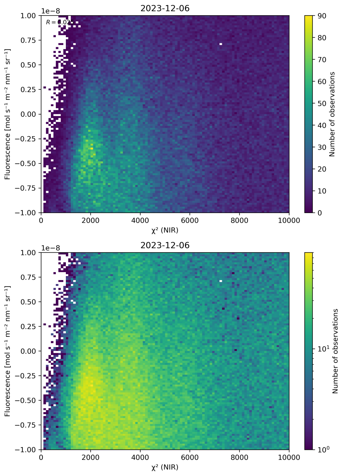
Figure 45: Scatter density plot of “ \chi^2 (NIR)” against “Fluorescence” for 2023-12-05 to 2023-12-07.
