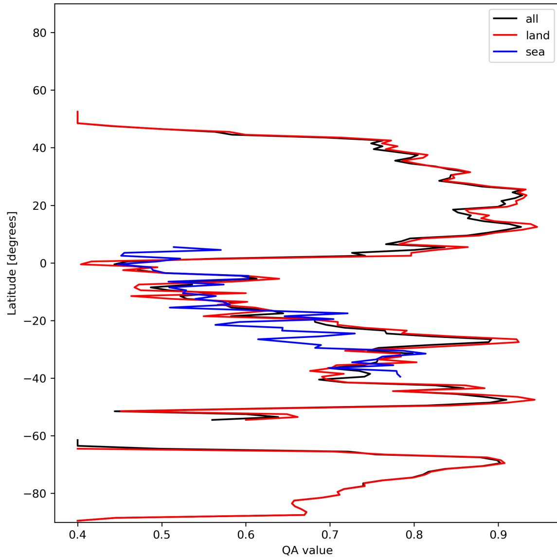
Figure 11: Zonal average of “QA value” for 2023-12-05 to 2023-12-07.
