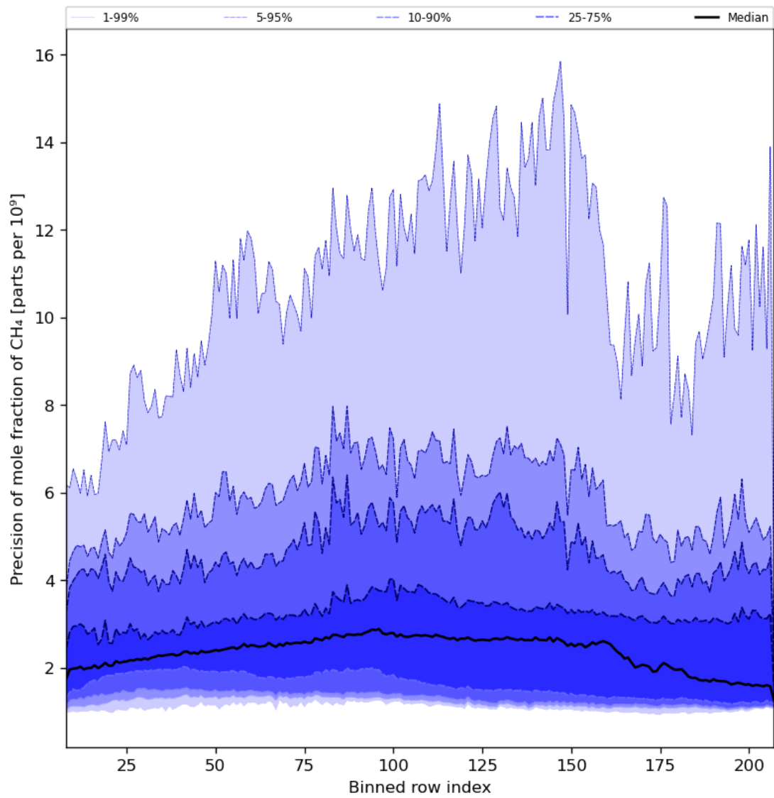
Figure 35: Along track statistics of “Precision of mole fraction of CH 4 ” for 2023-12-05 to 2023-12-07
