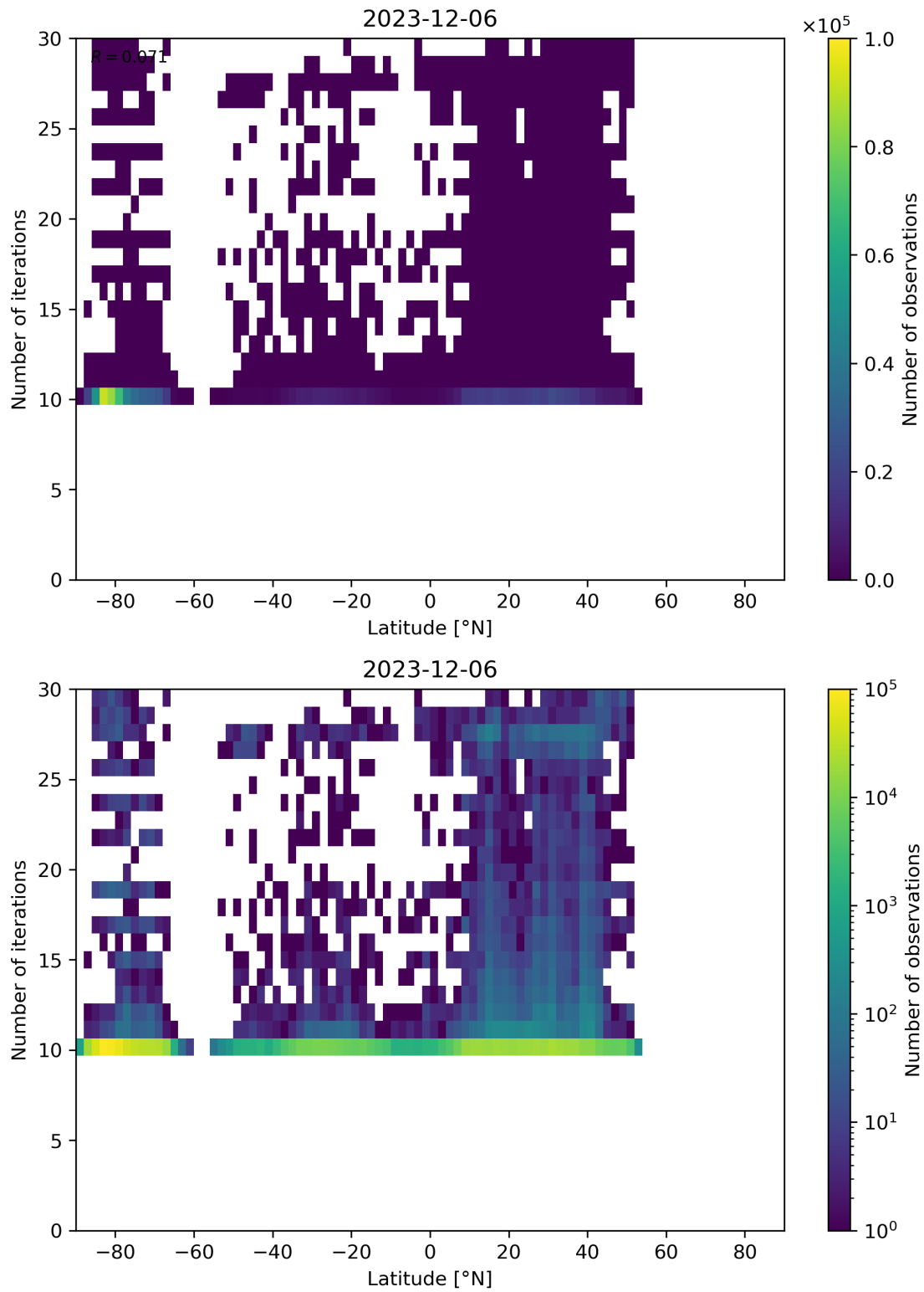
Figure 60: Scatter density plot of “Latitude” against “Number of iterations” for 2023-12-05 to 2023-12-07.
