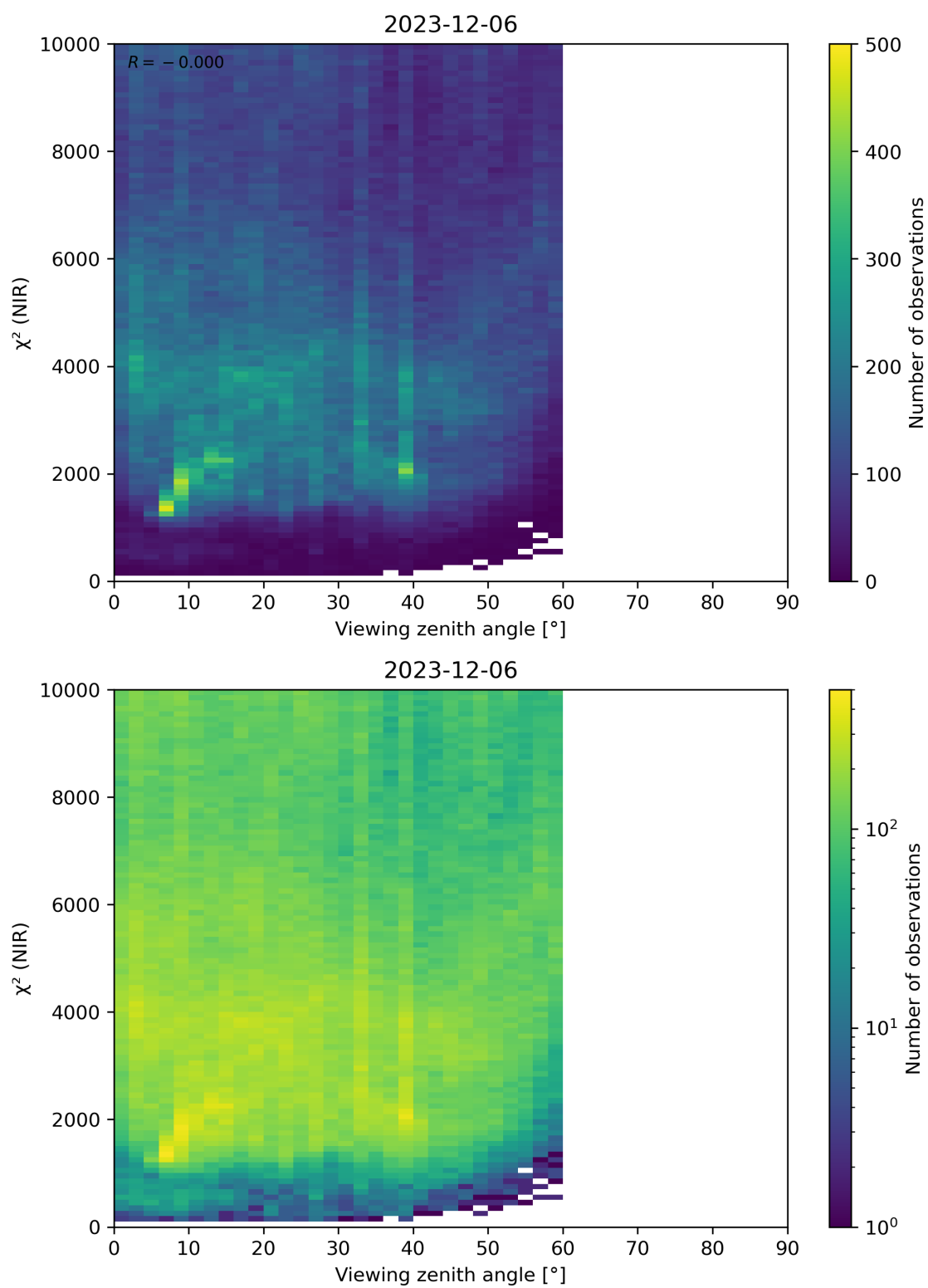
Figure 105: Scatter density plot of “Viewing zenith angle” against “ \chi^2 (NIR)” for 2023-12-05 to 2023-12-07.
