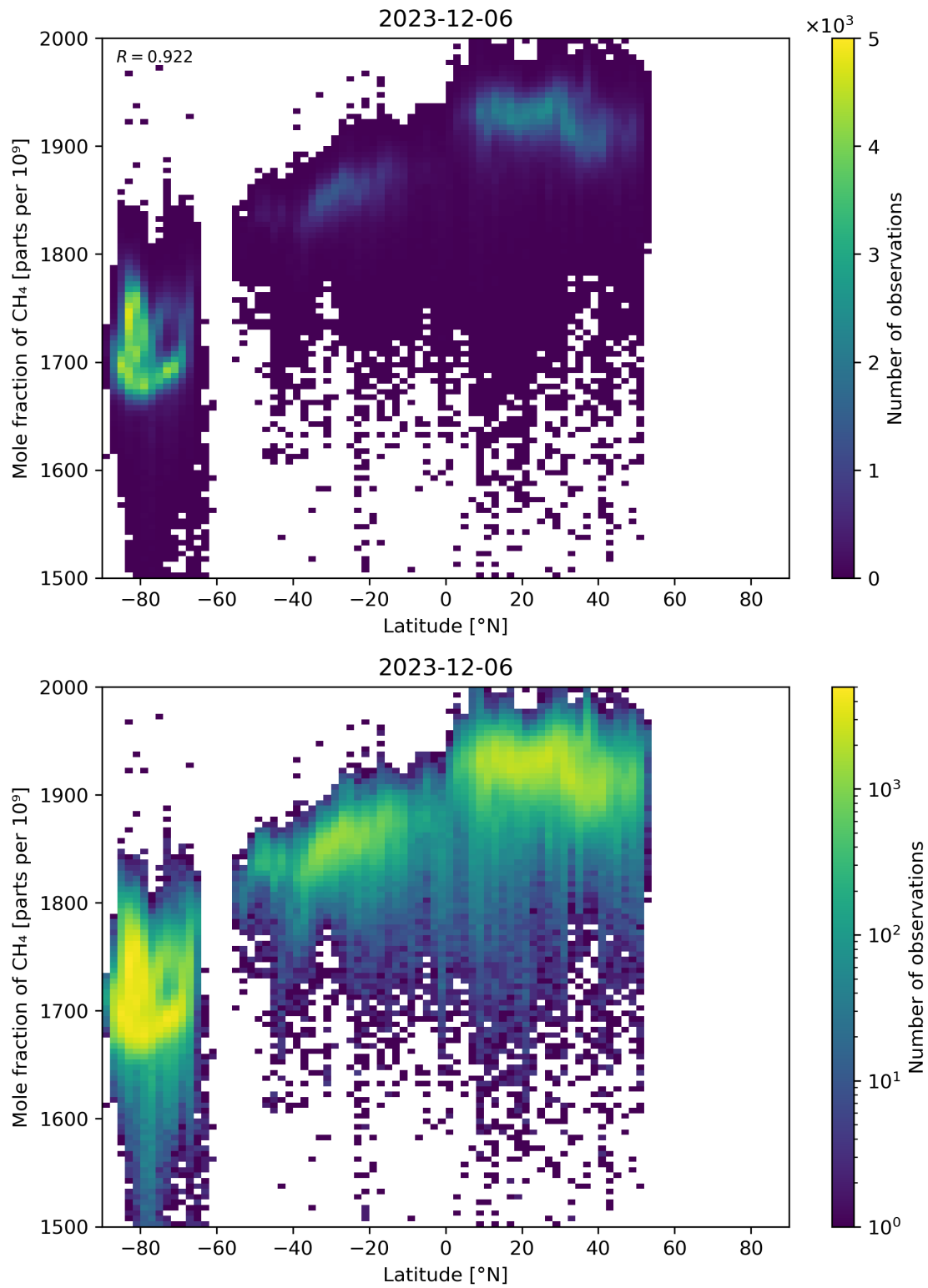
Figure 57: Scatter density plot of “Latitude” against “Mole fraction of CH 4 ” for 2023-12-05 to 2023-12-07.
