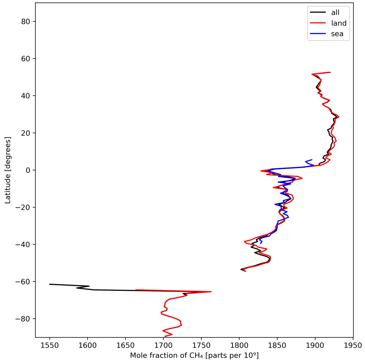
Figure 12: Zonal average of “Mole fraction of CH 4 ” for 2023-12-05 to 2023-12-07.
