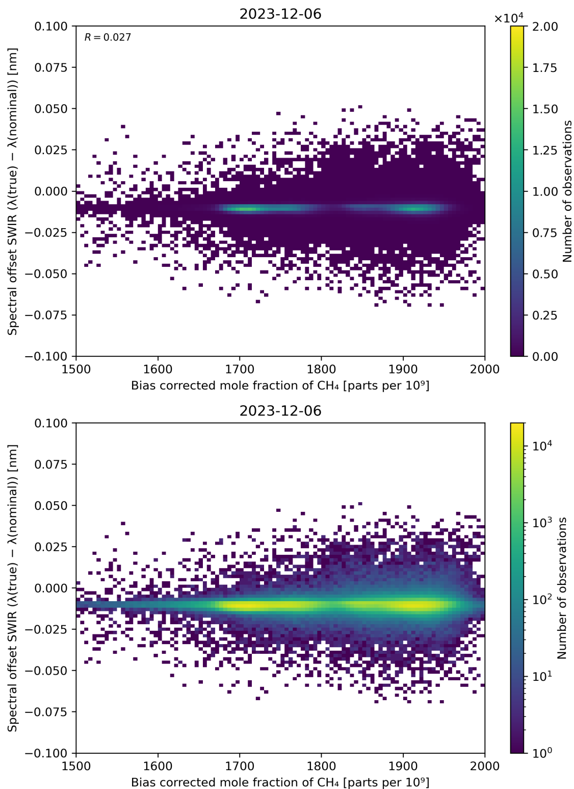
Figure 69: Scatter density plot of “Bias corrected mole fraction of \text{CH}_4 ” against “Spectral offset SWIR ( \lambda(\text{true}) - \lambda(\text{nominal}) )” for 2023-12-05 to 2023-12-07.
