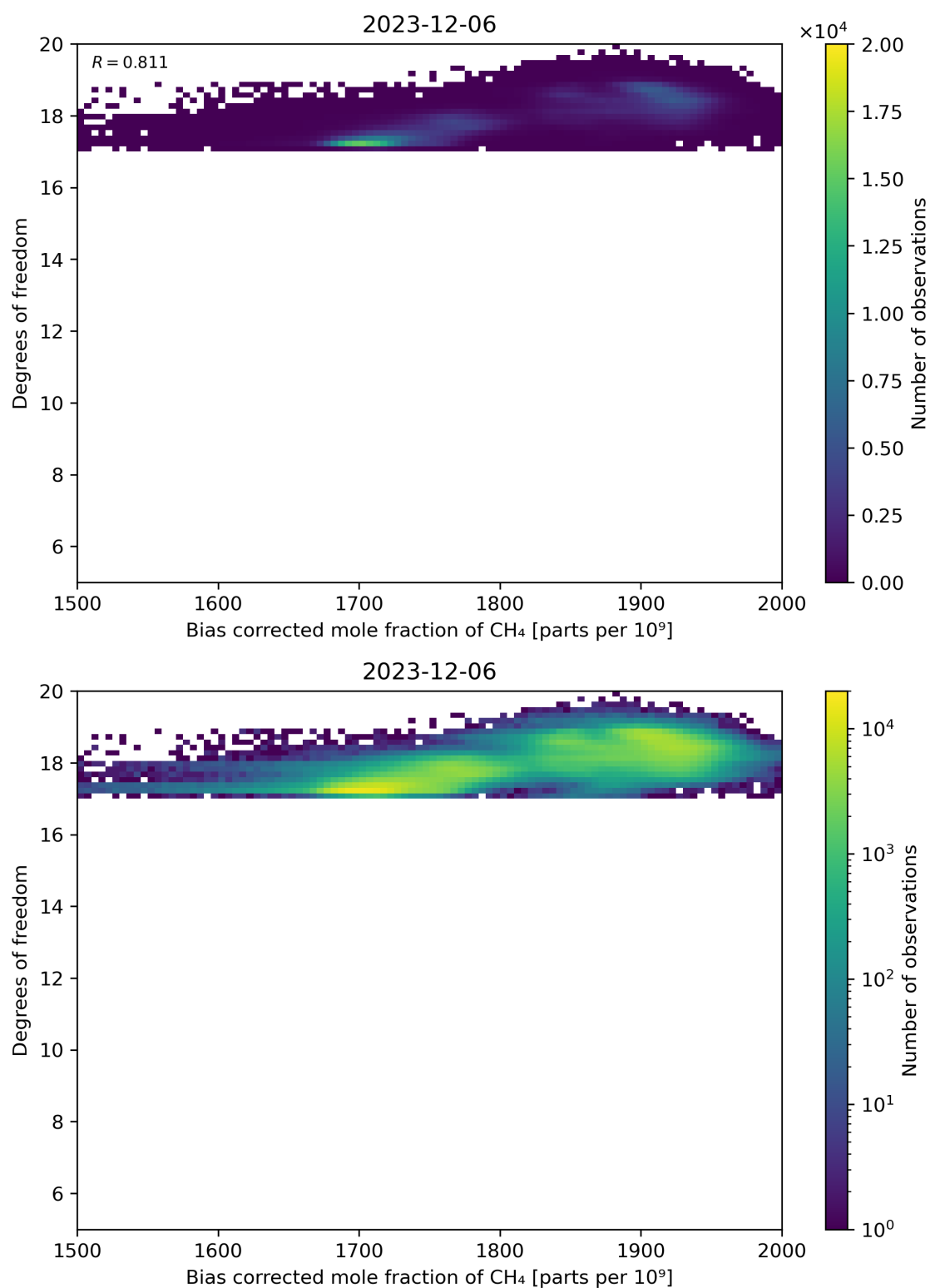
Figure 65: Scatter density plot of “Bias corrected mole fraction of CH 4 ” against “Degrees of freedom” for 2023-12-05 to 2023-12-07.
