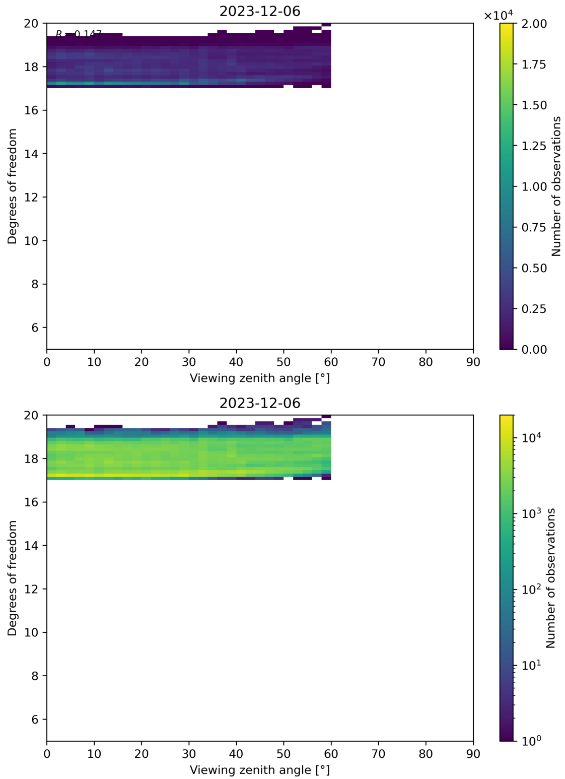
Figure 107: Scatter density plot of “Viewing zenith angle” against “Degrees of freedom” for 2023-12-05 to 2023-12-07.
