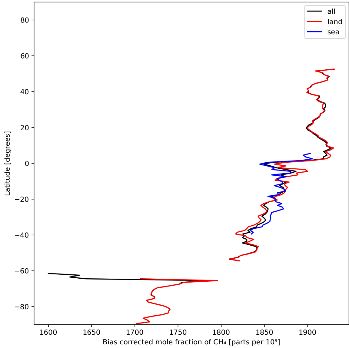
Figure 14: Zonal average of “Bias corrected mole fraction of CH 4 ” for 2023-12-05 to 2023-12-07.
