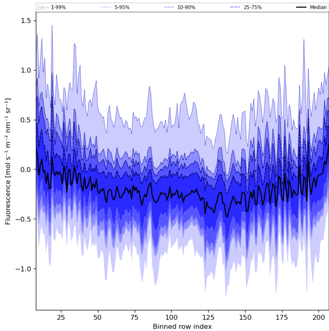
Figure 43: Along track statistics of “Fluorescence” for 2023-12-05 to 2023-12-07
