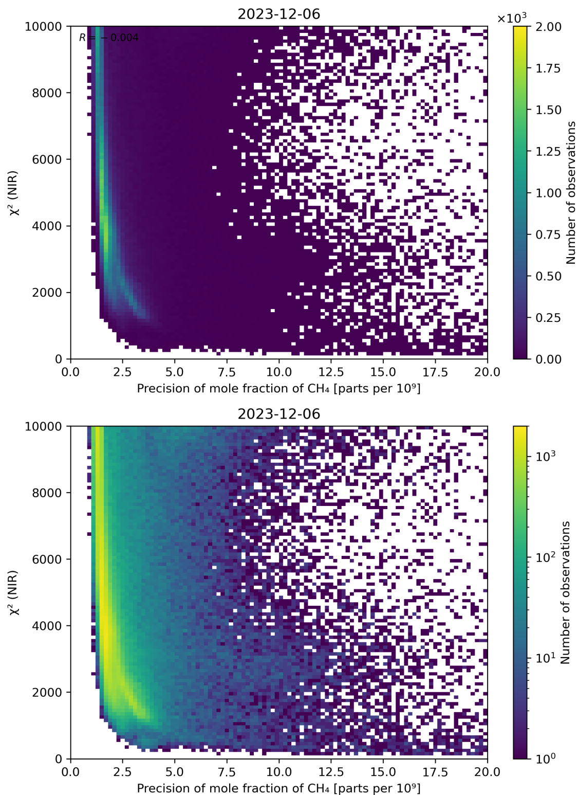
Figure 78: Scatter density plot of “Precision of mole fraction of CH 4 ” against “ \chi^2 (NIR)” for 2023-12-05 to 2023-12-07.
