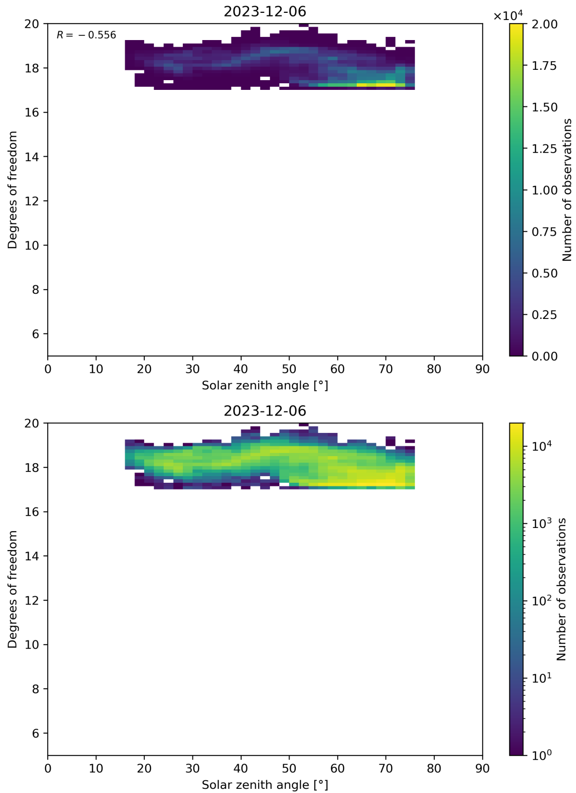
Figure 96: Scatter density plot of “Solar zenith angle” against “Degrees of freedom” for 2023-12-05 to 2023-12-07.
