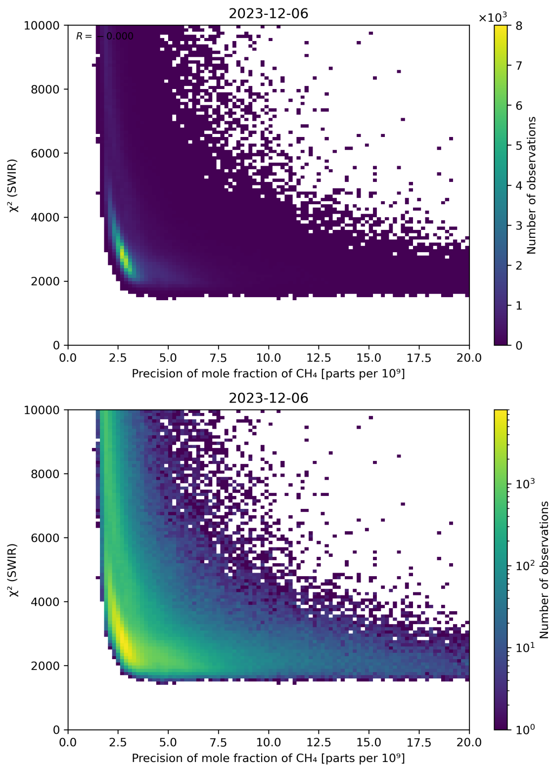
Figure 79: Scatter density plot of “Precision of mole fraction of CH 4 ” against “ \chi^2 (SWIR)” for 2023-12-05 to 2023-12-07.
