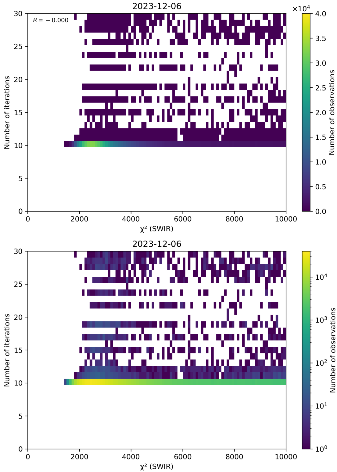
Figure 50: Scatter density plot of “ \chi^2 (SWIR)” against “Number of iterations” for 2023-12-05 to 2023-12-07.
