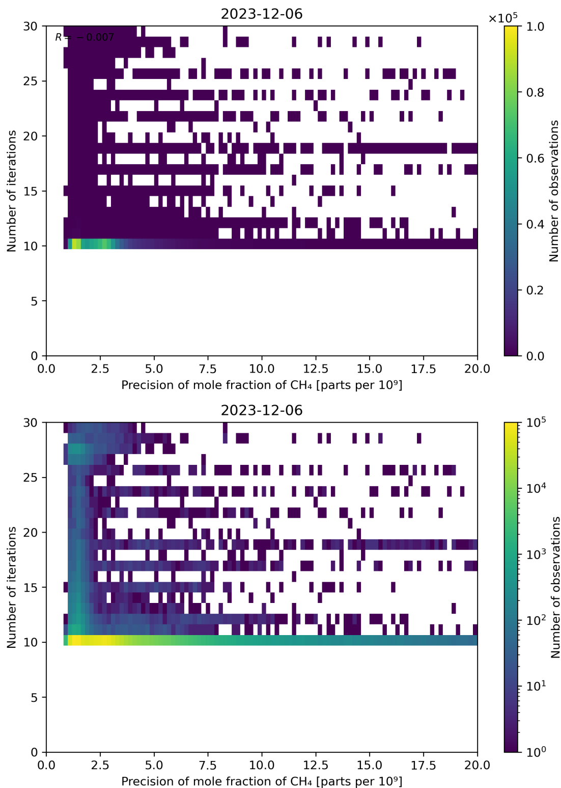
Figure 83: Scatter density plot of “Precision of mole fraction of CH 4 ” against “Number of iterations” for 2023-12-05 to 2023-12-07.
