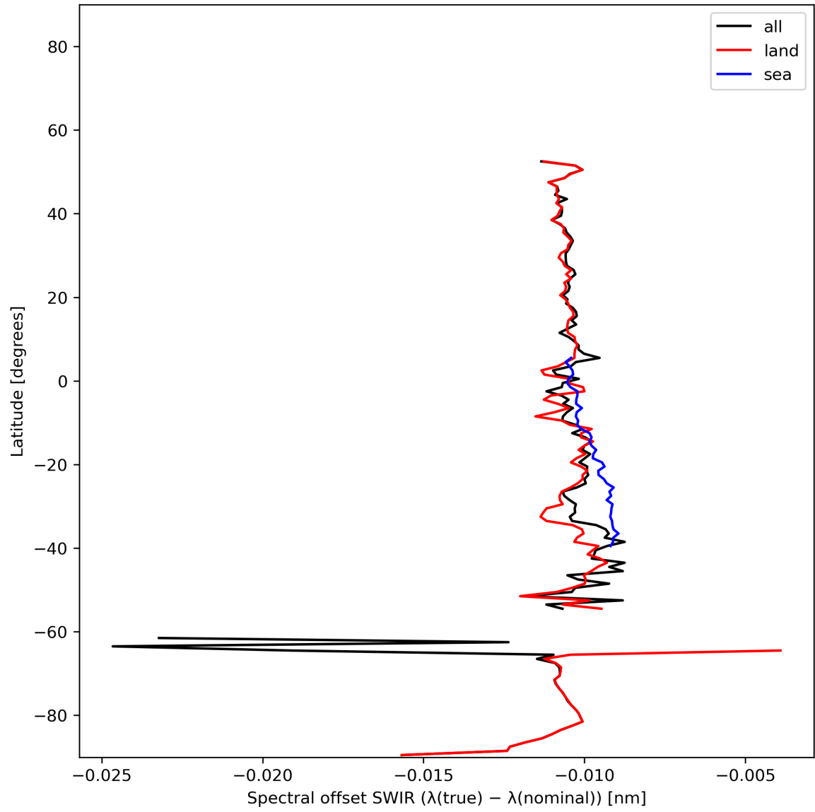
Figure 16: Zonal average of “Spectral offset SWIR ( \lambda(\text{true}) - \lambda(\text{nominal}) )” for 2023-12-05 to 2023-12-07.
