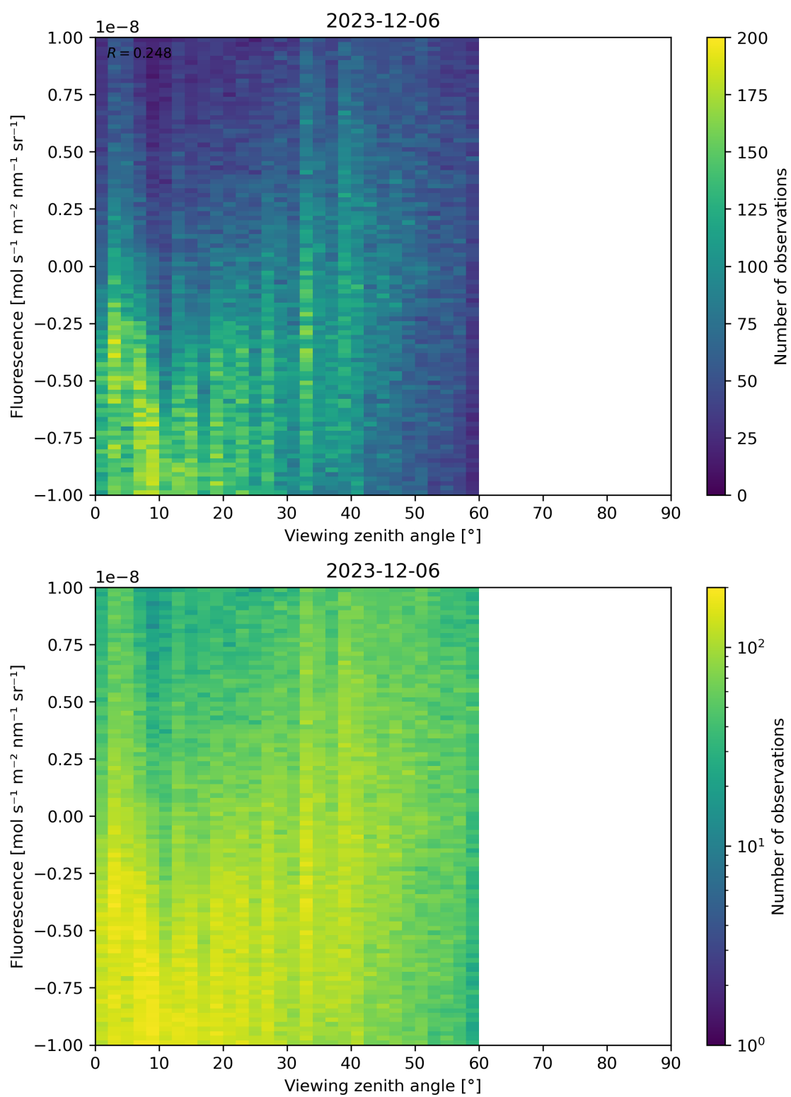
Figure 108: Scatter density plot of “Viewing zenith angle” against “Fluorescence” for 2023-12-05 to 2023-12-07.
