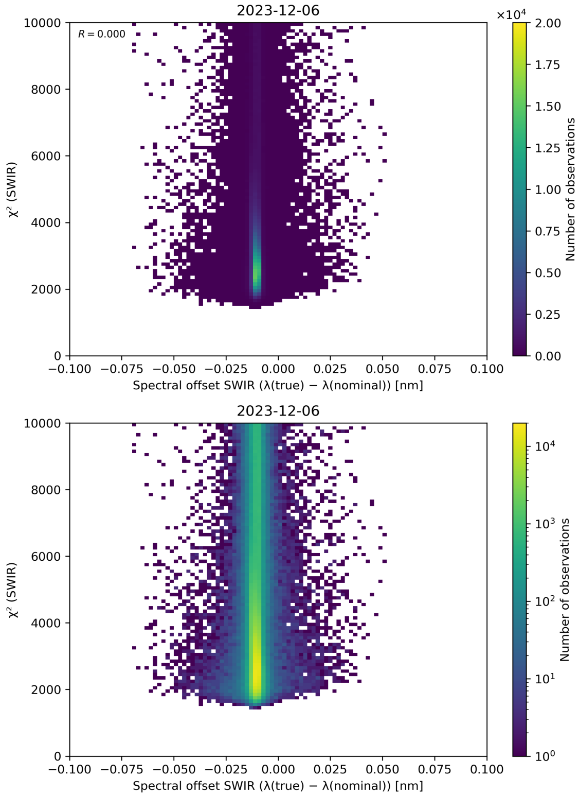
Figure 118: Scatter density plot of “Spectral offset SWIR ( \lambda(\text{true}) - \lambda(\text{nominal}) )” against “ \chi^2 (SWIR)” for 2023-12-05 to 2023-12-07.
