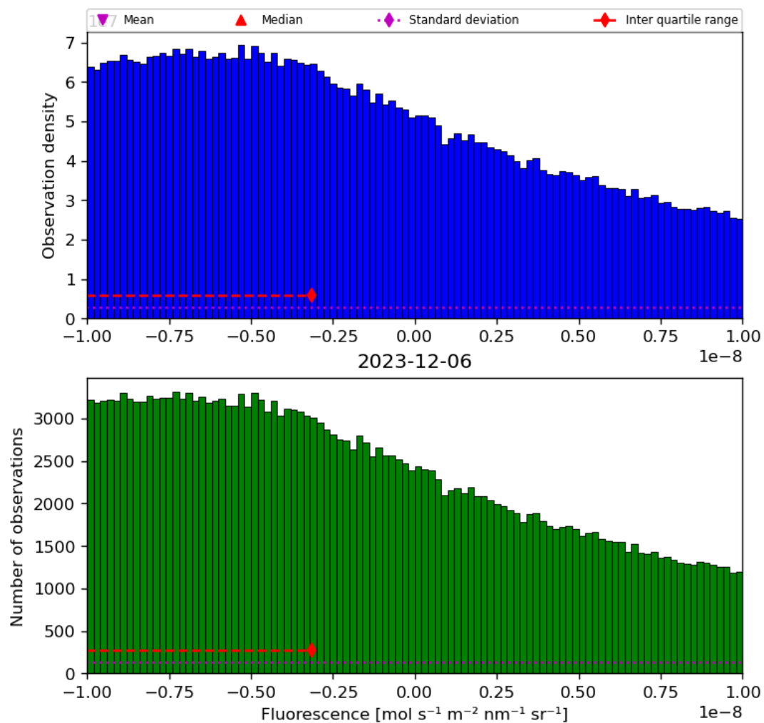
Figure 32: Histogram of “Fluorescence” for 2023-12-05 to 2023-12-07
