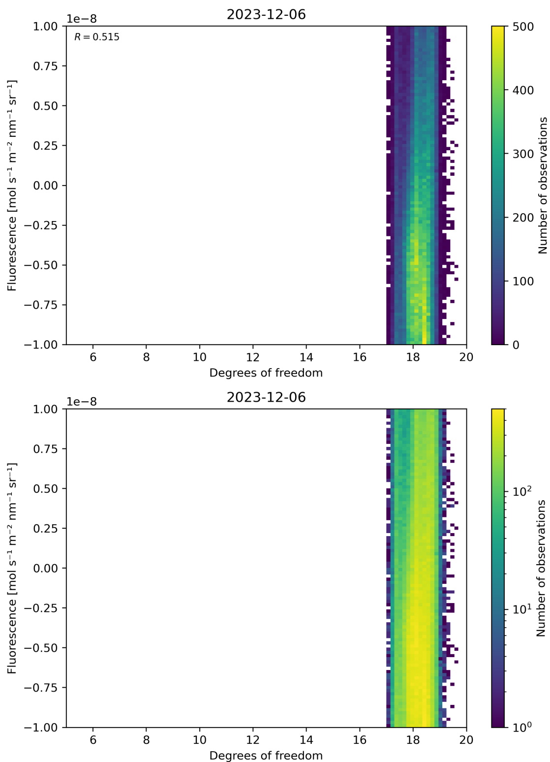
Figure 51: Scatter density plot of “Degrees of freedom” against “Fluorescence” for 2023-12-05 to 2023-12-07.
