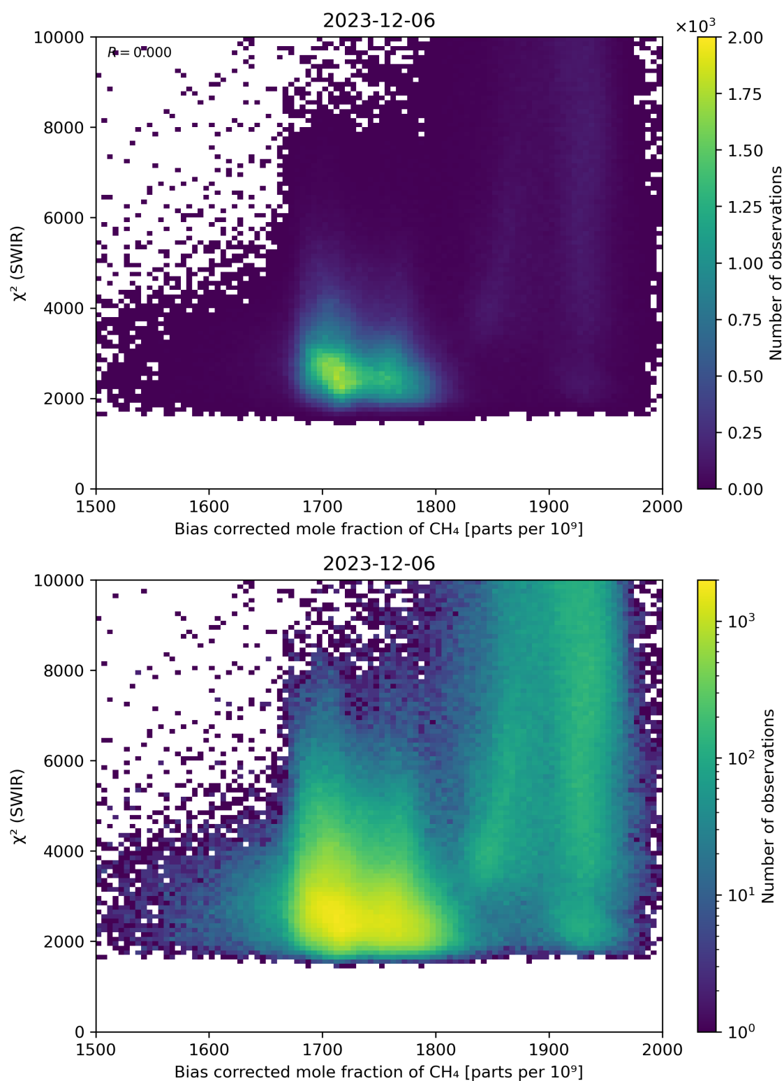
Figure 64: Scatter density plot of “Bias corrected mole fraction of CH 4 ” against “ \chi^2 (SWIR)” for 2023-12-05 to 2023-12-07.
