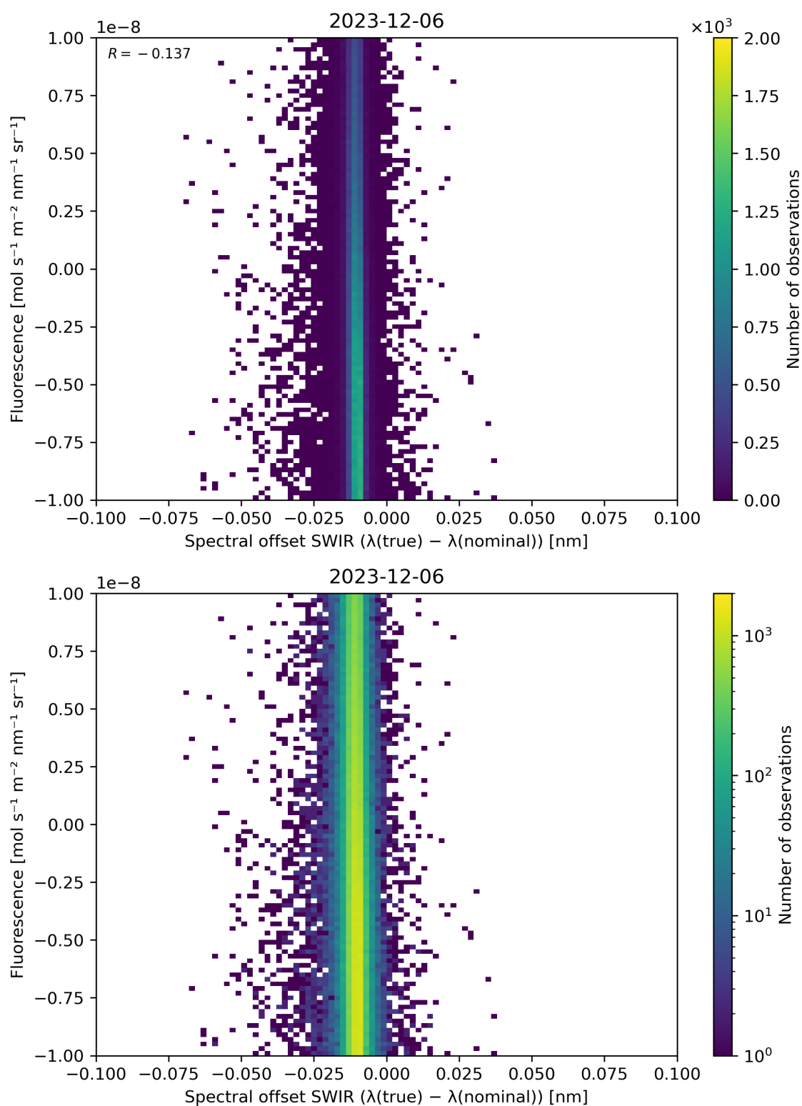
Figure 120: Scatter density plot of “Spectral offset SWIR ( \lambda(\text{true}) - \lambda(\text{nominal}) )” against “Fluorescence” for 2023-12-05 to 2023-12-07.
