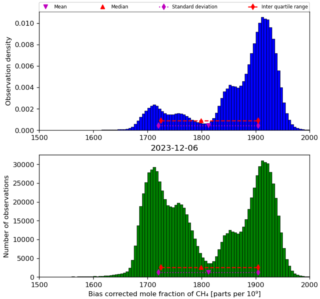
Figure 25: Histogram of “Bias corrected mole fraction of CH 4 ” for 2023-12-05 to 2023-12-07
