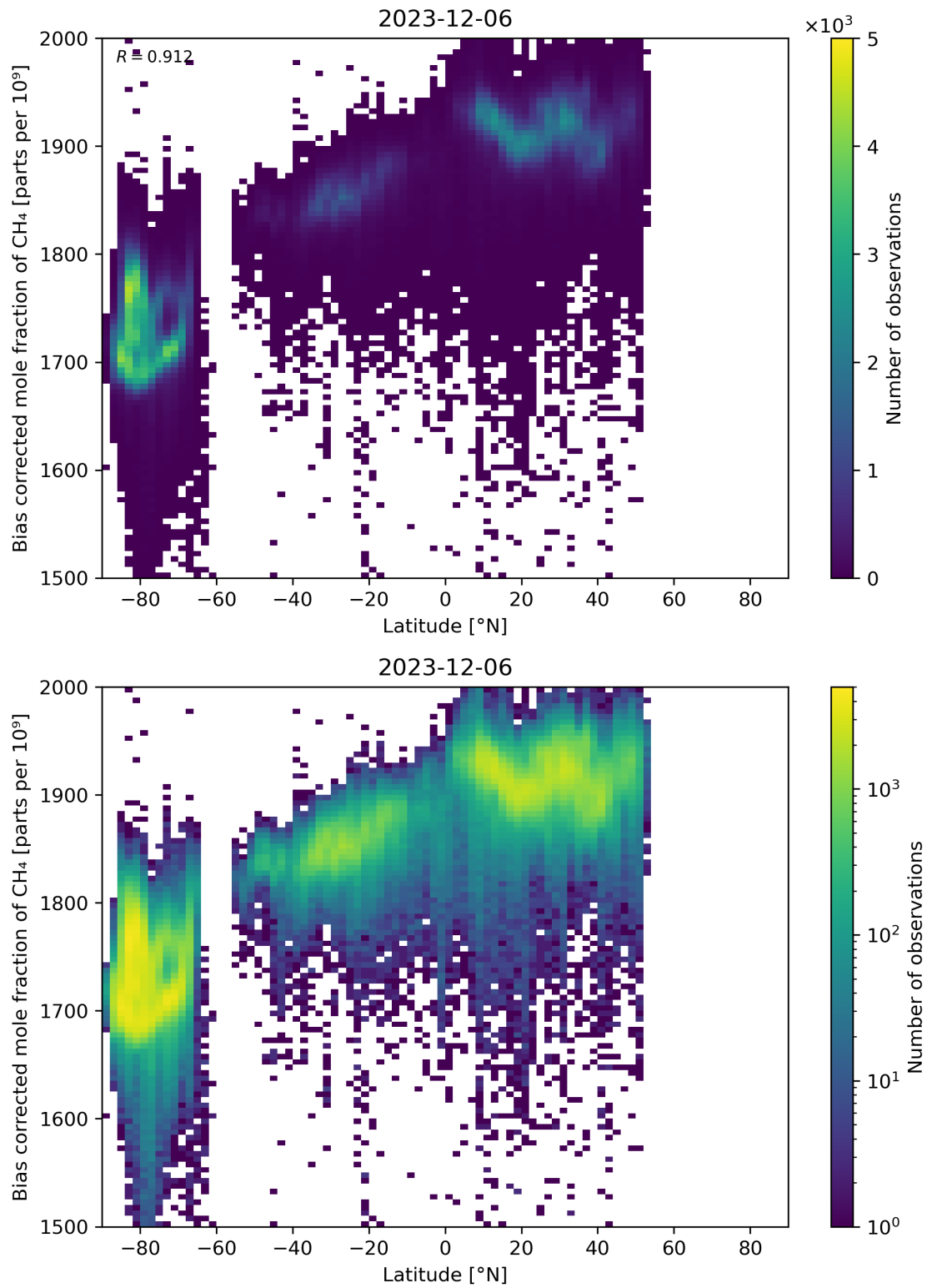
Figure 58: Scatter density plot of “Latitude” against “Bias corrected mole fraction of CH 4 ” for 2023-12-05 to 2023-12-07.
