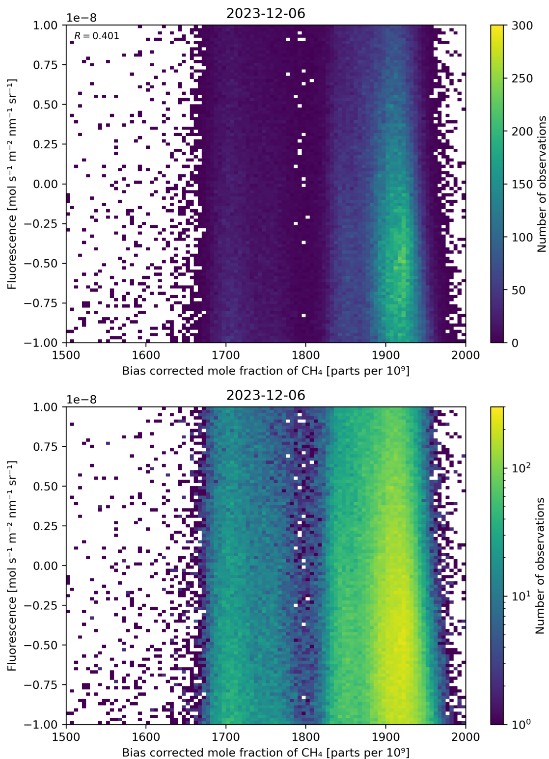
Figure 66: Scatter density plot of “Bias corrected mole fraction of \text{CH}_4 ” against “Fluorescence” for 2023-12-05 to 2023-12-07.
