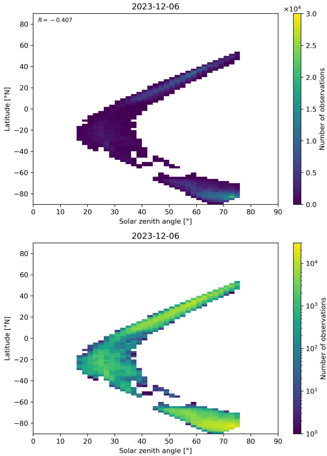
Figure 98: Scatter density plot of “Solar zenith angle” against “Latitude” for 2023-12-05 to 2023-12-07.
