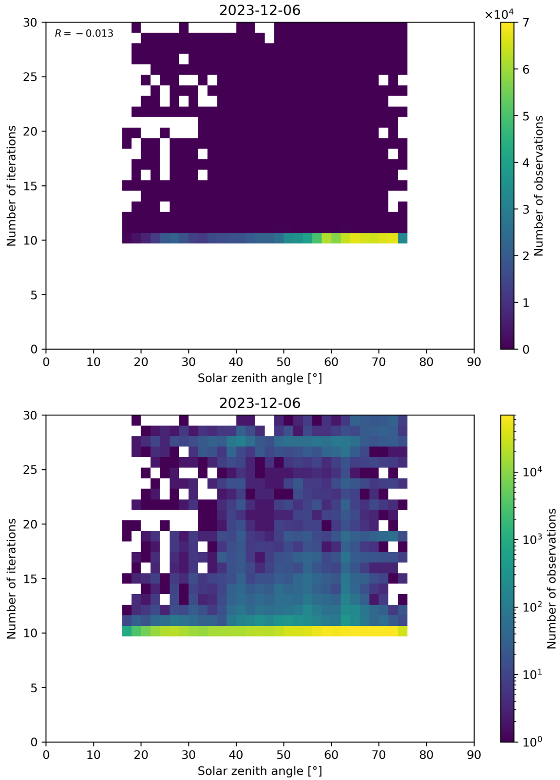
Figure 102: Scatter density plot of “Solar zenith angle” against “Number of iterations” for 2023-12-05 to 2023-12-07.
