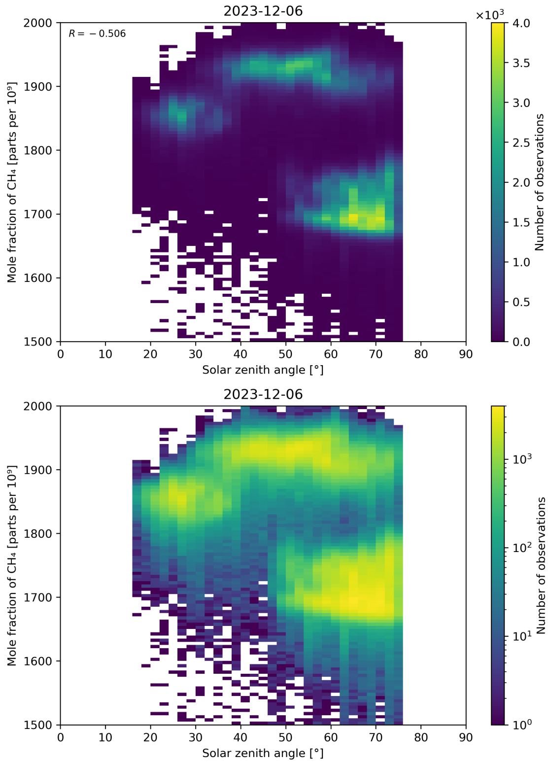
Figure 99: Scatter density plot of “Solar zenith angle” against “Mole fraction of CH 4 ” for 2023-12-05 to 2023-12-07.
