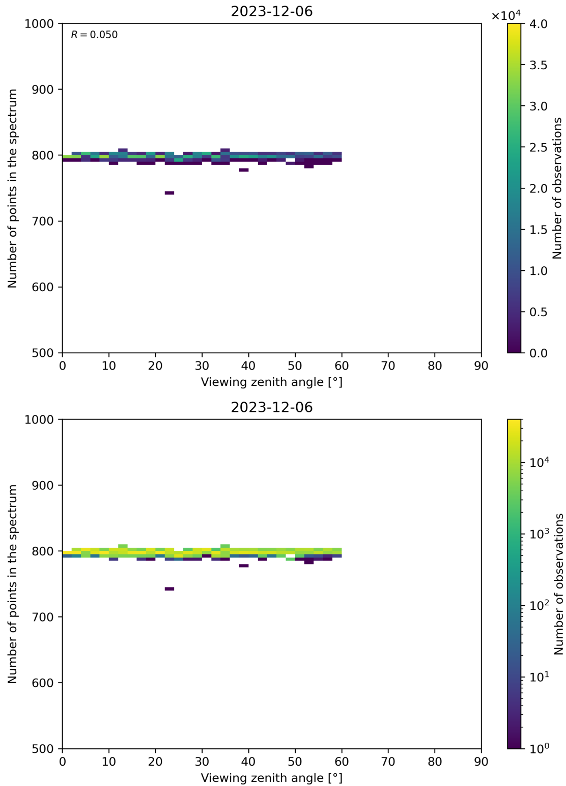
Figure 114: Scatter density plot of “Viewing zenith angle” against “Number of points in the spectrum” for 2023-12-05 to 2023-12-07.
