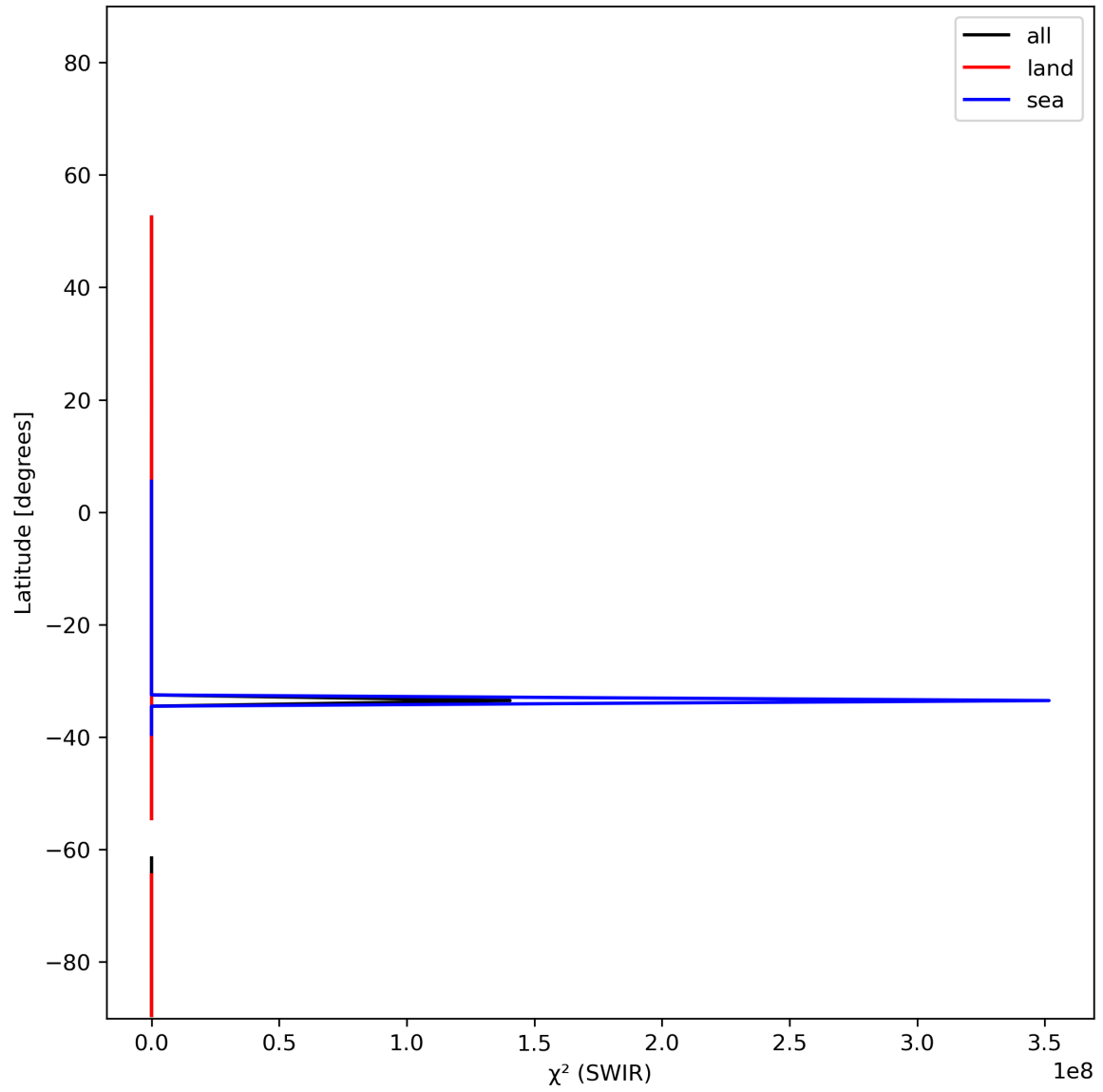
Figure 17: Zonal average of “ \chi^2 (SWIR)” for 2023-12-05 to 2023-12-07.
