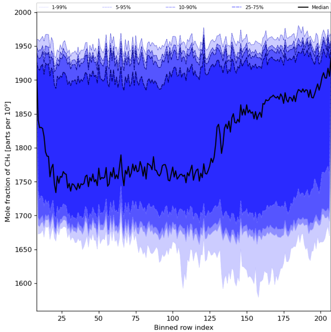
Figure 34: Along track statistics of “Mole fraction of CH 4 ” for 2023-12-05 to 2023-12-07
