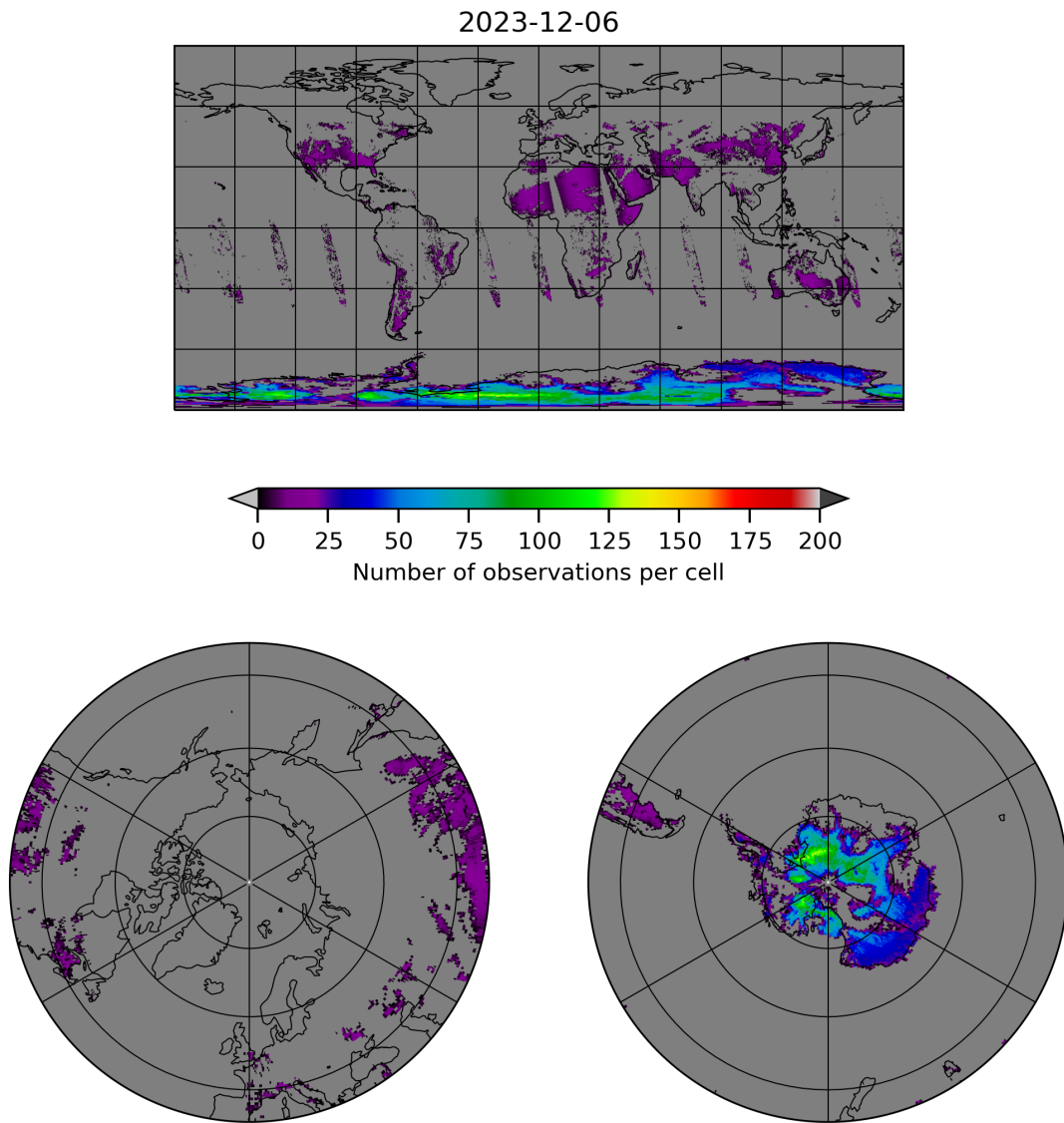
Figure 10: Map of the number of observations for 2023-12-05 to 2023-12-07
