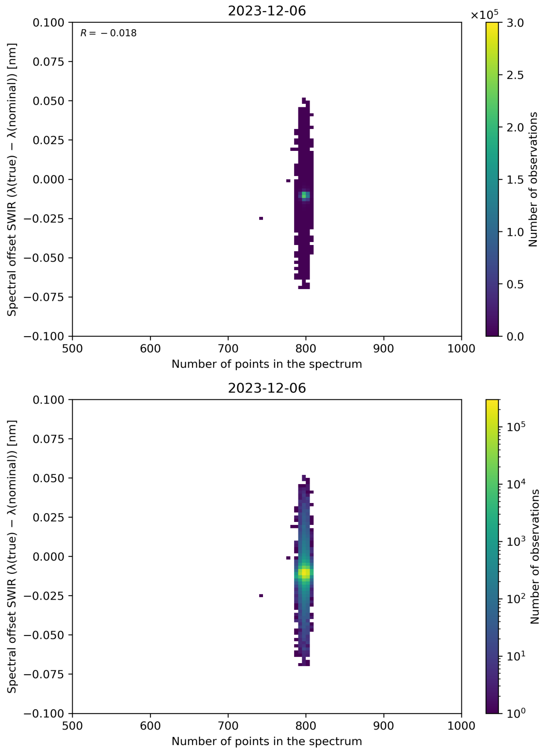
Figure 93: Scatter density plot of “Number of points in the spectrum” against “Spectral offset SWIR ( \lambda(\text{true}) - \lambda(\text{nominal}) )” for 2023-12-05 to 2023-12-07.
