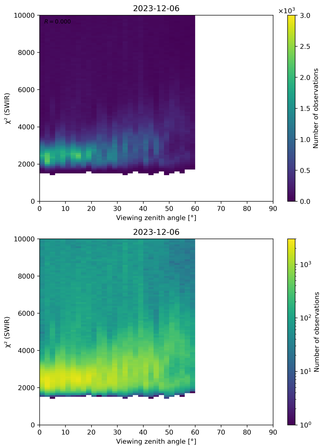
Figure 106: Scatter density plot of “Viewing zenith angle” against “ \chi^2 (SWIR)” for 2023-12-05 to 2023-12-07.
