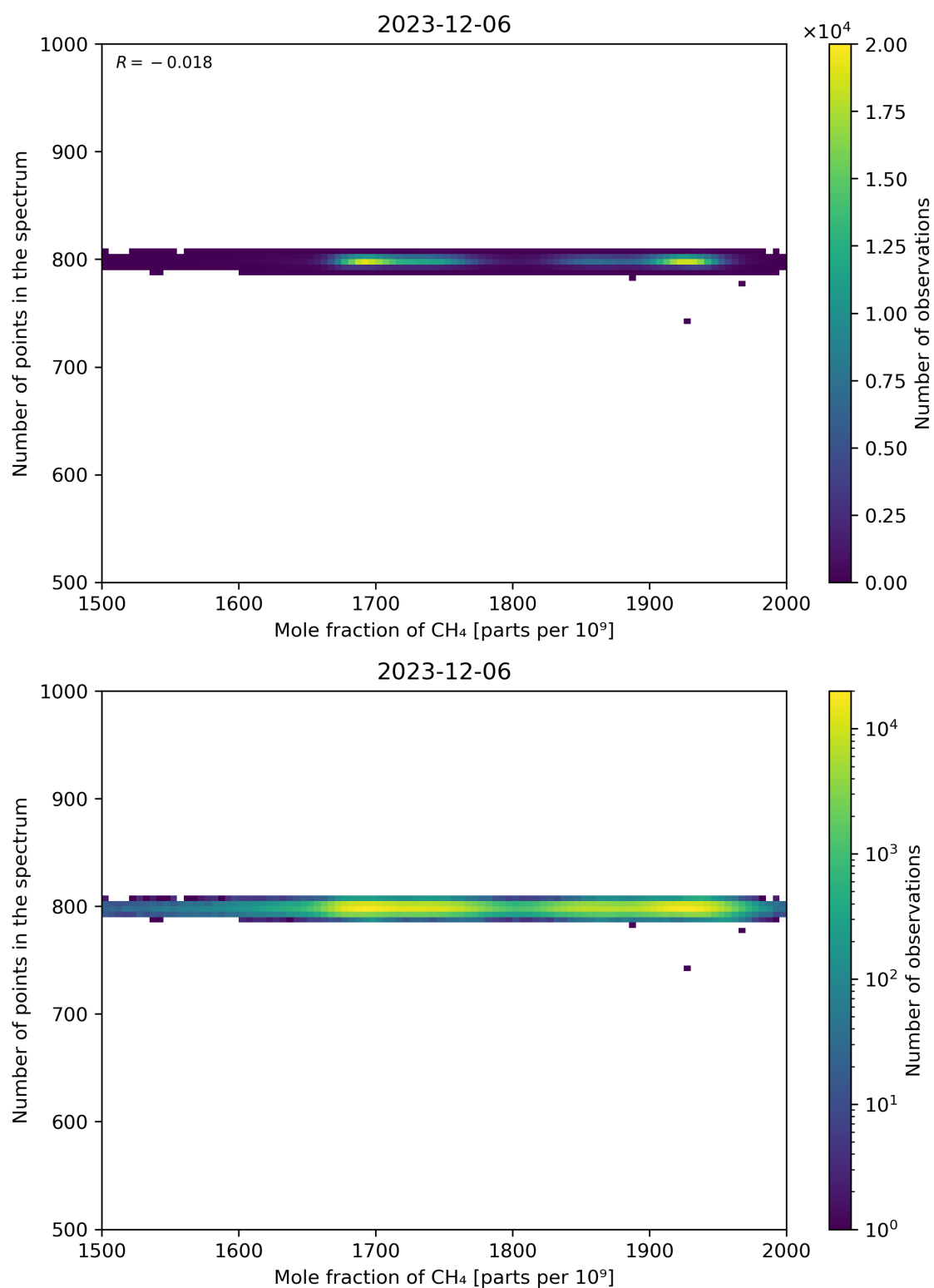
Figure 77: Scatter density plot of “Mole fraction of CH 4 ” against “Number of points in the spectrum” for 2023-12-05 to 2023-12-07.
