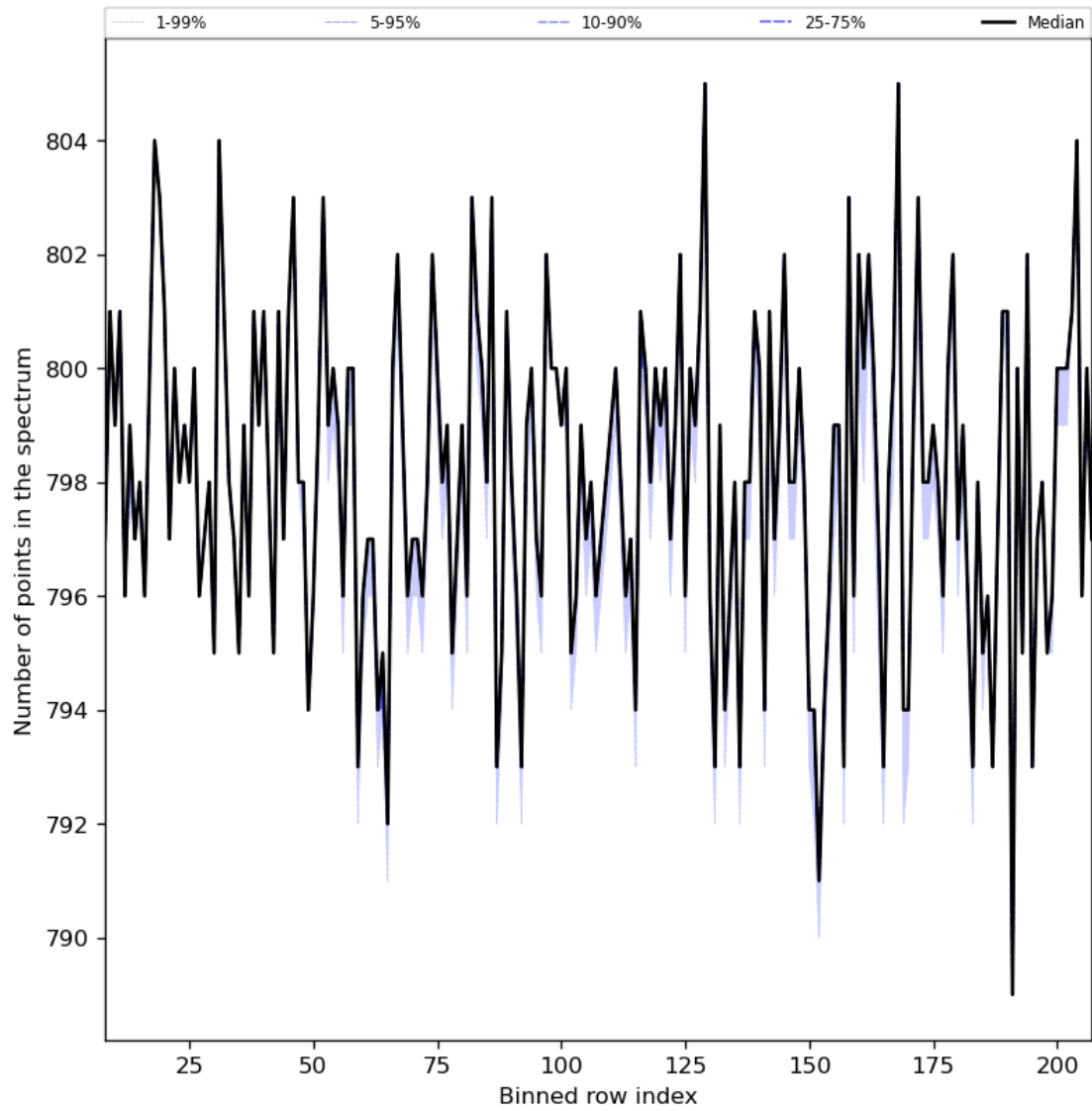
Figure 37: Along track statistics of “Number of points in the spectrum” for 2023-12-05 to 2023-12-07
