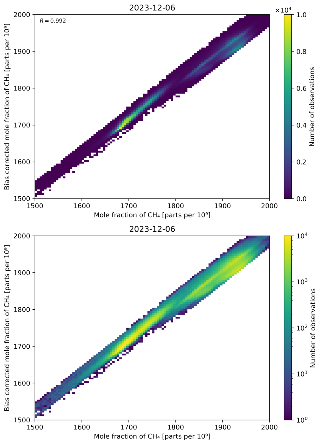
Figure 74: Scatter density plot of “Mole fraction of CH 4 ” against “Bias corrected mole fraction of CH 4 ” for 2023-12-05 to 2023-12-07.
