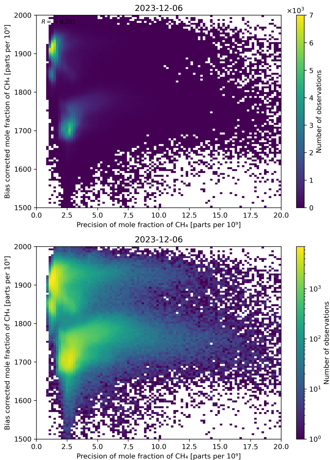
Figure 82: Scatter density plot of “Precision of mole fraction of \text{CH}_4 ” against “Bias corrected mole fraction of \text{CH}_4 ” for 2023-12-05 to 2023-12-07.
