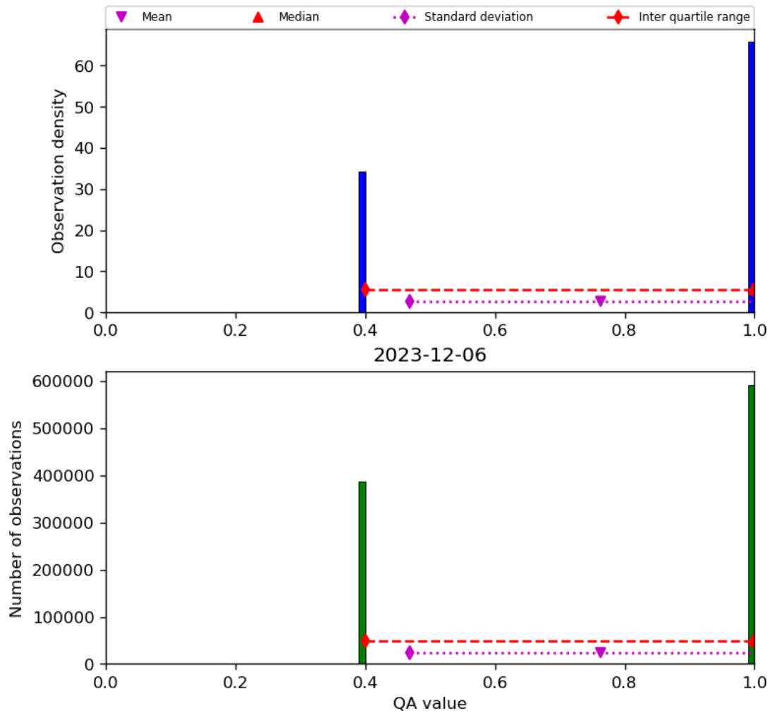
Figure 22: Histogram of “QA value” for 2023-12-05 to 2023-12-07
