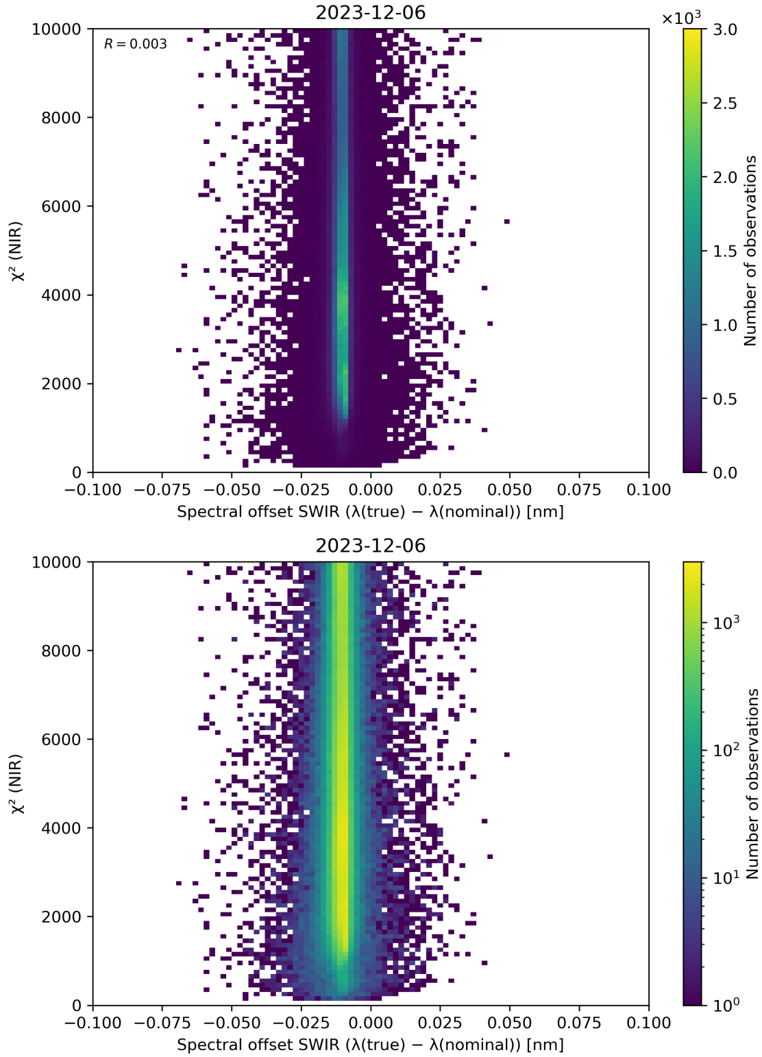
Figure 117: Scatter density plot of “Spectral offset SWIR ( \lambda(\text{true}) - \lambda(\text{nominal}) )” against “ \chi^2 (NIR)” for 2023-12-05 to 2023-12-07.
