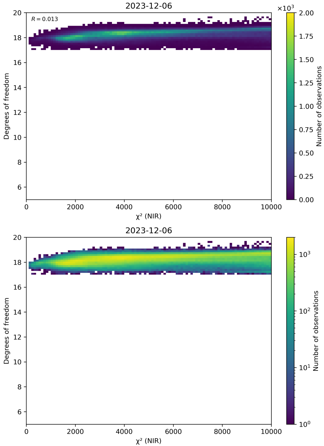
Figure 44: Scatter density plot of “ \chi^2 (NIR)” against “Degrees of freedom” for 2023-12-05 to 2023-12-07.
