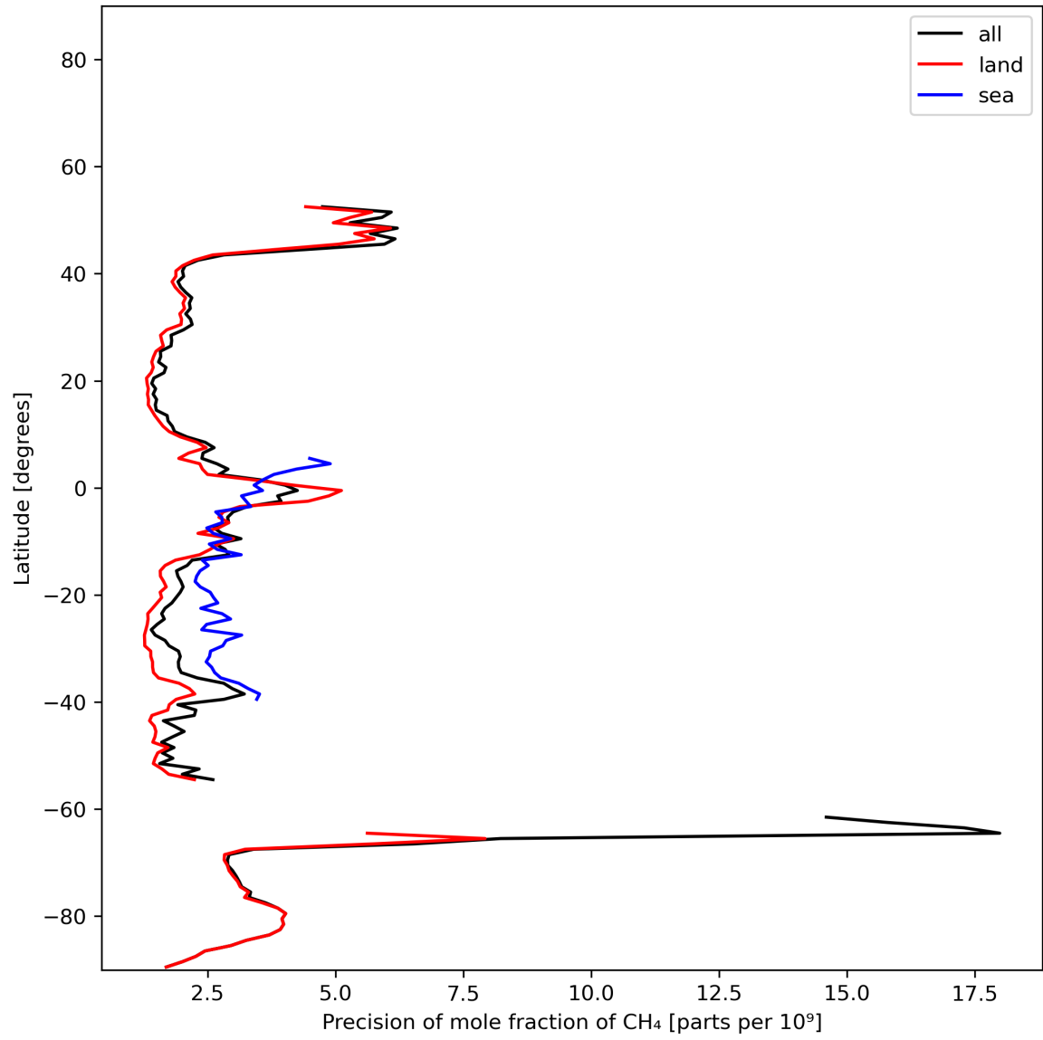
Figure 13: Zonal average of “Precision of mole fraction of CH 4 ” for 2023-12-05 to 2023-12-07.
