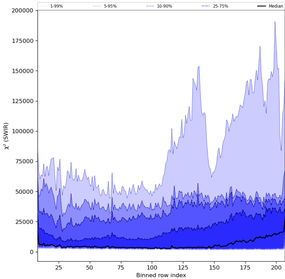
Figure 39: Along track statistics of “ \chi^2 (SWIR)” for 2023-12-05 to 2023-12-07
