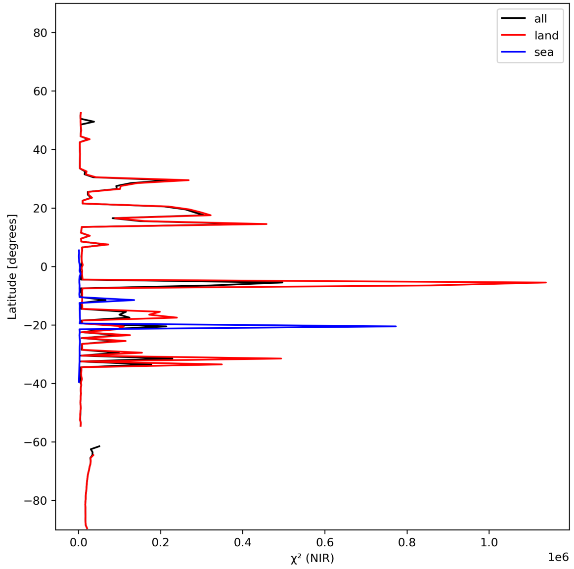
Figure 18: Zonal average of “ \chi^2 (NIR)” for 2023-12-05 to 2023-12-07.
