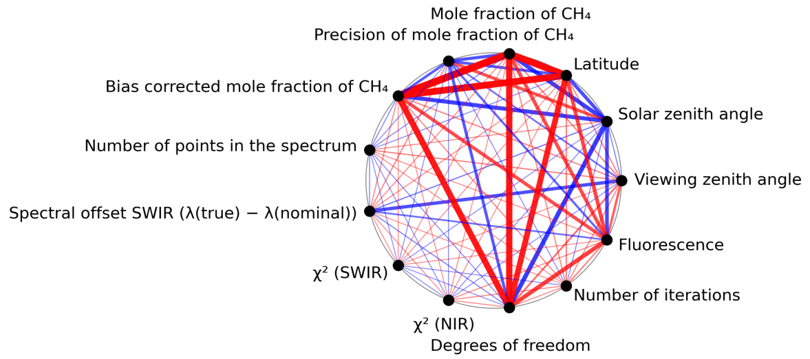
Figure 1: Map of correlation graph for 2023-12-05 to 2023-12-07.
