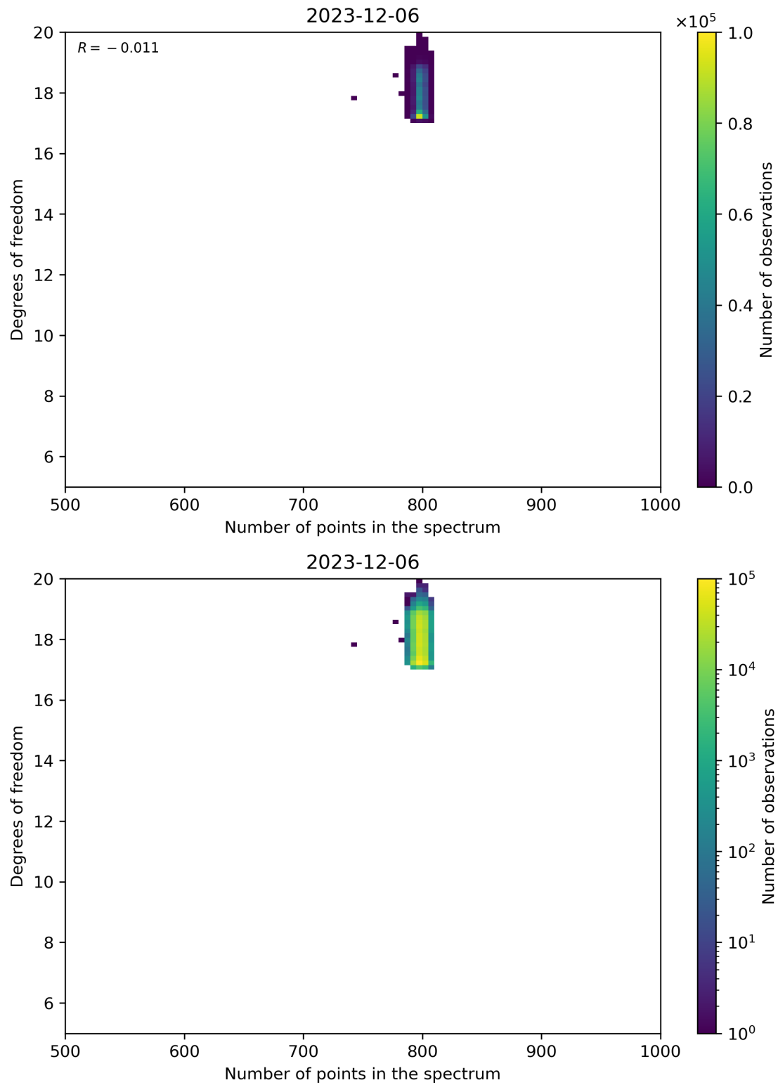
Figure 90: Scatter density plot of “Number of points in the spectrum” against “Degrees of freedom” for 2023-12-05 to 2023-12-07.
