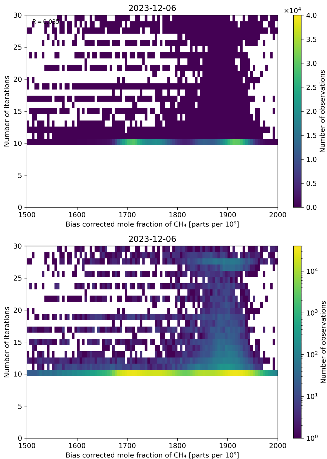
Figure 67: Scatter density plot of “Bias corrected mole fraction of CH 4 ” against “Number of iterations” for 2023-12-05 to 2023-12-07.
