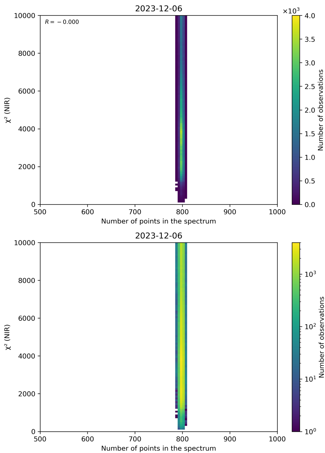
Figure 88: Scatter density plot of “Number of points in the spectrum” against “ \chi^2 (NIR)” for 2023-12-05 to 2023-12-07.
