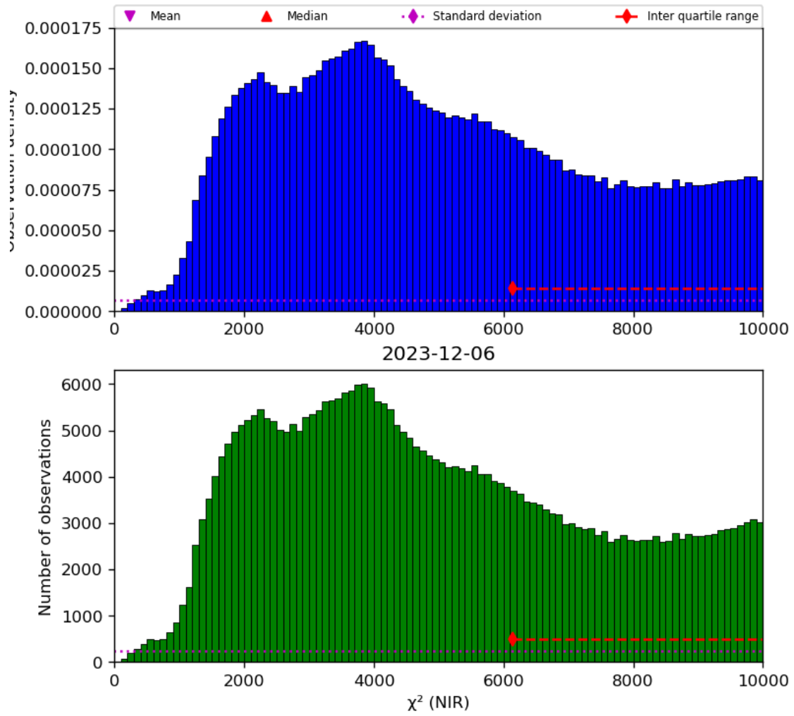
Figure 29: Histogram of “ \chi^2 (NIR)” for 2023-12-05 to 2023-12-07
