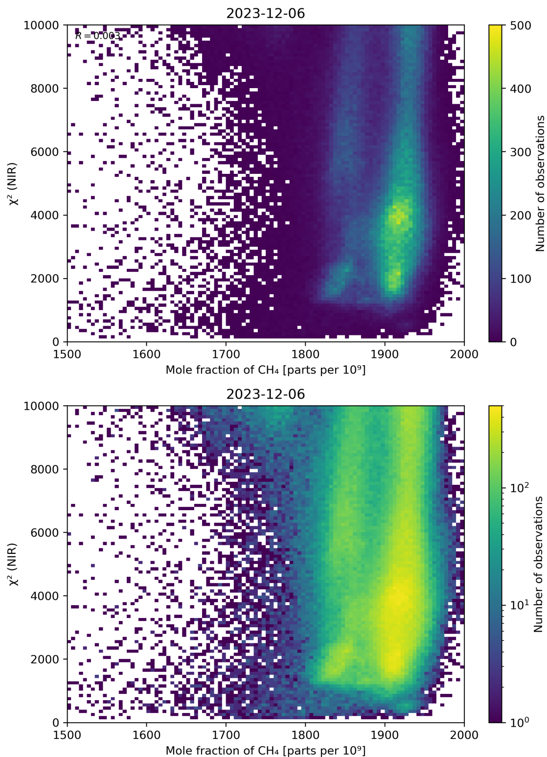
Figure 70: Scatter density plot of “Mole fraction of CH 4 ” against “ \chi^2 (NIR)” for 2023-12-05 to 2023-12-07.
