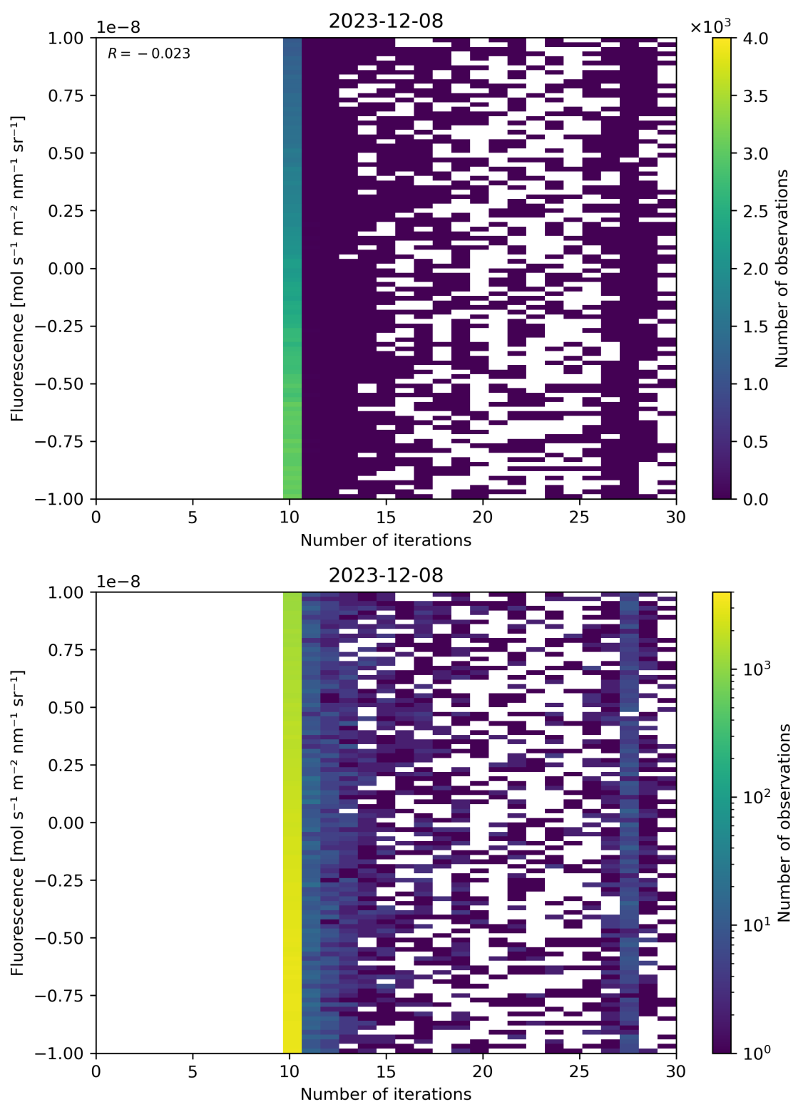
Figure 87: Scatter density plot of “Number of iterations” against “Fluorescence” for 2023-12-07 to 2023-12-09.
