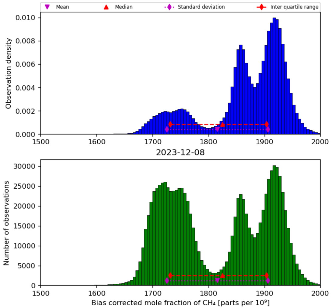
Figure 25: Histogram of “Bias corrected mole fraction of CH 4 ” for 2023-12-07 to 2023-12-09
