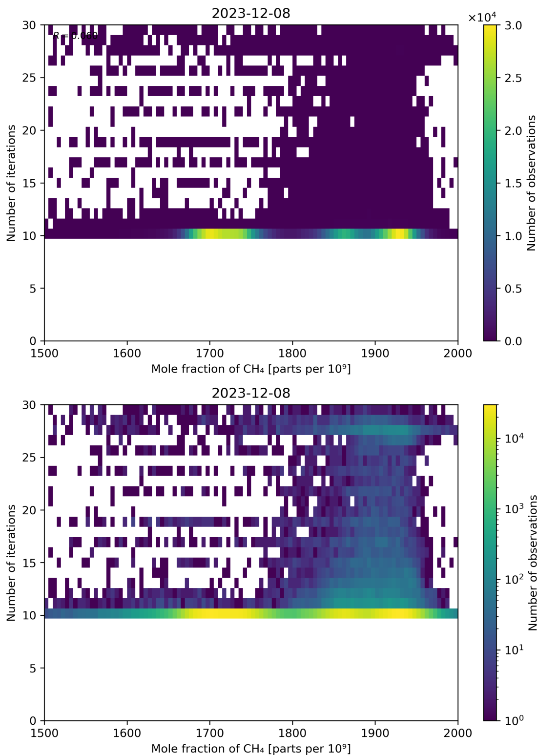
Figure 76: Scatter density plot of “Mole fraction of CH 4 ” against “Number of iterations” for 2023-12-07 to 2023-12-09.
