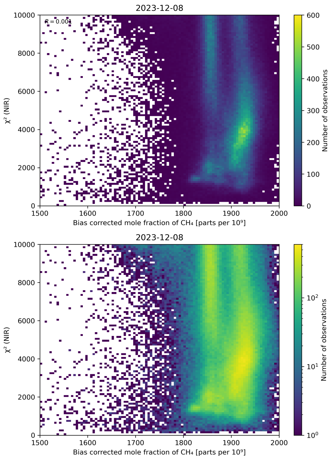
Figure 63: Scatter density plot of “Bias corrected mole fraction of CH 4 ” against “ \chi^2 (NIR)” for 2023-12-07 to 2023-12-09.
