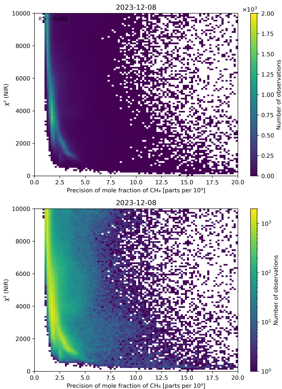
Figure 78: Scatter density plot of “Precision of mole fraction of CH 4 ” against “ \chi^2 (NIR)” for 2023-12-07 to 2023-12-09.
