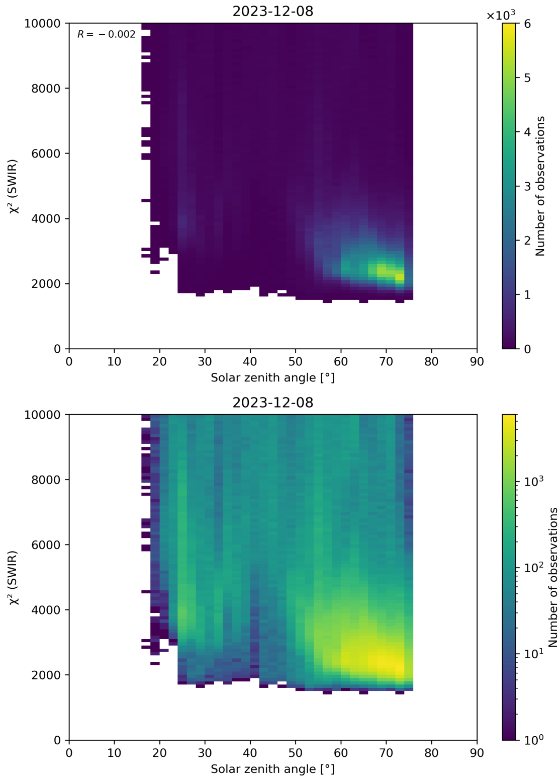
Figure 95: Scatter density plot of “Solar zenith angle” against “ \chi^2 (SWIR)” for 2023-12-07 to 2023-12-09.
