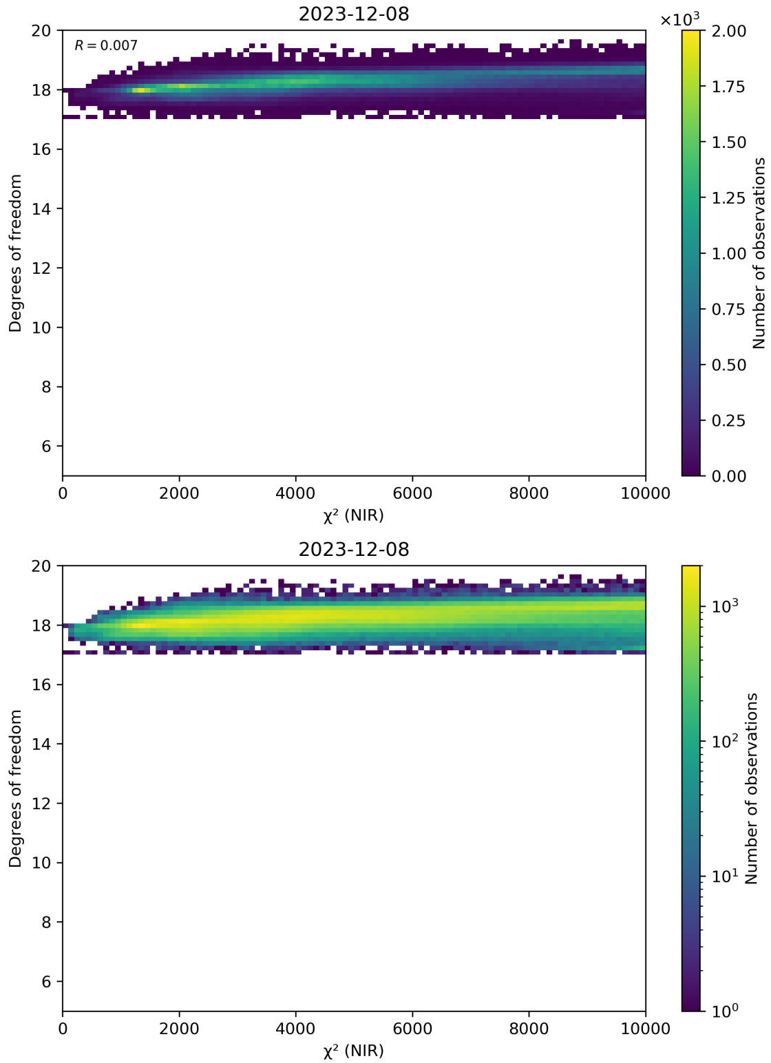
Figure 44: Scatter density plot of “ \chi^2 (NIR)” against “Degrees of freedom” for 2023-12-07 to 2023-12-09.
