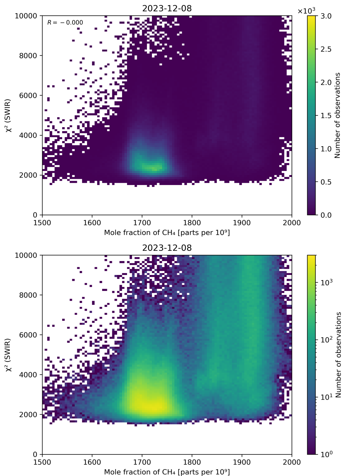
Figure 71: Scatter density plot of “Mole fraction of CH 4 ” against “ \chi^2 (SWIR)” for 2023-12-07 to 2023-12-09.
