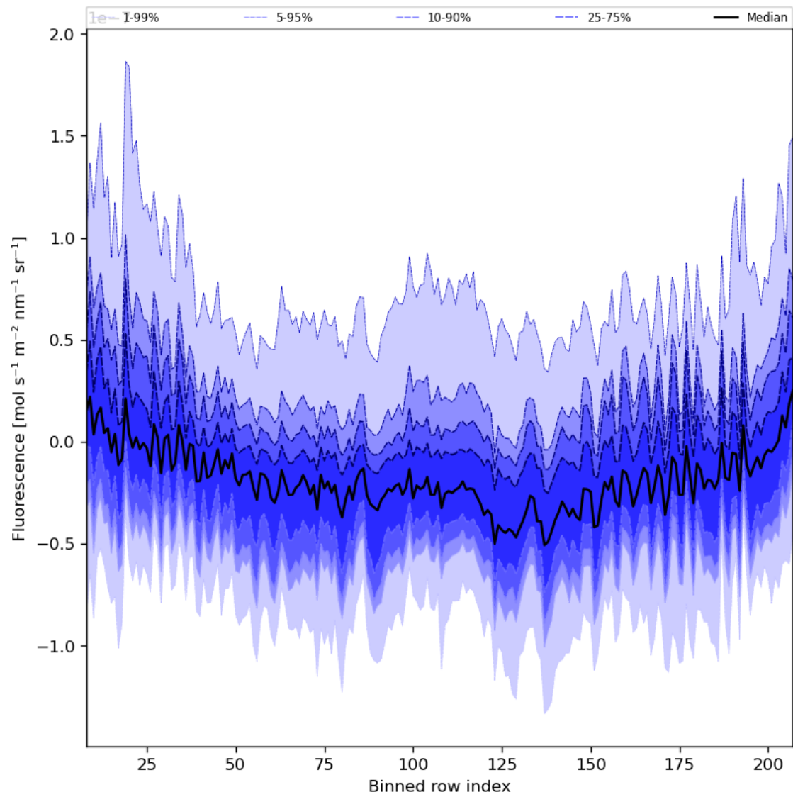
Figure 43: Along track statistics of “Fluorescence” for 2023-12-07 to 2023-12-09
