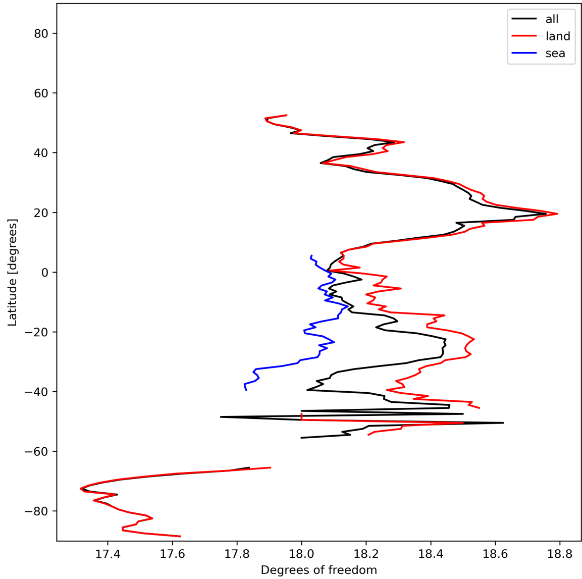
Figure 19: Zonal average of “Degrees of freedom” for 2023-12-07 to 2023-12-09.
