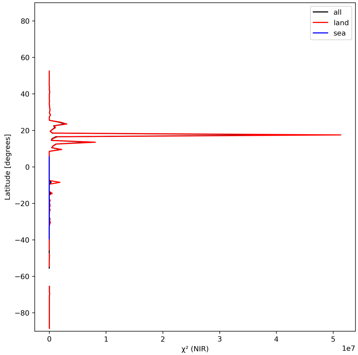
Figure 18: Zonal average of “ \chi^2 (NIR)” for 2023-12-07 to 2023-12-09.
