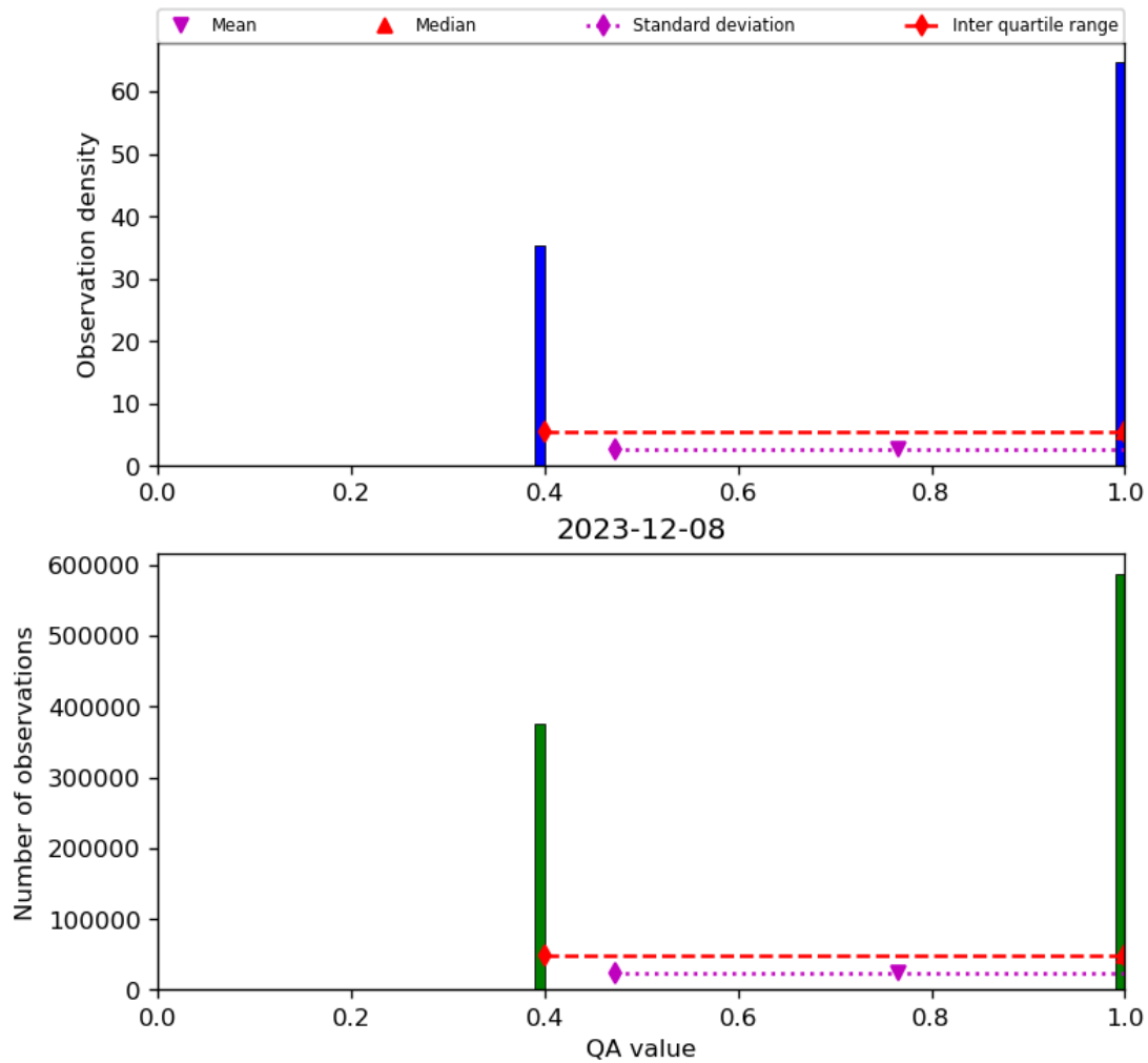
Figure 22: Histogram of “QA value” for 2023-12-07 to 2023-12-09
