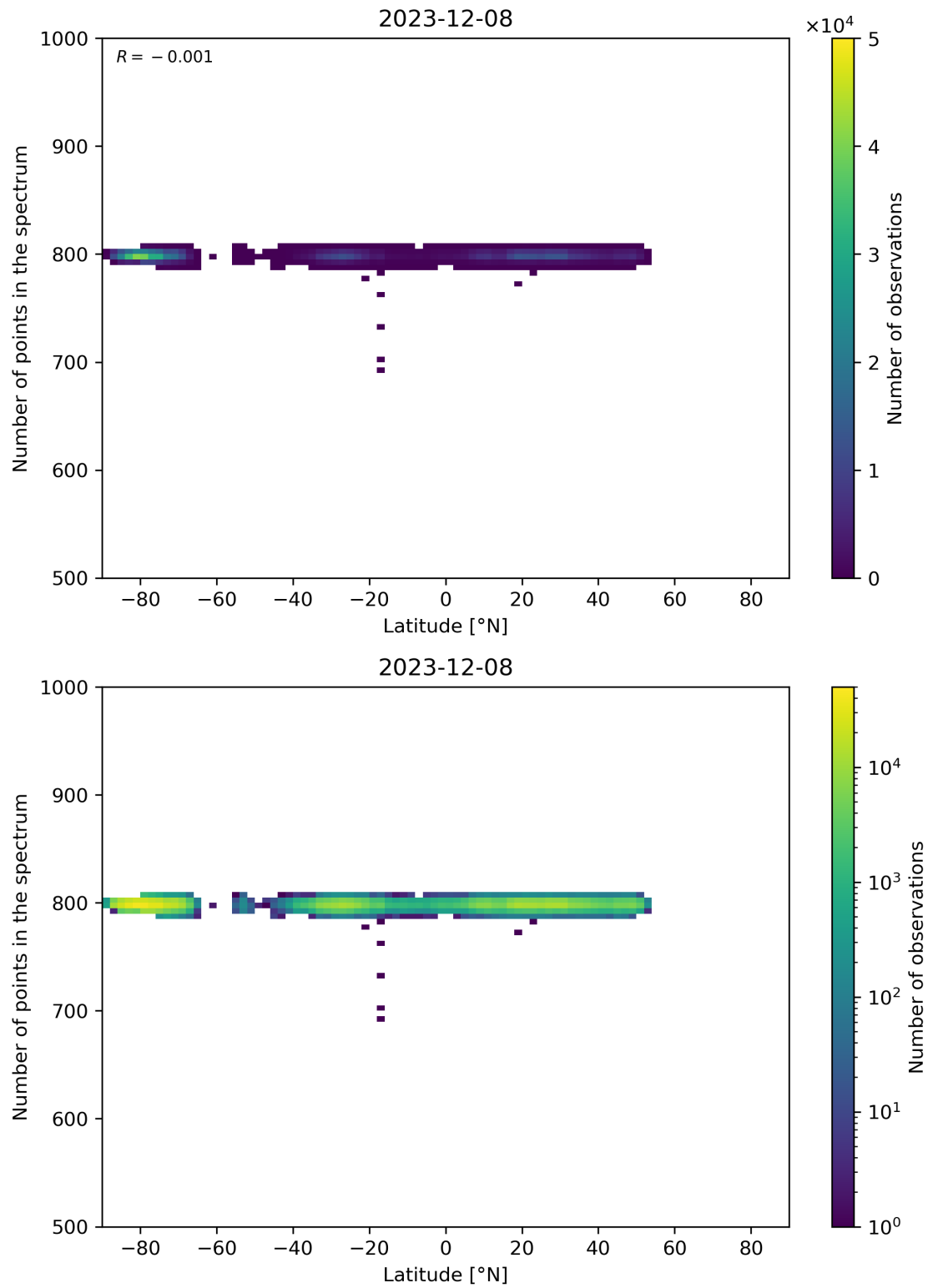
Figure 61: Scatter density plot of “Latitude” against “Number of points in the spectrum” for 2023-12-07 to 2023-12-09.
