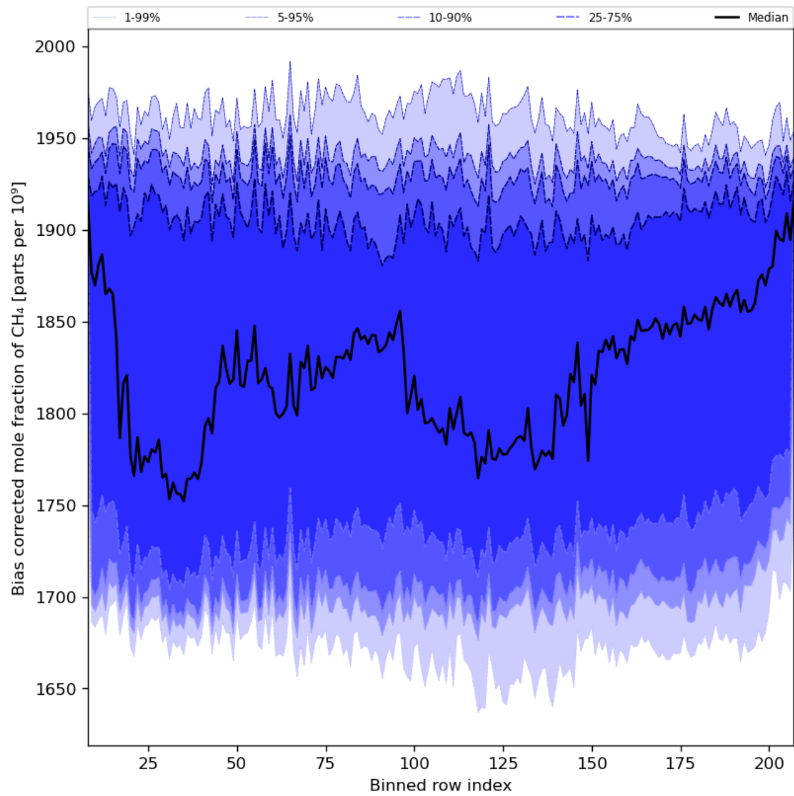
Figure 36: Along track statistics of “Bias corrected mole fraction of CH 4 ” for 2023-12-07 to 2023-12-09
