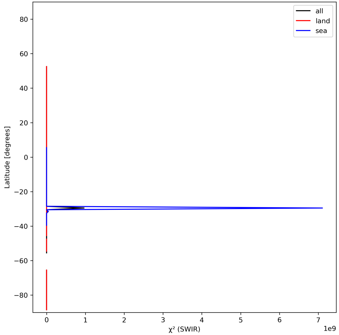
Figure 17: Zonal average of “ \chi^2 (SWIR)” for 2023-12-07 to 2023-12-09.
