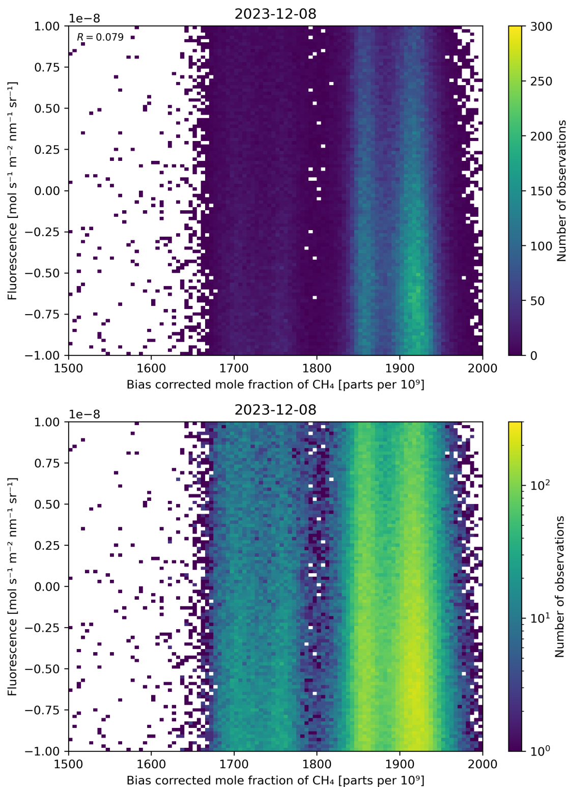
Figure 66: Scatter density plot of “Bias corrected mole fraction of \text{CH}_4 ” against “Fluorescence” for 2023-12-07 to 2023-12-09.
