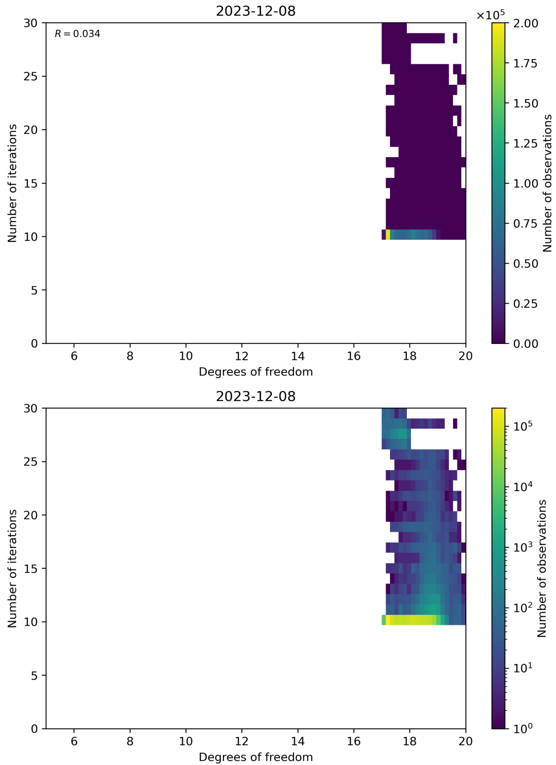
Figure 52: Scatter density plot of “Degrees of freedom” against “Number of iterations” for 2023-12-07 to 2023-12-09.
