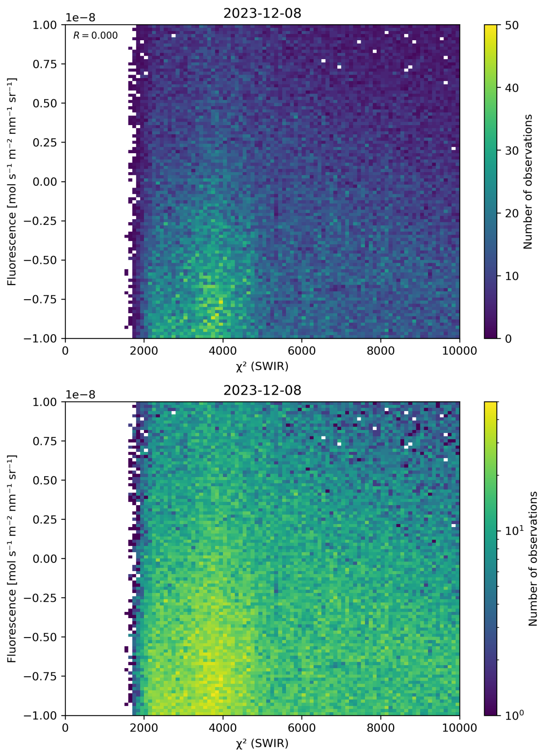
Figure 49: Scatter density plot of “ \chi^2 (SWIR)” against “Fluorescence” for 2023-12-07 to 2023-12-09.
