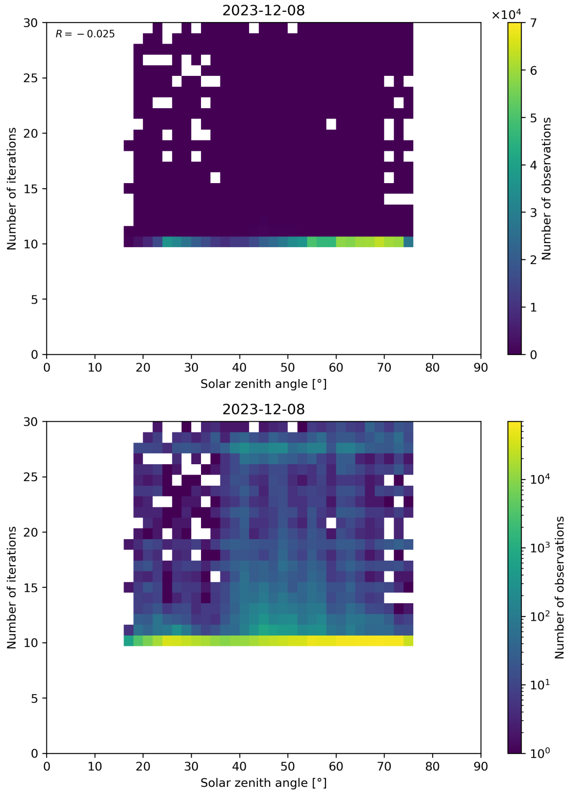
Figure 102: Scatter density plot of “Solar zenith angle” against “Number of iterations” for 2023-12-07 to 2023-12-09.
