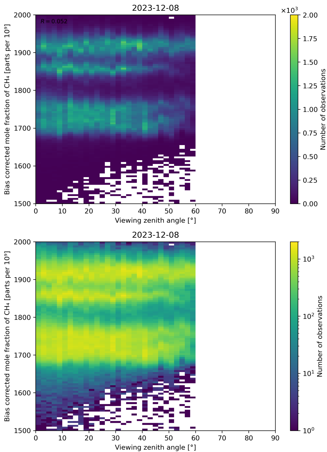
Figure 111: Scatter density plot of “Viewing zenith angle” against “Bias corrected mole fraction of CH 4 ” for 2023-12-07 to 2023-12-09.
