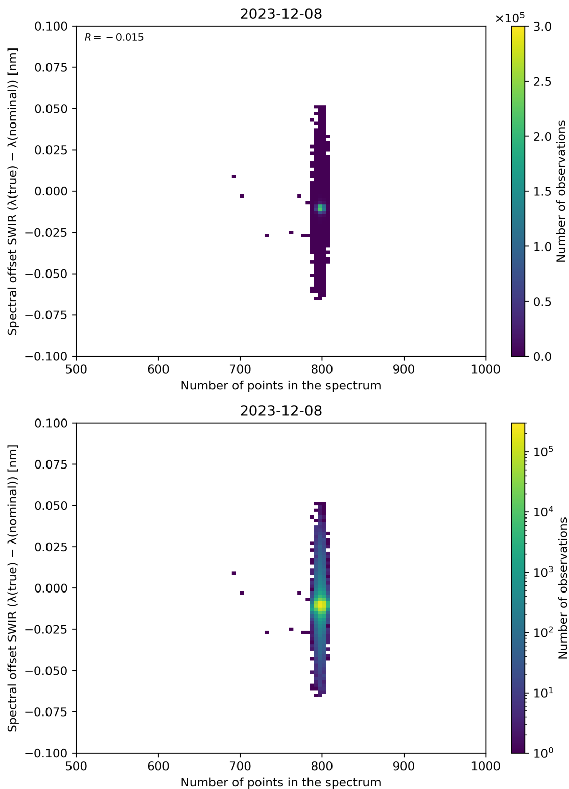
Figure 93: Scatter density plot of “Number of points in the spectrum” against “Spectral offset SWIR ( \lambda(\text{true}) - \lambda(\text{nominal}) )” for 2023-12-07 to 2023-12-09.
