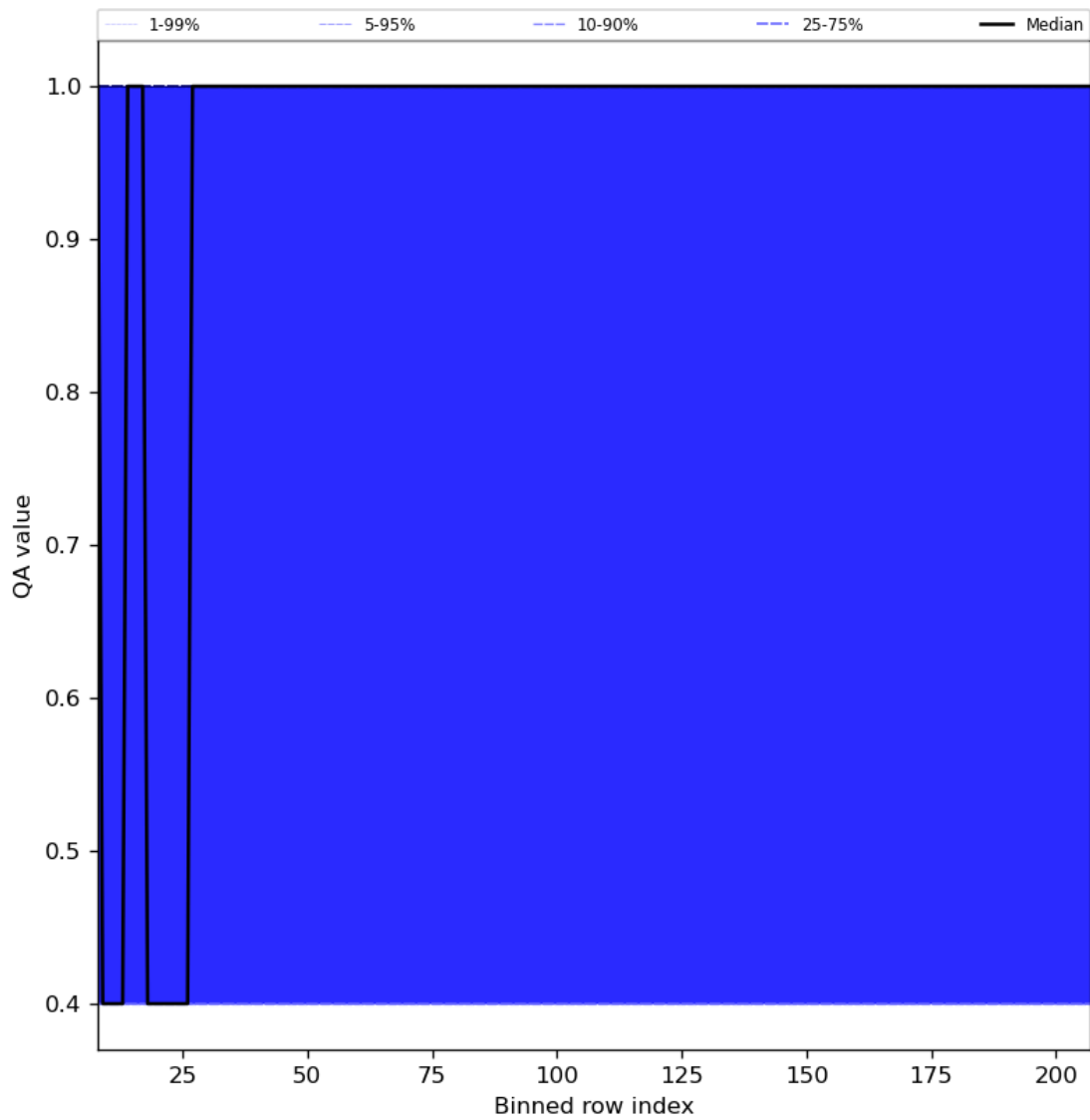
Figure 33: Along track statistics of “QA value” for 2023-12-07 to 2023-12-09
