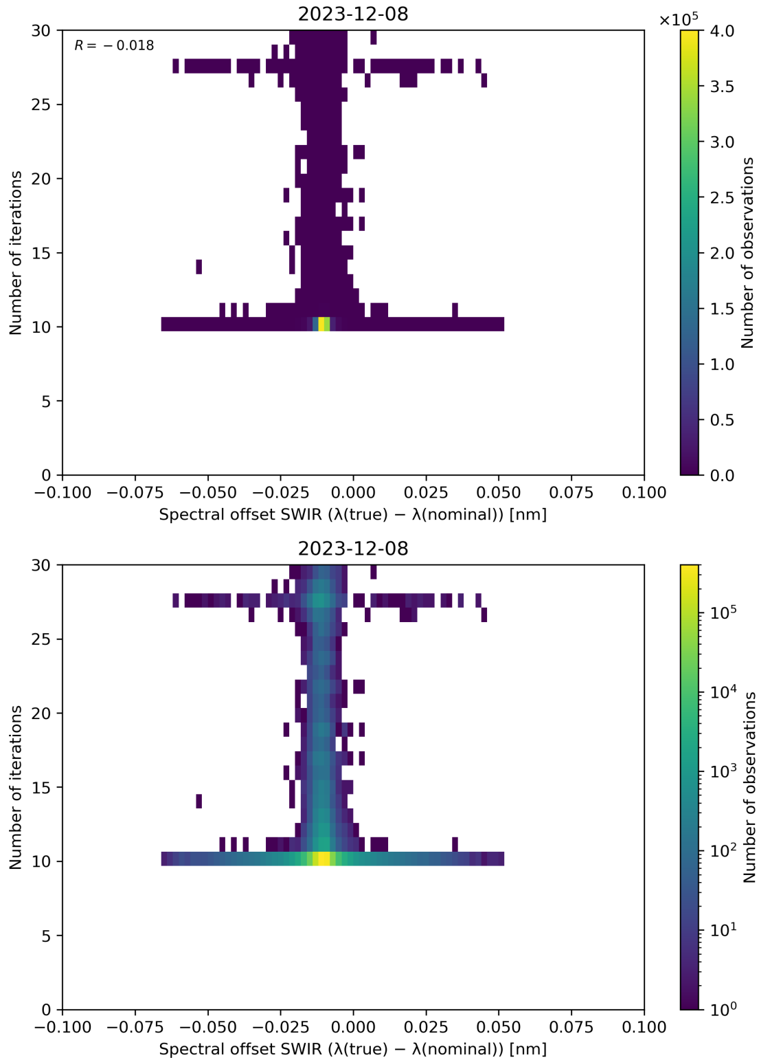
Figure 121: Scatter density plot of “Spectral offset SWIR ( \lambda(\text{true}) - \lambda(\text{nominal}) )” against “Number of iterations” for 2023-12-07 to 2023-12-09.
