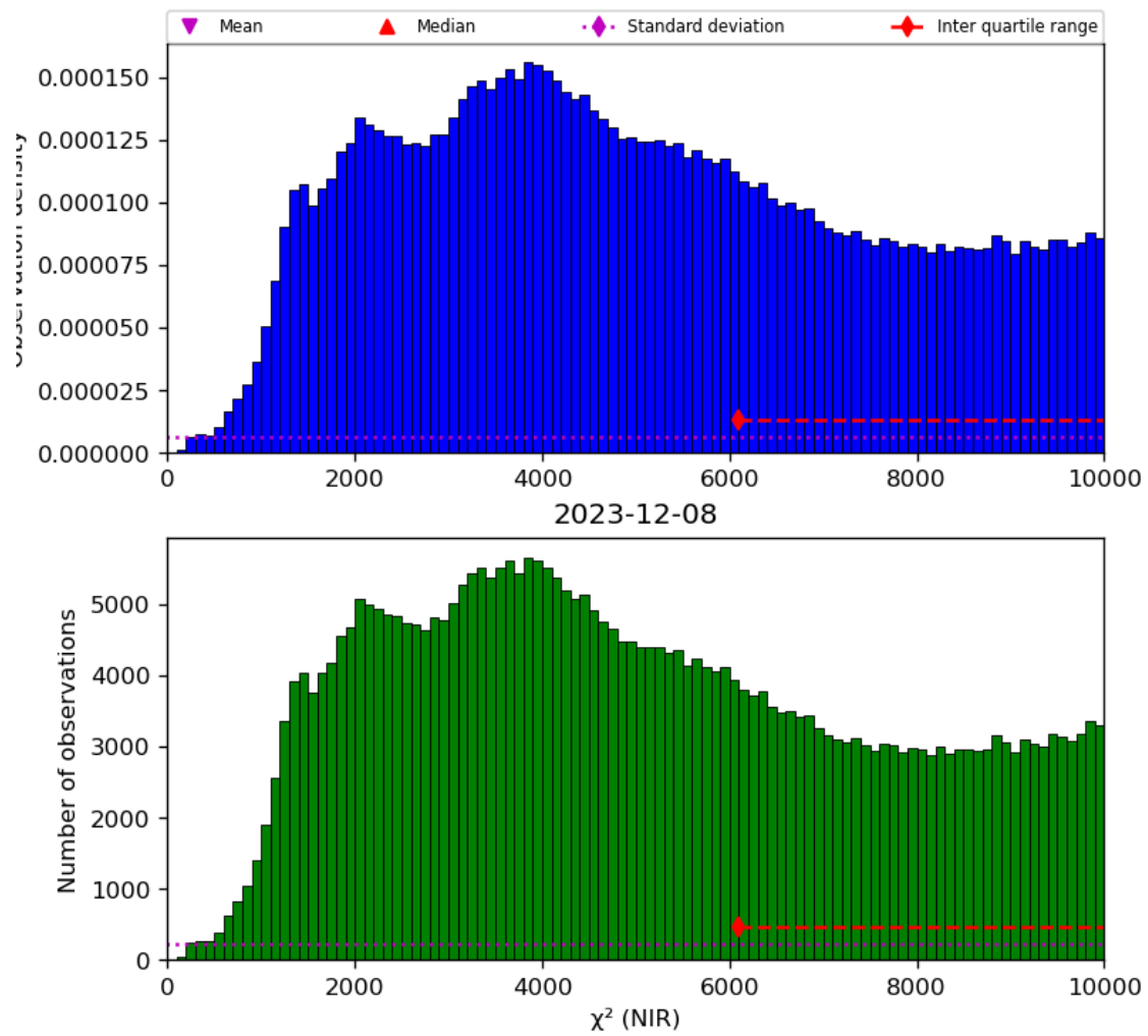
Figure 29: Histogram of “ \chi^2 (NIR)” for 2023-12-07 to 2023-12-09
