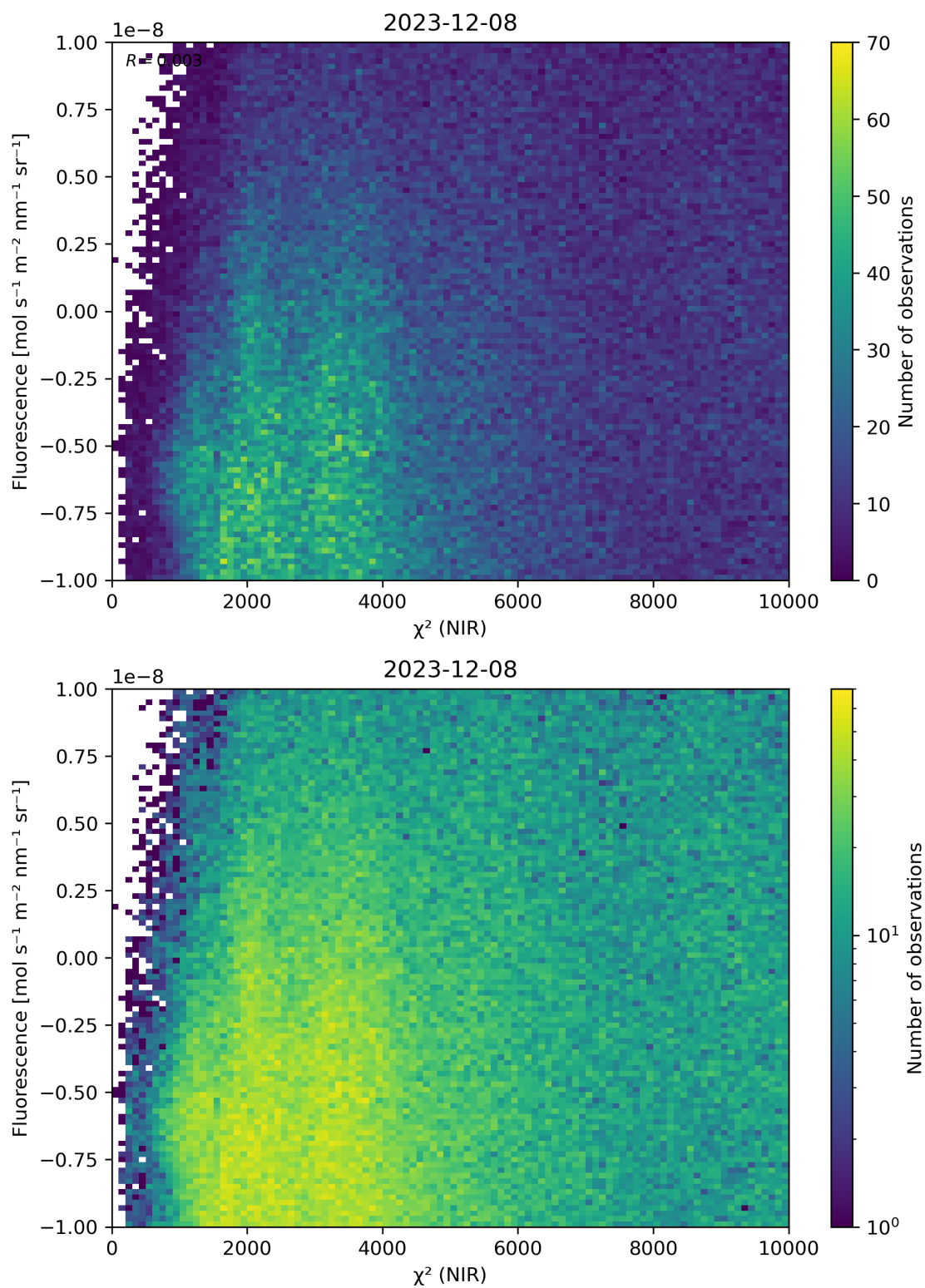
Figure 45: Scatter density plot of “ \chi^2 (NIR)” against “Fluorescence” for 2023-12-07 to 2023-12-09.
