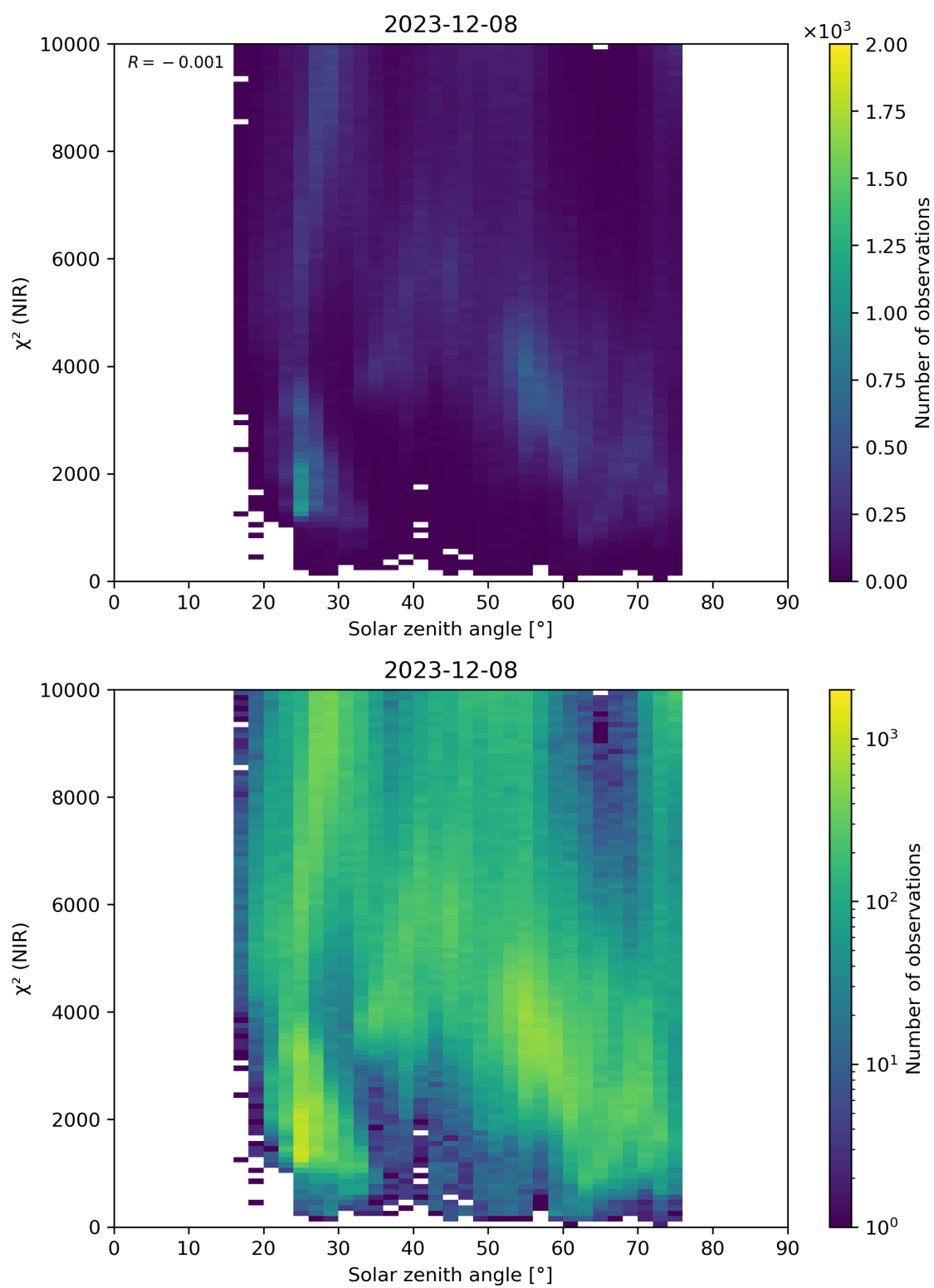
Figure 94: Scatter density plot of “Solar zenith angle” against “ \chi^2 (NIR)” for 2023-12-07 to 2023-12-09.
