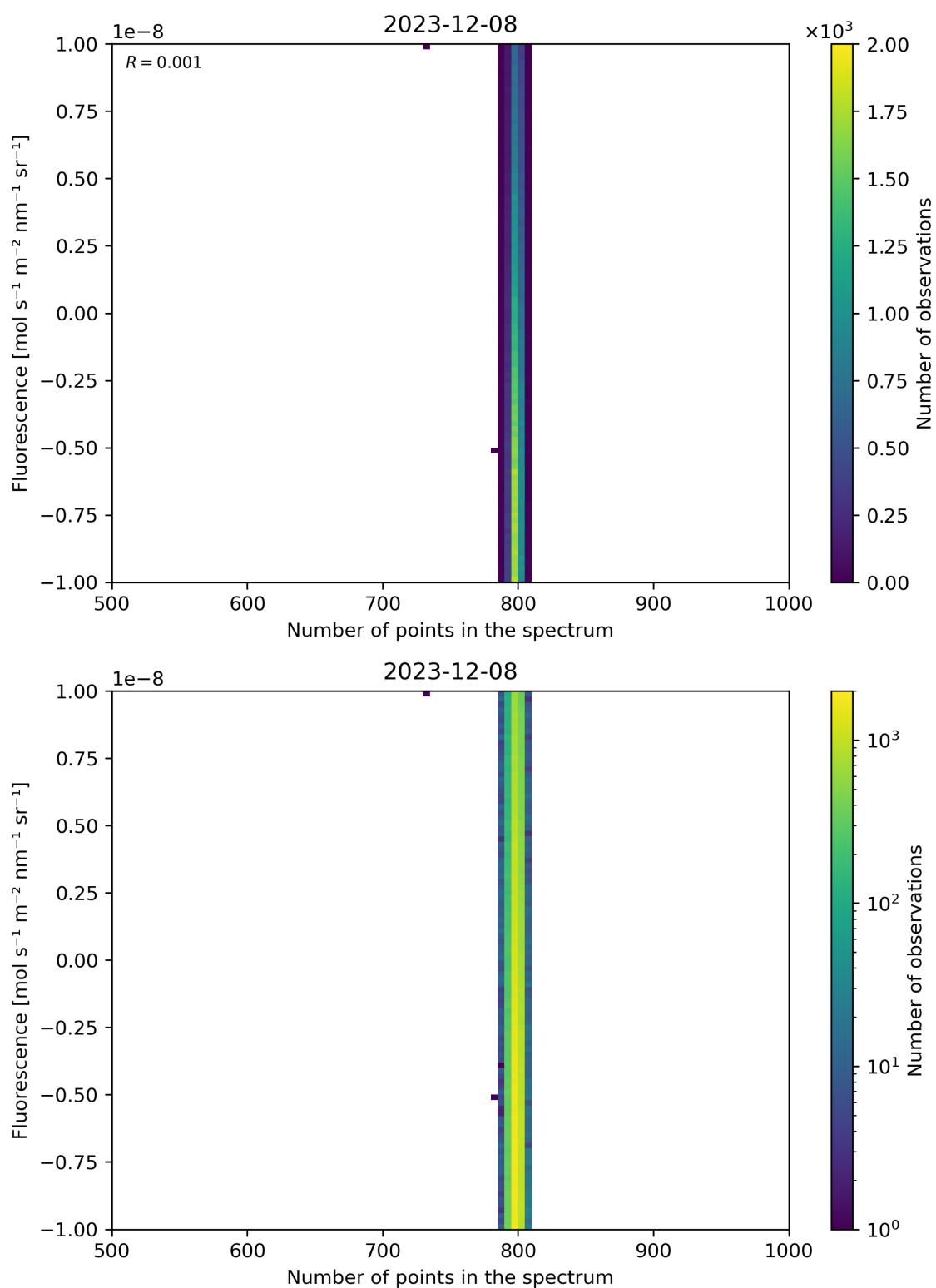
Figure 91: Scatter density plot of “Number of points in the spectrum” against “Fluorescence” for 2023-12-07 to 2023-12-09.
