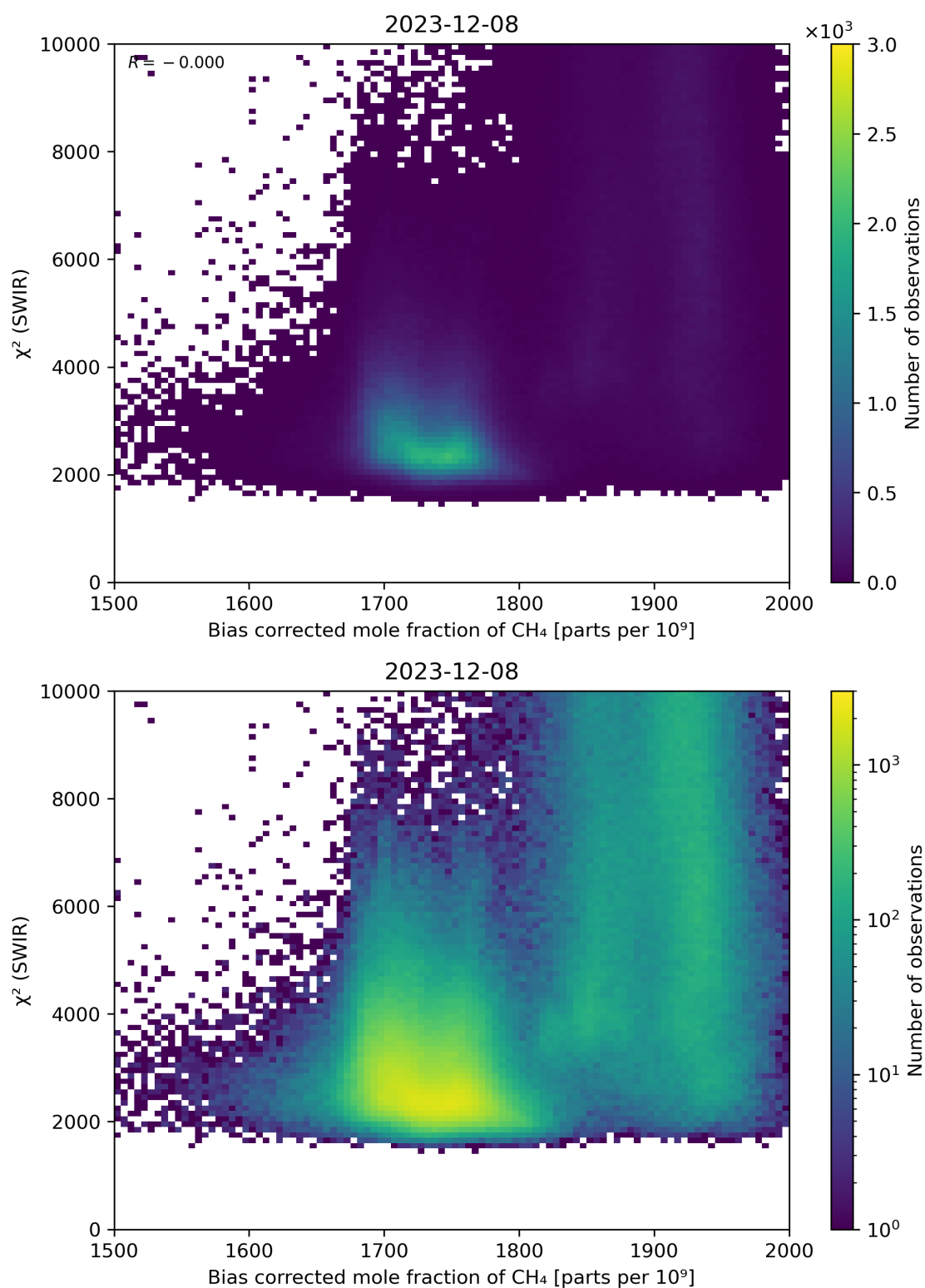
Figure 64: Scatter density plot of “Bias corrected mole fraction of CH 4 ” against “ \chi^2 (SWIR)” for 2023-12-07 to 2023-12-09.
