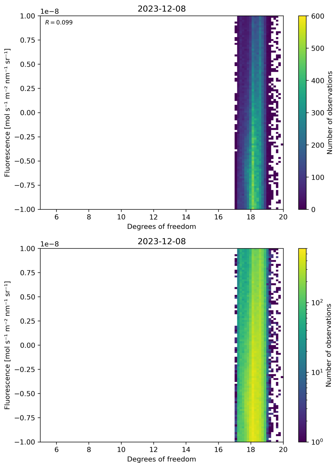
Figure 51: Scatter density plot of “Degrees of freedom” against “Fluorescence” for 2023-12-07 to 2023-12-09.
