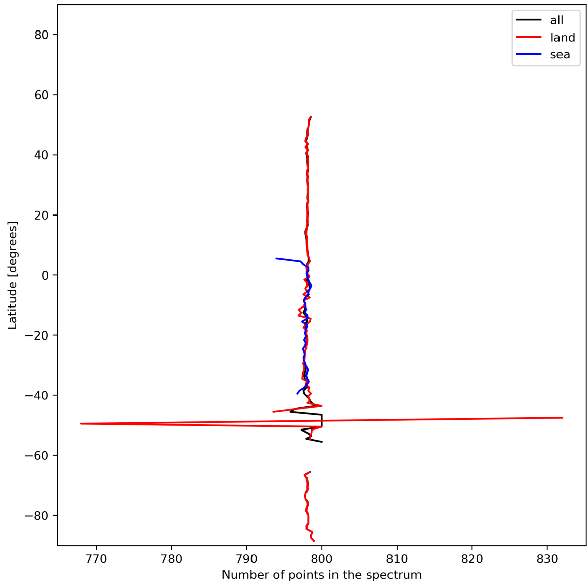
Figure 15: Zonal average of “Number of points in the spectrum” for 2023-12-07 to 2023-12-09.
