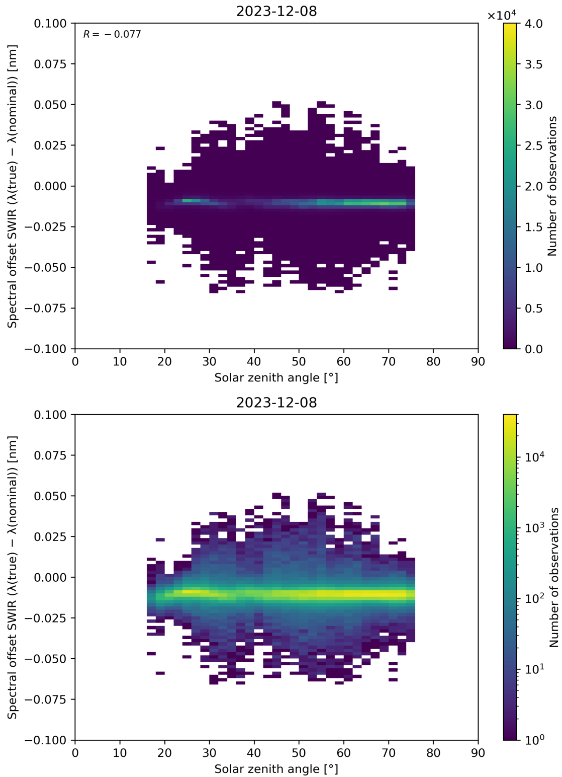
Figure 104: Scatter density plot of “Solar zenith angle” against “Spectral offset SWIR ( \lambda(\text{true}) - \lambda(\text{nominal}) )” for 2023-12-07 to 2023-12-09.
