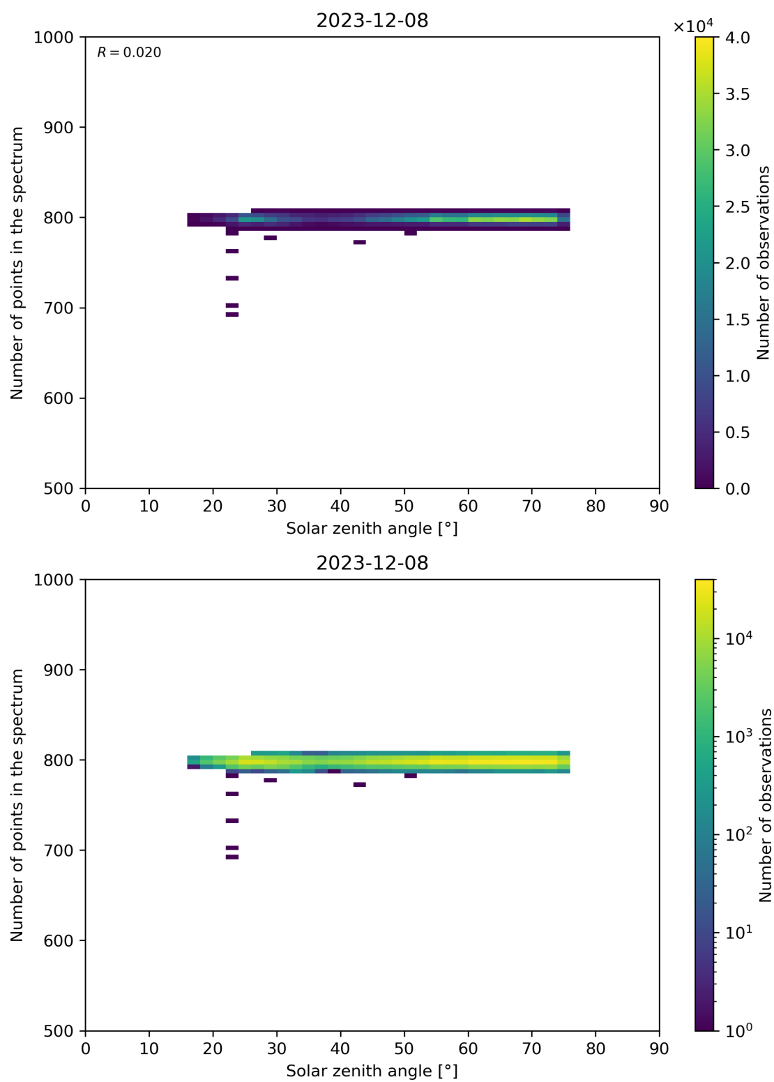
Figure 103: Scatter density plot of “Solar zenith angle” against “Number of points in the spectrum” for 2023-12-07 to 2023-12-09.
