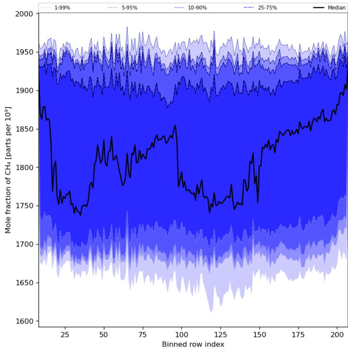
Figure 34: Along track statistics of “Mole fraction of CH 4 ” for 2023-12-07 to 2023-12-09
