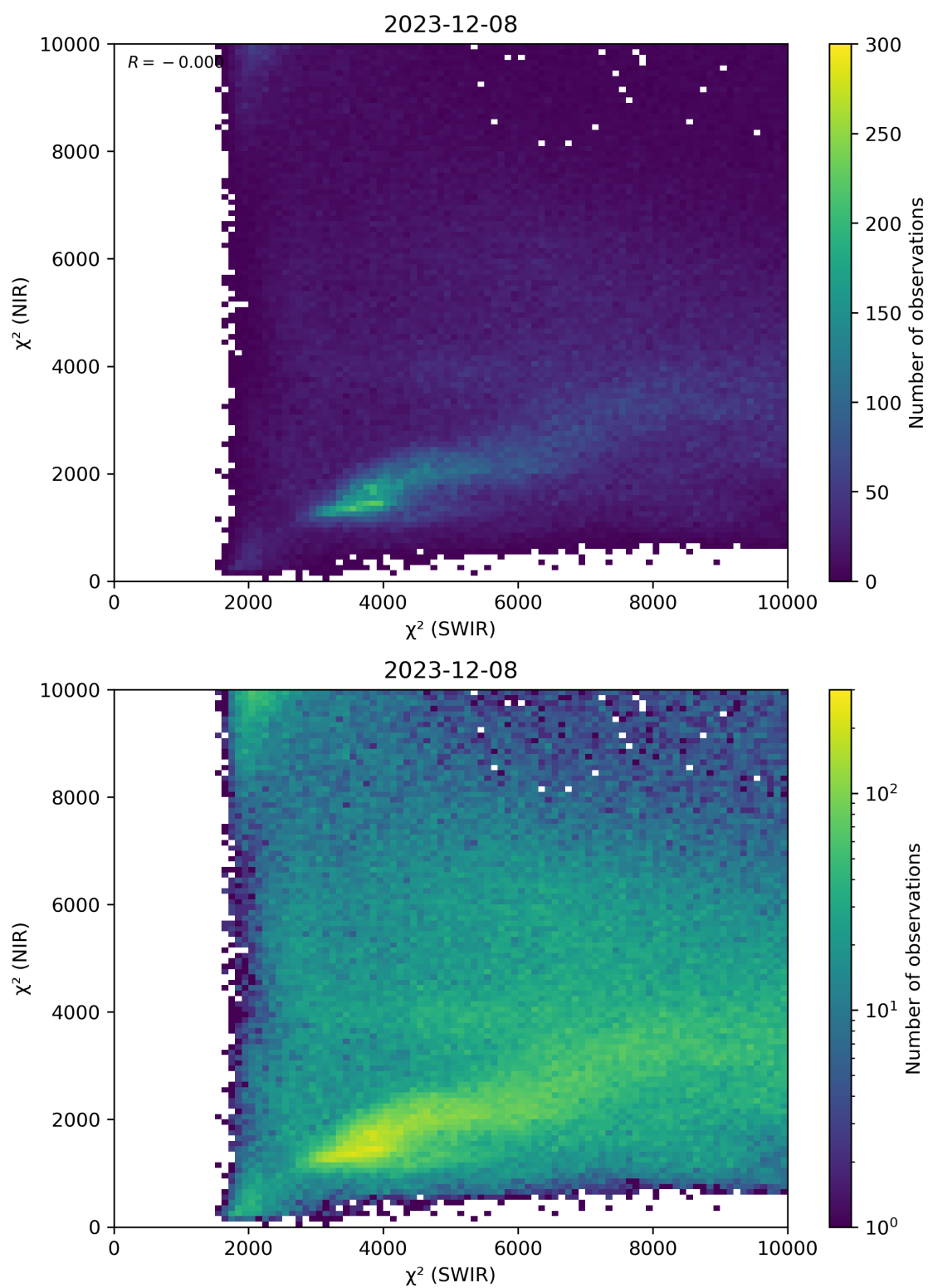
Figure 47: Scatter density plot of “ \chi^2 (SWIR)” against “ \chi^2 (NIR)” for 2023-12-07 to 2023-12-09.
