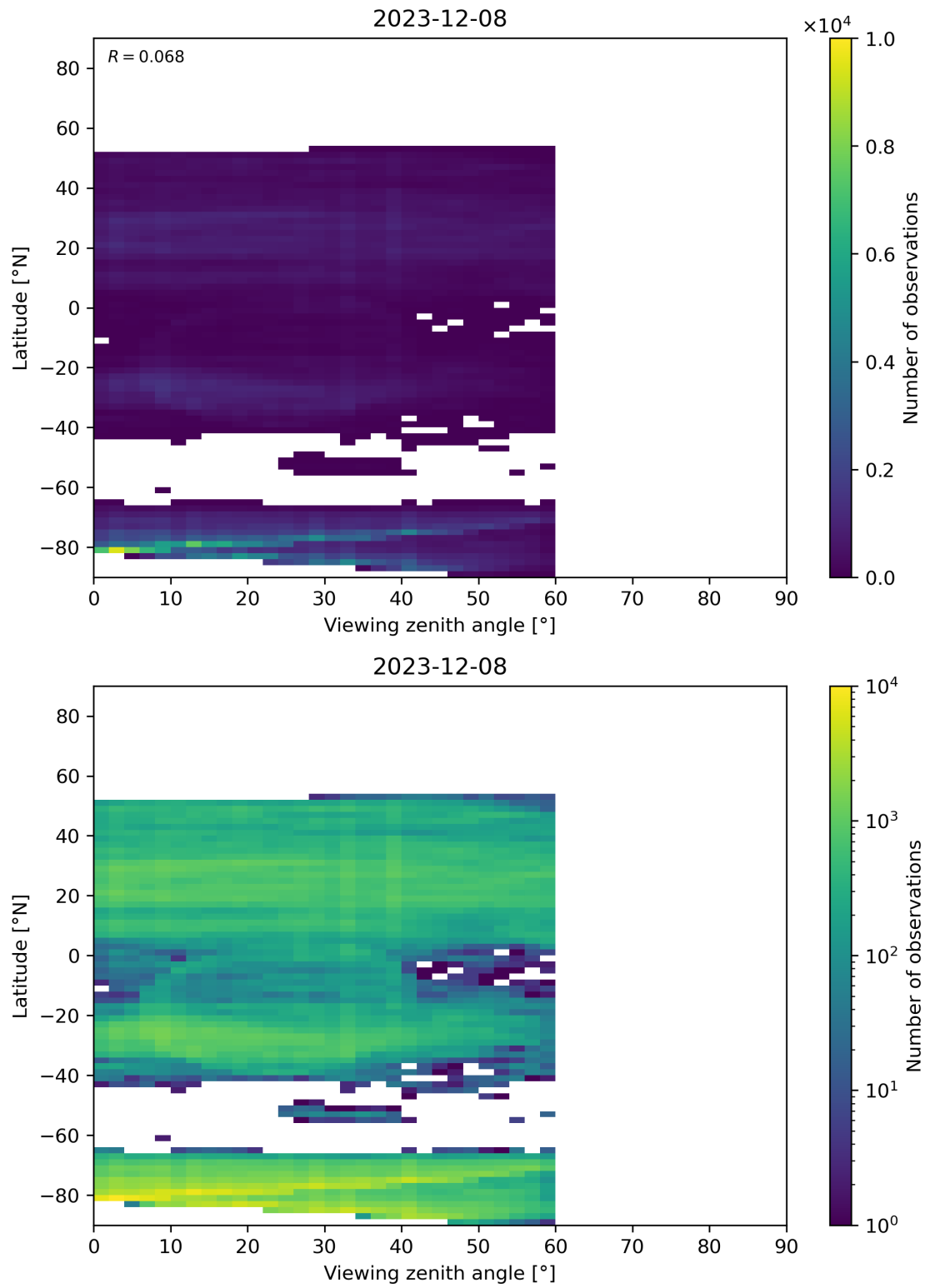
Figure 109: Scatter density plot of “Viewing zenith angle” against “Latitude” for 2023-12-07 to 2023-12-09.
