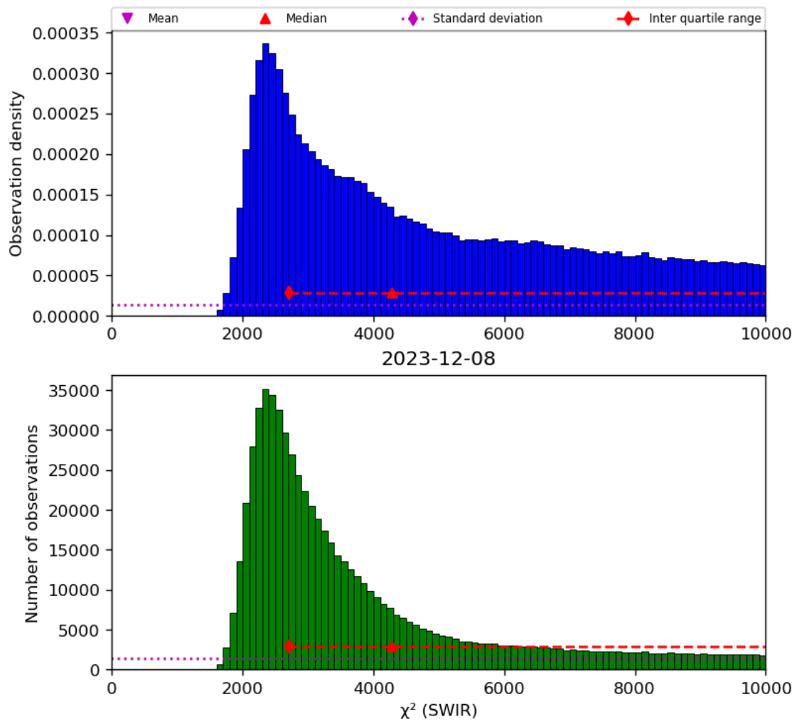
Figure 28: Histogram of “ \chi^2 (SWIR)” for 2023-12-07 to 2023-12-09
