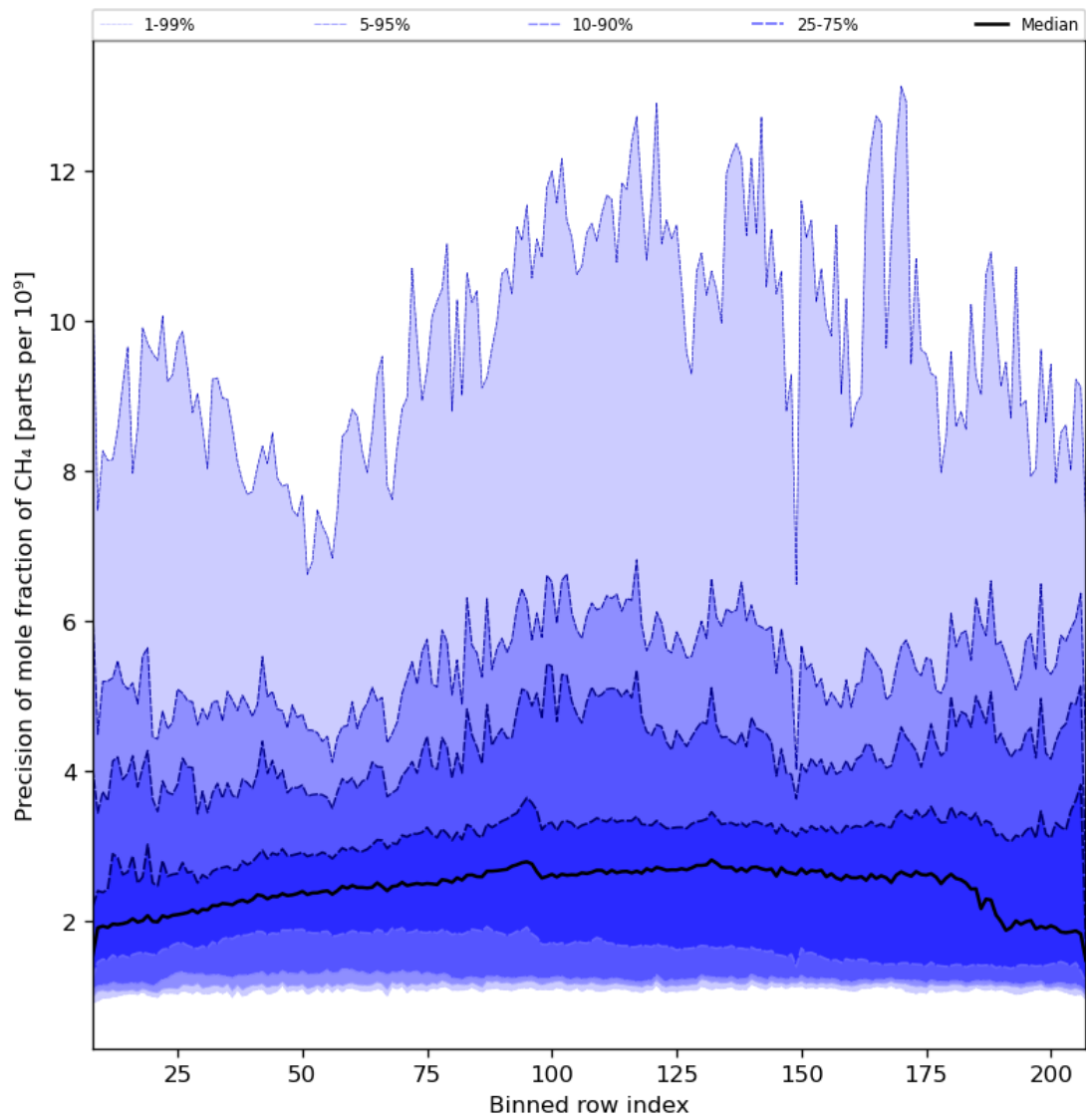
Figure 35: Along track statistics of “Precision of mole fraction of CH 4 ” for 2023-12-07 to 2023-12-09
