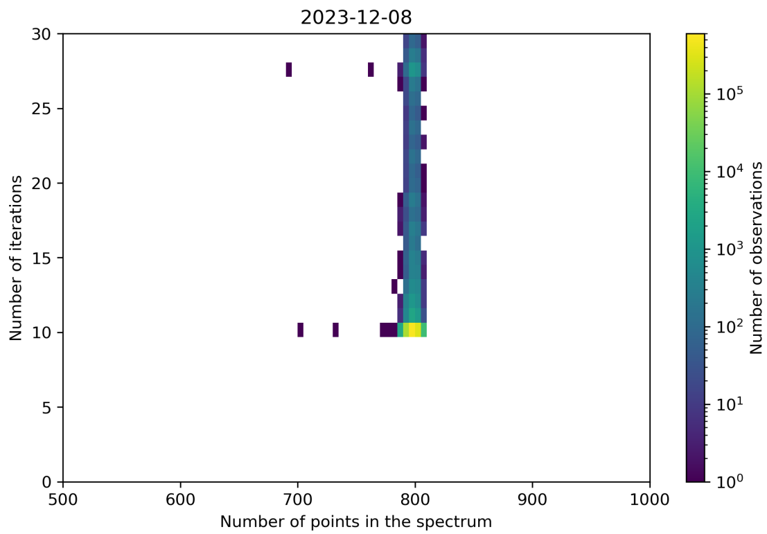
Figure 92: Scatter density plot of “Number of points in the spectrum” against “Number of iterations” for 2023-12-07 to 2023-12-09.
