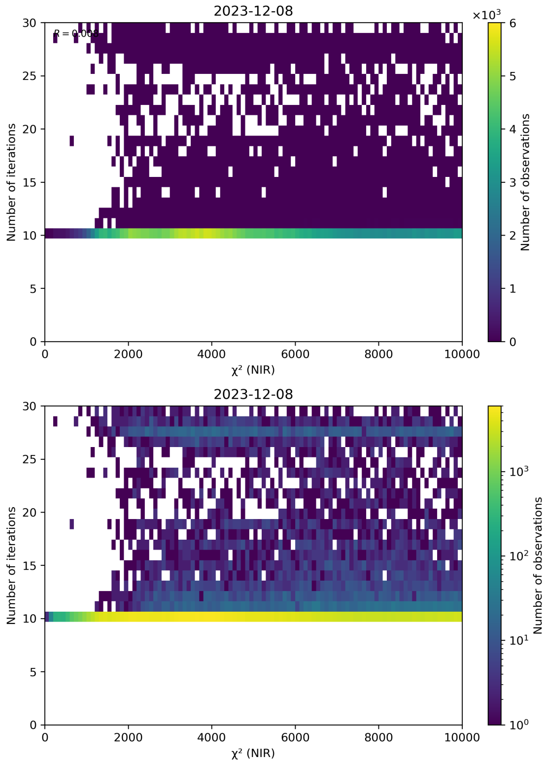
Figure 46: Scatter density plot of “ \chi^2 (NIR)” against “Number of iterations” for 2023-12-07 to 2023-12-09.
