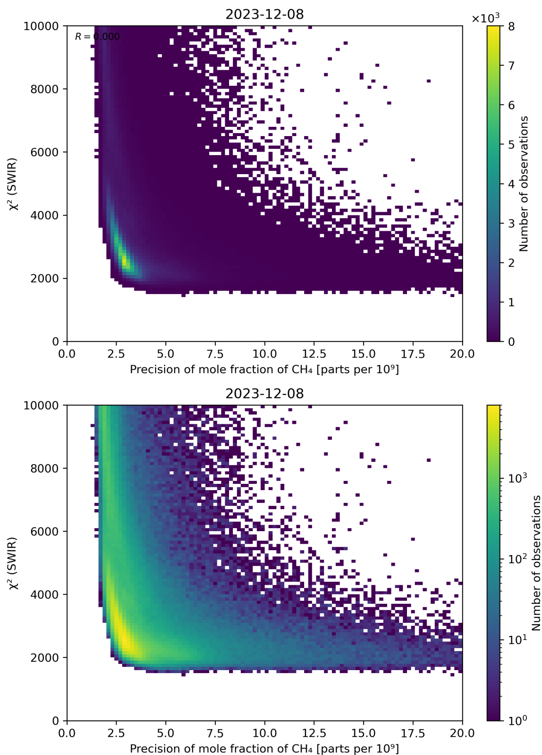
Figure 79: Scatter density plot of “Precision of mole fraction of CH 4 ” against “ \chi^2 (SWIR)” for 2023-12-07 to 2023-12-09.
