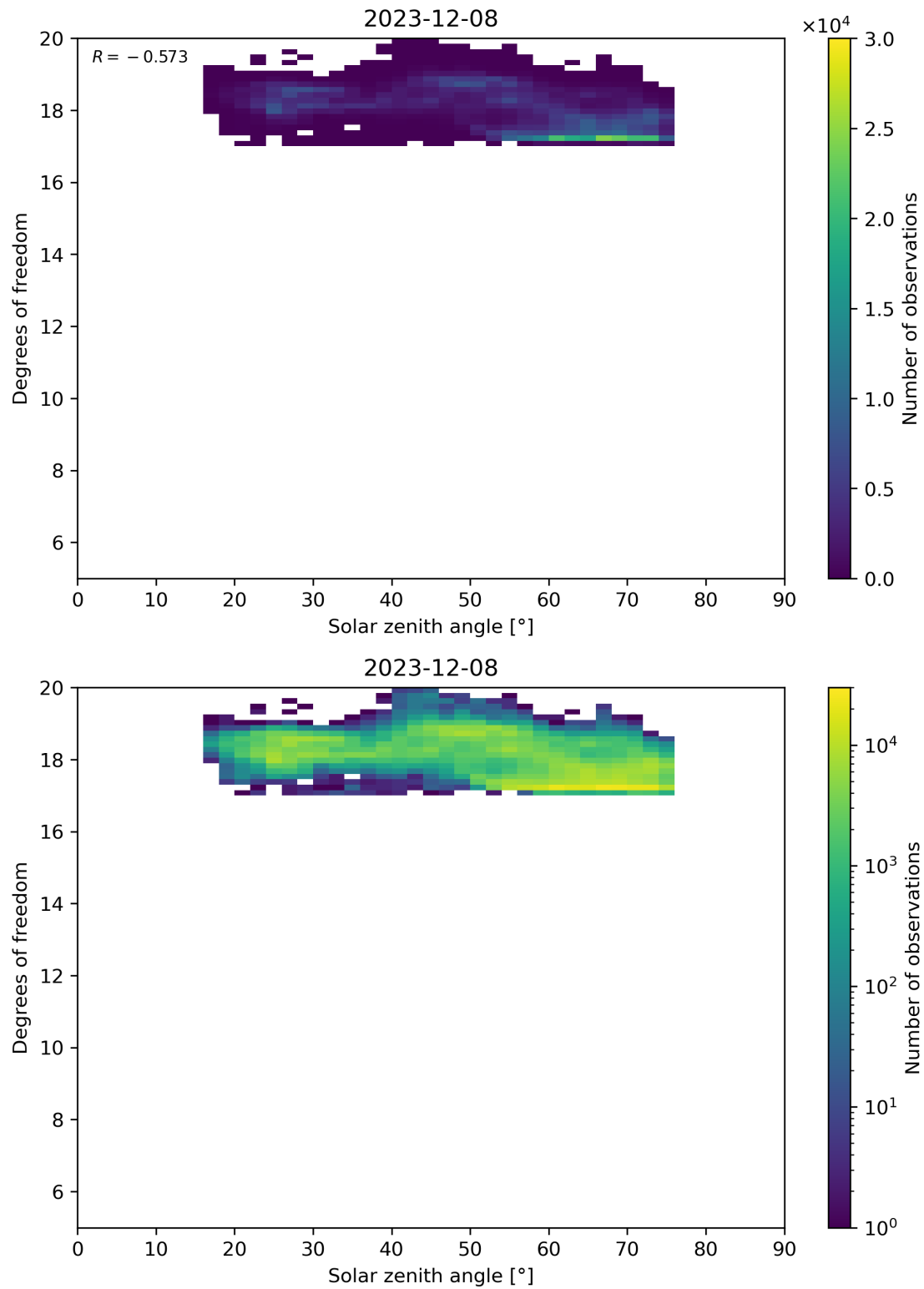
Figure 96: Scatter density plot of “Solar zenith angle” against “Degrees of freedom” for 2023-12-07 to 2023-12-09.
