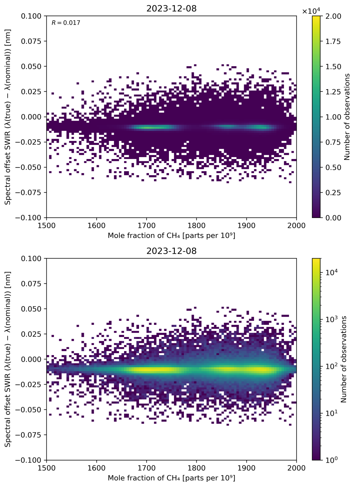
Figure 86: Scatter density plot of “Mole fraction of \text{CH}_4 ” against “Spectral offset SWIR ( \lambda(\text{true}) - \lambda(\text{nominal}) )” for 2023-12-07 to 2023-12-09.
