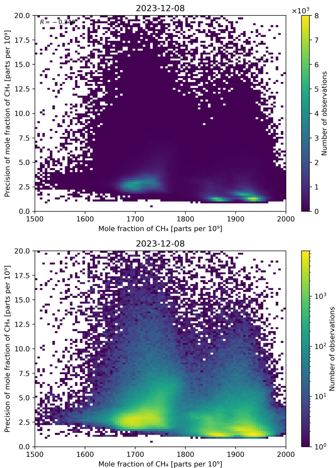
Figure 75: Scatter density plot of “Mole fraction of CH 4 ” against “Precision of mole fraction of CH 4 ” for 2023-12-07 to 2023-12-09.
