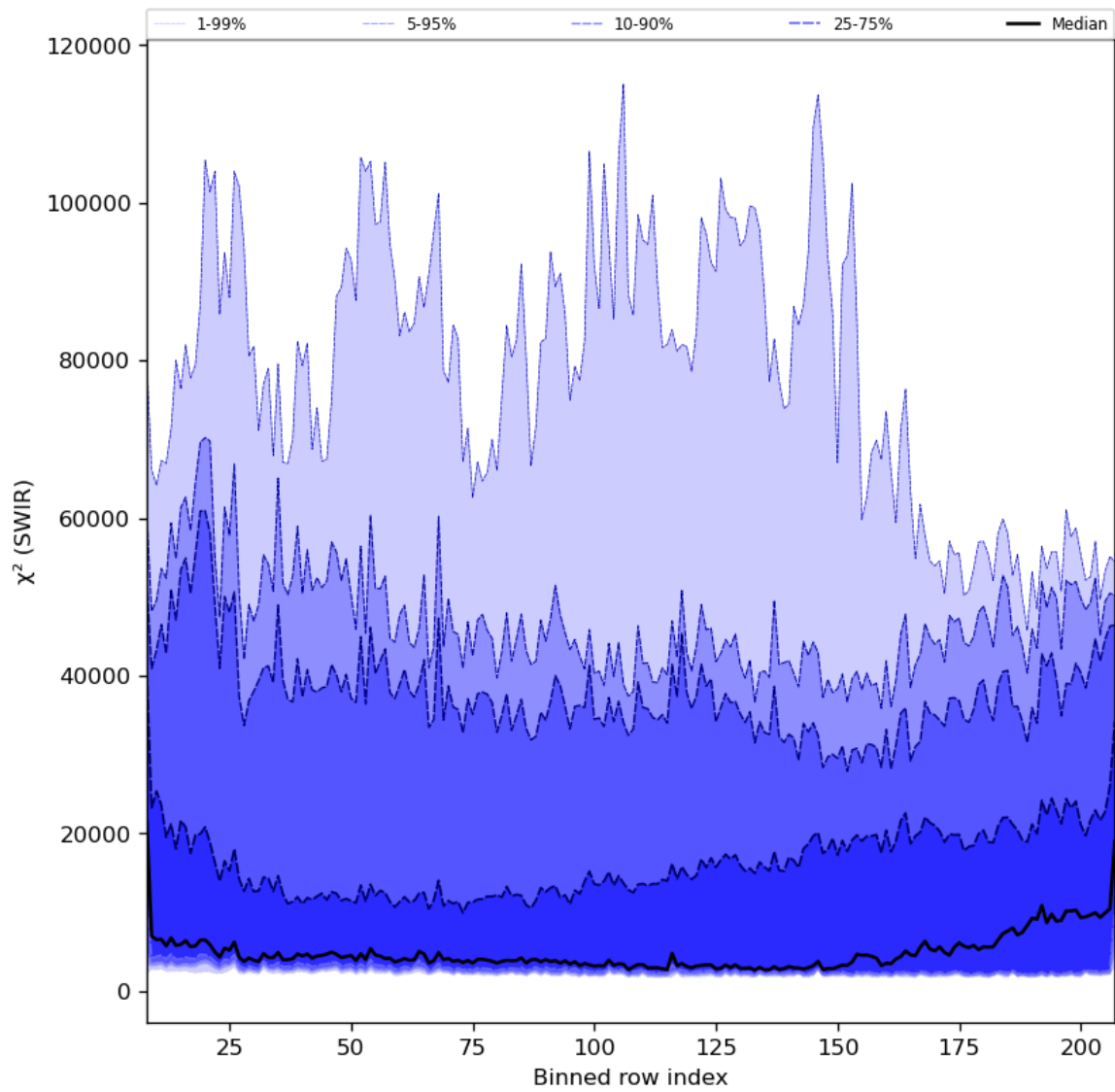
Figure 39: Along track statistics of " \chi^2 (SWIR)" for 2023-12-07 to 2023-12-09
