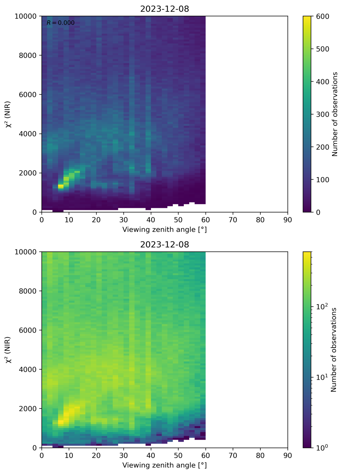
Figure 105: Scatter density plot of “Viewing zenith angle” against “ \chi^2 (NIR)” for 2023-12-07 to 2023-12-09.
