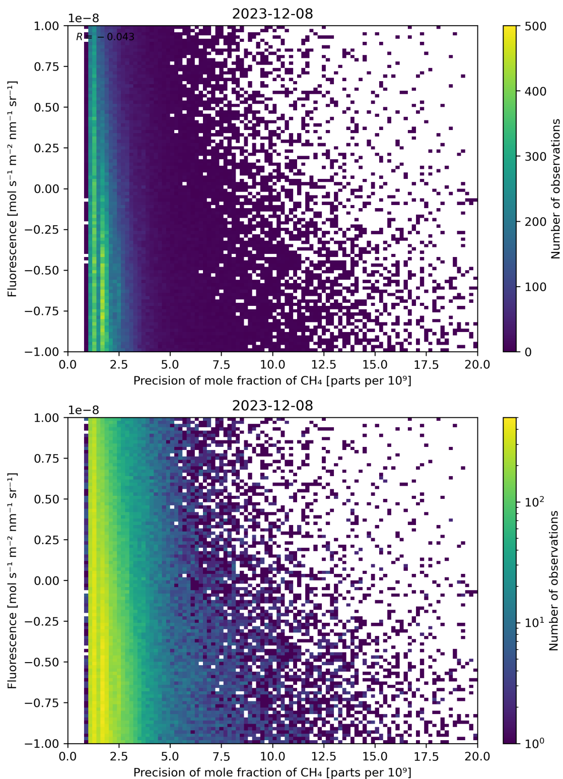
Figure 81: Scatter density plot of “Precision of mole fraction of \text{CH}_4 ” against “Fluorescence” for 2023-12-07 to 2023-12-09.
