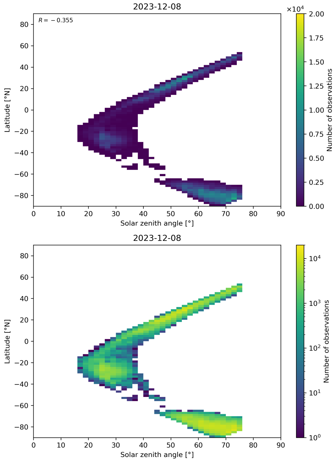
Figure 98: Scatter density plot of “Solar zenith angle” against “Latitude” for 2023-12-07 to 2023-12-09.
