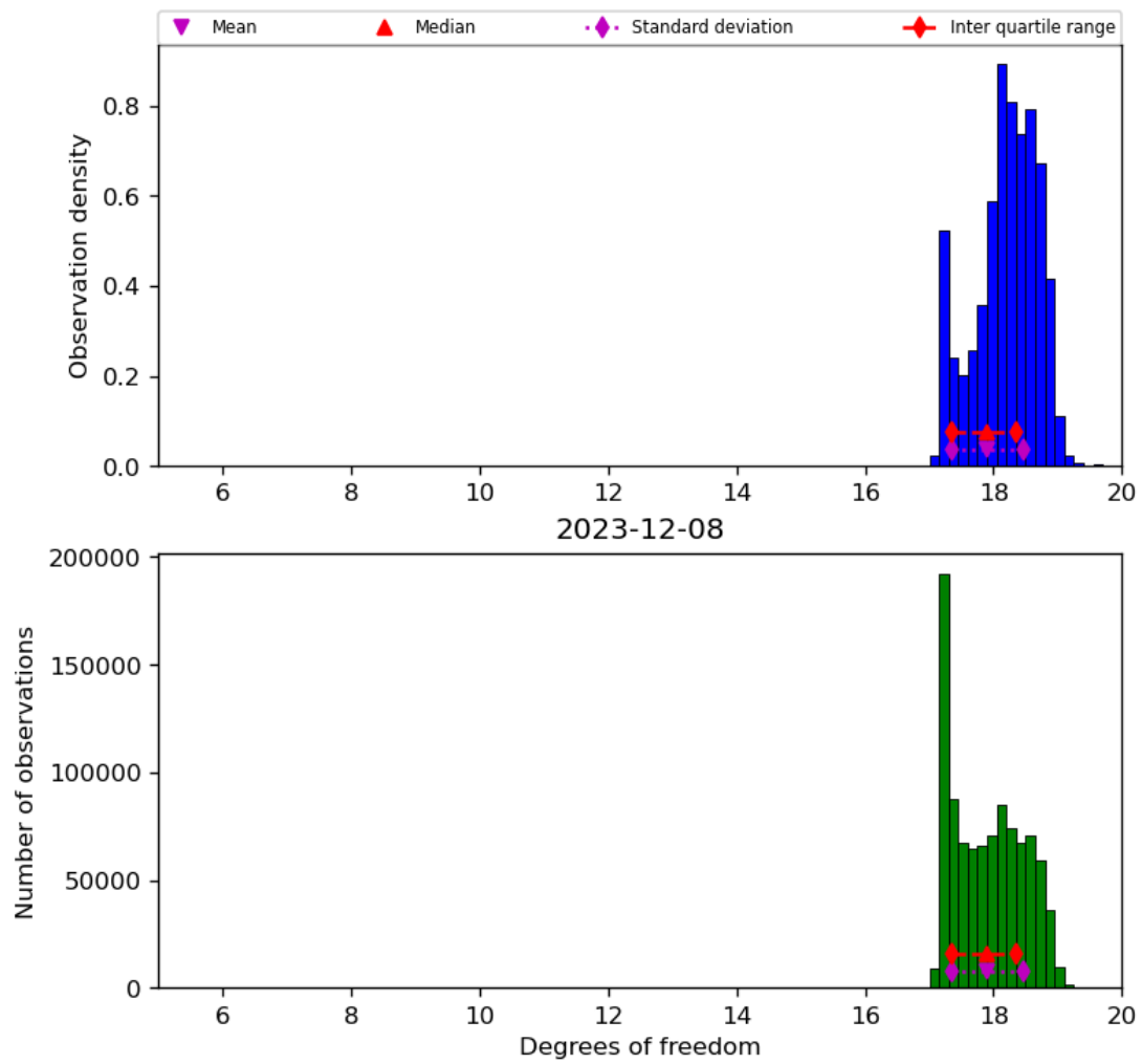
Figure 30: Histogram of “Degrees of freedom” for 2023-12-07 to 2023-12-09
