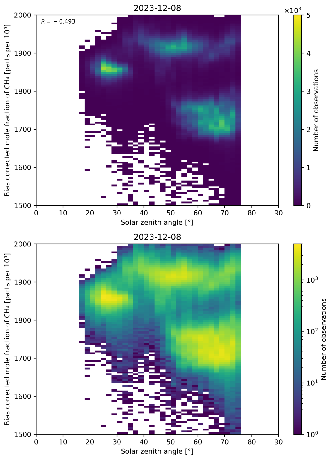
Figure 100: Scatter density plot of “Solar zenith angle” against “Bias corrected mole fraction of \text{CH}_4 ” for 2023-12-07 to 2023-12-09.
