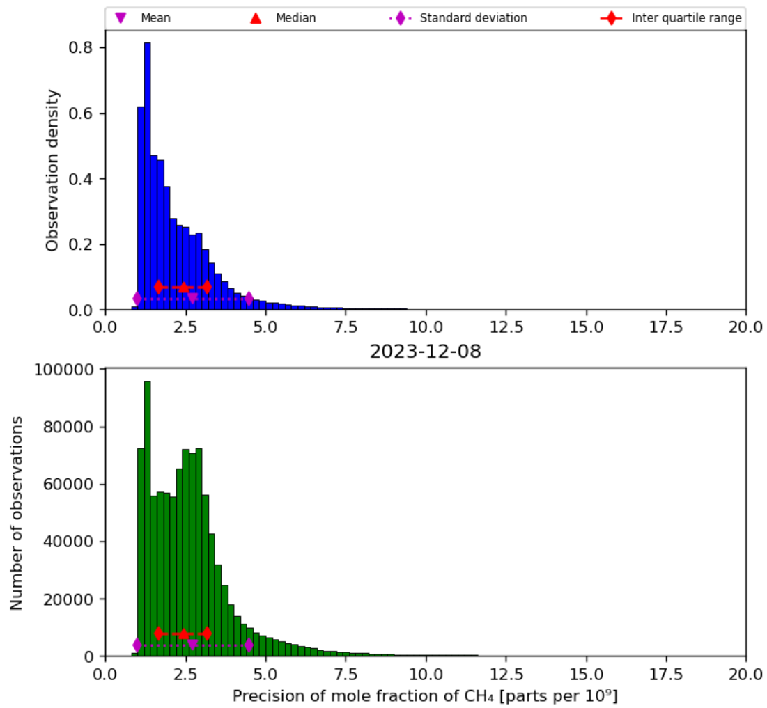
Figure 24: Histogram of “Precision of mole fraction of CH 4 ” for 2023-12-07 to 2023-12-09
