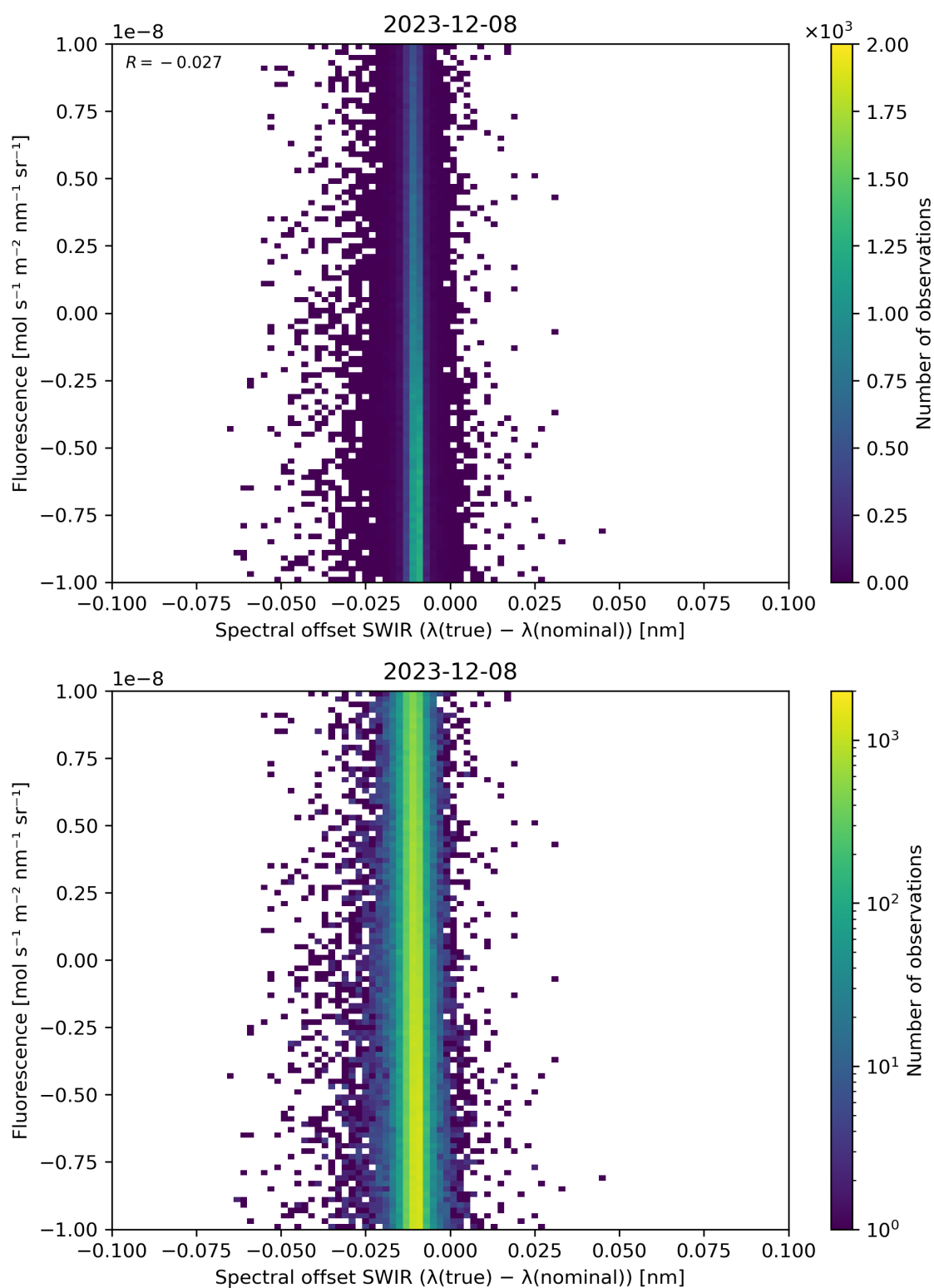
Figure 120: Scatter density plot of “Spectral offset SWIR ( \lambda(\text{true}) - \lambda(\text{nominal}) )” against “Fluorescence” for 2023-12-07 to 2023-12-09.
