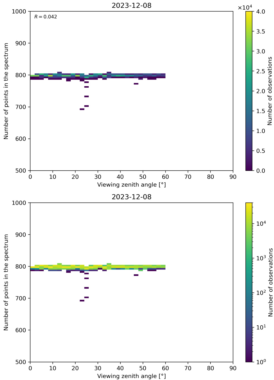
Figure 114: Scatter density plot of “Viewing zenith angle” against “Number of points in the spectrum” for 2023-12-07 to 2023-12-09.
