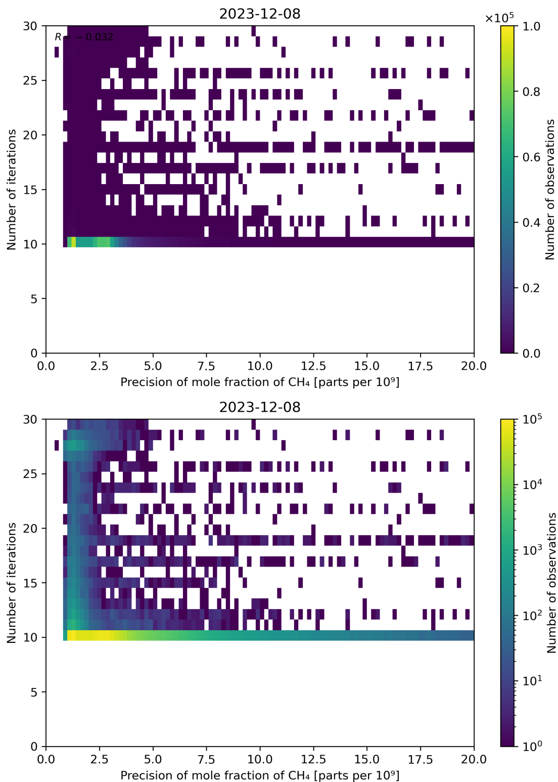
Figure 83: Scatter density plot of “Precision of mole fraction of CH 4 ” against “Number of iterations” for 2023-12-07 to 2023-12-09.
