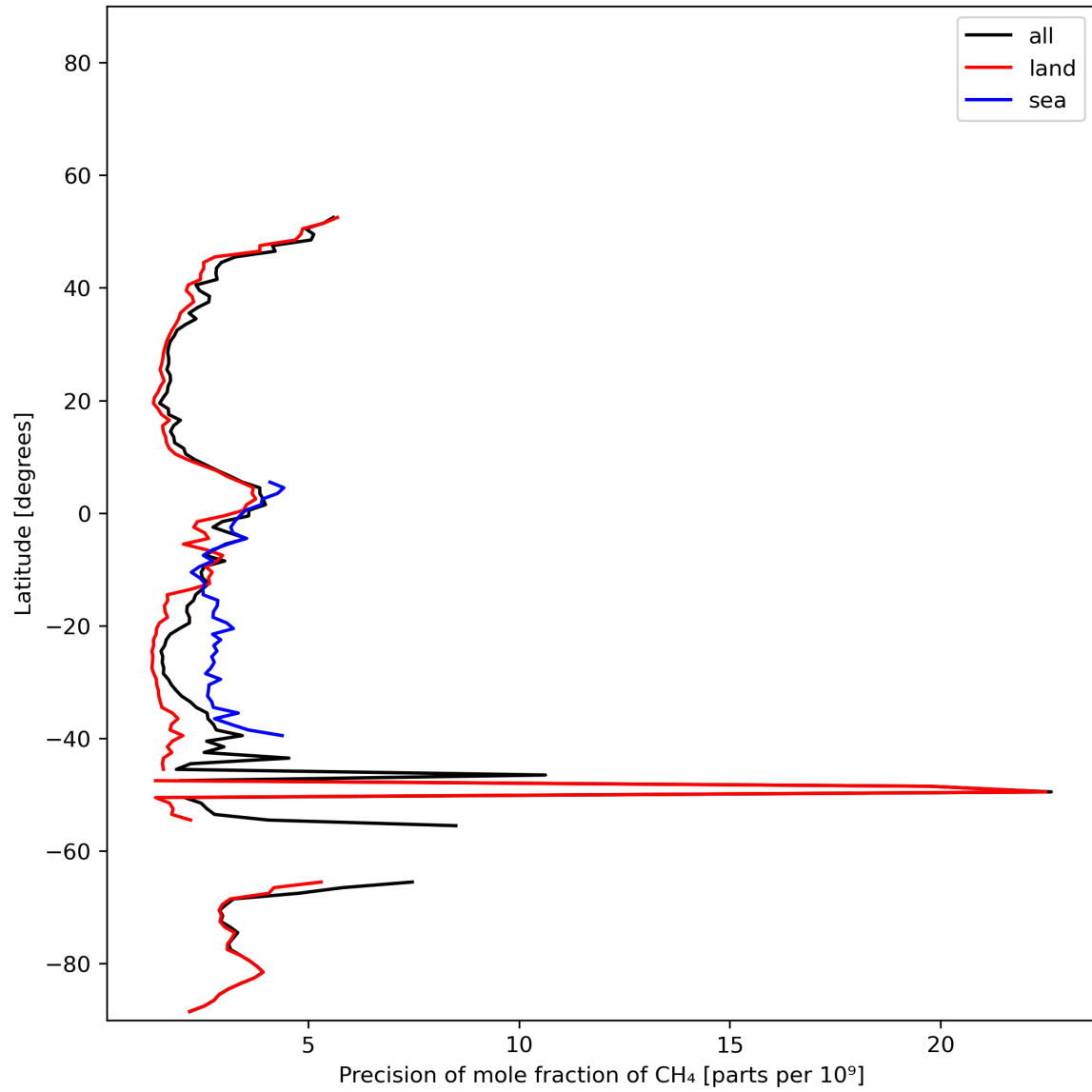
Figure 13: Zonal average of “Precision of mole fraction of CH 4 ” for 2023-12-07 to 2023-12-09.
