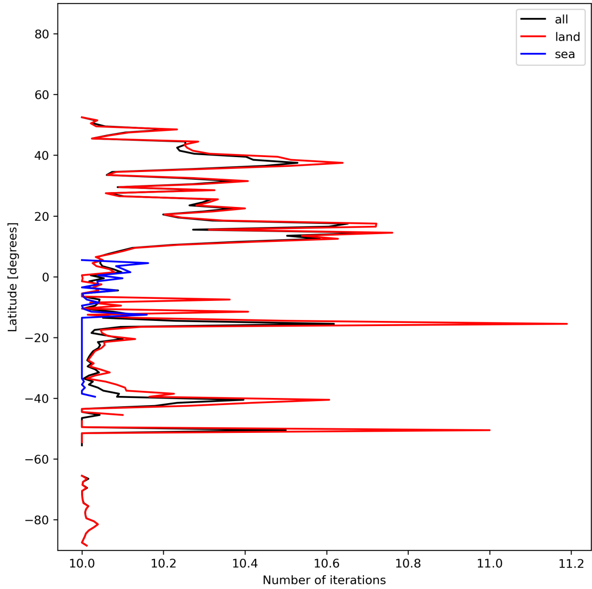
Figure 20: Zonal average of “Number of iterations” for 2023-12-07 to 2023-12-09.
