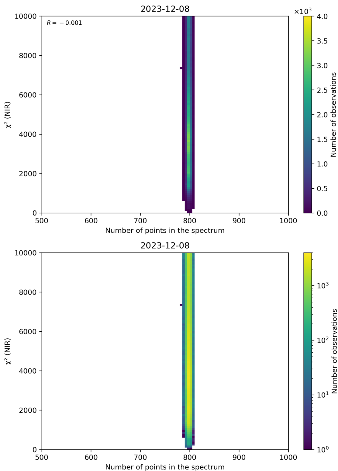
Figure 88: Scatter density plot of “Number of points in the spectrum” against “ \chi^2 (NIR)” for 2023-12-07 to 2023-12-09.
