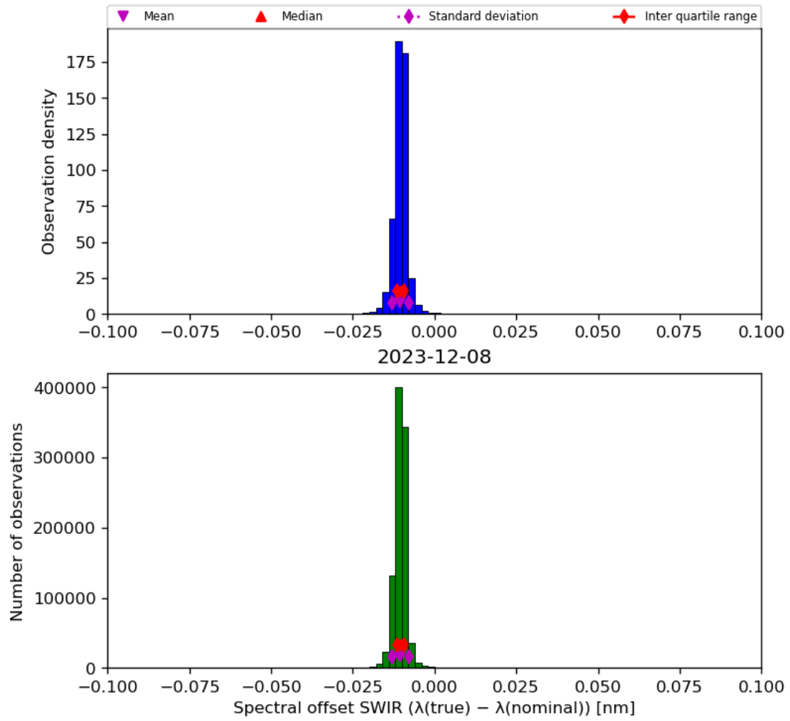
Figure 27: Histogram of “Spectral offset SWIR ( \lambda(\text{true}) - \lambda(\text{nominal}) )” for 2023-12-07 to 2023-12-09
