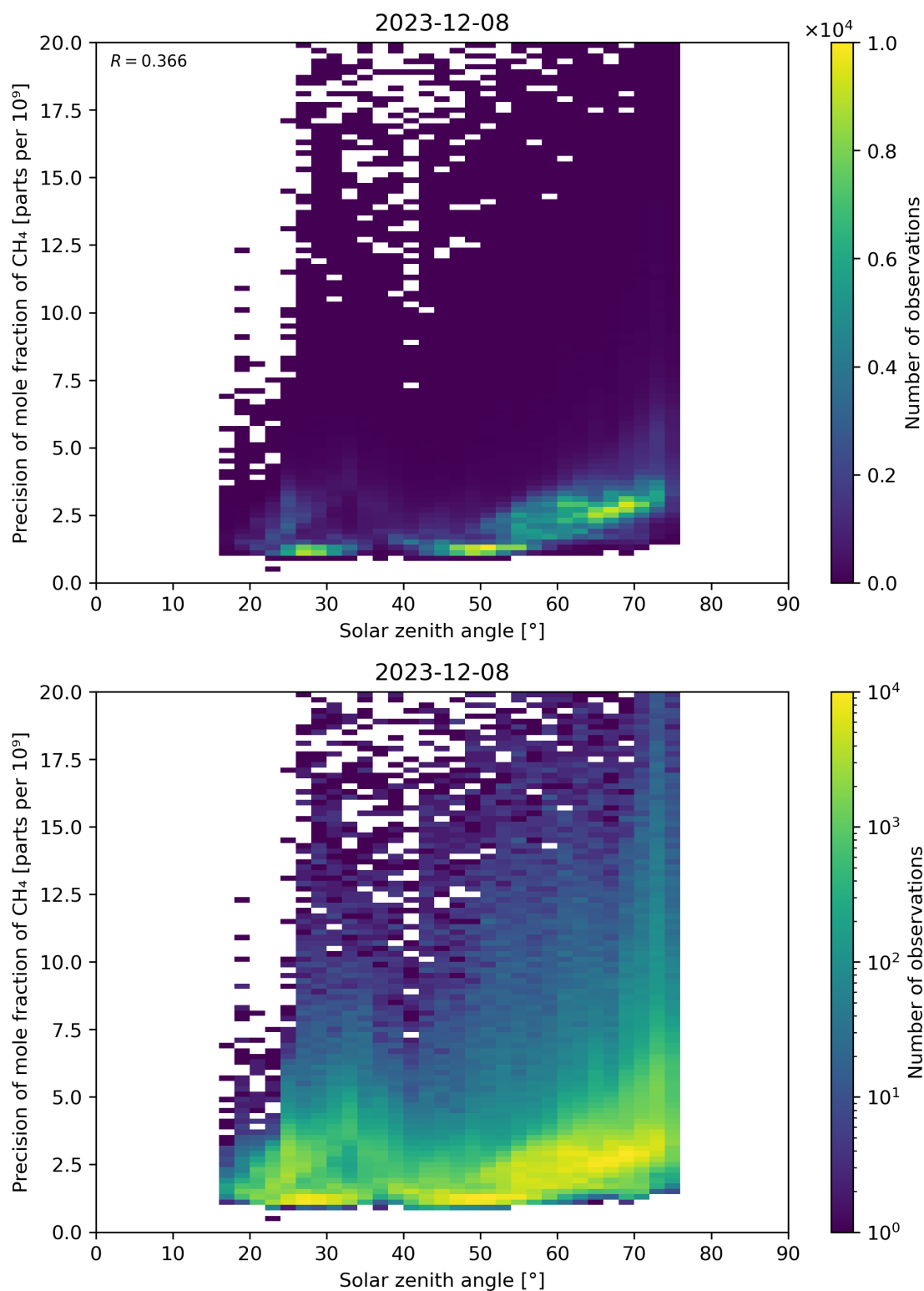
Figure 101: Scatter density plot of “Solar zenith angle” against “Precision of mole fraction of CH 4 ” for 2023-12-07 to 2023-12-09.
