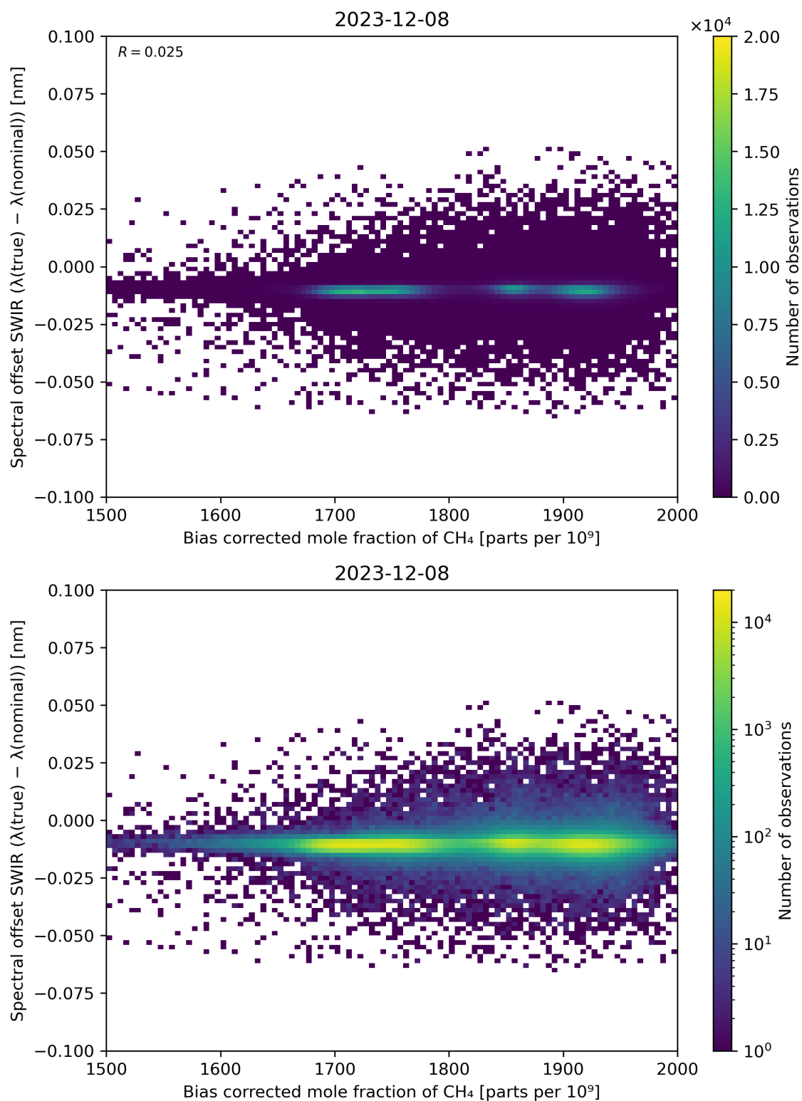
Figure 69: Scatter density plot of “Bias corrected mole fraction of \text{CH}_4 ” against “Spectral offset SWIR ( \lambda(\text{true}) - \lambda(\text{nominal}) )” for 2023-12-07 to 2023-12-09.
