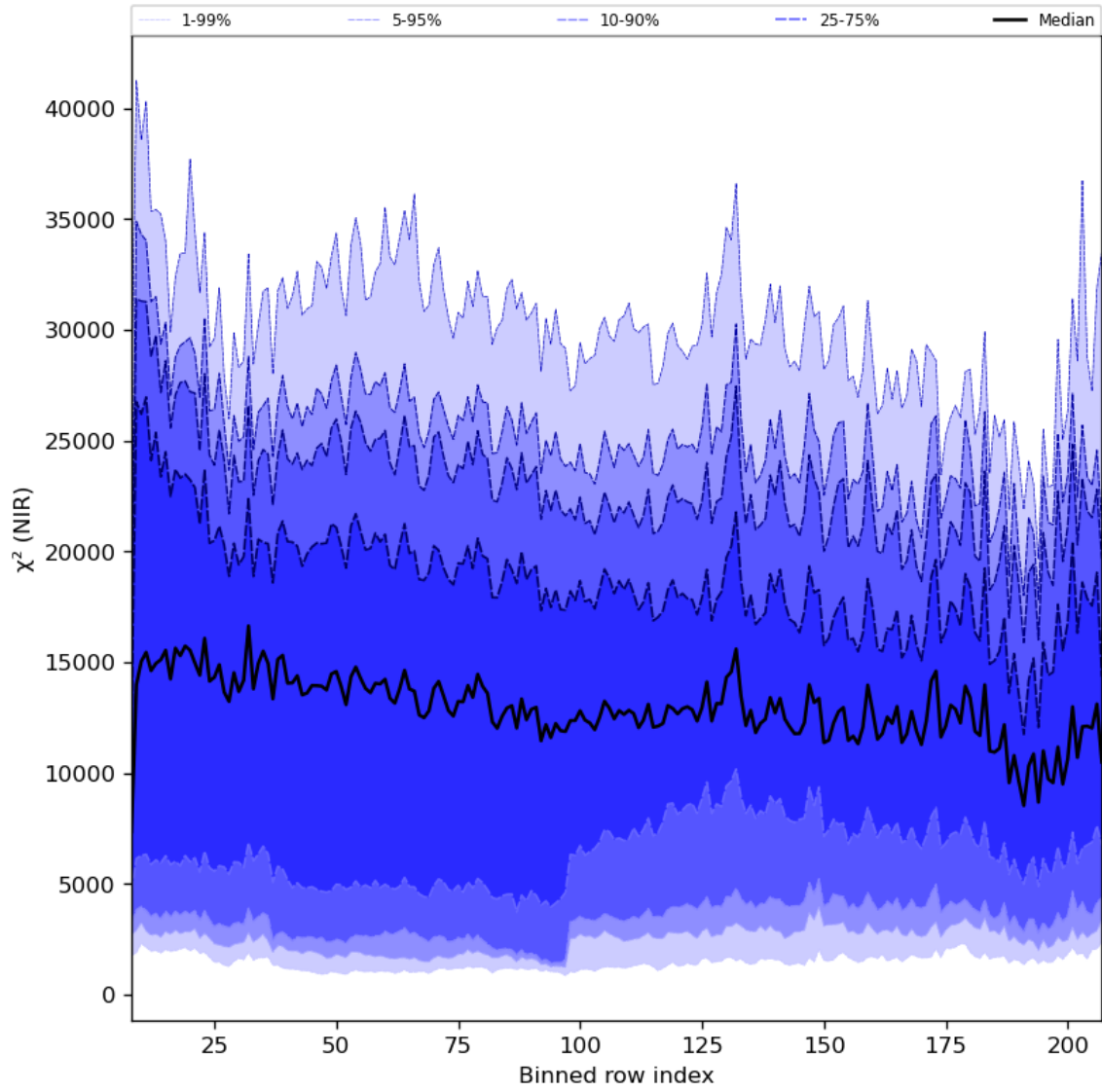
Figure 40: Along track statistics of “ \chi^2 (NIR)” for 2023-12-07 to 2023-12-09
