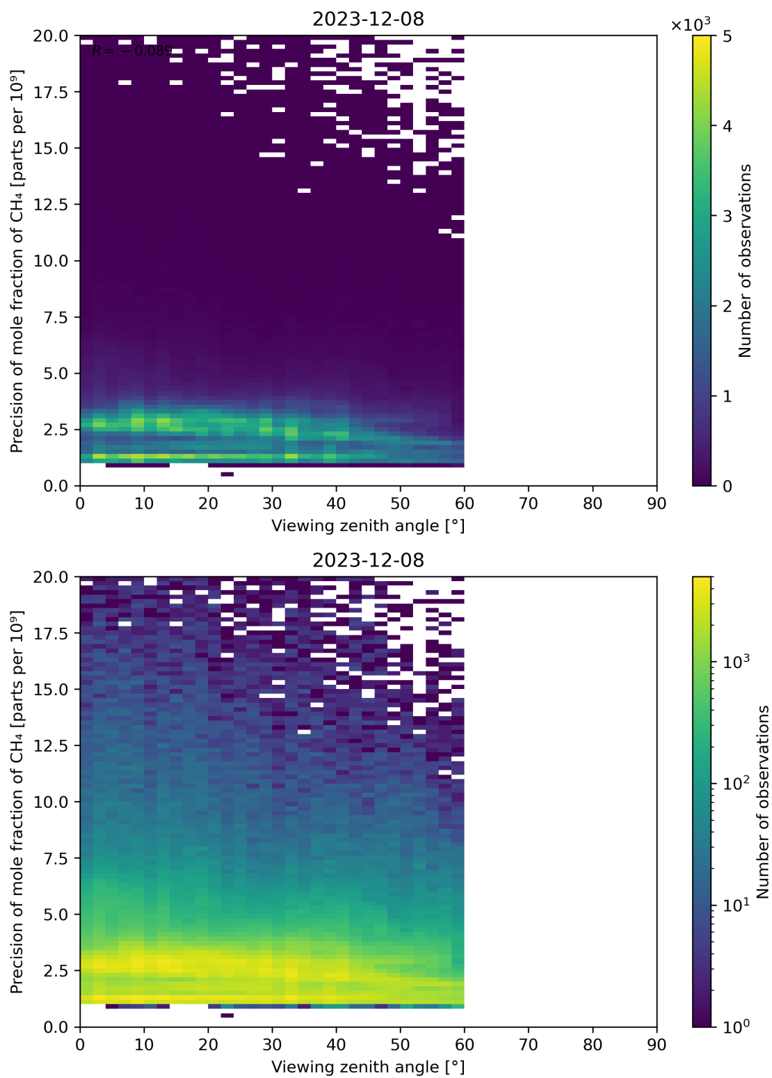
Figure 112: Scatter density plot of “Viewing zenith angle” against “Precision of mole fraction of CH 4 ” for 2023-12-07 to 2023-12-09.
