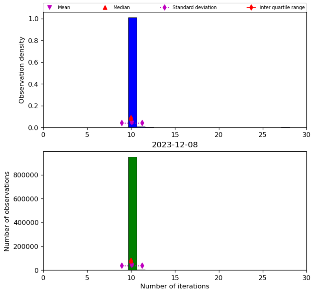
Figure 31: Histogram of “Number of iterations” for 2023-12-07 to 2023-12-09
