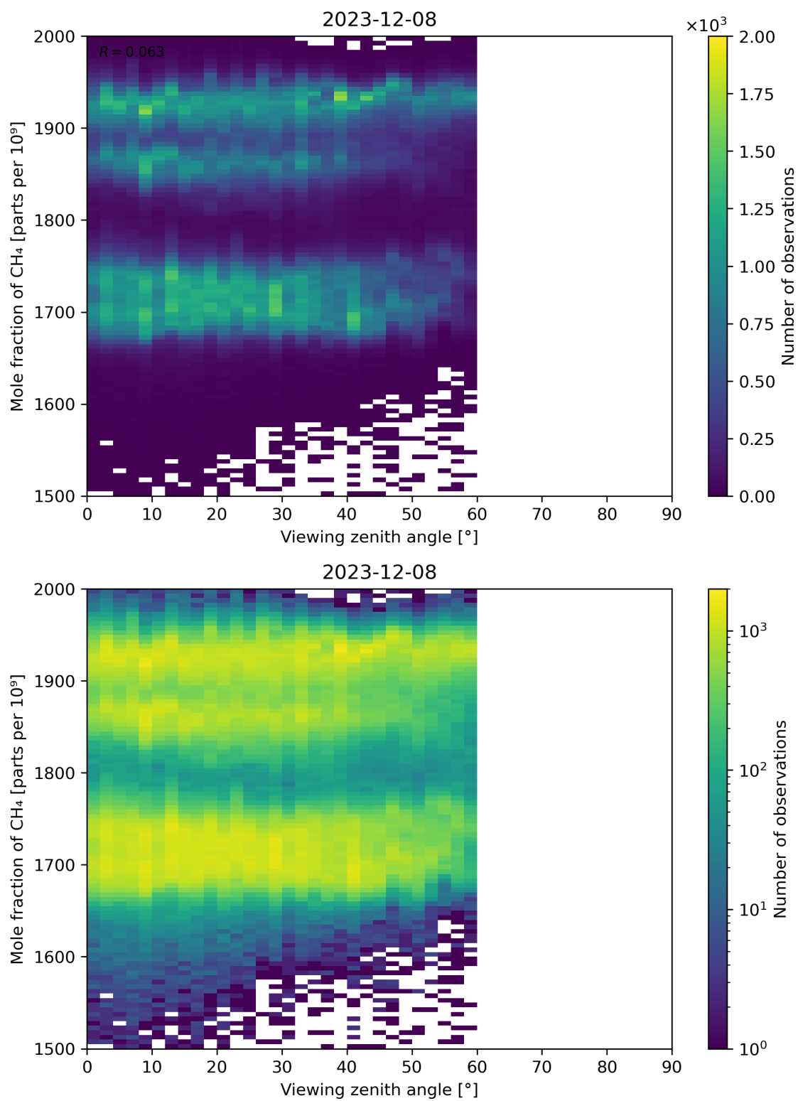
Figure 110: Scatter density plot of “Viewing zenith angle” against “Mole fraction of CH 4 ” for 2023-12-07 to 2023-12-09.
