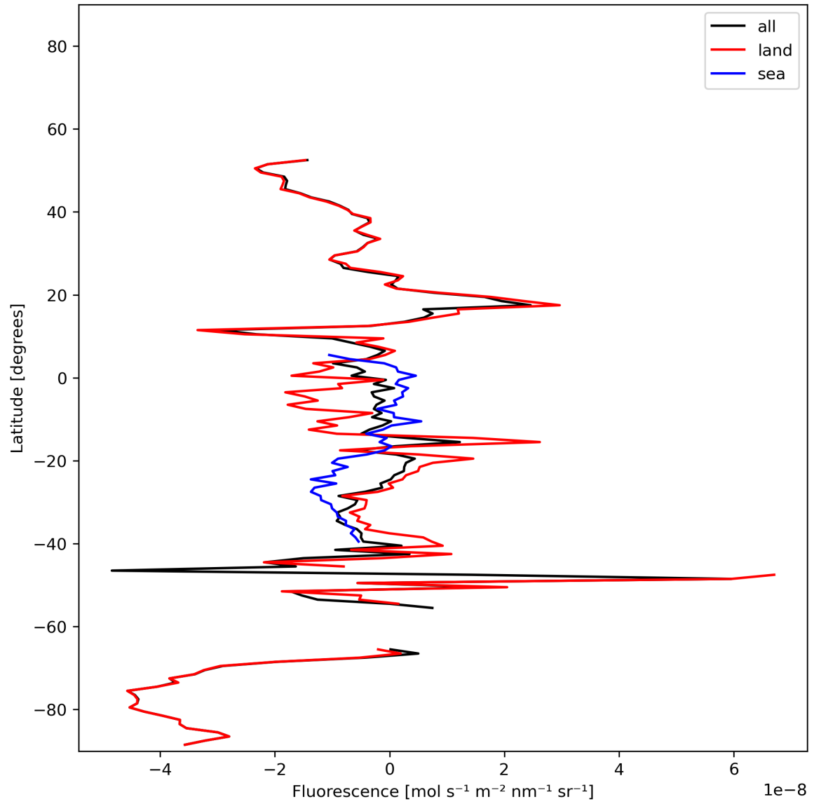
Figure 21: Zonal average of “Fluorescence” for 2023-12-07 to 2023-12-09.
