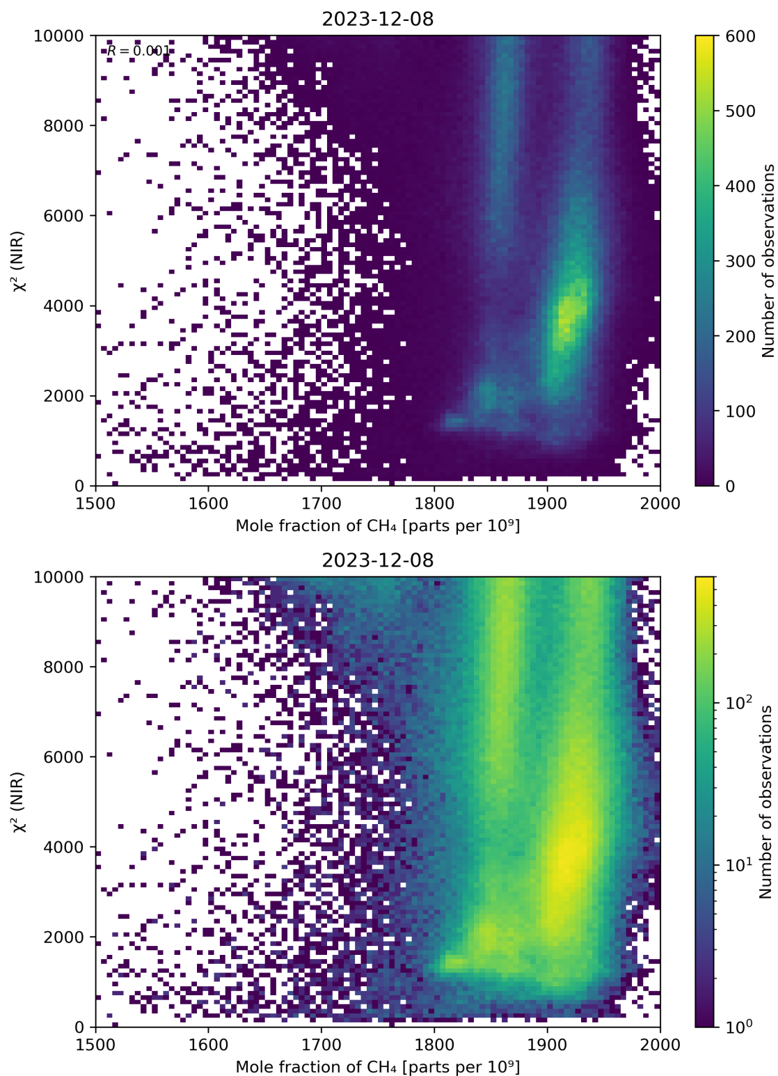
Figure 70: Scatter density plot of “Mole fraction of \text{CH}_4 ” against “ \chi^2 (NIR)” for 2023-12-07 to 2023-12-09.
