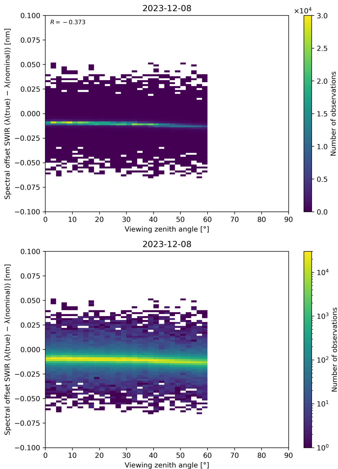
Figure 116: Scatter density plot of “Viewing zenith angle” against “Spectral offset SWIR ( \lambda(\text{true}) - \lambda(\text{nominal}) )” for 2023-12-07 to 2023-12-09.
