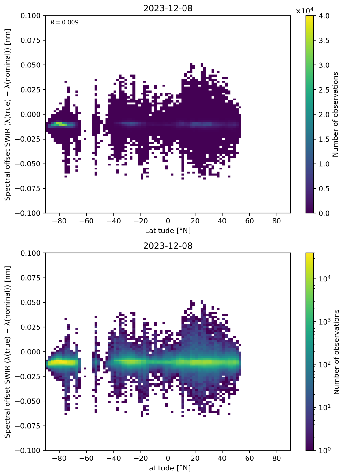
Figure 62: Scatter density plot of “Latitude” against “Spectral offset SWIR ( \lambda(\text{true}) - \lambda(\text{nominal}) )” for 2023-12-07 to 2023-12-09.
