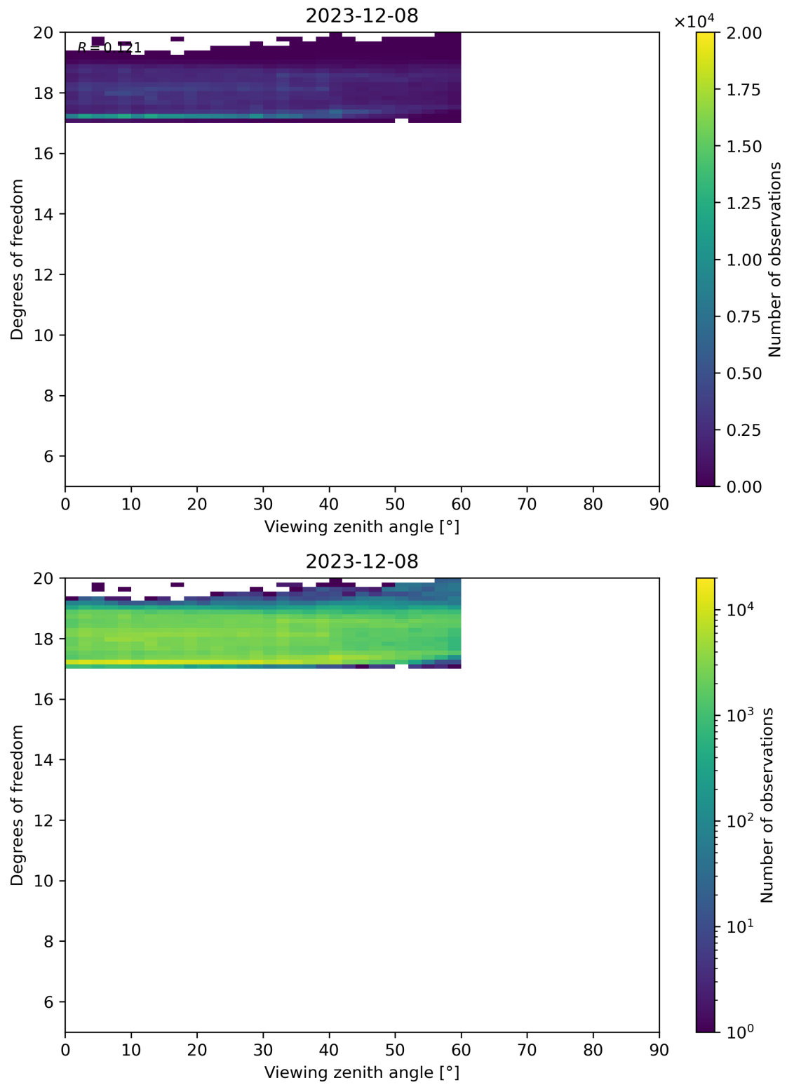
Figure 107: Scatter density plot of “Viewing zenith angle” against “Degrees of freedom” for 2023-12-07 to 2023-12-09.
