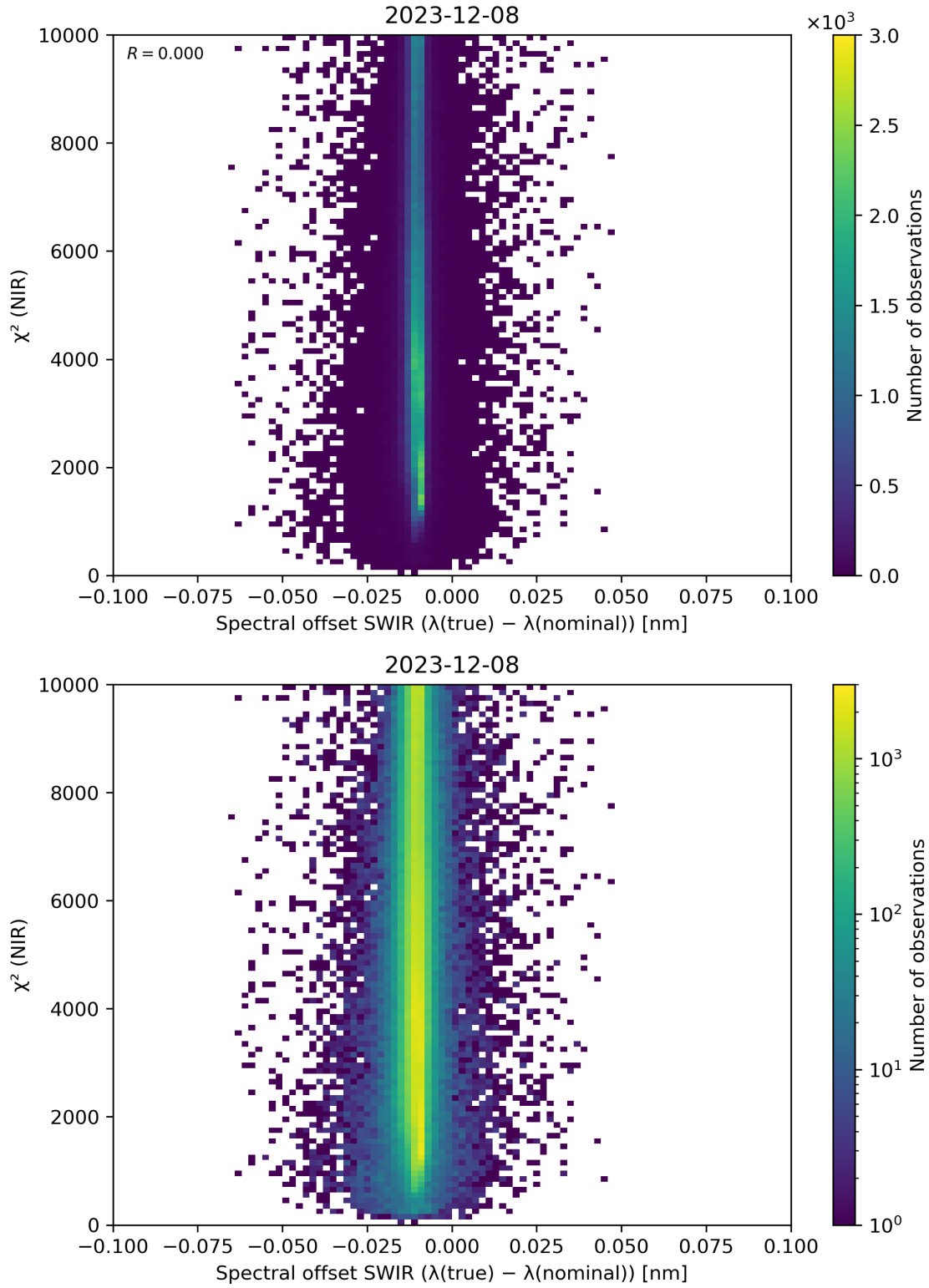
Figure 117: Scatter density plot of “Spectral offset SWIR ( \lambda(\text{true}) - \lambda(\text{nominal}) )” against “ \chi^2 (NIR)” for 2023-12-07 to 2023-12-09.
