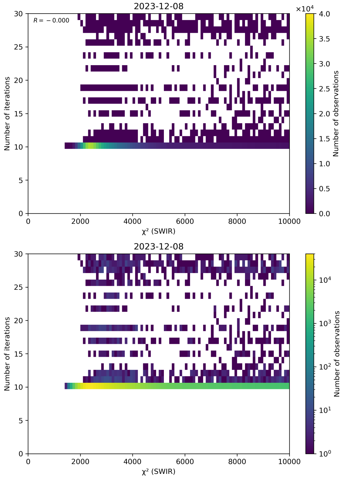
Figure 50: Scatter density plot of “ \chi^2 (SWIR)” against “Number of iterations” for 2023-12-07 to 2023-12-09.
