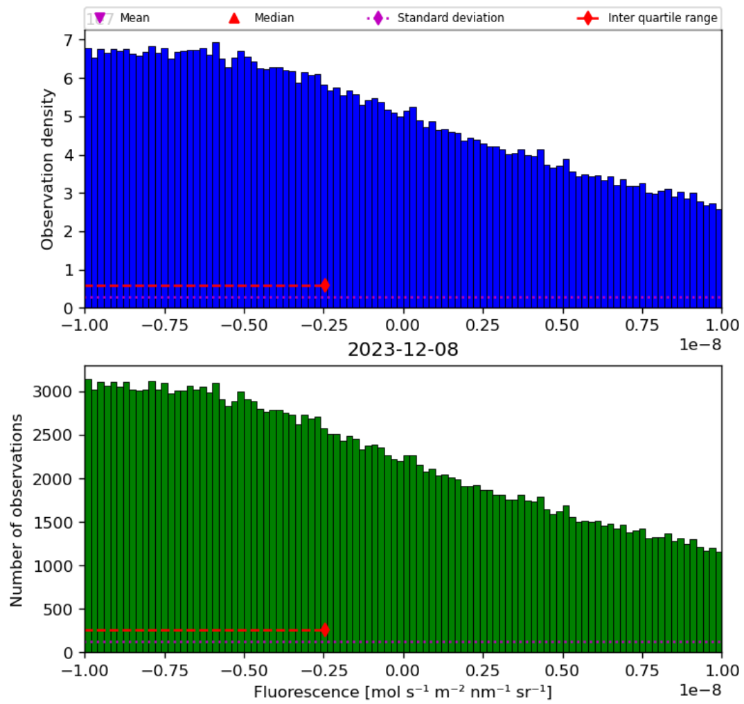
Figure 32: Histogram of “Fluorescence” for 2023-12-07 to 2023-12-09
