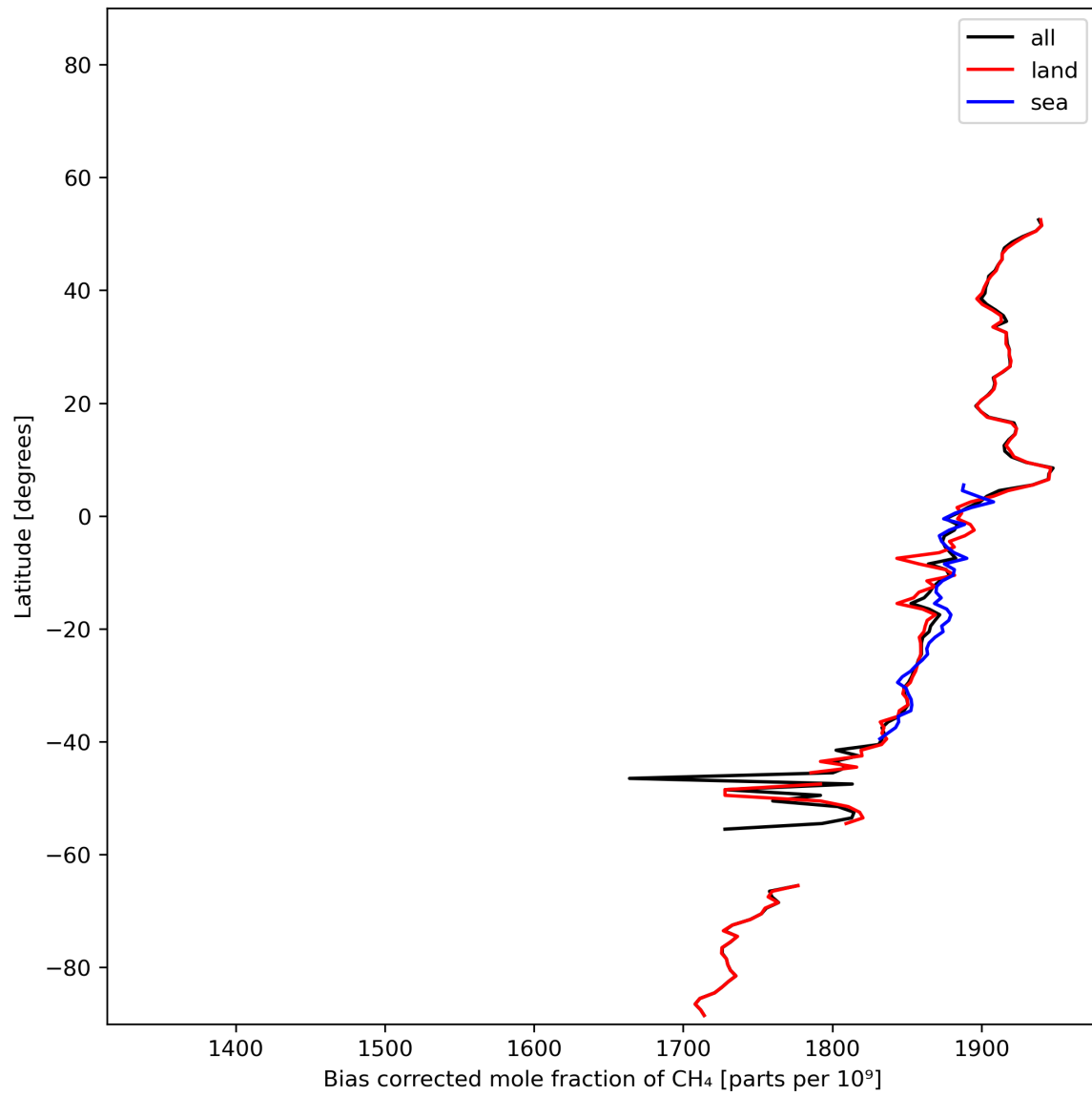
Figure 14: Zonal average of “Bias corrected mole fraction of CH 4 ” for 2023-12-07 to 2023-12-09.
