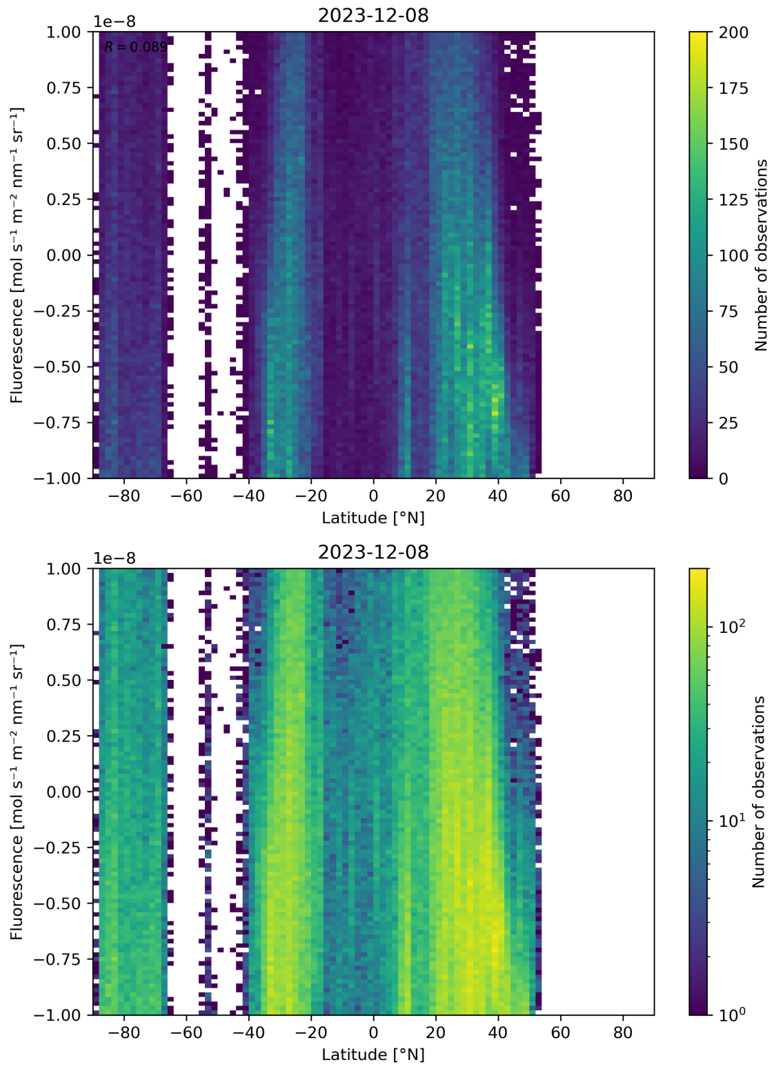
Figure 56: Scatter density plot of “Latitude” against “Fluorescence” for 2023-12-07 to 2023-12-09.
