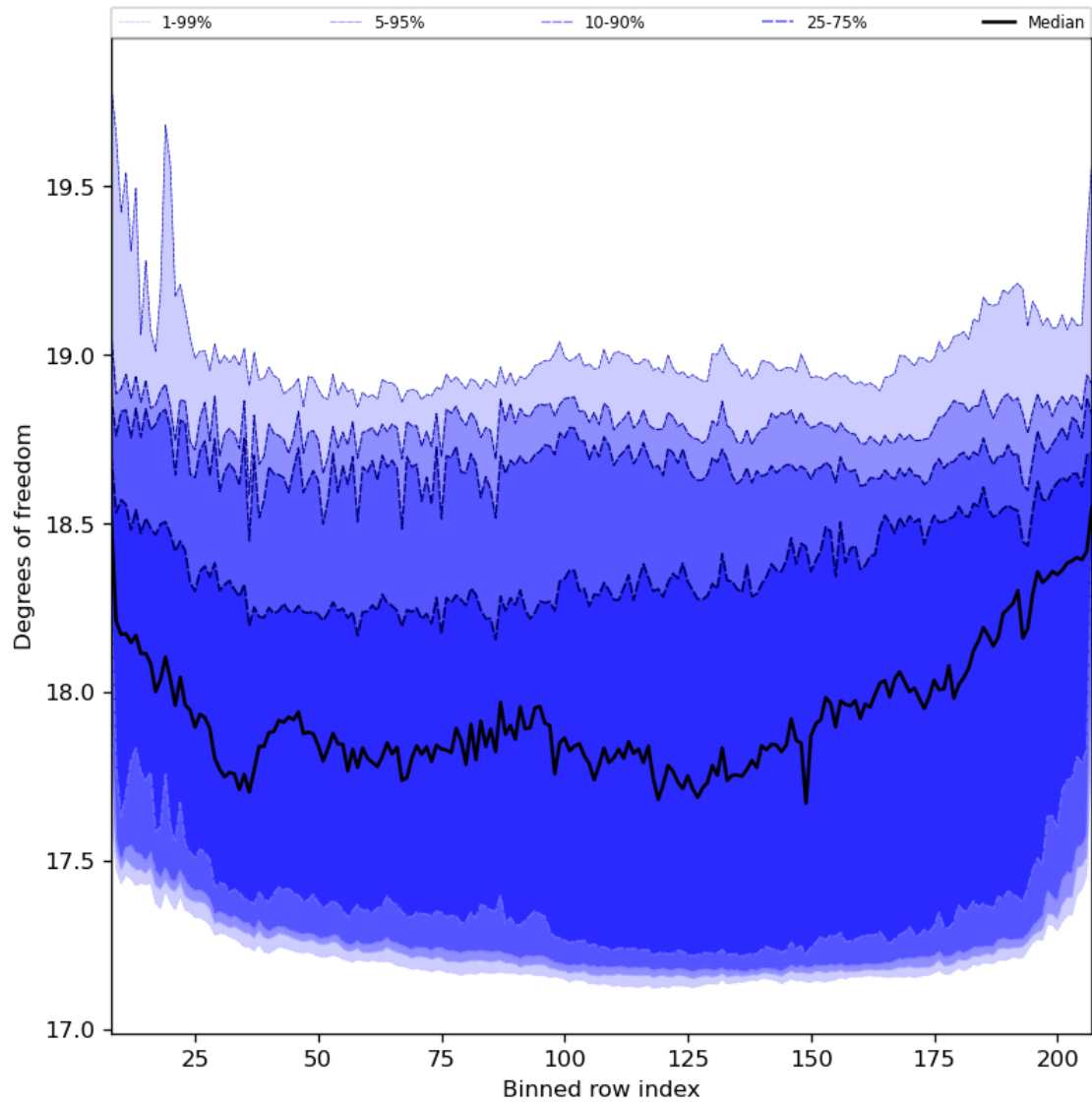
Figure 41: Along track statistics of “Degrees of freedom” for 2023-12-07 to 2023-12-09
