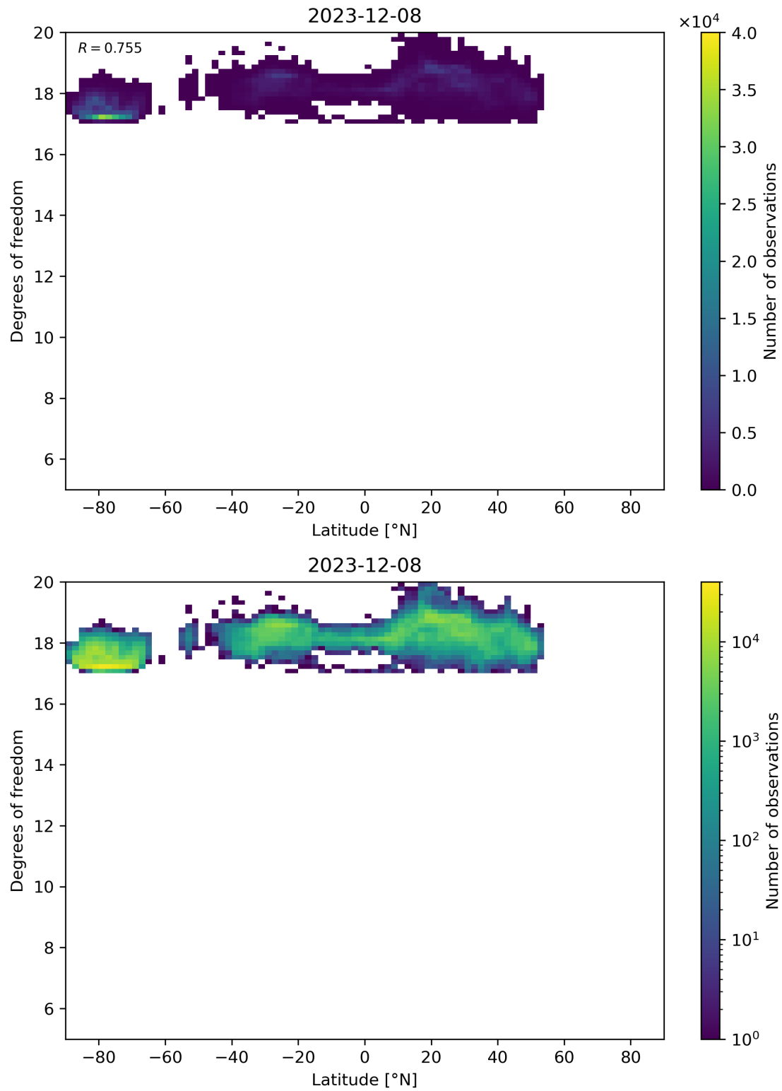
Figure 55: Scatter density plot of “Latitude” against “Degrees of freedom” for 2023-12-07 to 2023-12-09.
