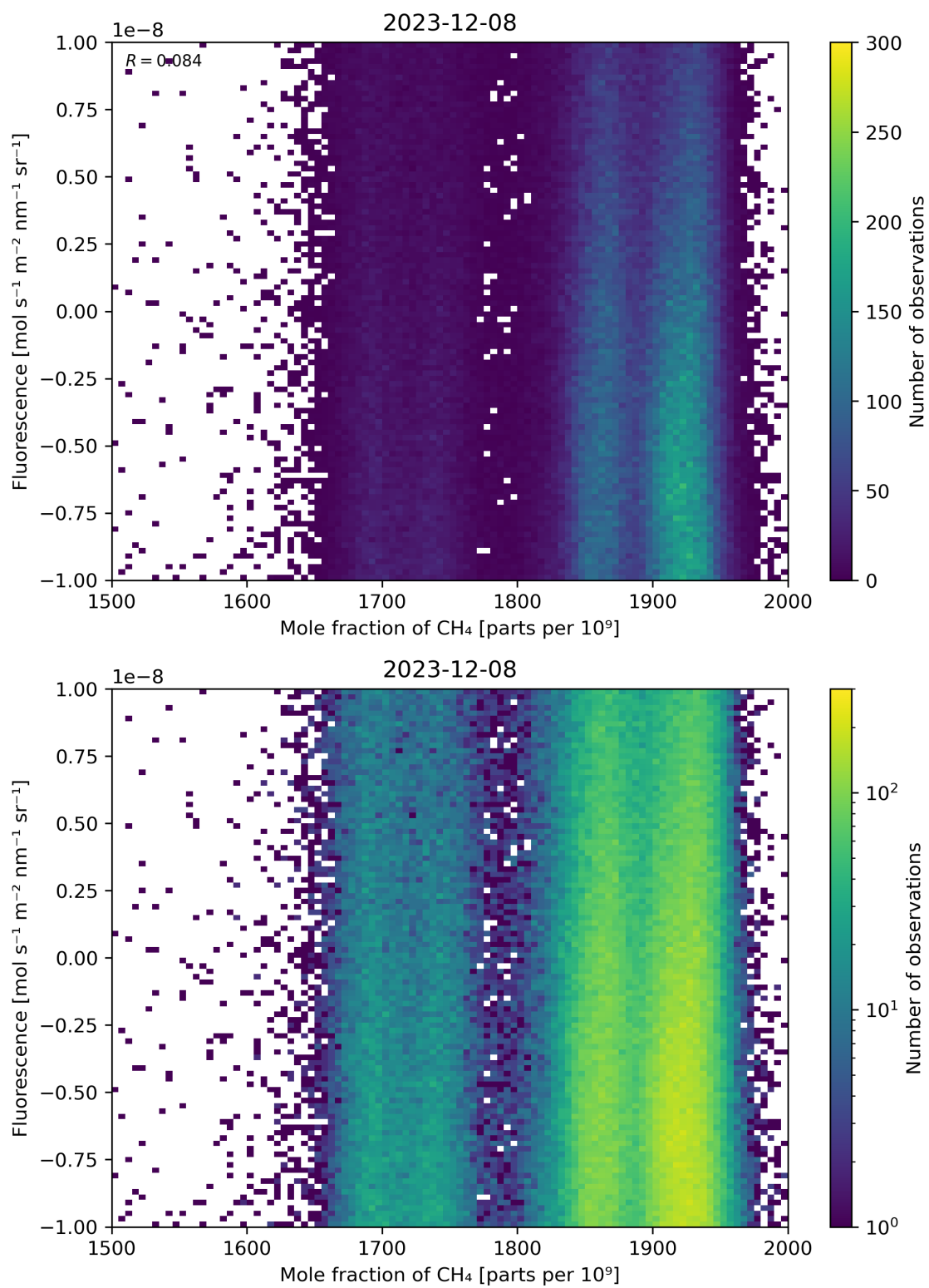
Figure 73: Scatter density plot of “Mole fraction of \text{CH}_4 ” against “Fluorescence” for 2023-12-07 to 2023-12-09.
