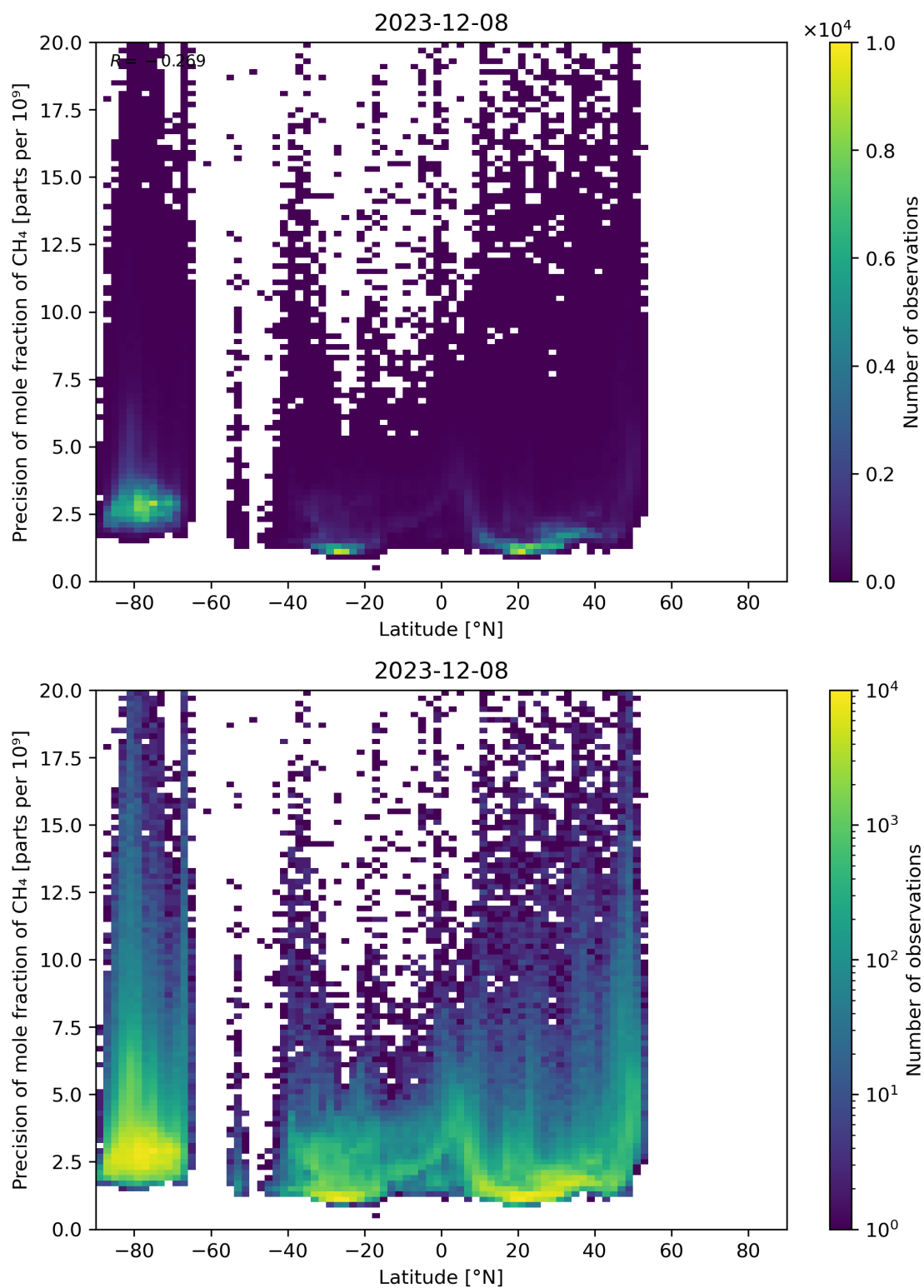
Figure 59: Scatter density plot of “Latitude” against “Precision of mole fraction of CH 4 ” for 2023-12-07 to 2023-12-09.
