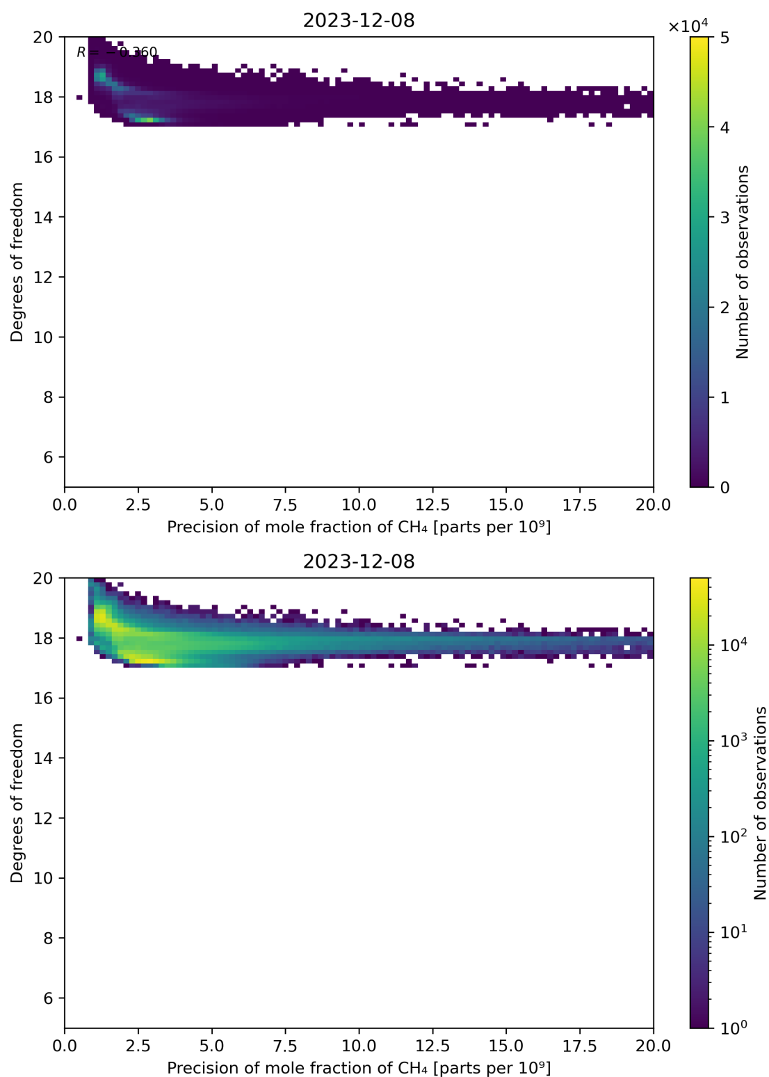
Figure 80: Scatter density plot of “Precision of mole fraction of CH 4 ” against “Degrees of freedom” for 2023-12-07 to 2023-12-09.
