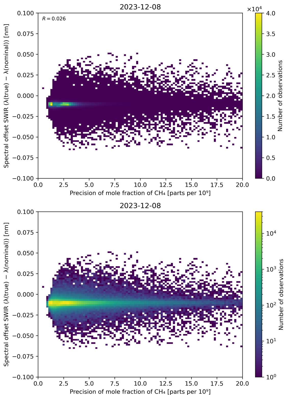
Figure 85: Scatter density plot of “Precision of mole fraction of \text{CH}_4 ” against “Spectral offset SWIR ( \lambda(\text{true}) - \lambda(\text{nominal}) )” for 2023-12-07 to 2023-12-09.
