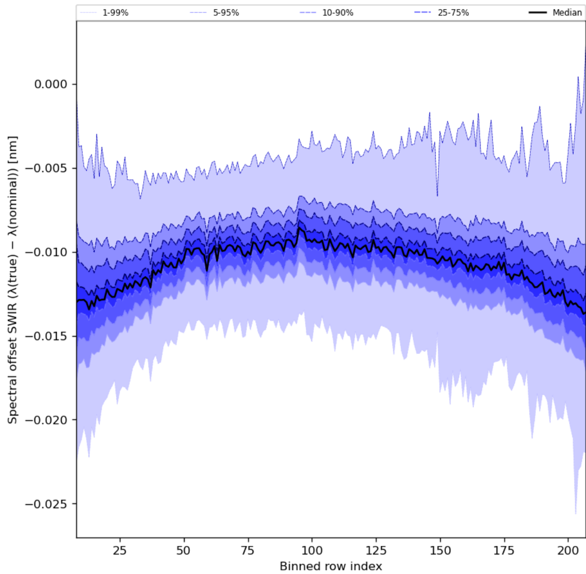
Figure 38: Along track statistics of “Spectral offset SWIR ( \lambda(\text{true}) - \lambda(\text{nominal}) )” for 2023-12-07 to 2023-12-09
