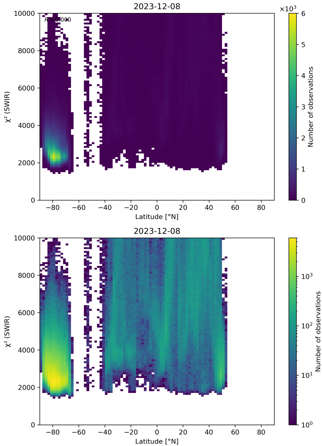
Figure 54: Scatter density plot of “Latitude” against “ \chi^2 (SWIR)” for 2023-12-07 to 2023-12-09.
