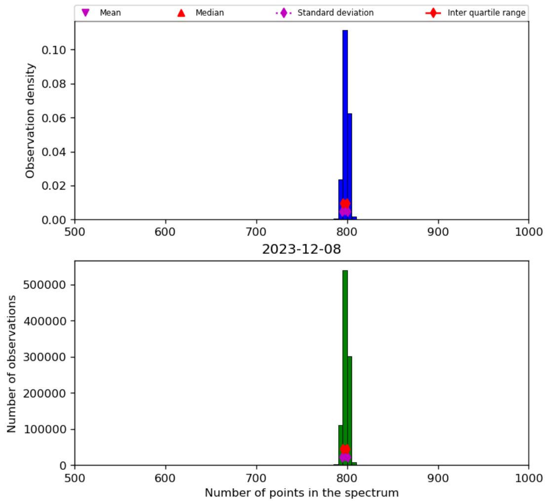
Figure 26: Histogram of “Number of points in the spectrum” for 2023-12-07 to 2023-12-09
