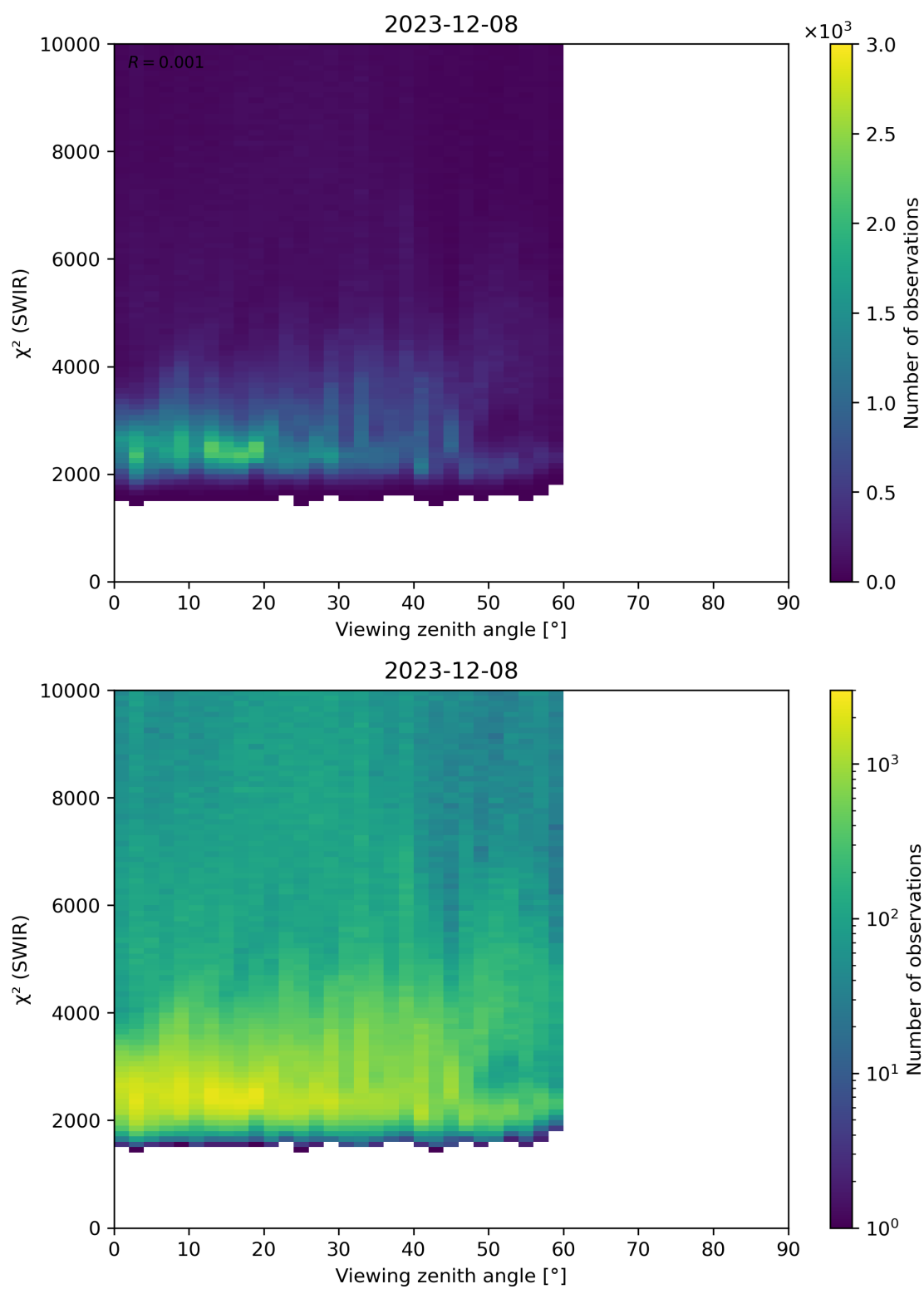
Figure 106: Scatter density plot of “Viewing zenith angle” against “ \chi^2 (SWIR)” for 2023-12-07 to 2023-12-09.
