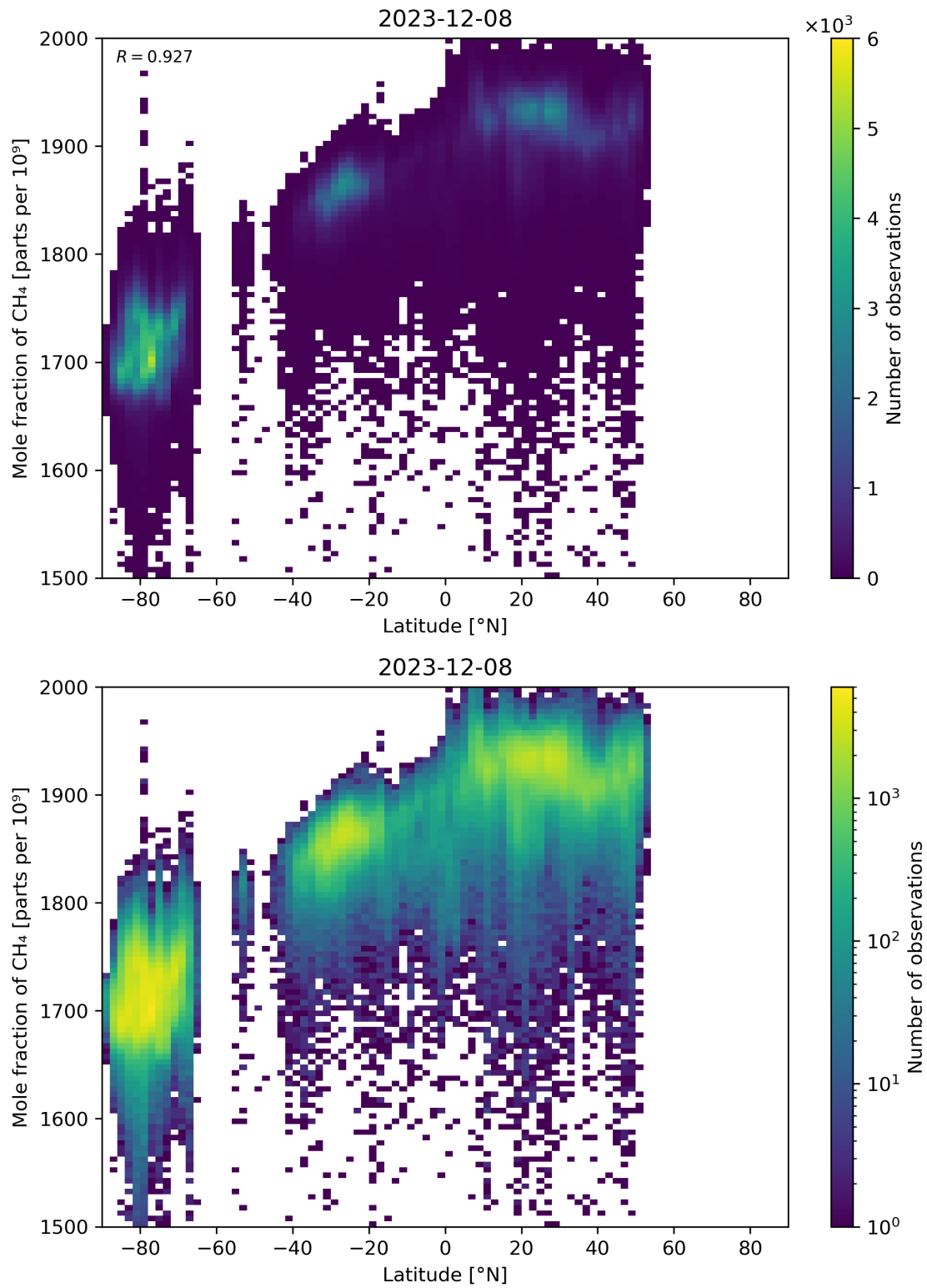
Figure 57: Scatter density plot of “Latitude” against “Mole fraction of CH 4 ” for 2023-12-07 to 2023-12-09.
