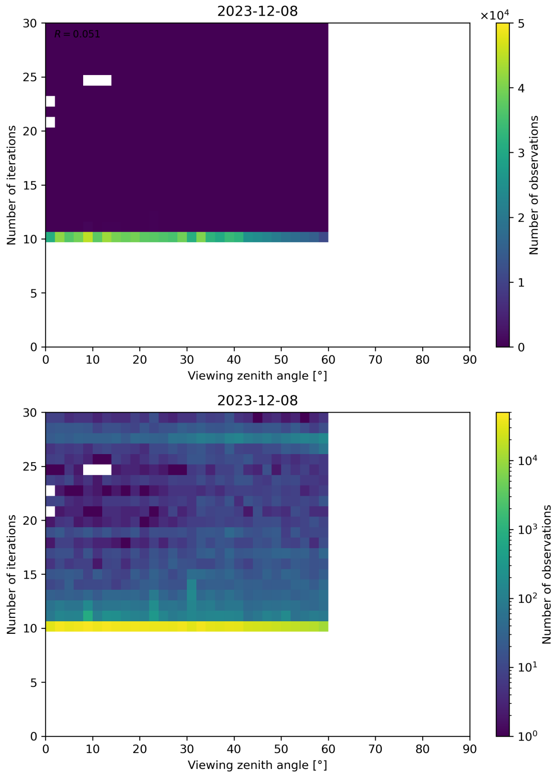
Figure 113: Scatter density plot of “Viewing zenith angle” against “Number of iterations” for 2023-12-07 to 2023-12-09.
