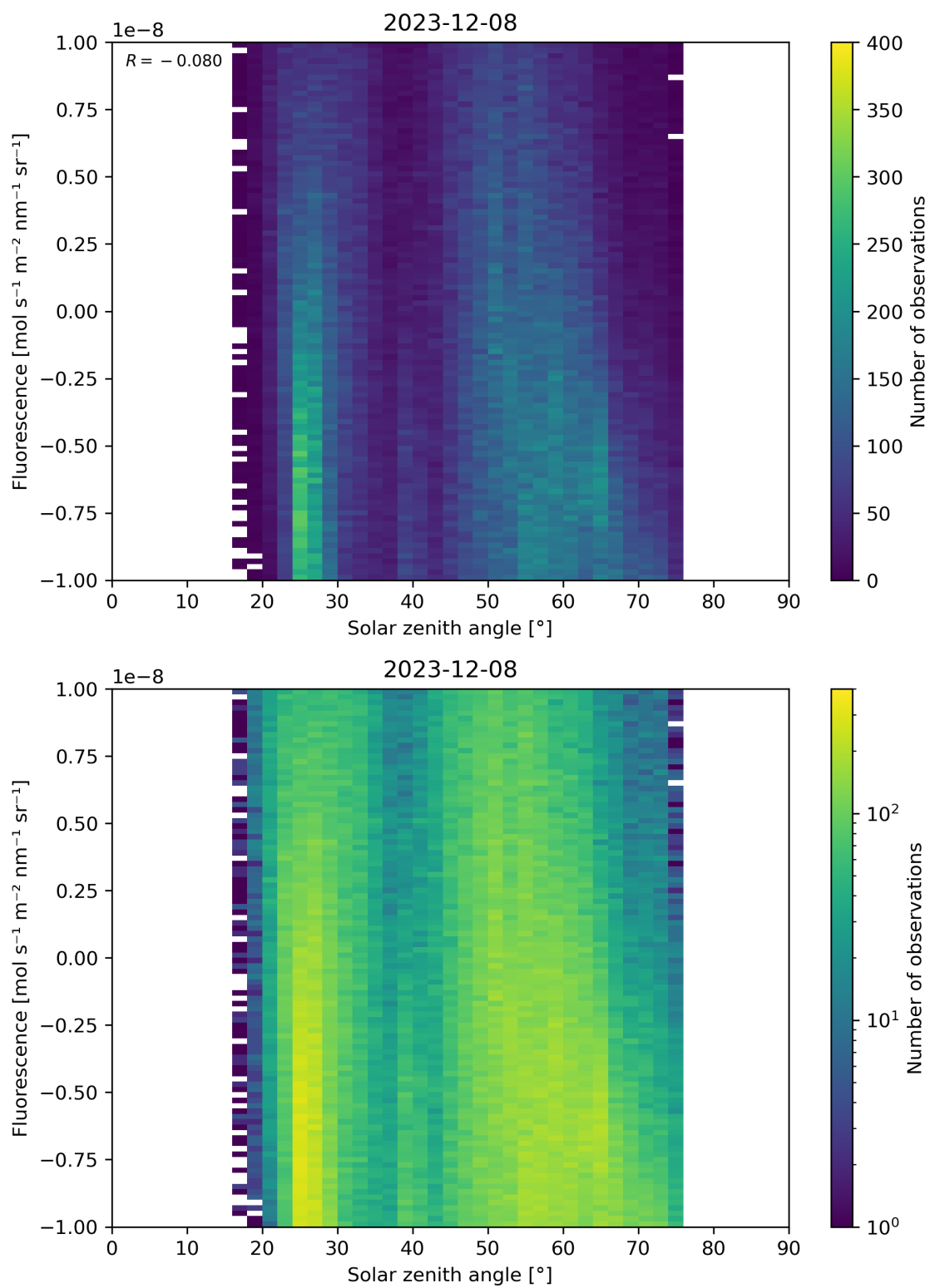
Figure 97: Scatter density plot of “Solar zenith angle” against “Fluorescence” for 2023-12-07 to 2023-12-09.
