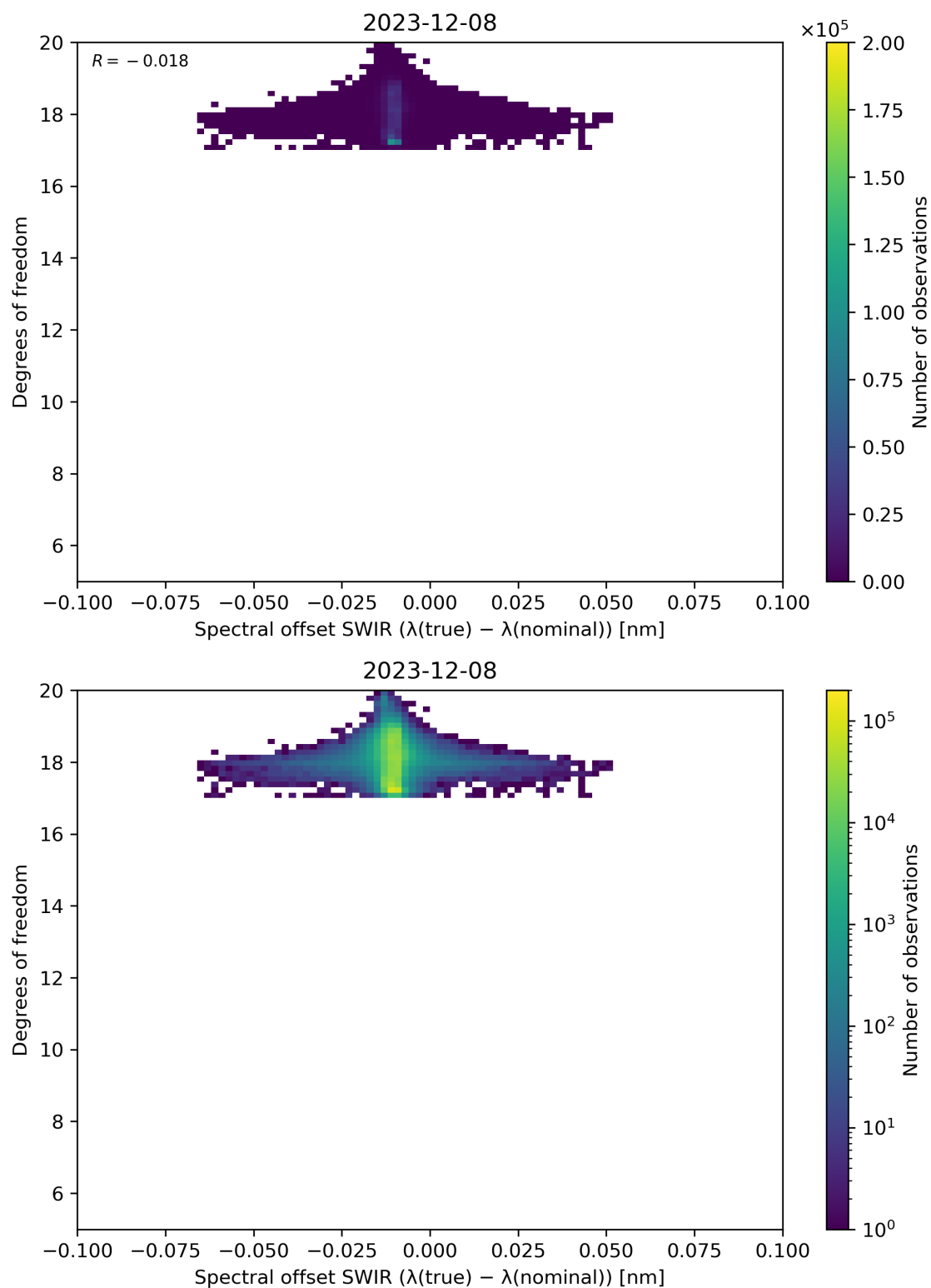
Figure 119: Scatter density plot of “Spectral offset SWIR ( \lambda(\text{true}) - \lambda(\text{nominal}) )” against “Degrees of freedom” for 2023-12-07 to 2023-12-09.
