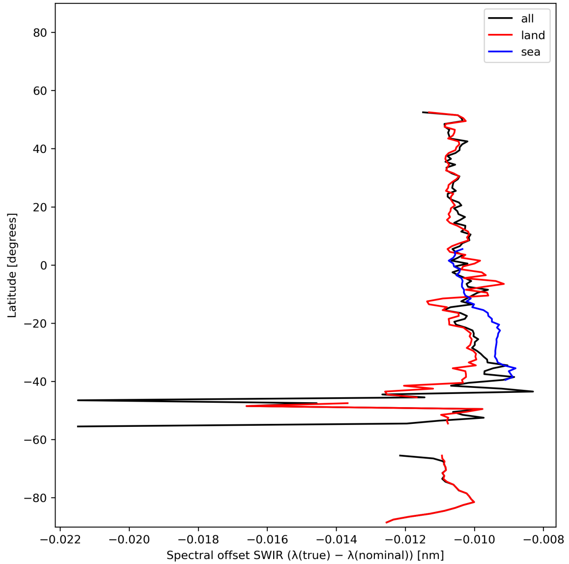
Figure 16: Zonal average of “Spectral offset SWIR ( \lambda(\text{true}) - \lambda(\text{nominal}) )” for 2023-12-07 to 2023-12-09.
