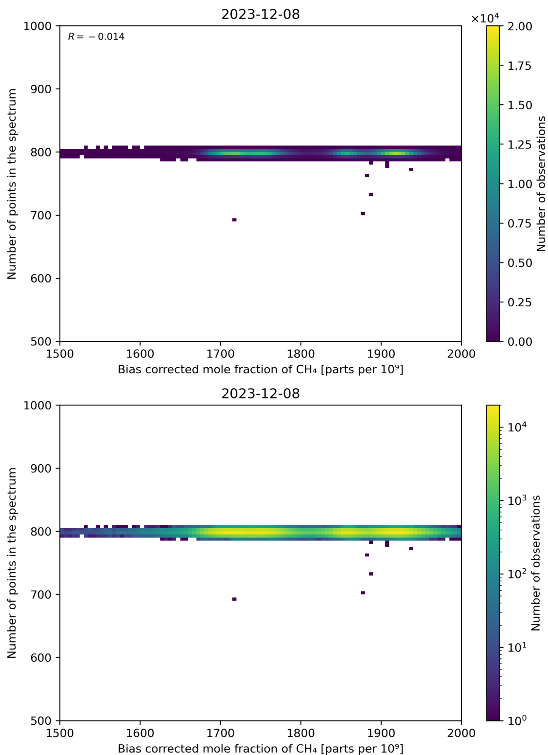
Figure 68: Scatter density plot of “Bias corrected mole fraction of CH 4 ” against “Number of points in the spectrum” for 2023-12-07 to 2023-12-09.
