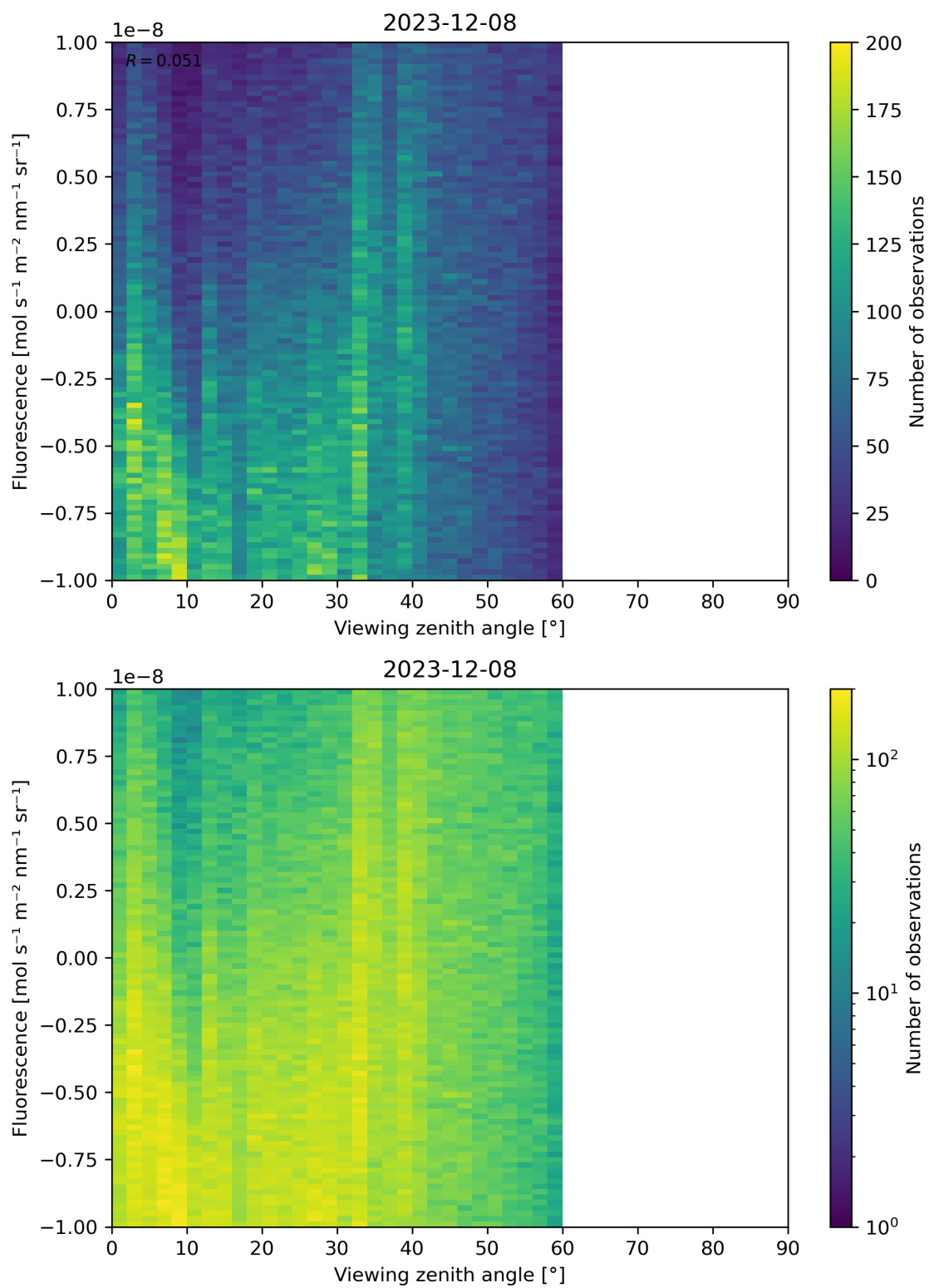
Figure 108: Scatter density plot of “Viewing zenith angle” against “Fluorescence” for 2023-12-07 to 2023-12-09.
