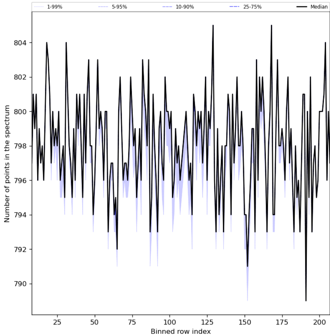
Figure 37: Along track statistics of “Number of points in the spectrum” for 2023-12-07 to 2023-12-09
