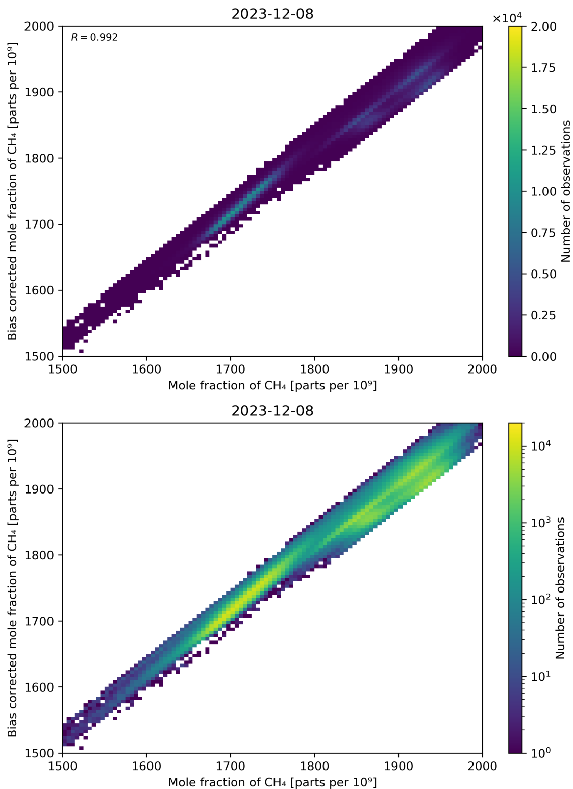
Figure 74: Scatter density plot of “Mole fraction of CH 4 ” against “Bias corrected mole fraction of CH 4 ” for 2023-12-07 to 2023-12-09.
