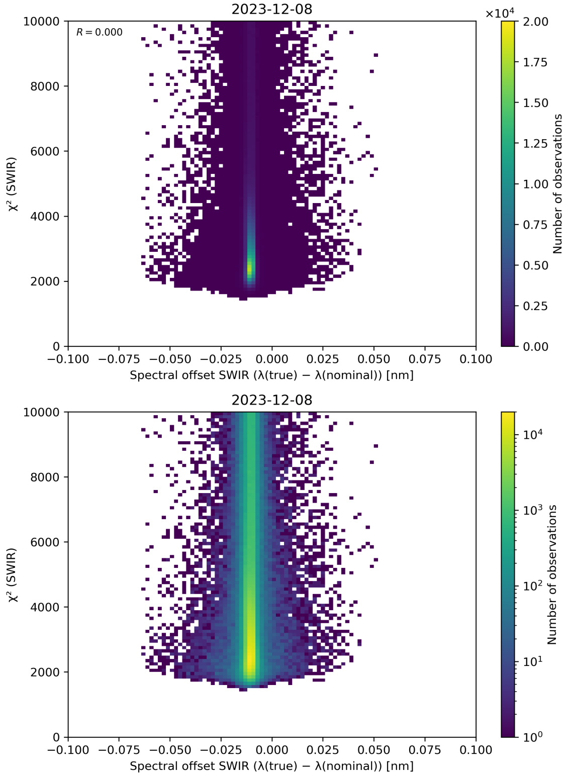
Figure 118: Scatter density plot of “Spectral offset SWIR ( \lambda(\text{true}) - \lambda(\text{nominal}) )” against “ \chi^2 (SWIR)” for 2023-12-07 to 2023-12-09.
