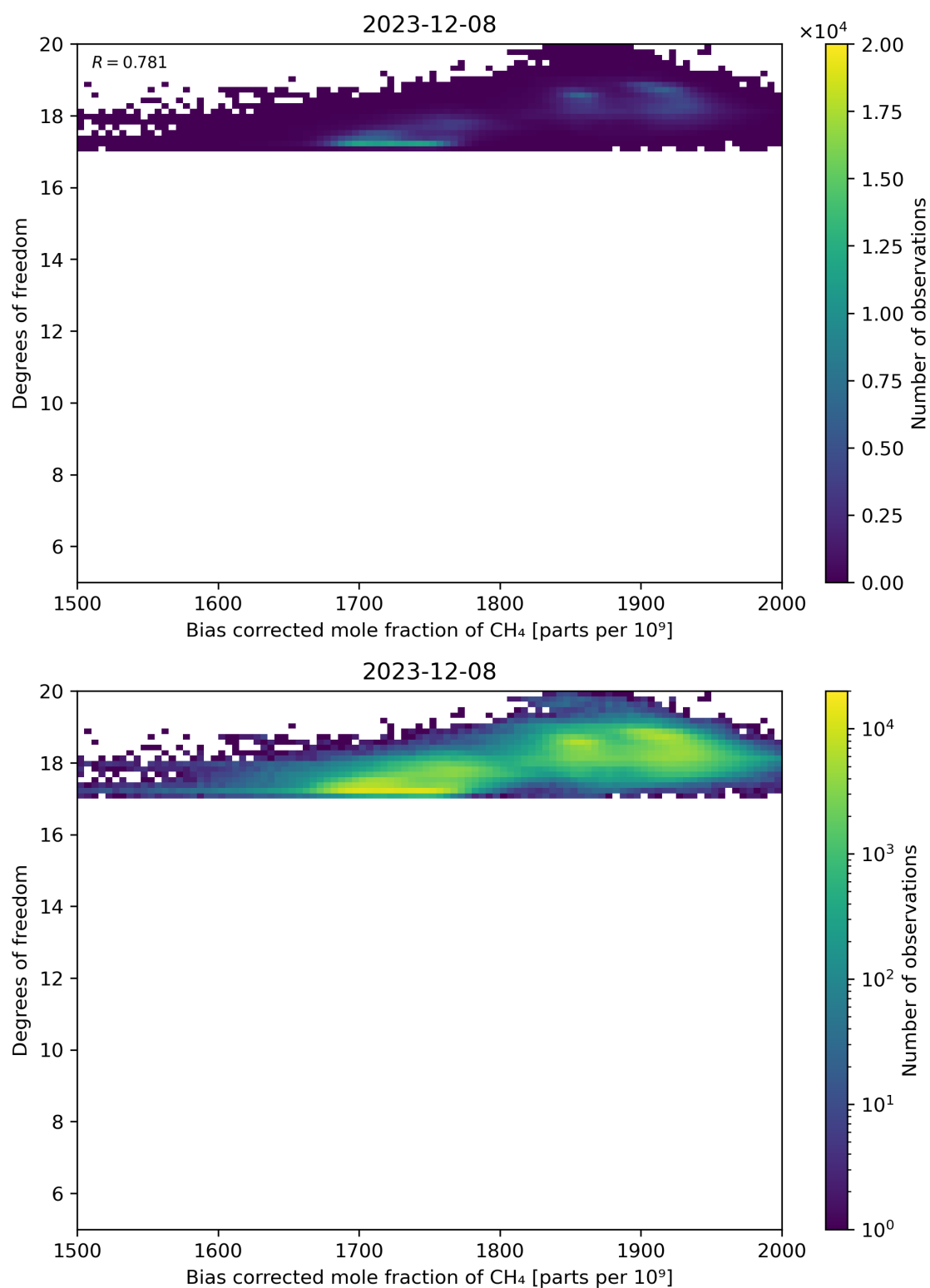
Figure 65: Scatter density plot of “Bias corrected mole fraction of CH 4 ” against “Degrees of freedom” for 2023-12-07 to 2023-12-09.
