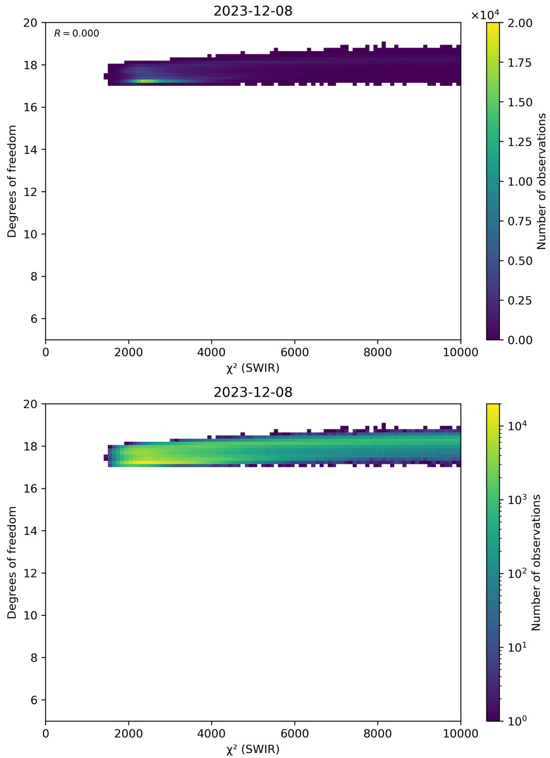
Figure 48: Scatter density plot of “ \chi^2 (SWIR)” against “Degrees of freedom” for 2023-12-07 to 2023-12-09.
