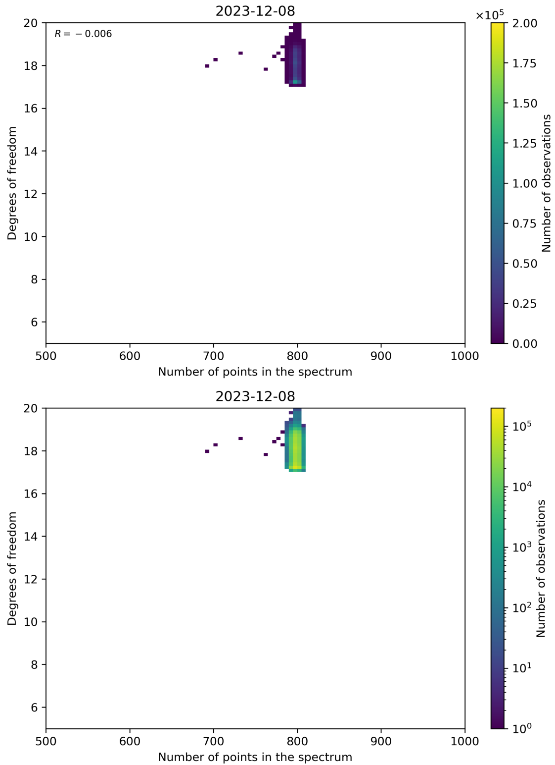
Figure 90: Scatter density plot of “Number of points in the spectrum” against “Degrees of freedom” for 2023-12-07 to 2023-12-09.
