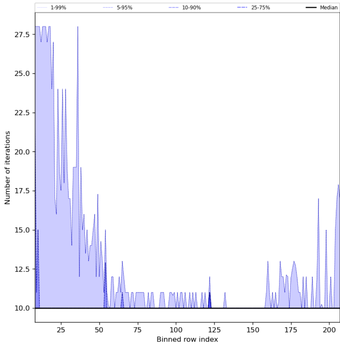
Figure 42: Along track statistics of “Number of iterations” for 2023-12-07 to 2023-12-09
