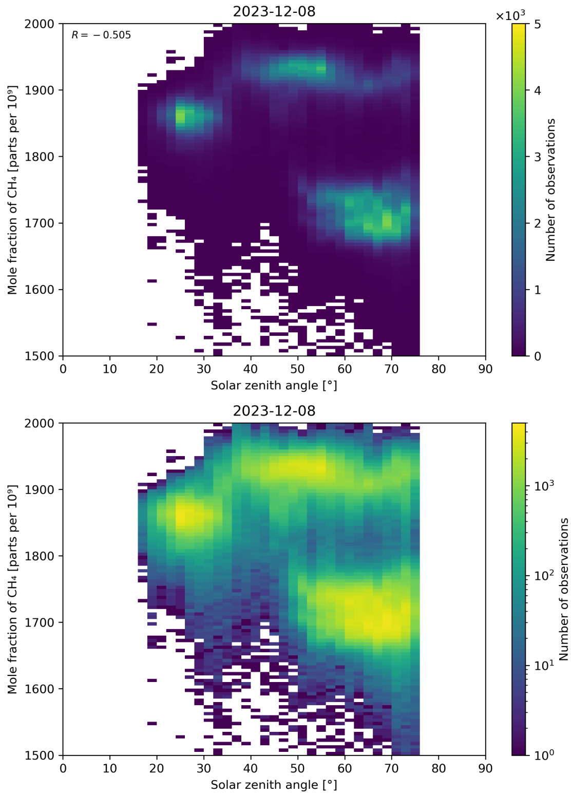
Figure 99: Scatter density plot of “Solar zenith angle” against “Mole fraction of CH 4 ” for 2023-12-07 to 2023-12-09.
