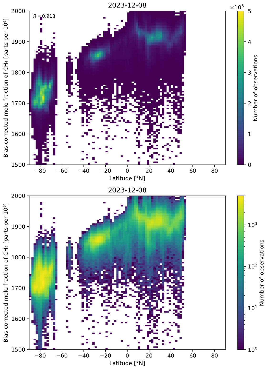
Figure 58: Scatter density plot of “Latitude” against “Bias corrected mole fraction of \text{CH}_4 ” for 2023-12-07 to 2023-12-09.
