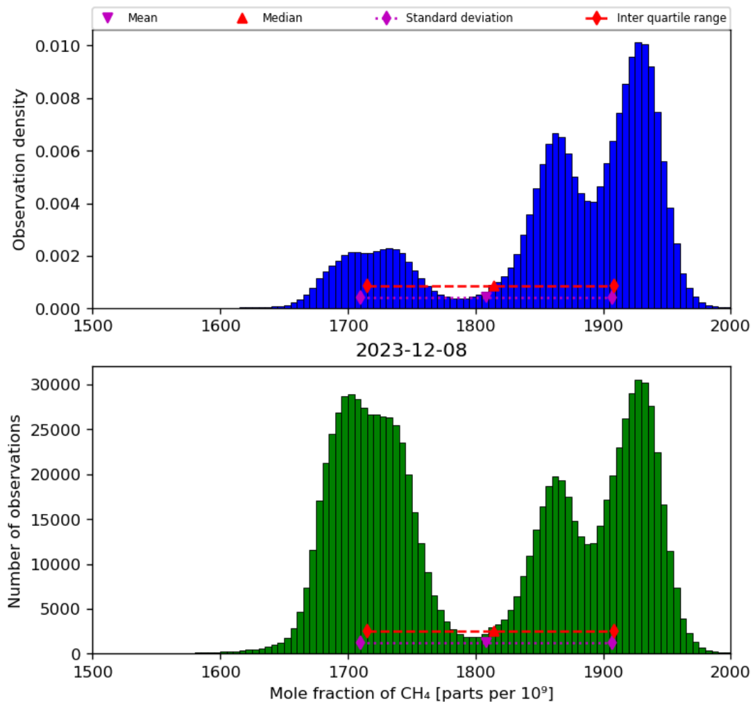
Figure 23: Histogram of “Mole fraction of CH 4 ” for 2023-12-07 to 2023-12-09
