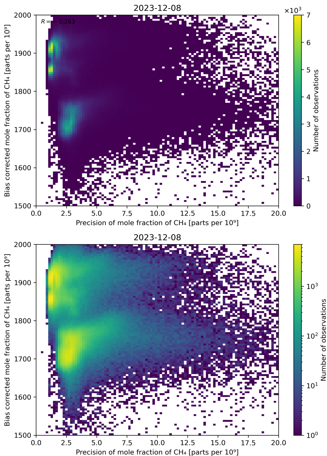
Figure 82: Scatter density plot of “Precision of mole fraction of CH 4 ” against “Bias corrected mole fraction of CH 4 ” for 2023-12-07 to 2023-12-09.
