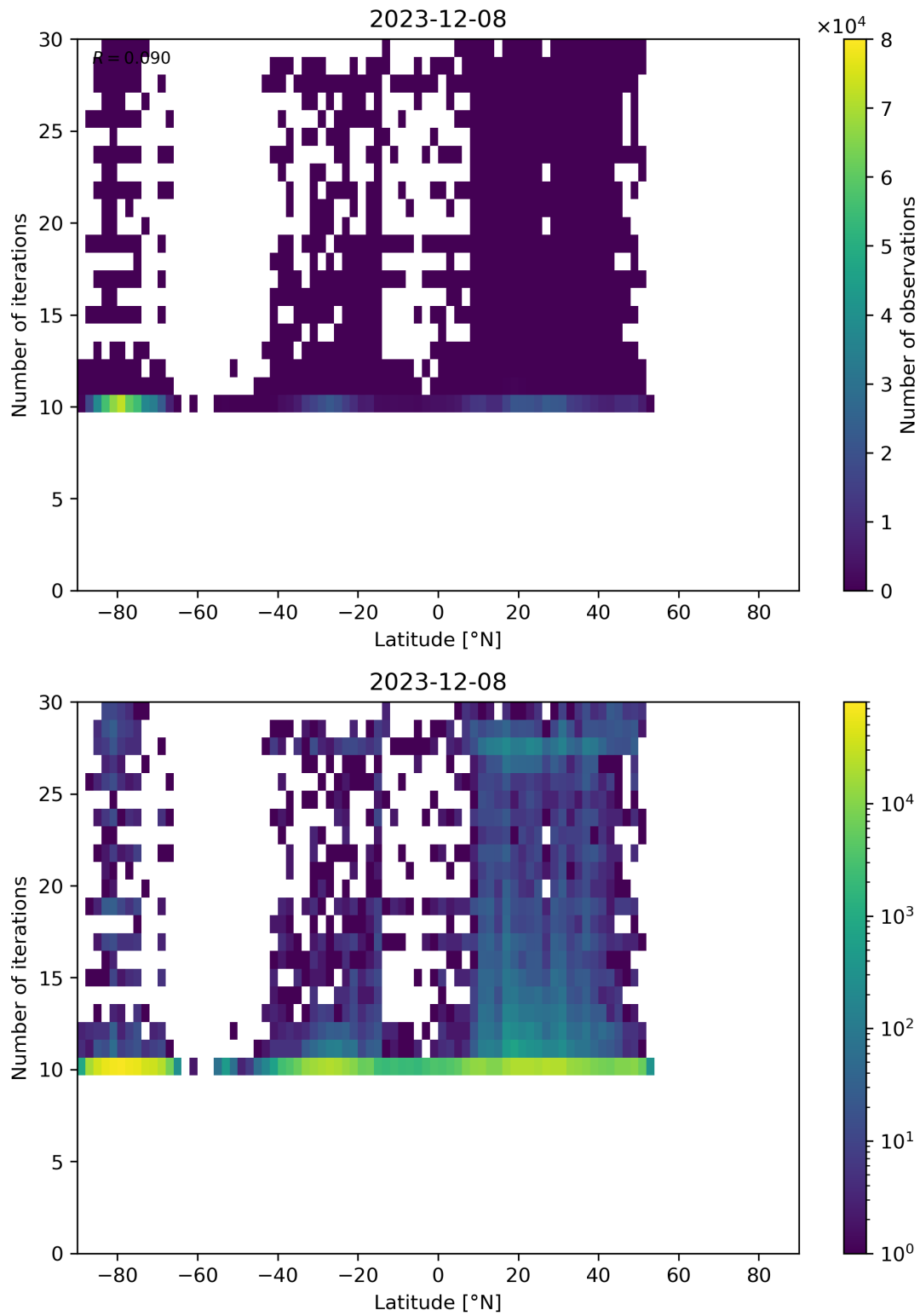
Figure 60: Scatter density plot of “Latitude” against “Number of iterations” for 2023-12-07 to 2023-12-09.
