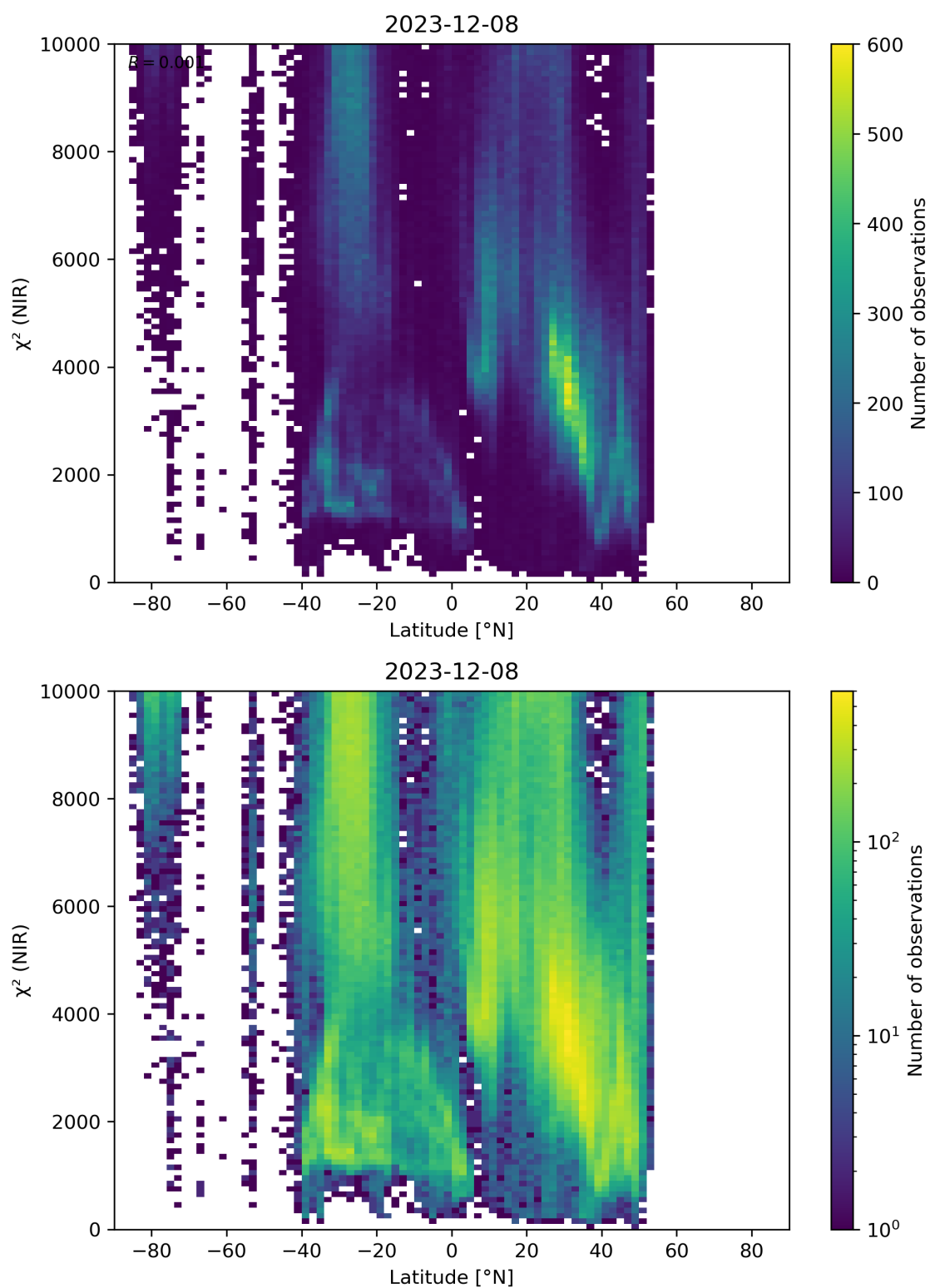
Figure 53: Scatter density plot of “Latitude” against “ \chi^2 (NIR)” for 2023-12-07 to 2023-12-09.
