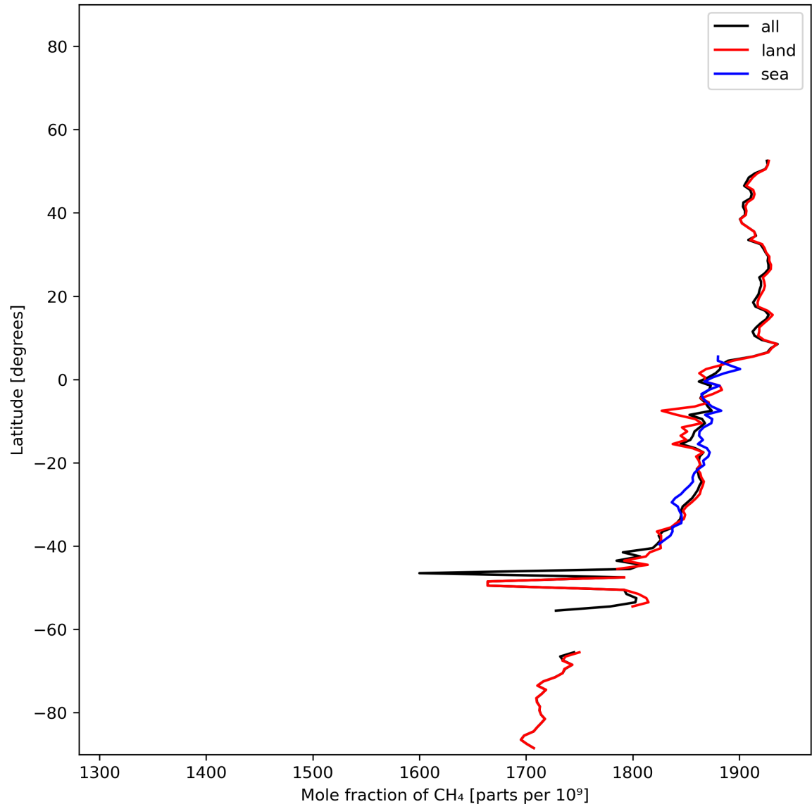
Figure 12: Zonal average of “Mole fraction of \text{CH}_4 ” for 2023-12-07 to 2023-12-09.
