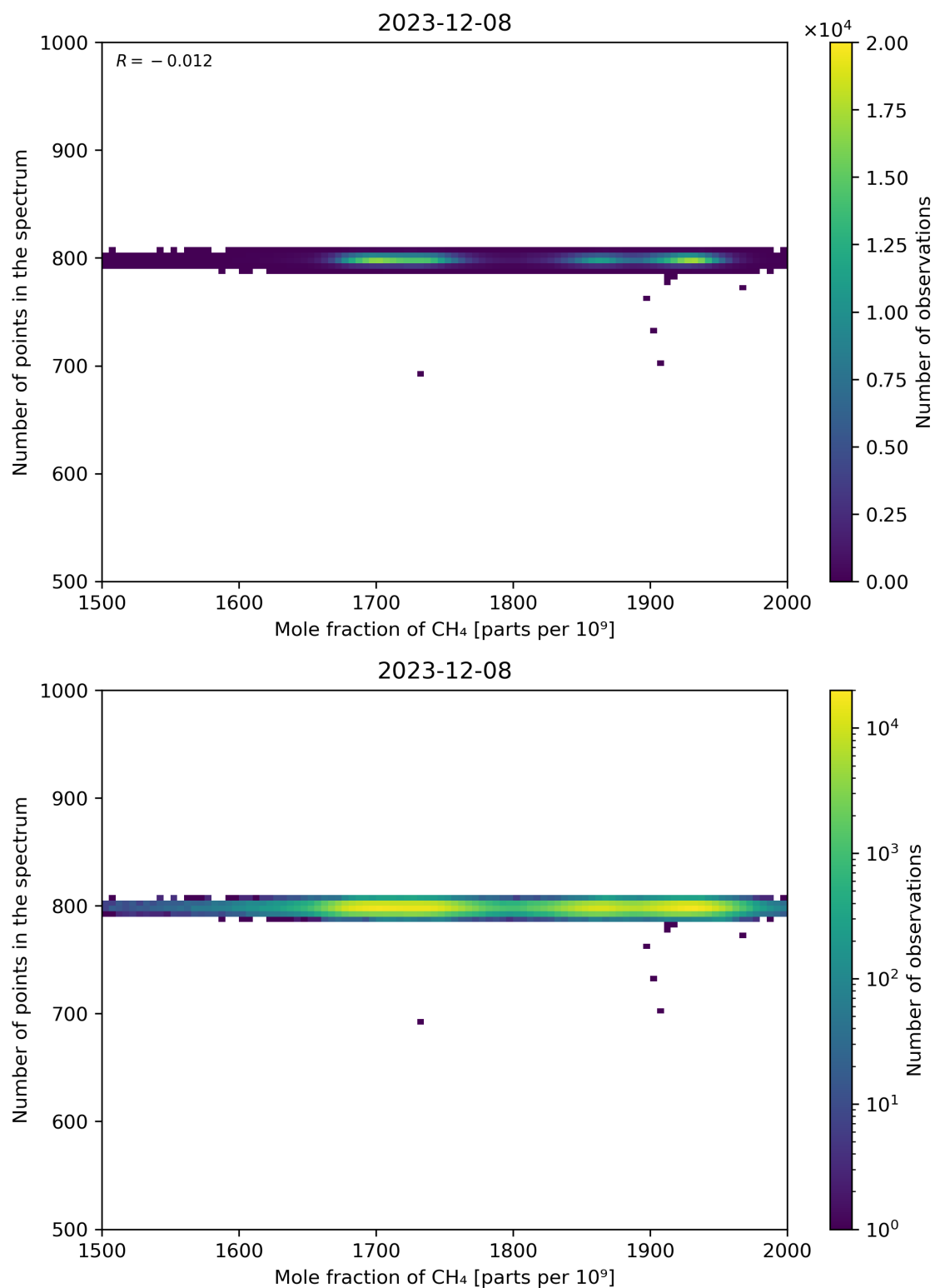
Figure 77: Scatter density plot of “Mole fraction of CH 4 ” against “Number of points in the spectrum” for 2023-12-07 to 2023-12-09.
