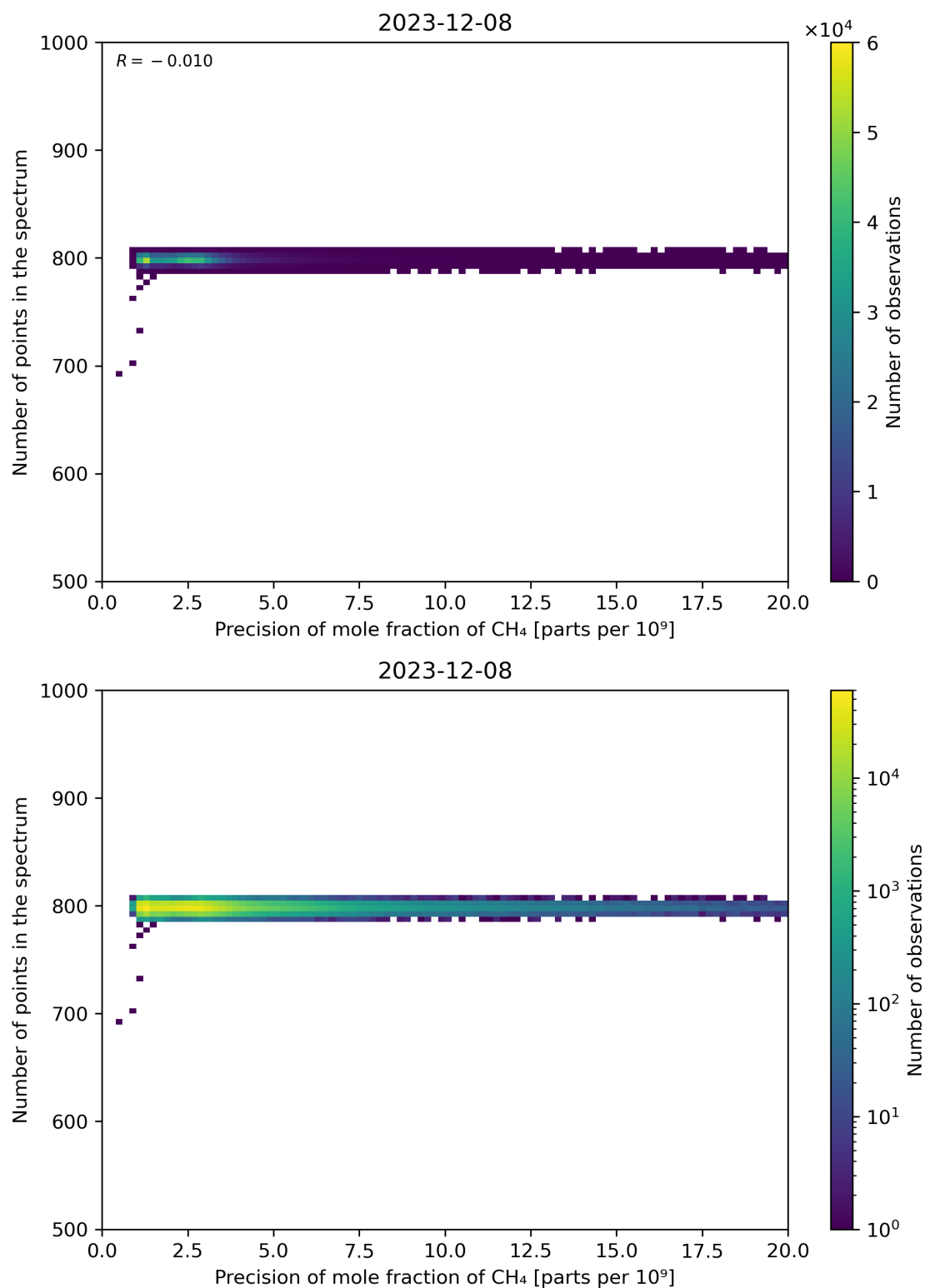
Figure 84: Scatter density plot of “Precision of mole fraction of CH 4 ” against “Number of points in the spectrum” for 2023-12-07 to 2023-12-09.
