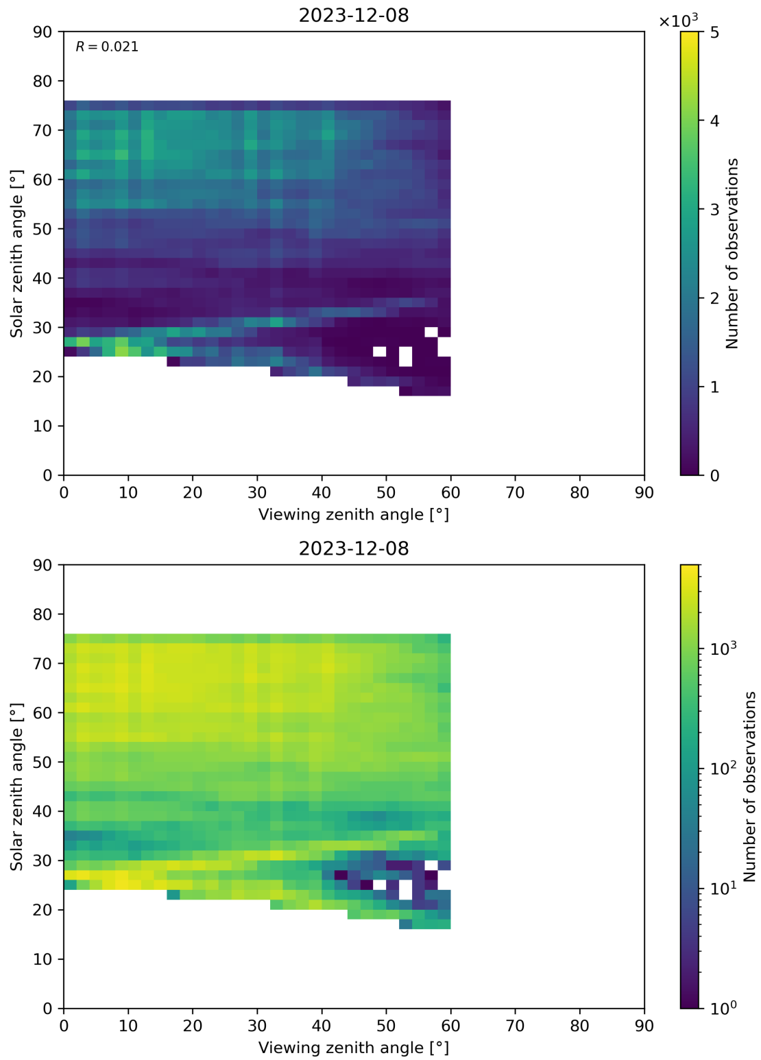
Figure 115: Scatter density plot of “Viewing zenith angle” against “Solar zenith angle” for 2023-12-07 to 2023-12-09.
