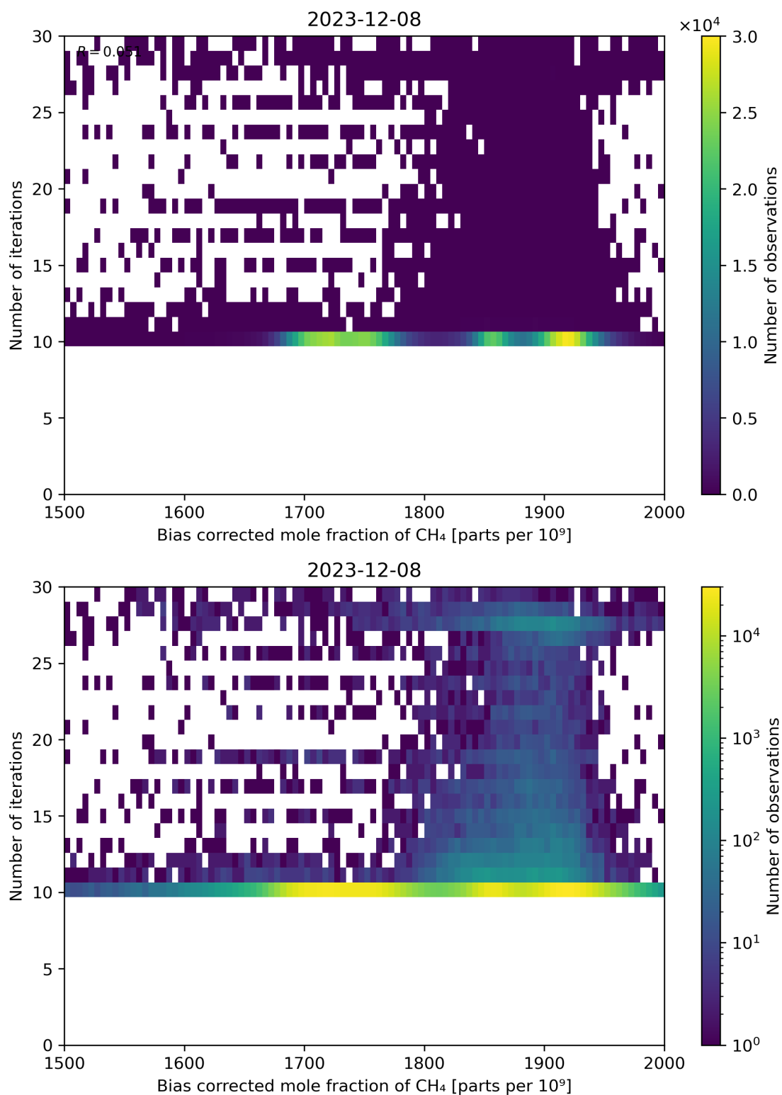
Figure 67: Scatter density plot of “Bias corrected mole fraction of CH 4 ” against “Number of iterations” for 2023-12-07 to 2023-12-09.
