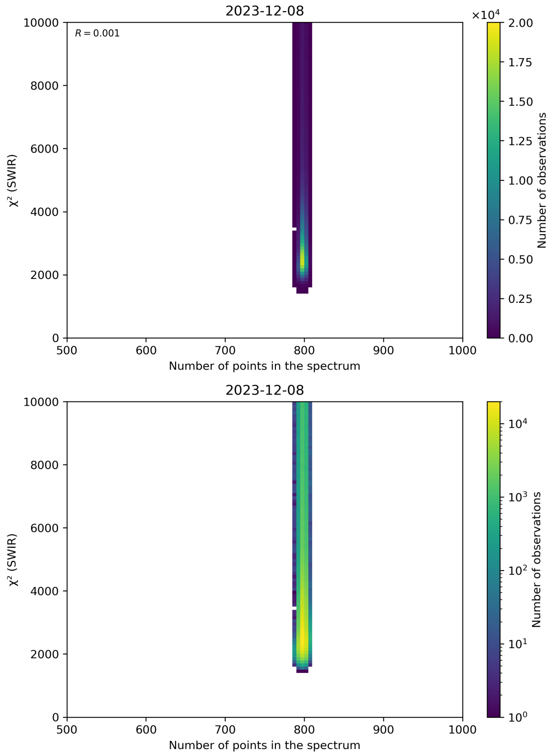
Figure 89: Scatter density plot of “Number of points in the spectrum” against “ \chi^2 (SWIR)” for 2023-12-07 to 2023-12-09.
