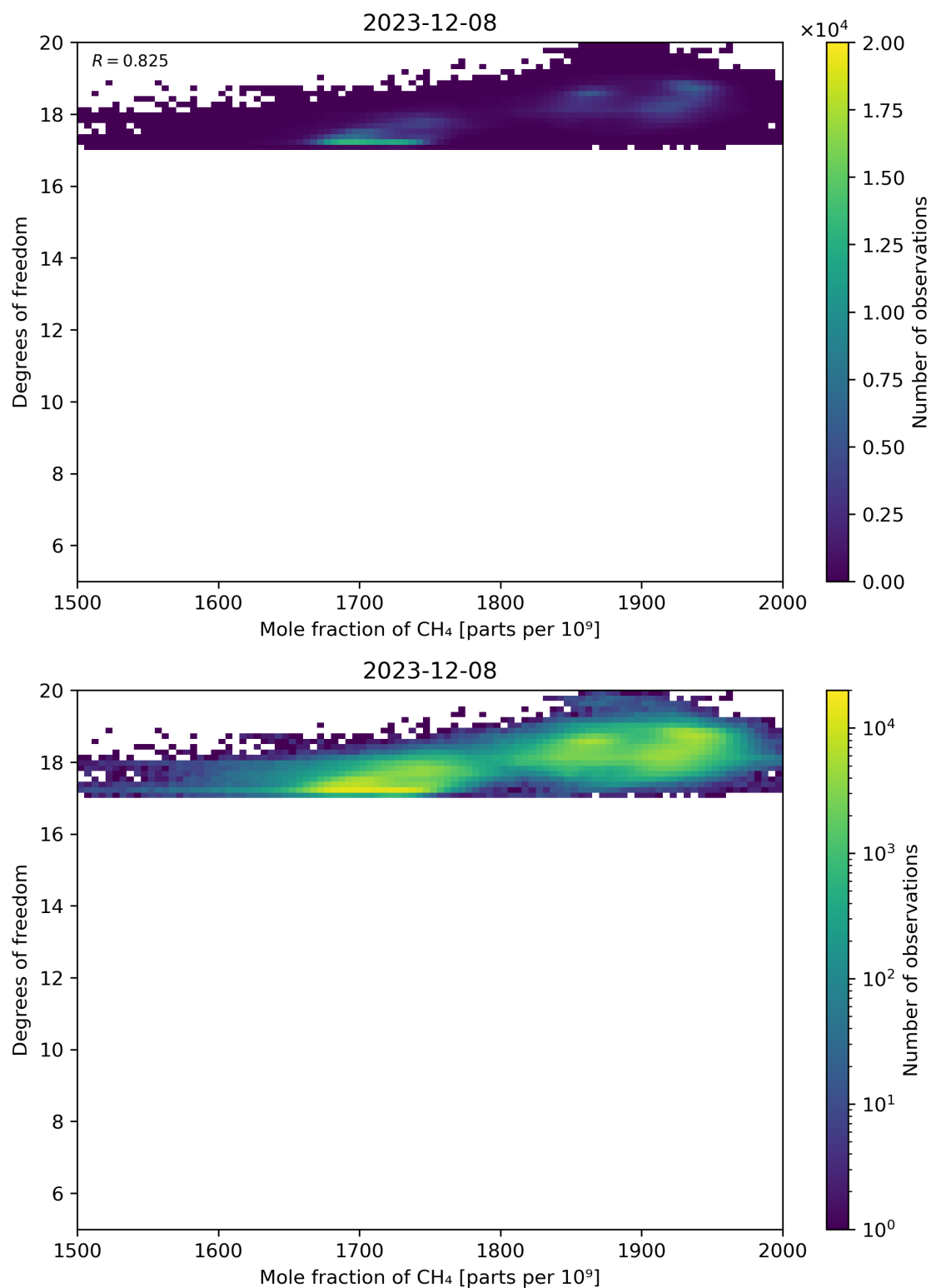
Figure 72: Scatter density plot of “Mole fraction of CH 4 ” against “Degrees of freedom” for 2023-12-07 to 2023-12-09.
