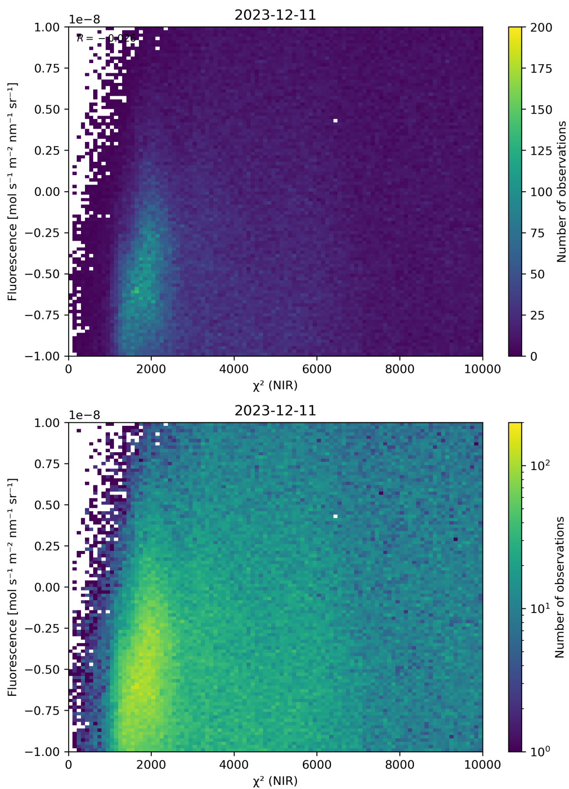
Figure 45: Scatter density plot of “ \chi^2 (NIR)” against “Fluorescence” for 2023-12-10 to 2023-12-12.
