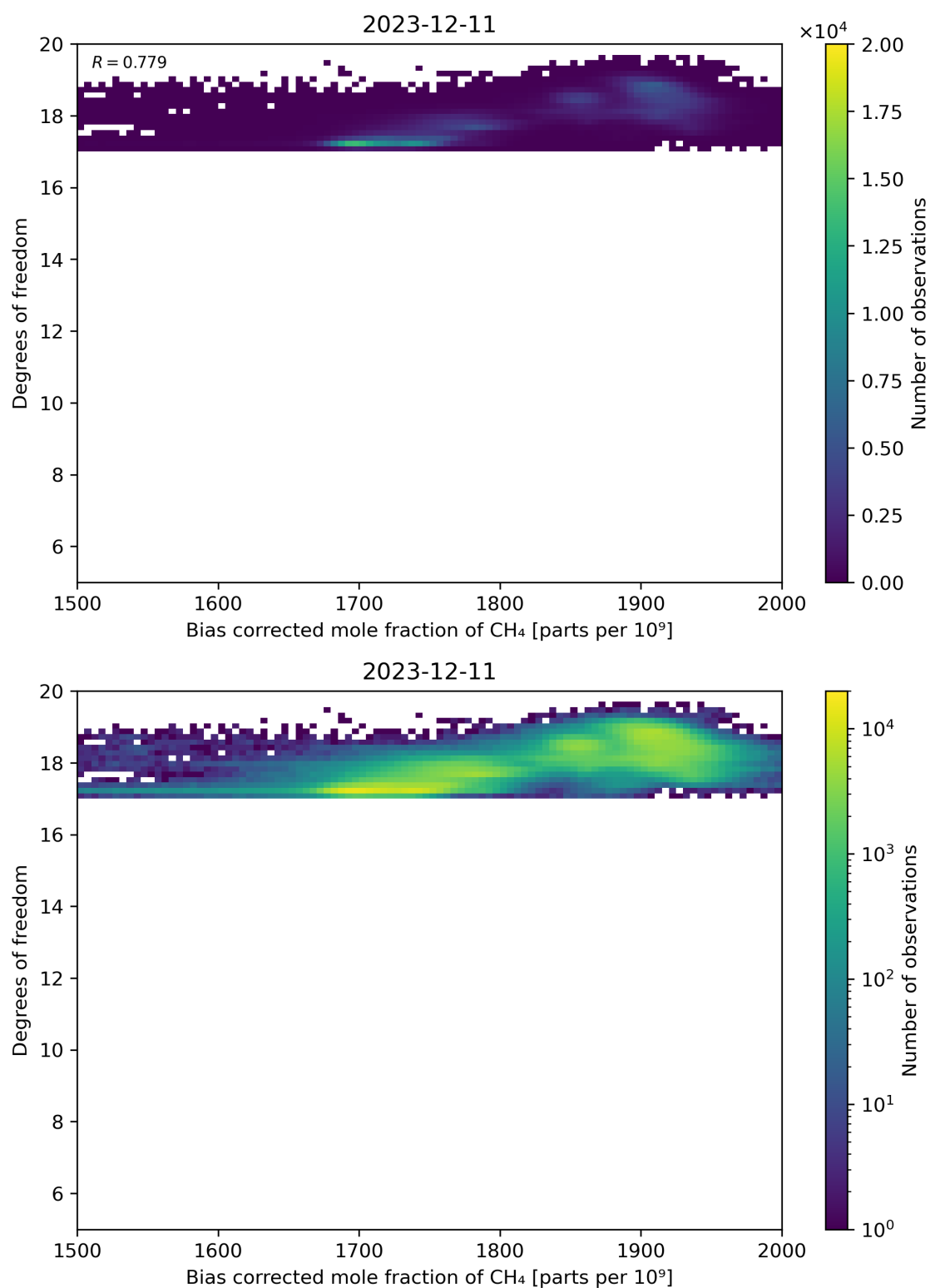
Figure 65: Scatter density plot of “Bias corrected mole fraction of CH 4 ” against “Degrees of freedom” for 2023-12-10 to 2023-12-12.
