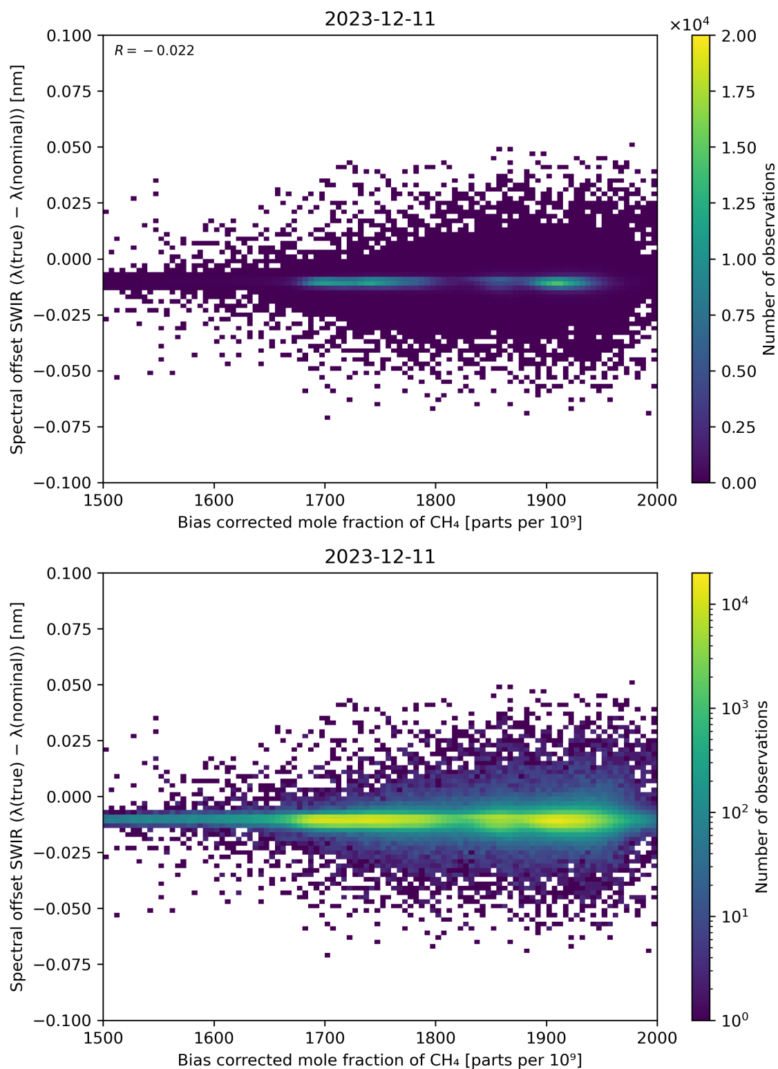
Figure 69: Scatter density plot of “Bias corrected mole fraction of \text{CH}_4 ” against “Spectral offset SWIR ( \lambda(\text{true}) - \lambda(\text{nominal}) )” for 2023-12-10 to 2023-12-12.
