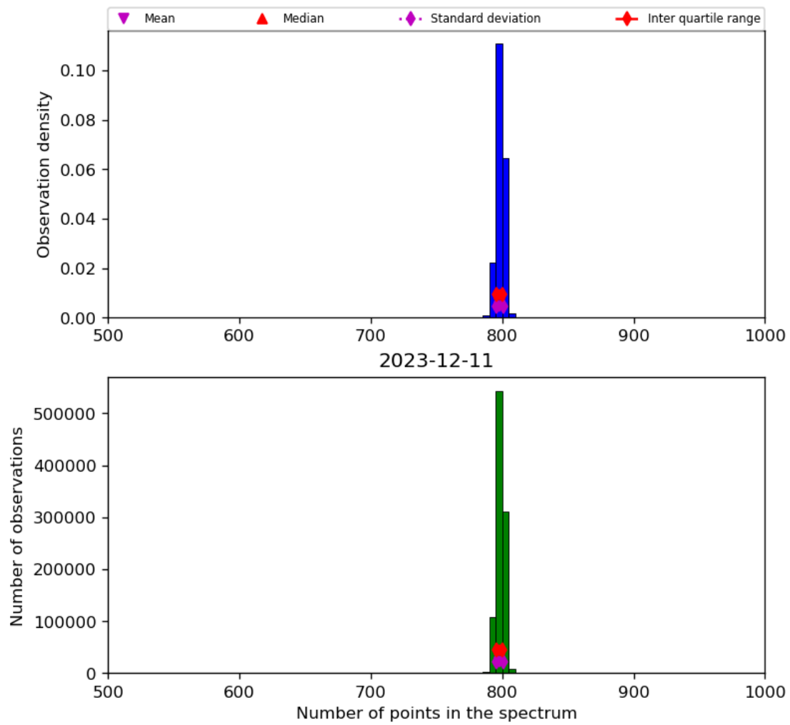
Figure 26: Histogram of “Number of points in the spectrum” for 2023-12-10 to 2023-12-12
