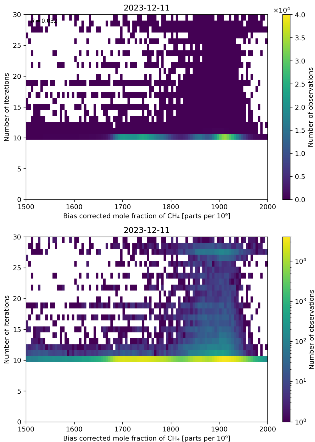
Figure 67: Scatter density plot of “Bias corrected mole fraction of \text{CH}_4 ” against “Number of iterations” for 2023-12-10 to 2023-12-12.
