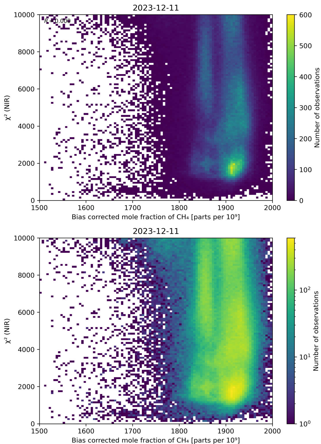
Figure 63: Scatter density plot of “Bias corrected mole fraction of \text{CH}_4 ” against “ \chi^2 (NIR)” for 2023-12-10 to 2023-12-12.
