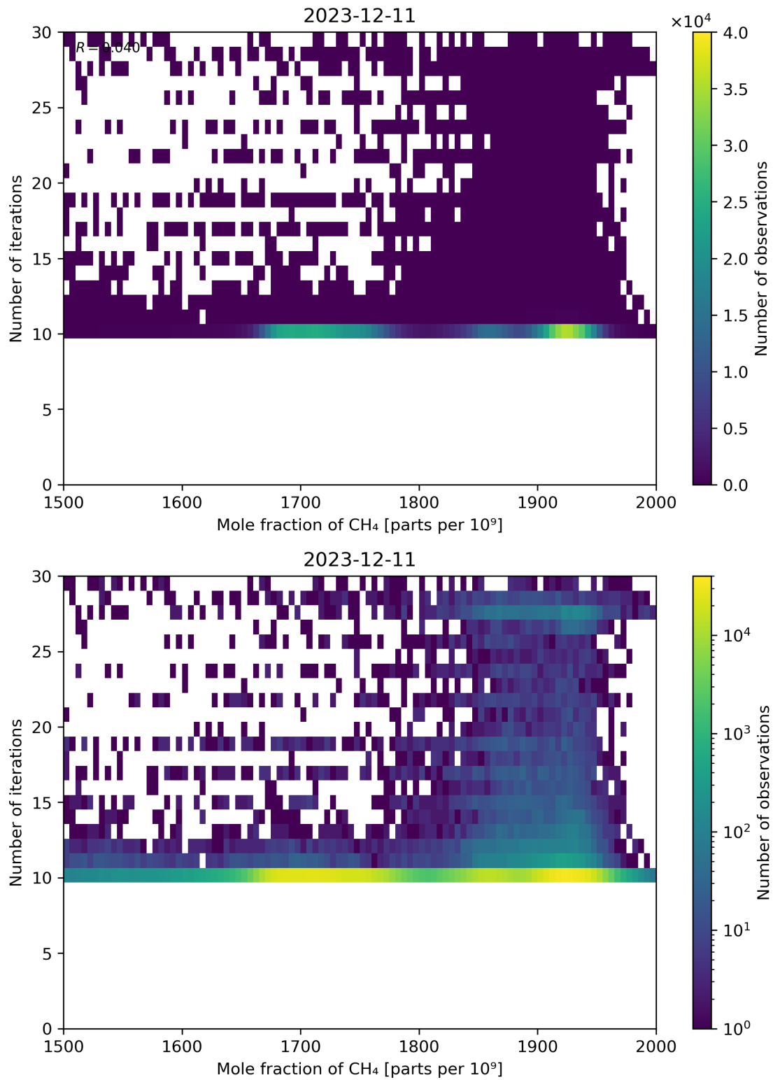
Figure 76: Scatter density plot of “Mole fraction of CH 4 ” against “Number of iterations” for 2023-12-10 to 2023-12-12.
