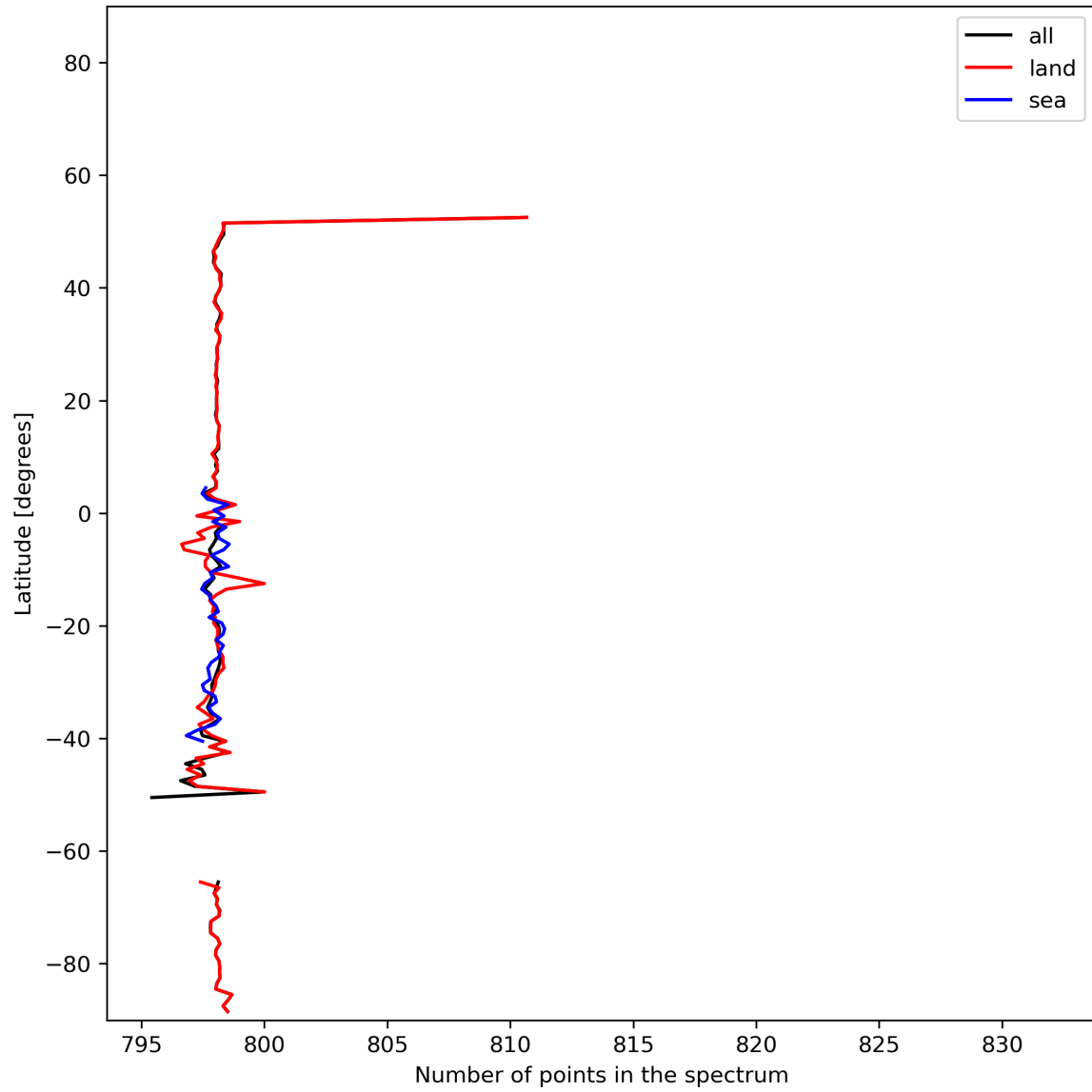
Figure 15: Zonal average of “Number of points in the spectrum” for 2023-12-10 to 2023-12-12.
