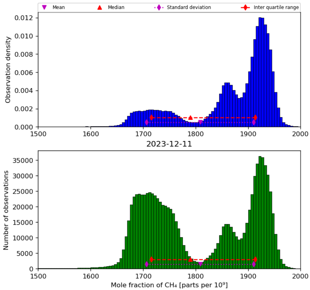
Figure 23: Histogram of “Mole fraction of CH 4 ” for 2023-12-10 to 2023-12-12
