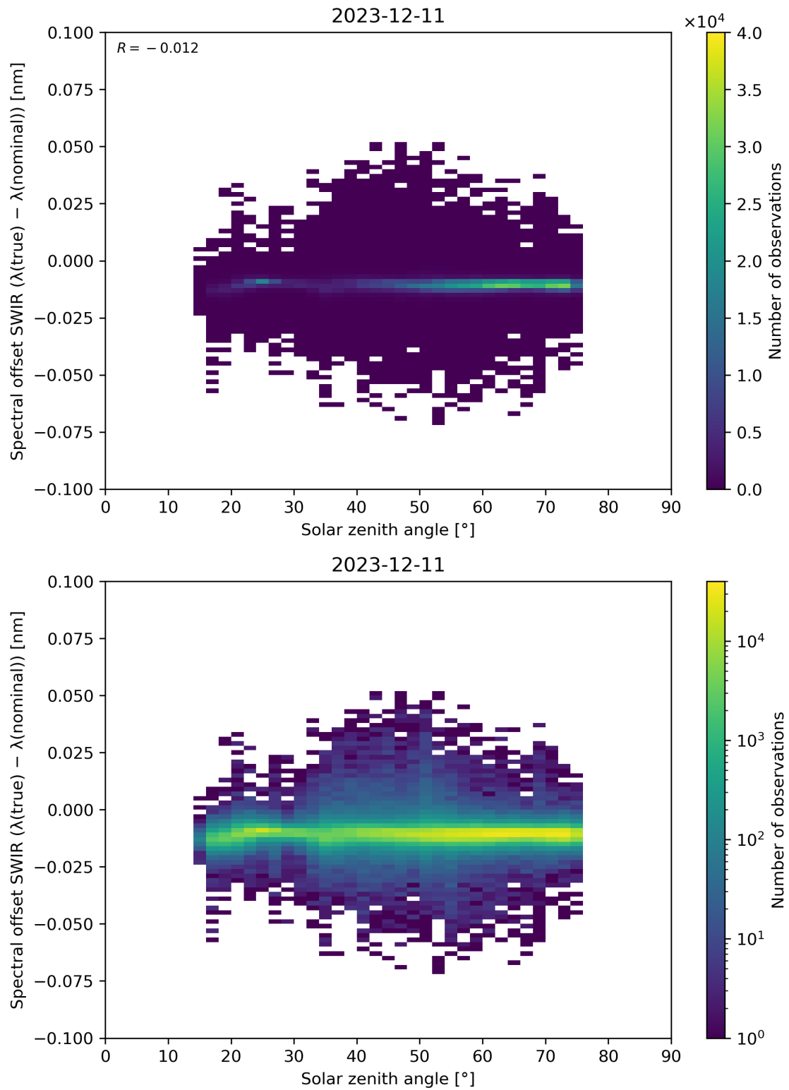
Figure 104: Scatter density plot of “Solar zenith angle” against “Spectral offset SWIR ( \lambda(\text{true}) - \lambda(\text{nominal}) )” for 2023-12-10 to 2023-12-12.
