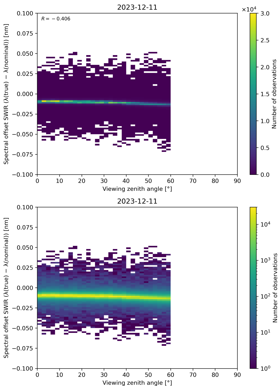
Figure 116: Scatter density plot of “Viewing zenith angle” against “Spectral offset SWIR ( \lambda(\text{true}) - \lambda(\text{nominal}) )” for 2023-12-10 to 2023-12-12.
