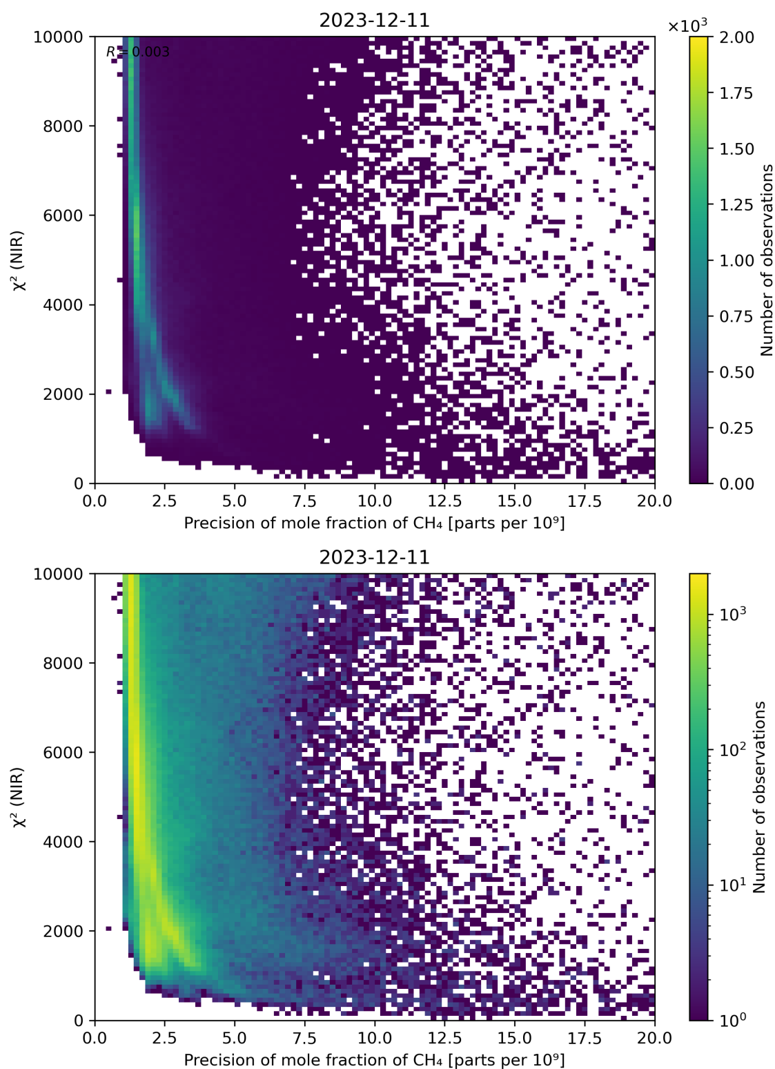
Figure 78: Scatter density plot of “Precision of mole fraction of CH 4 ” against “ \chi^2 (NIR)” for 2023-12-10 to 2023-12-12.
