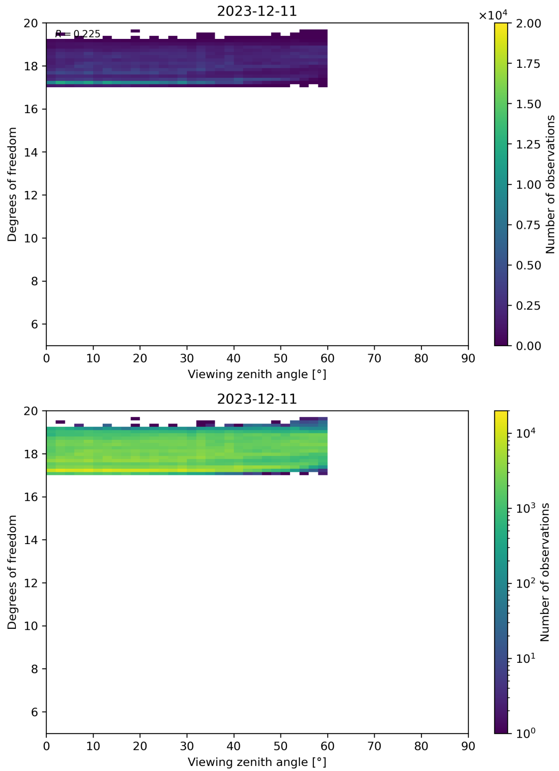
Figure 107: Scatter density plot of “Viewing zenith angle” against “Degrees of freedom” for 2023-12-10 to 2023-12-12.
