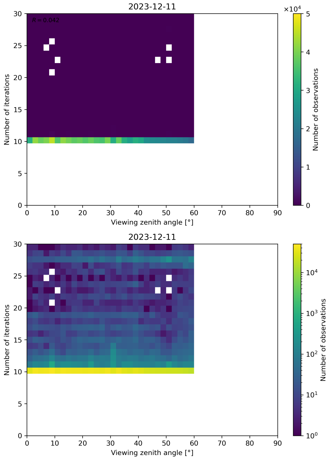
Figure 113: Scatter density plot of “Viewing zenith angle” against “Number of iterations” for 2023-12-10 to 2023-12-12.
