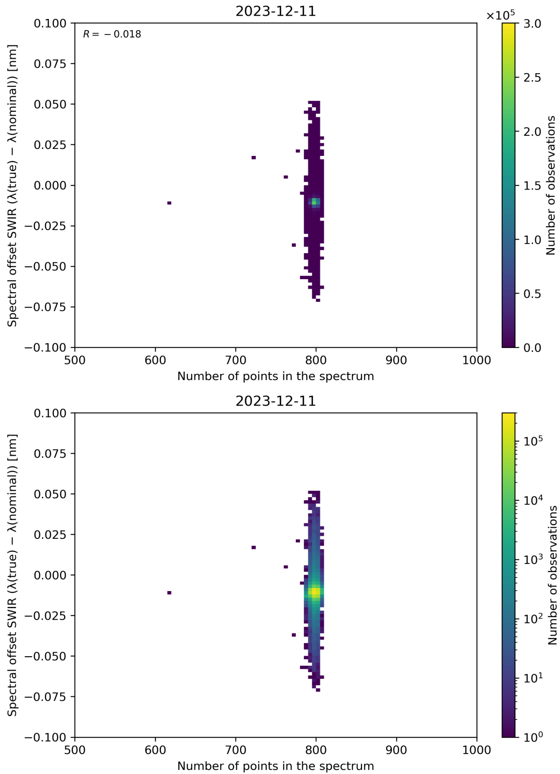
Figure 93: Scatter density plot of “Number of points in the spectrum” against “Spectral offset SWIR ( \lambda(\text{true}) - \lambda(\text{nominal}) )” for 2023-12-10 to 2023-12-12.
