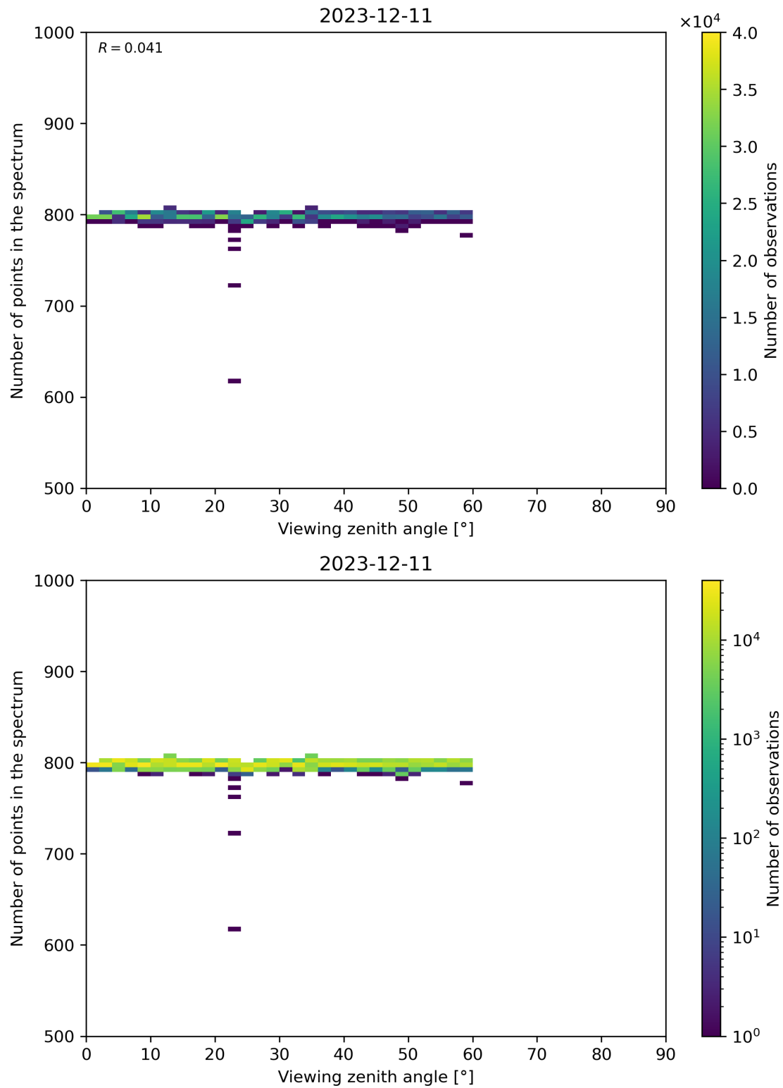
Figure 114: Scatter density plot of “Viewing zenith angle” against “Number of points in the spectrum” for 2023-12-10 to 2023-12-12.
