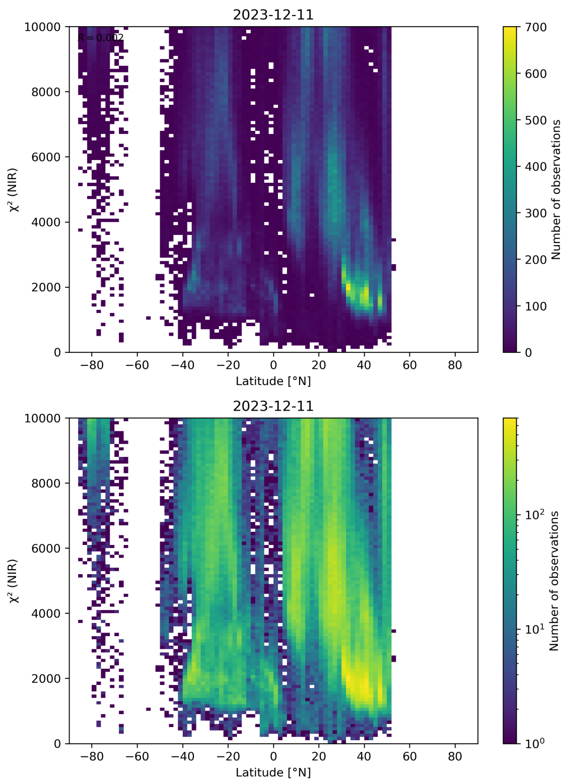
Figure 53: Scatter density plot of “Latitude” against “ \chi^2 (NIR)” for 2023-12-10 to 2023-12-12.
