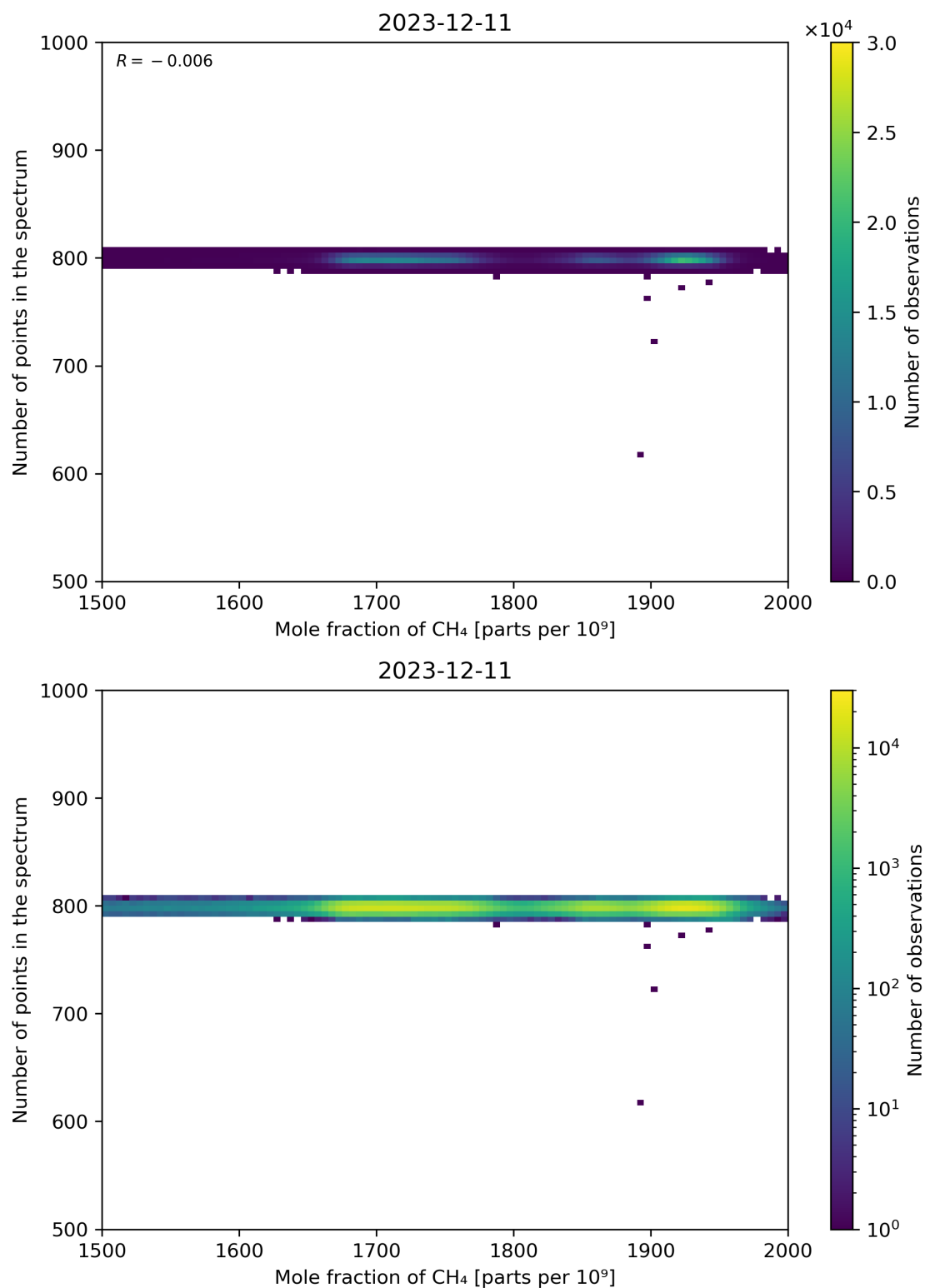
Figure 77: Scatter density plot of “Mole fraction of CH 4 ” against “Number of points in the spectrum” for 2023-12-10 to 2023-12-12.
