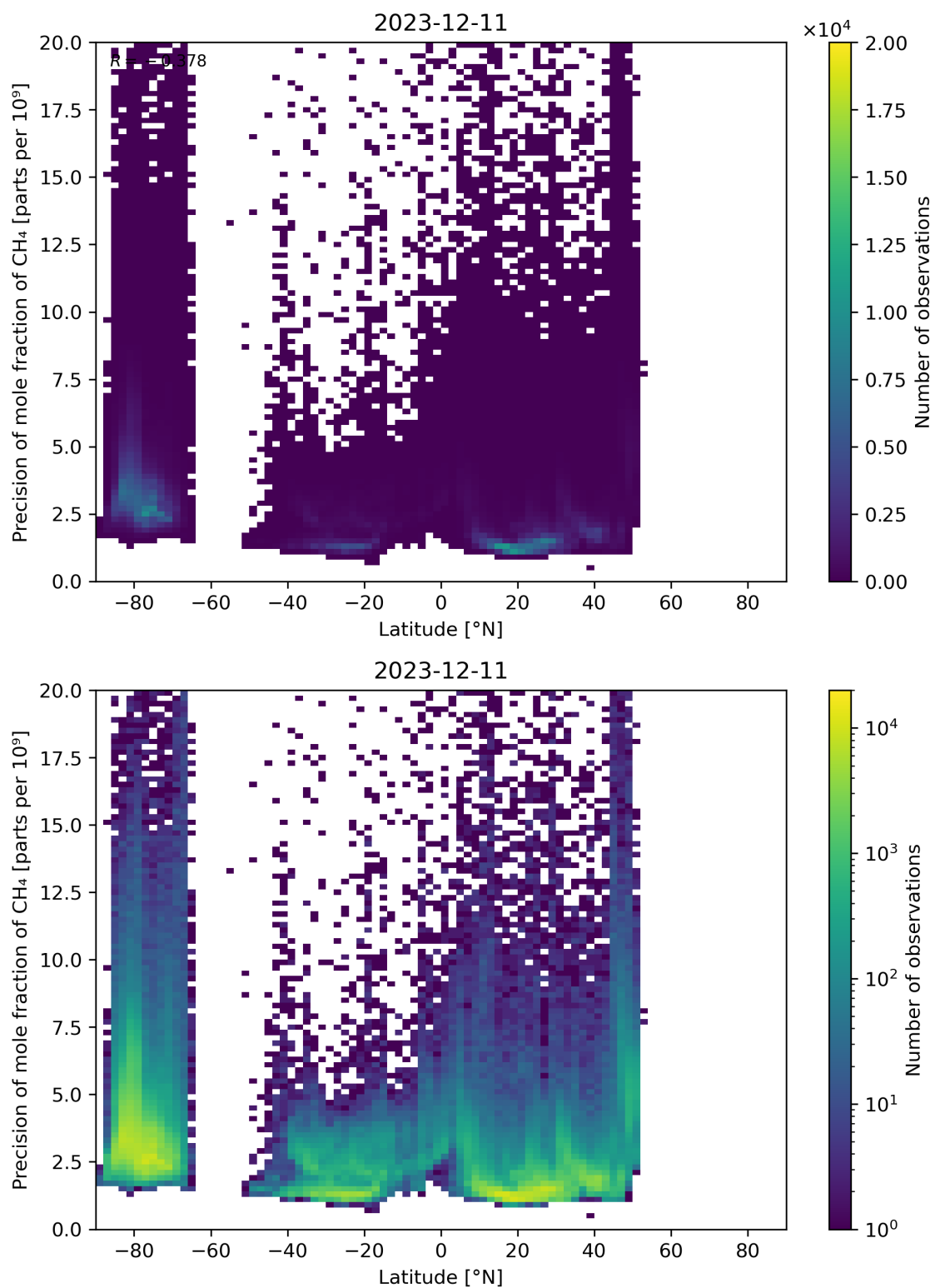
Figure 59: Scatter density plot of “Latitude” against “Precision of mole fraction of CH 4 ” for 2023-12-10 to 2023-12-12.
