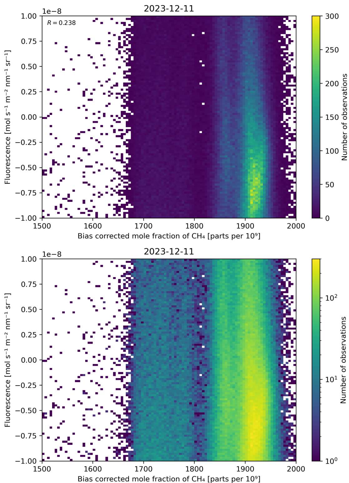
Figure 66: Scatter density plot of “Bias corrected mole fraction of \text{CH}_4 ” against “Fluorescence” for 2023-12-10 to 2023-12-12.
