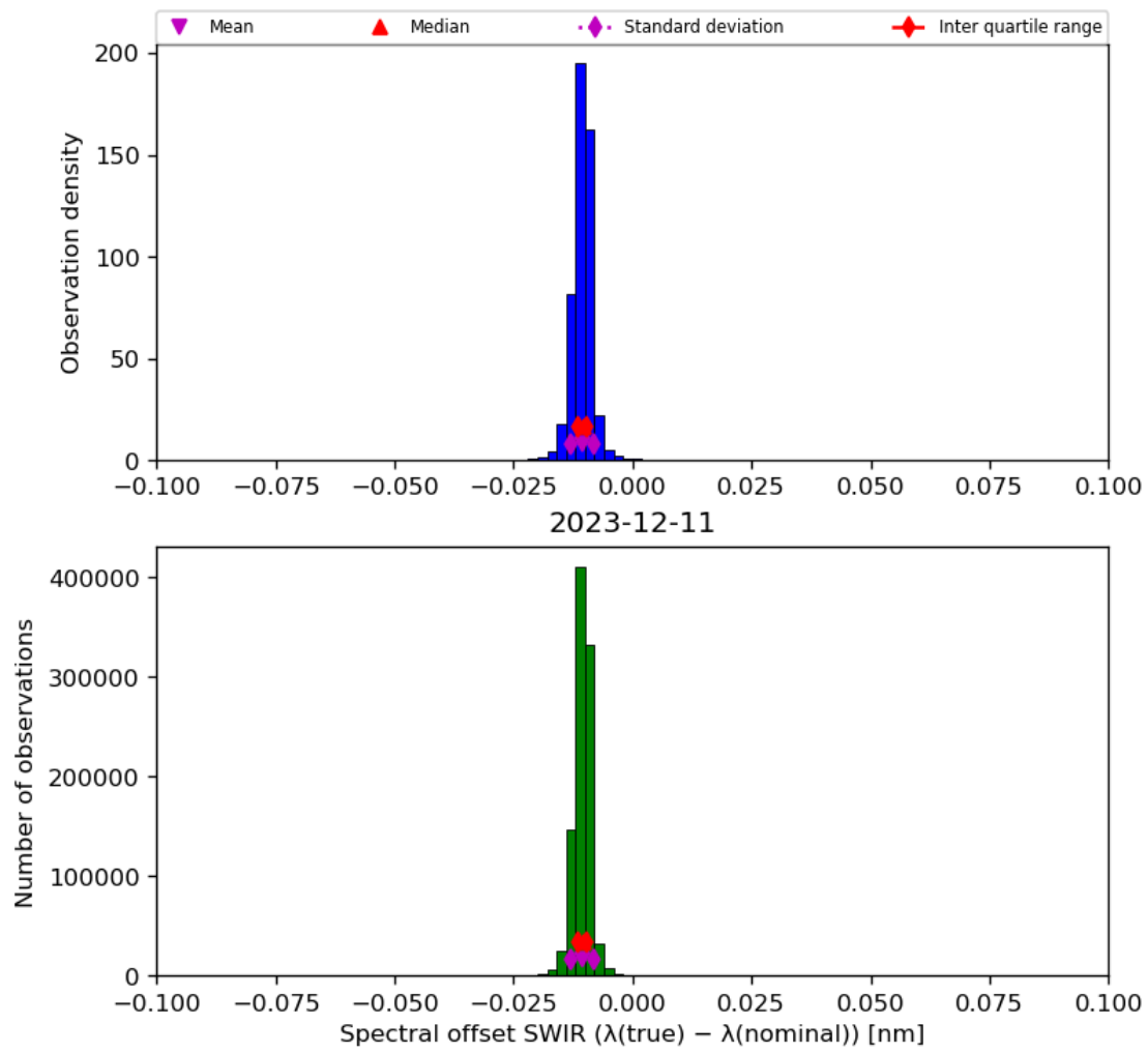
Figure 27: Histogram of “Spectral offset SWIR ( \lambda(\text{true}) - \lambda(\text{nominal}) )” for 2023-12-10 to 2023-12-12
