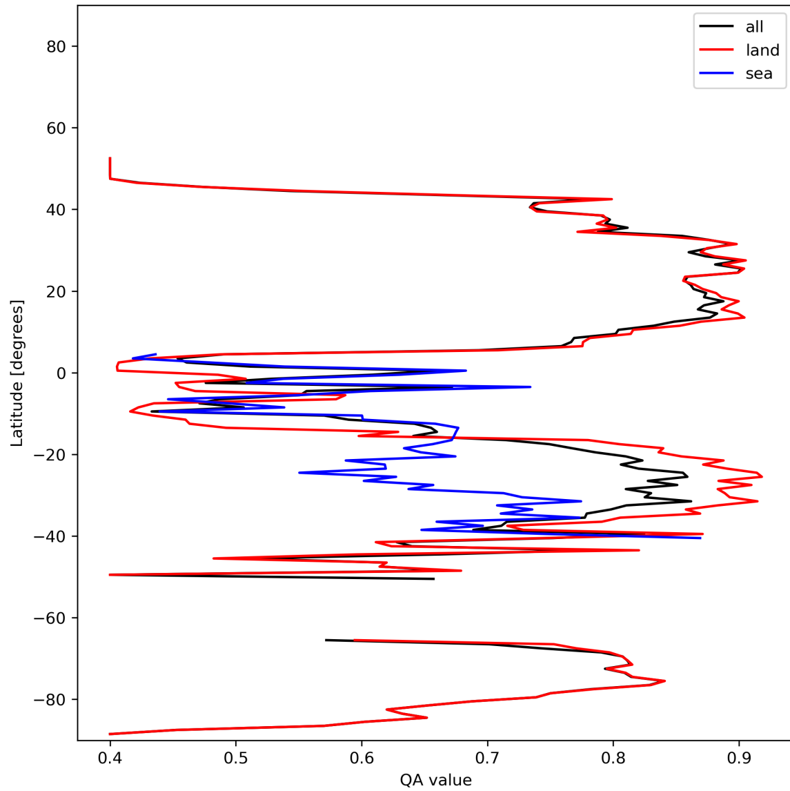
Figure 11: Zonal average of “QA value” for 2023-12-10 to 2023-12-12.
