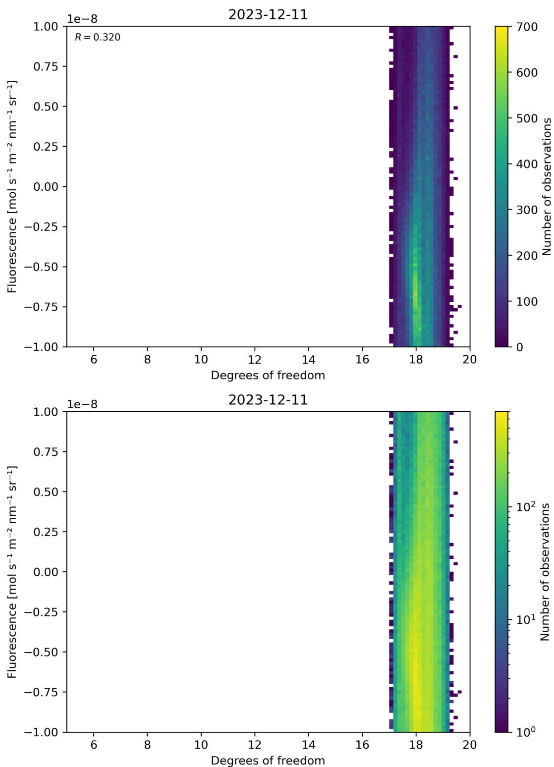
Figure 51: Scatter density plot of “Degrees of freedom” against “Fluorescence” for 2023-12-10 to 2023-12-12.
