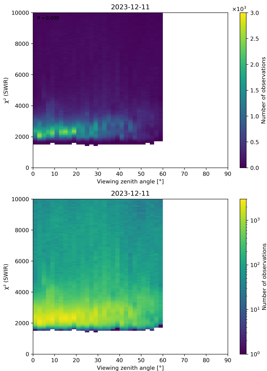
Figure 106: Scatter density plot of “Viewing zenith angle” against “ \chi^2 (SWIR)” for 2023-12-10 to 2023-12-12.
