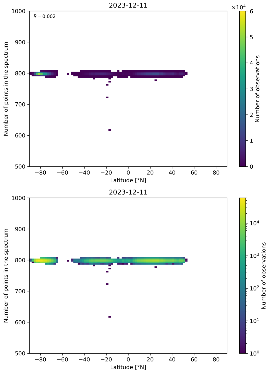
Figure 61: Scatter density plot of “Latitude” against “Number of points in the spectrum” for 2023-12-10 to 2023-12-12.
