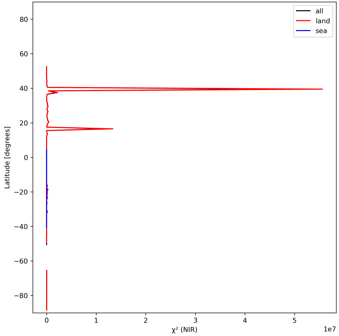
Figure 18: Zonal average of “ \chi^2 (NIR)” for 2023-12-10 to 2023-12-12.
