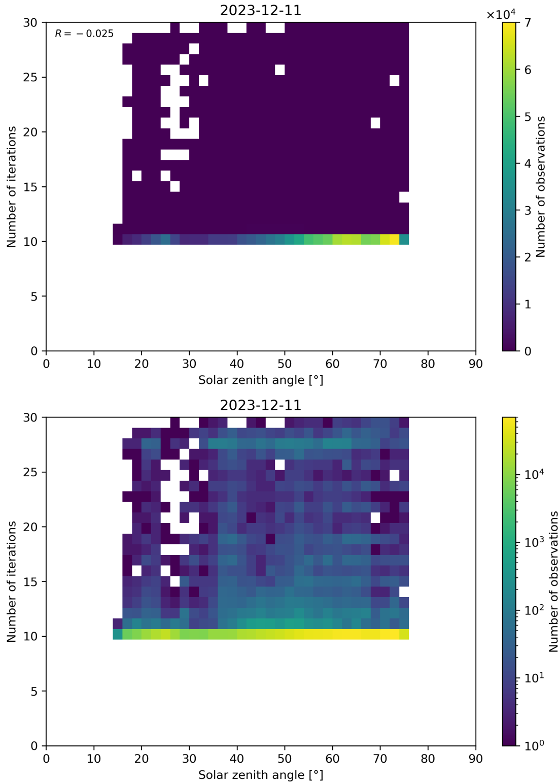
Figure 102: Scatter density plot of “Solar zenith angle” against “Number of iterations” for 2023-12-10 to 2023-12-12.
