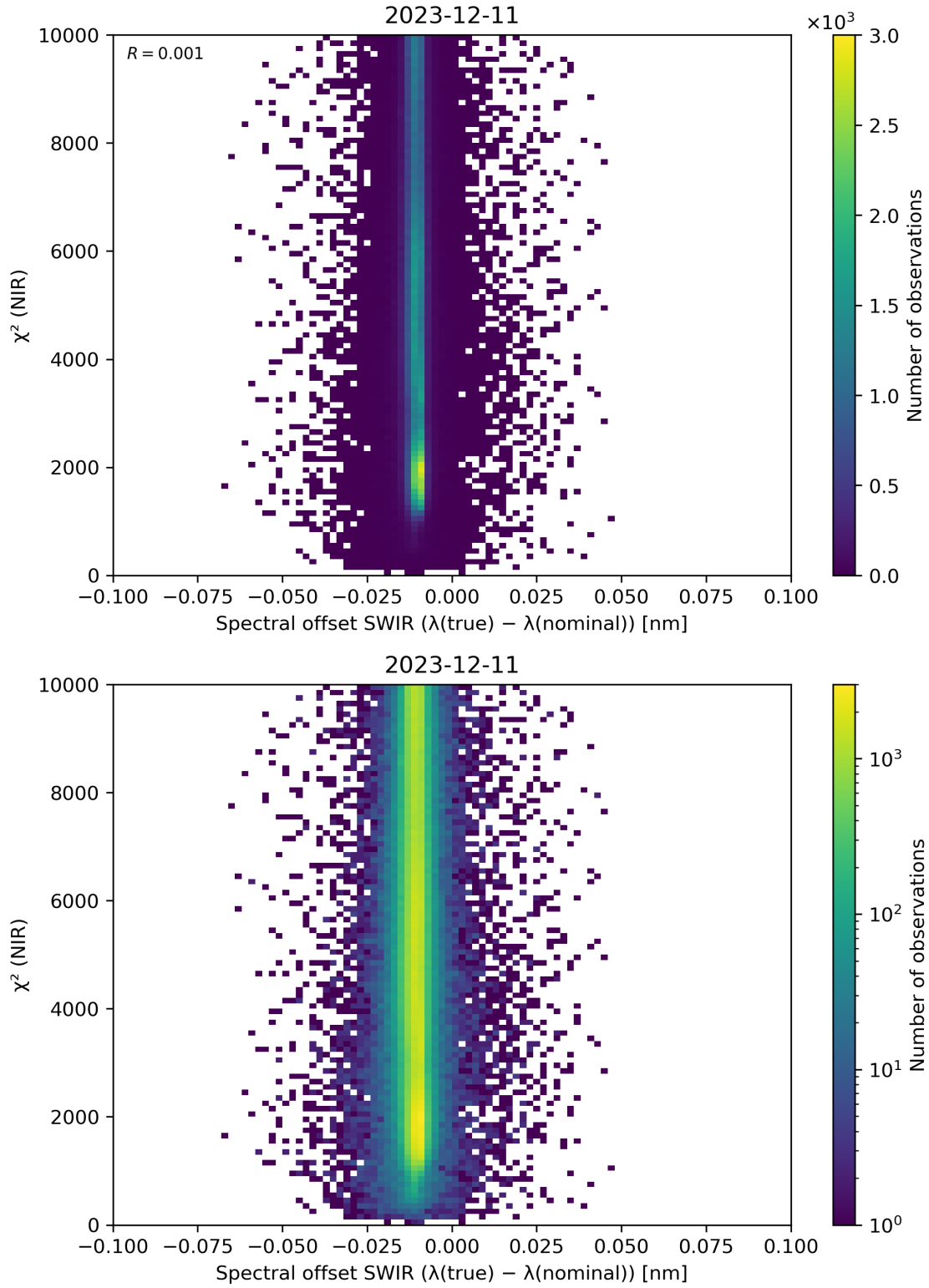
Figure 117: Scatter density plot of “Spectral offset SWIR ( \lambda(\text{true}) - \lambda(\text{nominal}) )” against “ \chi^2 (NIR)” for 2023-12-10 to 2023-12-12.
