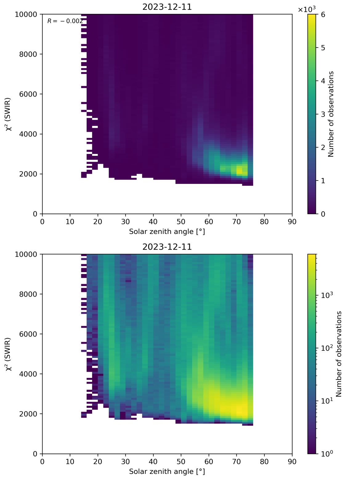
Figure 95: Scatter density plot of “Solar zenith angle” against “ \chi^2 (SWIR)” for 2023-12-10 to 2023-12-12.
