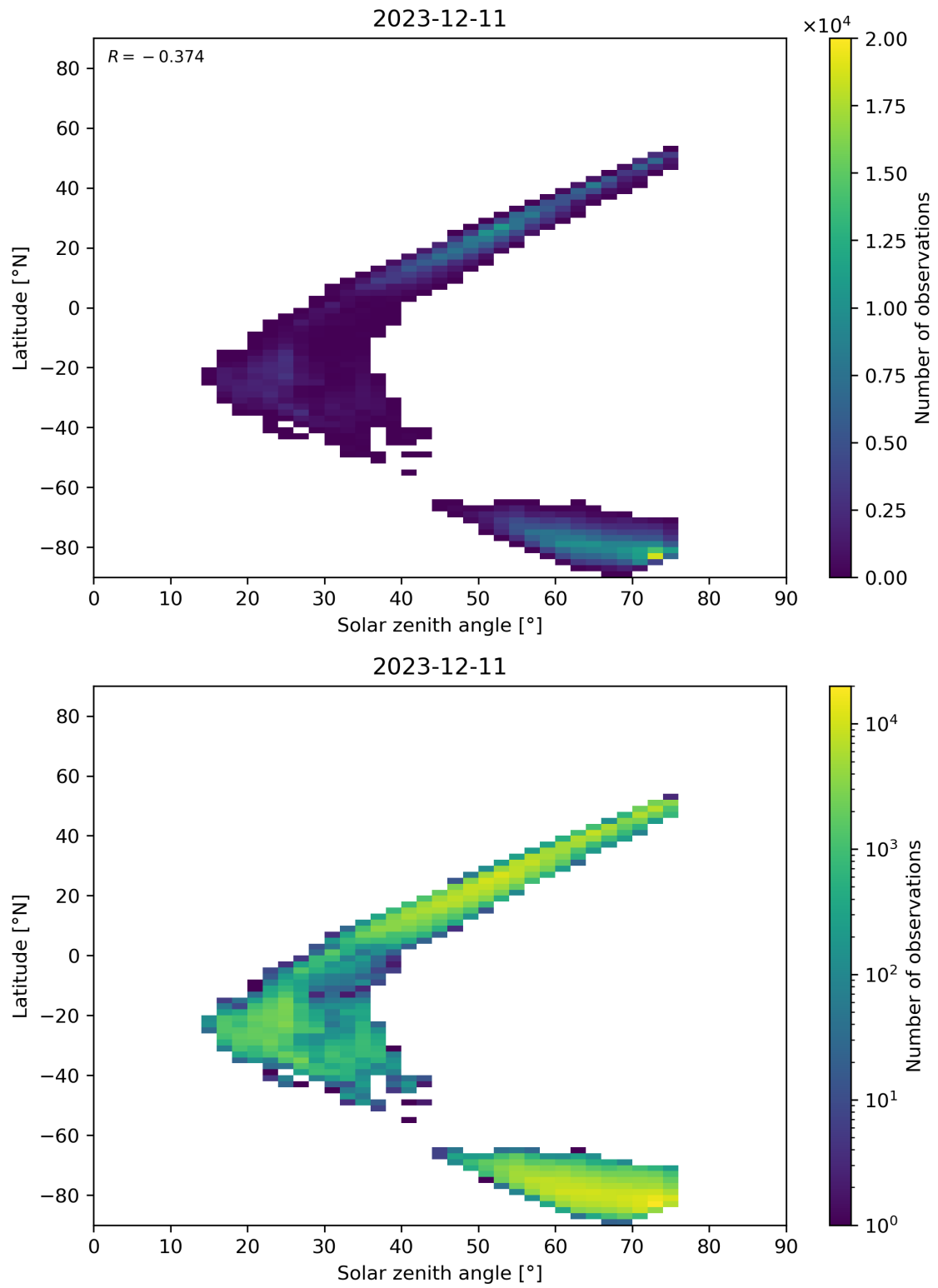
Figure 98: Scatter density plot of “Solar zenith angle” against “Latitude” for 2023-12-10 to 2023-12-12.
