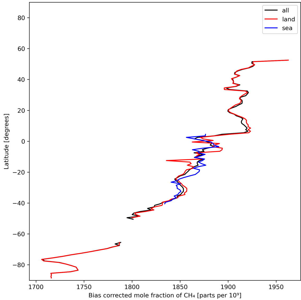
Figure 14: Zonal average of “Bias corrected mole fraction of CH 4 ” for 2023-12-10 to 2023-12-12.
