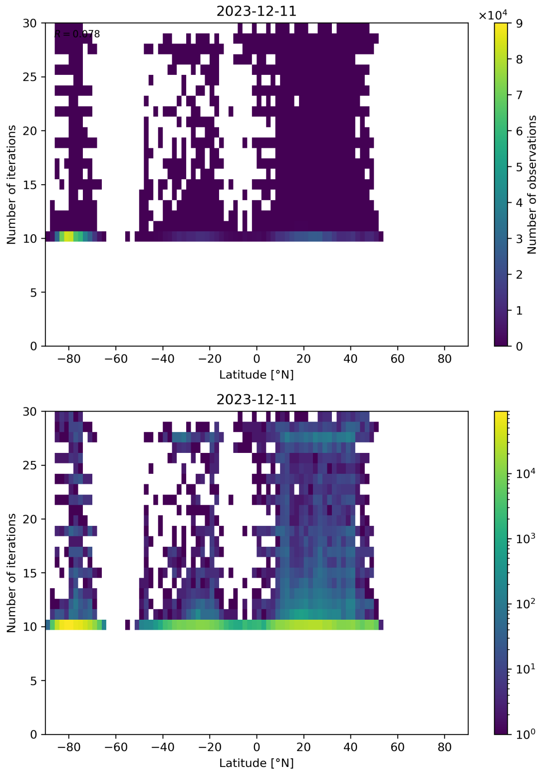
Figure 60: Scatter density plot of “Latitude” against “Number of iterations” for 2023-12-10 to 2023-12-12.
