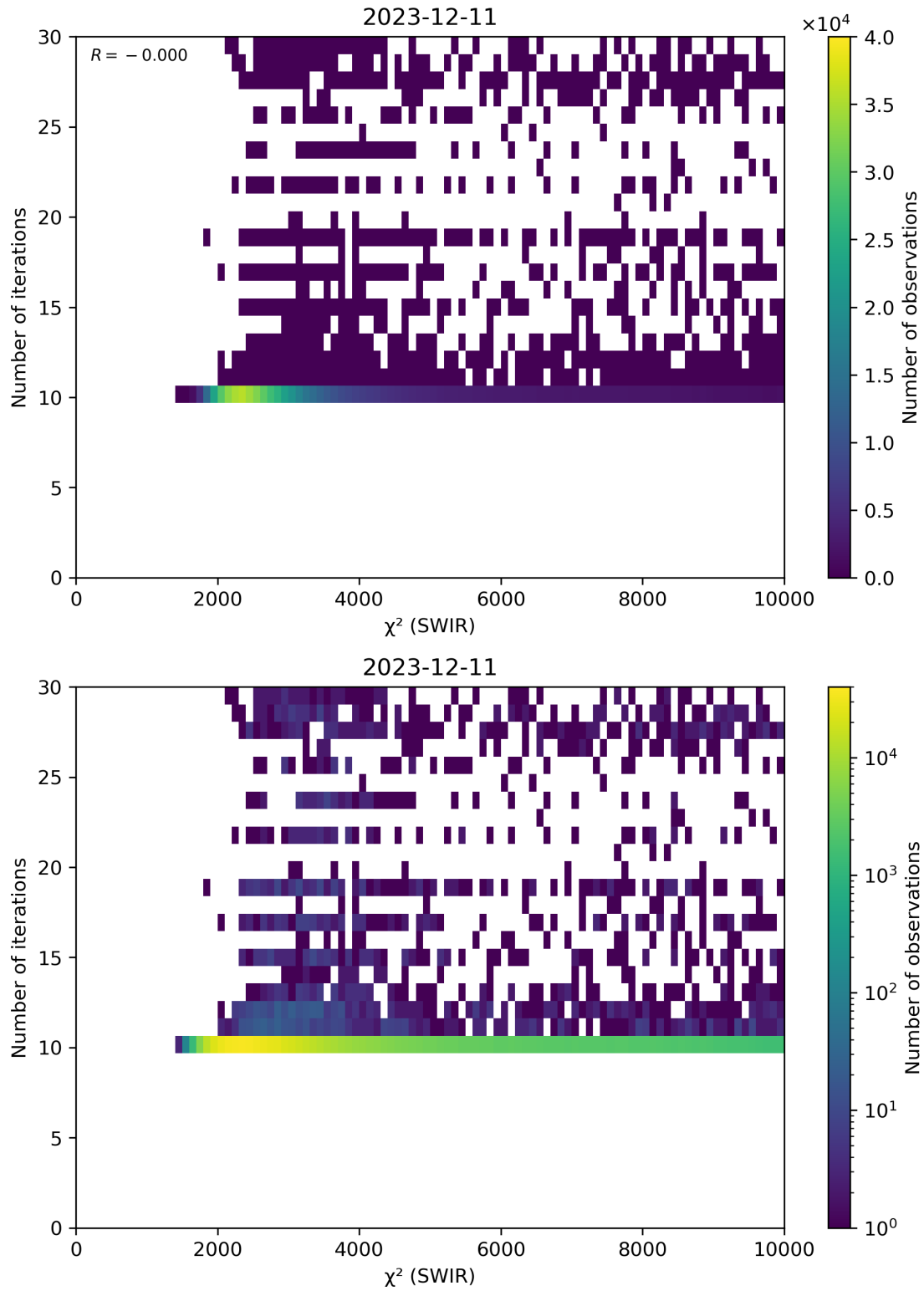
Figure 50: Scatter density plot of “ \chi^2 (SWIR)” against “Number of iterations” for 2023-12-10 to 2023-12-12.
