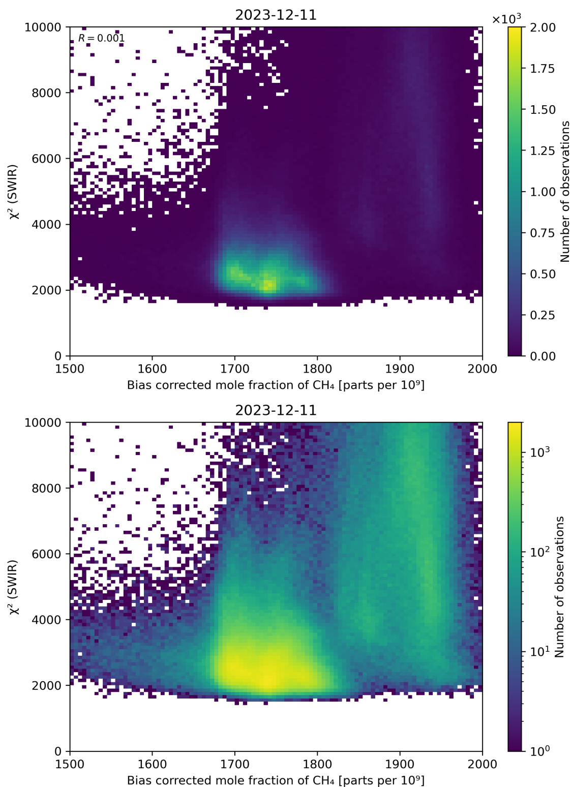
Figure 64: Scatter density plot of “Bias corrected mole fraction of CH 4 ” against “ \chi^2 (SWIR)” for 2023-12-10 to 2023-12-12.
