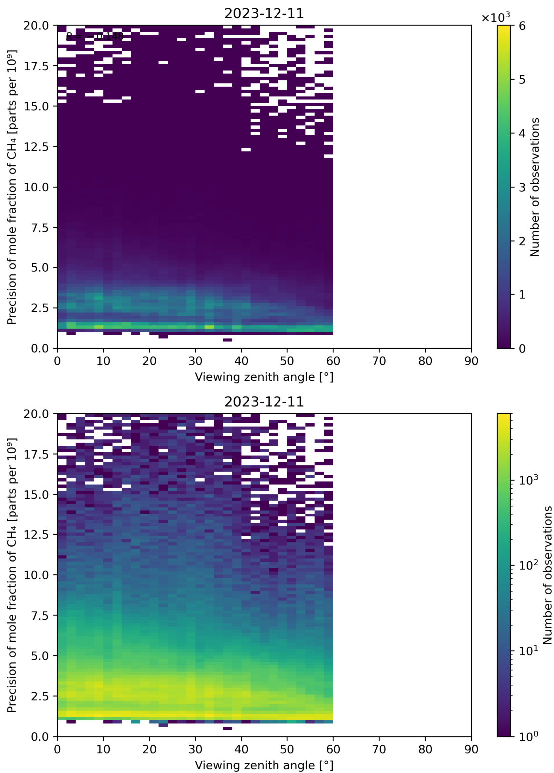
Figure 112: Scatter density plot of “Viewing zenith angle” against “Precision of mole fraction of CH 4 ” for 2023-12-10 to 2023-12-12.
