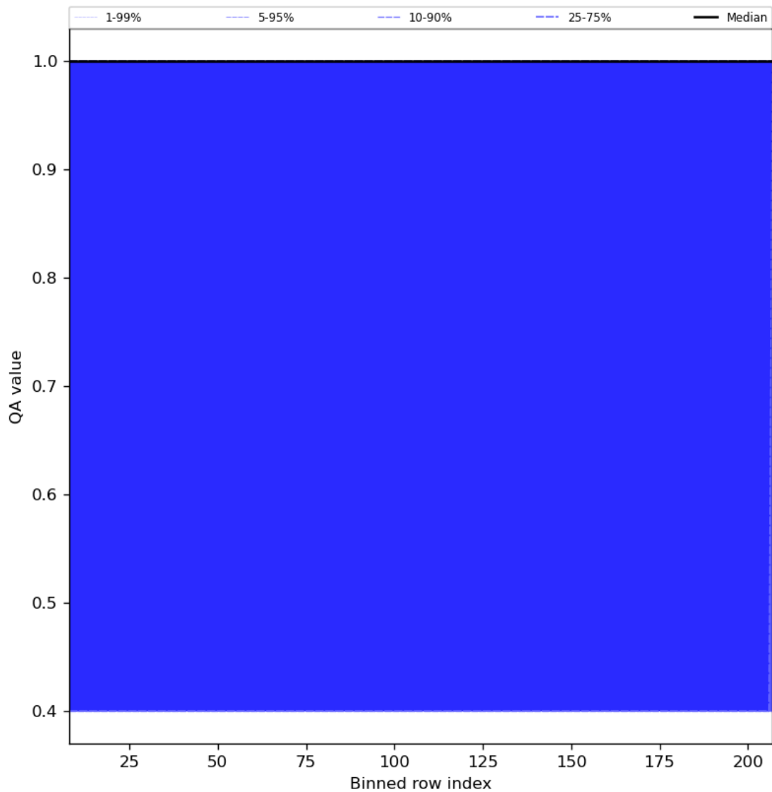
Figure 33: Along track statistics of “QA value” for 2023-12-10 to 2023-12-12
