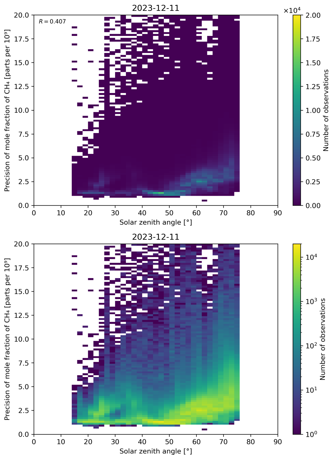
Figure 101: Scatter density plot of “Solar zenith angle” against “Precision of mole fraction of CH 4 ” for 2023-12-10 to 2023-12-12.
