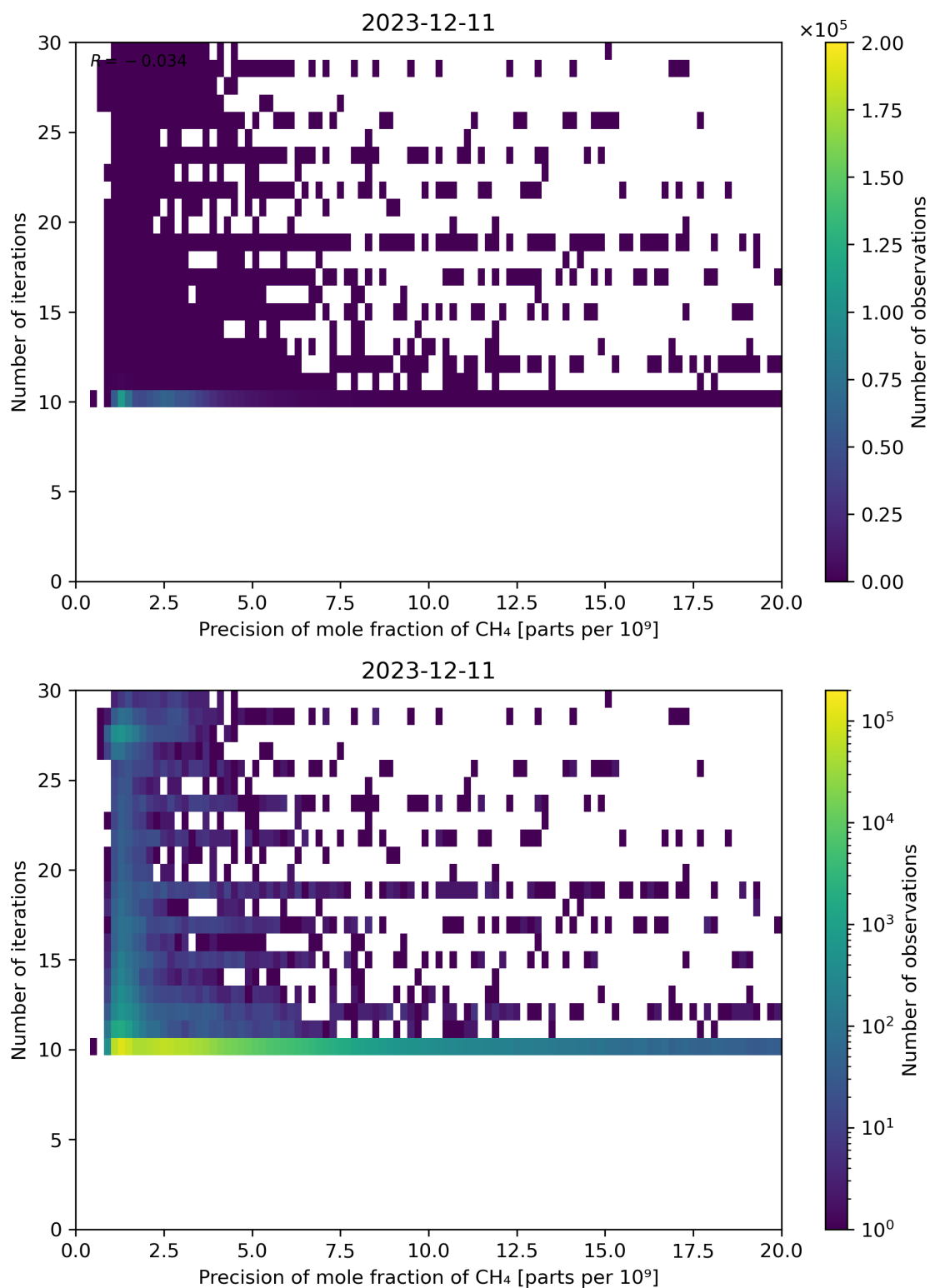
Figure 83: Scatter density plot of “Precision of mole fraction of CH 4 ” against “Number of iterations” for 2023-12-10 to 2023-12-12.
