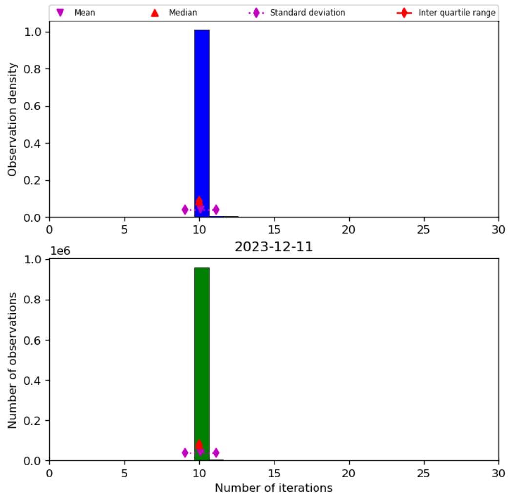
Figure 31: Histogram of “Number of iterations” for 2023-12-10 to 2023-12-12
