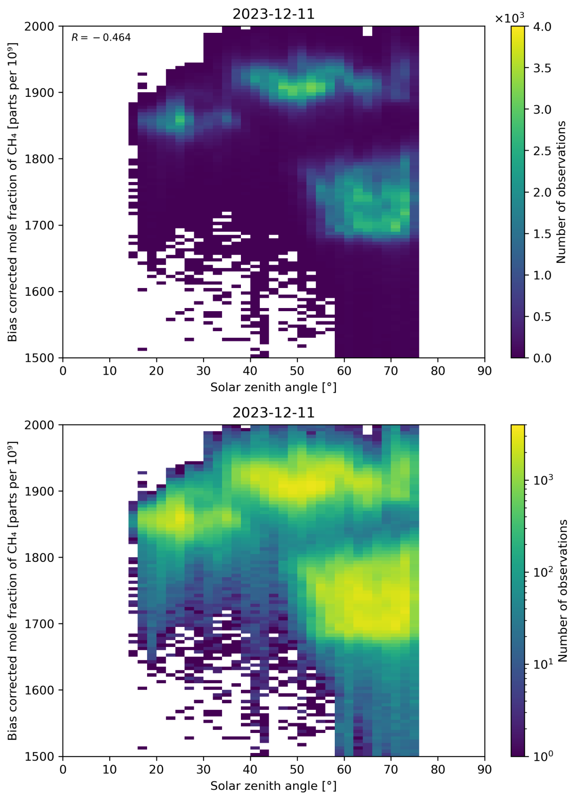
Figure 100: Scatter density plot of “Solar zenith angle” against “Bias corrected mole fraction of \text{CH}_4 ” for 2023-12-10 to 2023-12-12.
