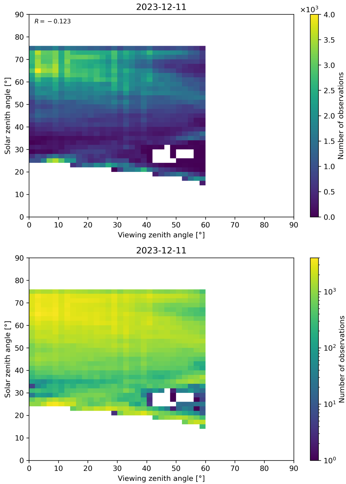
Figure 115: Scatter density plot of “Viewing zenith angle” against “Solar zenith angle” for 2023-12-10 to 2023-12-12.
