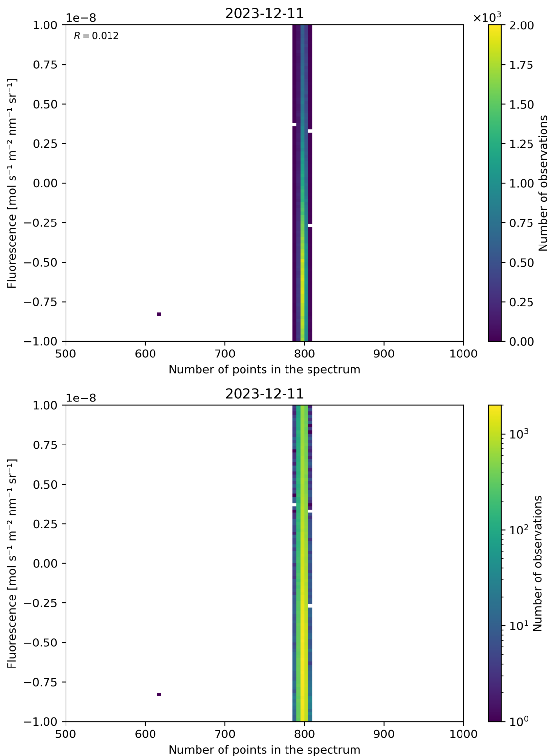
Figure 91: Scatter density plot of “Number of points in the spectrum” against “Fluorescence” for 2023-12-10 to 2023-12-12.
