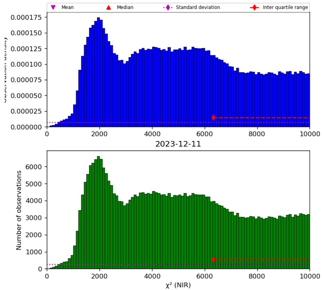
Figure 29: Histogram of “ \chi^2 (NIR)” for 2023-12-10 to 2023-12-12
