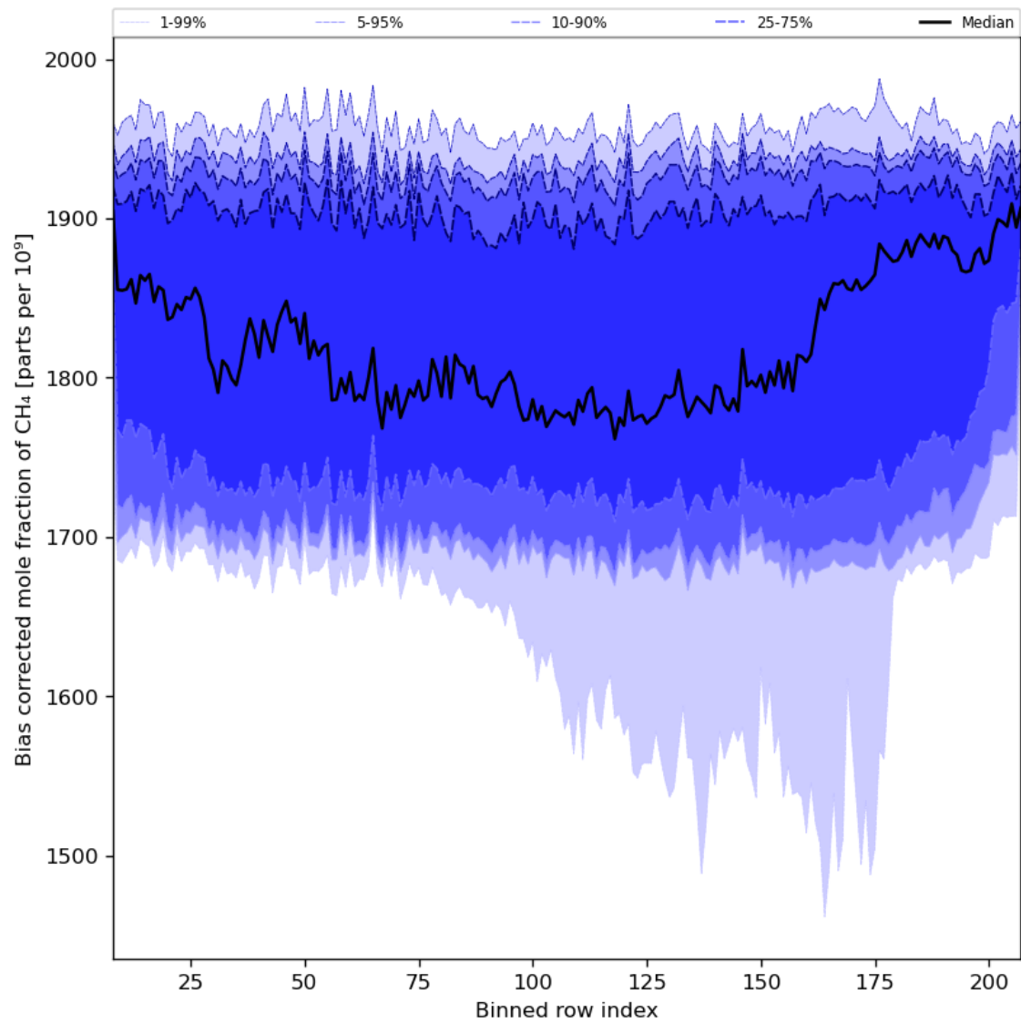
Figure 36: Along track statistics of “Bias corrected mole fraction of CH 4 ” for 2023-12-10 to 2023-12-12
