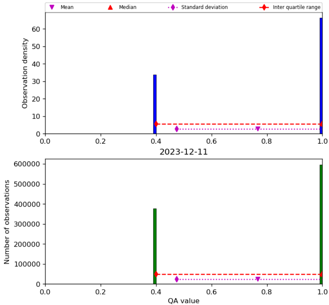
Figure 22: Histogram of “QA value” for 2023-12-10 to 2023-12-12
