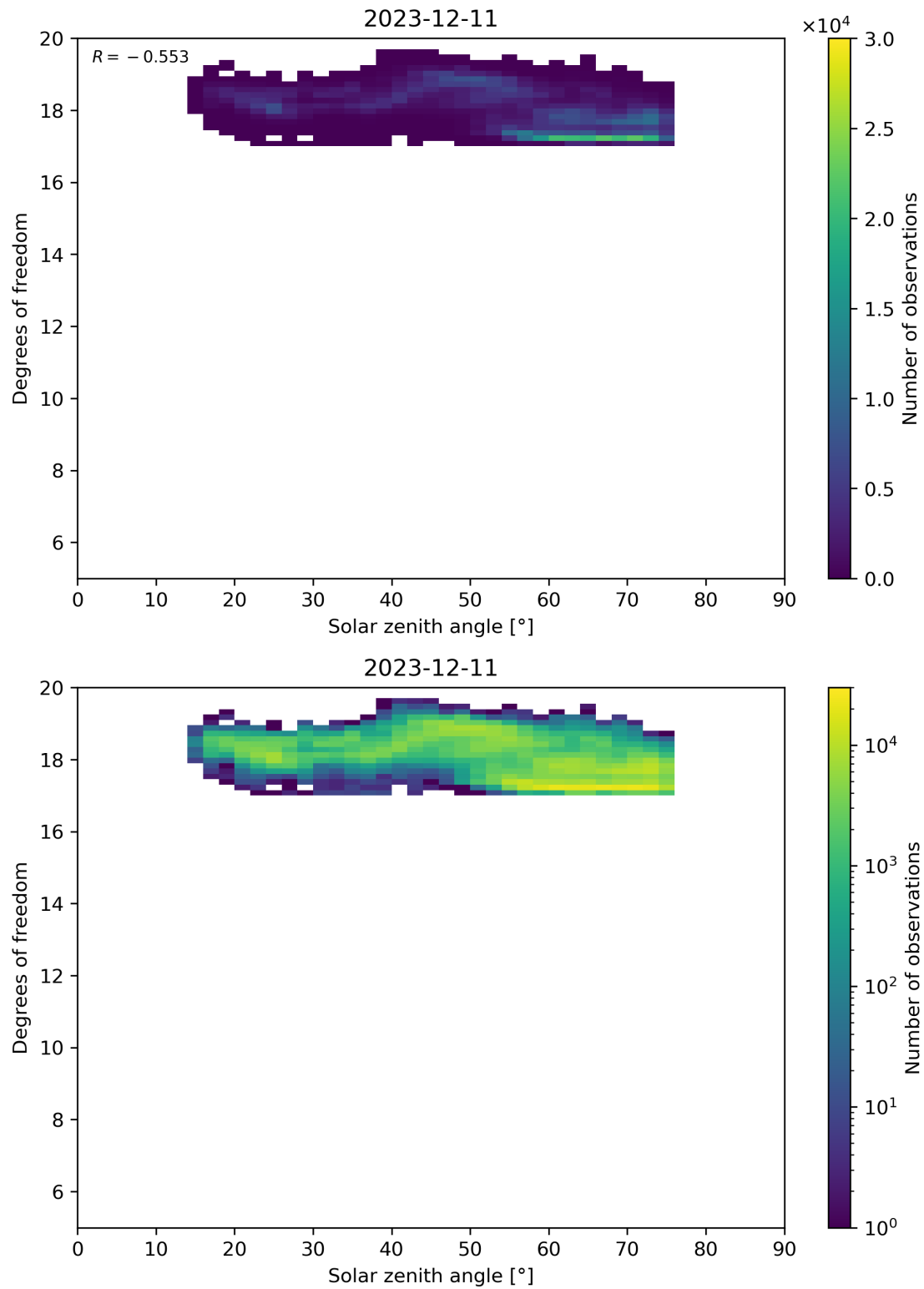
Figure 96: Scatter density plot of “Solar zenith angle” against “Degrees of freedom” for 2023-12-10 to 2023-12-12.
