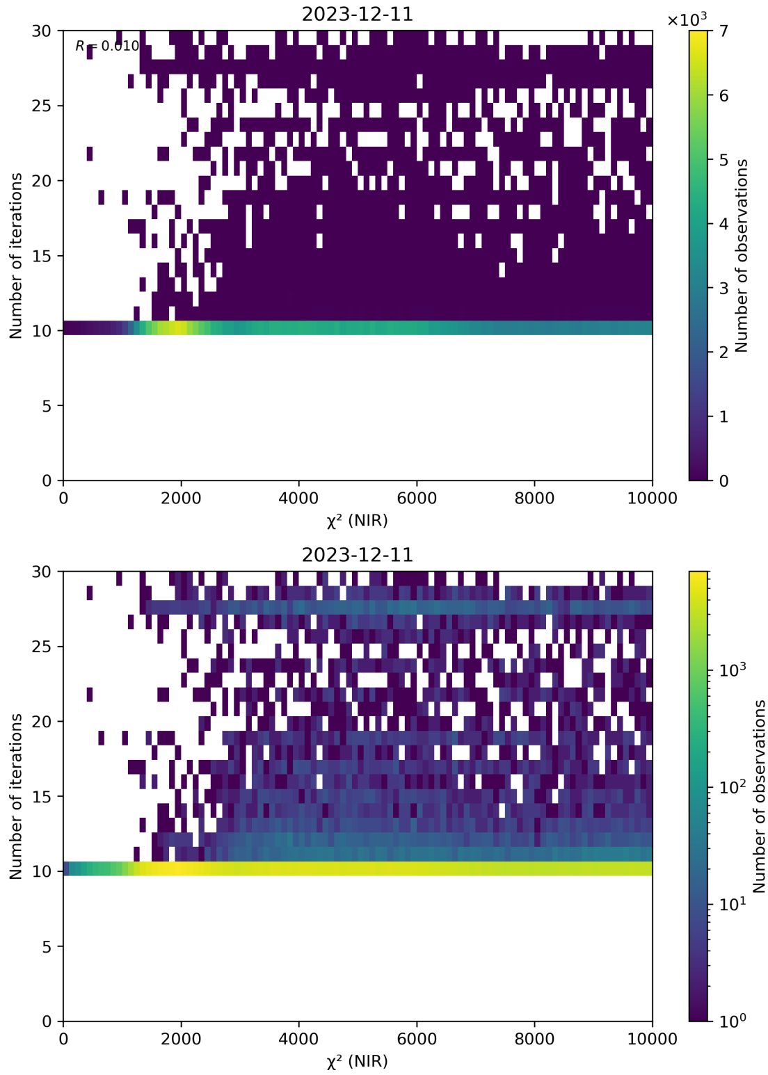
Figure 46: Scatter density plot of “ \chi^2 (NIR)” against “Number of iterations” for 2023-12-10 to 2023-12-12.
