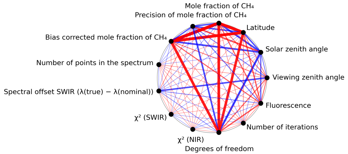
Figure 1: Map of correlation graph for 2023-12-10 to 2023-12-12.
