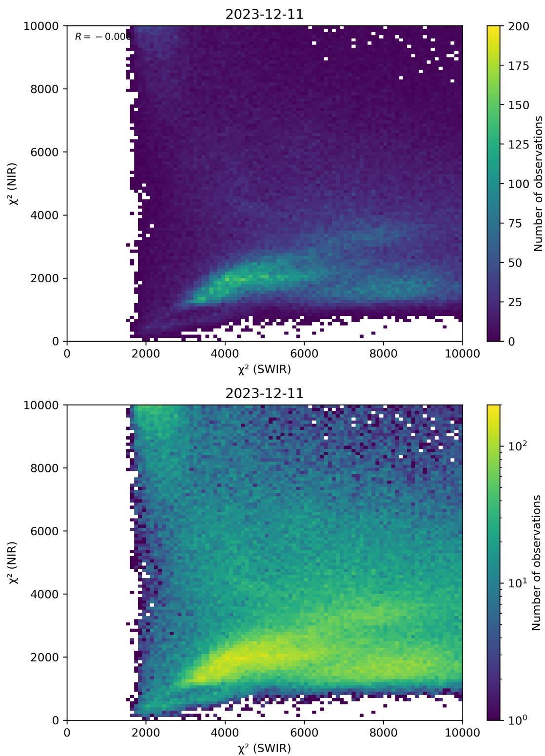
Figure 47: Scatter density plot of “ \chi^2 (SWIR)” against “ \chi^2 (NIR)” for 2023-12-10 to 2023-12-12.
