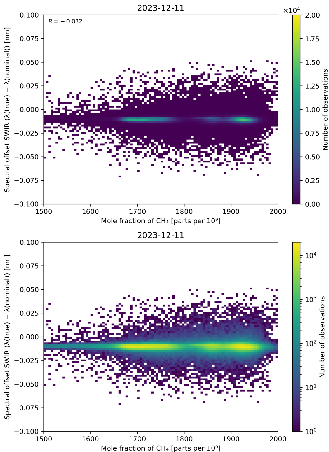
Figure 86: Scatter density plot of “Mole fraction of CH 4 ” against “Spectral offset SWIR ( \lambda(\text{true}) - \lambda(\text{nominal}) )” for 2023-12-10 to 2023-12-12.
