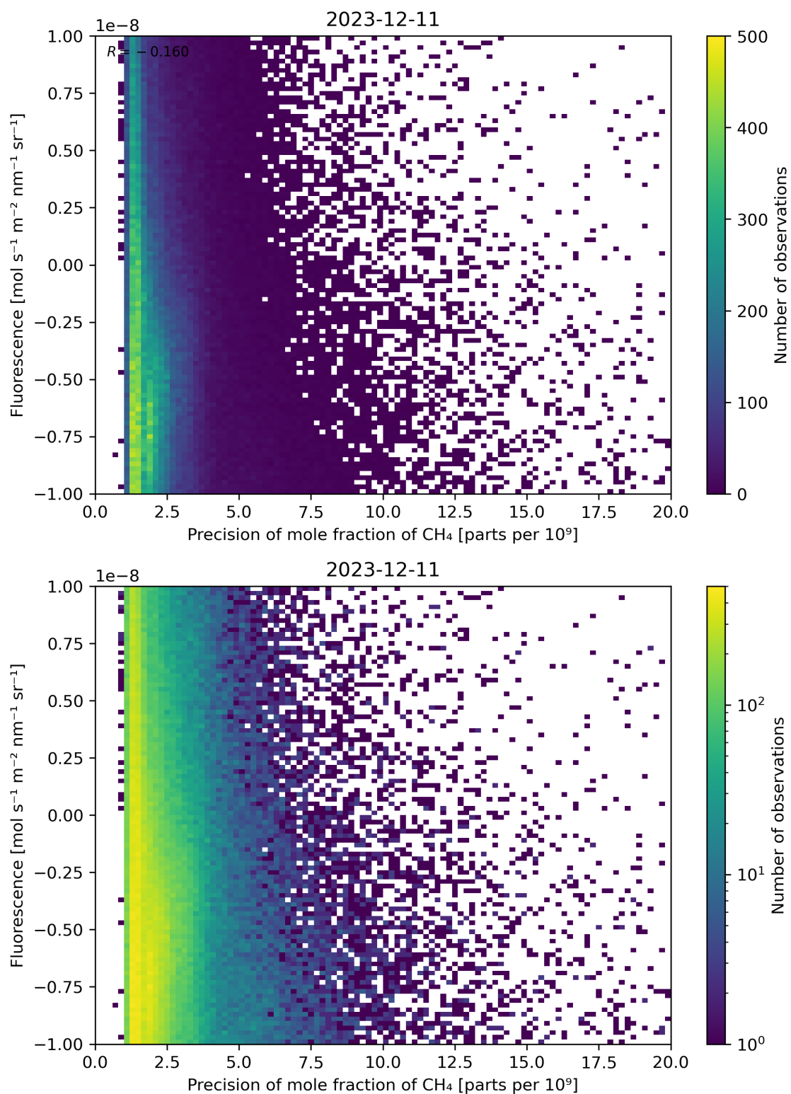
Figure 81: Scatter density plot of “Precision of mole fraction of \text{CH}_4 ” against “Fluorescence” for 2023-12-10 to 2023-12-12.
