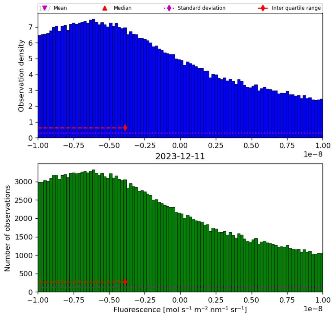
Figure 32: Histogram of “Fluorescence” for 2023-12-10 to 2023-12-12
