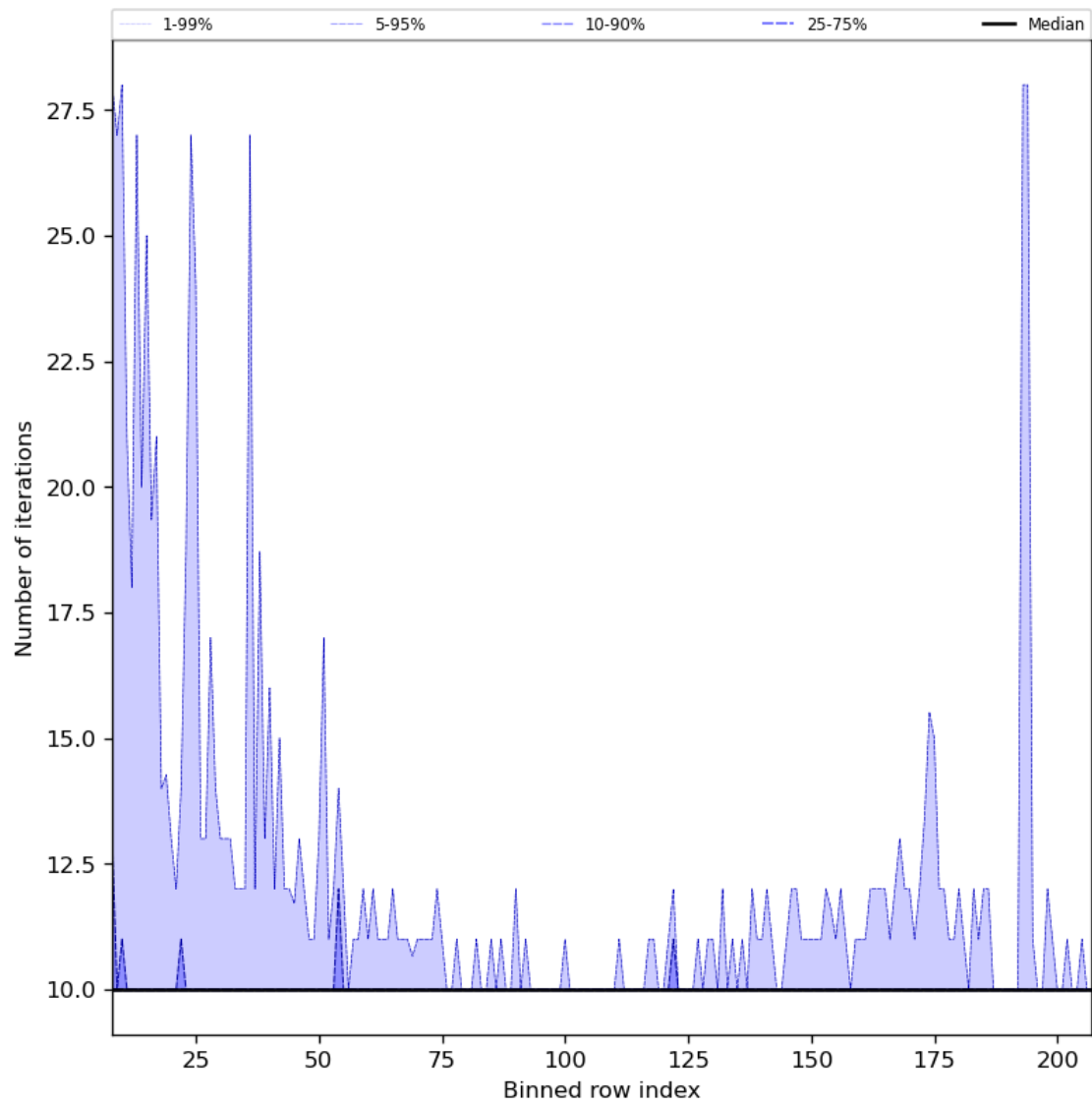
Figure 42: Along track statistics of “Number of iterations” for 2023-12-10 to 2023-12-12
