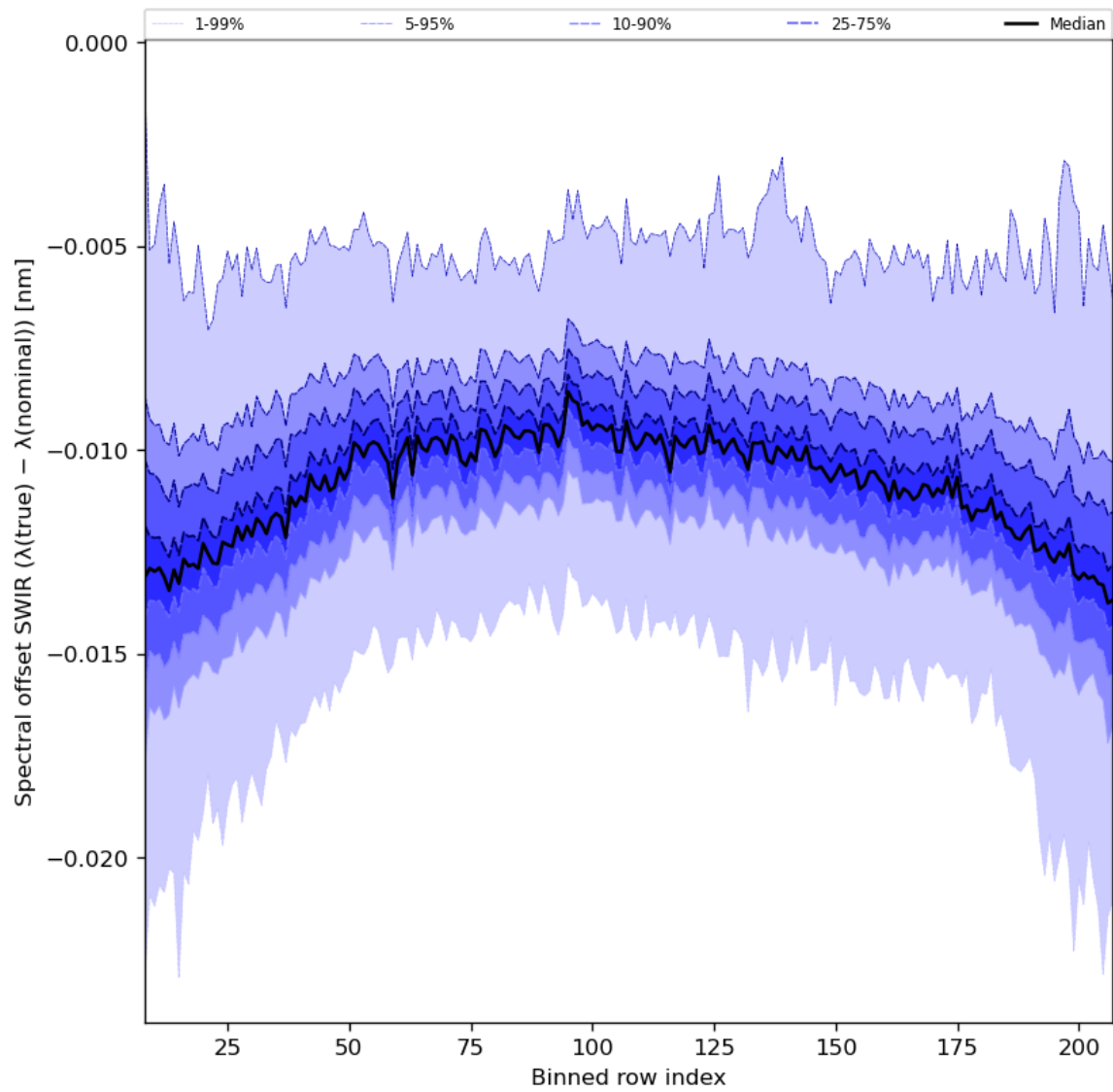
Figure 38: Along track statistics of “Spectral offset SWIR ( \lambda(\text{true}) - \lambda(\text{nominal}) )” for 2023-12-10 to 2023-12-12
