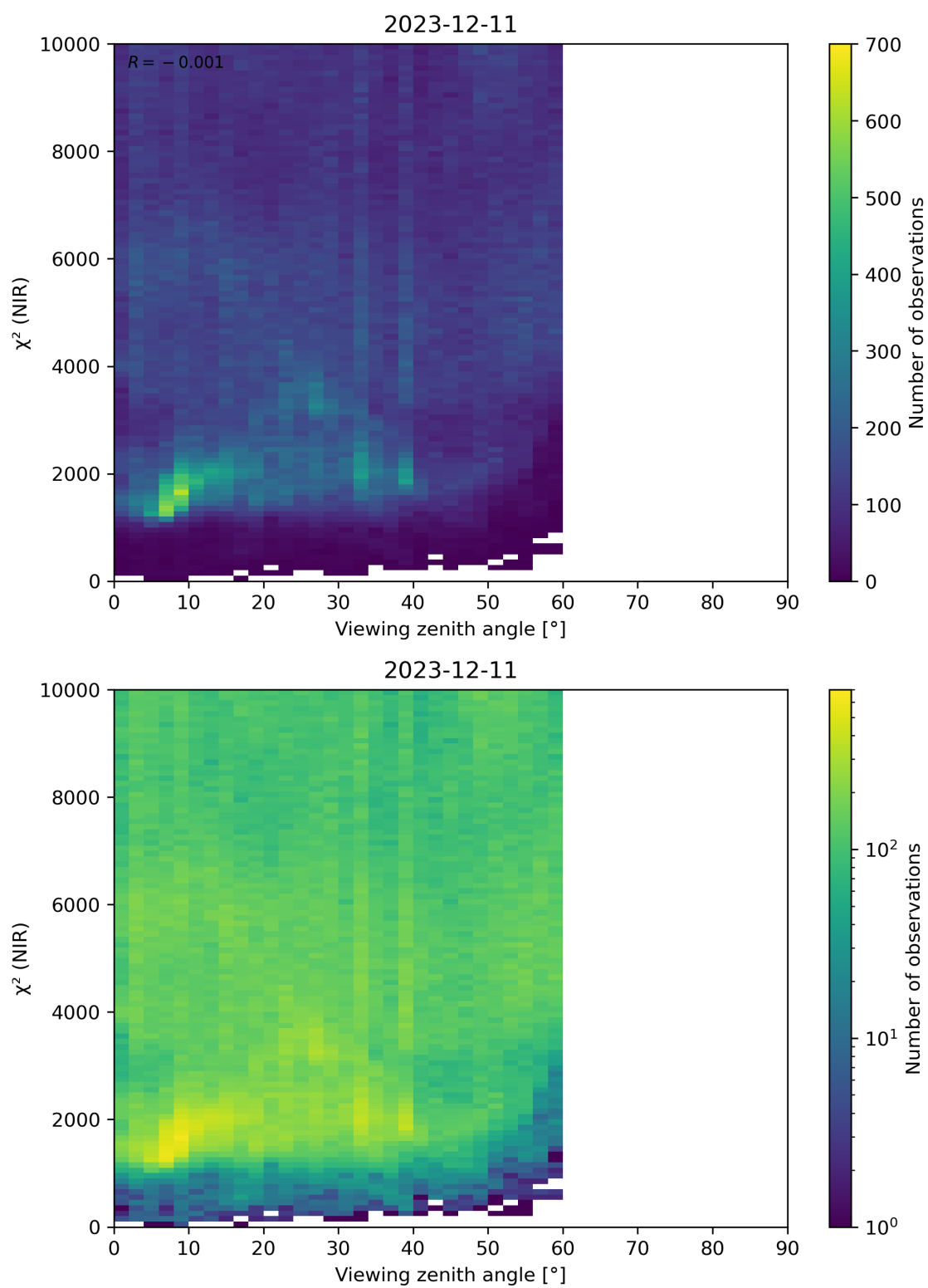
Figure 105: Scatter density plot of “Viewing zenith angle” against “ \chi^2 (NIR)” for 2023-12-10 to 2023-12-12.
