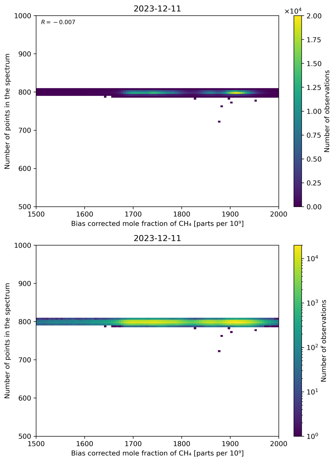
Figure 68: Scatter density plot of “Bias corrected mole fraction of CH 4 ” against “Number of points in the spectrum” for 2023-12-10 to 2023-12-12.
