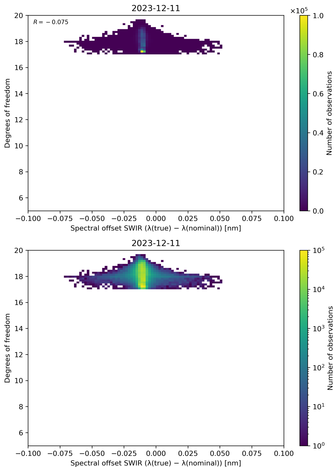
Figure 119: Scatter density plot of “Spectral offset SWIR ( \lambda(\text{true}) - \lambda(\text{nominal}) )” against “Degrees of freedom” for 2023-12-10 to 2023-12-12.
