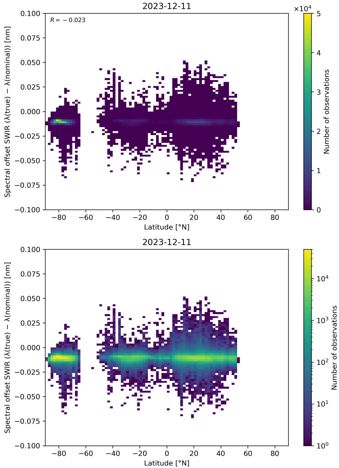
Figure 62: Scatter density plot of “Latitude” against “Spectral offset SWIR ( \lambda(\text{true}) - \lambda(\text{nominal}) )” for 2023-12-10 to 2023-12-12.
