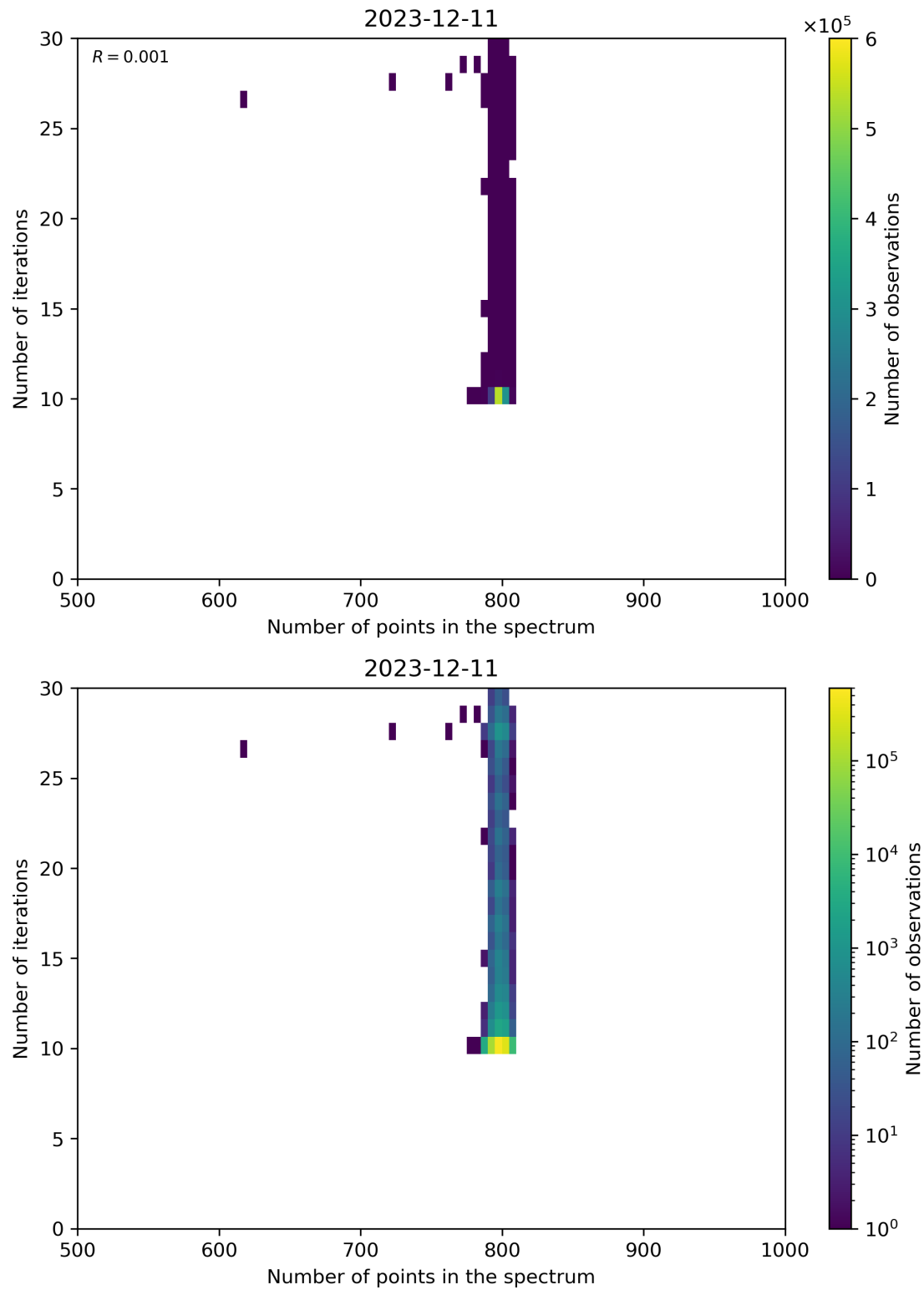
Figure 92: Scatter density plot of “Number of points in the spectrum” against “Number of iterations” for 2023-12-10 to 2023-12-12.
