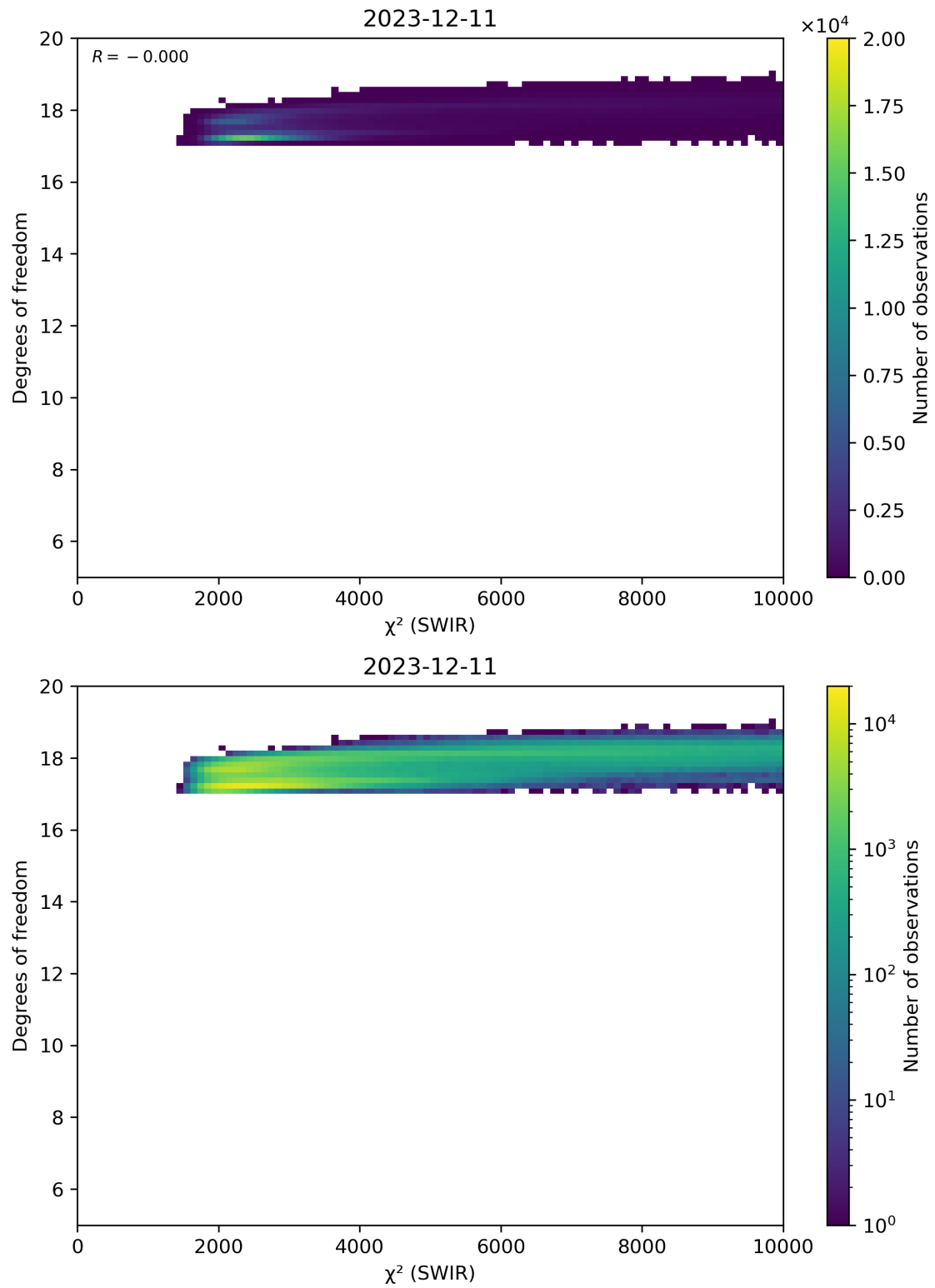
Figure 48: Scatter density plot of “ \chi^2 (SWIR)” against “Degrees of freedom” for 2023-12-10 to 2023-12-12.
