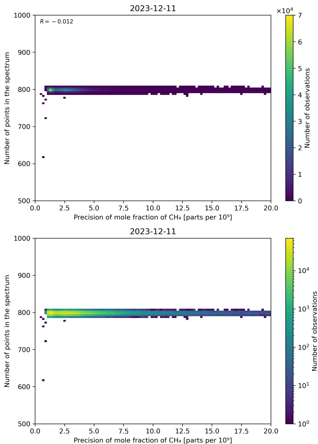
Figure 84: Scatter density plot of “Precision of mole fraction of CH 4 ” against “Number of points in the spectrum” for 2023-12-10 to 2023-12-12.
