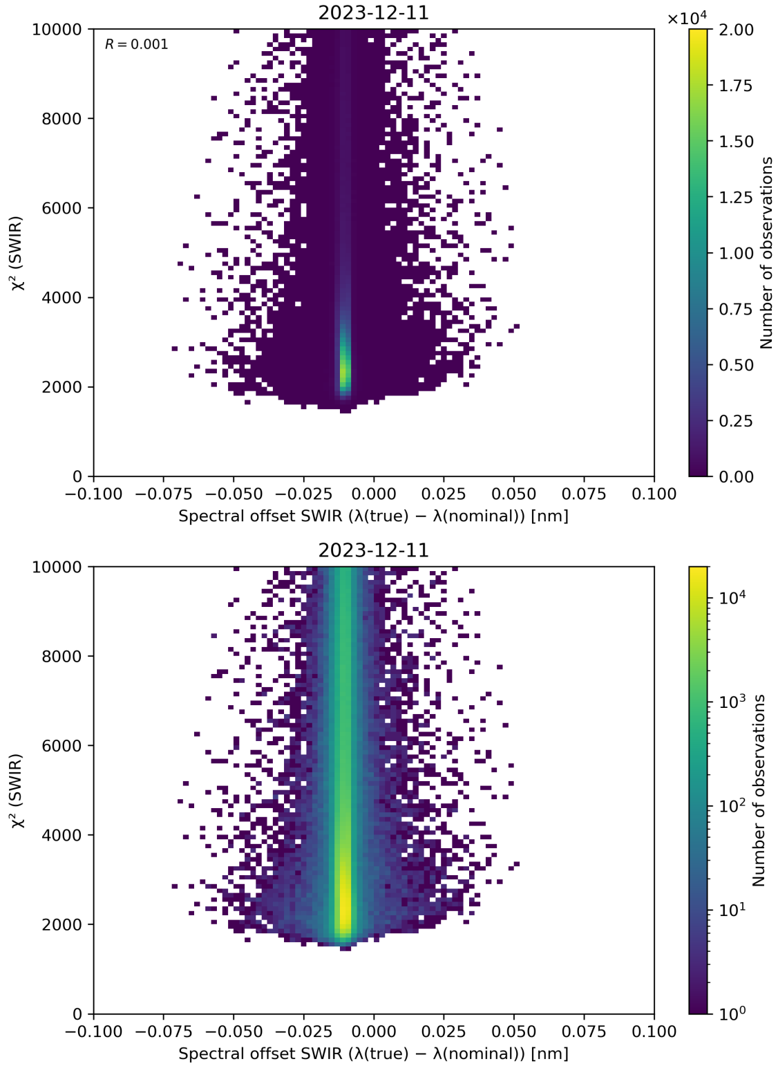
Figure 118: Scatter density plot of “Spectral offset SWIR ( \lambda(\text{true}) - \lambda(\text{nominal}) )” against “ \chi^2 (SWIR)” for 2023-12-10 to 2023-12-12.
