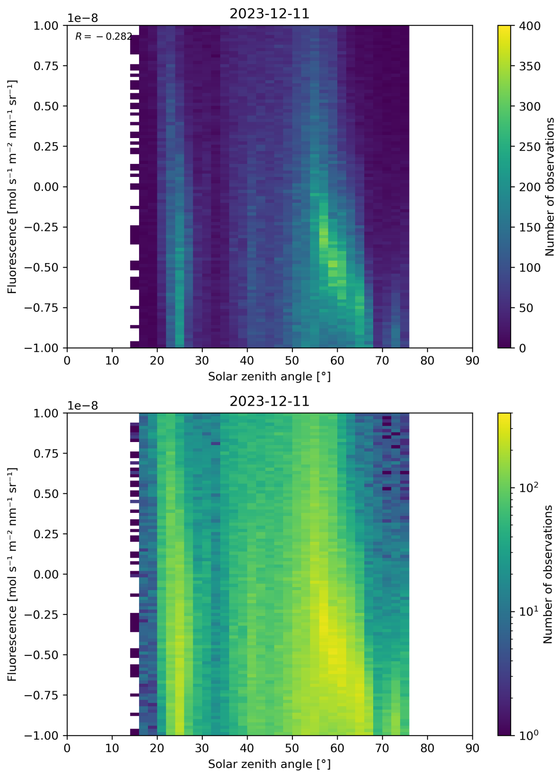
Figure 97: Scatter density plot of “Solar zenith angle” against “Fluorescence” for 2023-12-10 to 2023-12-12.
