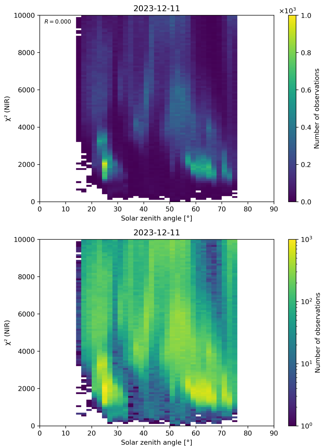
Figure 94: Scatter density plot of “Solar zenith angle” against “ \chi^2 (NIR)” for 2023-12-10 to 2023-12-12.
