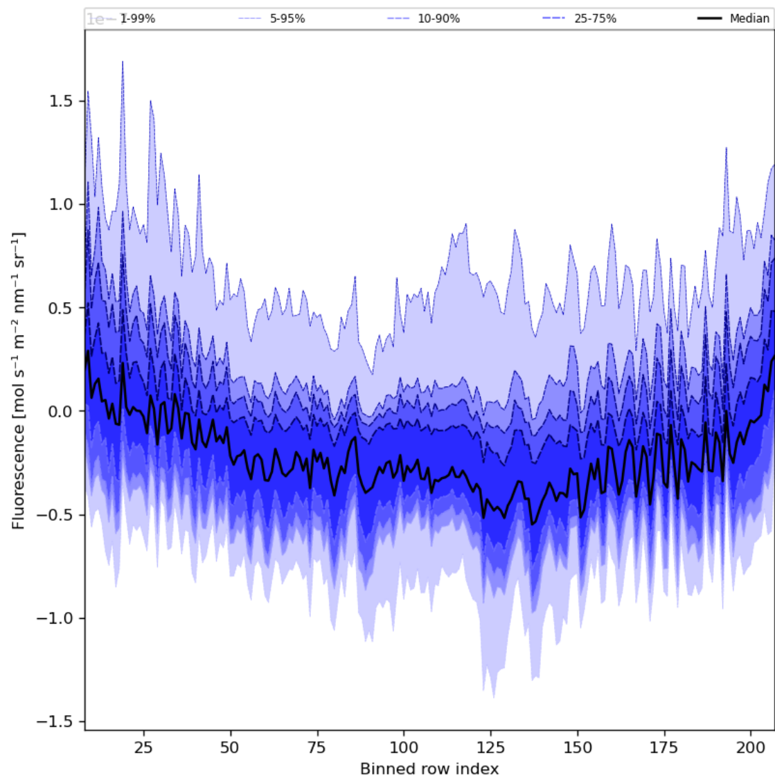
Figure 43: Along track statistics of “Fluorescence” for 2023-12-10 to 2023-12-12
