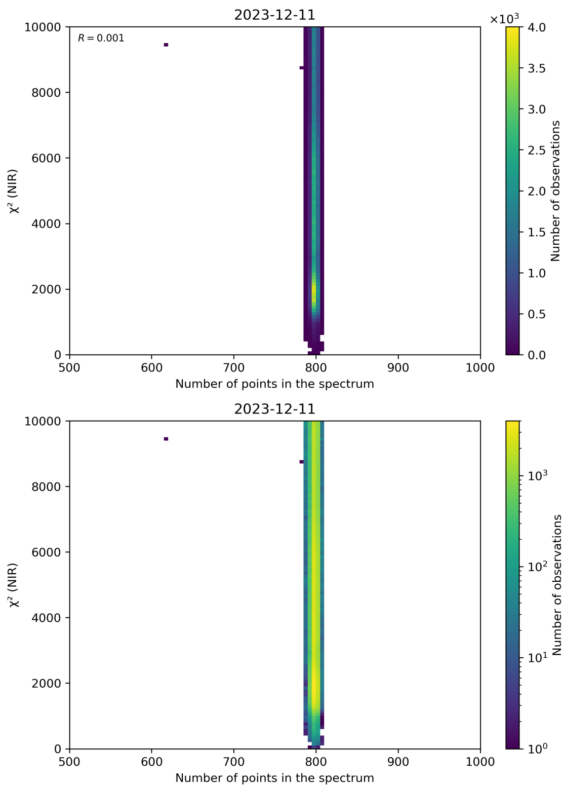
Figure 88: Scatter density plot of “Number of points in the spectrum” against “ \chi^2 (NIR)” for 2023-12-10 to 2023-12-12.
