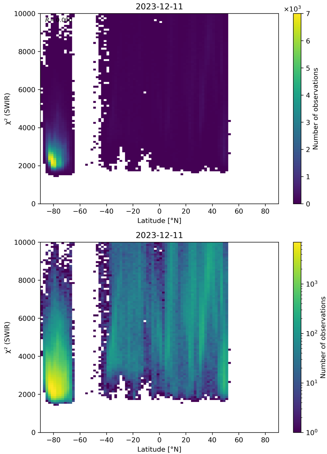
Figure 54: Scatter density plot of “Latitude” against “ \chi^2 (SWIR)” for 2023-12-10 to 2023-12-12.
