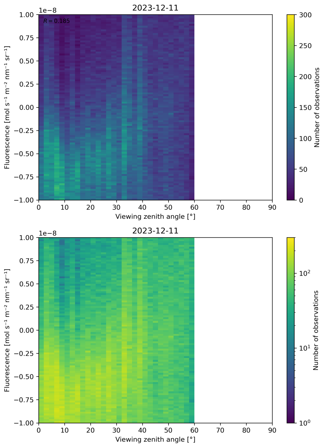
Figure 108: Scatter density plot of “Viewing zenith angle” against “Fluorescence” for 2023-12-10 to 2023-12-12.
