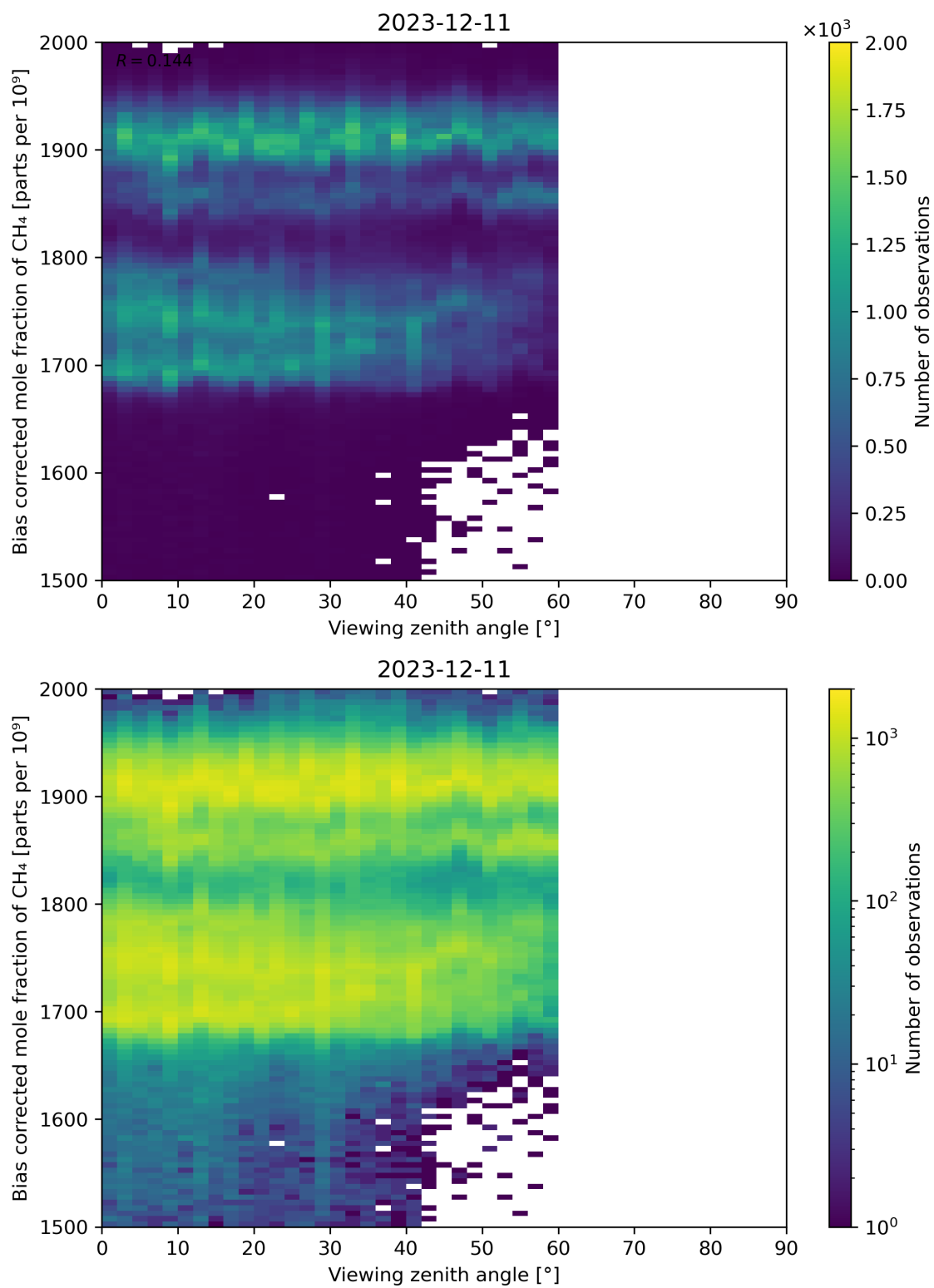
Figure 111: Scatter density plot of “Viewing zenith angle” against “Bias corrected mole fraction of CH 4 ” for 2023-12-10 to 2023-12-12.
