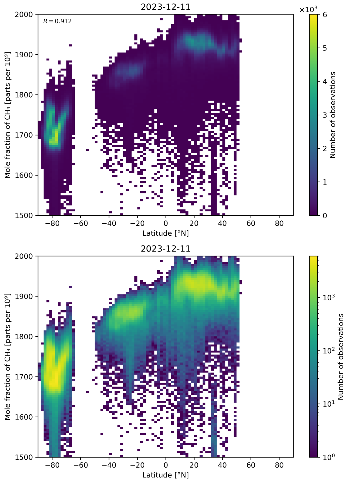
Figure 57: Scatter density plot of “Latitude” against “Mole fraction of CH 4 ” for 2023-12-10 to 2023-12-12.
