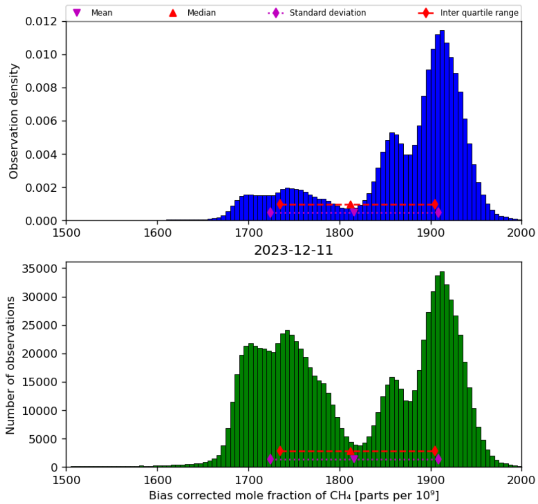
Figure 25: Histogram of “Bias corrected mole fraction of CH 4 ” for 2023-12-10 to 2023-12-12
