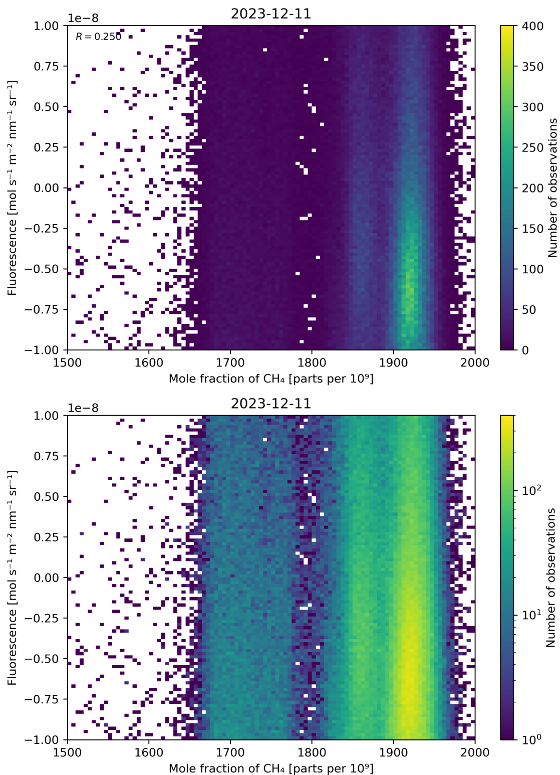
Figure 73: Scatter density plot of “Mole fraction of \text{CH}_4 ” against “Fluorescence” for 2023-12-10 to 2023-12-12.
