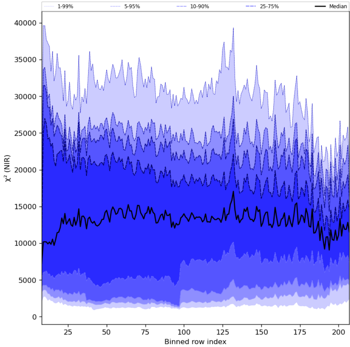
Figure 40: Along track statistics of “ \chi^2 (NIR)” for 2023-12-10 to 2023-12-12
