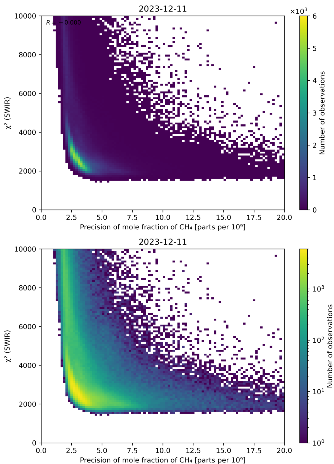
Figure 79: Scatter density plot of “Precision of mole fraction of CH 4 ” against “ \chi^2 (SWIR)” for 2023-12-10 to 2023-12-12.
