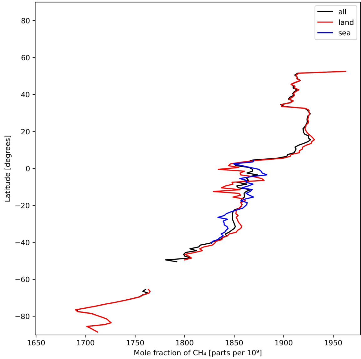
Figure 12: Zonal average of “Mole fraction of \text{CH}_4 ” for 2023-12-10 to 2023-12-12.
