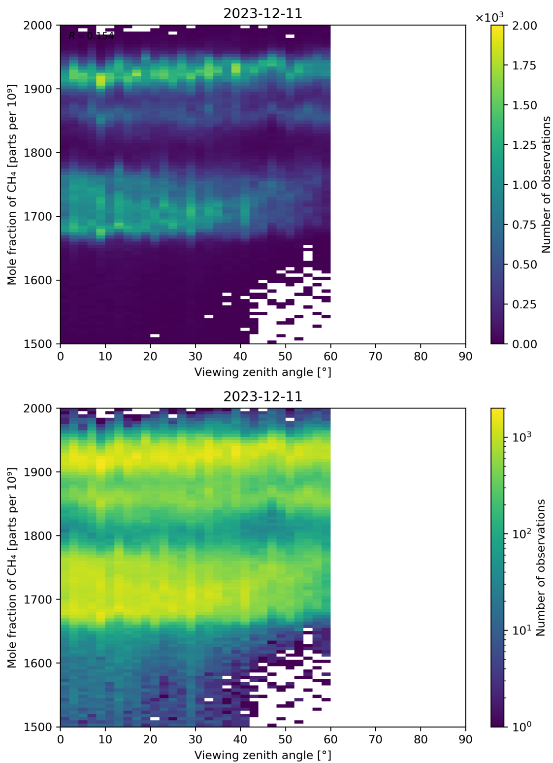
Figure 110: Scatter density plot of “Viewing zenith angle” against “Mole fraction of CH 4 ” for 2023-12-10 to 2023-12-12.
