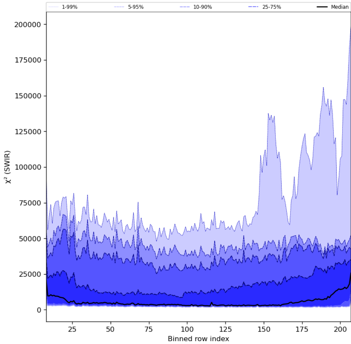
Figure 39: Along track statistics of “ \chi^2 (SWIR)” for 2023-12-10 to 2023-12-12
