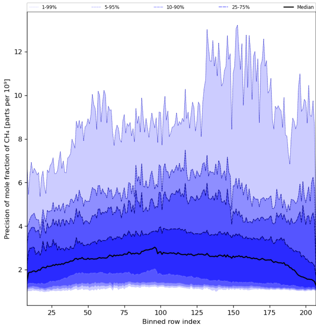
Figure 35: Along track statistics of “Precision of mole fraction of CH 4 ” for 2023-12-10 to 2023-12-12
