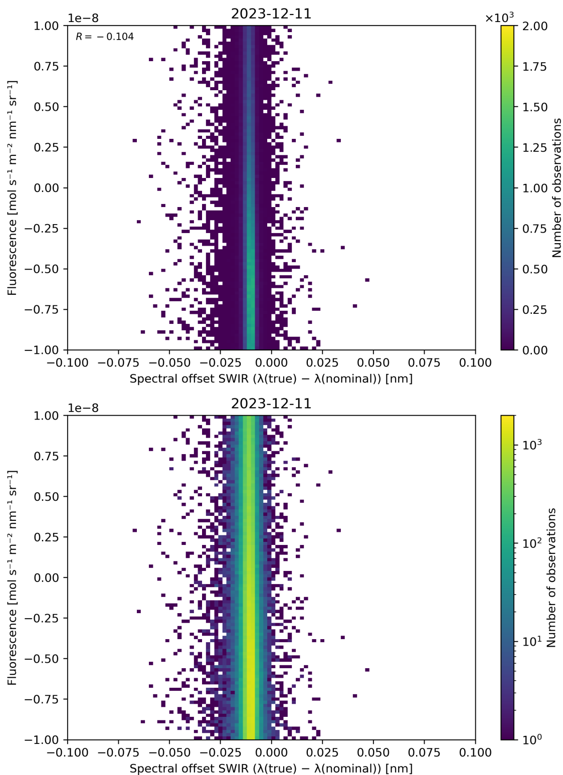
Figure 120: Scatter density plot of “Spectral offset SWIR ( \lambda(\text{true}) - \lambda(\text{nominal}) )” against “Fluorescence” for 2023-12-10 to 2023-12-12.
