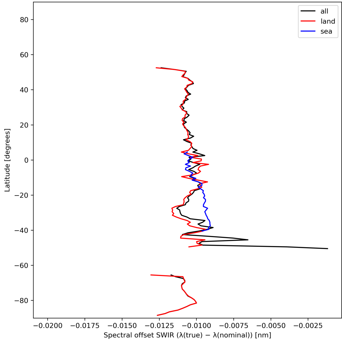
Figure 16: Zonal average of “Spectral offset SWIR ( \lambda(\text{true}) - \lambda(\text{nominal}) )” for 2023-12-10 to 2023-12-12.
