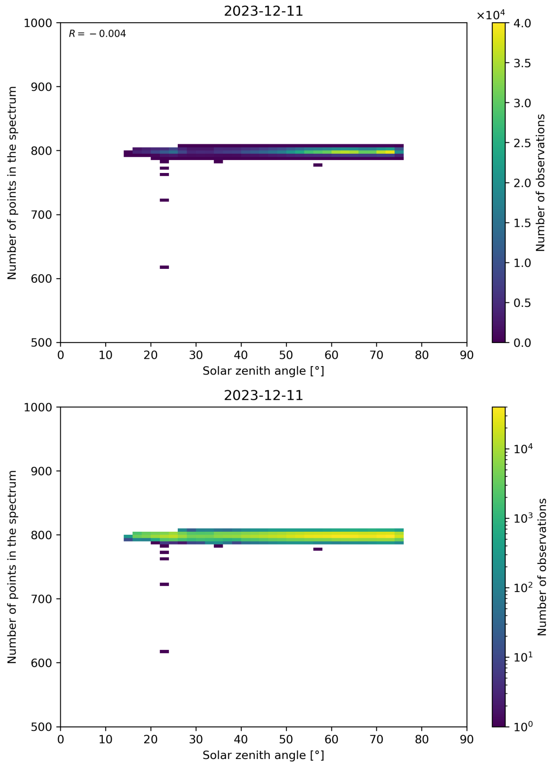
Figure 103: Scatter density plot of “Solar zenith angle” against “Number of points in the spectrum” for 2023-12-10 to 2023-12-12.
