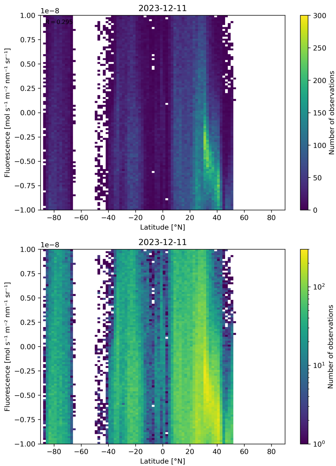
Figure 56: Scatter density plot of “Latitude” against “Fluorescence” for 2023-12-10 to 2023-12-12.
