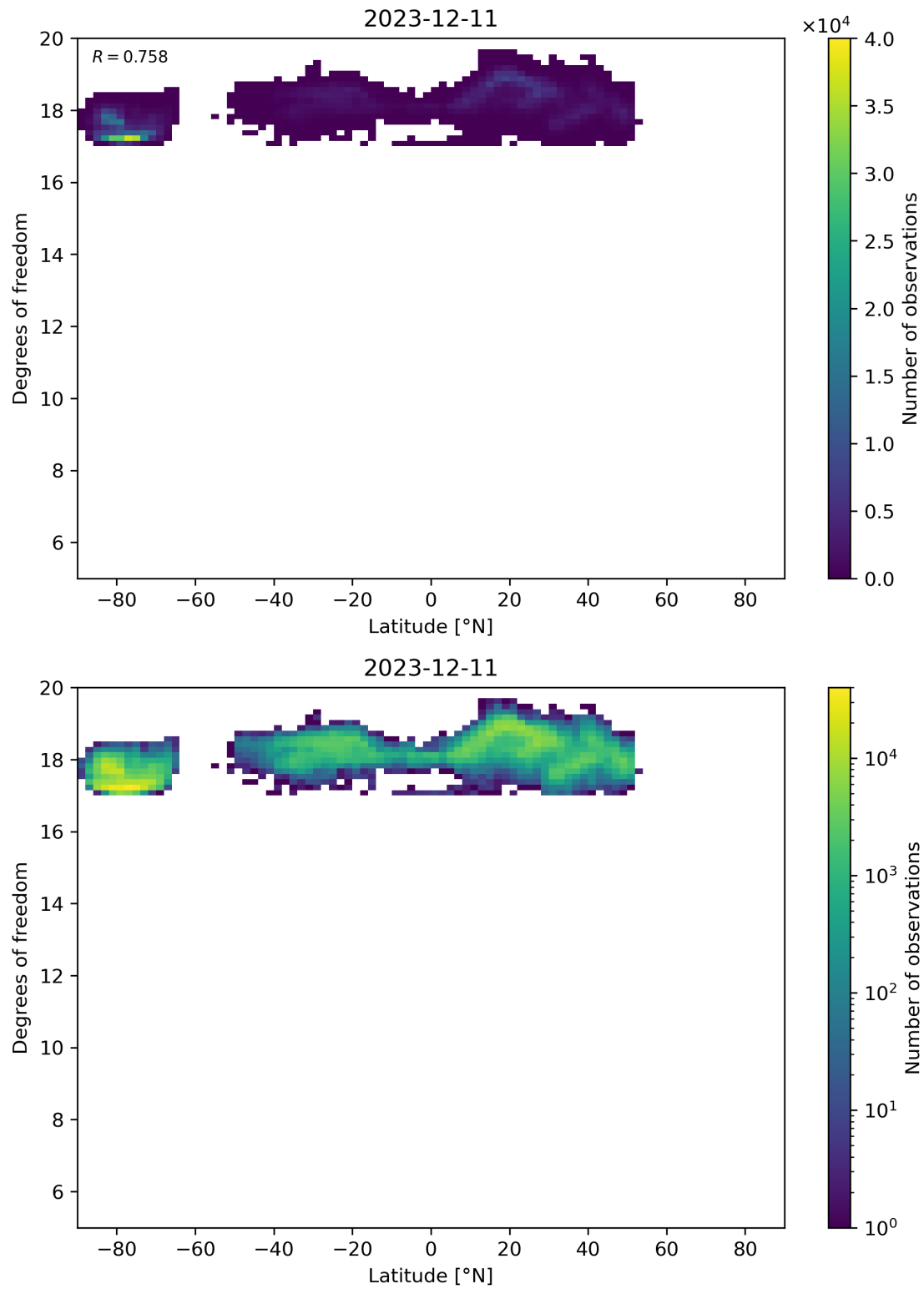
Figure 55: Scatter density plot of “Latitude” against “Degrees of freedom” for 2023-12-10 to 2023-12-12.
