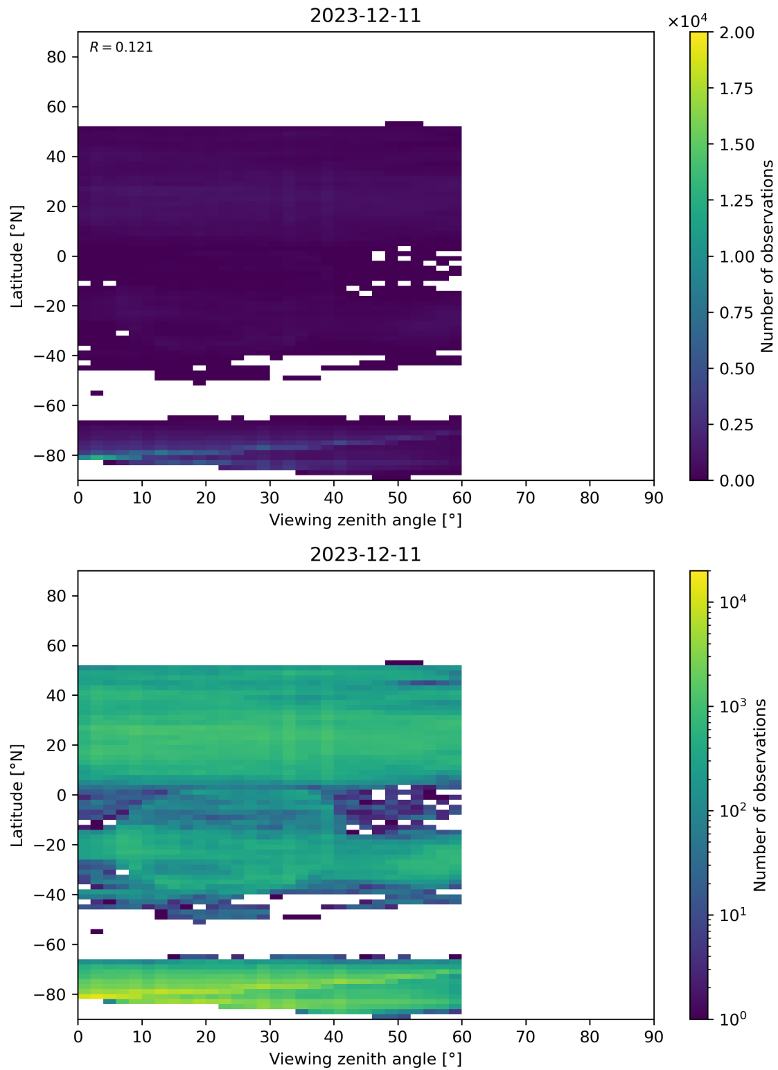
Figure 109: Scatter density plot of “Viewing zenith angle” against “Latitude” for 2023-12-10 to 2023-12-12.
