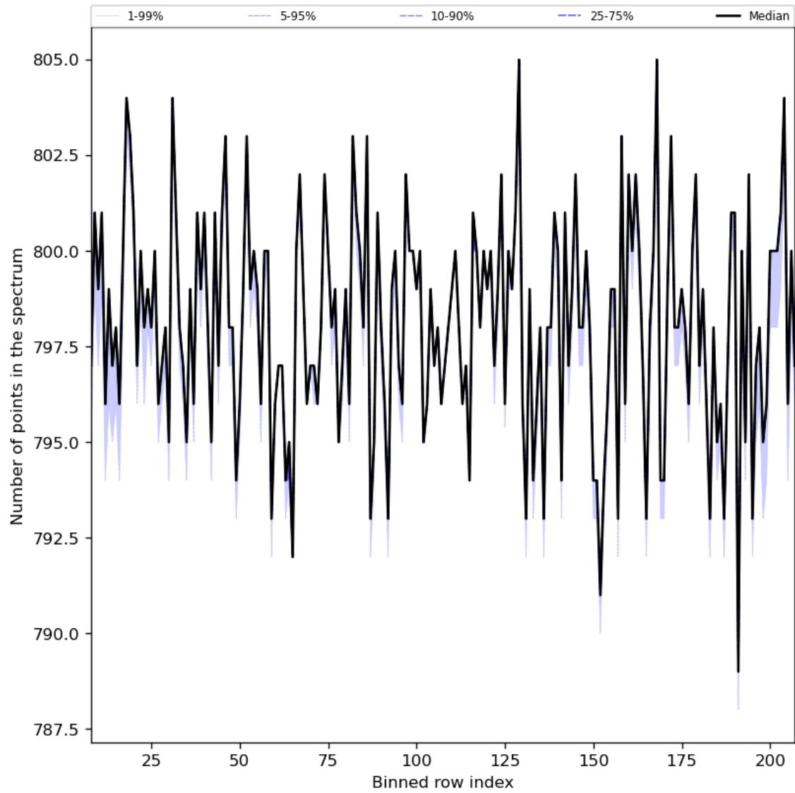
Figure 37: Along track statistics of “Number of points in the spectrum” for 2023-12-10 to 2023-12-12
