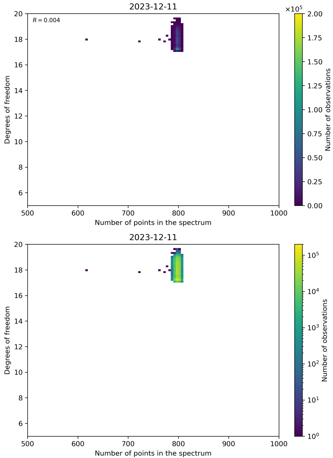
Figure 90: Scatter density plot of “Number of points in the spectrum” against “Degrees of freedom” for 2023-12-10 to 2023-12-12.
