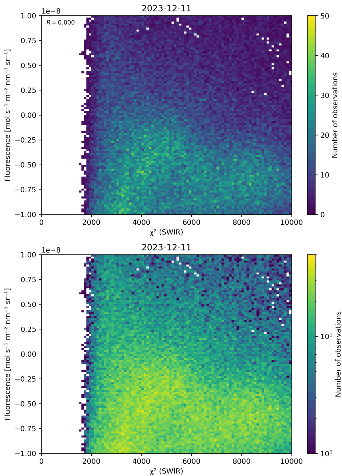
Figure 49: Scatter density plot of “ \chi^2 (SWIR)” against “Fluorescence” for 2023-12-10 to 2023-12-12.
