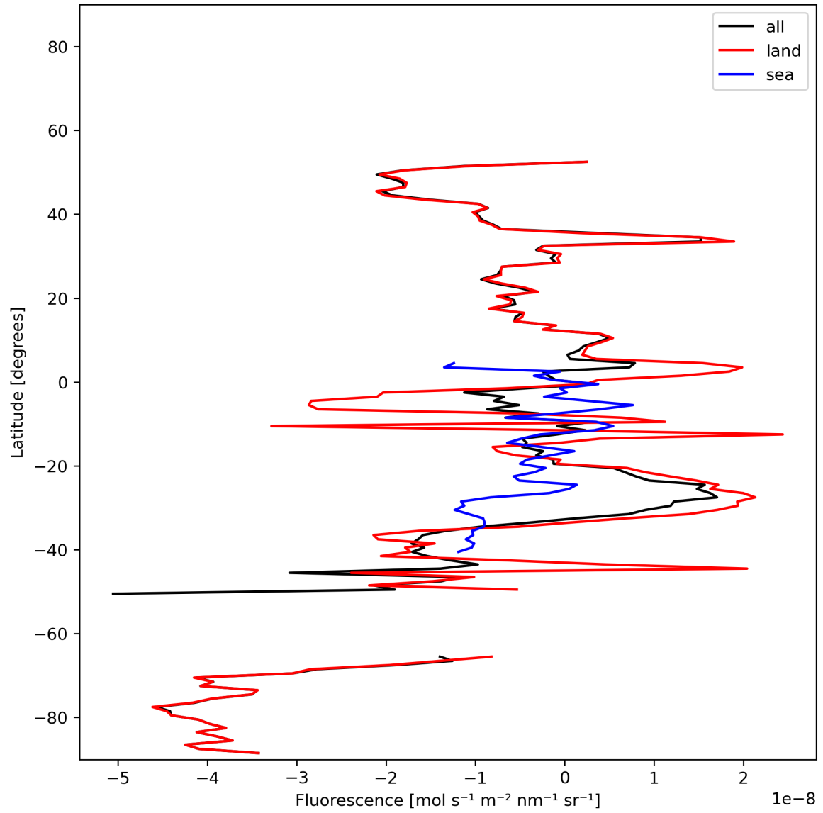
Figure 21: Zonal average of “Fluorescence” for 2023-12-10 to 2023-12-12.
