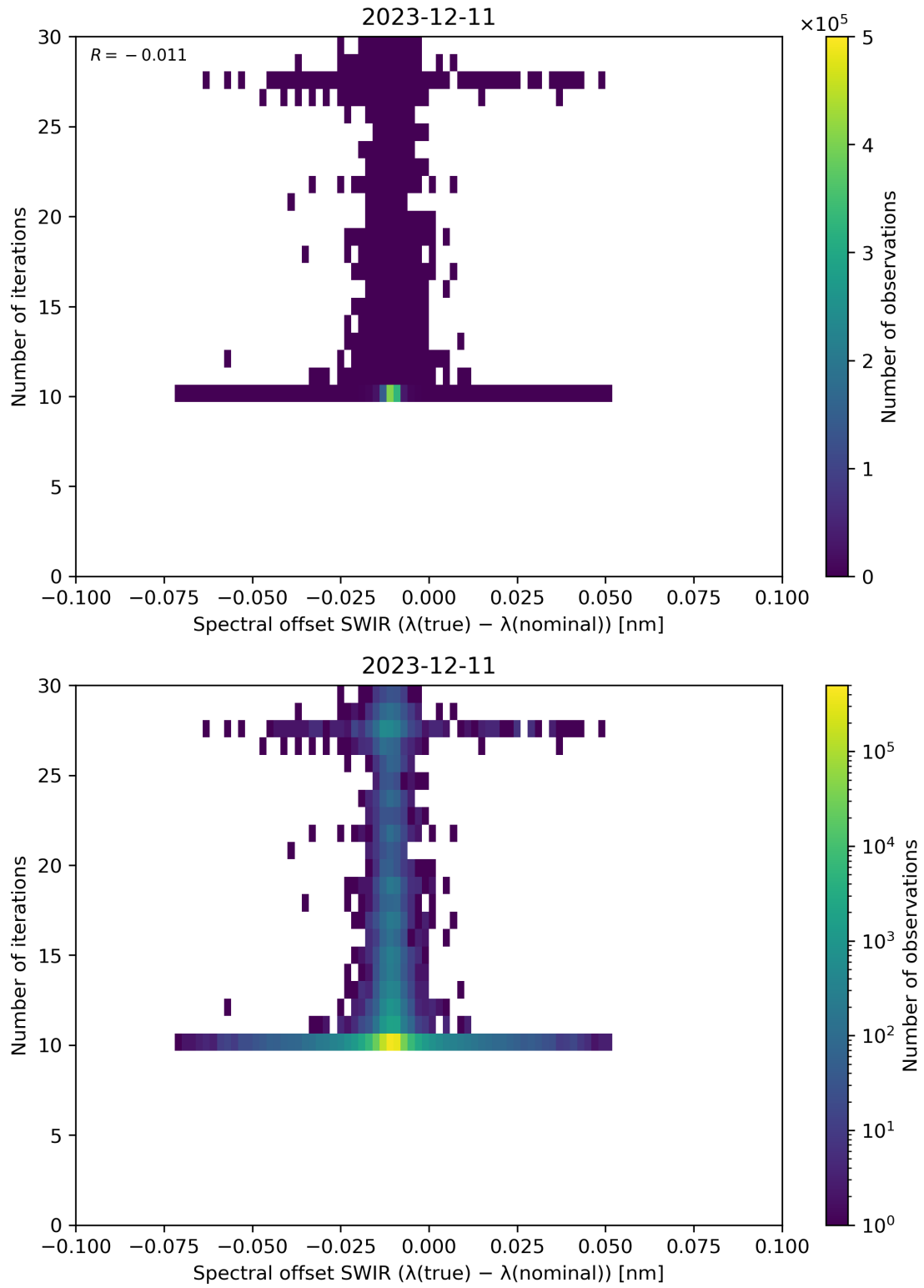
Figure 121: Scatter density plot of “Spectral offset SWIR ( \lambda(\text{true}) - \lambda(\text{nominal}) )” against “Number of iterations” for 2023-12-10 to 2023-12-12.
