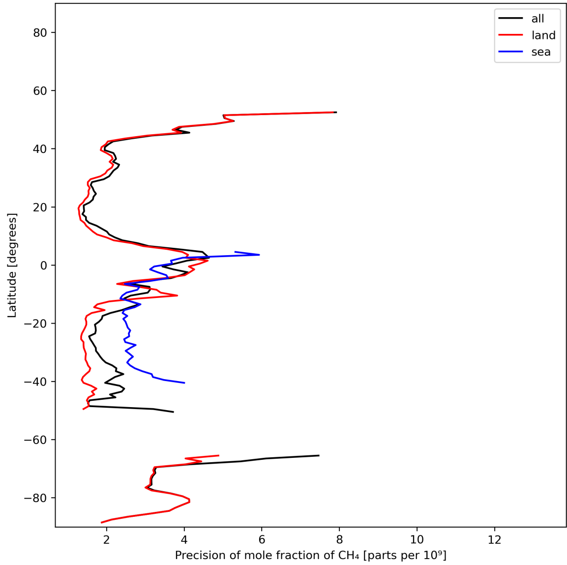
Figure 13: Zonal average of “Precision of mole fraction of CH 4 ” for 2023-12-10 to 2023-12-12.
