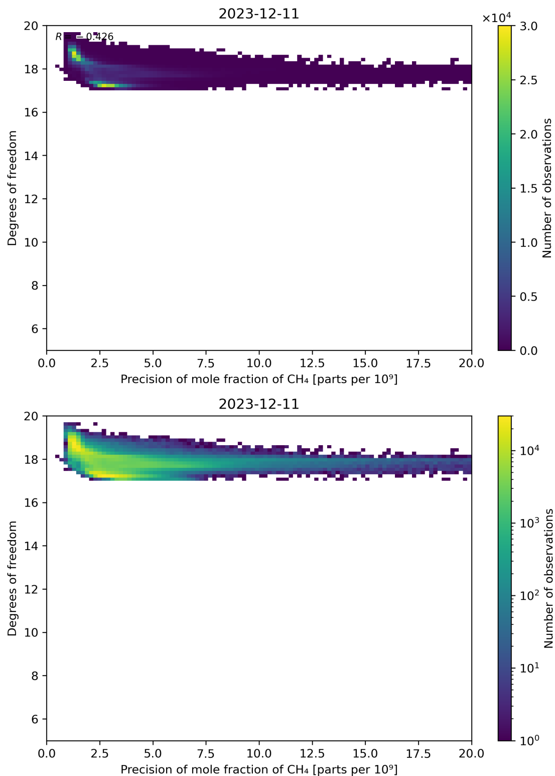
Figure 80: Scatter density plot of “Precision of mole fraction of CH 4 ” against “Degrees of freedom” for 2023-12-10 to 2023-12-12.
