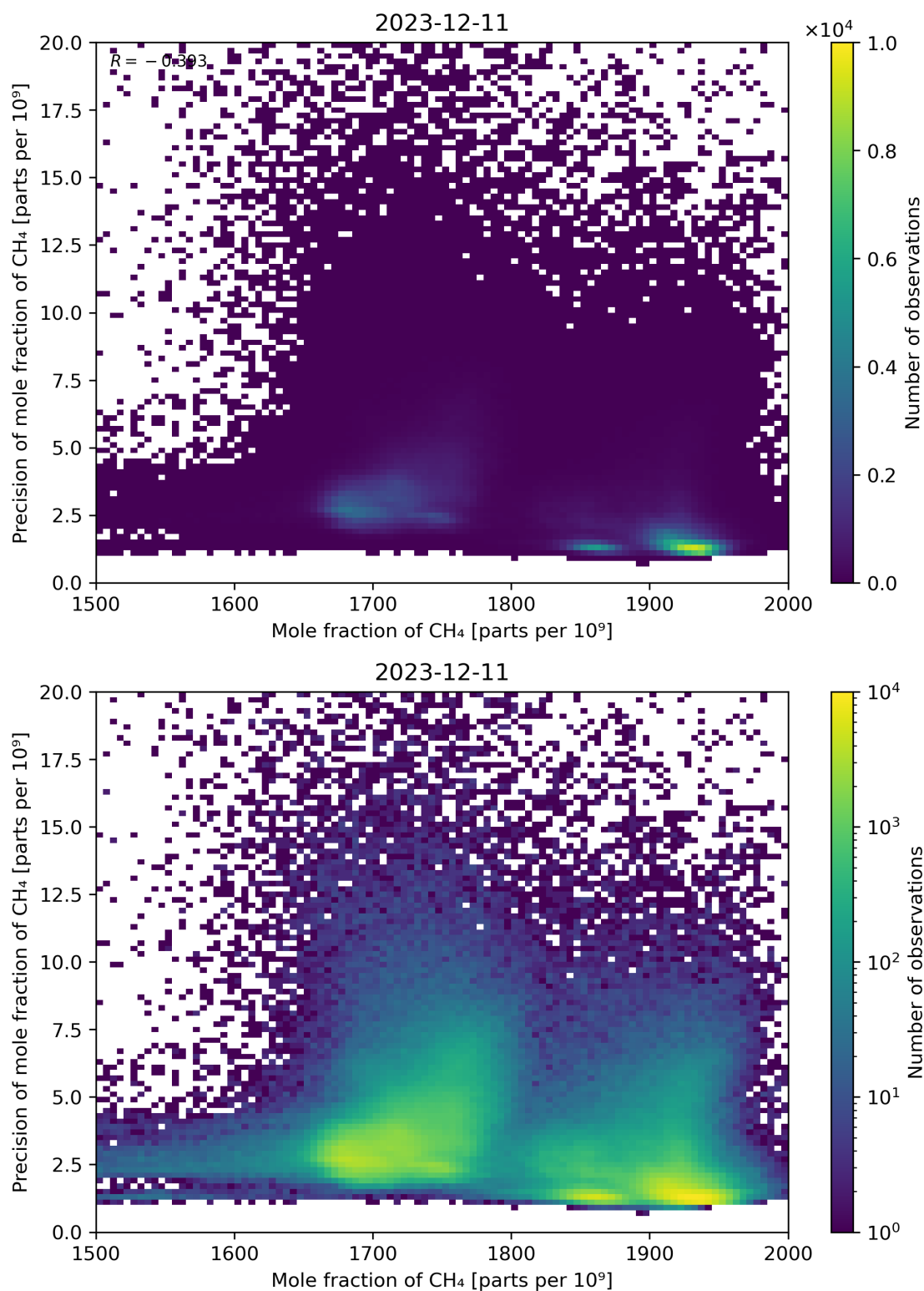
Figure 75: Scatter density plot of “Mole fraction of CH 4 ” against “Precision of mole fraction of CH 4 ” for 2023-12-10 to 2023-12-12.
