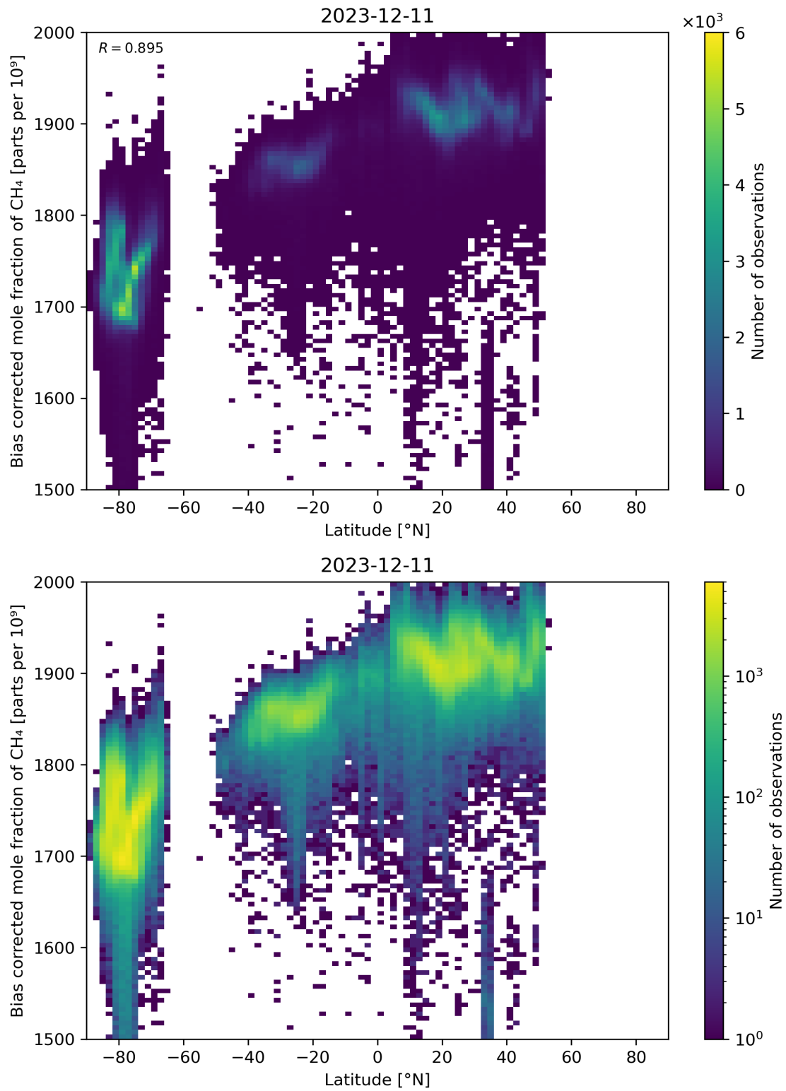
Figure 58: Scatter density plot of “Latitude” against “Bias corrected mole fraction of CH 4 ” for 2023-12-10 to 2023-12-12.
