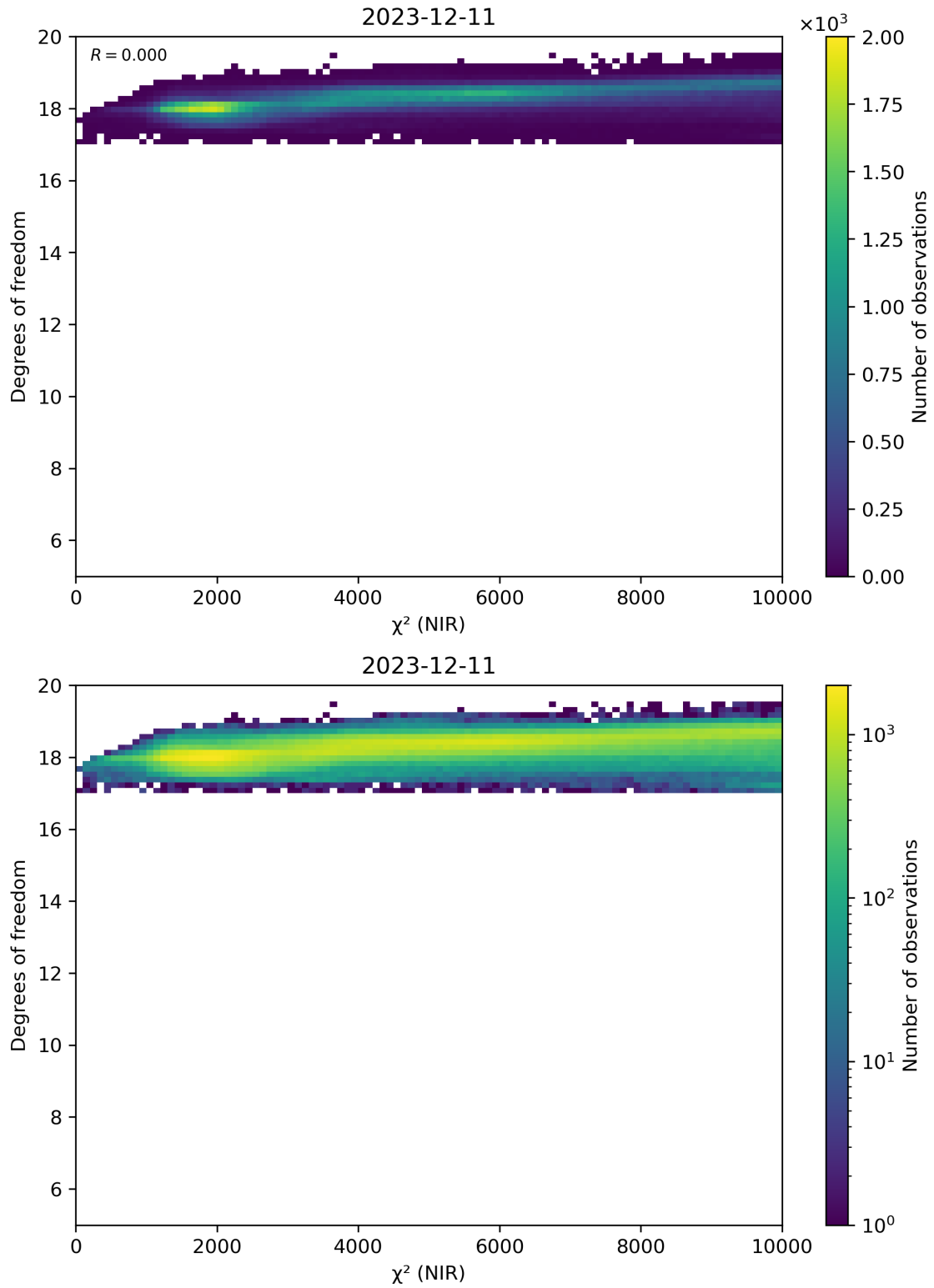
Figure 44: Scatter density plot of “ \chi^2 (NIR)” against “Degrees of freedom” for 2023-12-10 to 2023-12-12.
