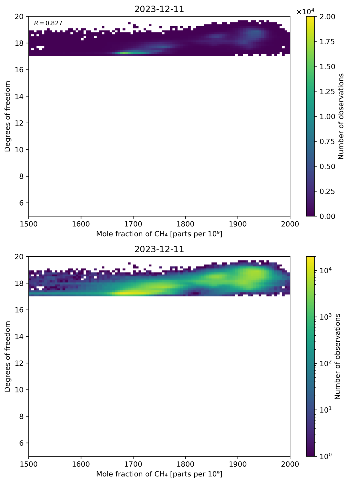
Figure 72: Scatter density plot of “Mole fraction of CH 4 ” against “Degrees of freedom” for 2023-12-10 to 2023-12-12.
