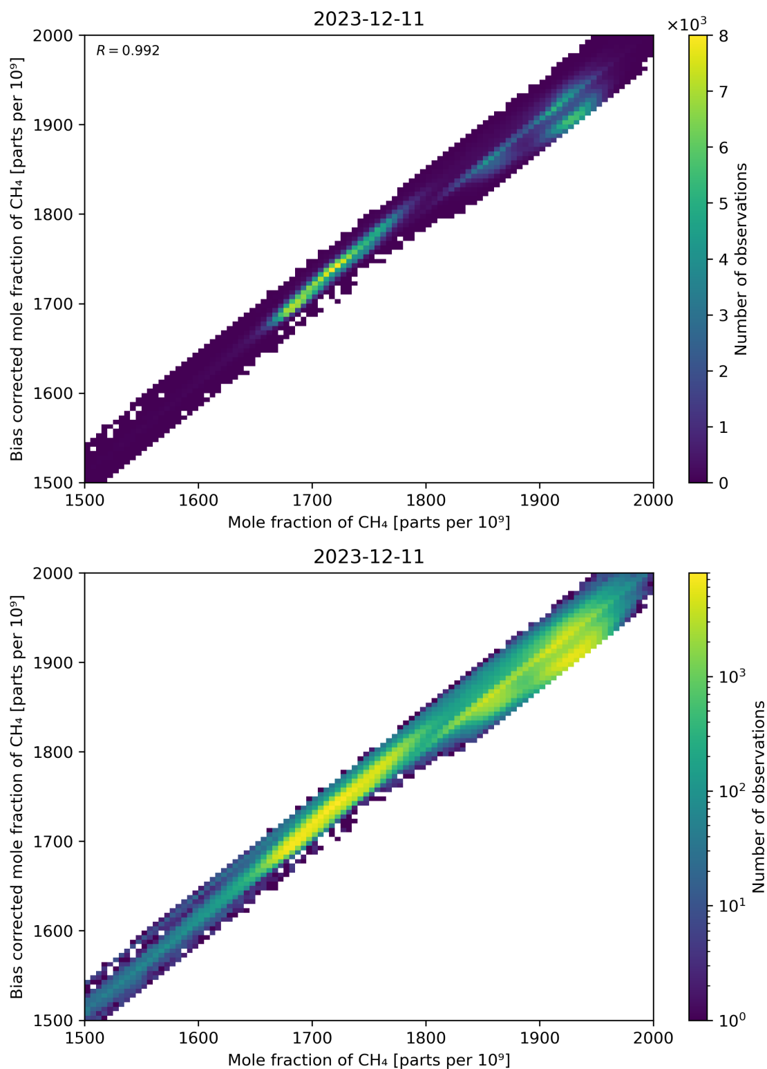
Figure 74: Scatter density plot of “Mole fraction of CH 4 ” against “Bias corrected mole fraction of CH 4 ” for 2023-12-10 to 2023-12-12.
