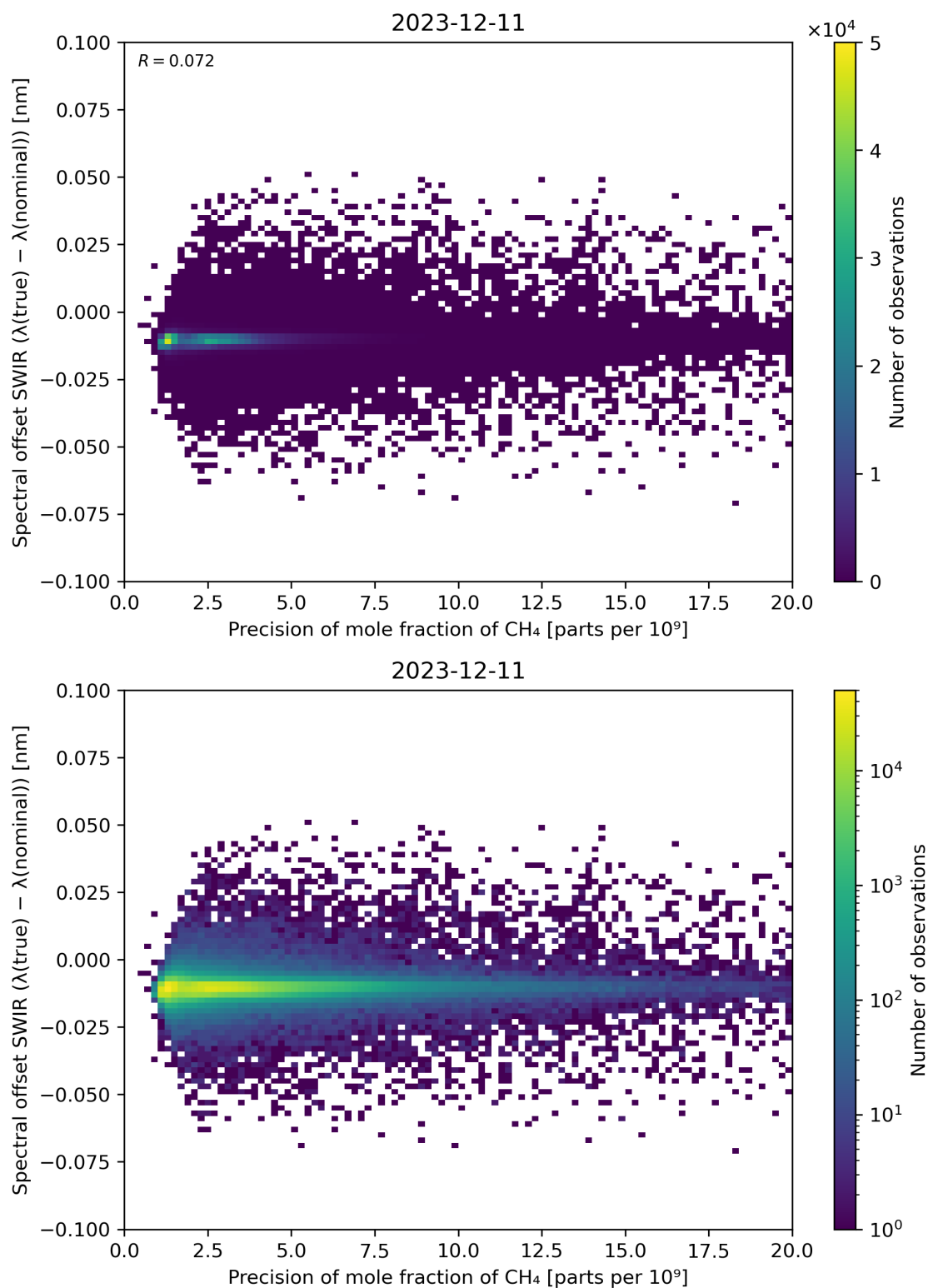
Figure 85: Scatter density plot of “Precision of mole fraction of CH 4 ” against “Spectral offset SWIR ( \lambda(\text{true}) - \lambda(\text{nominal}) )” for 2023-12-10 to 2023-12-12.
