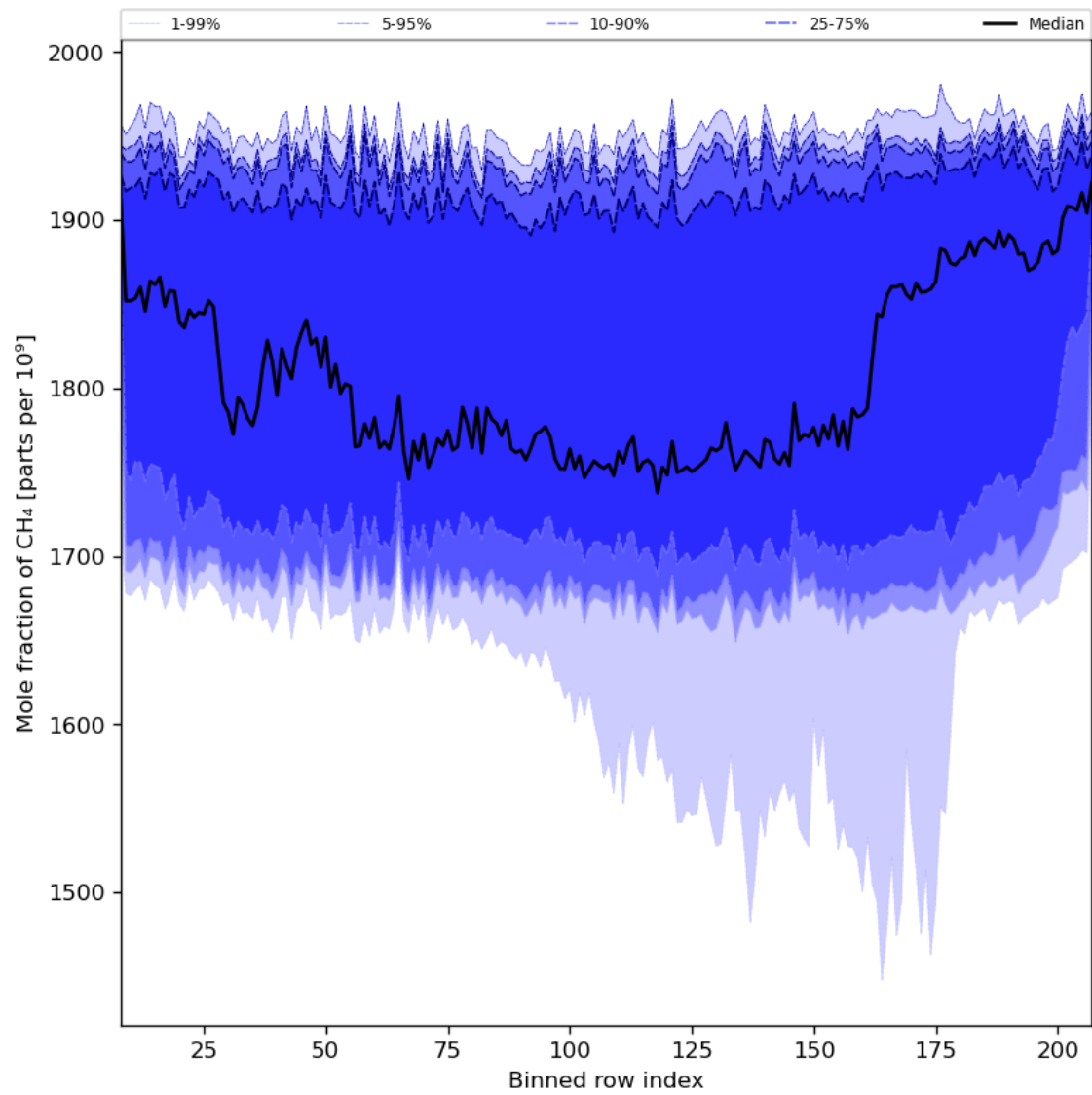
Figure 34: Along track statistics of “Mole fraction of CH 4 ” for 2023-12-10 to 2023-12-12
