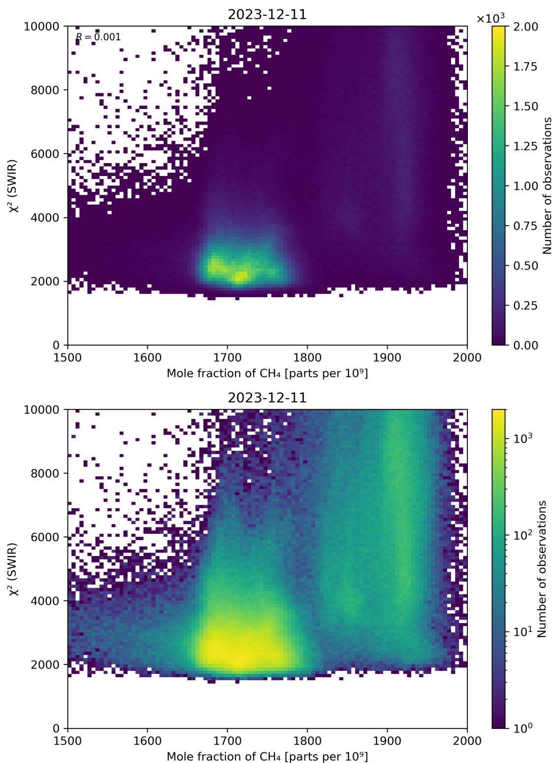
Figure 71: Scatter density plot of “Mole fraction of CH 4 ” against “ \chi^2 (SWIR)” for 2023-12-10 to 2023-12-12.
