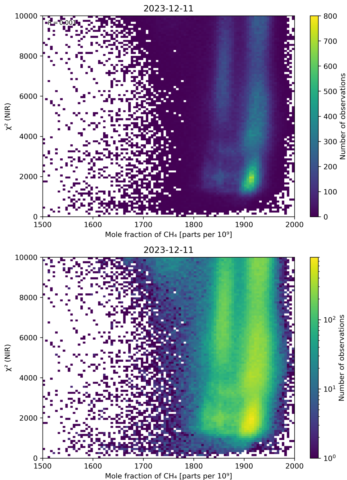
Figure 70: Scatter density plot of “Mole fraction of \text{CH}_4 ” against “ \chi^2 (NIR)” for 2023-12-10 to 2023-12-12.
