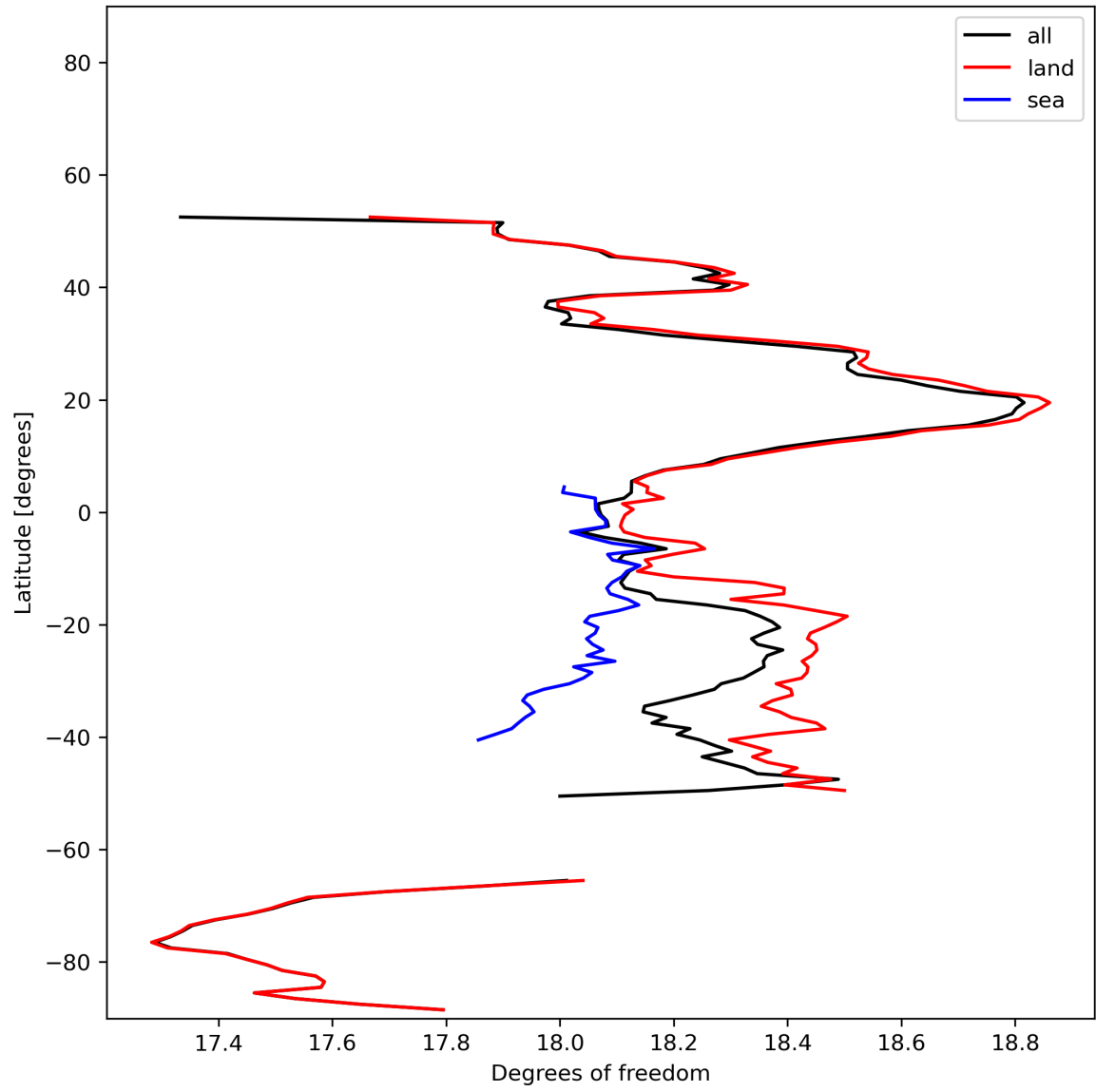
Figure 19: Zonal average of “Degrees of freedom” for 2023-12-10 to 2023-12-12.
