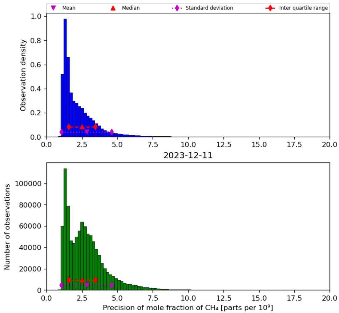
Figure 24: Histogram of “Precision of mole fraction of CH 4 ” for 2023-12-10 to 2023-12-12
