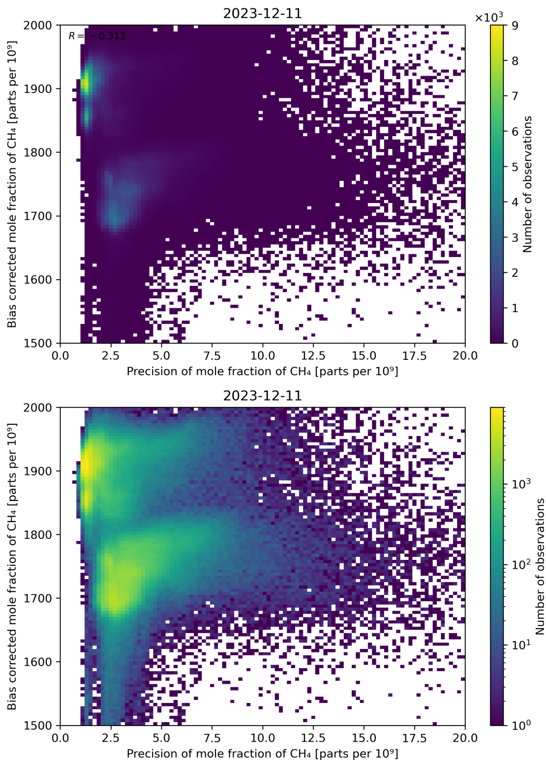
Figure 82: Scatter density plot of “Precision of mole fraction of CH 4 ” against “Bias corrected mole fraction of CH 4 ” for 2023-12-10 to 2023-12-12.
