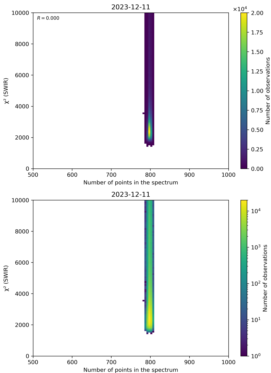
Figure 89: Scatter density plot of “Number of points in the spectrum” against “ \chi^2 (SWIR)” for 2023-12-10 to 2023-12-12.
