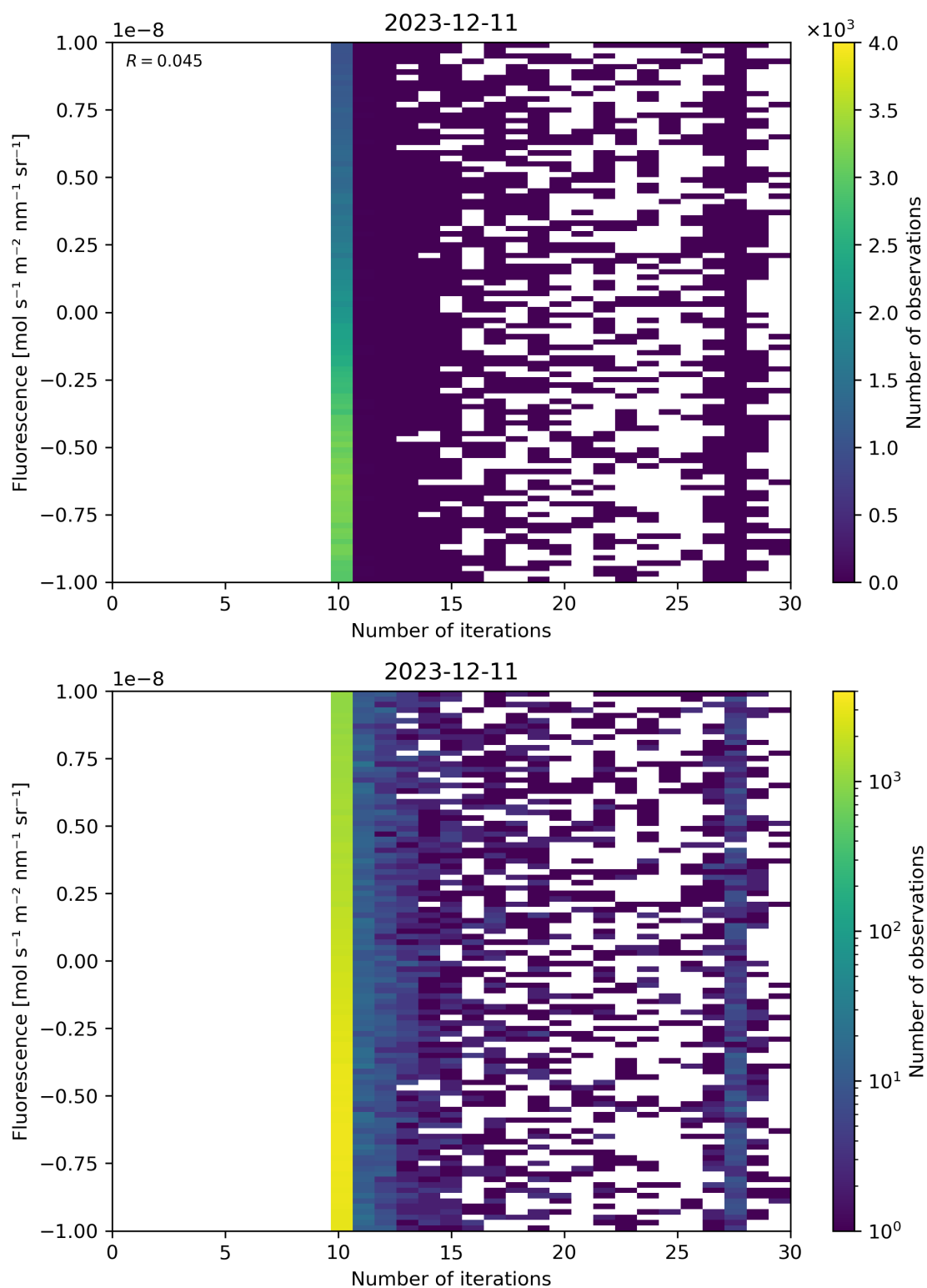
Figure 87: Scatter density plot of “Number of iterations” against “Fluorescence” for 2023-12-10 to 2023-12-12.
