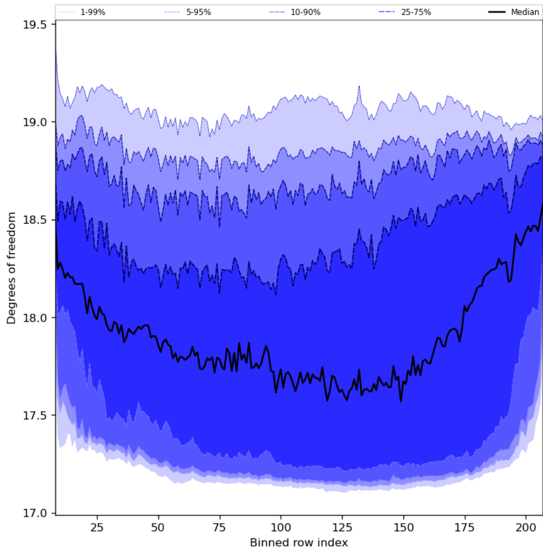
Figure 41: Along track statistics of “Degrees of freedom” for 2023-12-10 to 2023-12-12
