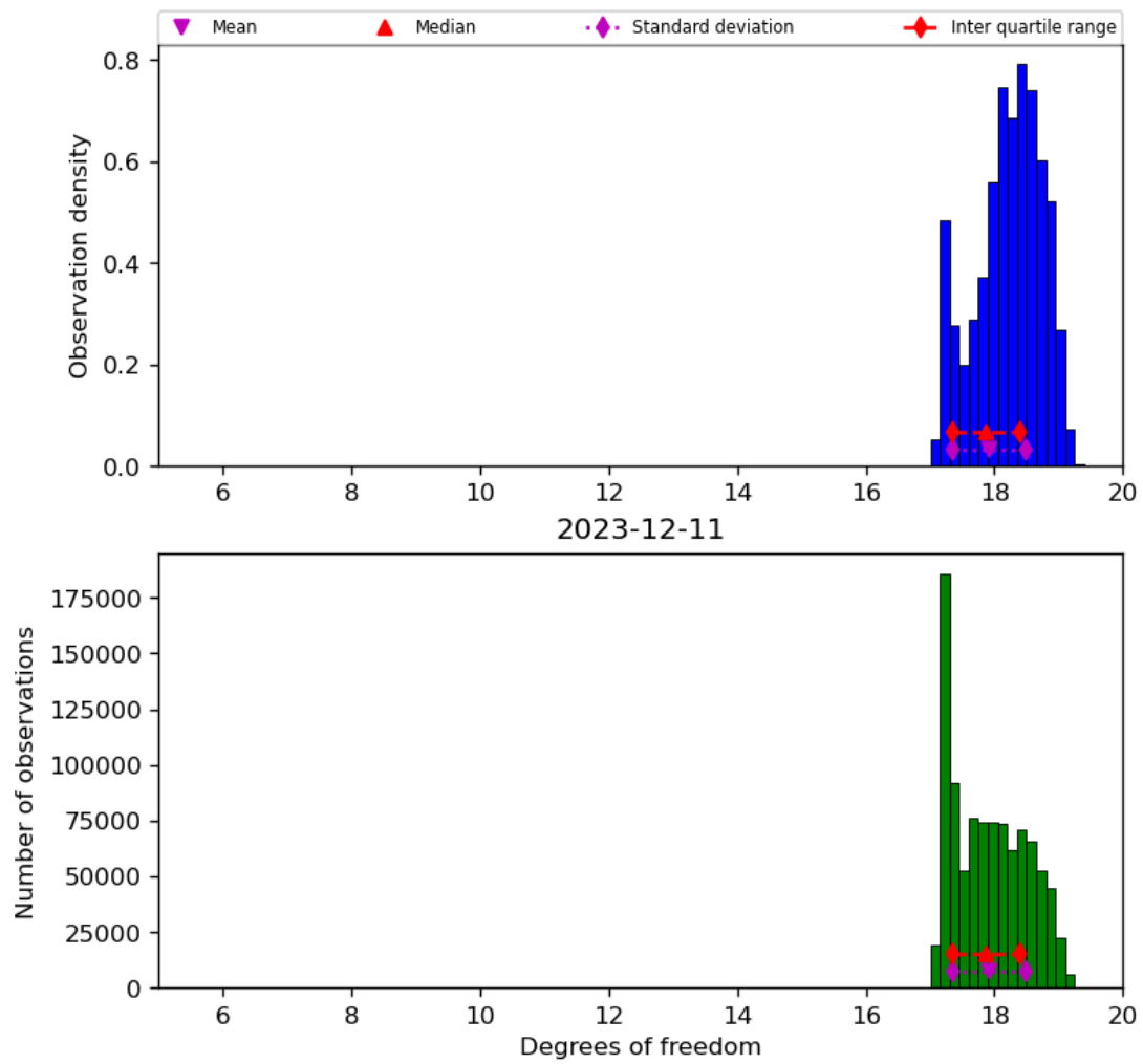
Figure 30: Histogram of “Degrees of freedom” for 2023-12-10 to 2023-12-12
