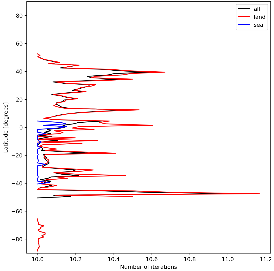
Figure 20: Zonal average of “Number of iterations” for 2023-12-10 to 2023-12-12.
