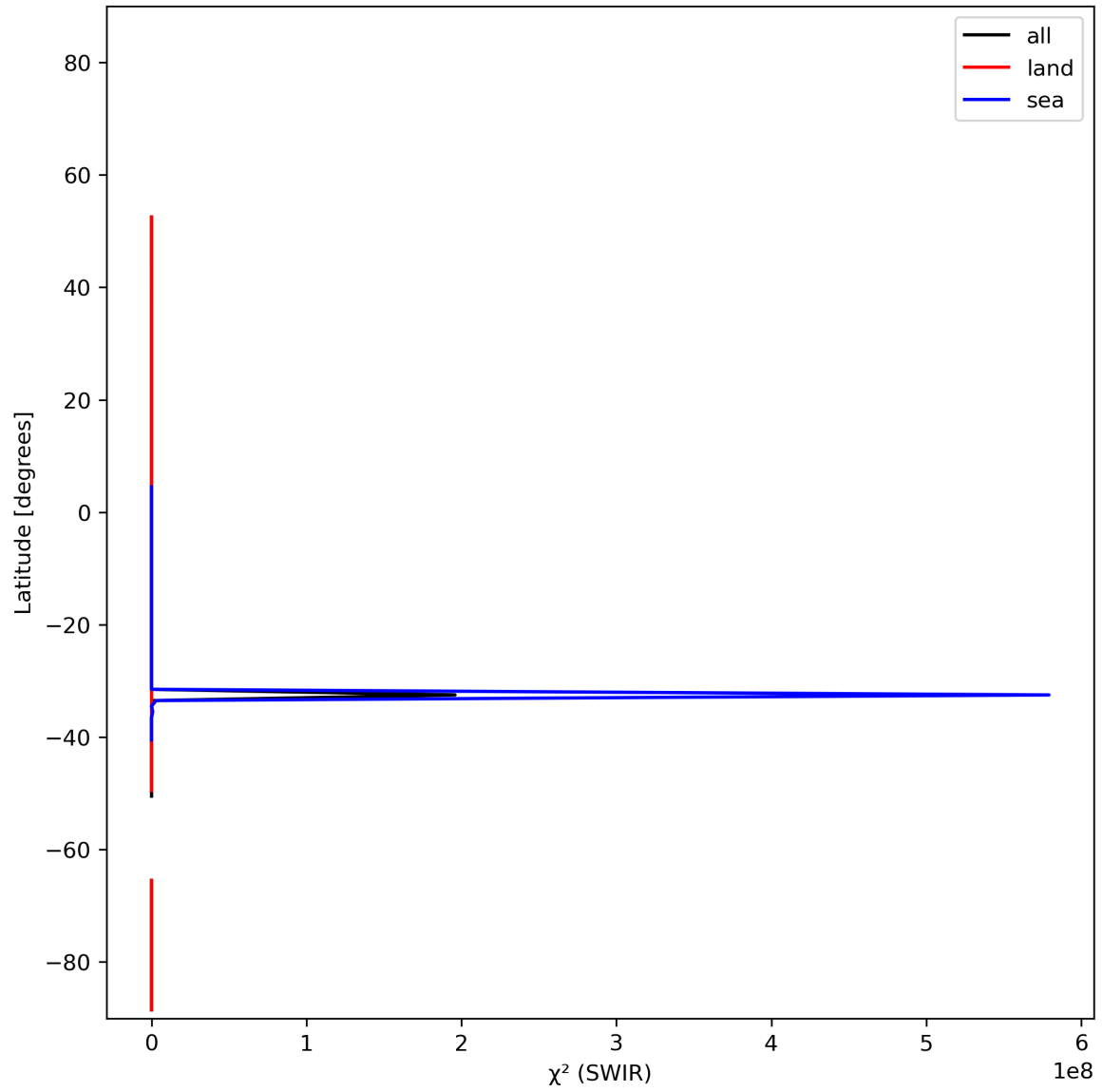
Figure 17: Zonal average of “ \chi^2 (SWIR)” for 2023-12-10 to 2023-12-12.
