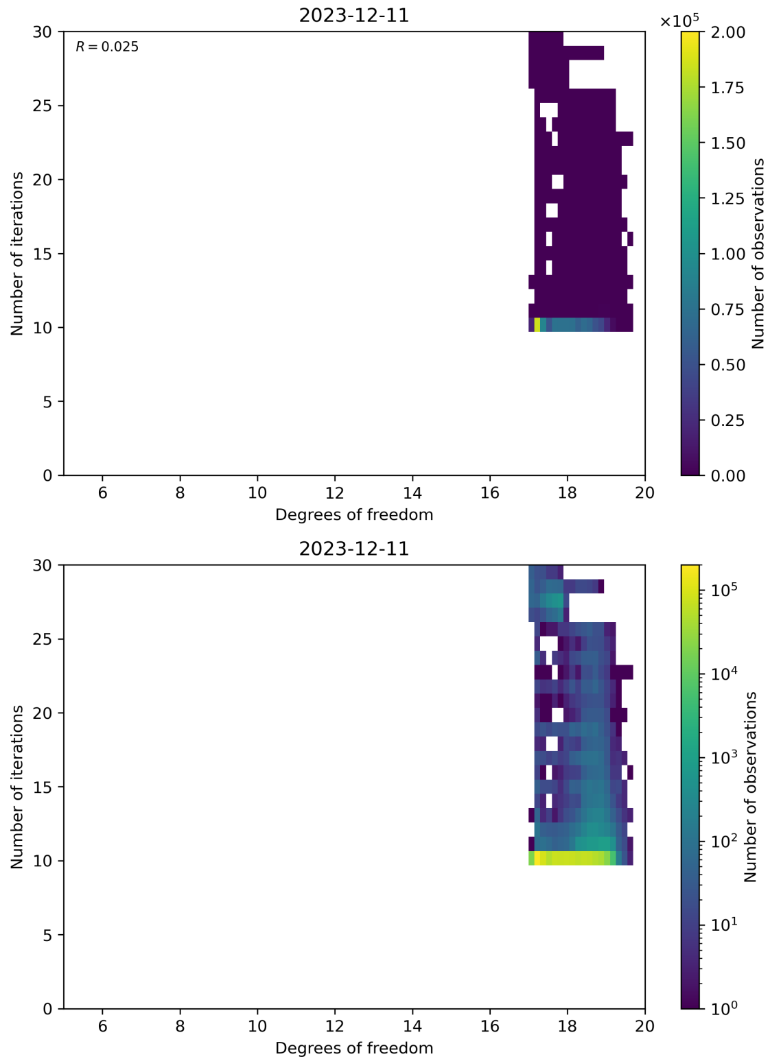
Figure 52: Scatter density plot of “Degrees of freedom” against “Number of iterations” for 2023-12-10 to 2023-12-12.
