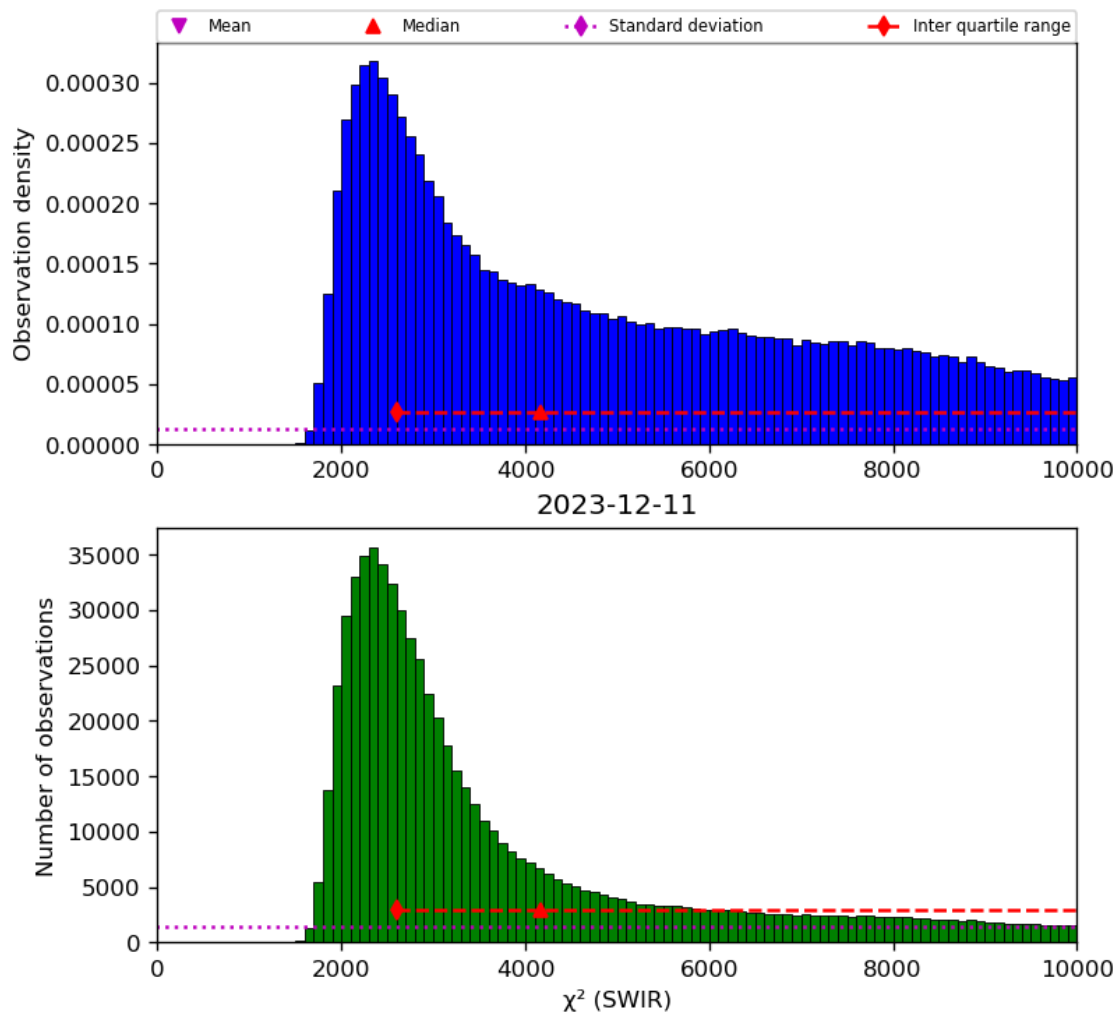
Figure 28: Histogram of “ \chi^2 (SWIR)” for 2023-12-10 to 2023-12-12
