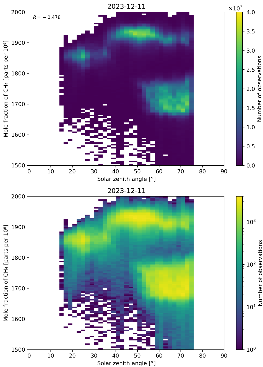
Figure 99: Scatter density plot of “Solar zenith angle” against “Mole fraction of CH 4 ” for 2023-12-10 to 2023-12-12.
