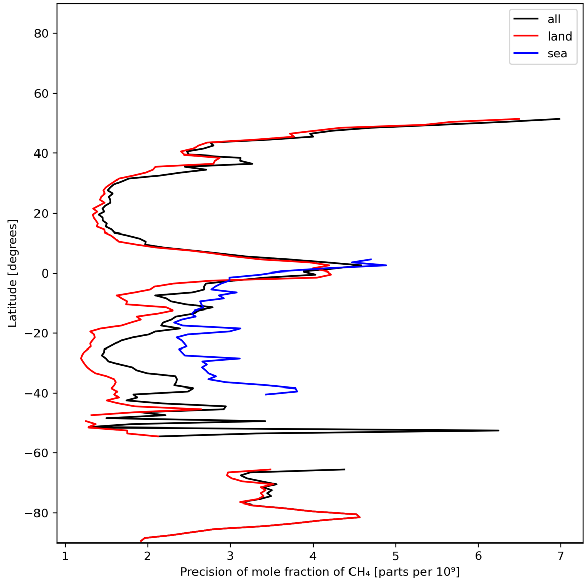
Figure 13: Zonal average of “Precision of mole fraction of CH 4 ” for 2023-12-12 to 2023-12-14.
