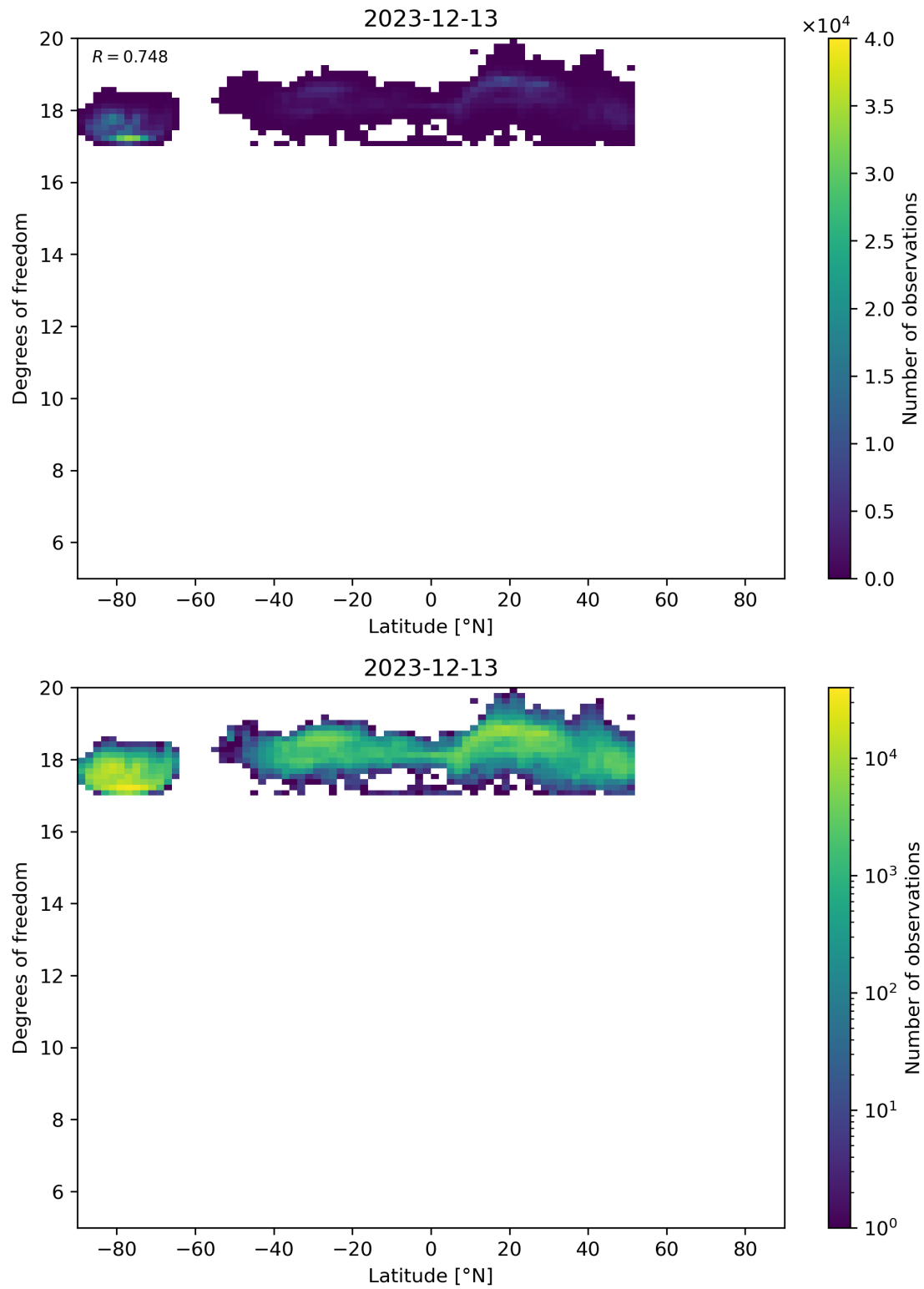
Figure 55: Scatter density plot of “Latitude” against “Degrees of freedom” for 2023-12-12 to 2023-12-14.
