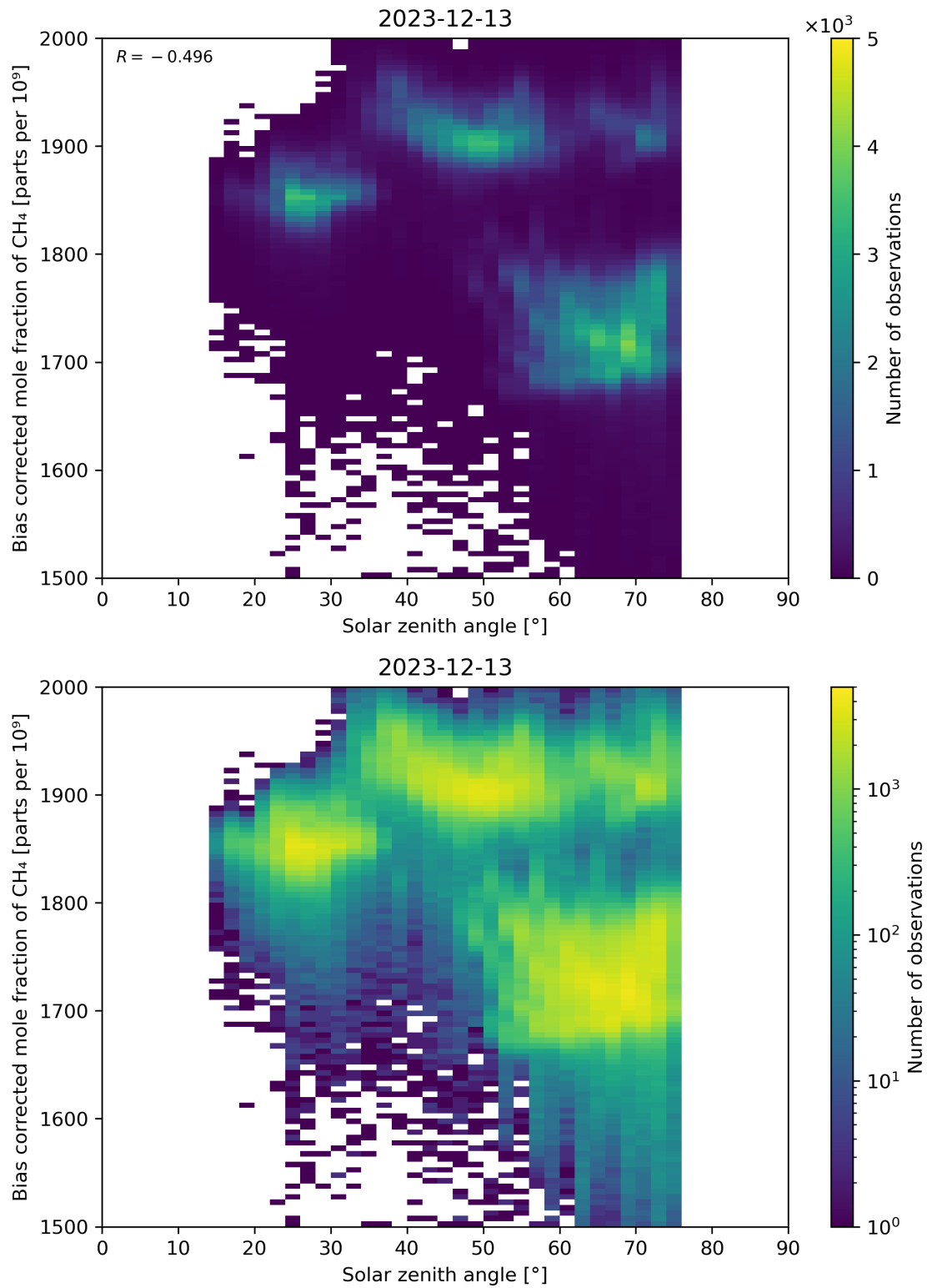
Figure 100: Scatter density plot of “Solar zenith angle” against “Bias corrected mole fraction of CH 4 ” for 2023-12-12 to 2023-12-14.
