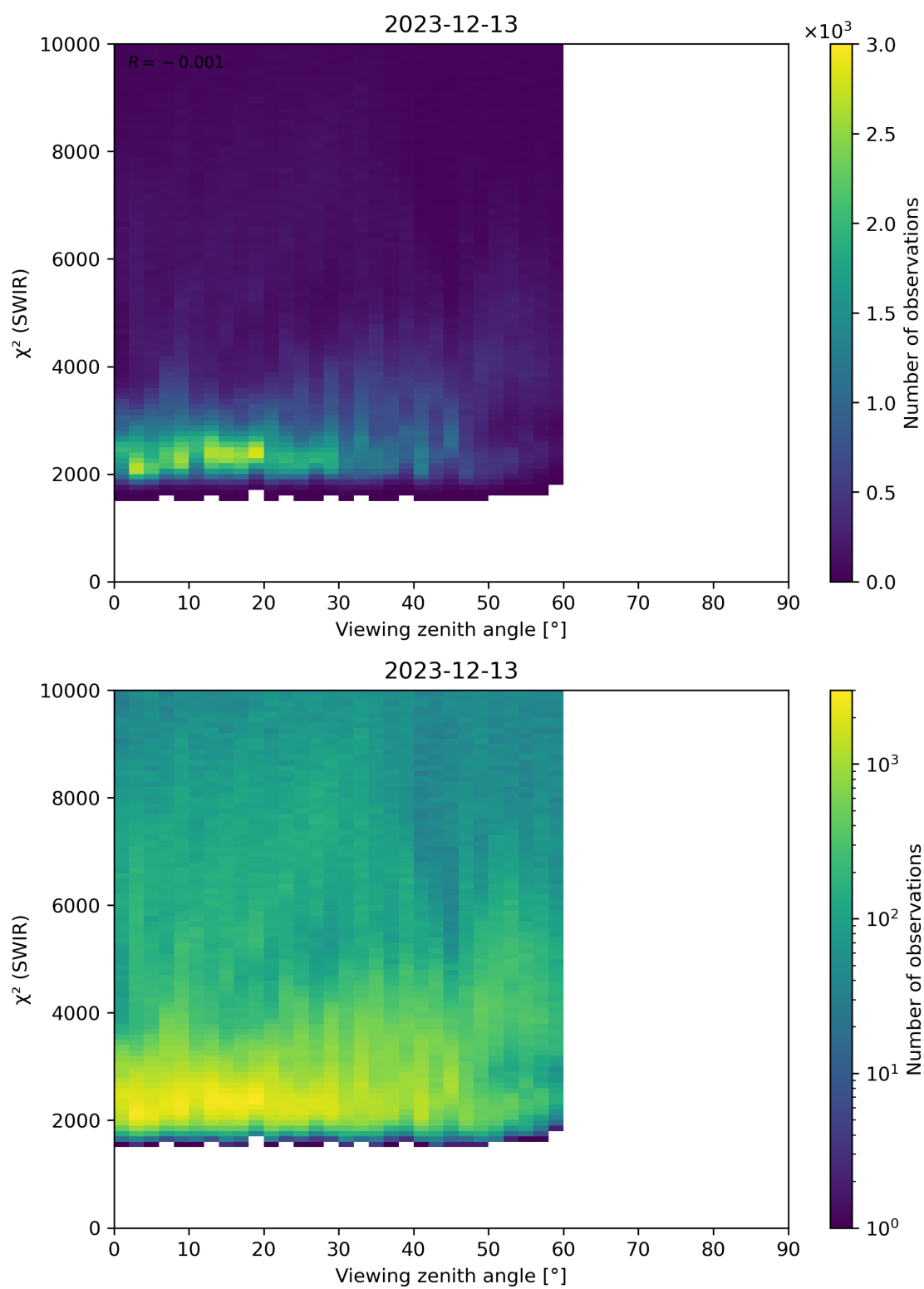
Figure 106: Scatter density plot of “Viewing zenith angle” against “ \chi^2 (SWIR)” for 2023-12-12 to 2023-12-14.
