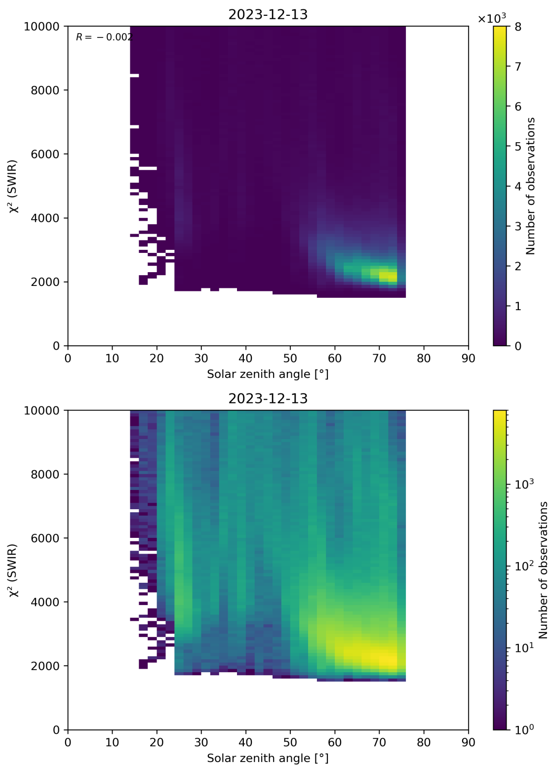
Figure 95: Scatter density plot of “Solar zenith angle” against “ \chi^2 (SWIR)” for 2023-12-12 to 2023-12-14.
