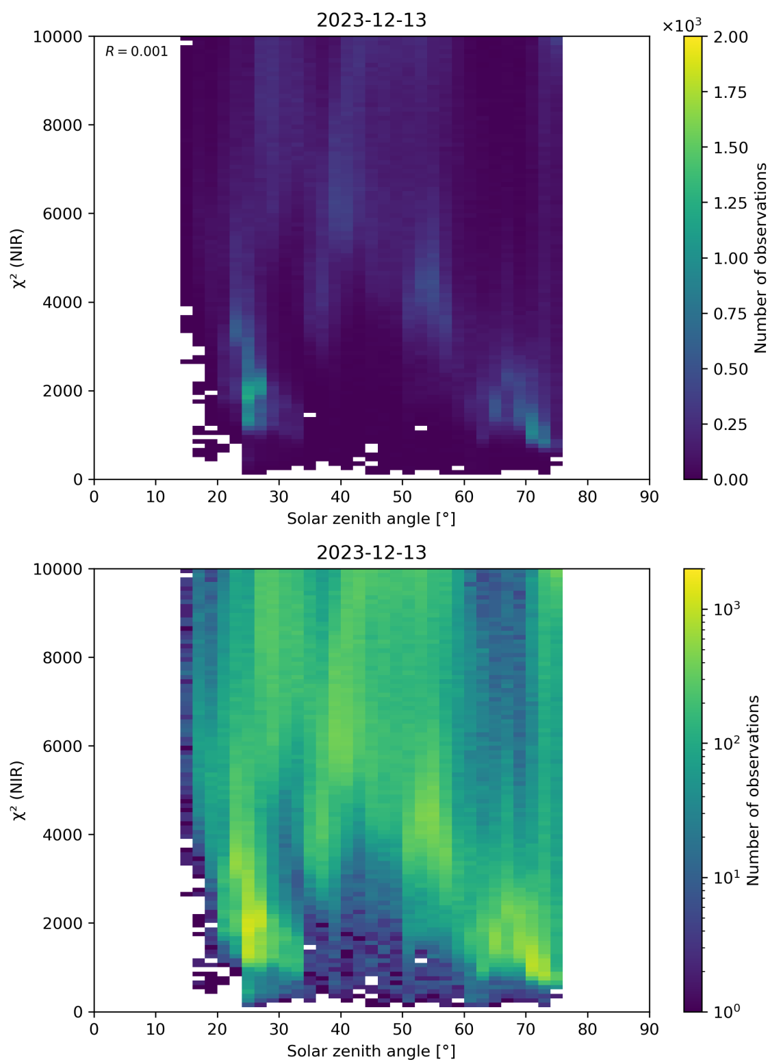
Figure 94: Scatter density plot of “Solar zenith angle” against “ \chi^2 (NIR)” for 2023-12-12 to 2023-12-14.
