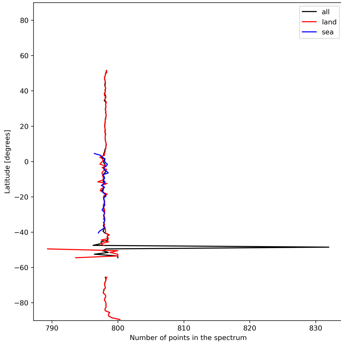
Figure 15: Zonal average of “Number of points in the spectrum” for 2023-12-12 to 2023-12-14.
