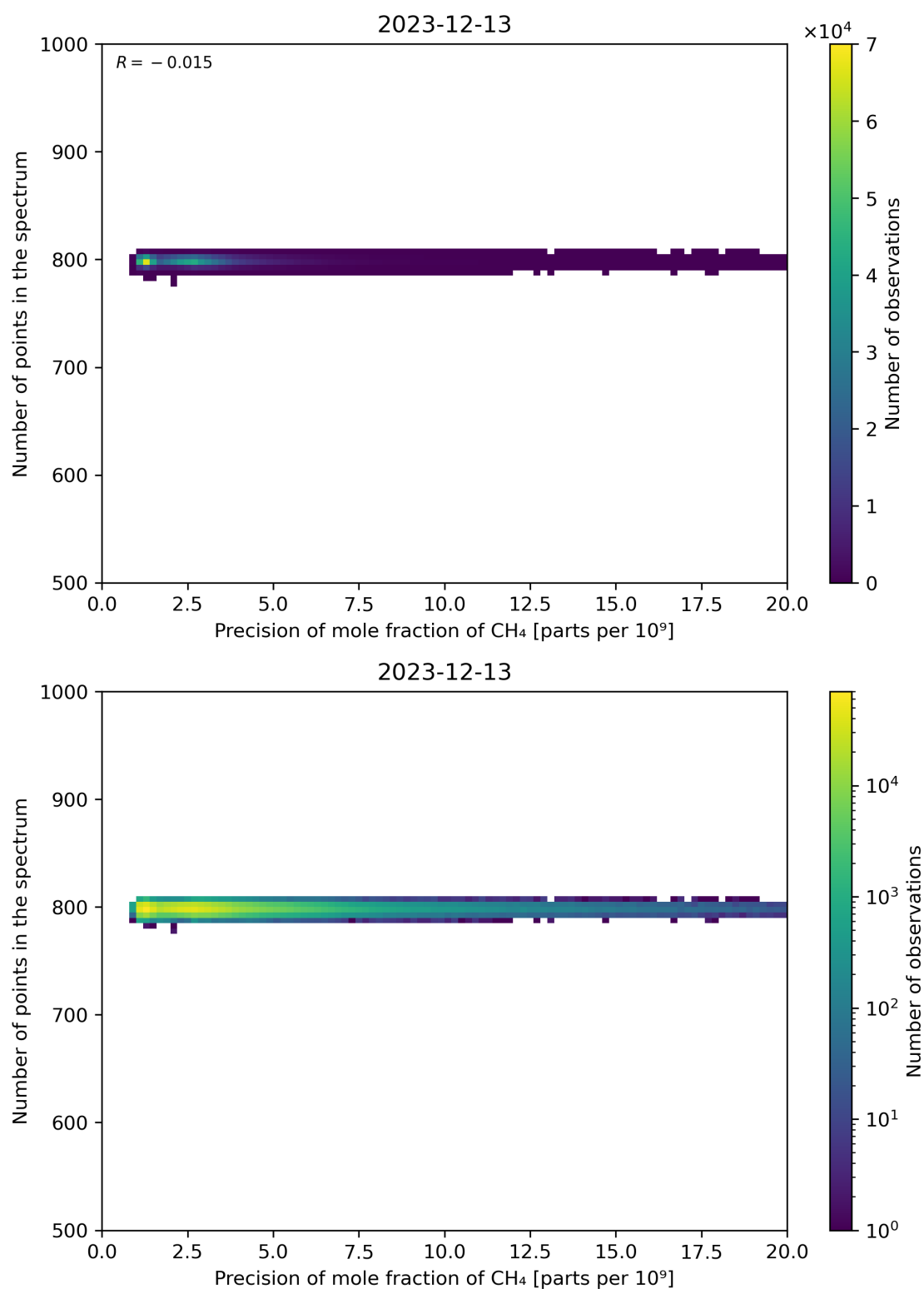
Figure 84: Scatter density plot of “Precision of mole fraction of CH 4 ” against “Number of points in the spectrum” for 2023-12-12 to 2023-12-14.
