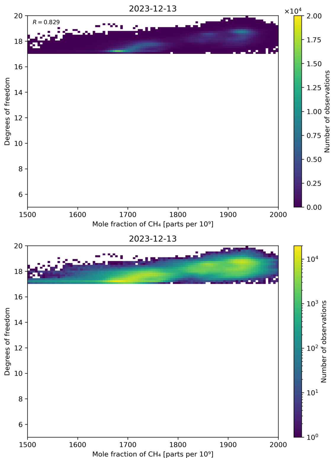
Figure 72: Scatter density plot of “Mole fraction of CH 4 ” against “Degrees of freedom” for 2023-12-12 to 2023-12-14.
