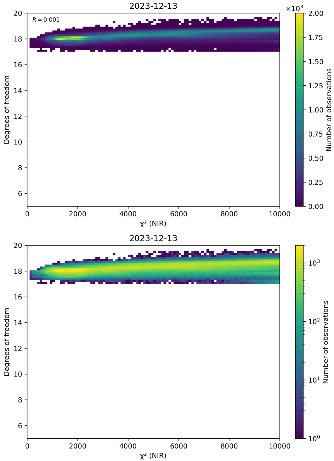
Figure 44: Scatter density plot of “ \chi^2 (NIR)” against “Degrees of freedom” for 2023-12-12 to 2023-12-14.
