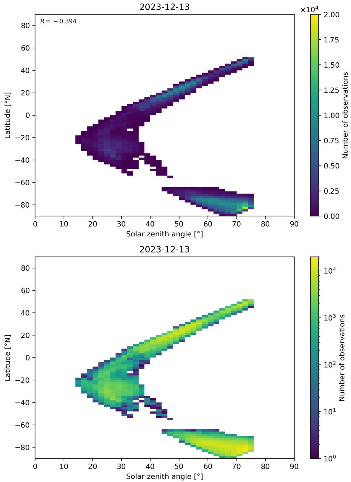
Figure 98: Scatter density plot of “Solar zenith angle” against “Latitude” for 2023-12-12 to 2023-12-14.
