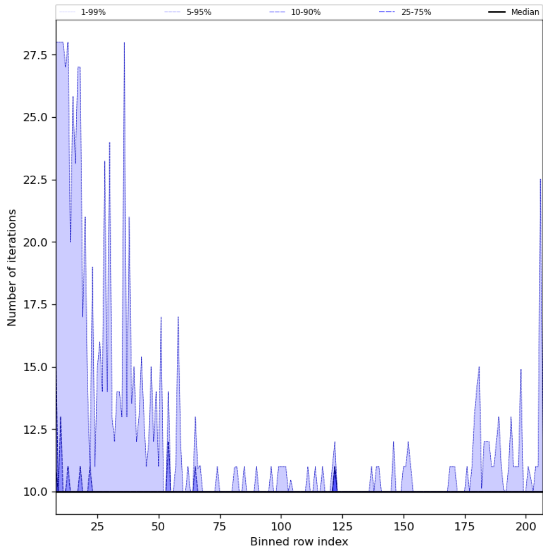
Figure 42: Along track statistics of “Number of iterations” for 2023-12-12 to 2023-12-14
