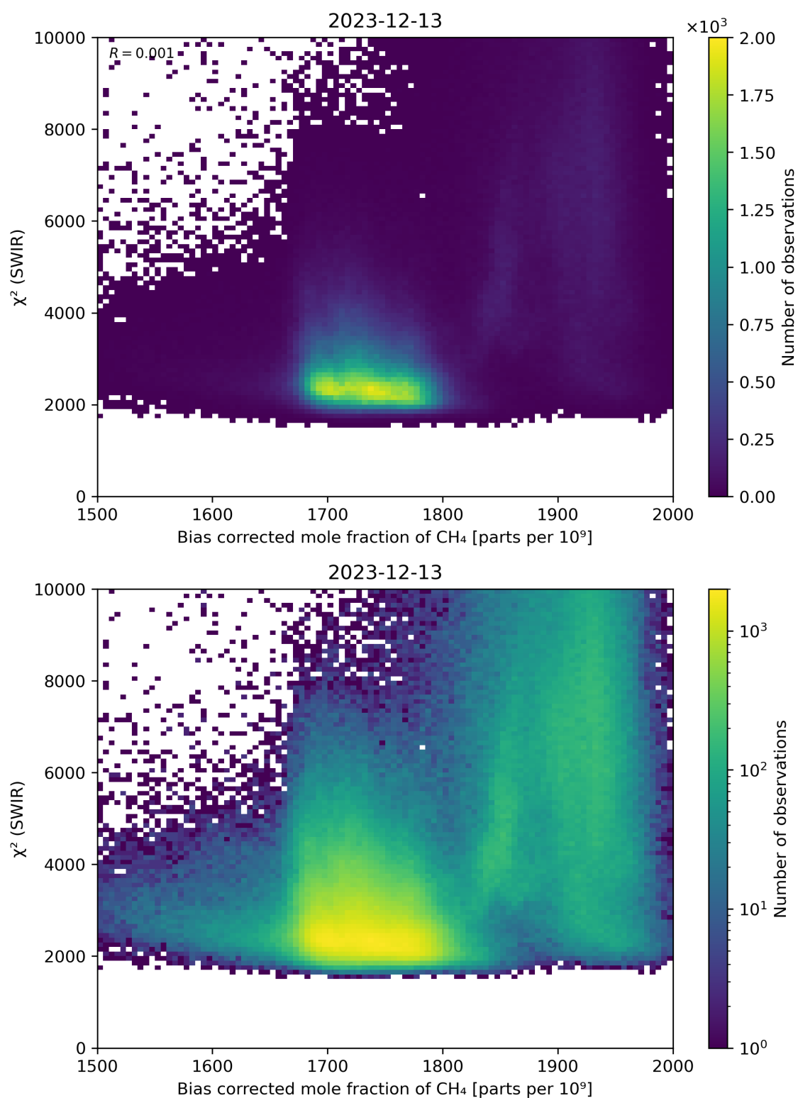
Figure 64: Scatter density plot of “Bias corrected mole fraction of CH 4 ” against “ \chi^2 (SWIR)” for 2023-12-12 to 2023-12-14.
