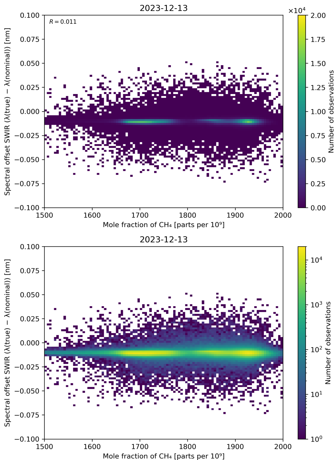
Figure 86: Scatter density plot of “Mole fraction of CH 4 ” against “Spectral offset SWIR ( \lambda(\text{true}) - \lambda(\text{nominal}) )” for 2023-12-12 to 2023-12-14.
