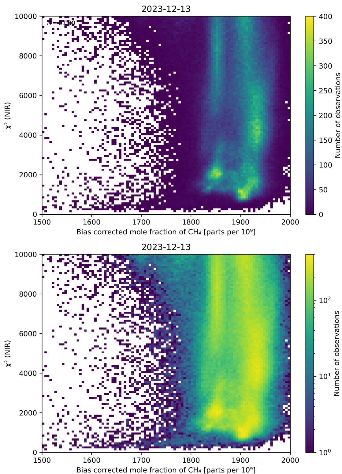
Figure 63: Scatter density plot of “Bias corrected mole fraction of \text{CH}_4 ” against “ \chi^2 (NIR)” for 2023-12-12 to 2023-12-14.
