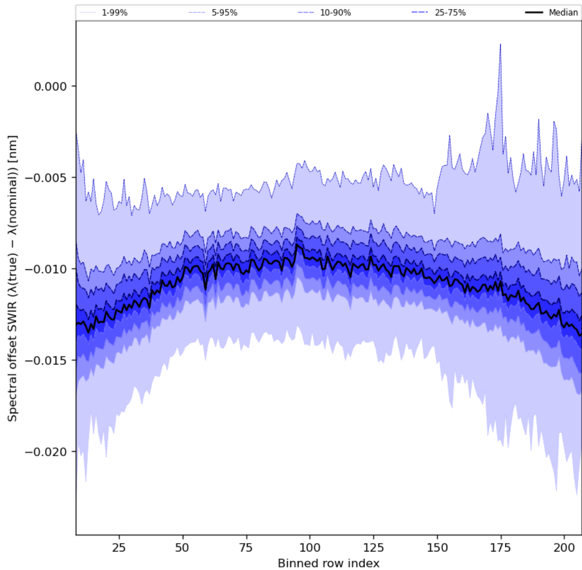
Figure 38: Along track statistics of “Spectral offset SWIR ( \lambda(\text{true}) - \lambda(\text{nominal}) )” for 2023-12-12 to 2023-12-14
