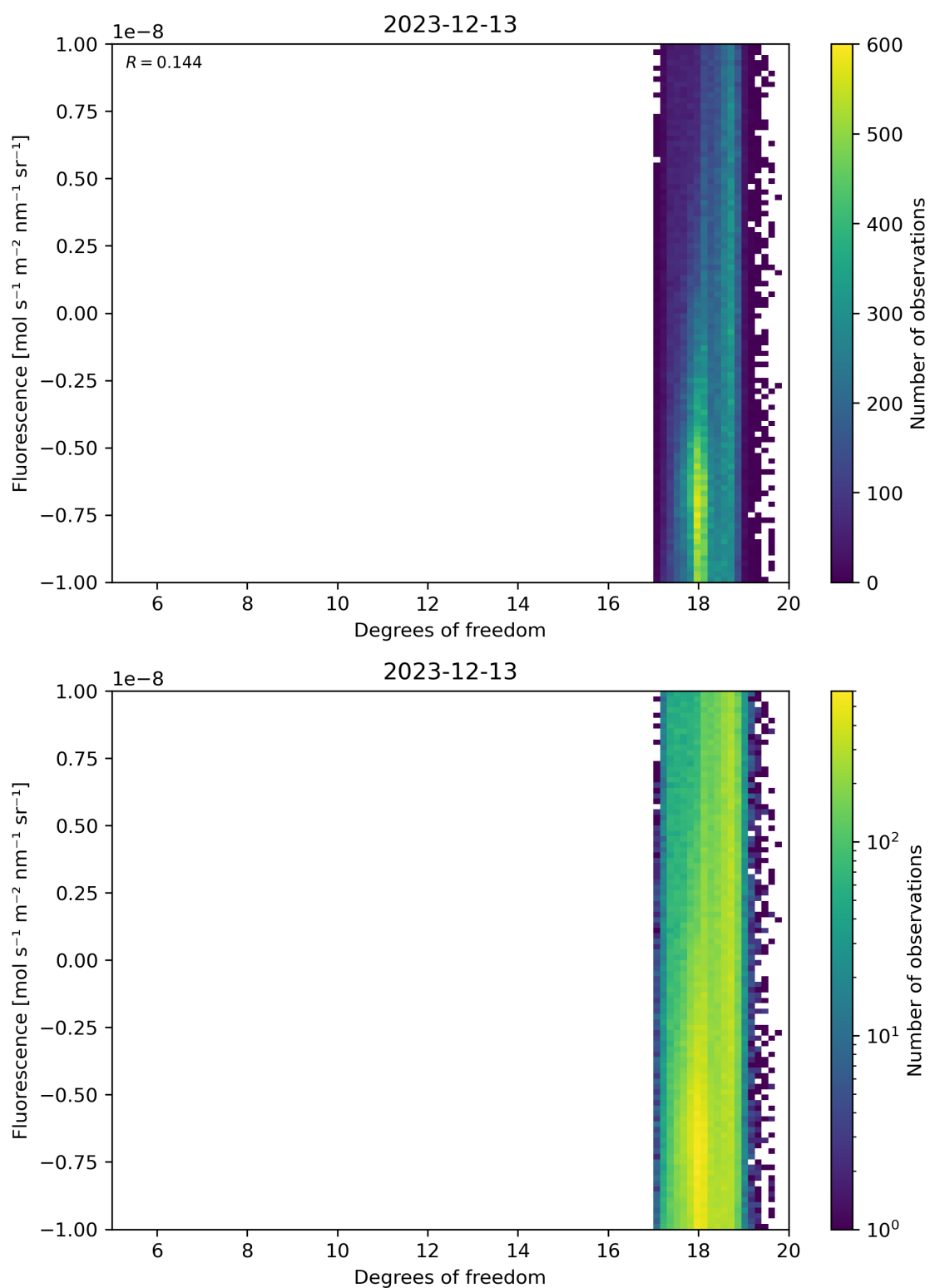
Figure 51: Scatter density plot of “Degrees of freedom” against “Fluorescence” for 2023-12-12 to 2023-12-14.
