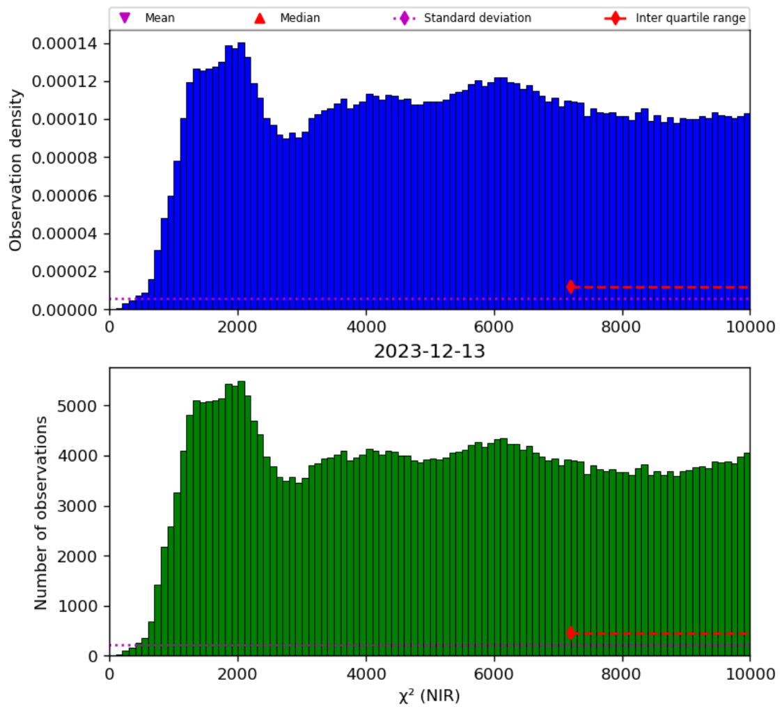
Figure 29: Histogram of “ \chi^2 (NIR)” for 2023-12-12 to 2023-12-14
