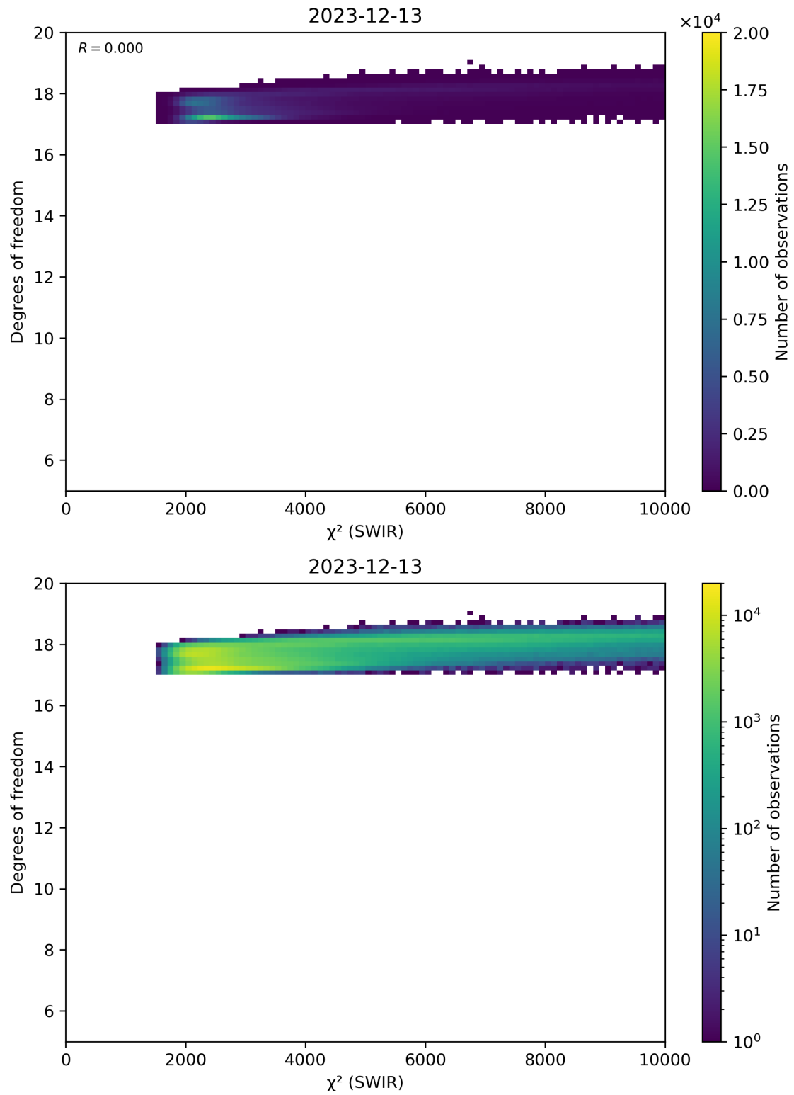
Figure 48: Scatter density plot of “ \chi^2 (SWIR)” against “Degrees of freedom” for 2023-12-12 to 2023-12-14.
