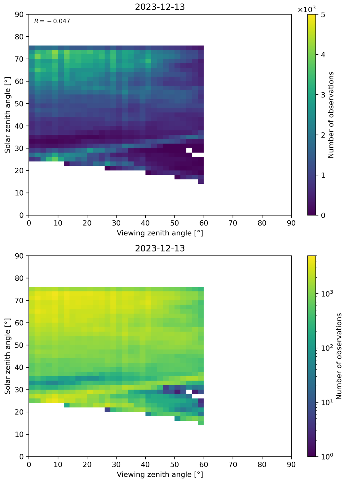
Figure 115: Scatter density plot of “Viewing zenith angle” against “Solar zenith angle” for 2023-12-12 to 2023-12-14.
