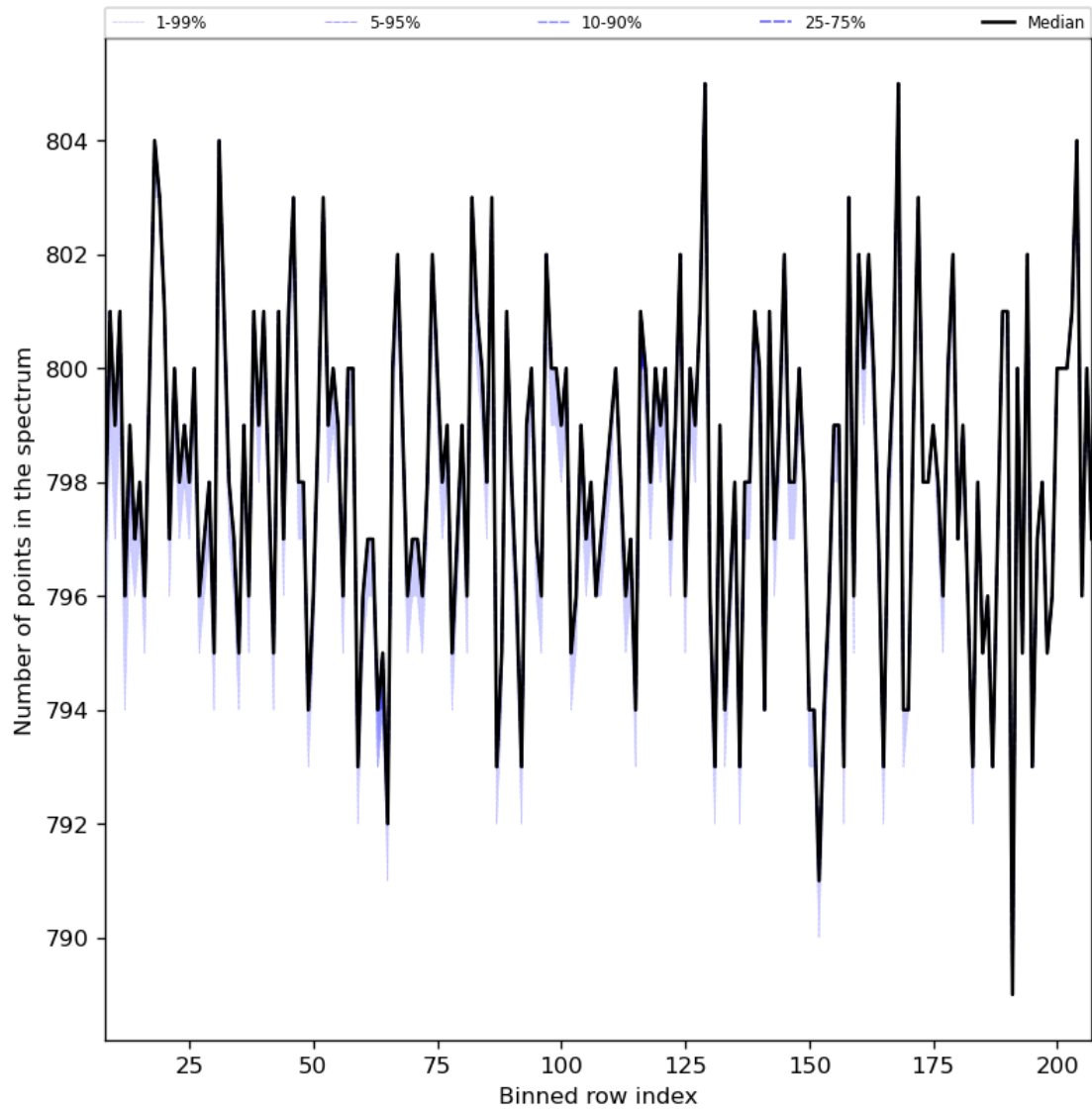
Figure 37: Along track statistics of “Number of points in the spectrum” for 2023-12-12 to 2023-12-14
