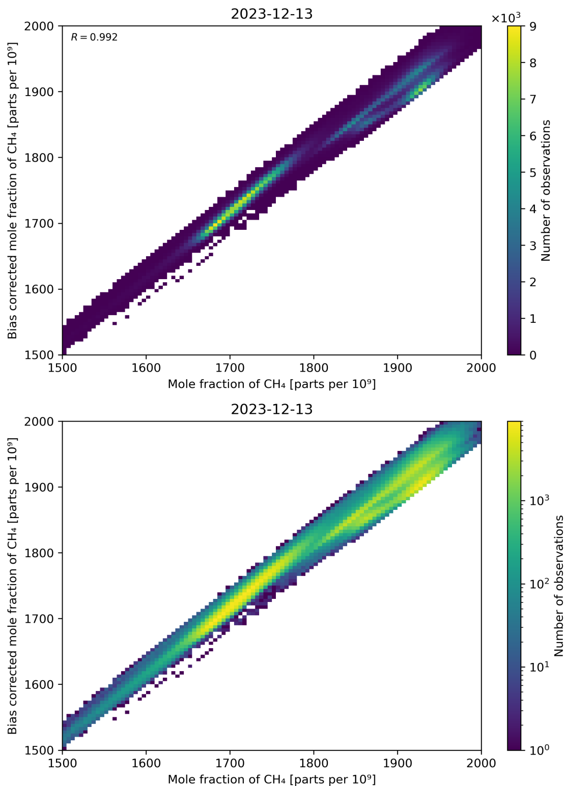
Figure 74: Scatter density plot of “Mole fraction of CH 4 ” against “Bias corrected mole fraction of CH 4 ” for 2023-12-12 to 2023-12-14.
