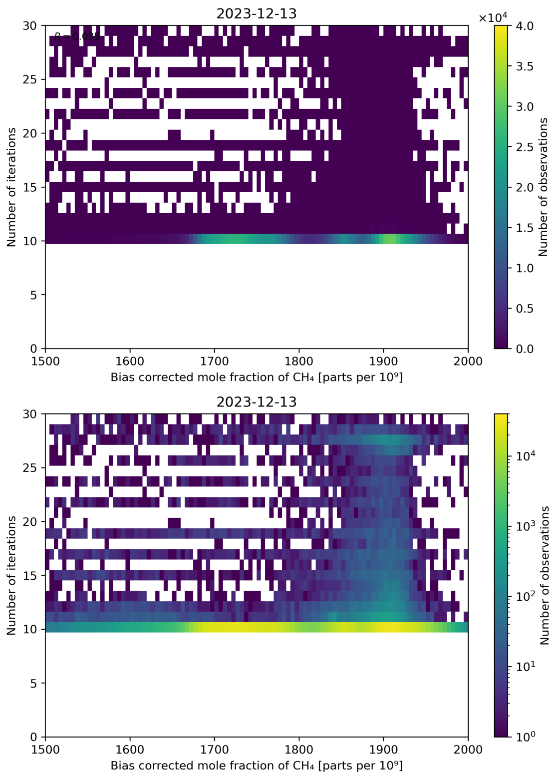
Figure 67: Scatter density plot of “Bias corrected mole fraction of CH 4 ” against “Number of iterations” for 2023-12-12 to 2023-12-14.
