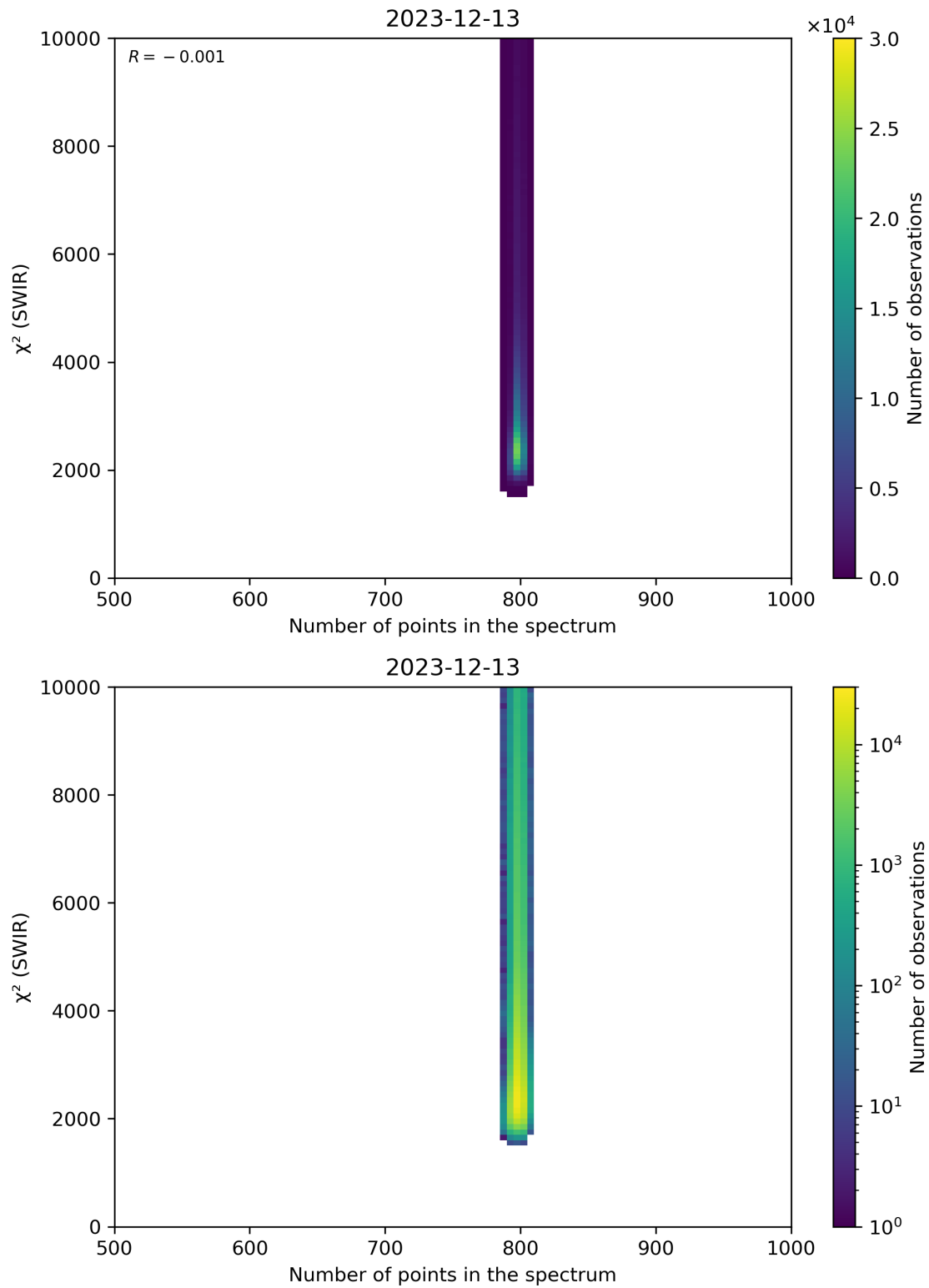
Figure 89: Scatter density plot of “Number of points in the spectrum” against “ \chi^2 (SWIR)” for 2023-12-12 to 2023-12-14.
