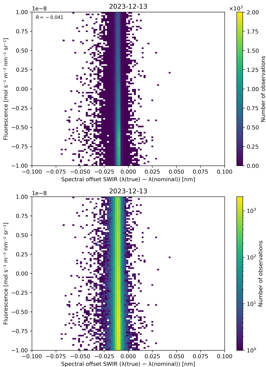
Figure 120: Scatter density plot of “Spectral offset SWIR ( \lambda(\text{true}) - \lambda(\text{nominal}) )” against “Fluorescence” for 2023-12-12 to 2023-12-14.
