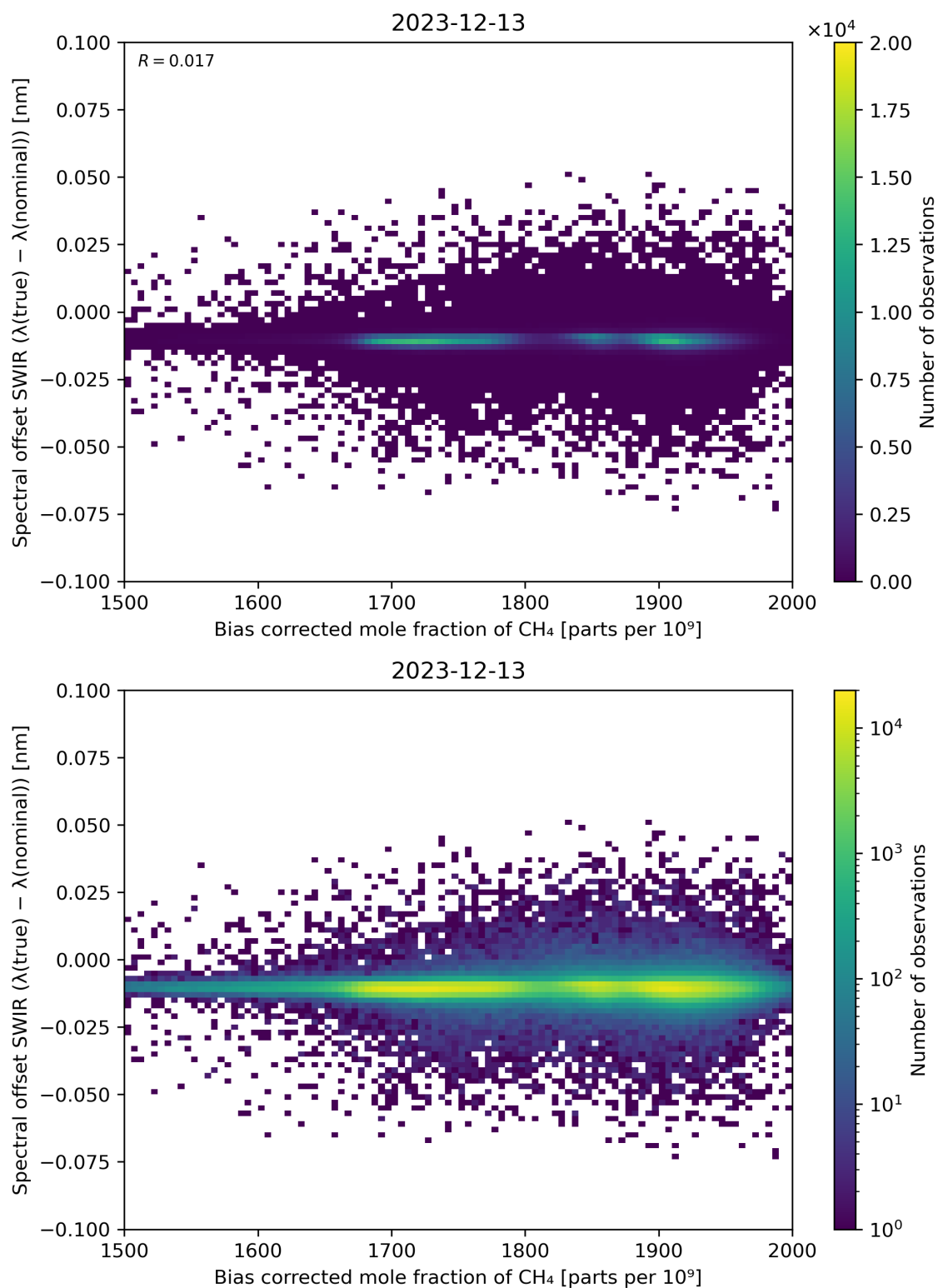
Figure 69: Scatter density plot of “Bias corrected mole fraction of \text{CH}_4 ” against “Spectral offset SWIR ( \lambda(\text{true}) - \lambda(\text{nominal}) )” for 2023-12-12 to 2023-12-14.
