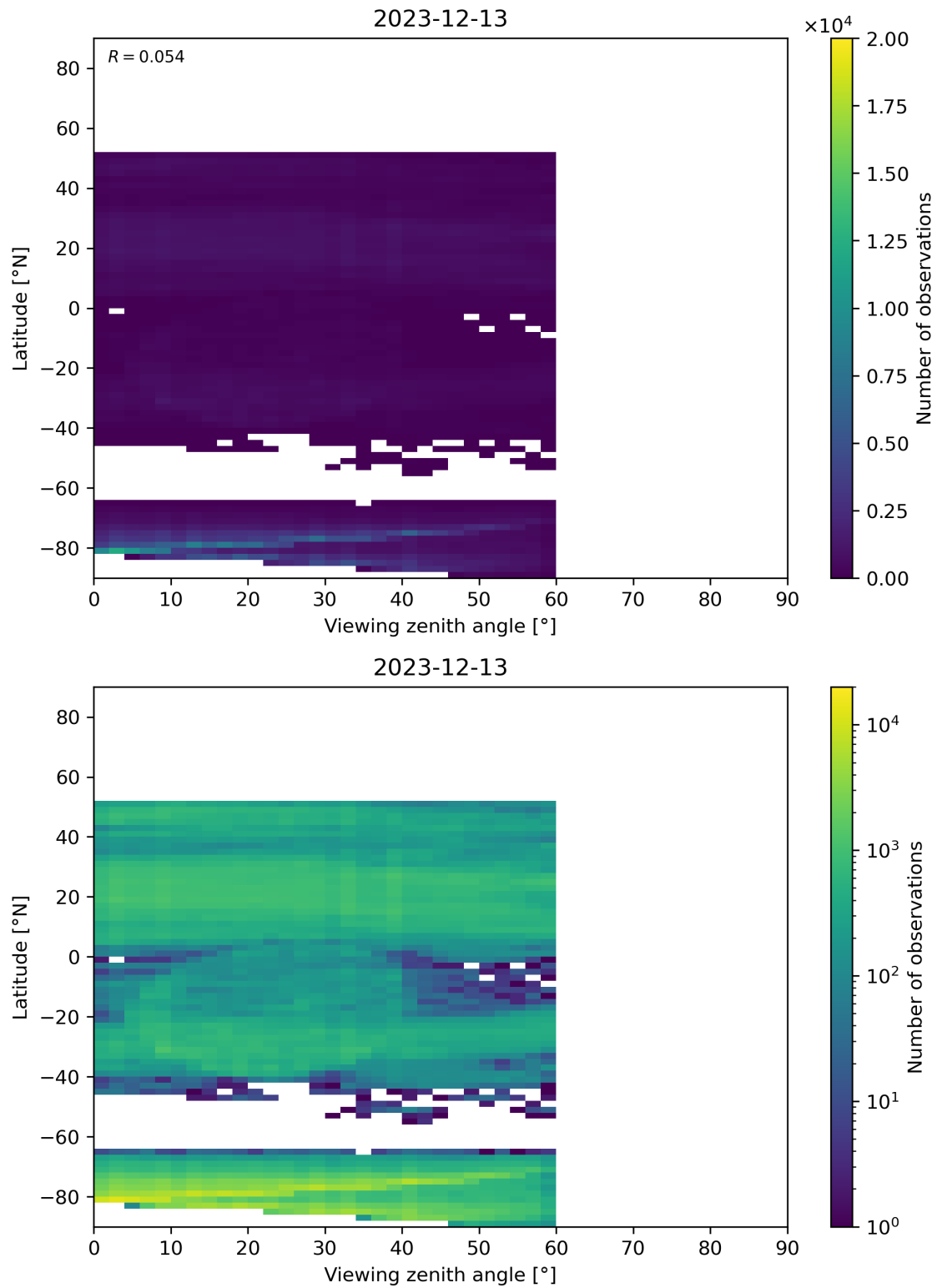
Figure 109: Scatter density plot of “Viewing zenith angle” against “Latitude” for 2023-12-12 to 2023-12-14.
