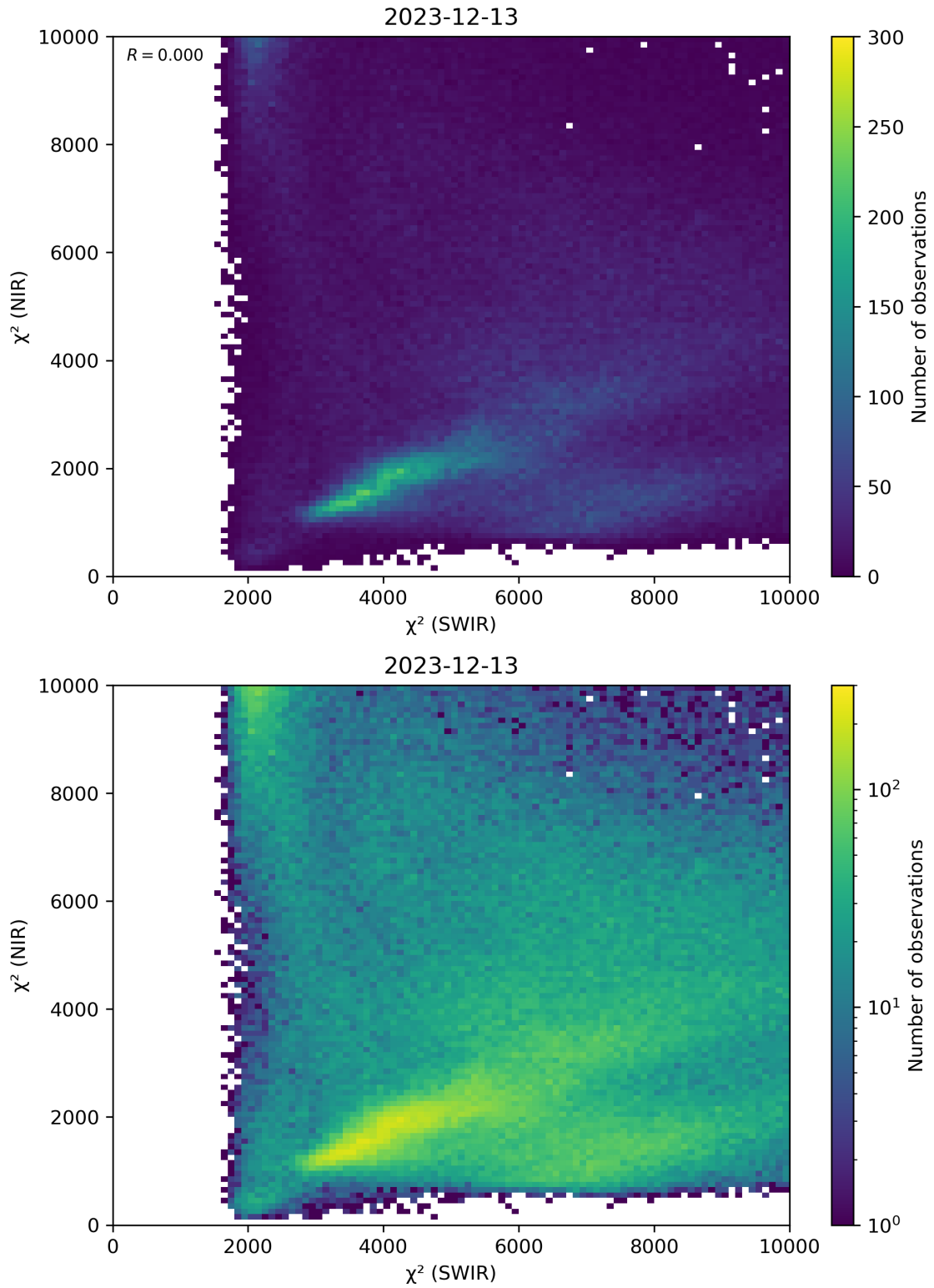
Figure 47: Scatter density plot of “ \chi^2 (SWIR)” against “ \chi^2 (NIR)” for 2023-12-12 to 2023-12-14.
