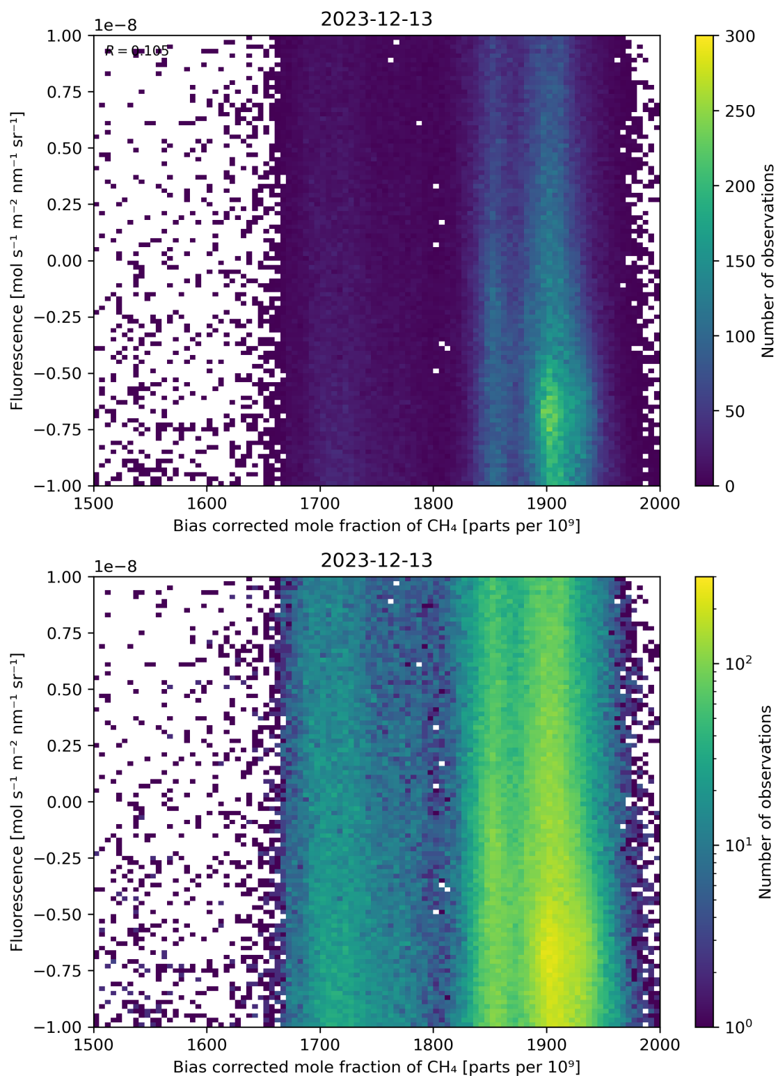
Figure 66: Scatter density plot of “Bias corrected mole fraction of \text{CH}_4 ” against “Fluorescence” for 2023-12-12 to 2023-12-14.
