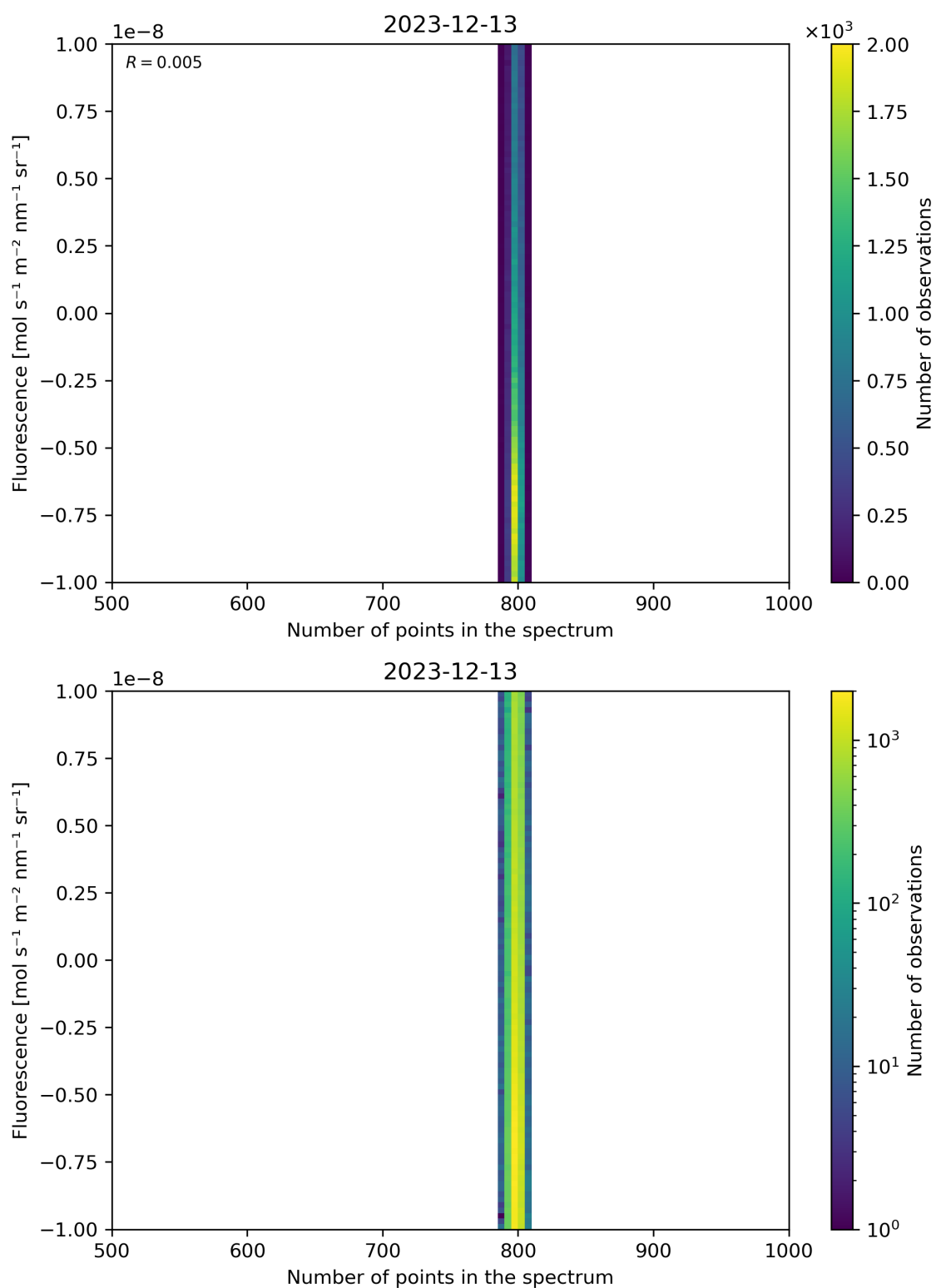
Figure 91: Scatter density plot of “Number of points in the spectrum” against “Fluorescence” for 2023-12-12 to 2023-12-14.
