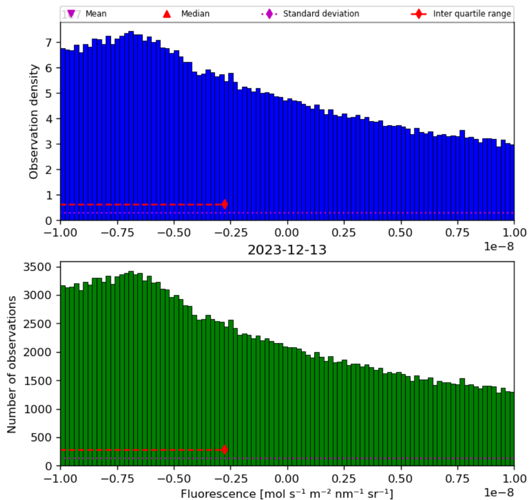
Figure 32: Histogram of “Fluorescence” for 2023-12-12 to 2023-12-14
