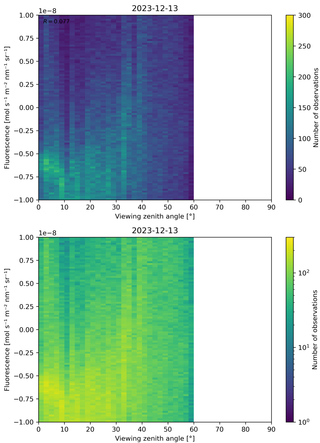
Figure 108: Scatter density plot of “Viewing zenith angle” against “Fluorescence” for 2023-12-12 to 2023-12-14.
