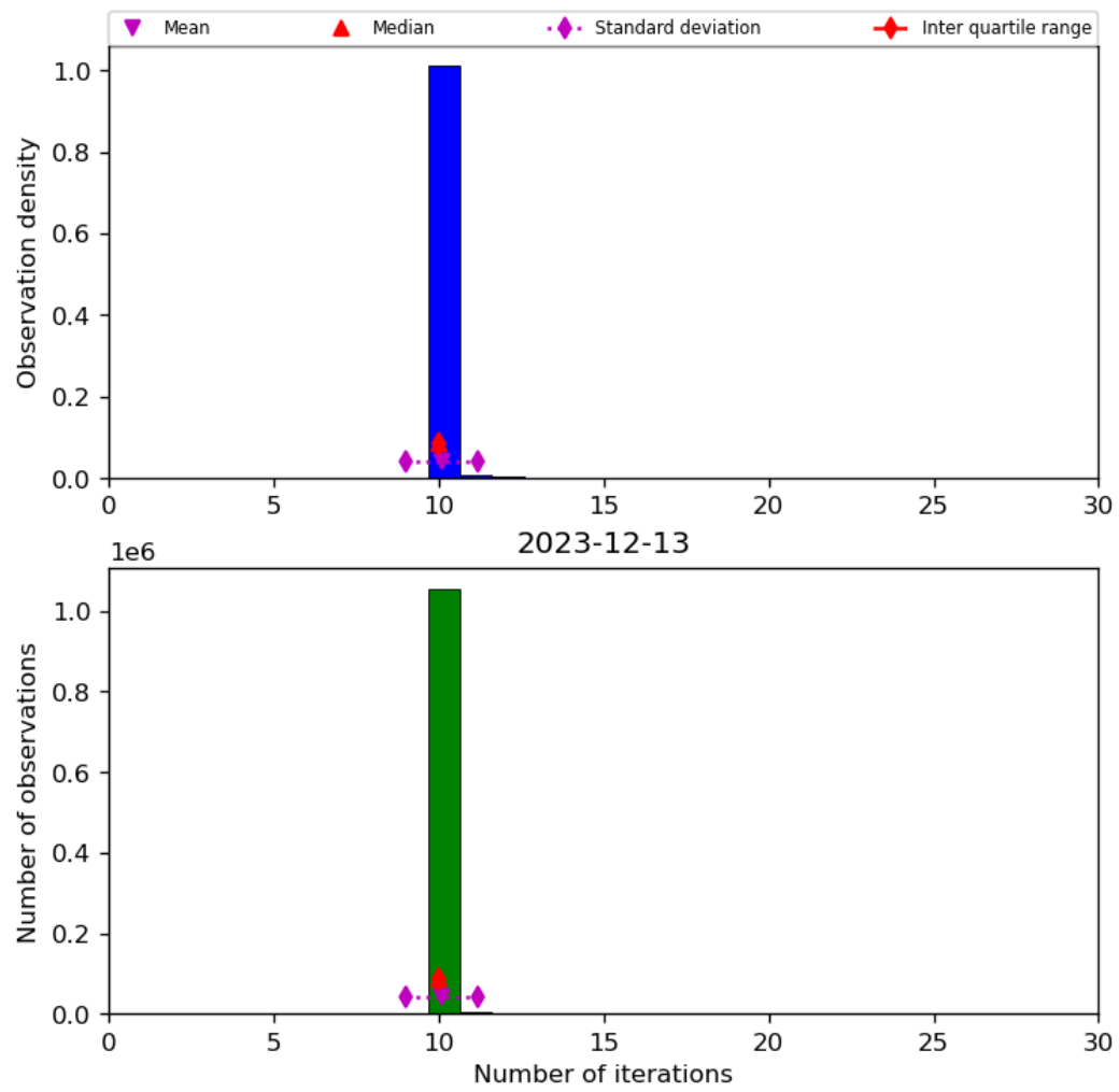
Figure 31: Histogram of “Number of iterations” for 2023-12-12 to 2023-12-14
