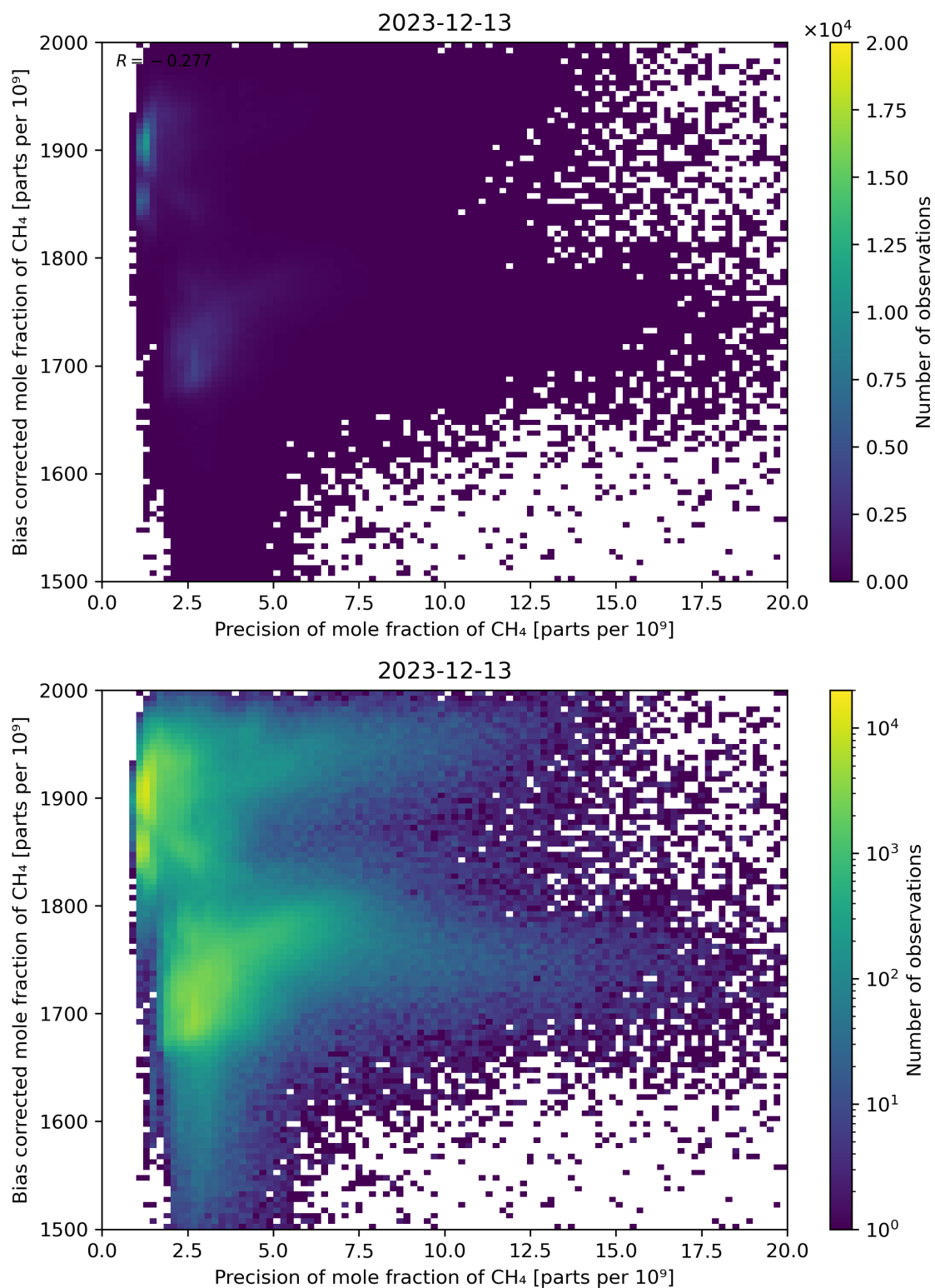
Figure 82: Scatter density plot of “Precision of mole fraction of CH 4 ” against “Bias corrected mole fraction of CH 4 ” for 2023-12-12 to 2023-12-14.
