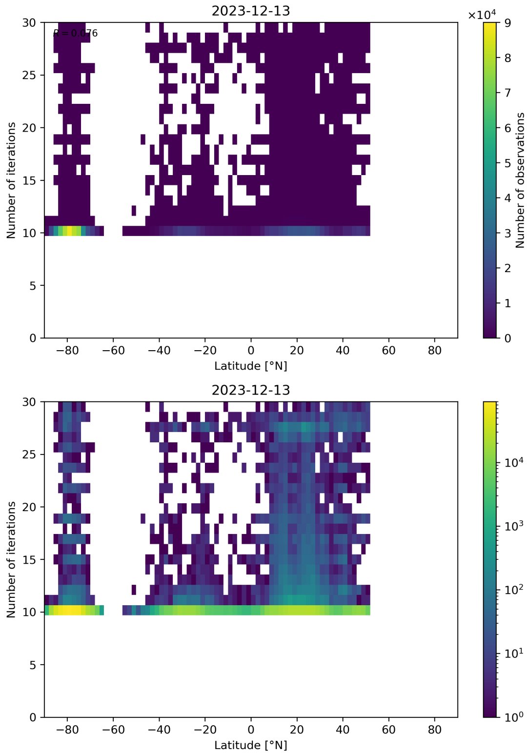
Figure 60: Scatter density plot of “Latitude” against “Number of iterations” for 2023-12-12 to 2023-12-14.
