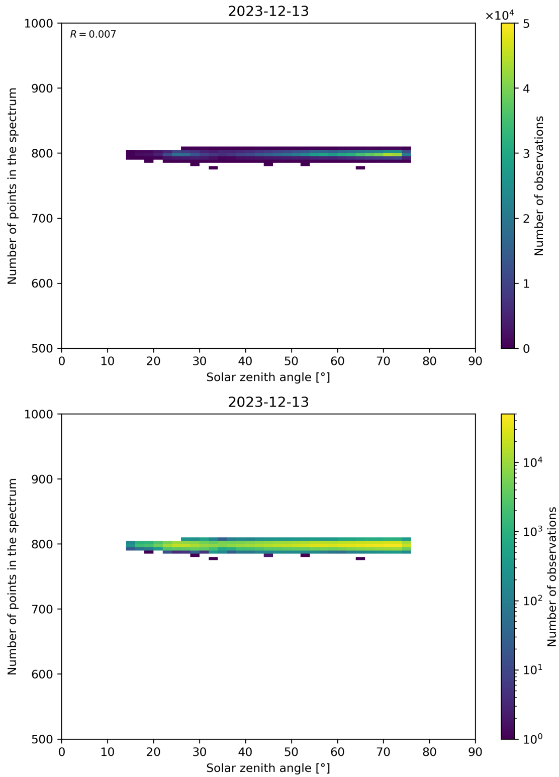
Figure 103: Scatter density plot of “Solar zenith angle” against “Number of points in the spectrum” for 2023-12-12 to 2023-12-14.
