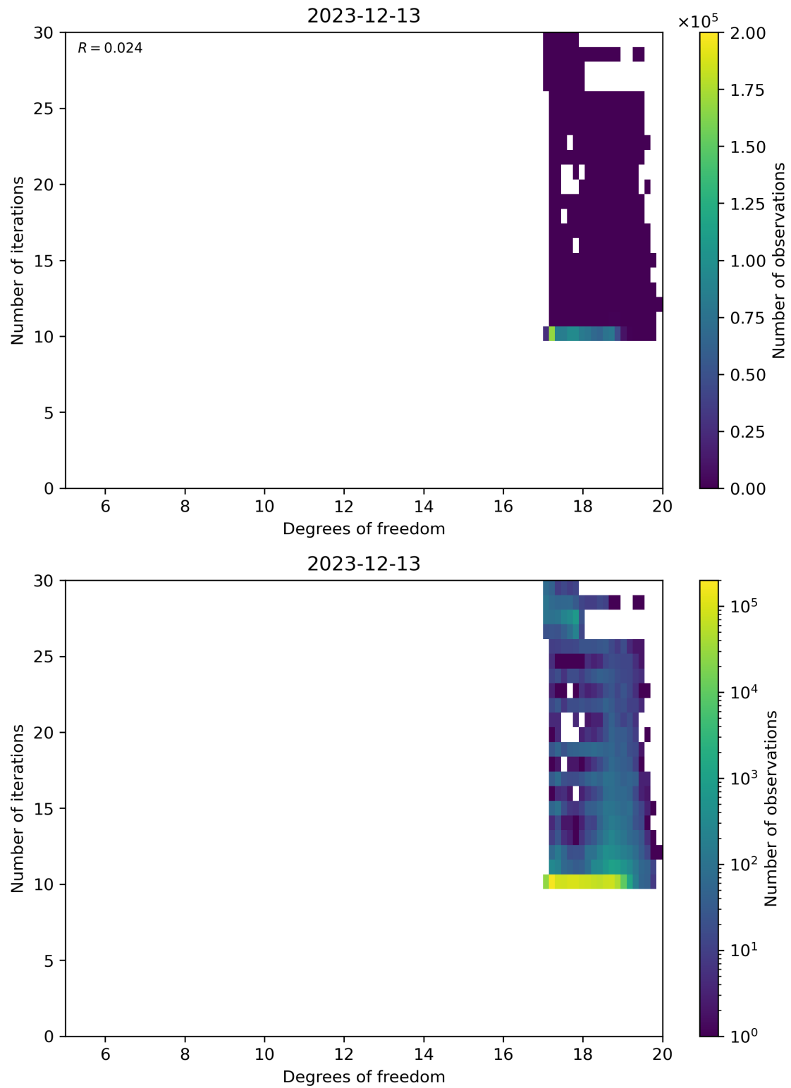
Figure 52: Scatter density plot of “Degrees of freedom” against “Number of iterations” for 2023-12-12 to 2023-12-14.
