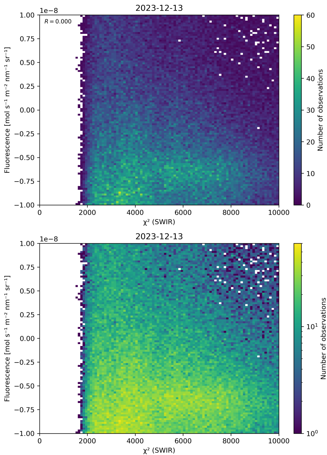
Figure 49: Scatter density plot of “ \chi^2 (SWIR)” against “Fluorescence” for 2023-12-12 to 2023-12-14.
