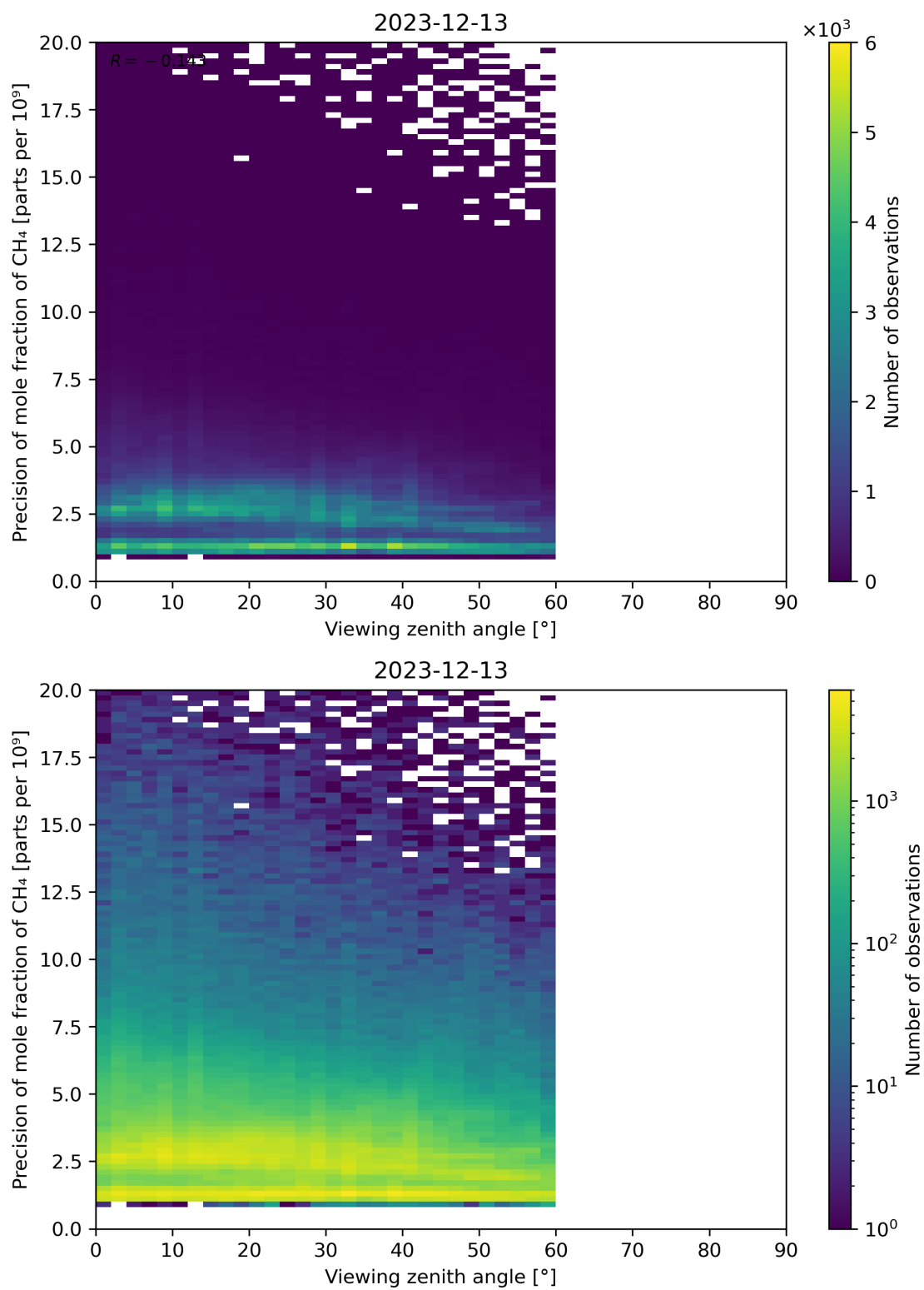
Figure 112: Scatter density plot of “Viewing zenith angle” against “Precision of mole fraction of CH 4 ” for 2023-12-12 to 2023-12-14.
