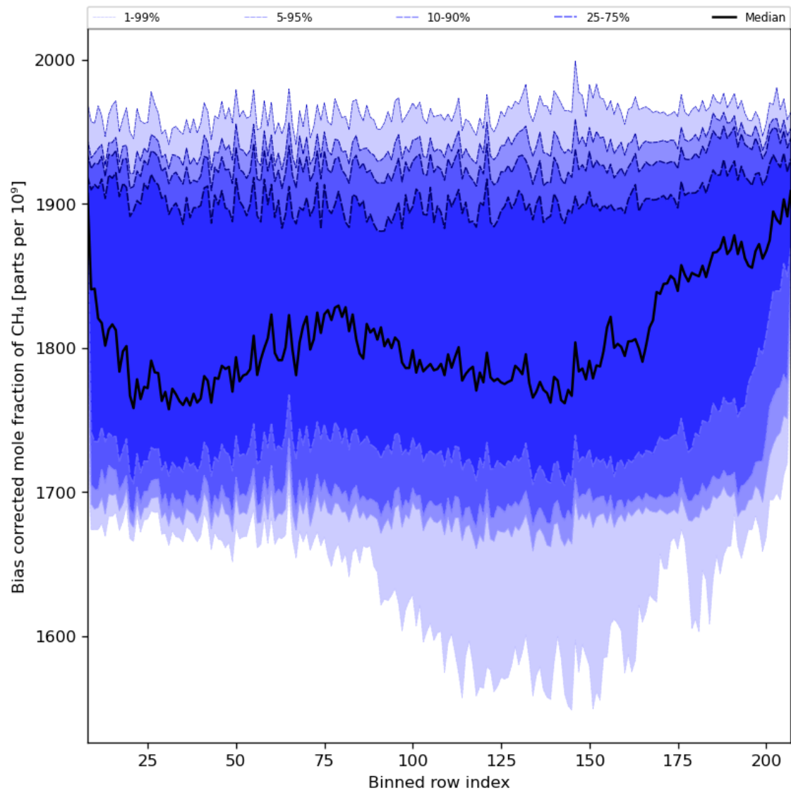
Figure 36: Along track statistics of “Bias corrected mole fraction of CH 4 ” for 2023-12-12 to 2023-12-14
