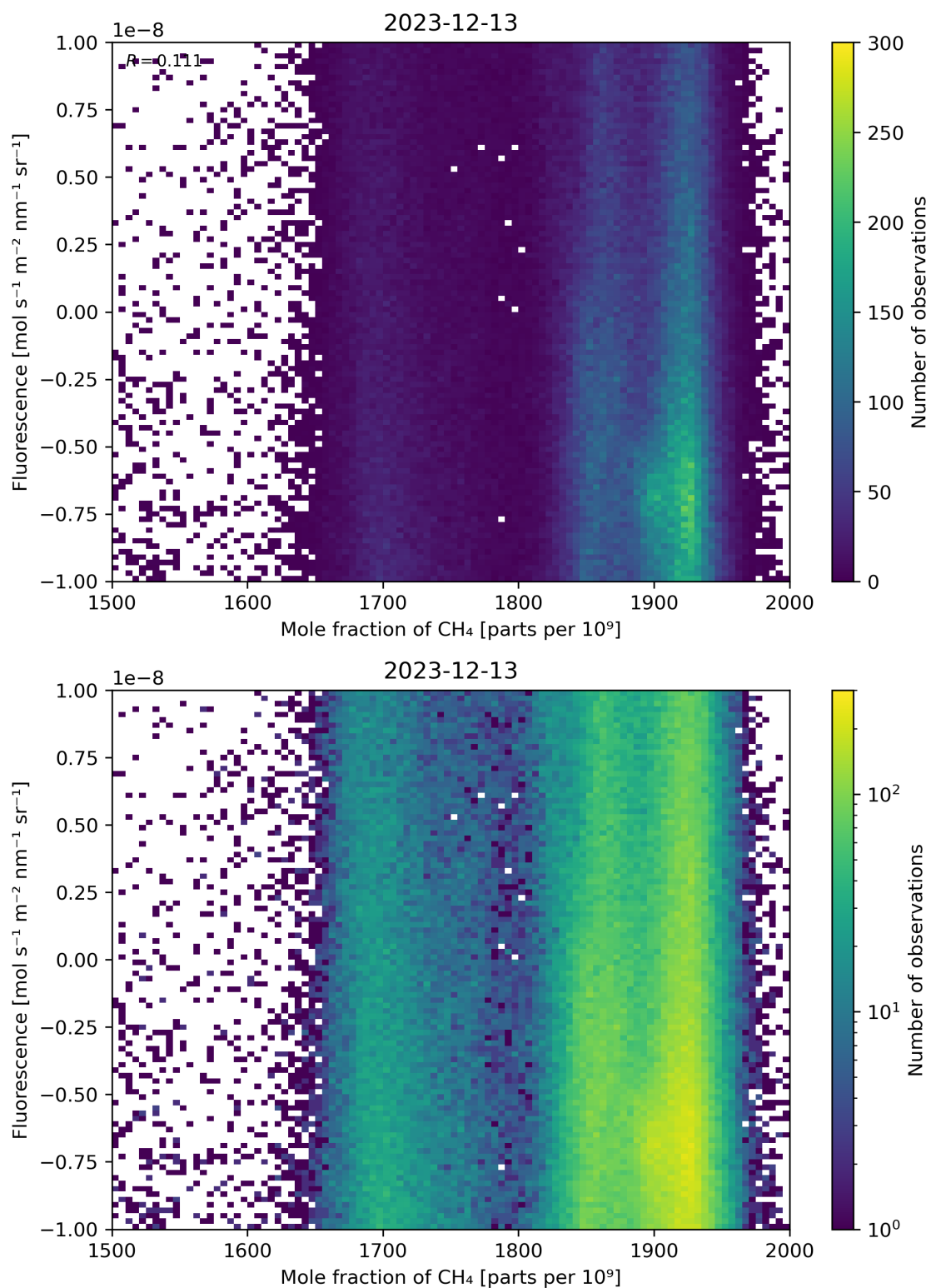
Figure 73: Scatter density plot of “Mole fraction of CH 4 ” against “Fluorescence” for 2023-12-12 to 2023-12-14.
