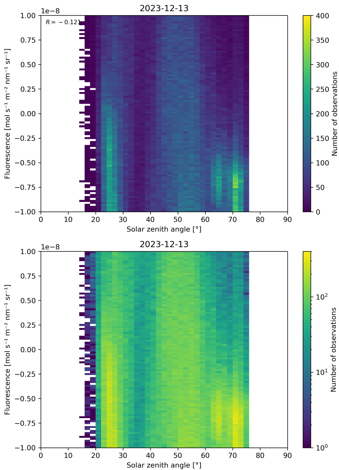
Figure 97: Scatter density plot of “Solar zenith angle” against “Fluorescence” for 2023-12-12 to 2023-12-14.
