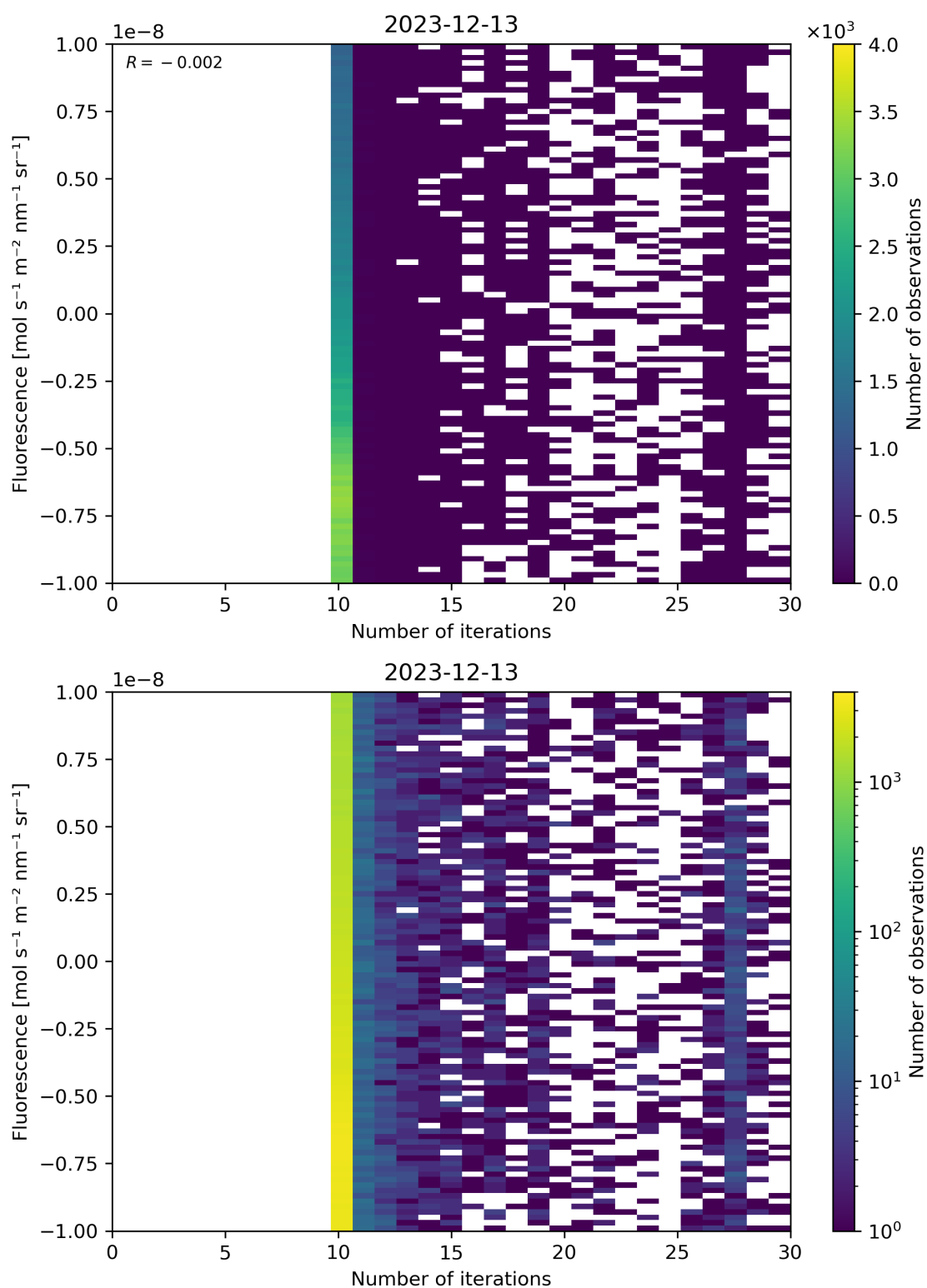
Figure 87: Scatter density plot of “Number of iterations” against “Fluorescence” for 2023-12-12 to 2023-12-14.
