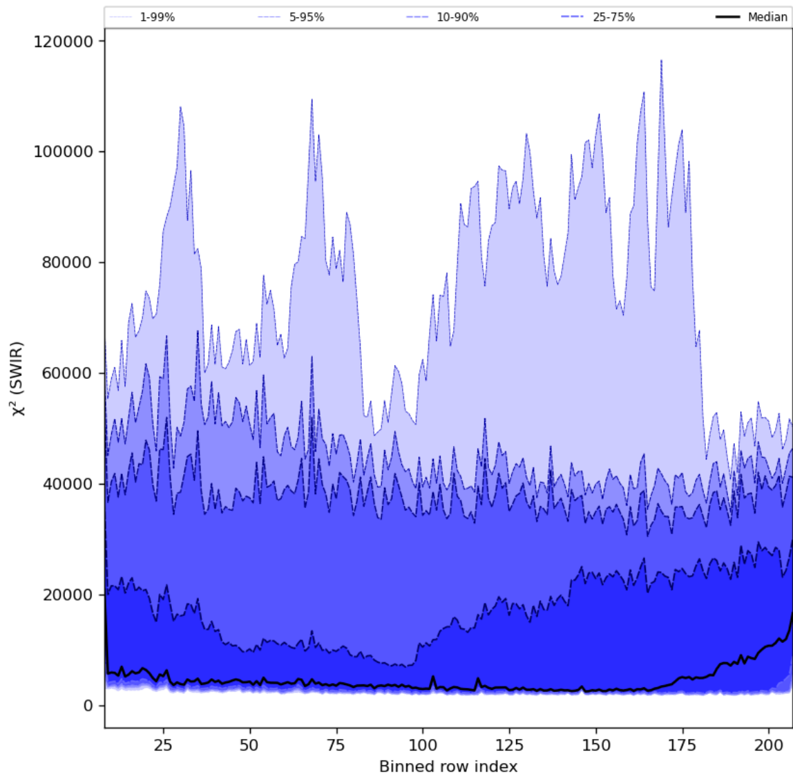
Figure 39: Along track statistics of " \chi^2 (SWIR)" for 2023-12-12 to 2023-12-14
