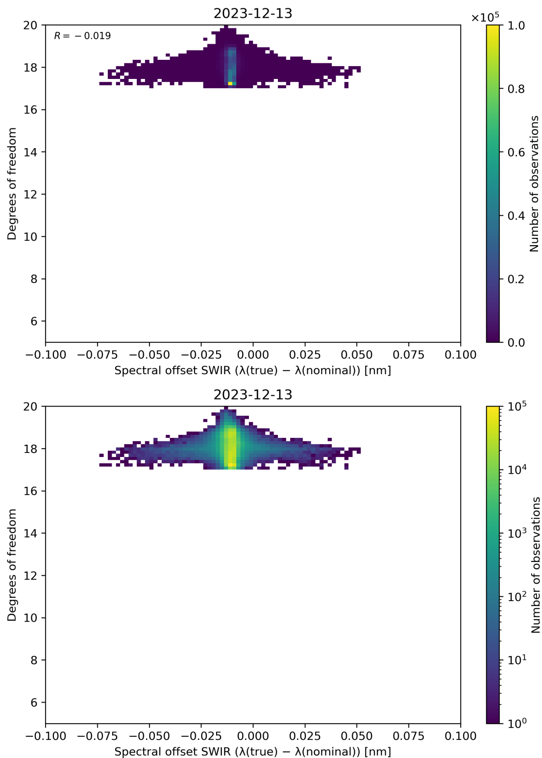
Figure 119: Scatter density plot of “Spectral offset SWIR ( \lambda(\text{true}) - \lambda(\text{nominal}) )” against “Degrees of freedom” for 2023-12-12 to 2023-12-14.
