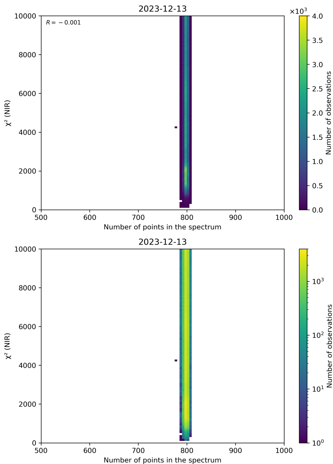
Figure 88: Scatter density plot of “Number of points in the spectrum” against “ \chi^2 (NIR)” for 2023-12-12 to 2023-12-14.
