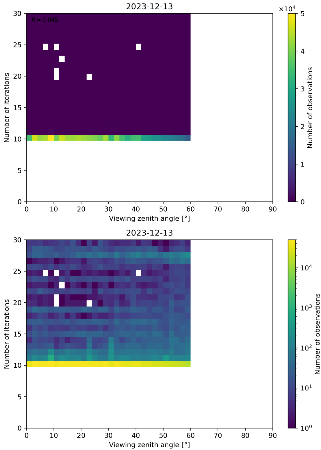
Figure 113: Scatter density plot of “Viewing zenith angle” against “Number of iterations” for 2023-12-12 to 2023-12-14.
