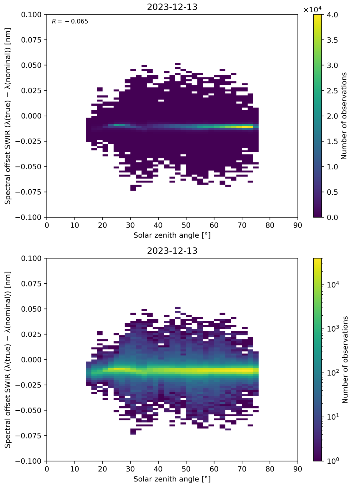
Figure 104: Scatter density plot of “Solar zenith angle” against “Spectral offset SWIR ( \lambda(\text{true}) - \lambda(\text{nominal}) )” for 2023-12-12 to 2023-12-14.
