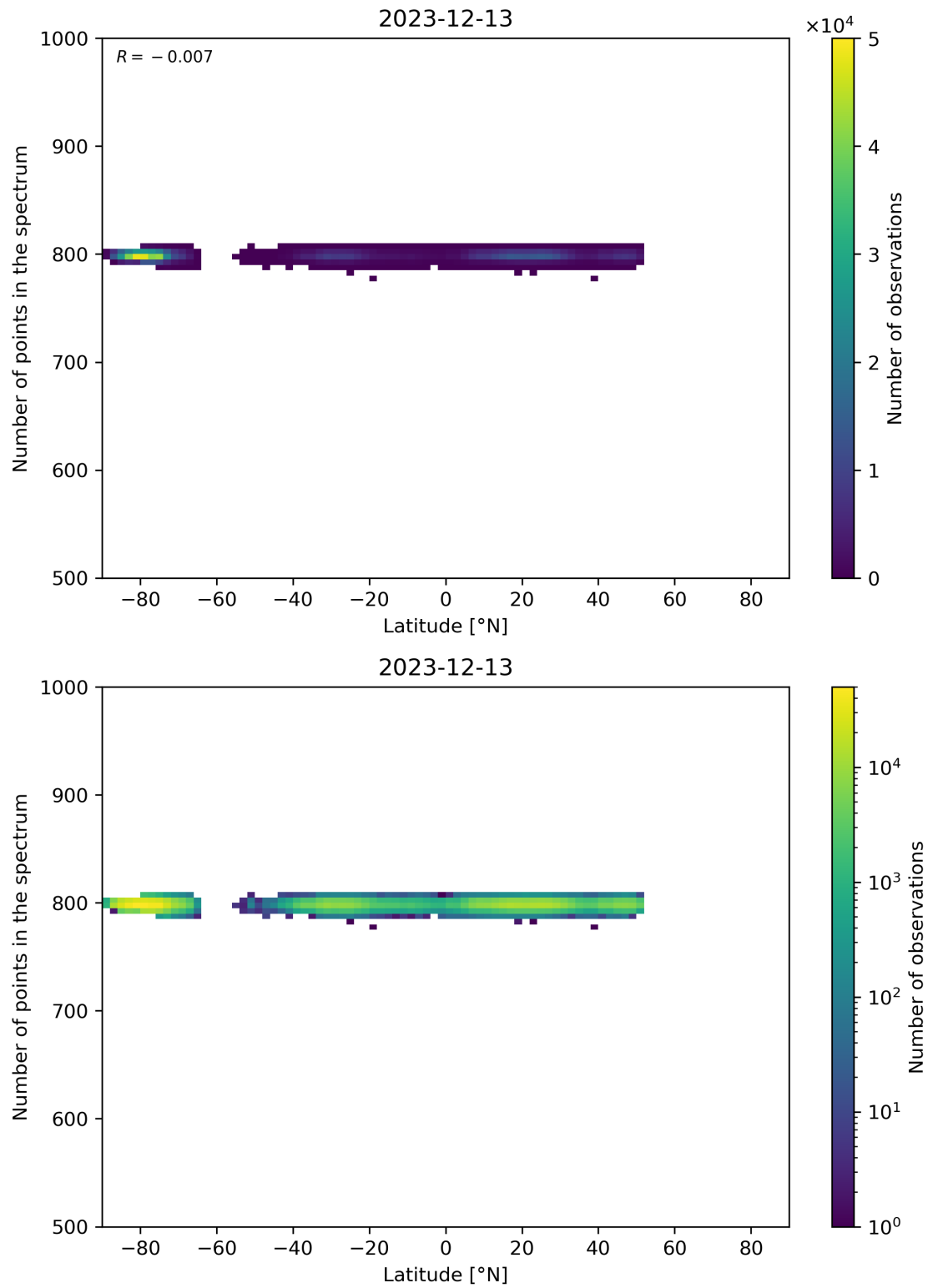
Figure 61: Scatter density plot of “Latitude” against “Number of points in the spectrum” for 2023-12-12 to 2023-12-14.
