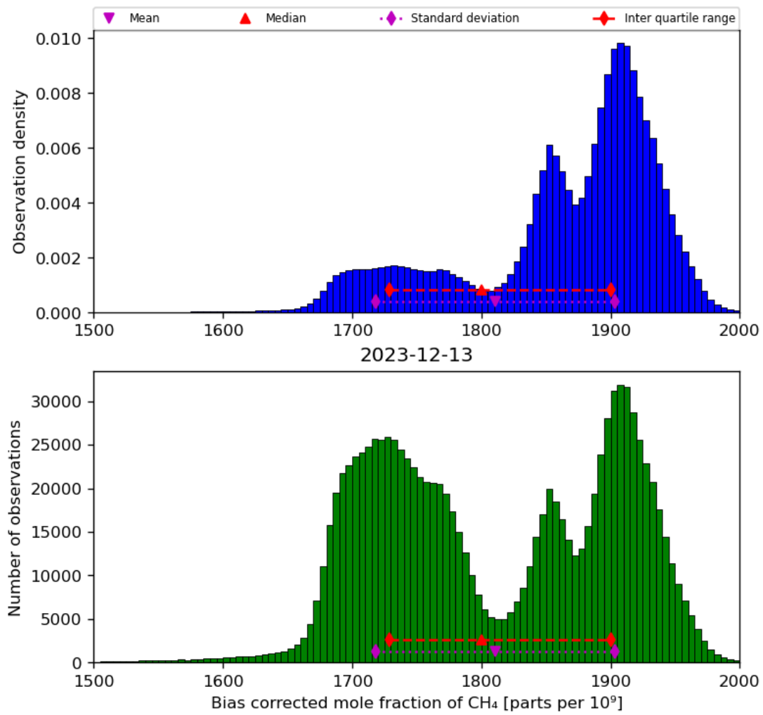
Figure 25: Histogram of “Bias corrected mole fraction of CH 4 ” for 2023-12-12 to 2023-12-14
