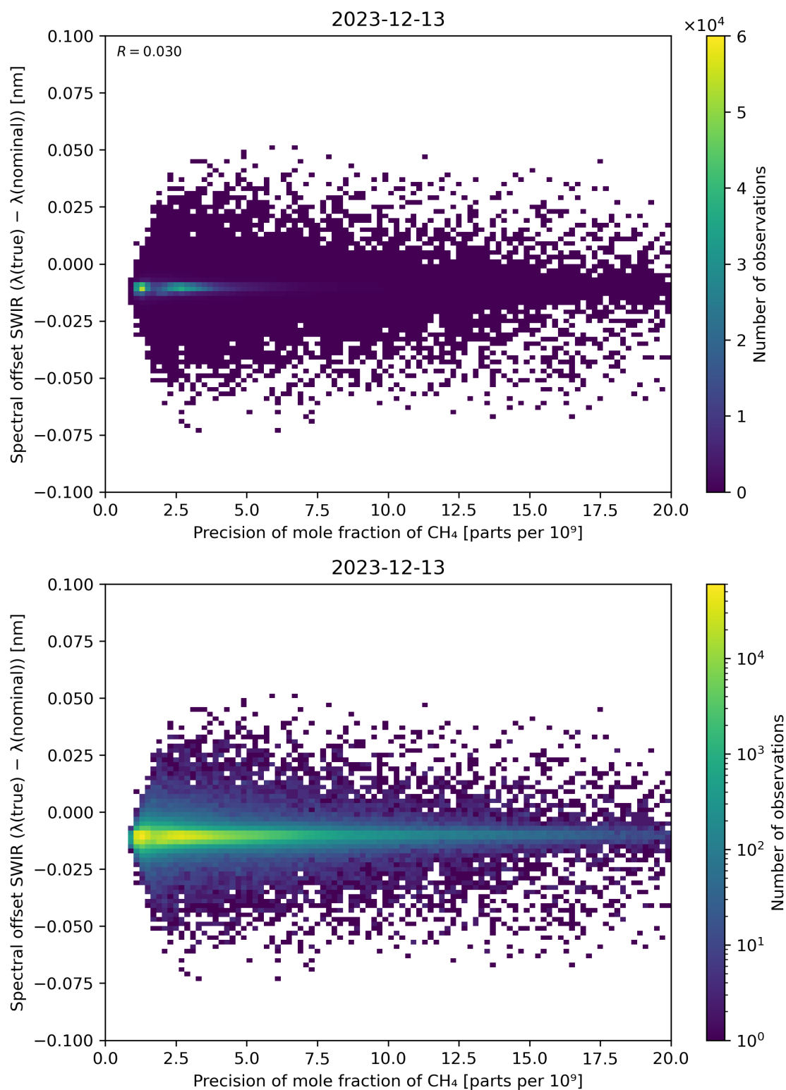
Figure 85: Scatter density plot of “Precision of mole fraction of CH 4 ” against “Spectral offset SWIR ( \lambda(\text{true}) - \lambda(\text{nominal}) )” for 2023-12-12 to 2023-12-14.
