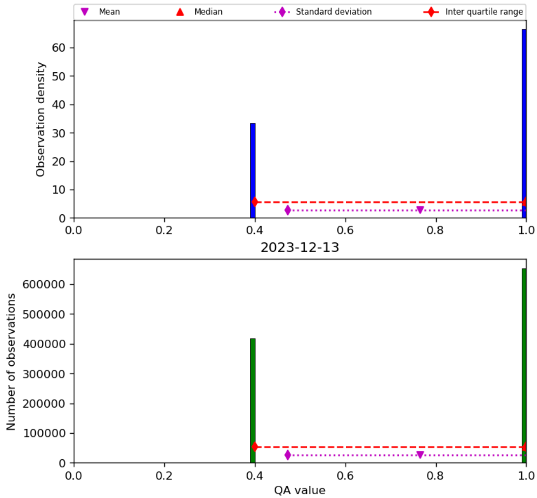
Figure 22: Histogram of “QA value” for 2023-12-12 to 2023-12-14
