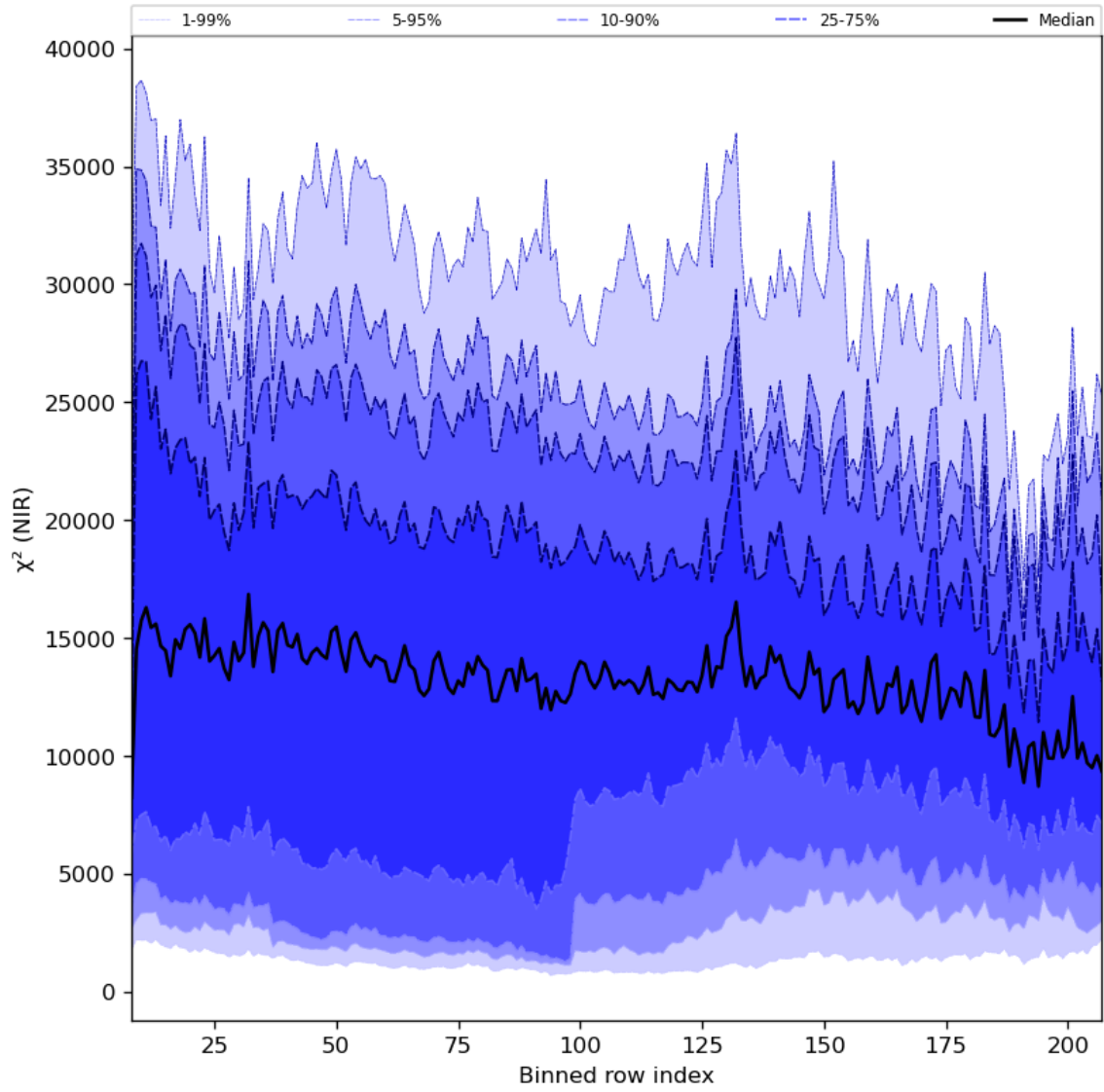
Figure 40: Along track statistics of “ \chi^2 (NIR)” for 2023-12-12 to 2023-12-14
