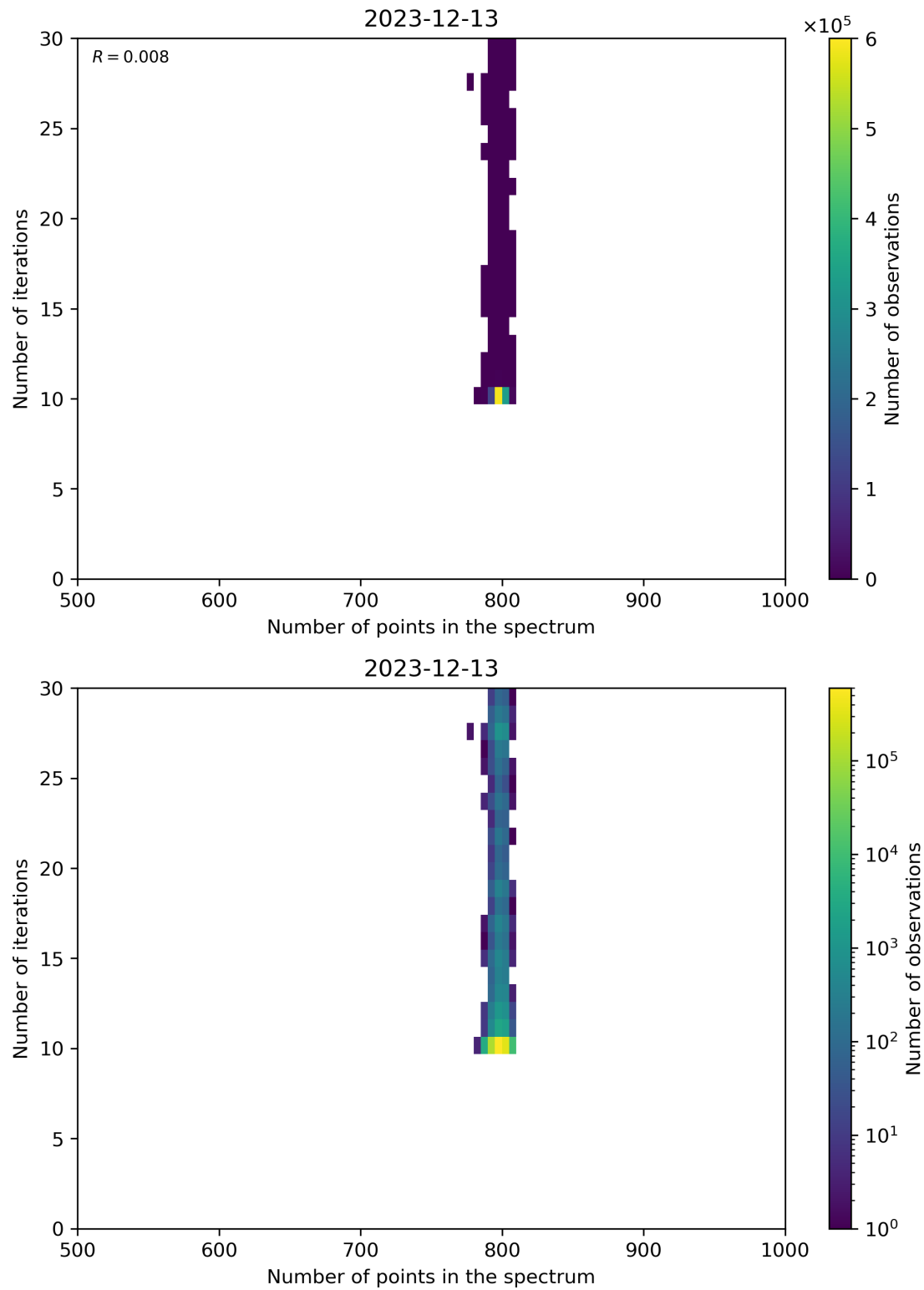
Figure 92: Scatter density plot of “Number of points in the spectrum” against “Number of iterations” for 2023-12-12 to 2023-12-14.
