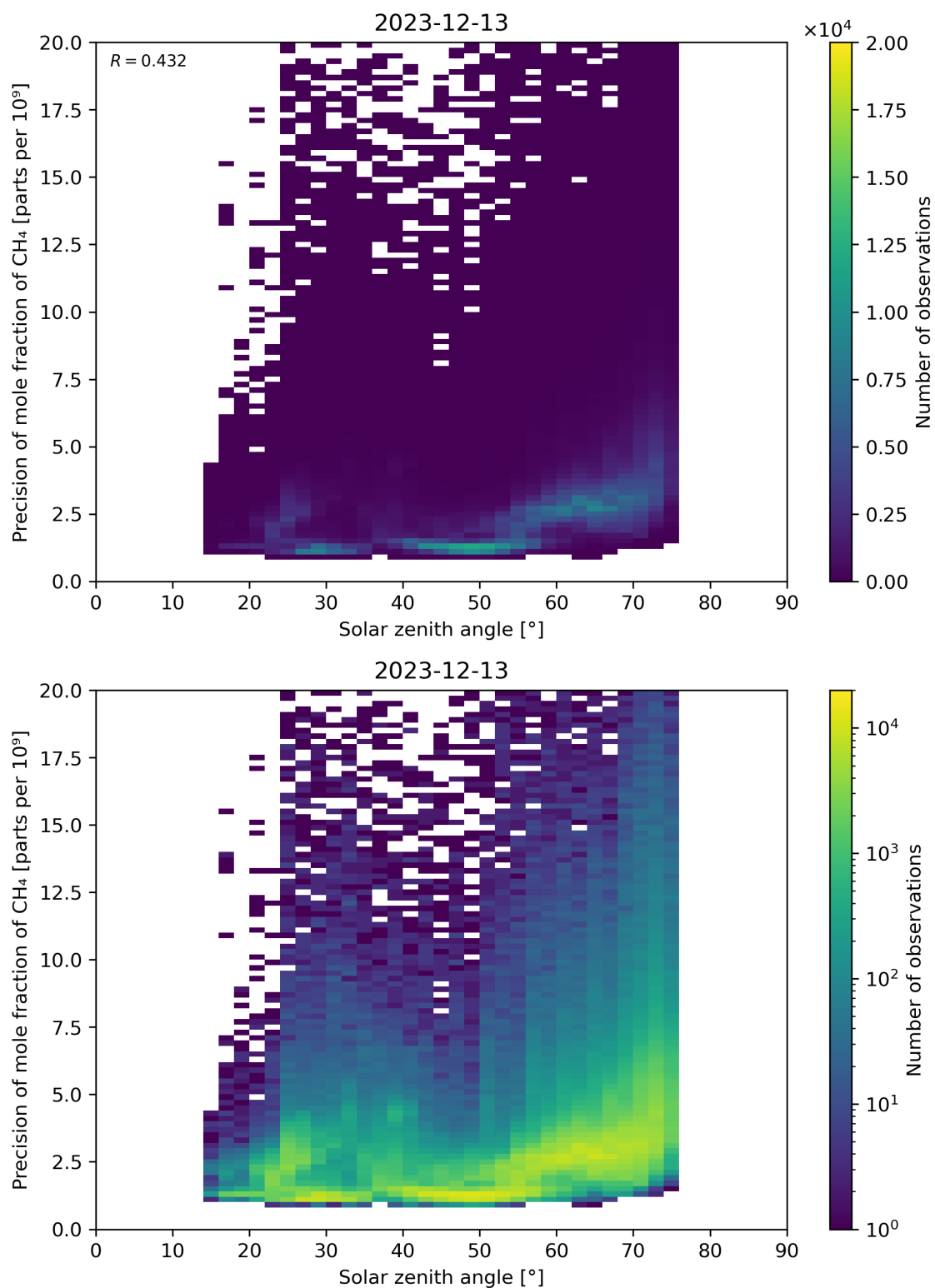
Figure 101: Scatter density plot of “Solar zenith angle” against “Precision of mole fraction of \text{CH}_4 ” for 2023-12-12 to 2023-12-14.
