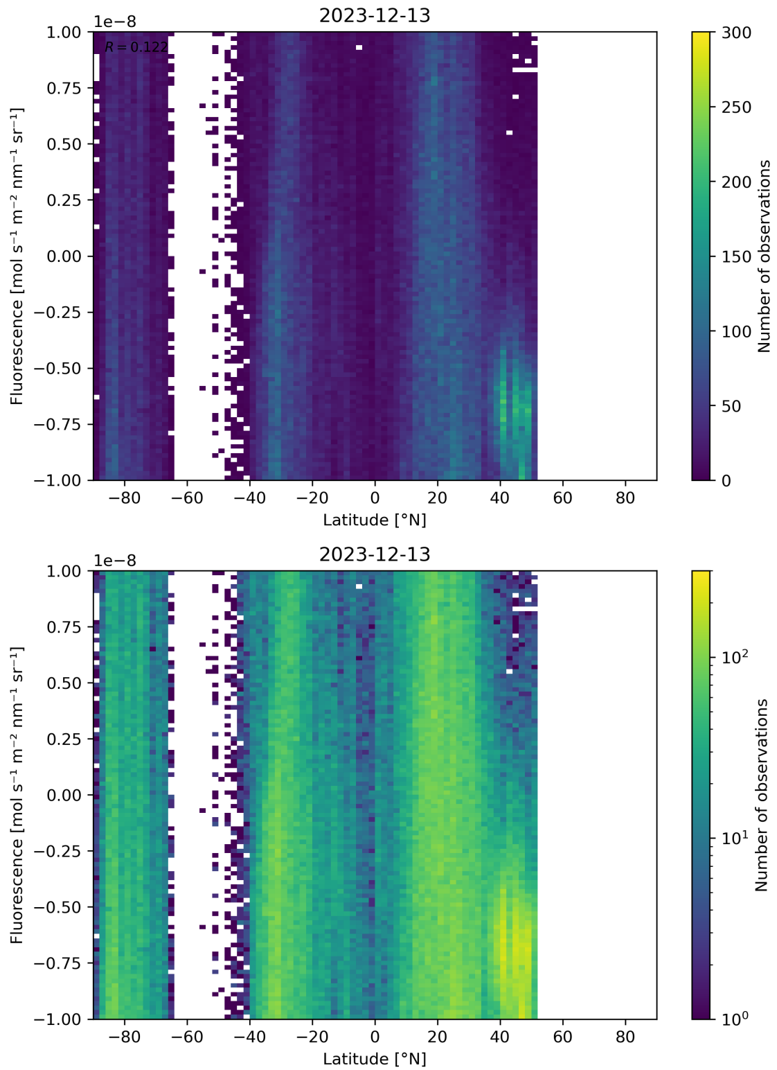
Figure 56: Scatter density plot of “Latitude” against “Fluorescence” for 2023-12-12 to 2023-12-14.
