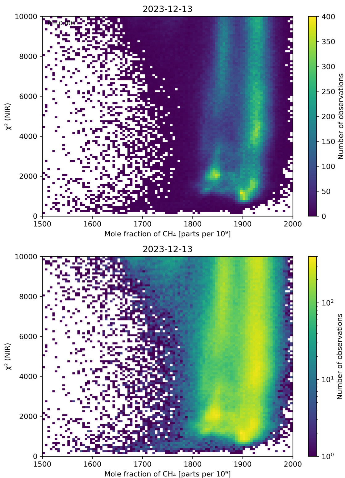
Figure 70: Scatter density plot of “Mole fraction of \text{CH}_4 ” against “ \chi^2 (NIR)” for 2023-12-12 to 2023-12-14.
