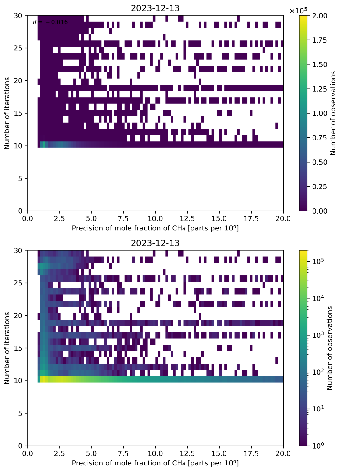
Figure 83: Scatter density plot of “Precision of mole fraction of CH 4 ” against “Number of iterations” for 2023-12-12 to 2023-12-14.
