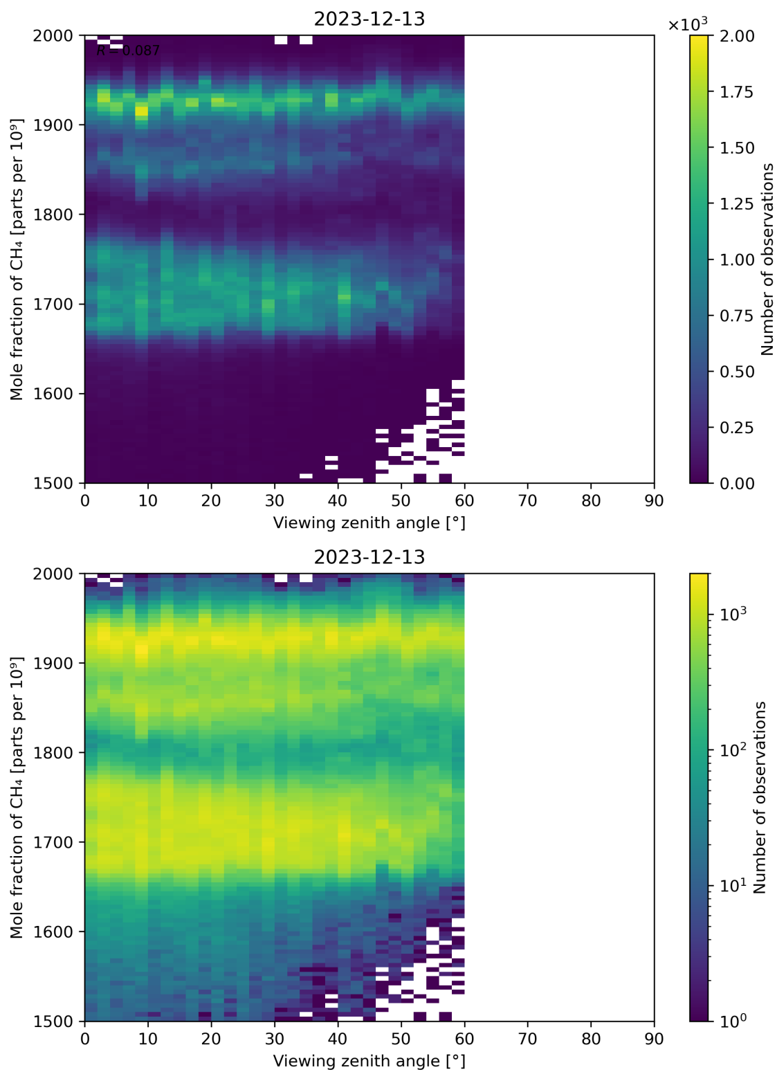
Figure 110: Scatter density plot of “Viewing zenith angle” against “Mole fraction of CH 4 ” for 2023-12-12 to 2023-12-14.
