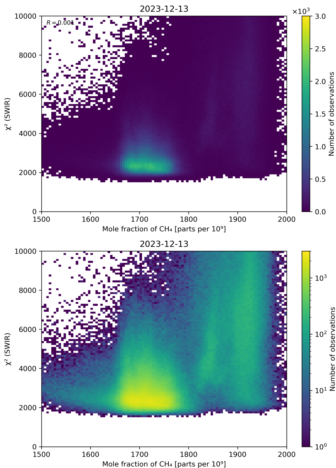
Figure 71: Scatter density plot of “Mole fraction of CH 4 ” against “ \chi^2 (SWIR)” for 2023-12-12 to 2023-12-14.
