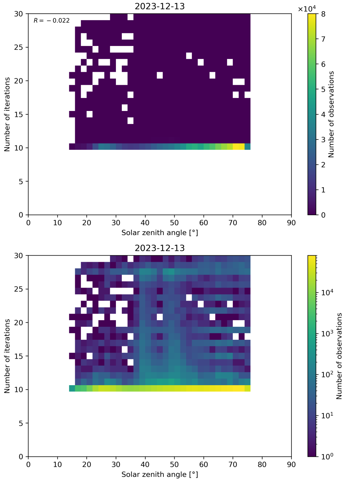
Figure 102: Scatter density plot of “Solar zenith angle” against “Number of iterations” for 2023-12-12 to 2023-12-14.
