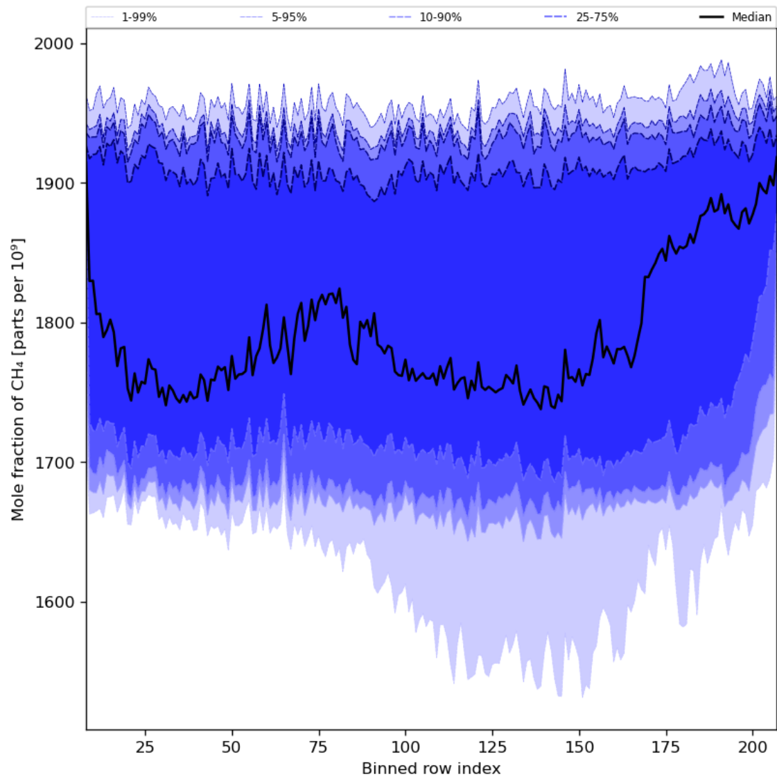
Figure 34: Along track statistics of “Mole fraction of CH 4 ” for 2023-12-12 to 2023-12-14
