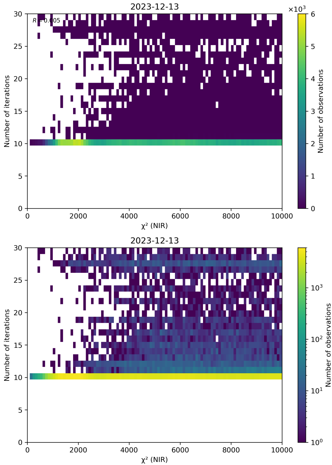
Figure 46: Scatter density plot of “ \chi^2 (NIR)” against “Number of iterations” for 2023-12-12 to 2023-12-14.
