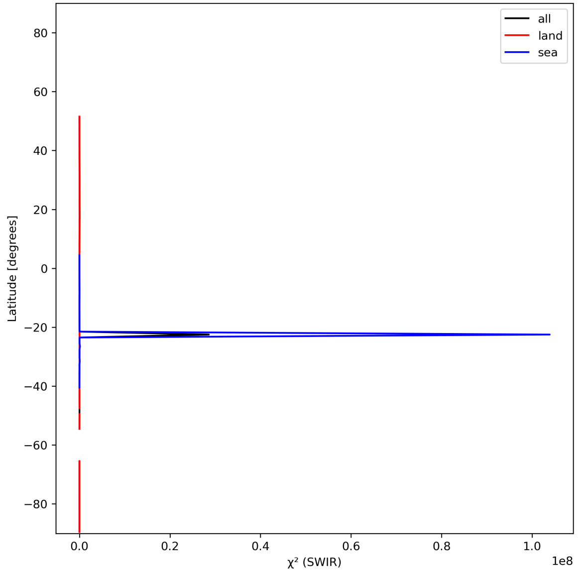
Figure 17: Zonal average of “ \chi^2 (SWIR)” for 2023-12-12 to 2023-12-14.
