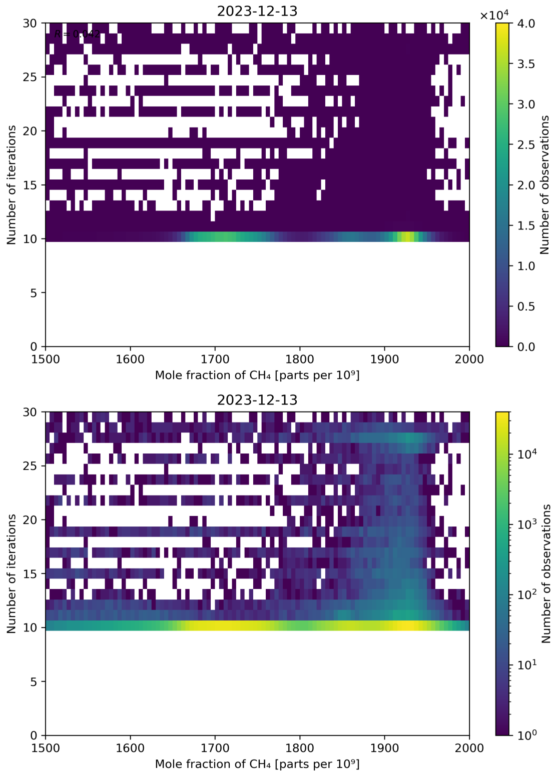
Figure 76: Scatter density plot of “Mole fraction of CH 4 ” against “Number of iterations” for 2023-12-12 to 2023-12-14.
