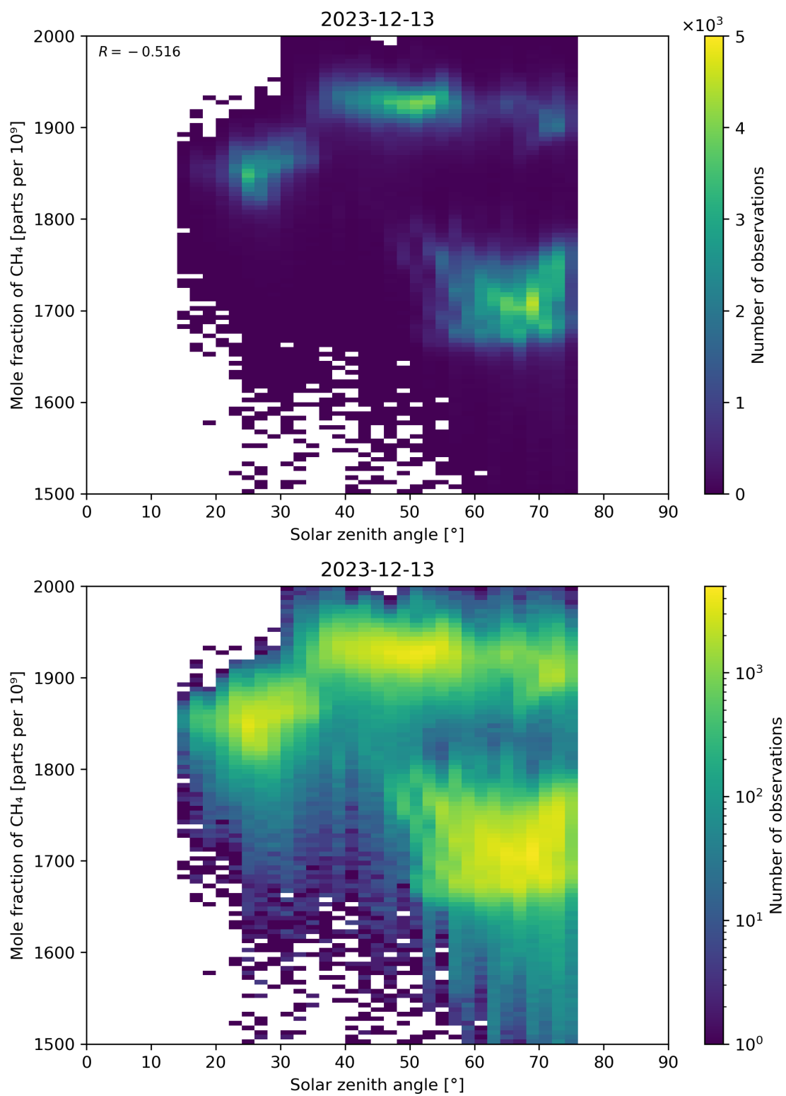
Figure 99: Scatter density plot of “Solar zenith angle” against “Mole fraction of CH 4 ” for 2023-12-12 to 2023-12-14.
