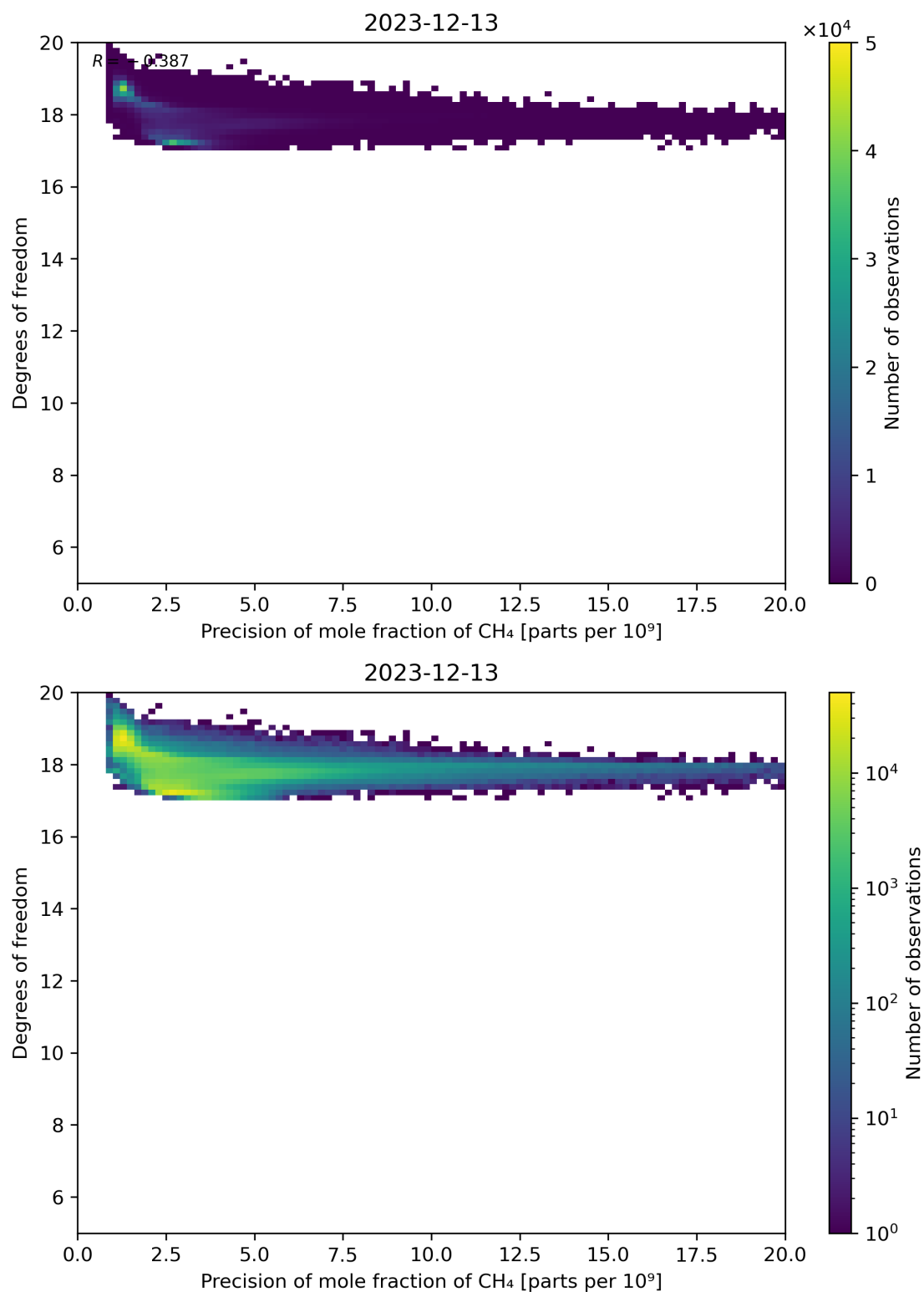
Figure 80: Scatter density plot of “Precision of mole fraction of CH 4 ” against “Degrees of freedom” for 2023-12-12 to 2023-12-14.
