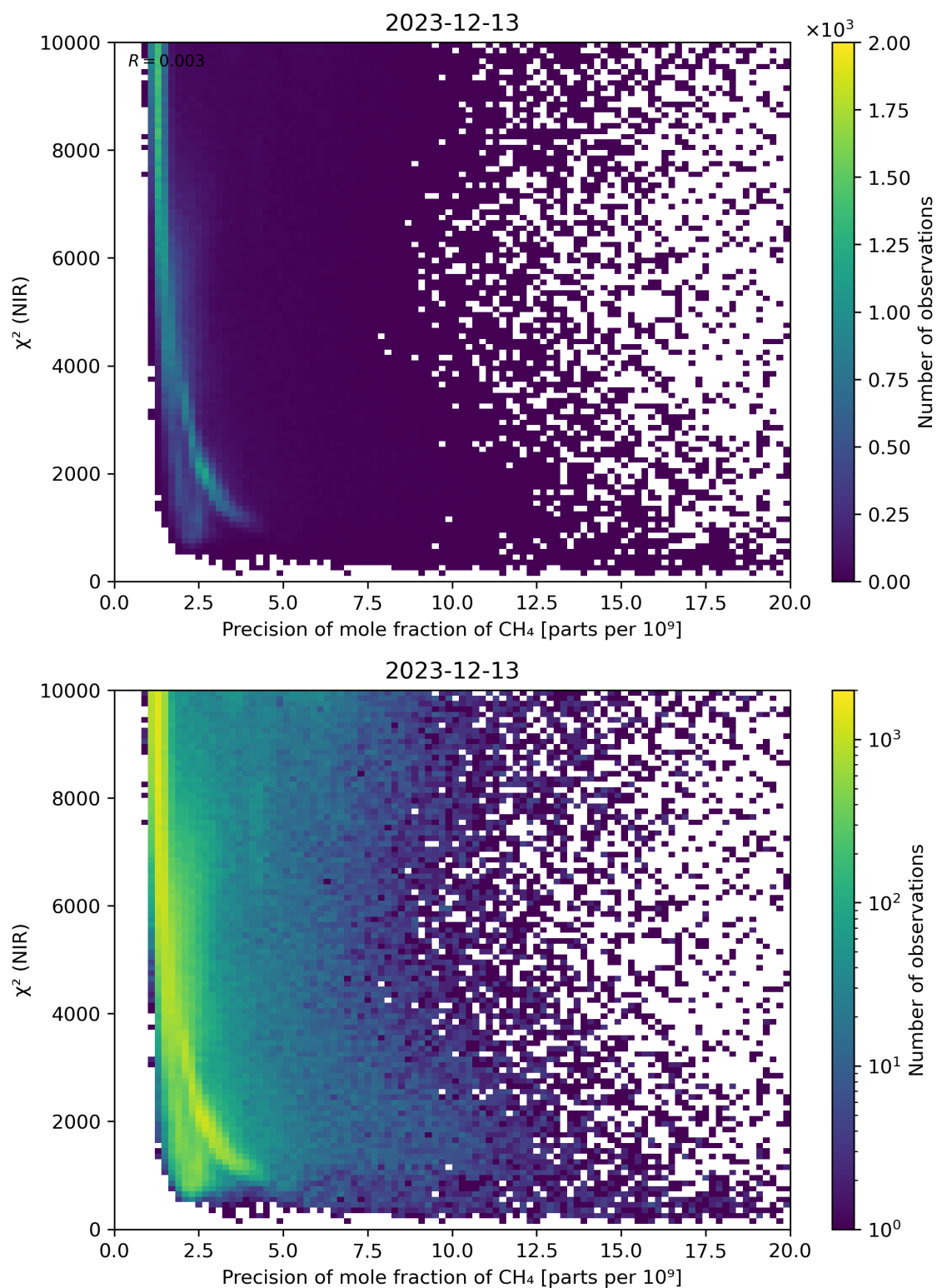
Figure 78: Scatter density plot of “Precision of mole fraction of \text{CH}_4 ” against “ \chi^2 (NIR)” for 2023-12-12 to 2023-12-14.
