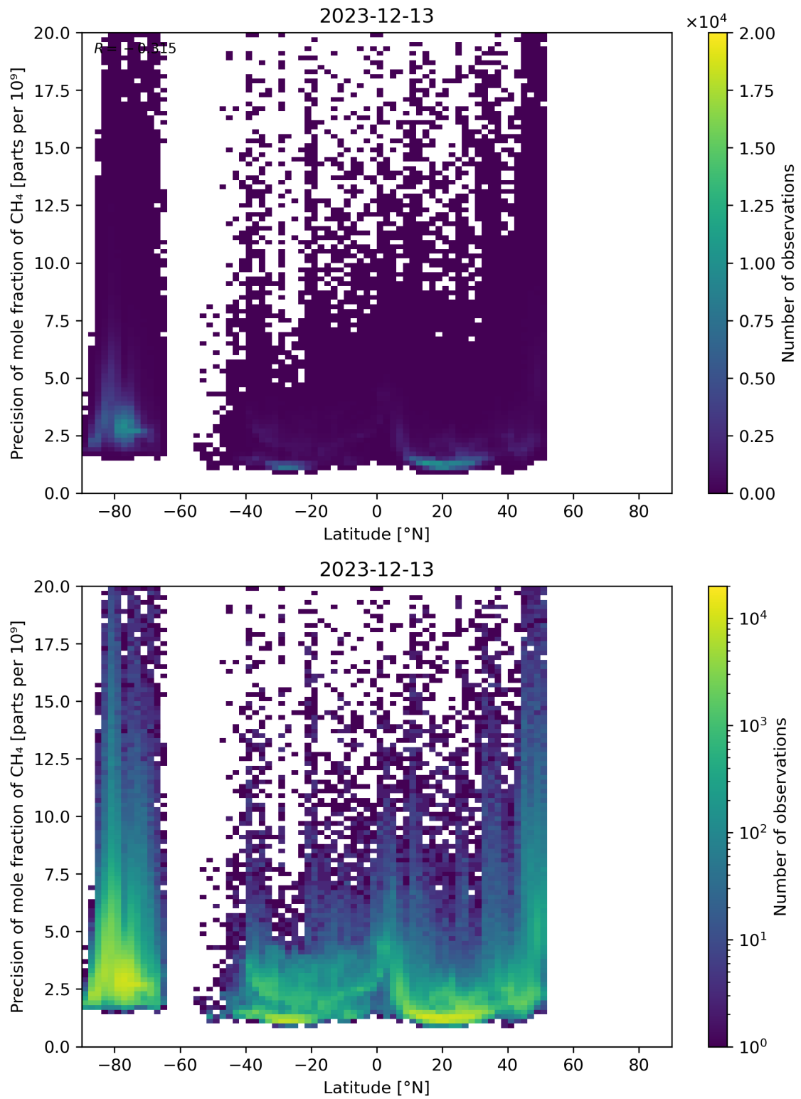
Figure 59: Scatter density plot of “Latitude” against “Precision of mole fraction of CH 4 ” for 2023-12-12 to 2023-12-14.
