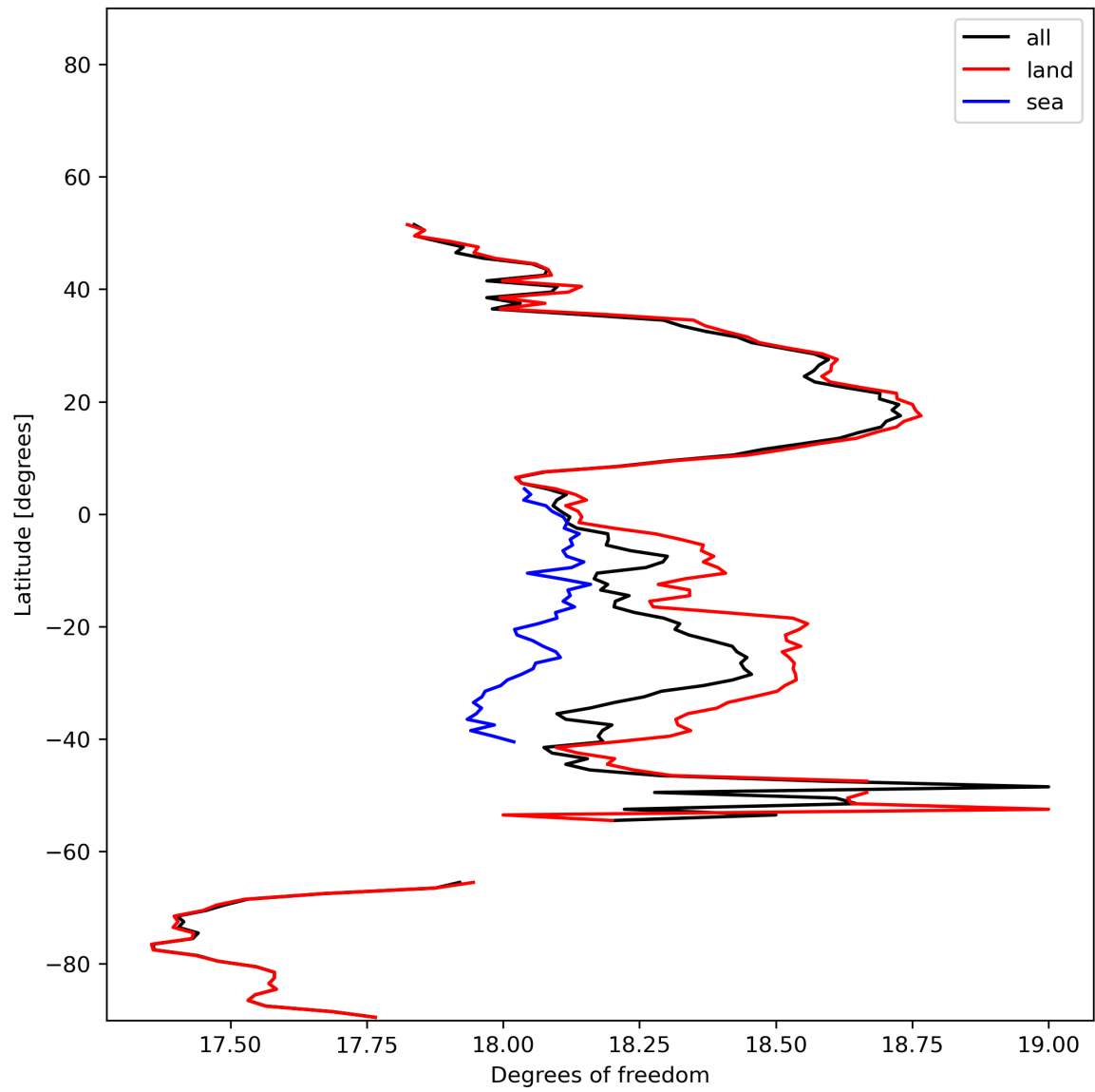
Figure 19: Zonal average of “Degrees of freedom” for 2023-12-12 to 2023-12-14.
