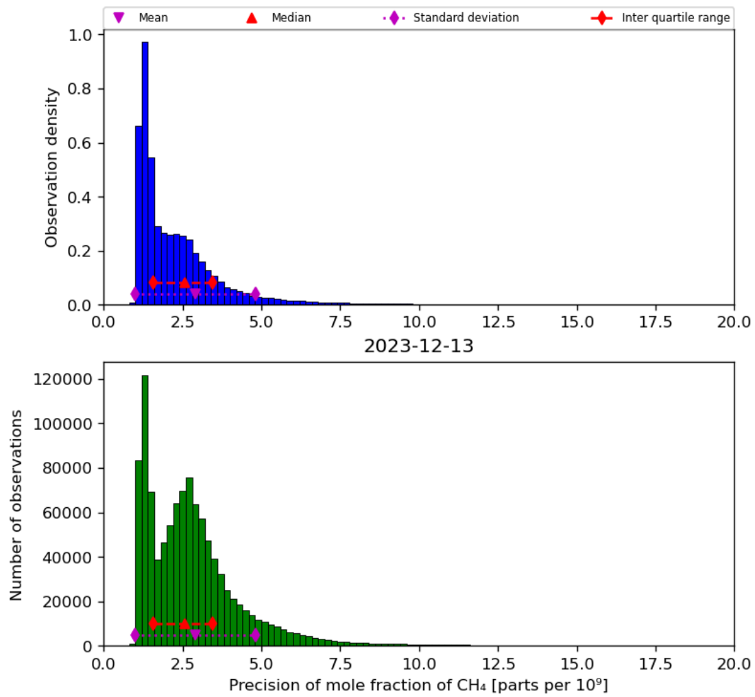
Figure 24: Histogram of “Precision of mole fraction of CH 4 ” for 2023-12-12 to 2023-12-14
