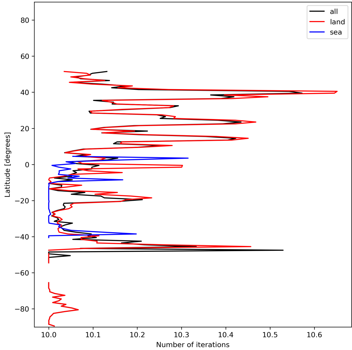
Figure 20: Zonal average of “Number of iterations” for 2023-12-12 to 2023-12-14.
