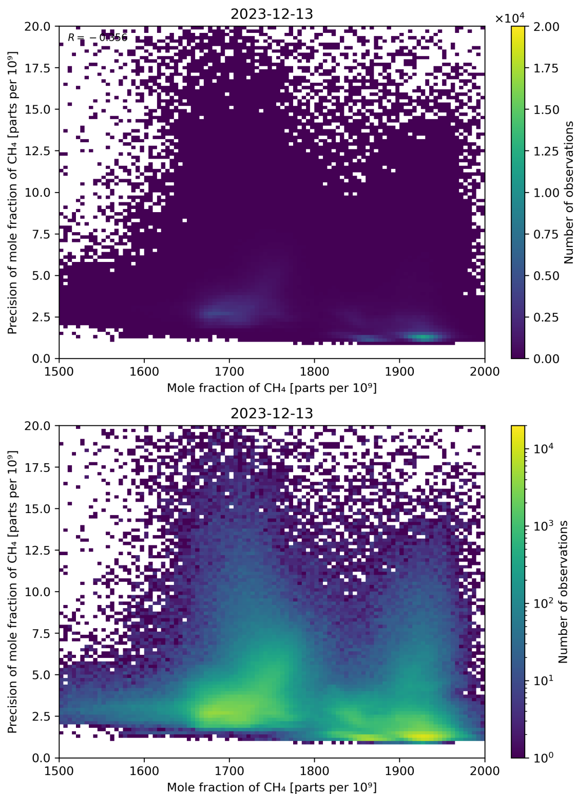
Figure 75: Scatter density plot of “Mole fraction of CH 4 ” against “Precision of mole fraction of CH 4 ” for 2023-12-12 to 2023-12-14.
