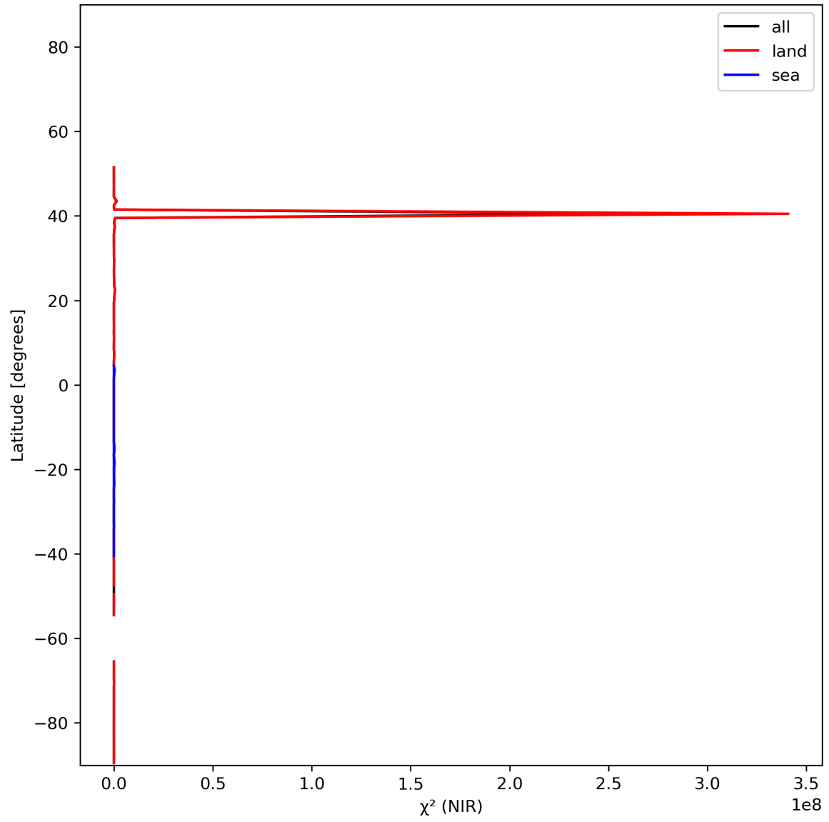
Figure 18: Zonal average of “ \chi^2 (NIR)” for 2023-12-12 to 2023-12-14.
