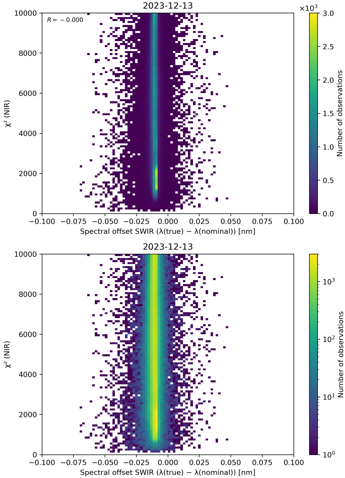
Figure 117: Scatter density plot of “Spectral offset SWIR ( \lambda(\text{true}) - \lambda(\text{nominal}) )” against “ \chi^2 (NIR)” for 2023-12-12 to 2023-12-14.
