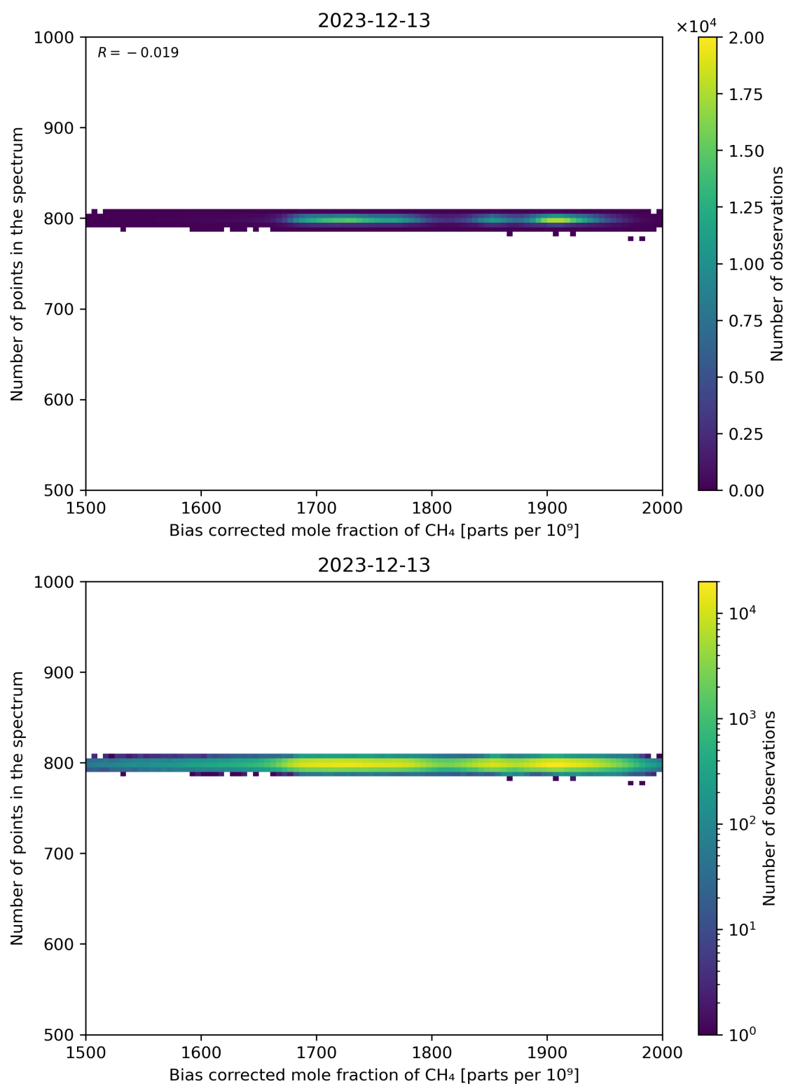
Figure 68: Scatter density plot of “Bias corrected mole fraction of CH 4 ” against “Number of points in the spectrum” for 2023-12-12 to 2023-12-14.
