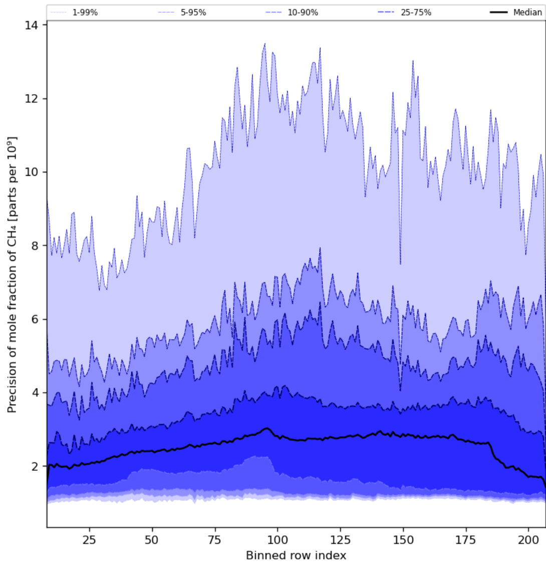
Figure 35: Along track statistics of “Precision of mole fraction of CH 4 ” for 2023-12-12 to 2023-12-14
