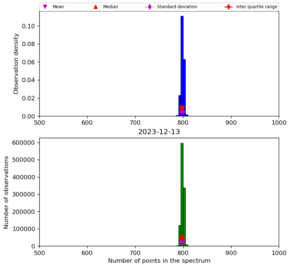
Figure 26: Histogram of “Number of points in the spectrum” for 2023-12-12 to 2023-12-14
