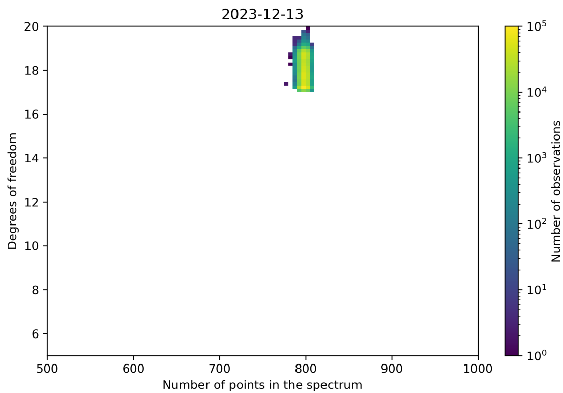
Figure 90: Scatter density plot of “Number of points in the spectrum” against “Degrees of freedom” for 2023-12-12 to 2023-12-14.
