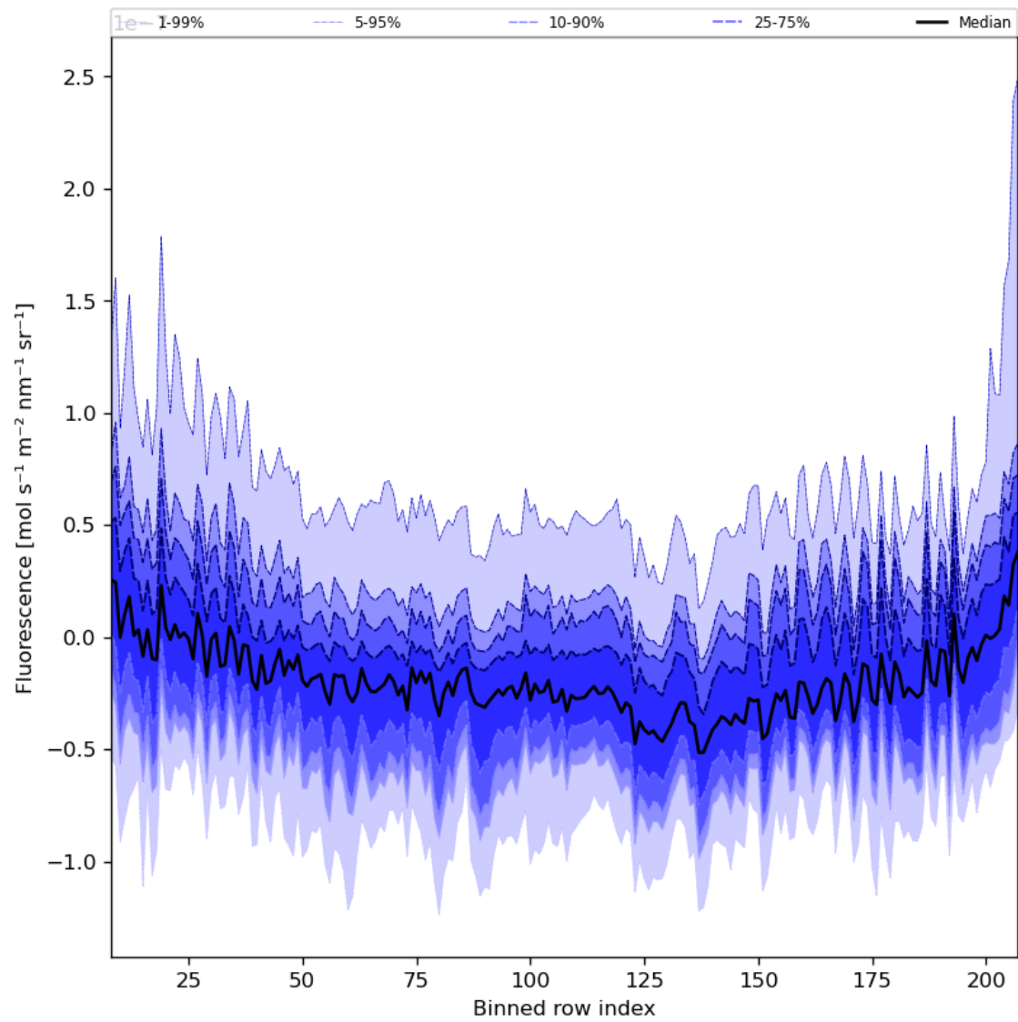
Figure 43: Along track statistics of “Fluorescence” for 2023-12-12 to 2023-12-14
