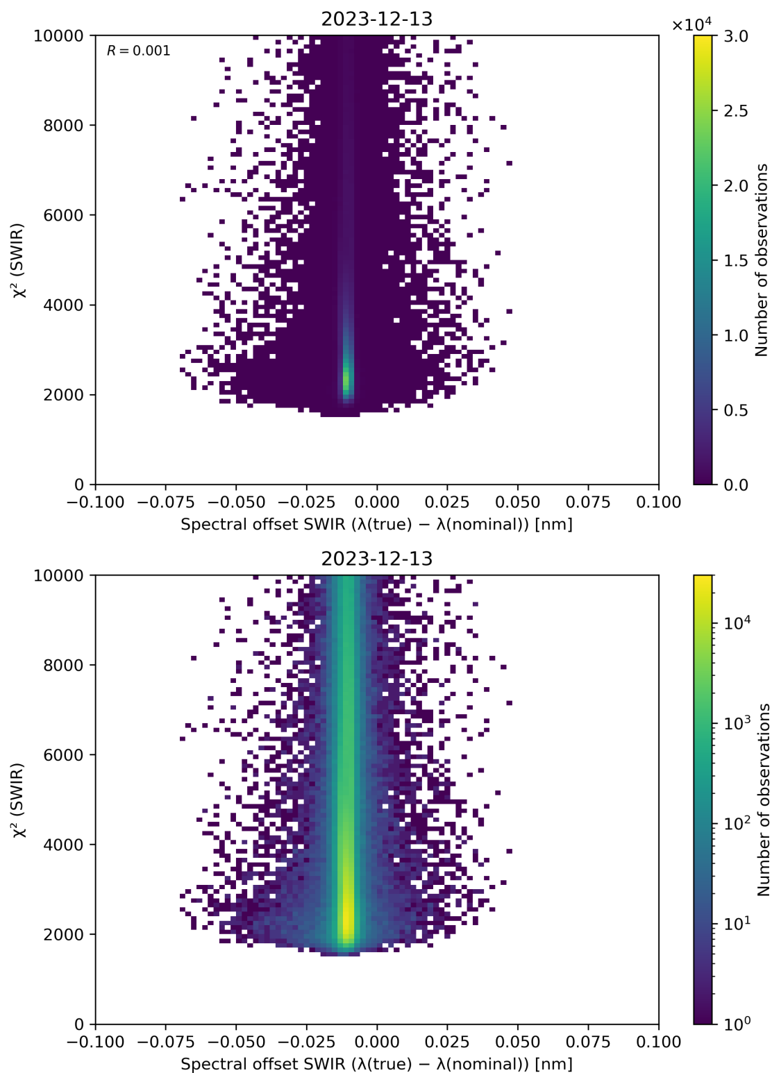
Figure 118: Scatter density plot of “Spectral offset SWIR ( \lambda(\text{true}) - \lambda(\text{nominal}) )” against “ \chi^2 (SWIR)” for 2023-12-12 to 2023-12-14.
