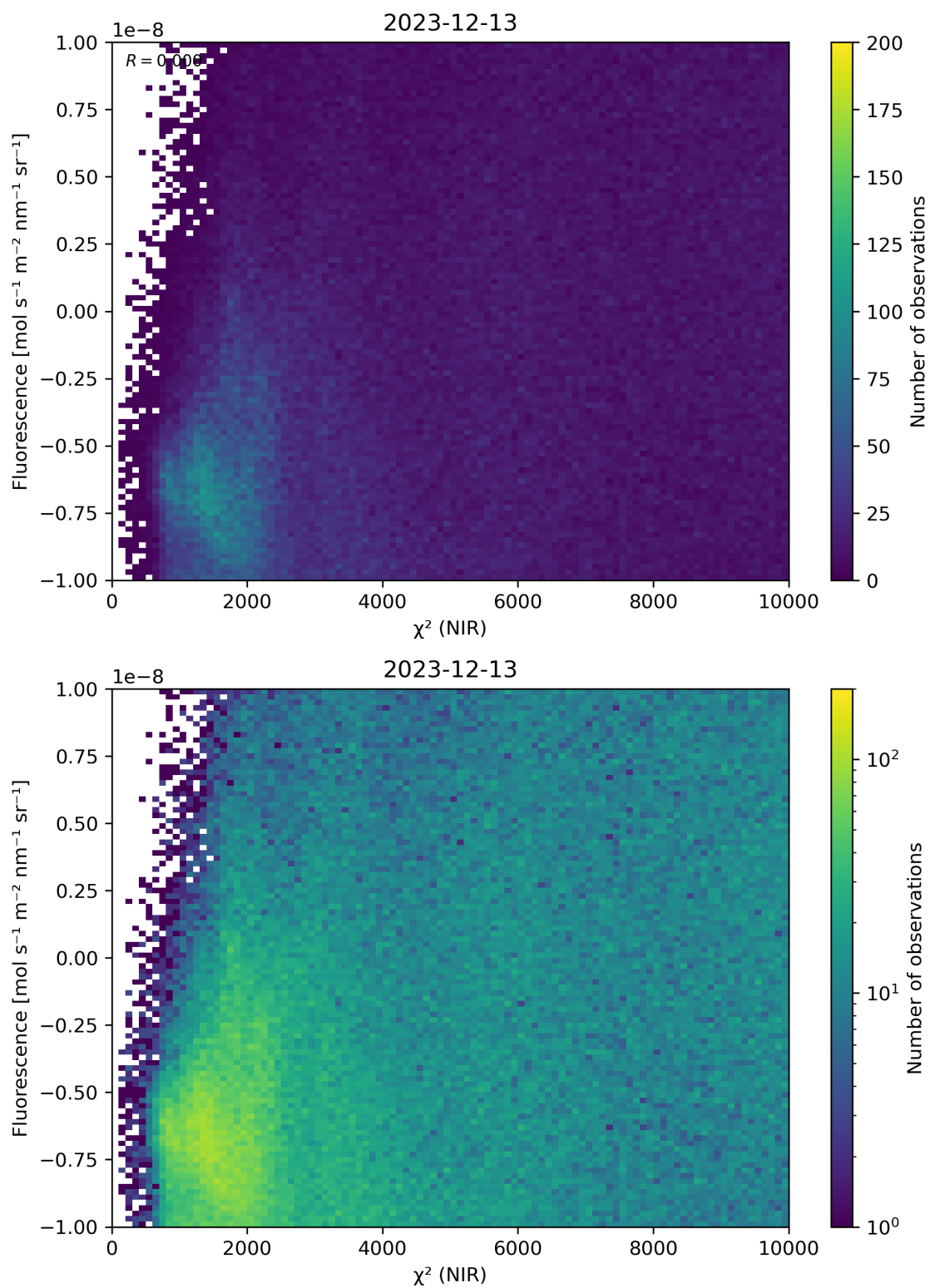
Figure 45: Scatter density plot of “ \chi^2 (NIR)” against “Fluorescence” for 2023-12-12 to 2023-12-14.
