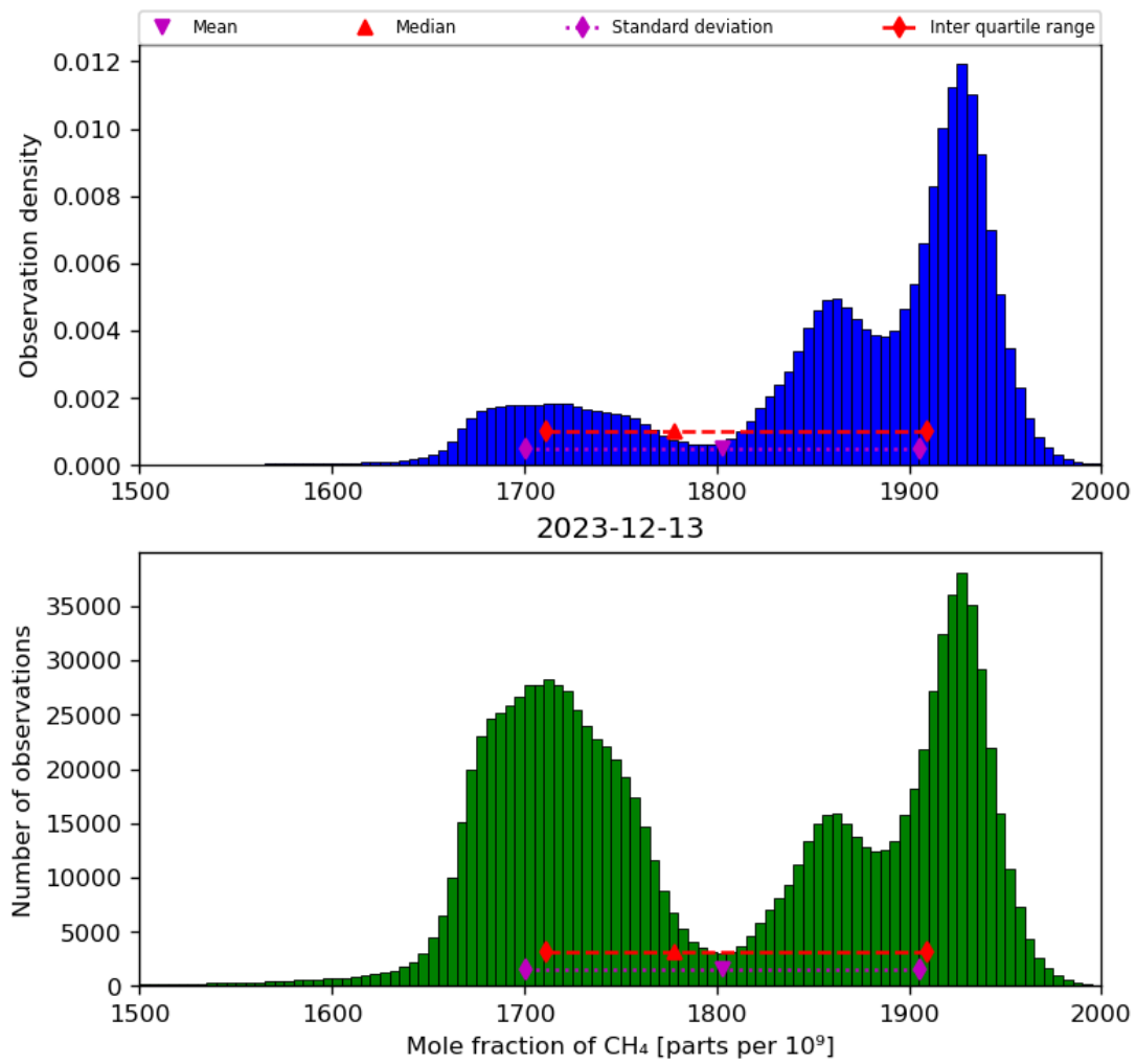
Figure 23: Histogram of “Mole fraction of CH 4 ” for 2023-12-12 to 2023-12-14
