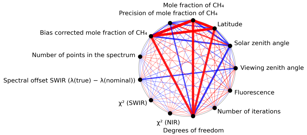
Figure 1: Map of correlation graph for 2023-12-12 to 2023-12-14.
