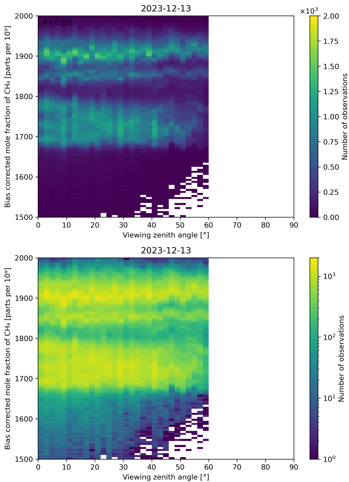
Figure 111: Scatter density plot of “Viewing zenith angle” against “Bias corrected mole fraction of CH 4 ” for 2023-12-12 to 2023-12-14.
