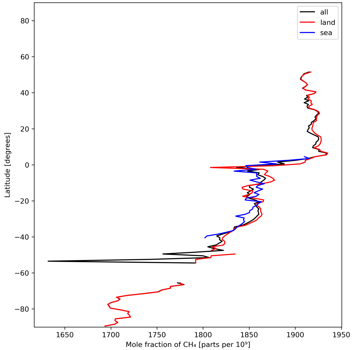
Figure 12: Zonal average of “Mole fraction of CH 4 ” for 2023-12-12 to 2023-12-14.
