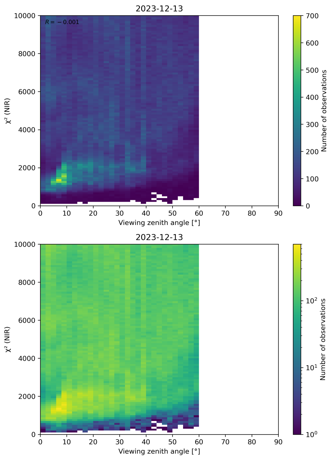
Figure 105: Scatter density plot of “Viewing zenith angle” against “ \chi^2 (NIR)” for 2023-12-12 to 2023-12-14.
