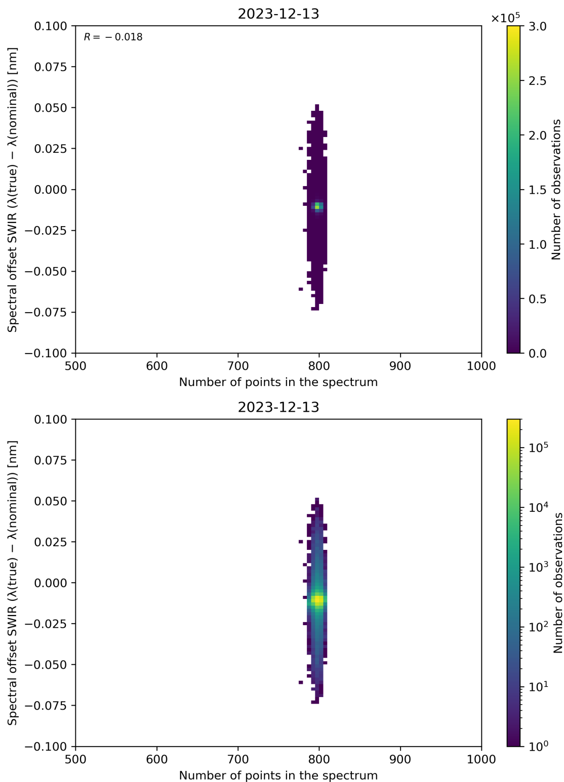
Figure 93: Scatter density plot of “Number of points in the spectrum” against “Spectral offset SWIR ( \lambda(\text{true}) - \lambda(\text{nominal}) )” for 2023-12-12 to 2023-12-14.
