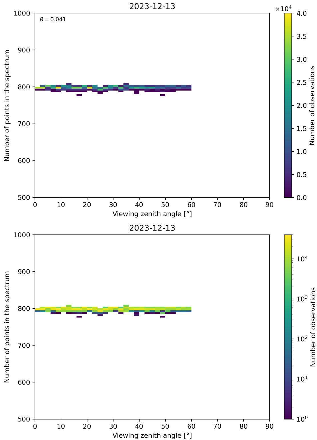
Figure 114: Scatter density plot of “Viewing zenith angle” against “Number of points in the spectrum” for 2023-12-12 to 2023-12-14.
