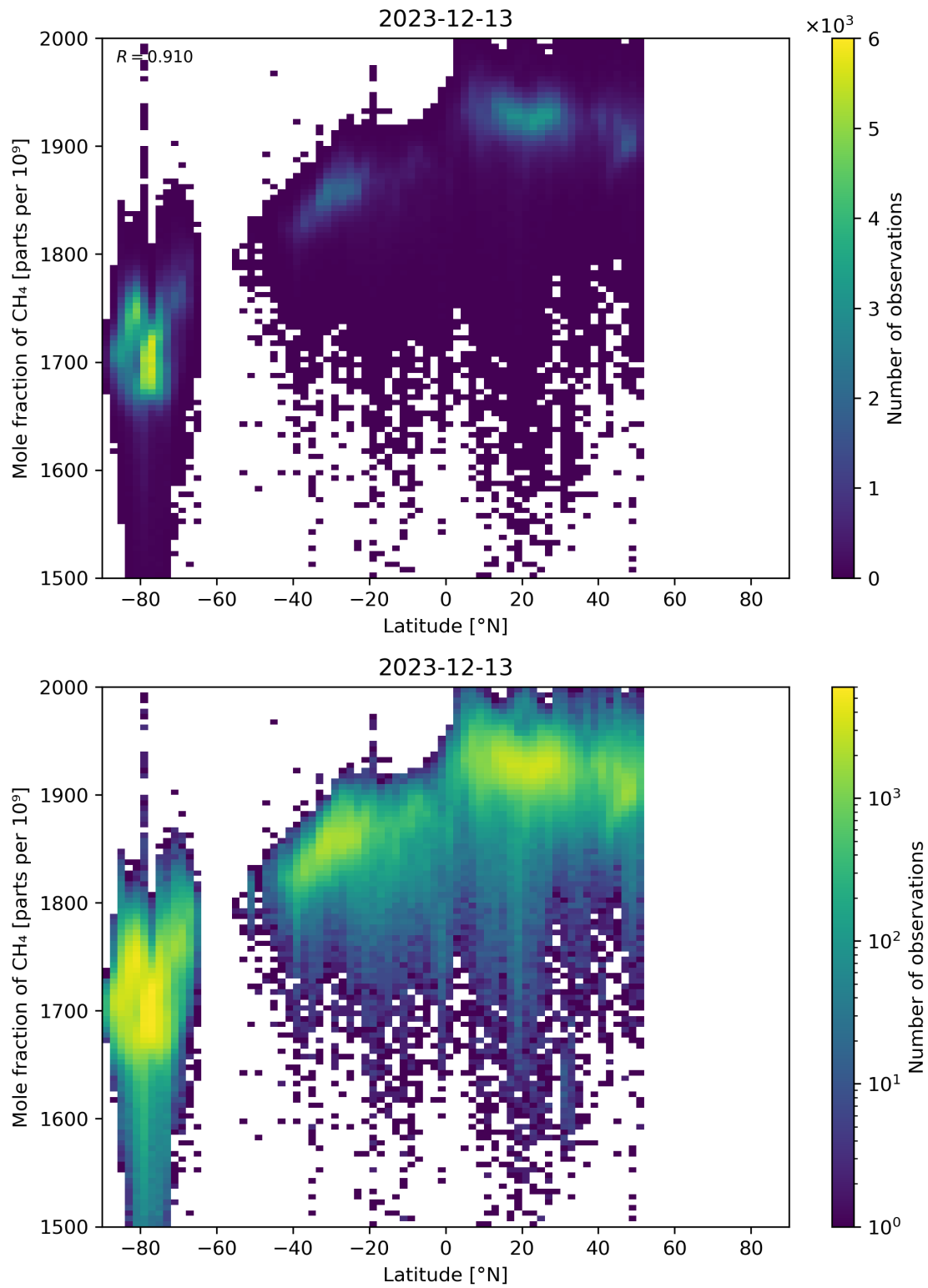
Figure 57: Scatter density plot of “Latitude” against “Mole fraction of CH 4 ” for 2023-12-12 to 2023-12-14.
