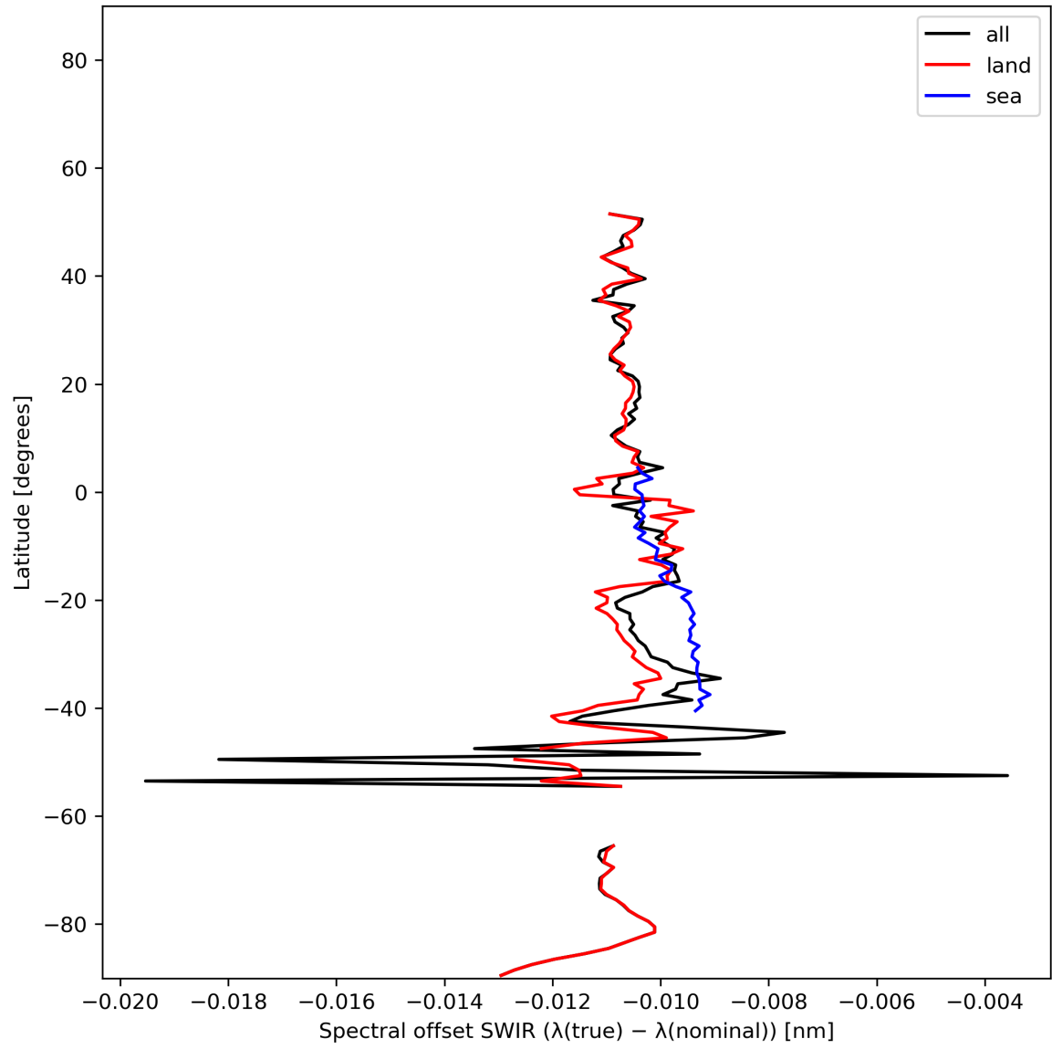
Figure 16: Zonal average of “Spectral offset SWIR ( \lambda(\text{true}) - \lambda(\text{nominal}) )” for 2023-12-12 to 2023-12-14.
