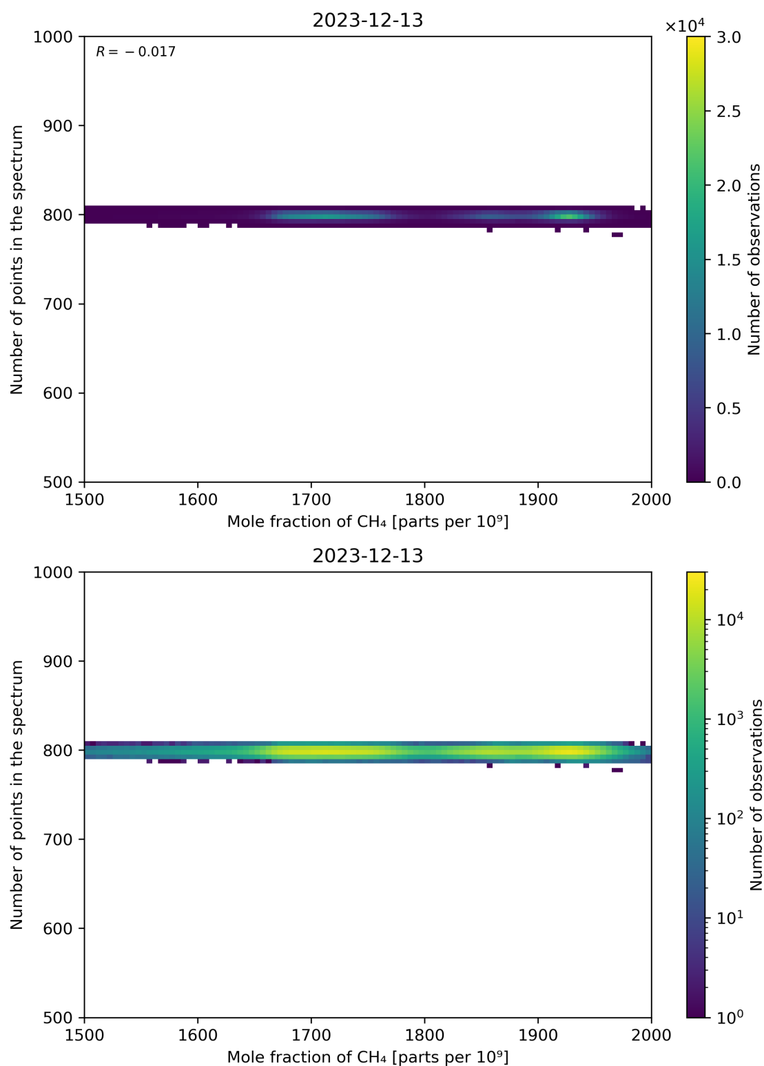
Figure 77: Scatter density plot of “Mole fraction of CH 4 ” against “Number of points in the spectrum” for 2023-12-12 to 2023-12-14.
