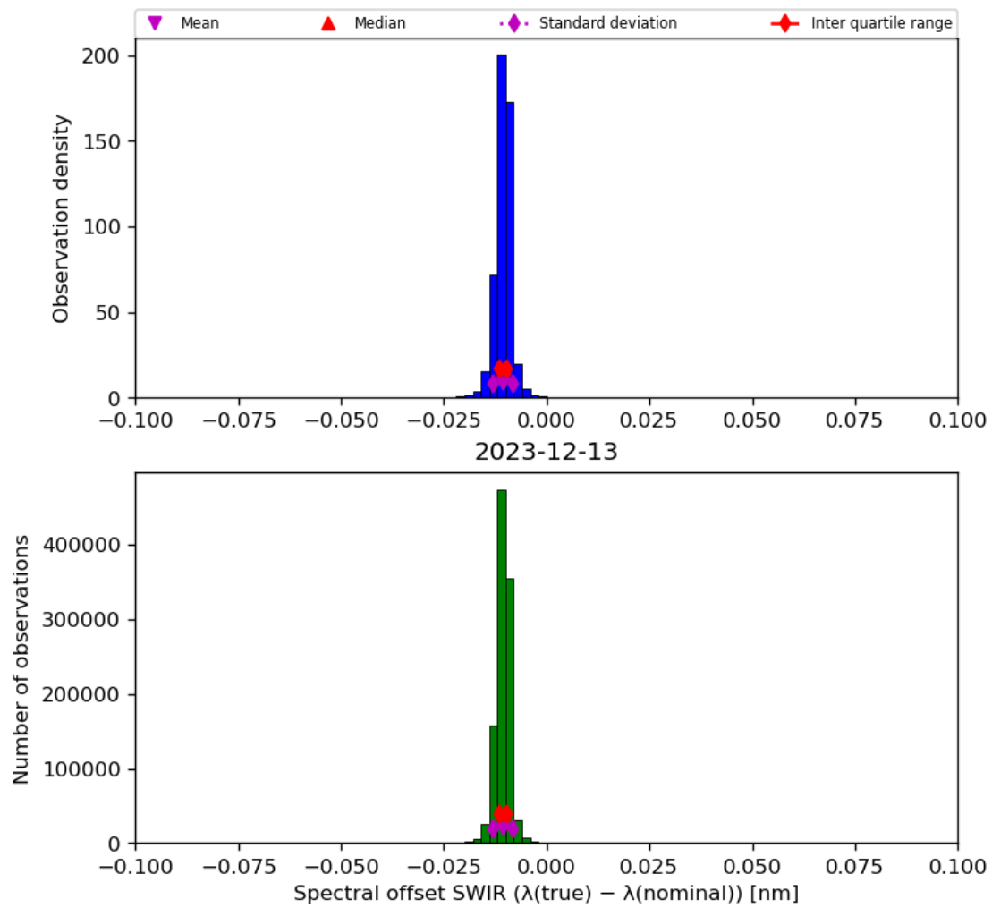
Figure 27: Histogram of “Spectral offset SWIR ( \lambda(\text{true}) - \lambda(\text{nominal}) )” for 2023-12-12 to 2023-12-14
