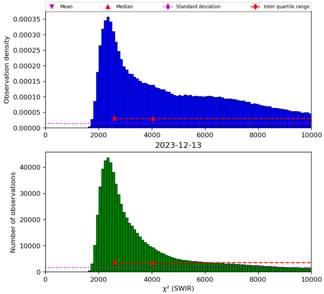
Figure 28: Histogram of “ \chi^2 (SWIR)” for 2023-12-12 to 2023-12-14
