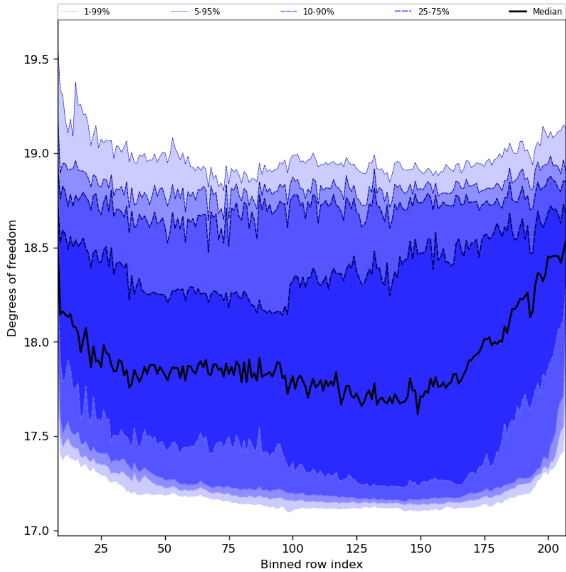
Figure 41: Along track statistics of “Degrees of freedom” for 2023-12-12 to 2023-12-14
