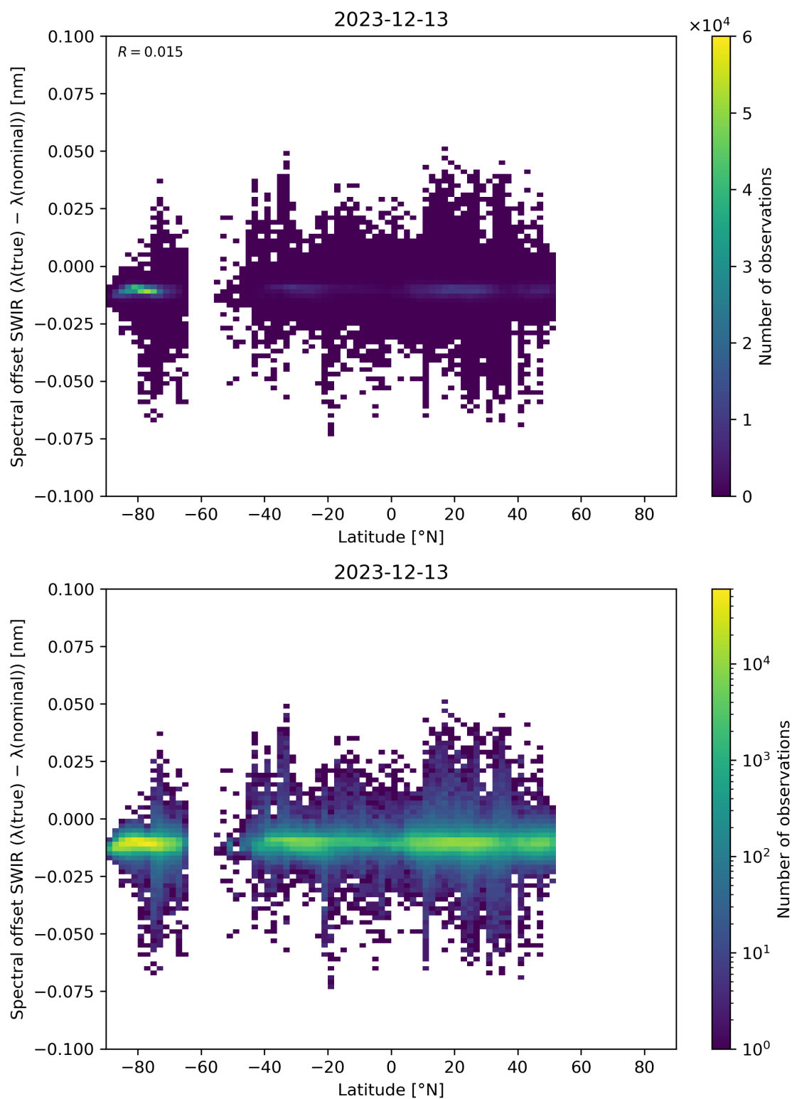
Figure 62: Scatter density plot of “Latitude” against “Spectral offset SWIR ( \lambda(\text{true}) - \lambda(\text{nominal}) )” for 2023-12-12 to 2023-12-14.
