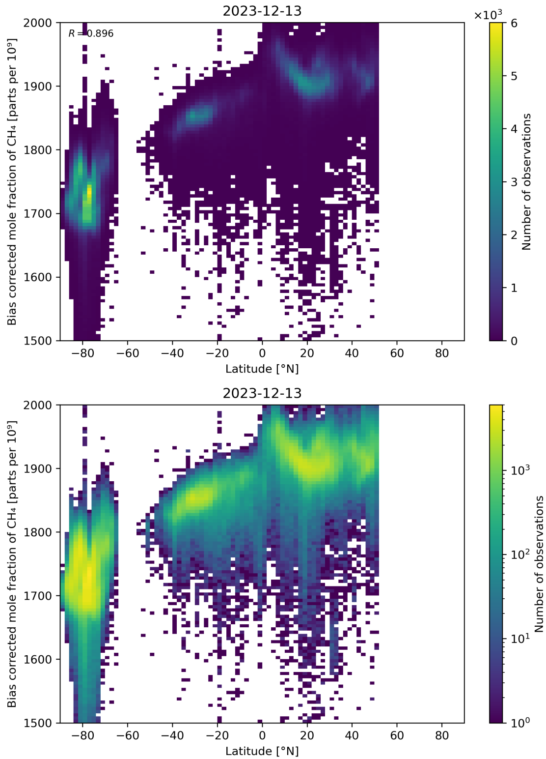
Figure 58: Scatter density plot of “Latitude” against “Bias corrected mole fraction of CH 4 ” for 2023-12-12 to 2023-12-14.
