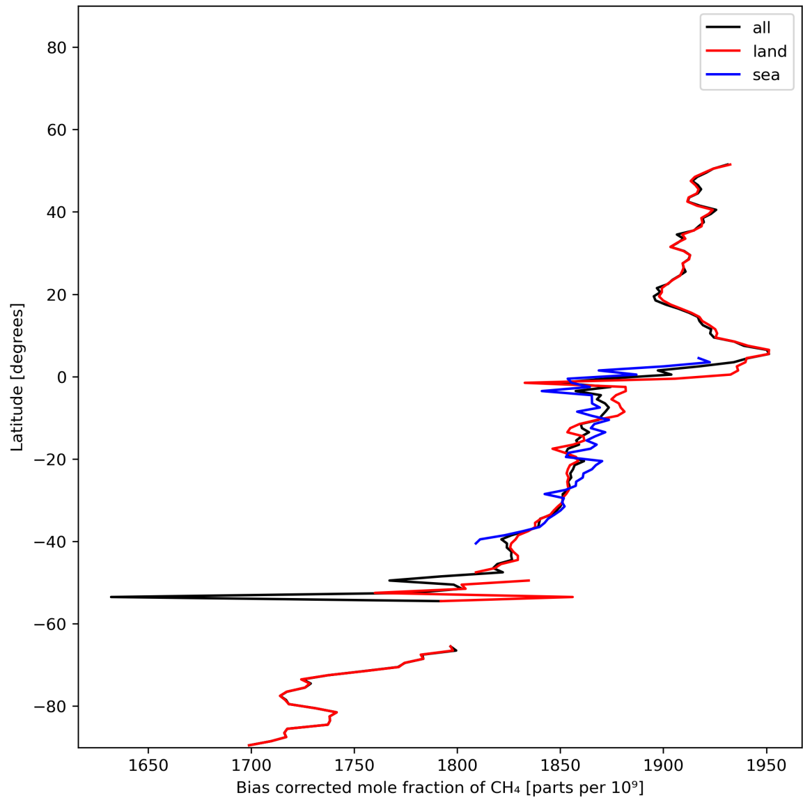
Figure 14: Zonal average of “Bias corrected mole fraction of \text{CH}_4 ” for 2023-12-12 to 2023-12-14.
