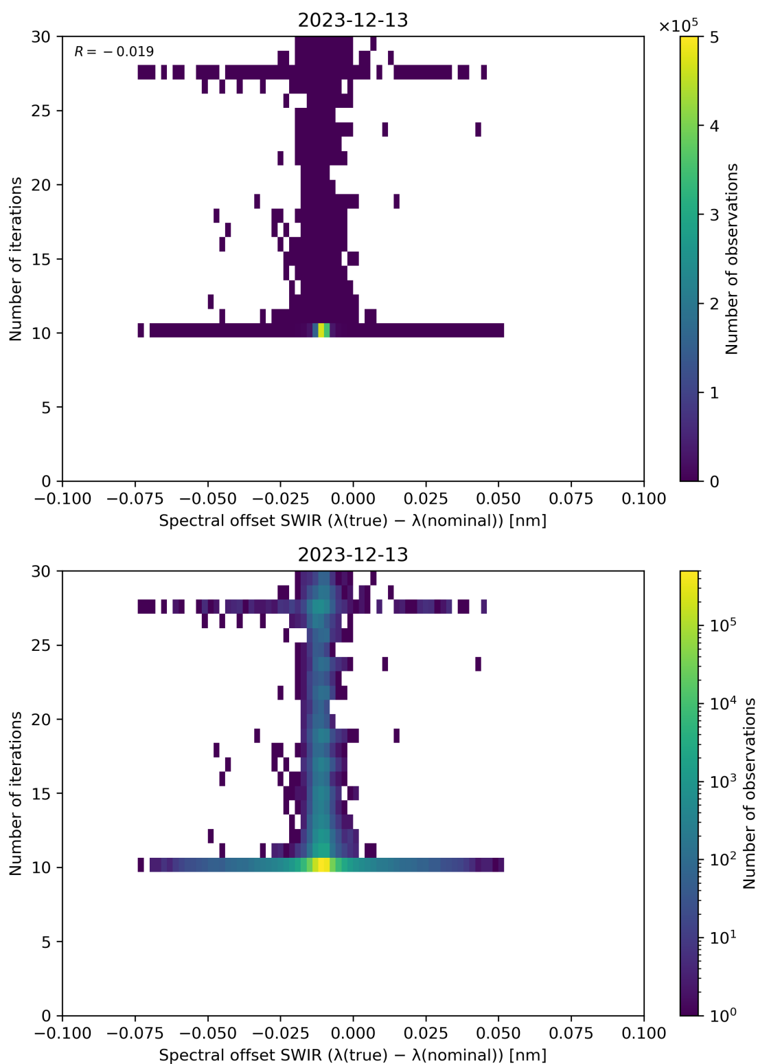
Figure 121: Scatter density plot of “Spectral offset SWIR ( \lambda(\text{true}) - \lambda(\text{nominal}) )” against “Number of iterations” for 2023-12-12 to 2023-12-14.
