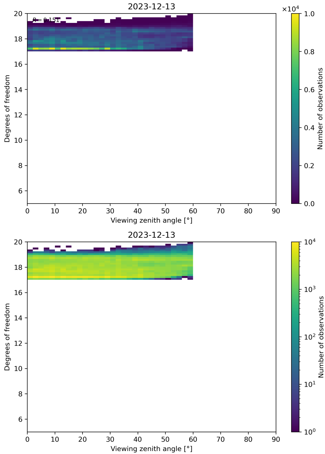
Figure 107: Scatter density plot of “Viewing zenith angle” against “Degrees of freedom” for 2023-12-12 to 2023-12-14.
