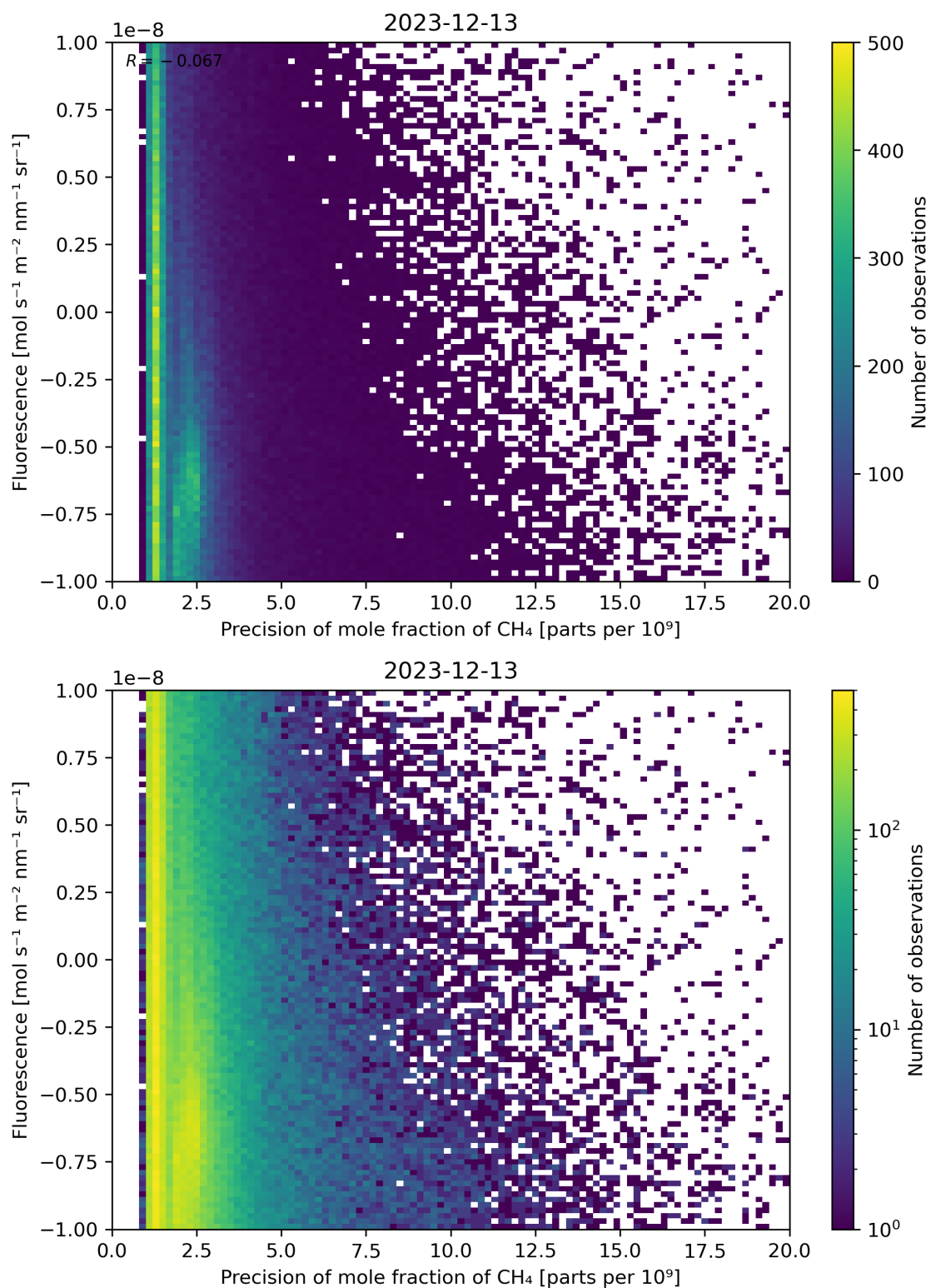
Figure 81: Scatter density plot of “Precision of mole fraction of \text{CH}_4 ” against “Fluorescence” for 2023-12-12 to 2023-12-14.
