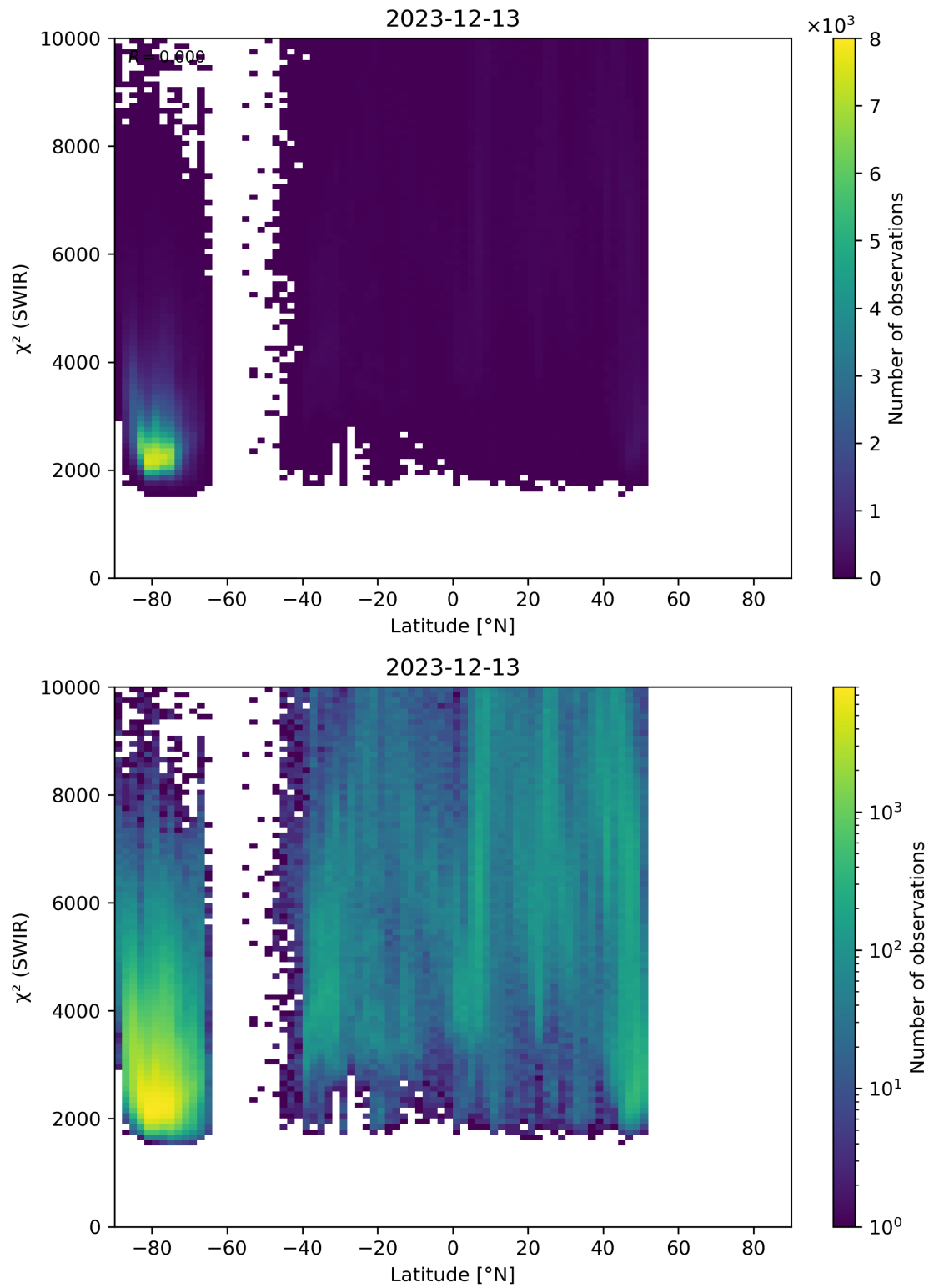
Figure 54: Scatter density plot of “Latitude” against “ \chi^2 (SWIR)” for 2023-12-12 to 2023-12-14.
