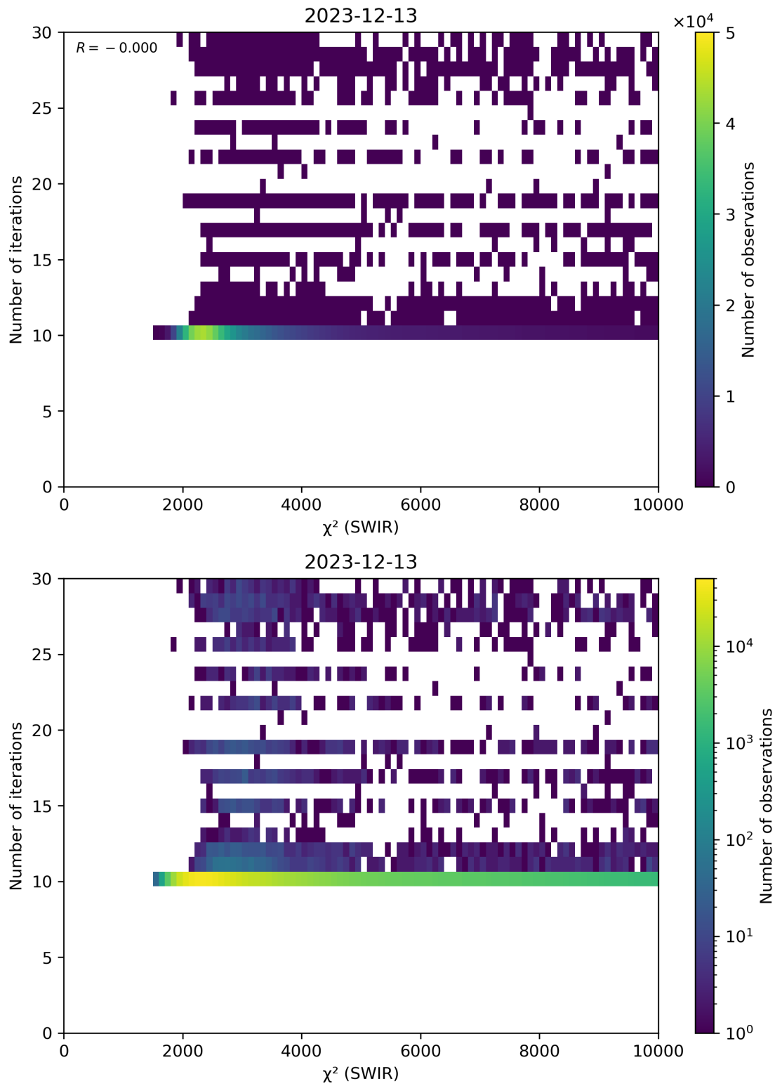
Figure 50: Scatter density plot of “ \chi^2 (SWIR)” against “Number of iterations” for 2023-12-12 to 2023-12-14.
