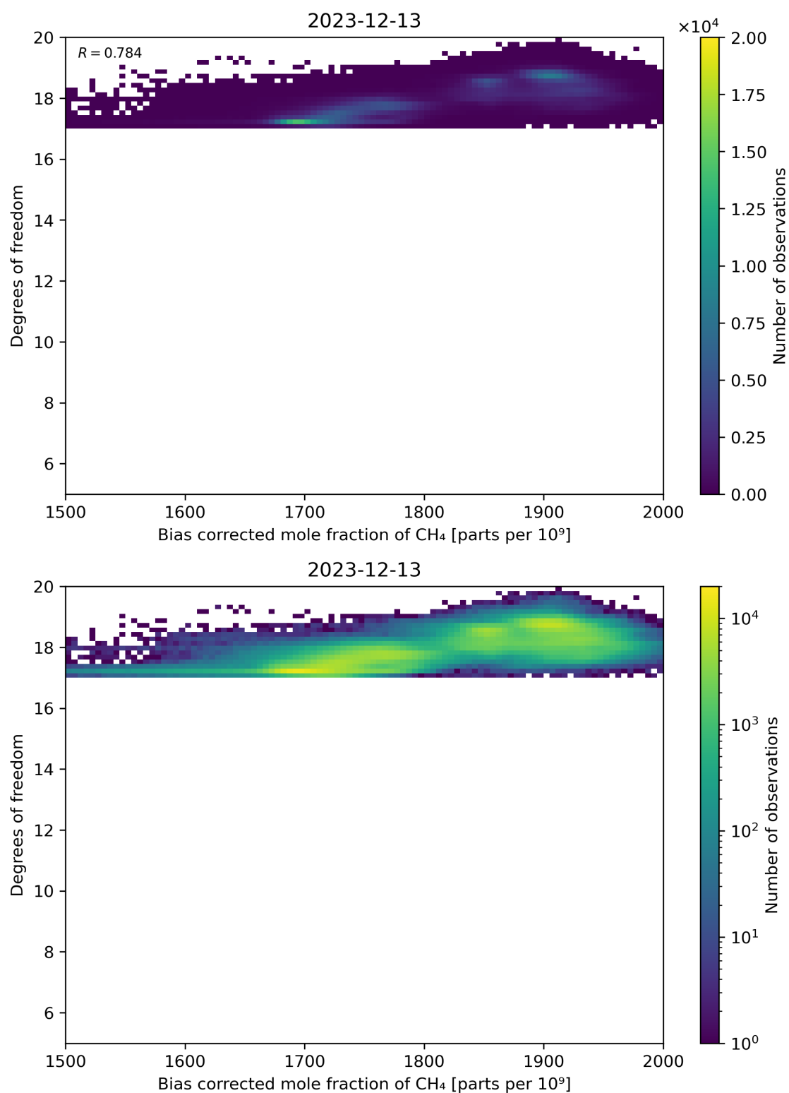
Figure 65: Scatter density plot of “Bias corrected mole fraction of CH 4 ” against “Degrees of freedom” for 2023-12-12 to 2023-12-14.
