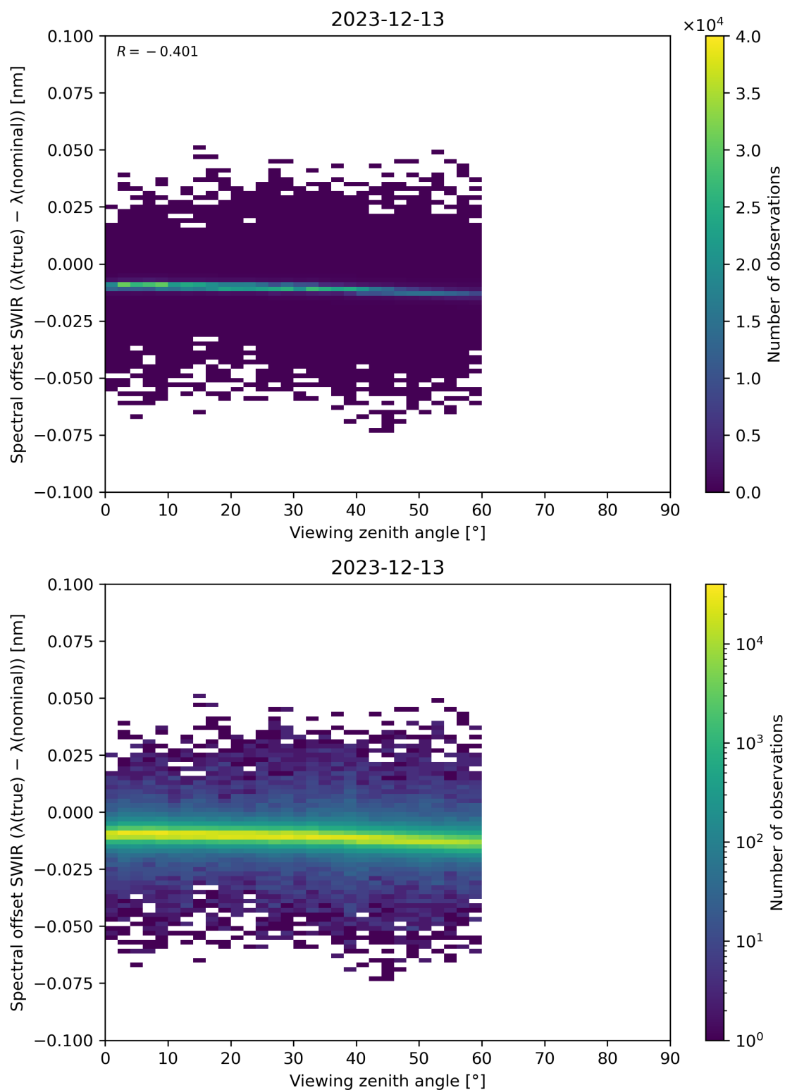
Figure 116: Scatter density plot of “Viewing zenith angle” against “Spectral offset SWIR ( \lambda(\text{true}) - \lambda(\text{nominal}) )” for 2023-12-12 to 2023-12-14.
