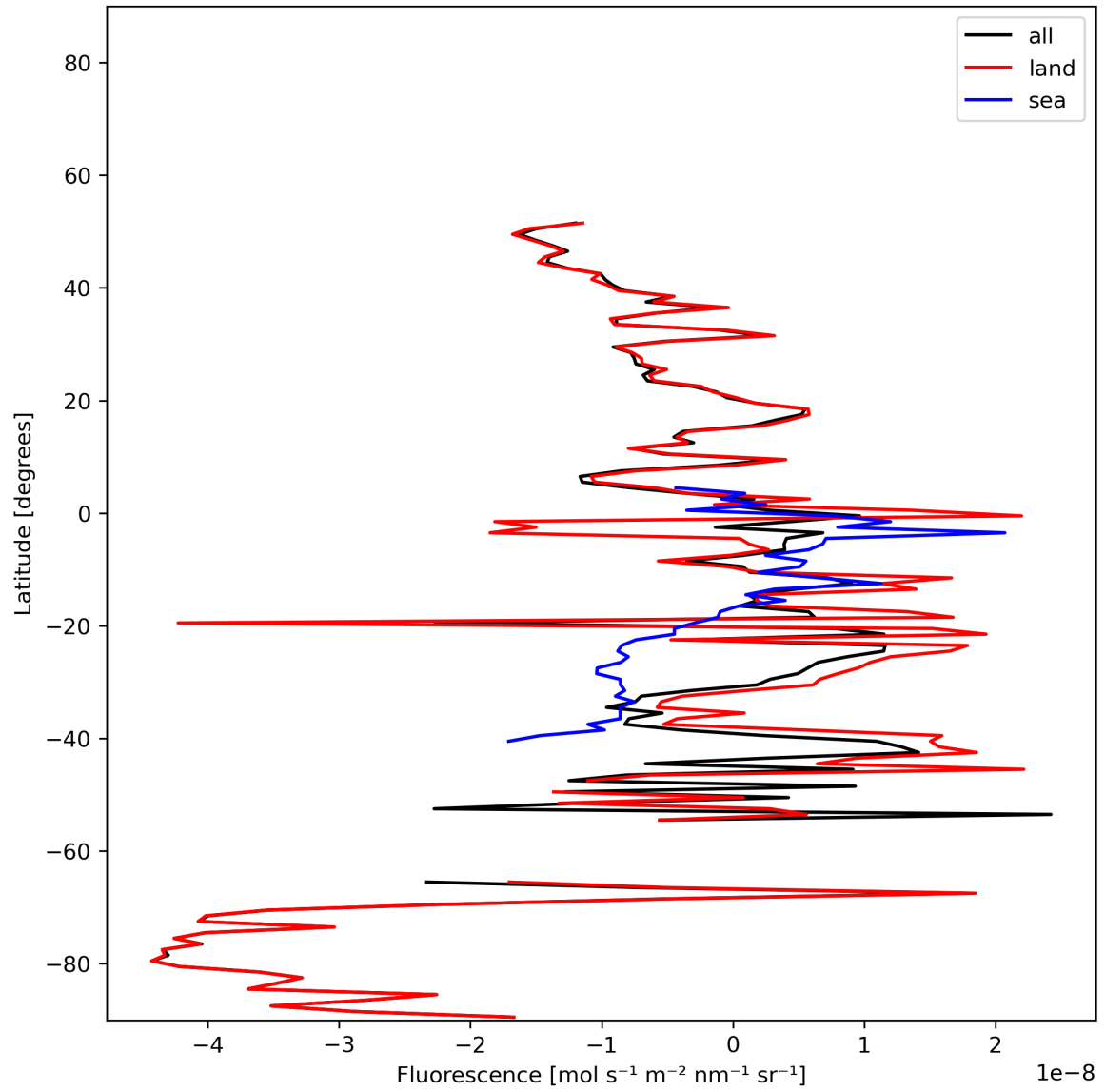
Figure 21: Zonal average of “Fluorescence” for 2023-12-12 to 2023-12-14.
