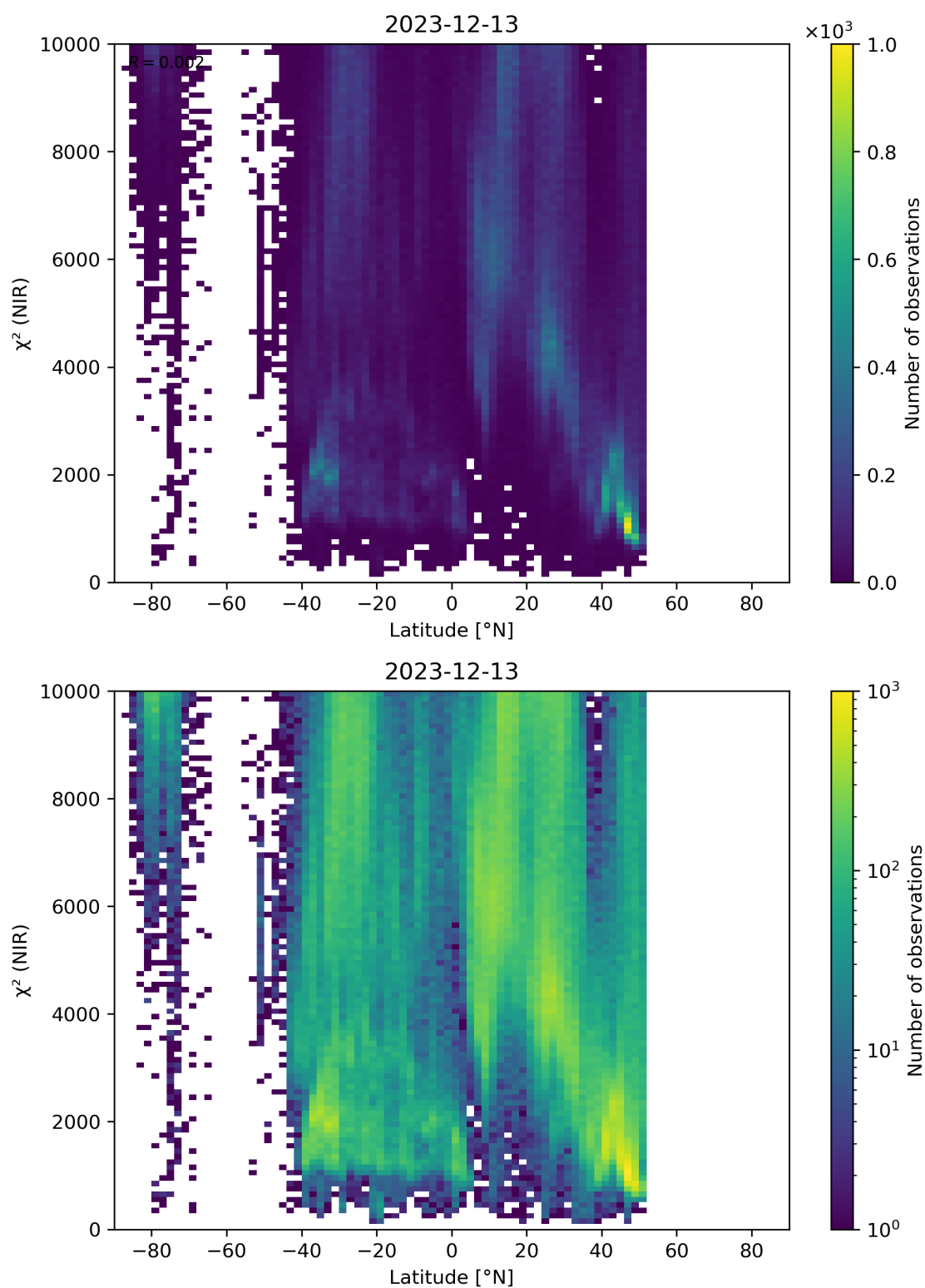
Figure 53: Scatter density plot of “Latitude” against “ \chi^2 (NIR)” for 2023-12-12 to 2023-12-14.
