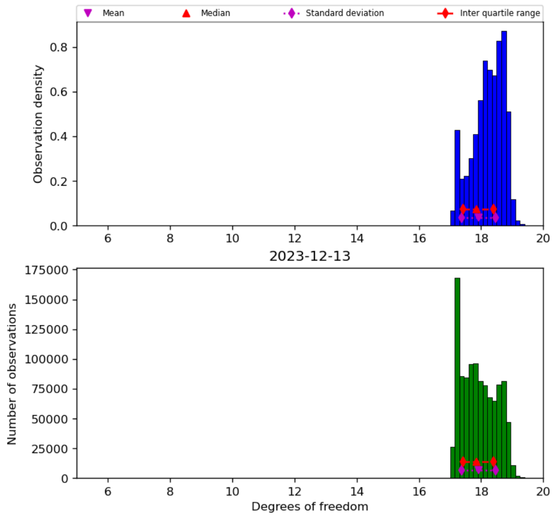
Figure 30: Histogram of "Degrees of freedom" for 2023-12-12 to 2023-12-14
