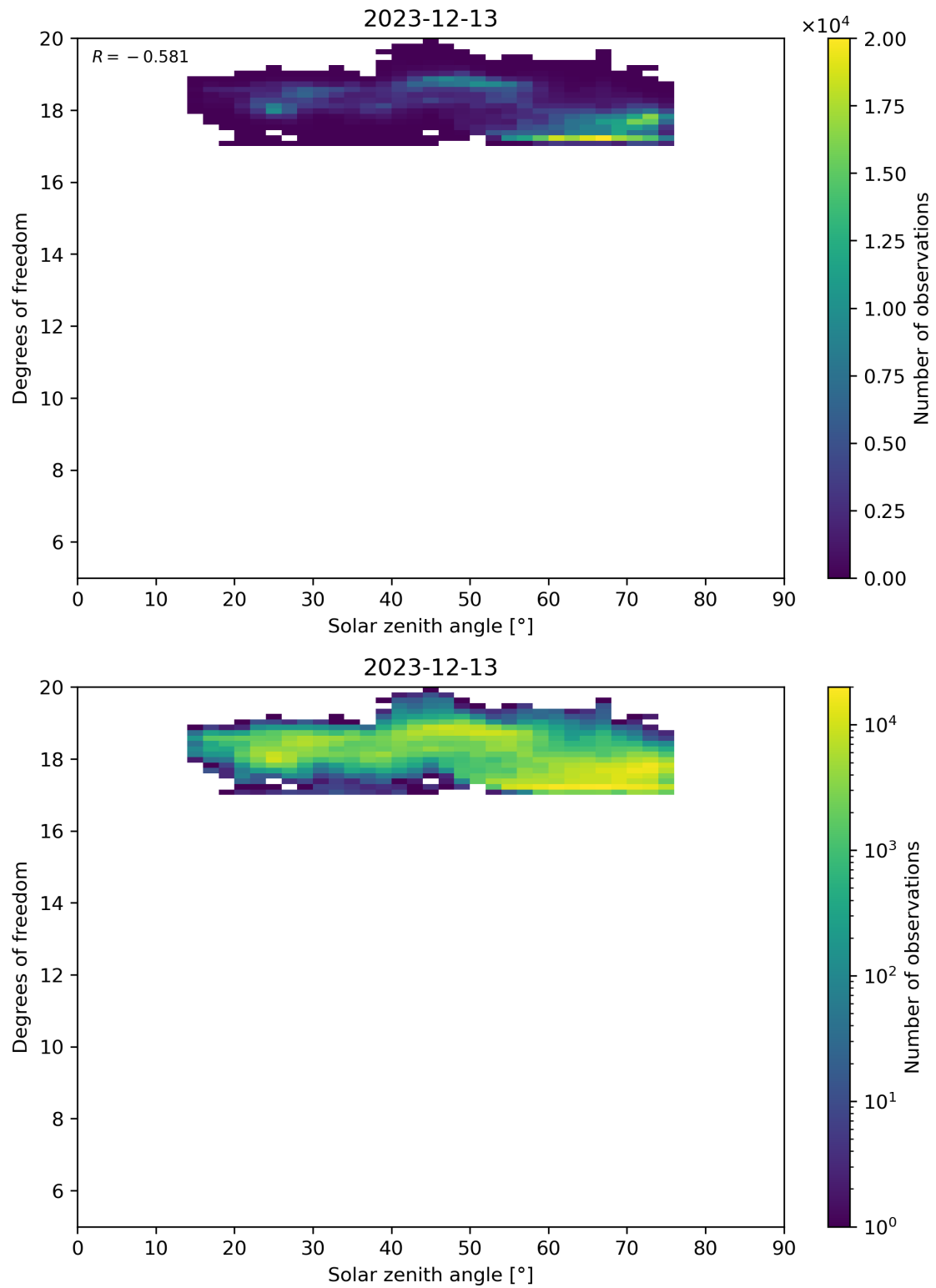
Figure 96: Scatter density plot of “Solar zenith angle” against “Degrees of freedom” for 2023-12-12 to 2023-12-14.
