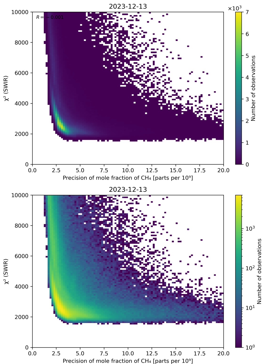
Figure 79: Scatter density plot of “Precision of mole fraction of CH 4 ” against “ \chi^2 (SWIR)” for 2023-12-12 to 2023-12-14.
