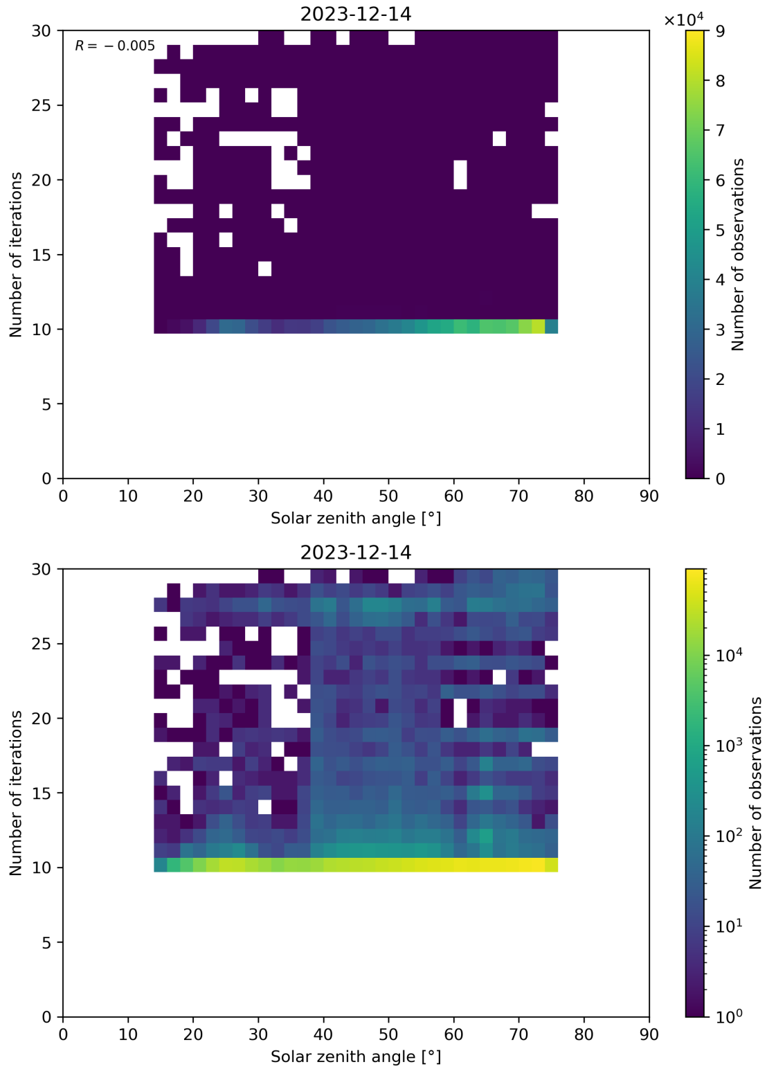
Figure 102: Scatter density plot of “Solar zenith angle” against “Number of iterations” for 2023-12-14 to 2023-12-15.
