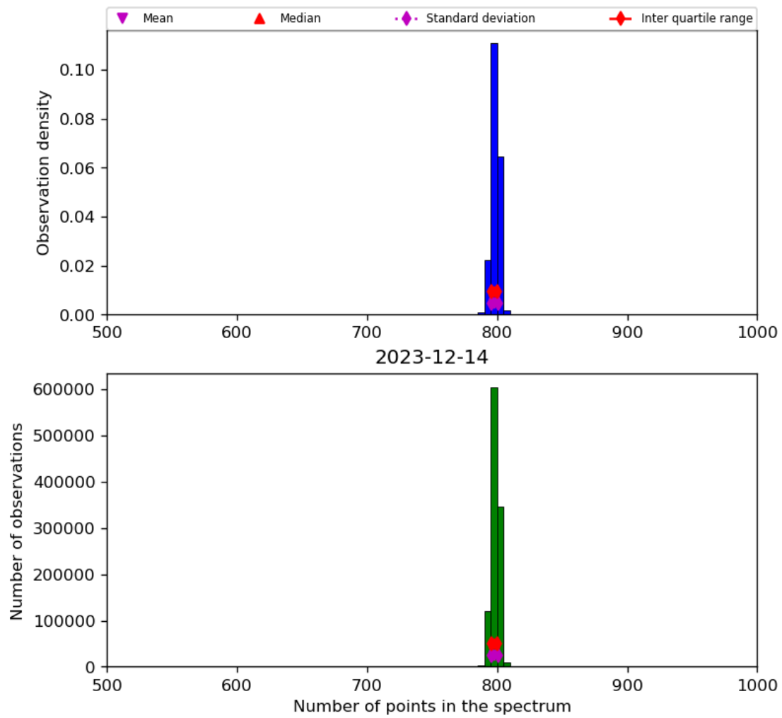
Figure 26: Histogram of “Number of points in the spectrum” for 2023-12-14 to 2023-12-15
