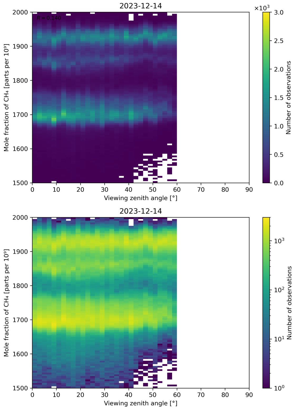
Figure 110: Scatter density plot of “Viewing zenith angle” against “Mole fraction of CH 4 ” for 2023-12-14 to 2023-12-15.
