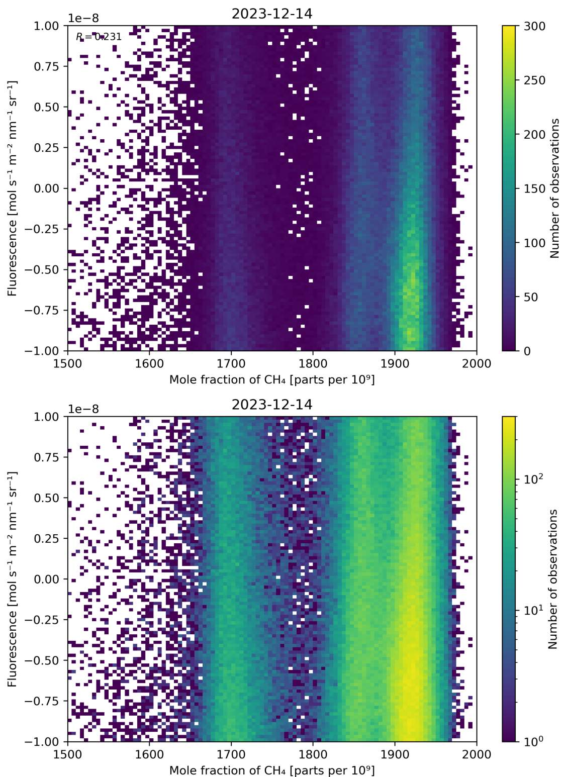
Figure 73: Scatter density plot of “Mole fraction of \text{CH}_4 ” against “Fluorescence” for 2023-12-14 to 2023-12-15.
