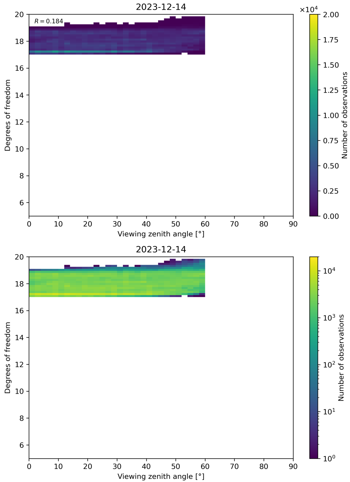
Figure 107: Scatter density plot of “Viewing zenith angle” against “Degrees of freedom” for 2023-12-14 to 2023-12-15.
