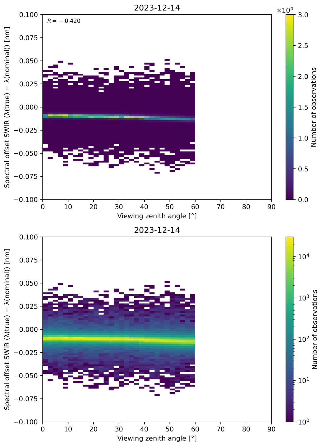
Figure 116: Scatter density plot of “Viewing zenith angle” against “Spectral offset SWIR ( \lambda(\text{true}) - \lambda(\text{nominal}) )” for 2023-12-14 to 2023-12-15.
