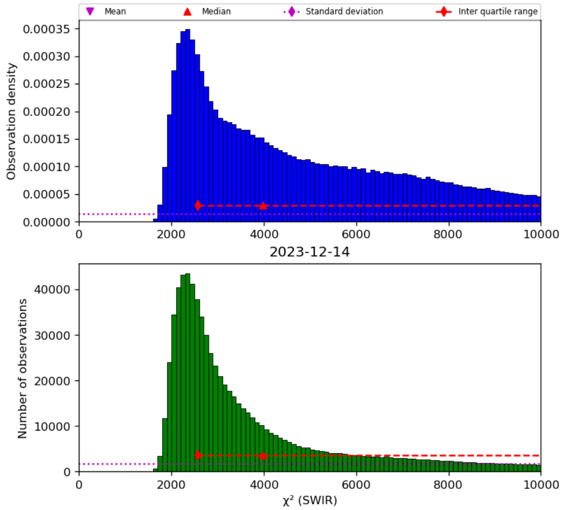
Figure 28: Histogram of “ \chi^2 (SWIR)” for 2023-12-14 to 2023-12-15
