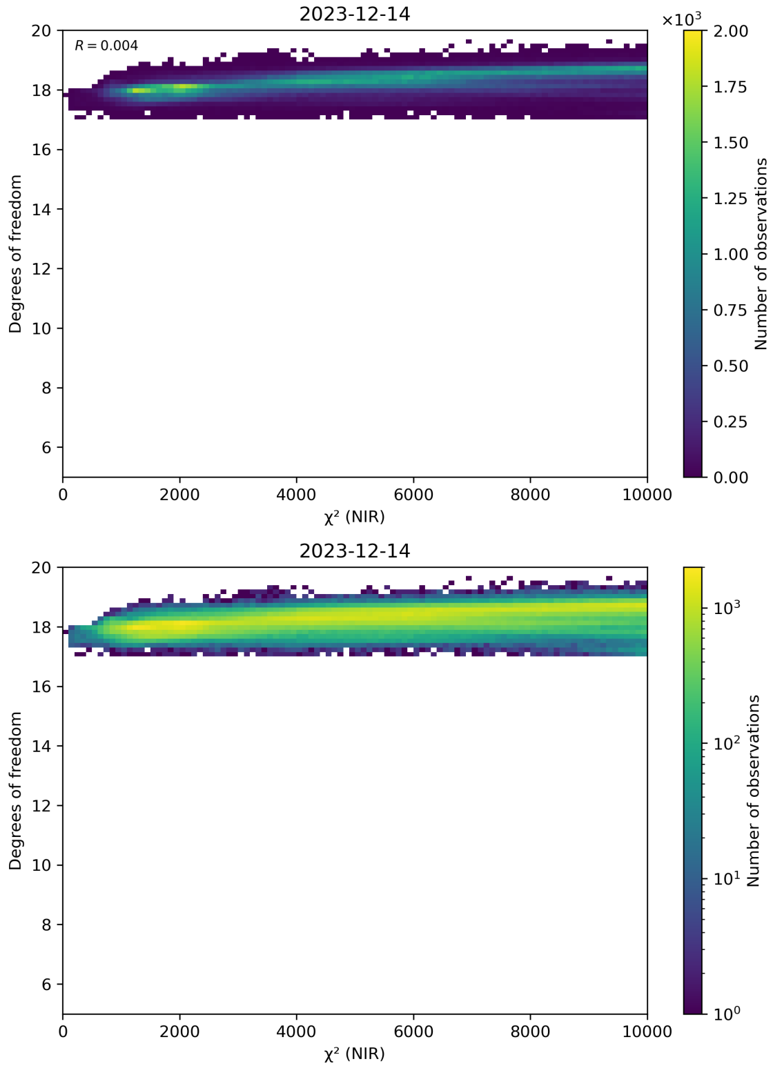
Figure 44: Scatter density plot of “ \chi^2 (NIR)” against “Degrees of freedom” for 2023-12-14 to 2023-12-15.
