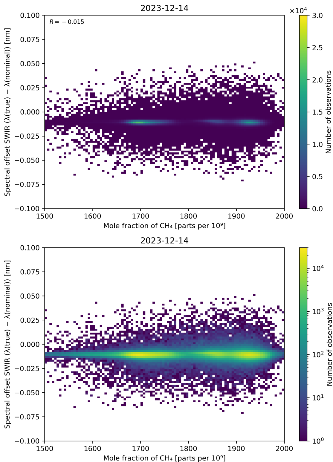
Figure 86: Scatter density plot of “Mole fraction of CH 4 ” against “Spectral offset SWIR ( \lambda(\text{true}) - \lambda(\text{nominal}) )” for 2023-12-14 to 2023-12-15.
