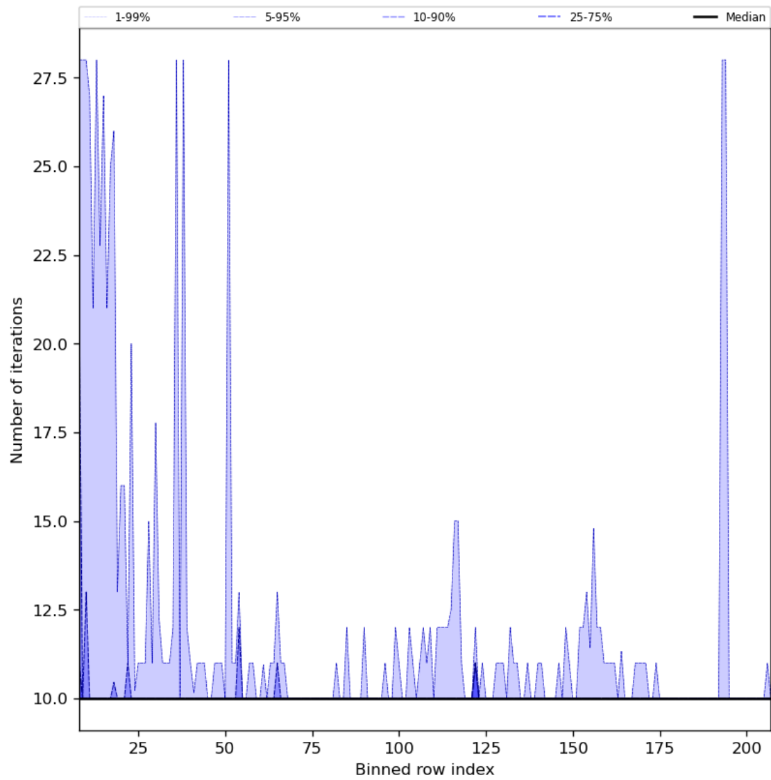
Figure 42: Along track statistics of “Number of iterations” for 2023-12-14 to 2023-12-15
