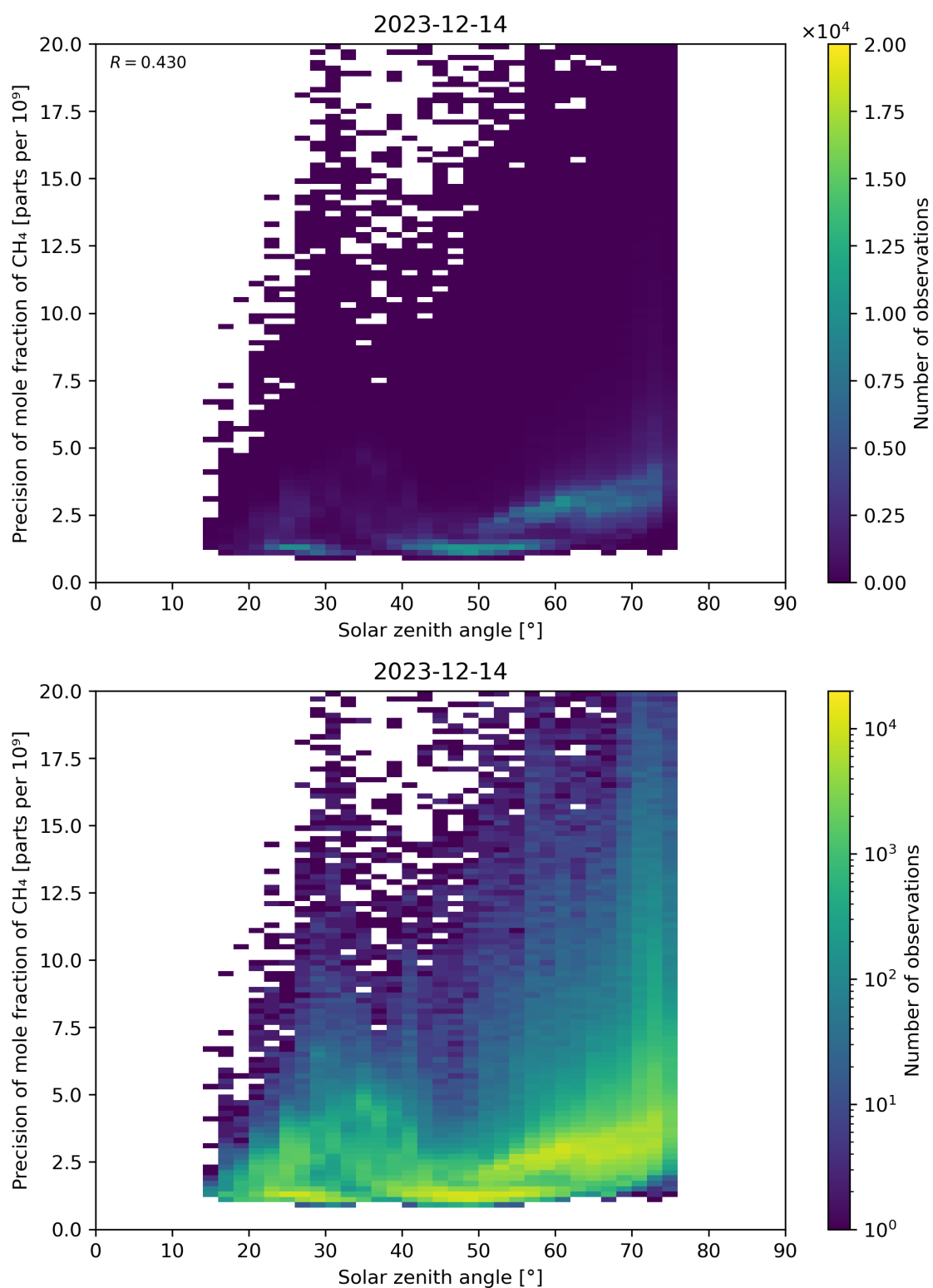
Figure 101: Scatter density plot of “Solar zenith angle” against “Precision of mole fraction of \text{CH}_4 ” for 2023-12-14 to 2023-12-15.
