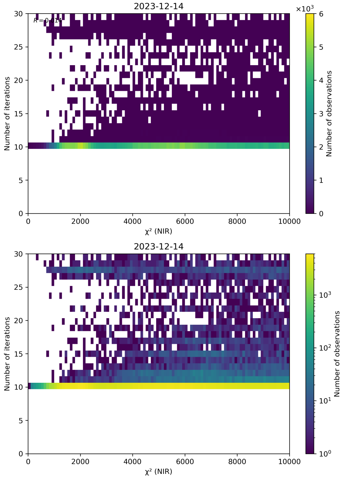
Figure 46: Scatter density plot of “ \chi^2 (NIR)” against “Number of iterations” for 2023-12-14 to 2023-12-15.
