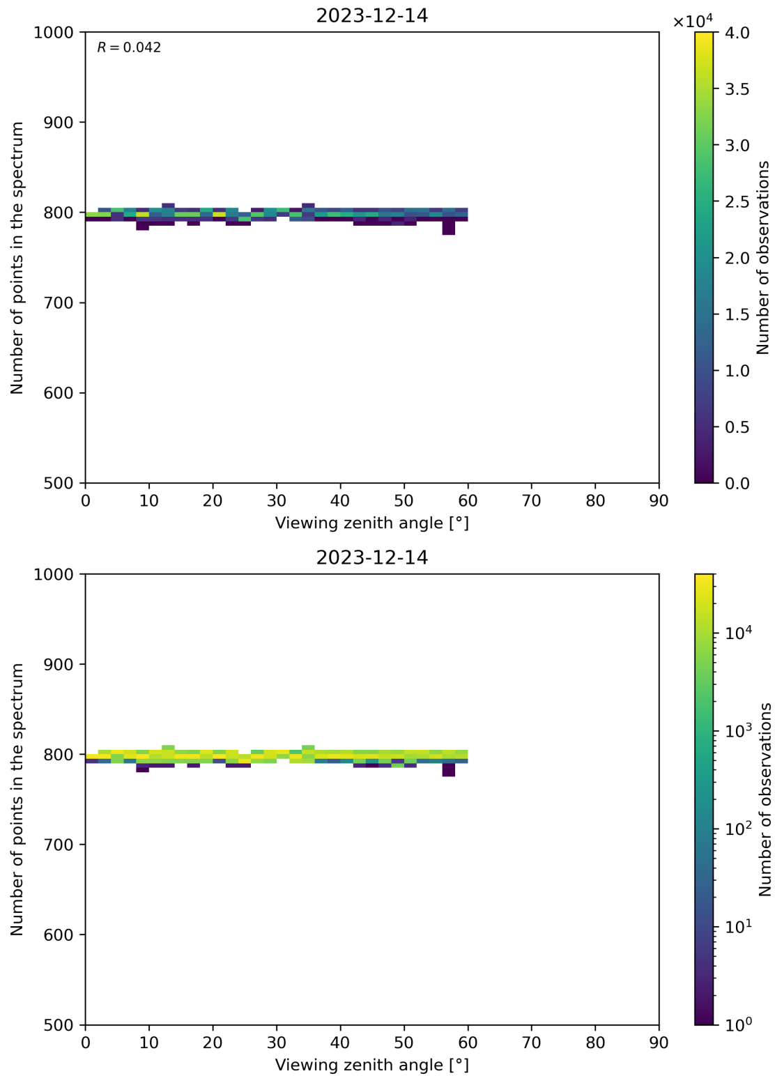
Figure 114: Scatter density plot of “Viewing zenith angle” against “Number of points in the spectrum” for 2023-12-14 to 2023-12-15.
