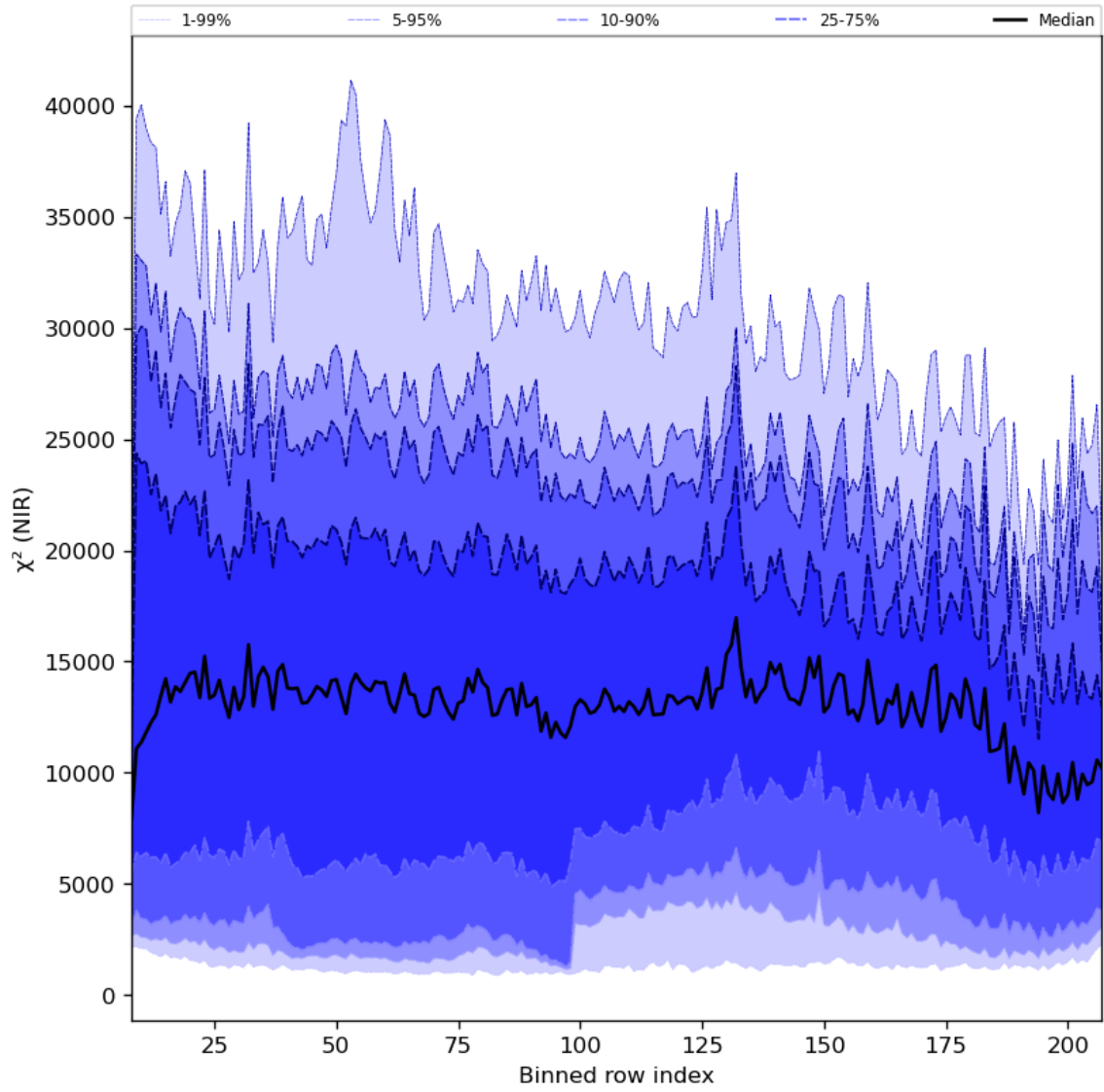
Figure 40: Along track statistics of “ \chi^2 (NIR)” for 2023-12-14 to 2023-12-15
