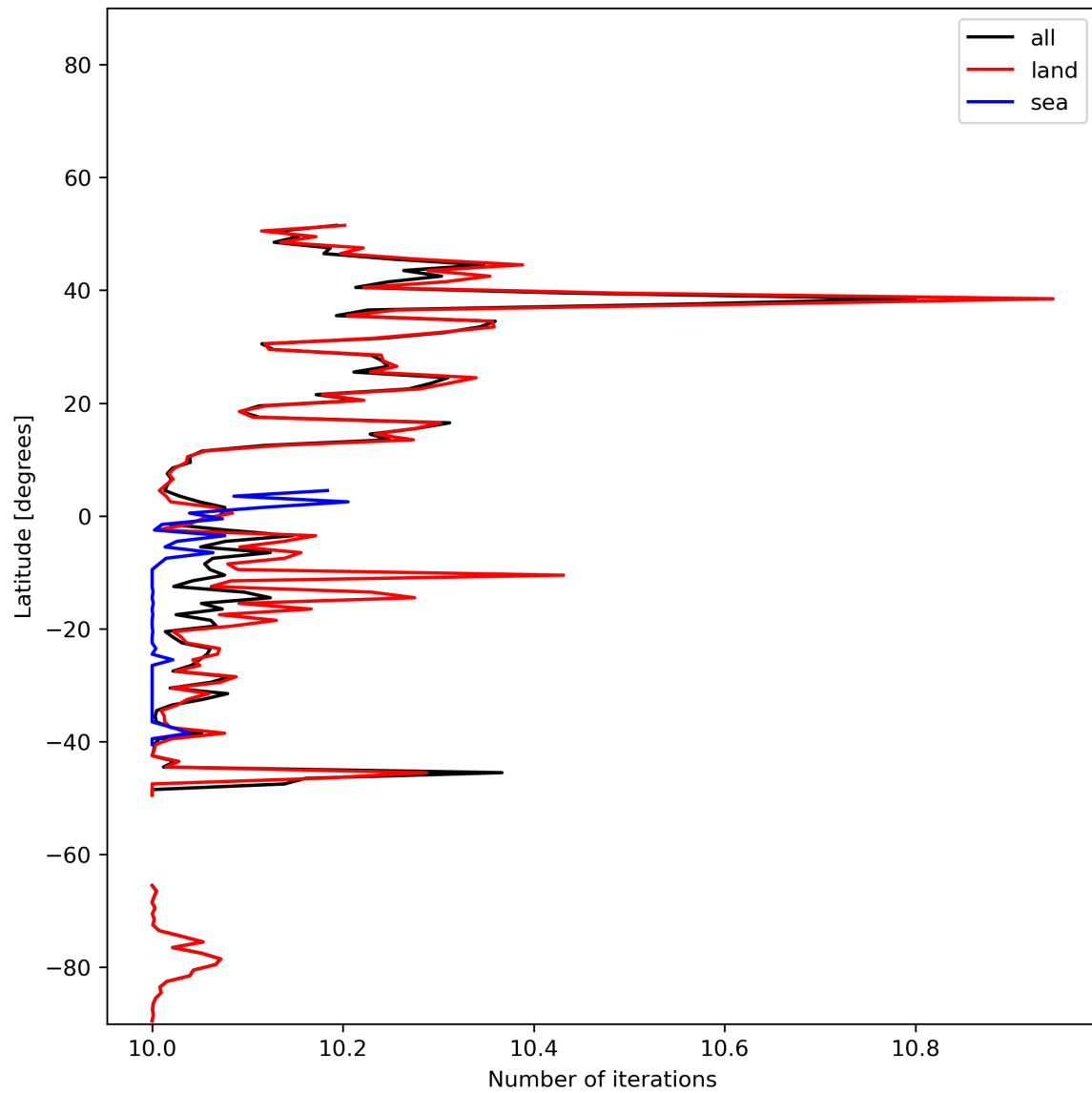
Figure 20: Zonal average of “Number of iterations” for 2023-12-14 to 2023-12-15.
