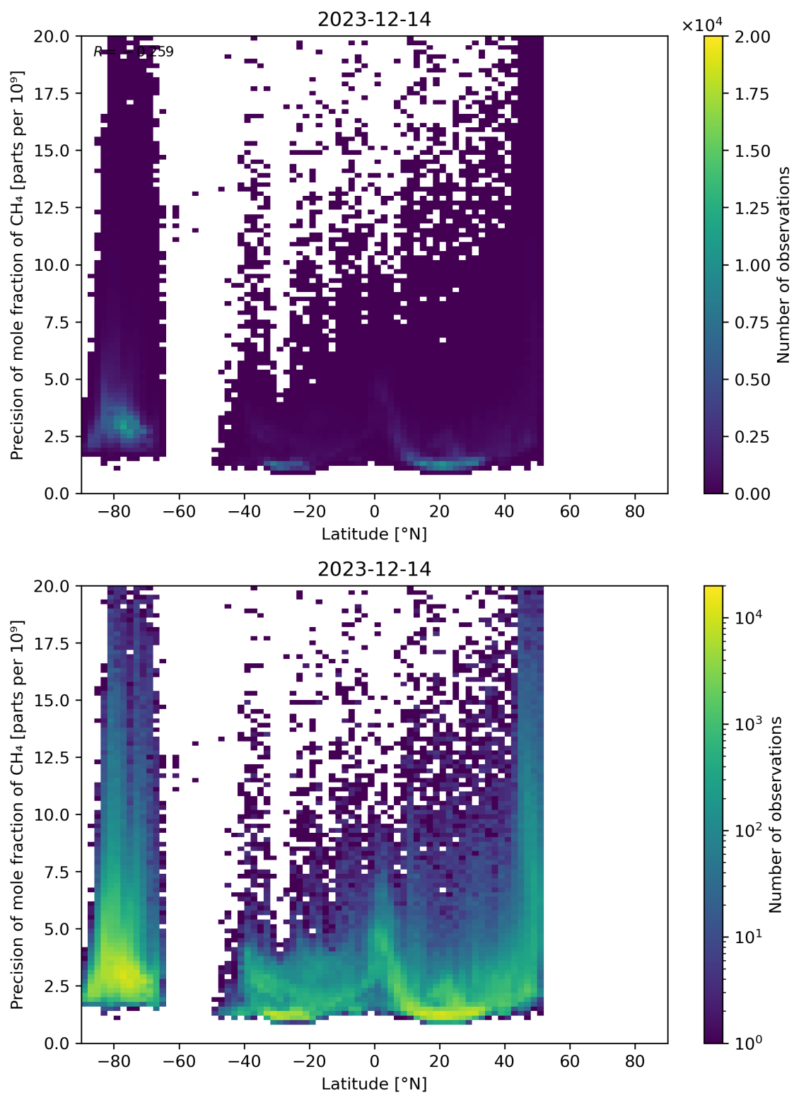
Figure 59: Scatter density plot of “Latitude” against “Precision of mole fraction of CH 4 ” for 2023-12-14 to 2023-12-15.
