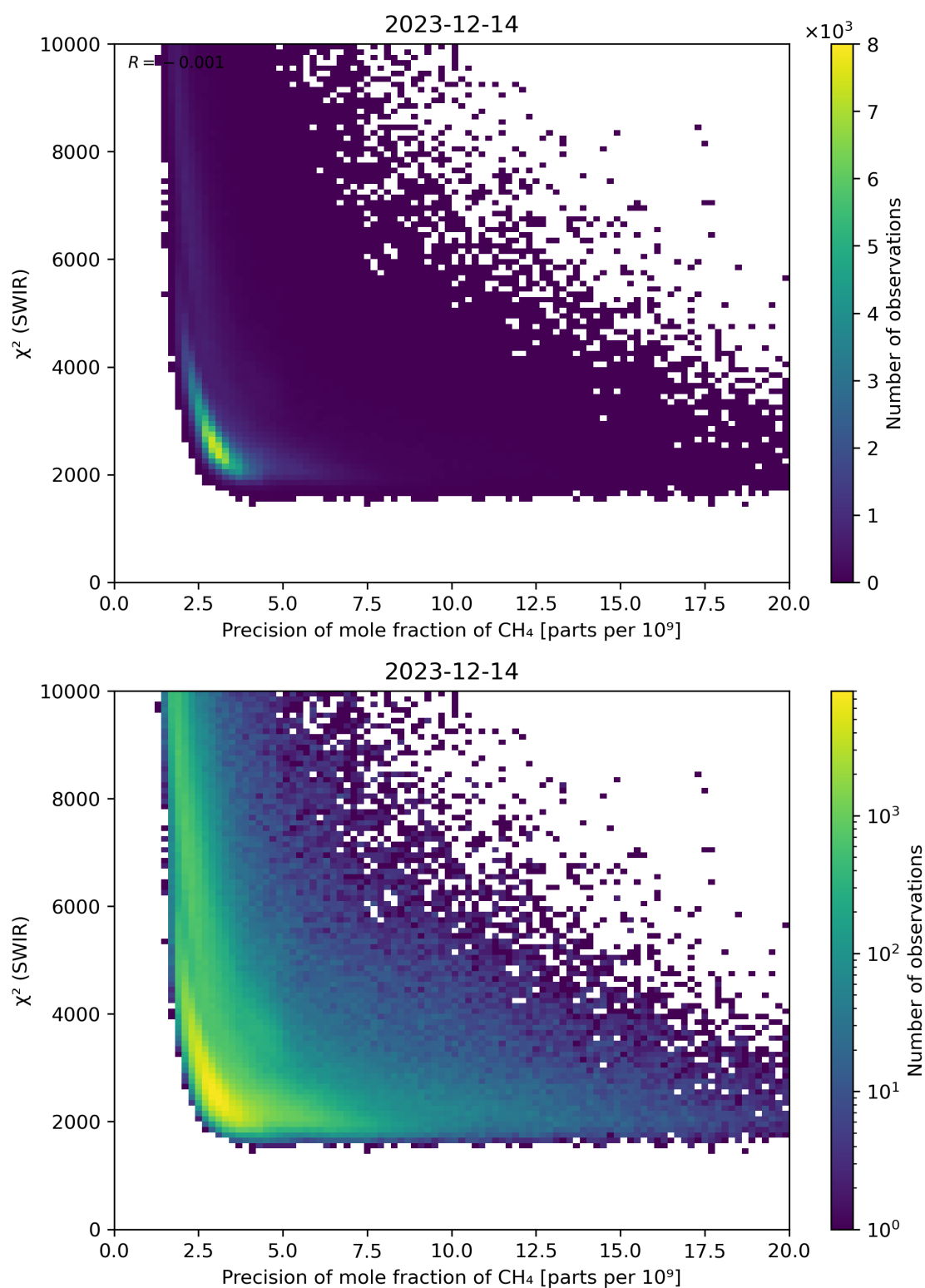
Figure 79: Scatter density plot of “Precision of mole fraction of \text{CH}_4 ” against “ \chi^2 (SWIR)” for 2023-12-14 to 2023-12-15.
