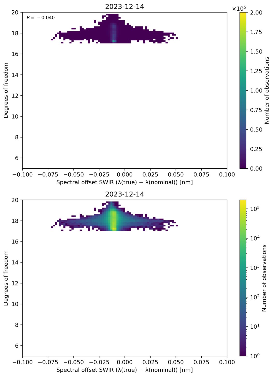
Figure 119: Scatter density plot of “Spectral offset SWIR ( \lambda(\text{true}) - \lambda(\text{nominal}) )” against “Degrees of freedom” for 2023-12-14 to 2023-12-15.
