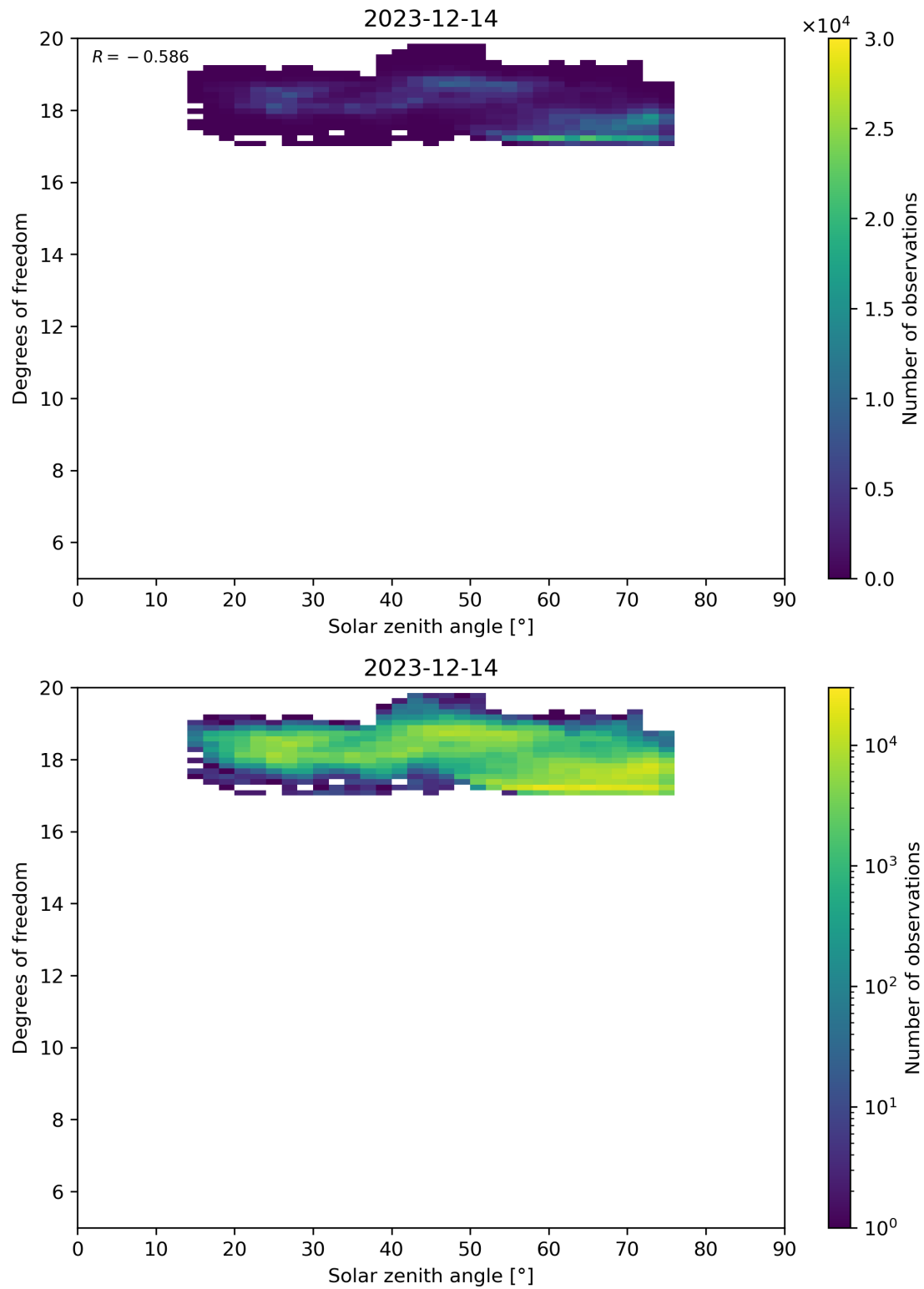
Figure 96: Scatter density plot of “Solar zenith angle” against “Degrees of freedom” for 2023-12-14 to 2023-12-15.
