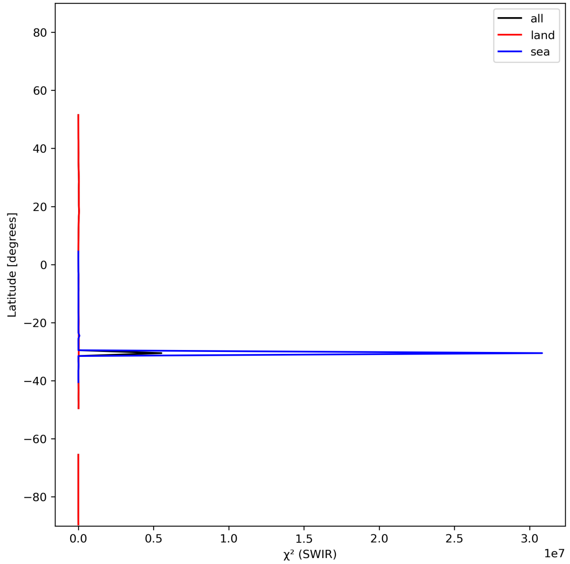
Figure 17: Zonal average of “ \chi^2 (SWIR)” for 2023-12-14 to 2023-12-15.
