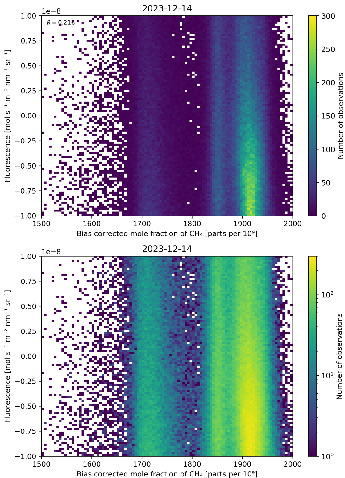
Figure 66: Scatter density plot of “Bias corrected mole fraction of \text{CH}_4 ” against “Fluorescence” for 2023-12-14 to 2023-12-15.
