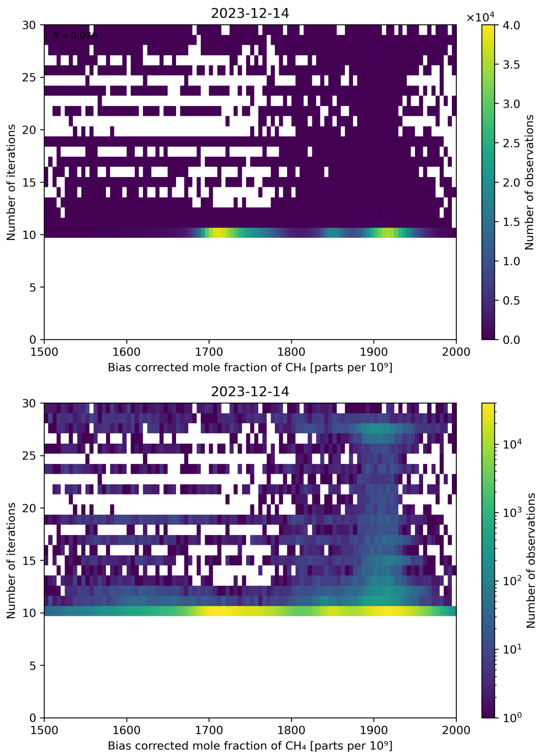
Figure 67: Scatter density plot of “Bias corrected mole fraction of \text{CH}_4 ” against “Number of iterations” for 2023-12-14 to 2023-12-15.
