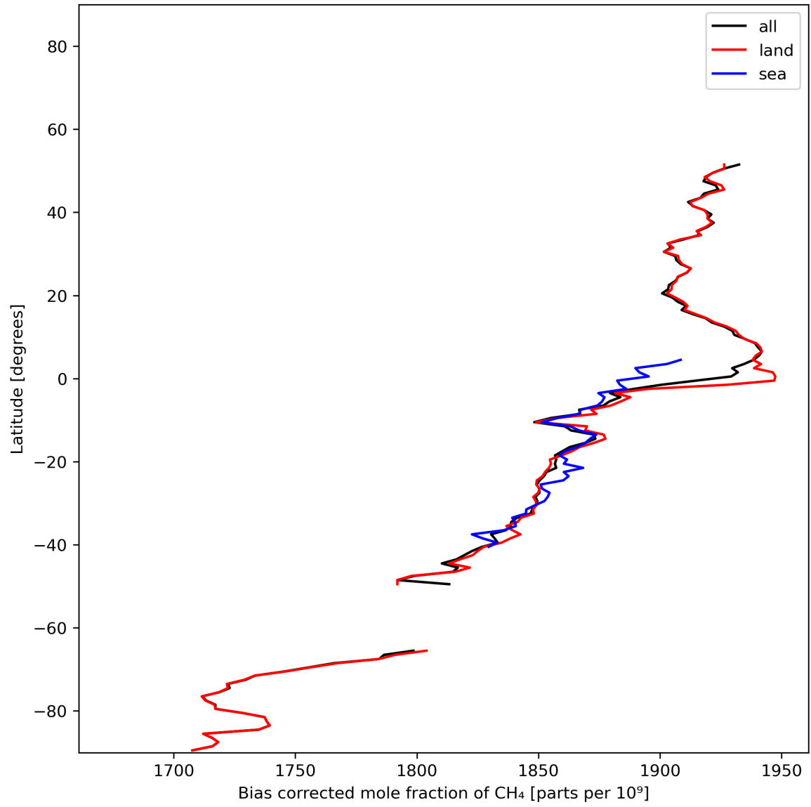
Figure 14: Zonal average of “Bias corrected mole fraction of CH 4 ” for 2023-12-14 to 2023-12-15.
