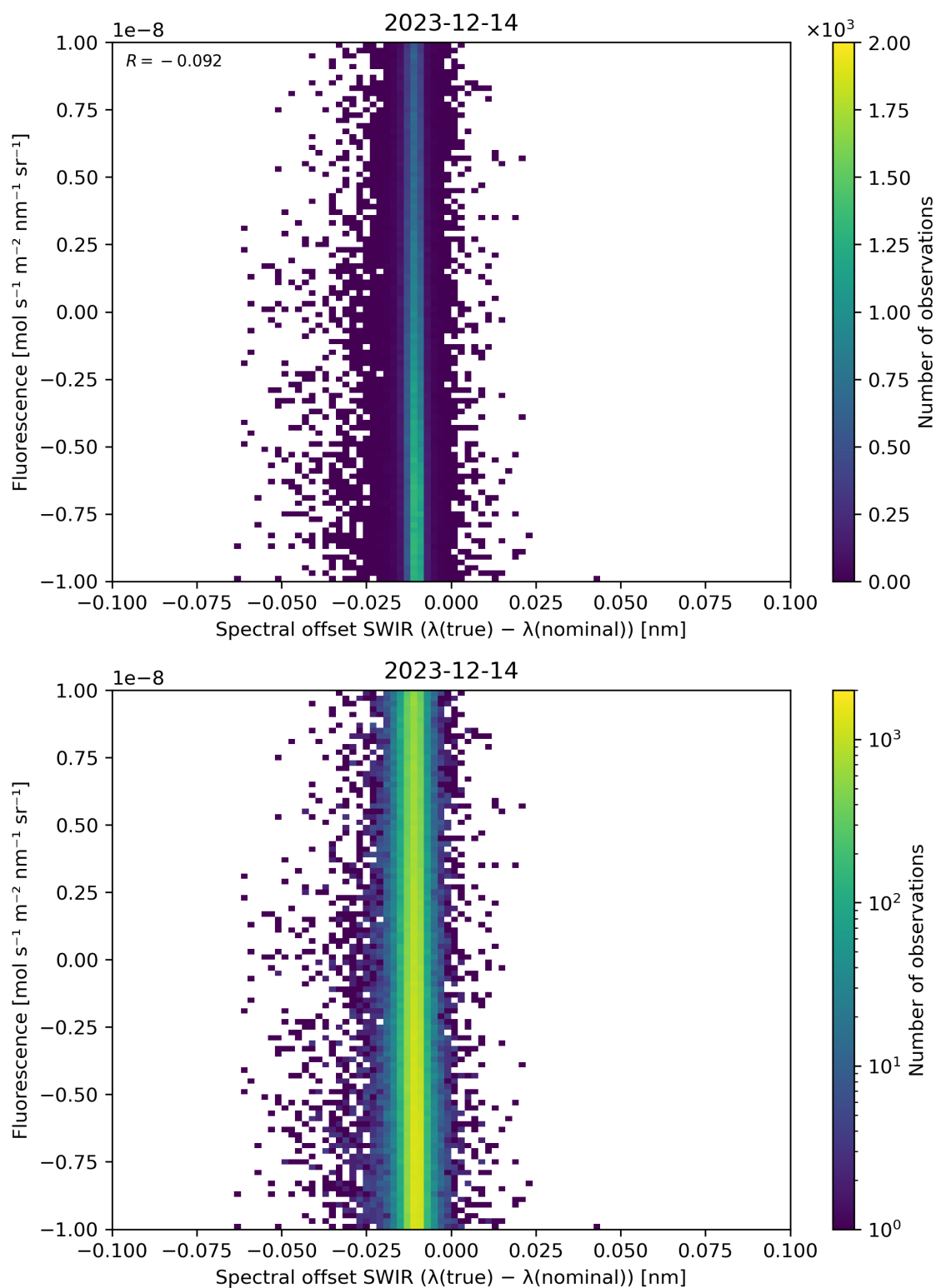
Figure 120: Scatter density plot of “Spectral offset SWIR ( \lambda(\text{true}) - \lambda(\text{nominal}) )” against “Fluorescence” for 2023-12-14 to 2023-12-15.
