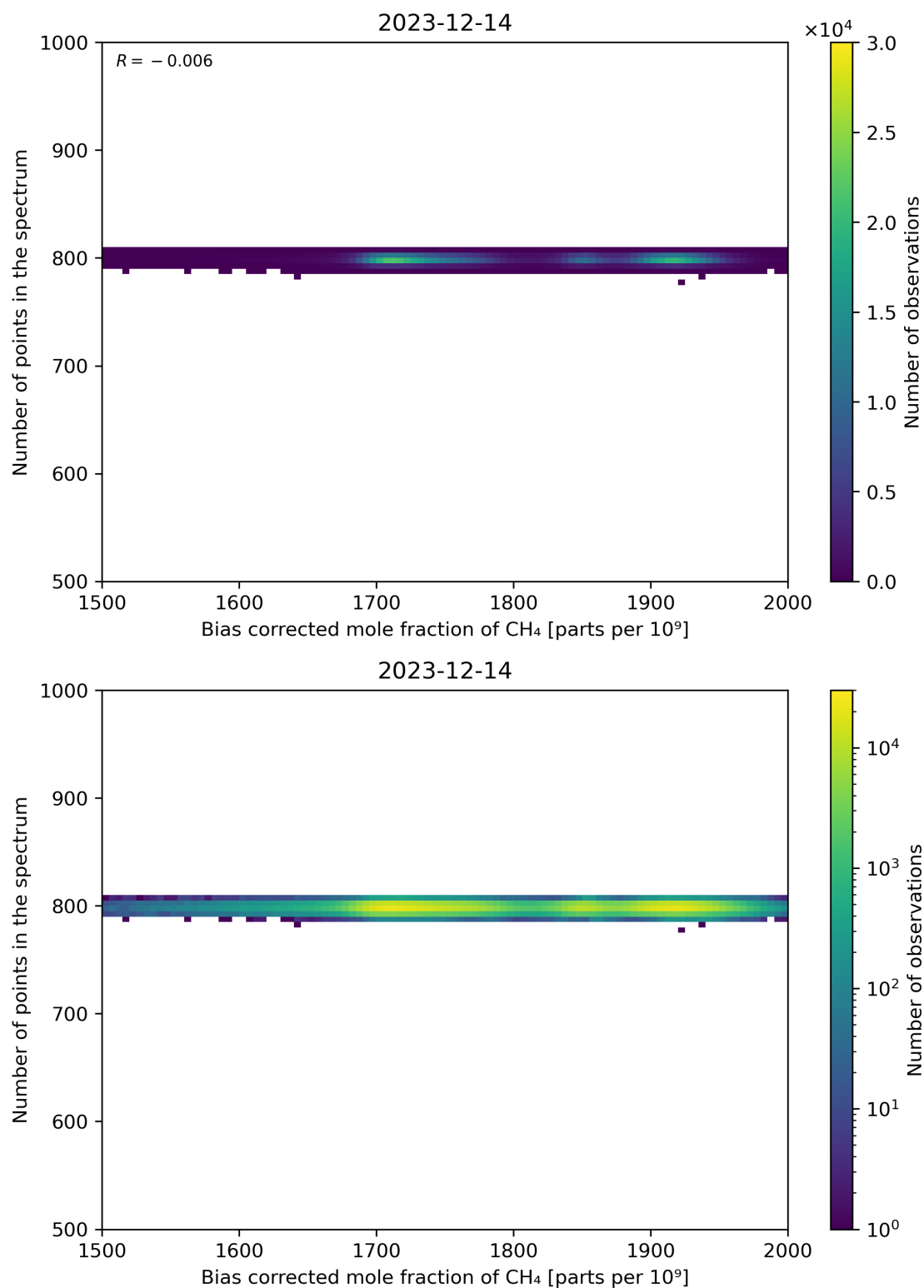
Figure 68: Scatter density plot of “Bias corrected mole fraction of CH 4 ” against “Number of points in the spectrum” for 2023-12-14 to 2023-12-15.
