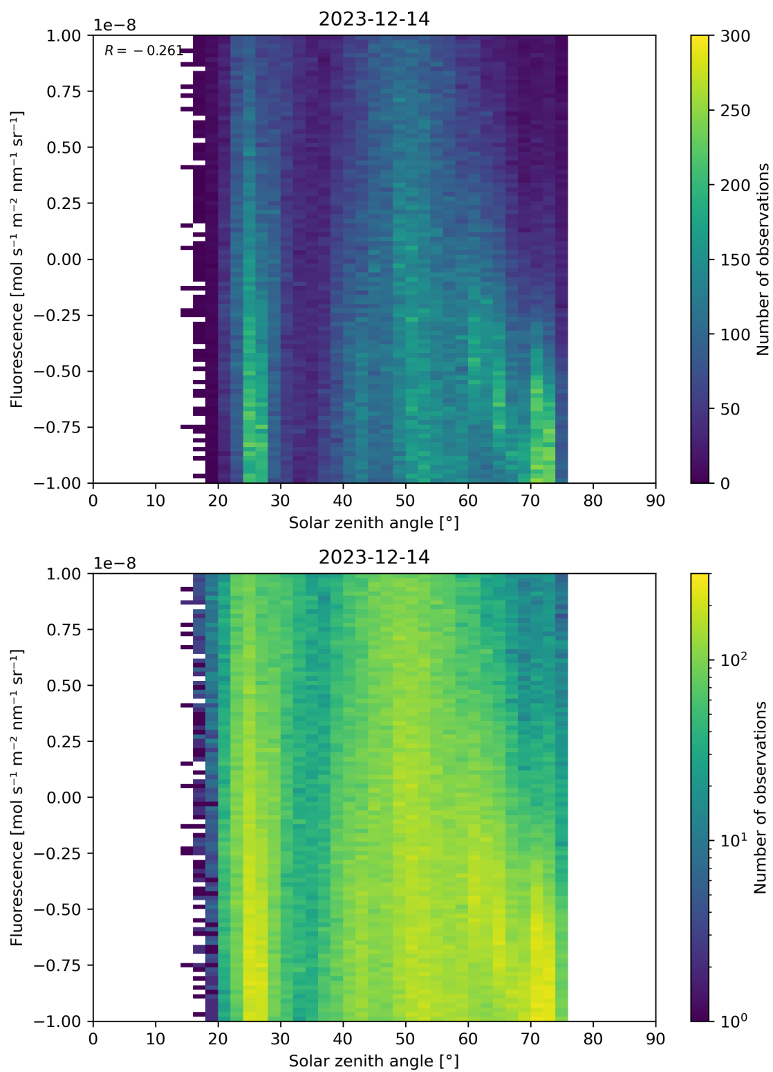
Figure 97: Scatter density plot of “Solar zenith angle” against “Fluorescence” for 2023-12-14 to 2023-12-15.
