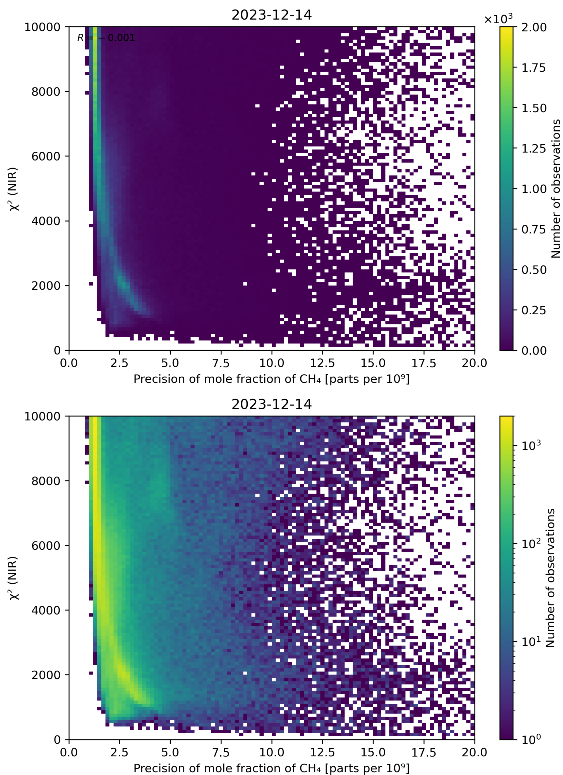
Figure 78: Scatter density plot of “Precision of mole fraction of \text{CH}_4 ” against “ \chi^2 (NIR)” for 2023-12-14 to 2023-12-15.
