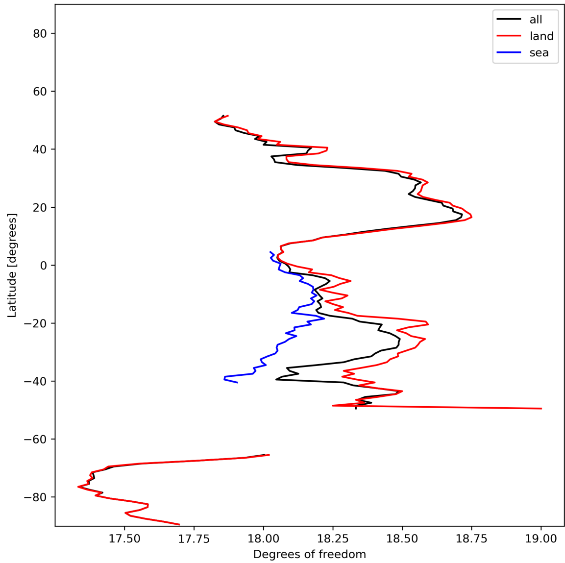
Figure 19: Zonal average of “Degrees of freedom” for 2023-12-14 to 2023-12-15.
