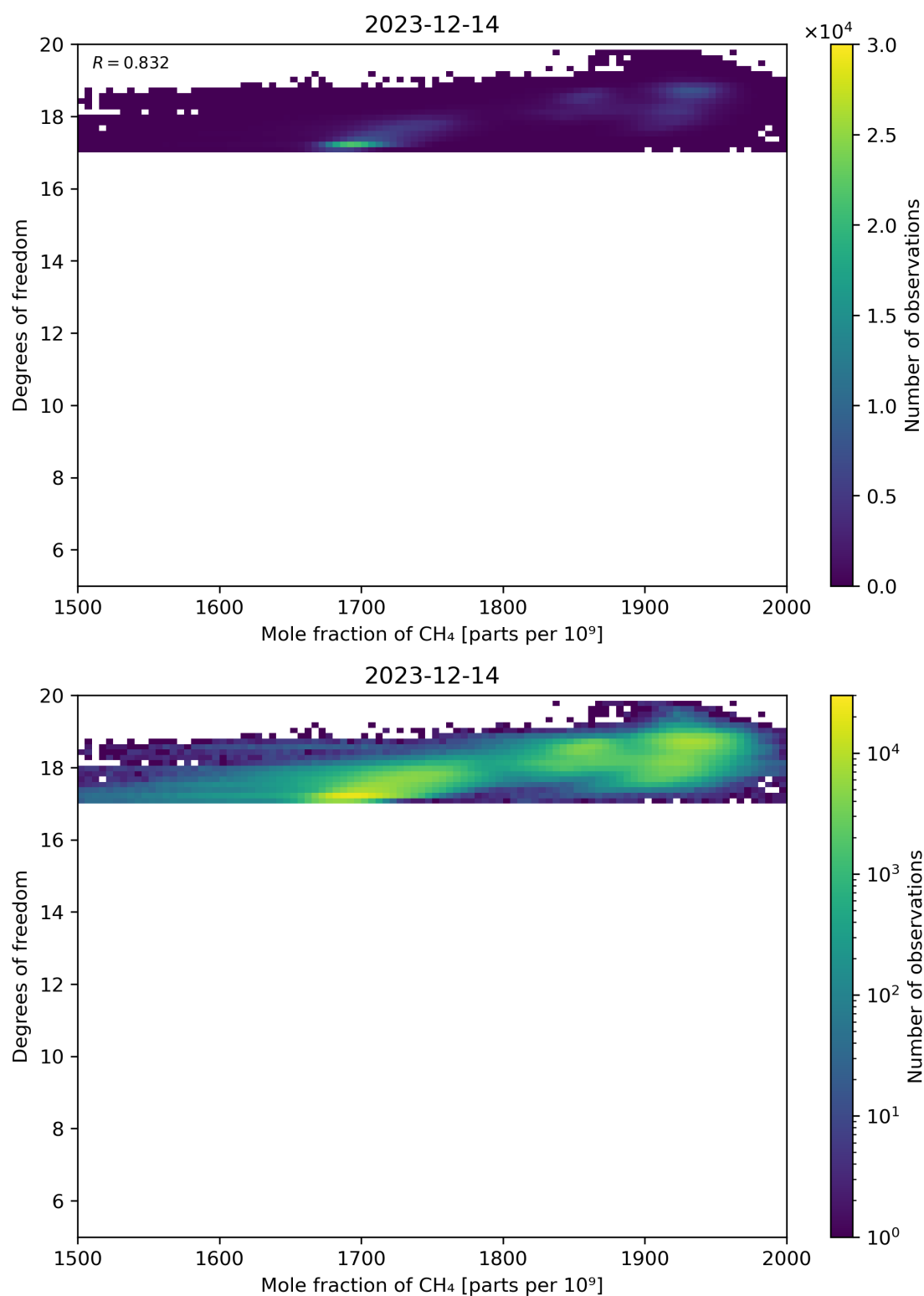
Figure 72: Scatter density plot of “Mole fraction of CH 4 ” against “Degrees of freedom” for 2023-12-14 to 2023-12-15.
