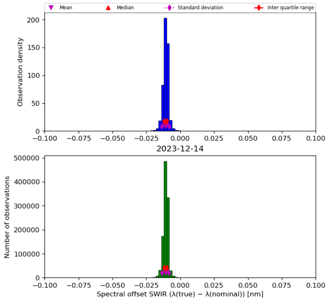
Figure 27: Histogram of “Spectral offset SWIR ( \lambda(\text{true}) - \lambda(\text{nominal}) )” for 2023-12-14 to 2023-12-15
