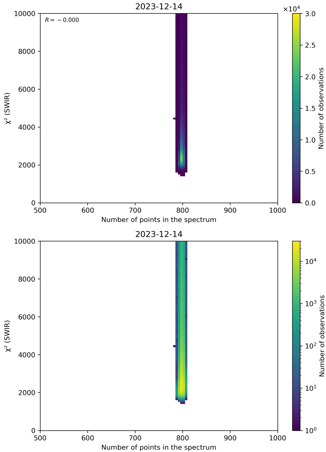
Figure 89: Scatter density plot of “Number of points in the spectrum” against “ \chi^2 (SWIR)” for 2023-12-14 to 2023-12-15.
