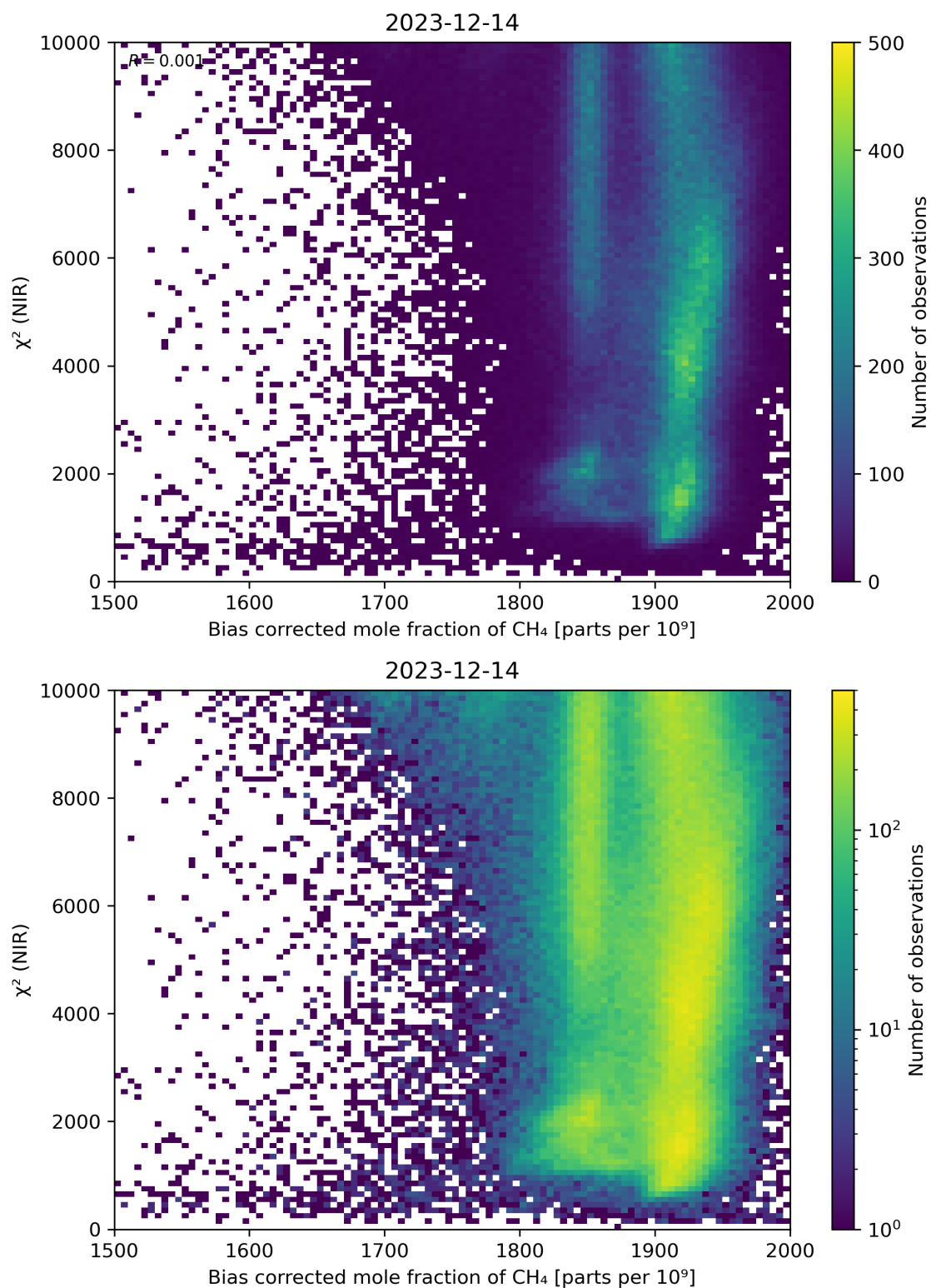
Figure 63: Scatter density plot of “Bias corrected mole fraction of CH 4 ” against “ \chi^2 (NIR)” for 2023-12-14 to 2023-12-15.
