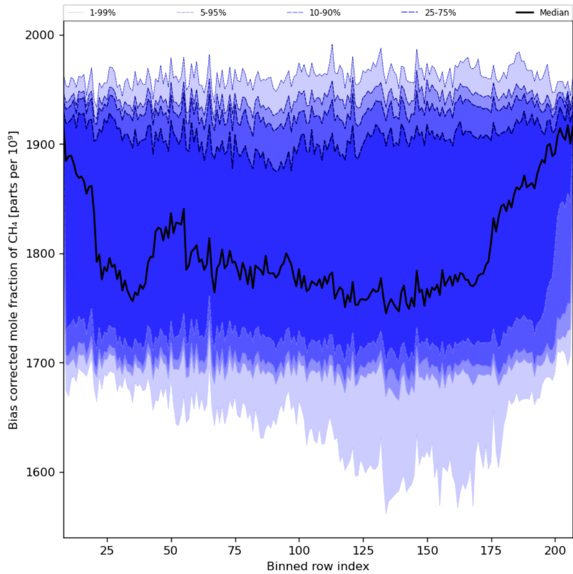
Figure 36: Along track statistics of “Bias corrected mole fraction of \text{CH}_4 ” for 2023-12-14 to 2023-12-15
