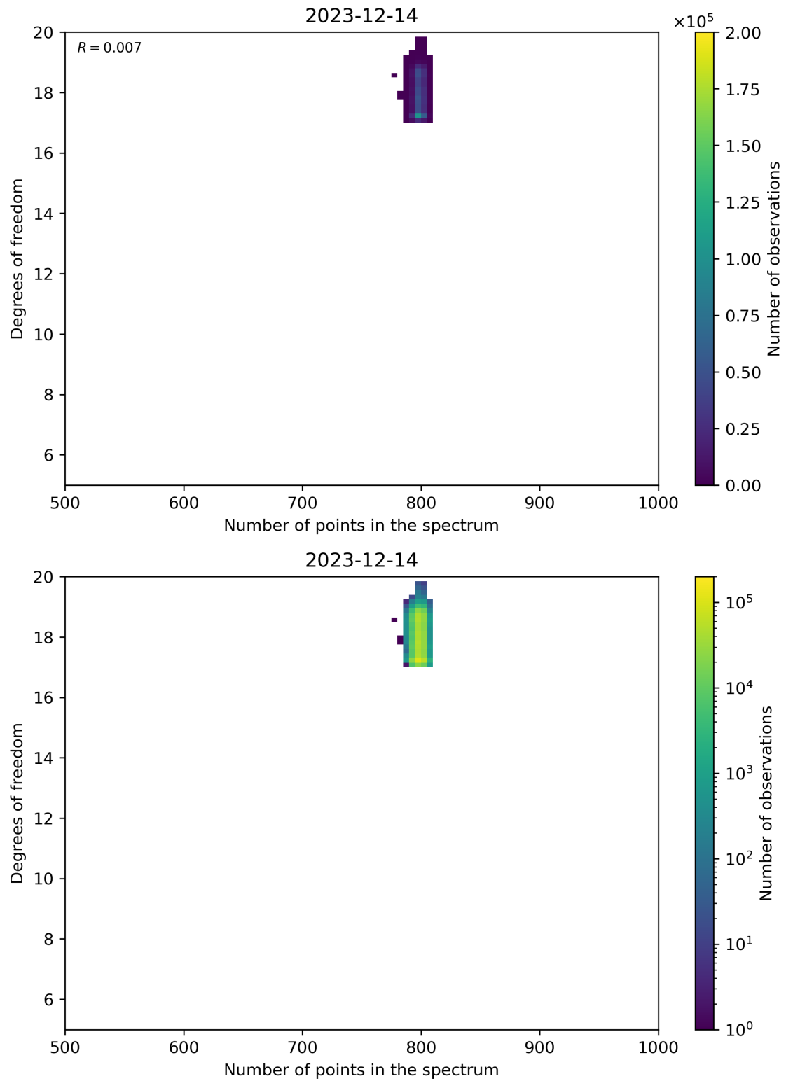
Figure 90: Scatter density plot of “Number of points in the spectrum” against “Degrees of freedom” for 2023-12-14 to 2023-12-15.
