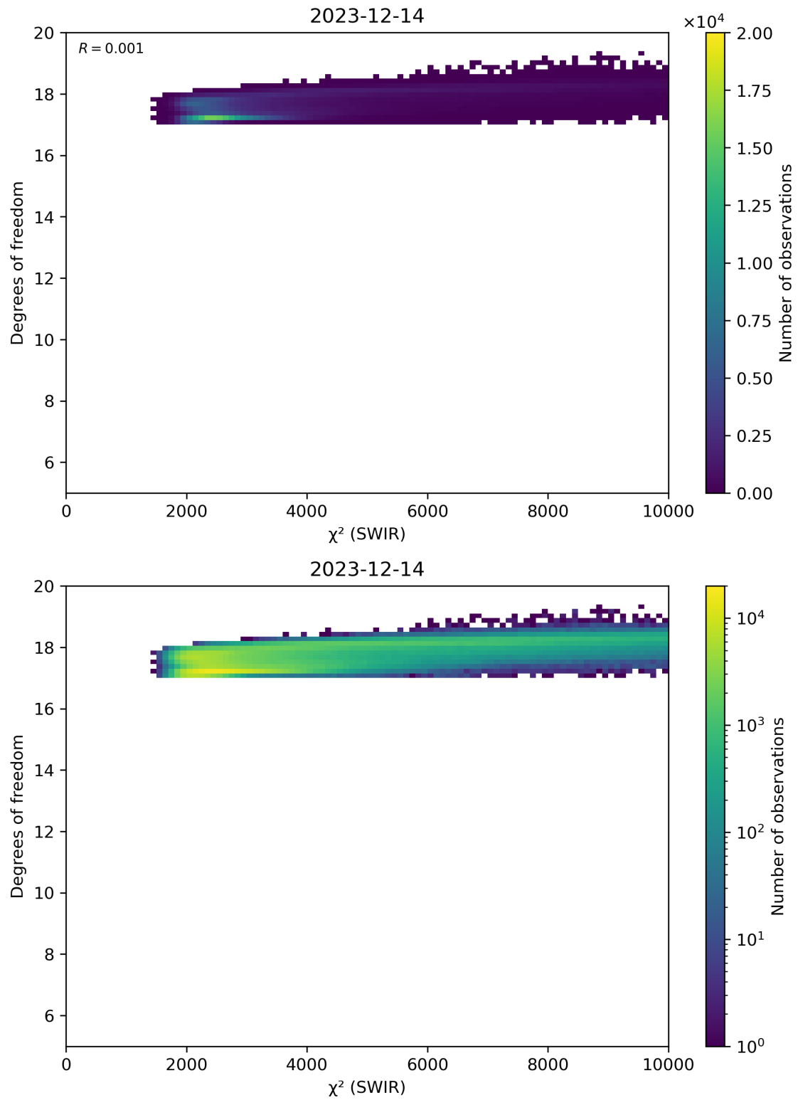
Figure 48: Scatter density plot of “ \chi^2 (SWIR)” against “Degrees of freedom” for 2023-12-14 to 2023-12-15.
