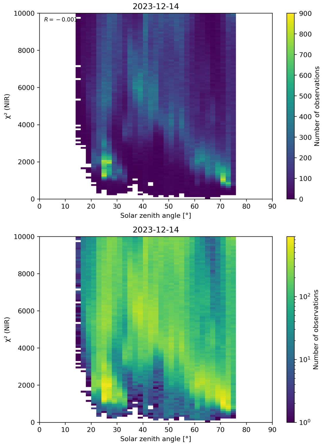
Figure 94: Scatter density plot of “Solar zenith angle” against “ \chi^2 (NIR)” for 2023-12-14 to 2023-12-15.
