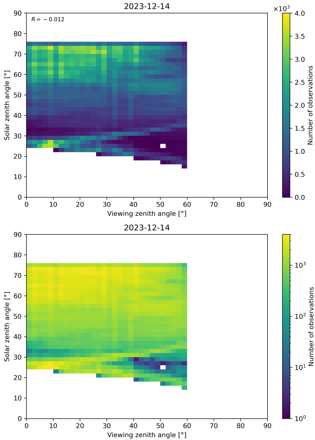
Figure 115: Scatter density plot of “Viewing zenith angle” against “Solar zenith angle” for 2023-12-14 to 2023-12-15.
