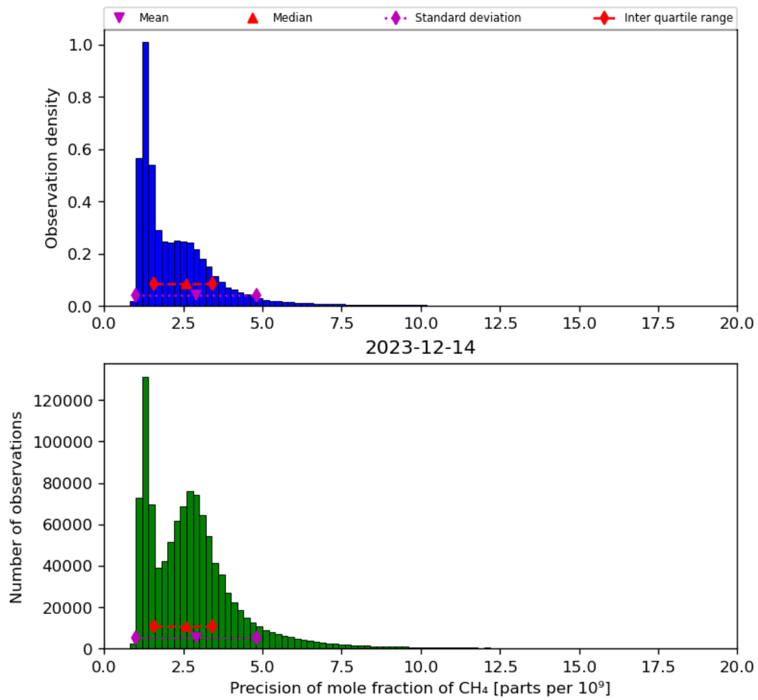
Figure 24: Histogram of “Precision of mole fraction of CH 4 ” for 2023-12-14 to 2023-12-15
