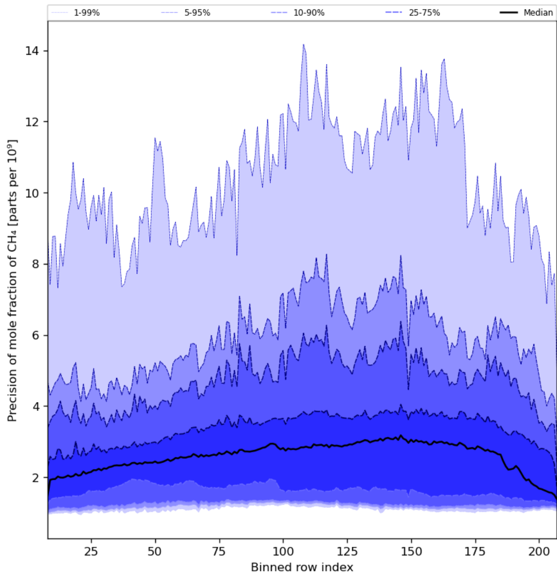
Figure 35: Along track statistics of “Precision of mole fraction of CH 4 ” for 2023-12-14 to 2023-12-15
