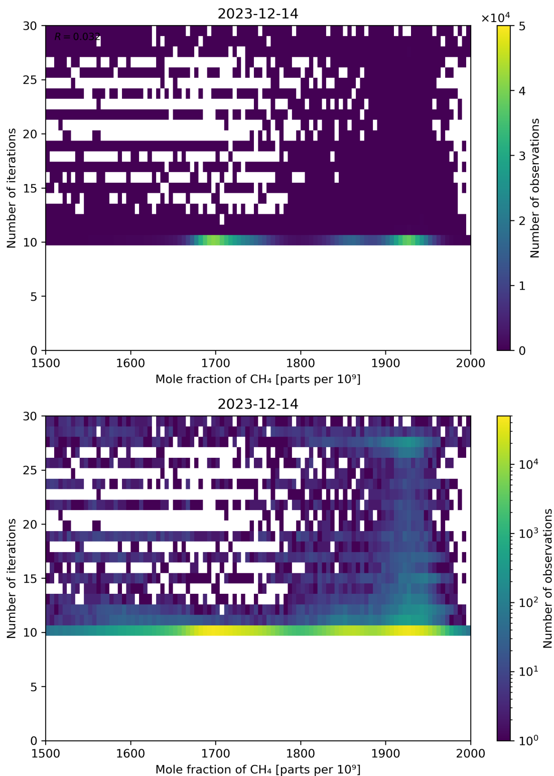
Figure 76: Scatter density plot of “Mole fraction of CH 4 ” against “Number of iterations” for 2023-12-14 to 2023-12-15.
