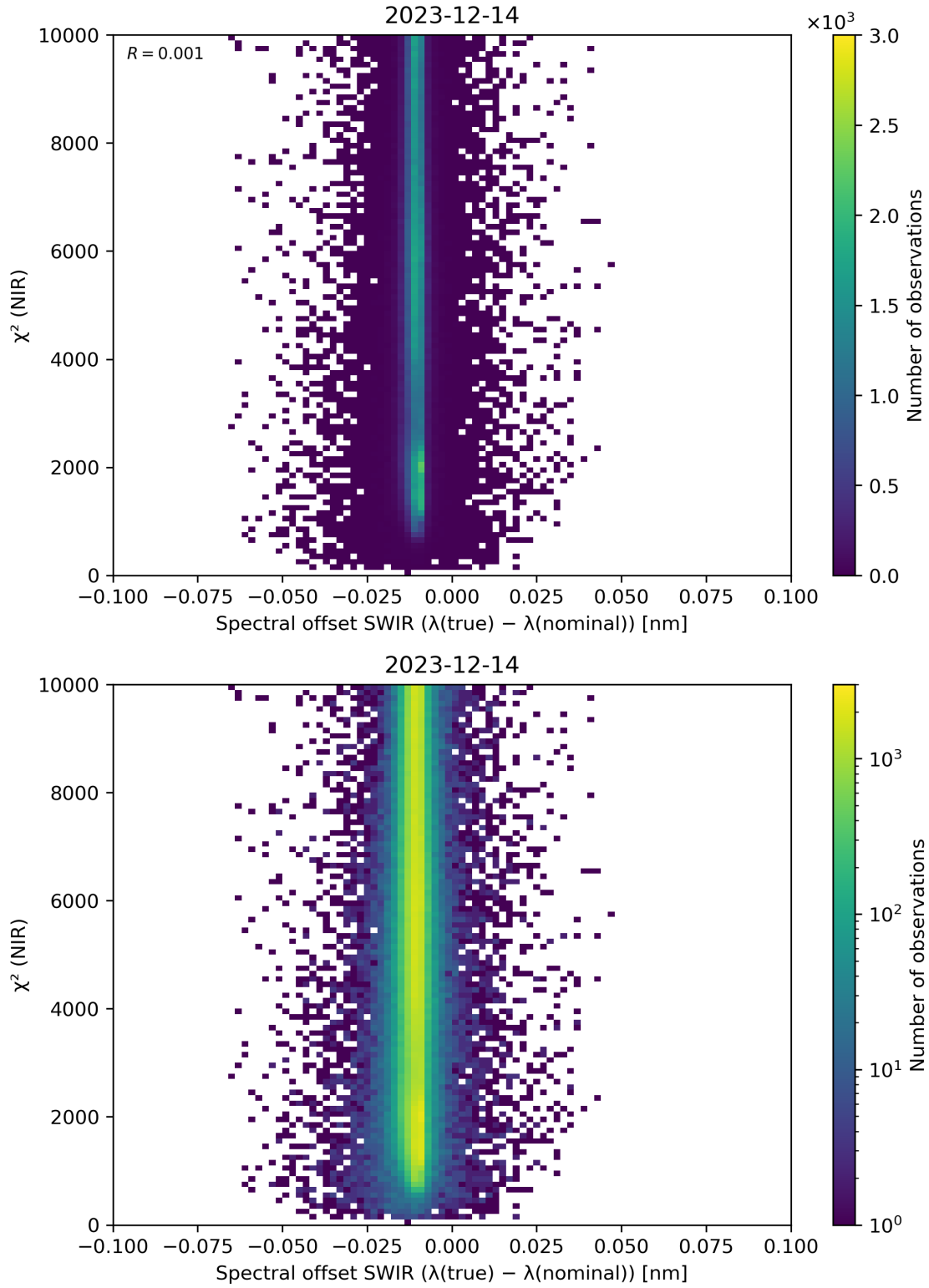
Figure 117: Scatter density plot of “Spectral offset SWIR ( \lambda(\text{true}) - \lambda(\text{nominal}) )” against “ \chi^2 (NIR)” for 2023-12-14 to 2023-12-15.
