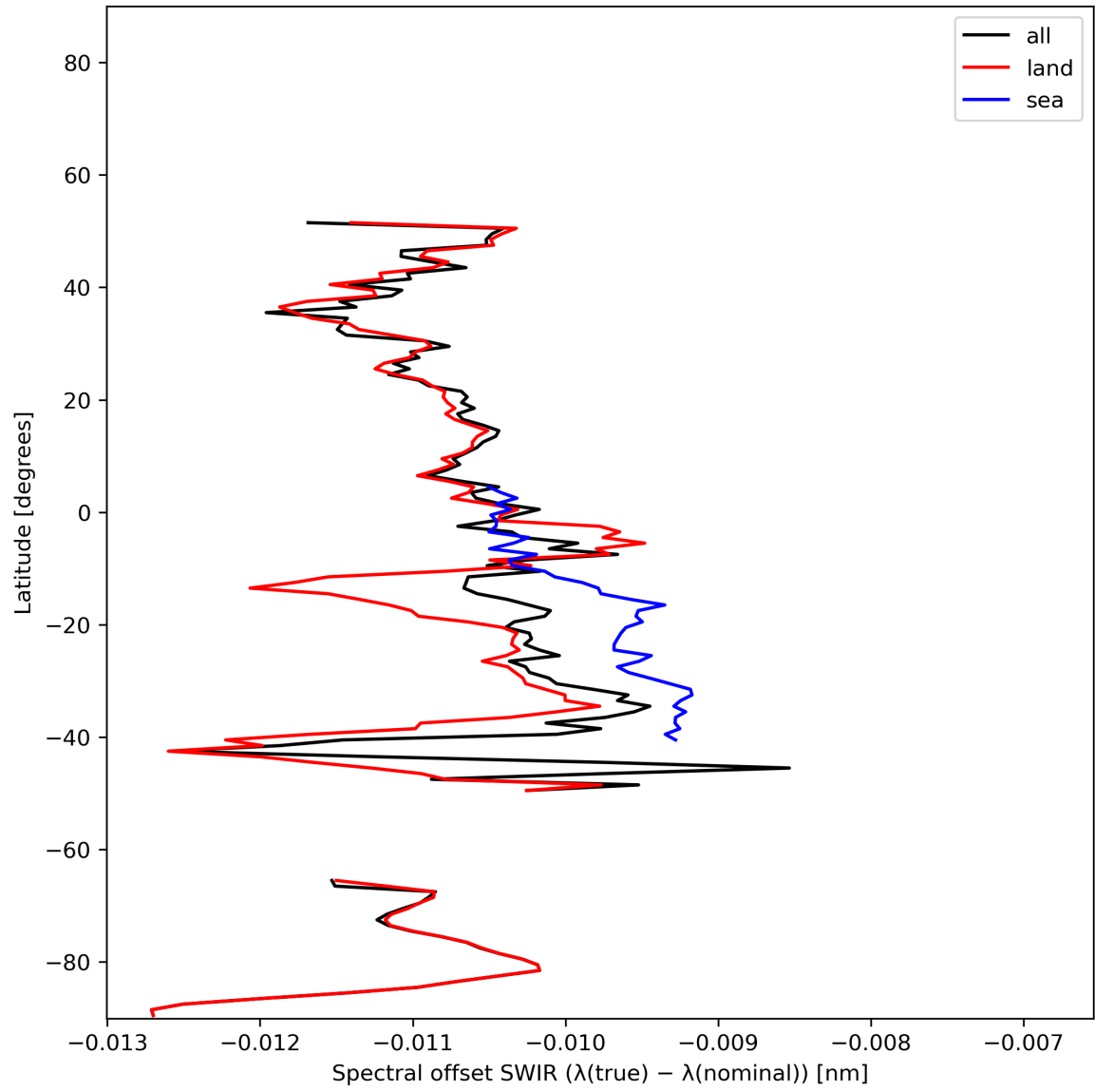
Figure 16: Zonal average of “Spectral offset SWIR ( \lambda(\text{true}) - \lambda(\text{nominal}) )” for 2023-12-14 to 2023-12-15.
