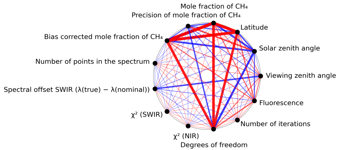
Figure 1: Map of correlation graph for 2023-12-14 to 2023-12-15.
