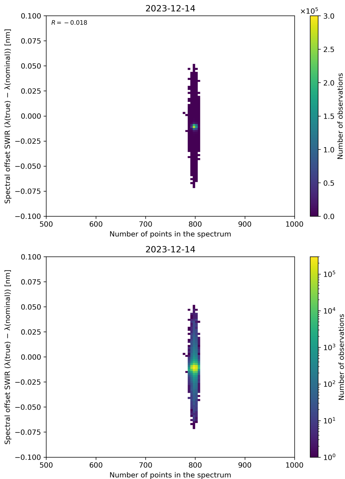
Figure 93: Scatter density plot of “Number of points in the spectrum” against “Spectral offset SWIR ( \lambda(\text{true}) - \lambda(\text{nominal}) )” for 2023-12-14 to 2023-12-15.
