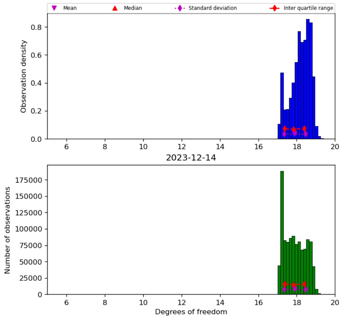
Figure 30: Histogram of “Degrees of freedom” for 2023-12-14 to 2023-12-15
