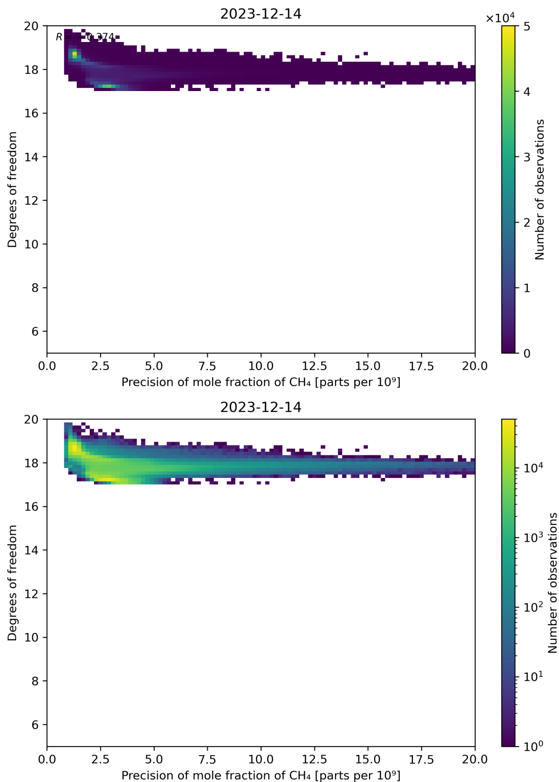
Figure 80: Scatter density plot of “Precision of mole fraction of CH 4 ” against “Degrees of freedom” for 2023-12-14 to 2023-12-15.
