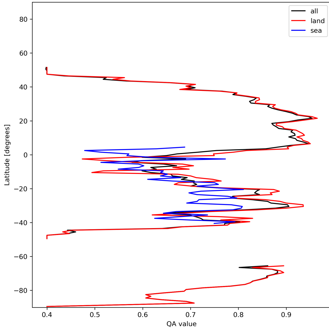
Figure 11: Zonal average of “QA value” for 2023-12-14 to 2023-12-15.
