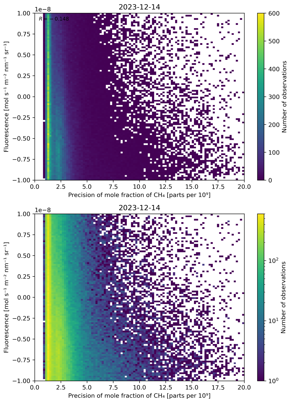
Figure 81: Scatter density plot of “Precision of mole fraction of \text{CH}_4 ” against “Fluorescence” for 2023-12-14 to 2023-12-15.
