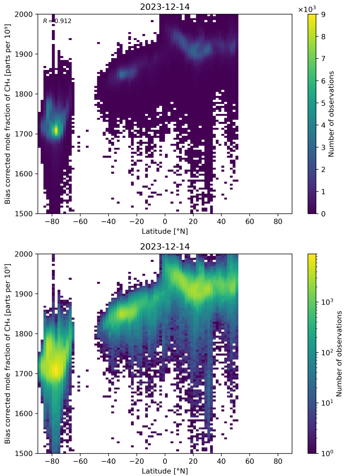
Figure 58: Scatter density plot of “Latitude” against “Bias corrected mole fraction of CH 4 ” for 2023-12-14 to 2023-12-15.
