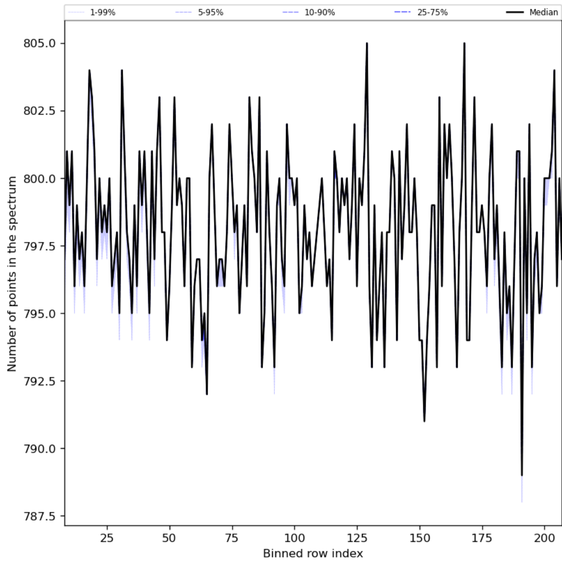
Figure 37: Along track statistics of “Number of points in the spectrum” for 2023-12-14 to 2023-12-15
