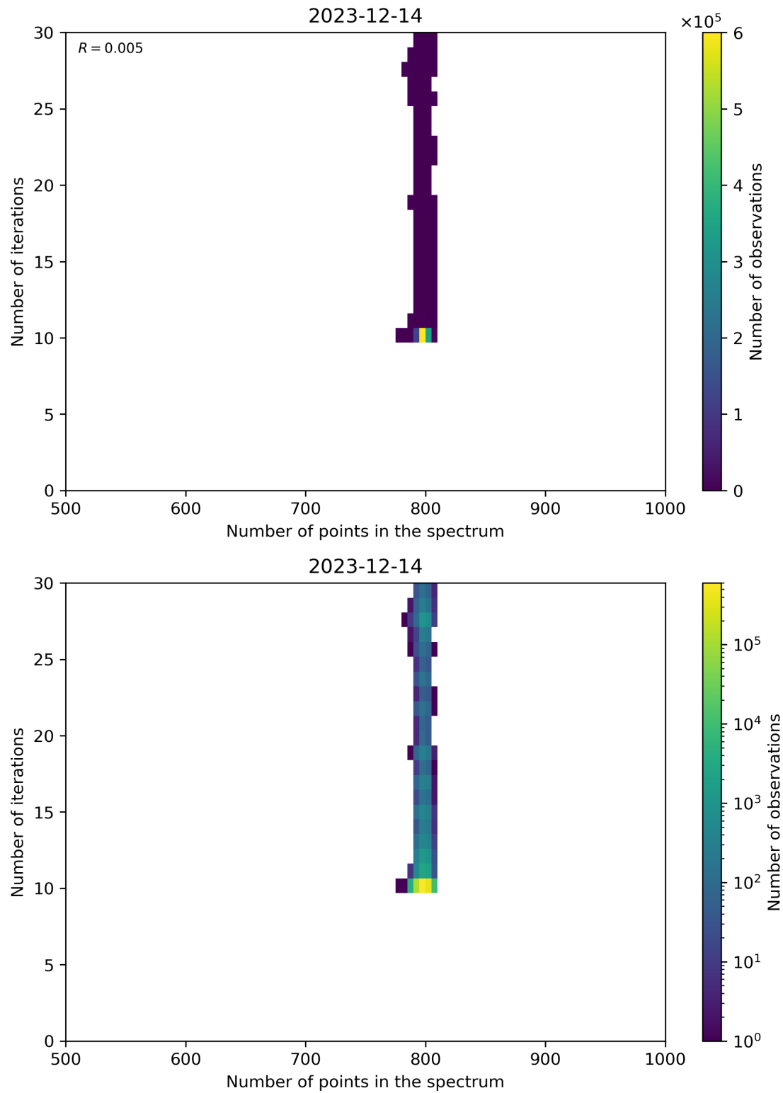
Figure 92: Scatter density plot of “Number of points in the spectrum” against “Number of iterations” for 2023-12-14 to 2023-12-15.
