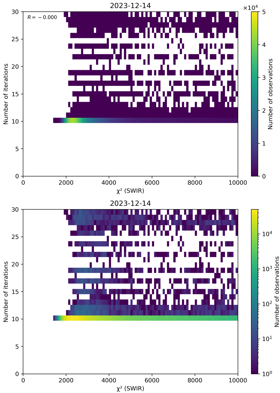
Figure 50: Scatter density plot of “ \chi^2 (SWIR)” against “Number of iterations” for 2023-12-14 to 2023-12-15.
