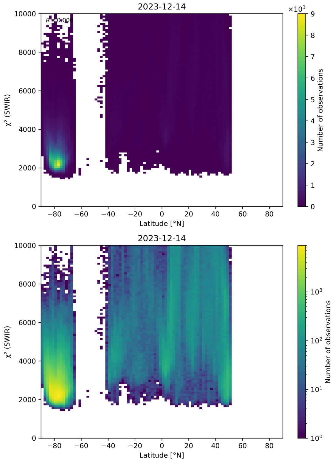
Figure 54: Scatter density plot of “Latitude” against “ \chi^2 (SWIR)” for 2023-12-14 to 2023-12-15.
