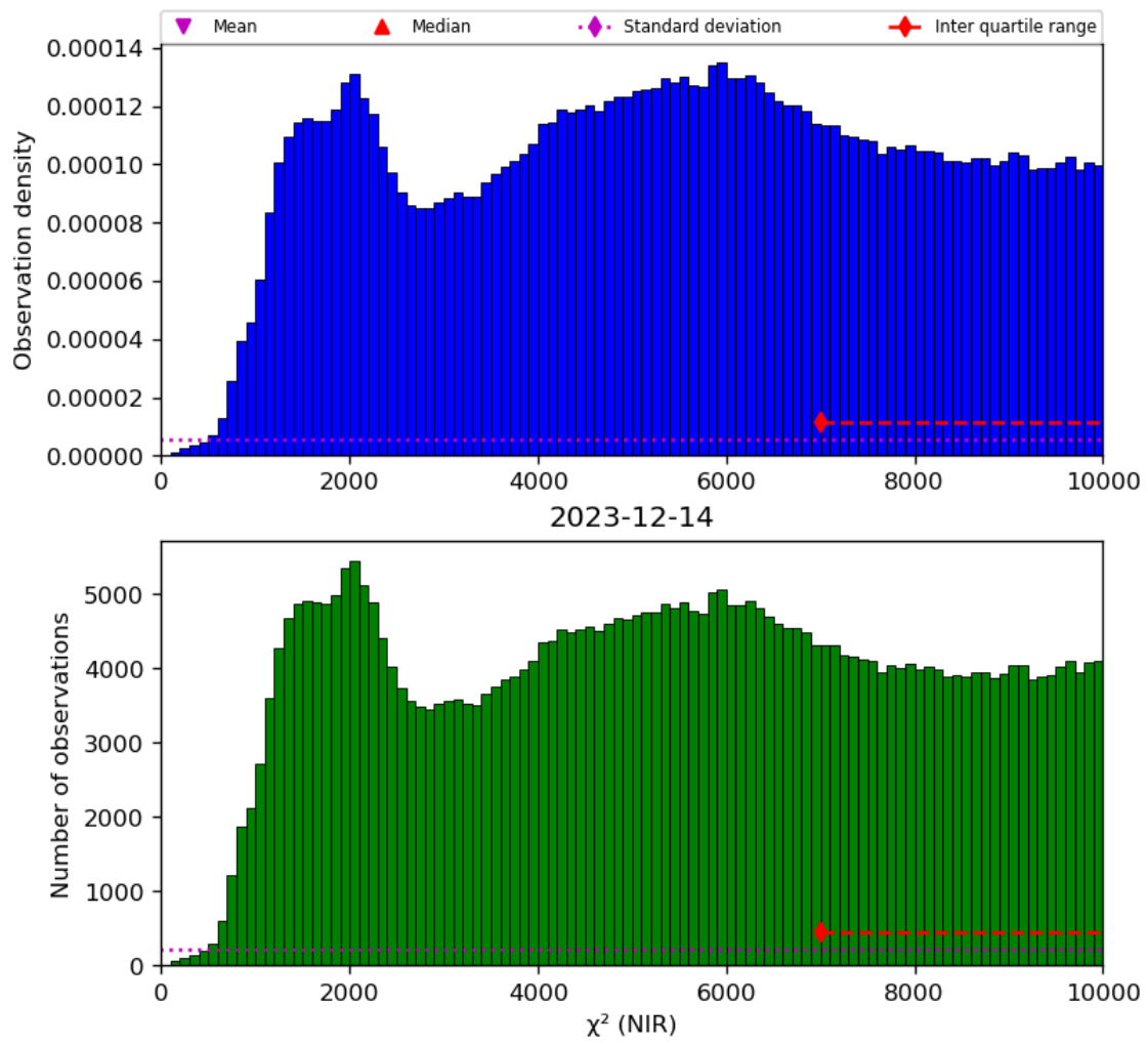
Figure 29: Histogram of “ \chi^2 (NIR)” for 2023-12-14 to 2023-12-15
