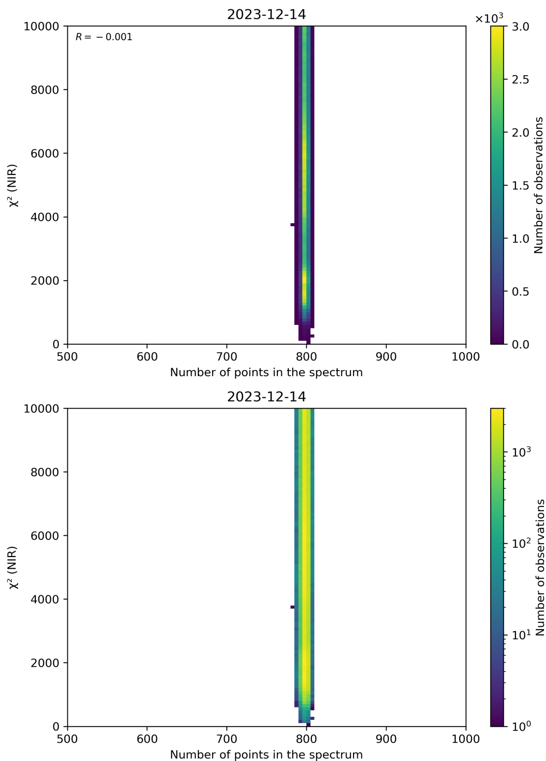
Figure 88: Scatter density plot of “Number of points in the spectrum” against “ \chi^2 (NIR)” for 2023-12-14 to 2023-12-15.
