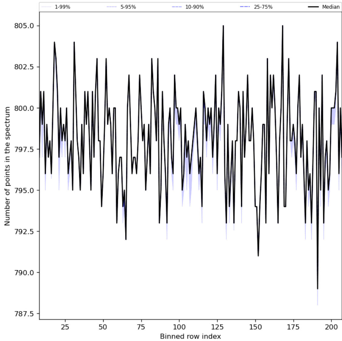
Figure 37: Along track statistics of “Number of points in the spectrum” for 2023-12-14 to 2023-12-16
