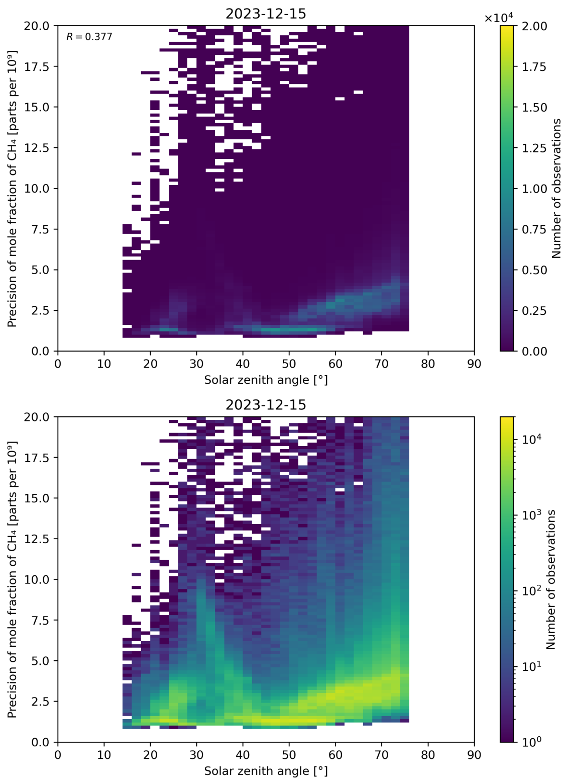
Figure 101: Scatter density plot of “Solar zenith angle” against “Precision of mole fraction of \text{CH}_4 ” for 2023-12-14 to 2023-12-16.
