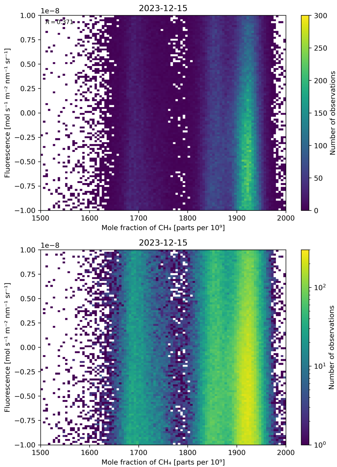
Figure 73: Scatter density plot of “Mole fraction of CH 4 ” against “Fluorescence” for 2023-12-14 to 2023-12-16.
