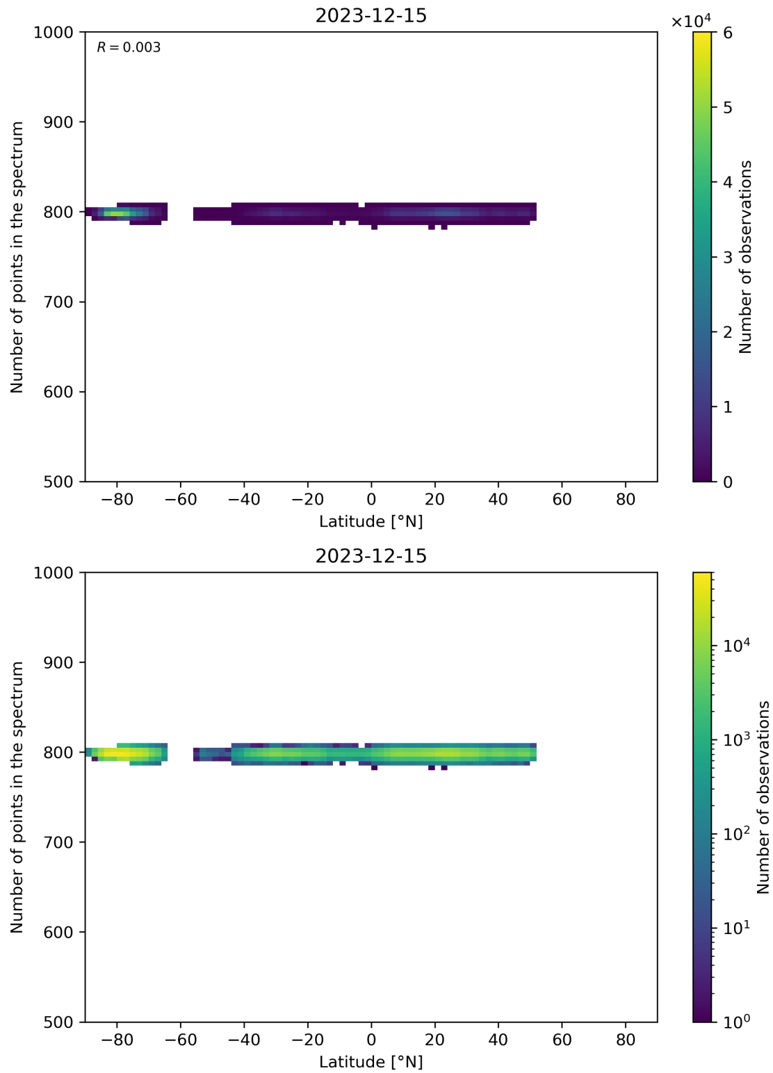
Figure 61: Scatter density plot of “Latitude” against “Number of points in the spectrum” for 2023-12-14 to 2023-12-16.
