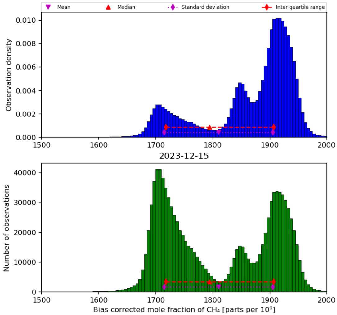
Figure 25: Histogram of “Bias corrected mole fraction of CH 4 ” for 2023-12-14 to 2023-12-16
