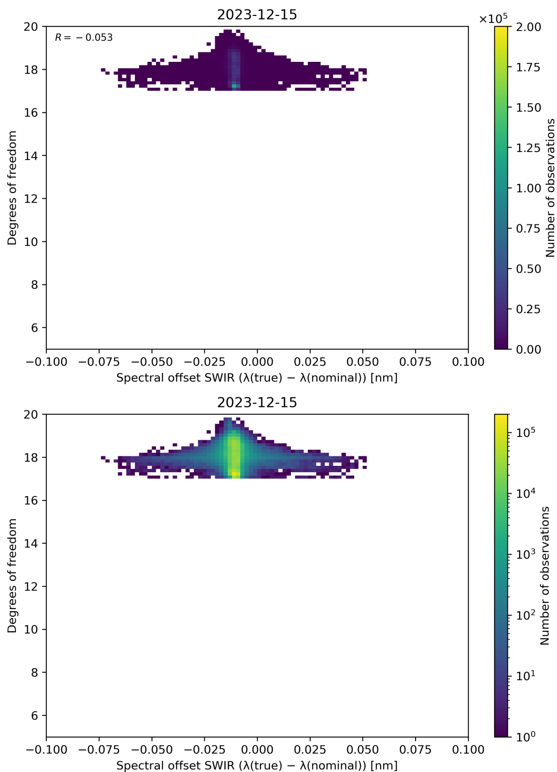
Figure 119: Scatter density plot of “Spectral offset SWIR ( \lambda(\text{true}) - \lambda(\text{nominal}) )” against “Degrees of freedom” for 2023-12-14 to 2023-12-16.
