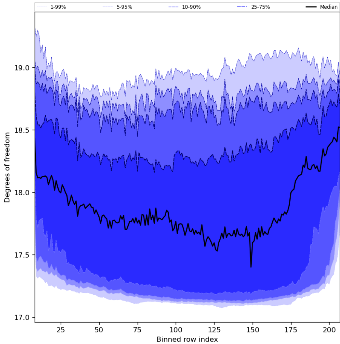
Figure 41: Along track statistics of “Degrees of freedom” for 2023-12-14 to 2023-12-16
