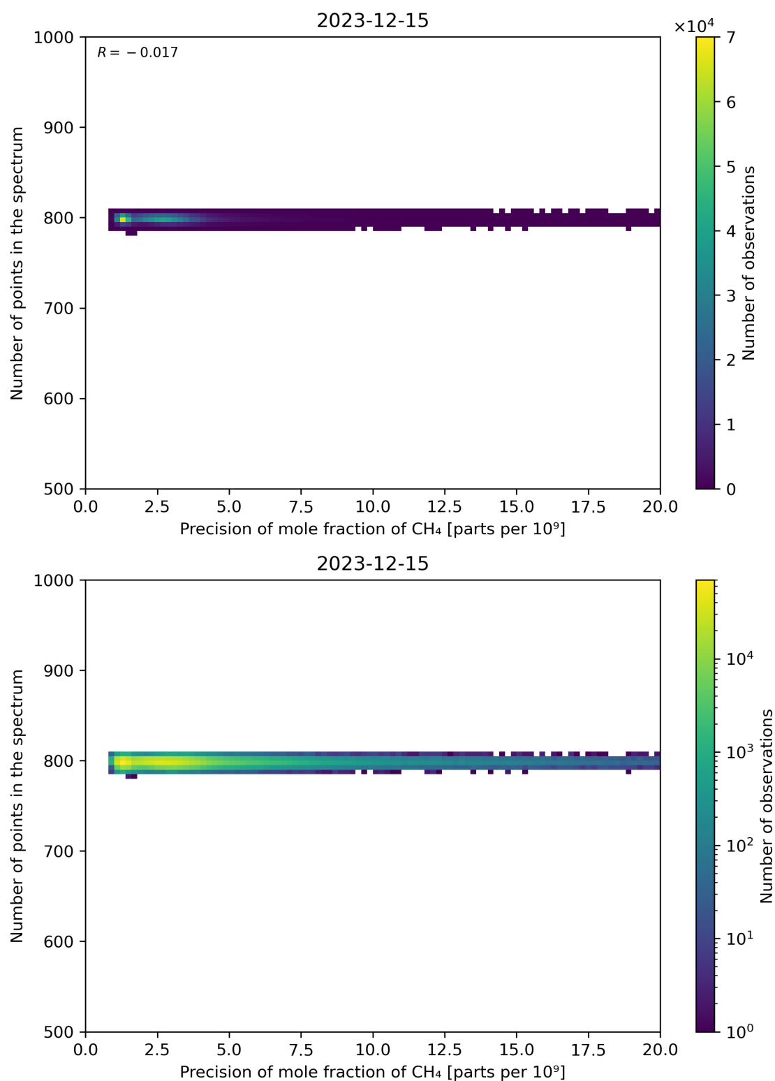
Figure 84: Scatter density plot of “Precision of mole fraction of CH 4 ” against “Number of points in the spectrum” for 2023-12-14 to 2023-12-16.
