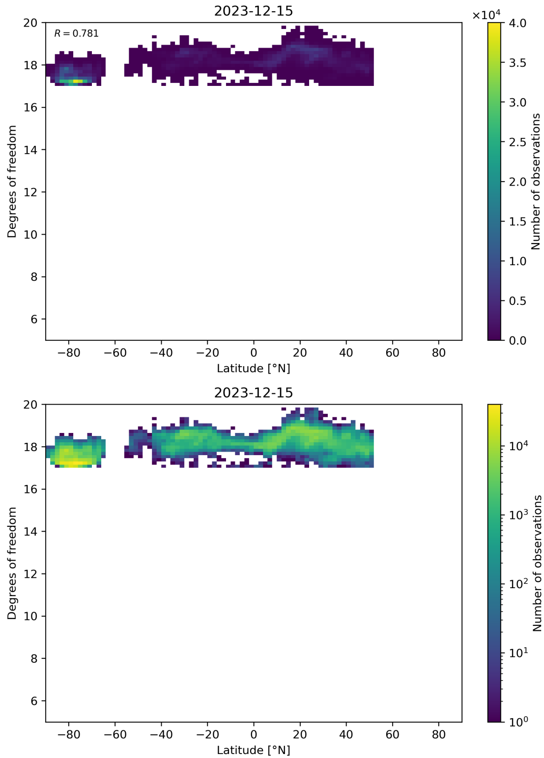
Figure 55: Scatter density plot of “Latitude” against “Degrees of freedom” for 2023-12-14 to 2023-12-16.
