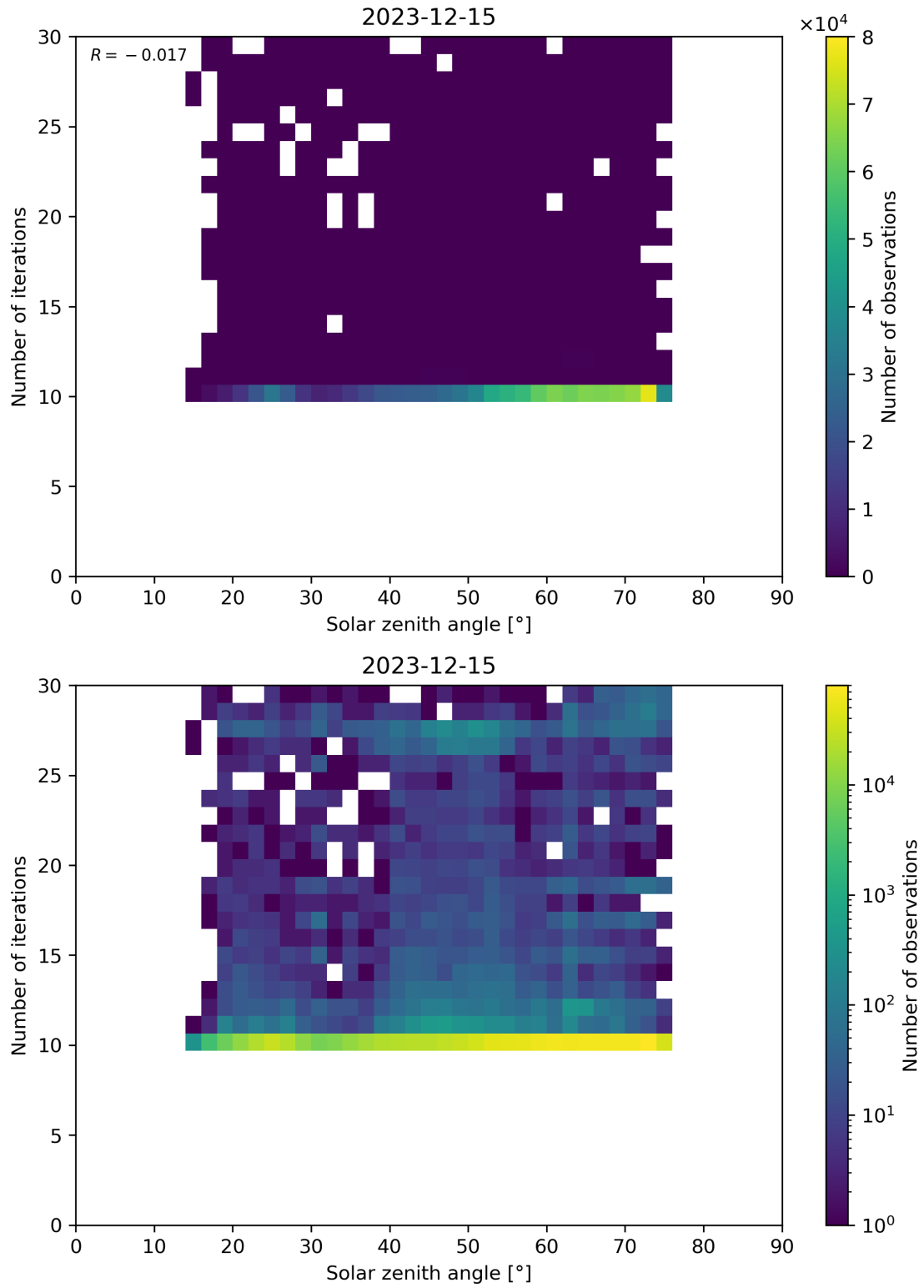
Figure 102: Scatter density plot of “Solar zenith angle” against “Number of iterations” for 2023-12-14 to 2023-12-16.
