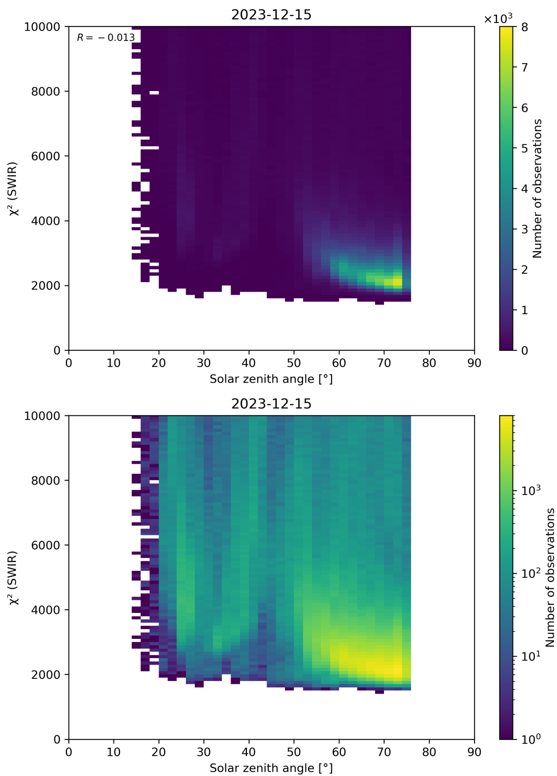
Figure 95: Scatter density plot of “Solar zenith angle” against “ \chi^2 (SWIR)” for 2023-12-14 to 2023-12-16.
