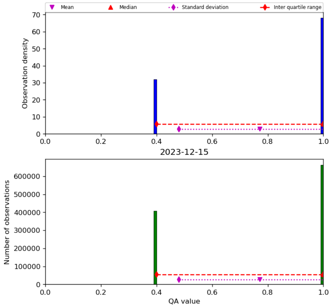
Figure 22: Histogram of “QA value” for 2023-12-14 to 2023-12-16
