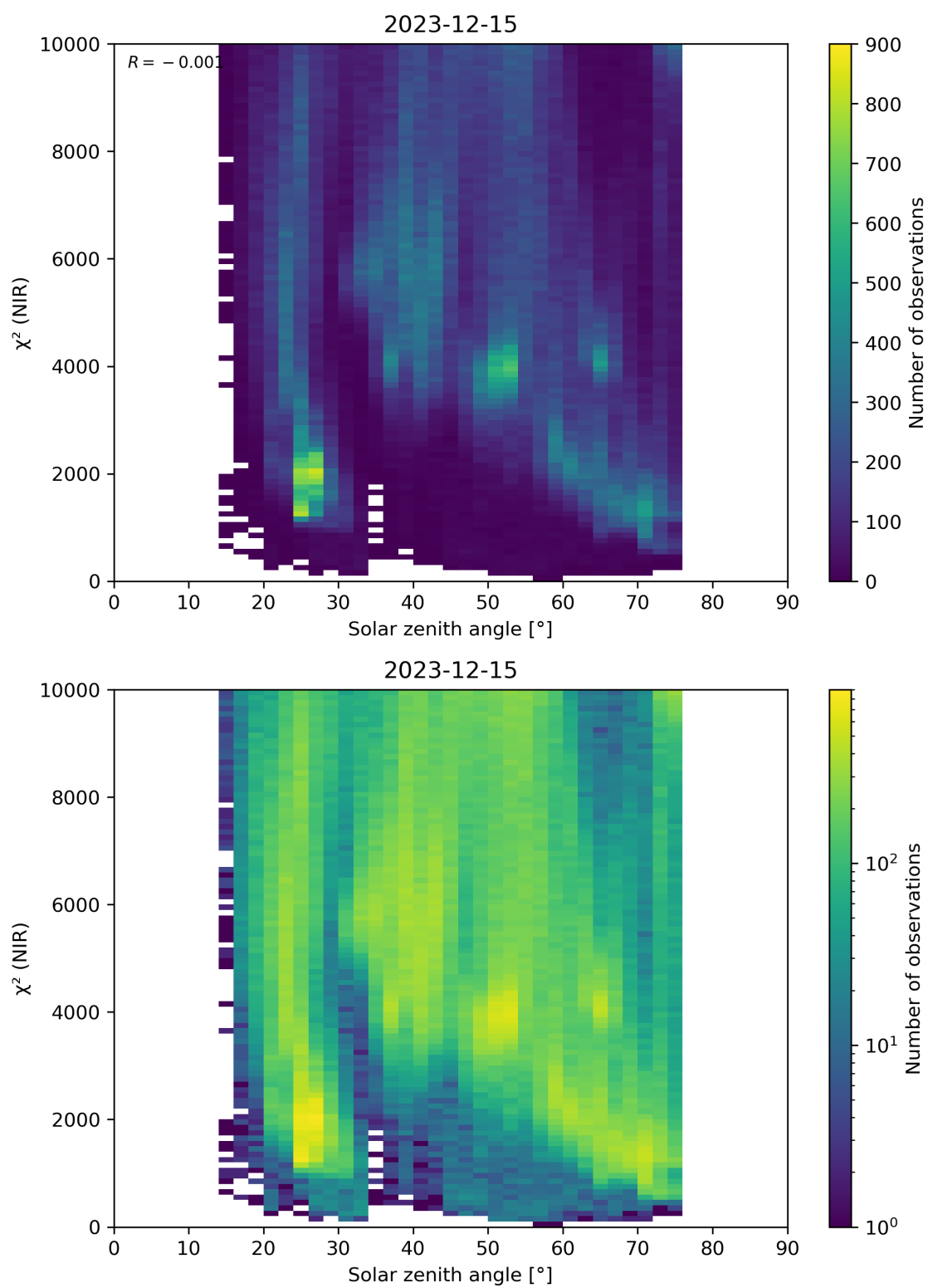
Figure 94: Scatter density plot of “Solar zenith angle” against “ \chi^2 (NIR)” for 2023-12-14 to 2023-12-16.
