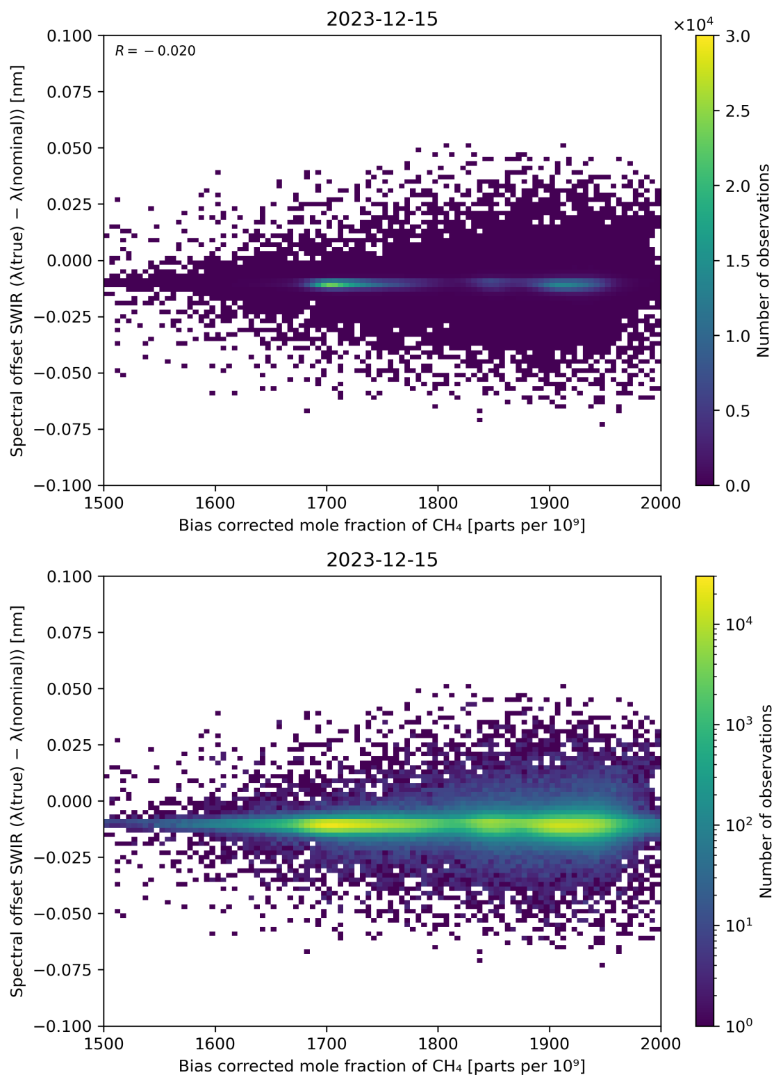
Figure 69: Scatter density plot of “Bias corrected mole fraction of \text{CH}_4 ” against “Spectral offset SWIR ( \lambda(\text{true}) - \lambda(\text{nominal}) )” for 2023-12-14 to 2023-12-16.
