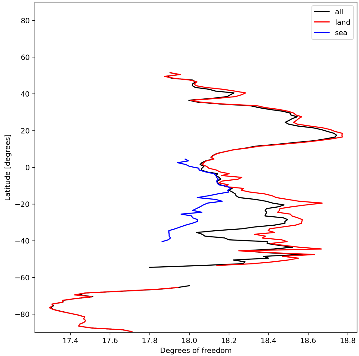
Figure 19: Zonal average of “Degrees of freedom” for 2023-12-14 to 2023-12-16.
