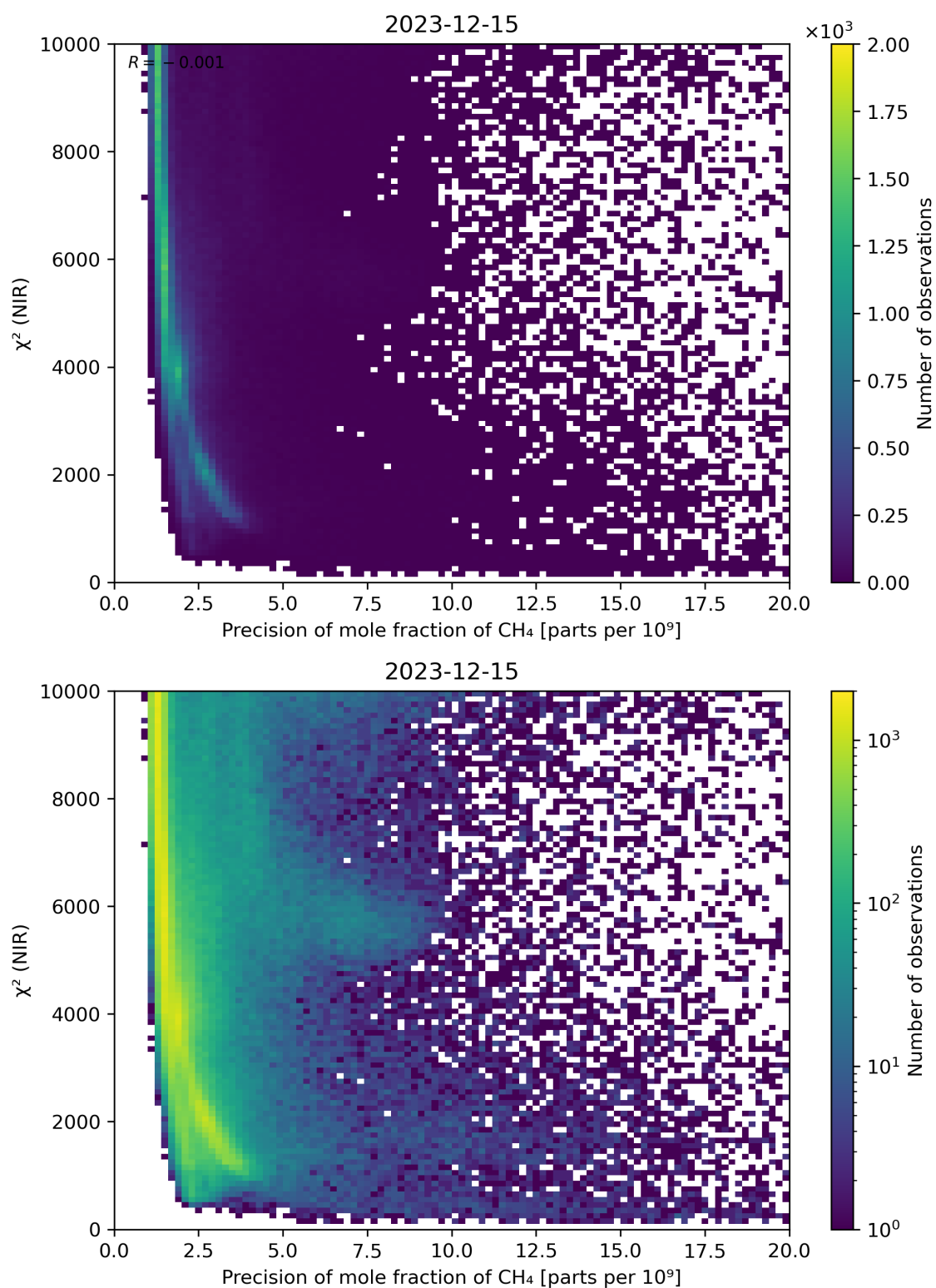
Figure 78: Scatter density plot of “Precision of mole fraction of CH 4 ” against “ \chi^2 (NIR)” for 2023-12-14 to 2023-12-16.
