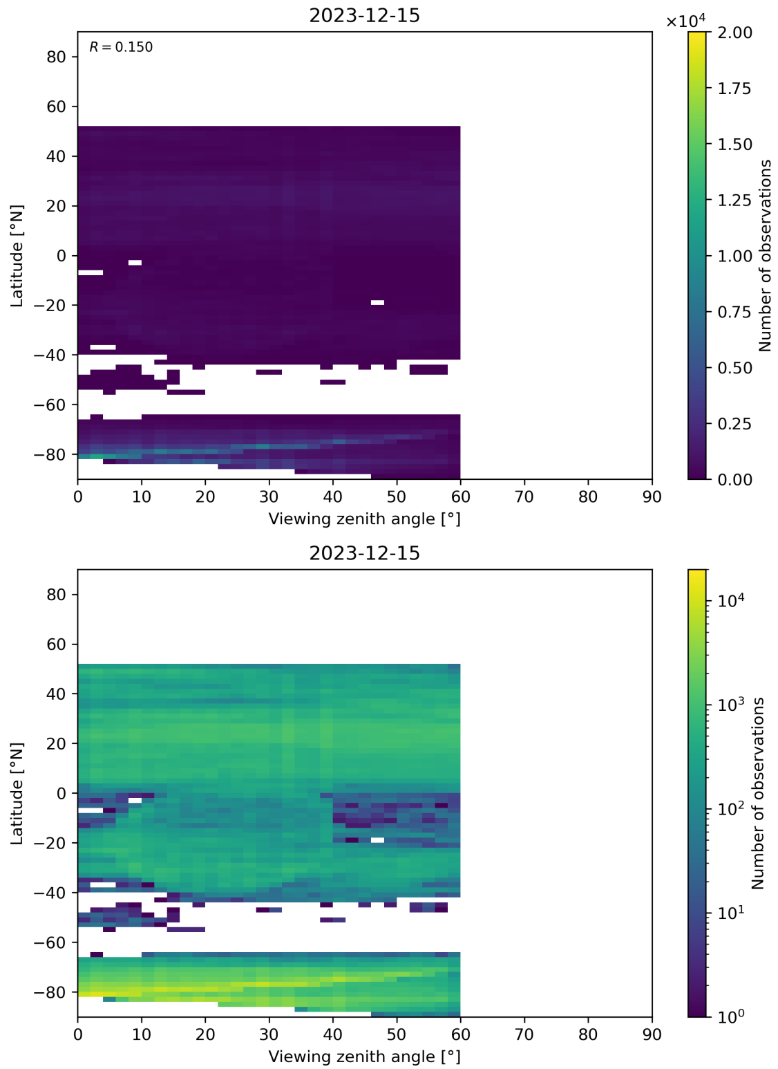
Figure 109: Scatter density plot of “Viewing zenith angle” against “Latitude” for 2023-12-14 to 2023-12-16.
