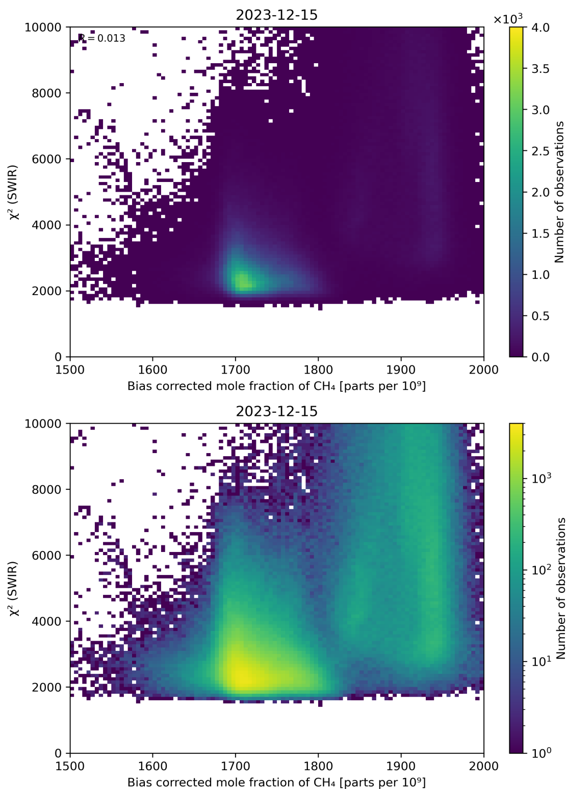
Figure 64: Scatter density plot of “Bias corrected mole fraction of CH 4 ” against “ \chi^2 (SWIR)” for 2023-12-14 to 2023-12-16.
