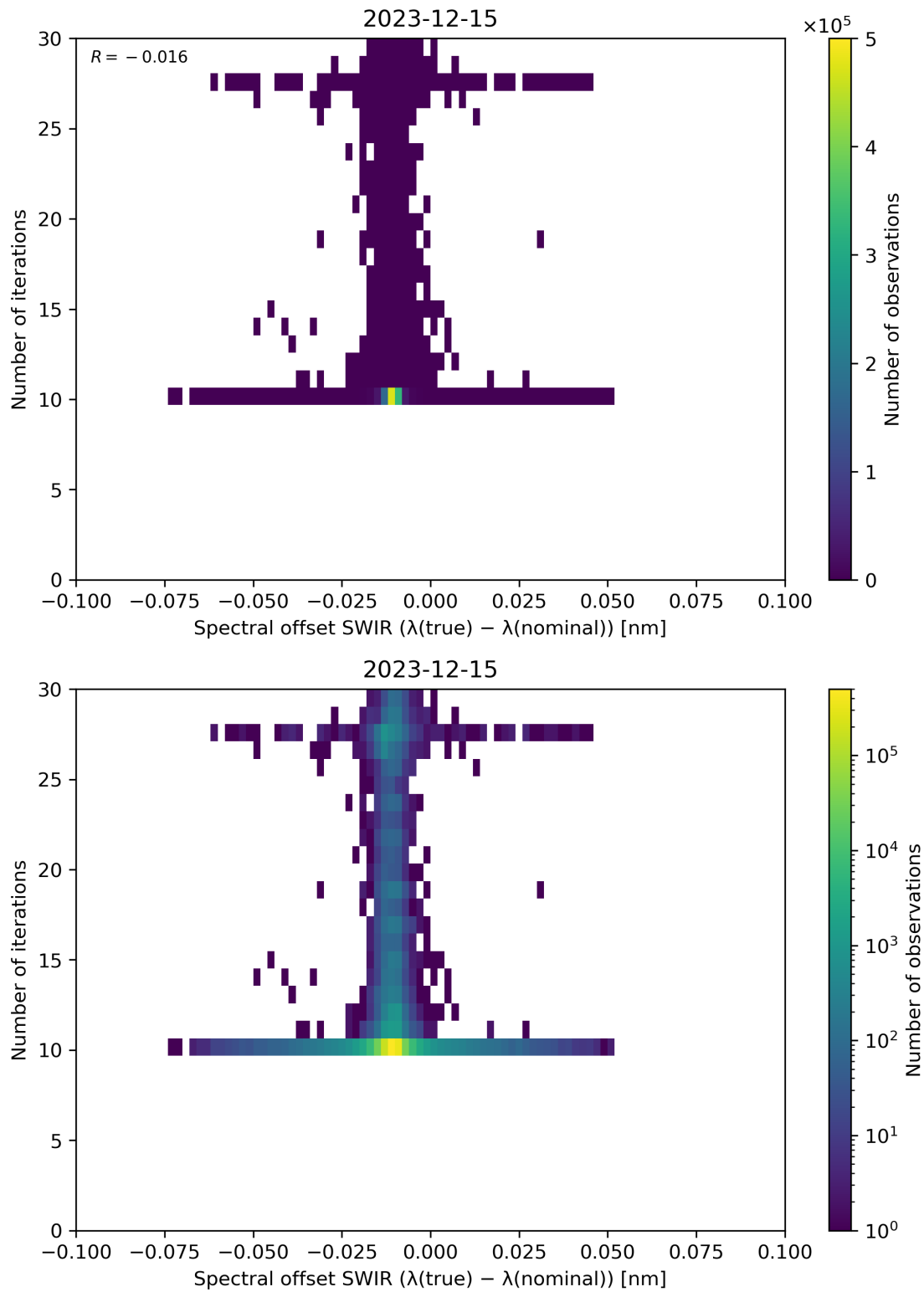
Figure 121: Scatter density plot of “Spectral offset SWIR ( \lambda(\text{true}) - \lambda(\text{nominal}) )” against “Number of iterations” for 2023-12-14 to 2023-12-16.
