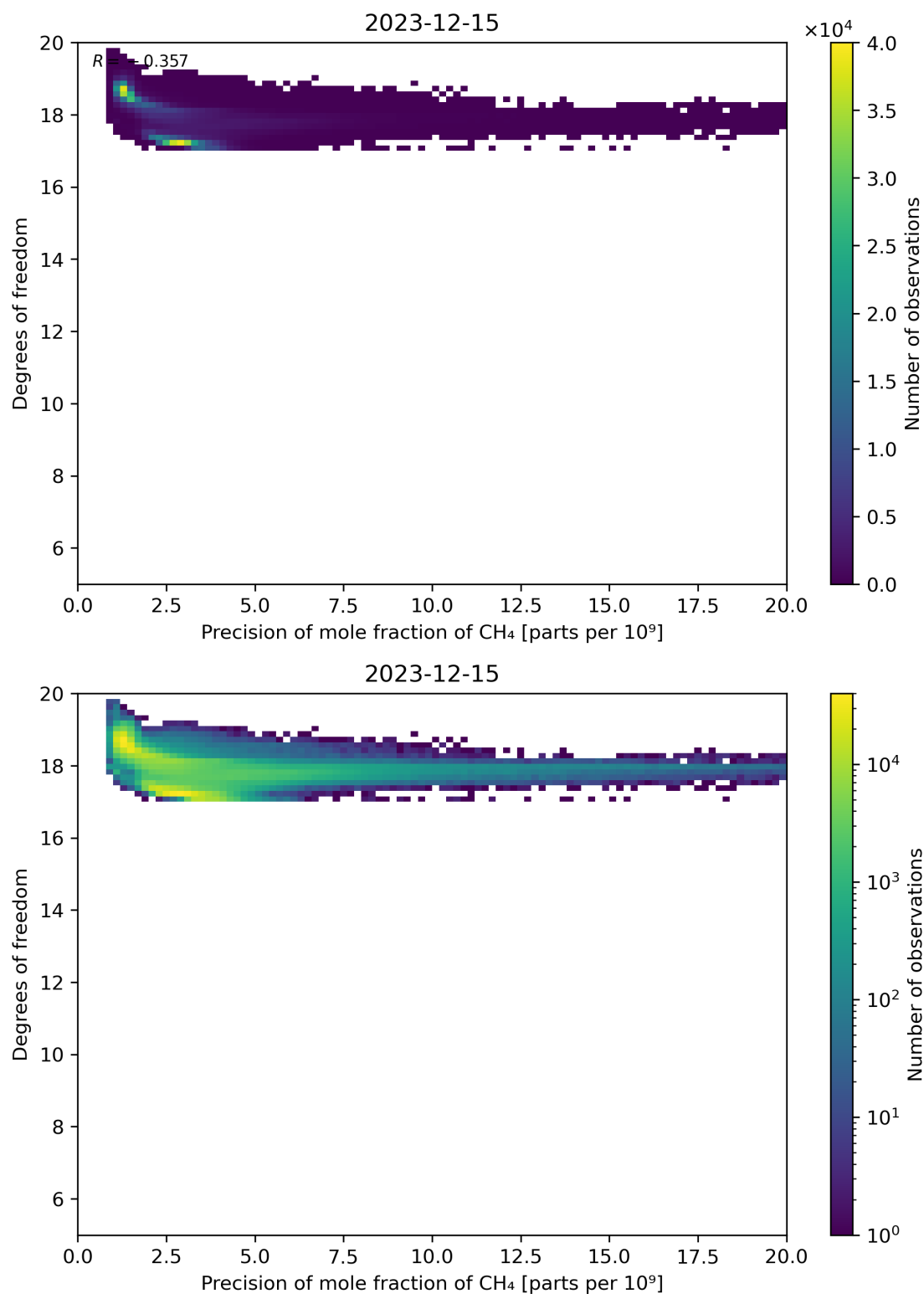
Figure 80: Scatter density plot of “Precision of mole fraction of CH 4 ” against “Degrees of freedom” for 2023-12-14 to 2023-12-16.
