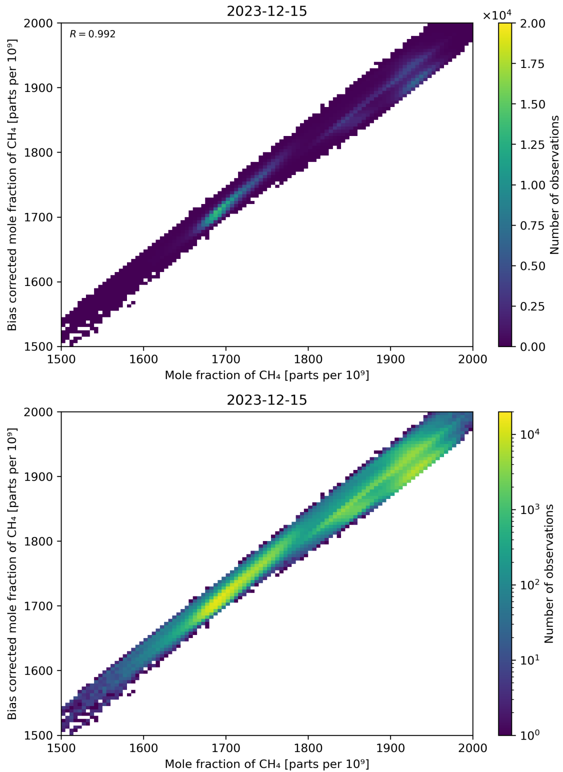
Figure 74: Scatter density plot of “Mole fraction of CH 4 ” against “Bias corrected mole fraction of CH 4 ” for 2023-12-14 to 2023-12-16.
