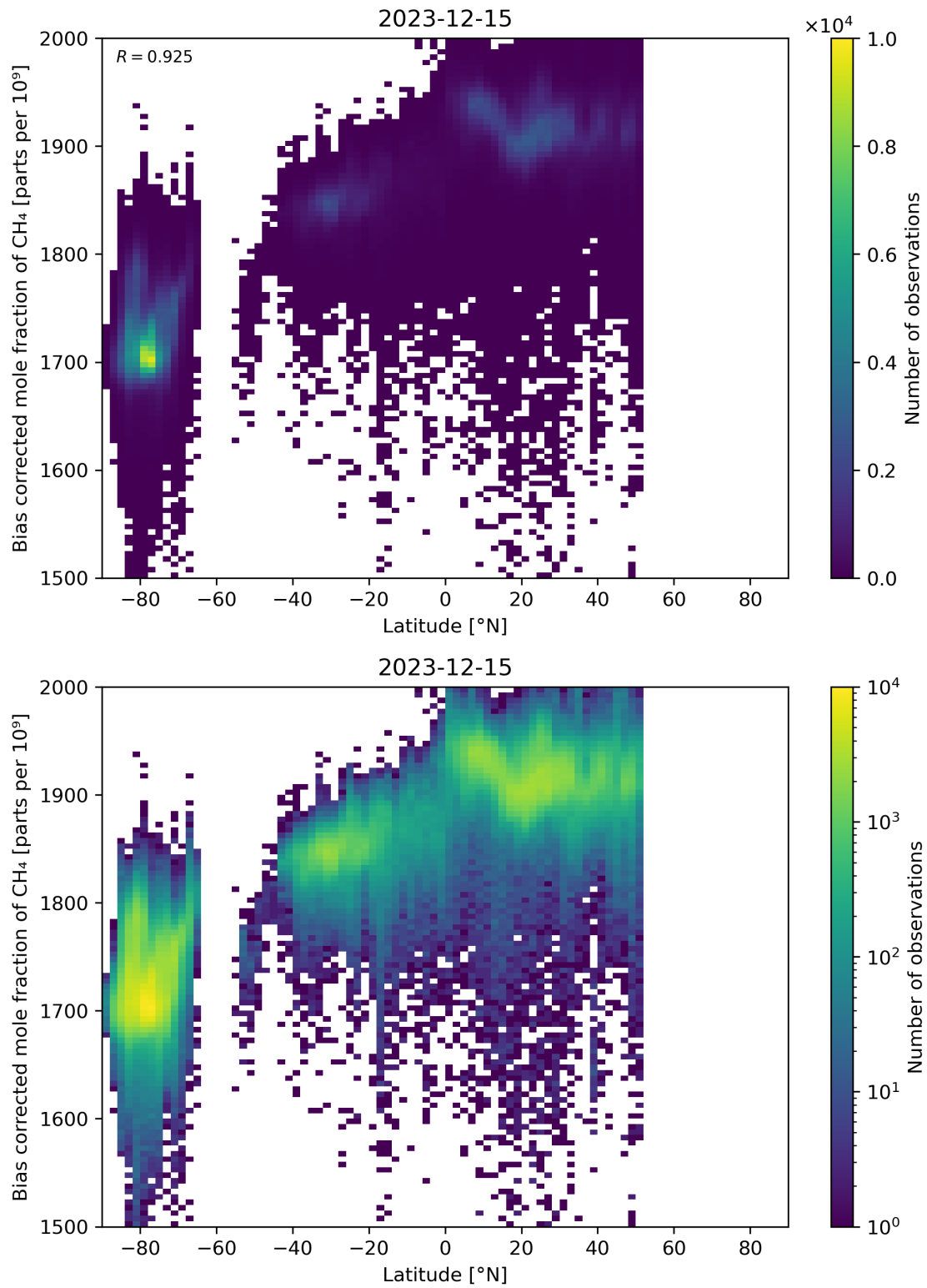
Figure 58: Scatter density plot of “Latitude” against “Bias corrected mole fraction of CH 4 ” for 2023-12-14 to 2023-12-16.
