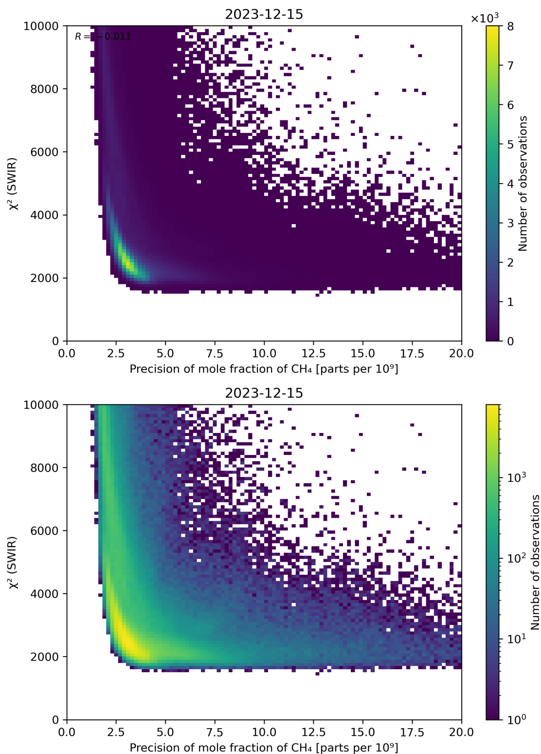
Figure 79: Scatter density plot of “Precision of mole fraction of CH 4 ” against “ \chi^2 (SWIR)” for 2023-12-14 to 2023-12-16.
