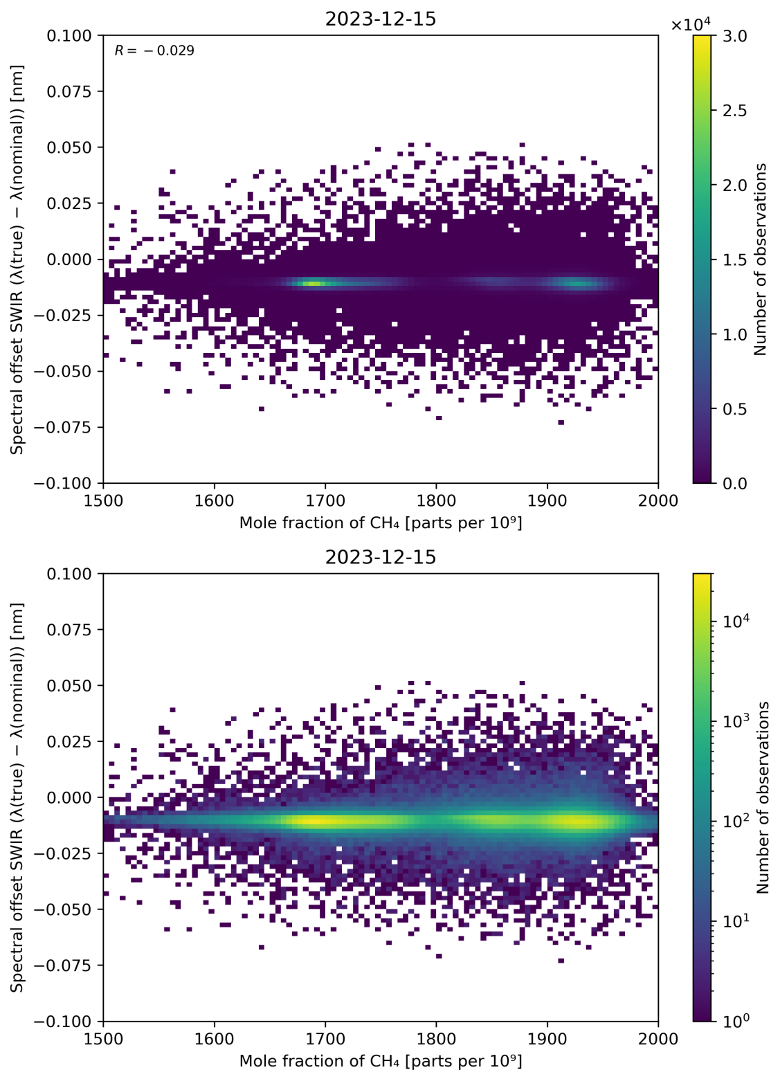
Figure 86: Scatter density plot of “Mole fraction of CH 4 ” against “Spectral offset SWIR ( \lambda(\text{true}) - \lambda(\text{nominal}) )” for 2023-12-14 to 2023-12-16.
