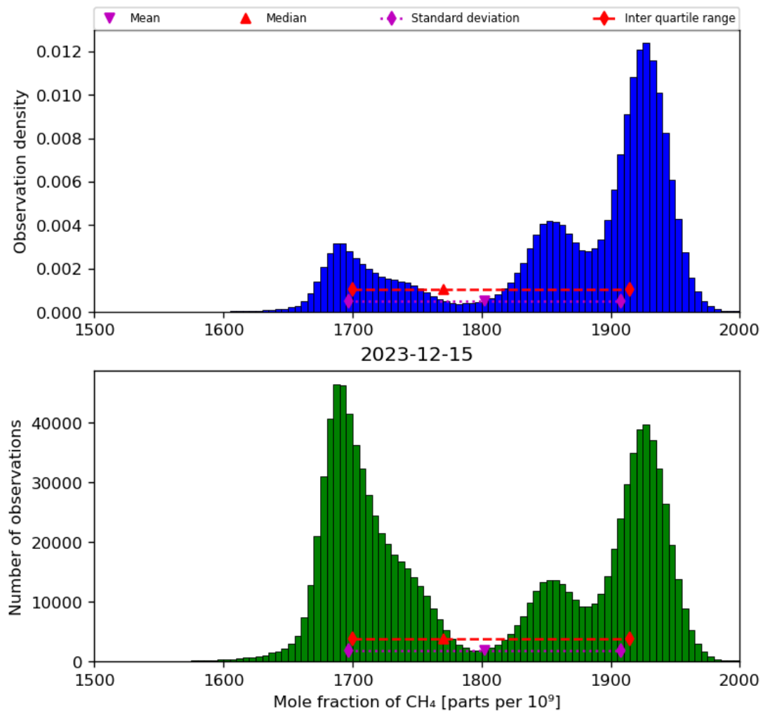
Figure 23: Histogram of “Mole fraction of CH 4 ” for 2023-12-14 to 2023-12-16
