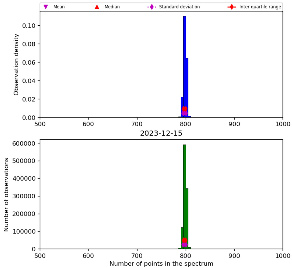
Figure 26: Histogram of “Number of points in the spectrum” for 2023-12-14 to 2023-12-16
