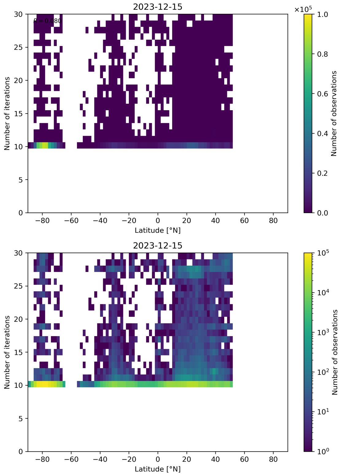
Figure 60: Scatter density plot of “Latitude” against “Number of iterations” for 2023-12-14 to 2023-12-16.
