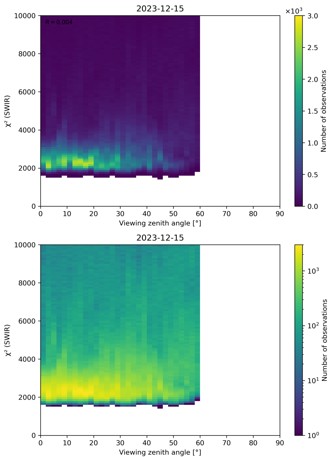
Figure 106: Scatter density plot of “Viewing zenith angle” against “ \chi^2 (SWIR)” for 2023-12-14 to 2023-12-16.
