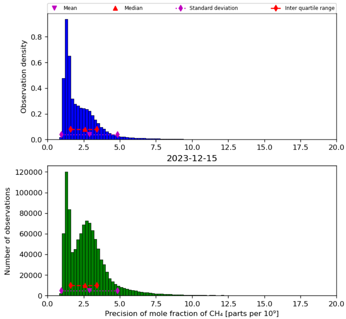
Figure 24: Histogram of “Precision of mole fraction of CH 4 ” for 2023-12-14 to 2023-12-16
