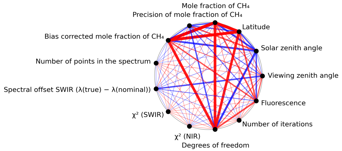
Figure 1: Map of correlation graph for 2023-12-14 to 2023-12-16.
