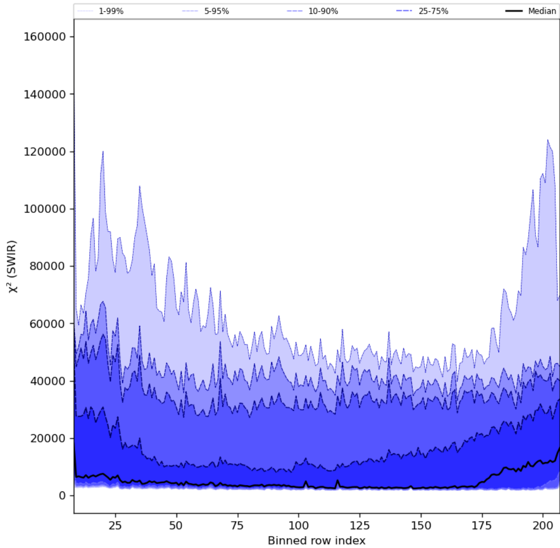
Figure 39: Along track statistics of “ \chi^2 (SWIR)” for 2023-12-14 to 2023-12-16
