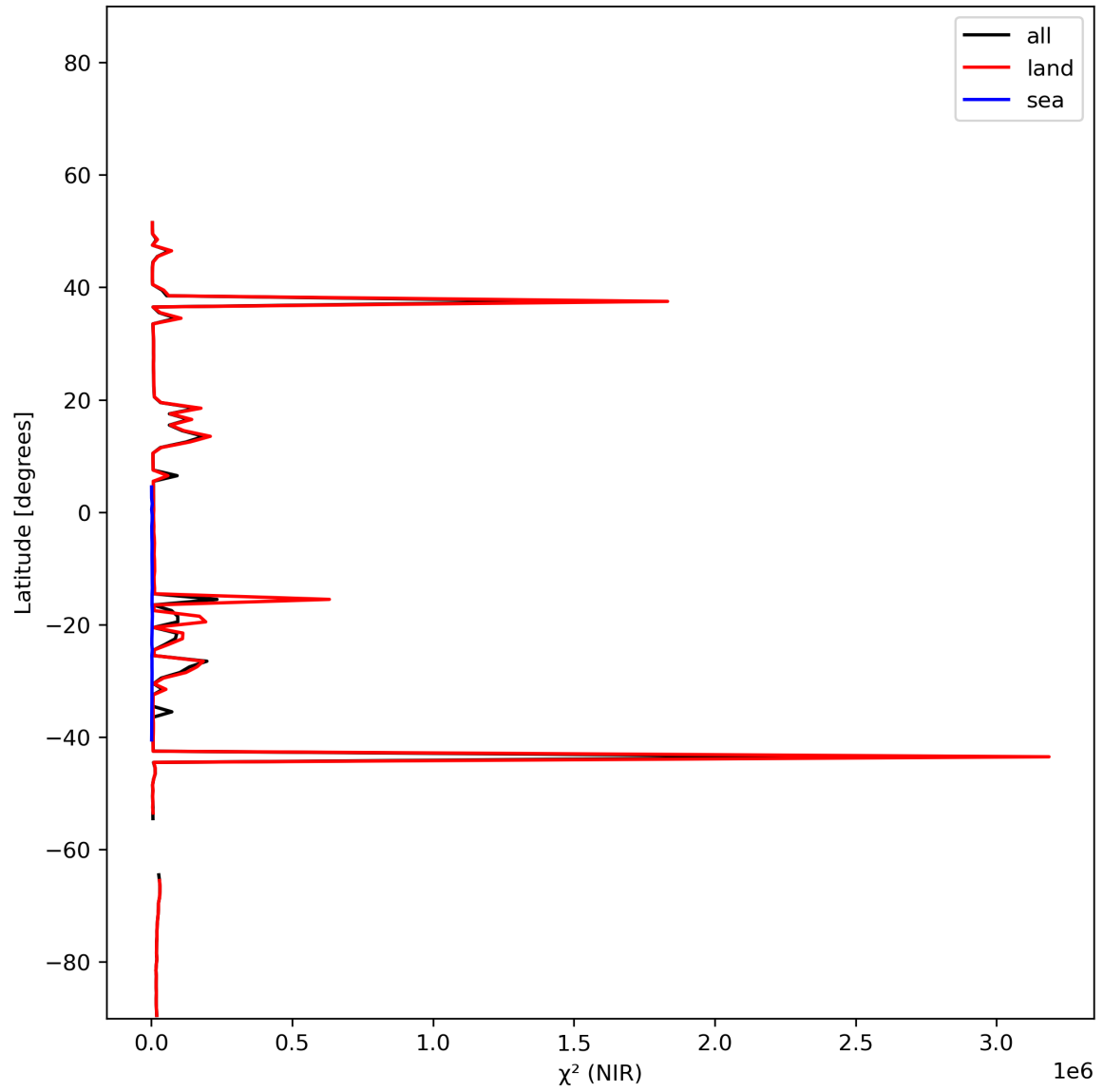
Figure 18: Zonal average of “ \chi^2 (NIR)” for 2023-12-14 to 2023-12-16.
