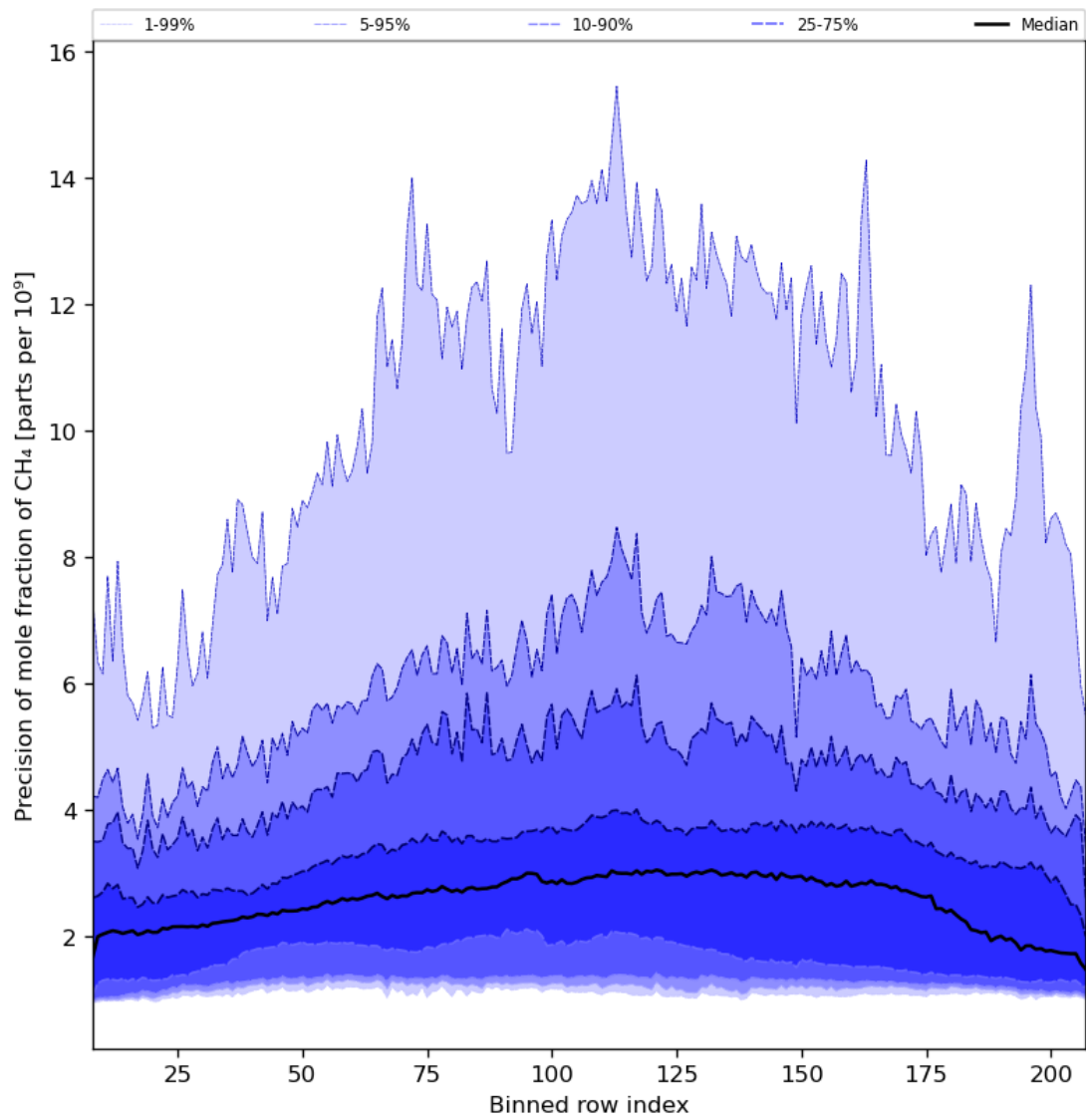
Figure 35: Along track statistics of “Precision of mole fraction of CH 4 ” for 2023-12-14 to 2023-12-16
