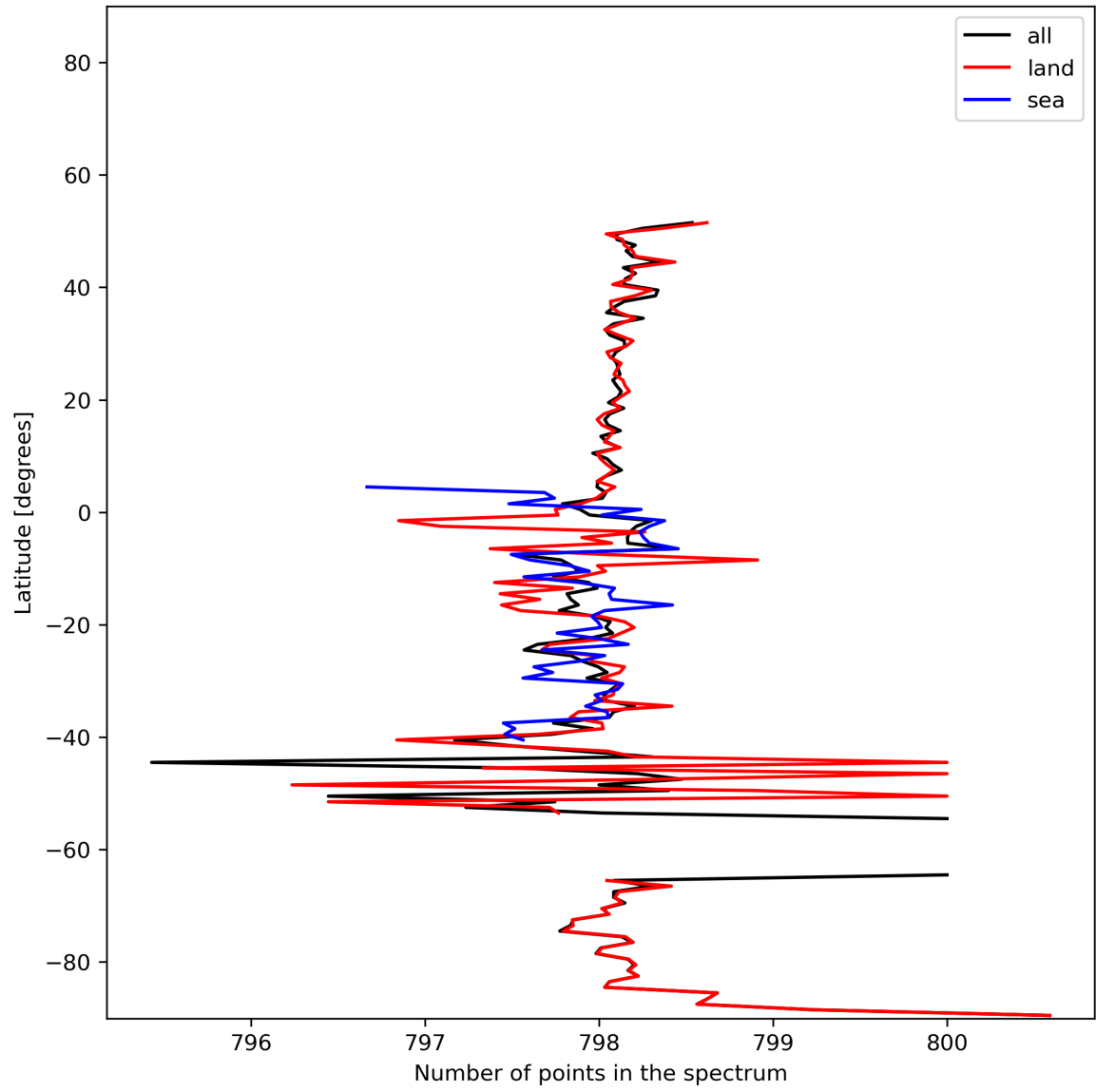
Figure 15: Zonal average of “Number of points in the spectrum” for 2023-12-14 to 2023-12-16.
