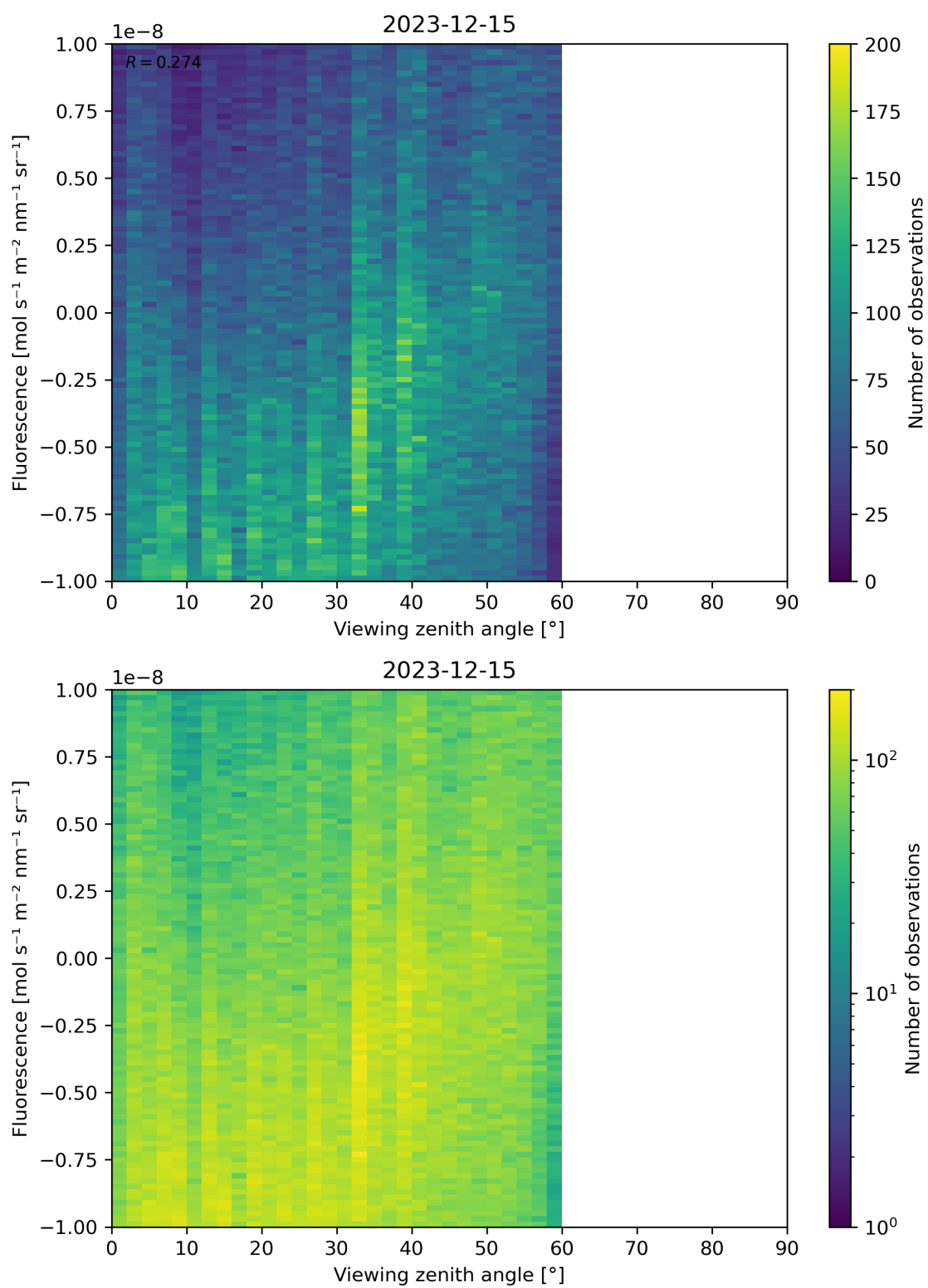
Figure 108: Scatter density plot of “Viewing zenith angle” against “Fluorescence” for 2023-12-14 to 2023-12-16.
