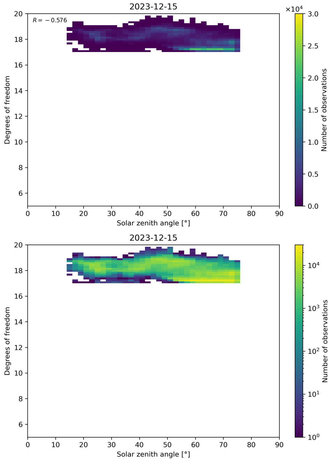
Figure 96: Scatter density plot of “Solar zenith angle” against “Degrees of freedom” for 2023-12-14 to 2023-12-16.
