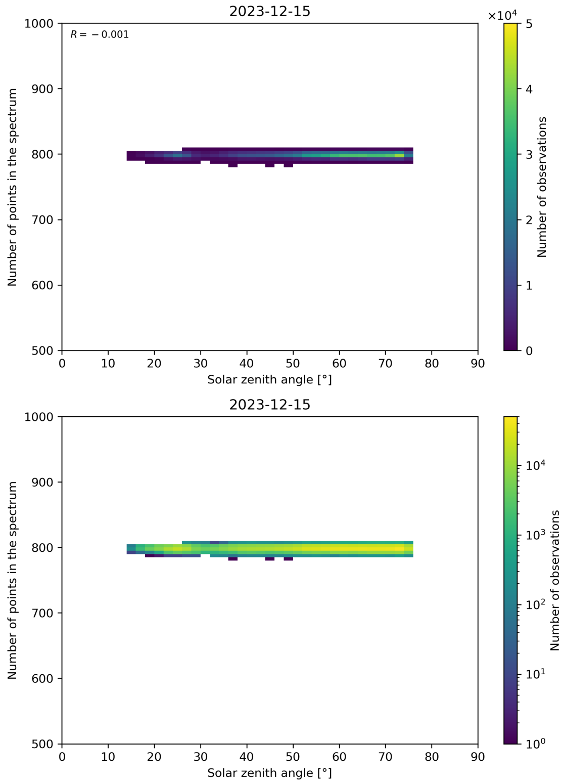
Figure 103: Scatter density plot of “Solar zenith angle” against “Number of points in the spectrum” for 2023-12-14 to 2023-12-16.
