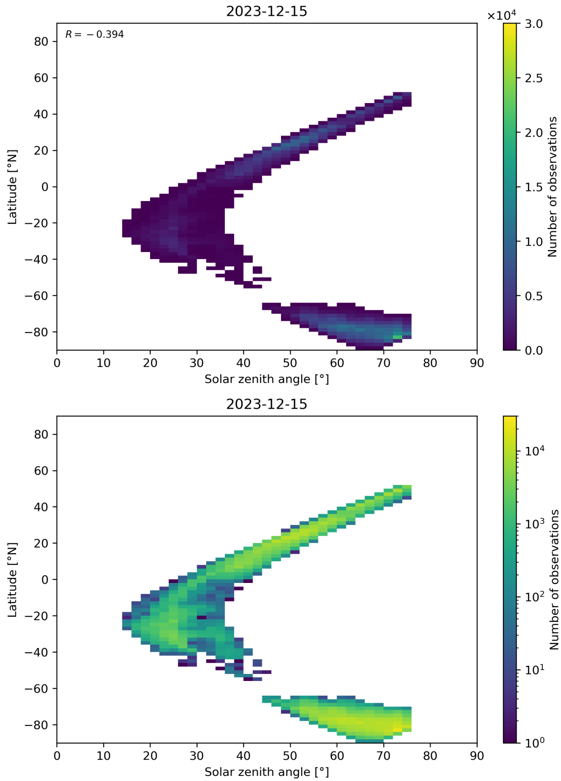
Figure 98: Scatter density plot of “Solar zenith angle” against “Latitude” for 2023-12-14 to 2023-12-16.
