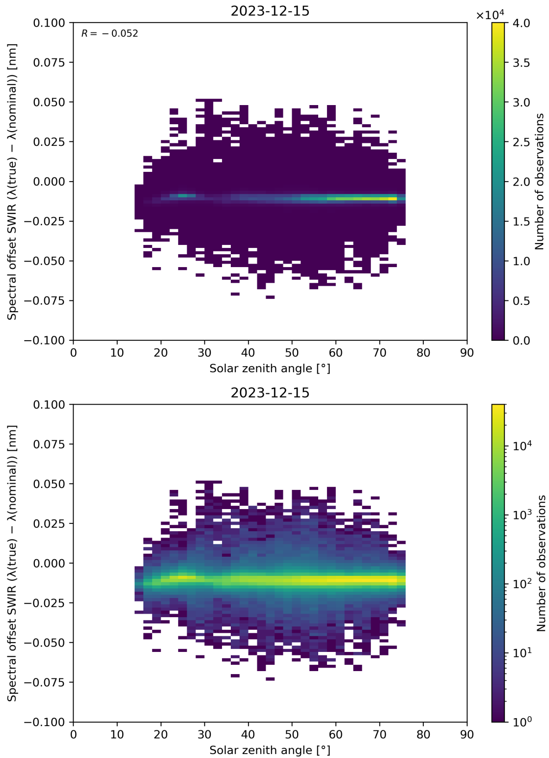
Figure 104: Scatter density plot of “Solar zenith angle” against “Spectral offset SWIR ( \lambda(\text{true}) - \lambda(\text{nominal}) )” for 2023-12-14 to 2023-12-16.
