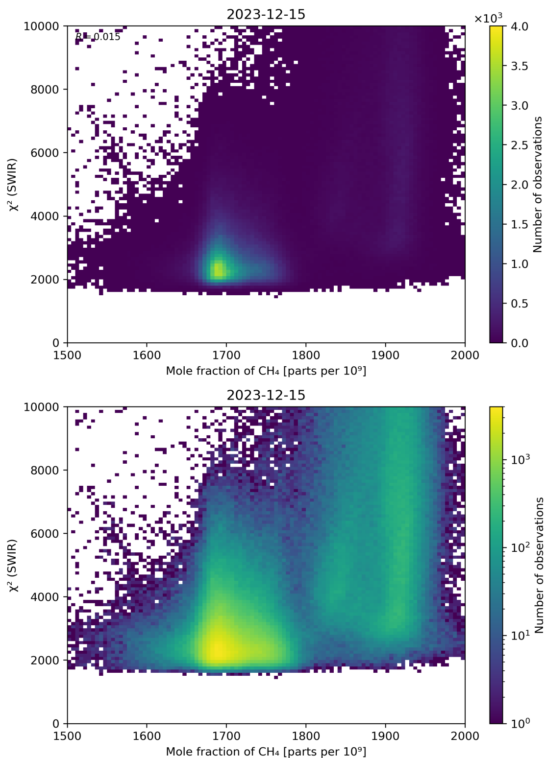
Figure 71: Scatter density plot of “Mole fraction of \text{CH}_4 ” against “ \chi^2 (SWIR)” for 2023-12-14 to 2023-12-16.
