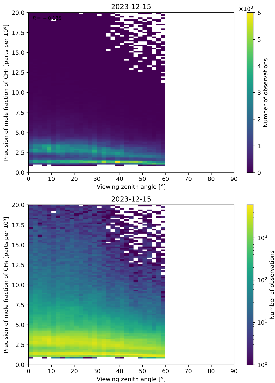
Figure 112: Scatter density plot of “Viewing zenith angle” against “Precision of mole fraction of \text{CH}_4 ” for 2023-12-14 to 2023-12-16.
