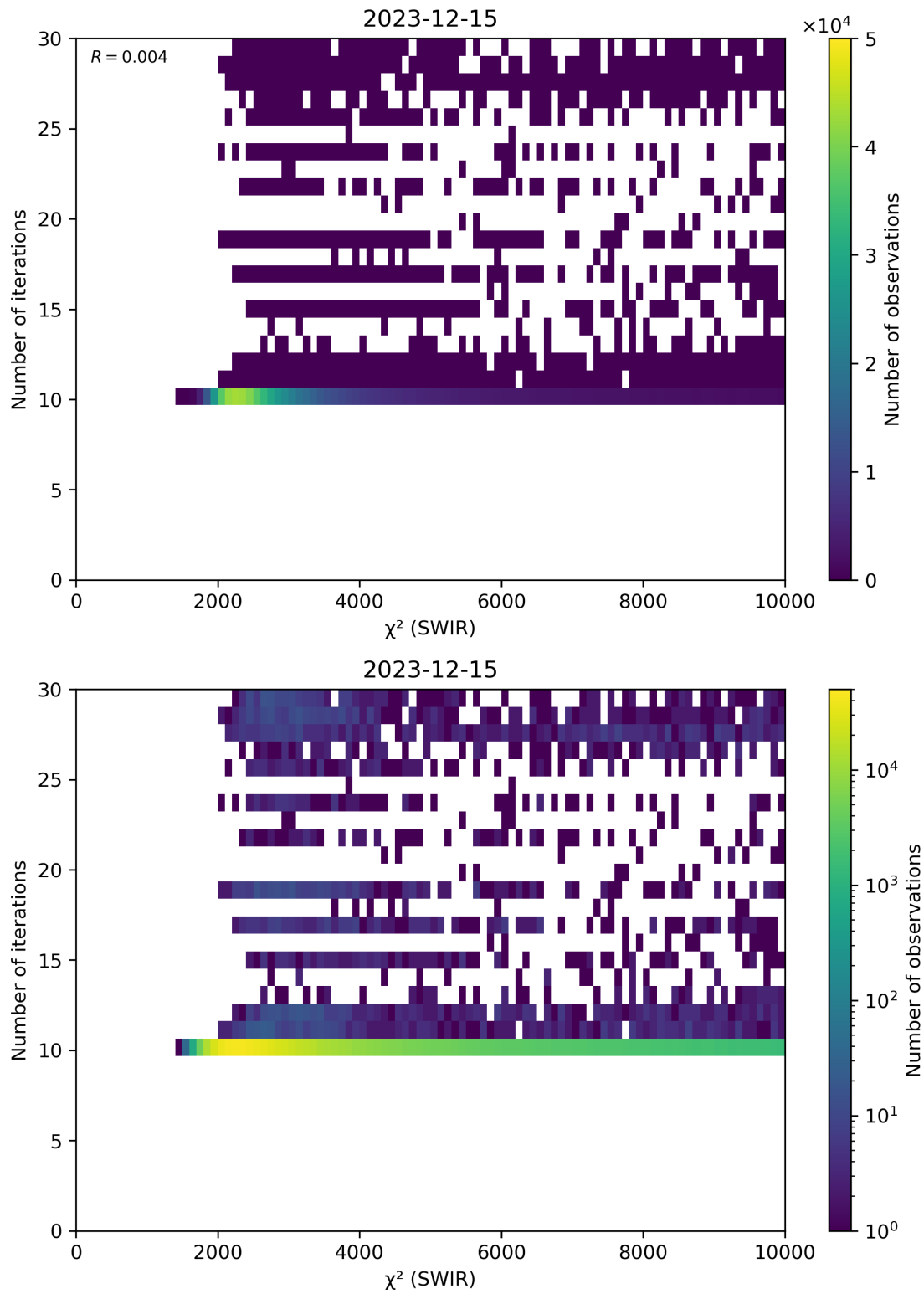
Figure 50: Scatter density plot of “ \chi^2 (SWIR)” against “Number of iterations” for 2023-12-14 to 2023-12-16.
