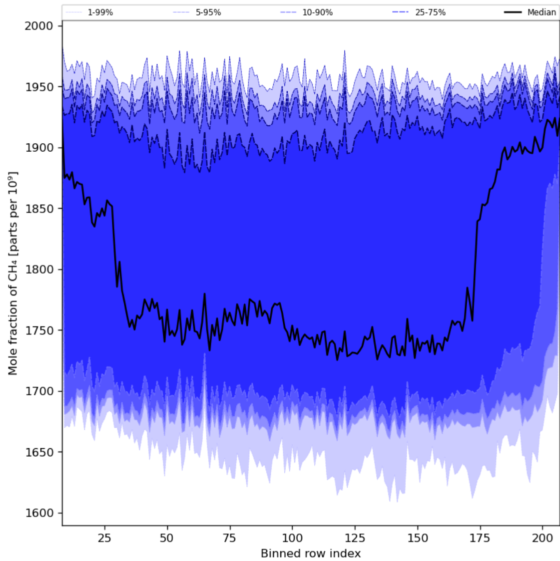
Figure 34: Along track statistics of “Mole fraction of CH 4 ” for 2023-12-14 to 2023-12-16
