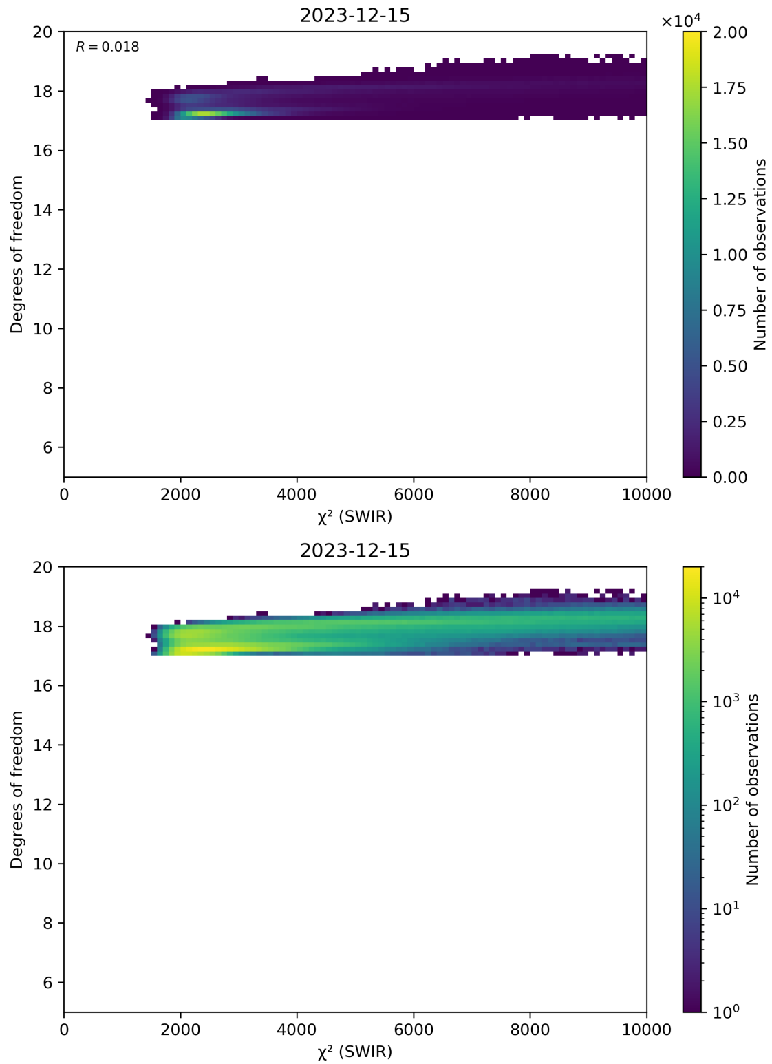
Figure 48: Scatter density plot of “ \chi^2 (SWIR)” against “Degrees of freedom” for 2023-12-14 to 2023-12-16.
