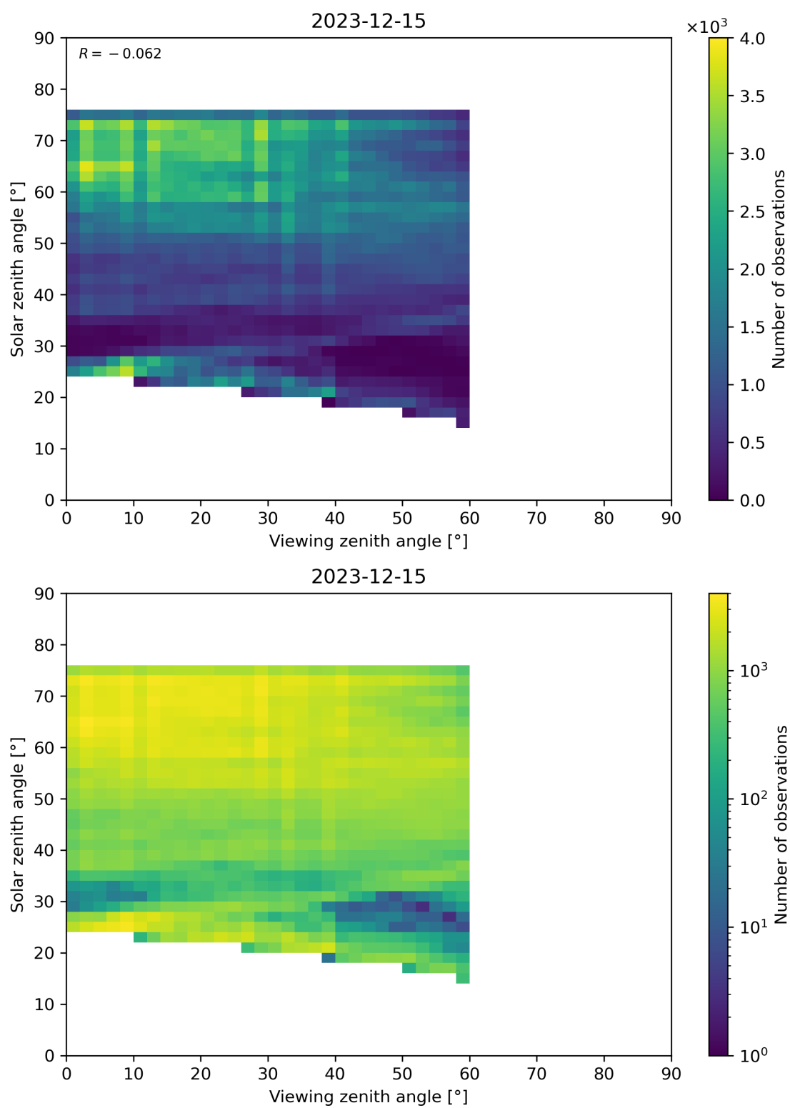
Figure 115: Scatter density plot of “Viewing zenith angle” against “Solar zenith angle” for 2023-12-14 to 2023-12-16.
