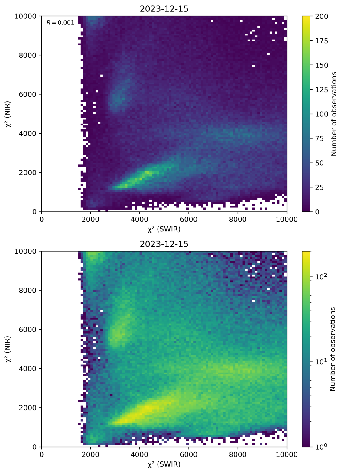
Figure 47: Scatter density plot of “ \chi^2 (SWIR)” against “ \chi^2 (NIR)” for 2023-12-14 to 2023-12-16.
