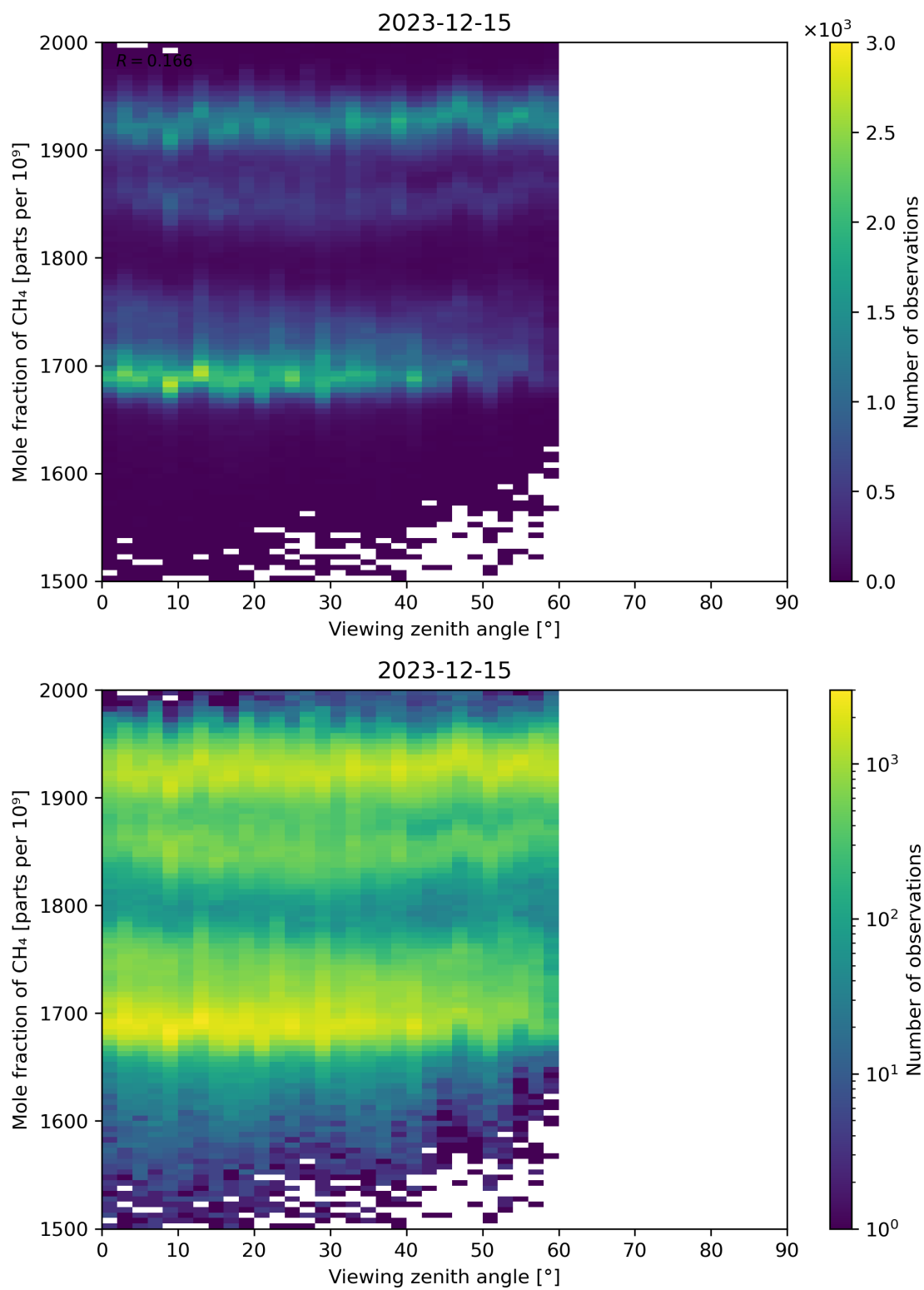
Figure 110: Scatter density plot of “Viewing zenith angle” against “Mole fraction of CH 4 ” for 2023-12-14 to 2023-12-16.
