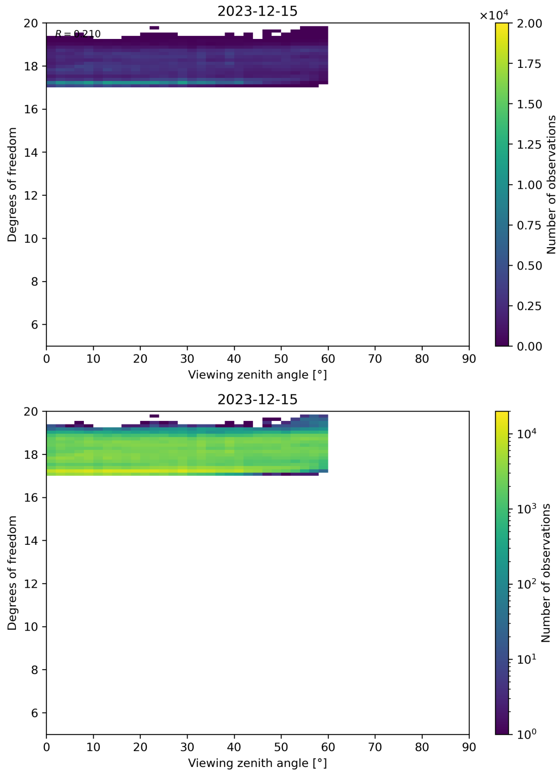
Figure 107: Scatter density plot of “Viewing zenith angle” against “Degrees of freedom” for 2023-12-14 to 2023-12-16.
