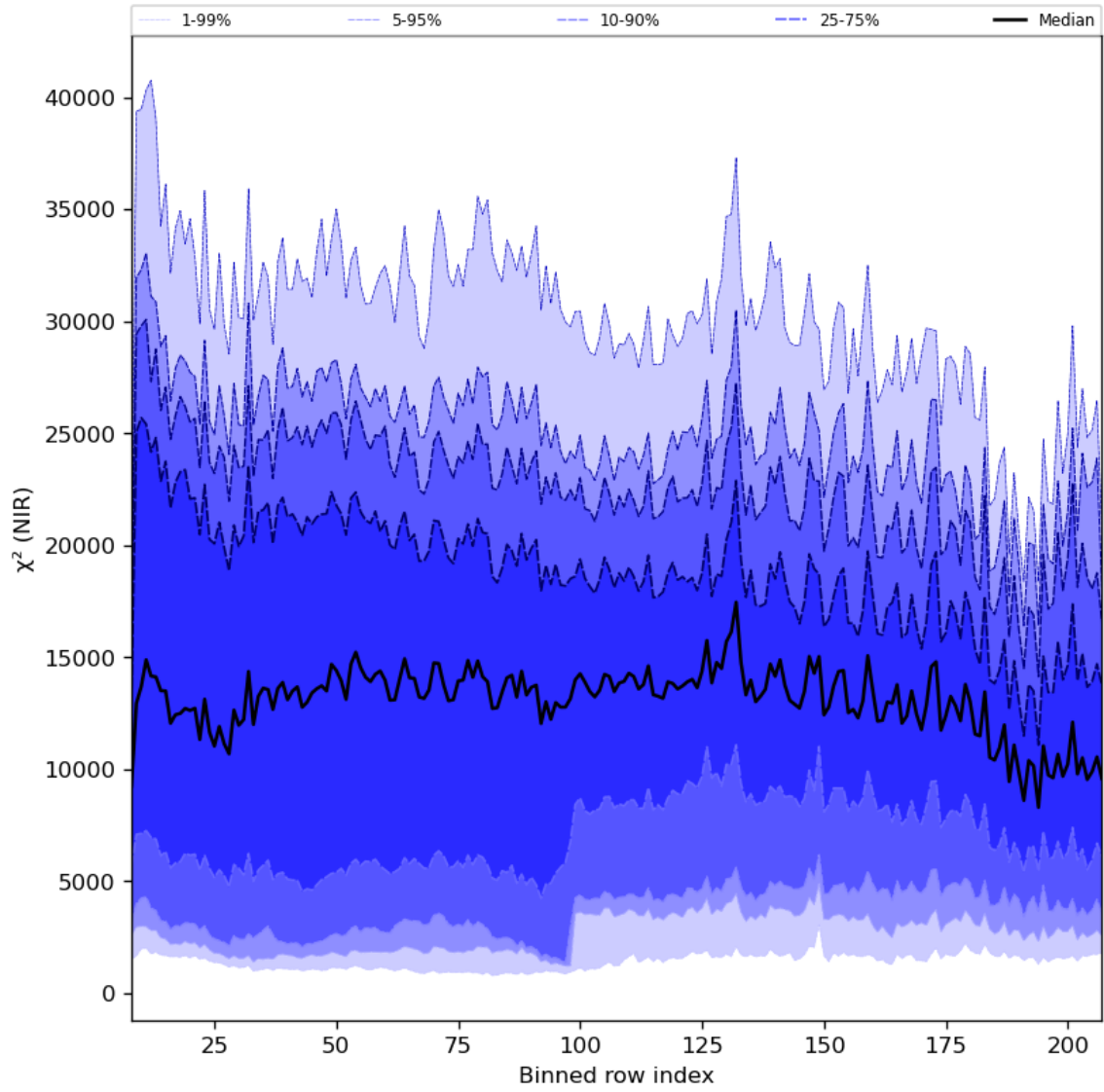
Figure 40: Along track statistics of “ \chi^2 (NIR)” for 2023-12-14 to 2023-12-16
