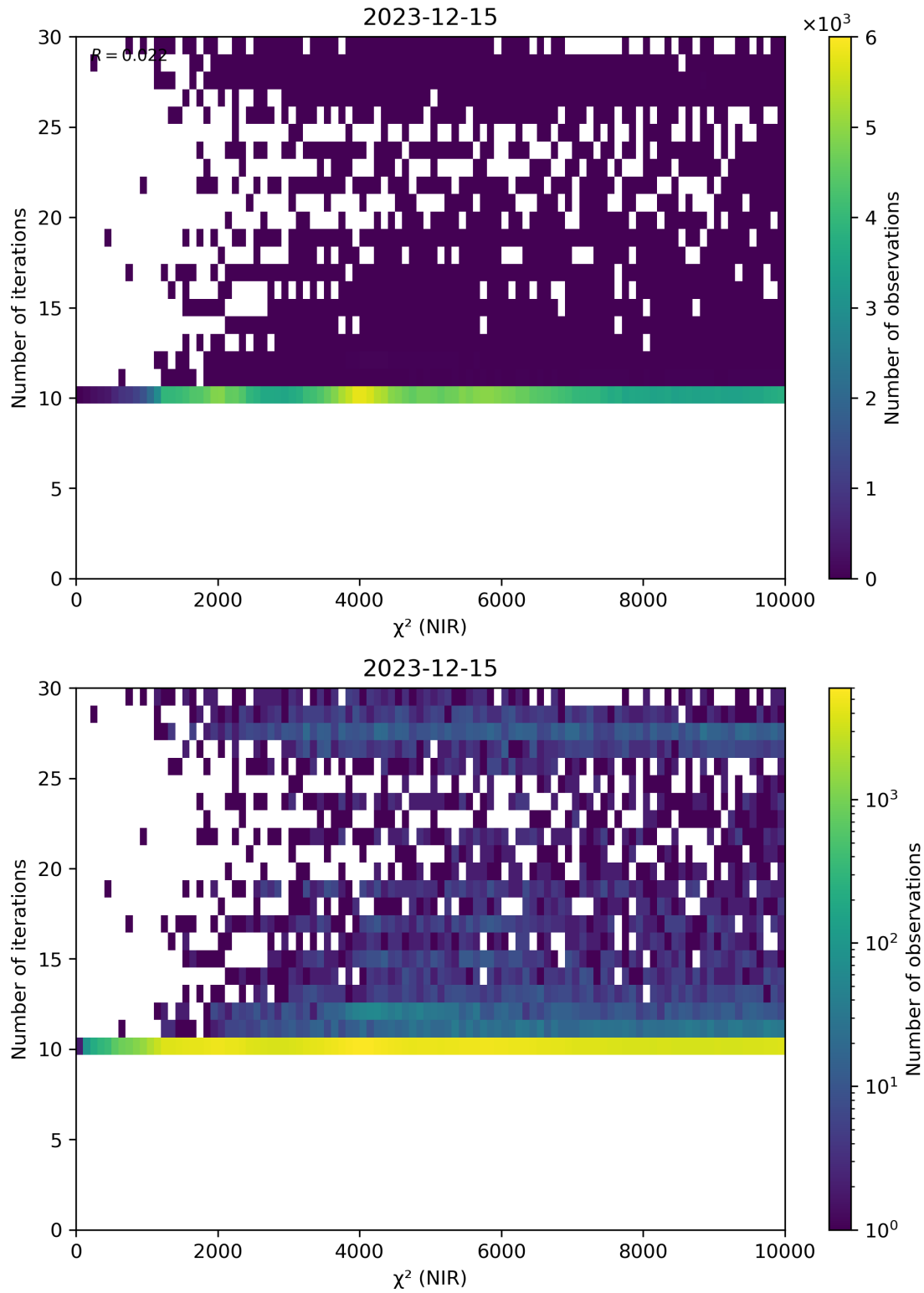
Figure 46: Scatter density plot of “ \chi^2 (NIR)” against “Number of iterations” for 2023-12-14 to 2023-12-16.
