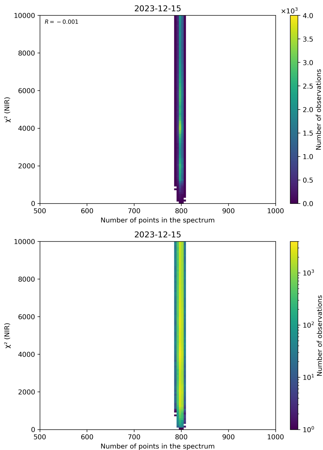
Figure 88: Scatter density plot of “Number of points in the spectrum” against “ \chi^2 (NIR)” for 2023-12-14 to 2023-12-16.
