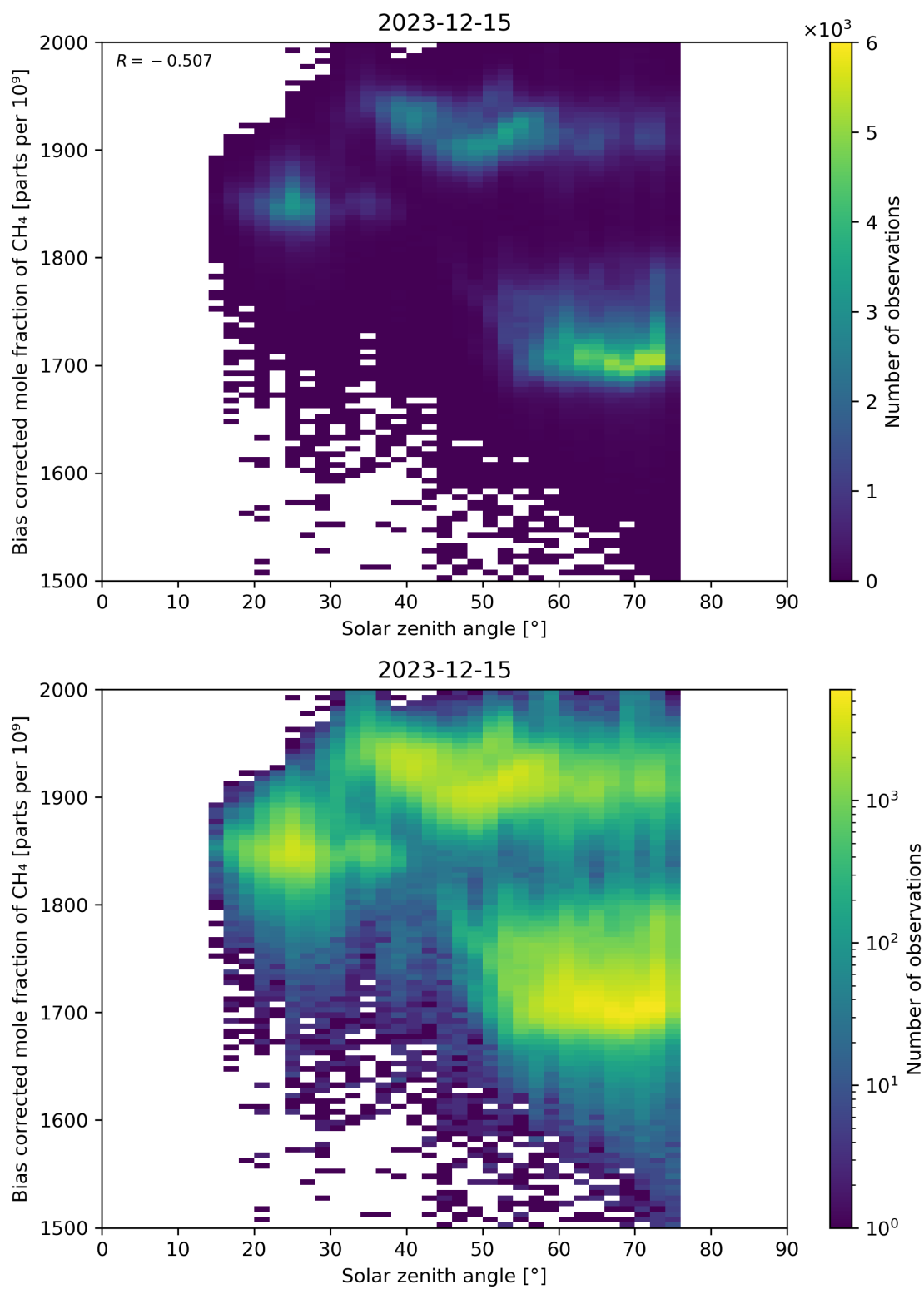
Figure 100: Scatter density plot of “Solar zenith angle” against “Bias corrected mole fraction of CH 4 ” for 2023-12-14 to 2023-12-16.
