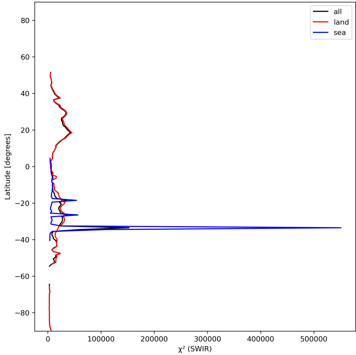
Figure 17: Zonal average of “ \chi^2 (SWIR)” for 2023-12-14 to 2023-12-16.
