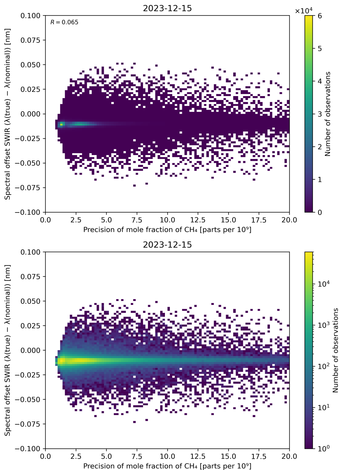
Figure 85: Scatter density plot of “Precision of mole fraction of CH 4 ” against “Spectral offset SWIR ( \lambda(\text{true}) - \lambda(\text{nominal}) )” for 2023-12-14 to 2023-12-16.
