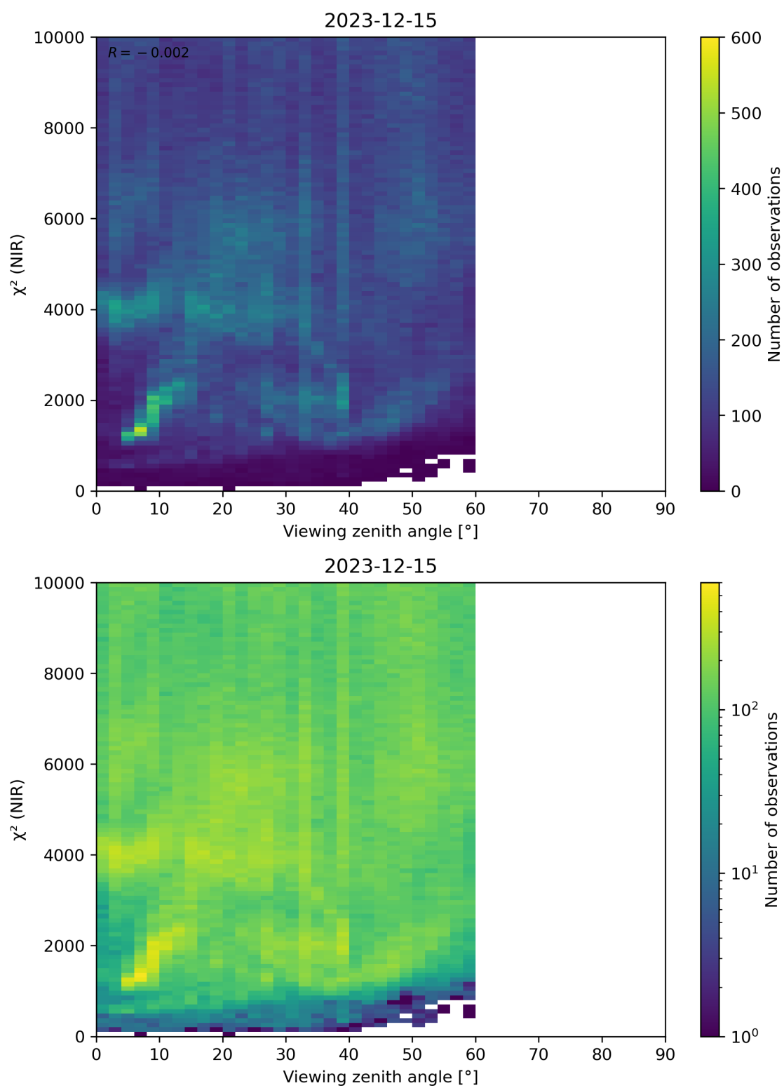
Figure 105: Scatter density plot of “Viewing zenith angle” against “ \chi^2 (NIR)” for 2023-12-14 to 2023-12-16.
