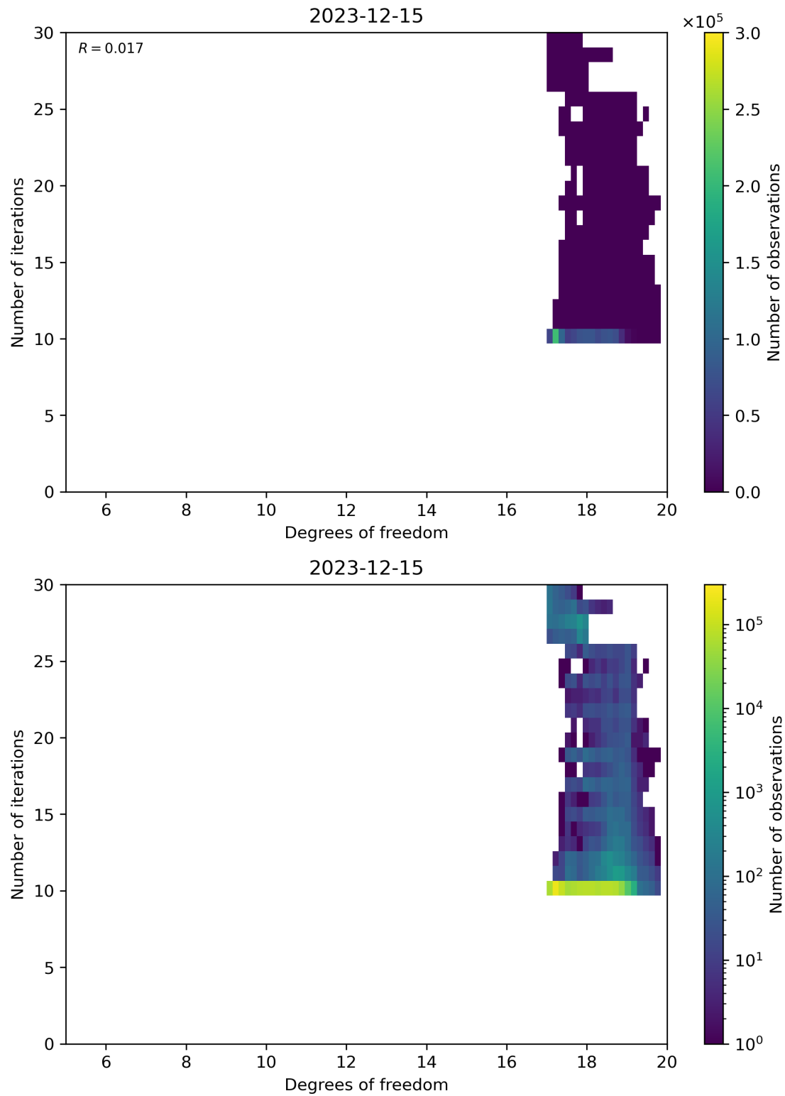
Figure 52: Scatter density plot of “Degrees of freedom” against “Number of iterations” for 2023-12-14 to 2023-12-16.
