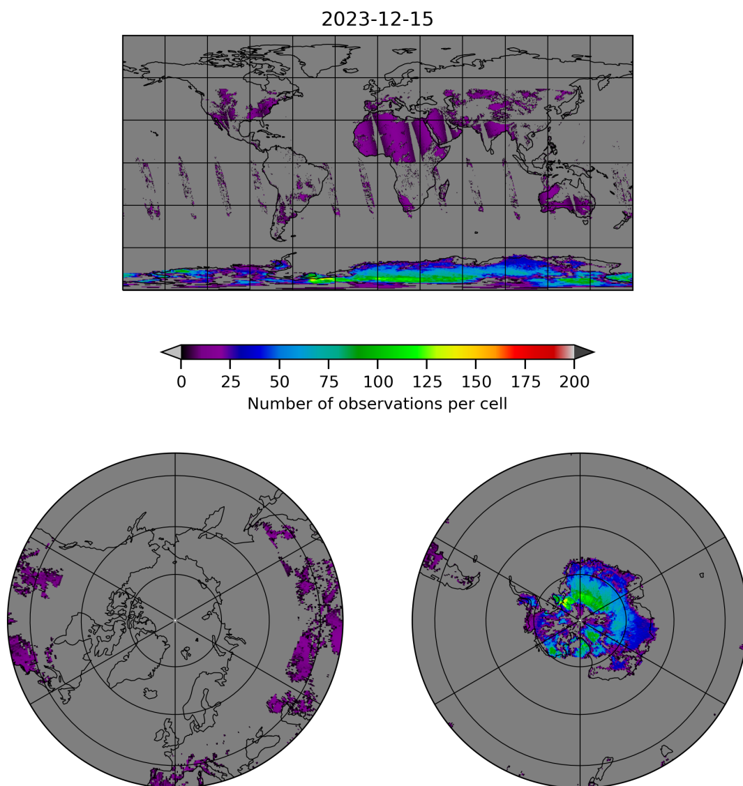
Figure 10: Map of the number of observations for 2023-12-14 to 2023-12-16
