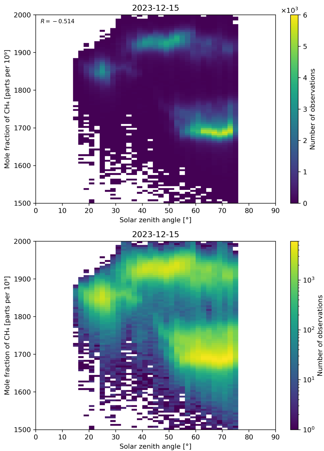
Figure 99: Scatter density plot of “Solar zenith angle” against “Mole fraction of CH 4 ” for 2023-12-14 to 2023-12-16.
