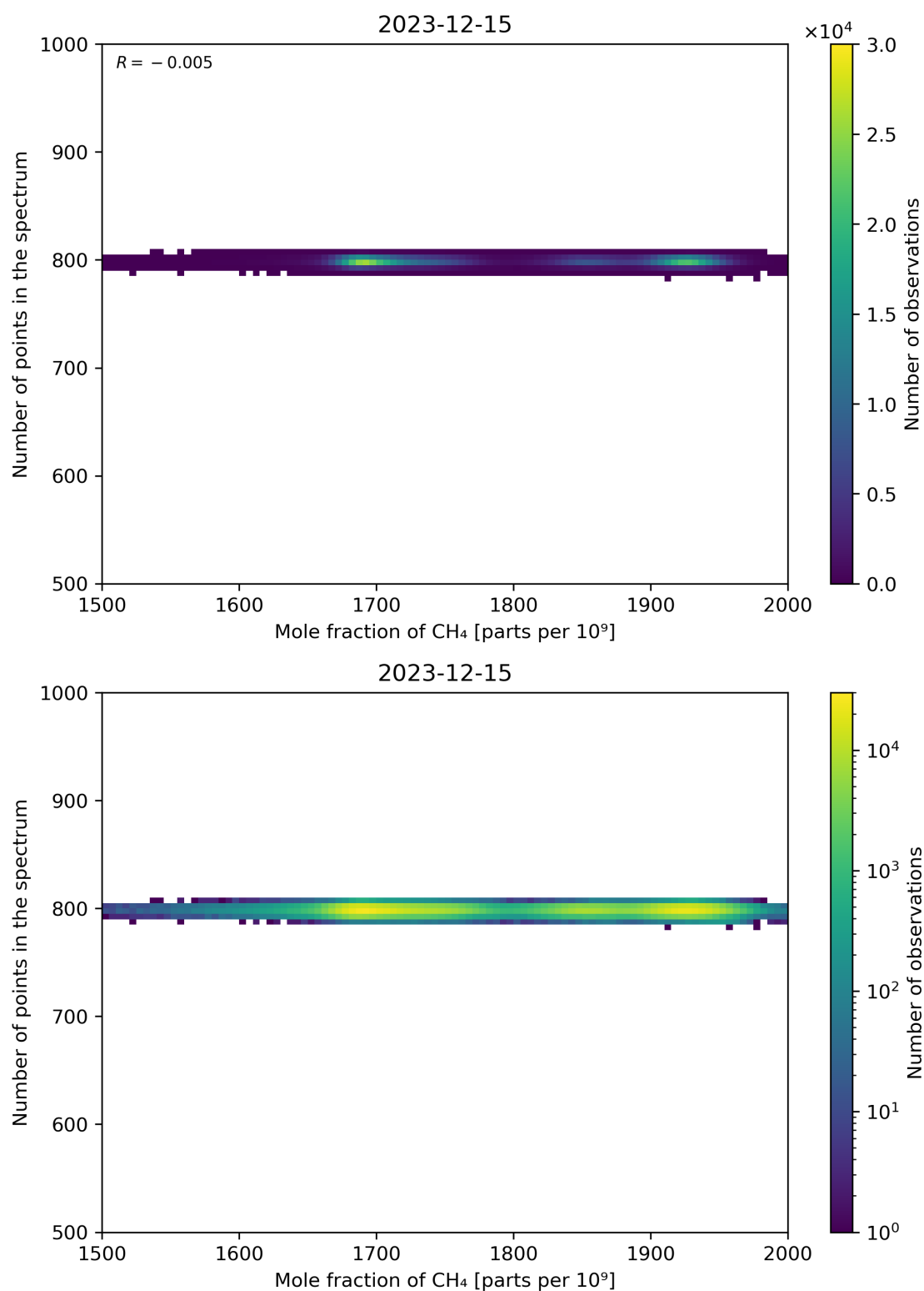
Figure 77: Scatter density plot of “Mole fraction of CH 4 ” against “Number of points in the spectrum” for 2023-12-14 to 2023-12-16.
