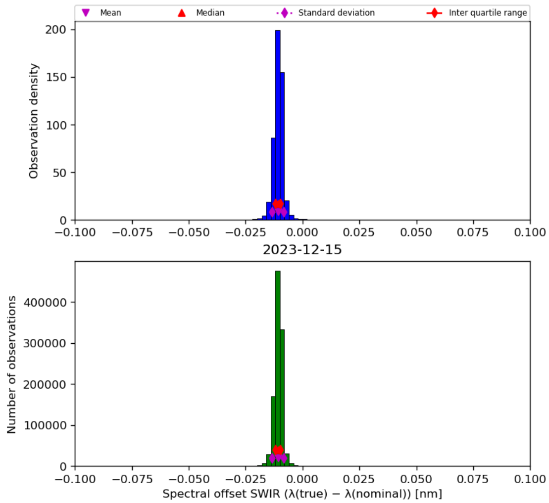
Figure 27: Histogram of “Spectral offset SWIR ( \lambda(\text{true}) - \lambda(\text{nominal}) )” for 2023-12-14 to 2023-12-16
