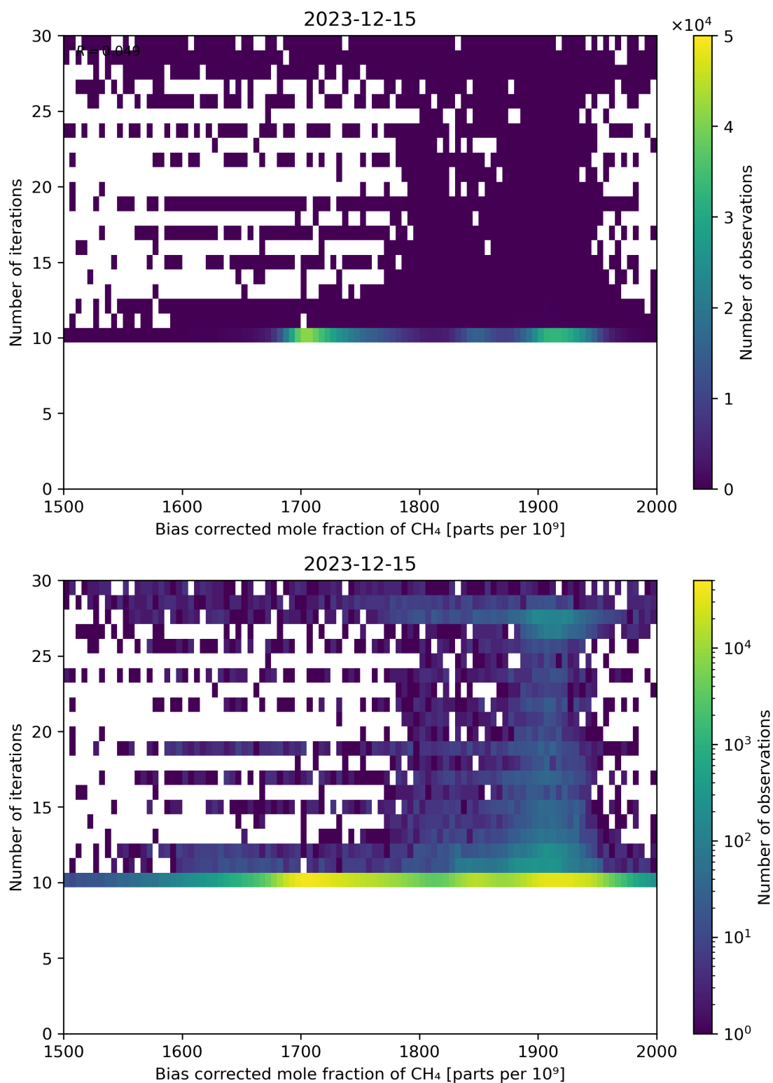
Figure 67: Scatter density plot of “Bias corrected mole fraction of \text{CH}_4 ” against “Number of iterations” for 2023-12-14 to 2023-12-16.
