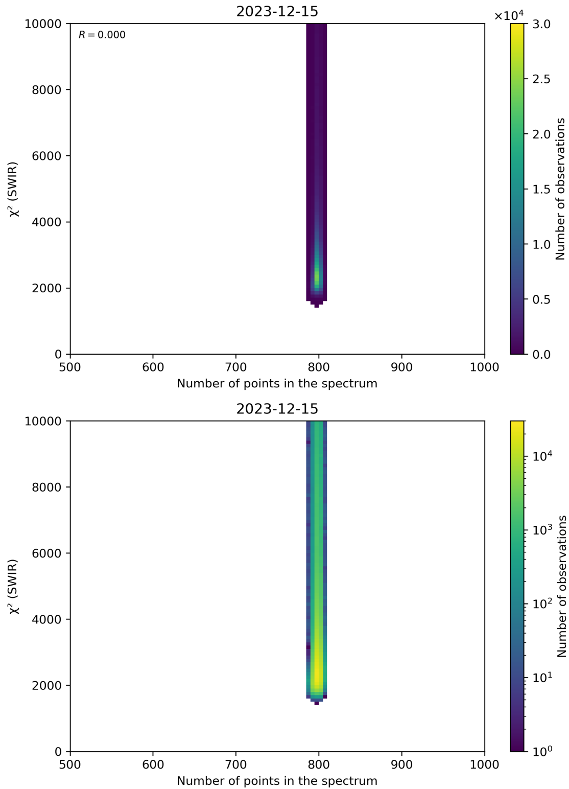
Figure 89: Scatter density plot of “Number of points in the spectrum” against “ \chi^2 (SWIR)” for 2023-12-14 to 2023-12-16.
