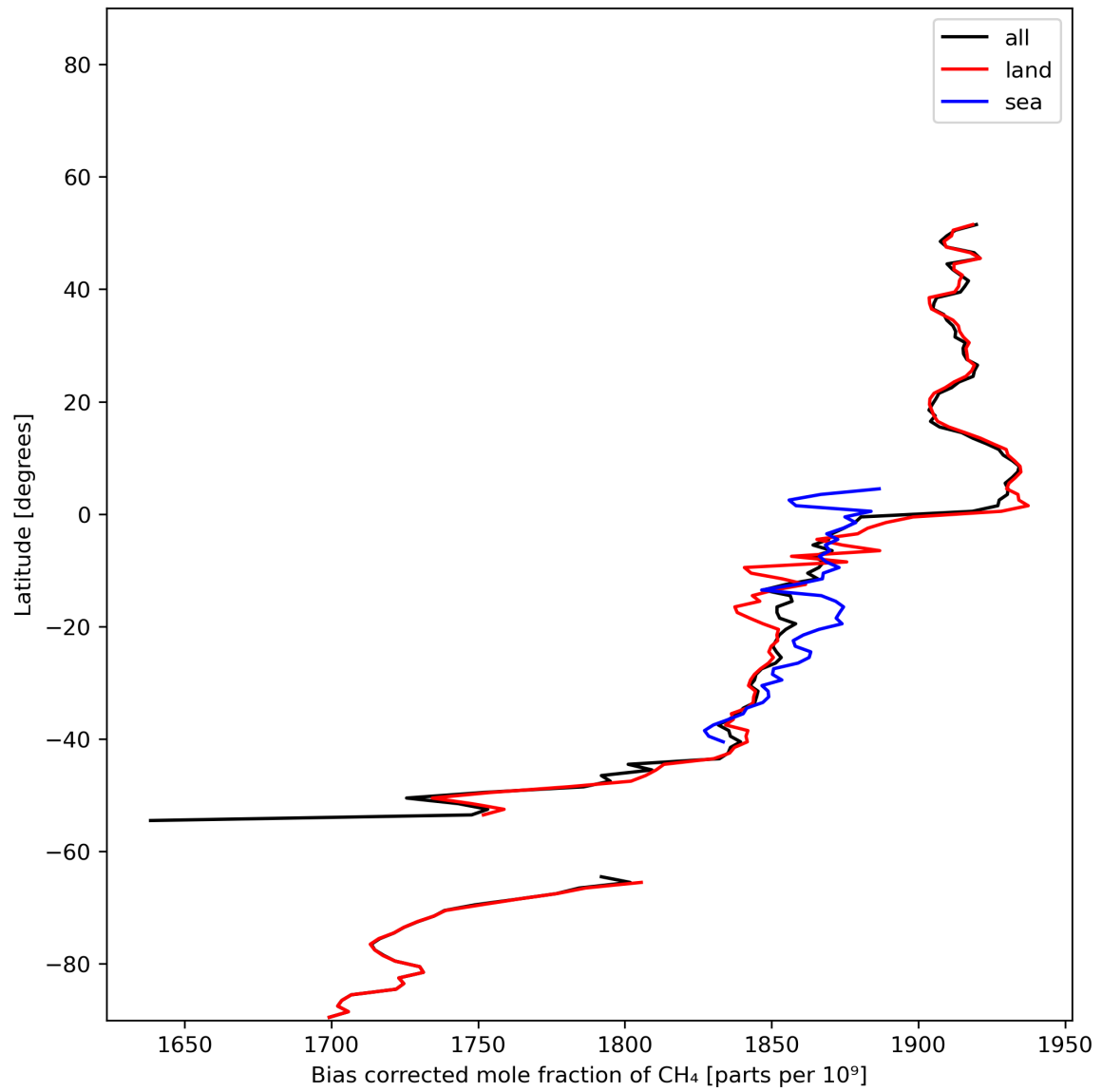
Figure 14: Zonal average of “Bias corrected mole fraction of CH 4 ” for 2023-12-14 to 2023-12-16.
