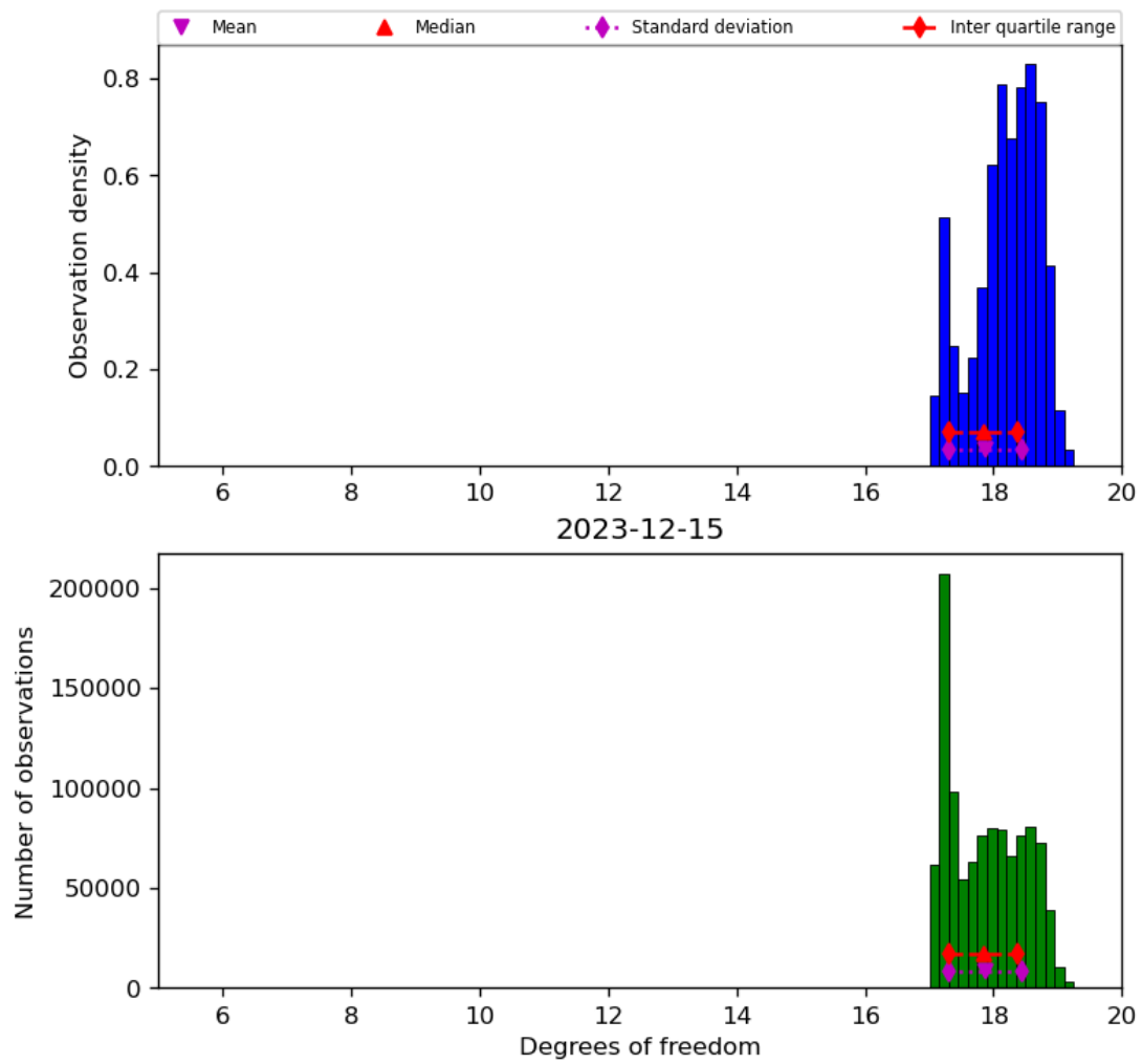
Figure 30: Histogram of “Degrees of freedom” for 2023-12-14 to 2023-12-16
