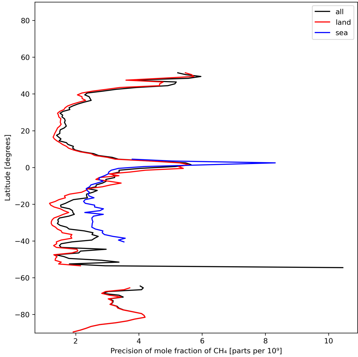
Figure 13: Zonal average of “Precision of mole fraction of CH 4 ” for 2023-12-14 to 2023-12-16.
