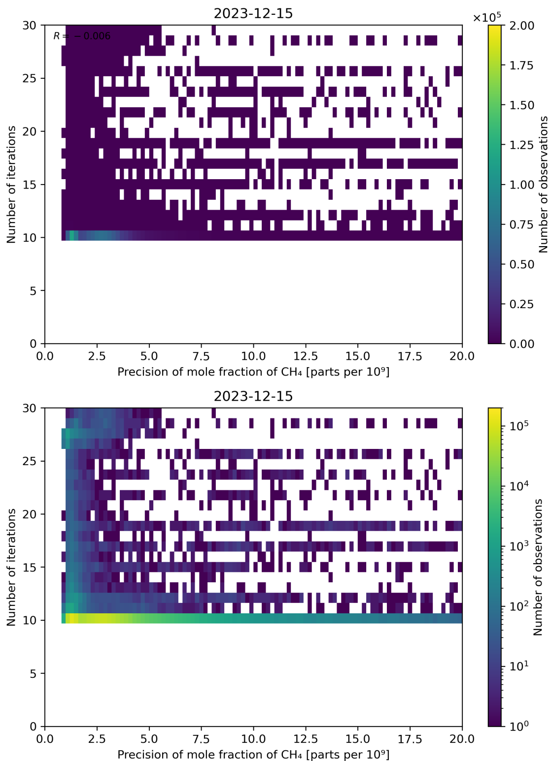
Figure 83: Scatter density plot of “Precision of mole fraction of CH 4 ” against “Number of iterations” for 2023-12-14 to 2023-12-16.
