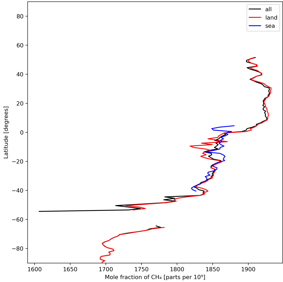
Figure 12: Zonal average of “Mole fraction of \text{CH}_4 ” for 2023-12-14 to 2023-12-16.
