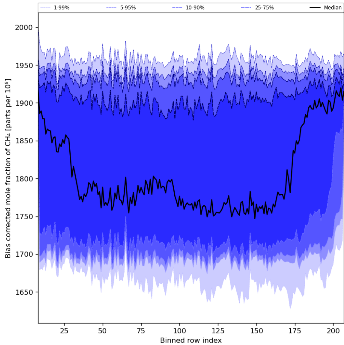
Figure 36: Along track statistics of “Bias corrected mole fraction of CH 4 ” for 2023-12-14 to 2023-12-16
