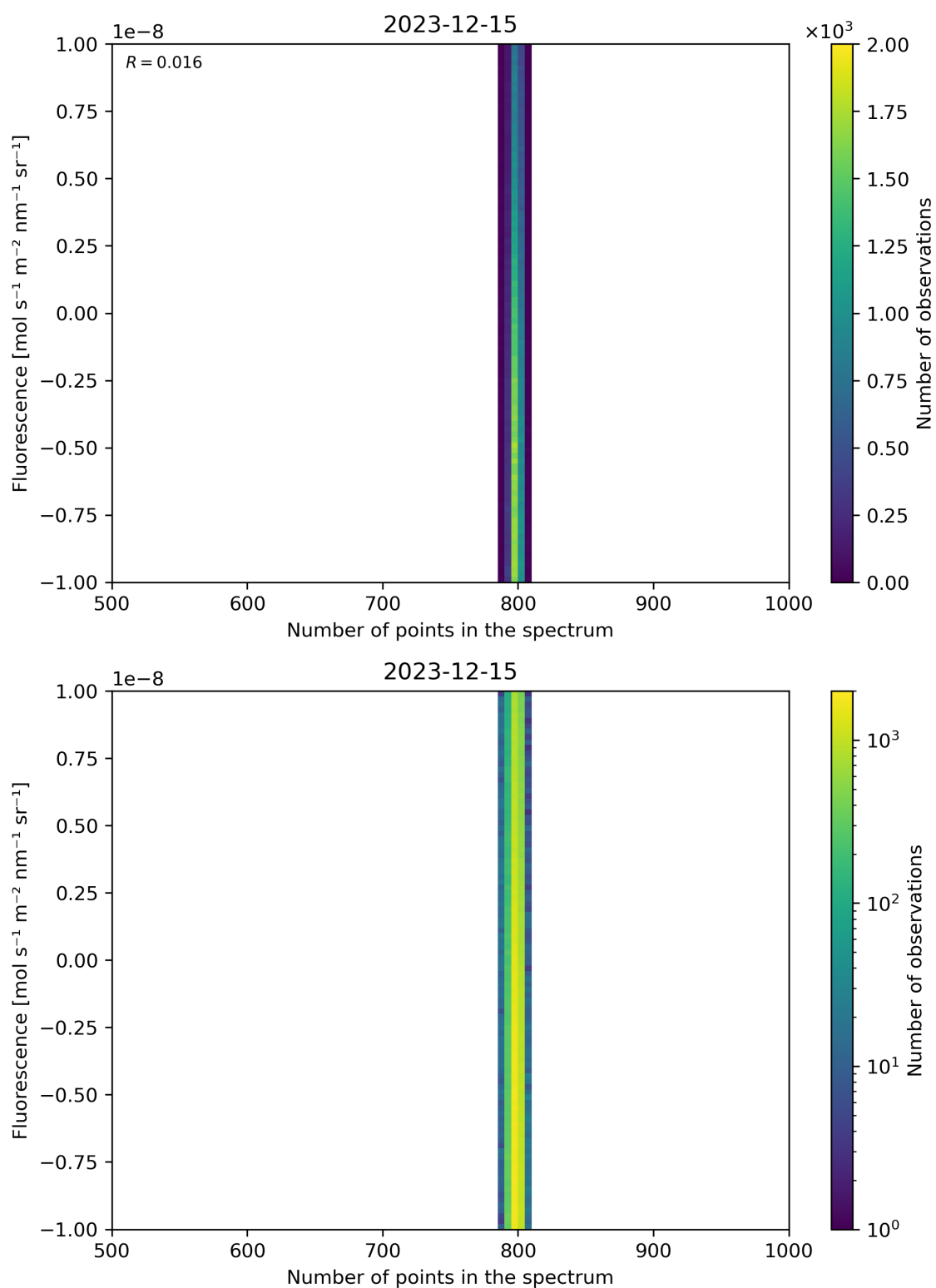
Figure 91: Scatter density plot of “Number of points in the spectrum” against “Fluorescence” for 2023-12-14 to 2023-12-16.
