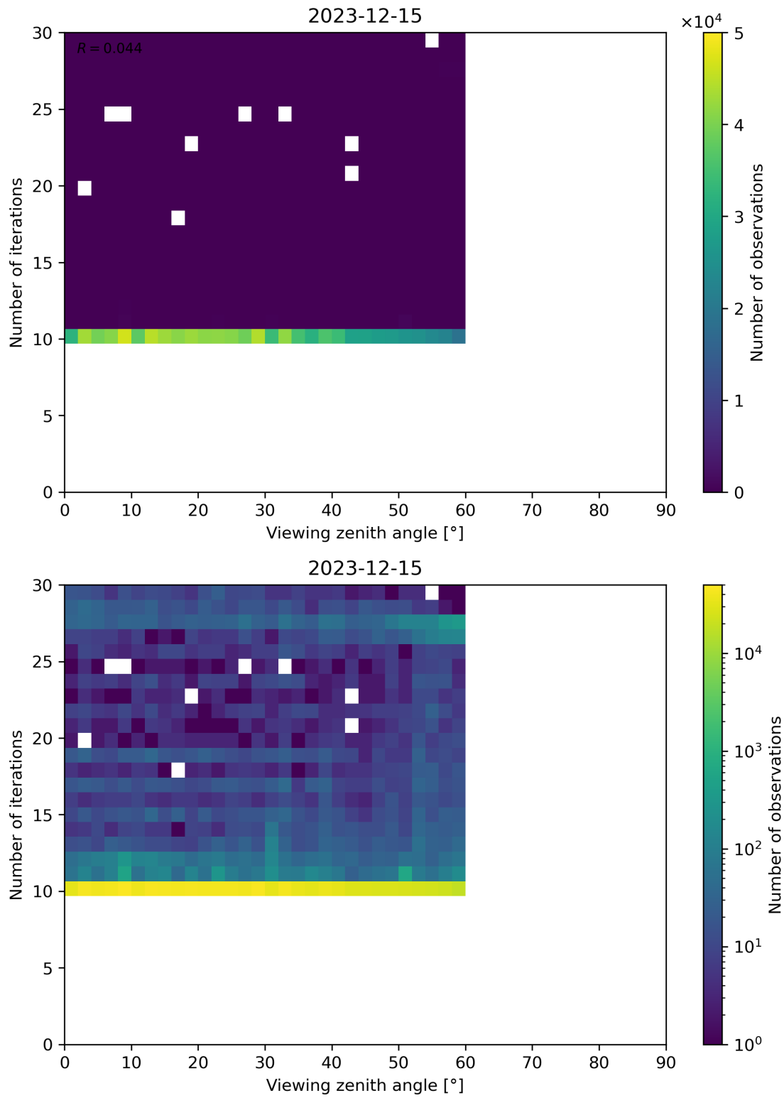
Figure 113: Scatter density plot of “Viewing zenith angle” against “Number of iterations” for 2023-12-14 to 2023-12-16.
