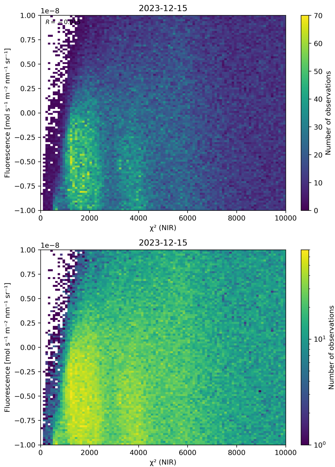
Figure 45: Scatter density plot of “ \chi^2 (NIR)” against “Fluorescence” for 2023-12-14 to 2023-12-16.
