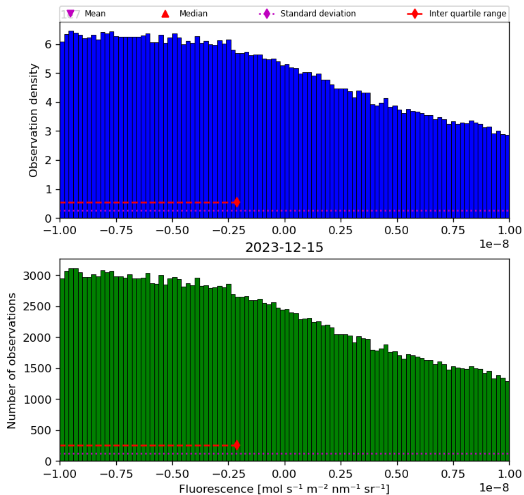
Figure 32: Histogram of “Fluorescence” for 2023-12-14 to 2023-12-16
