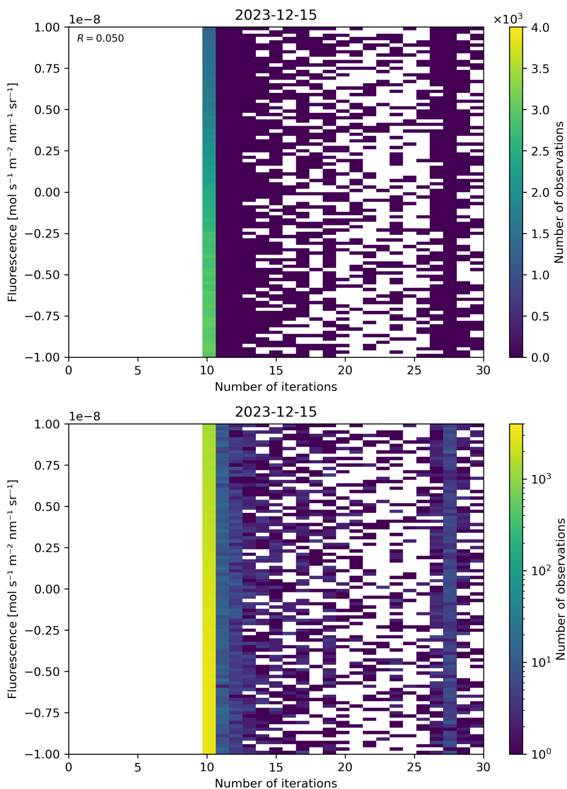
Figure 87: Scatter density plot of “Number of iterations” against “Fluorescence” for 2023-12-14 to 2023-12-16.
