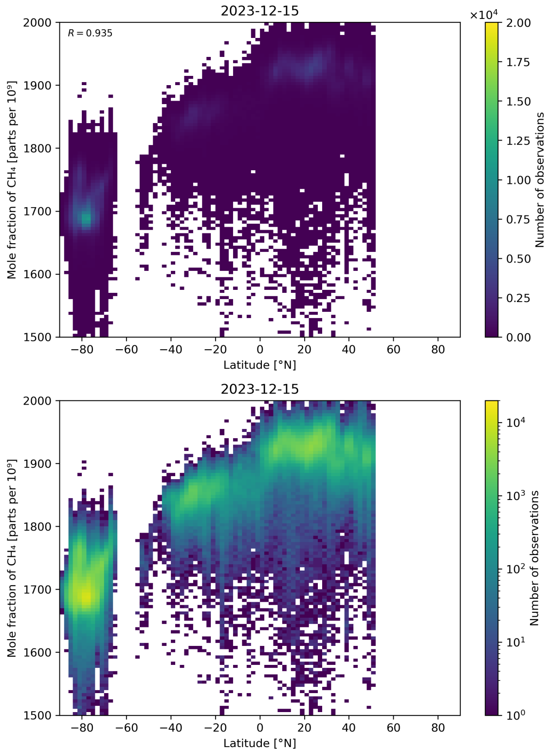
Figure 57: Scatter density plot of “Latitude” against “Mole fraction of CH 4 ” for 2023-12-14 to 2023-12-16.
