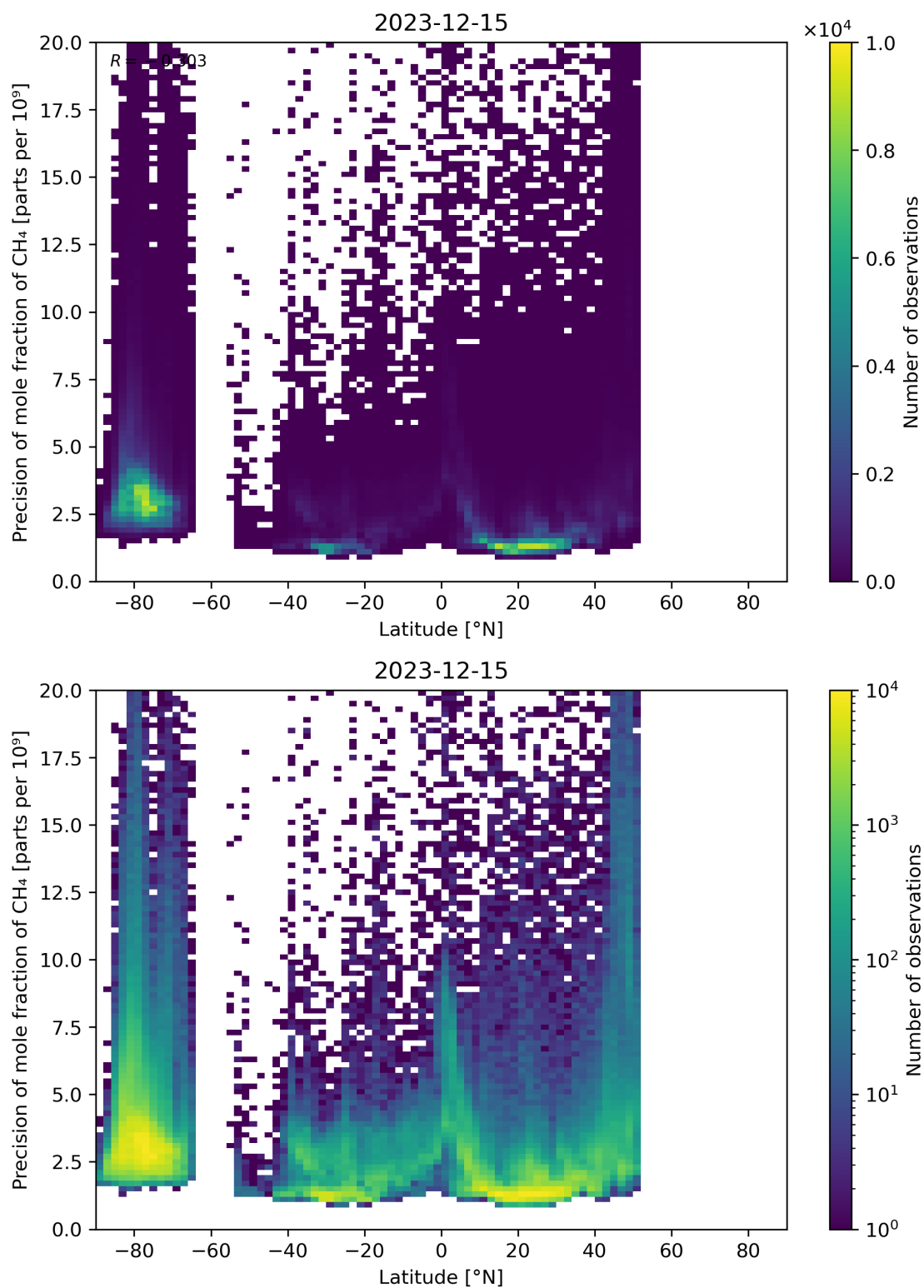
Figure 59: Scatter density plot of “Latitude” against “Precision of mole fraction of CH 4 ” for 2023-12-14 to 2023-12-16.
