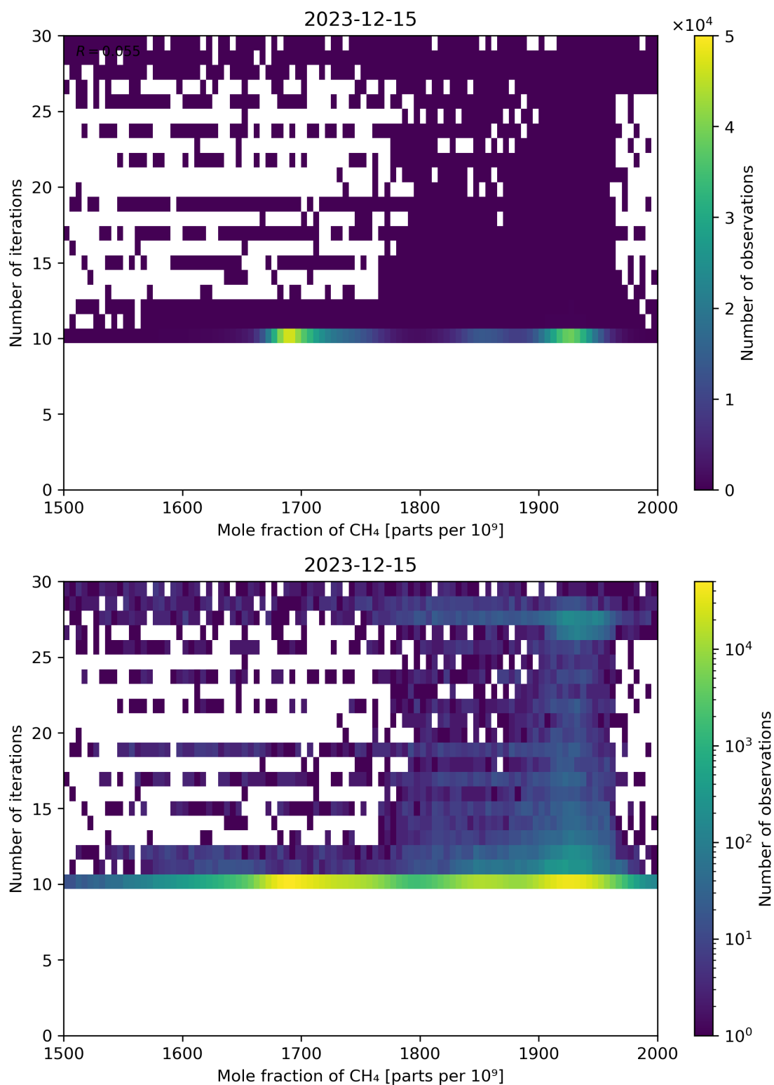
Figure 76: Scatter density plot of “Mole fraction of CH 4 ” against “Number of iterations” for 2023-12-14 to 2023-12-16.
