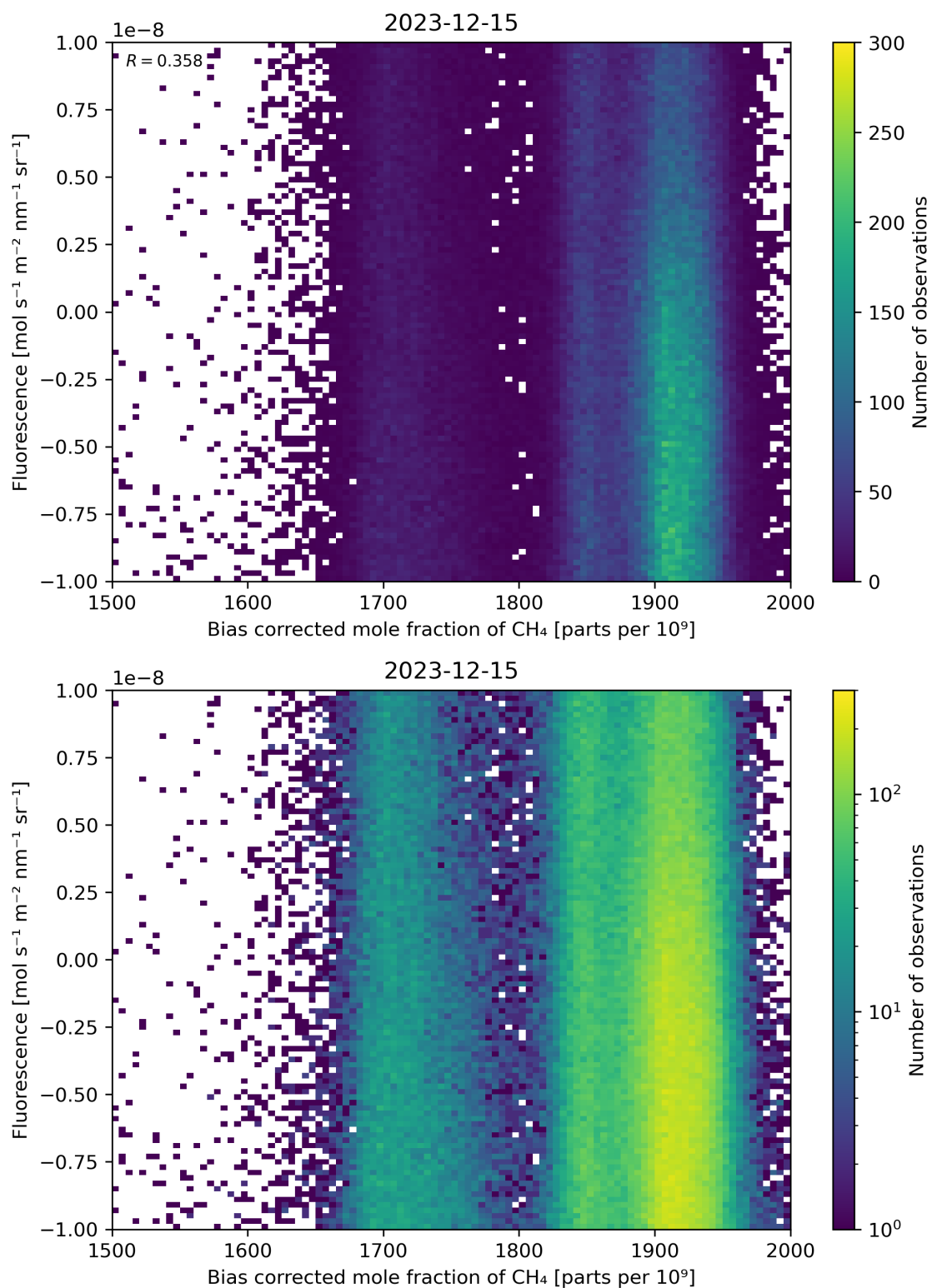
Figure 66: Scatter density plot of “Bias corrected mole fraction of \text{CH}_4 ” against “Fluorescence” for 2023-12-14 to 2023-12-16.
