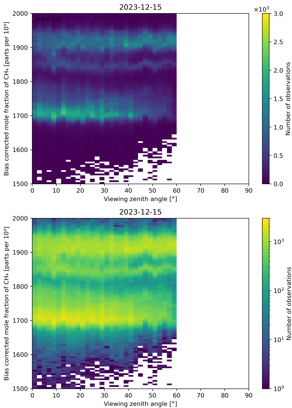
Figure 111: Scatter density plot of “Viewing zenith angle” against “Bias corrected mole fraction of CH 4 ” for 2023-12-14 to 2023-12-16.
