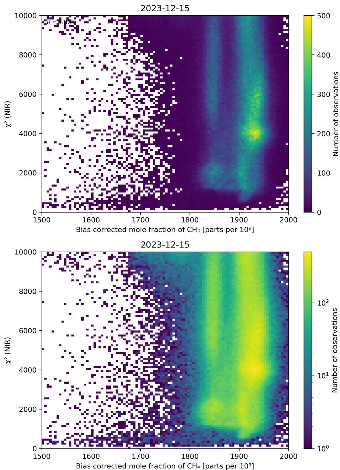
Figure 63: Scatter density plot of “Bias corrected mole fraction of CH 4 ” against “ \chi^2 (NIR)” for 2023-12-14 to 2023-12-16.
