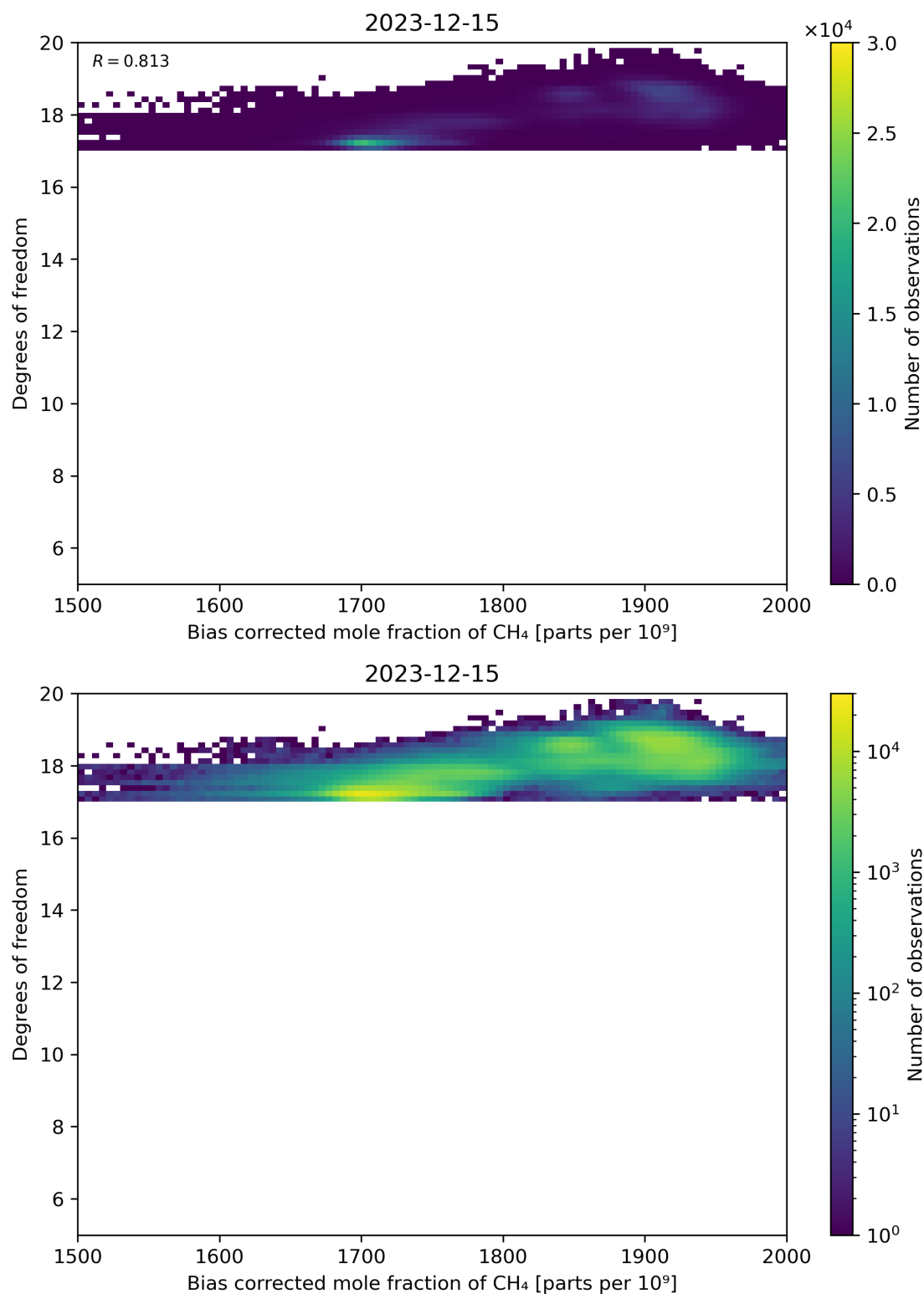
Figure 65: Scatter density plot of “Bias corrected mole fraction of CH 4 ” against “Degrees of freedom” for 2023-12-14 to 2023-12-16.
