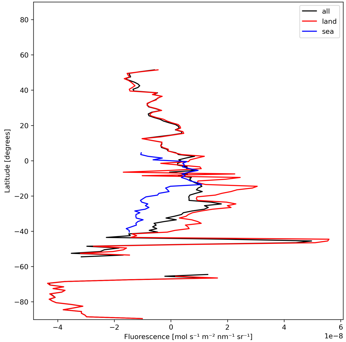
Figure 21: Zonal average of “Fluorescence” for 2023-12-14 to 2023-12-16.
