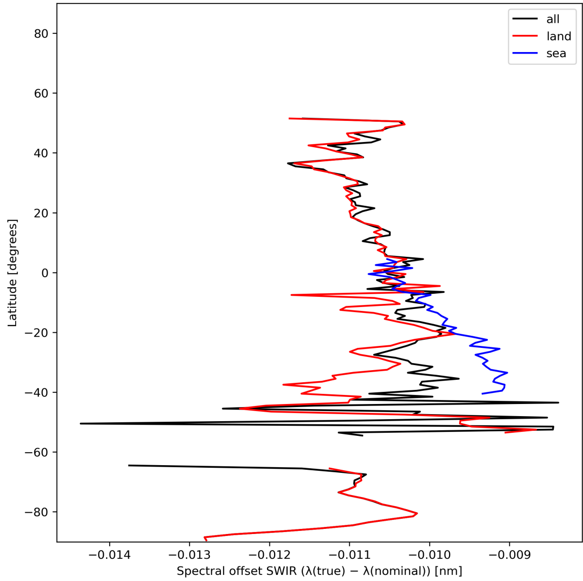
Figure 16: Zonal average of “Spectral offset SWIR ( \lambda(\text{true}) - \lambda(\text{nominal}) )” for 2023-12-14 to 2023-12-16.
