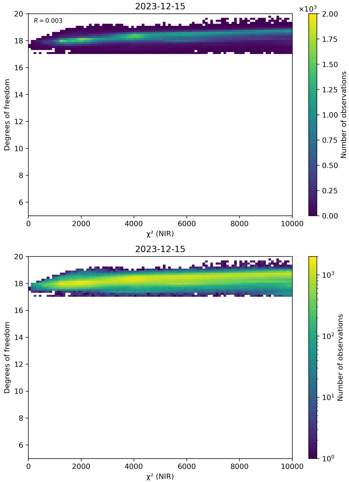
Figure 44: Scatter density plot of “ \chi^2 (NIR)” against “Degrees of freedom” for 2023-12-14 to 2023-12-16.
