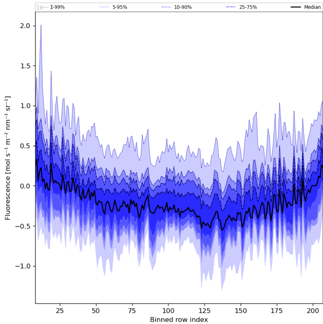
Figure 43: Along track statistics of “Fluorescence” for 2023-12-14 to 2023-12-16
