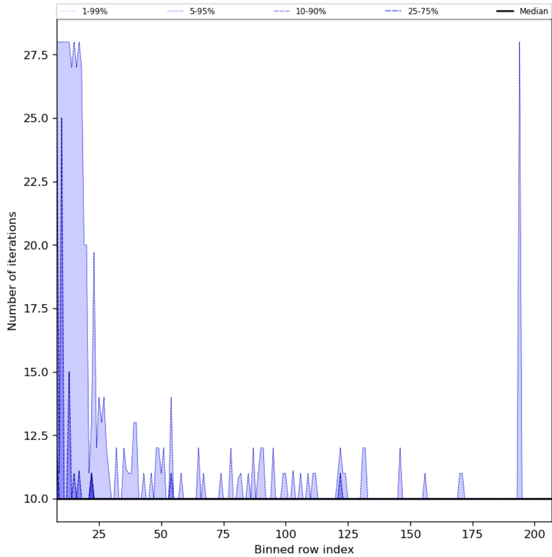
Figure 42: Along track statistics of “Number of iterations” for 2023-12-14 to 2023-12-16
