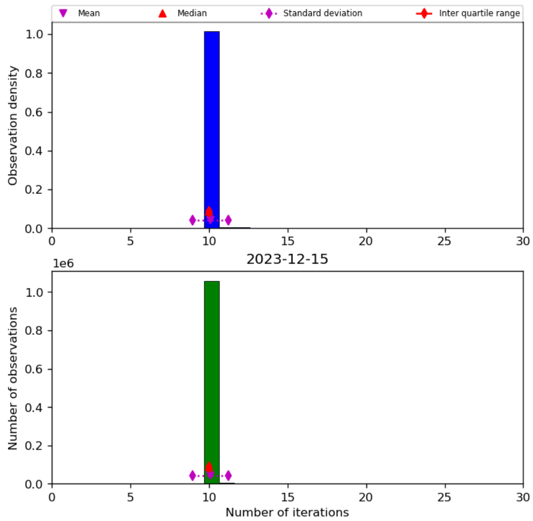
Figure 31: Histogram of "Number of iterations" for 2023-12-14 to 2023-12-16
