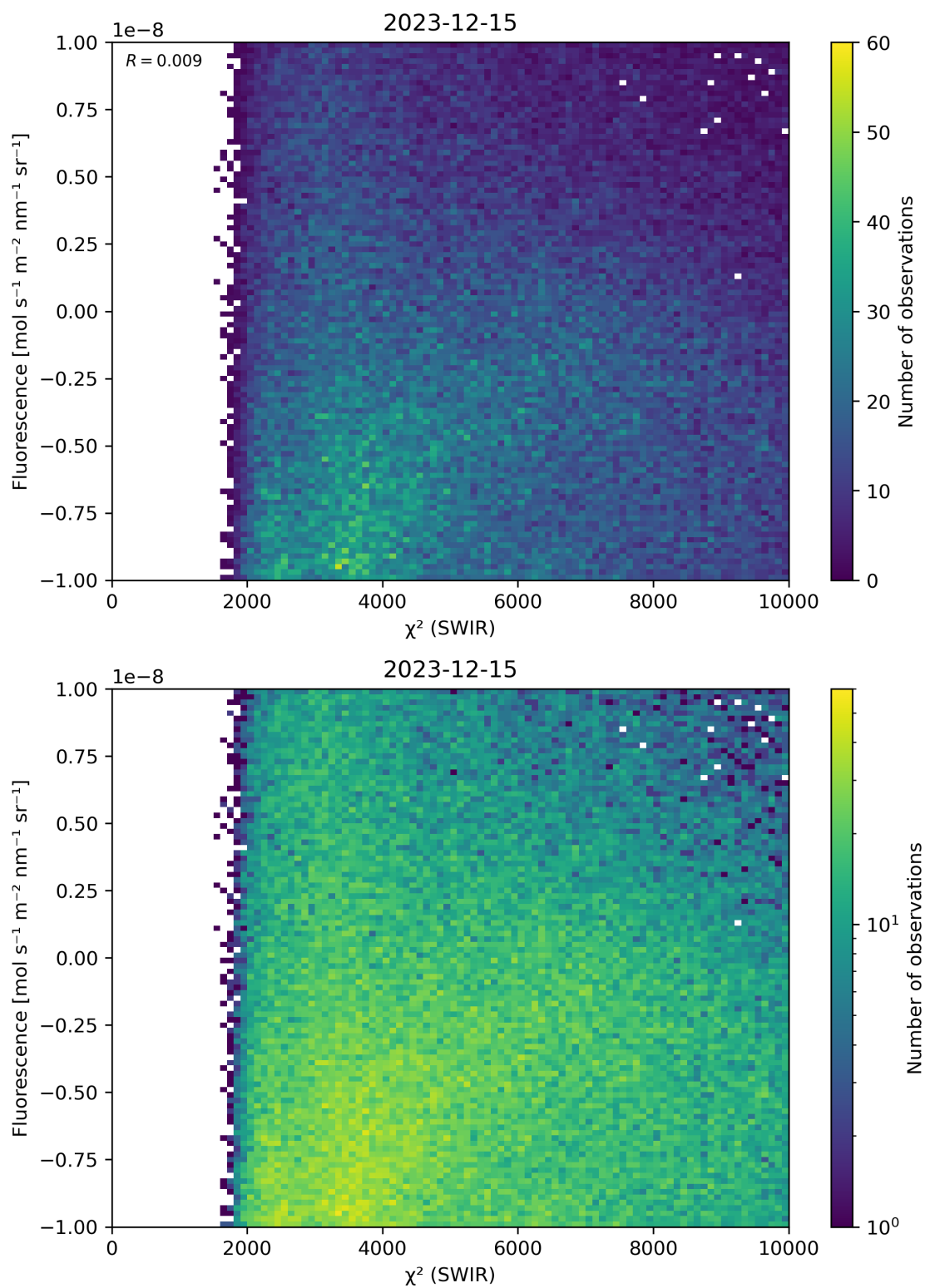
Figure 49: Scatter density plot of “ \chi^2 (SWIR)” against “Fluorescence” for 2023-12-14 to 2023-12-16.
