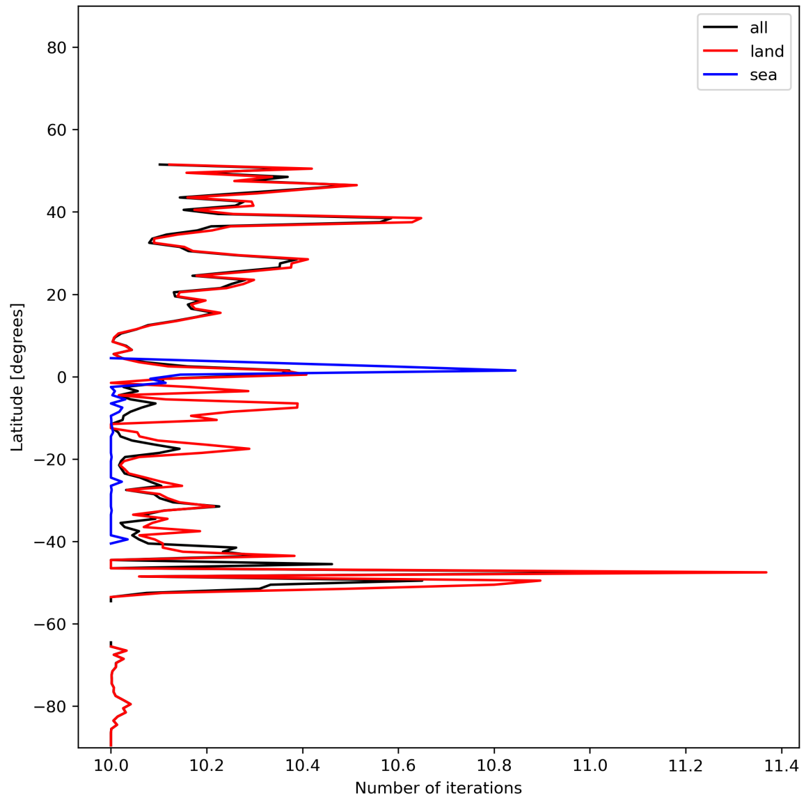
Figure 20: Zonal average of “Number of iterations” for 2023-12-14 to 2023-12-16.
