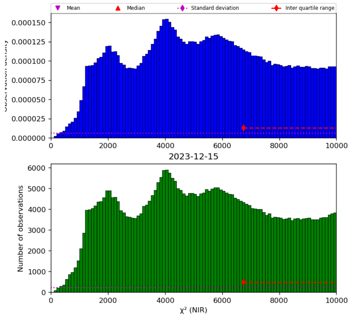
Figure 29: Histogram of “ \chi^2 (NIR)” for 2023-12-14 to 2023-12-16
