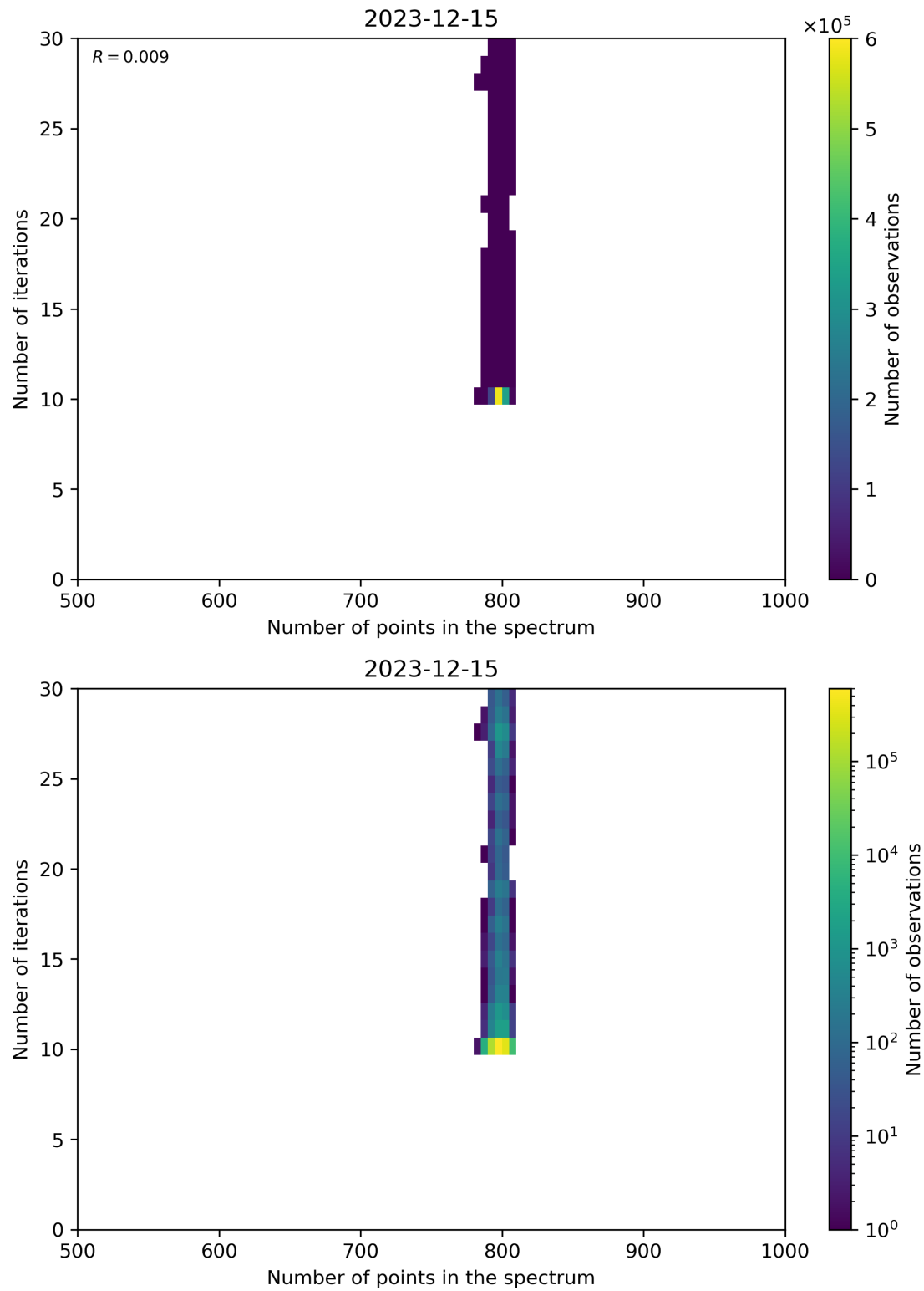
Figure 92: Scatter density plot of “Number of points in the spectrum” against “Number of iterations” for 2023-12-14 to 2023-12-16.
