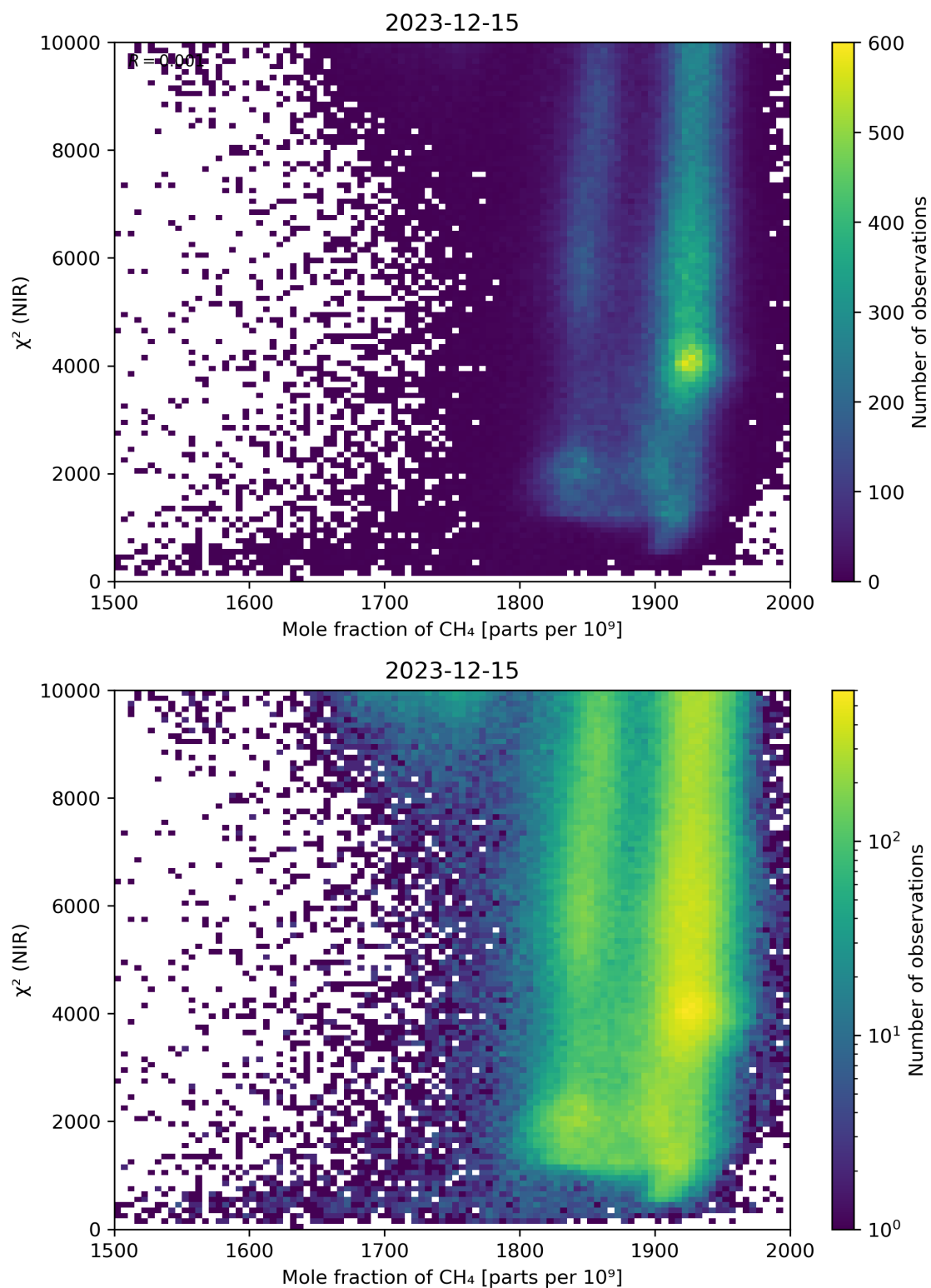
Figure 70: Scatter density plot of “Mole fraction of \text{CH}_4 ” against “ \chi^2 (NIR)” for 2023-12-14 to 2023-12-16.
