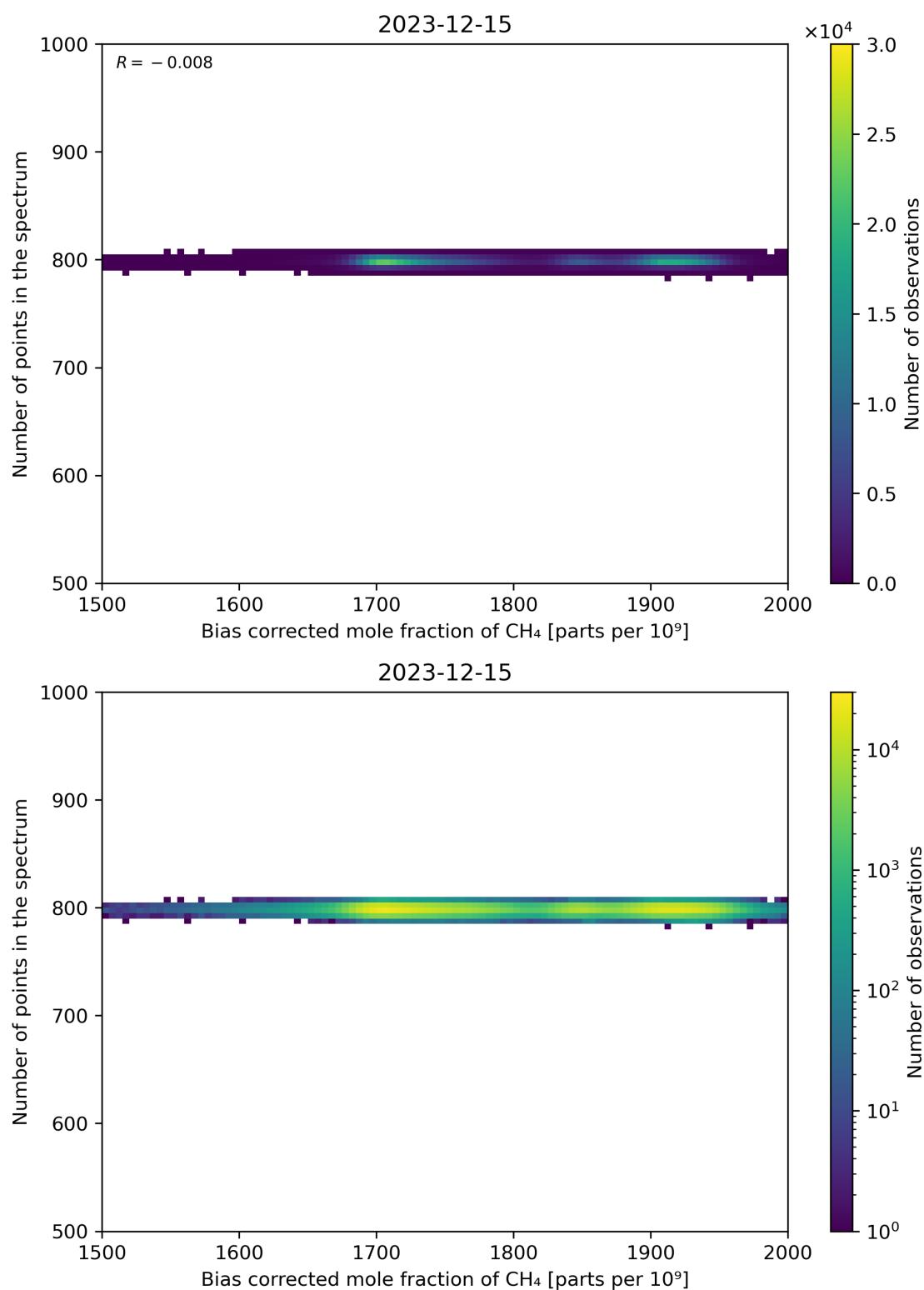
Figure 68: Scatter density plot of “Bias corrected mole fraction of CH 4 ” against “Number of points in the spectrum” for 2023-12-14 to 2023-12-16.
