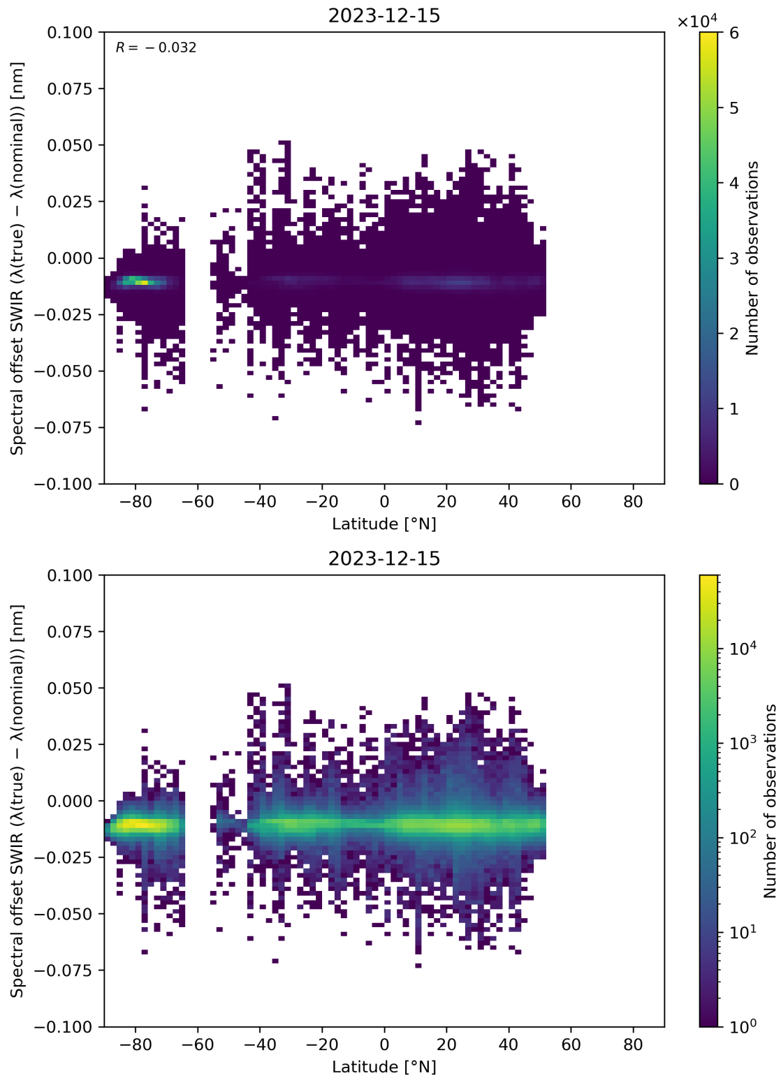
Figure 62: Scatter density plot of “Latitude” against “Spectral offset SWIR ( \lambda(\text{true}) - \lambda(\text{nominal}) )” for 2023-12-14 to 2023-12-16.
