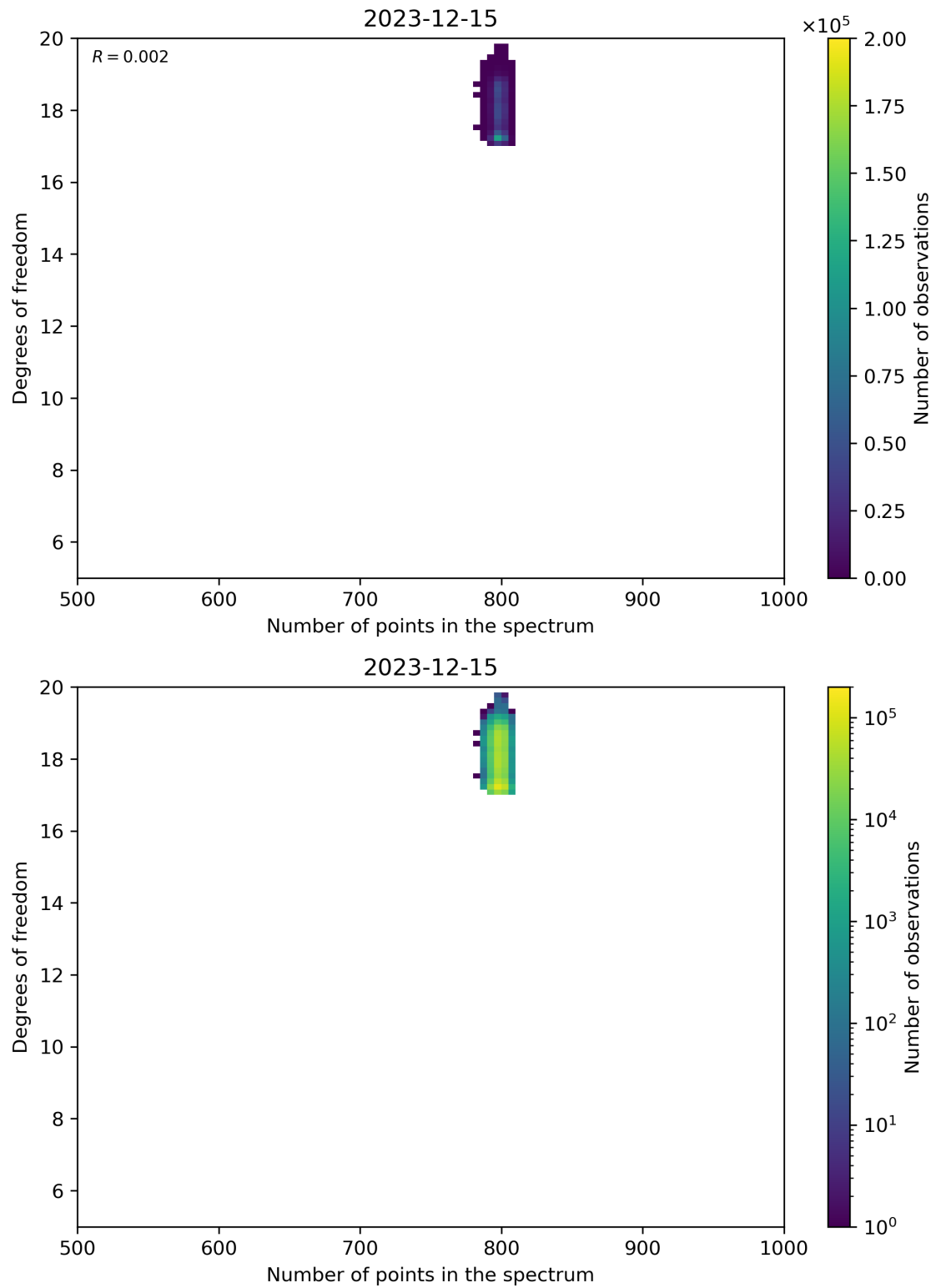
Figure 90: Scatter density plot of “Number of points in the spectrum” against “Degrees of freedom” for 2023-12-14 to 2023-12-16.
