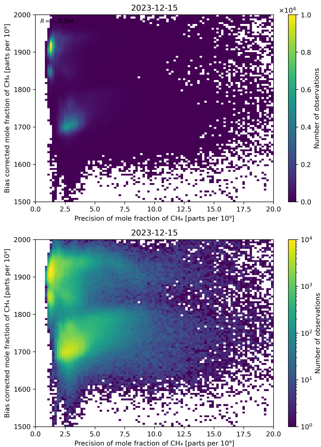
Figure 82: Scatter density plot of “Precision of mole fraction of \text{CH}_4 ” against “Bias corrected mole fraction of \text{CH}_4 ” for 2023-12-14 to 2023-12-16.
