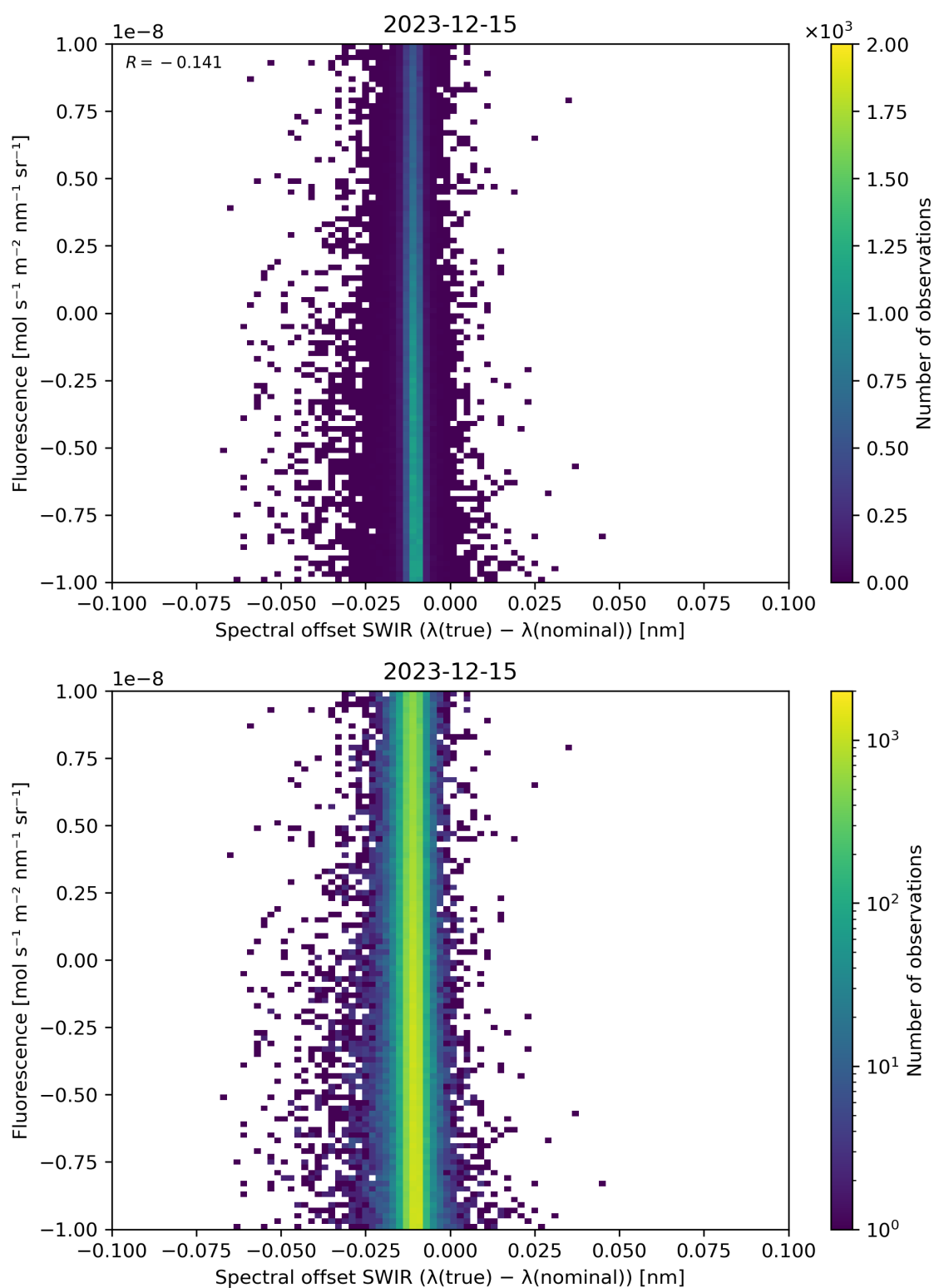
Figure 120: Scatter density plot of “Spectral offset SWIR ( \lambda(\text{true}) - \lambda(\text{nominal}) )” against “Fluorescence” for 2023-12-14 to 2023-12-16.
