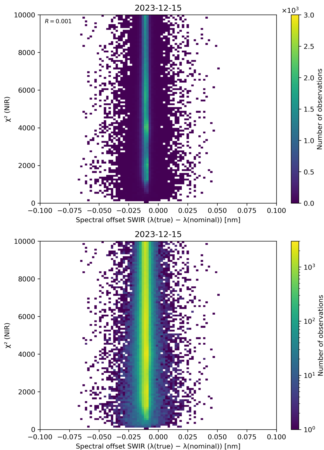
Figure 117: Scatter density plot of “Spectral offset SWIR ( \lambda(\text{true}) - \lambda(\text{nominal}) )” against “ \chi^2 (NIR)” for 2023-12-14 to 2023-12-16.
