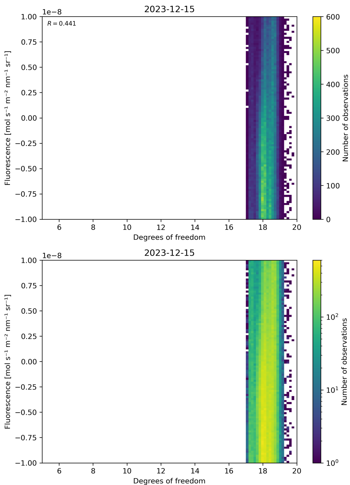
Figure 51: Scatter density plot of “Degrees of freedom” against “Fluorescence” for 2023-12-14 to 2023-12-16.
