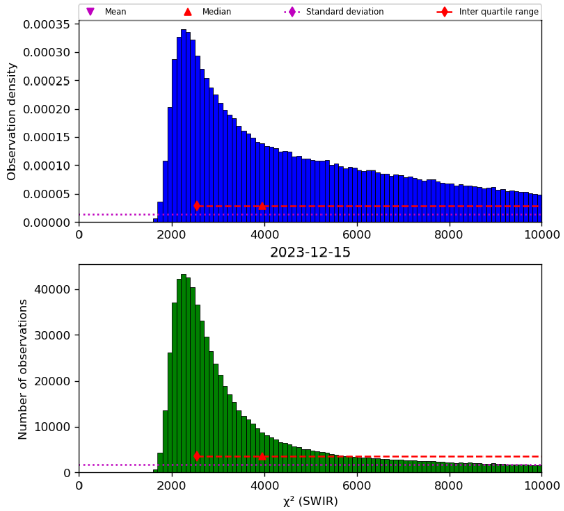
Figure 28: Histogram of “ \chi^2 (SWIR)” for 2023-12-14 to 2023-12-16
