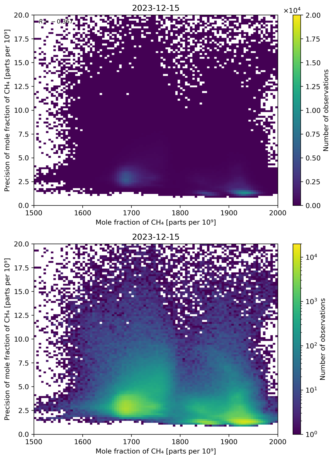
Figure 75: Scatter density plot of “Mole fraction of CH 4 ” against “Precision of mole fraction of CH 4 ” for 2023-12-14 to 2023-12-16.
