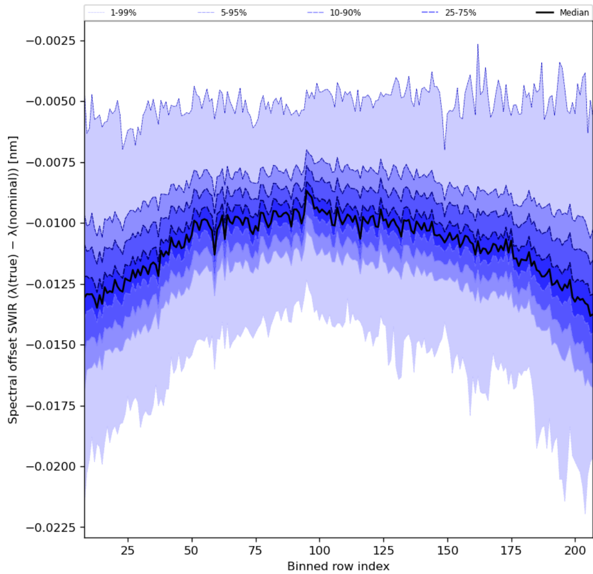
Figure 38: Along track statistics of “Spectral offset SWIR ( \lambda(\text{true}) - \lambda(\text{nominal}) )” for 2023-12-14 to 2023-12-16
