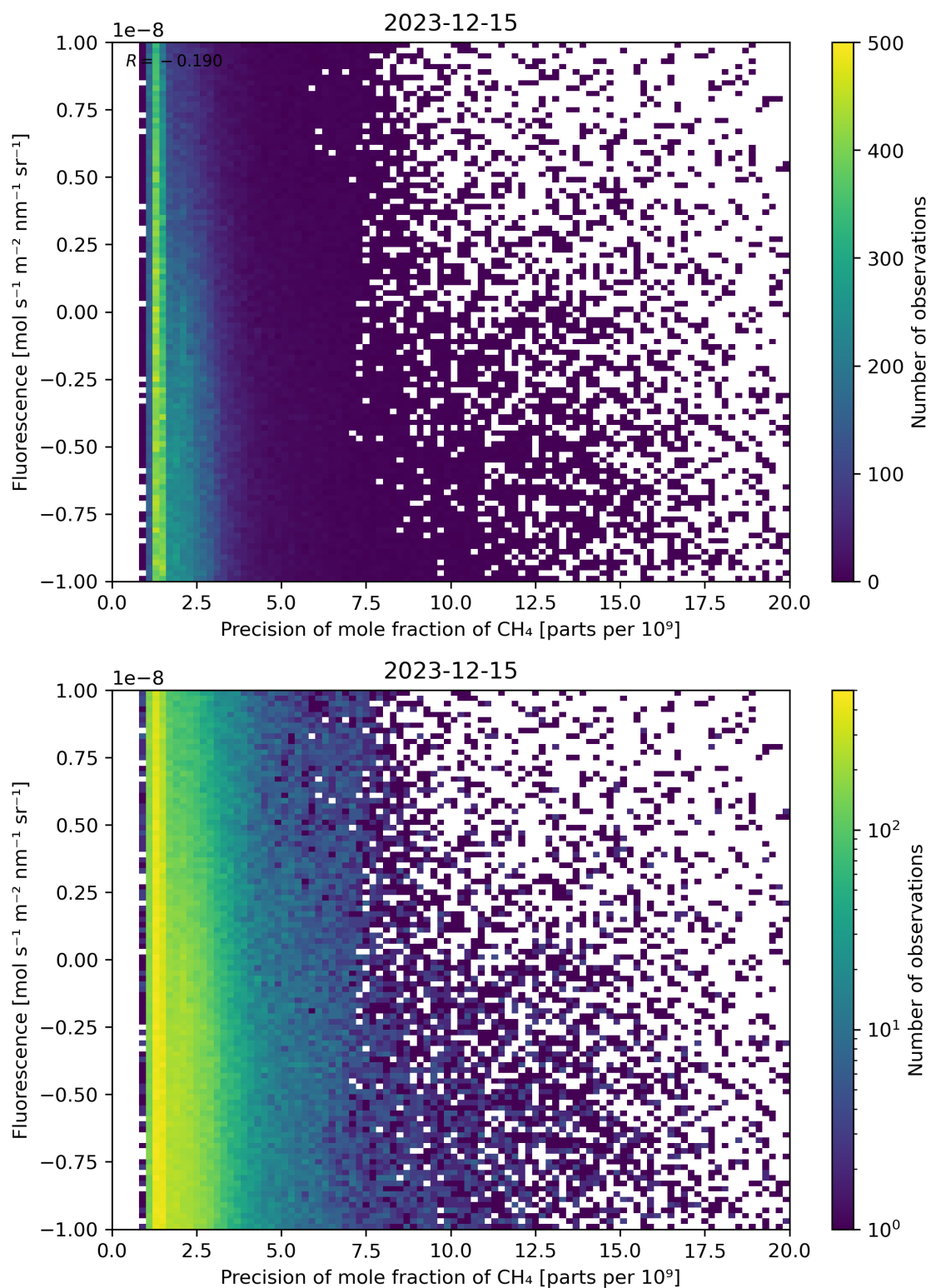
Figure 81: Scatter density plot of “Precision of mole fraction of \text{CH}_4 ” against “Fluorescence” for 2023-12-14 to 2023-12-16.
