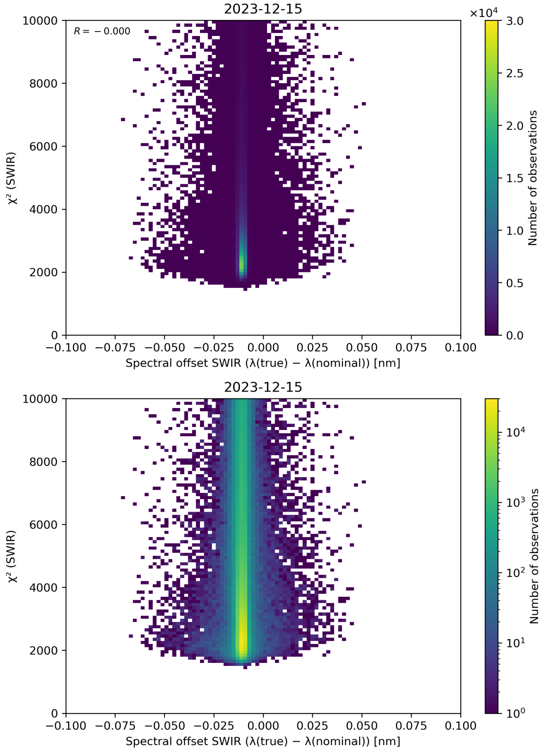
Figure 118: Scatter density plot of “Spectral offset SWIR ( \lambda(\text{true}) - \lambda(\text{nominal}) )” against “ \chi^2 (SWIR)” for 2023-12-14 to 2023-12-16.
