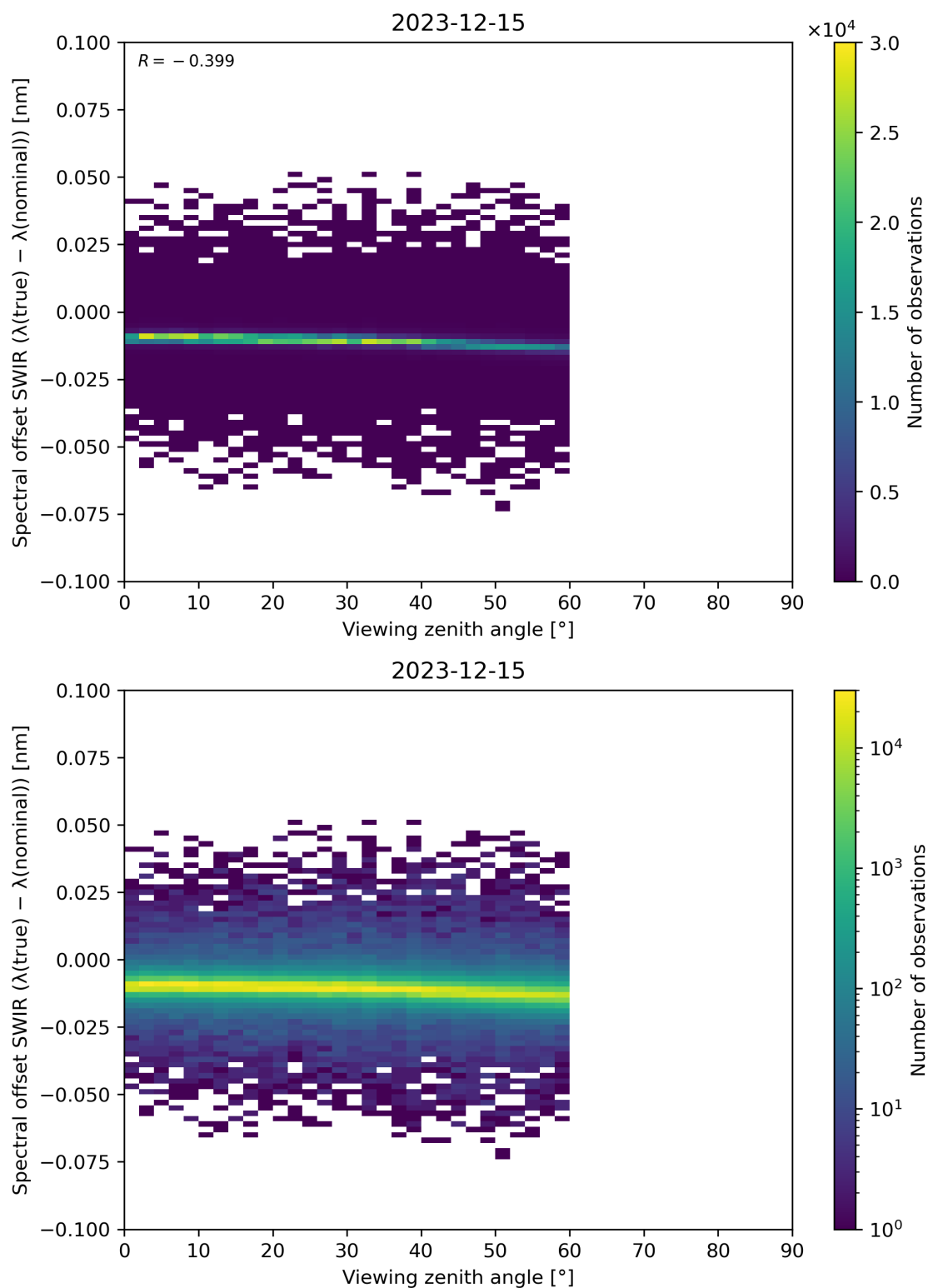
Figure 116: Scatter density plot of “Viewing zenith angle” against “Spectral offset SWIR ( \lambda(\text{true}) - \lambda(\text{nominal}) )” for 2023-12-14 to 2023-12-16.
