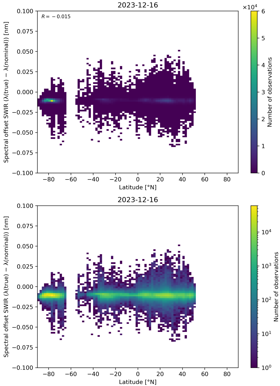
Figure 62: Scatter density plot of “Latitude” against “Spectral offset SWIR ( \lambda(\text{true}) - \lambda(\text{nominal}) )” for 2023-12-15 to 2023-12-17.
