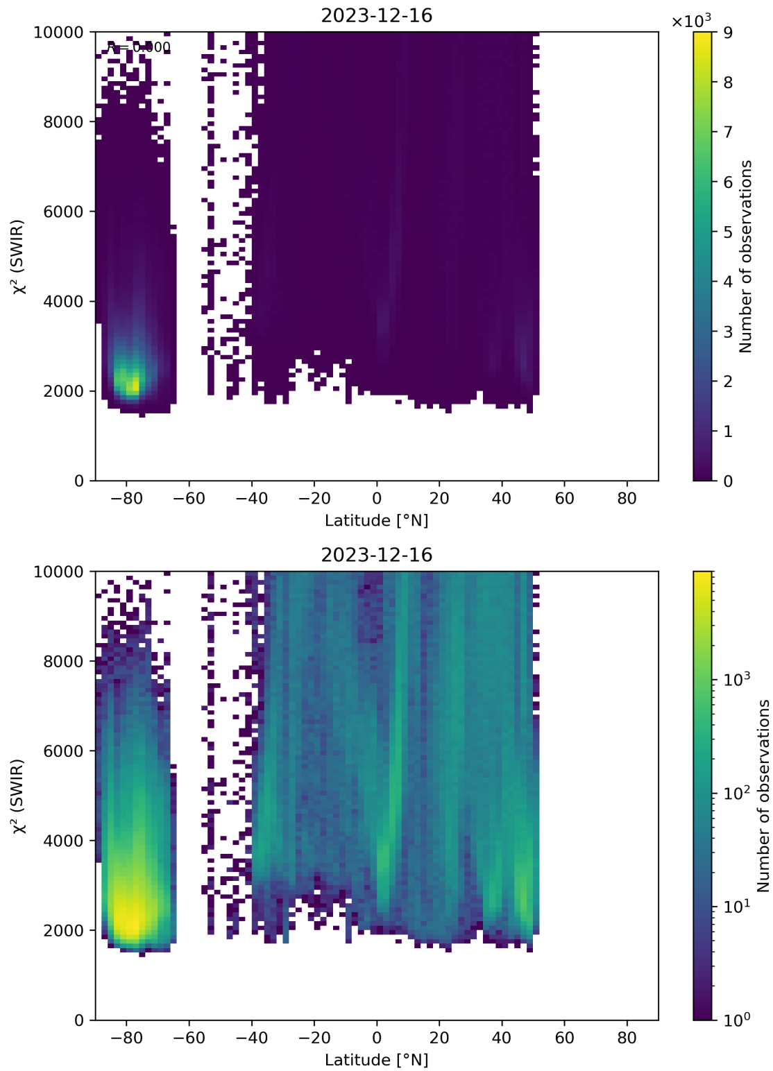
Figure 54: Scatter density plot of “Latitude” against “ \chi^2 (SWIR)” for 2023-12-15 to 2023-12-17.
