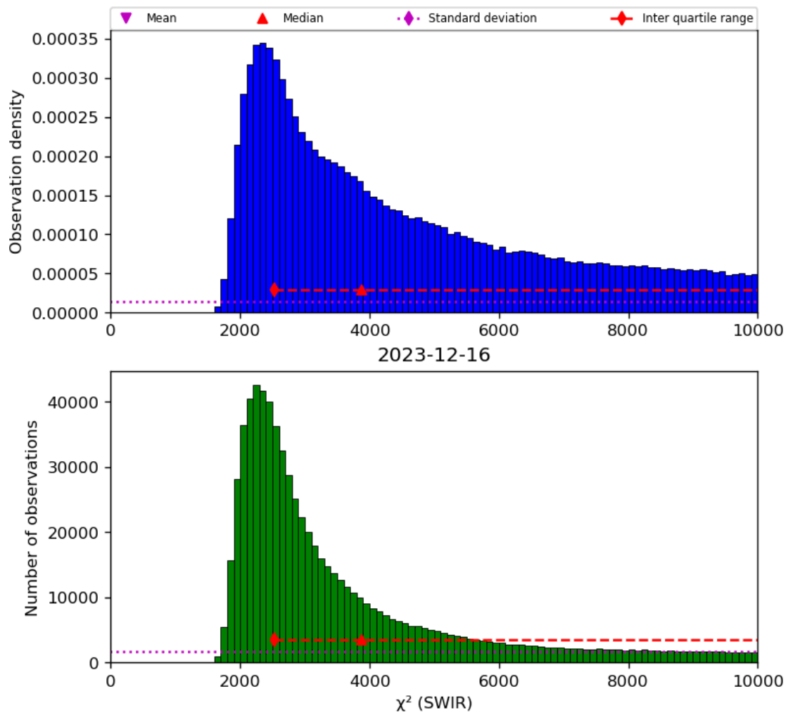
Figure 28: Histogram of “ \chi^2 (SWIR)” for 2023-12-15 to 2023-12-17
