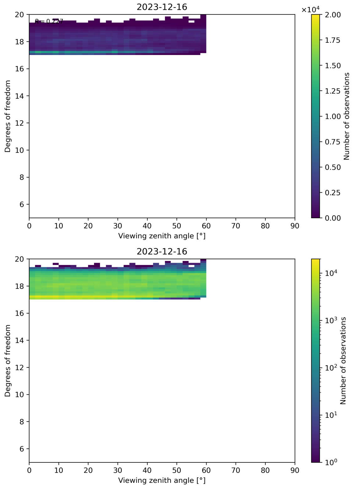
Figure 107: Scatter density plot of “Viewing zenith angle” against “Degrees of freedom” for 2023-12-15 to 2023-12-17.
