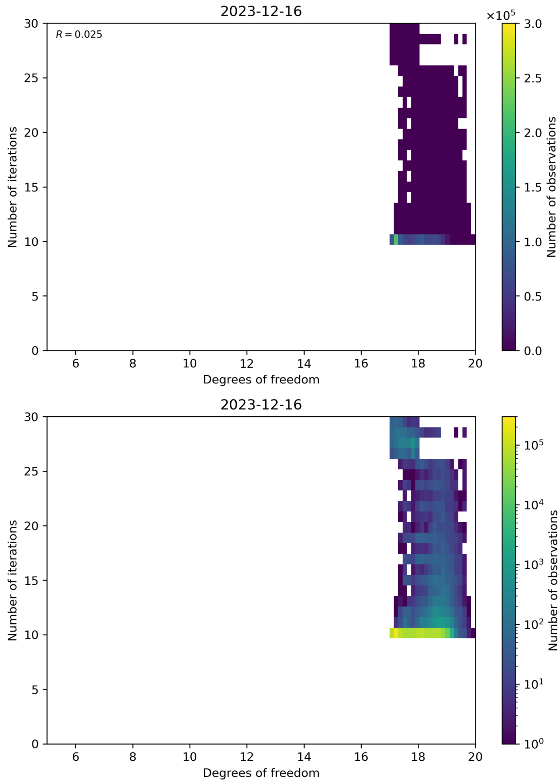
Figure 52: Scatter density plot of “Degrees of freedom” against “Number of iterations” for 2023-12-15 to 2023-12-17.
