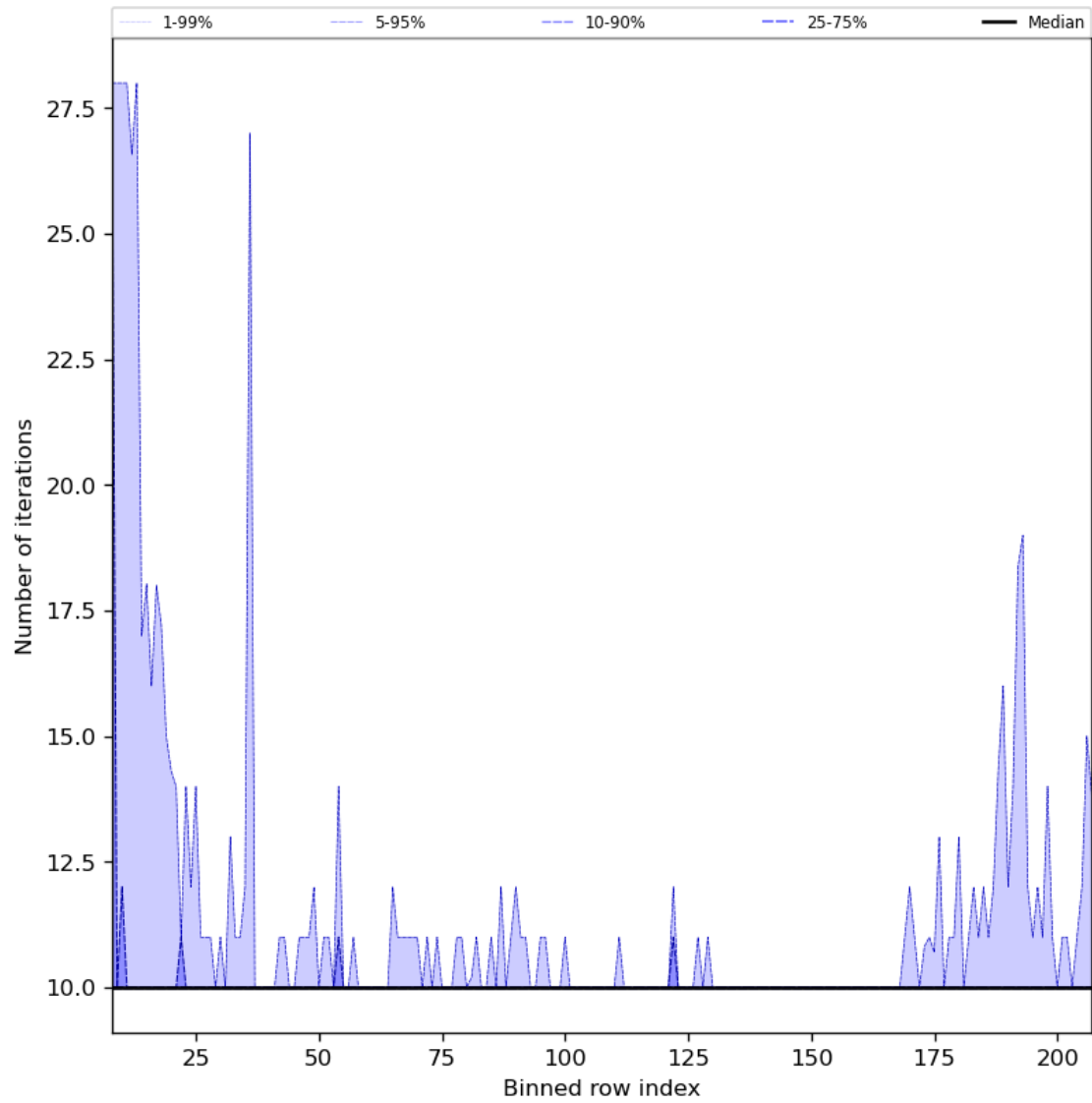
Figure 42: Along track statistics of “Number of iterations” for 2023-12-15 to 2023-12-17
