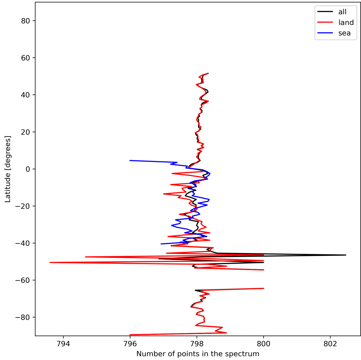
Figure 15: Zonal average of “Number of points in the spectrum” for 2023-12-15 to 2023-12-17.
