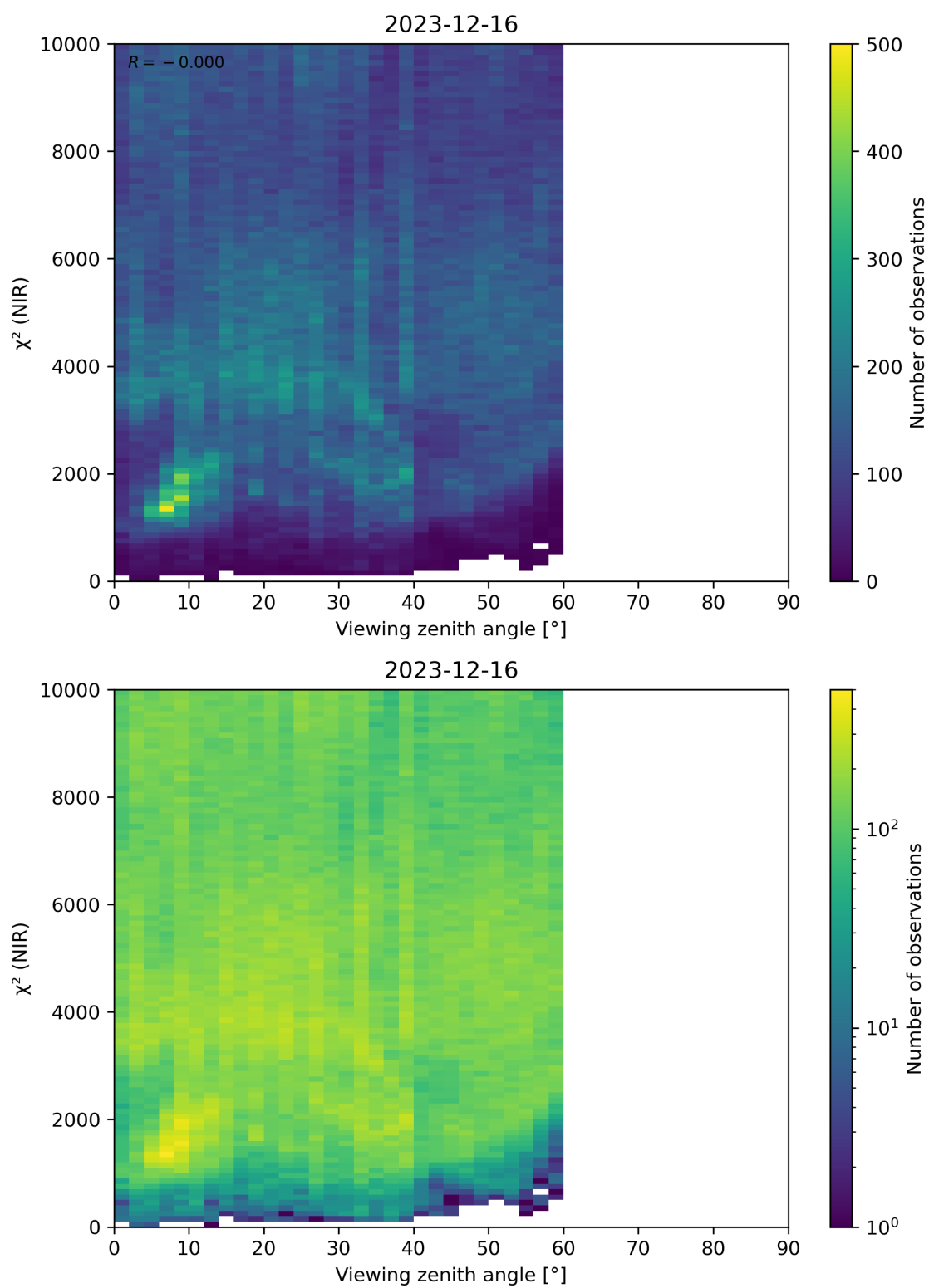
Figure 105: Scatter density plot of “Viewing zenith angle” against “ \chi^2 (NIR)” for 2023-12-15 to 2023-12-17.
