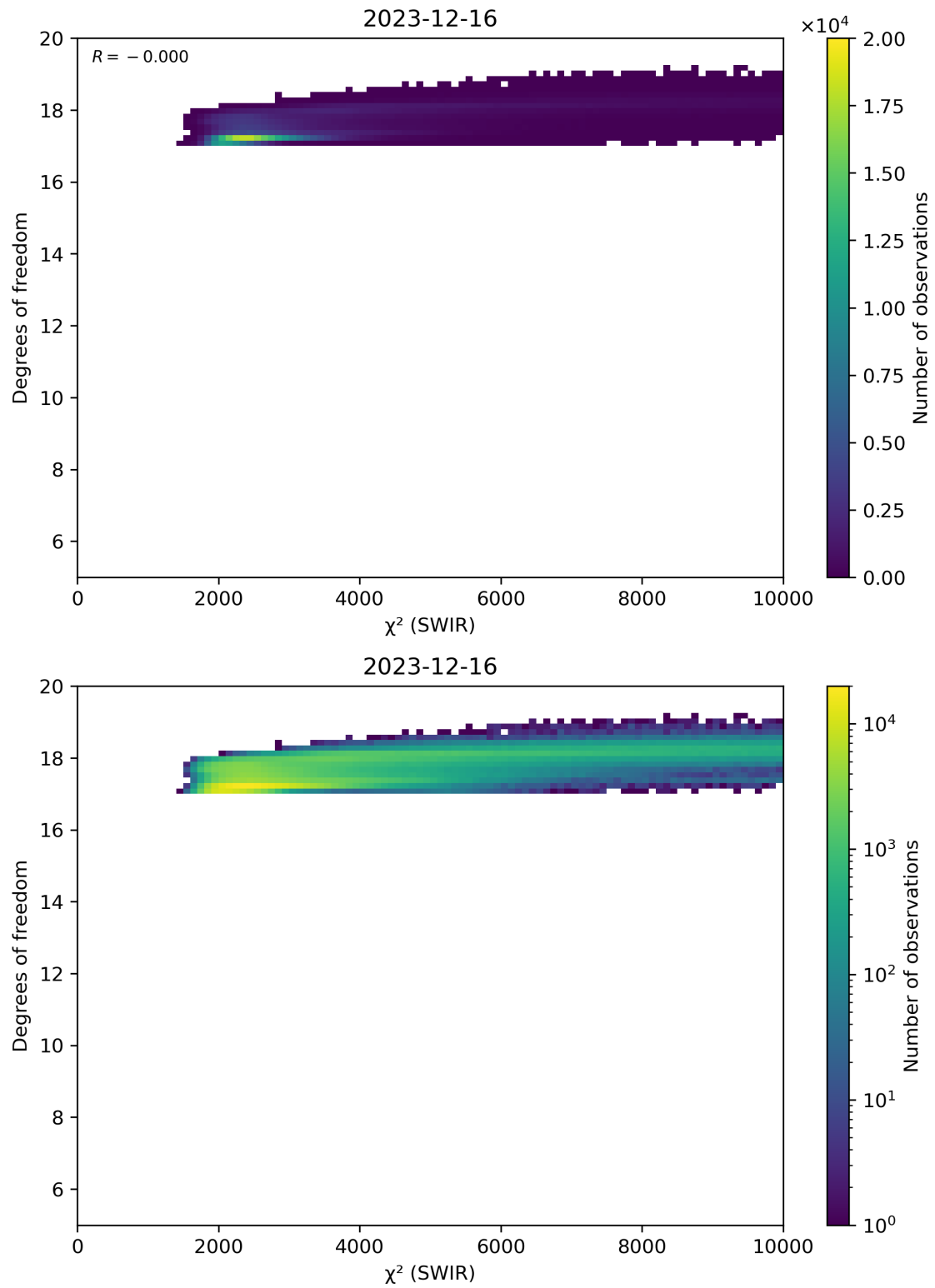
Figure 48: Scatter density plot of “ \chi^2 (SWIR)” against “Degrees of freedom” for 2023-12-15 to 2023-12-17.
