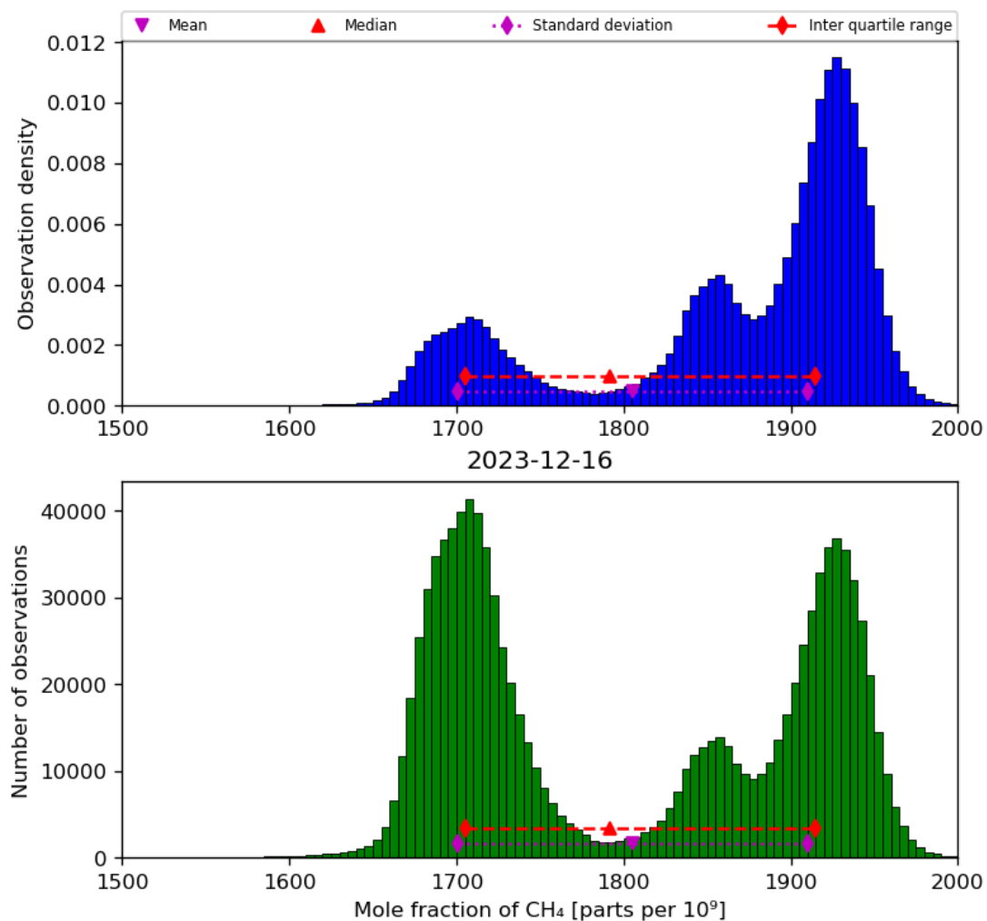
Figure 23: Histogram of “Mole fraction of CH 4 ” for 2023-12-15 to 2023-12-17
