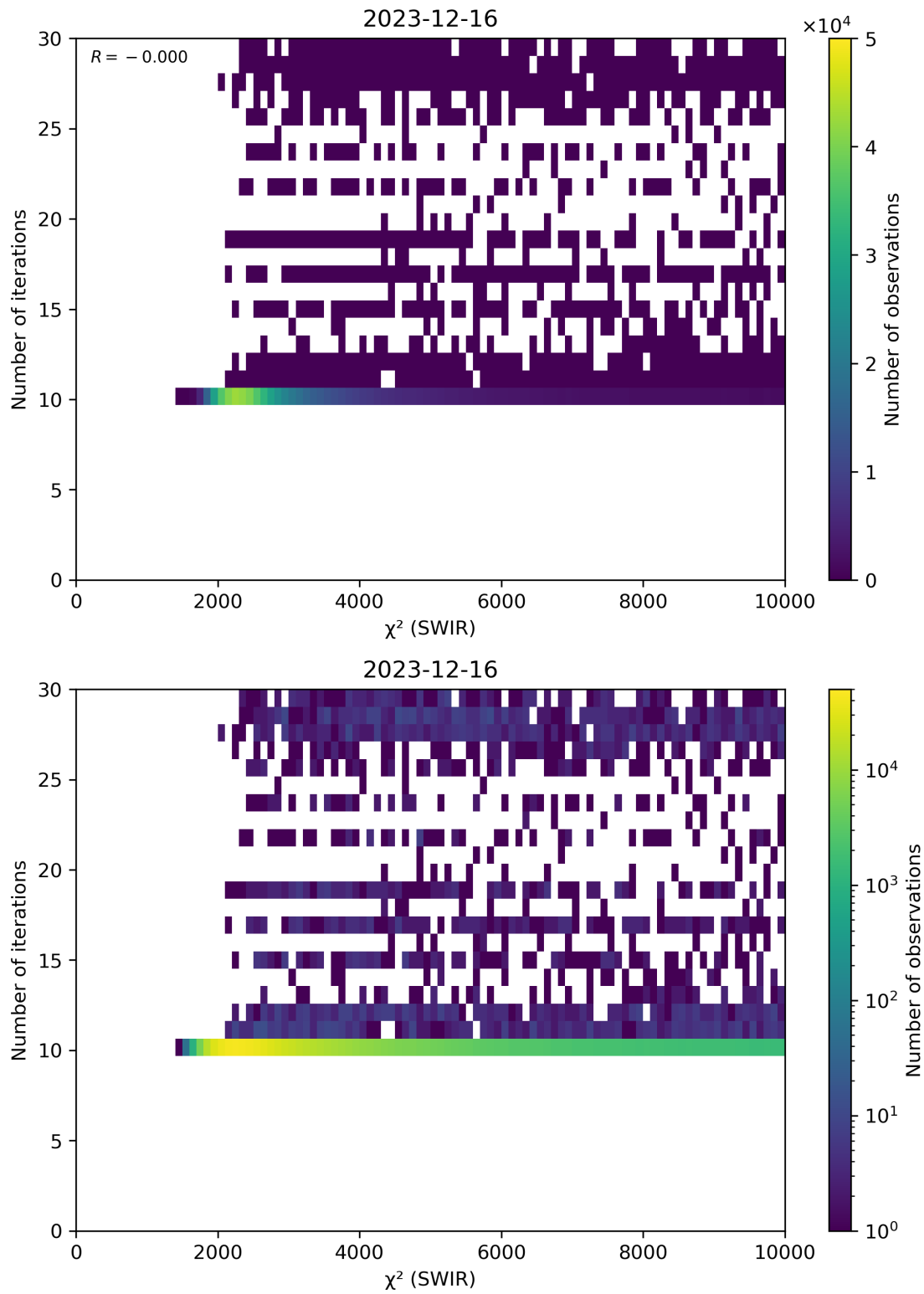
Figure 50: Scatter density plot of “ \chi^2 (SWIR)” against “Number of iterations” for 2023-12-15 to 2023-12-17.
