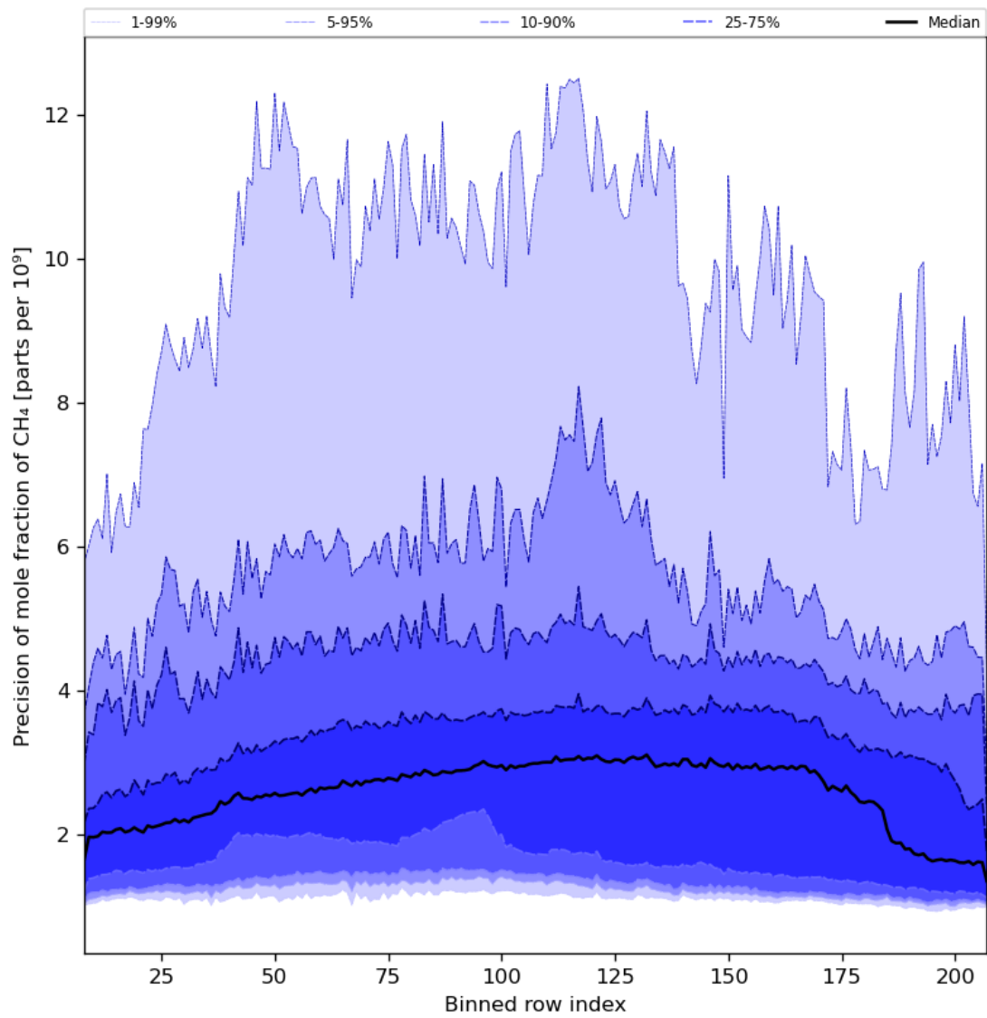
Figure 35: Along track statistics of “Precision of mole fraction of CH 4 ” for 2023-12-15 to 2023-12-17
