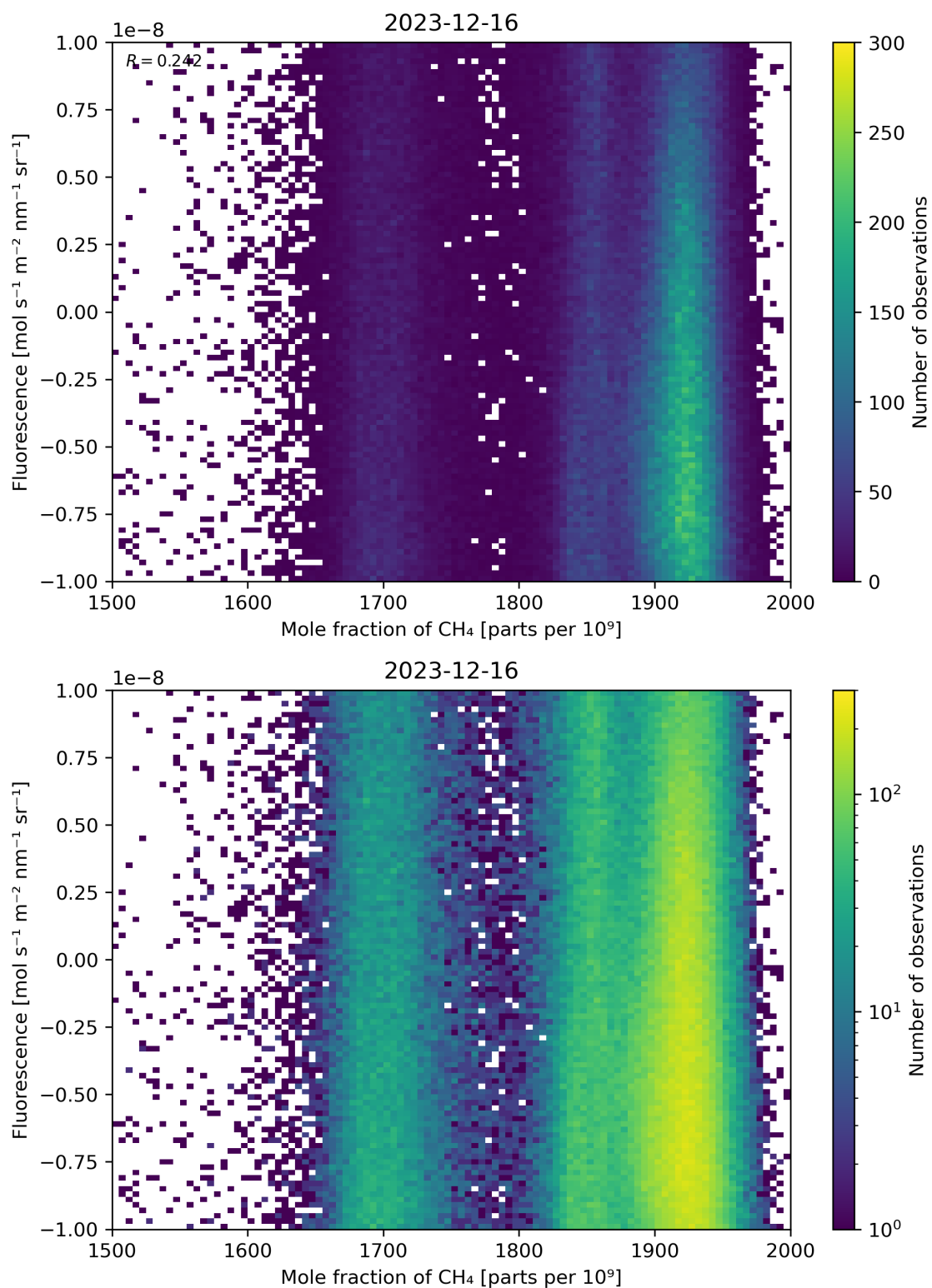
Figure 73: Scatter density plot of “Mole fraction of \text{CH}_4 ” against “Fluorescence” for 2023-12-15 to 2023-12-17.
