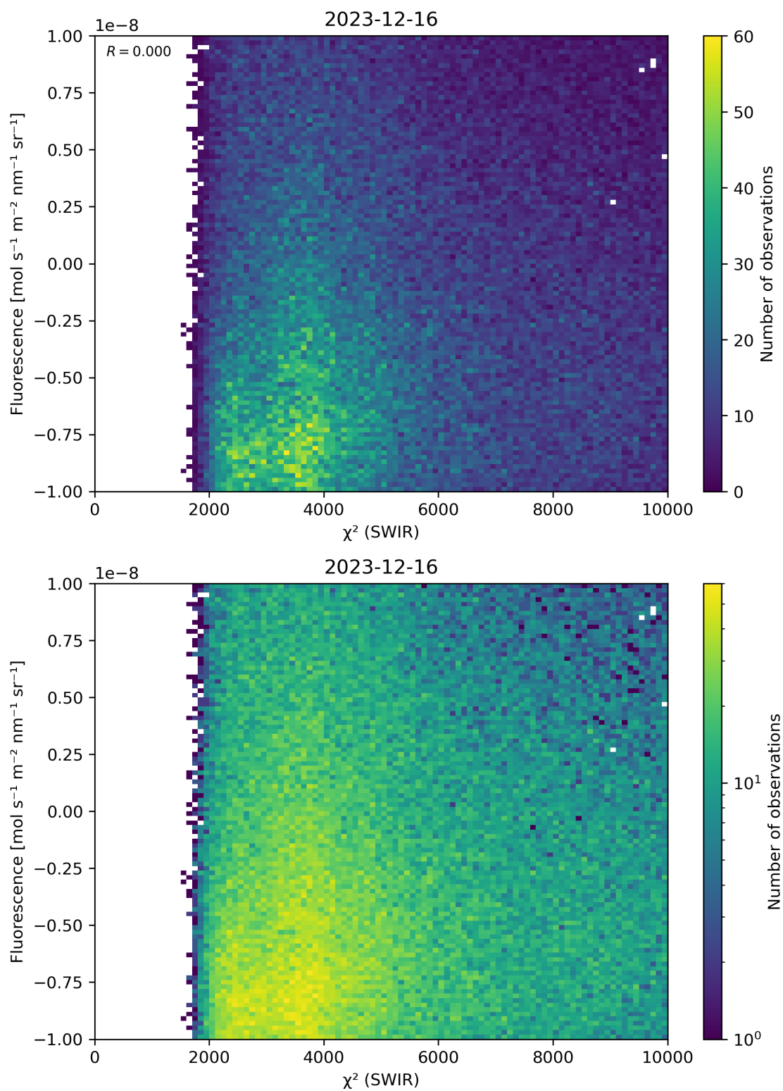
Figure 49: Scatter density plot of “ \chi^2 (SWIR)” against “Fluorescence” for 2023-12-15 to 2023-12-17.
