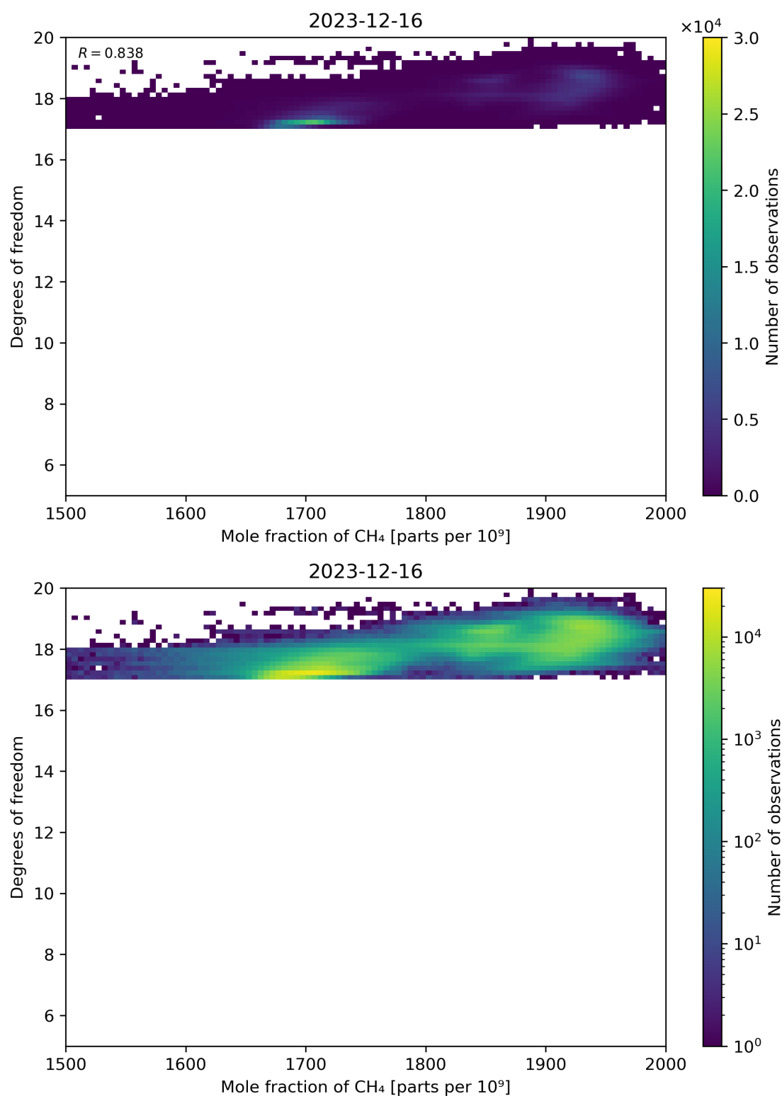
Figure 72: Scatter density plot of “Mole fraction of CH 4 ” against “Degrees of freedom” for 2023-12-15 to 2023-12-17.
