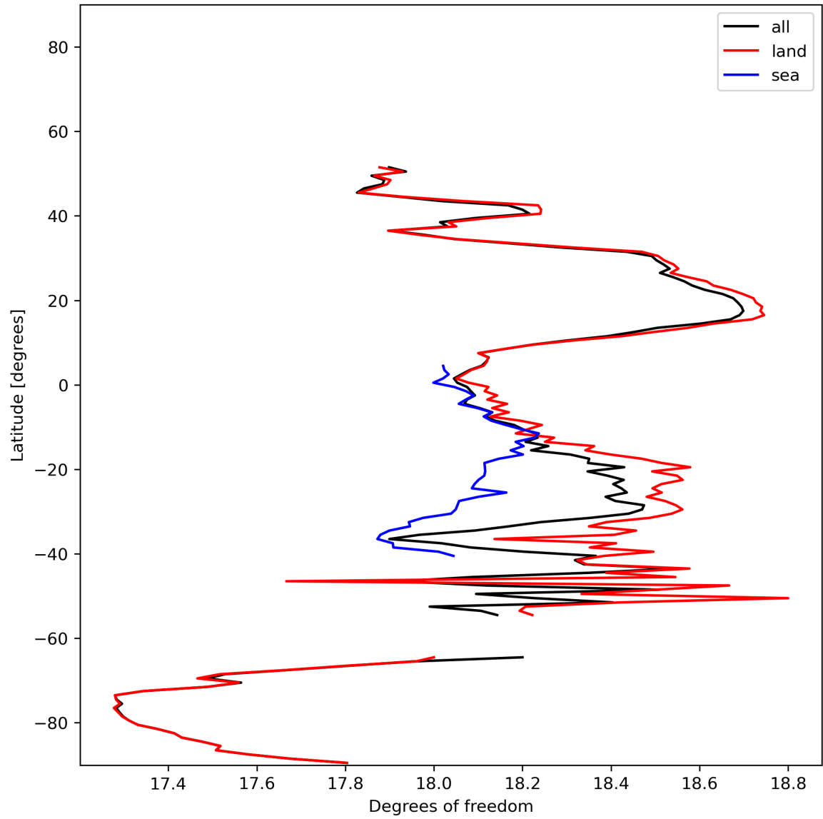
Figure 19: Zonal average of “Degrees of freedom” for 2023-12-15 to 2023-12-17.
