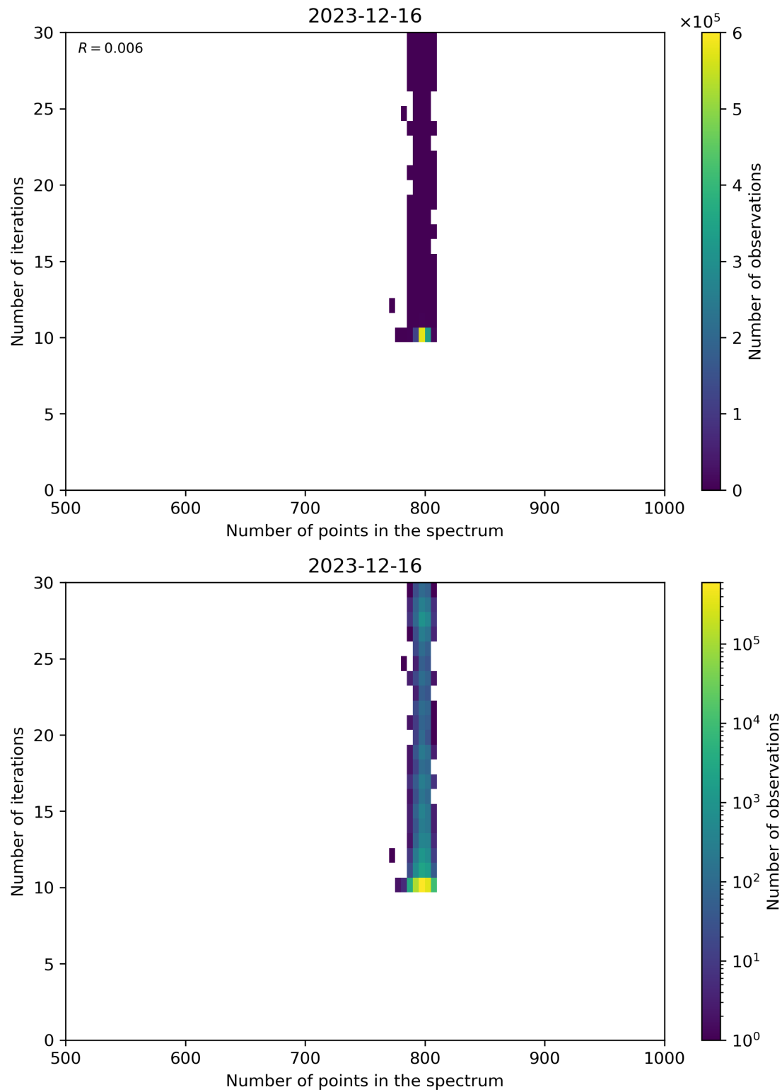
Figure 92: Scatter density plot of “Number of points in the spectrum” against “Number of iterations” for 2023-12-15 to 2023-12-17.
