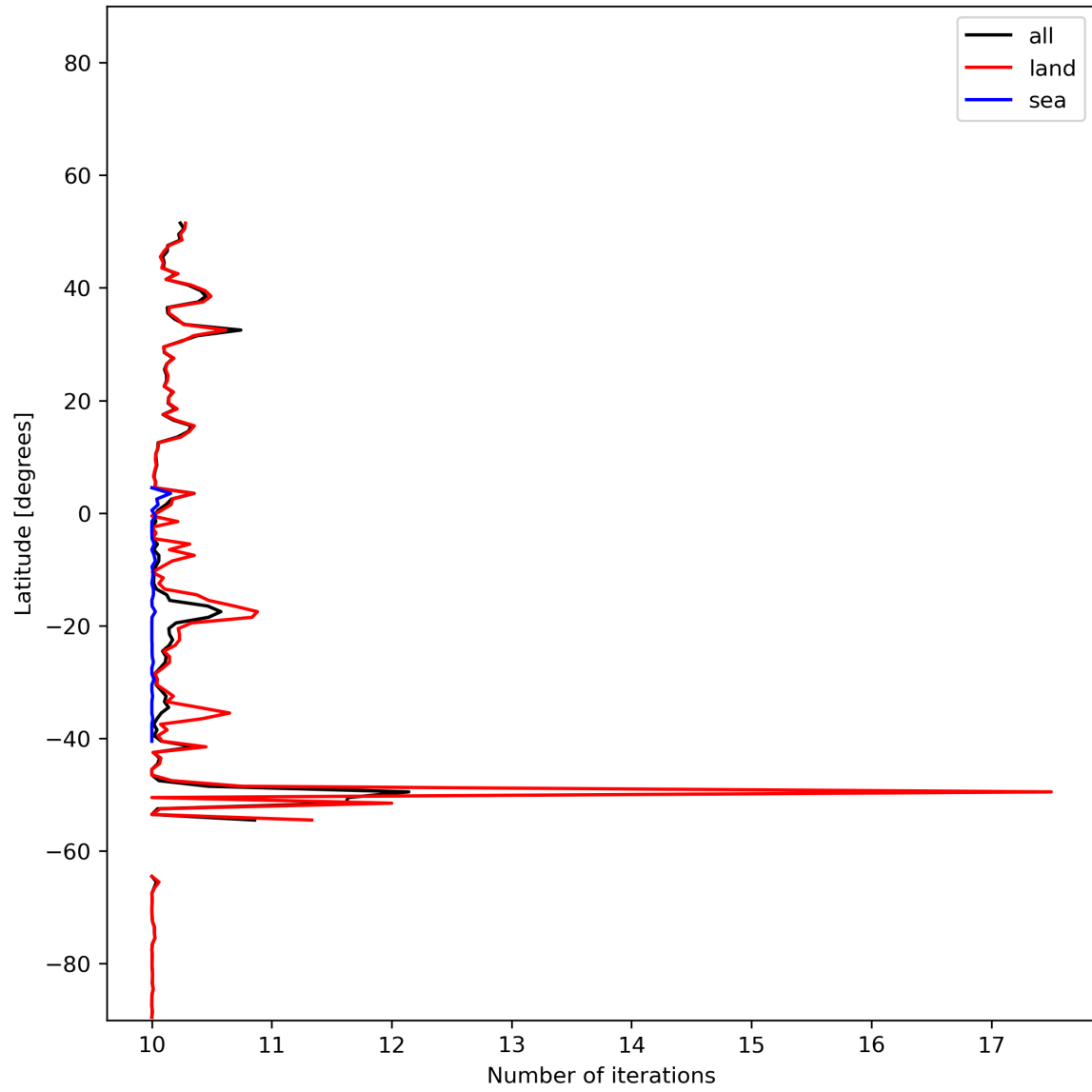
Figure 20: Zonal average of “Number of iterations” for 2023-12-15 to 2023-12-17.
