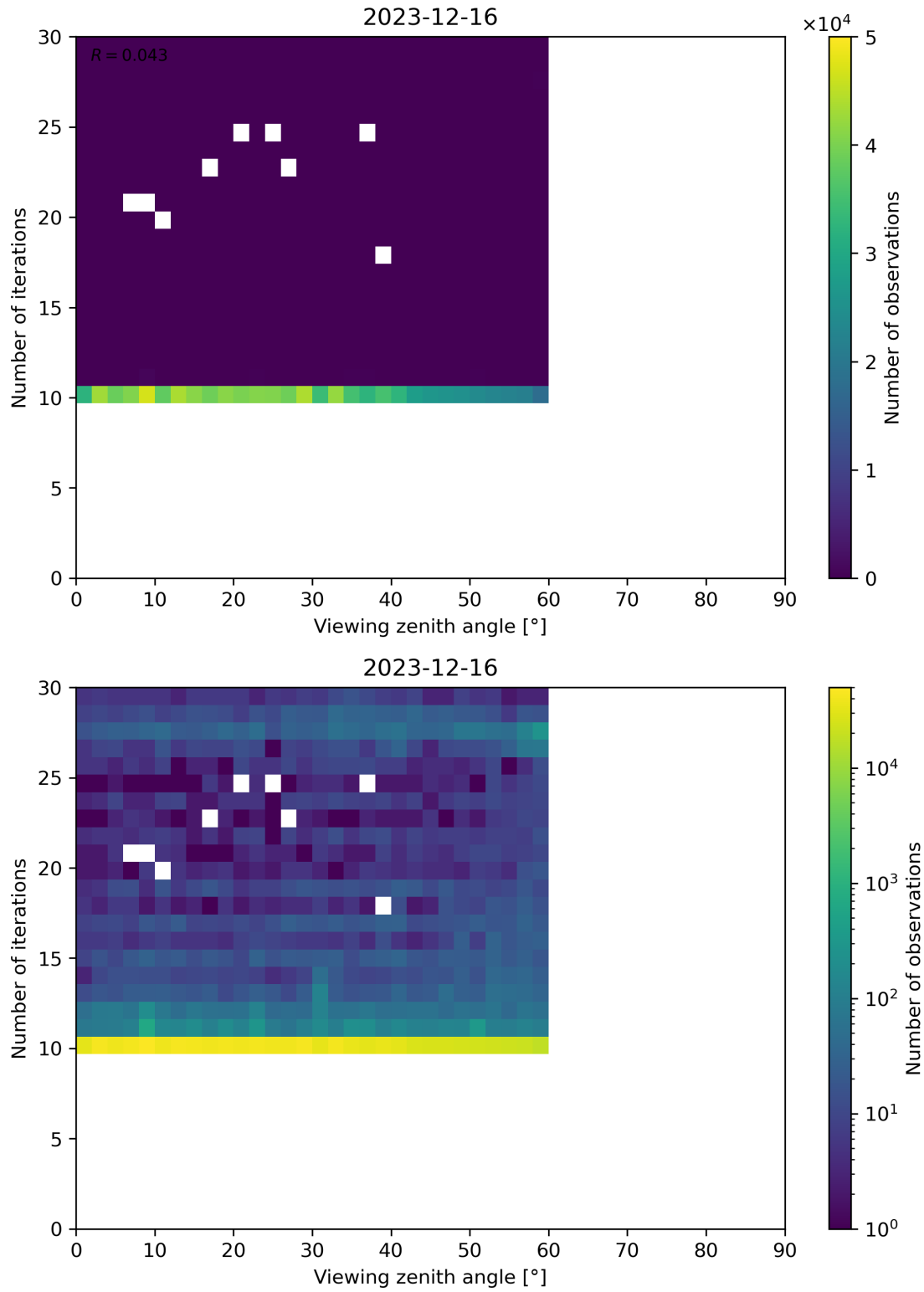
Figure 113: Scatter density plot of “Viewing zenith angle” against “Number of iterations” for 2023-12-15 to 2023-12-17.
