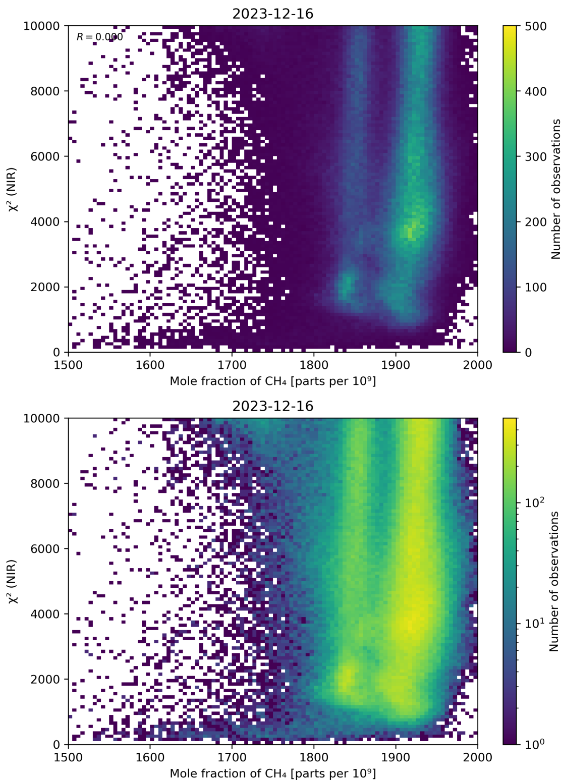
Figure 70: Scatter density plot of “Mole fraction of CH 4 ” against “ \chi^2 (NIR)” for 2023-12-15 to 2023-12-17.
