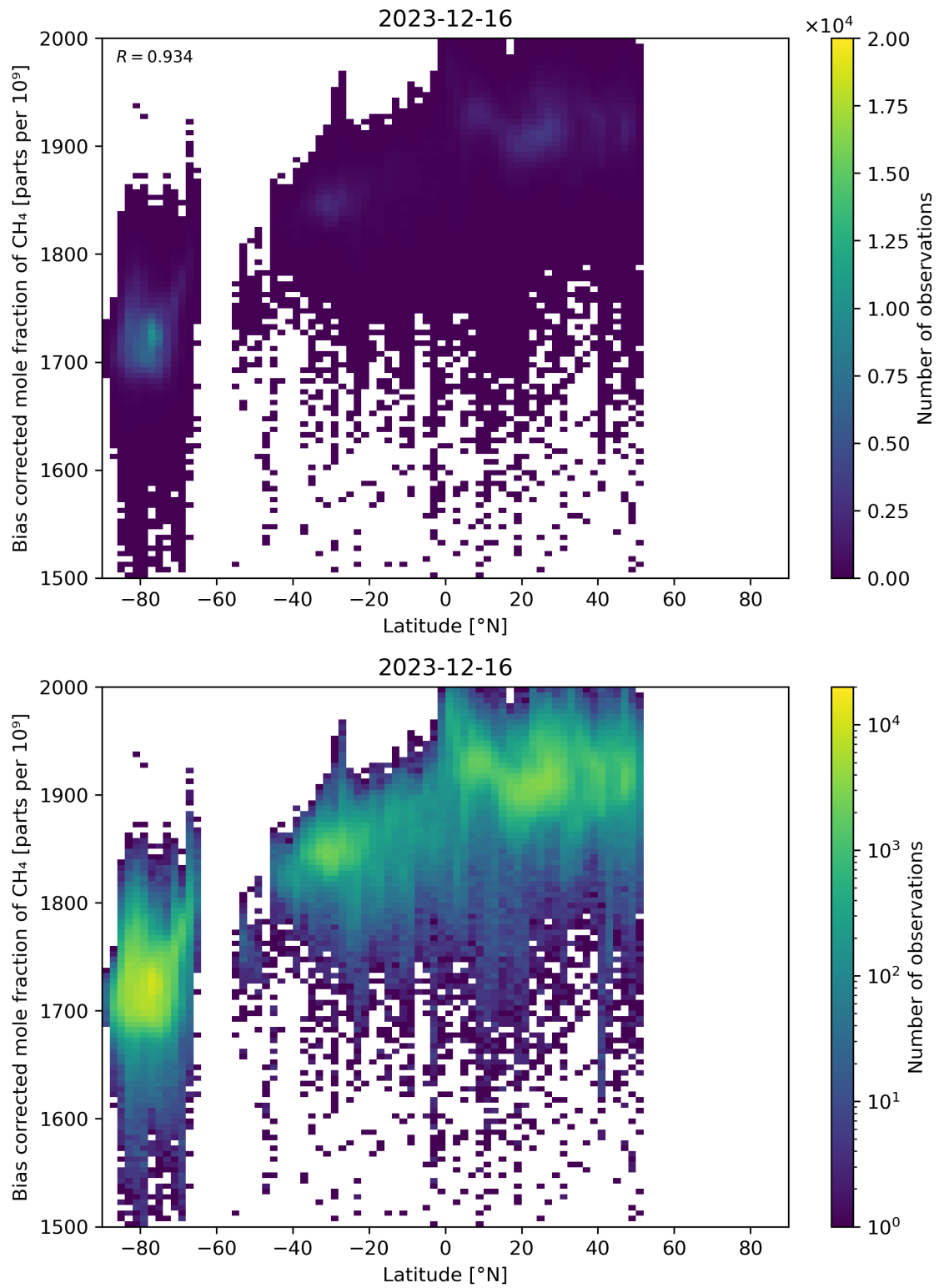
Figure 58: Scatter density plot of “Latitude” against “Bias corrected mole fraction of CH 4 ” for 2023-12-15 to 2023-12-17.
