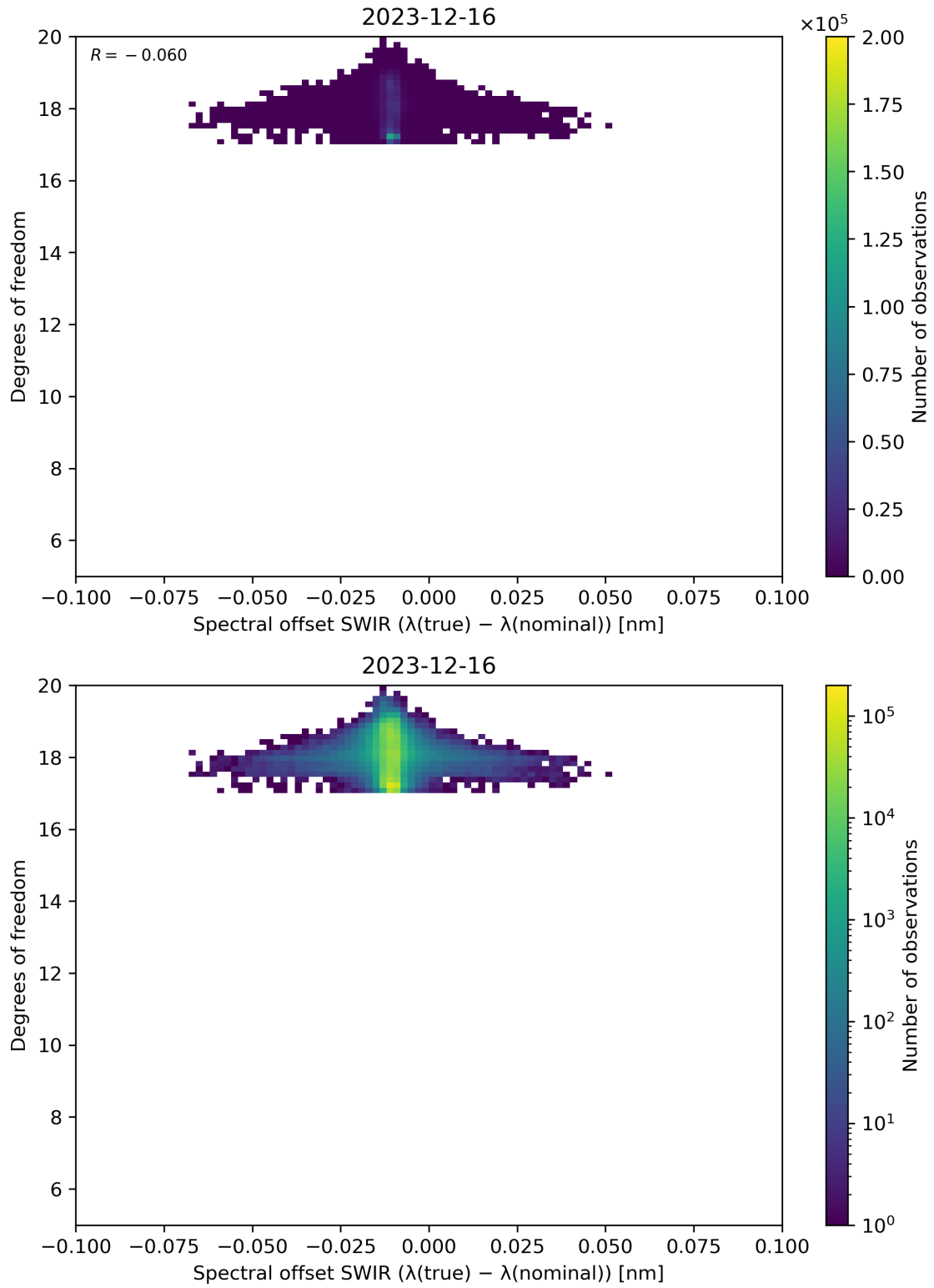
Figure 119: Scatter density plot of “Spectral offset SWIR ( \lambda(\text{true}) - \lambda(\text{nominal}) )” against “Degrees of freedom” for 2023-12-15 to 2023-12-17.
