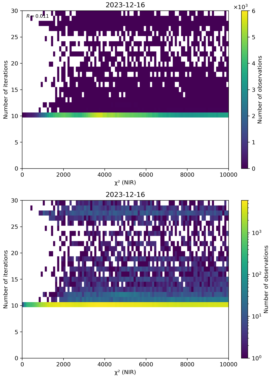
Figure 46: Scatter density plot of “ \chi^2 (NIR)” against “Number of iterations” for 2023-12-15 to 2023-12-17.
