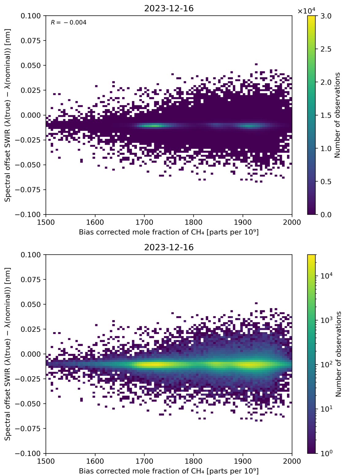
Figure 69: Scatter density plot of “Bias corrected mole fraction of \text{CH}_4 ” against “Spectral offset SWIR ( \lambda(\text{true}) - \lambda(\text{nominal}) )” for 2023-12-15 to 2023-12-17.
