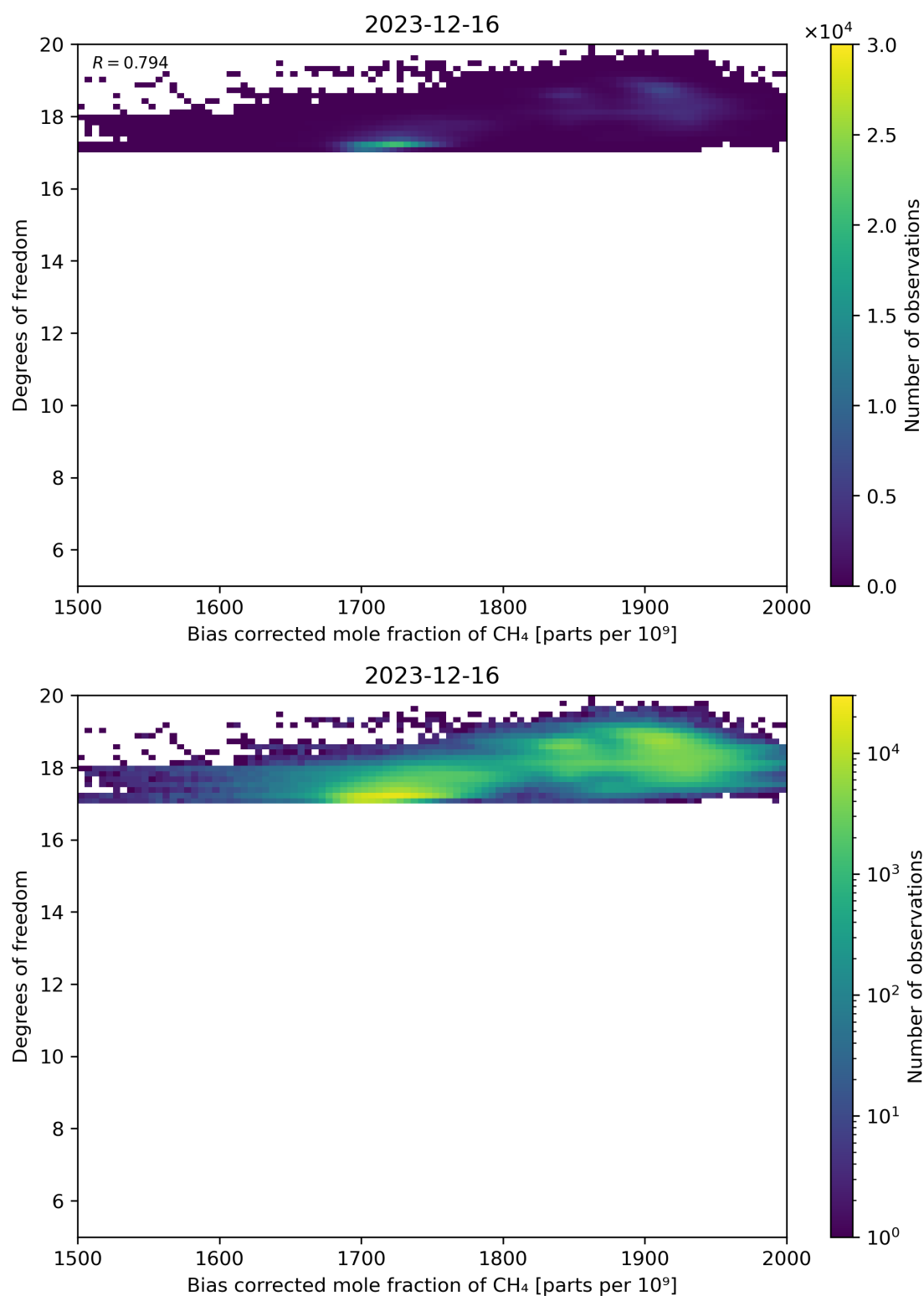
Figure 65: Scatter density plot of “Bias corrected mole fraction of CH 4 ” against “Degrees of freedom” for 2023-12-15 to 2023-12-17.
