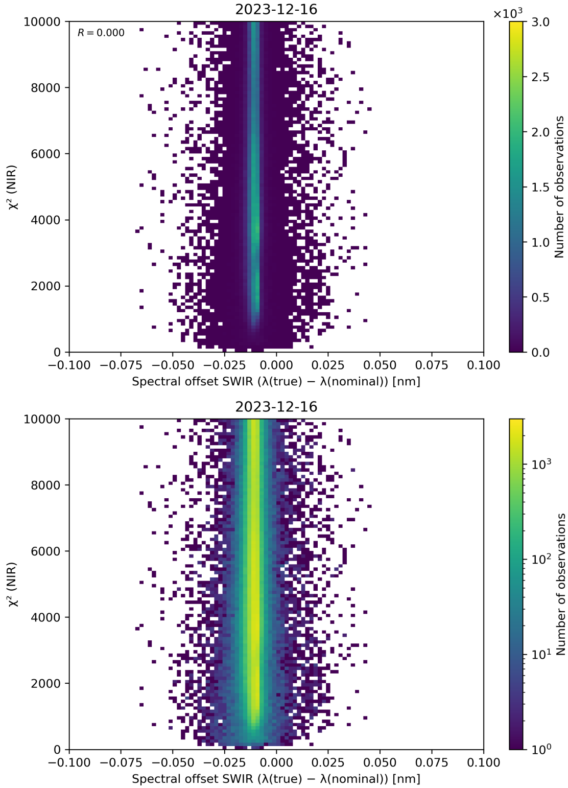
Figure 117: Scatter density plot of “Spectral offset SWIR ( \lambda(\text{true}) - \lambda(\text{nominal}) )” against “ \chi^2 (NIR)” for 2023-12-15 to 2023-12-17.
