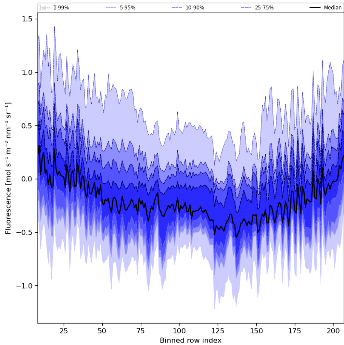
Figure 43: Along track statistics of “Fluorescence” for 2023-12-15 to 2023-12-17
