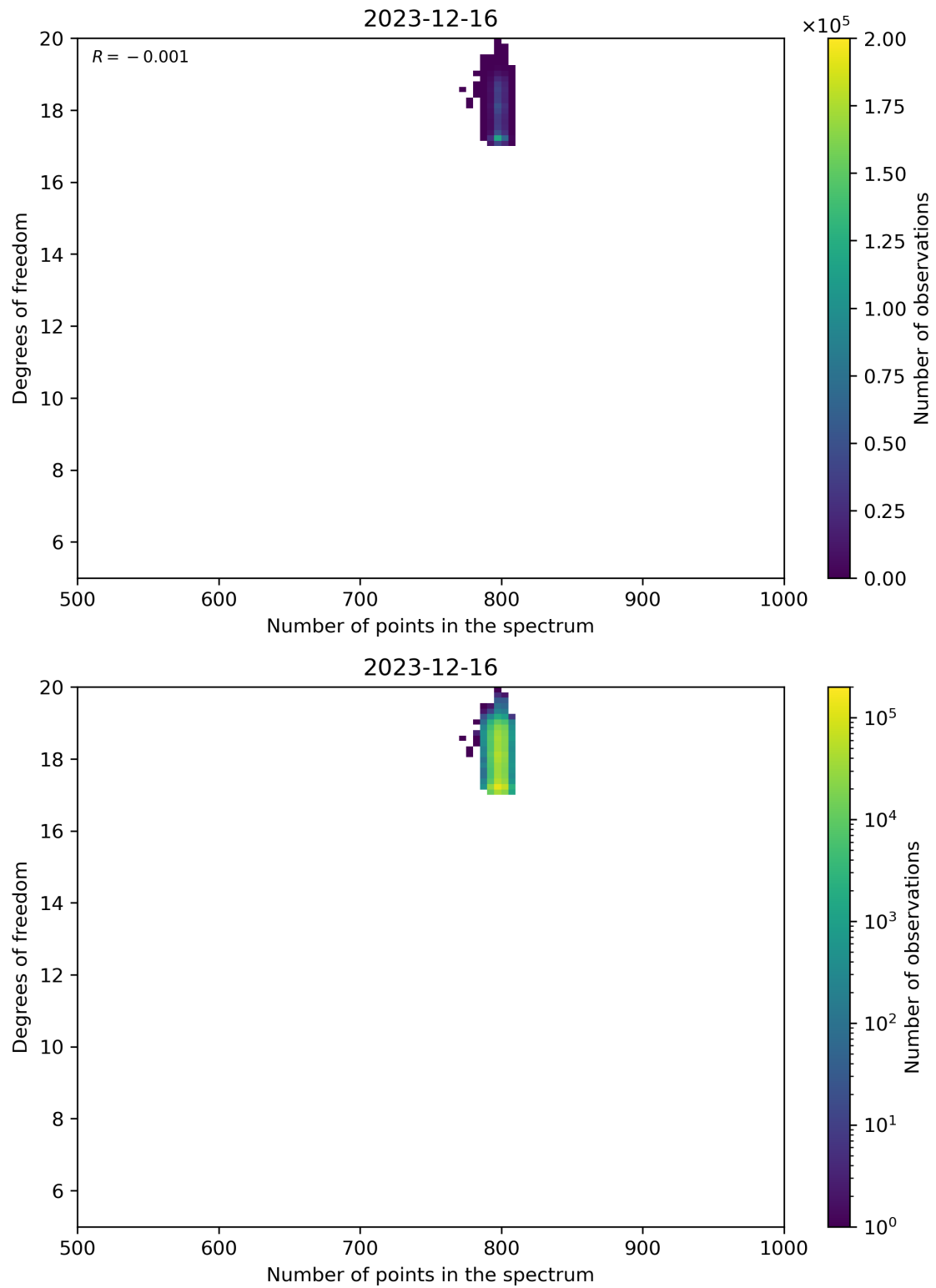
Figure 90: Scatter density plot of “Number of points in the spectrum” against “Degrees of freedom” for 2023-12-15 to 2023-12-17.
