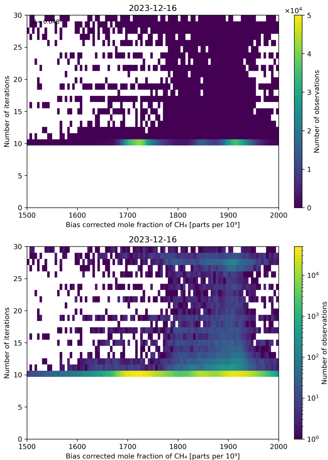
Figure 67: Scatter density plot of “Bias corrected mole fraction of \text{CH}_4 ” against “Number of iterations” for 2023-12-15 to 2023-12-17.
