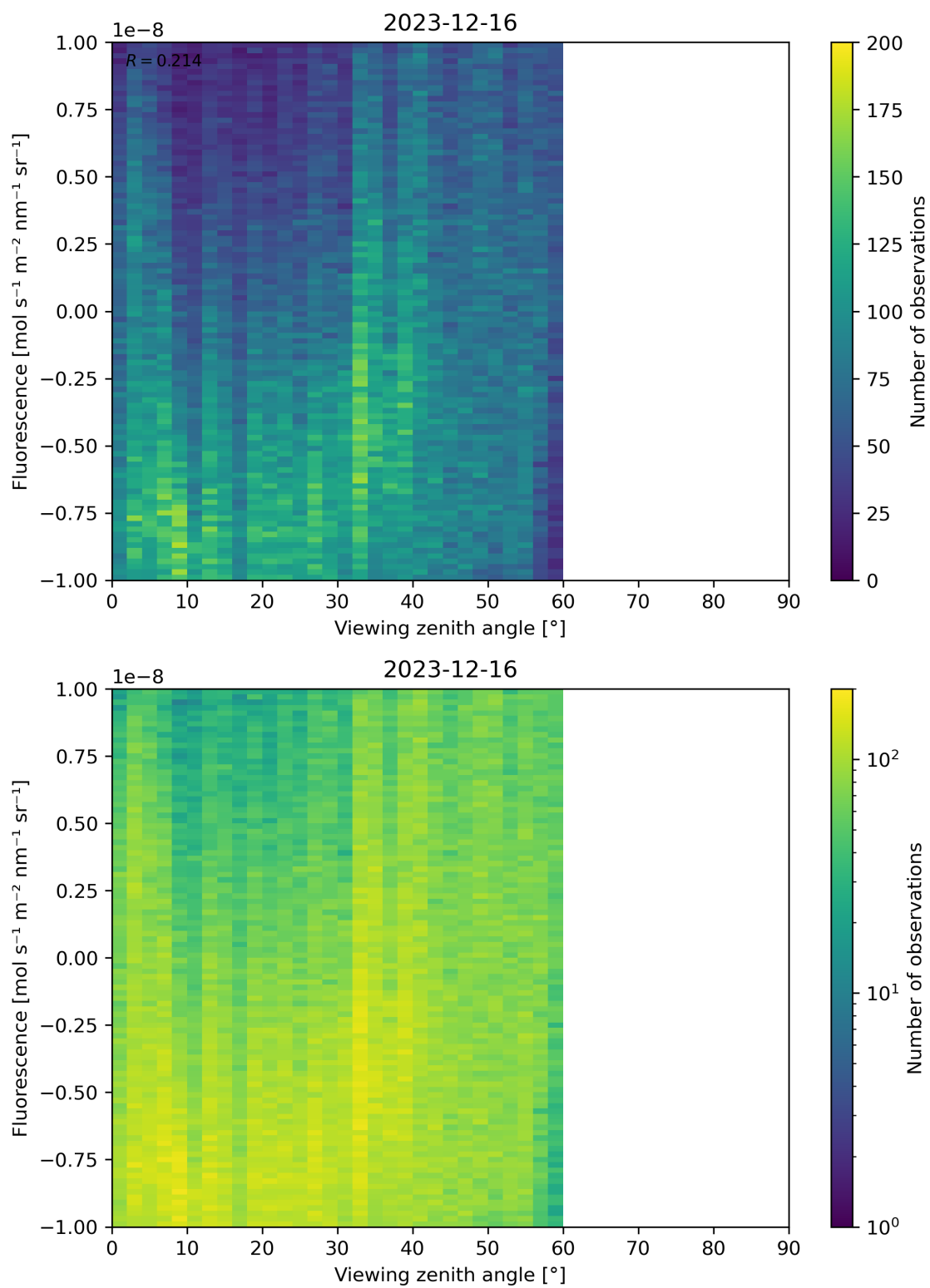
Figure 108: Scatter density plot of “Viewing zenith angle” against “Fluorescence” for 2023-12-15 to 2023-12-17.
