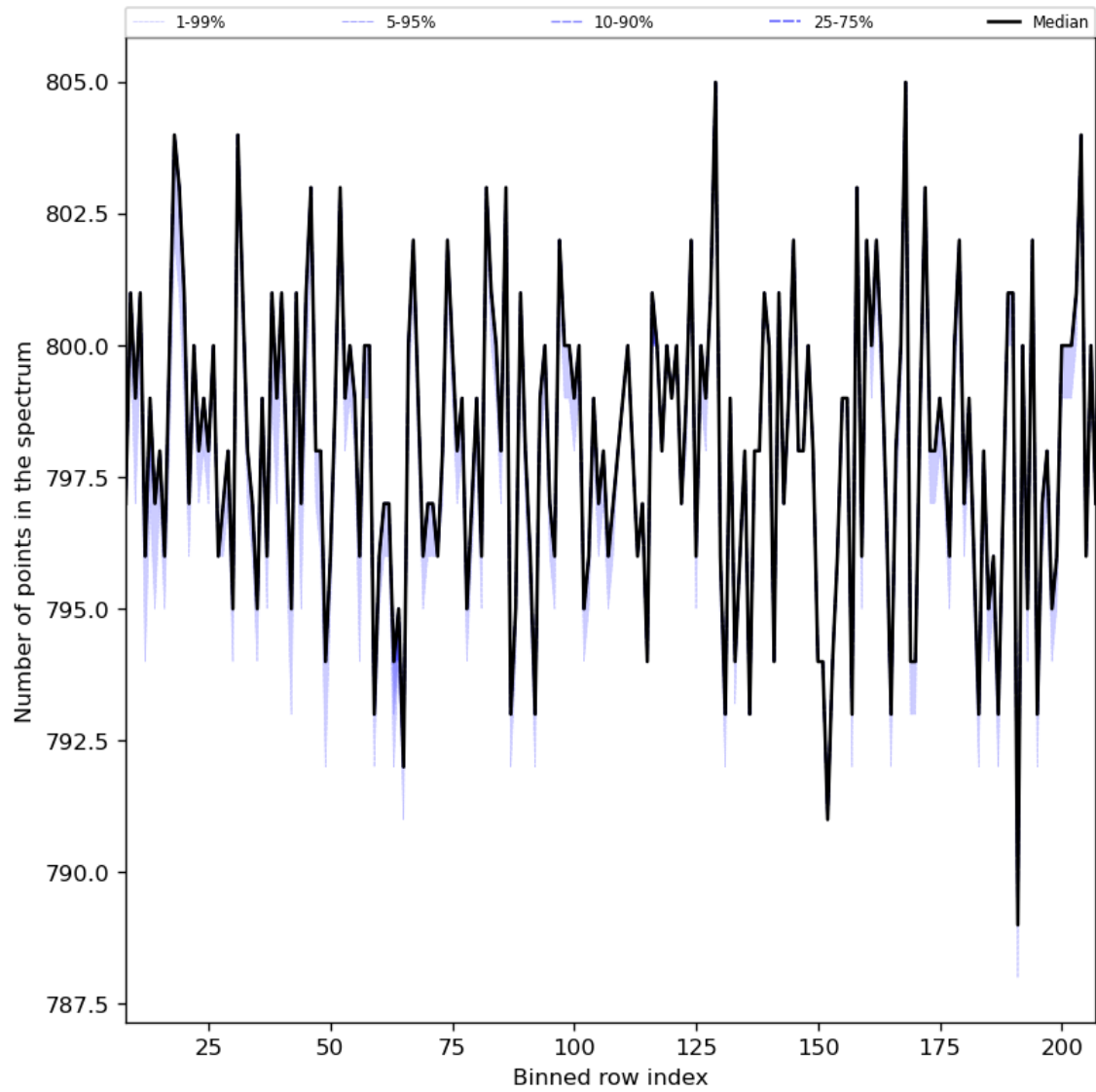
Figure 37: Along track statistics of “Number of points in the spectrum” for 2023-12-15 to 2023-12-17
