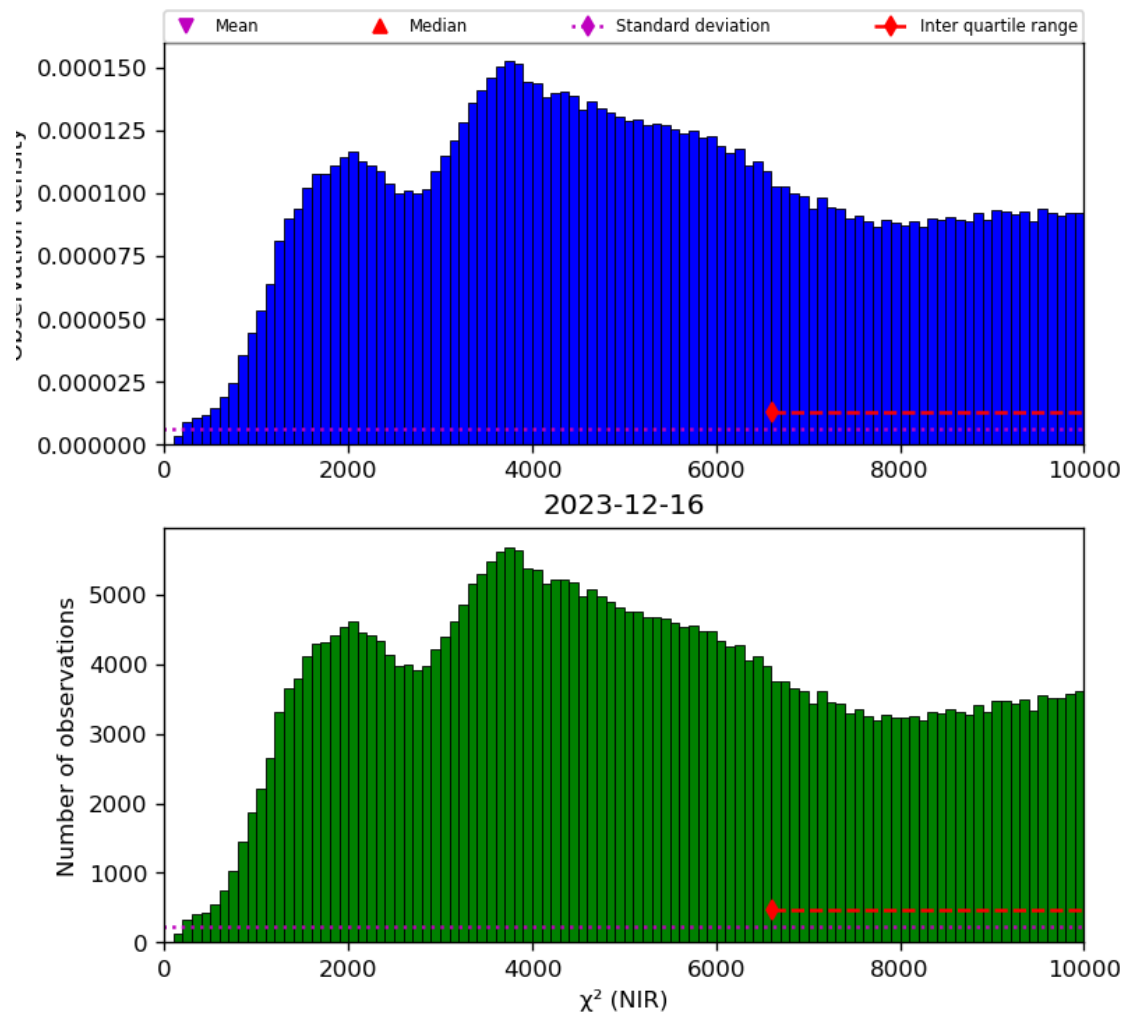
Figure 29: Histogram of “ \chi^2 (NIR)” for 2023-12-15 to 2023-12-17
