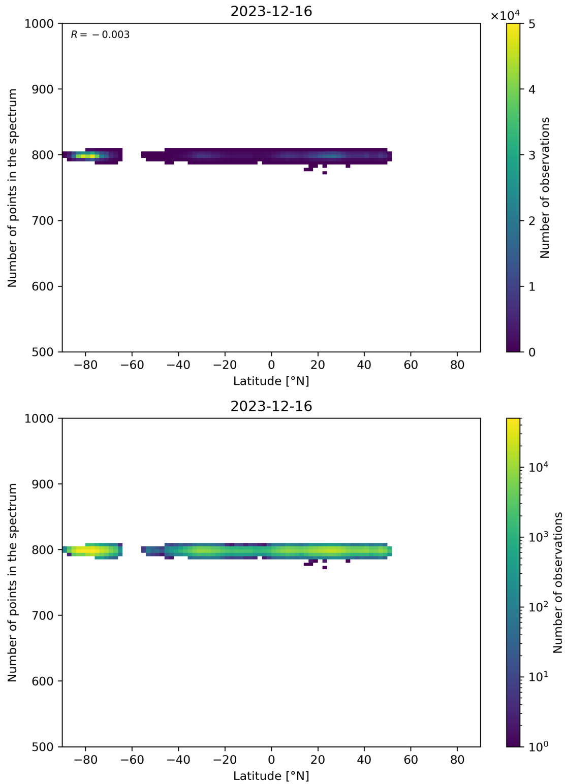
Figure 61: Scatter density plot of “Latitude” against “Number of points in the spectrum” for 2023-12-15 to 2023-12-17.
