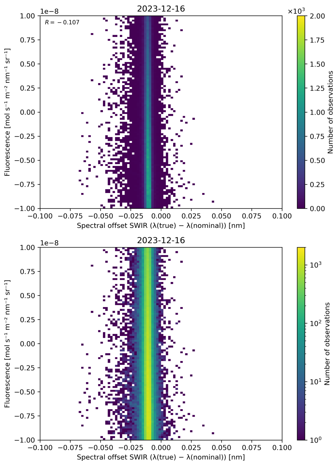
Figure 120: Scatter density plot of “Spectral offset SWIR ( \lambda(\text{true}) - \lambda(\text{nominal}) )” against “Fluorescence” for 2023-12-15 to 2023-12-17.
