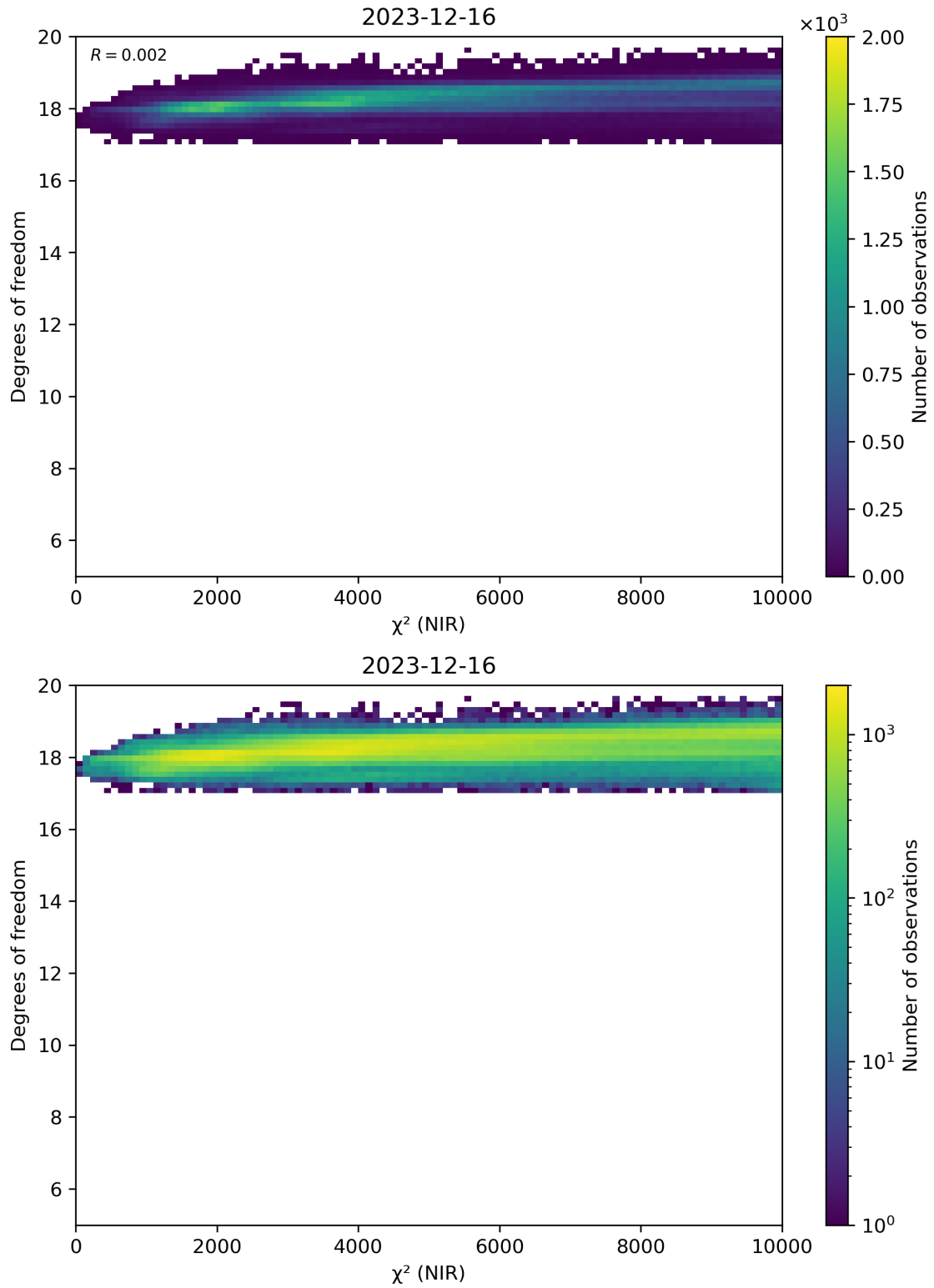
Figure 44: Scatter density plot of “ \chi^2 (NIR)” against “Degrees of freedom” for 2023-12-15 to 2023-12-17.
