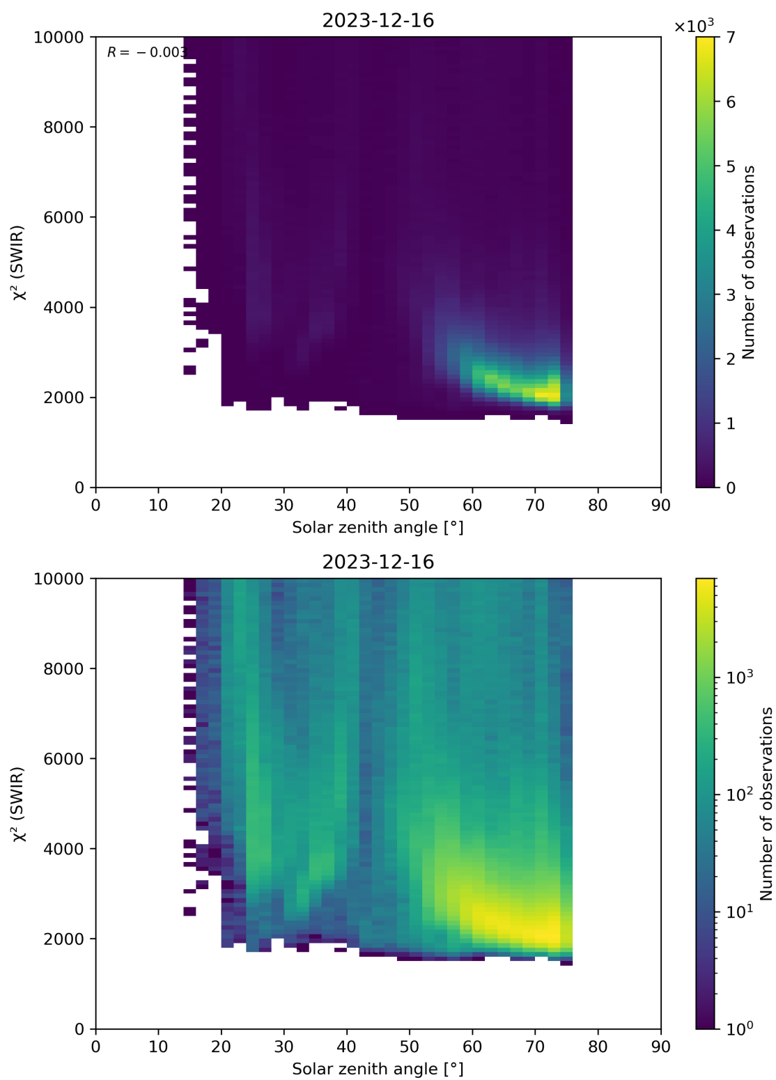
Figure 95: Scatter density plot of “Solar zenith angle” against “ \chi^2 (SWIR)” for 2023-12-15 to 2023-12-17.
