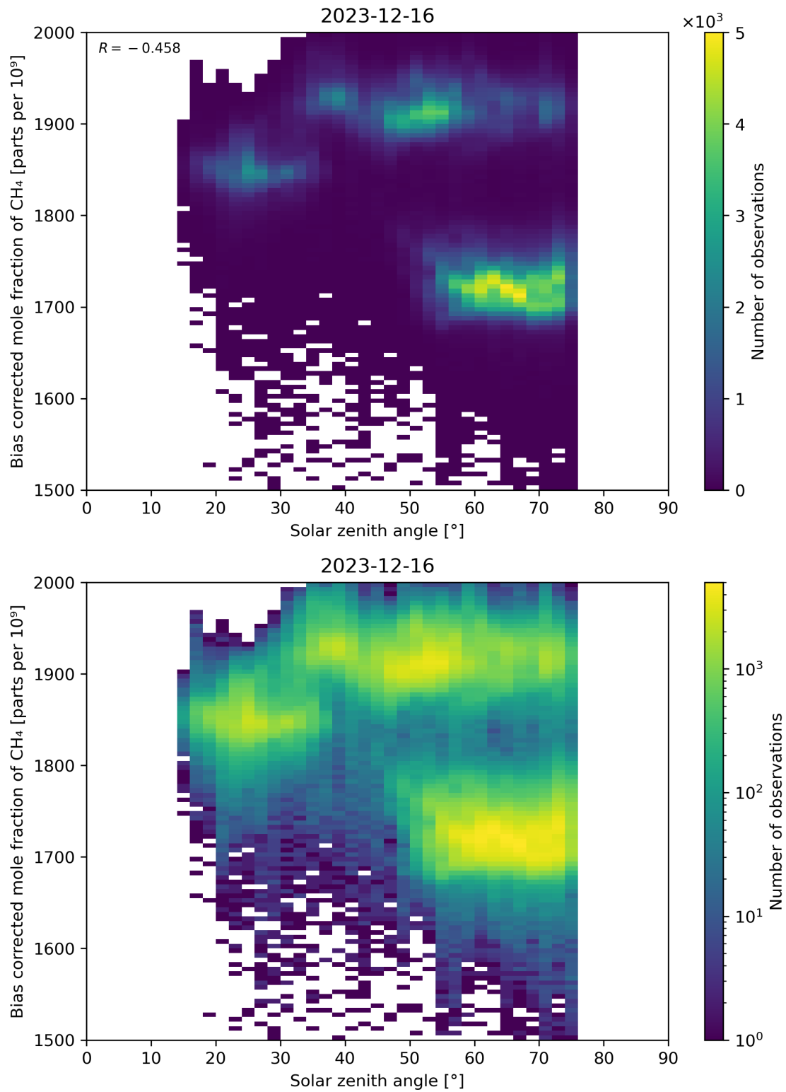
Figure 100: Scatter density plot of “Solar zenith angle” against “Bias corrected mole fraction of \text{CH}_4 ” for 2023-12-15 to 2023-12-17.
