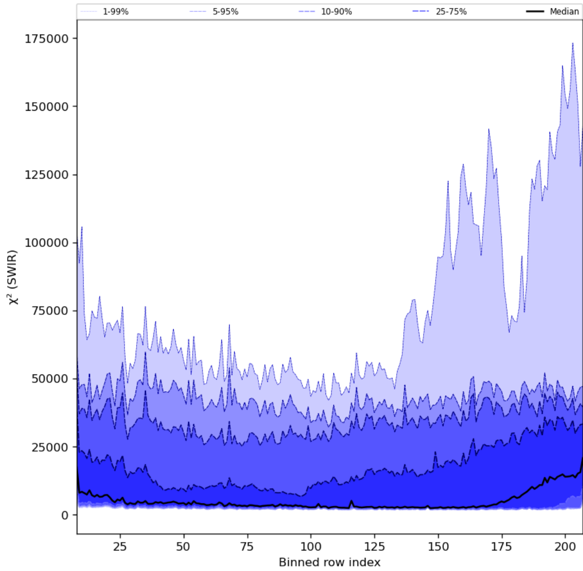
Figure 39: Along track statistics of “ \chi^2 (SWIR)” for 2023-12-15 to 2023-12-17
