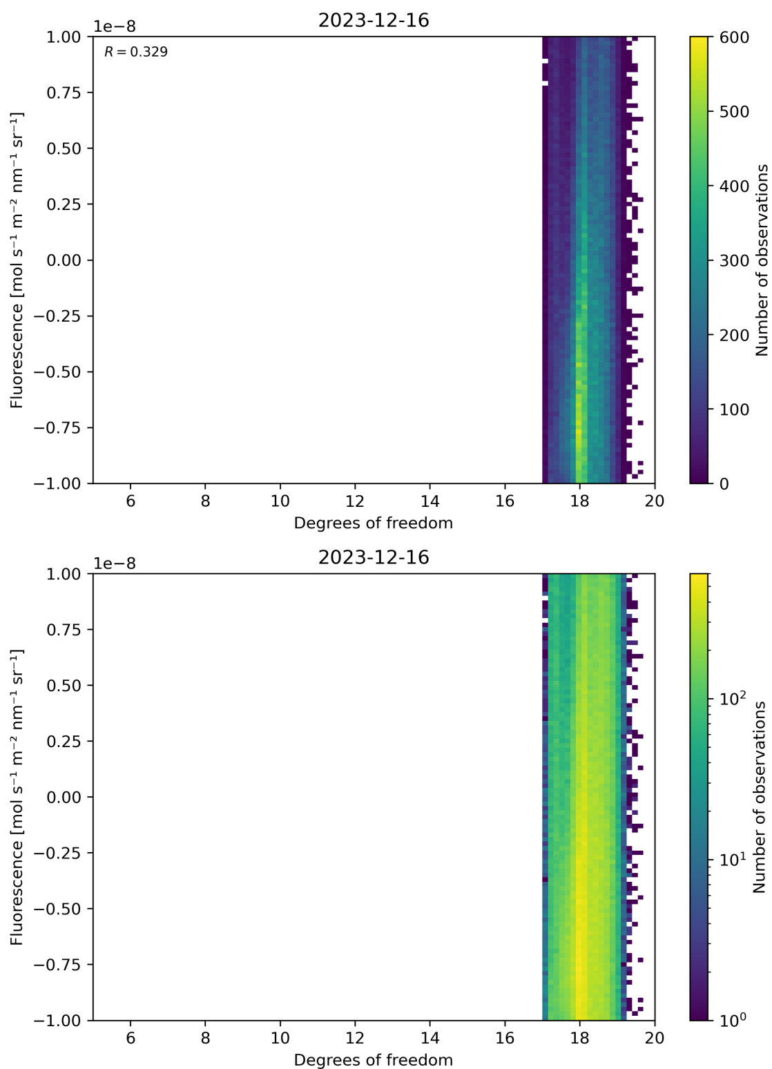
Figure 51: Scatter density plot of “Degrees of freedom” against “Fluorescence” for 2023-12-15 to 2023-12-17.
