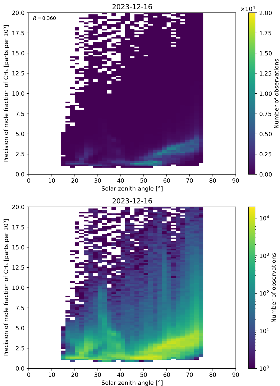
Figure 101: Scatter density plot of “Solar zenith angle” against “Precision of mole fraction of \text{CH}_4 ” for 2023-12-15 to 2023-12-17.
