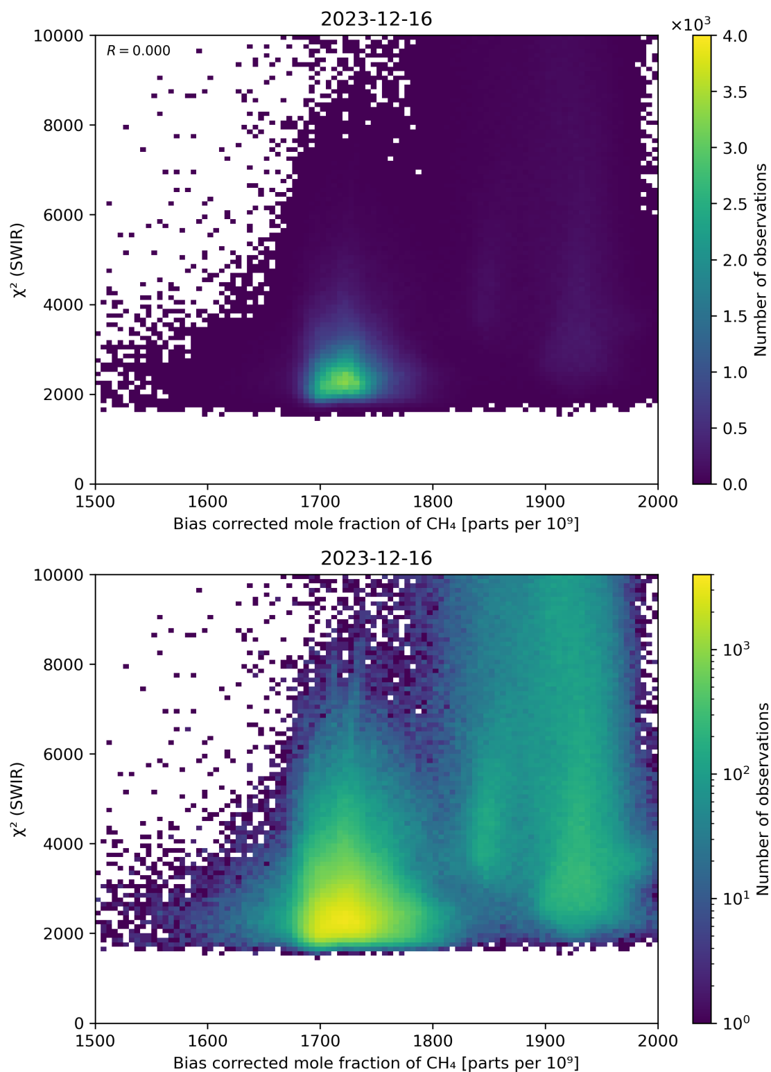
Figure 64: Scatter density plot of “Bias corrected mole fraction of CH 4 ” against “ \chi^2 (SWIR)” for 2023-12-15 to 2023-12-17.
