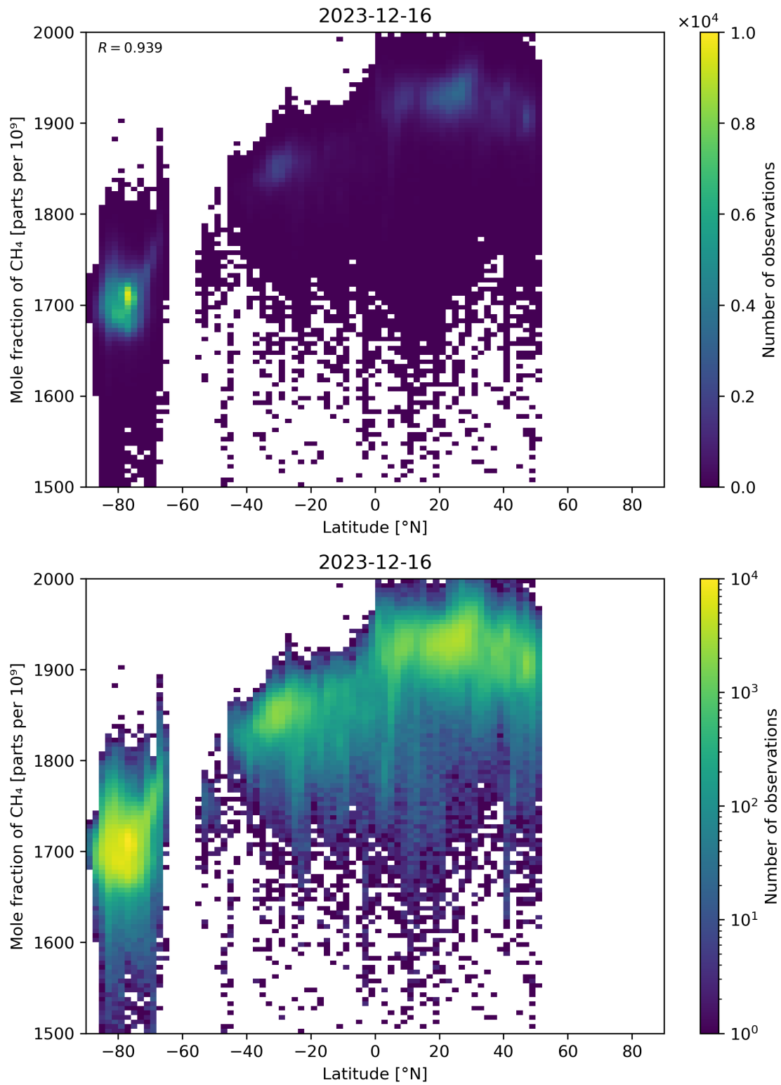
Figure 57: Scatter density plot of “Latitude” against “Mole fraction of \text{CH}_4 ” for 2023-12-15 to 2023-12-17.
