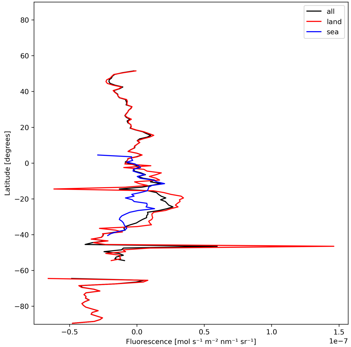
Figure 21: Zonal average of “Fluorescence” for 2023-12-15 to 2023-12-17.
