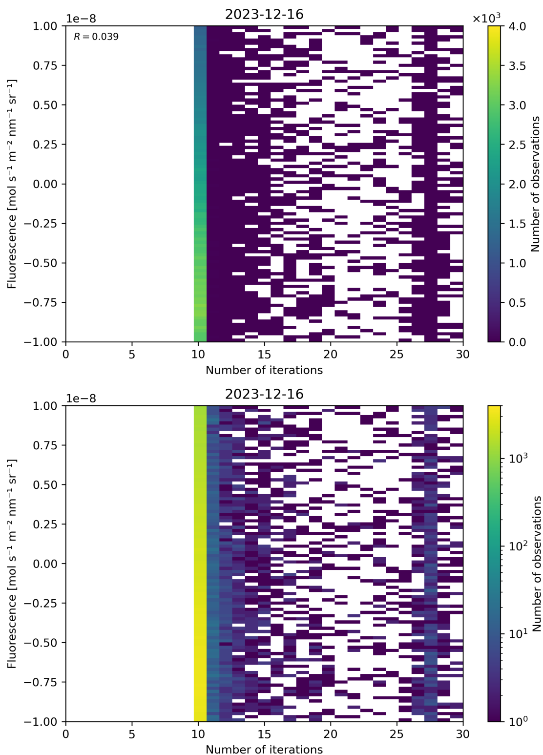
Figure 87: Scatter density plot of “Number of iterations” against “Fluorescence” for 2023-12-15 to 2023-12-17.
