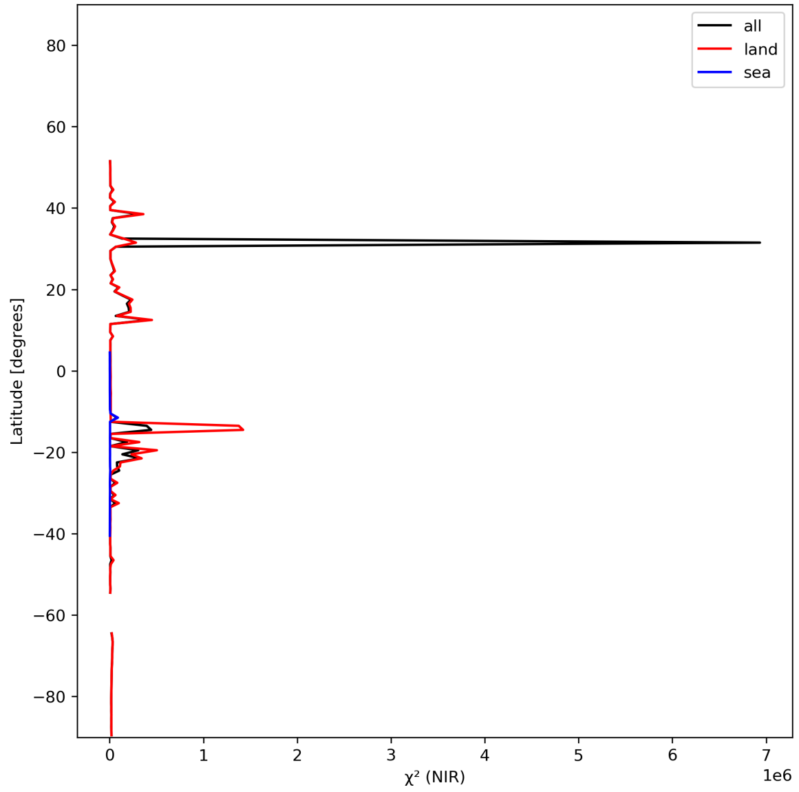
Figure 18: Zonal average of “ \chi^2 (NIR)” for 2023-12-15 to 2023-12-17.
