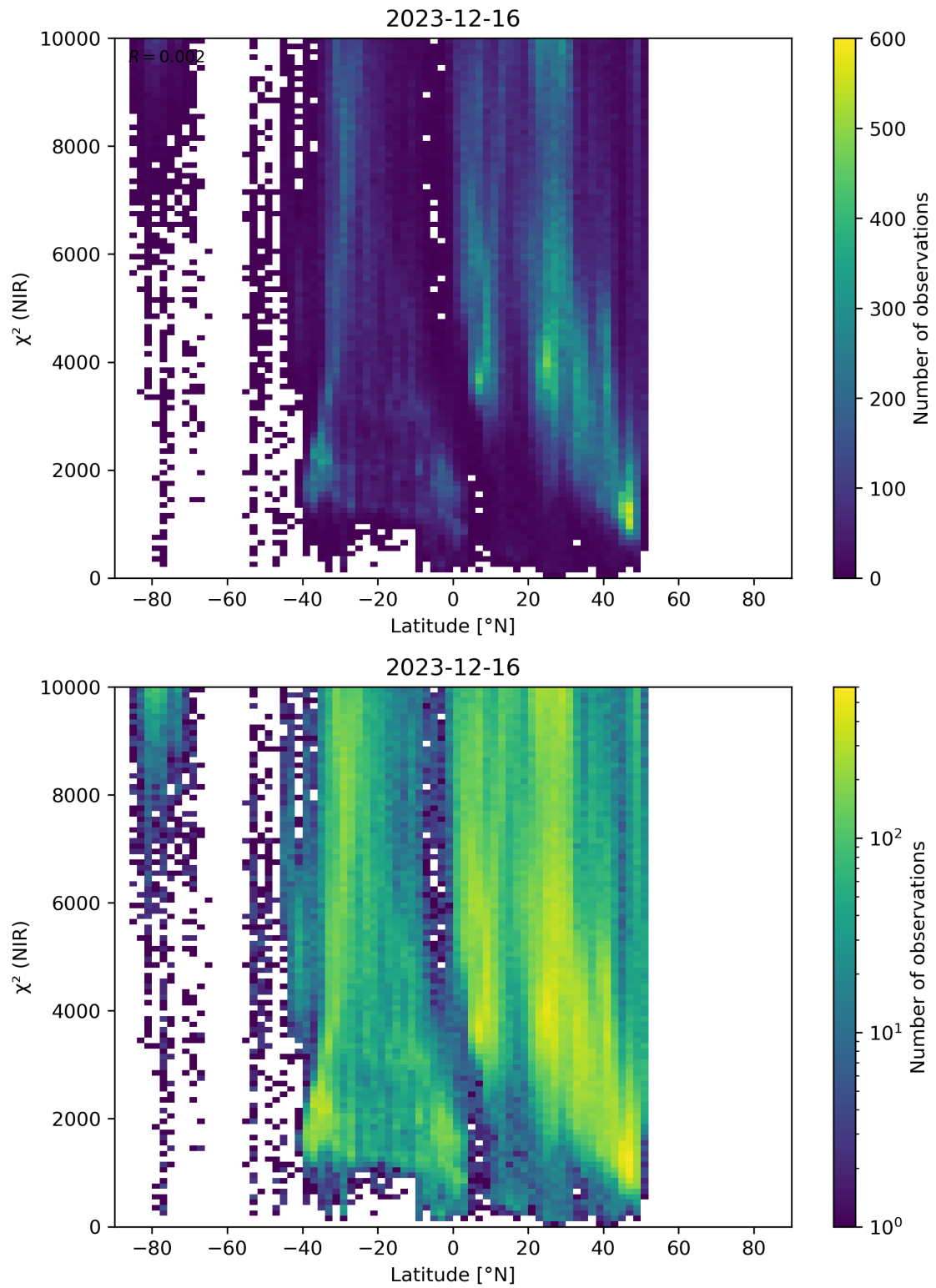
Figure 53: Scatter density plot of “Latitude” against “ \chi^2 (NIR)” for 2023-12-15 to 2023-12-17.
