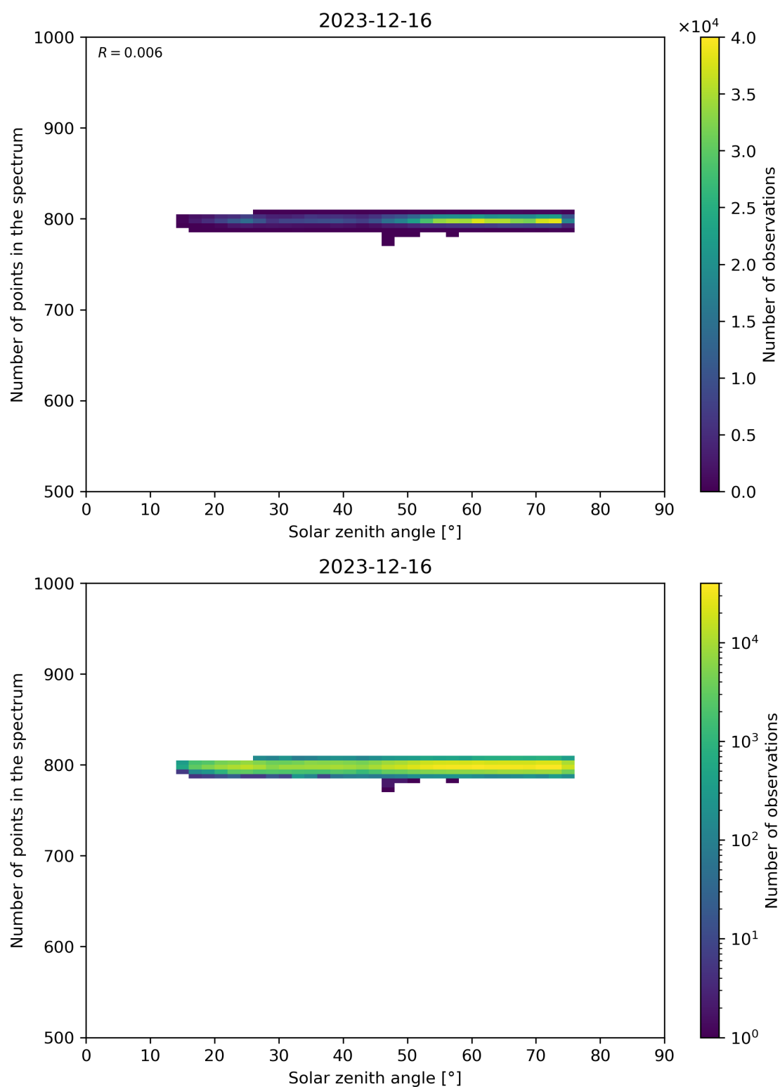
Figure 103: Scatter density plot of “Solar zenith angle” against “Number of points in the spectrum” for 2023-12-15 to 2023-12-17.
