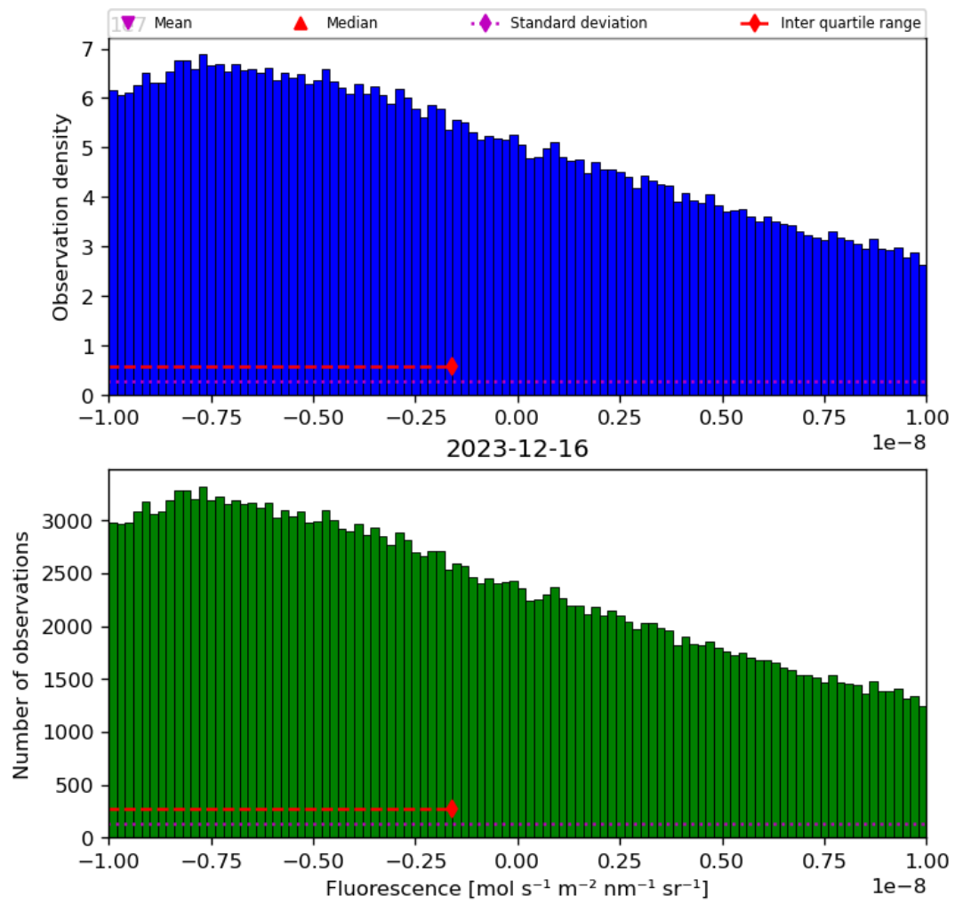
Figure 32: Histogram of “Fluorescence” for 2023-12-15 to 2023-12-17
