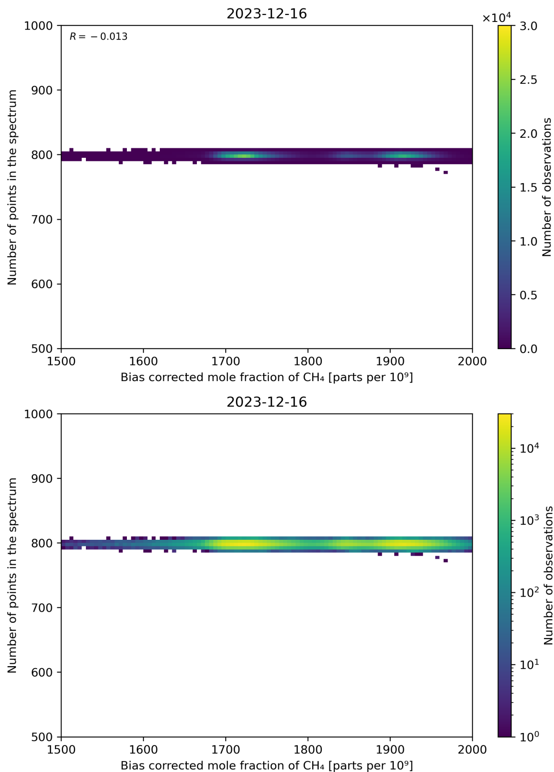
Figure 68: Scatter density plot of “Bias corrected mole fraction of CH 4 ” against “Number of points in the spectrum” for 2023-12-15 to 2023-12-17.
