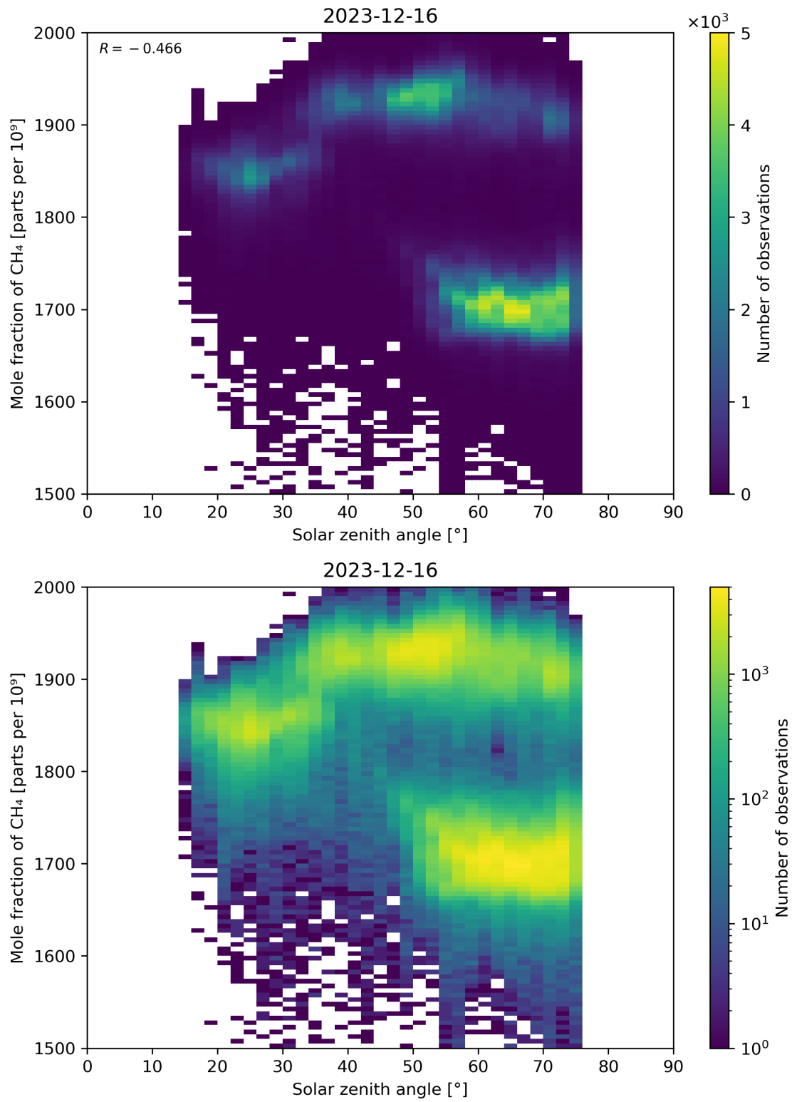
Figure 99: Scatter density plot of “Solar zenith angle” against “Mole fraction of \text{CH}_4 ” for 2023-12-15 to 2023-12-17.
