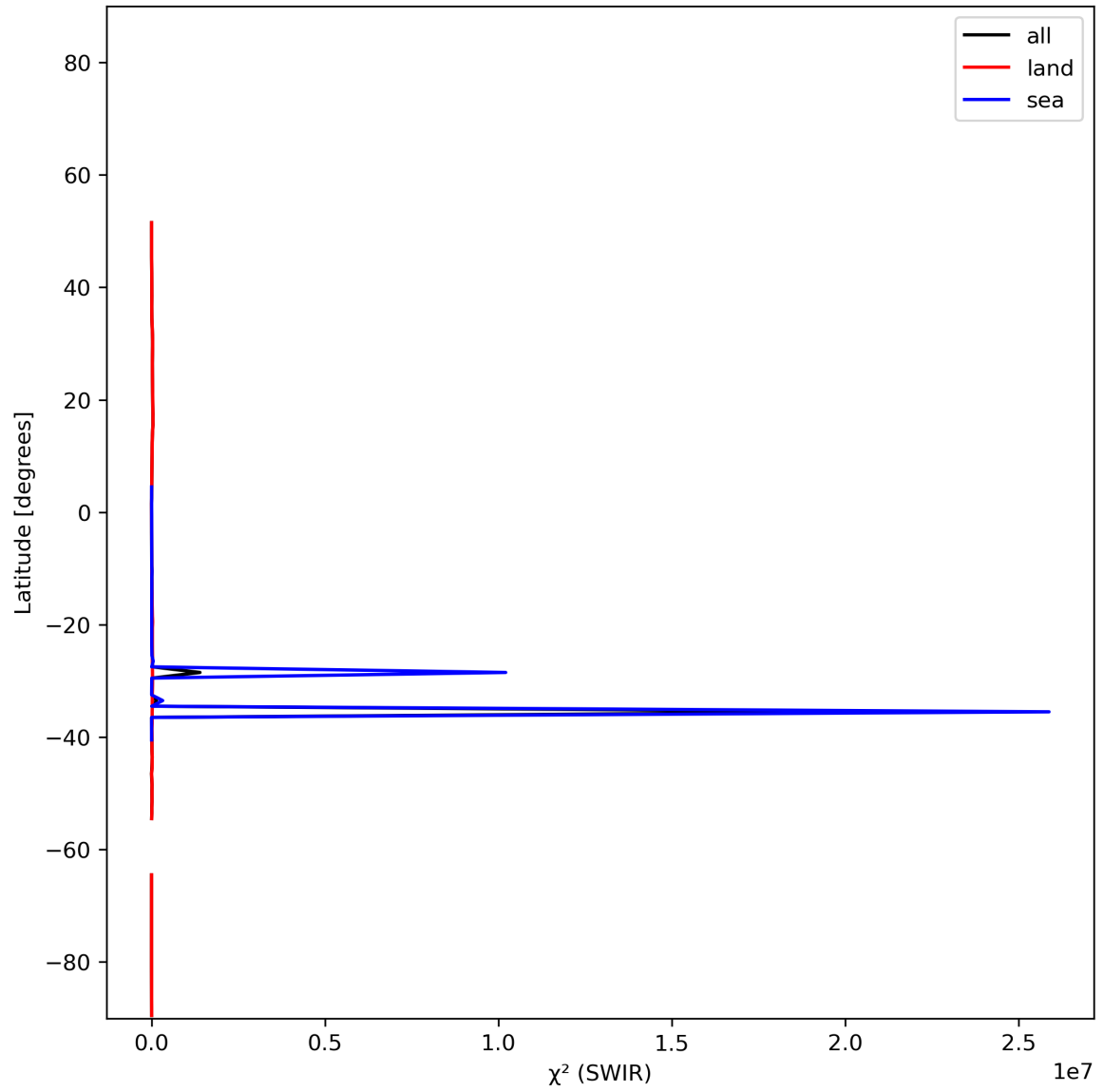
Figure 17: Zonal average of “ \chi^2 (SWIR)” for 2023-12-15 to 2023-12-17.
