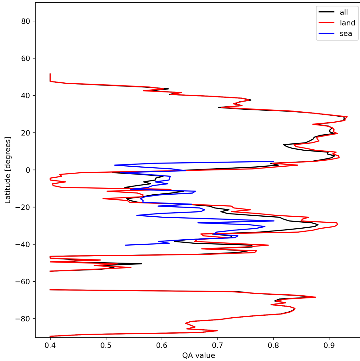
Figure 11: Zonal average of “QA value” for 2023-12-15 to 2023-12-17.
