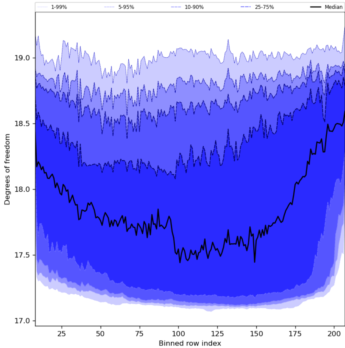
Figure 41: Along track statistics of “Degrees of freedom” for 2023-12-15 to 2023-12-17
