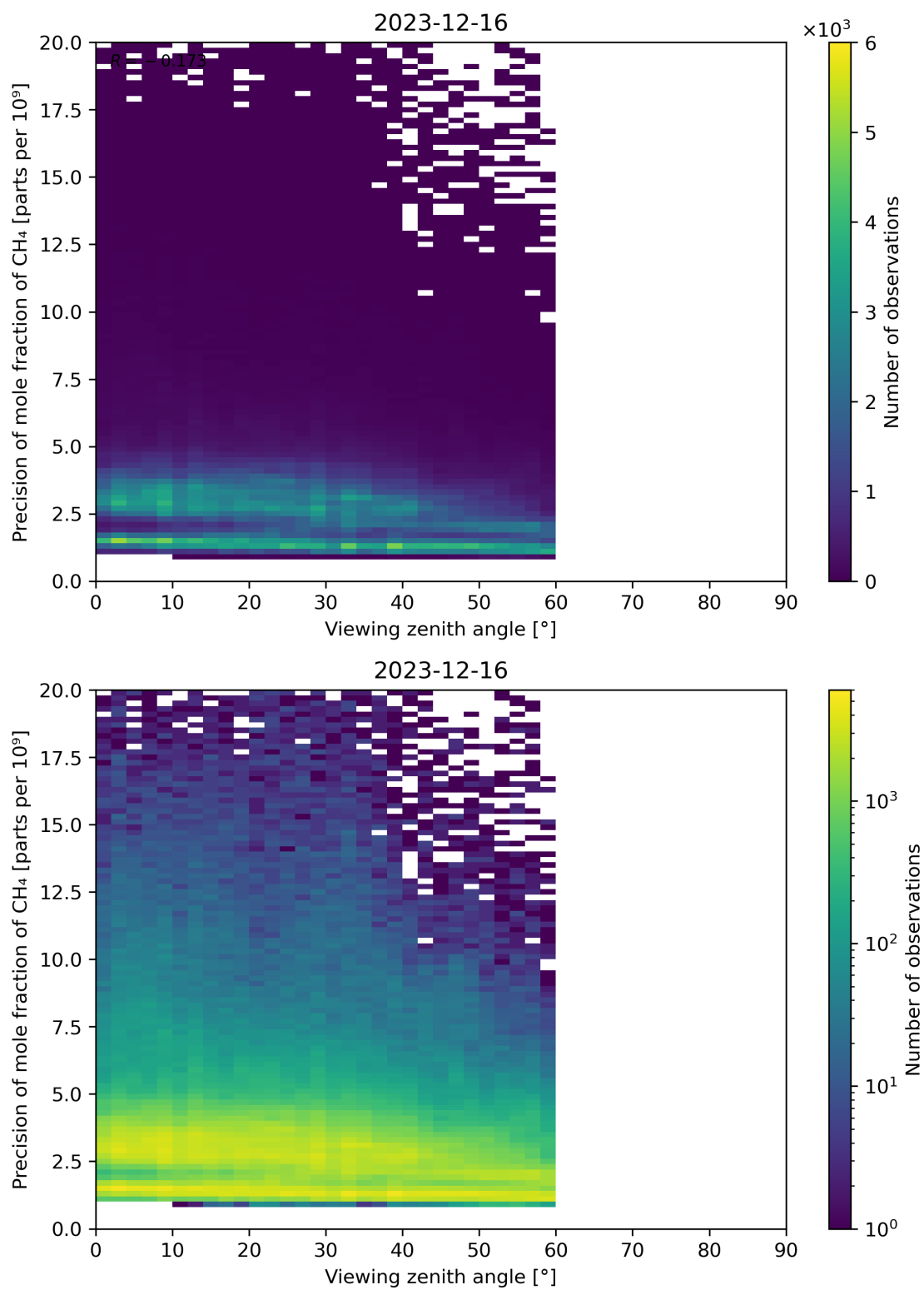
Figure 112: Scatter density plot of “Viewing zenith angle” against “Precision of mole fraction of CH 4 ” for 2023-12-15 to 2023-12-17.
