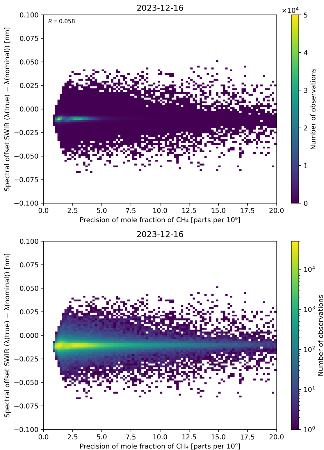
Figure 85: Scatter density plot of “Precision of mole fraction of CH 4 ” against “Spectral offset SWIR ( \lambda(\text{true}) - \lambda(\text{nominal}) )” for 2023-12-15 to 2023-12-17.
