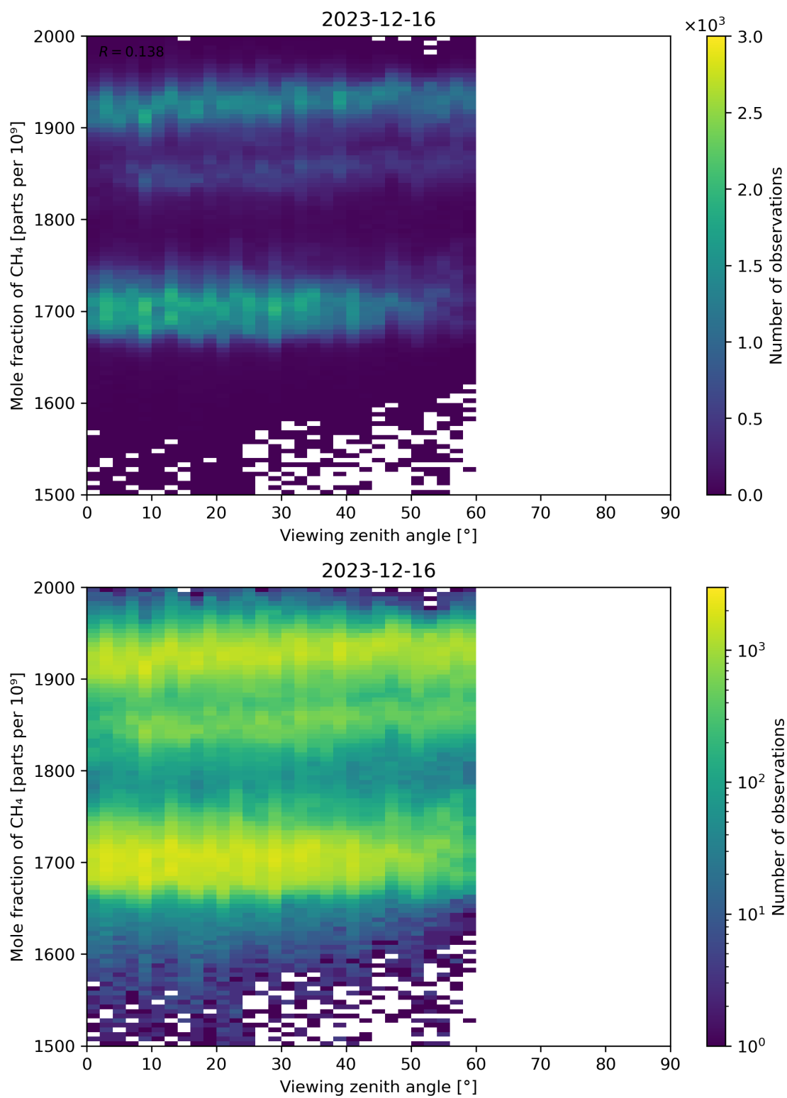
Figure 110: Scatter density plot of “Viewing zenith angle” against “Mole fraction of CH 4 ” for 2023-12-15 to 2023-12-17.
