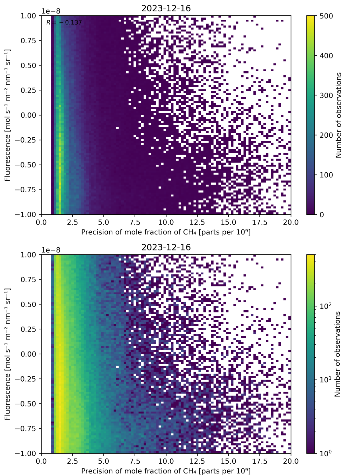
Figure 81: Scatter density plot of “Precision of mole fraction of \text{CH}_4 ” against “Fluorescence” for 2023-12-15 to 2023-12-17.
