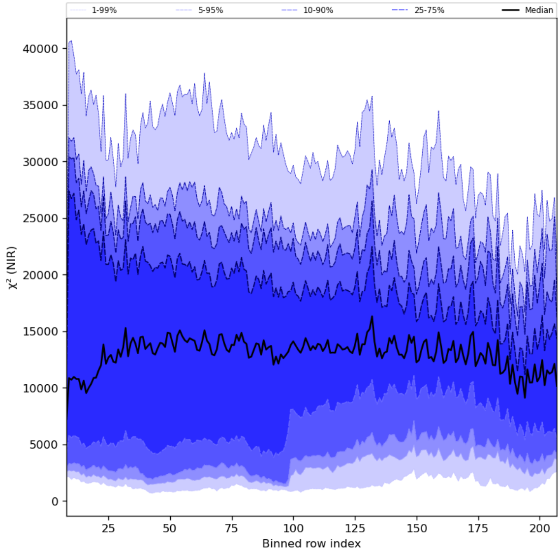
Figure 40: Along track statistics of “ \chi^2 (NIR)” for 2023-12-15 to 2023-12-17
