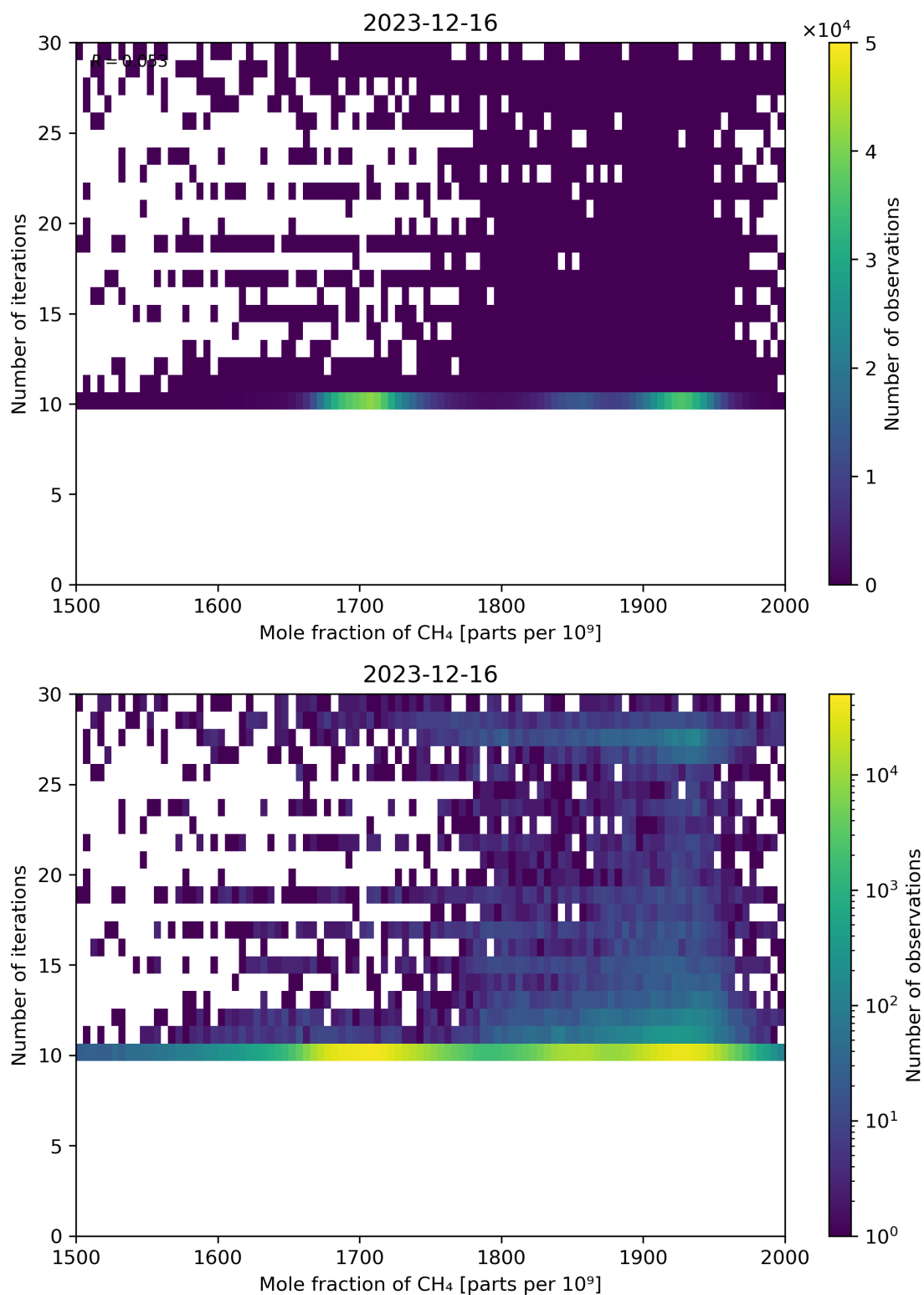
Figure 76: Scatter density plot of “Mole fraction of CH 4 ” against “Number of iterations” for 2023-12-15 to 2023-12-17.
