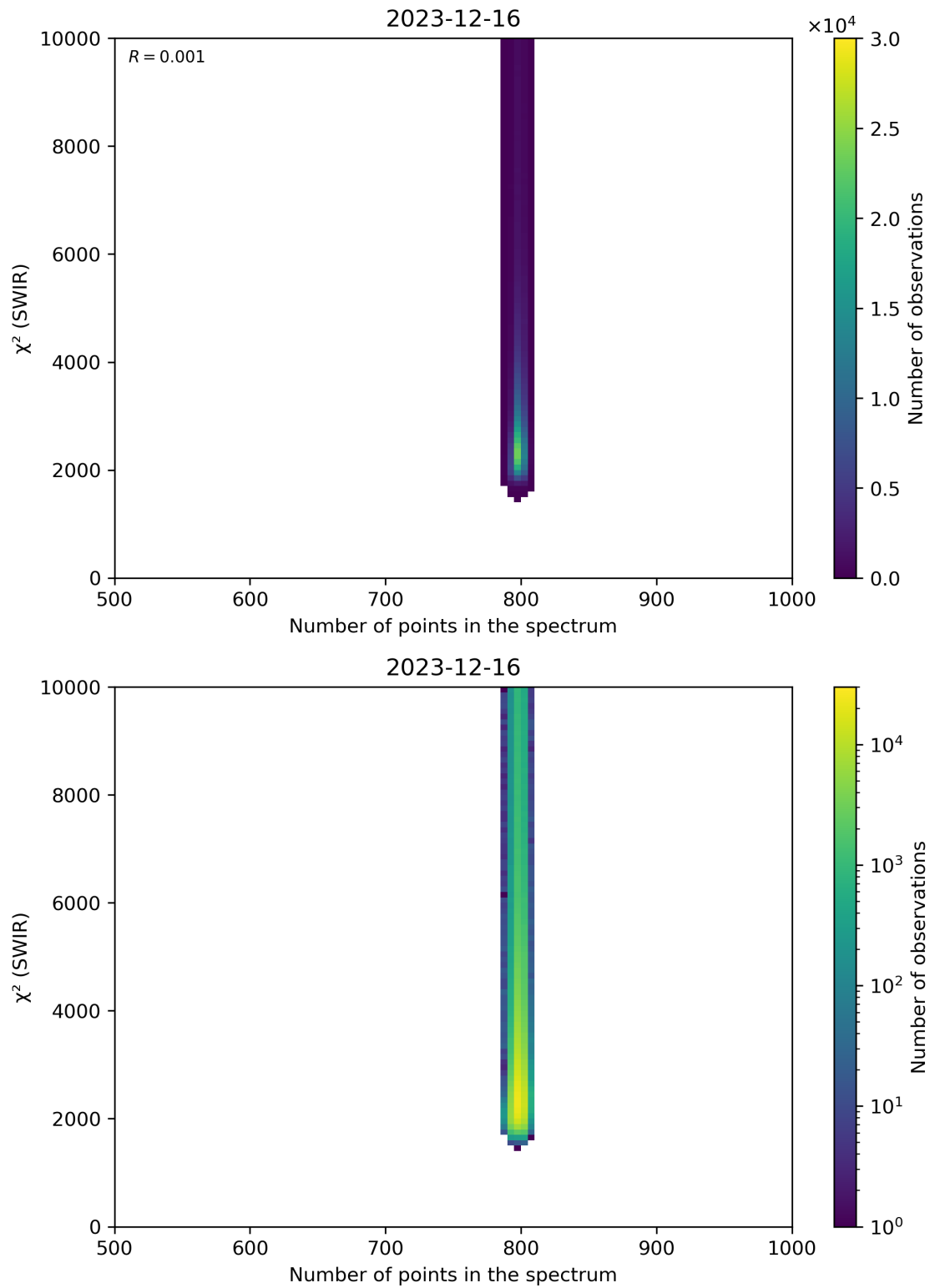
Figure 89: Scatter density plot of “Number of points in the spectrum” against “ \chi^2 (SWIR)” for 2023-12-15 to 2023-12-17.
