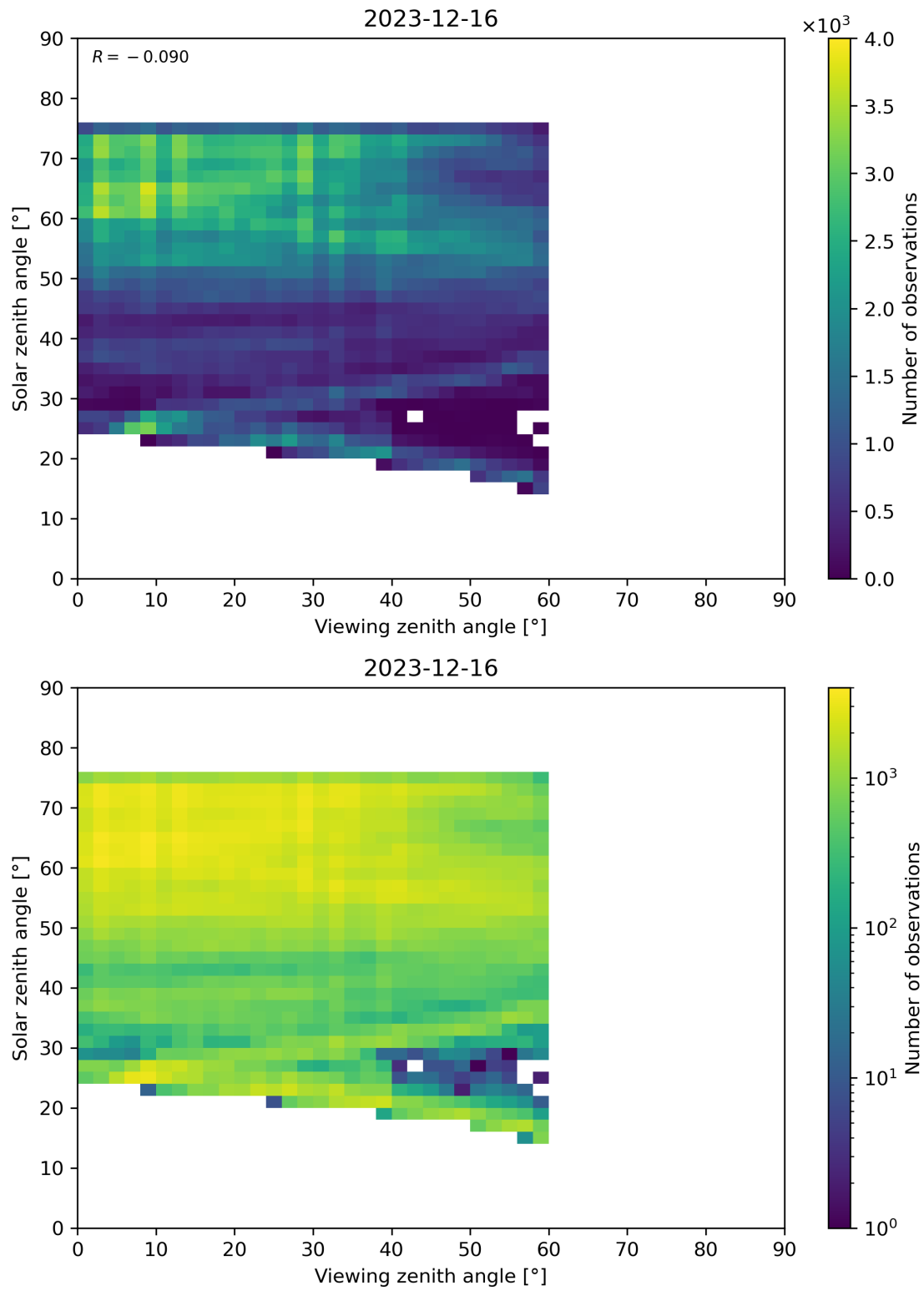
Figure 115: Scatter density plot of “Viewing zenith angle” against “Solar zenith angle” for 2023-12-15 to 2023-12-17.
