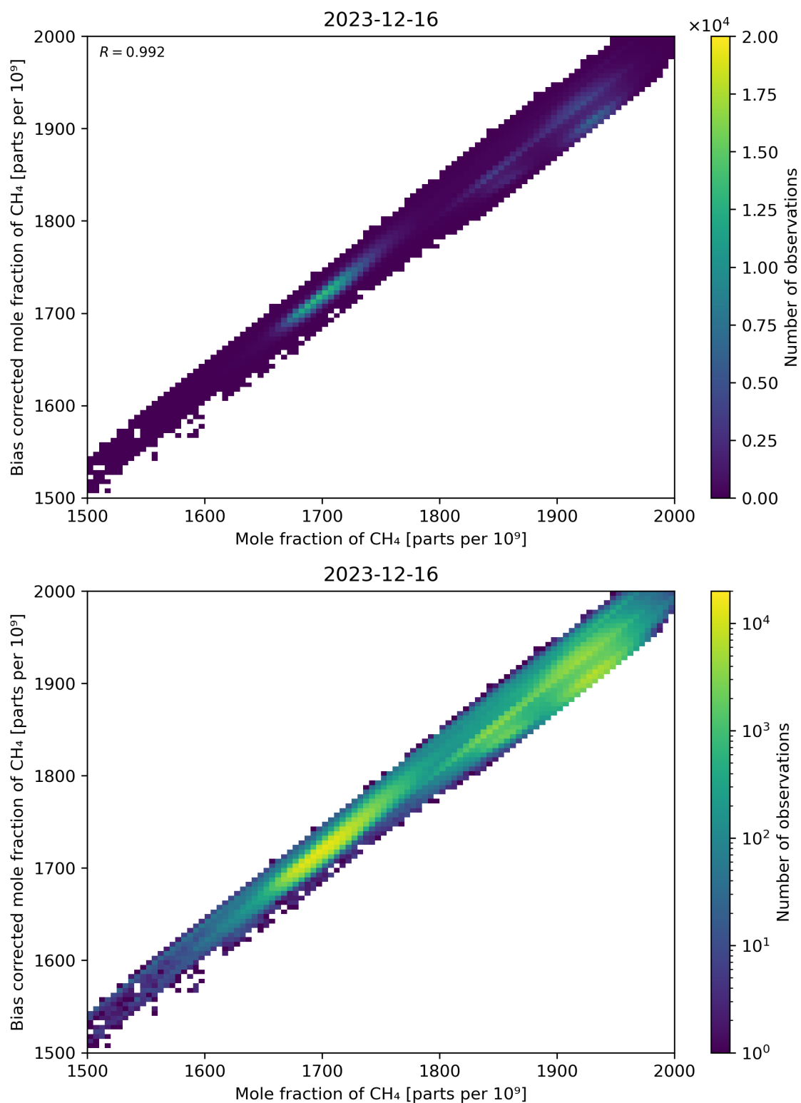
Figure 74: Scatter density plot of “Mole fraction of CH 4 ” against “Bias corrected mole fraction of CH 4 ” for 2023-12-15 to 2023-12-17.
