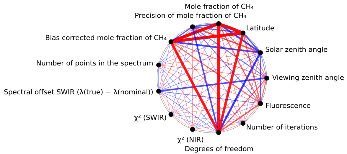
Figure 1: Map of correlation graph for 2023-12-15 to 2023-12-17.
