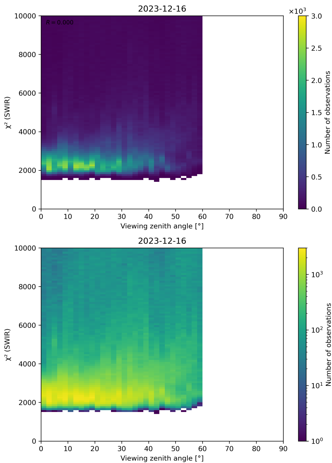
Figure 106: Scatter density plot of “Viewing zenith angle” against “ \chi^2 (SWIR)” for 2023-12-15 to 2023-12-17.
