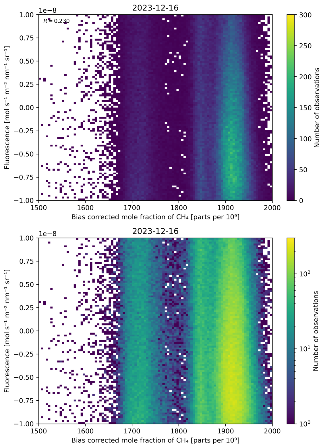
Figure 66: Scatter density plot of “Bias corrected mole fraction of \text{CH}_4 ” against “Fluorescence” for 2023-12-15 to 2023-12-17.
