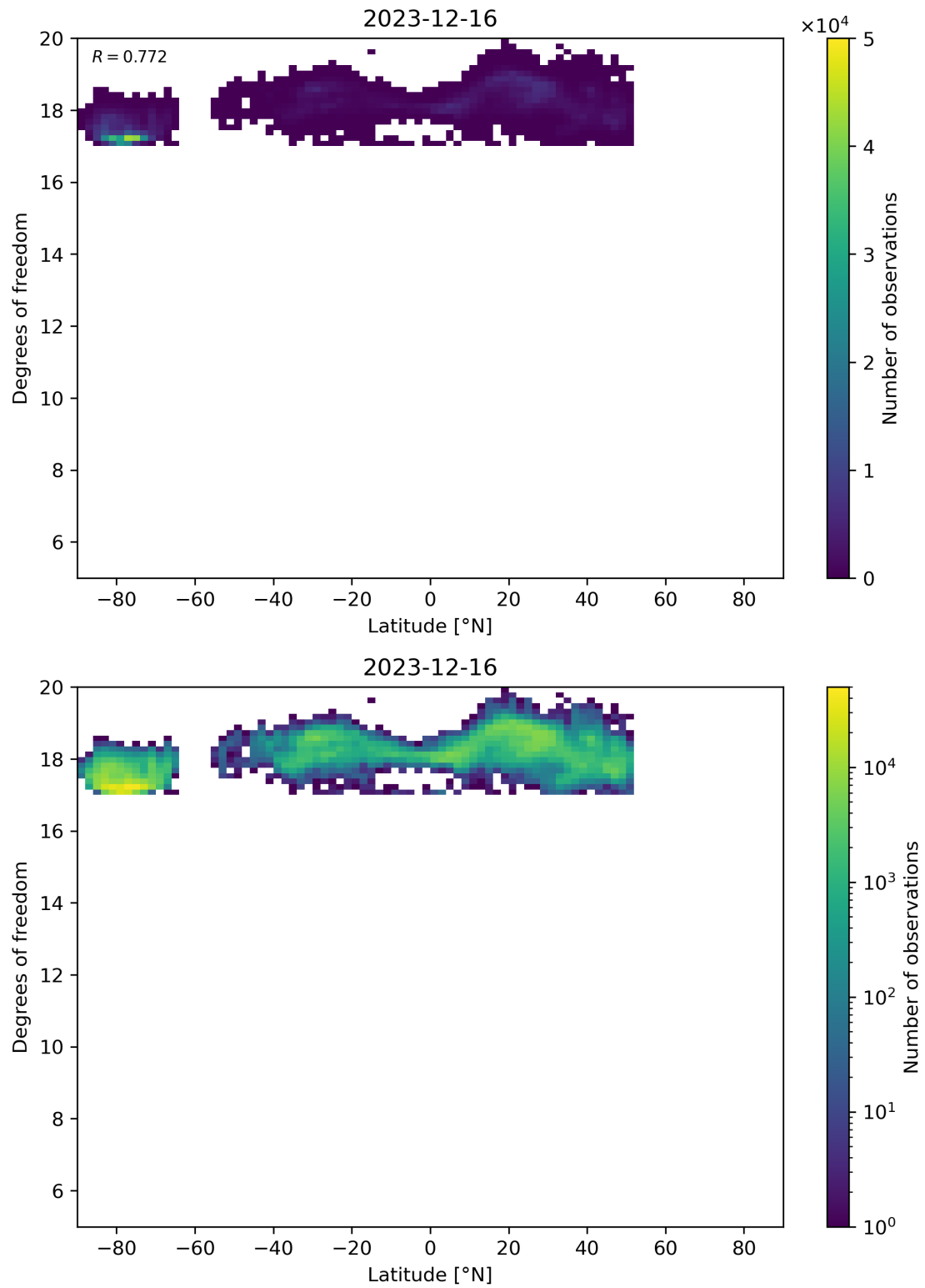
Figure 55: Scatter density plot of “Latitude” against “Degrees of freedom” for 2023-12-15 to 2023-12-17.
