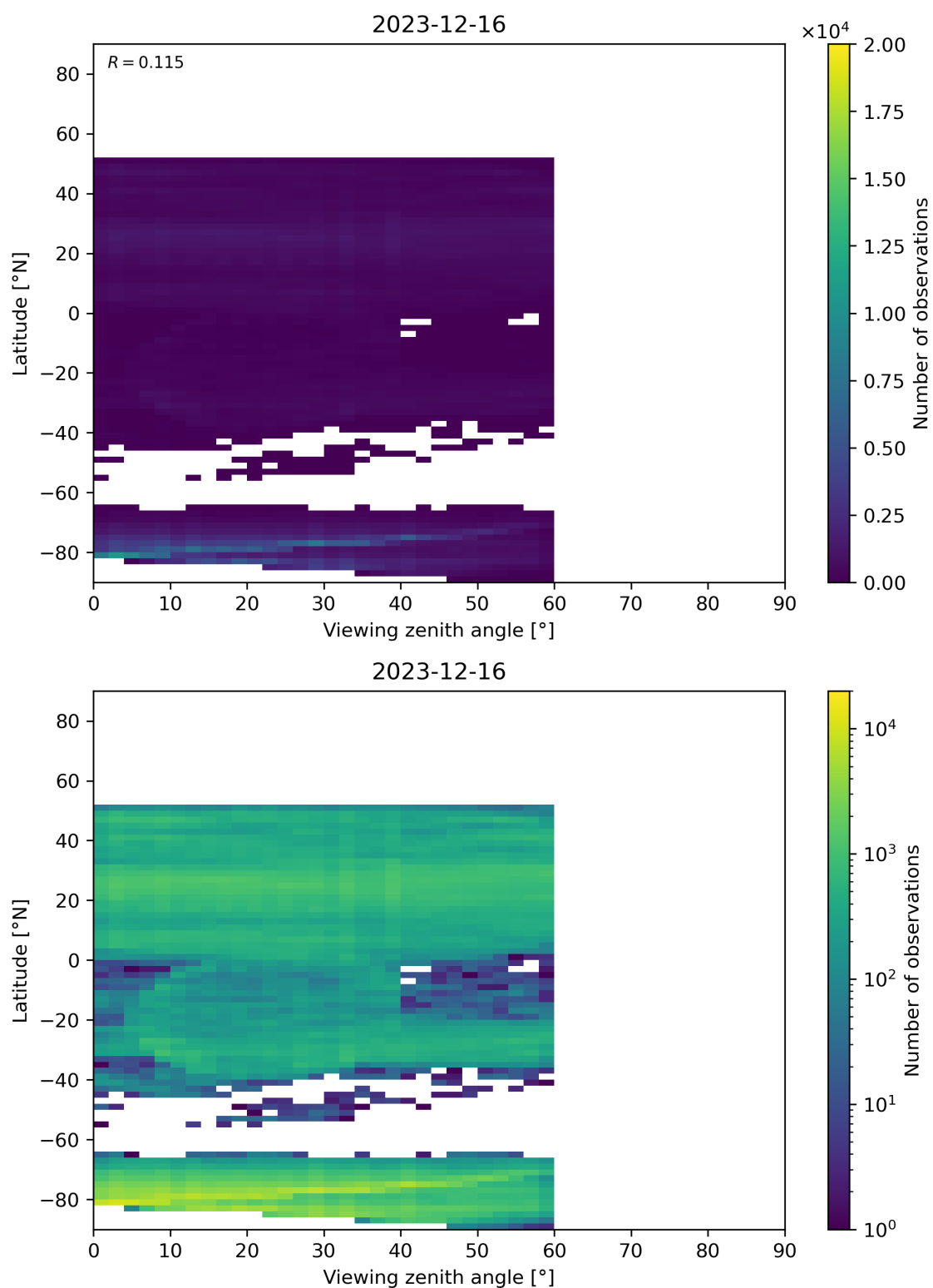
Figure 109: Scatter density plot of “Viewing zenith angle” against “Latitude” for 2023-12-15 to 2023-12-17.
