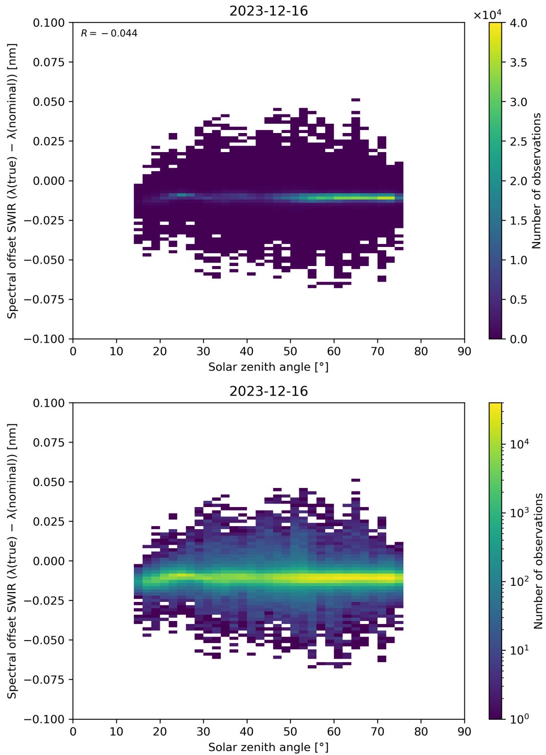
Figure 104: Scatter density plot of “Solar zenith angle” against “Spectral offset SWIR ( \lambda(\text{true}) - \lambda(\text{nominal}) )” for 2023-12-15 to 2023-12-17.
