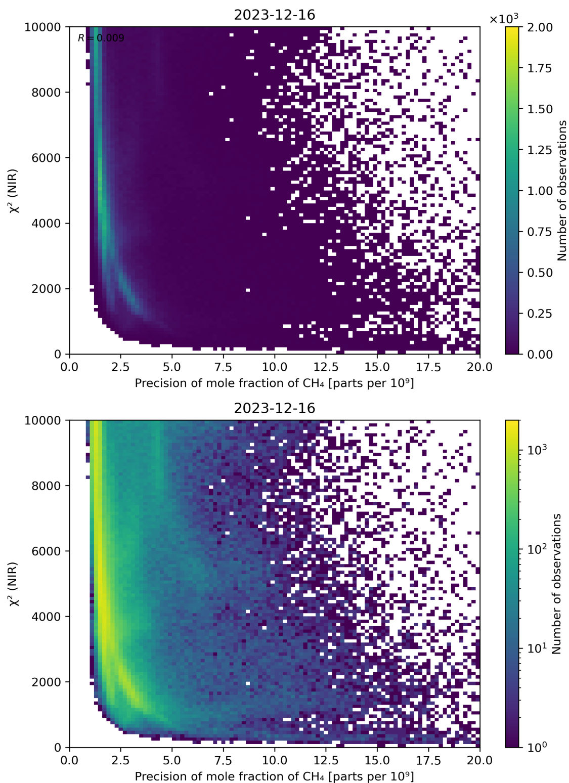
Figure 78: Scatter density plot of “Precision of mole fraction of CH 4 ” against “ \chi^2 (NIR)” for 2023-12-15 to 2023-12-17.
