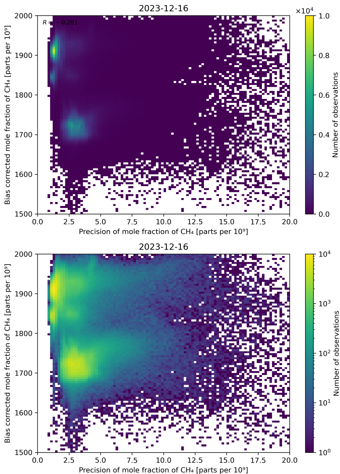
Figure 82: Scatter density plot of “Precision of mole fraction of \text{CH}_4 ” against “Bias corrected mole fraction of \text{CH}_4 ” for 2023-12-15 to 2023-12-17.
