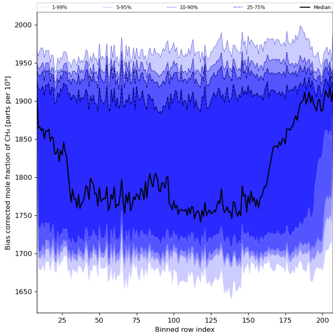
Figure 36: Along track statistics of “Bias corrected mole fraction of CH 4 ” for 2023-12-15 to 2023-12-17
