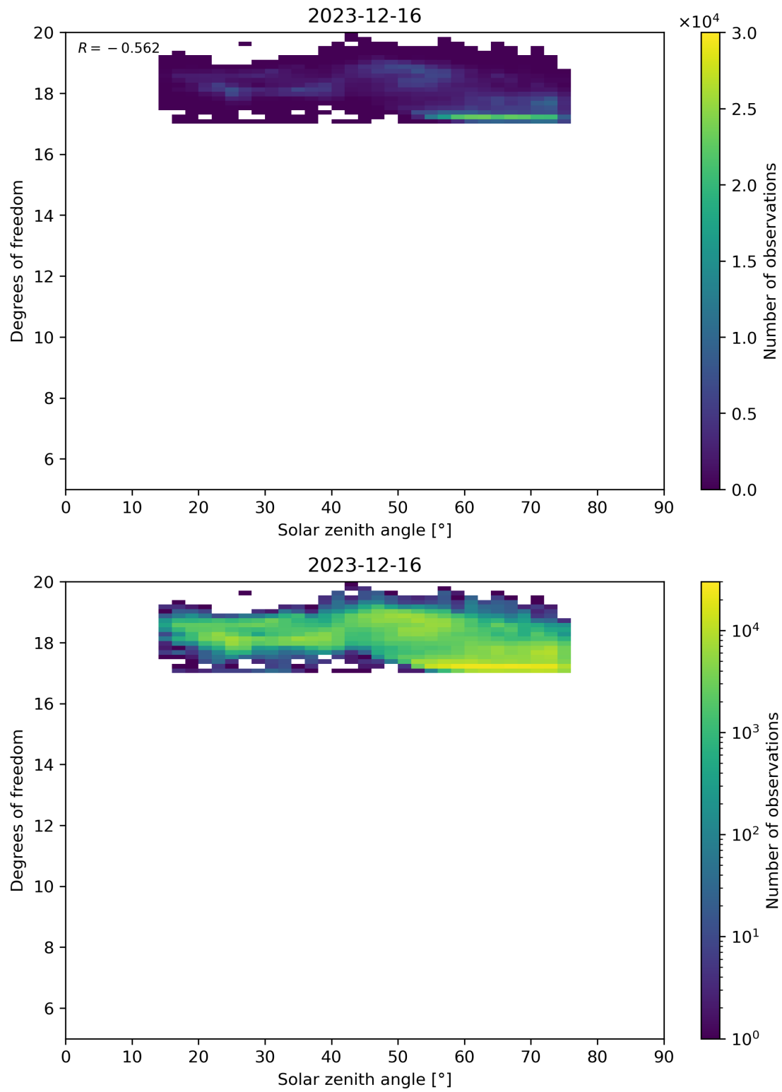
Figure 96: Scatter density plot of “Solar zenith angle” against “Degrees of freedom” for 2023-12-15 to 2023-12-17.
