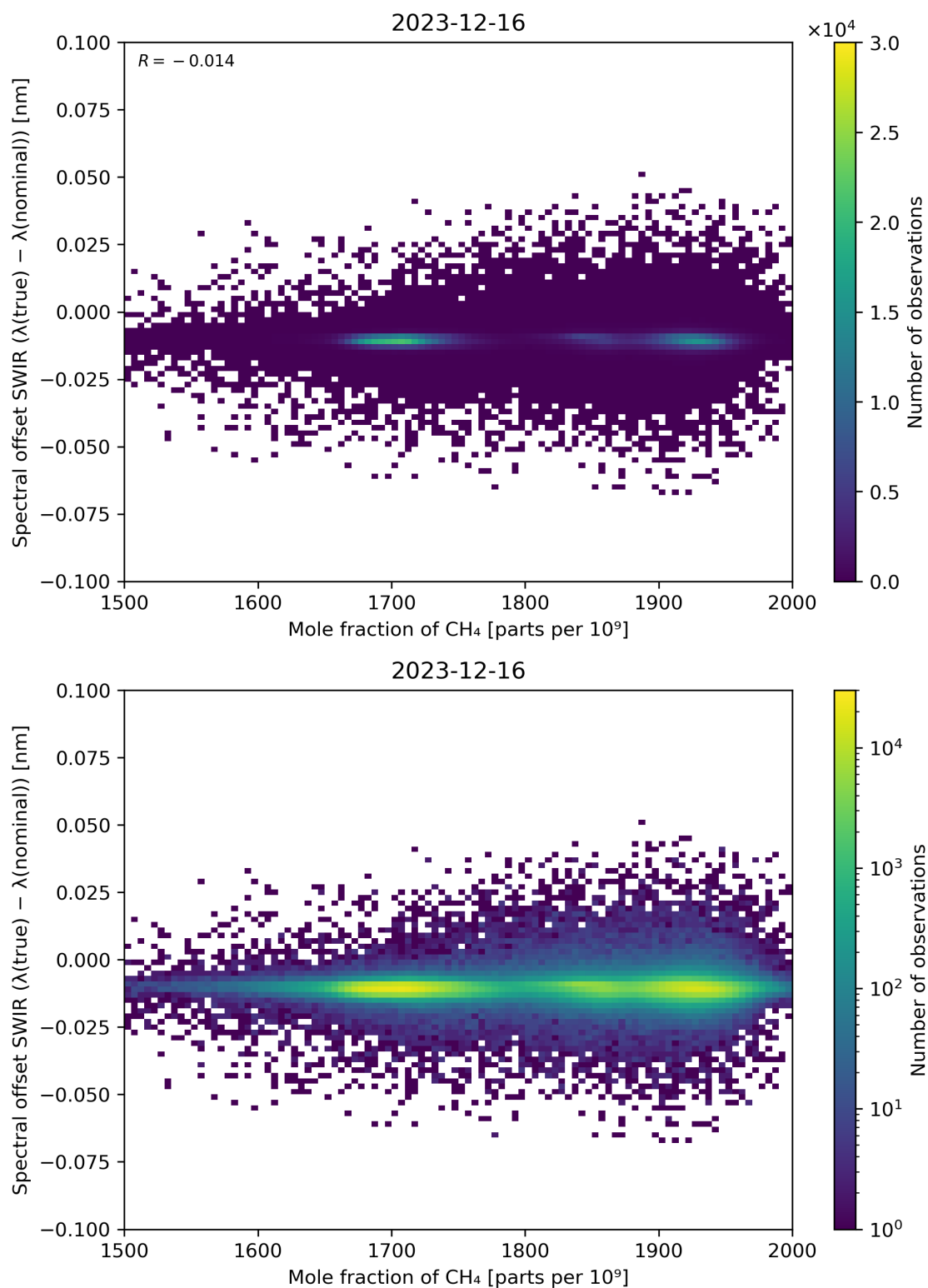
Figure 86: Scatter density plot of “Mole fraction of \text{CH}_4 ” against “Spectral offset SWIR ( \lambda(\text{true}) - \lambda(\text{nominal}) )” for 2023-12-15 to 2023-12-17.
