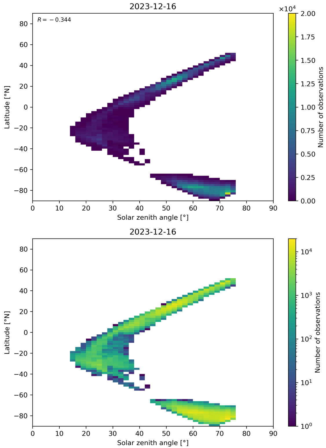
Figure 98: Scatter density plot of “Solar zenith angle” against “Latitude” for 2023-12-15 to 2023-12-17.
