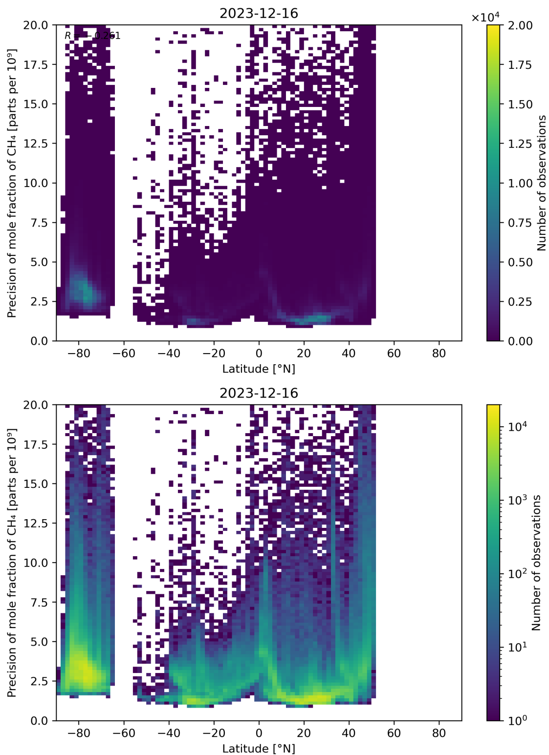
Figure 59: Scatter density plot of “Latitude” against “Precision of mole fraction of CH 4 ” for 2023-12-15 to 2023-12-17.
