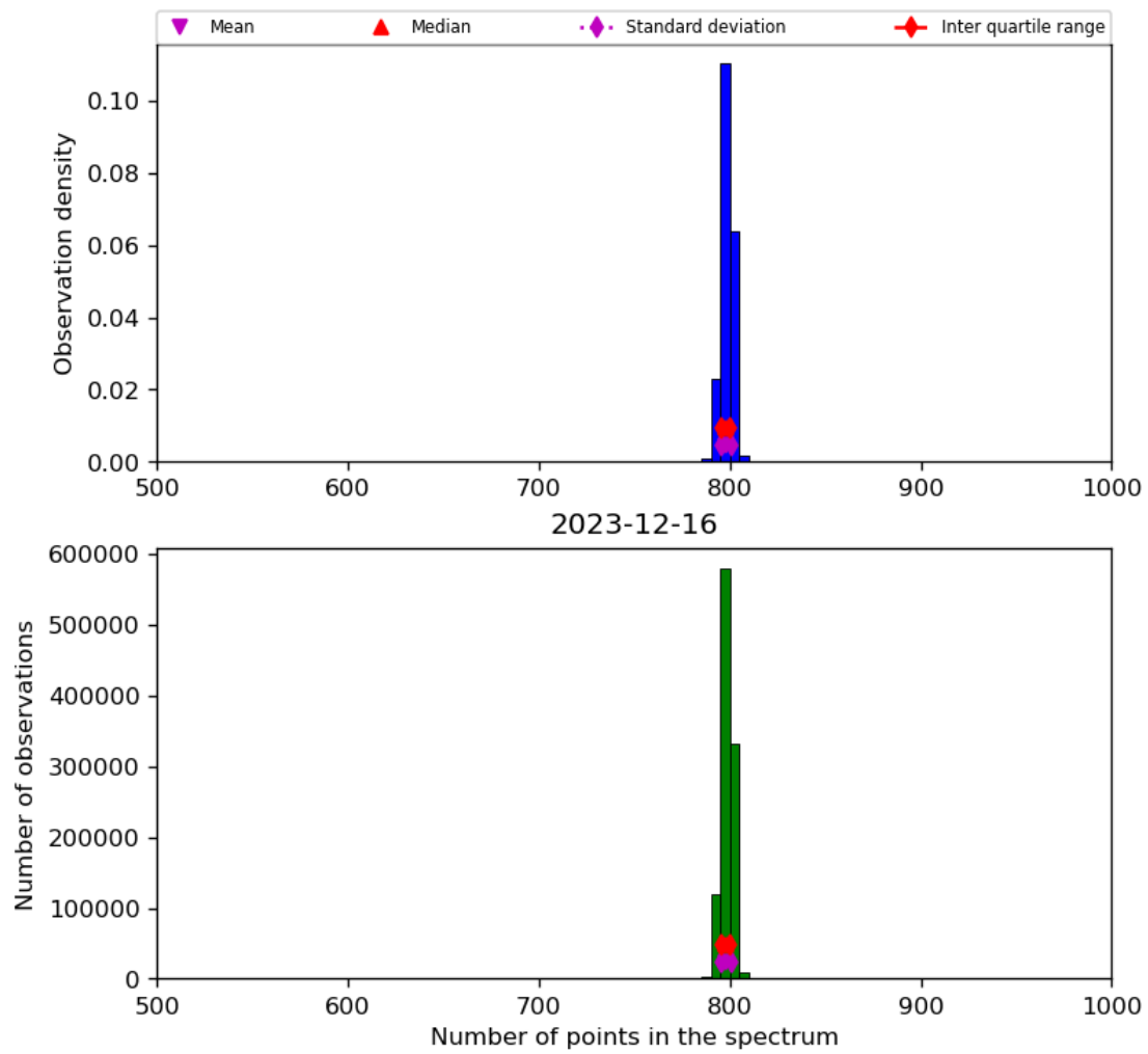
Figure 26: Histogram of “Number of points in the spectrum” for 2023-12-15 to 2023-12-17
