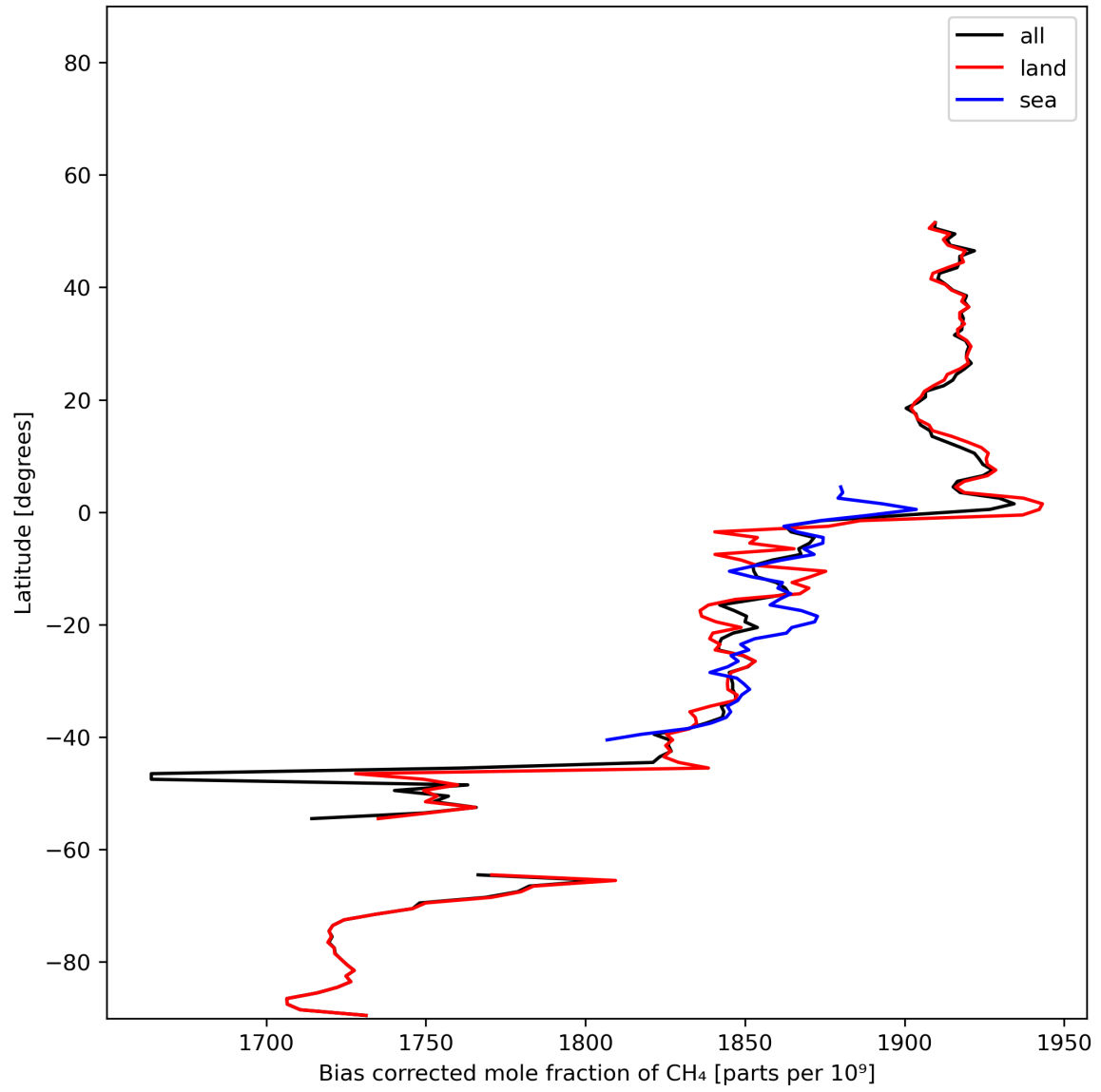
Figure 14: Zonal average of “Bias corrected mole fraction of CH 4 ” for 2023-12-15 to 2023-12-17.
