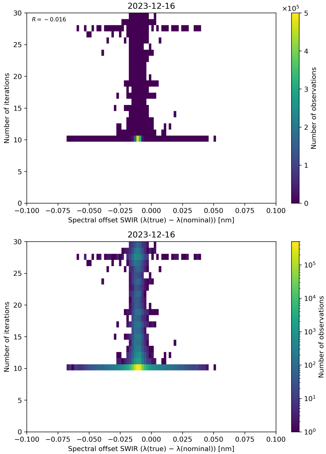
Figure 121: Scatter density plot of “Spectral offset SWIR ( \lambda(\text{true}) - \lambda(\text{nominal}) )” against “Number of iterations” for 2023-12-15 to 2023-12-17.
