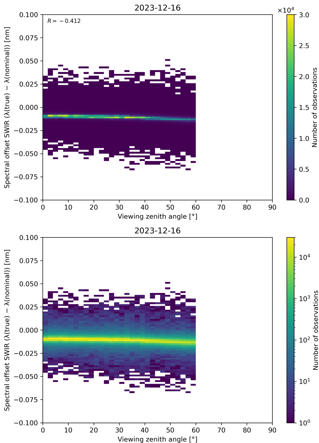
Figure 116: Scatter density plot of “Viewing zenith angle” against “Spectral offset SWIR ( \lambda(\text{true}) - \lambda(\text{nominal}) )” for 2023-12-15 to 2023-12-17.
