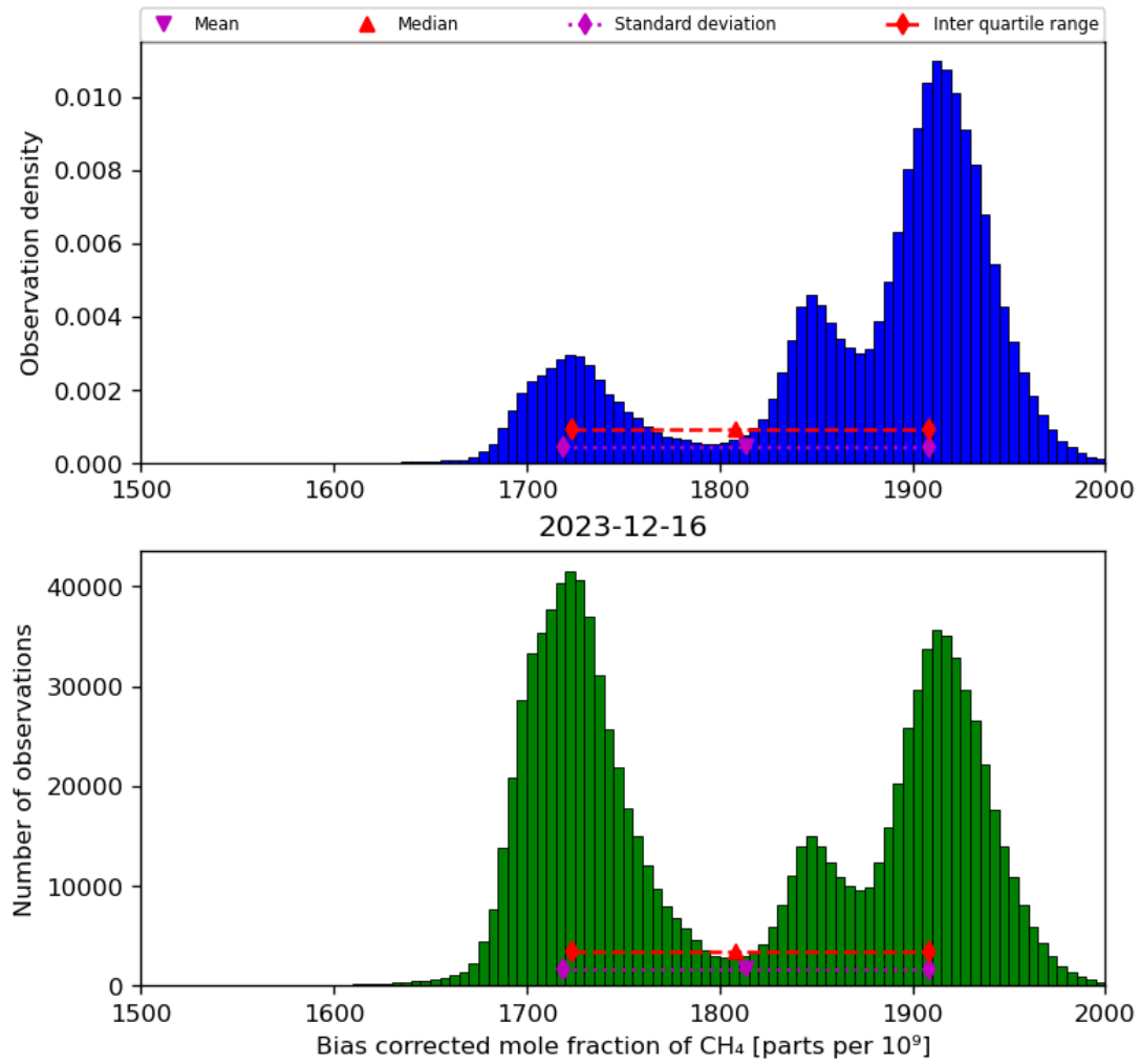
Figure 25: Histogram of “Bias corrected mole fraction of CH 4 ” for 2023-12-15 to 2023-12-17
