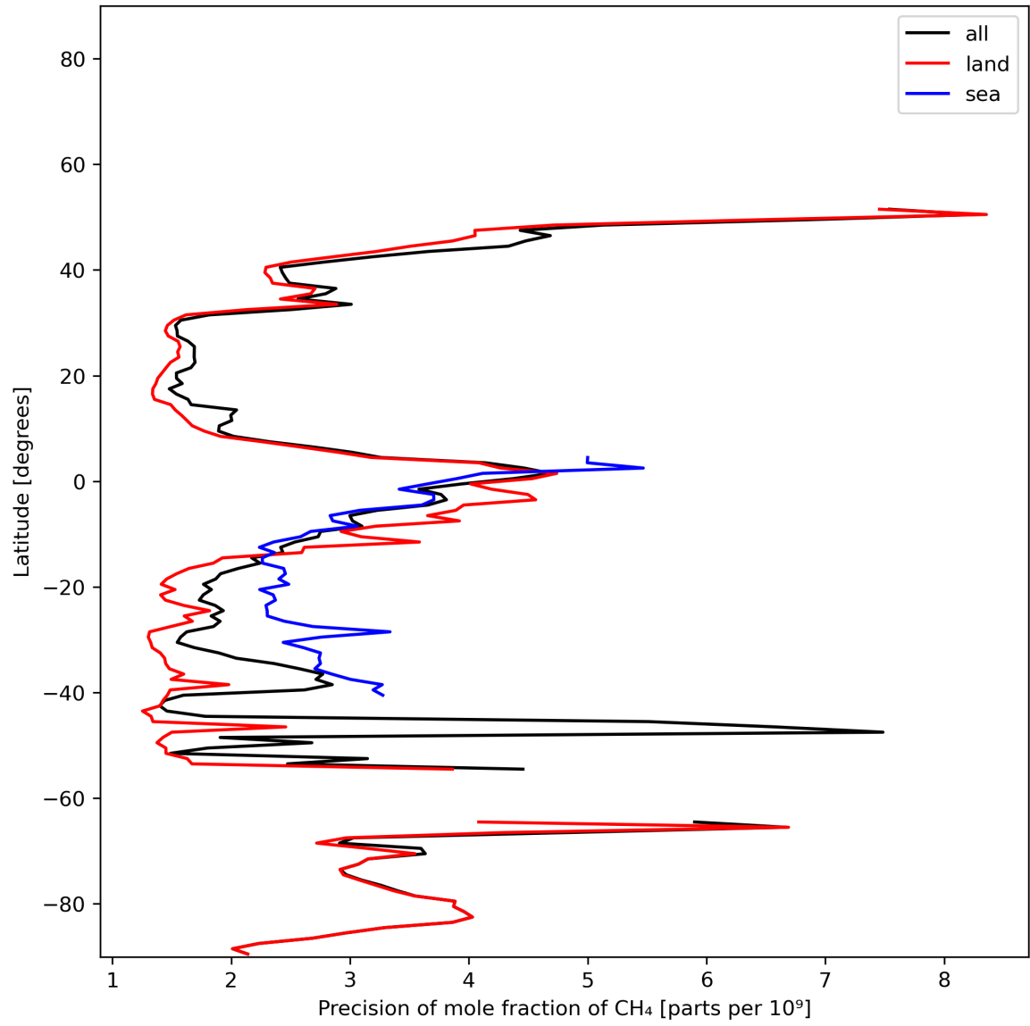
Figure 13: Zonal average of “Precision of mole fraction of CH 4 ” for 2023-12-15 to 2023-12-17.
