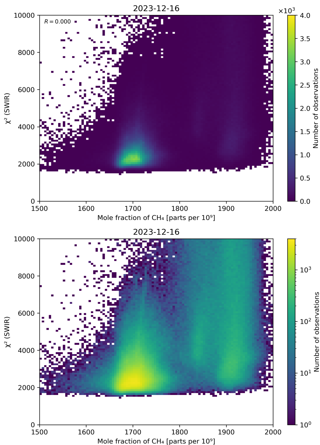
Figure 71: Scatter density plot of “Mole fraction of \text{CH}_4 ” against “ \chi^2 (SWIR)” for 2023-12-15 to 2023-12-17.
