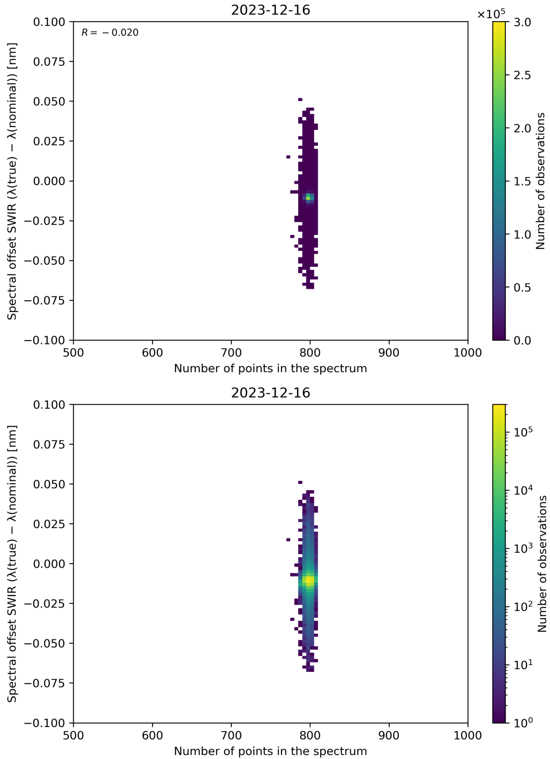
Figure 93: Scatter density plot of “Number of points in the spectrum” against “Spectral offset SWIR ( \lambda(\text{true}) - \lambda(\text{nominal}) )” for 2023-12-15 to 2023-12-17.
