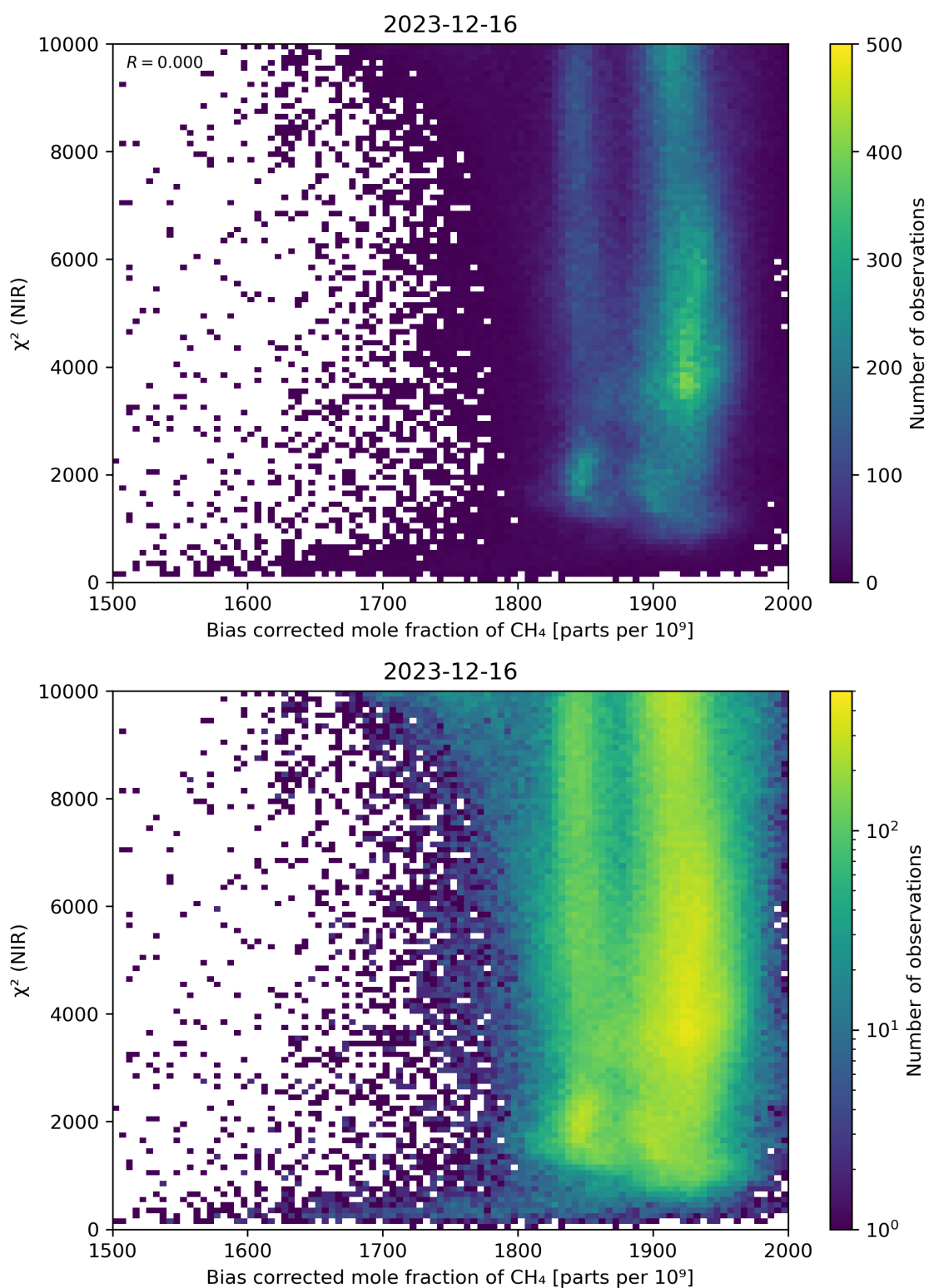
Figure 63: Scatter density plot of “Bias corrected mole fraction of \text{CH}_4 ” against “ \chi^2 (NIR)” for 2023-12-15 to 2023-12-17.
