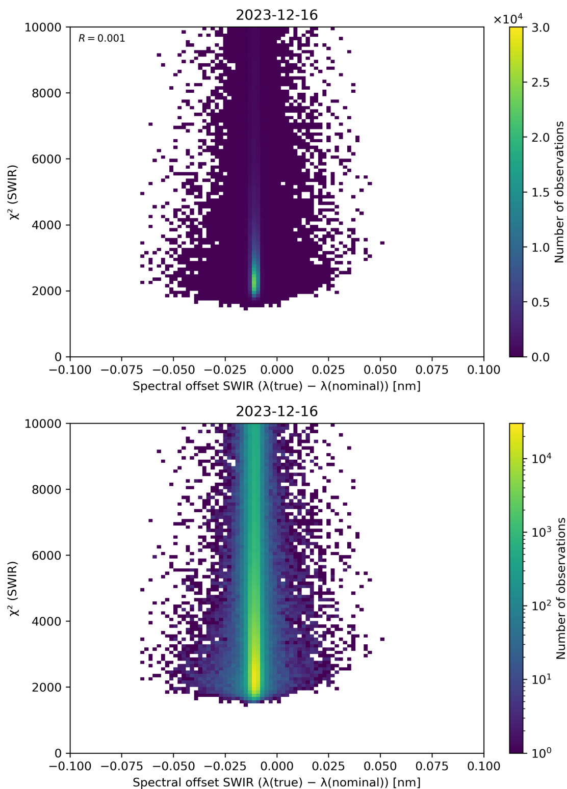
Figure 118: Scatter density plot of “Spectral offset SWIR ( \lambda(\text{true}) - \lambda(\text{nominal}) )” against “ \chi^2 (SWIR)” for 2023-12-15 to 2023-12-17.
