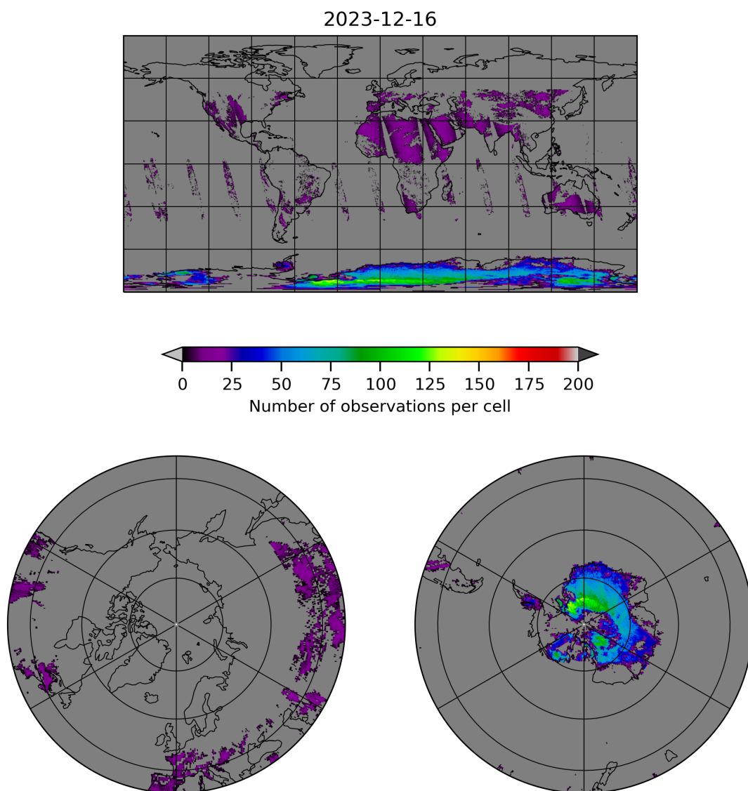
Figure 10: Map of the number of observations for 2023-12-15 to 2023-12-17
