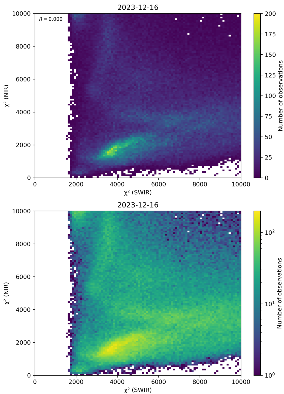
Figure 47: Scatter density plot of “ \chi^2 (SWIR)” against “ \chi^2 (NIR)” for 2023-12-15 to 2023-12-17.
