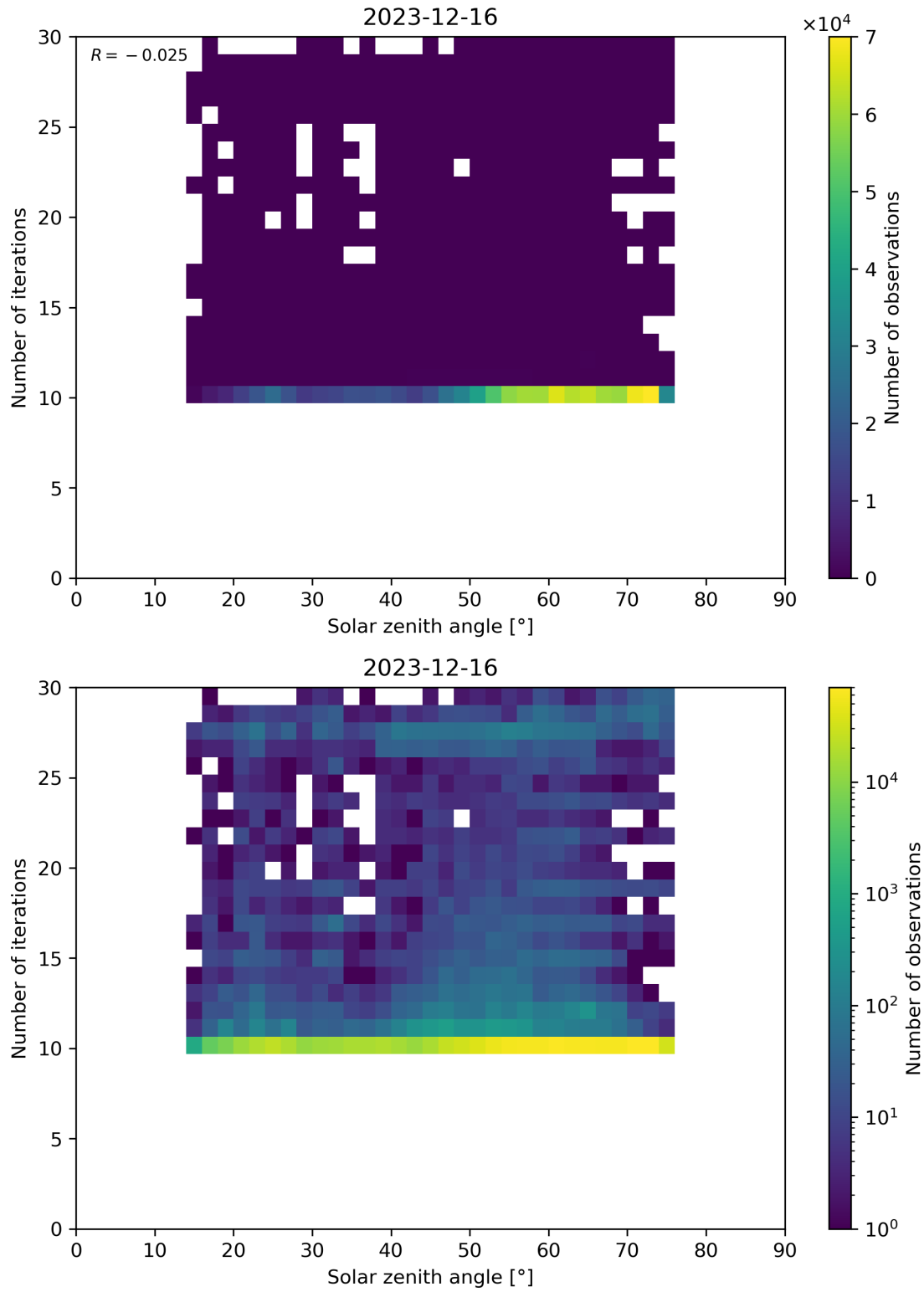
Figure 102: Scatter density plot of “Solar zenith angle” against “Number of iterations” for 2023-12-15 to 2023-12-17.
