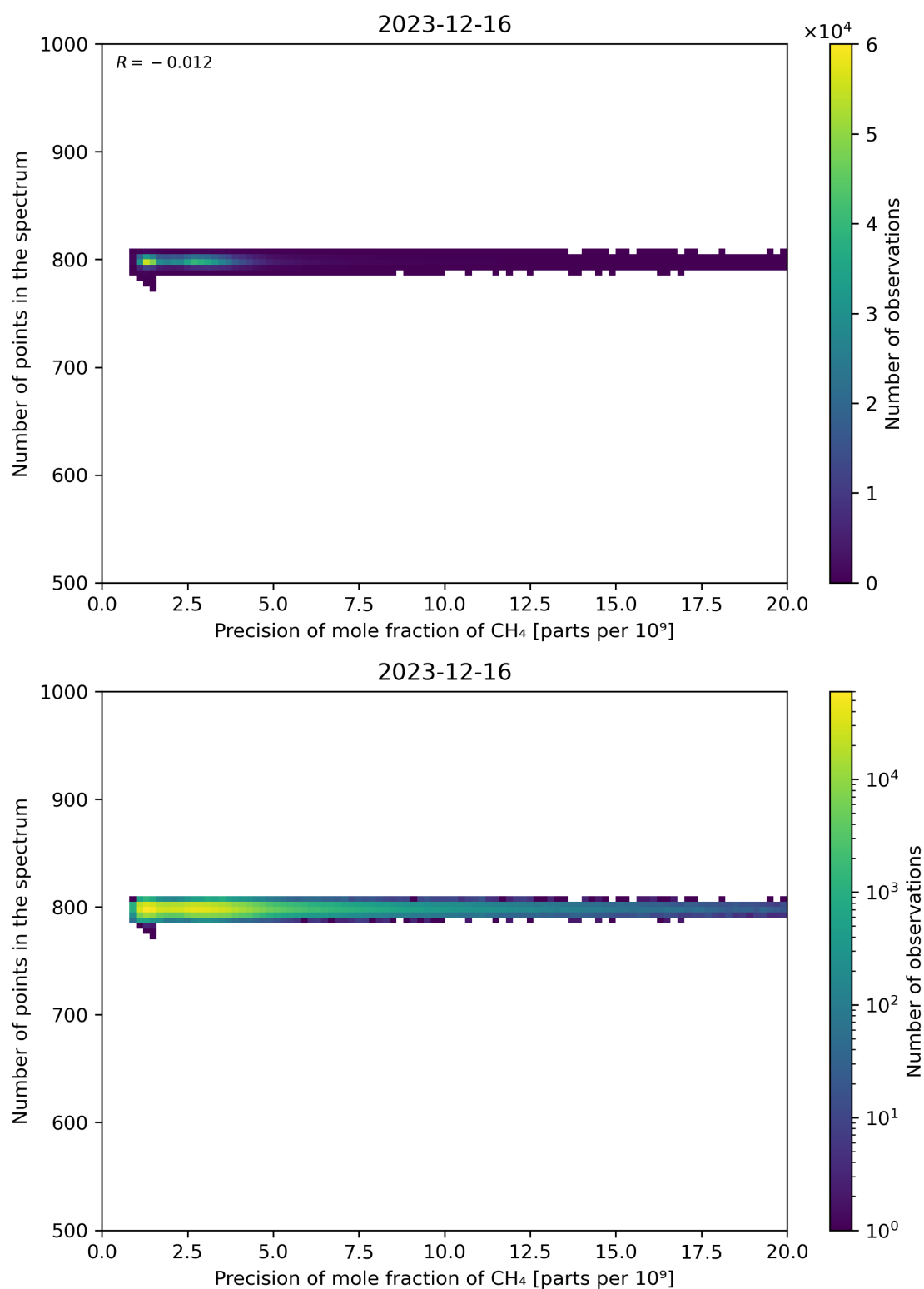
Figure 84: Scatter density plot of “Precision of mole fraction of CH 4 ” against “Number of points in the spectrum” for 2023-12-15 to 2023-12-17.
