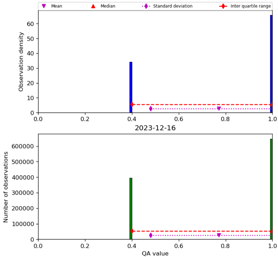
Figure 22: Histogram of “QA value” for 2023-12-15 to 2023-12-17
