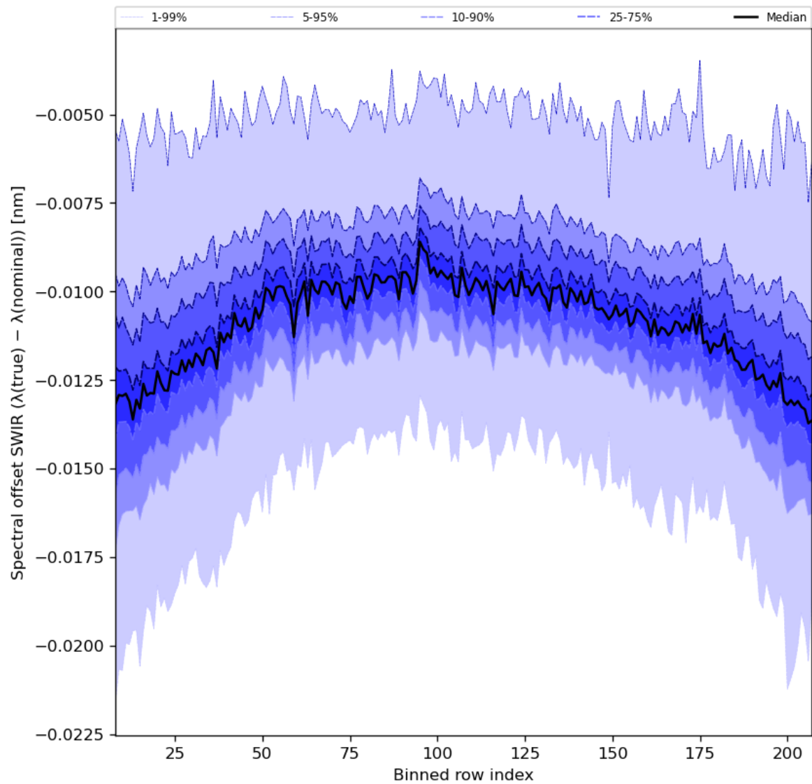
Figure 38: Along track statistics of “Spectral offset SWIR ( \lambda(\text{true}) - \lambda(\text{nominal}) )” for 2023-12-15 to 2023-12-17
