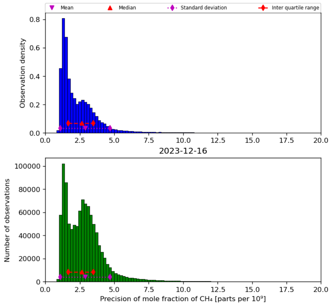
Figure 24: Histogram of “Precision of mole fraction of CH 4 ” for 2023-12-15 to 2023-12-17
