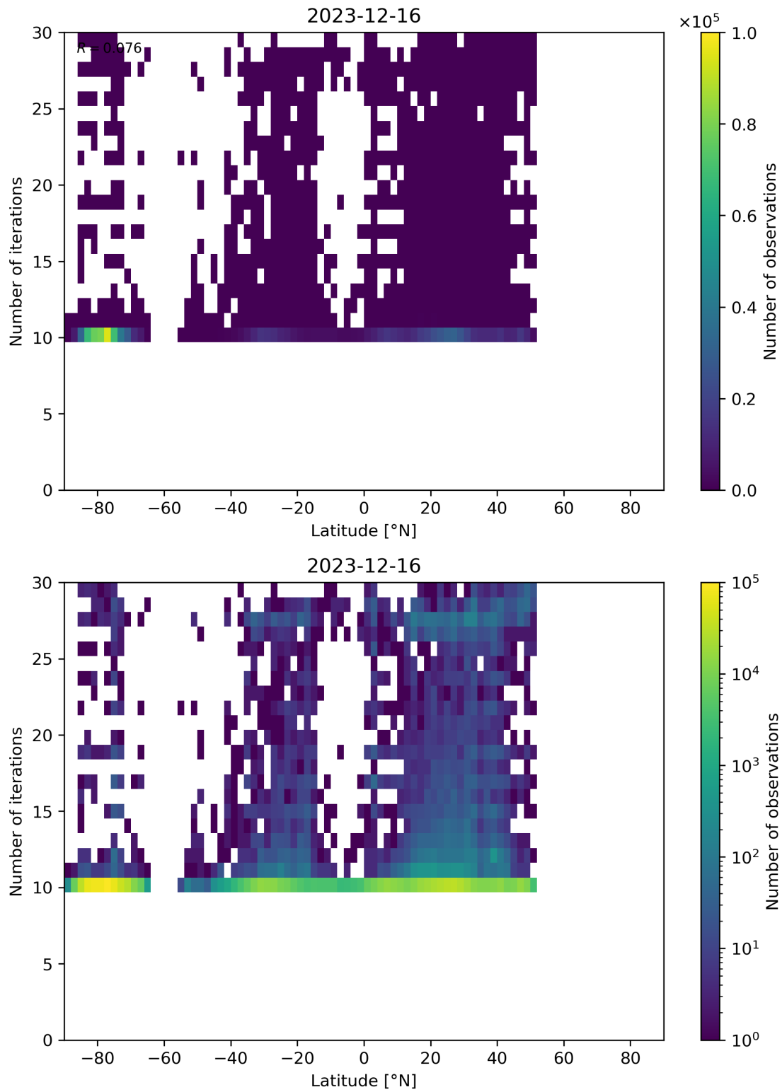
Figure 60: Scatter density plot of “Latitude” against “Number of iterations” for 2023-12-15 to 2023-12-17.
