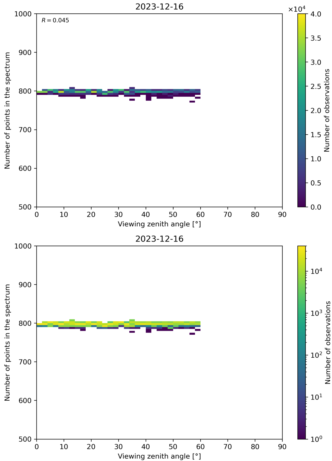
Figure 114: Scatter density plot of “Viewing zenith angle” against “Number of points in the spectrum” for 2023-12-15 to 2023-12-17.
