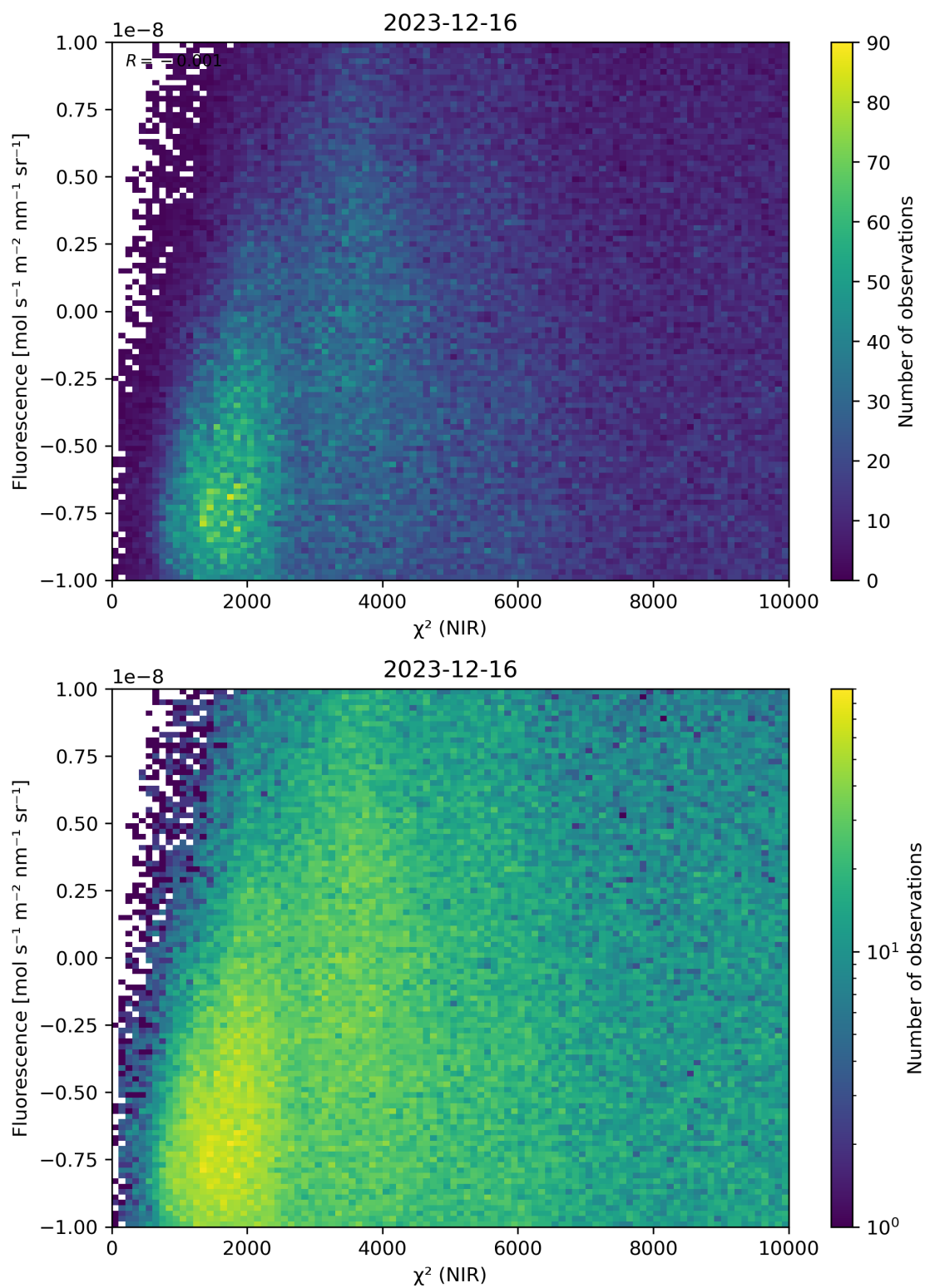
Figure 45: Scatter density plot of “ \chi^2 (NIR)” against “Fluorescence” for 2023-12-15 to 2023-12-17.
