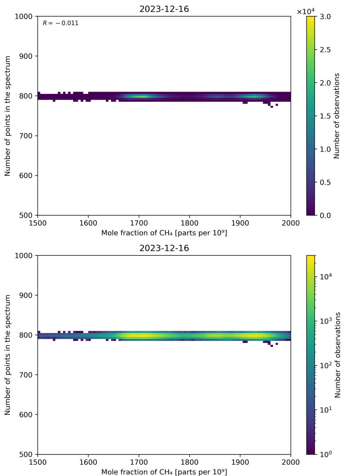
Figure 77: Scatter density plot of “Mole fraction of CH 4 ” against “Number of points in the spectrum” for 2023-12-15 to 2023-12-17.
