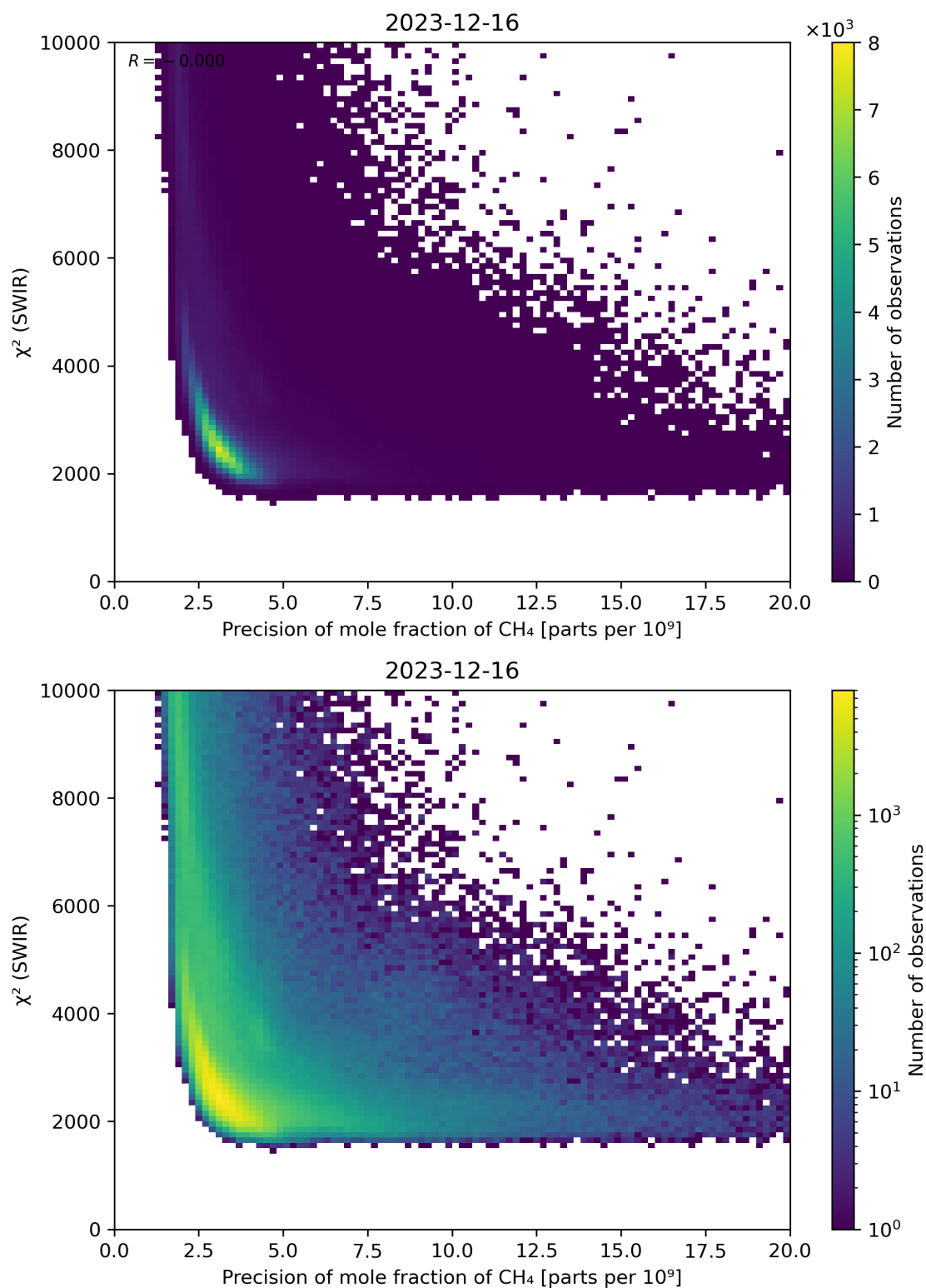
Figure 79: Scatter density plot of “Precision of mole fraction of CH 4 ” against “ \chi^2 (SWIR)” for 2023-12-15 to 2023-12-17.
