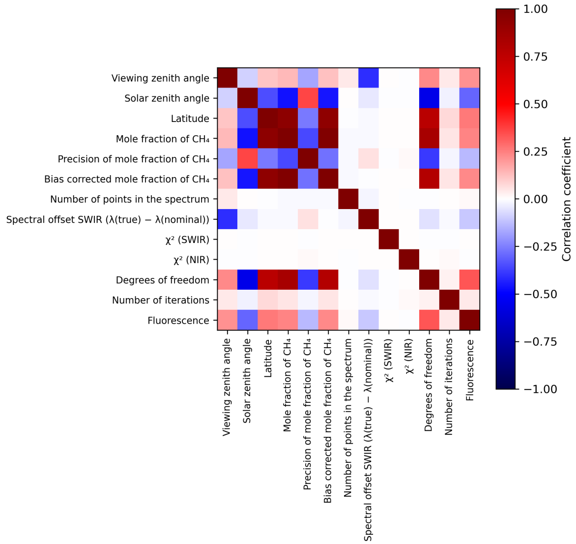
Figure 2: Map of correlation matrix for 2023-12-15 to 2023-12-17.
