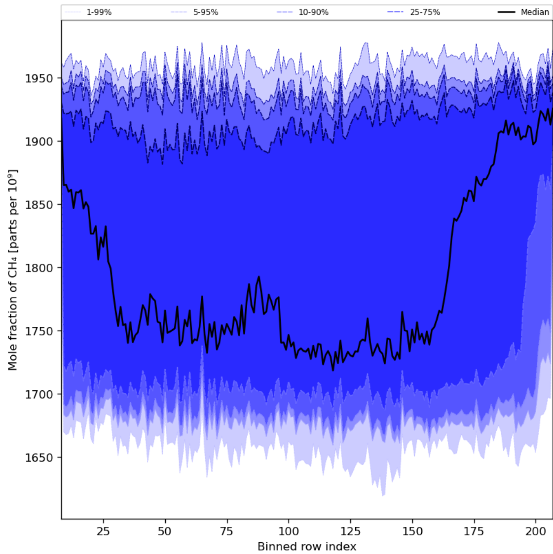
Figure 34: Along track statistics of “Mole fraction of CH 4 ” for 2023-12-15 to 2023-12-17
