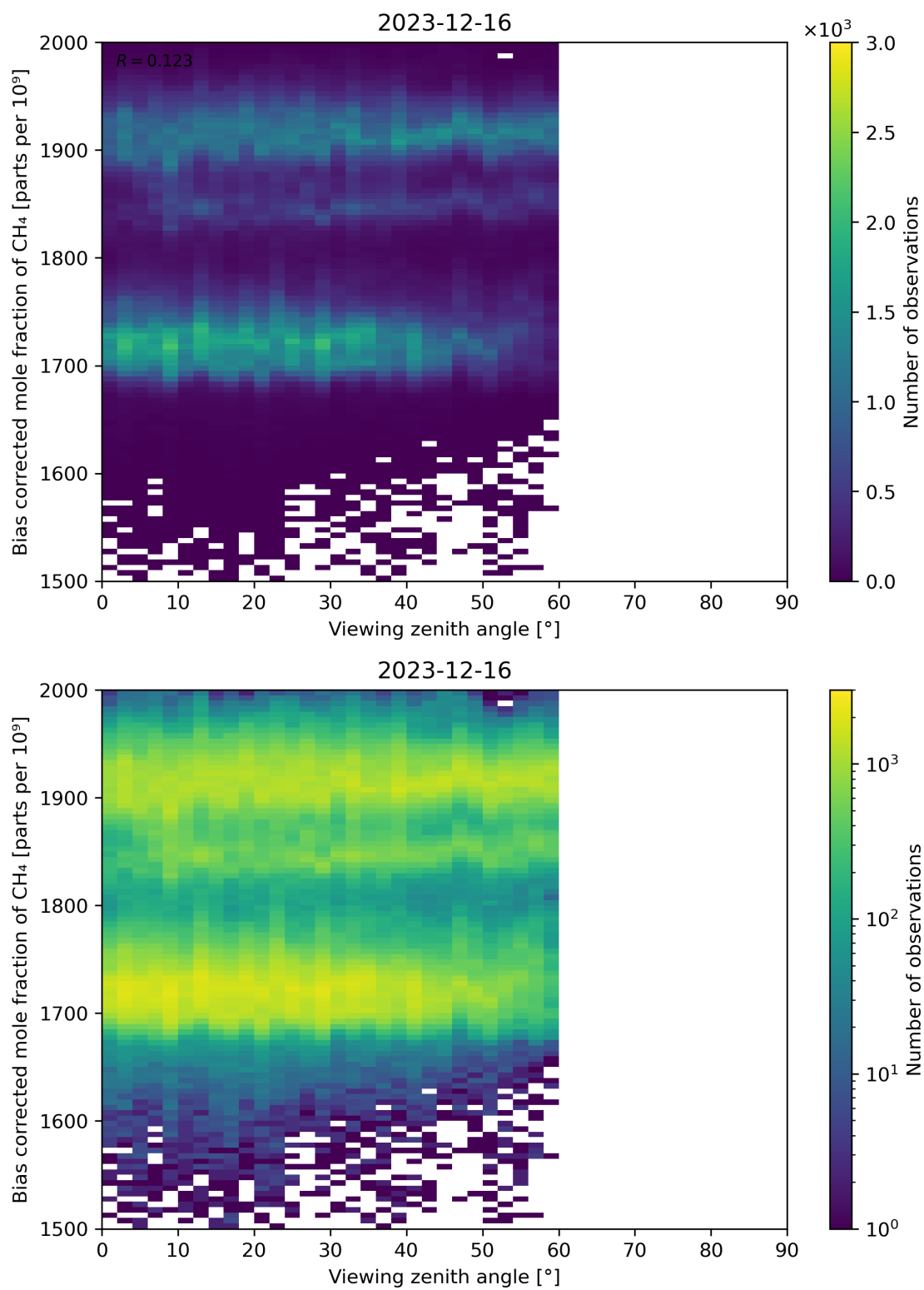
Figure 111: Scatter density plot of “Viewing zenith angle” against “Bias corrected mole fraction of CH 4 ” for 2023-12-15 to 2023-12-17.
