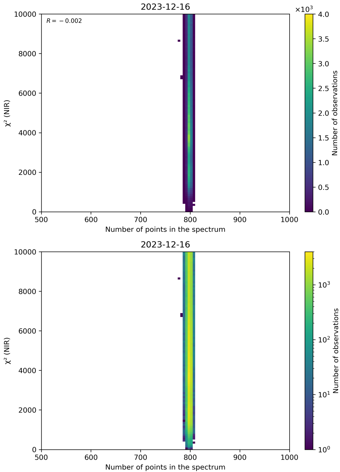
Figure 88: Scatter density plot of “Number of points in the spectrum” against “ \chi^2 (NIR)” for 2023-12-15 to 2023-12-17.
