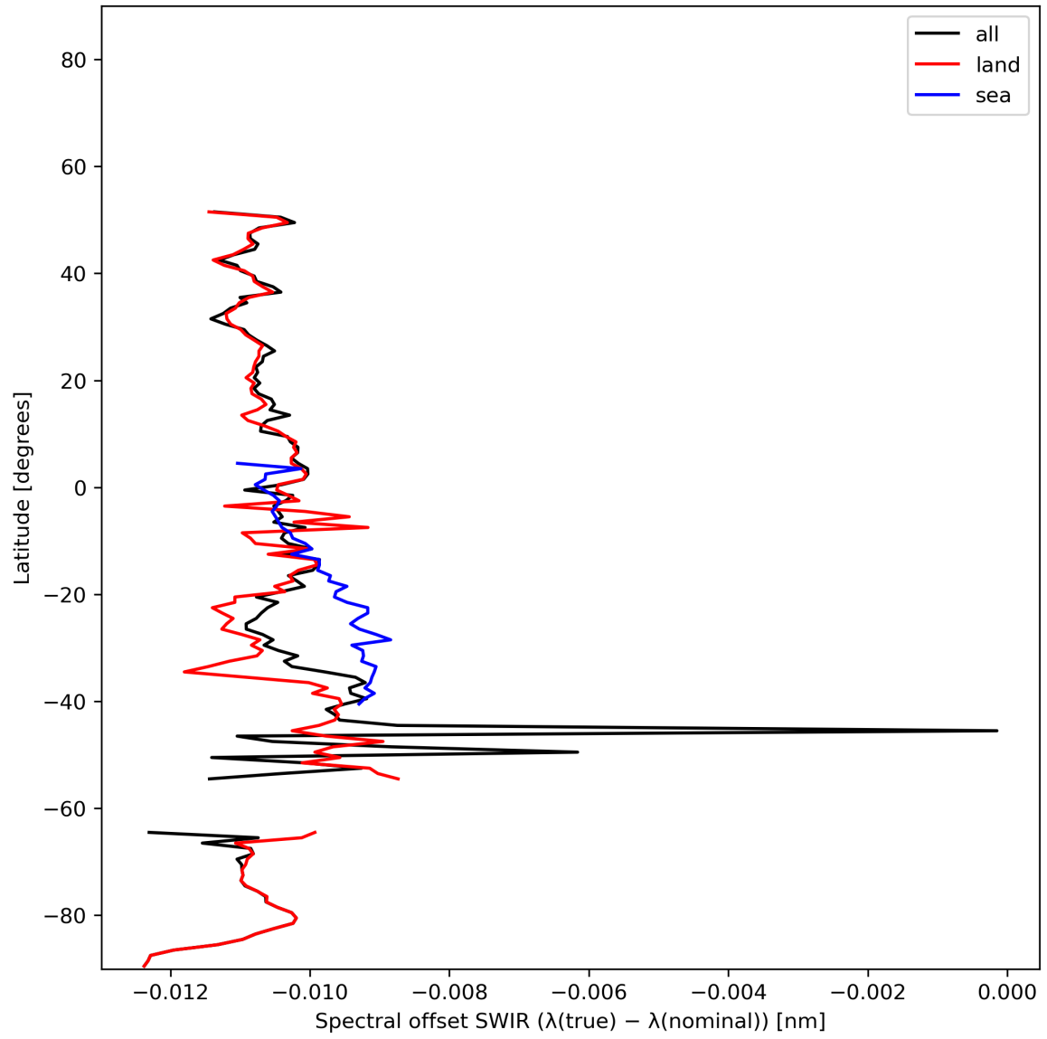
Figure 16: Zonal average of “Spectral offset SWIR ( \lambda(\text{true}) - \lambda(\text{nominal}) )” for 2023-12-15 to 2023-12-17.
