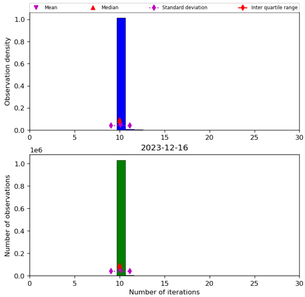
Figure 31: Histogram of “Number of iterations” for 2023-12-15 to 2023-12-17
