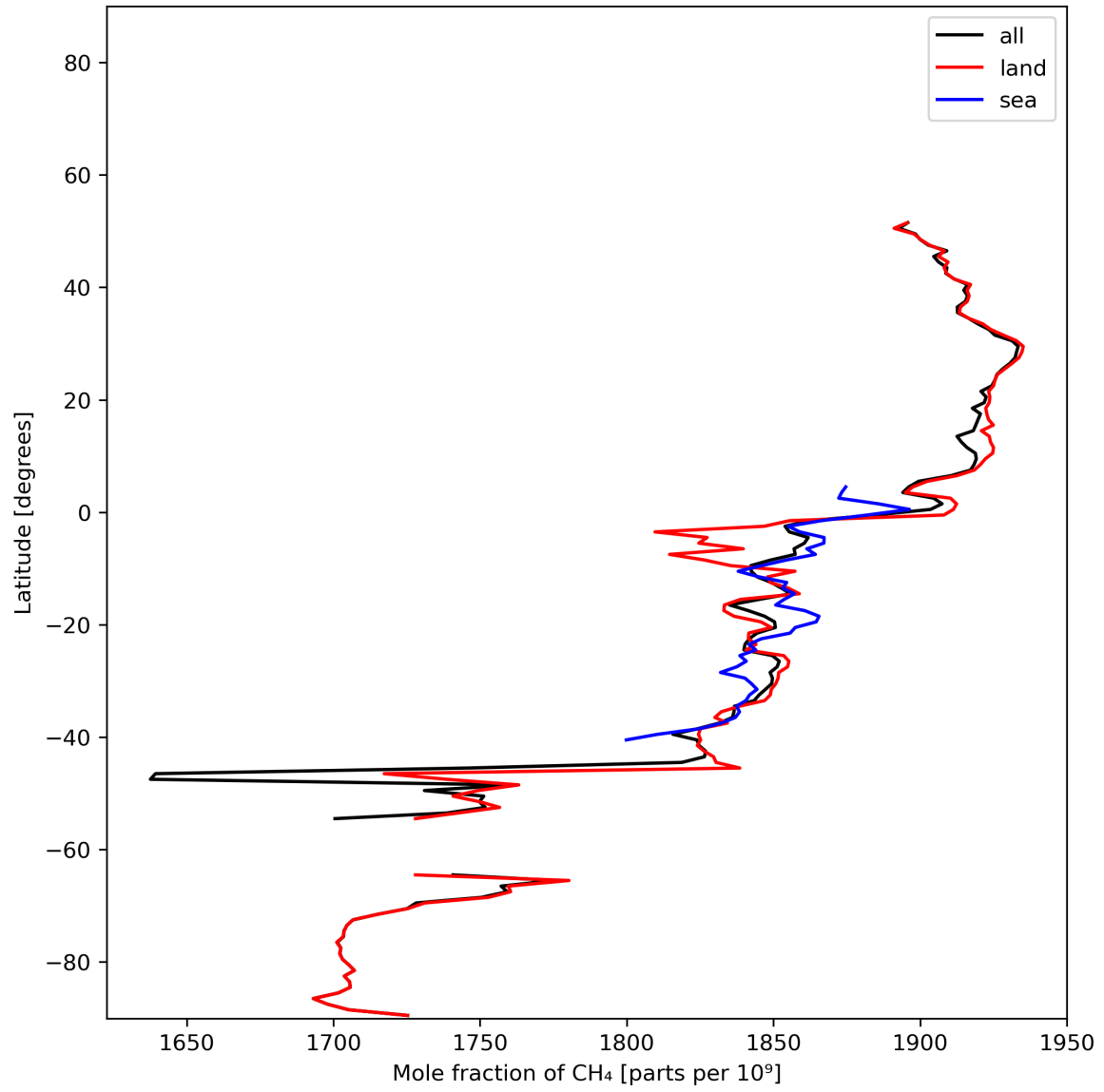
Figure 12: Zonal average of “Mole fraction of \text{CH}_4 ” for 2023-12-15 to 2023-12-17.
