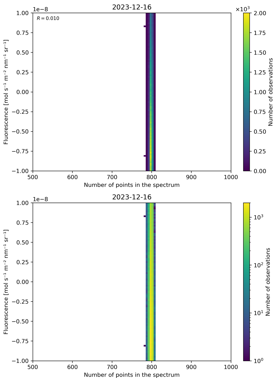
Figure 91: Scatter density plot of “Number of points in the spectrum” against “Fluorescence” for 2023-12-15 to 2023-12-17.
