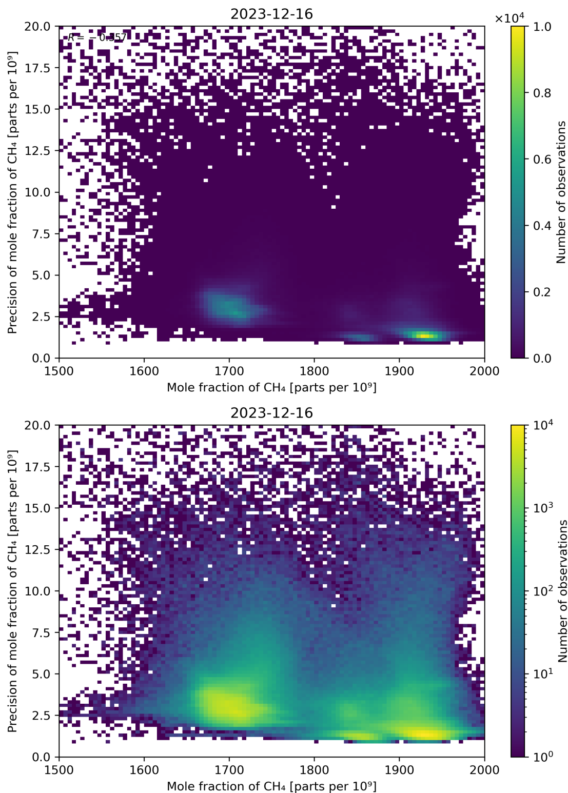
Figure 75: Scatter density plot of “Mole fraction of CH 4 ” against “Precision of mole fraction of CH 4 ” for 2023-12-15 to 2023-12-17.
