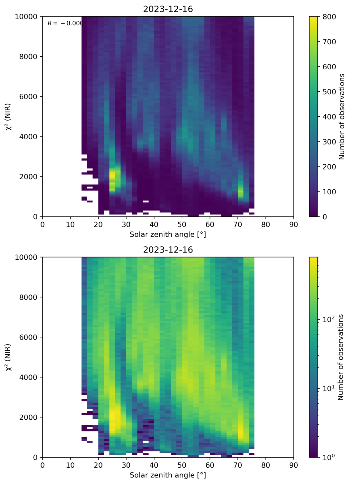
Figure 94: Scatter density plot of “Solar zenith angle” against “ \chi^2 (NIR)” for 2023-12-15 to 2023-12-17.
