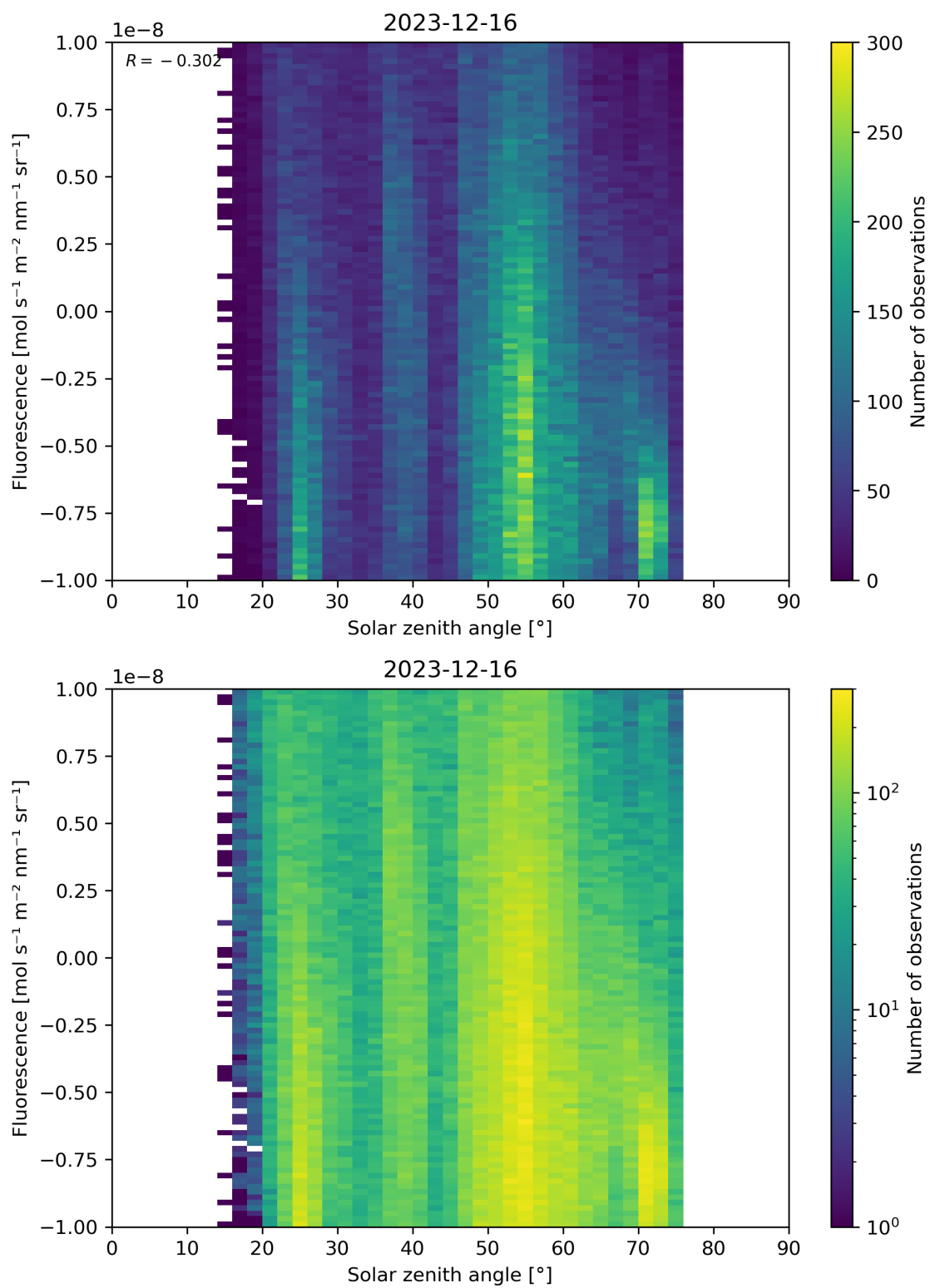
Figure 97: Scatter density plot of “Solar zenith angle” against “Fluorescence” for 2023-12-15 to 2023-12-17.
