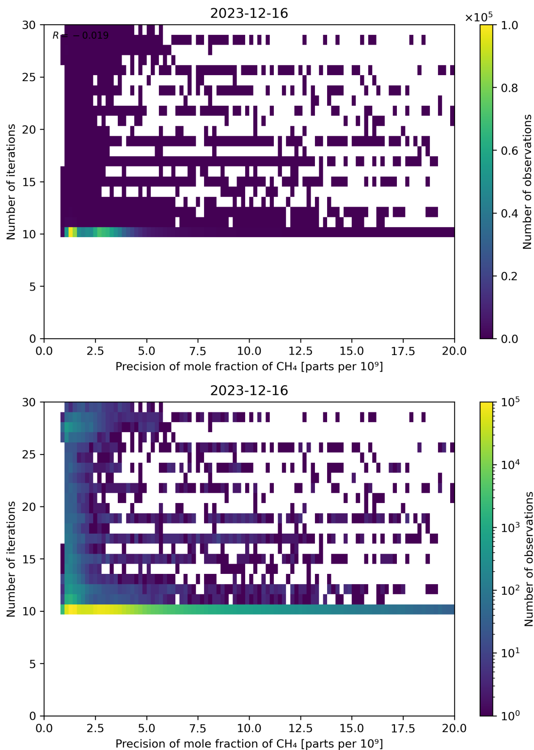
Figure 83: Scatter density plot of “Precision of mole fraction of CH 4 ” against “Number of iterations” for 2023-12-15 to 2023-12-17.
