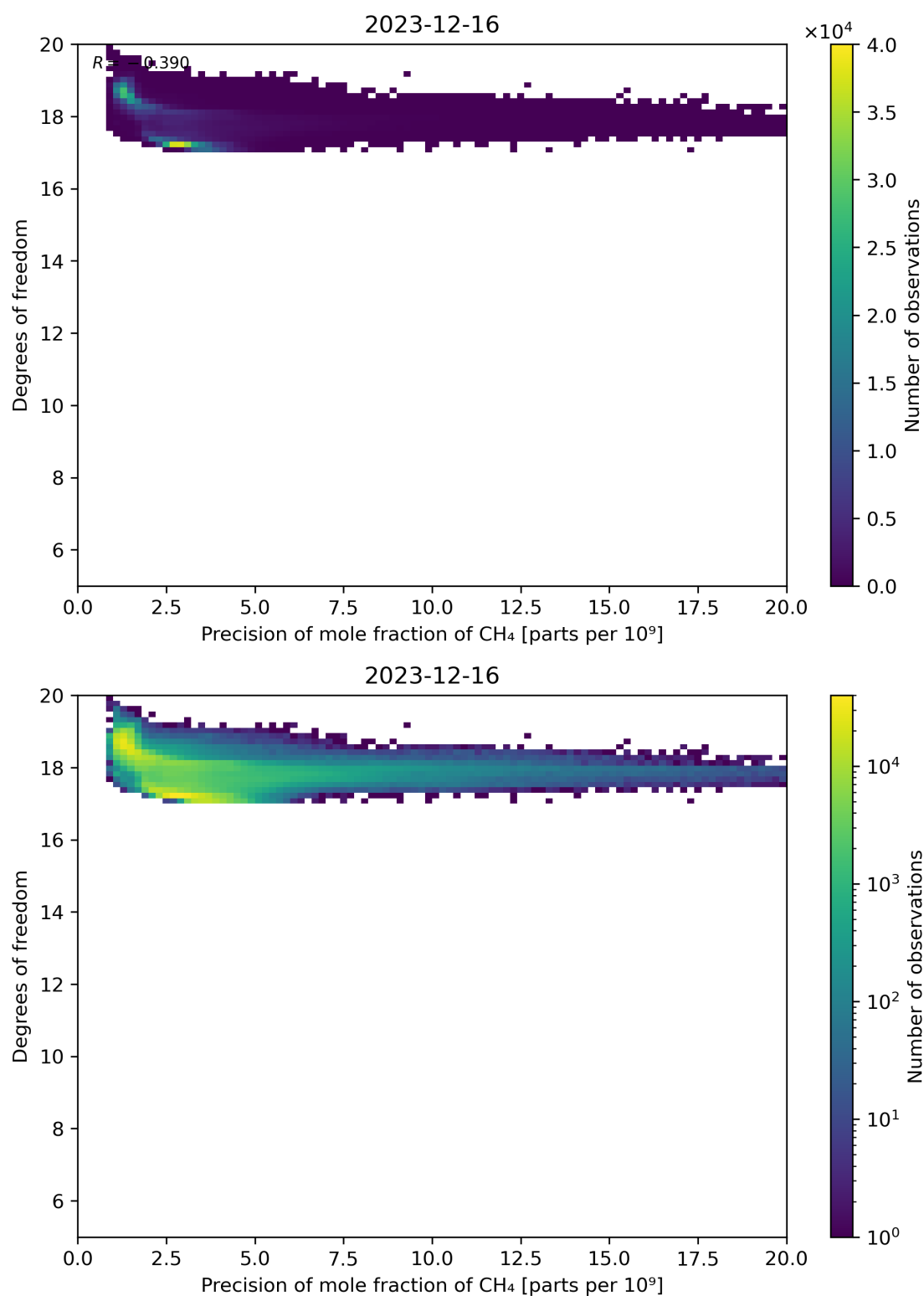
Figure 80: Scatter density plot of “Precision of mole fraction of CH 4 ” against “Degrees of freedom” for 2023-12-15 to 2023-12-17.
