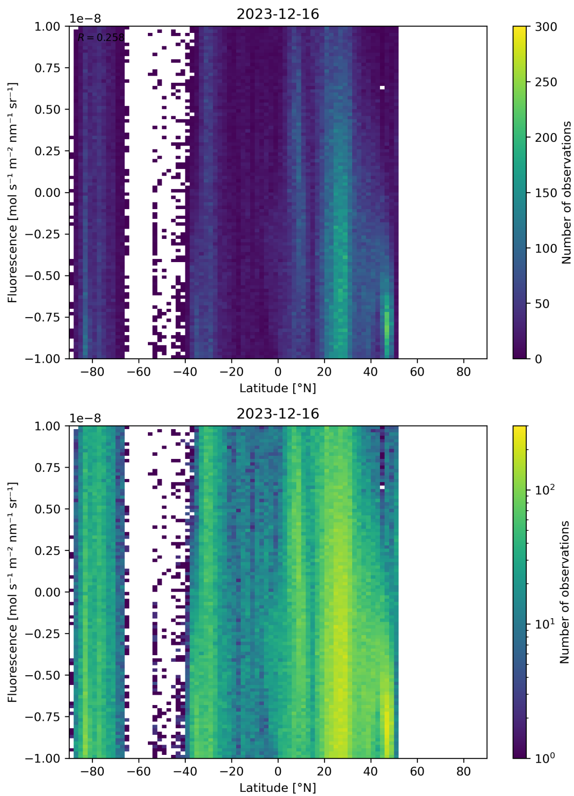
Figure 56: Scatter density plot of “Latitude” against “Fluorescence” for 2023-12-15 to 2023-12-17.
