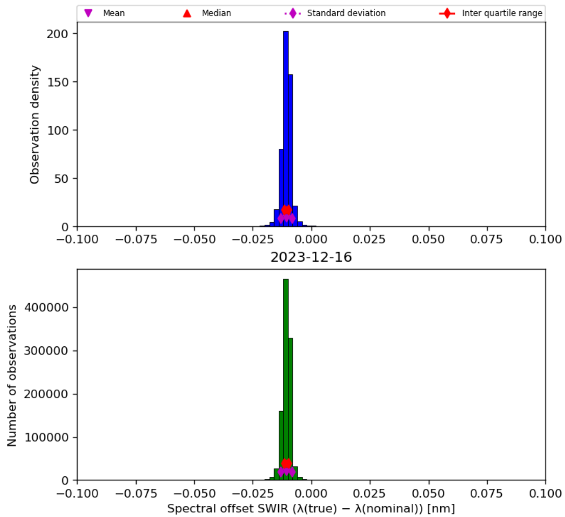
Figure 27: Histogram of “Spectral offset SWIR ( \lambda(\text{true}) - \lambda(\text{nominal}) )” for 2023-12-15 to 2023-12-17
