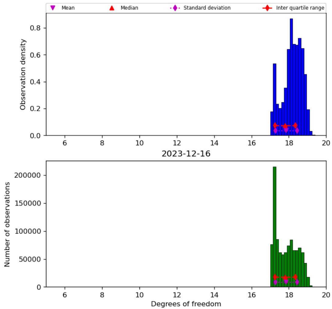
Figure 30: Histogram of “Degrees of freedom” for 2023-12-15 to 2023-12-17
