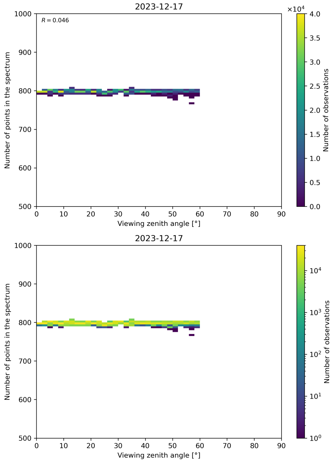
Figure 114: Scatter density plot of “Viewing zenith angle” against “Number of points in the spectrum” for 2023-12-16 to 2023-12-18.
