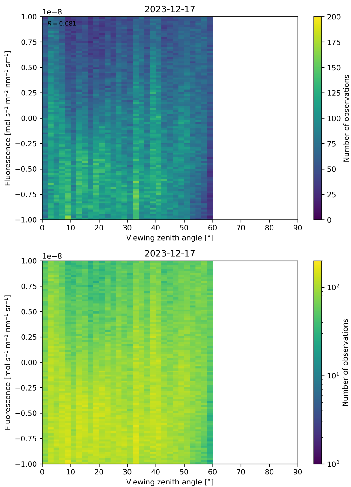
Figure 108: Scatter density plot of “Viewing zenith angle” against “Fluorescence” for 2023-12-16 to 2023-12-18.
