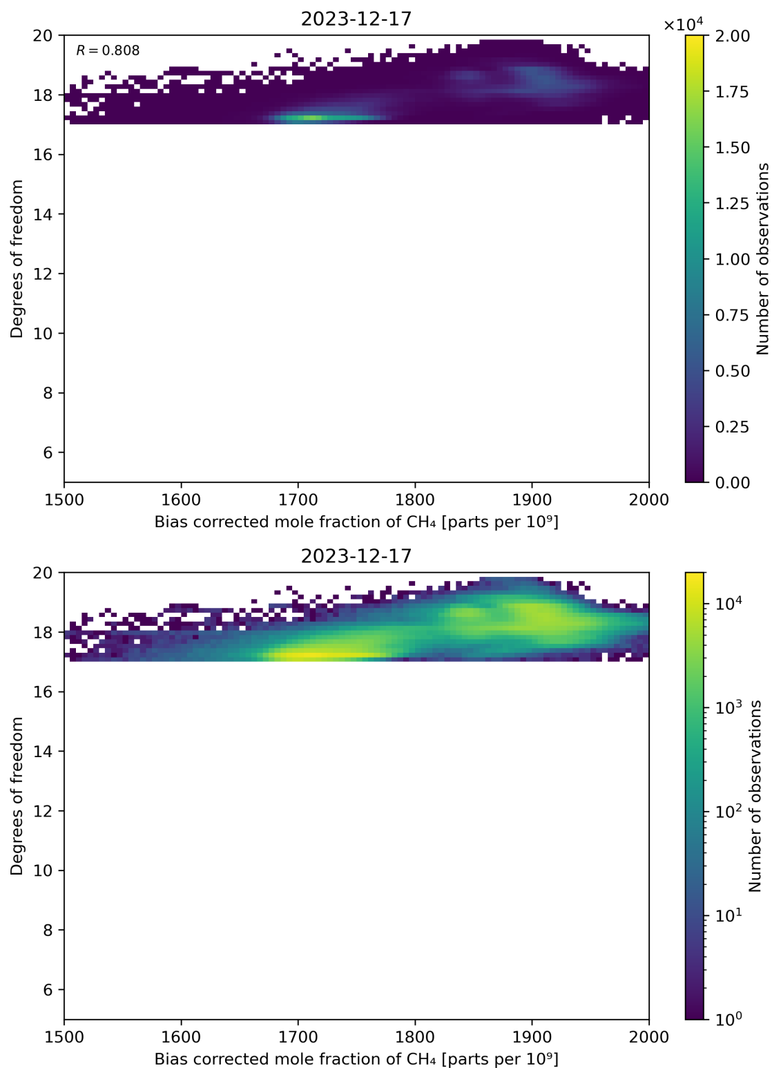
Figure 65: Scatter density plot of “Bias corrected mole fraction of CH 4 ” against “Degrees of freedom” for 2023-12-16 to 2023-12-18.
