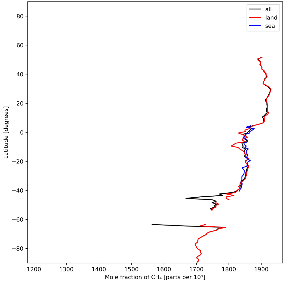
Figure 12: Zonal average of “Mole fraction of \text{CH}_4 ” for 2023-12-16 to 2023-12-18.
