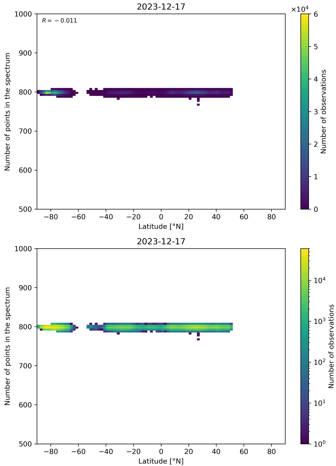
Figure 61: Scatter density plot of “Latitude” against “Number of points in the spectrum” for 2023-12-16 to 2023-12-18.
