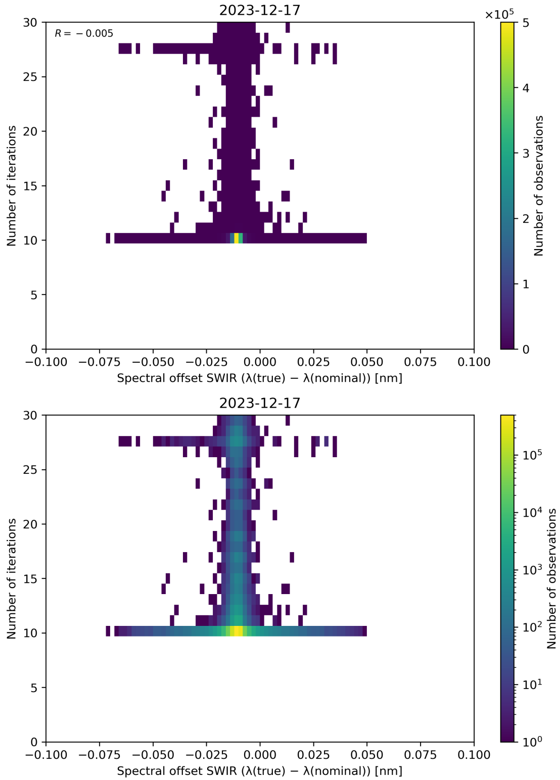
Figure 121: Scatter density plot of “Spectral offset SWIR ( \lambda(\text{true}) - \lambda(\text{nominal}) )” against “Number of iterations” for 2023-12-16 to 2023-12-18.
