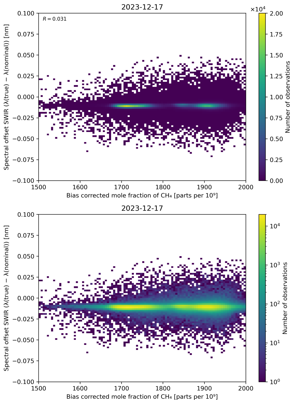
Figure 69: Scatter density plot of “Bias corrected mole fraction of \text{CH}_4 ” against “Spectral offset SWIR ( \lambda(\text{true}) - \lambda(\text{nominal}) )” for 2023-12-16 to 2023-12-18.
