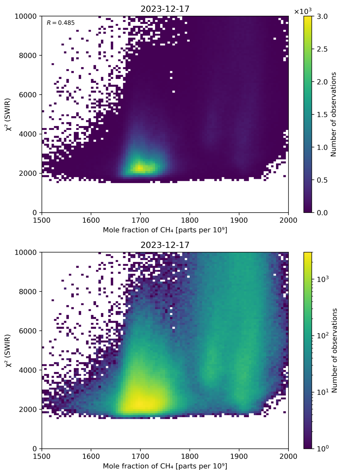
Figure 71: Scatter density plot of “Mole fraction of \text{CH}_4 ” against “ \chi^2 (SWIR)” for 2023-12-16 to 2023-12-18.
