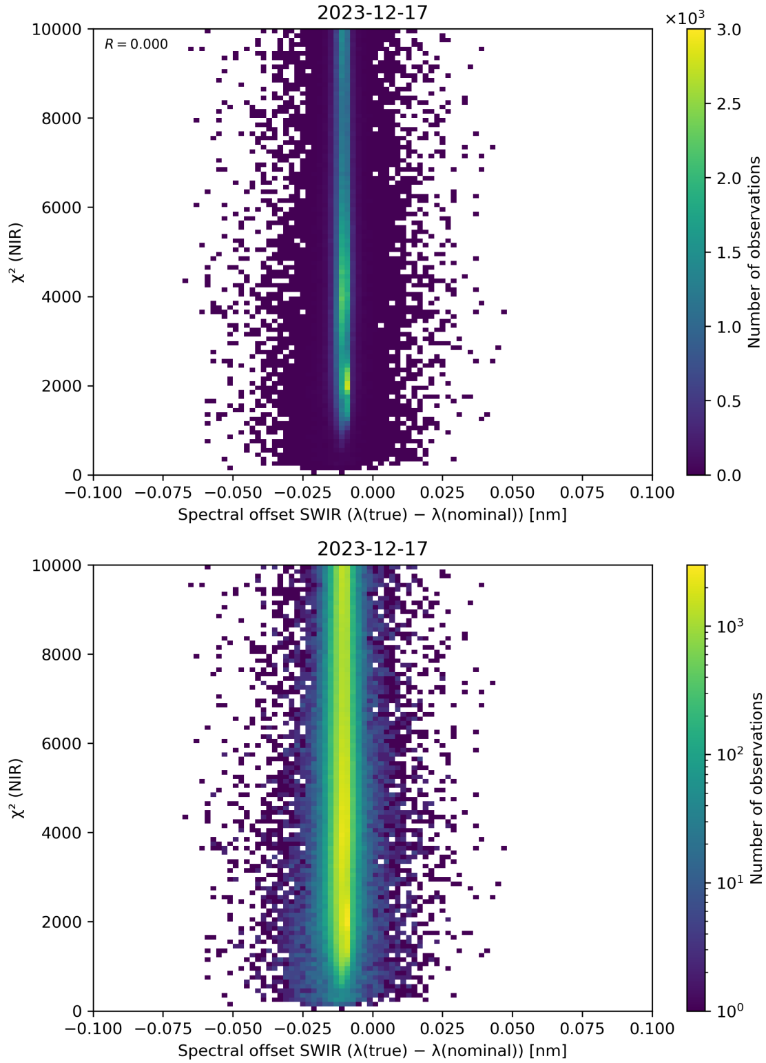
Figure 117: Scatter density plot of “Spectral offset SWIR ( \lambda(\text{true}) - \lambda(\text{nominal}) )” against “ \chi^2 (NIR)” for 2023-12-16 to 2023-12-18.
