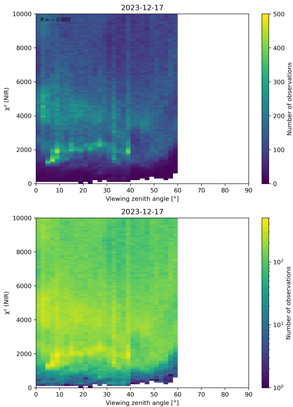
Figure 105: Scatter density plot of “Viewing zenith angle” against “ \chi^2 (NIR)” for 2023-12-16 to 2023-12-18.
