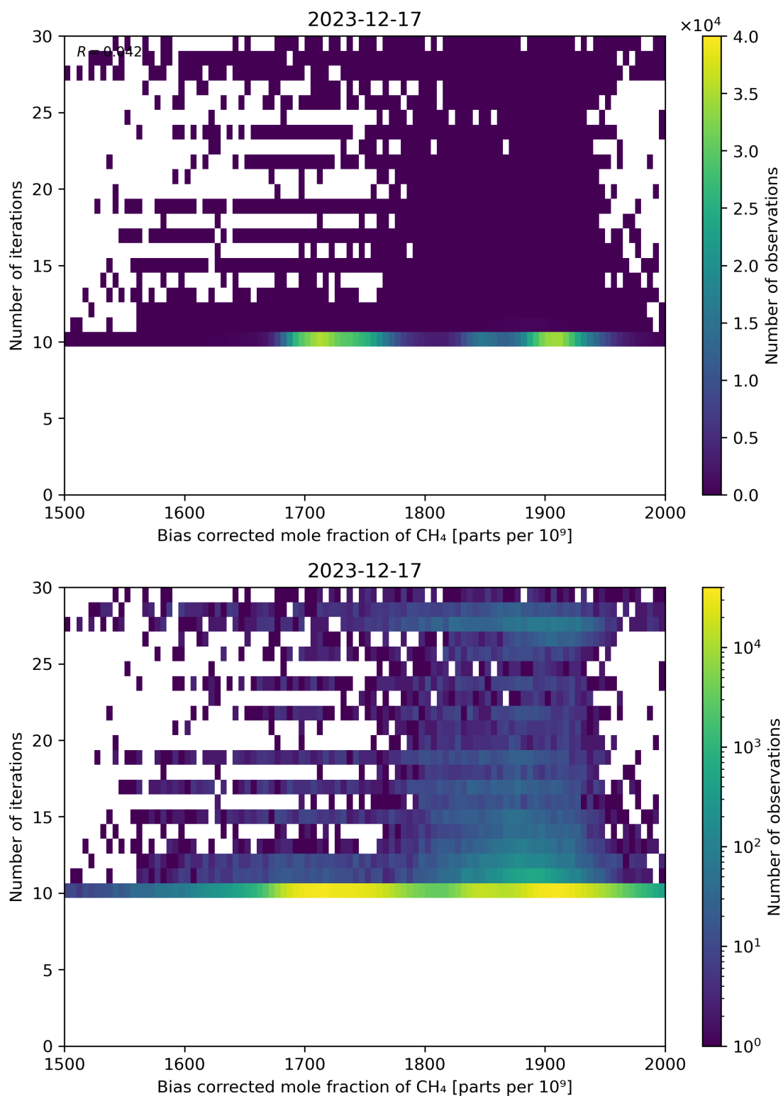
Figure 67: Scatter density plot of “Bias corrected mole fraction of CH 4 ” against “Number of iterations” for 2023-12-16 to 2023-12-18.
