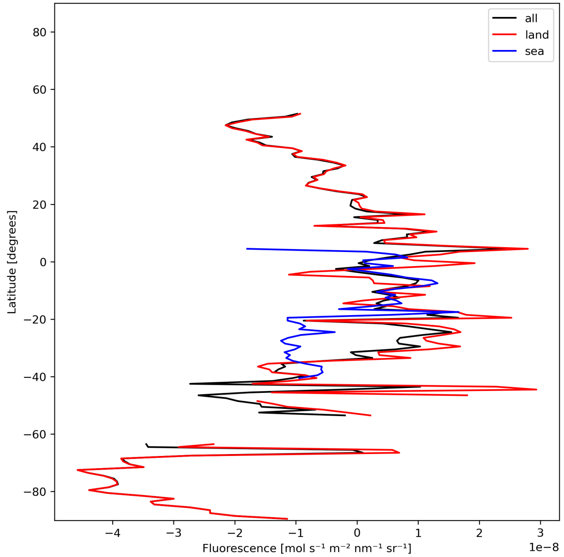
Figure 21: Zonal average of “Fluorescence” for 2023-12-16 to 2023-12-18.
