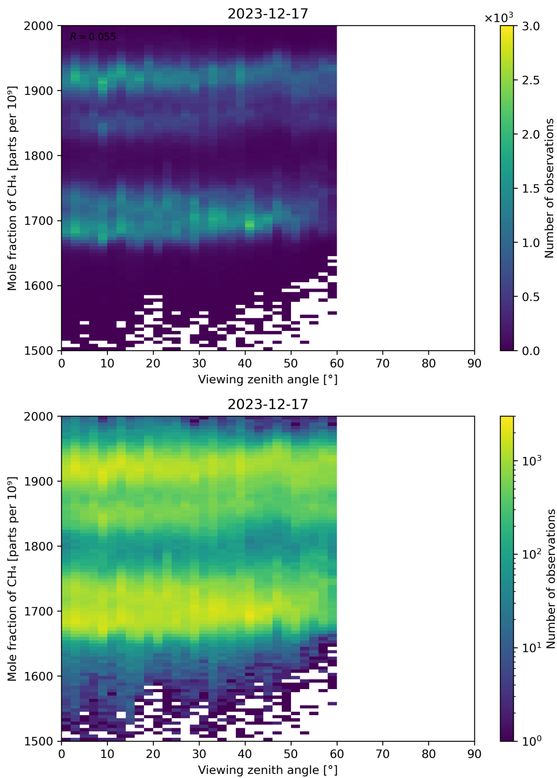
Figure 110: Scatter density plot of “Viewing zenith angle” against “Mole fraction of CH 4 ” for 2023-12-16 to 2023-12-18.
