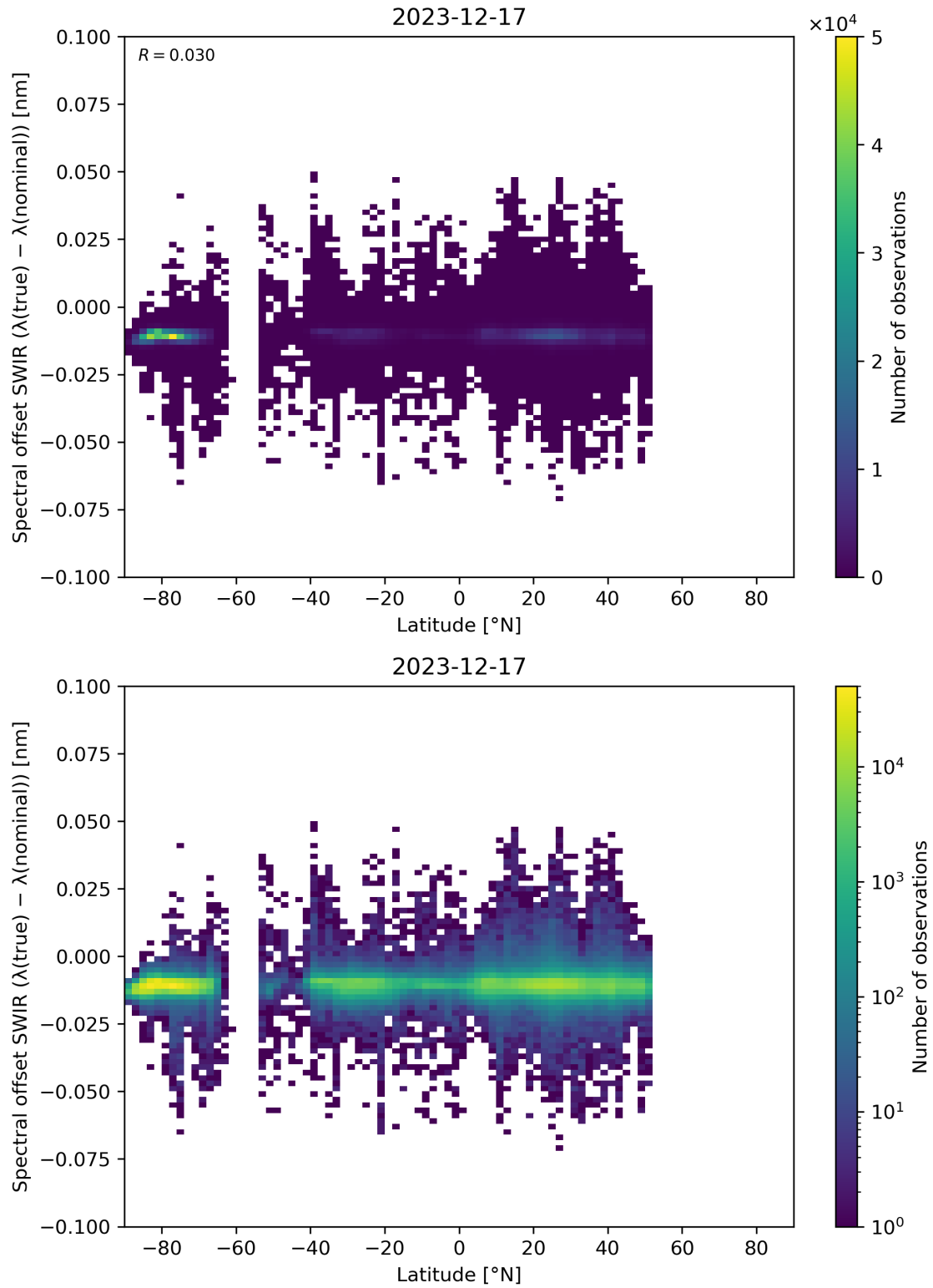
Figure 62: Scatter density plot of “Latitude” against “Spectral offset SWIR ( \lambda(\text{true}) - \lambda(\text{nominal}) )” for 2023-12-16 to 2023-12-18.
