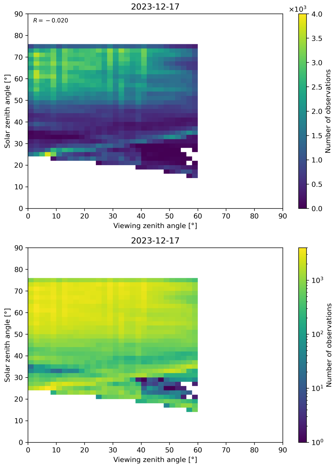
Figure 115: Scatter density plot of “Viewing zenith angle” against “Solar zenith angle” for 2023-12-16 to 2023-12-18.
