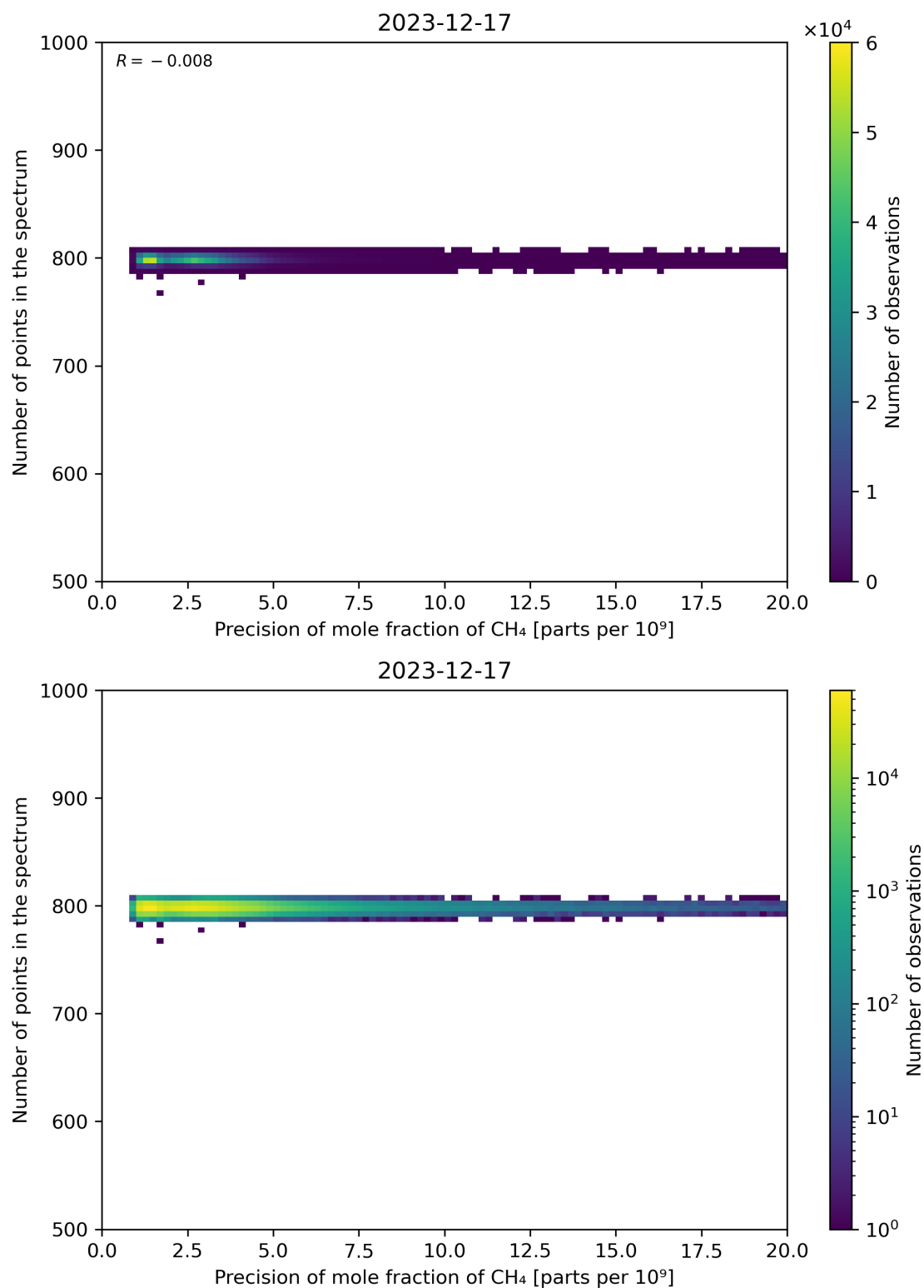
Figure 84: Scatter density plot of “Precision of mole fraction of CH 4 ” against “Number of points in the spectrum” for 2023-12-16 to 2023-12-18.
