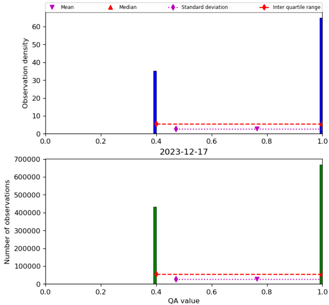
Figure 22: Histogram of “QA value” for 2023-12-16 to 2023-12-18
