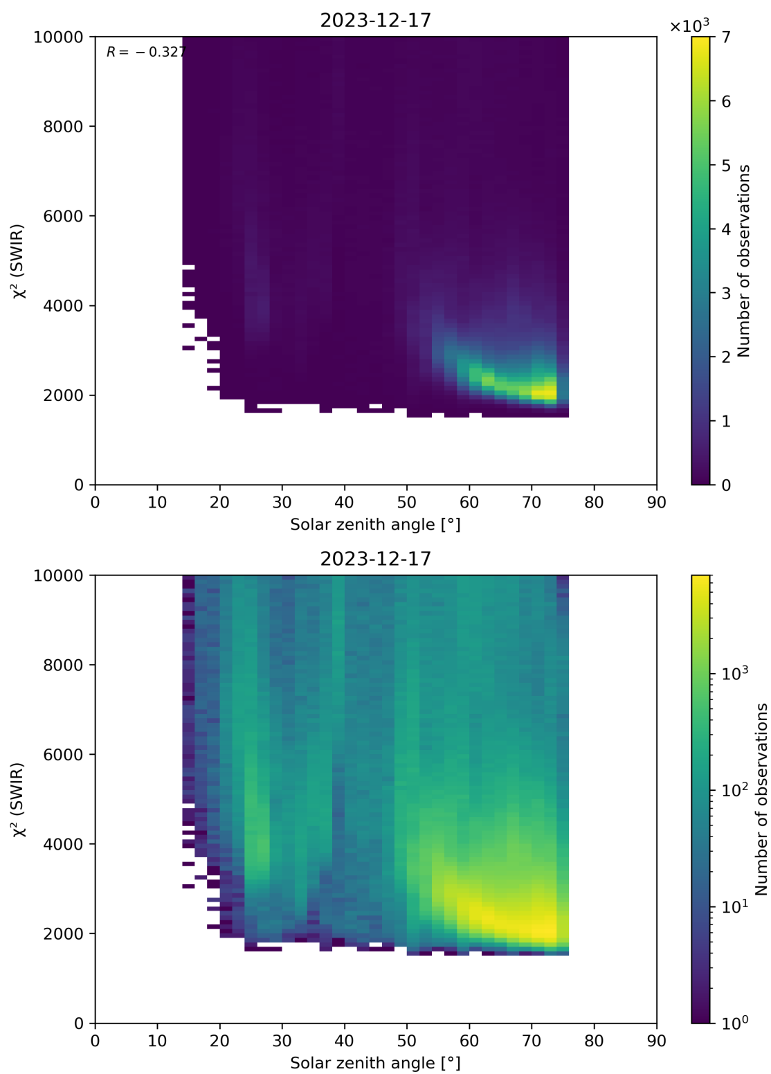
Figure 95: Scatter density plot of “Solar zenith angle” against “ \chi^2 (SWIR)” for 2023-12-16 to 2023-12-18.
