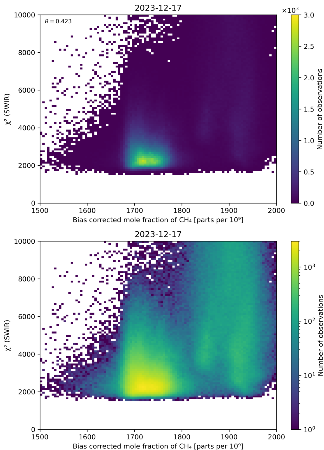
Figure 64: Scatter density plot of “Bias corrected mole fraction of CH 4 ” against “ \chi^2 (SWIR)” for 2023-12-16 to 2023-12-18.
