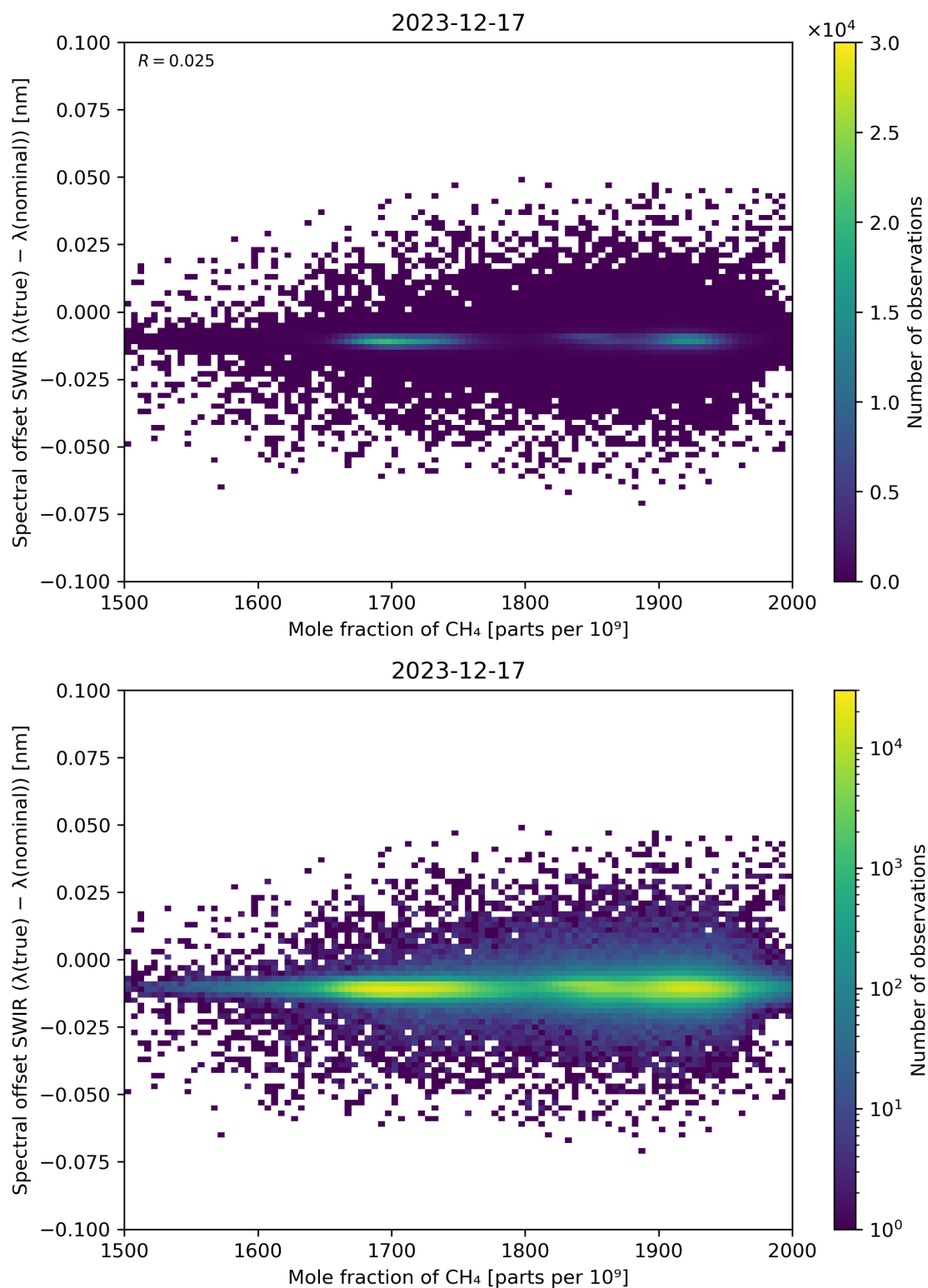
Figure 86: Scatter density plot of “Mole fraction of CH 4 ” against “Spectral offset SWIR ( \lambda(\text{true}) - \lambda(\text{nominal}) )” for 2023-12-16 to 2023-12-18.
