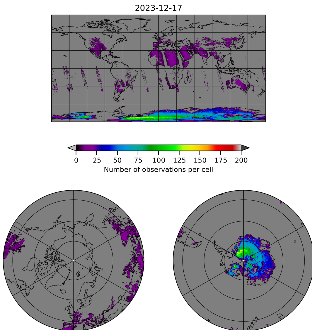
Figure 10: Map of the number of observations for 2023-12-16 to 2023-12-18
