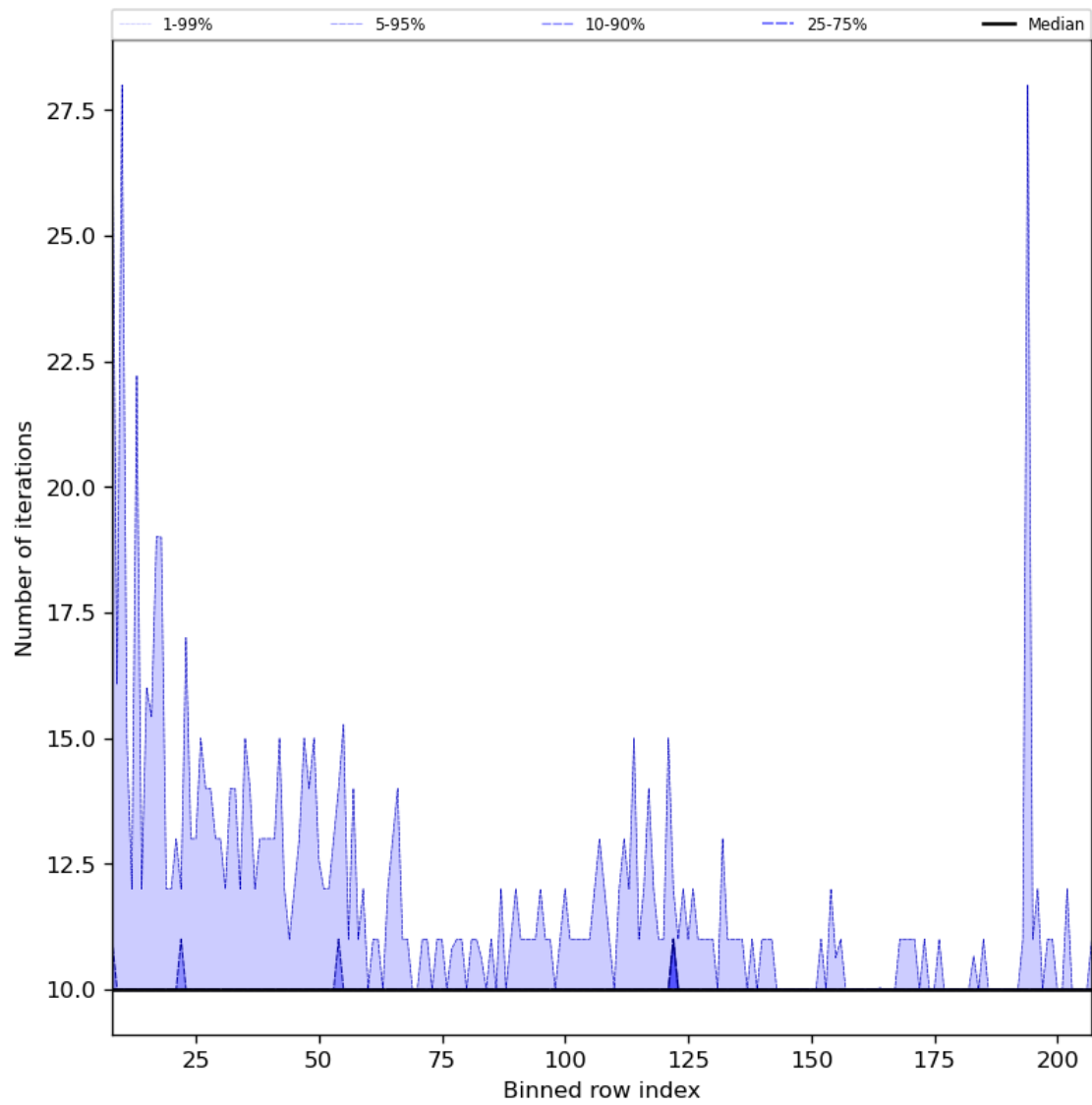
Figure 42: Along track statistics of “Number of iterations” for 2023-12-16 to 2023-12-18
