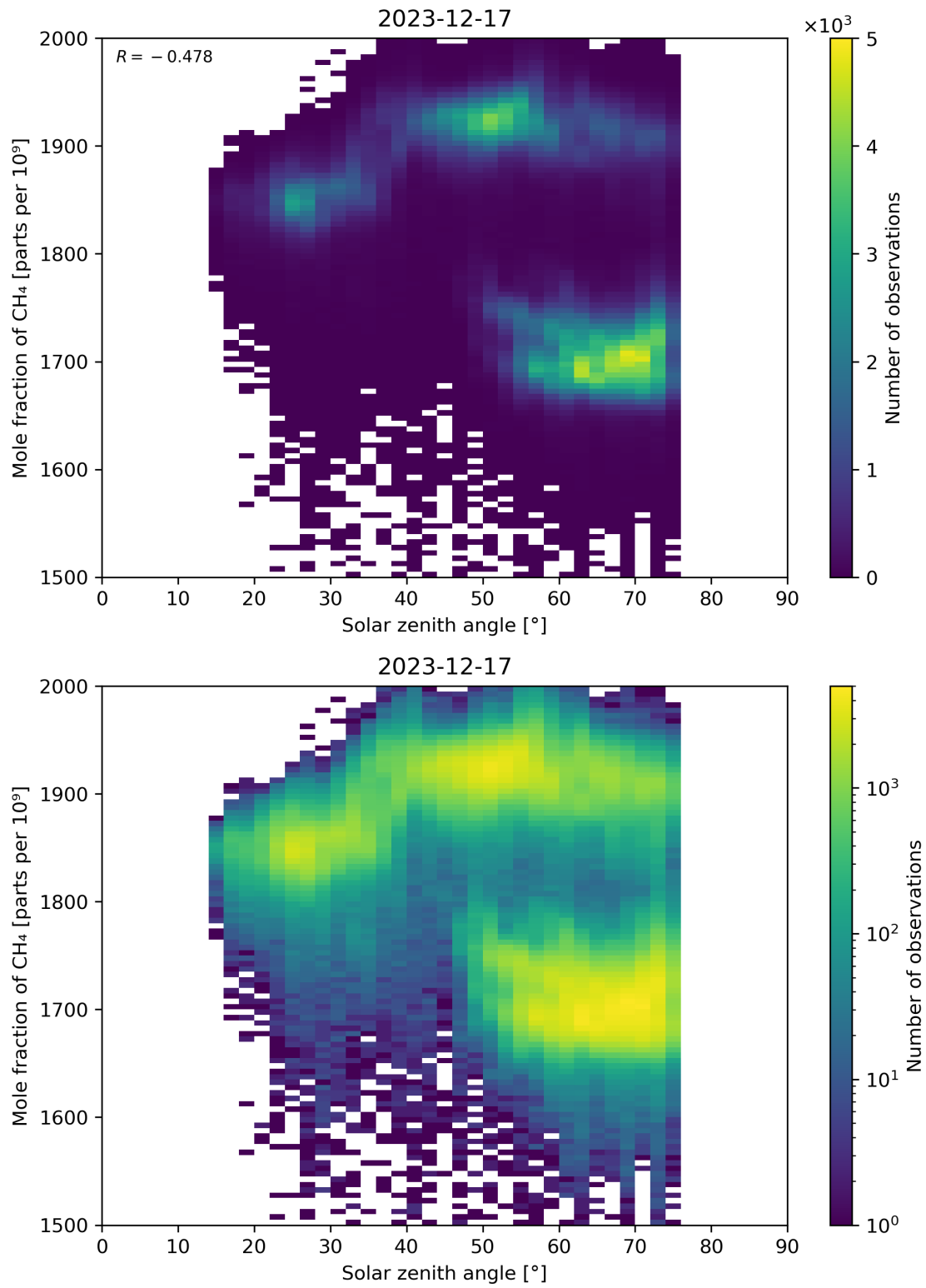
Figure 99: Scatter density plot of “Solar zenith angle” against “Mole fraction of \text{CH}_4 ” for 2023-12-16 to 2023-12-18.
