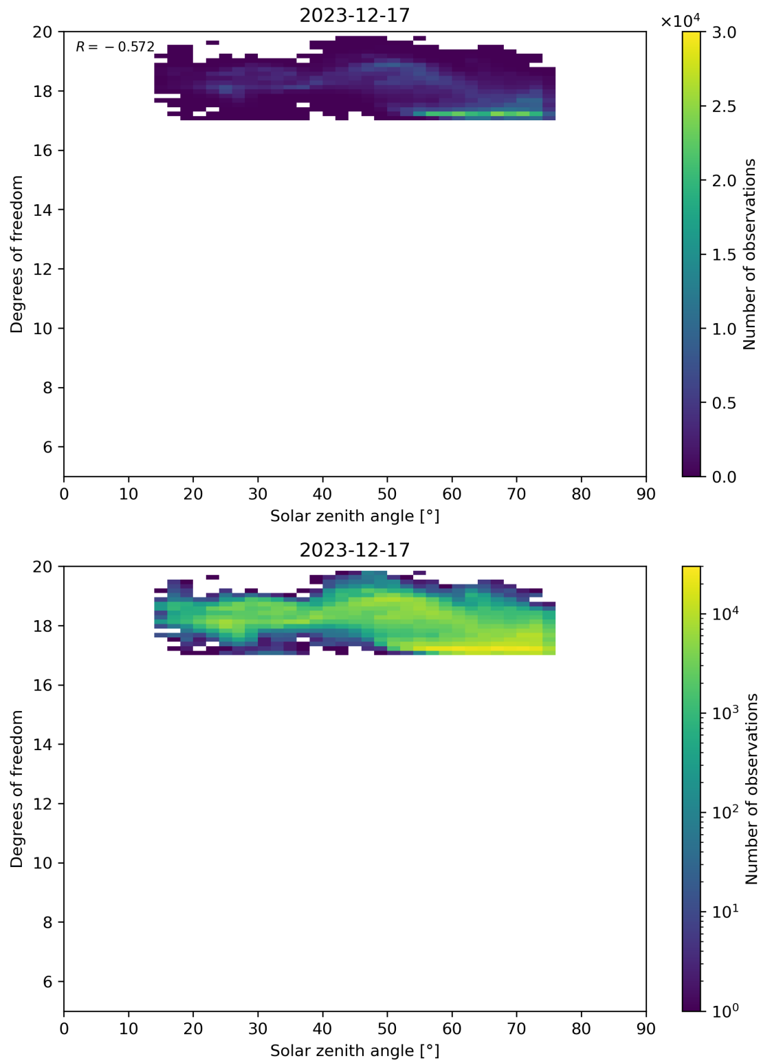
Figure 96: Scatter density plot of “Solar zenith angle” against “Degrees of freedom” for 2023-12-16 to 2023-12-18.
