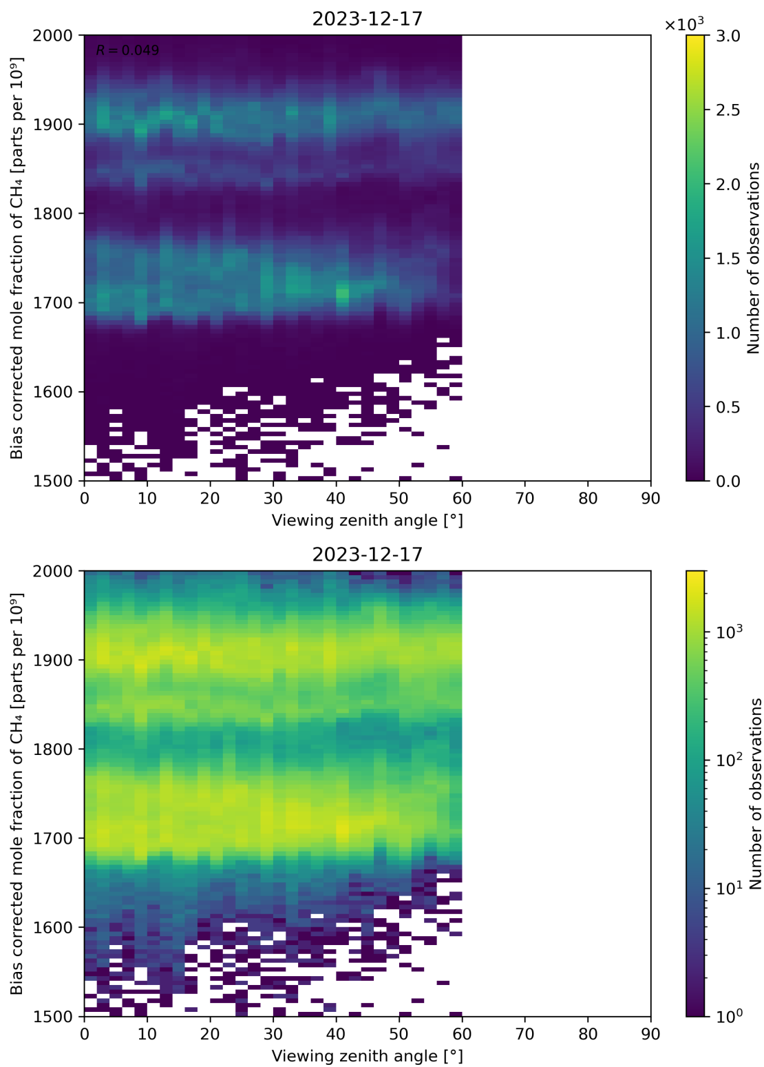
Figure 111: Scatter density plot of “Viewing zenith angle” against “Bias corrected mole fraction of CH 4 ” for 2023-12-16 to 2023-12-18.
