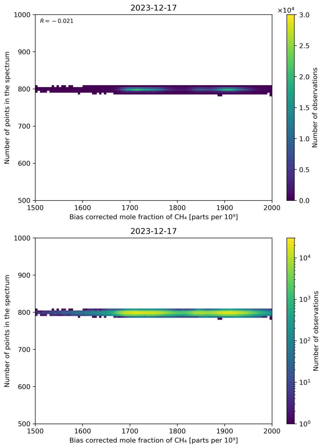
Figure 68: Scatter density plot of “Bias corrected mole fraction of CH 4 ” against “Number of points in the spectrum” for 2023-12-16 to 2023-12-18.
