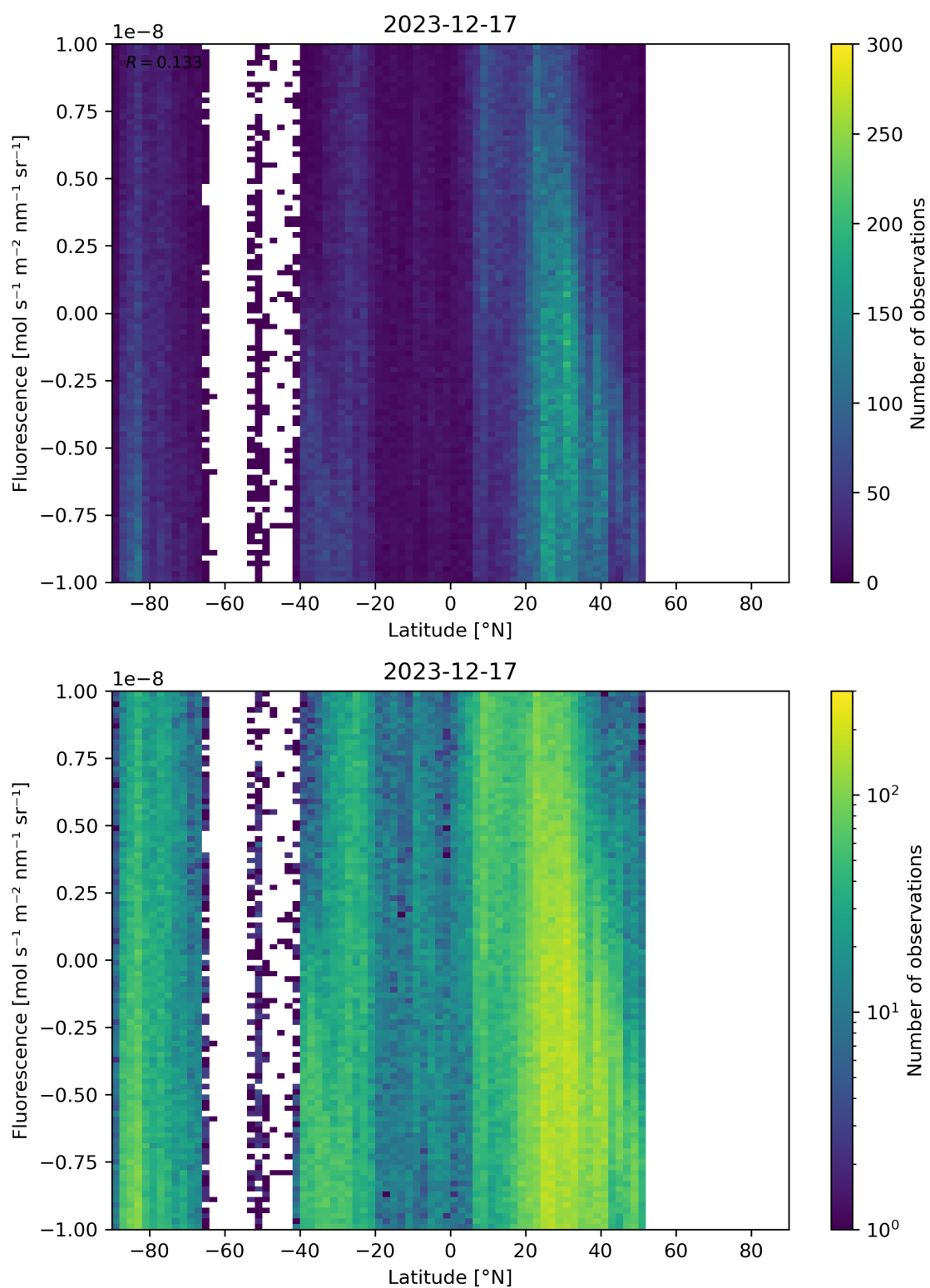
Figure 56: Scatter density plot of “Latitude” against “Fluorescence” for 2023-12-16 to 2023-12-18.
