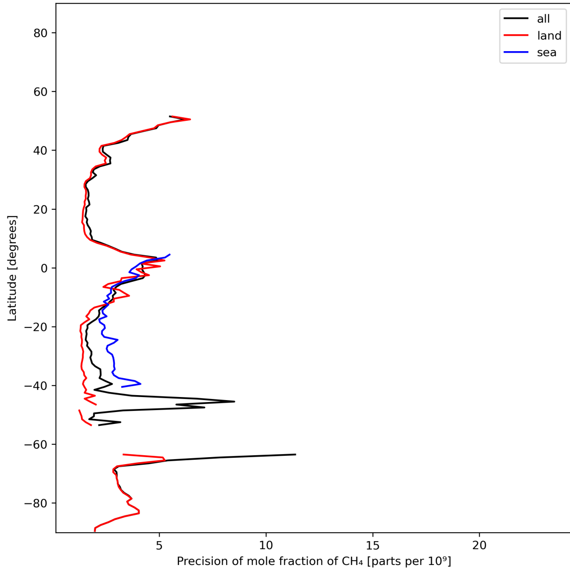
Figure 13: Zonal average of “Precision of mole fraction of CH 4 ” for 2023-12-16 to 2023-12-18.
