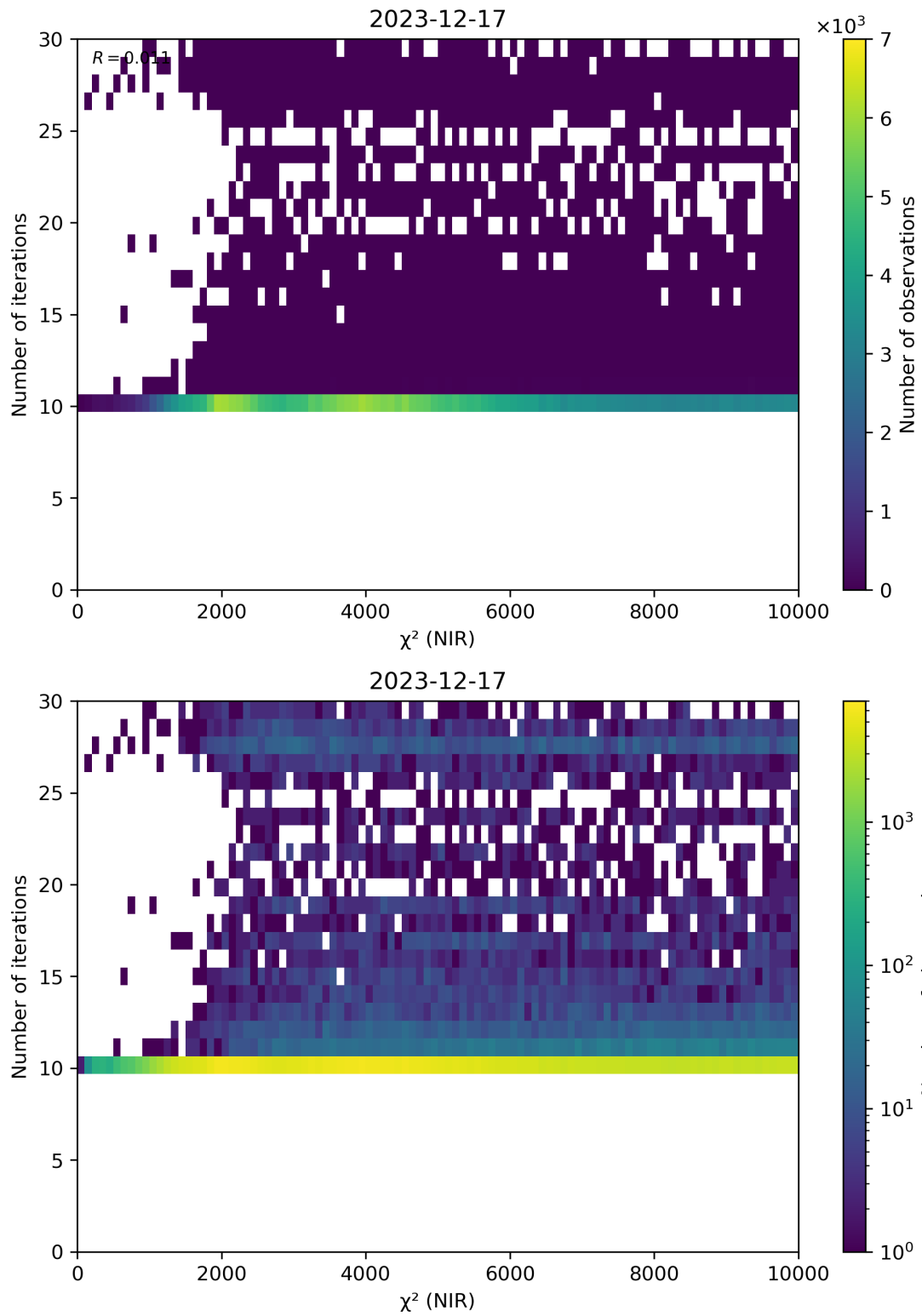
Figure 46: Scatter density plot of “ \chi^2 (NIR)” against “Number of iterations” for 2023-12-16 to 2023-12-18.
