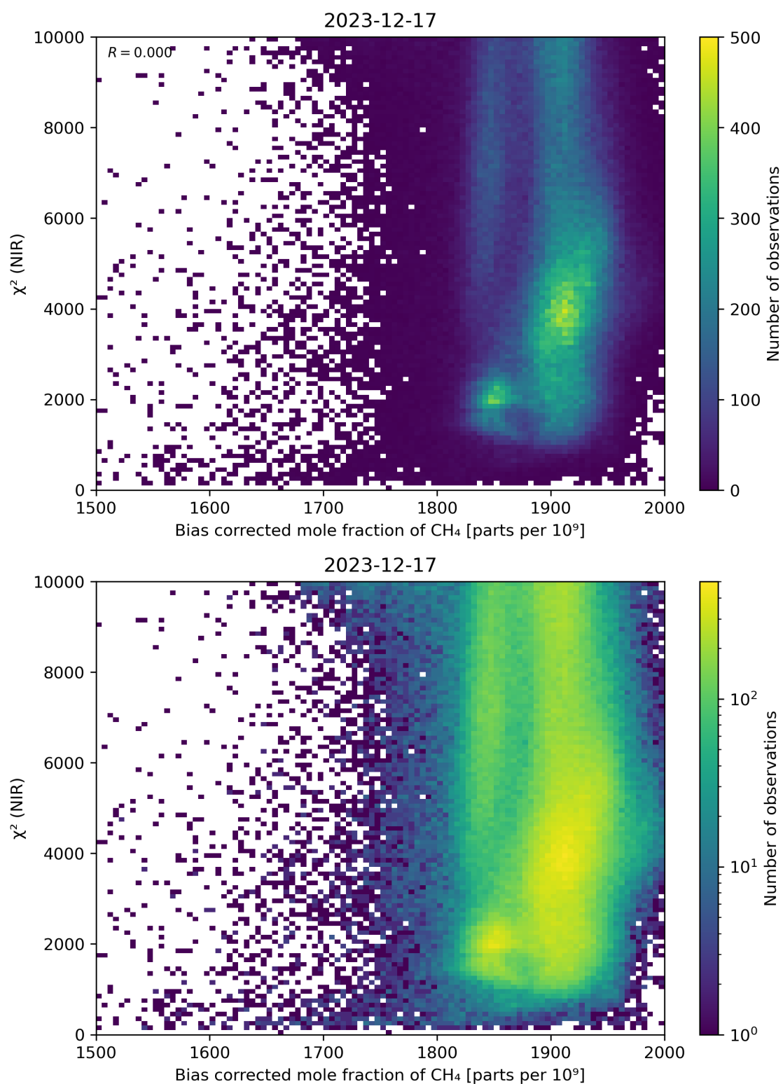
Figure 63: Scatter density plot of “Bias corrected mole fraction of CH 4 ” against “ \chi^2 (NIR)” for 2023-12-16 to 2023-12-18.
