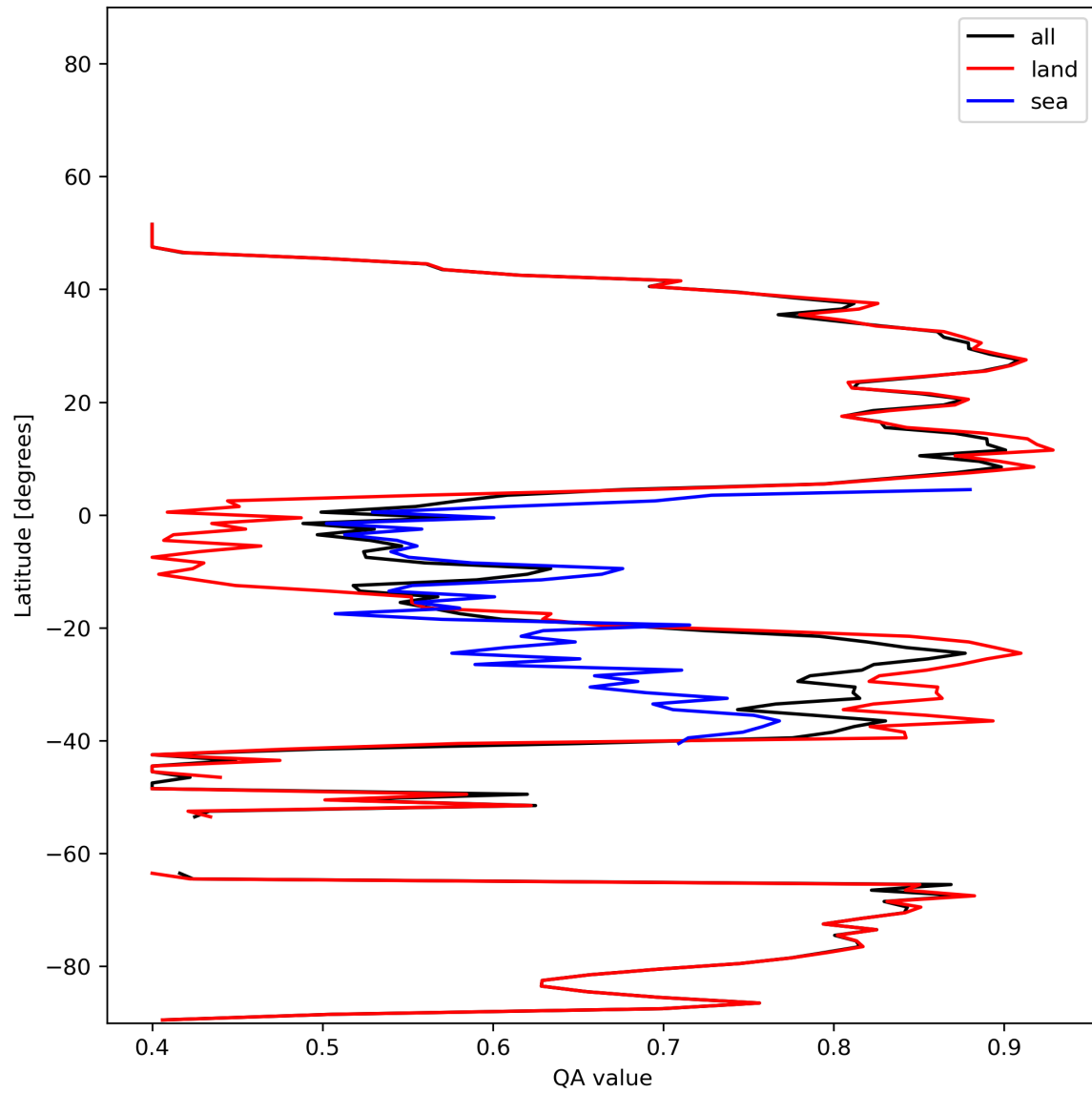
Figure 11: Zonal average of “QA value” for 2023-12-16 to 2023-12-18.
