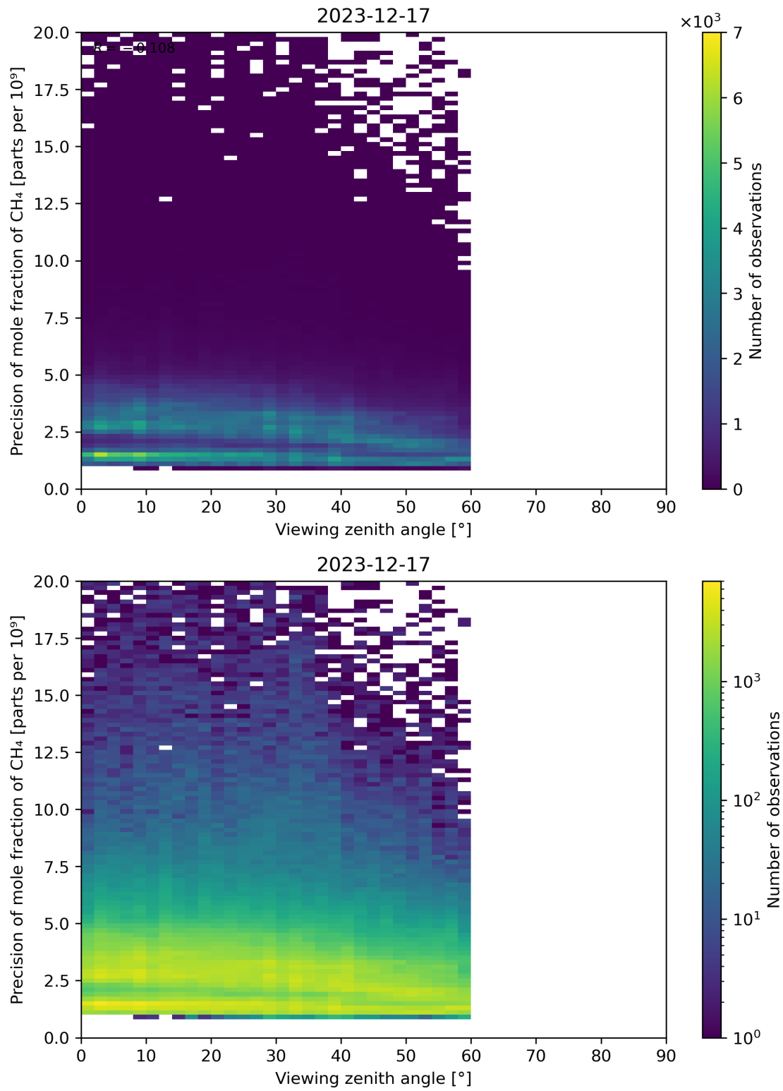
Figure 112: Scatter density plot of “Viewing zenith angle” against “Precision of mole fraction of CH 4 ” for 2023-12-16 to 2023-12-18.
