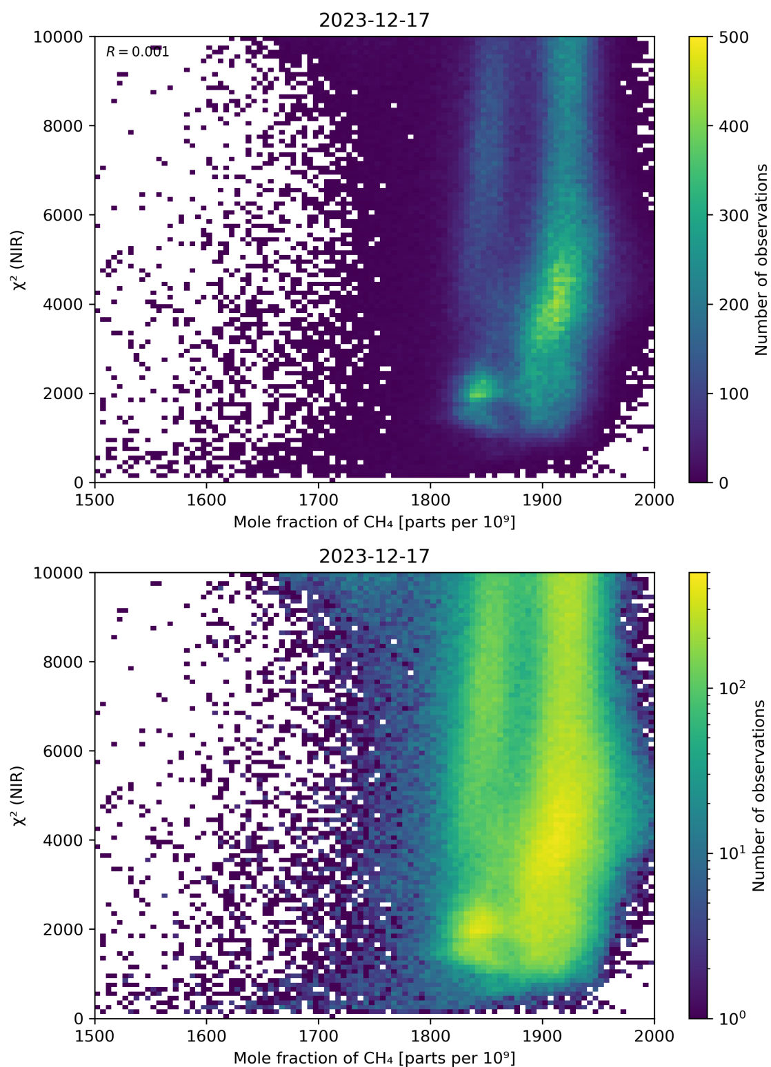
Figure 70: Scatter density plot of “Mole fraction of CH 4 ” against “ \chi^2 (NIR)” for 2023-12-16 to 2023-12-18.
