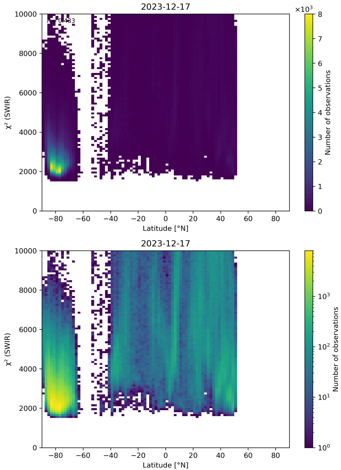
Figure 54: Scatter density plot of “Latitude” against “ \chi^2 (SWIR)” for 2023-12-16 to 2023-12-18.
