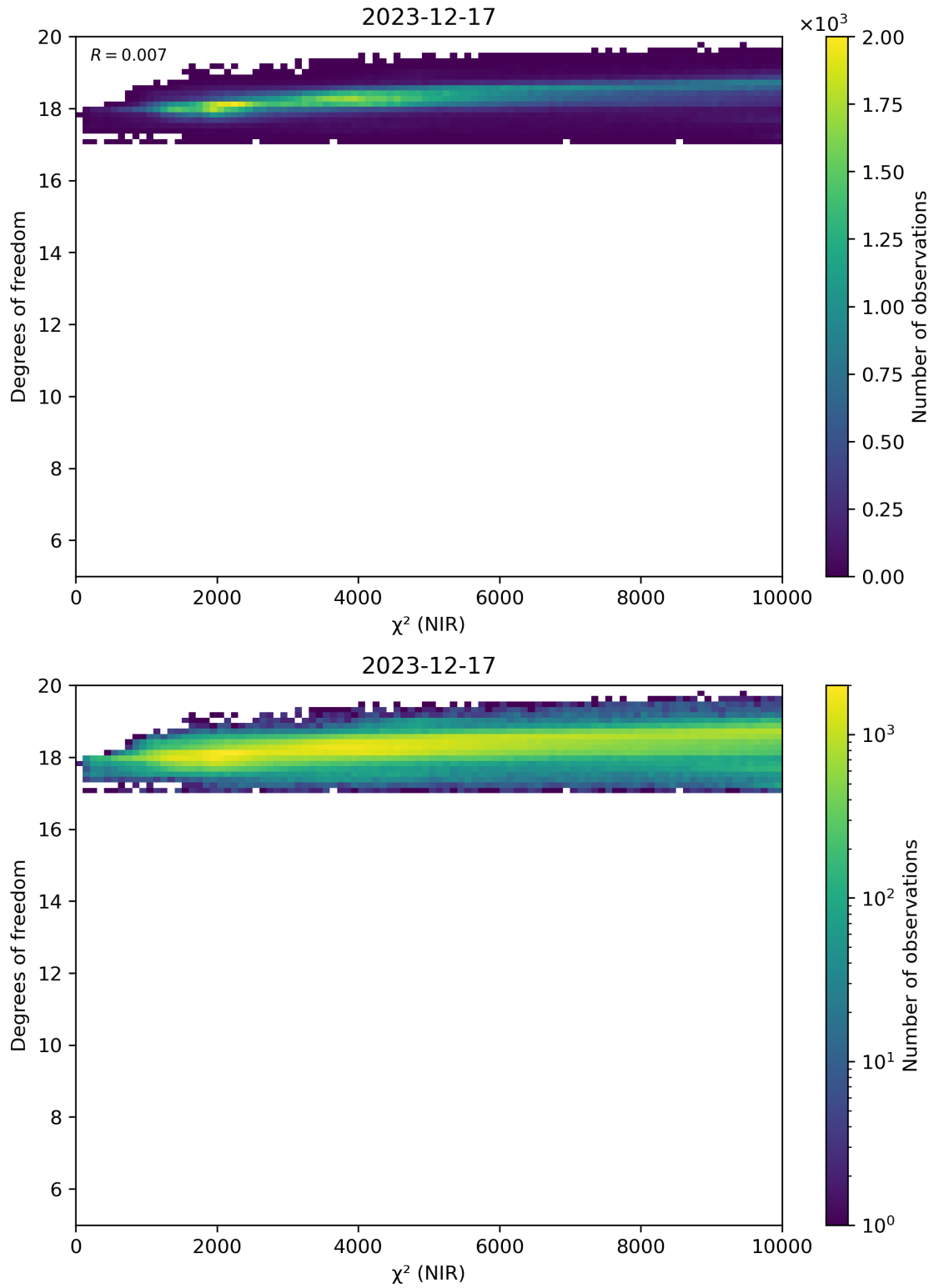
Figure 44: Scatter density plot of “ \chi^2 (NIR)” against “Degrees of freedom” for 2023-12-16 to 2023-12-18.
