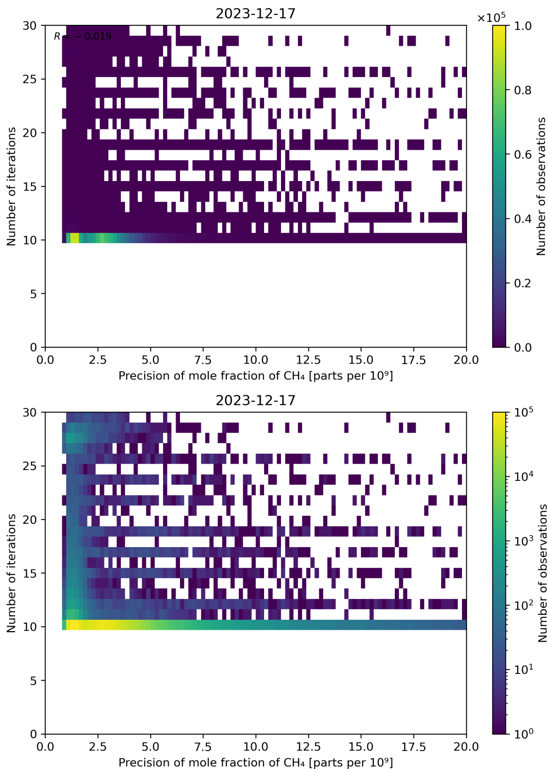
Figure 83: Scatter density plot of “Precision of mole fraction of CH 4 ” against “Number of iterations” for 2023-12-16 to 2023-12-18.
