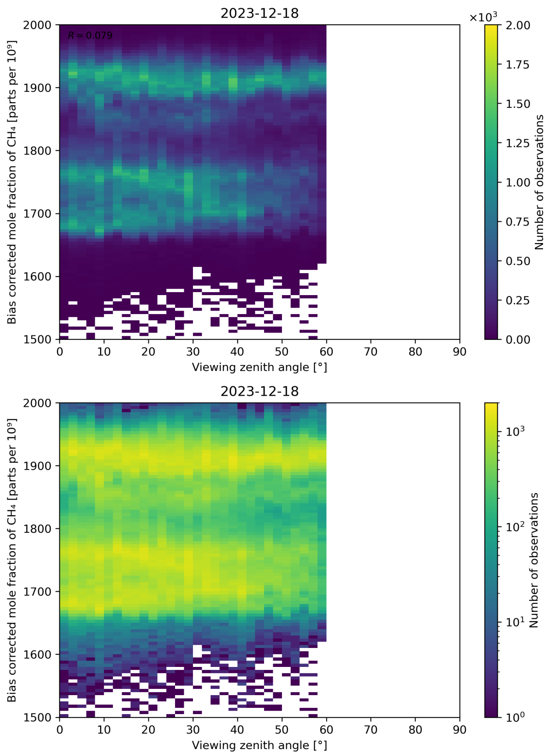
Figure 111: Scatter density plot of “Viewing zenith angle” against “Bias corrected mole fraction of CH 4 ” for 2023-12-17 to 2023-12-19.
