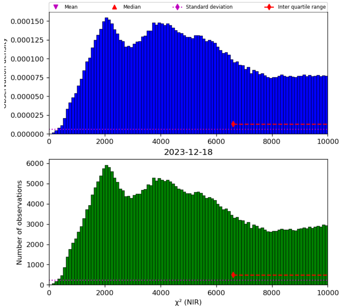
Figure 29: Histogram of “ \chi^2 (NIR)” for 2023-12-17 to 2023-12-19
