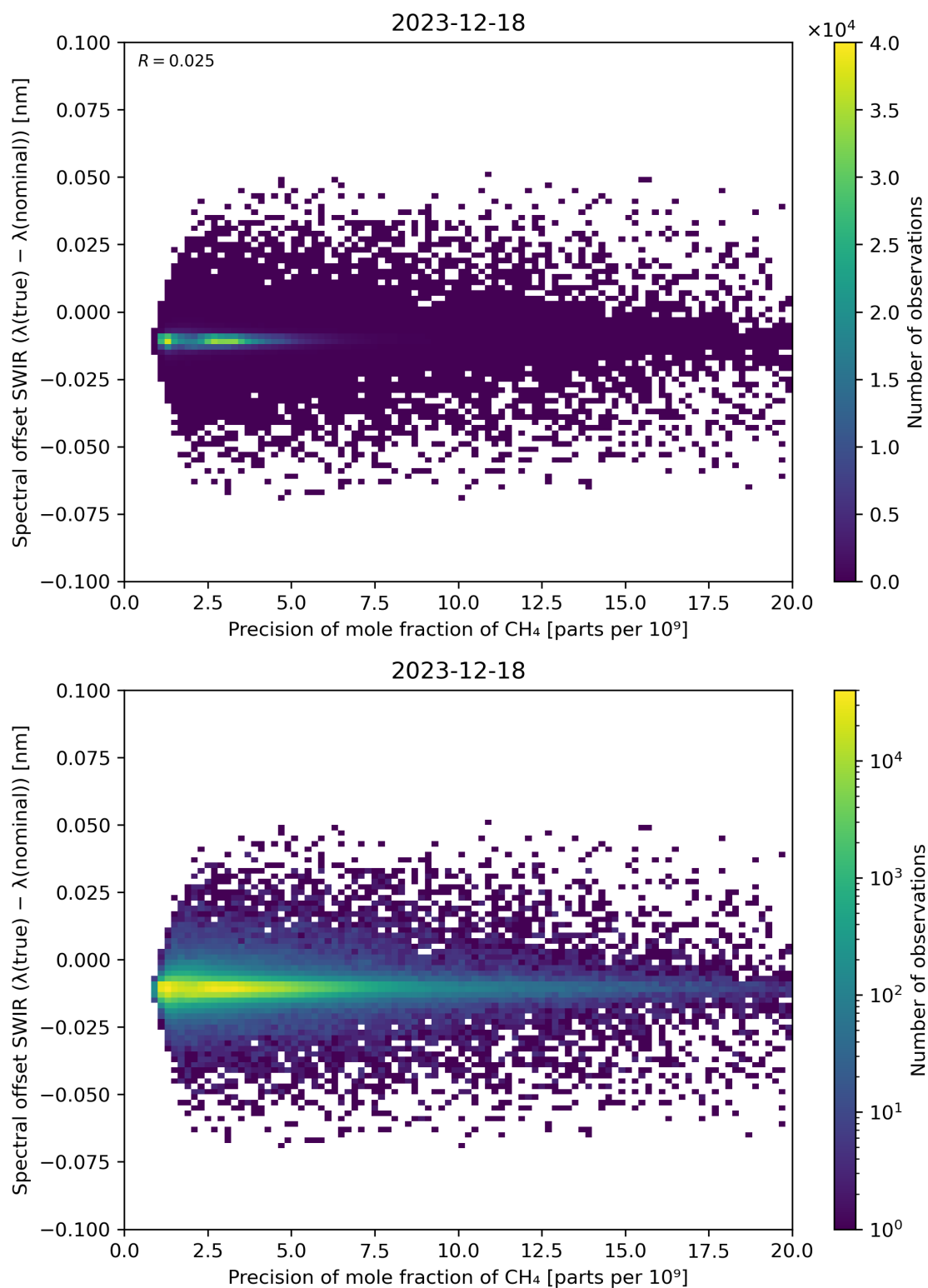
Figure 85: Scatter density plot of “Precision of mole fraction of \text{CH}_4 ” against “Spectral offset SWIR ( \lambda(\text{true}) - \lambda(\text{nominal}) )” for 2023-12-17 to 2023-12-19.
