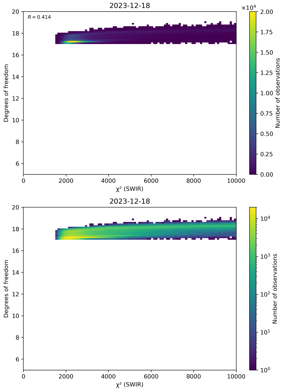
Figure 48: Scatter density plot of “ \chi^2 (SWIR)” against “Degrees of freedom” for 2023-12-17 to 2023-12-19.
