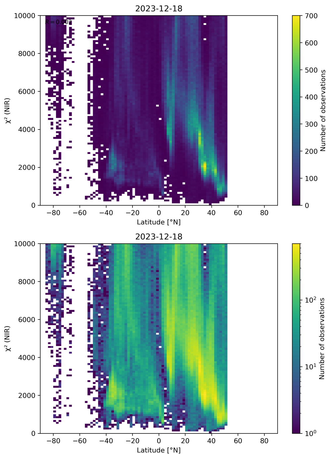
Figure 53: Scatter density plot of “Latitude” against “ \chi^2 (NIR)” for 2023-12-17 to 2023-12-19.
