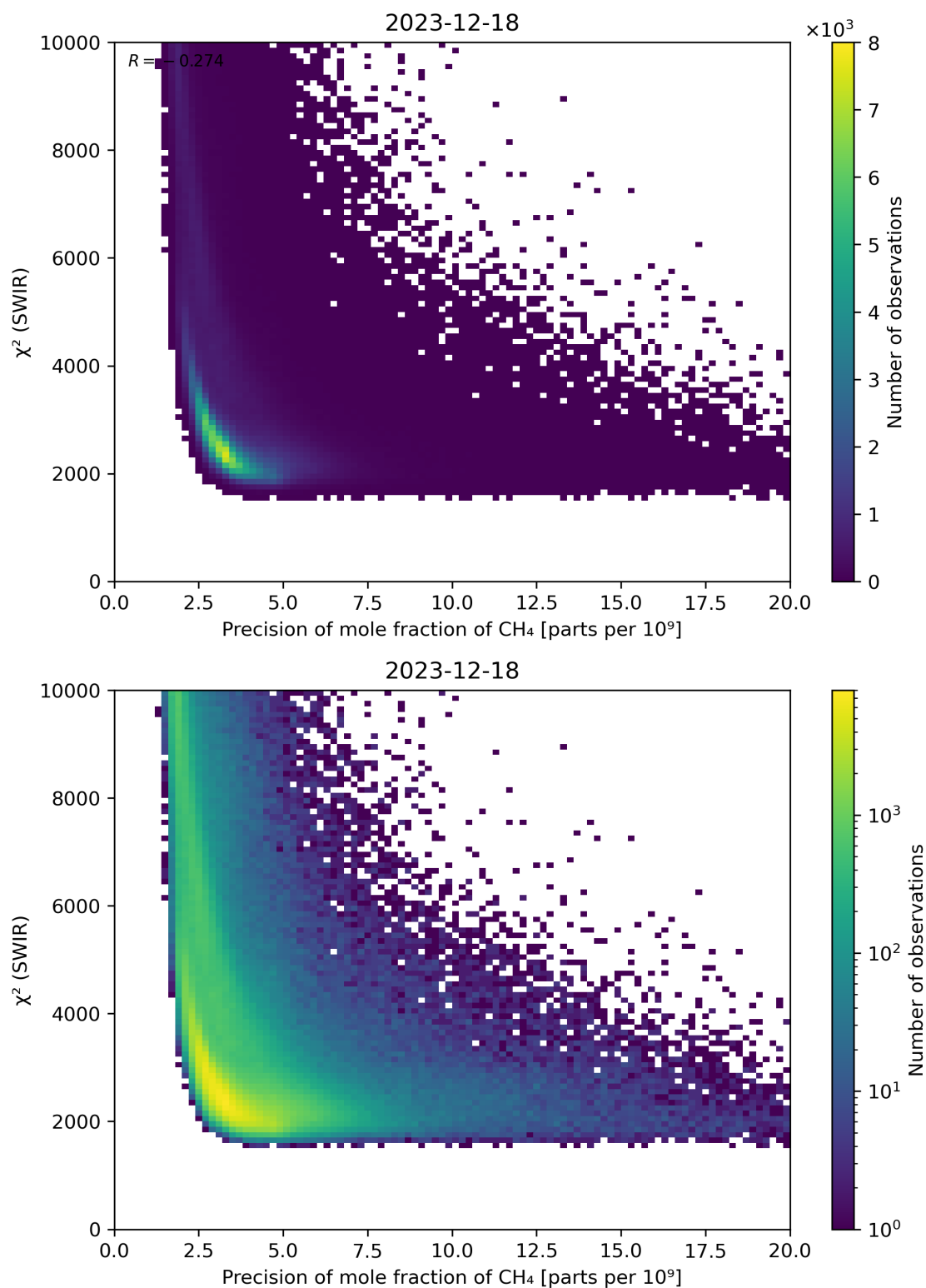
Figure 79: Scatter density plot of “Precision of mole fraction of \text{CH}_4 ” against “ \chi^2 (SWIR)” for 2023-12-17 to 2023-12-19.
