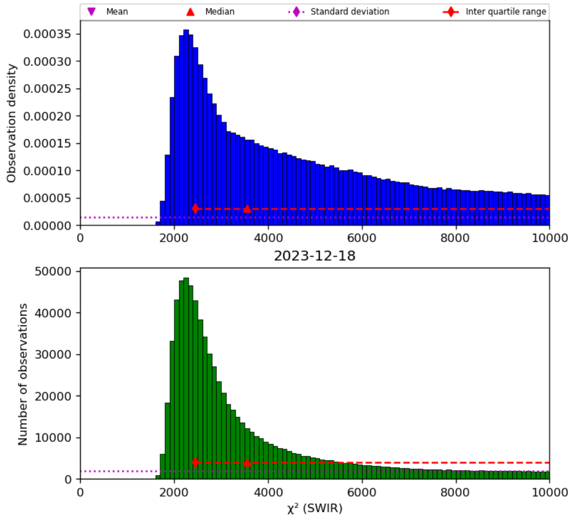
Figure 28: Histogram of “ \chi^2 (SWIR)” for 2023-12-17 to 2023-12-19
