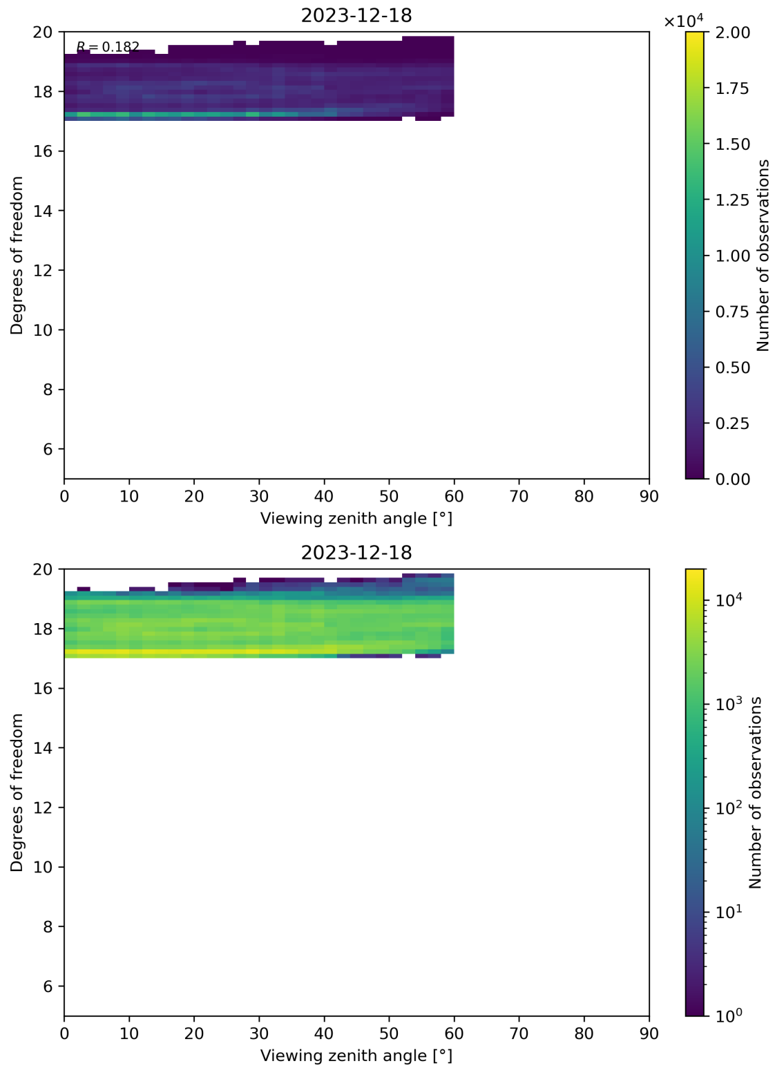
Figure 107: Scatter density plot of “Viewing zenith angle” against “Degrees of freedom” for 2023-12-17 to 2023-12-19.
