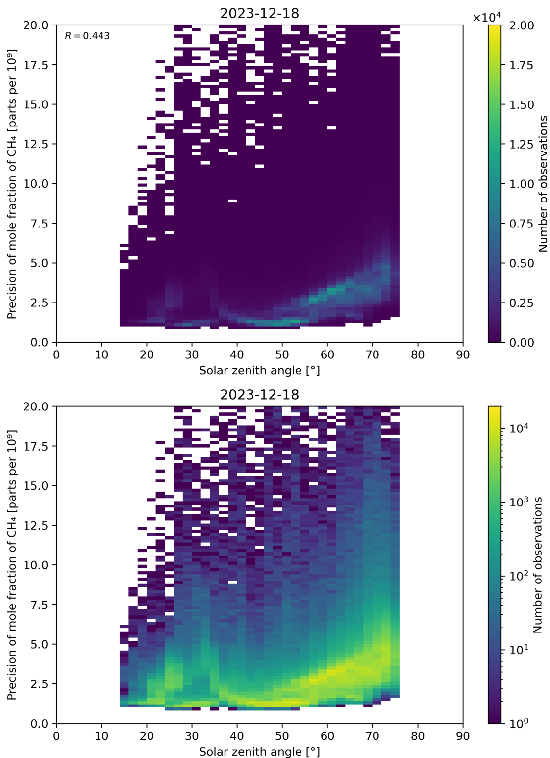
Figure 101: Scatter density plot of “Solar zenith angle” against “Precision of mole fraction of CH 4 ” for 2023-12-17 to 2023-12-19.
