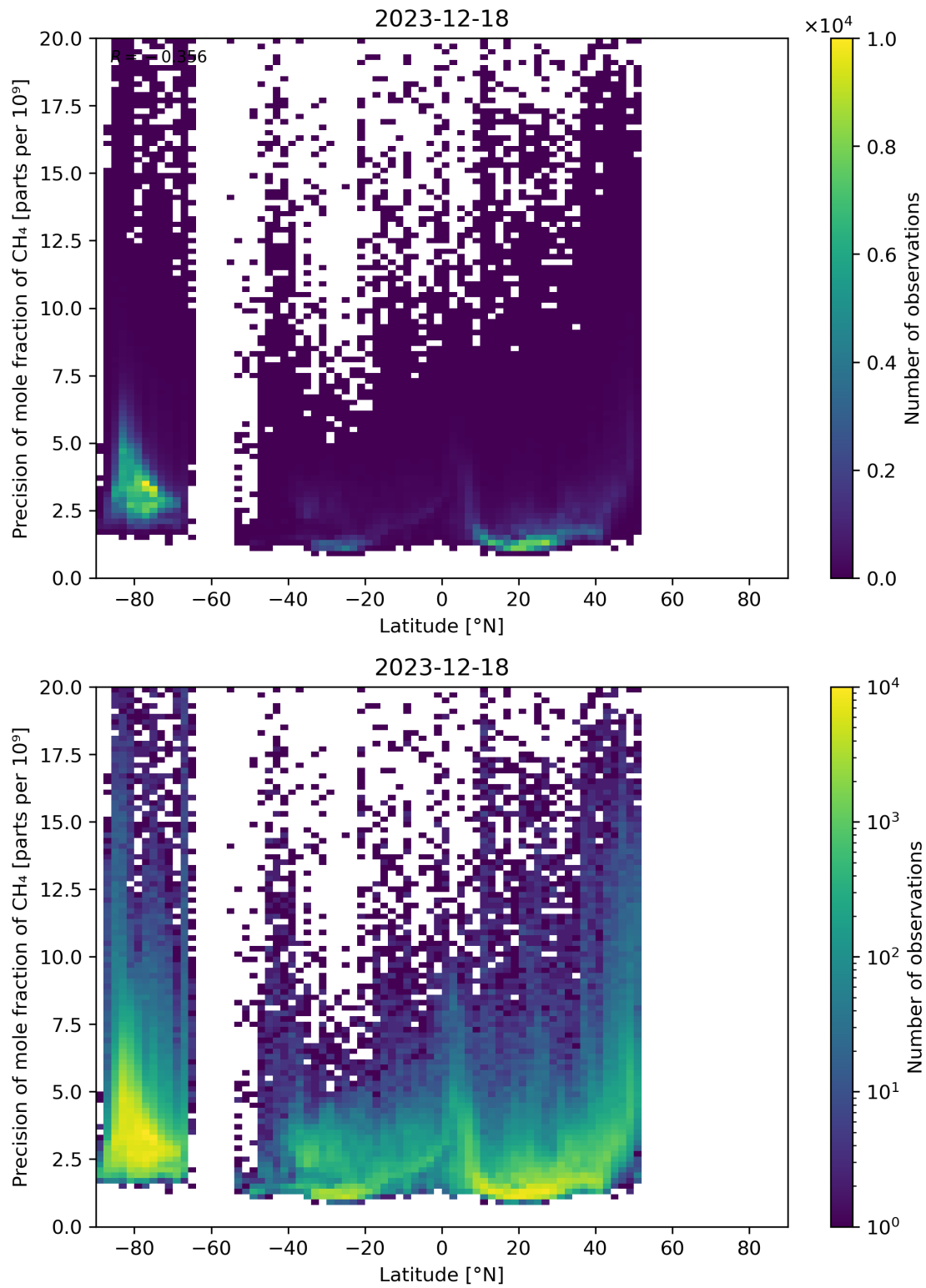
Figure 59: Scatter density plot of “Latitude” against “Precision of mole fraction of CH 4 ” for 2023-12-17 to 2023-12-19.
