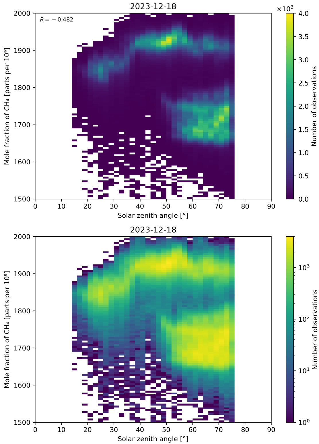
Figure 99: Scatter density plot of “Solar zenith angle” against “Mole fraction of CH 4 ” for 2023-12-17 to 2023-12-19.
