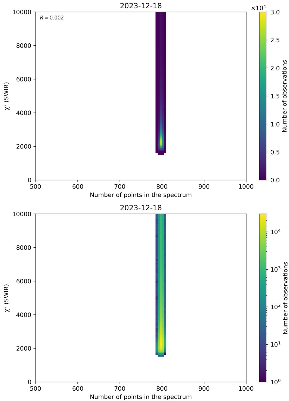
Figure 89: Scatter density plot of “Number of points in the spectrum” against “ \chi^2 (SWIR)” for 2023-12-17 to 2023-12-19.
