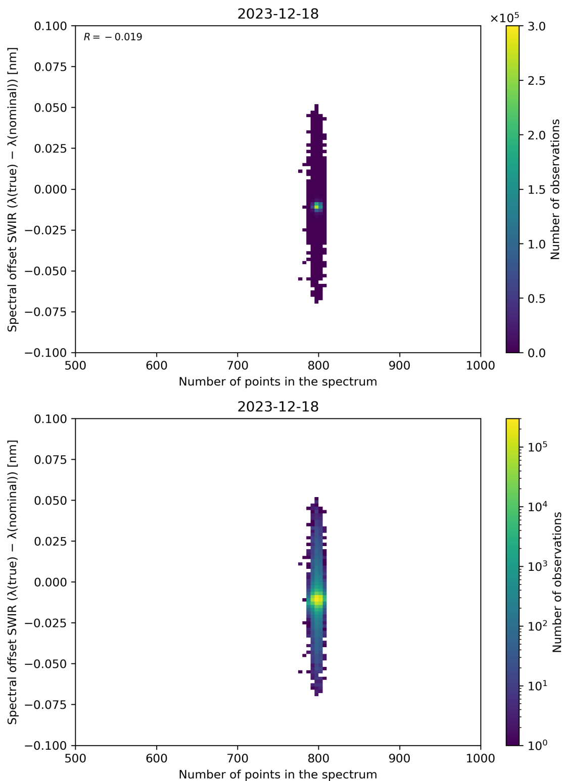
Figure 93: Scatter density plot of “Number of points in the spectrum” against “Spectral offset SWIR ( \lambda(\text{true}) - \lambda(\text{nominal}) )” for 2023-12-17 to 2023-12-19.
