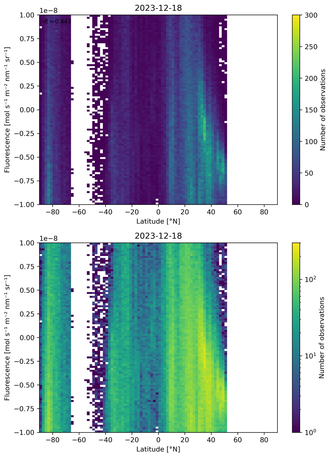
Figure 56: Scatter density plot of “Latitude” against “Fluorescence” for 2023-12-17 to 2023-12-19.
