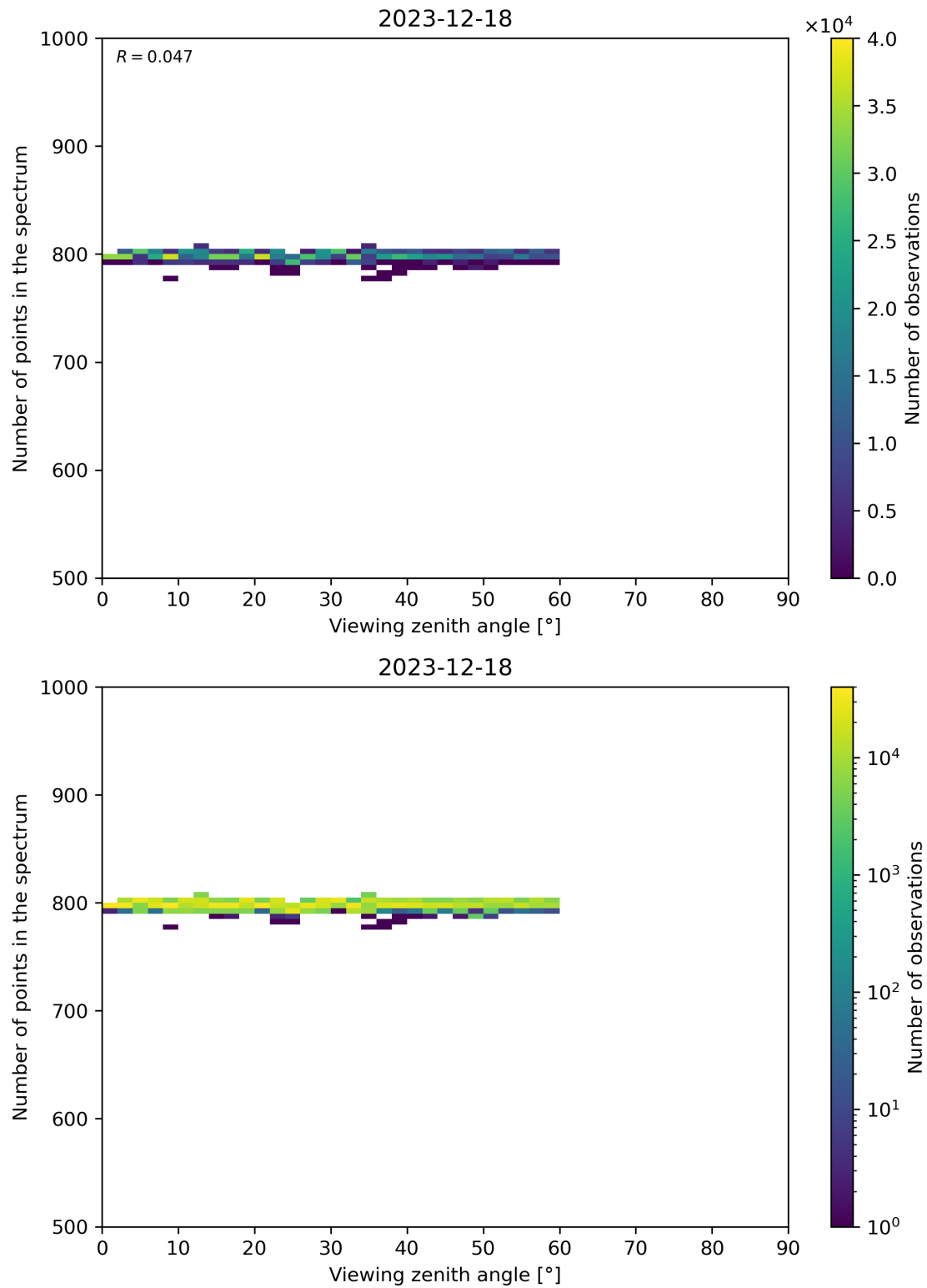
Figure 114: Scatter density plot of “Viewing zenith angle” against “Number of points in the spectrum” for 2023-12-17 to 2023-12-19.
