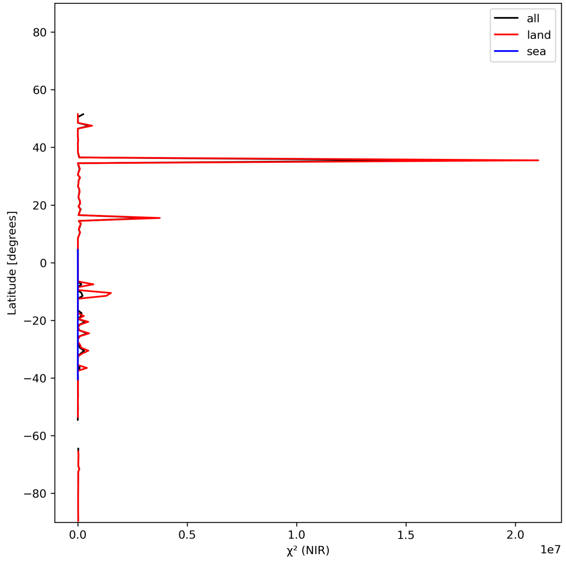
Figure 18: Zonal average of “ \chi^2 (NIR)” for 2023-12-17 to 2023-12-19.
