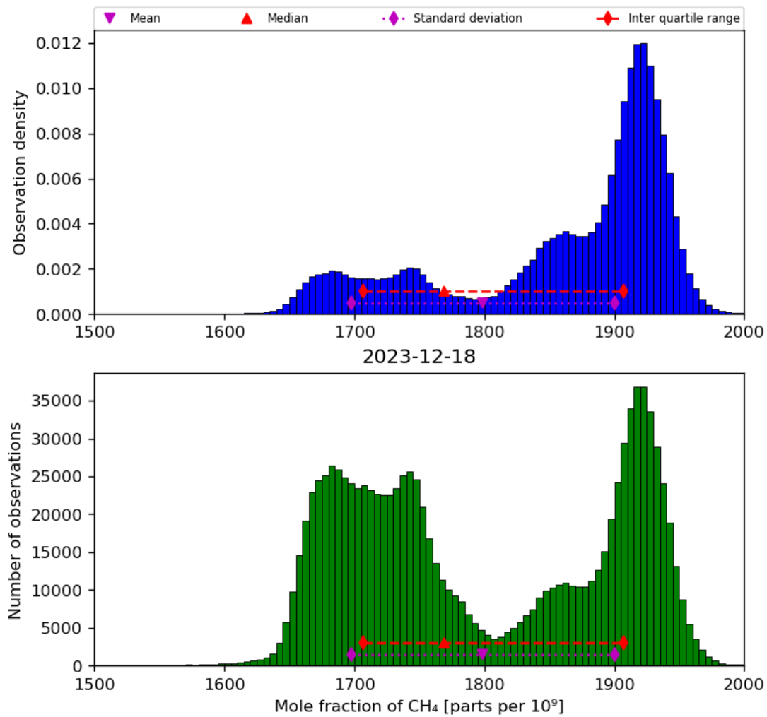
Figure 23: Histogram of “Mole fraction of CH 4 ” for 2023-12-17 to 2023-12-19
