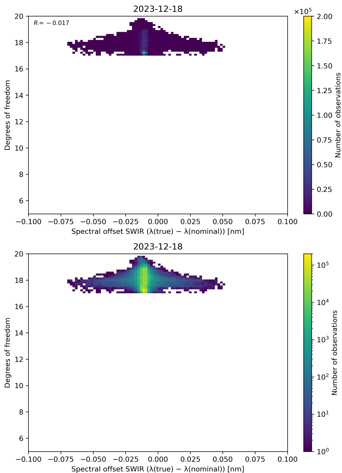
Figure 119: Scatter density plot of “Spectral offset SWIR ( \lambda(\text{true}) - \lambda(\text{nominal}) )” against “Degrees of freedom” for 2023-12-17 to 2023-12-19.
