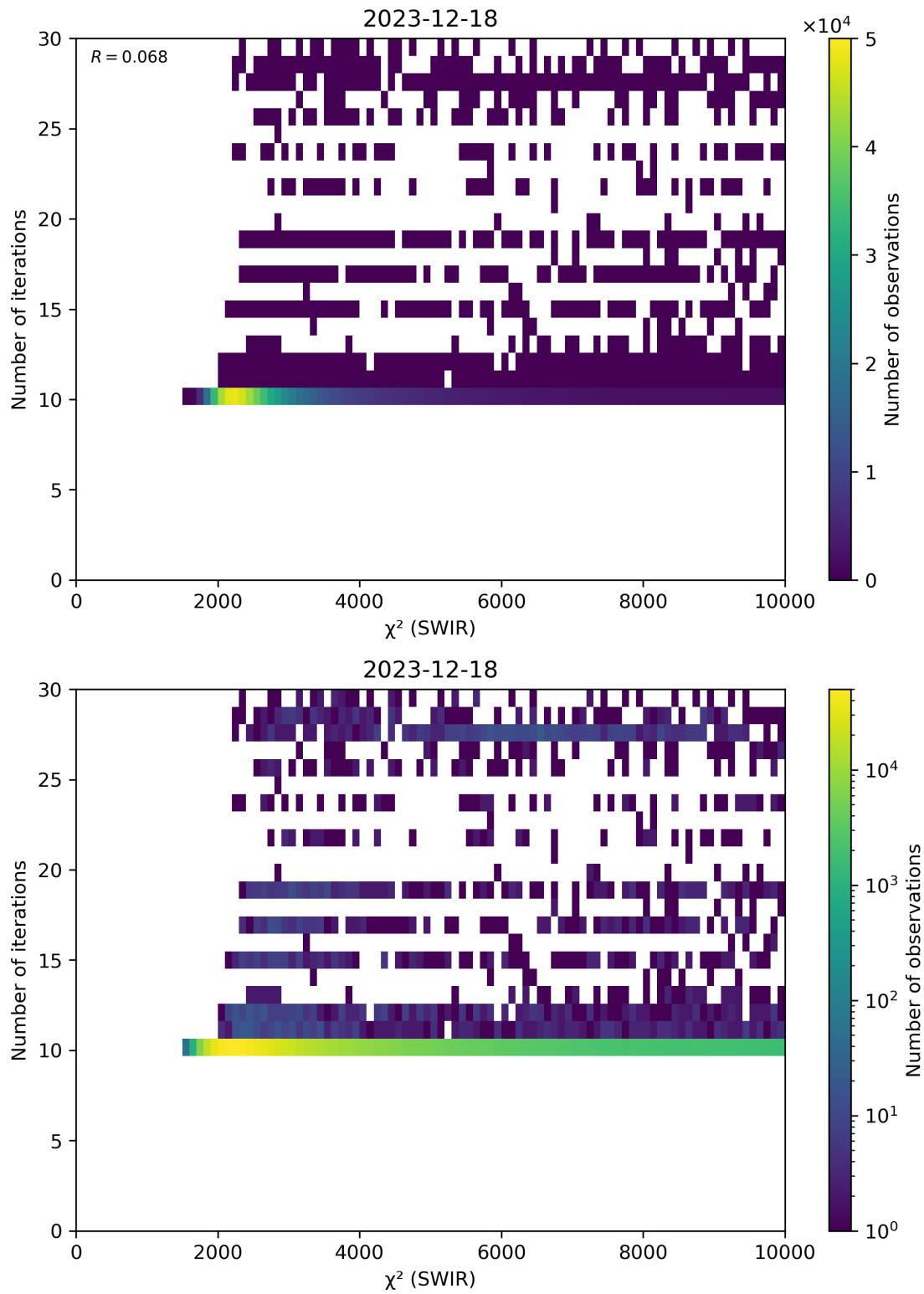
Figure 50: Scatter density plot of “ \chi^2 (SWIR)” against “Number of iterations” for 2023-12-17 to 2023-12-19.
