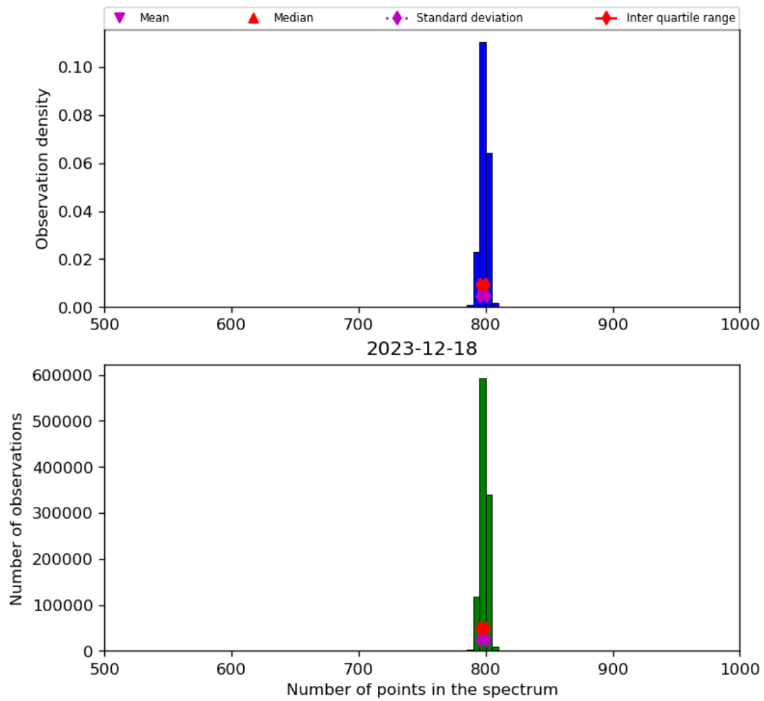
Figure 26: Histogram of “Number of points in the spectrum” for 2023-12-17 to 2023-12-19
