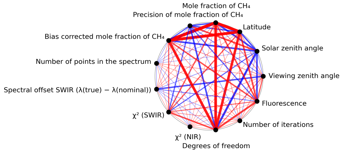
Figure 1: Map of correlation graph for 2023-12-17 to 2023-12-19.
