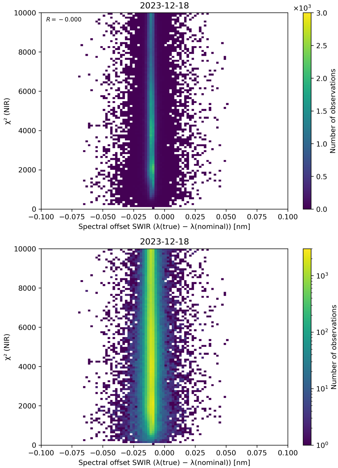
Figure 117: Scatter density plot of “Spectral offset SWIR ( \lambda(\text{true}) - \lambda(\text{nominal}) )” against “ \chi^2 (NIR)” for 2023-12-17 to 2023-12-19.
