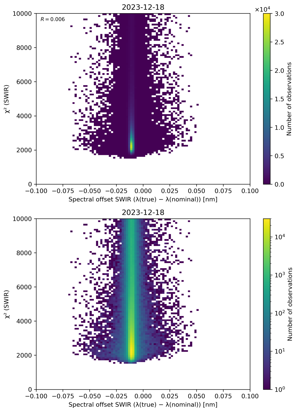
Figure 118: Scatter density plot of “Spectral offset SWIR ( \lambda(\text{true}) - \lambda(\text{nominal}) )” against “ \chi^2 (SWIR)” for 2023-12-17 to 2023-12-19.
