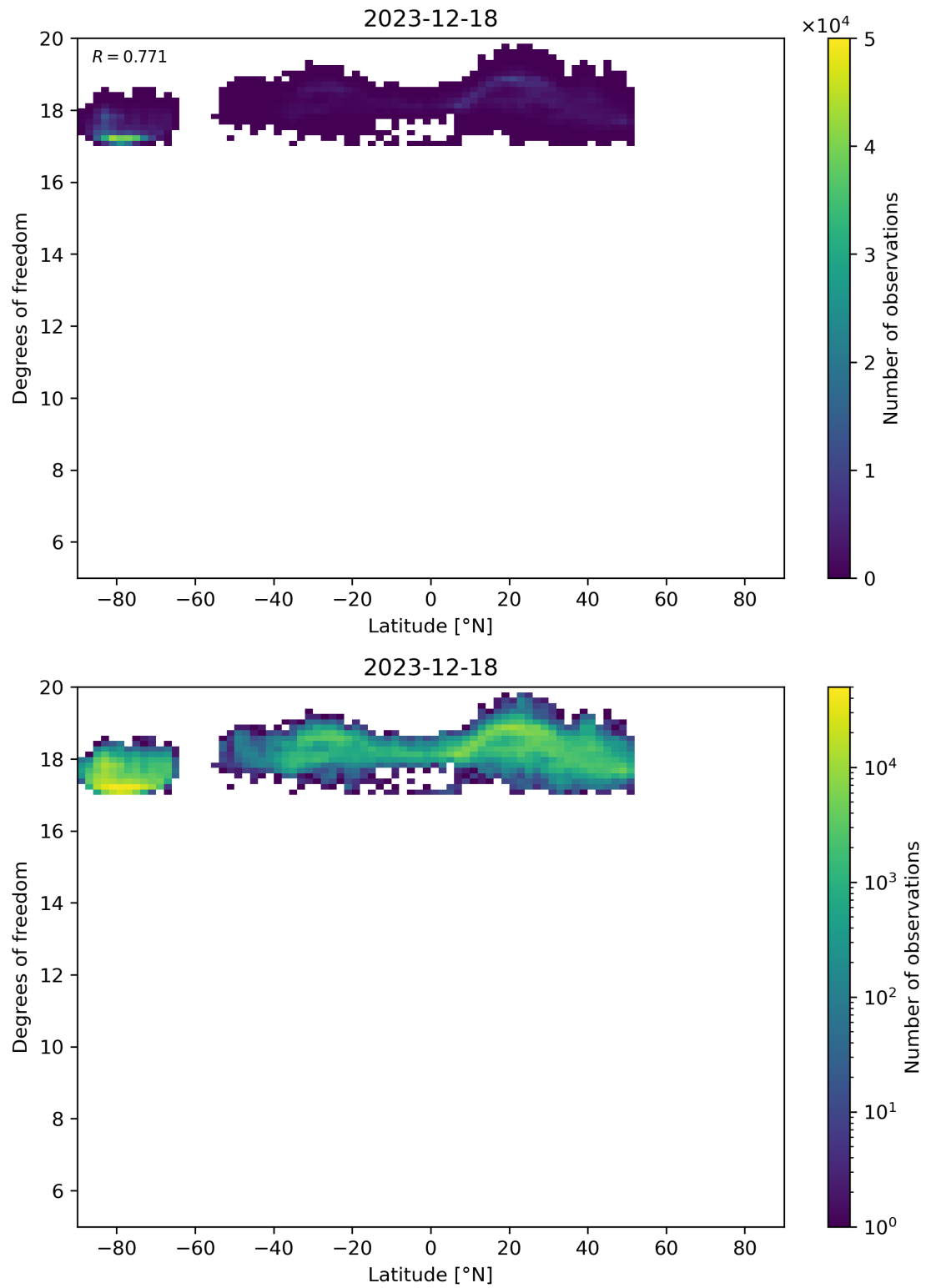
Figure 55: Scatter density plot of “Latitude” against “Degrees of freedom” for 2023-12-17 to 2023-12-19.
