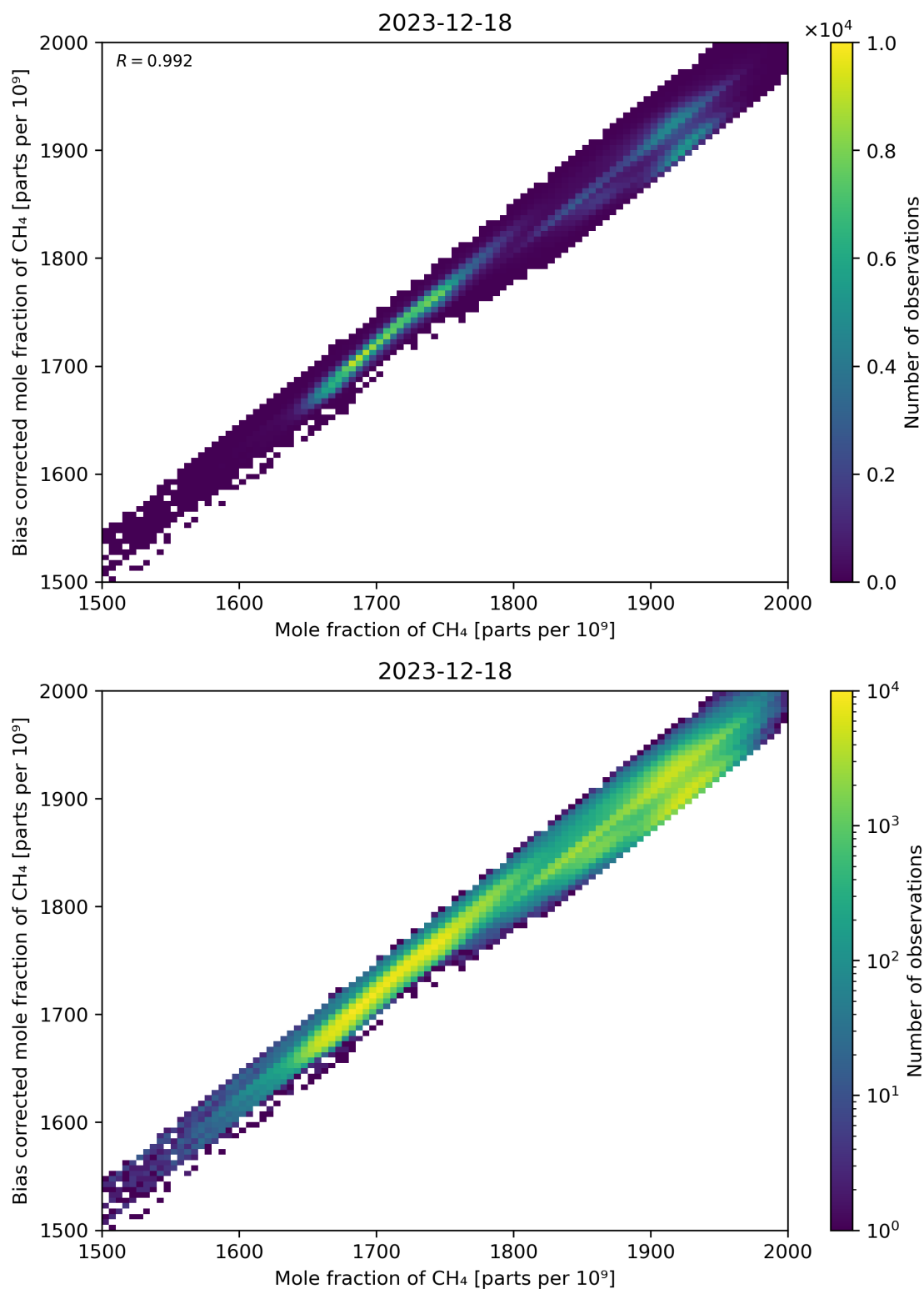
Figure 74: Scatter density plot of “Mole fraction of CH 4 ” against “Bias corrected mole fraction of CH 4 ” for 2023-12-17 to 2023-12-19.
