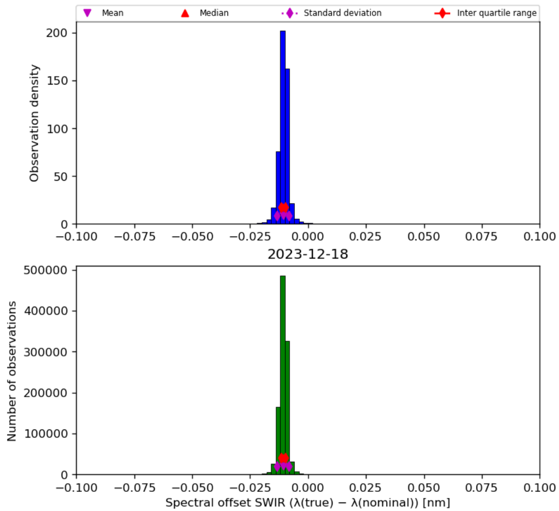
Figure 27: Histogram of “Spectral offset SWIR ( \lambda(\text{true}) - \lambda(\text{nominal}) )” for 2023-12-17 to 2023-12-19
