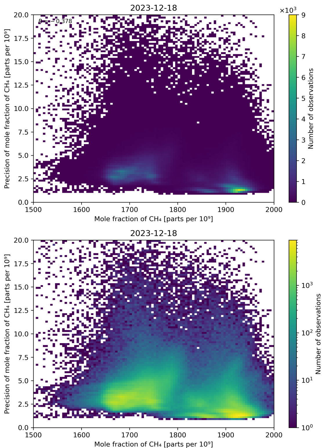
Figure 75: Scatter density plot of “Mole fraction of CH 4 ” against “Precision of mole fraction of CH 4 ” for 2023-12-17 to 2023-12-19.
