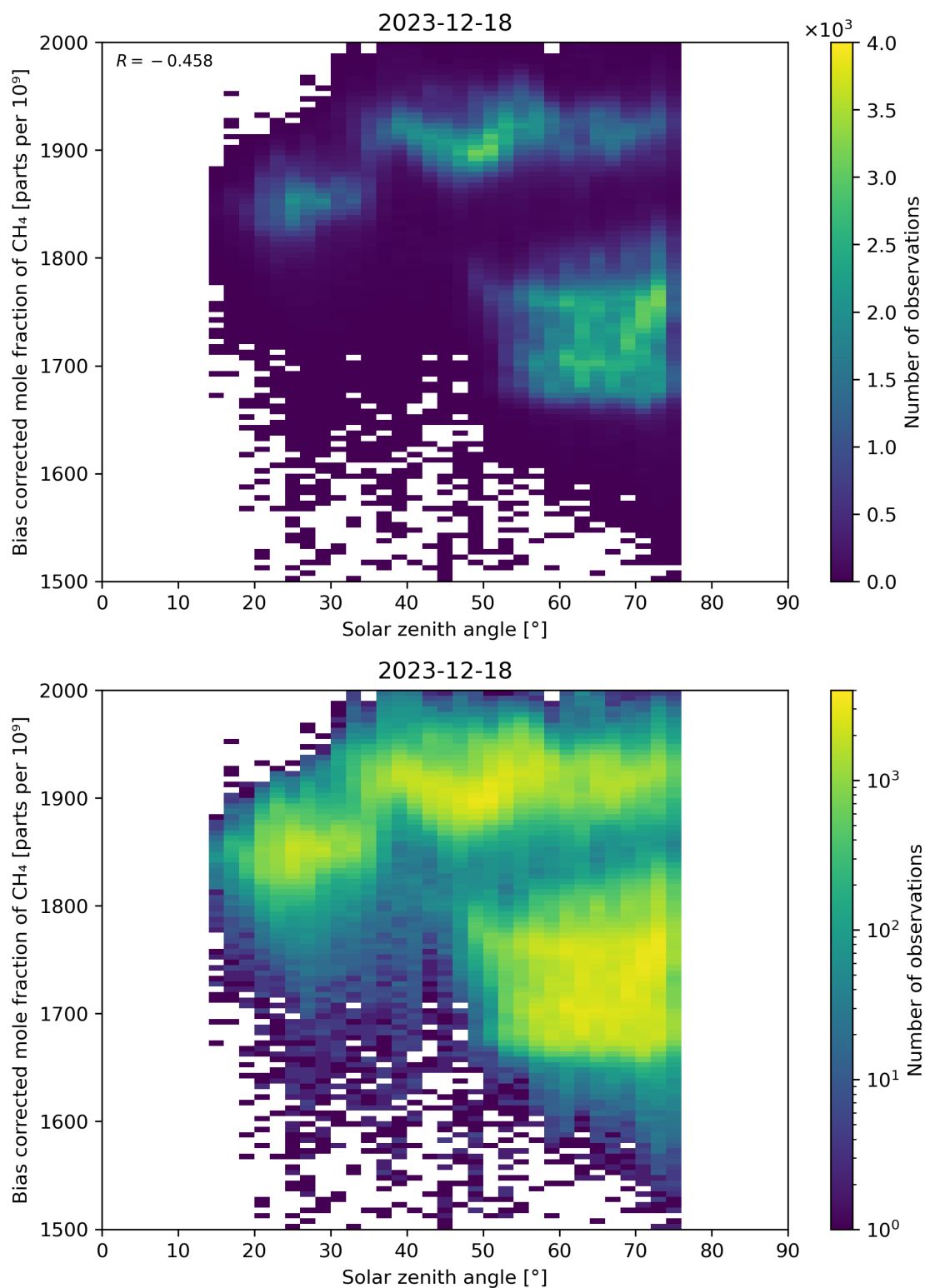
Figure 100: Scatter density plot of “Solar zenith angle” against “Bias corrected mole fraction of \text{CH}_4 ” for 2023-12-17 to 2023-12-19.
