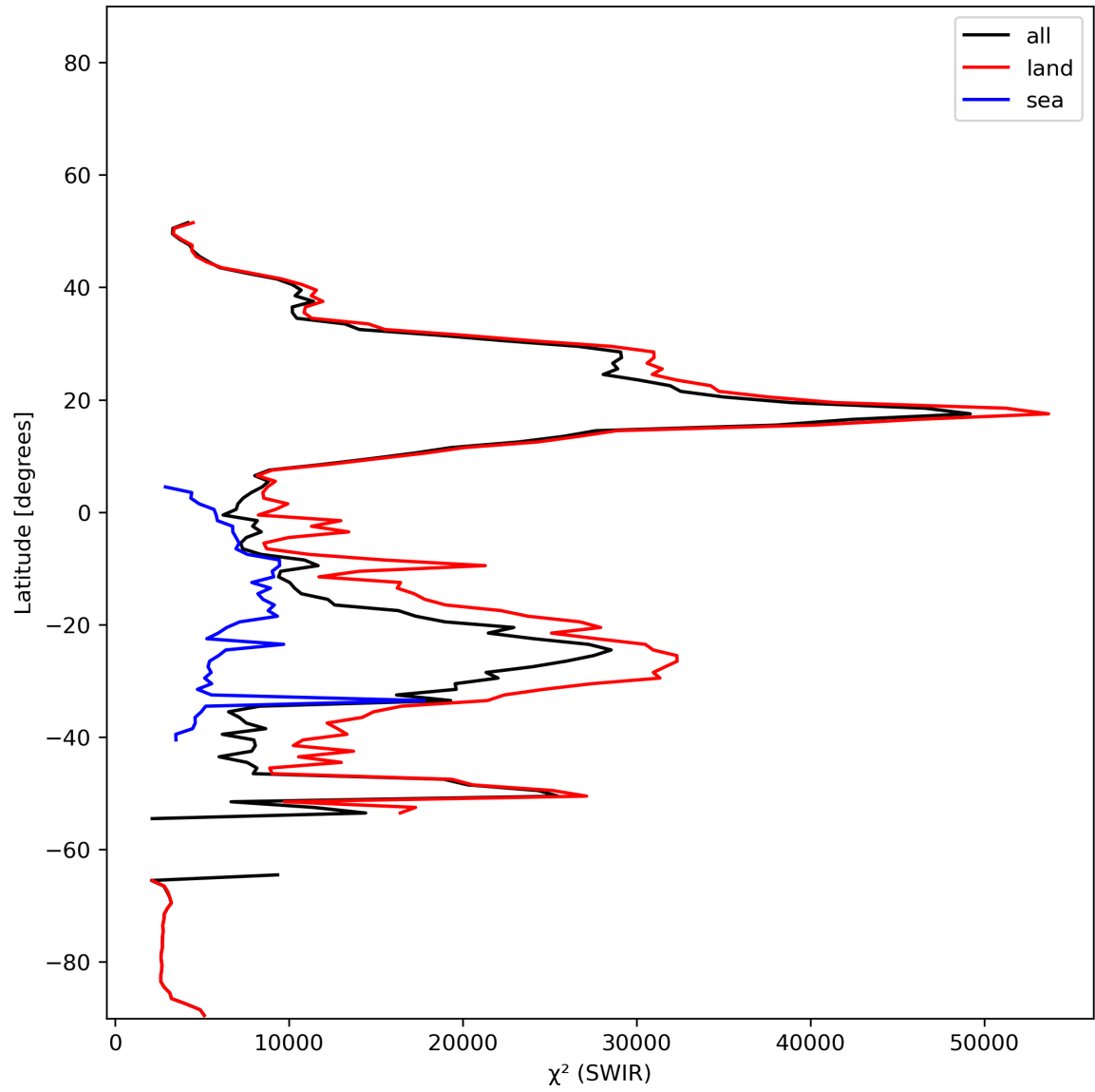
Figure 17: Zonal average of “ \chi^2 (SWIR)” for 2023-12-17 to 2023-12-19.
