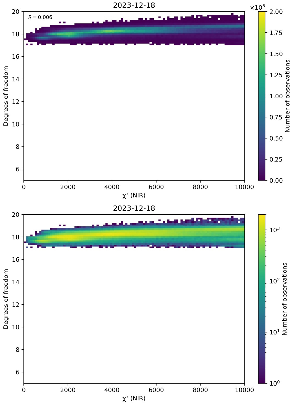
Figure 44: Scatter density plot of “ \chi^2 (NIR)” against “Degrees of freedom” for 2023-12-17 to 2023-12-19.
