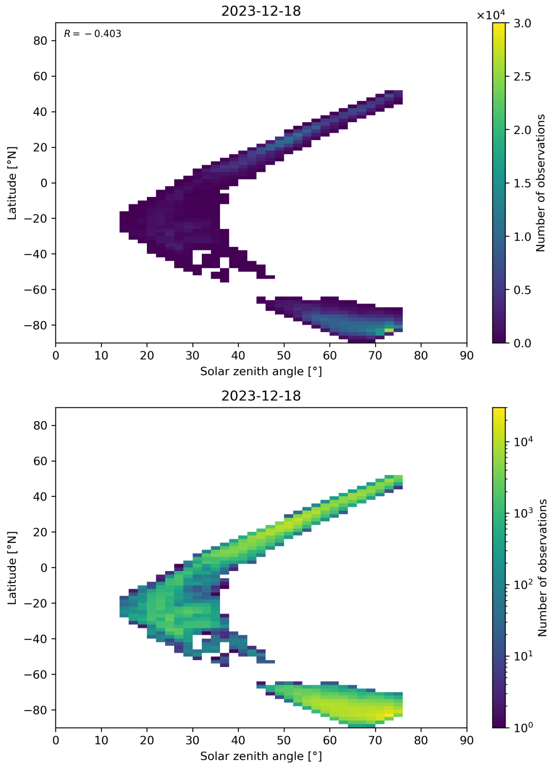
Figure 98: Scatter density plot of “Solar zenith angle” against “Latitude” for 2023-12-17 to 2023-12-19.
