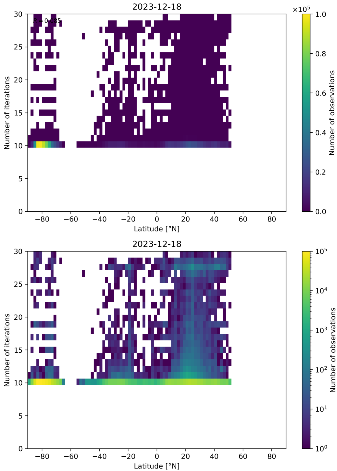
Figure 60: Scatter density plot of “Latitude” against “Number of iterations” for 2023-12-17 to 2023-12-19.
