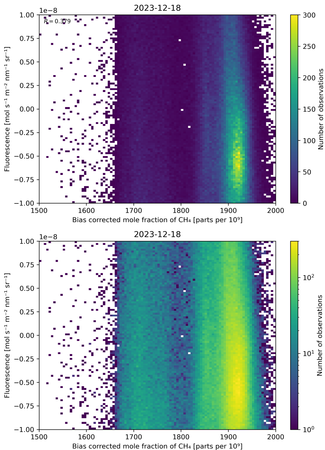
Figure 66: Scatter density plot of “Bias corrected mole fraction of \text{CH}_4 ” against “Fluorescence” for 2023-12-17 to 2023-12-19.
