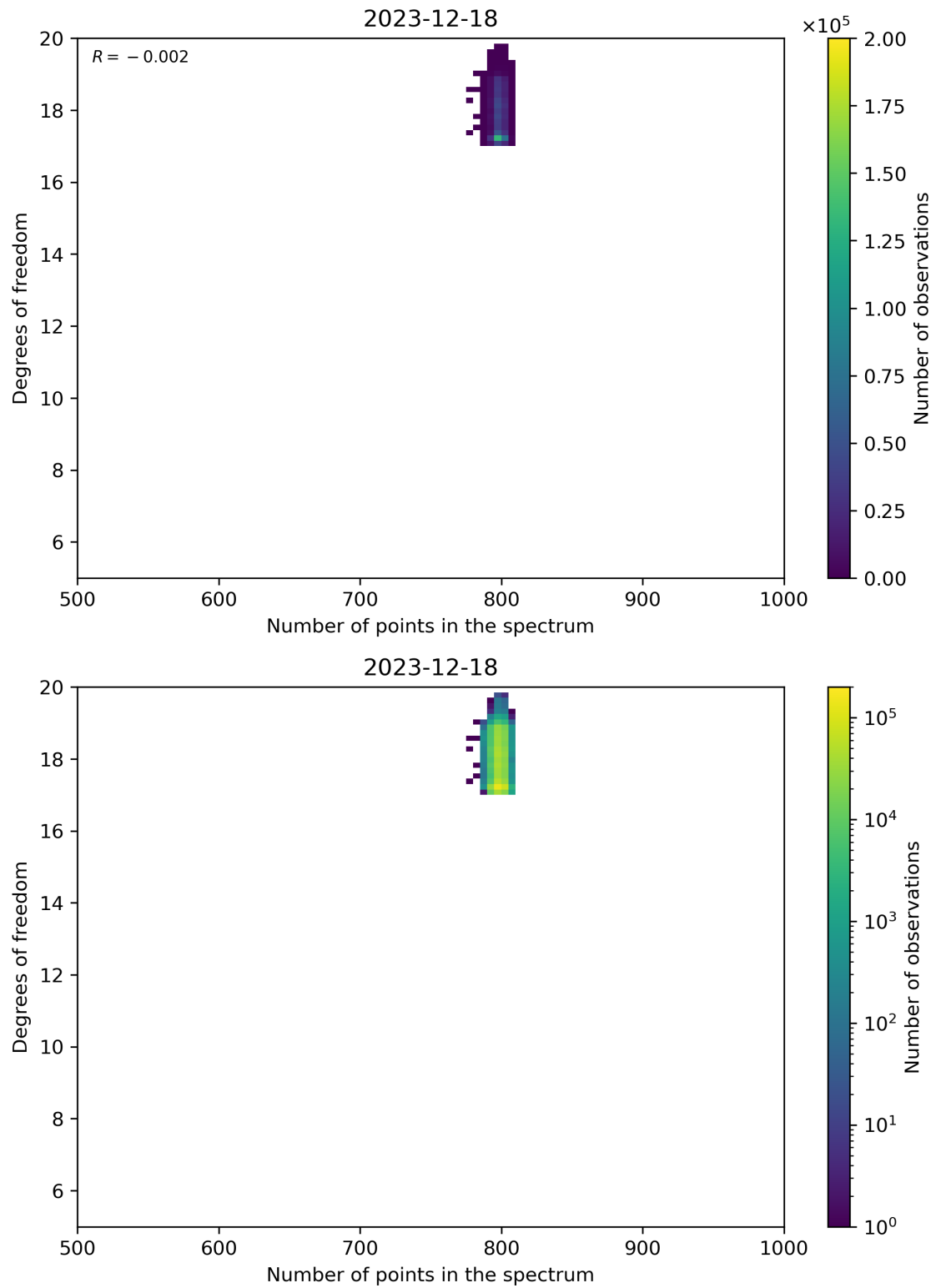
Figure 90: Scatter density plot of “Number of points in the spectrum” against “Degrees of freedom” for 2023-12-17 to 2023-12-19.
