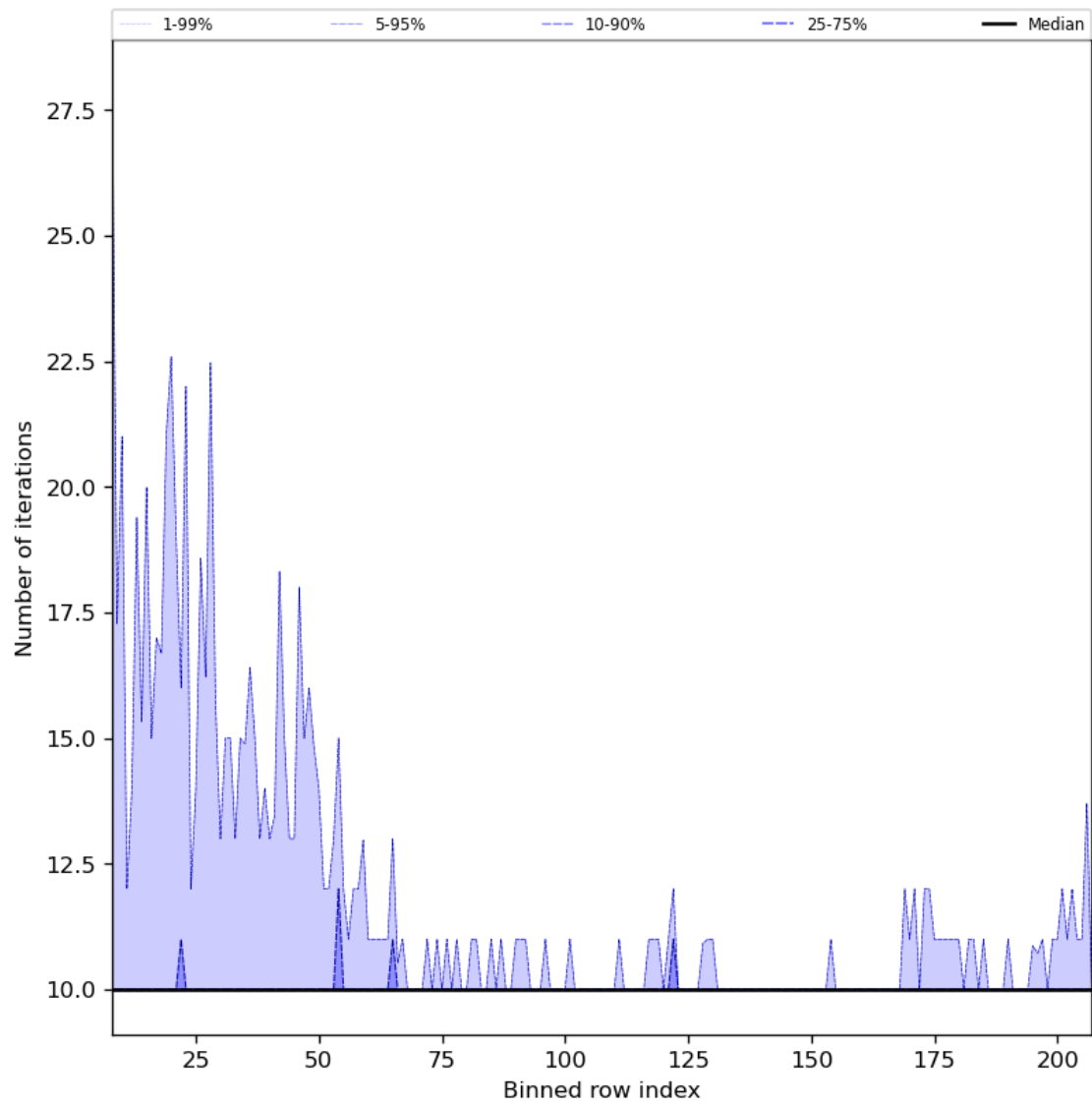
Figure 42: Along track statistics of “Number of iterations” for 2023-12-17 to 2023-12-19
