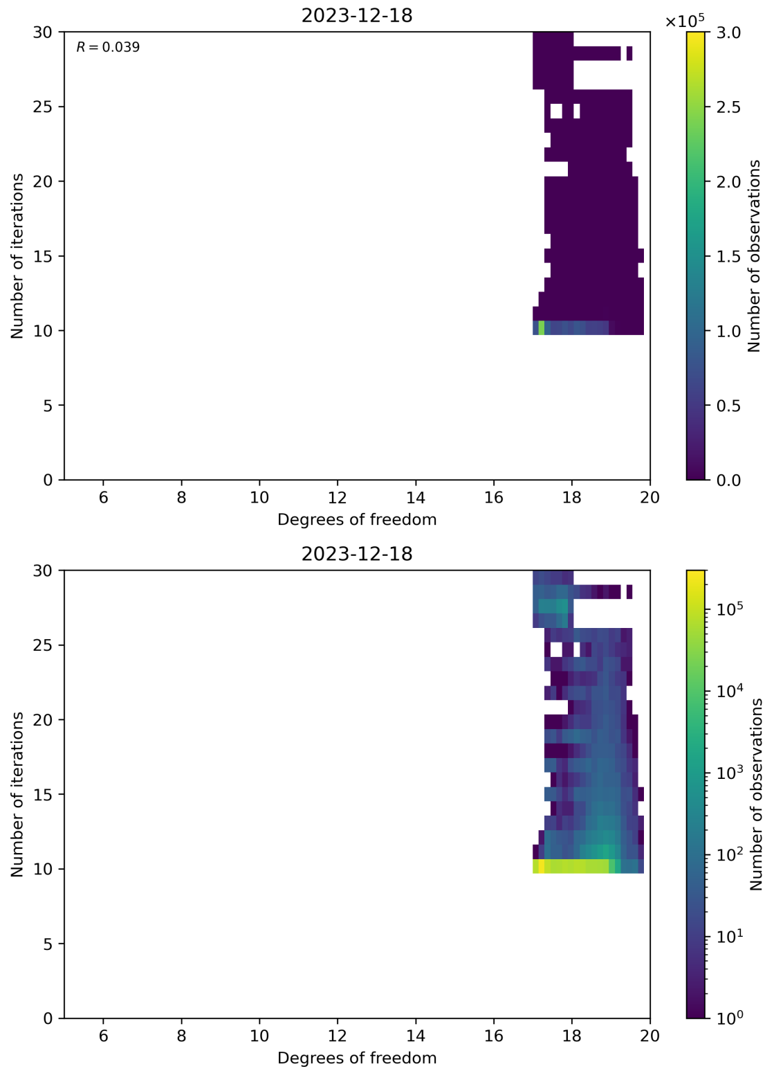
Figure 52: Scatter density plot of “Degrees of freedom” against “Number of iterations” for 2023-12-17 to 2023-12-19.
