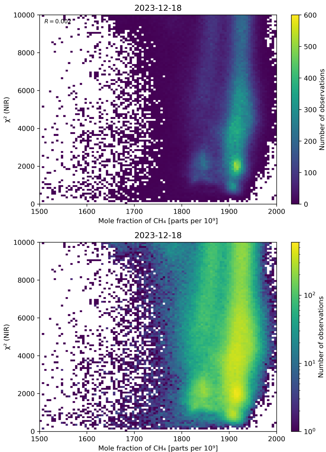
Figure 70: Scatter density plot of “Mole fraction of \text{CH}_4 ” against “ \chi^2 (NIR)” for 2023-12-17 to 2023-12-19.
