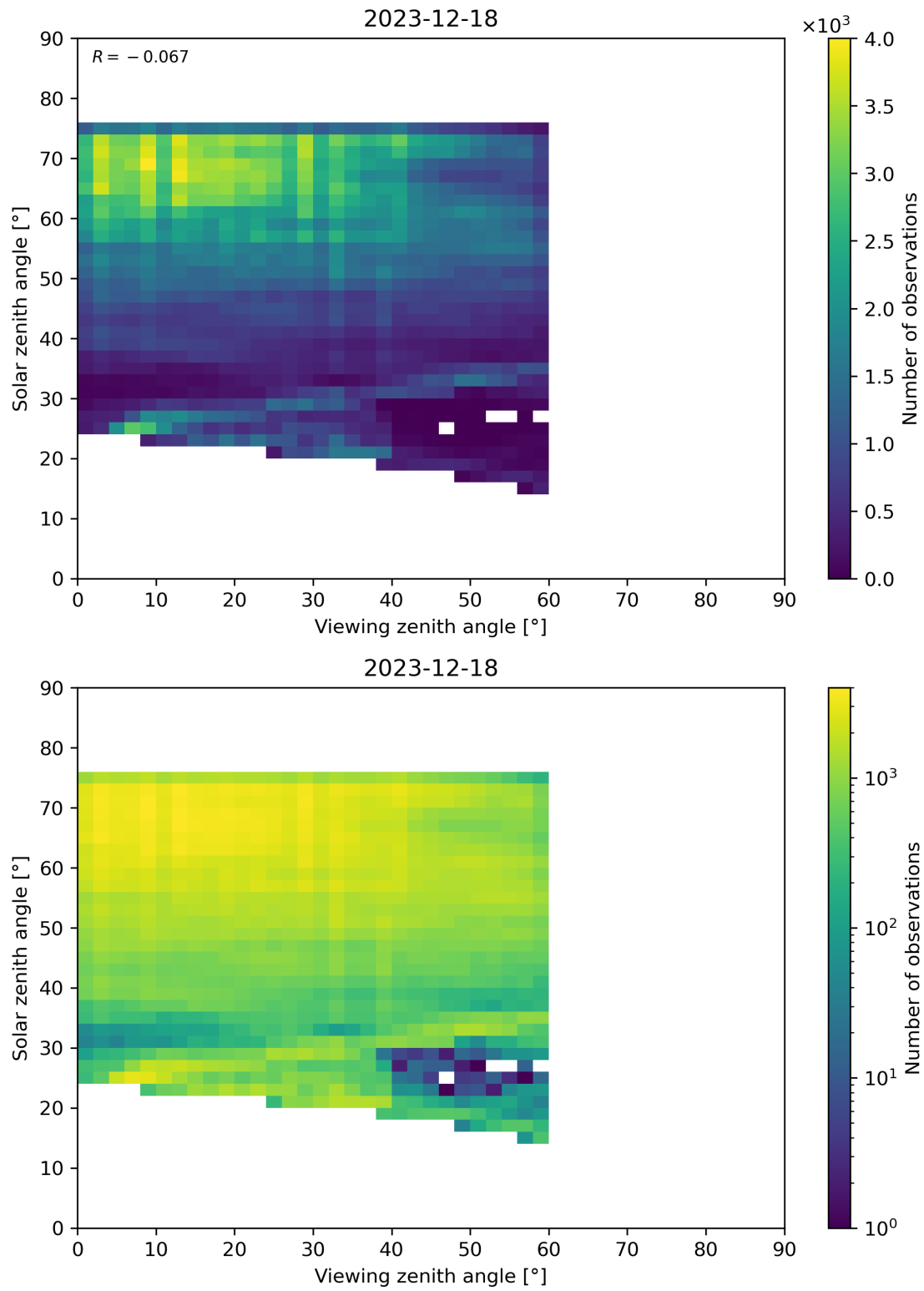
Figure 115: Scatter density plot of “Viewing zenith angle” against “Solar zenith angle” for 2023-12-17 to 2023-12-19.
