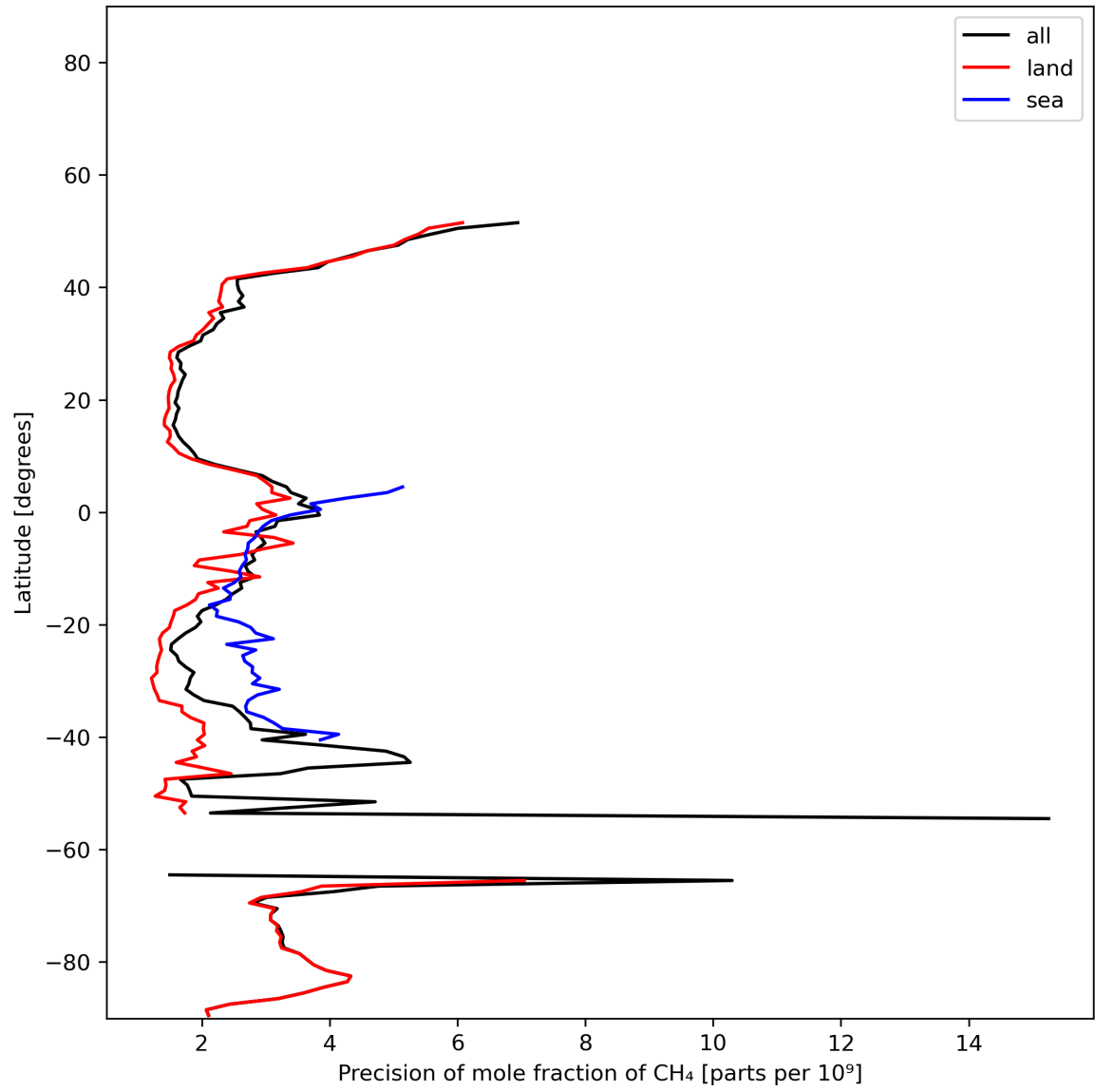
Figure 13: Zonal average of “Precision of mole fraction of CH 4 ” for 2023-12-17 to 2023-12-19.
