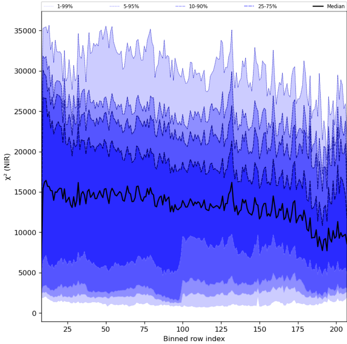
Figure 40: Along track statistics of “ \chi^2 (NIR)” for 2023-12-17 to 2023-12-19
