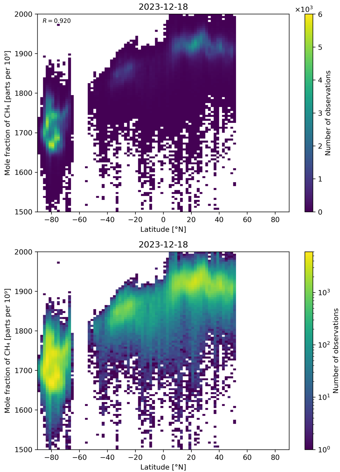
Figure 57: Scatter density plot of “Latitude” against “Mole fraction of CH 4 ” for 2023-12-17 to 2023-12-19.
