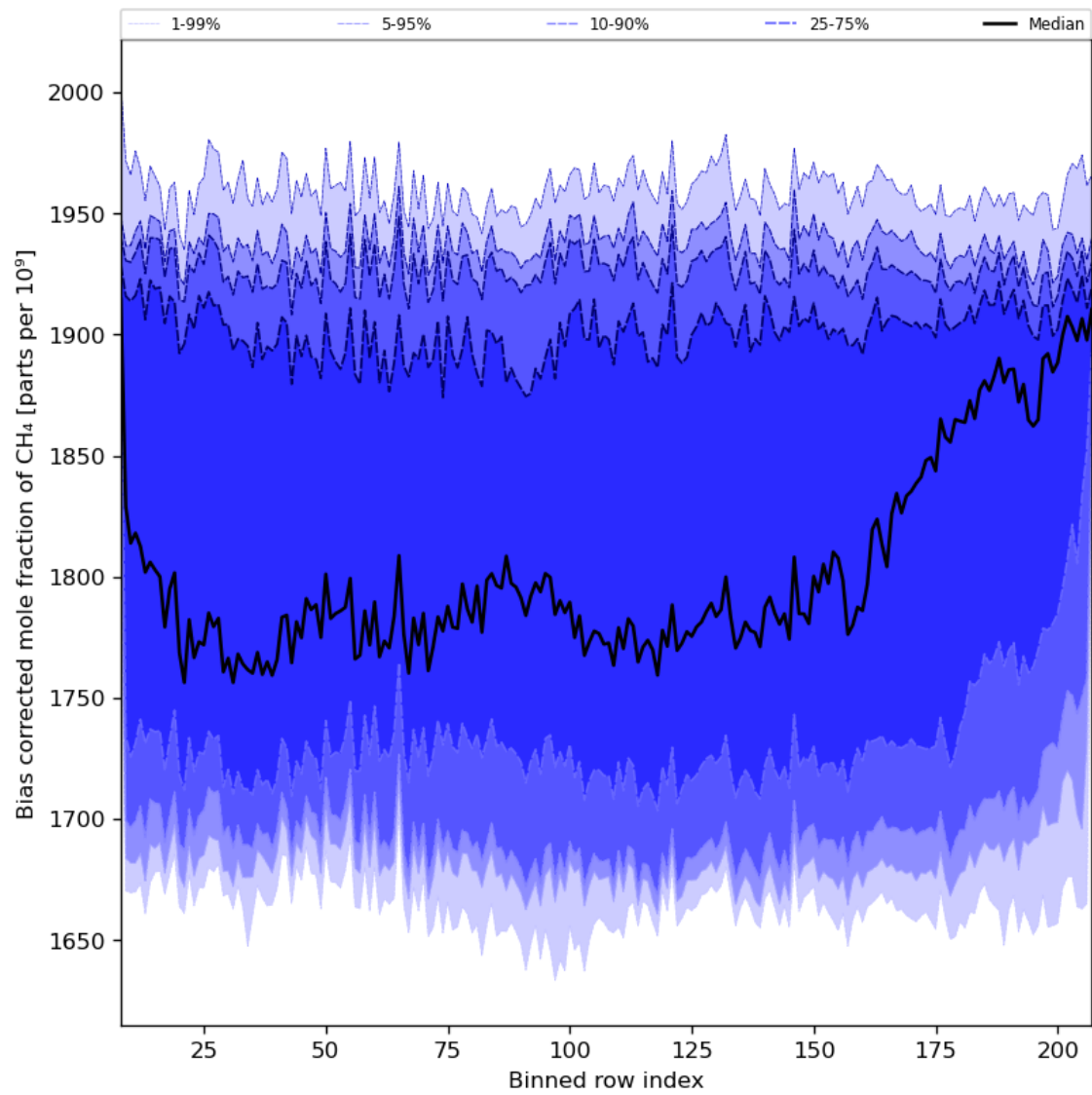
Figure 36: Along track statistics of “Bias corrected mole fraction of CH 4 ” for 2023-12-17 to 2023-12-19
