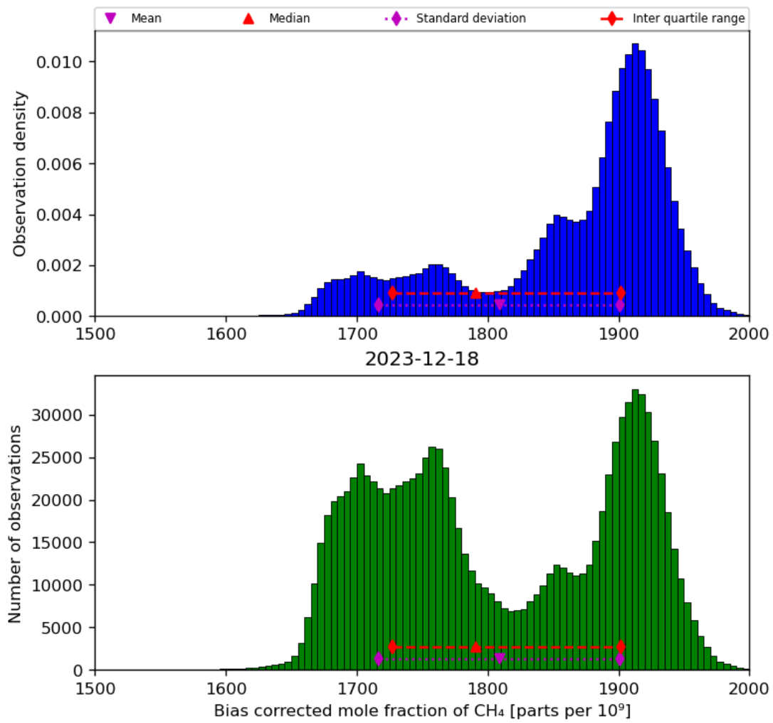
Figure 25: Histogram of “Bias corrected mole fraction of CH 4 ” for 2023-12-17 to 2023-12-19
