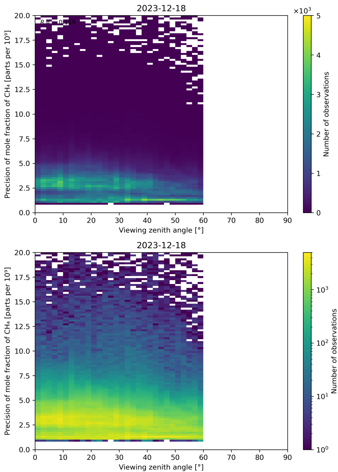
Figure 112: Scatter density plot of “Viewing zenith angle” against “Precision of mole fraction of CH 4 ” for 2023-12-17 to 2023-12-19.
