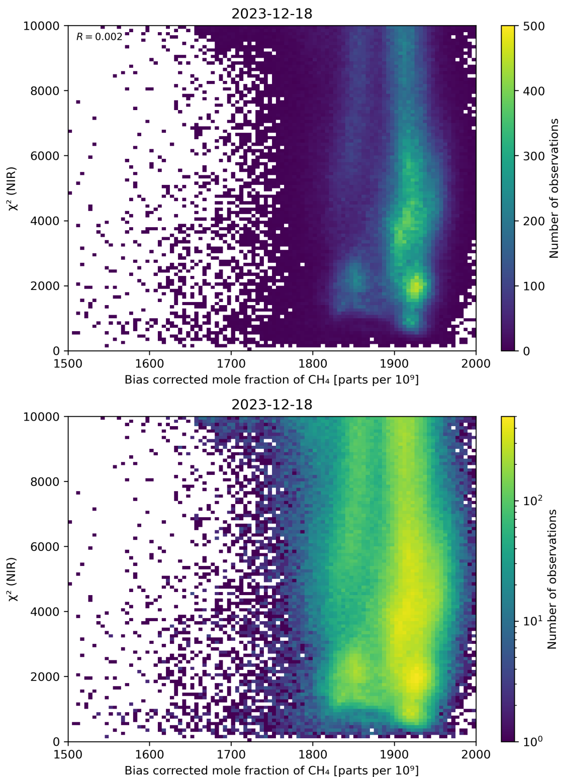
Figure 63: Scatter density plot of “Bias corrected mole fraction of CH 4 ” against “ \chi^2 (NIR)” for 2023-12-17 to 2023-12-19.
