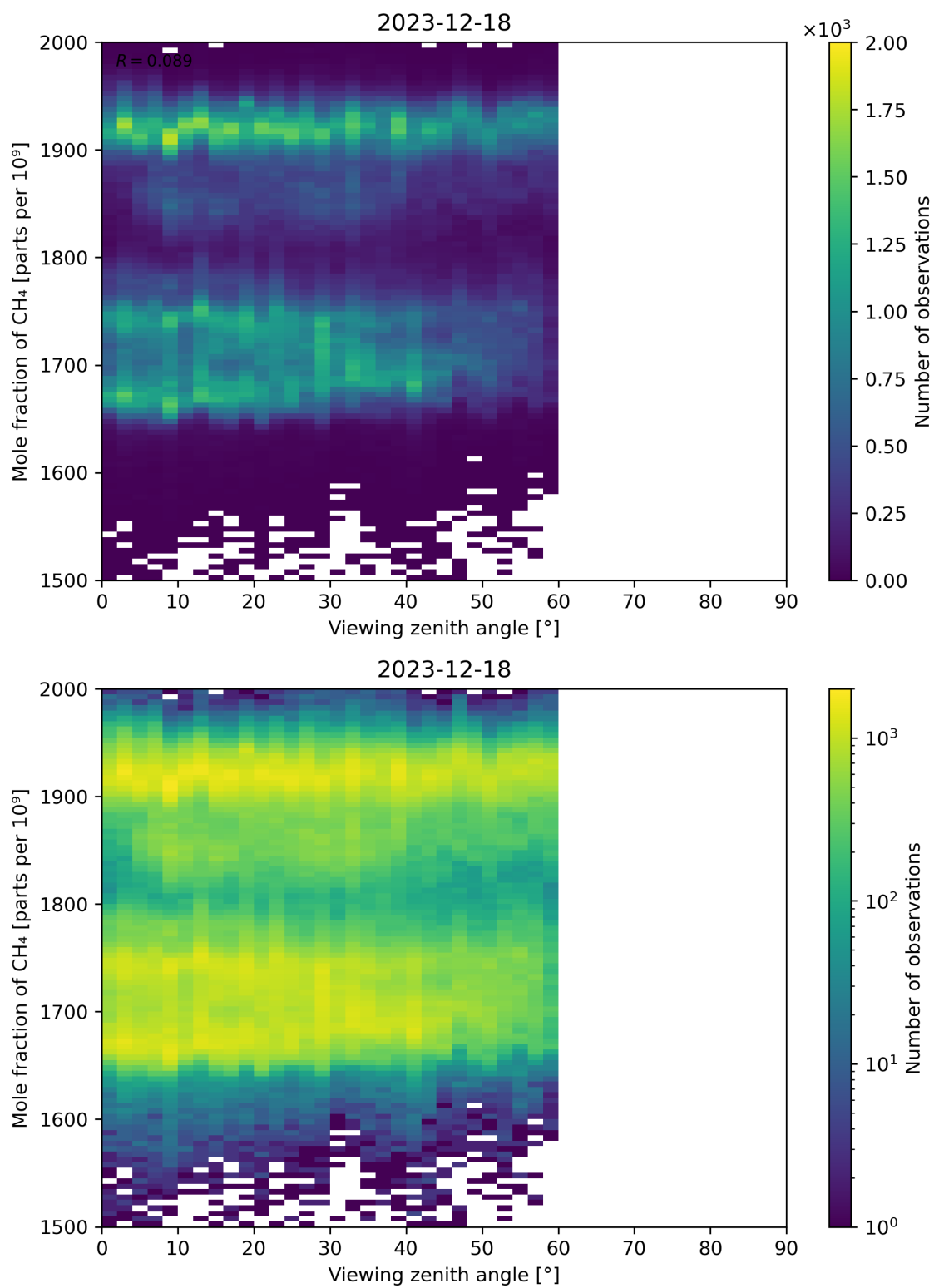
Figure 110: Scatter density plot of “Viewing zenith angle” against “Mole fraction of CH 4 ” for 2023-12-17 to 2023-12-19.
