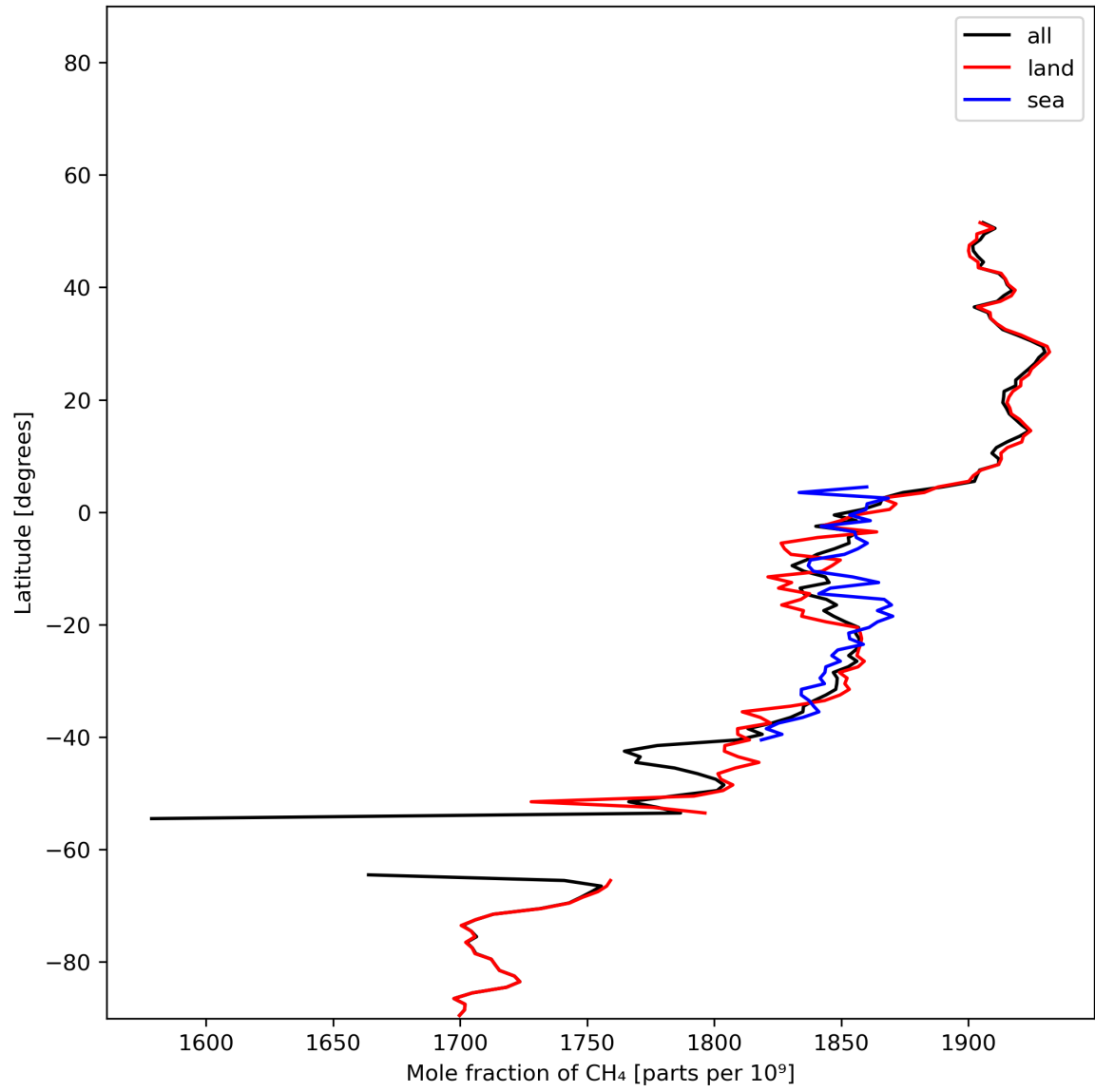
Figure 12: Zonal average of “Mole fraction of \text{CH}_4 ” for 2023-12-17 to 2023-12-19.
