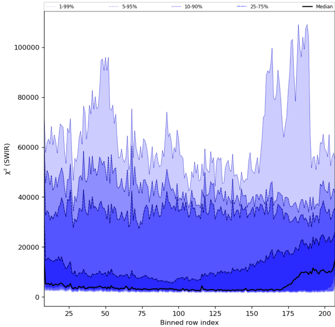
Figure 39: Along track statistics of " \chi^2 (SWIR)" for 2023-12-17 to 2023-12-19
