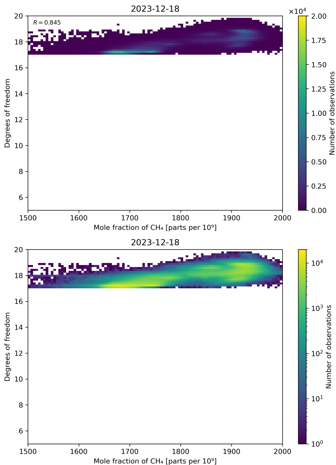
Figure 72: Scatter density plot of “Mole fraction of CH 4 ” against “Degrees of freedom” for 2023-12-17 to 2023-12-19.
