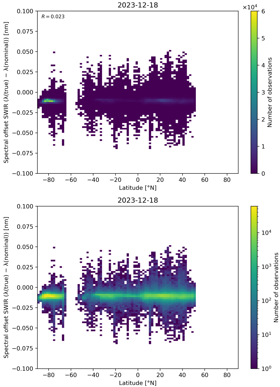
Figure 62: Scatter density plot of “Latitude” against “Spectral offset SWIR ( \lambda(\text{true}) - \lambda(\text{nominal}) )” for 2023-12-17 to 2023-12-19.
