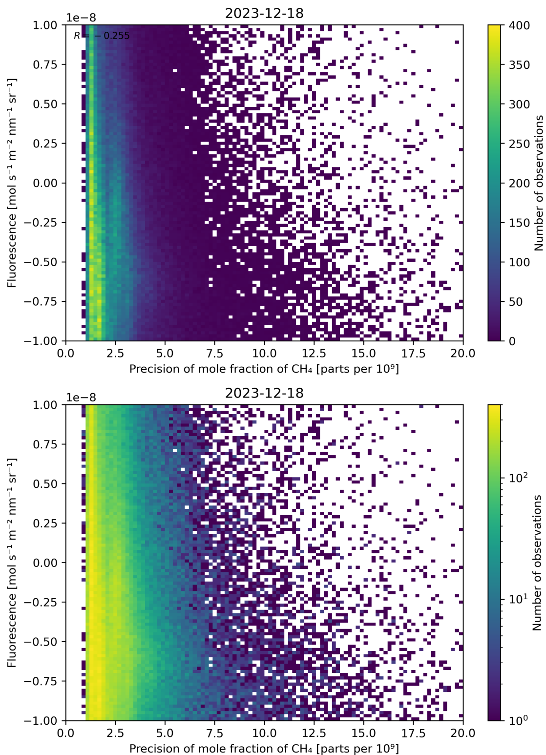
Figure 81: Scatter density plot of “Precision of mole fraction of CH 4 ” against “Fluorescence” for 2023-12-17 to 2023-12-19.
