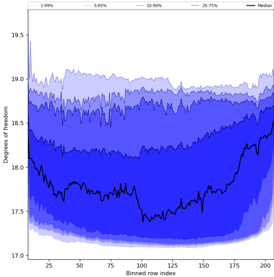
Figure 41: Along track statistics of “Degrees of freedom” for 2023-12-17 to 2023-12-19
