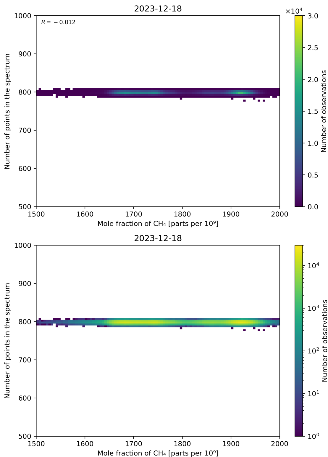
Figure 77: Scatter density plot of “Mole fraction of CH 4 ” against “Number of points in the spectrum” for 2023-12-17 to 2023-12-19.
