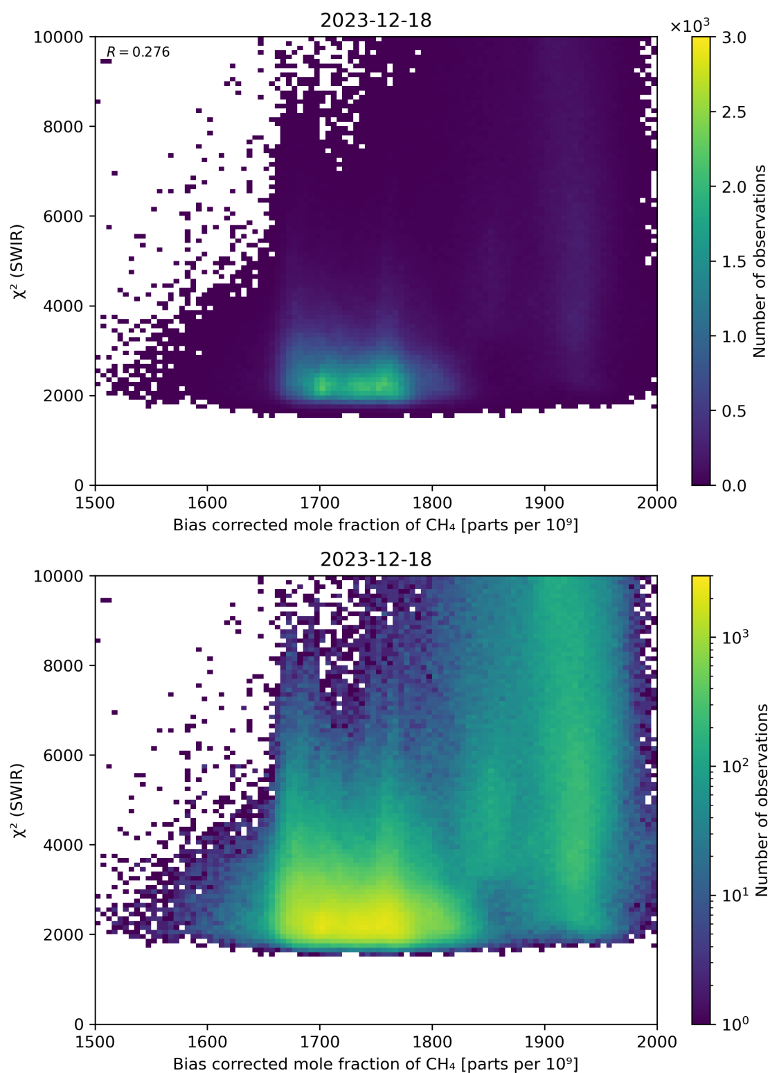
Figure 64: Scatter density plot of “Bias corrected mole fraction of \text{CH}_4 ” against “ \chi^2 (SWIR)” for 2023-12-17 to 2023-12-19.
