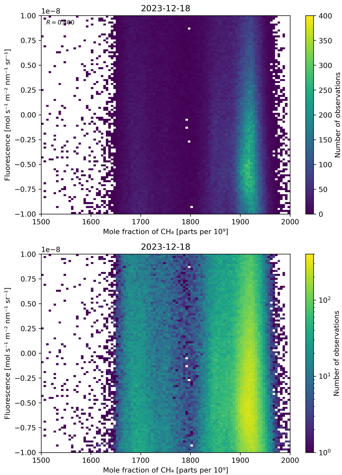
Figure 73: Scatter density plot of “Mole fraction of CH 4 ” against “Fluorescence” for 2023-12-17 to 2023-12-19.
