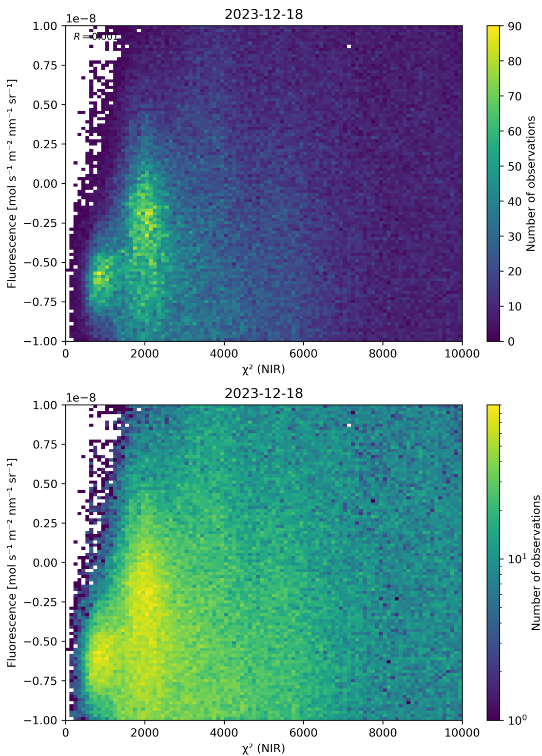
Figure 45: Scatter density plot of “ \chi^2 (NIR)” against “Fluorescence” for 2023-12-17 to 2023-12-19.
