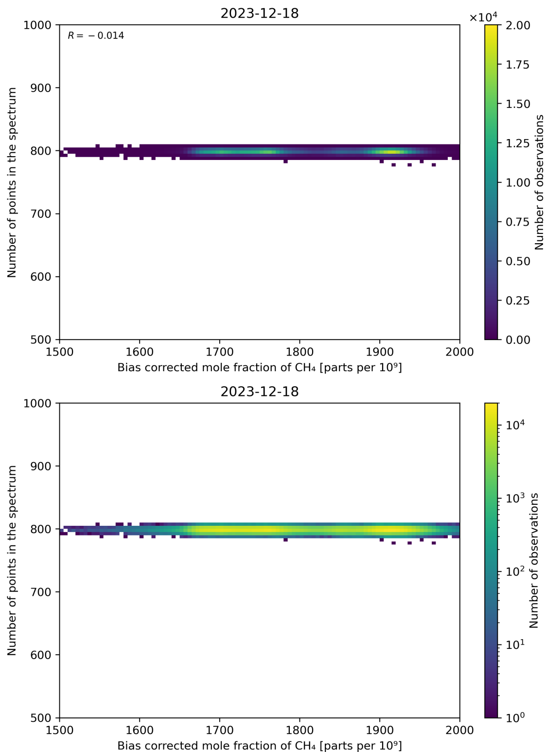
Figure 68: Scatter density plot of “Bias corrected mole fraction of CH 4 ” against “Number of points in the spectrum” for 2023-12-17 to 2023-12-19.
