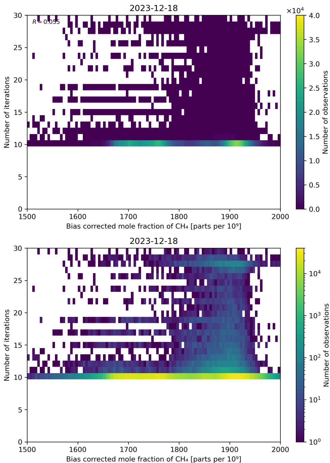
Figure 67: Scatter density plot of “Bias corrected mole fraction of \text{CH}_4 ” against “Number of iterations” for 2023-12-17 to 2023-12-19.
