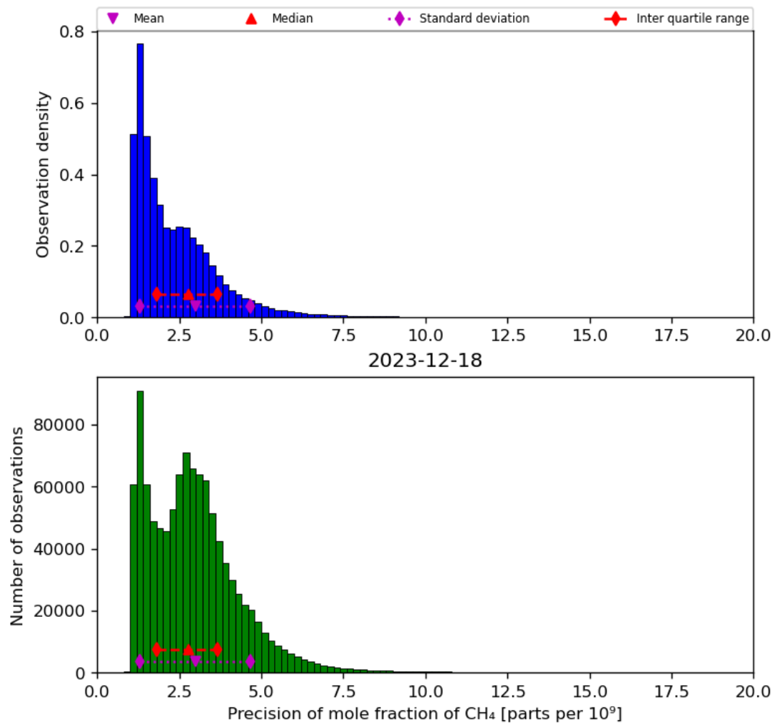
Figure 24: Histogram of “Precision of mole fraction of CH 4 ” for 2023-12-17 to 2023-12-19
