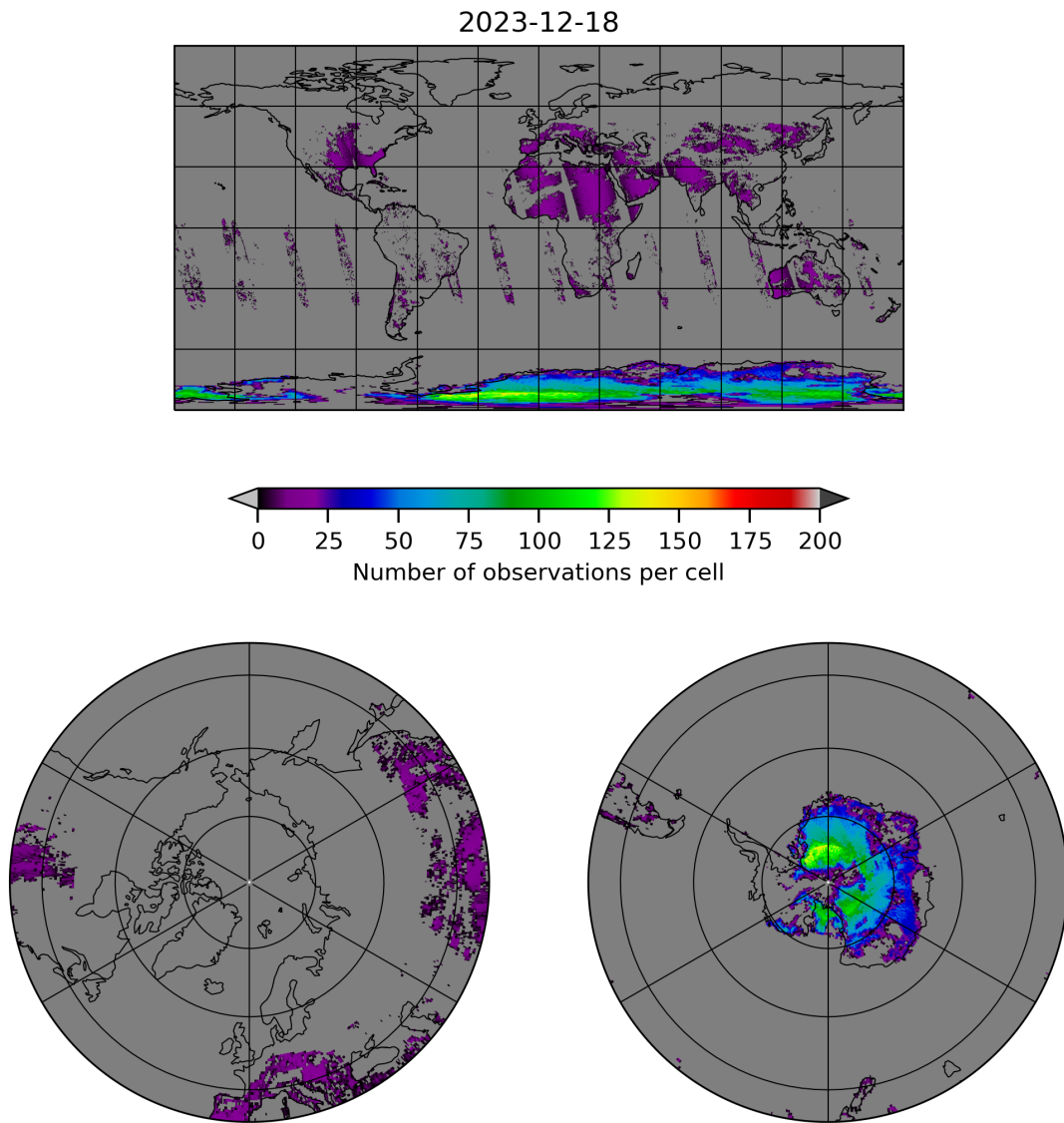
Figure 10: Map of the number of observations for 2023-12-17 to 2023-12-19
