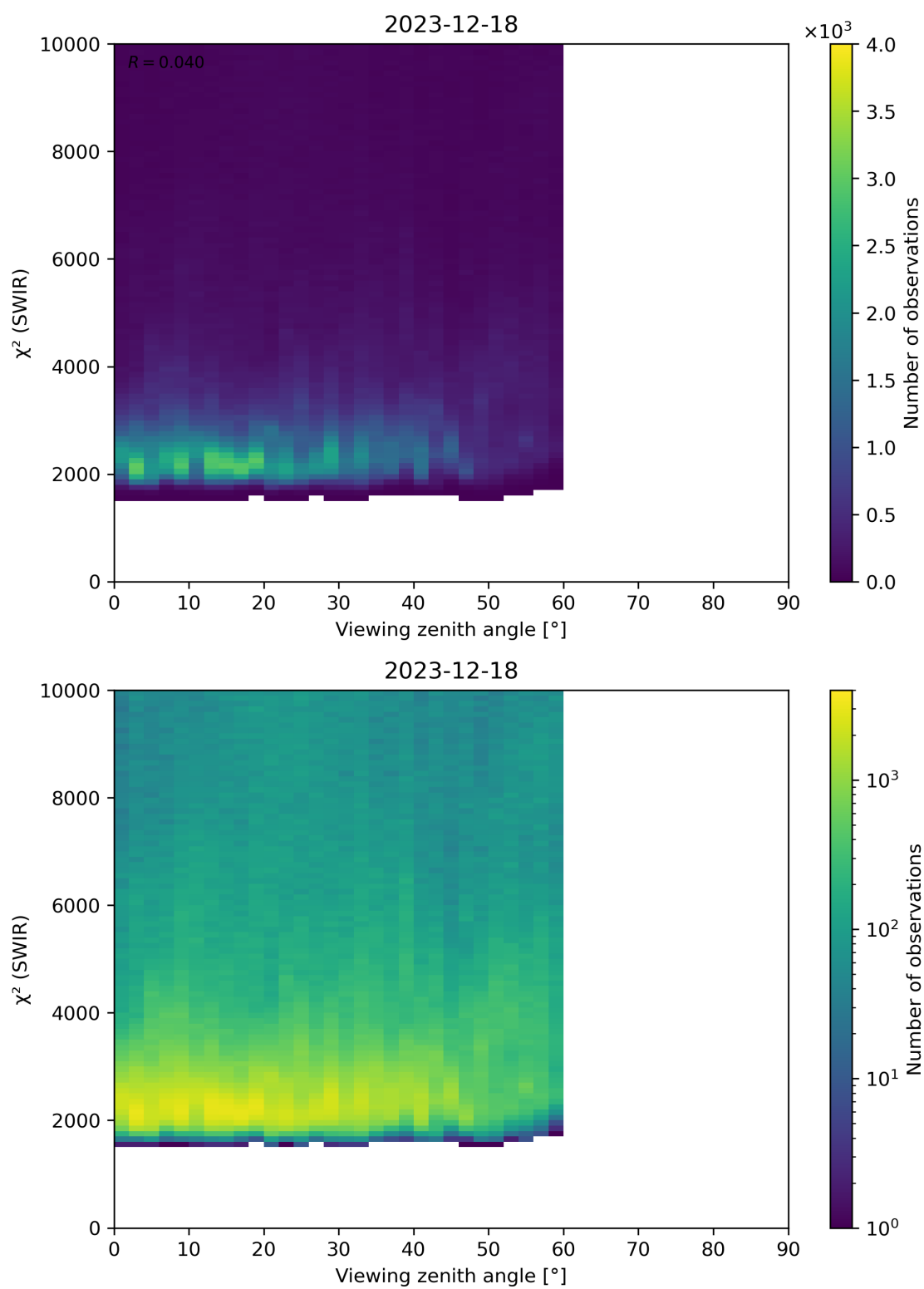
Figure 106: Scatter density plot of “Viewing zenith angle” against “ \chi^2 (SWIR)” for 2023-12-17 to 2023-12-19.
