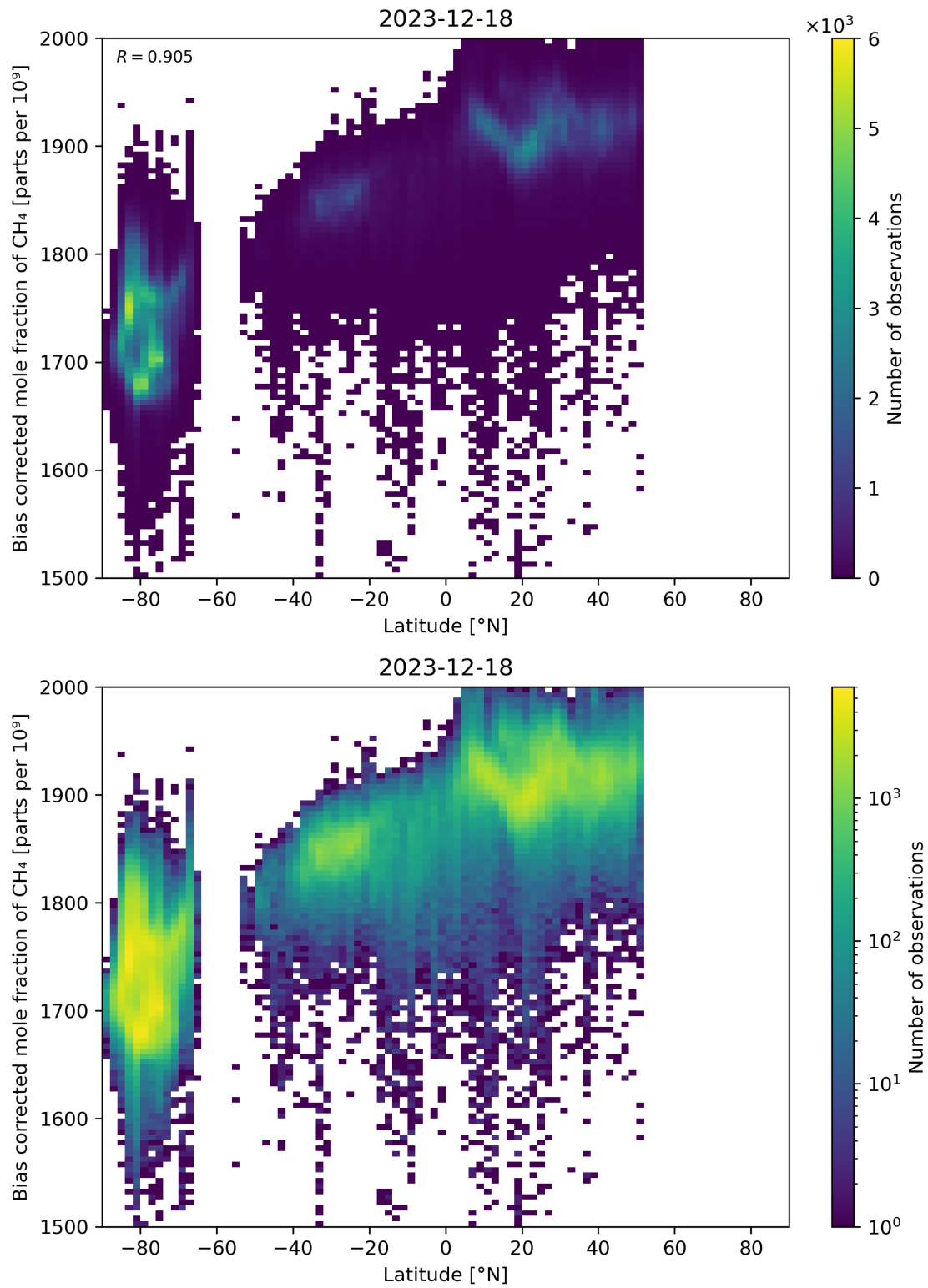
Figure 58: Scatter density plot of “Latitude” against “Bias corrected mole fraction of CH 4 ” for 2023-12-17 to 2023-12-19.
