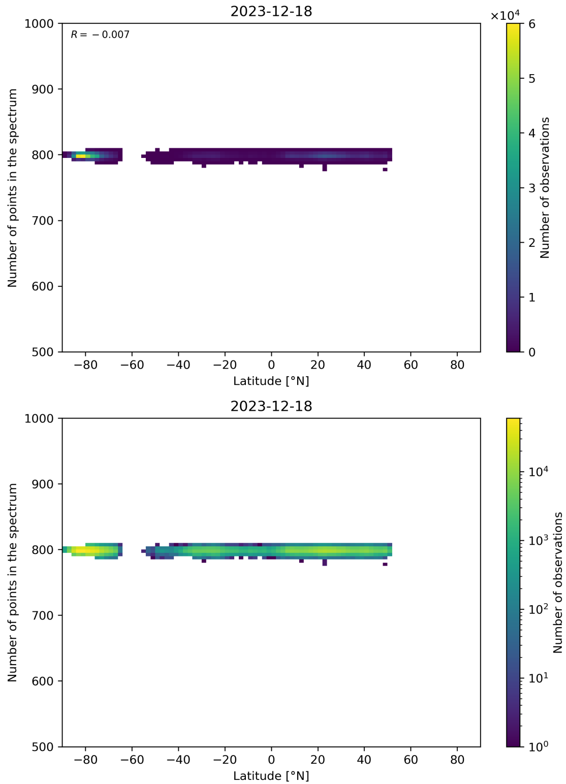
Figure 61: Scatter density plot of “Latitude” against “Number of points in the spectrum” for 2023-12-17 to 2023-12-19.
