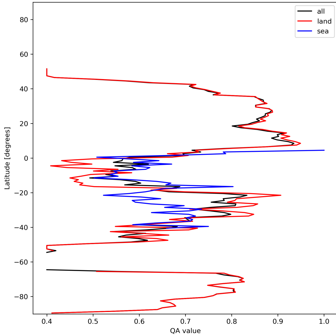
Figure 11: Zonal average of “QA value” for 2023-12-17 to 2023-12-19.
