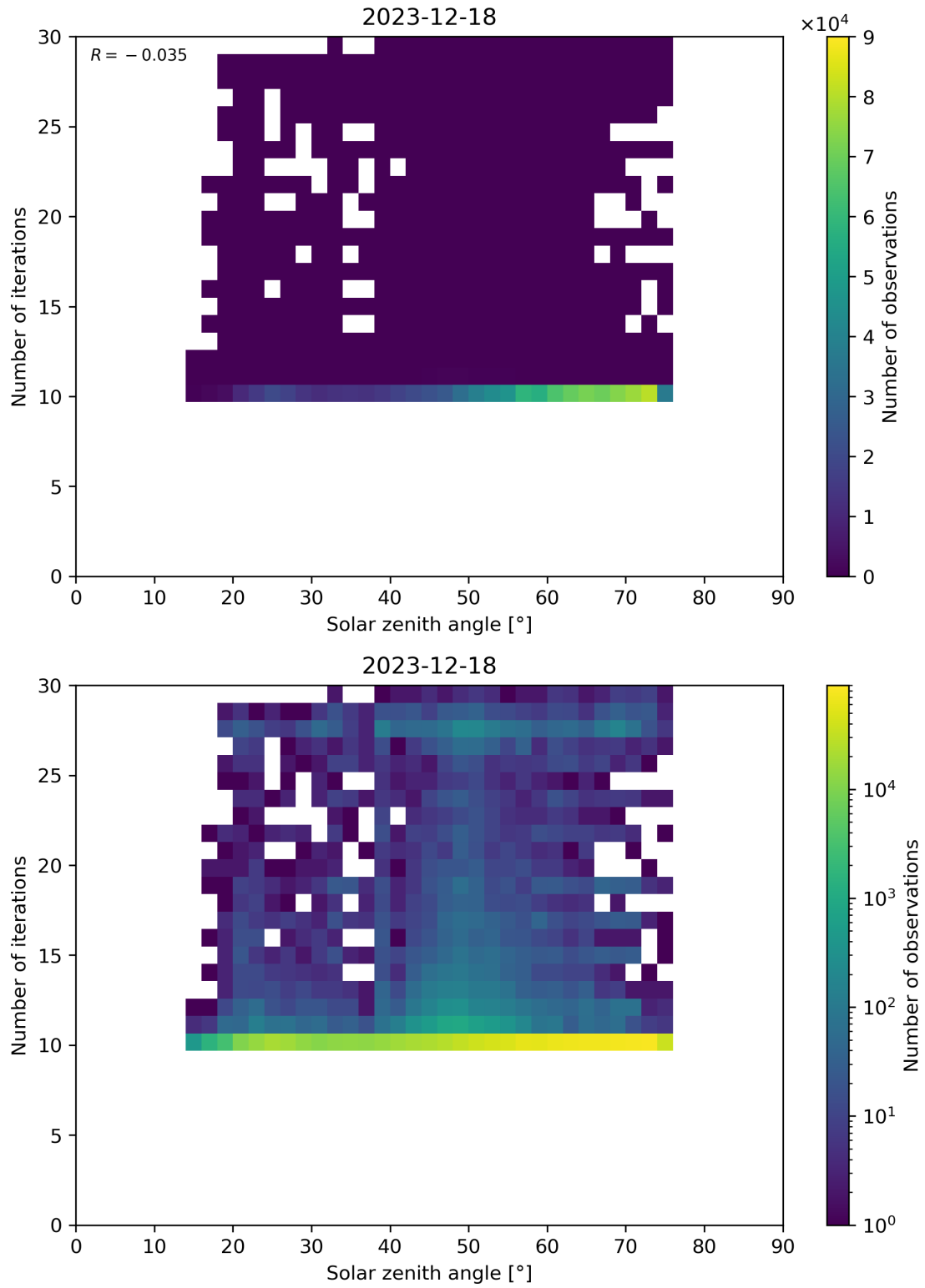
Figure 102: Scatter density plot of “Solar zenith angle” against “Number of iterations” for 2023-12-17 to 2023-12-19.
