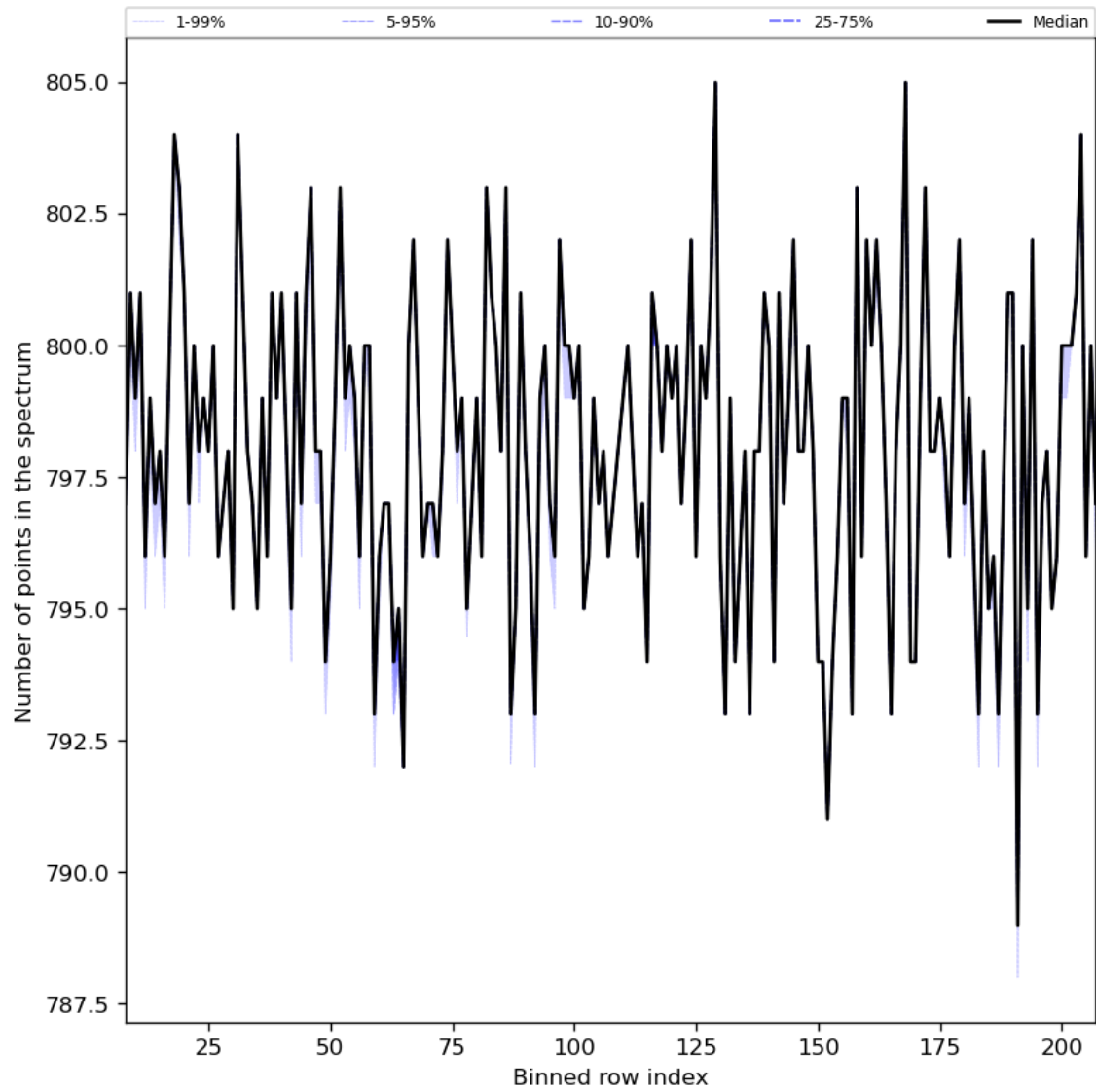
Figure 37: Along track statistics of “Number of points in the spectrum” for 2023-12-17 to 2023-12-19
