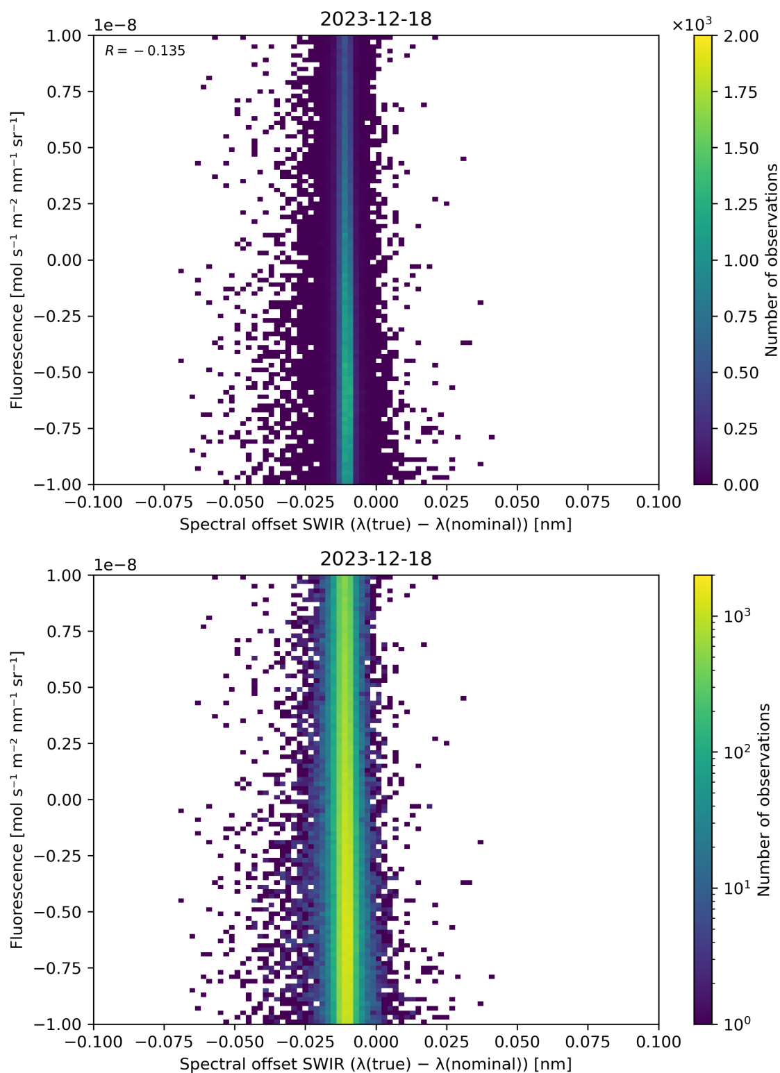
Figure 120: Scatter density plot of “Spectral offset SWIR ( \lambda(\text{true}) - \lambda(\text{nominal}) )” against “Fluorescence” for 2023-12-17 to 2023-12-19.
