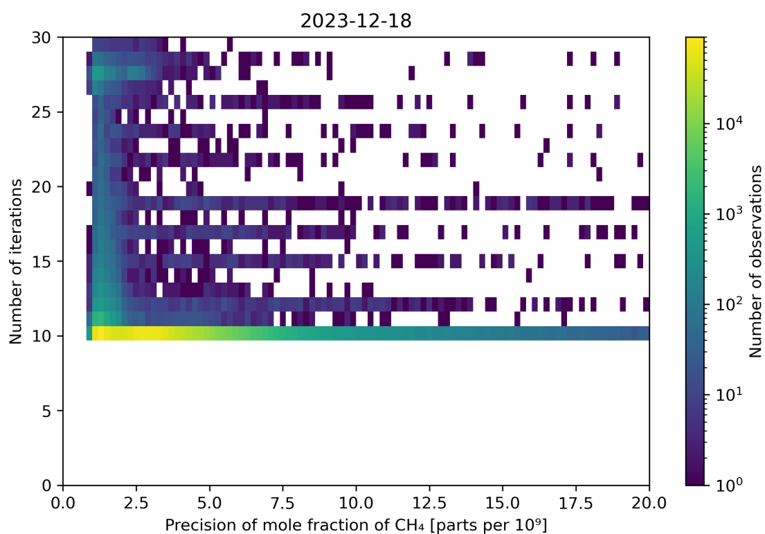
Figure 83: Scatter density plot of “Precision of mole fraction of CH 4 ” against “Number of iterations” for 2023-12-17 to 2023-12-19.
