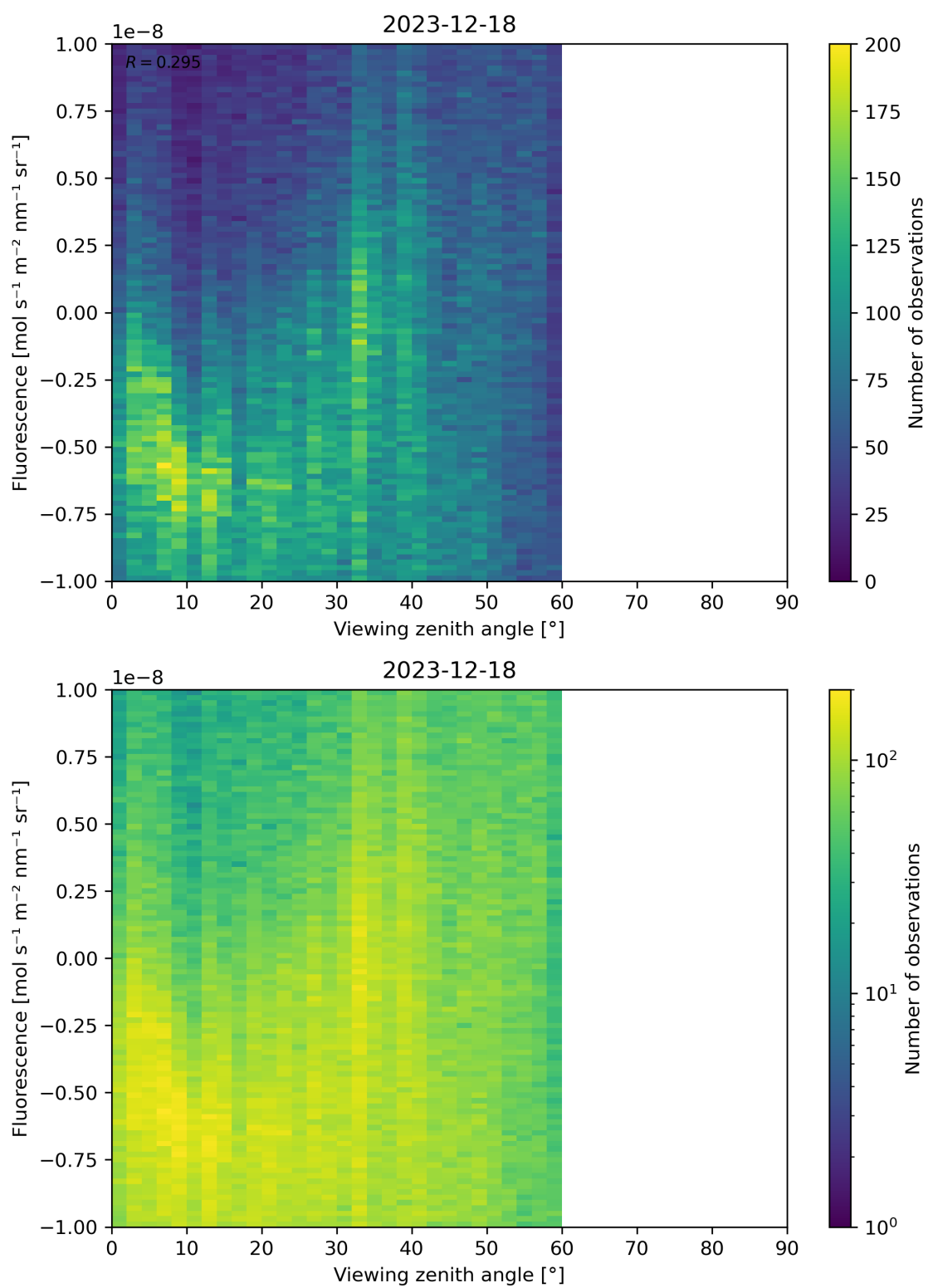
Figure 108: Scatter density plot of “Viewing zenith angle” against “Fluorescence” for 2023-12-17 to 2023-12-19.
