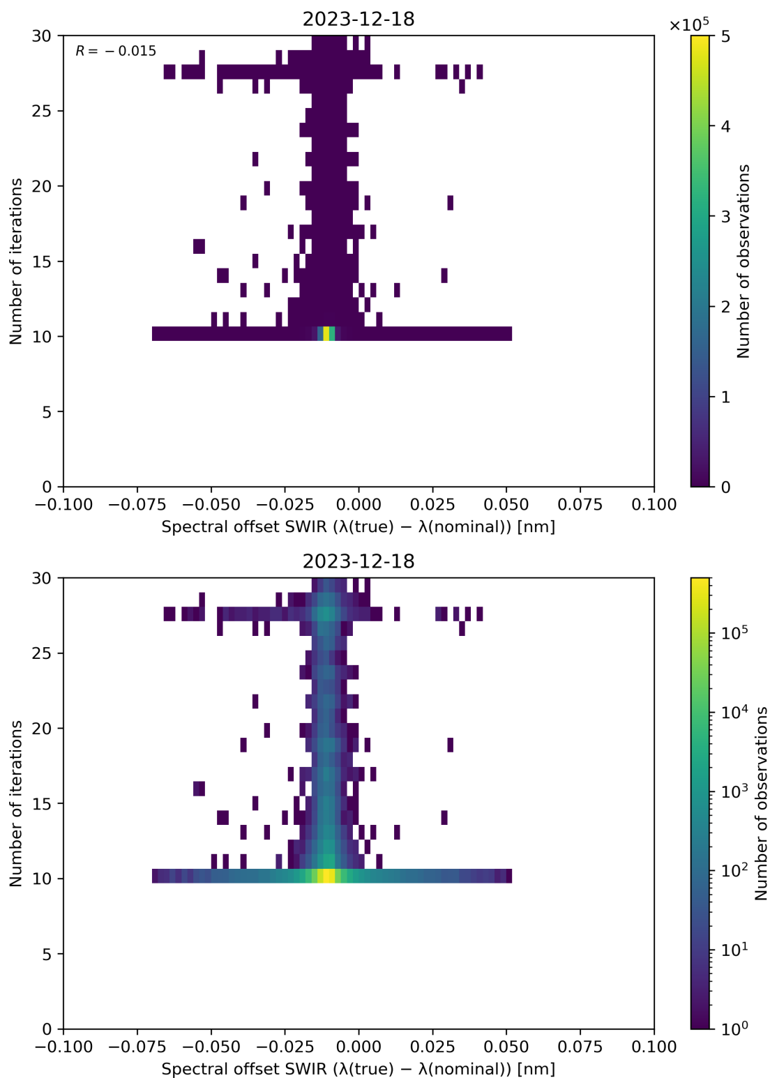
Figure 121: Scatter density plot of “Spectral offset SWIR ( \lambda(\text{true}) - \lambda(\text{nominal}) )” against “Number of iterations” for 2023-12-17 to 2023-12-19.
