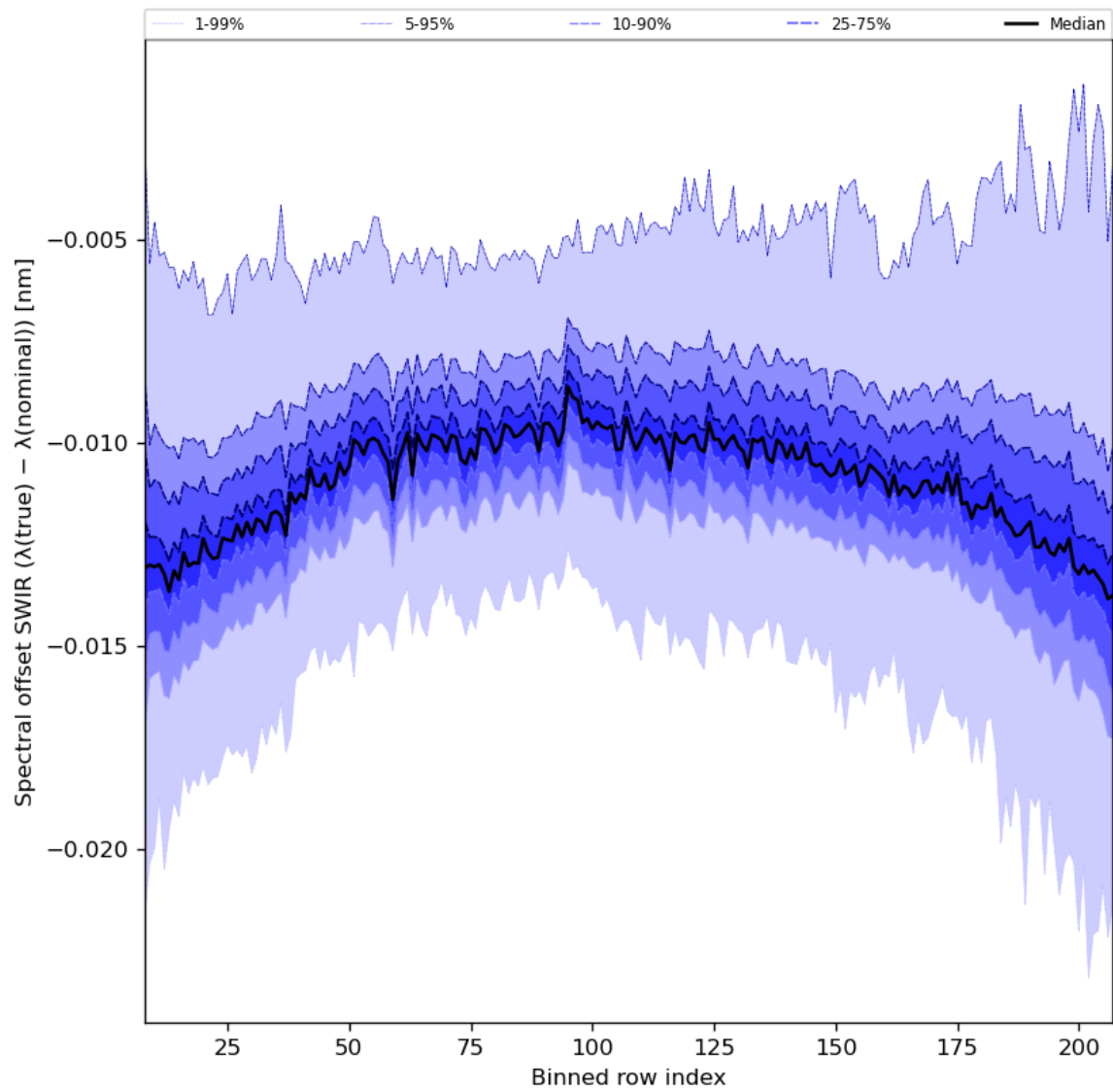
Figure 38: Along track statistics of “Spectral offset SWIR ( \lambda(\text{true}) - \lambda(\text{nominal}) )” for 2023-12-17 to 2023-12-19
