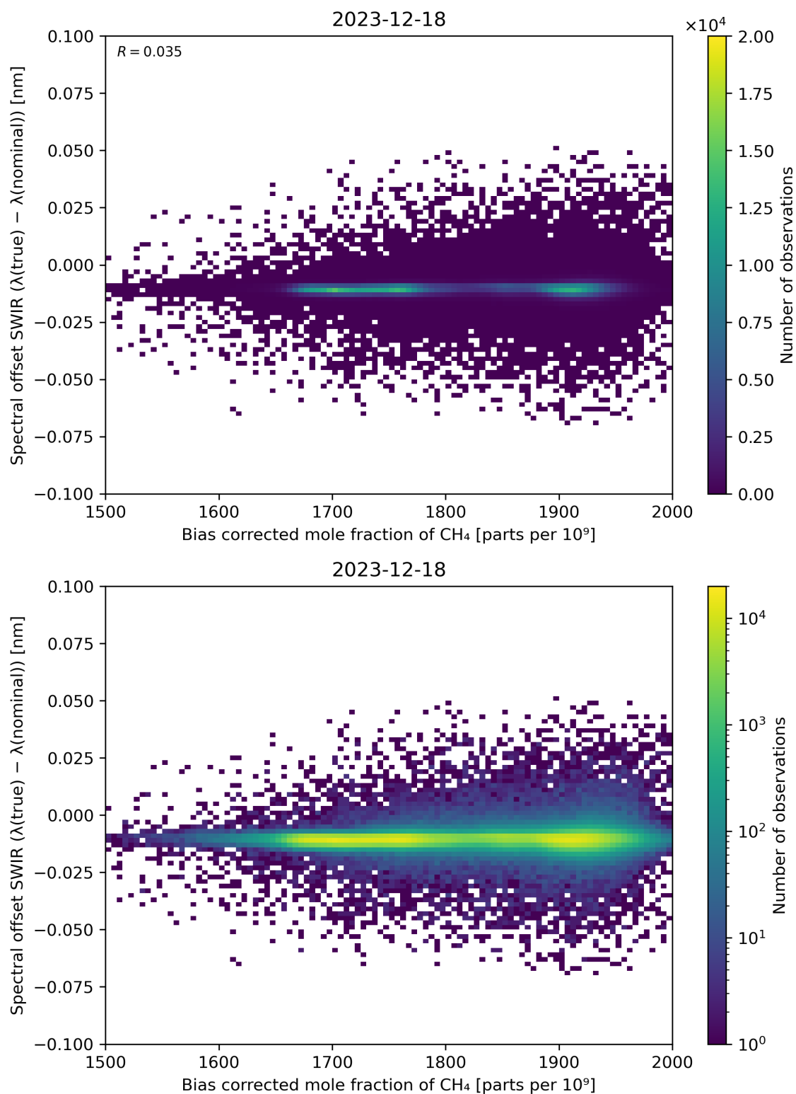
Figure 69: Scatter density plot of “Bias corrected mole fraction of \text{CH}_4 ” against “Spectral offset SWIR ( \lambda(\text{true}) - \lambda(\text{nominal}) )” for 2023-12-17 to 2023-12-19.
