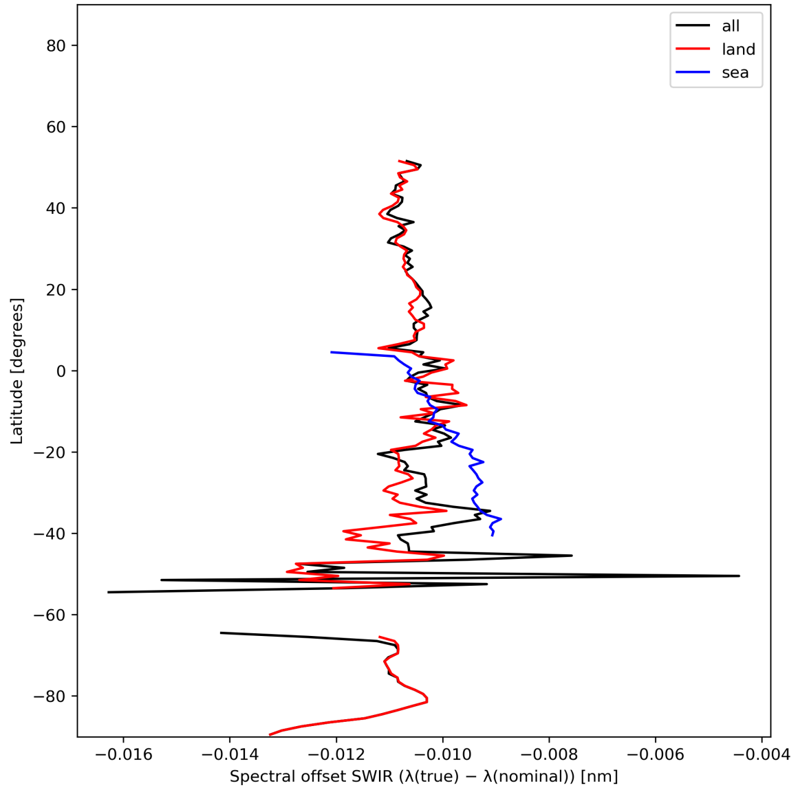
Figure 16: Zonal average of “Spectral offset SWIR ( \lambda(\text{true}) - \lambda(\text{nominal}) )” for 2023-12-17 to 2023-12-19.
