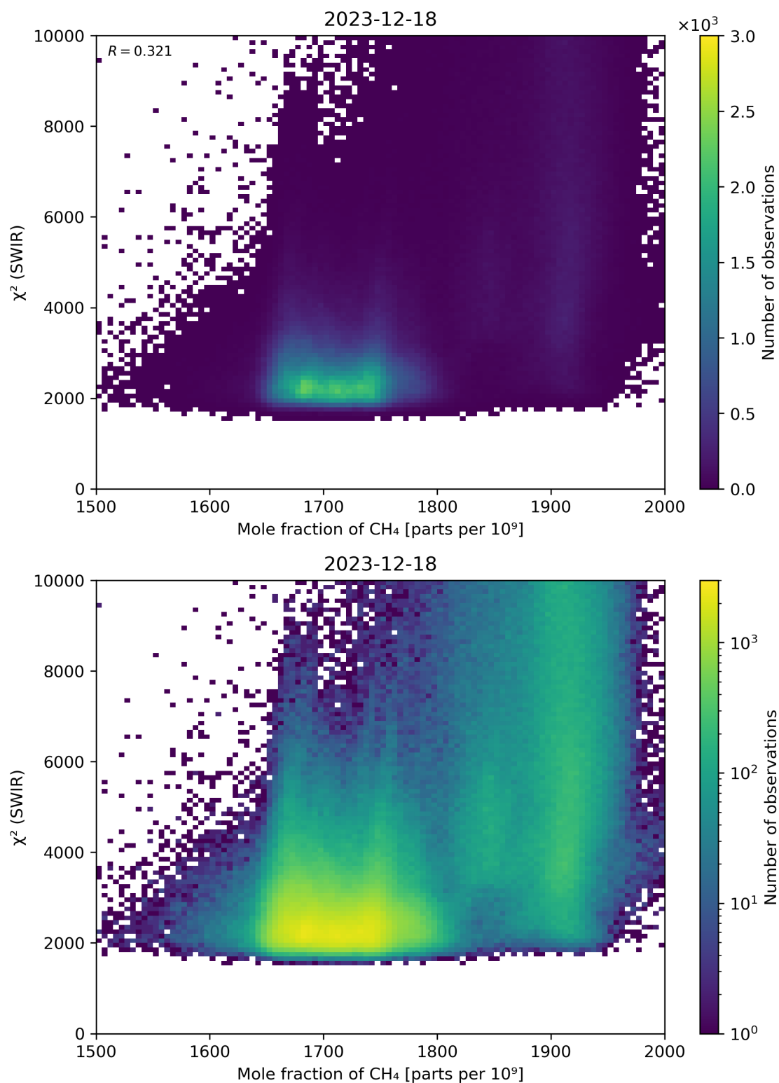
Figure 71: Scatter density plot of “Mole fraction of \text{CH}_4 ” against “ \chi^2 (SWIR)” for 2023-12-17 to 2023-12-19.
