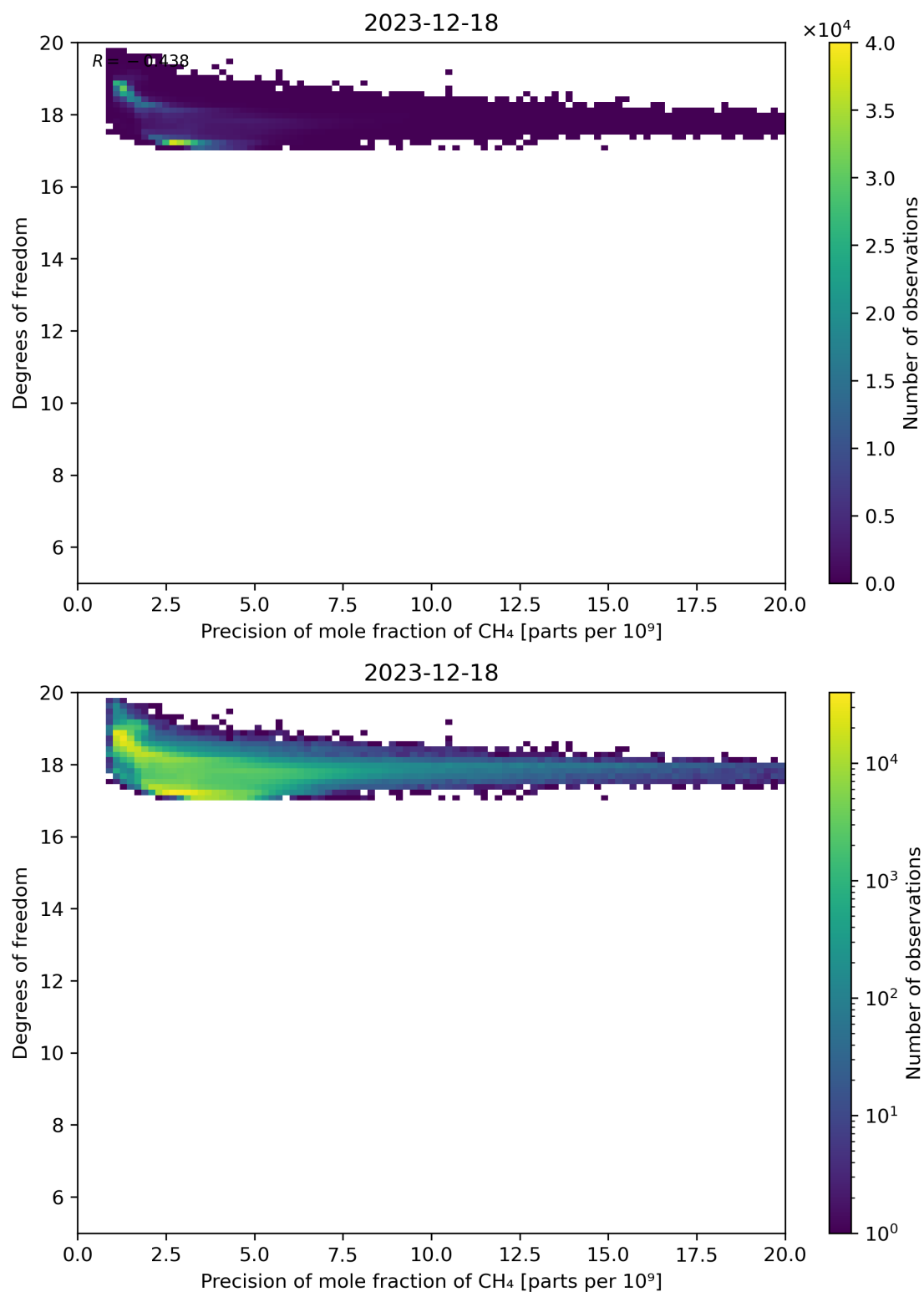
Figure 80: Scatter density plot of “Precision of mole fraction of \text{CH}_4 ” against “Degrees of freedom” for 2023-12-17 to 2023-12-19.
