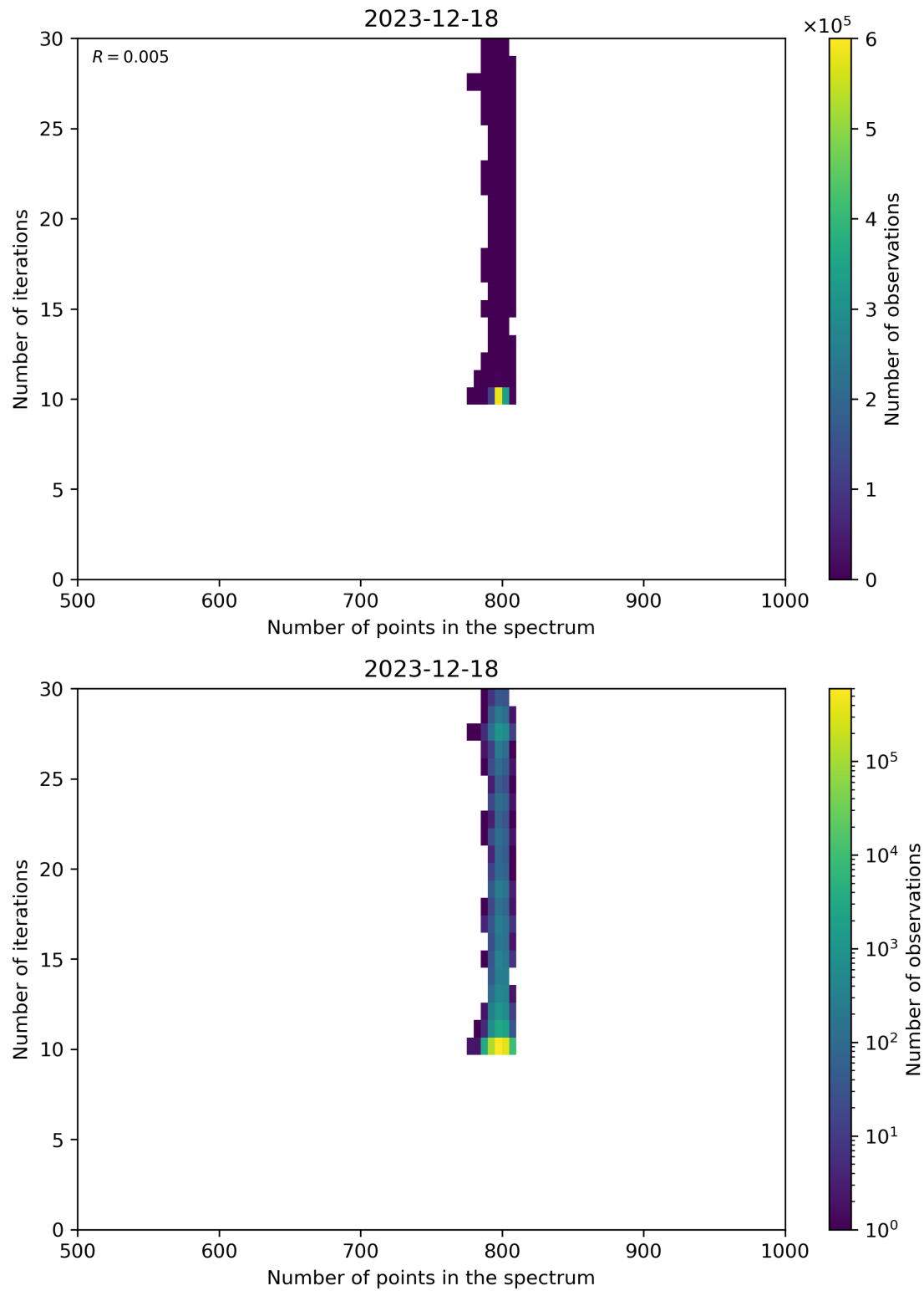
Figure 92: Scatter density plot of “Number of points in the spectrum” against “Number of iterations” for 2023-12-17 to 2023-12-19.
