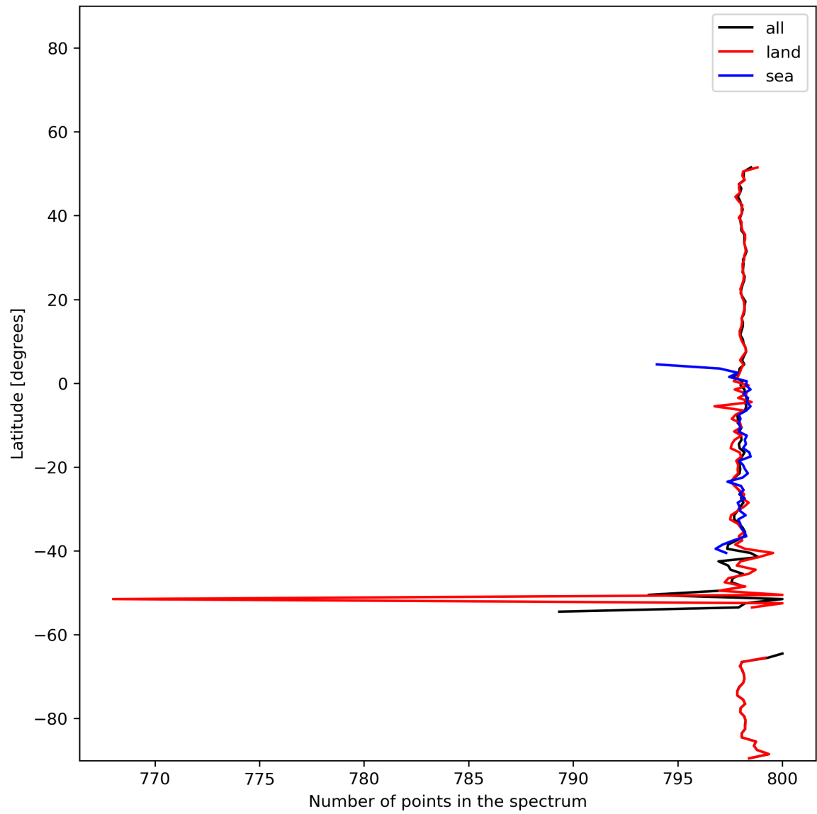
Figure 15: Zonal average of “Number of points in the spectrum” for 2023-12-17 to 2023-12-19.
