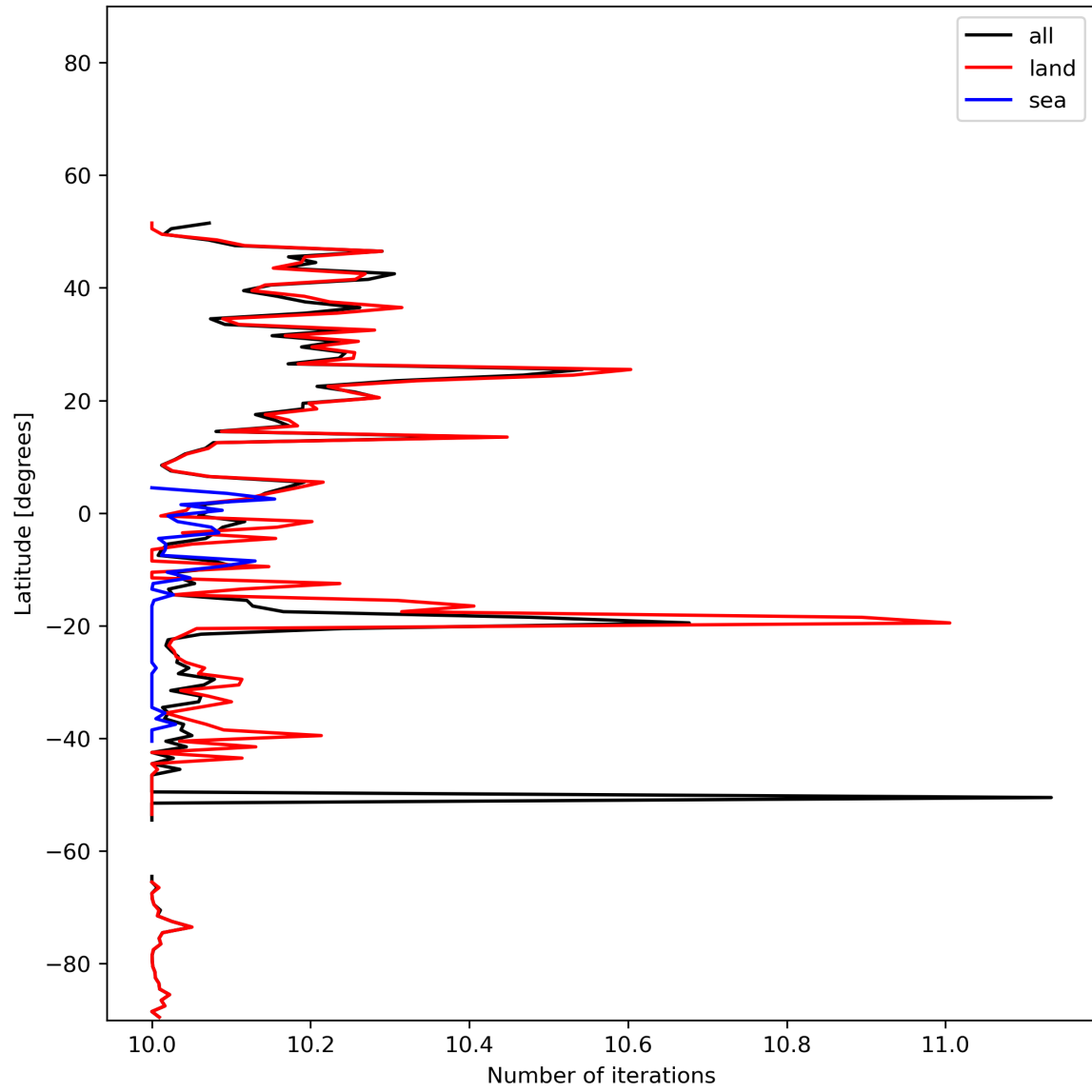
Figure 20: Zonal average of “Number of iterations” for 2023-12-17 to 2023-12-19.
