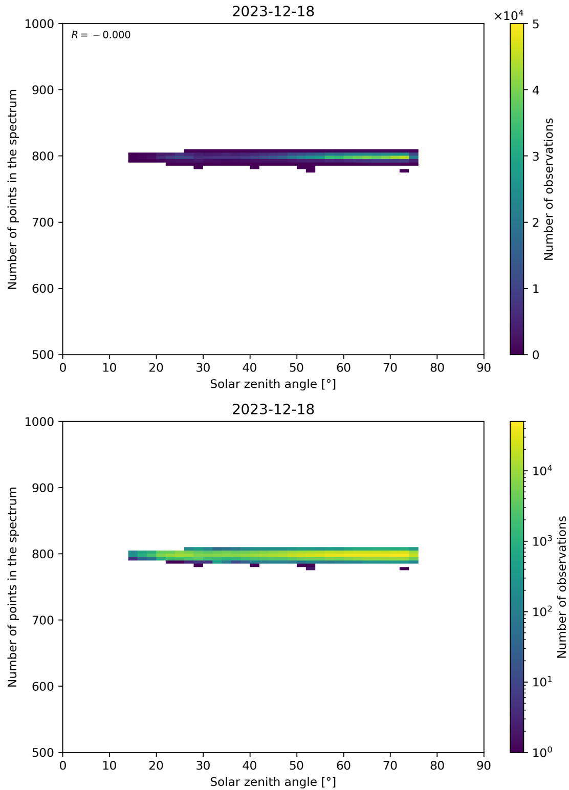
Figure 103: Scatter density plot of “Solar zenith angle” against “Number of points in the spectrum” for 2023-12-17 to 2023-12-19.
