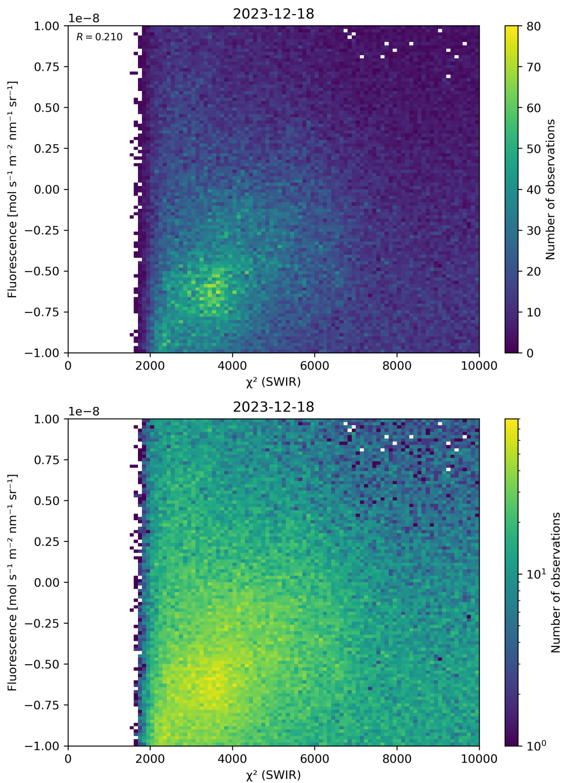
Figure 49: Scatter density plot of “ \chi^2 (SWIR)” against “Fluorescence” for 2023-12-17 to 2023-12-19.
