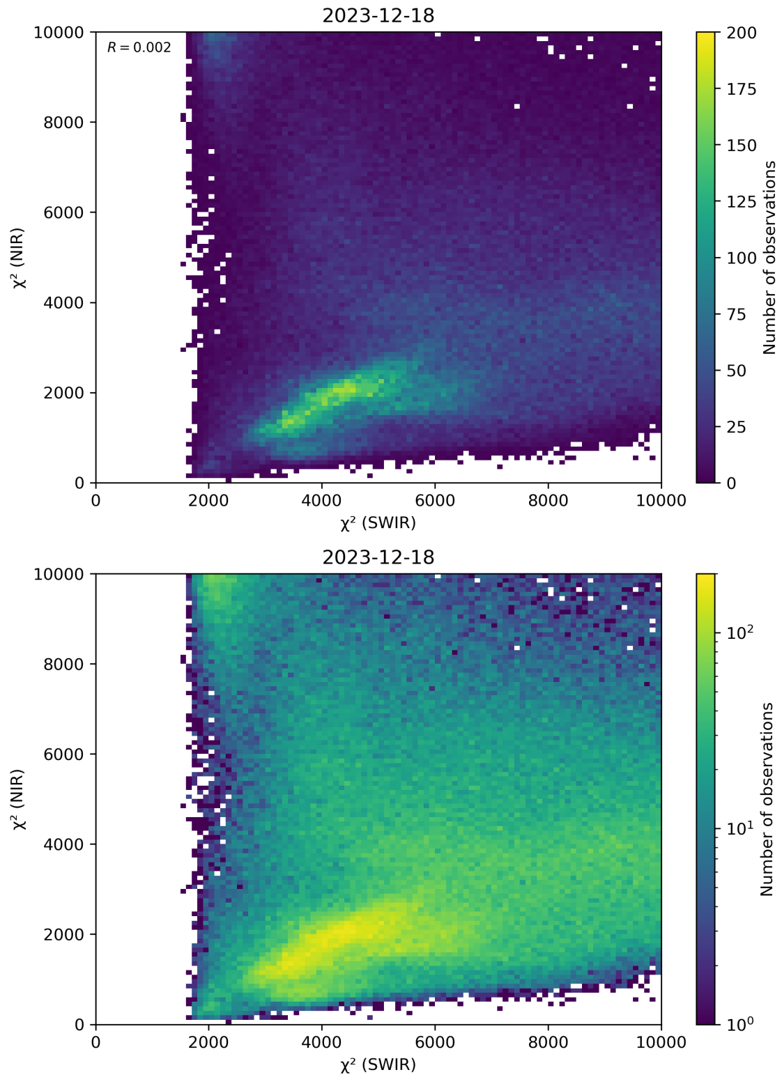
Figure 47: Scatter density plot of “ \chi^2 (SWIR)” against “ \chi^2 (NIR)” for 2023-12-17 to 2023-12-19.
