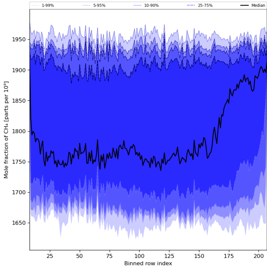
Figure 34: Along track statistics of “Mole fraction of CH 4 ” for 2023-12-17 to 2023-12-19
