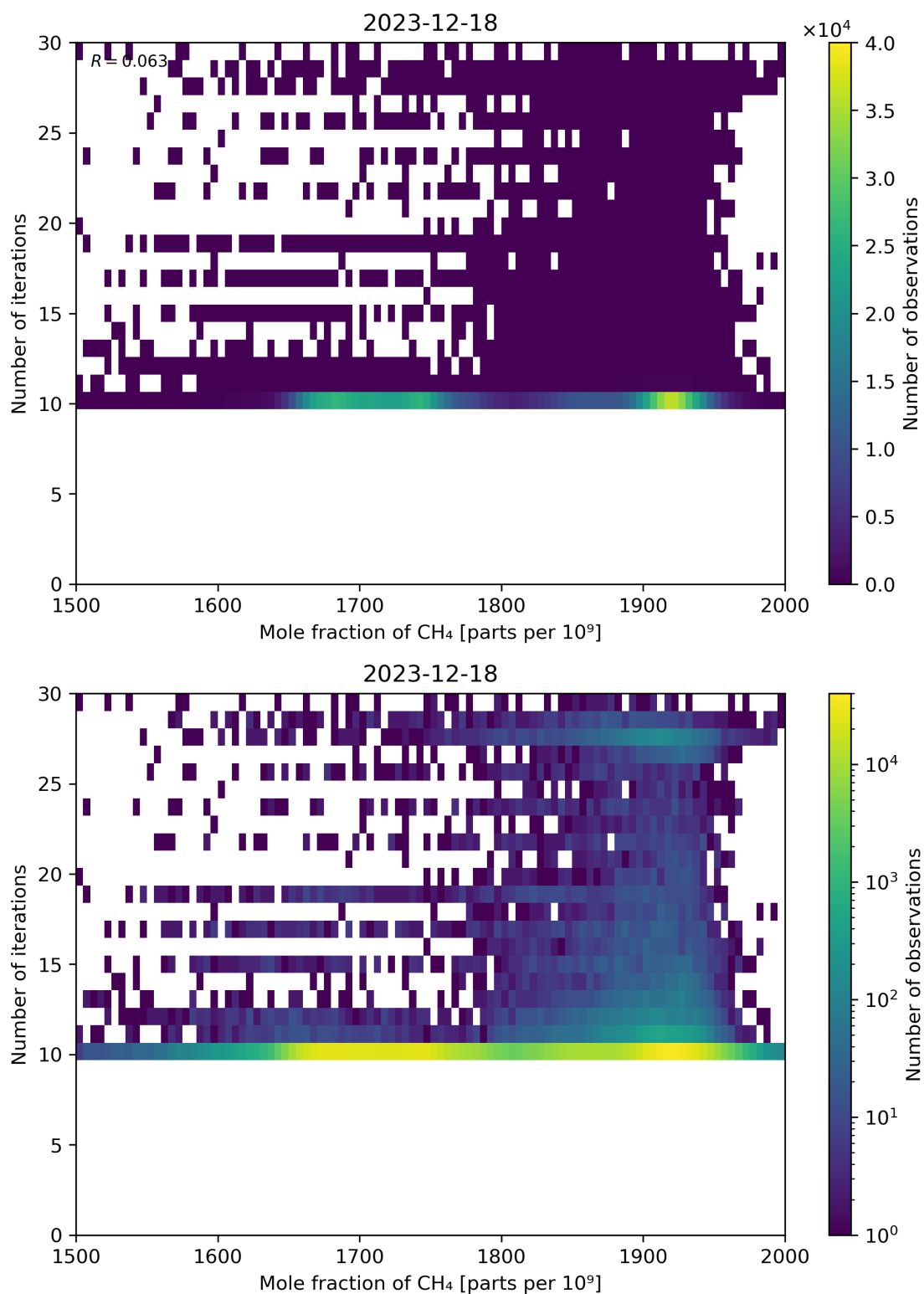
Figure 76: Scatter density plot of “Mole fraction of CH 4 ” against “Number of iterations” for 2023-12-17 to 2023-12-19.
