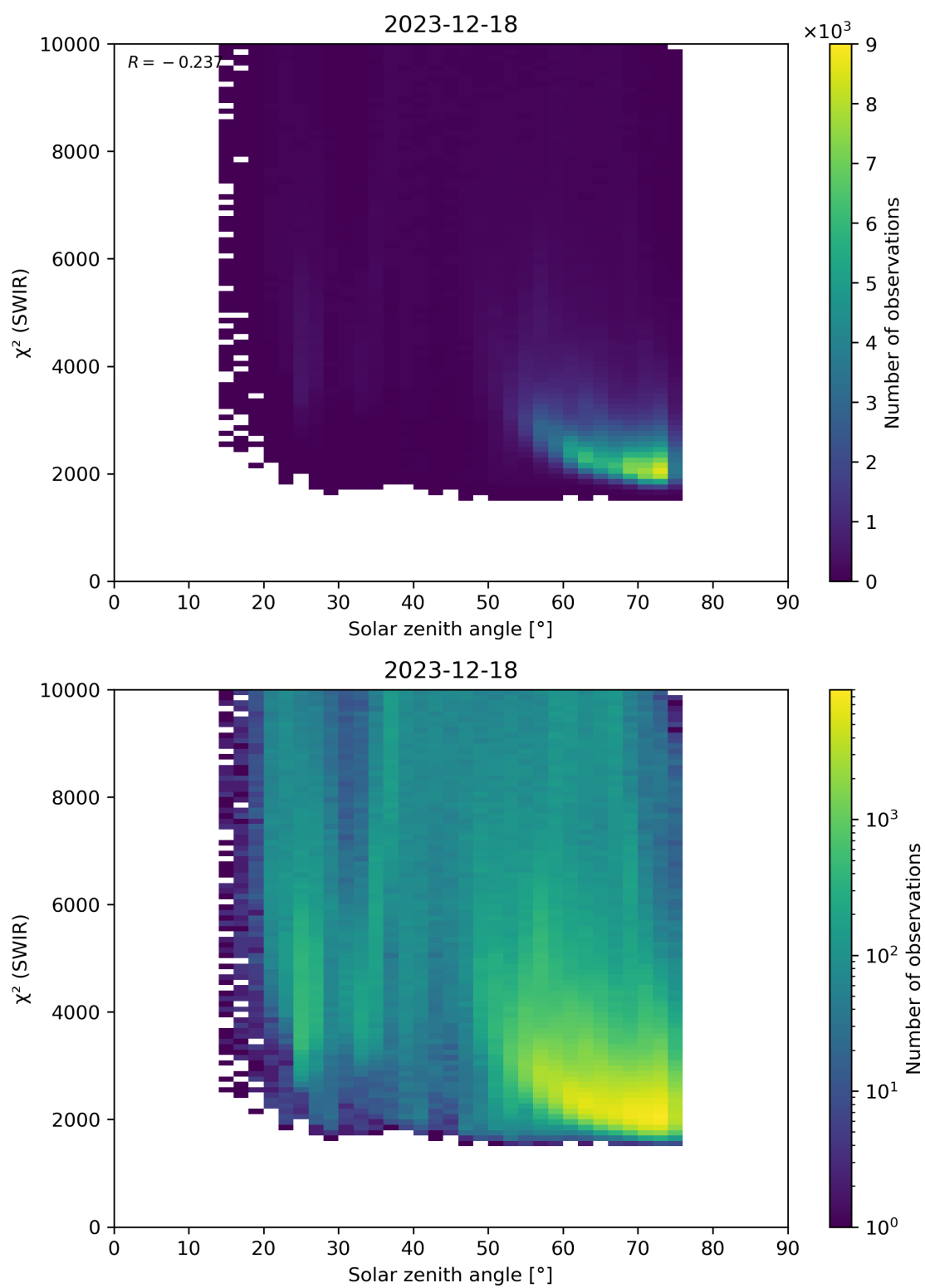
Figure 95: Scatter density plot of “Solar zenith angle” against “ \chi^2 (SWIR)” for 2023-12-17 to 2023-12-19.
