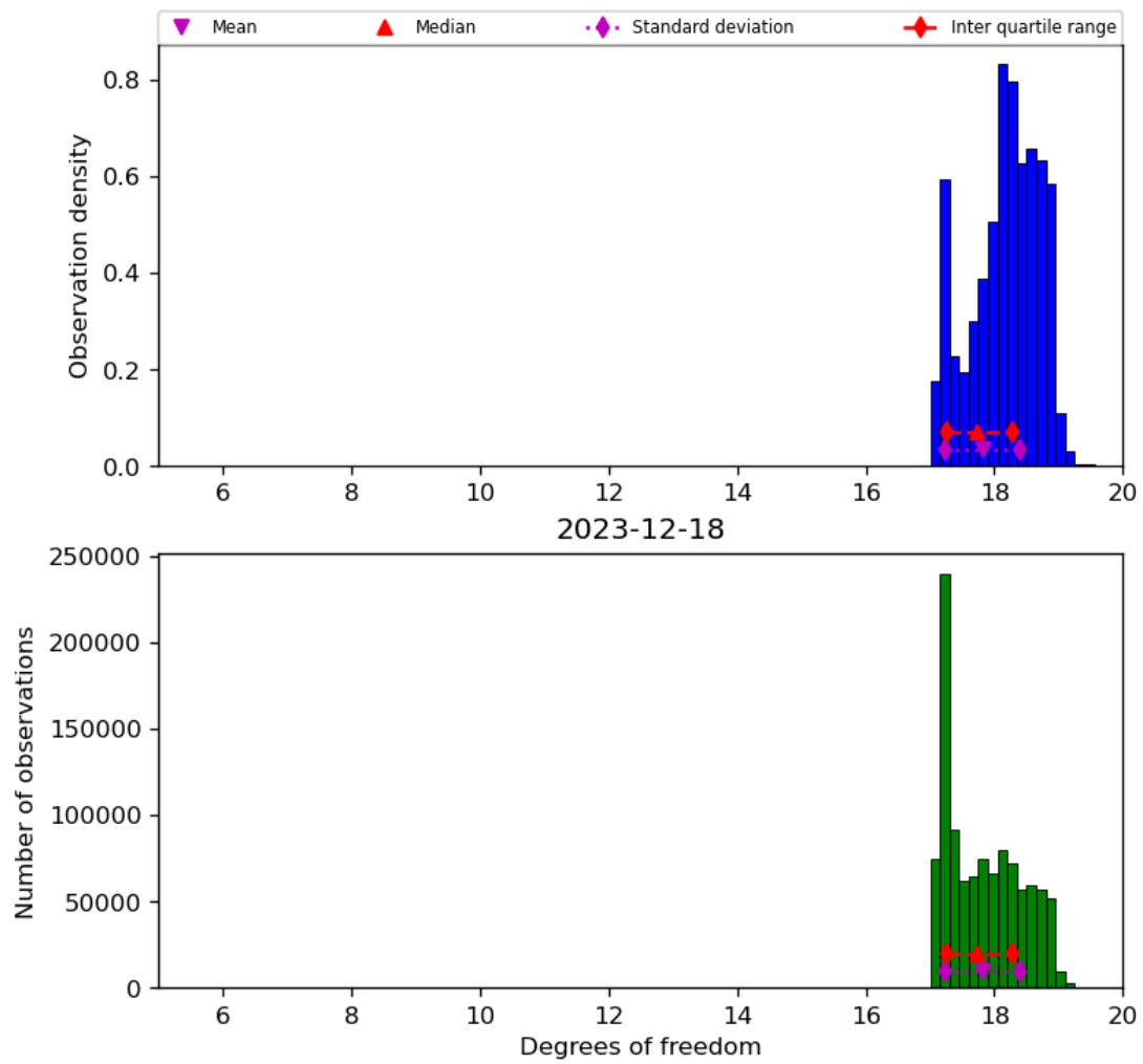
Figure 30: Histogram of “Degrees of freedom” for 2023-12-17 to 2023-12-19
