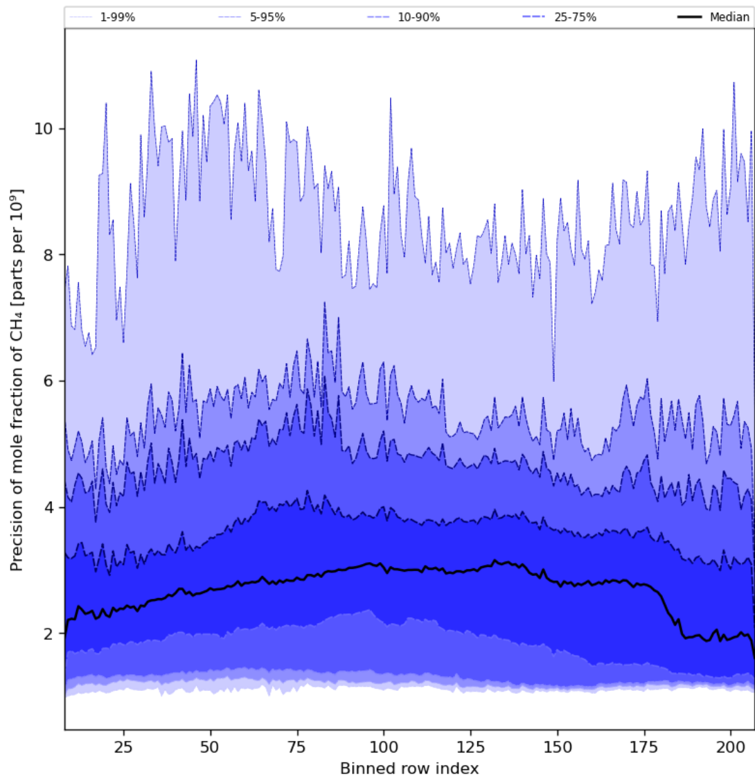
Figure 35: Along track statistics of “Precision of mole fraction of CH 4 ” for 2023-12-17 to 2023-12-19
