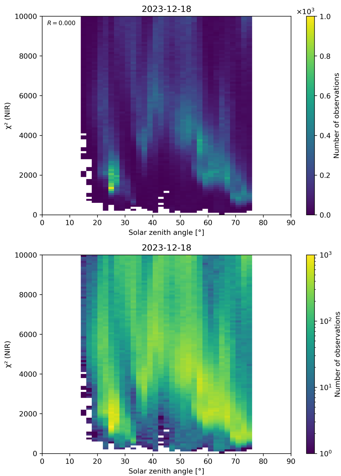
Figure 94: Scatter density plot of “Solar zenith angle” against “ \chi^2 (NIR)” for 2023-12-17 to 2023-12-19.
