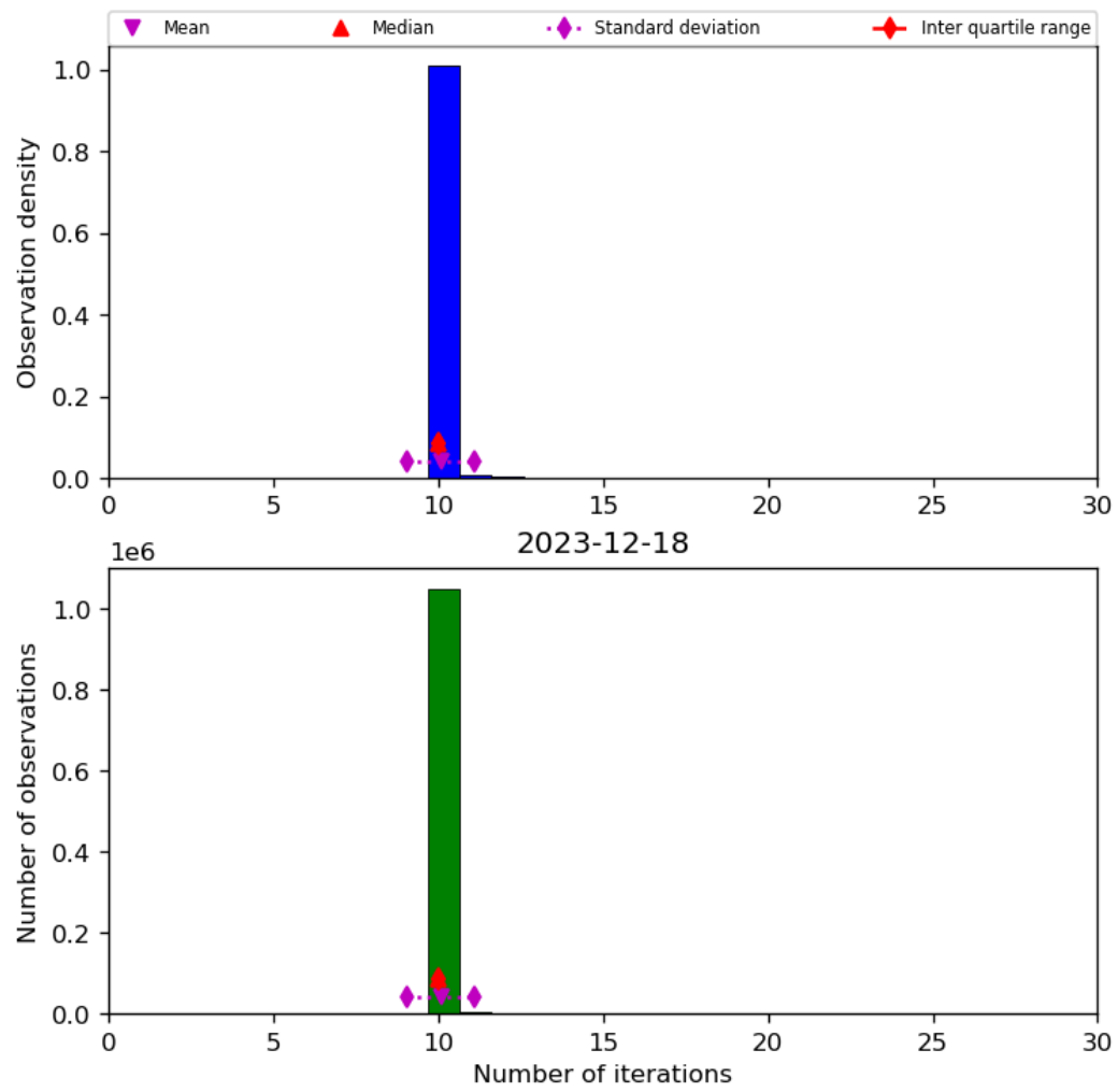
Figure 31: Histogram of “Number of iterations” for 2023-12-17 to 2023-12-19
