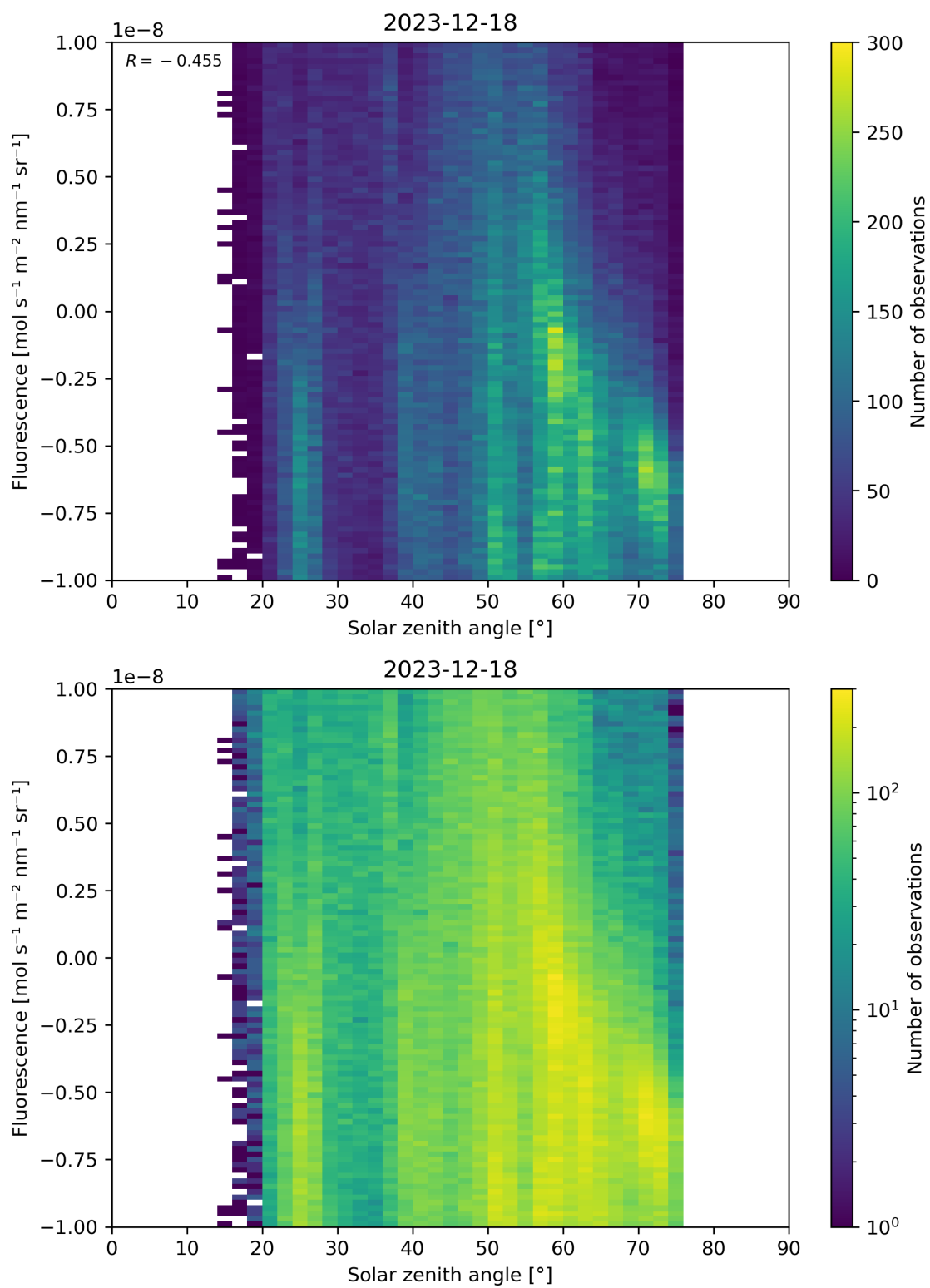
Figure 97: Scatter density plot of “Solar zenith angle” against “Fluorescence” for 2023-12-17 to 2023-12-19.
