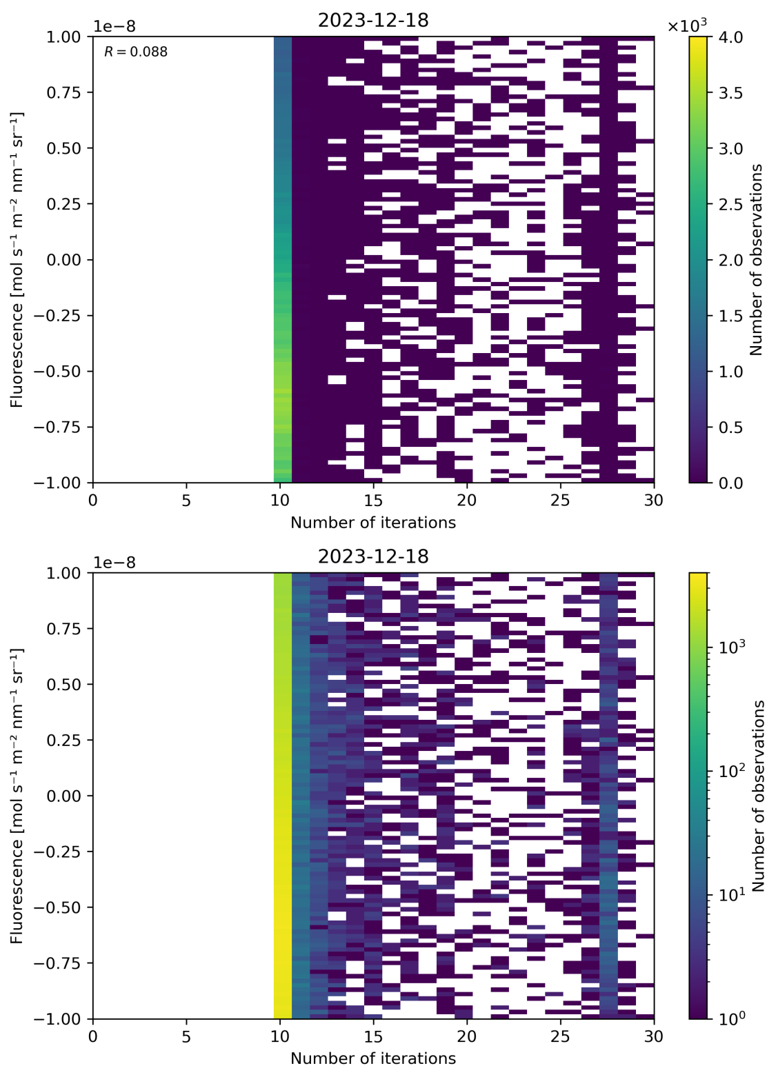
Figure 87: Scatter density plot of “Number of iterations” against “Fluorescence” for 2023-12-17 to 2023-12-19.
