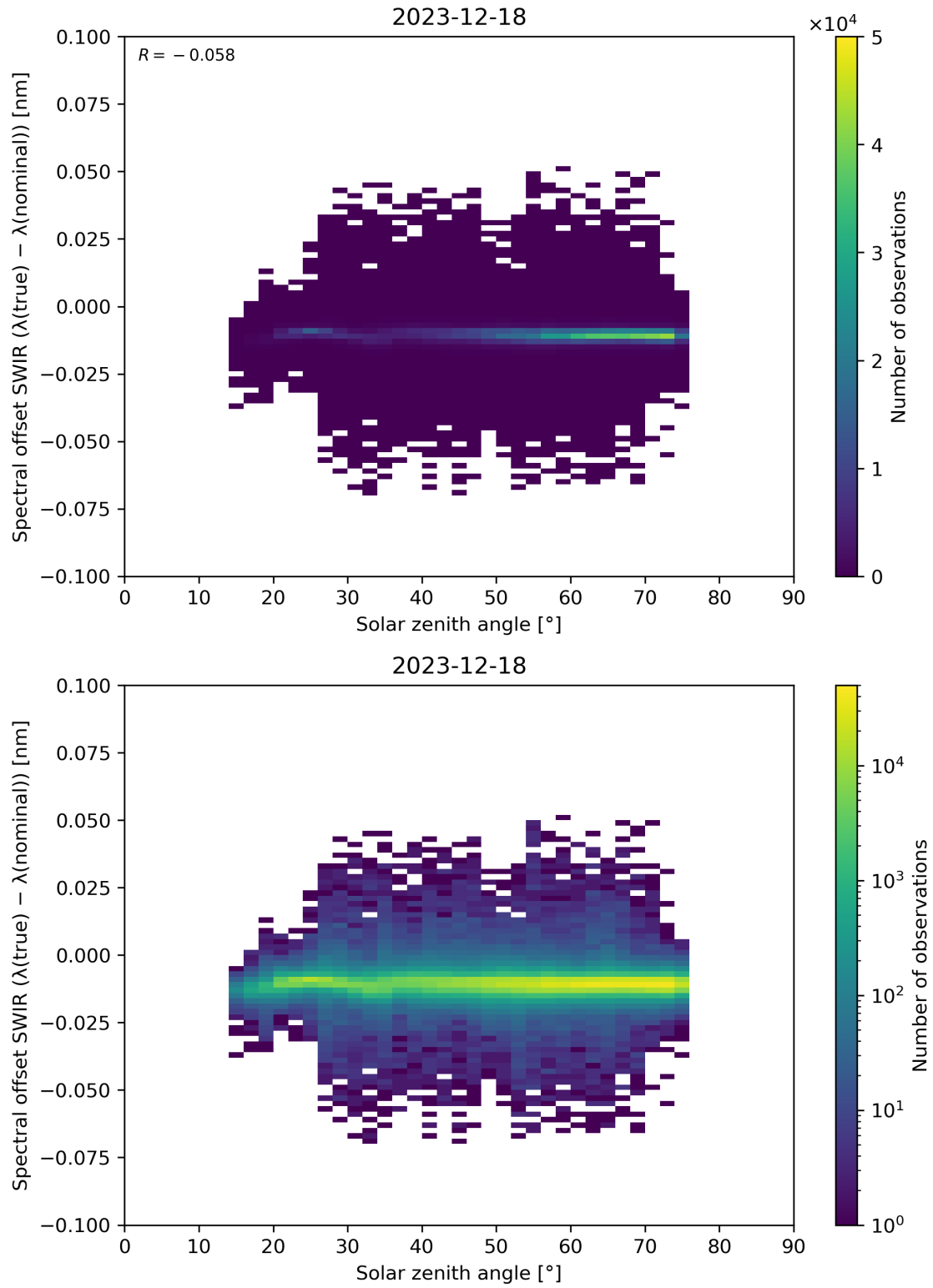
Figure 104: Scatter density plot of “Solar zenith angle” against “Spectral offset SWIR ( \lambda(\text{true}) - \lambda(\text{nominal}) )” for 2023-12-17 to 2023-12-19.
