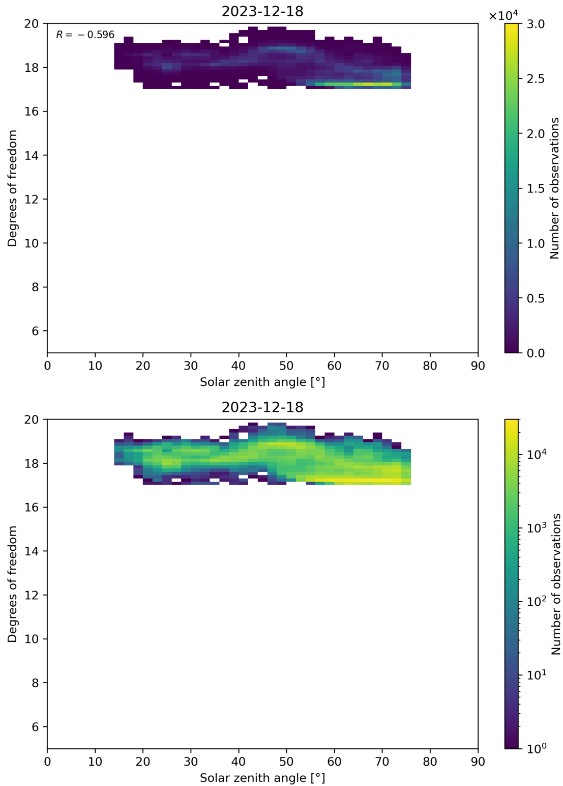
Figure 96: Scatter density plot of “Solar zenith angle” against “Degrees of freedom” for 2023-12-17 to 2023-12-19.
