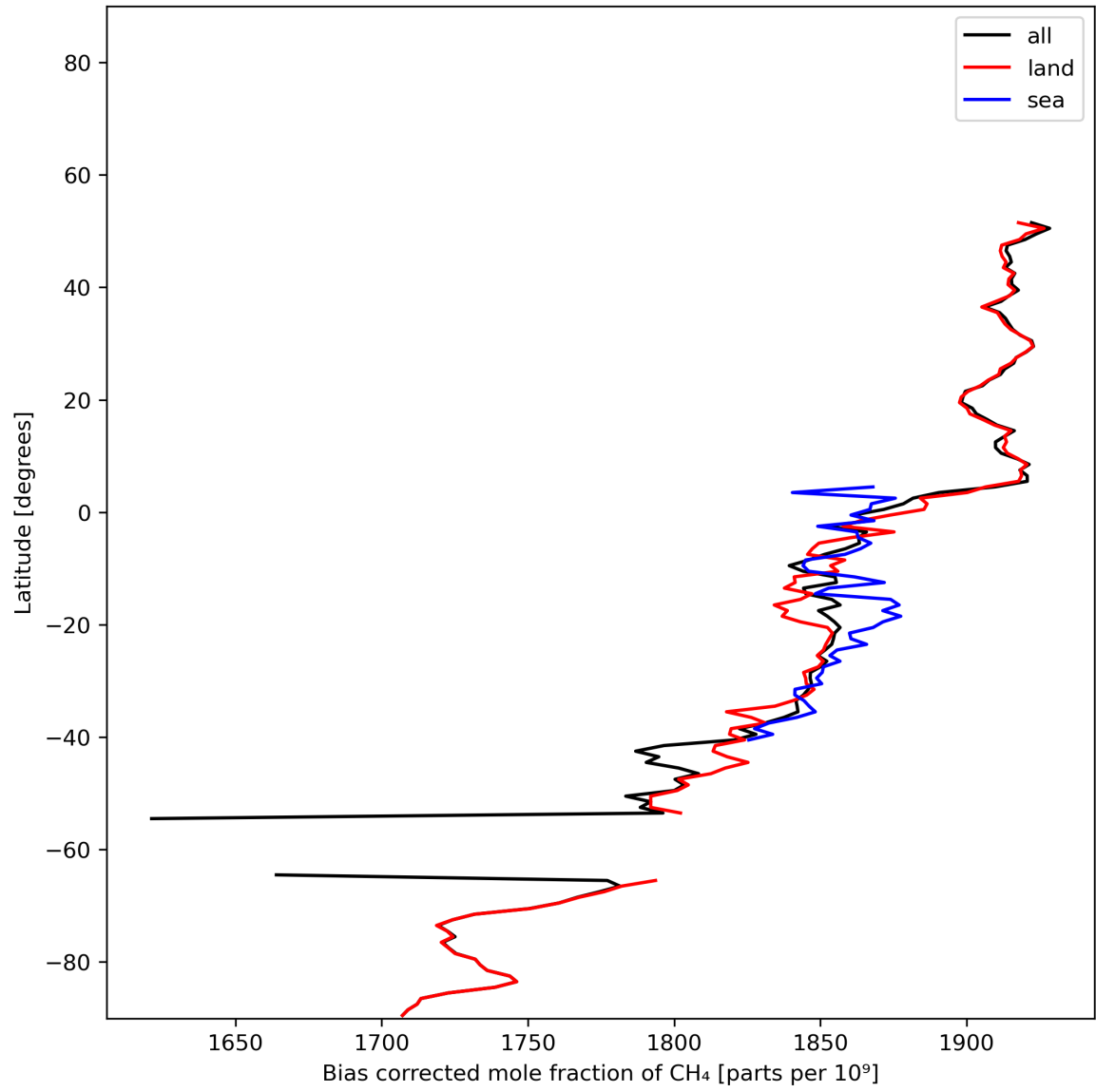
Figure 14: Zonal average of “Bias corrected mole fraction of CH 4 ” for 2023-12-17 to 2023-12-19.
