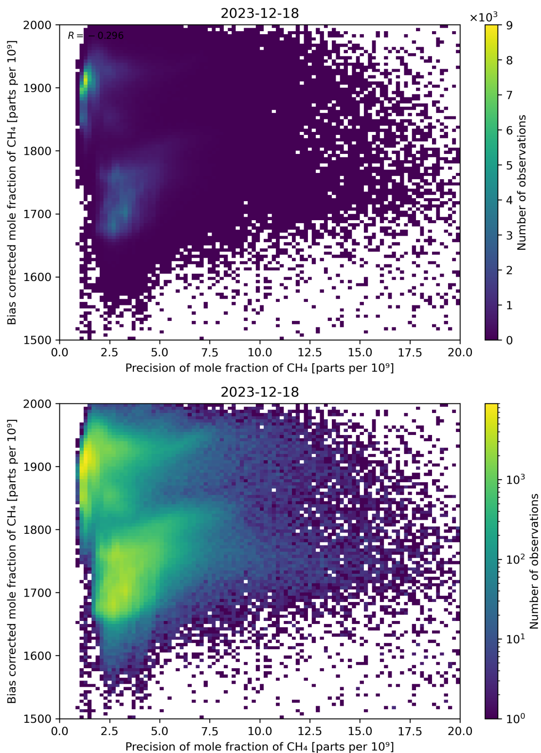
Figure 82: Scatter density plot of “Precision of mole fraction of CH 4 ” against “Bias corrected mole fraction of CH 4 ” for 2023-12-17 to 2023-12-19.
