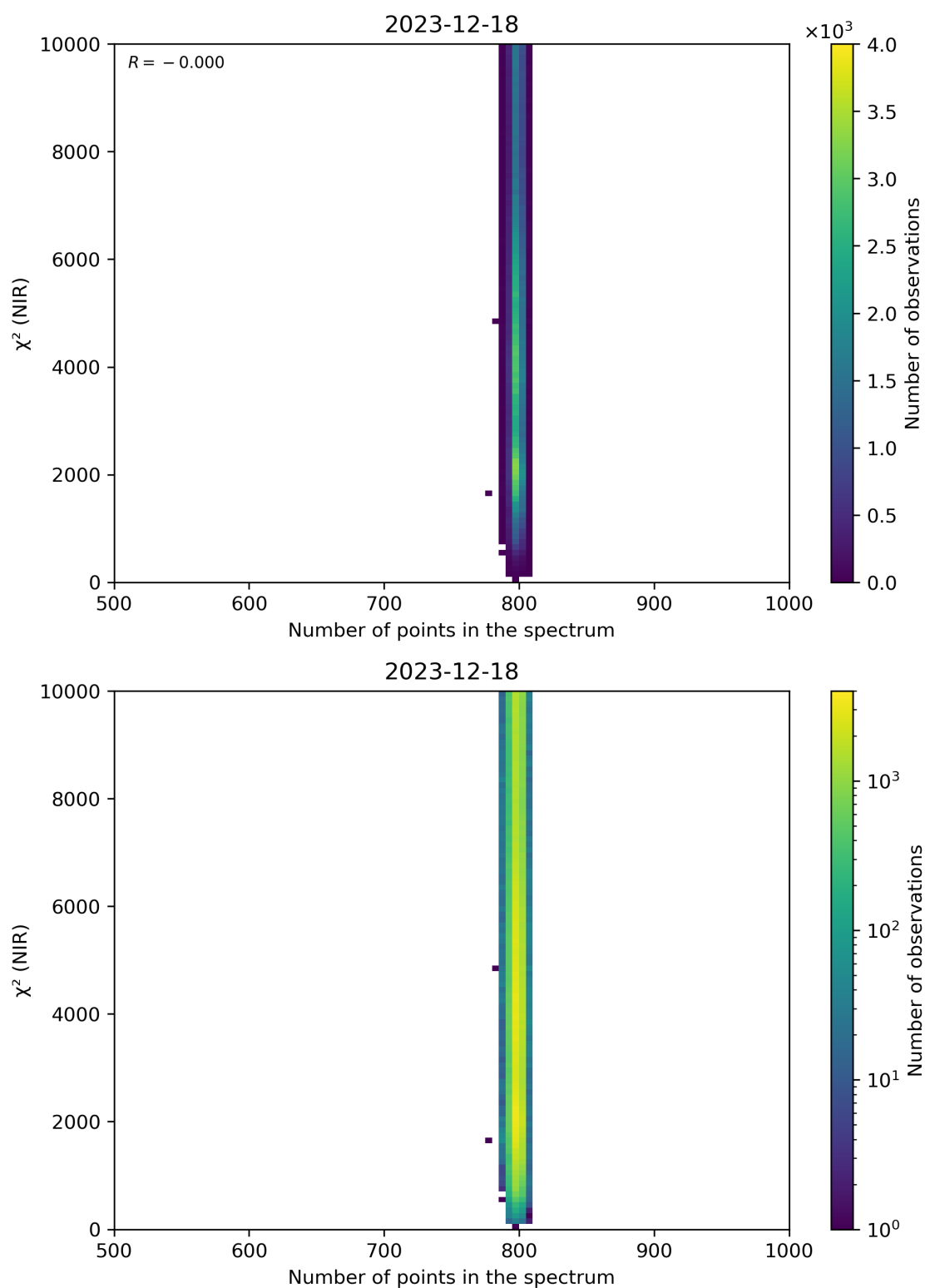
Figure 88: Scatter density plot of “Number of points in the spectrum” against “ \chi^2 (NIR)” for 2023-12-17 to 2023-12-19.
