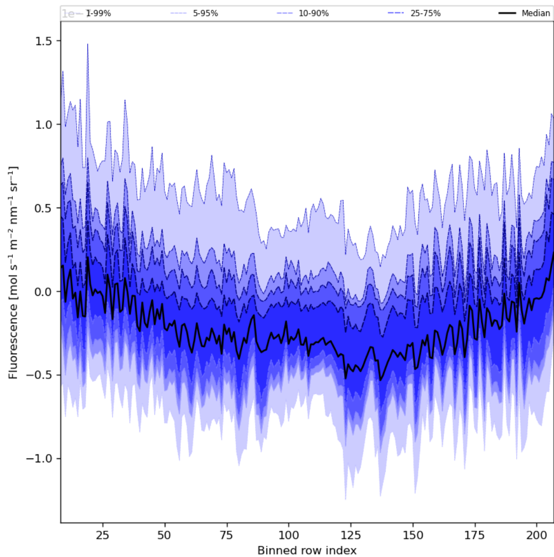
Figure 43: Along track statistics of “Fluorescence” for 2023-12-17 to 2023-12-19
