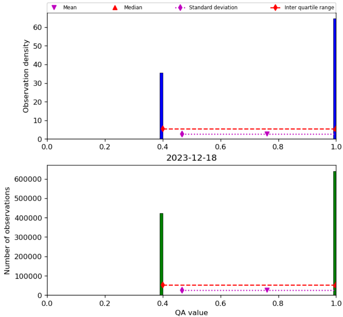
Figure 22: Histogram of “QA value” for 2023-12-17 to 2023-12-19
