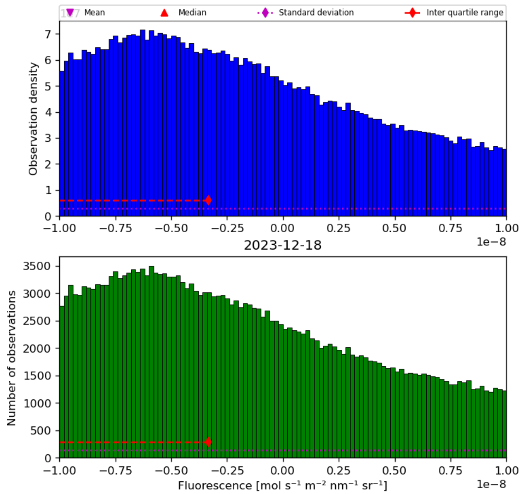
Figure 32: Histogram of “Fluorescence” for 2023-12-17 to 2023-12-19
