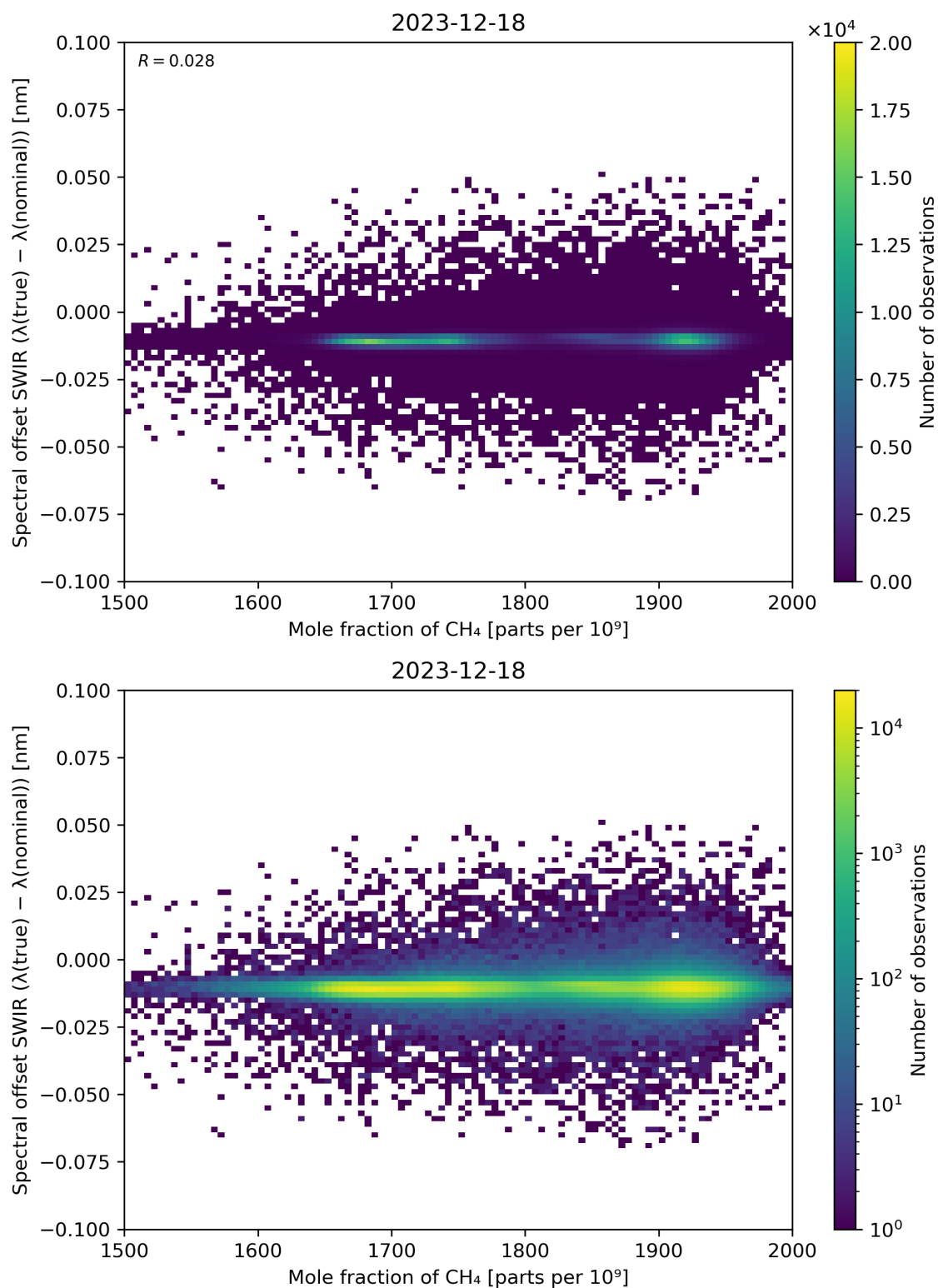
Figure 86: Scatter density plot of “Mole fraction of CH 4 ” against “Spectral offset SWIR ( \lambda(\text{true}) - \lambda(\text{nominal}) )” for 2023-12-17 to 2023-12-19.
