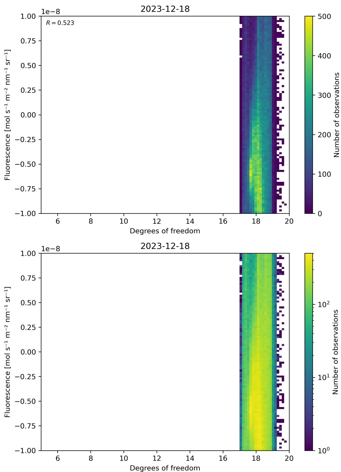
Figure 51: Scatter density plot of “Degrees of freedom” against “Fluorescence” for 2023-12-17 to 2023-12-19.
