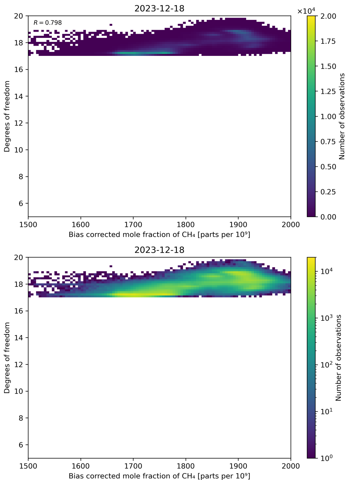
Figure 65: Scatter density plot of “Bias corrected mole fraction of CH 4 ” against “Degrees of freedom” for 2023-12-17 to 2023-12-19.
