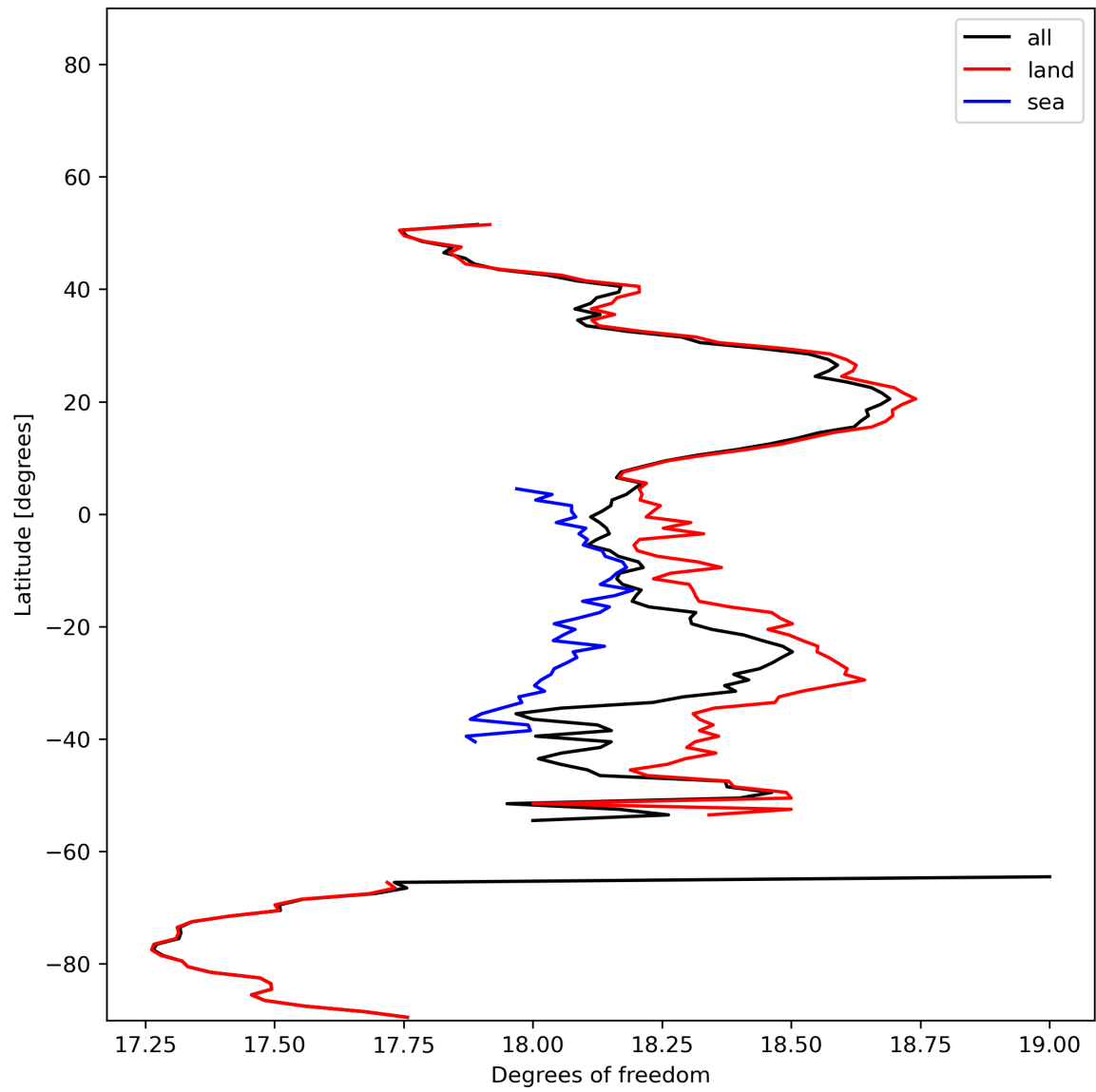
Figure 19: Zonal average of “Degrees of freedom” for 2023-12-17 to 2023-12-19.
