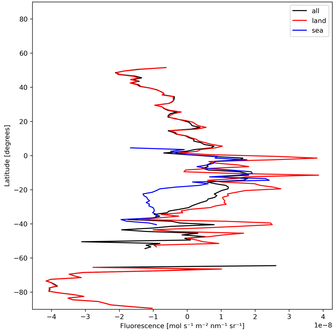
Figure 21: Zonal average of “Fluorescence” for 2023-12-17 to 2023-12-19.
