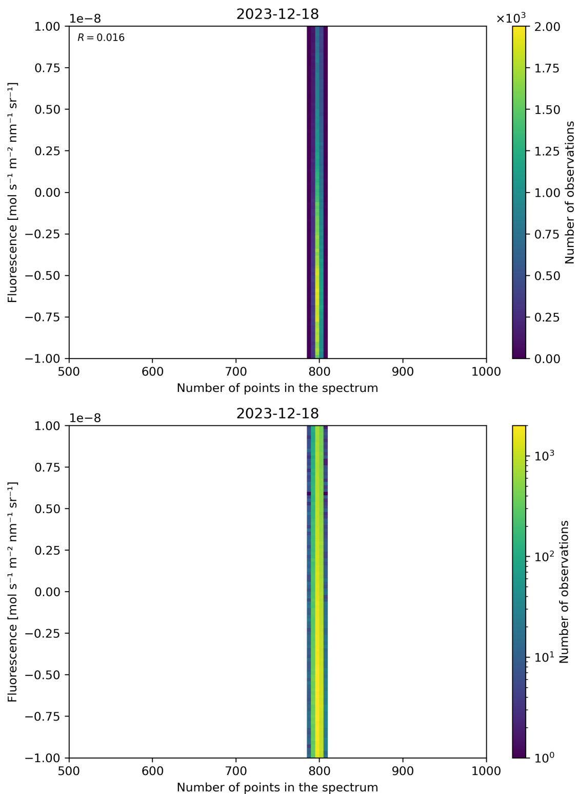
Figure 91: Scatter density plot of “Number of points in the spectrum” against “Fluorescence” for 2023-12-17 to 2023-12-19.
