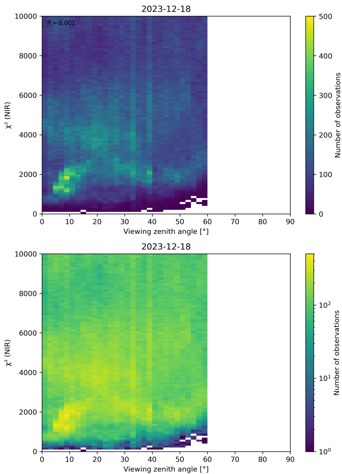
Figure 105: Scatter density plot of “Viewing zenith angle” against “ \chi^2 (NIR)” for 2023-12-17 to 2023-12-19.
