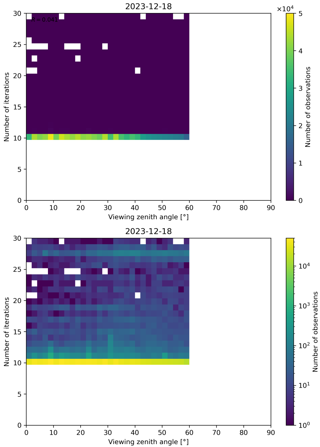
Figure 113: Scatter density plot of “Viewing zenith angle” against “Number of iterations” for 2023-12-17 to 2023-12-19.
