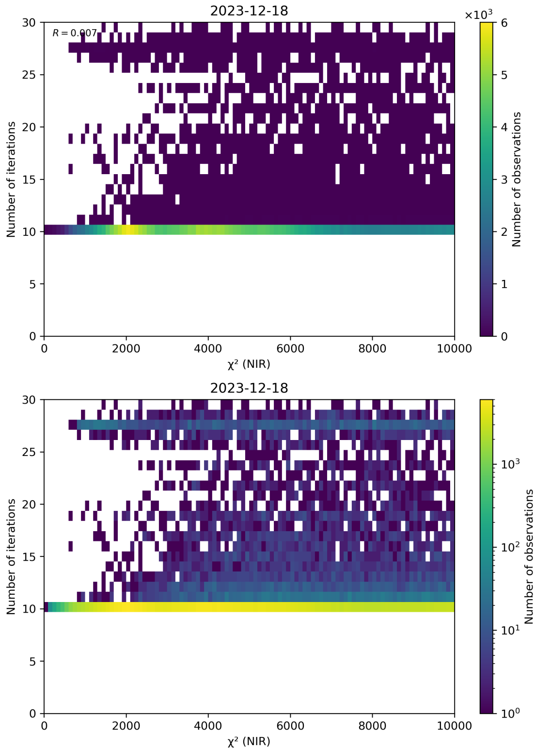
Figure 46: Scatter density plot of “ \chi^2 (NIR)” against “Number of iterations” for 2023-12-17 to 2023-12-19.
