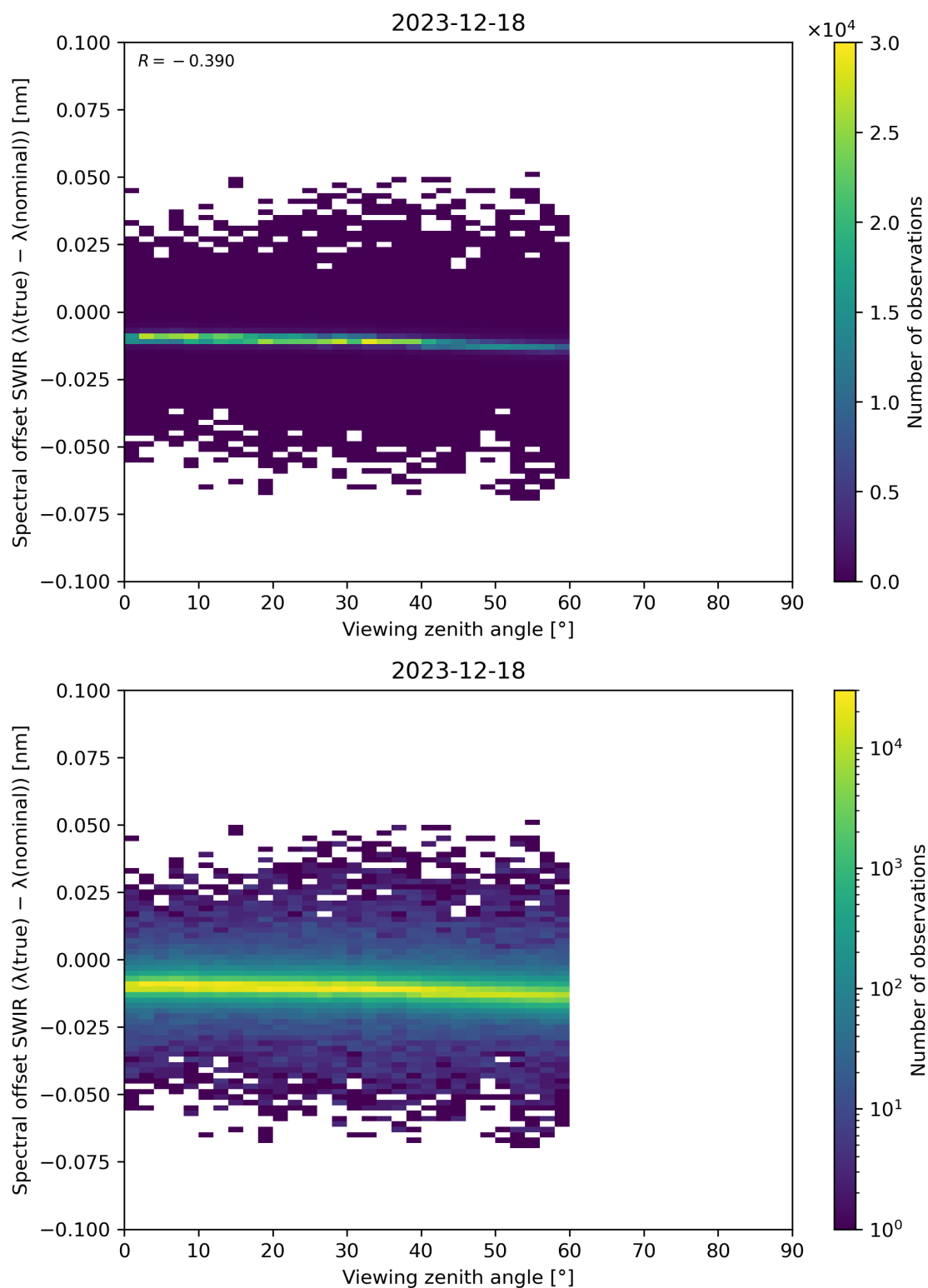
Figure 116: Scatter density plot of “Viewing zenith angle” against “Spectral offset SWIR ( \lambda(\text{true}) - \lambda(\text{nominal}) )” for 2023-12-17 to 2023-12-19.
