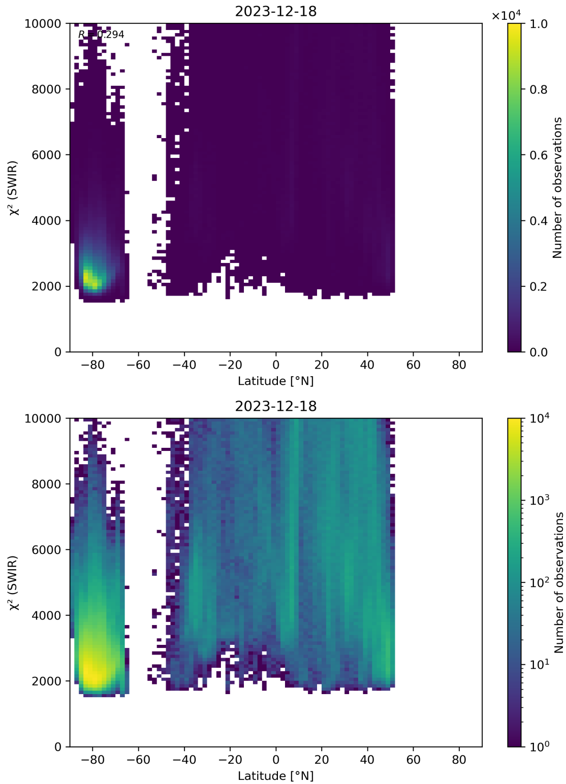
Figure 54: Scatter density plot of “Latitude” against “ \chi^2 (SWIR)” for 2023-12-17 to 2023-12-19.
