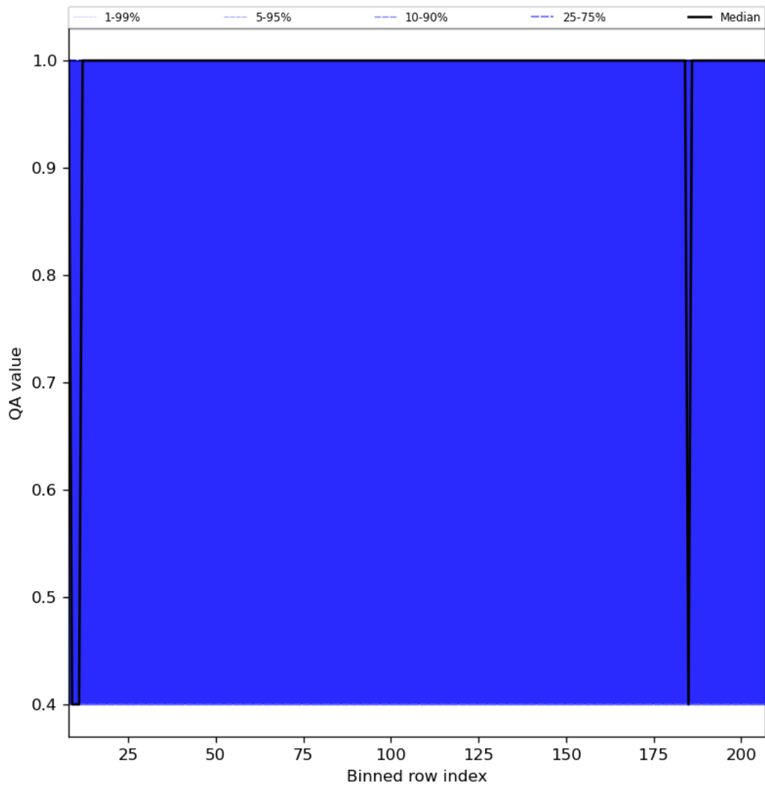
Figure 33: Along track statistics of “QA value” for 2023-12-17 to 2023-12-19
