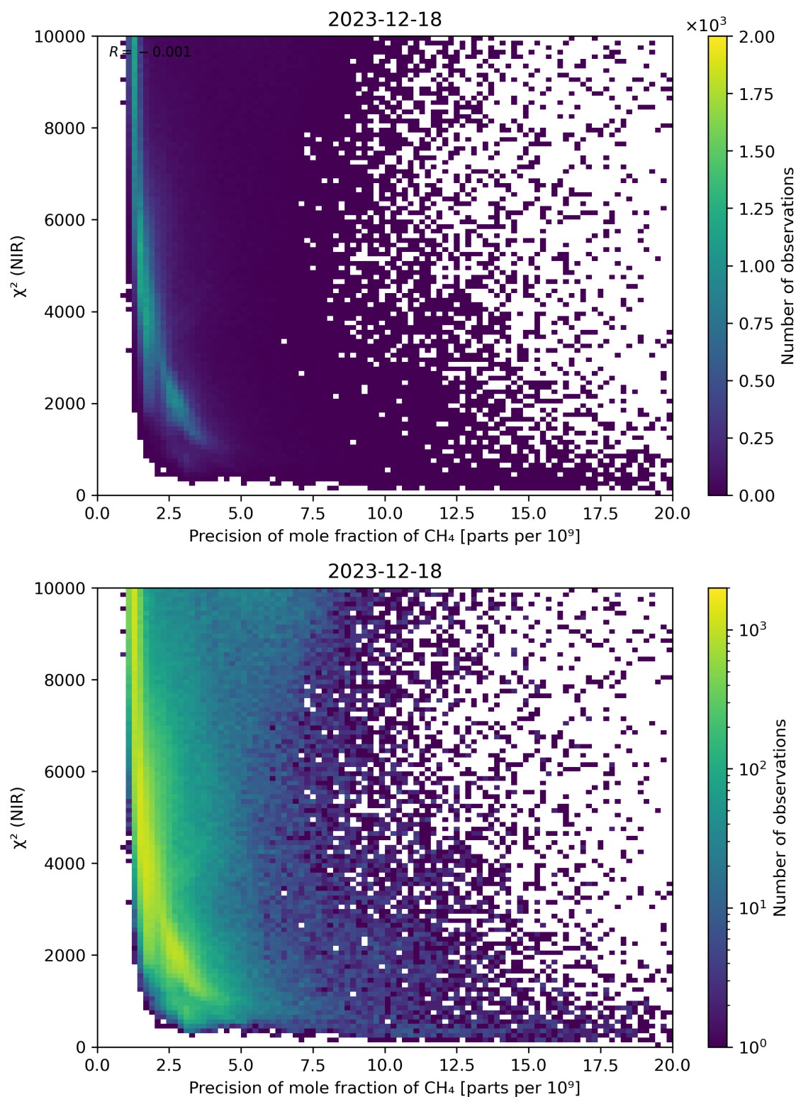
Figure 78: Scatter density plot of “Precision of mole fraction of CH 4 ” against “ \chi^2 (NIR)” for 2023-12-17 to 2023-12-19.
