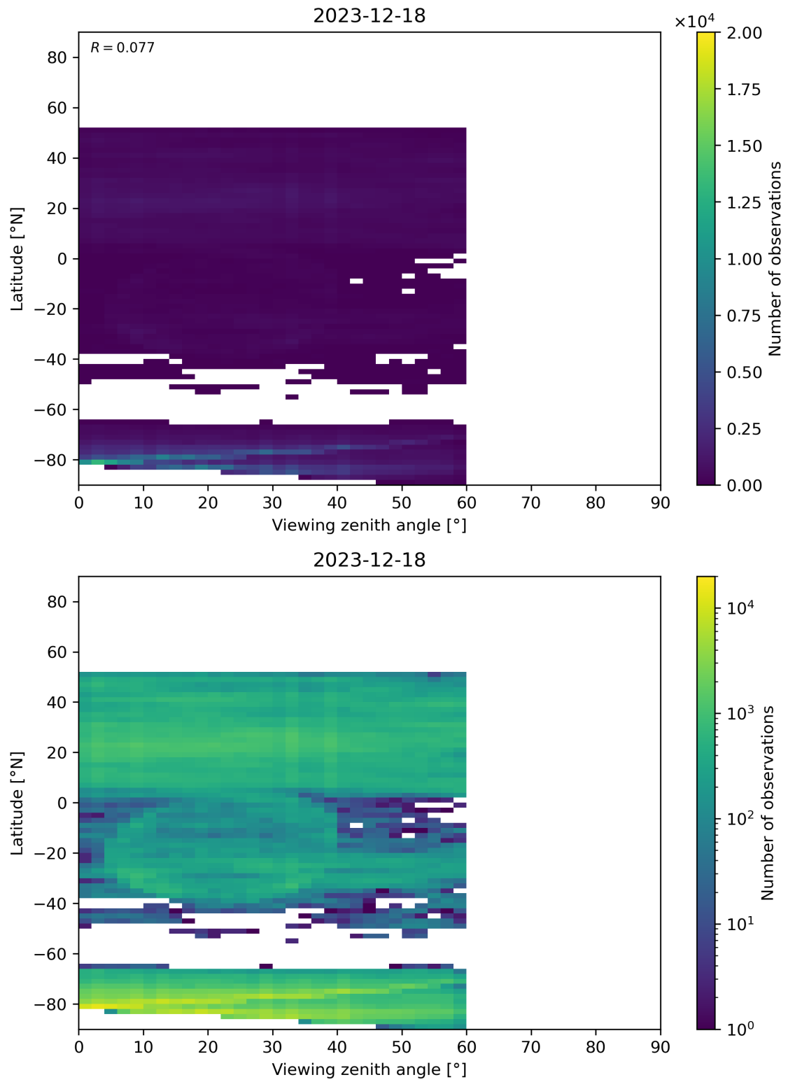
Figure 109: Scatter density plot of “Viewing zenith angle” against “Latitude” for 2023-12-17 to 2023-12-19.
