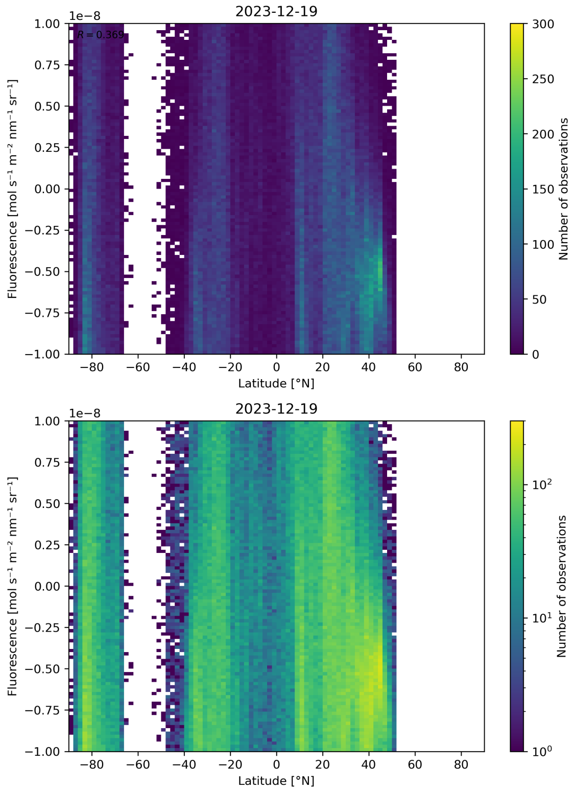
Figure 56: Scatter density plot of “Latitude” against “Fluorescence” for 2023-12-18 to 2023-12-20.
