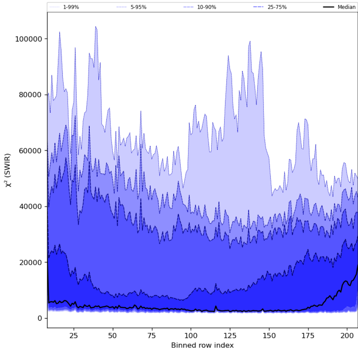
Figure 39: Along track statistics of “ \chi^2 (SWIR)” for 2023-12-18 to 2023-12-20
