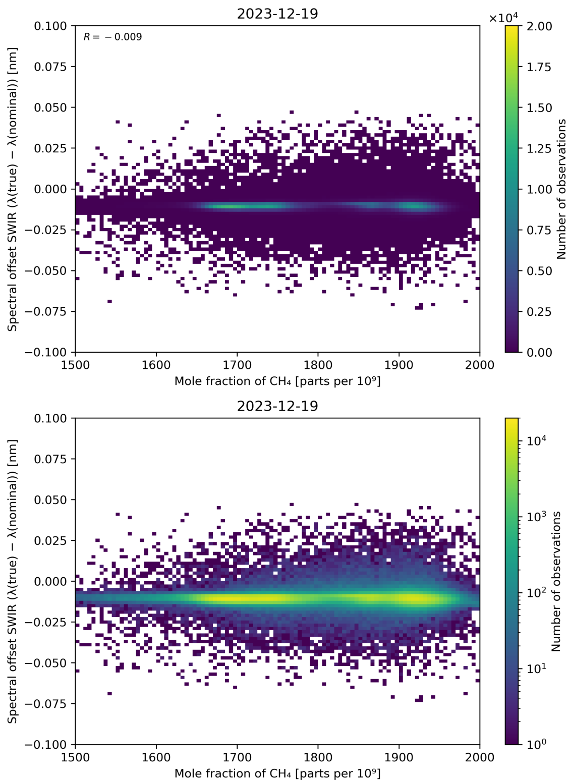
Figure 86: Scatter density plot of “Mole fraction of CH 4 ” against “Spectral offset SWIR ( \lambda(\text{true}) - \lambda(\text{nominal}) )” for 2023-12-18 to 2023-12-20.
