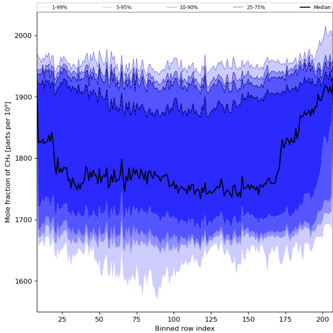
Figure 34: Along track statistics of “Mole fraction of CH 4 ” for 2023-12-18 to 2023-12-20
