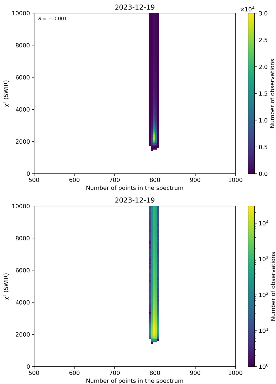
Figure 89: Scatter density plot of “Number of points in the spectrum” against “ \chi^2 (SWIR)” for 2023-12-18 to 2023-12-20.
