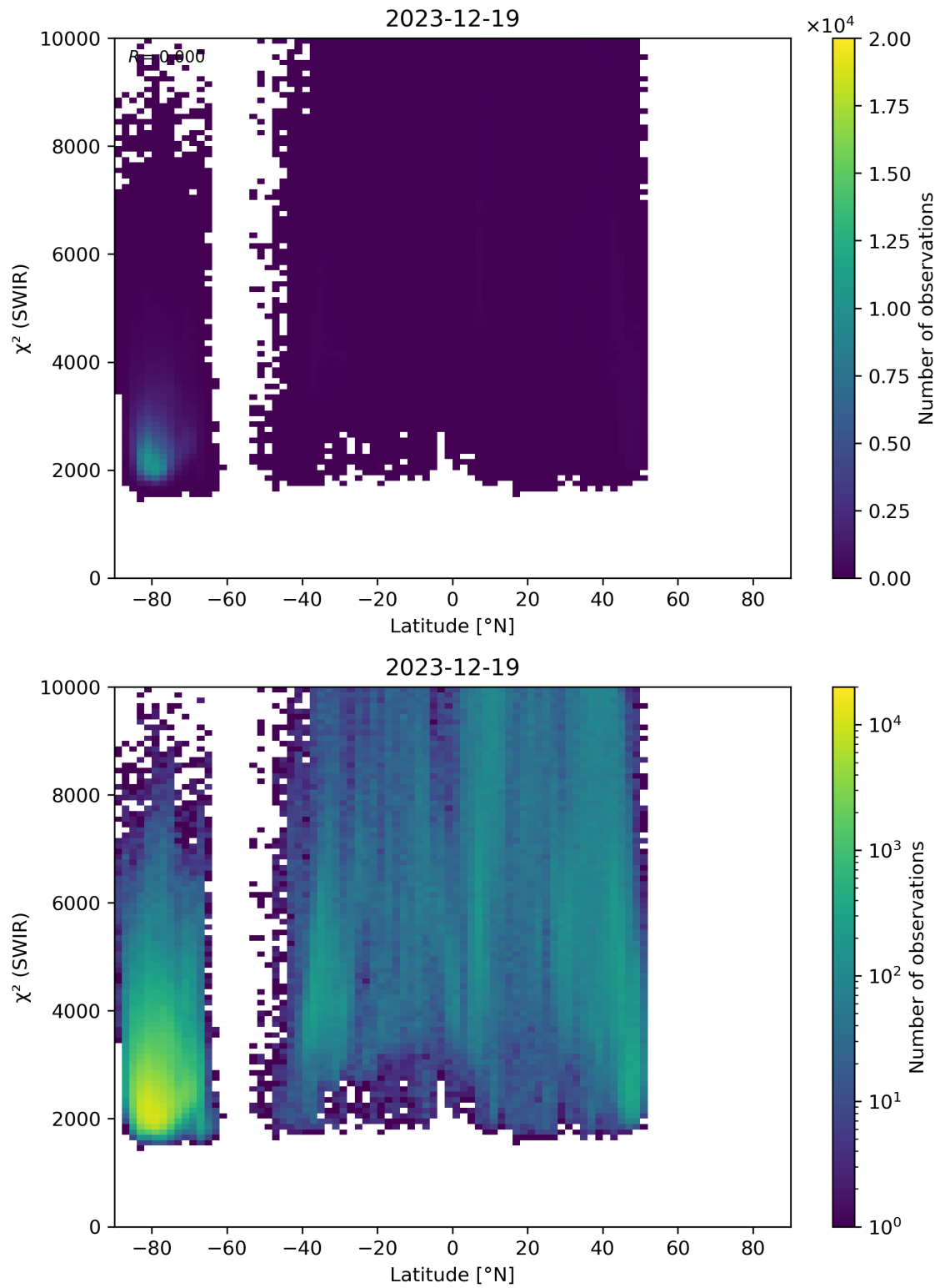
Figure 54: Scatter density plot of “Latitude” against “ \chi^2 (SWIR)” for 2023-12-18 to 2023-12-20.
