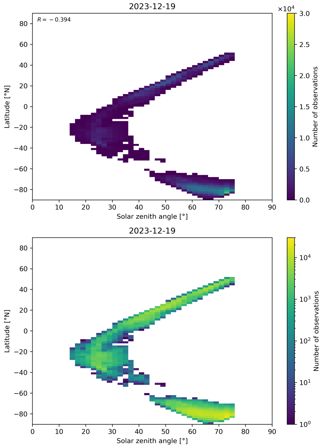
Figure 98: Scatter density plot of “Solar zenith angle” against “Latitude” for 2023-12-18 to 2023-12-20.
