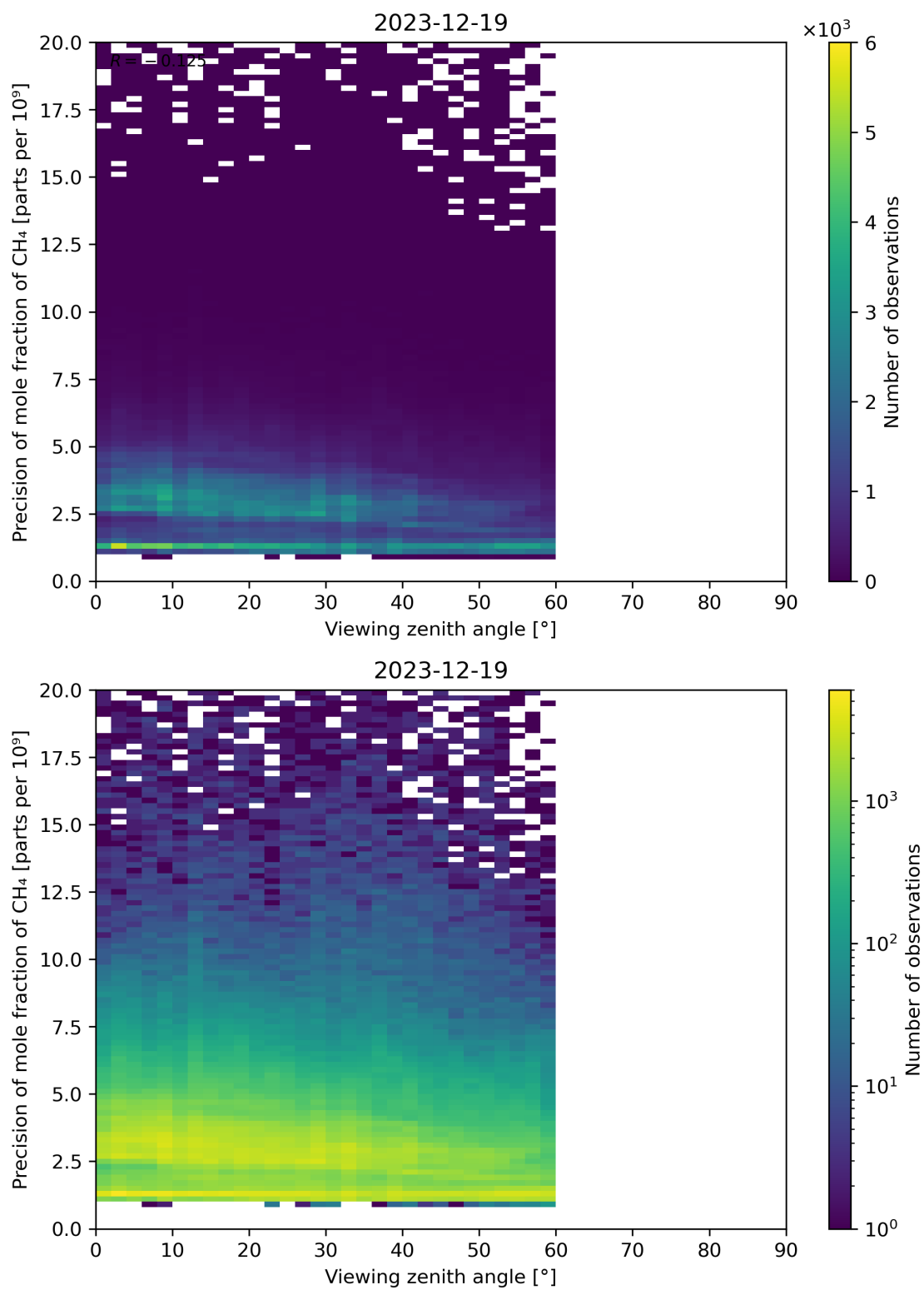
Figure 112: Scatter density plot of “Viewing zenith angle” against “Precision of mole fraction of CH 4 ” for 2023-12-18 to 2023-12-20.
