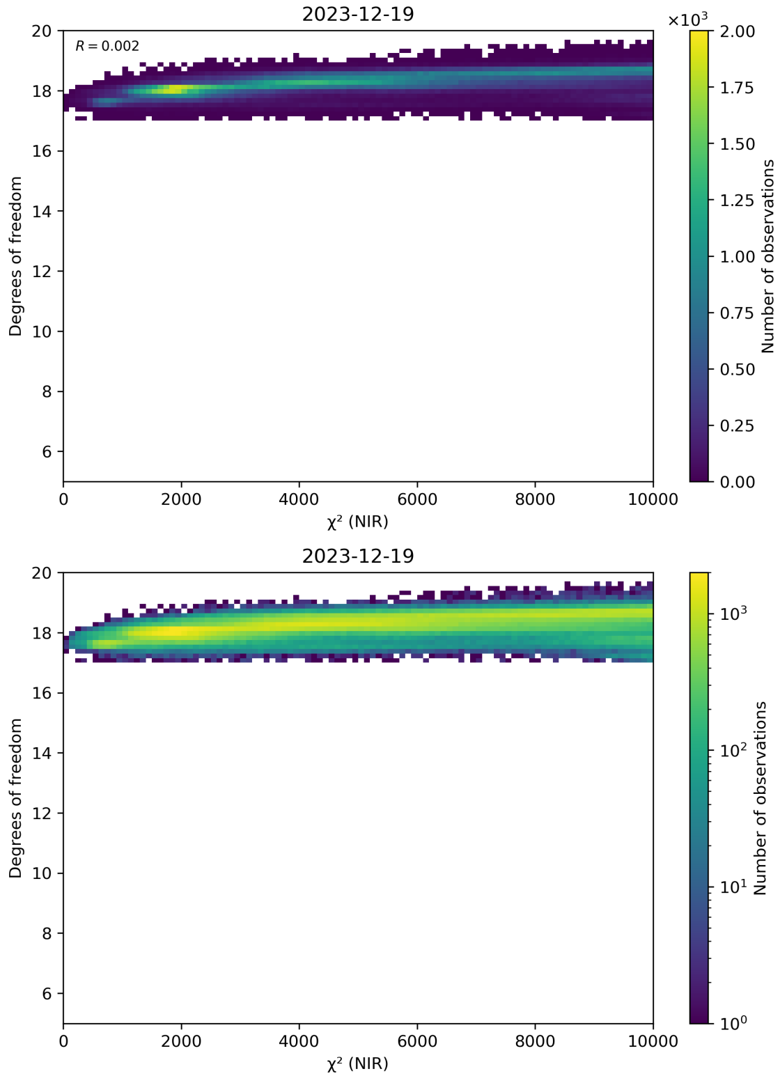
Figure 44: Scatter density plot of “ \chi^2 (NIR)” against “Degrees of freedom” for 2023-12-18 to 2023-12-20.
