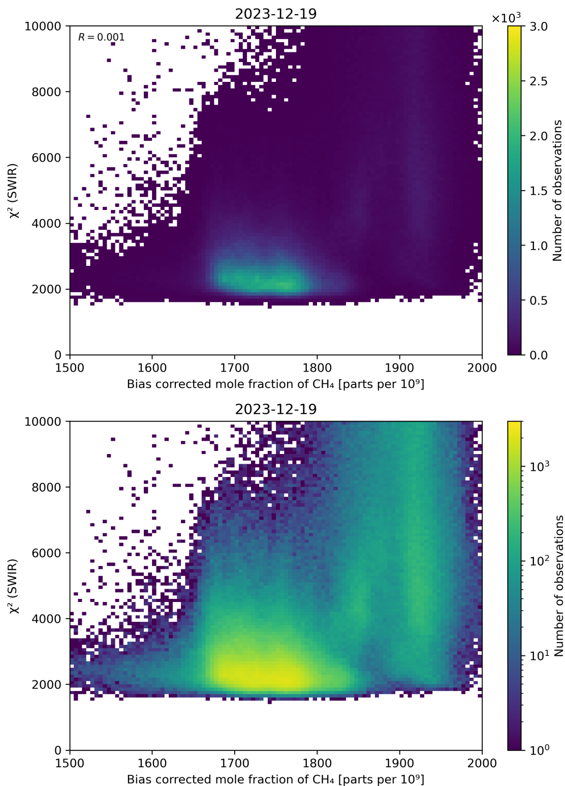
Figure 64: Scatter density plot of “Bias corrected mole fraction of CH 4 ” against “ \chi^2 (SWIR)” for 2023-12-18 to 2023-12-20.
