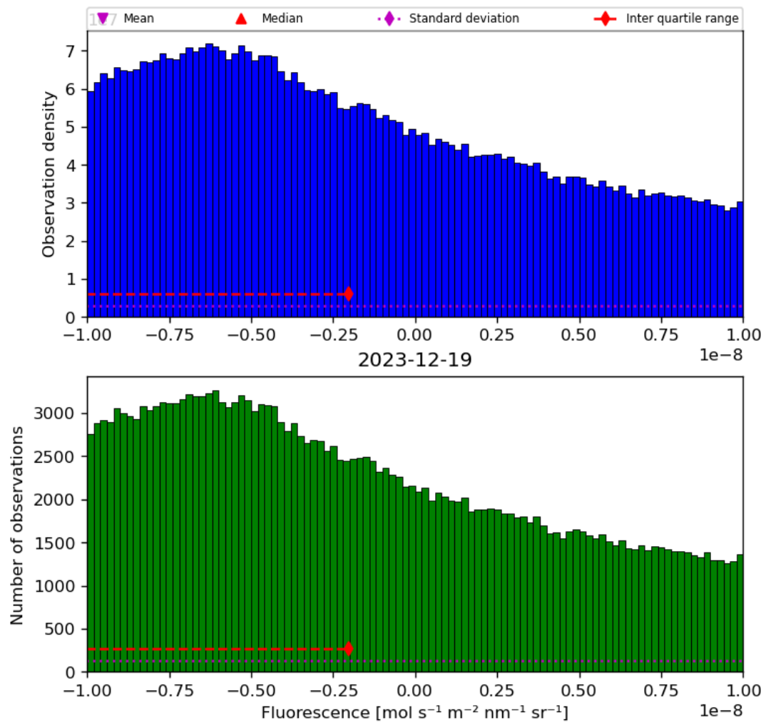
Figure 32: Histogram of “Fluorescence” for 2023-12-18 to 2023-12-20
