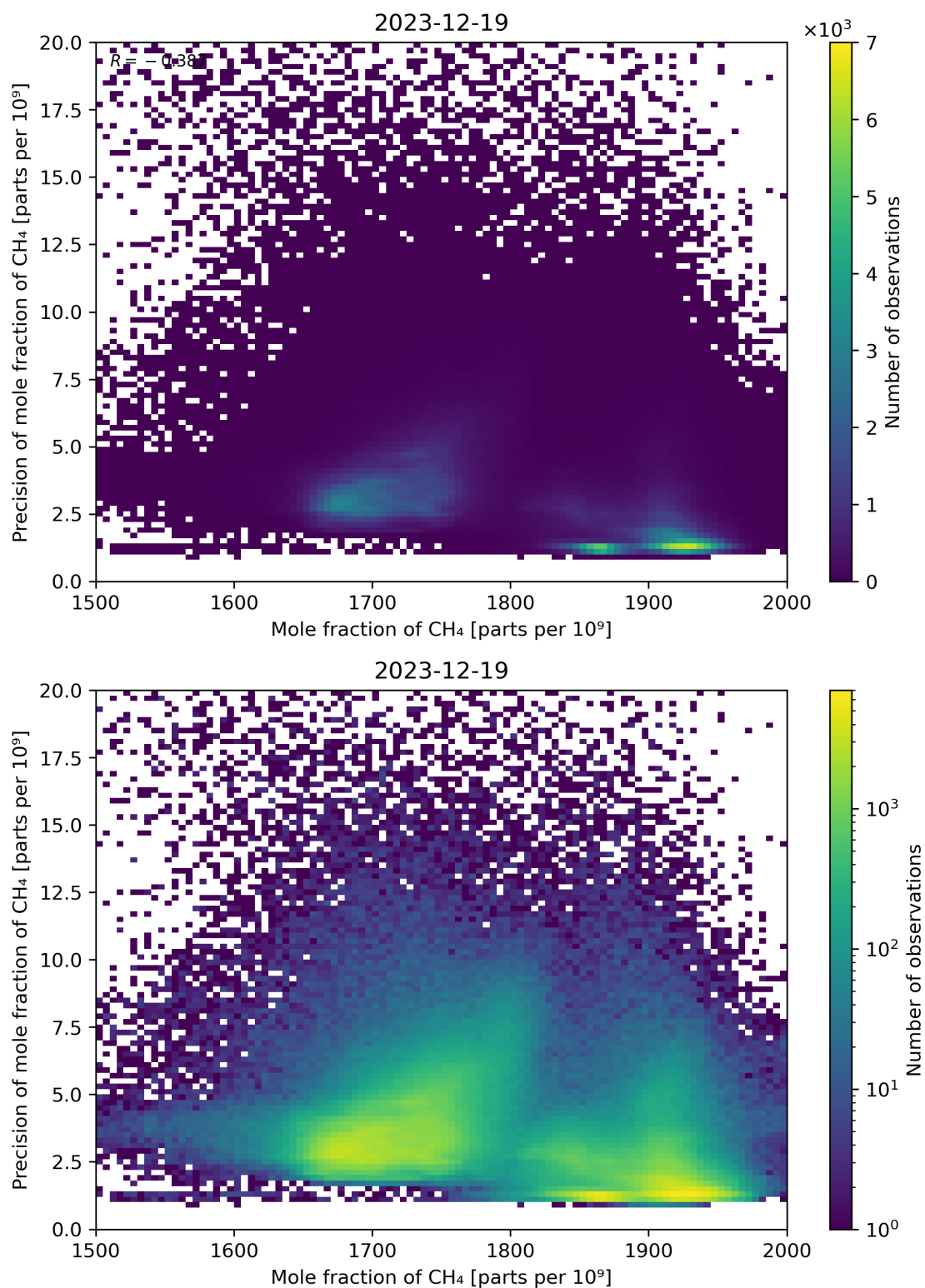
Figure 75: Scatter density plot of “Mole fraction of CH 4 ” against “Precision of mole fraction of CH 4 ” for 2023-12-18 to 2023-12-20.
