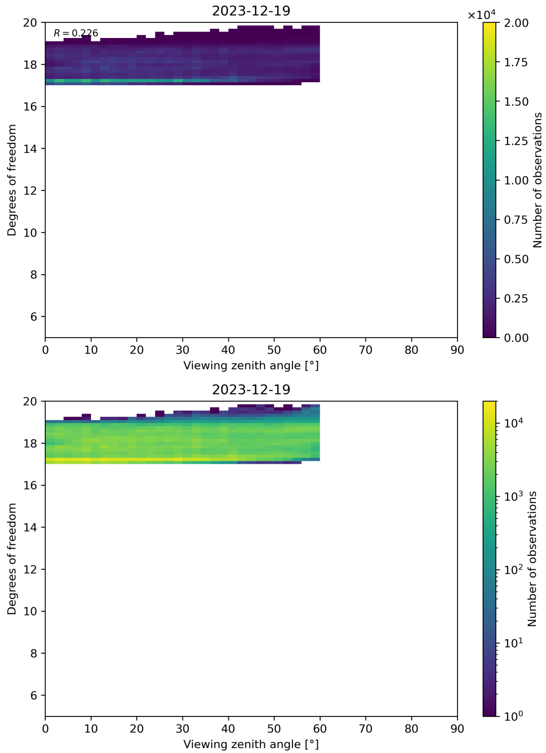
Figure 107: Scatter density plot of “Viewing zenith angle” against “Degrees of freedom” for 2023-12-18 to 2023-12-20.
