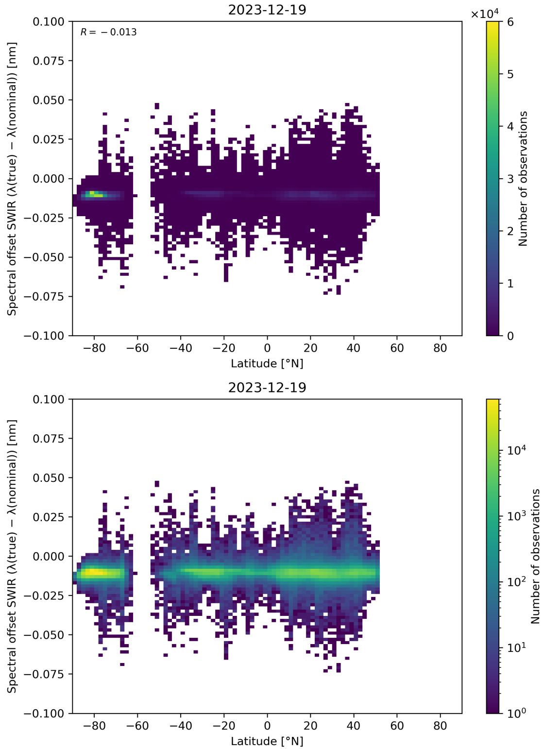
Figure 62: Scatter density plot of “Latitude” against “Spectral offset SWIR ( \lambda(\text{true}) - \lambda(\text{nominal}) )” for 2023-12-18 to 2023-12-20.
