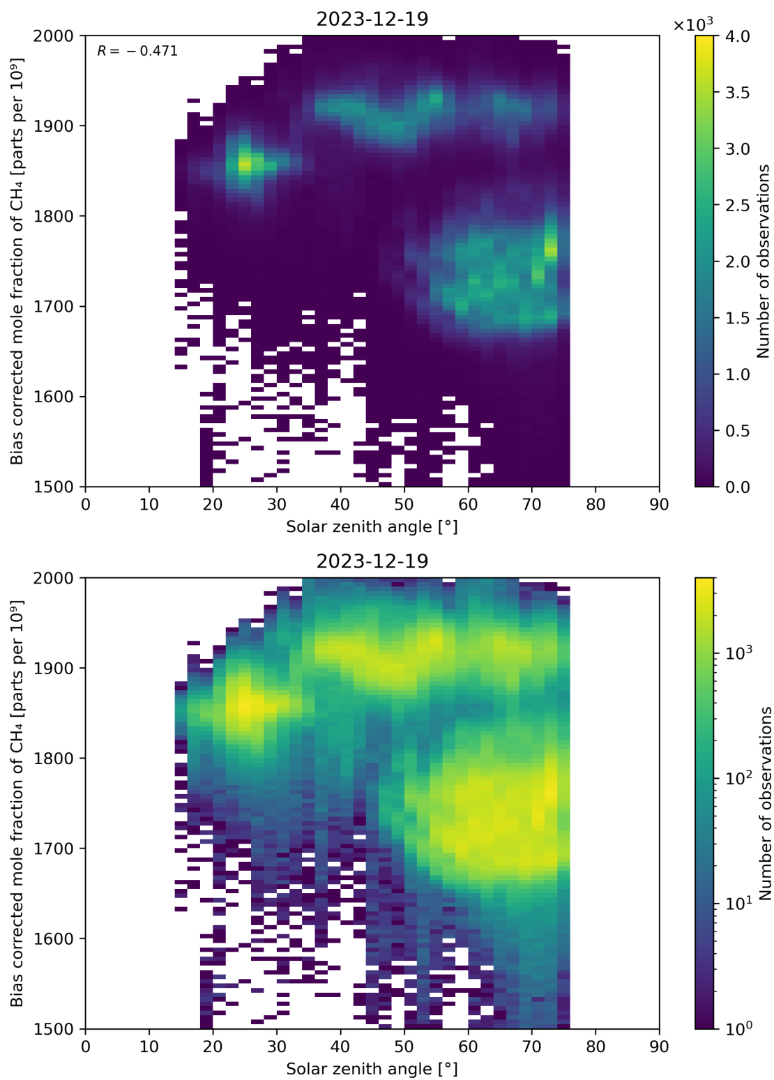
Figure 100: Scatter density plot of “Solar zenith angle” against “Bias corrected mole fraction of CH 4 ” for 2023-12-18 to 2023-12-20.
