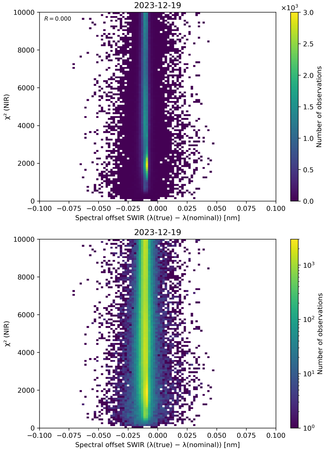
Figure 117: Scatter density plot of “Spectral offset SWIR ( \lambda(\text{true}) - \lambda(\text{nominal}) )” against “ \chi^2 (NIR)” for 2023-12-18 to 2023-12-20.
