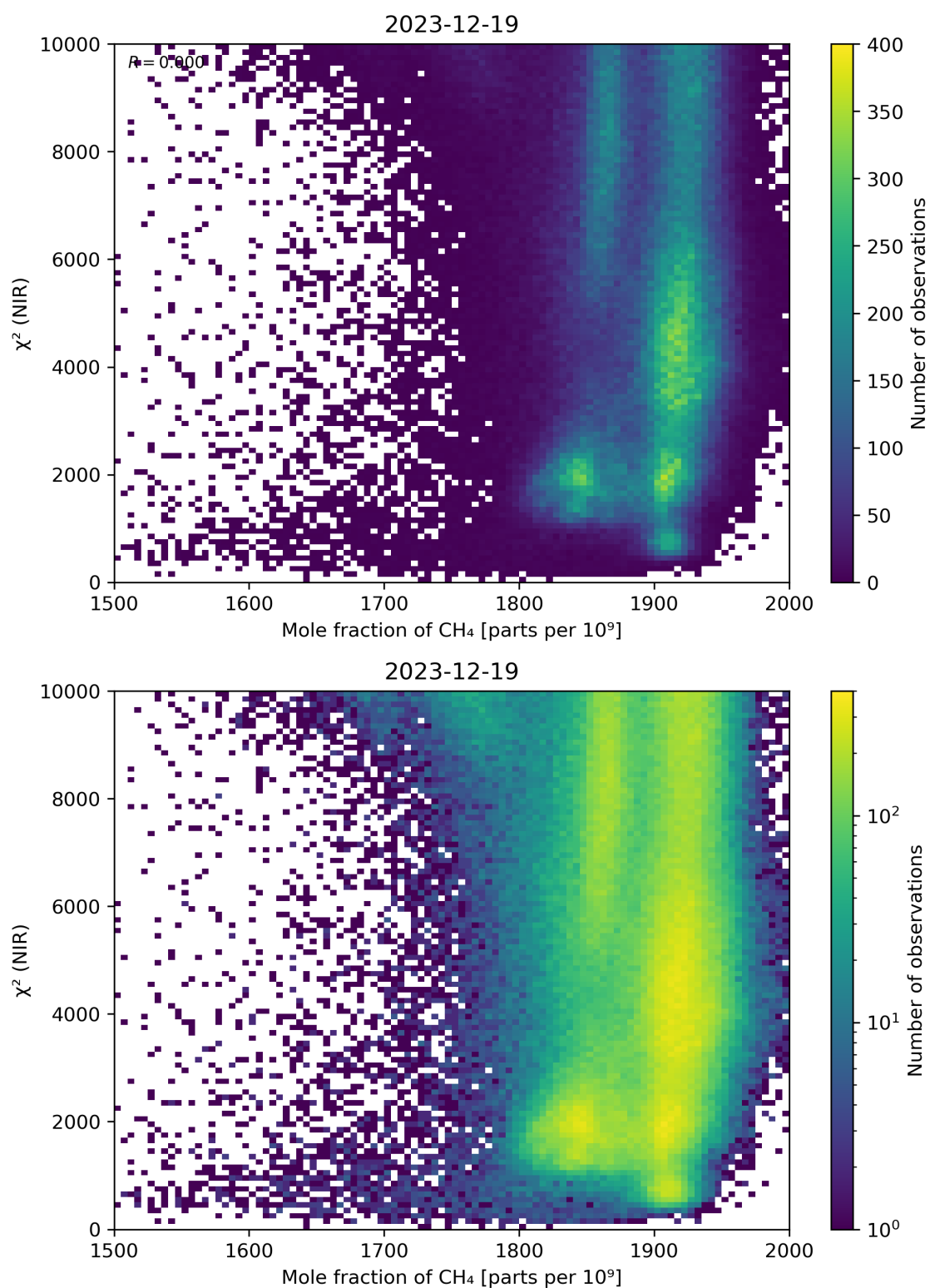
Figure 70: Scatter density plot of “Mole fraction of \text{CH}_4 ” against “ \chi^2 (NIR)” for 2023-12-18 to 2023-12-20.
