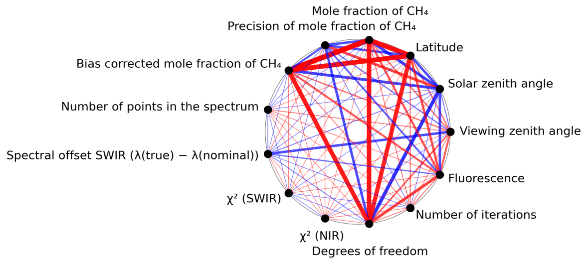
Figure 1: Map of correlation graph for 2023-12-18 to 2023-12-20.
