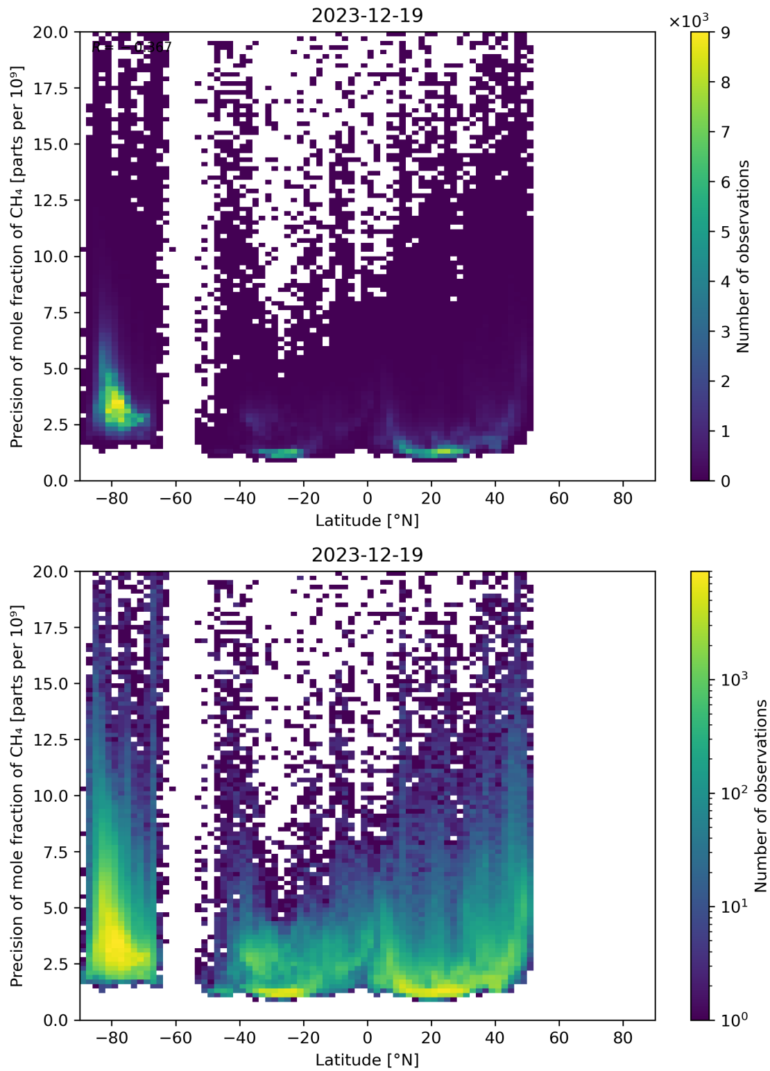
Figure 59: Scatter density plot of “Latitude” against “Precision of mole fraction of CH 4 ” for 2023-12-18 to 2023-12-20.
