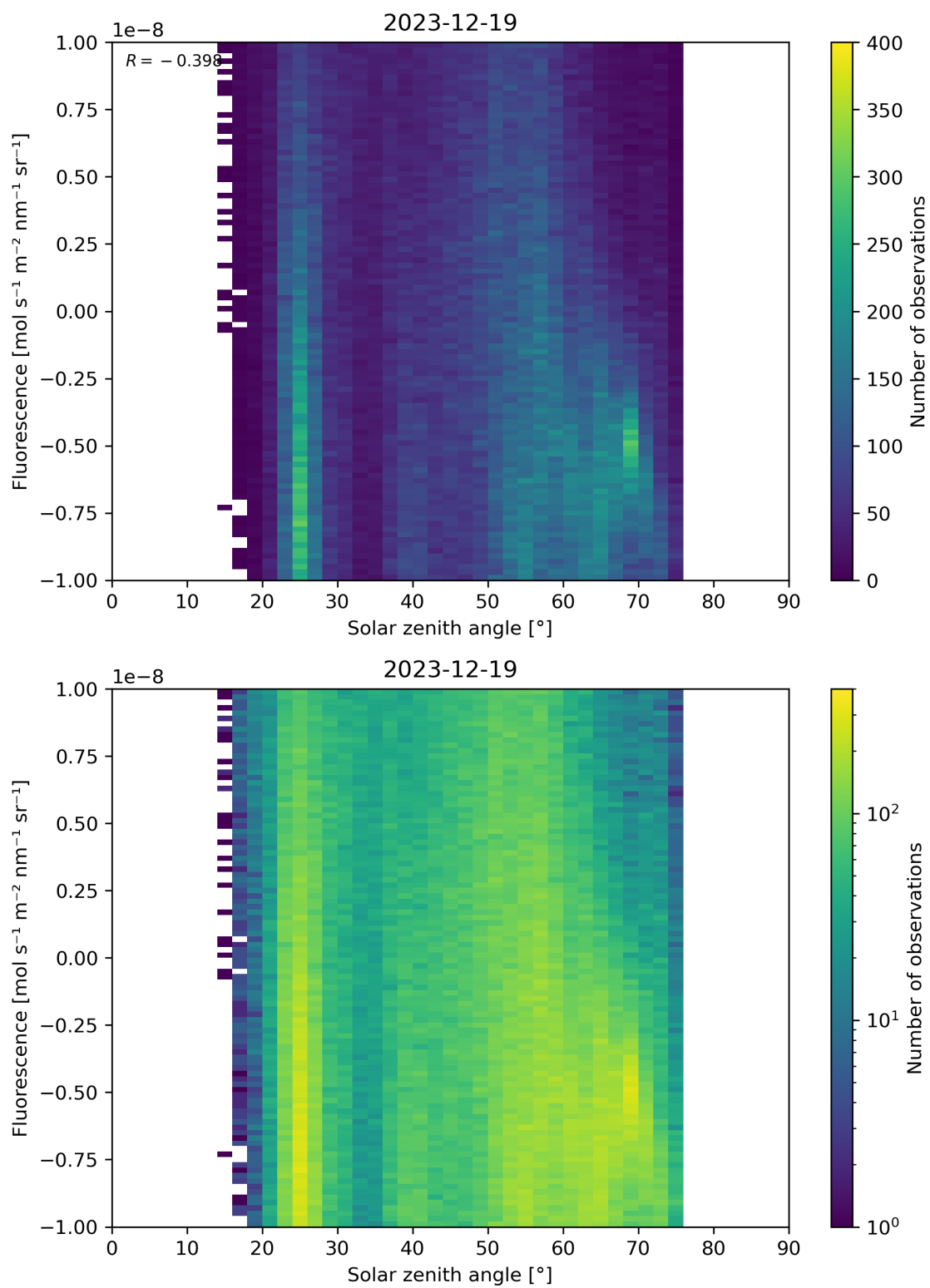
Figure 97: Scatter density plot of “Solar zenith angle” against “Fluorescence” for 2023-12-18 to 2023-12-20.
