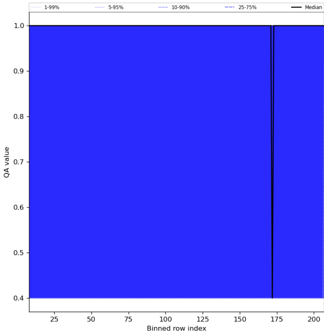
Figure 33: Along track statistics of “QA value” for 2023-12-18 to 2023-12-20
