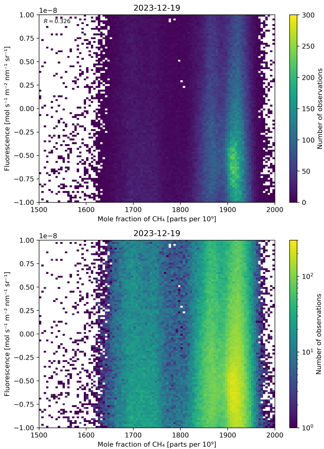
Figure 73: Scatter density plot of “Mole fraction of \text{CH}_4 ” against “Fluorescence” for 2023-12-18 to 2023-12-20.
