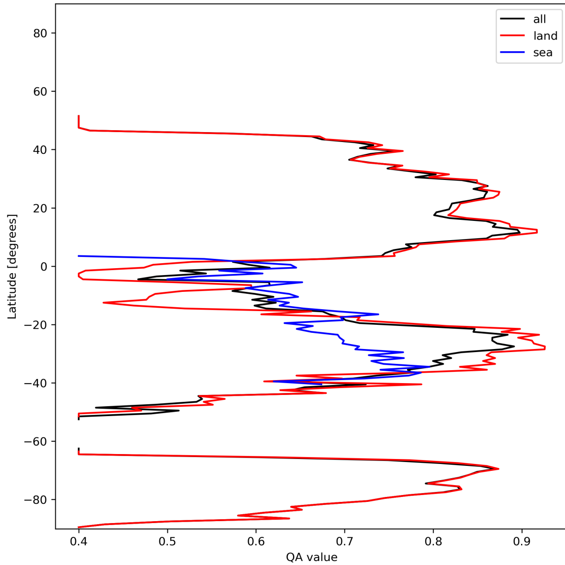
Figure 11: Zonal average of “QA value” for 2023-12-18 to 2023-12-20.
