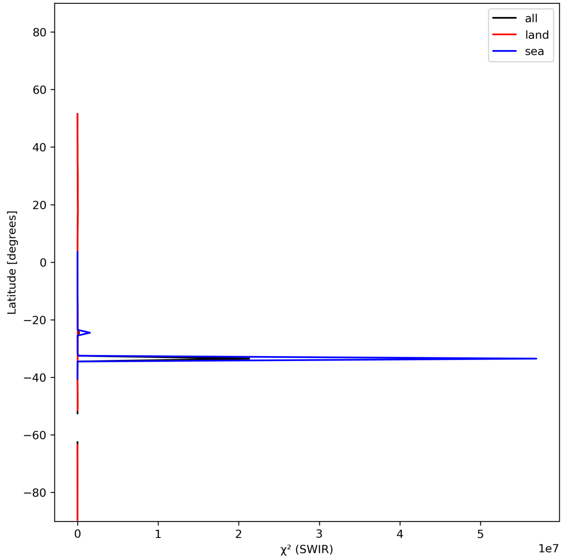
Figure 17: Zonal average of “ \chi^2 (SWIR)” for 2023-12-18 to 2023-12-20.
