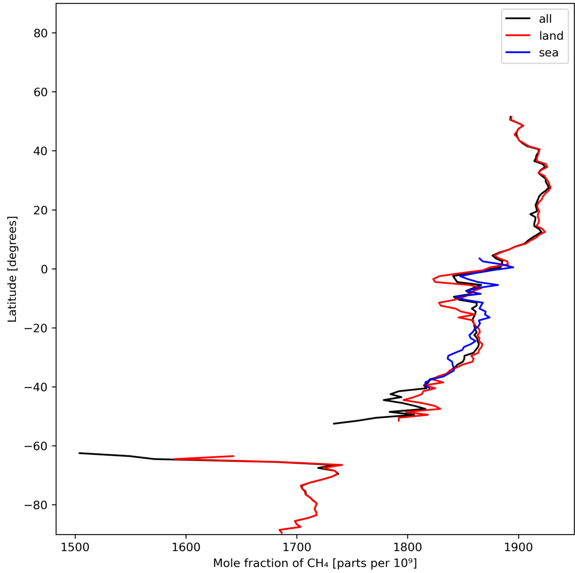
Figure 12: Zonal average of “Mole fraction of \text{CH}_4 ” for 2023-12-18 to 2023-12-20.
