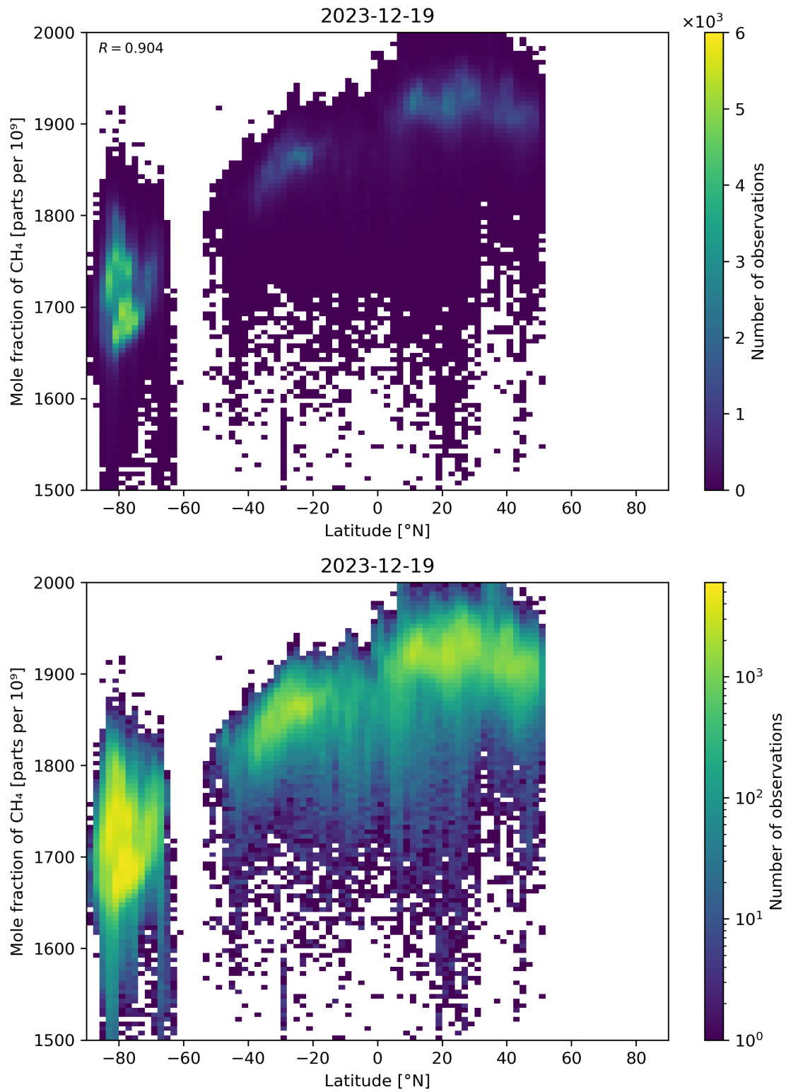
Figure 57: Scatter density plot of “Latitude” against “Mole fraction of \text{CH}_4 ” for 2023-12-18 to 2023-12-20.
