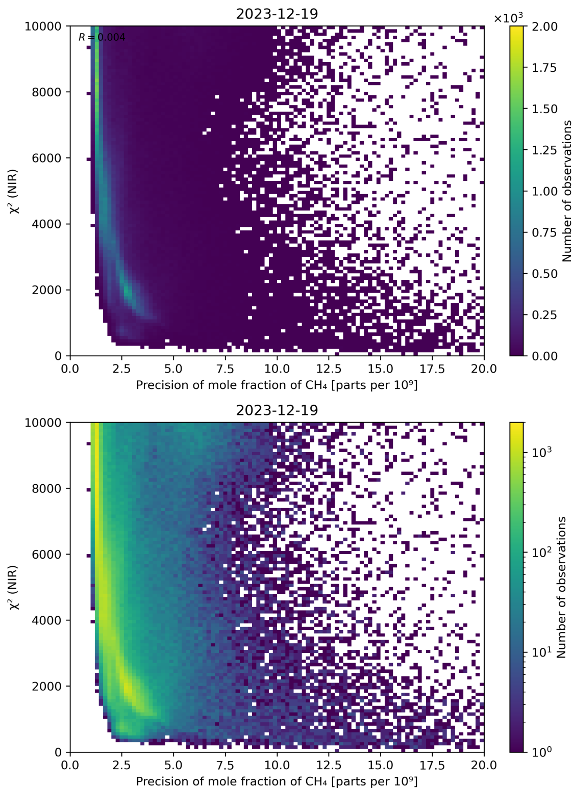
Figure 78: Scatter density plot of “Precision of mole fraction of \text{CH}_4 ” against “ \chi^2 (NIR)” for 2023-12-18 to 2023-12-20.
