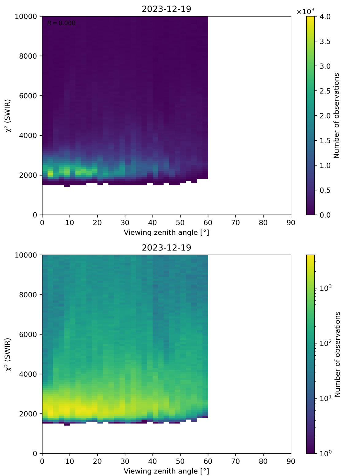
Figure 106: Scatter density plot of “Viewing zenith angle” against “ \chi^2 (SWIR)” for 2023-12-18 to 2023-12-20.
