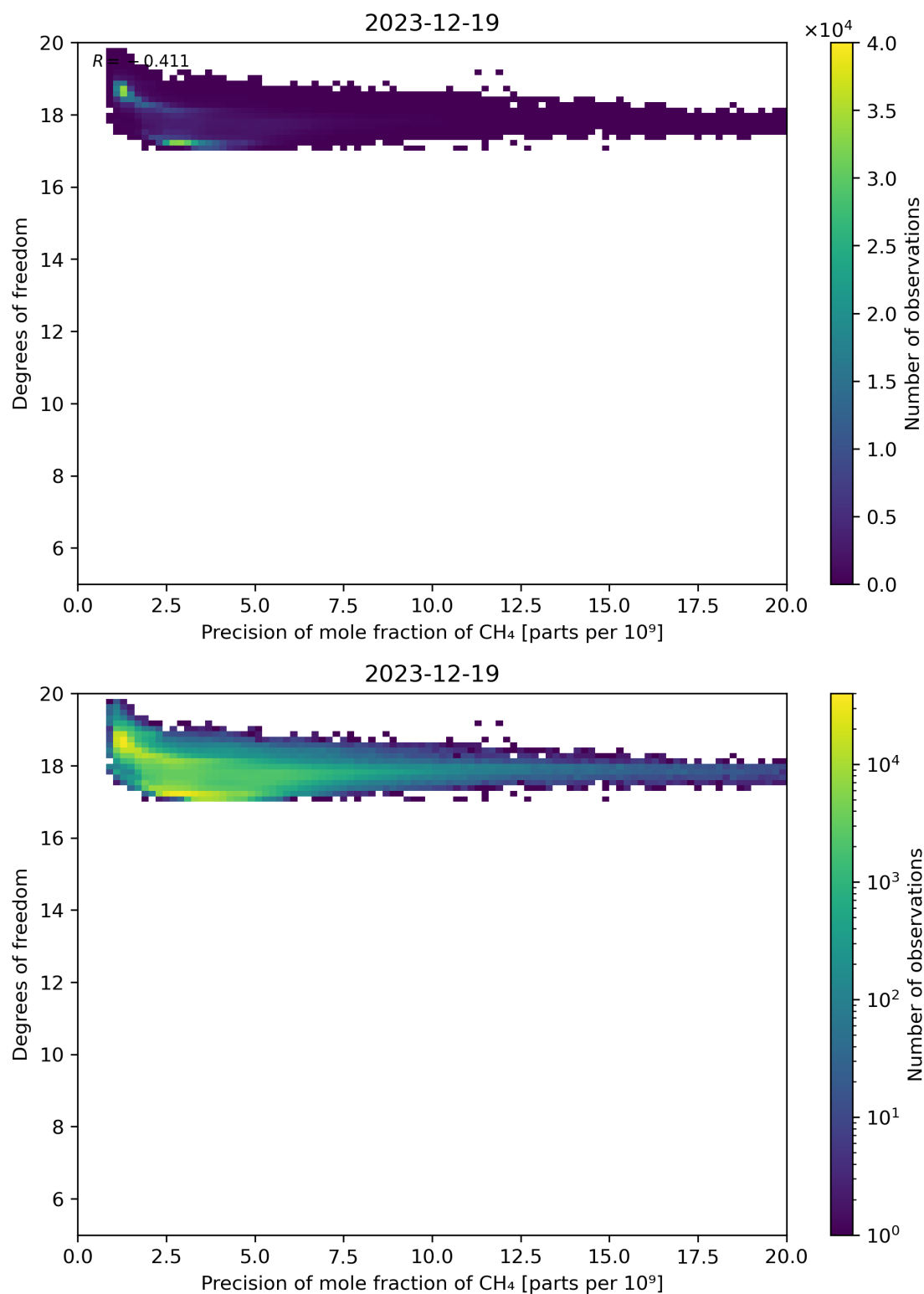
Figure 80: Scatter density plot of “Precision of mole fraction of CH 4 ” against “Degrees of freedom” for 2023-12-18 to 2023-12-20.
