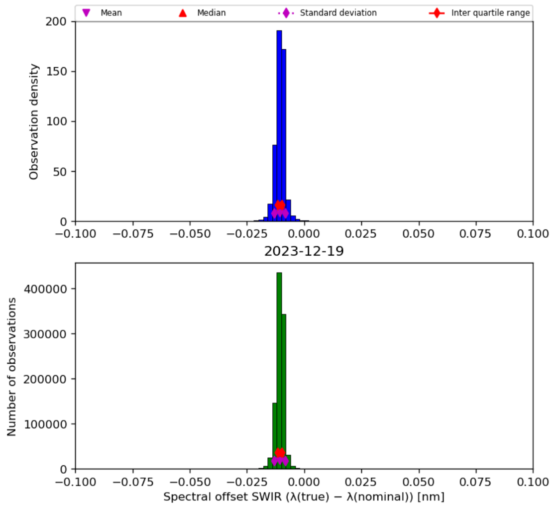
Figure 27: Histogram of “Spectral offset SWIR ( \lambda(\text{true}) - \lambda(\text{nominal}) )” for 2023-12-18 to 2023-12-20
