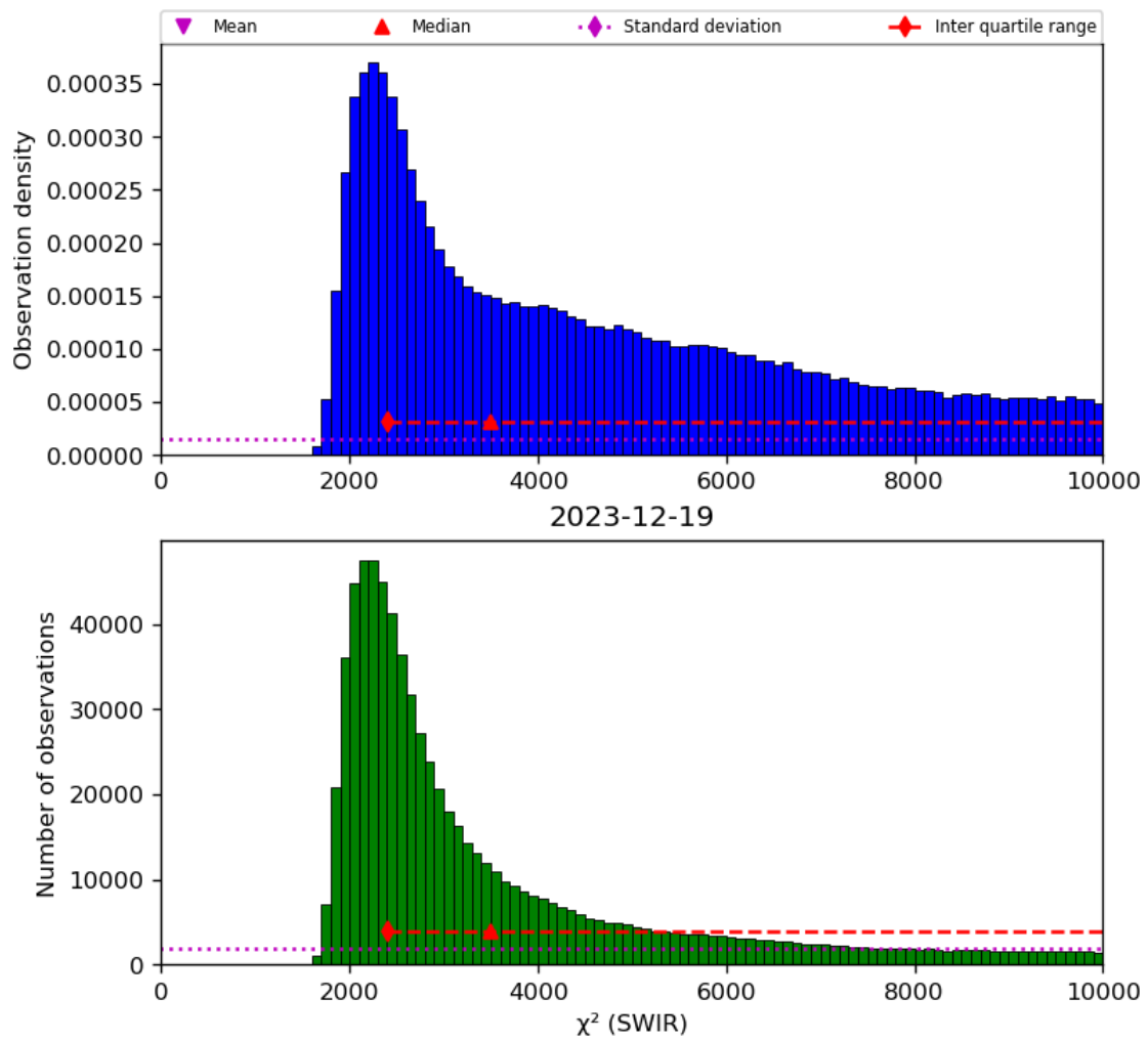
Figure 28: Histogram of “ \chi^2 (SWIR)” for 2023-12-18 to 2023-12-20
