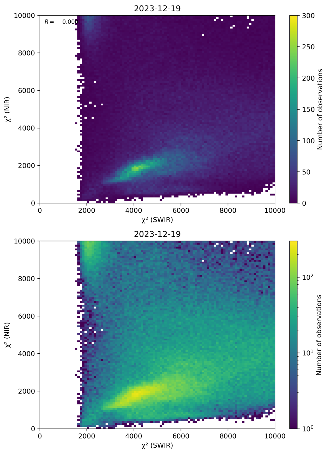
Figure 47: Scatter density plot of “ \chi^2 (SWIR)” against “ \chi^2 (NIR)” for 2023-12-18 to 2023-12-20.
