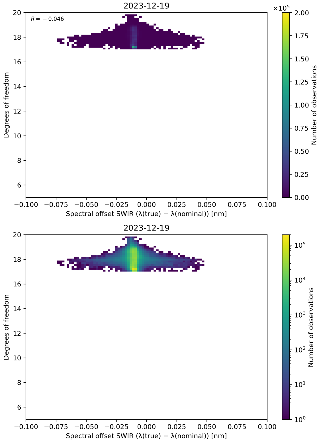
Figure 119: Scatter density plot of “Spectral offset SWIR ( \lambda(\text{true}) - \lambda(\text{nominal}) )” against “Degrees of freedom” for 2023-12-18 to 2023-12-20.
