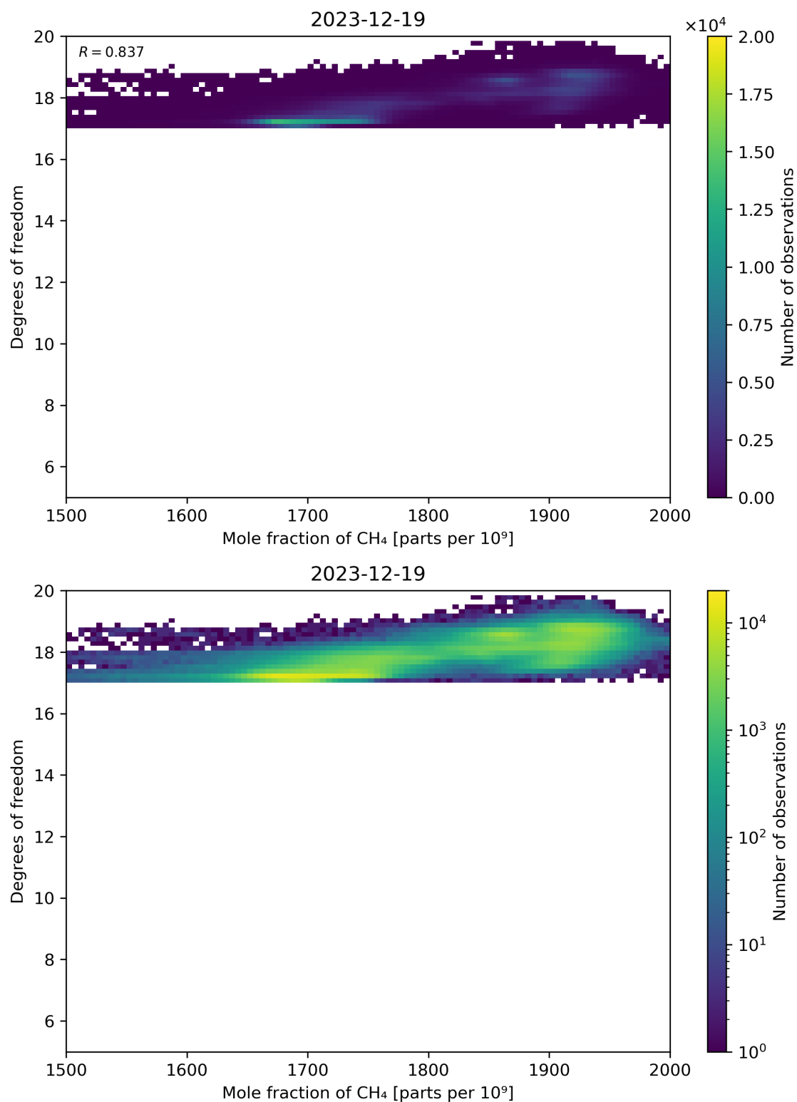
Figure 72: Scatter density plot of “Mole fraction of CH 4 ” against “Degrees of freedom” for 2023-12-18 to 2023-12-20.
