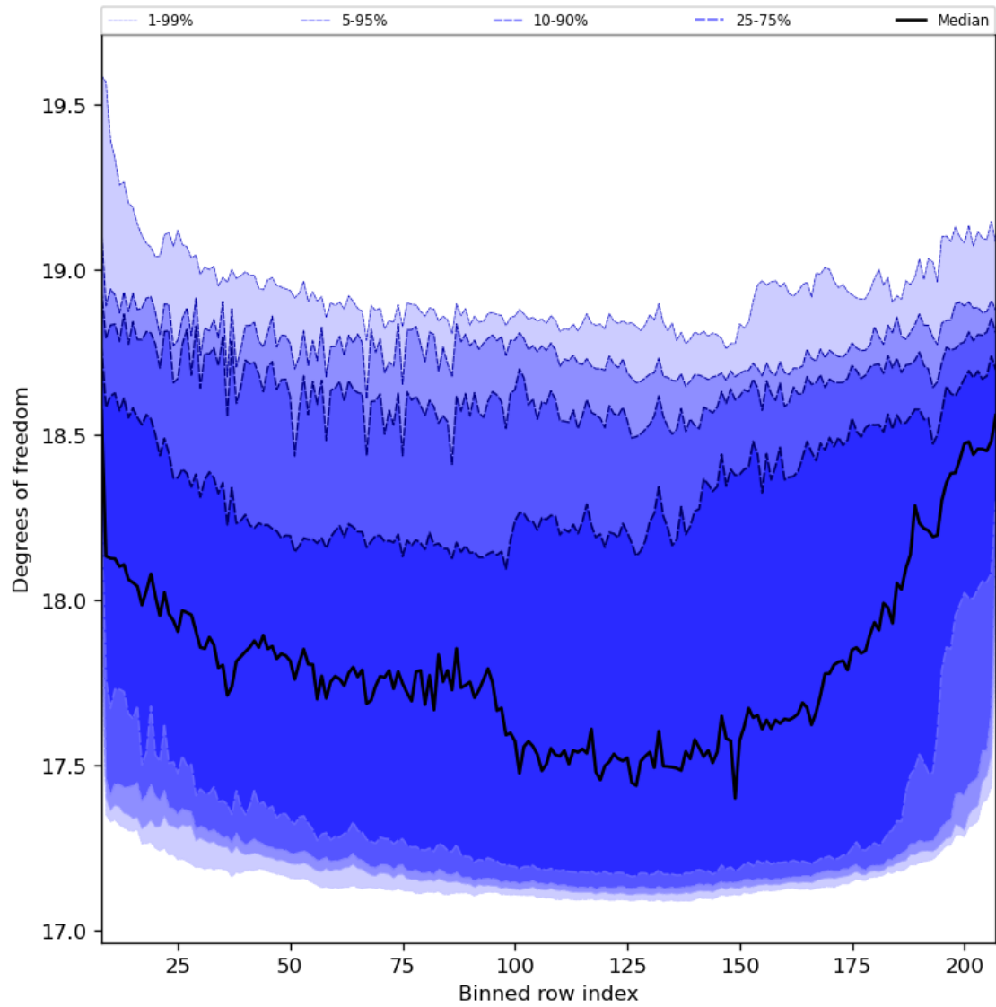
Figure 41: Along track statistics of “Degrees of freedom” for 2023-12-18 to 2023-12-20
