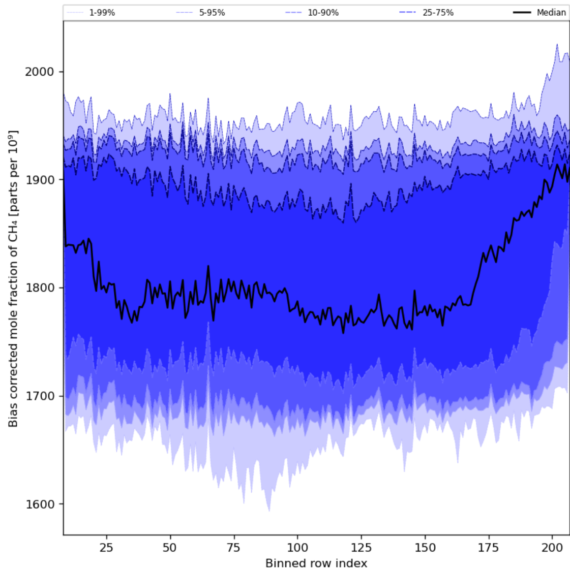
Figure 36: Along track statistics of “Bias corrected mole fraction of CH 4 ” for 2023-12-18 to 2023-12-20
