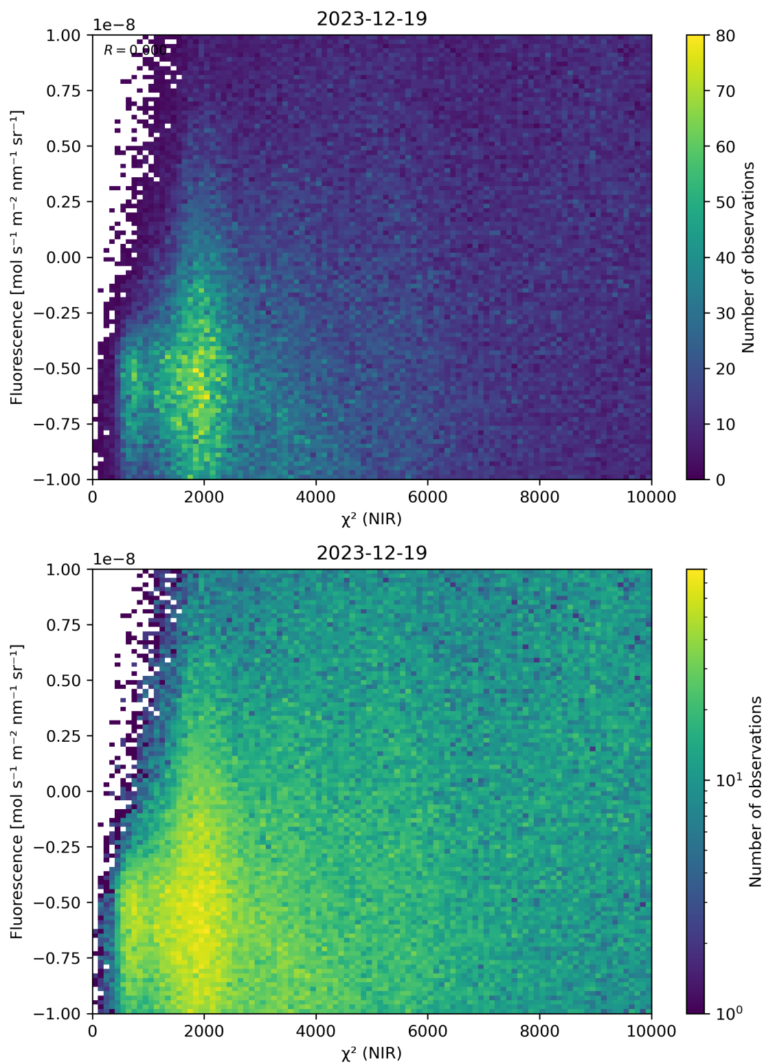
Figure 45: Scatter density plot of “ \chi^2 (NIR)” against “Fluorescence” for 2023-12-18 to 2023-12-20.
