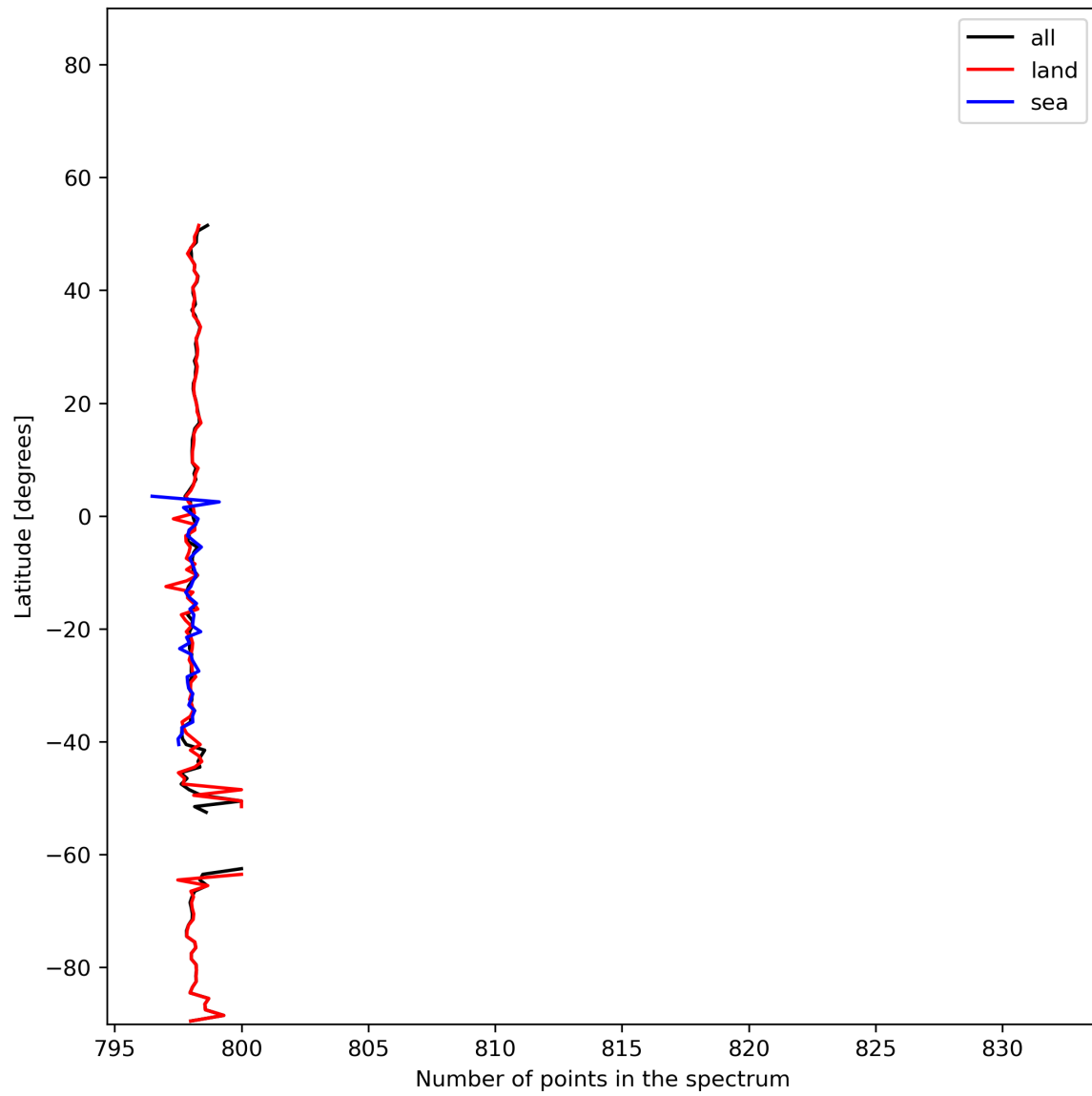
Figure 15: Zonal average of “Number of points in the spectrum” for 2023-12-18 to 2023-12-20.
