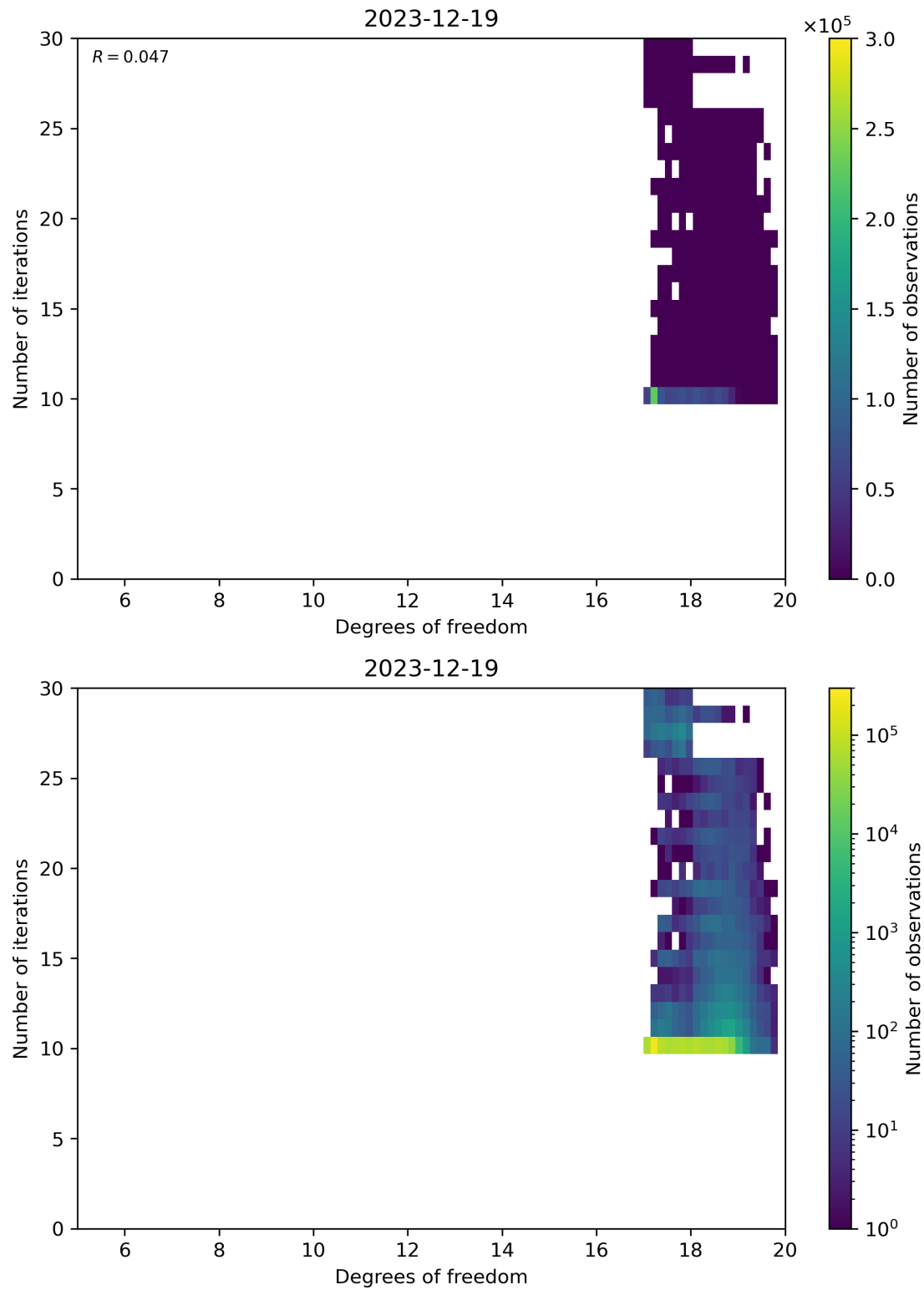
Figure 52: Scatter density plot of “Degrees of freedom” against “Number of iterations” for 2023-12-18 to 2023-12-20.
