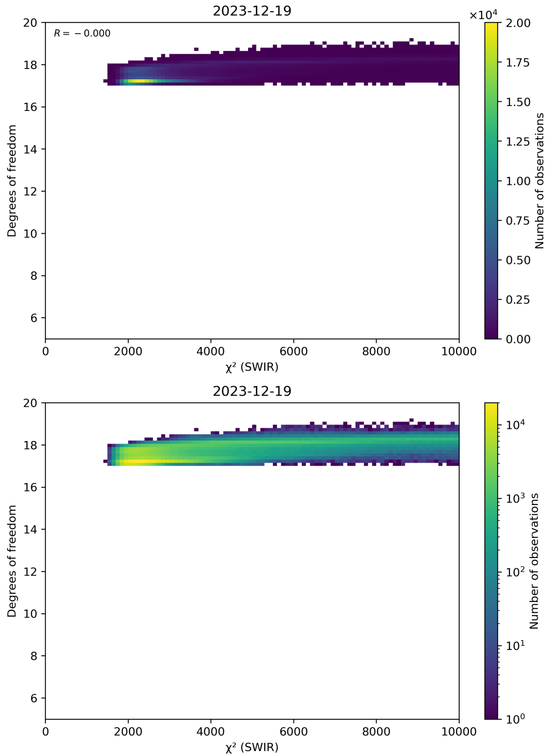
Figure 48: Scatter density plot of “ \chi^2 (SWIR)” against “Degrees of freedom” for 2023-12-18 to 2023-12-20.
