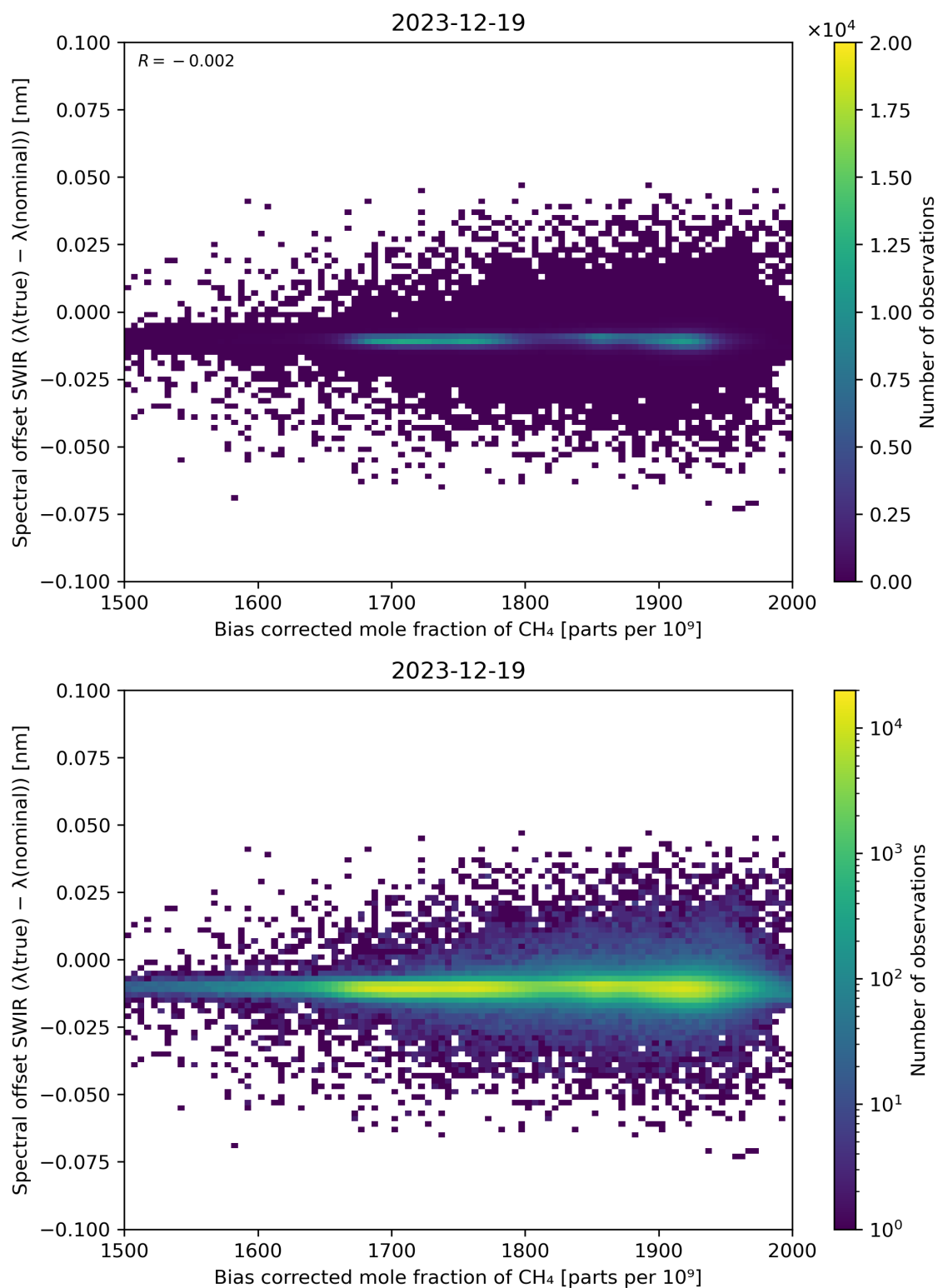
Figure 69: Scatter density plot of “Bias corrected mole fraction of \text{CH}_4 ” against “Spectral offset SWIR ( \lambda(\text{true}) - \lambda(\text{nominal}) )” for 2023-12-18 to 2023-12-20.
