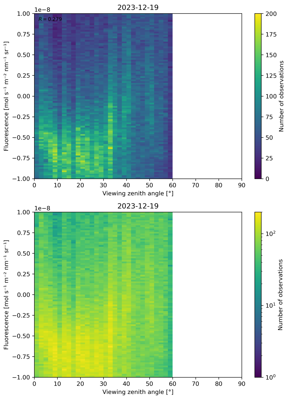
Figure 108: Scatter density plot of “Viewing zenith angle” against “Fluorescence” for 2023-12-18 to 2023-12-20.
