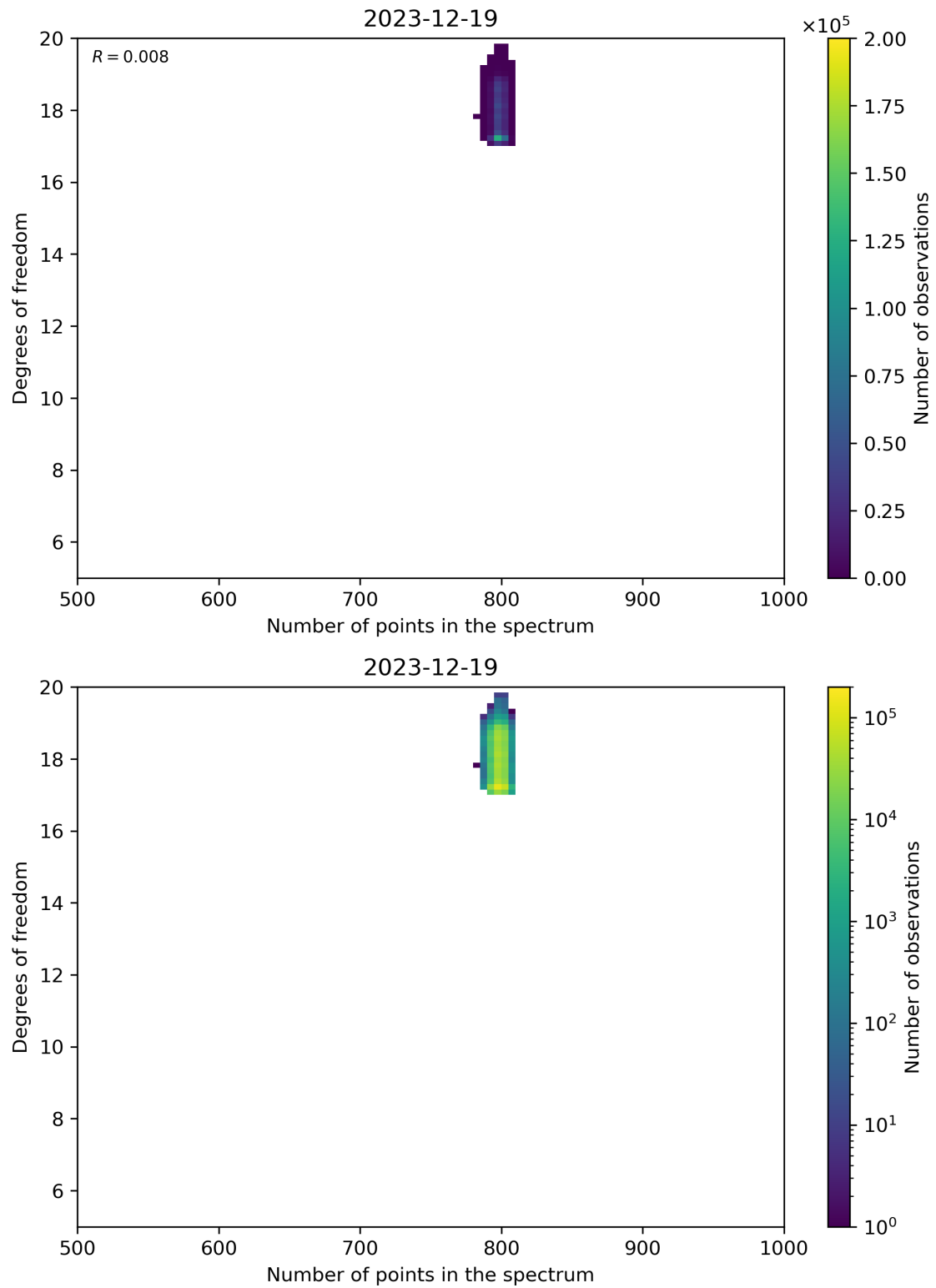
Figure 90: Scatter density plot of “Number of points in the spectrum” against “Degrees of freedom” for 2023-12-18 to 2023-12-20.
