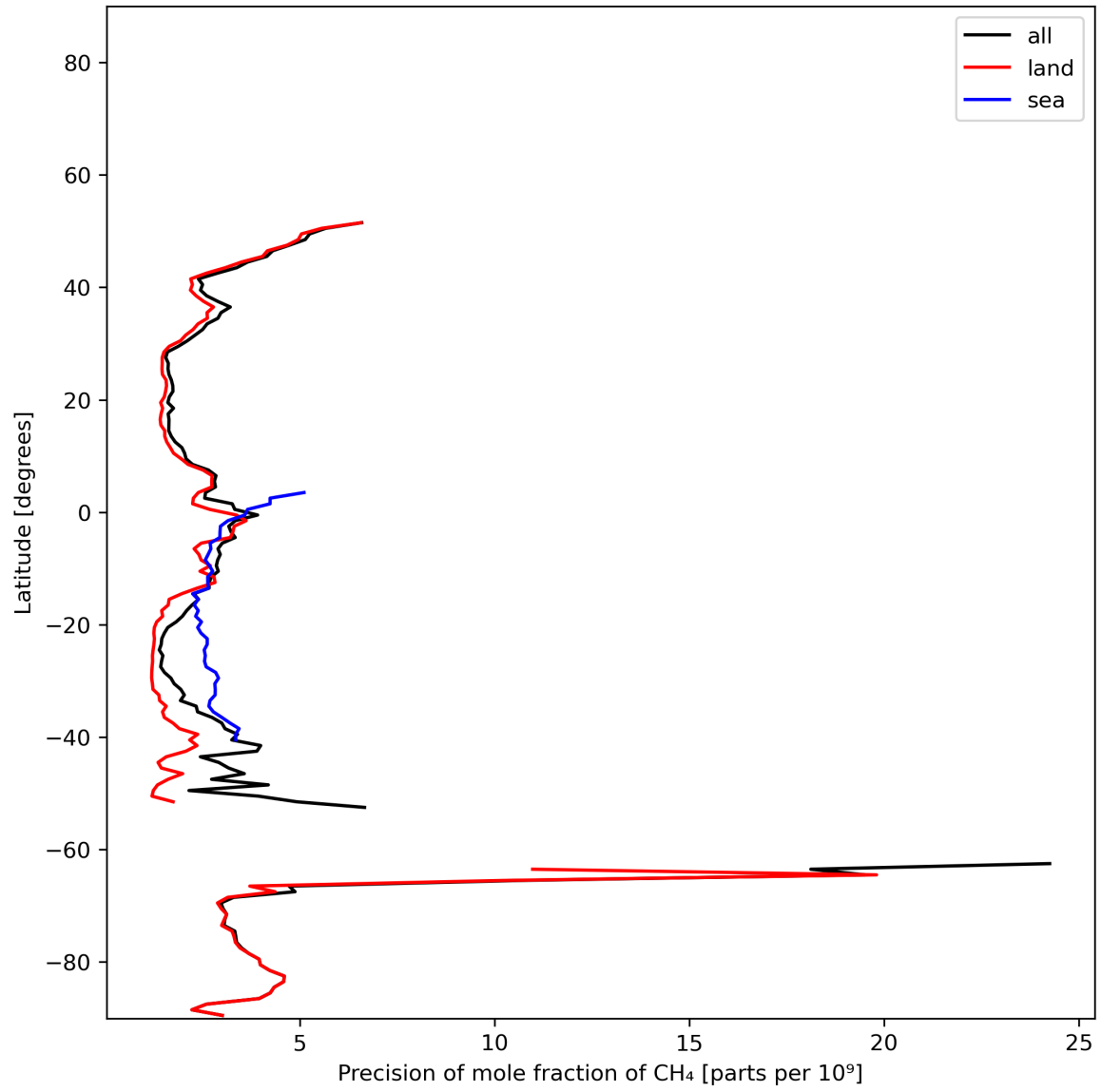
Figure 13: Zonal average of “Precision of mole fraction of CH 4 ” for 2023-12-18 to 2023-12-20.
