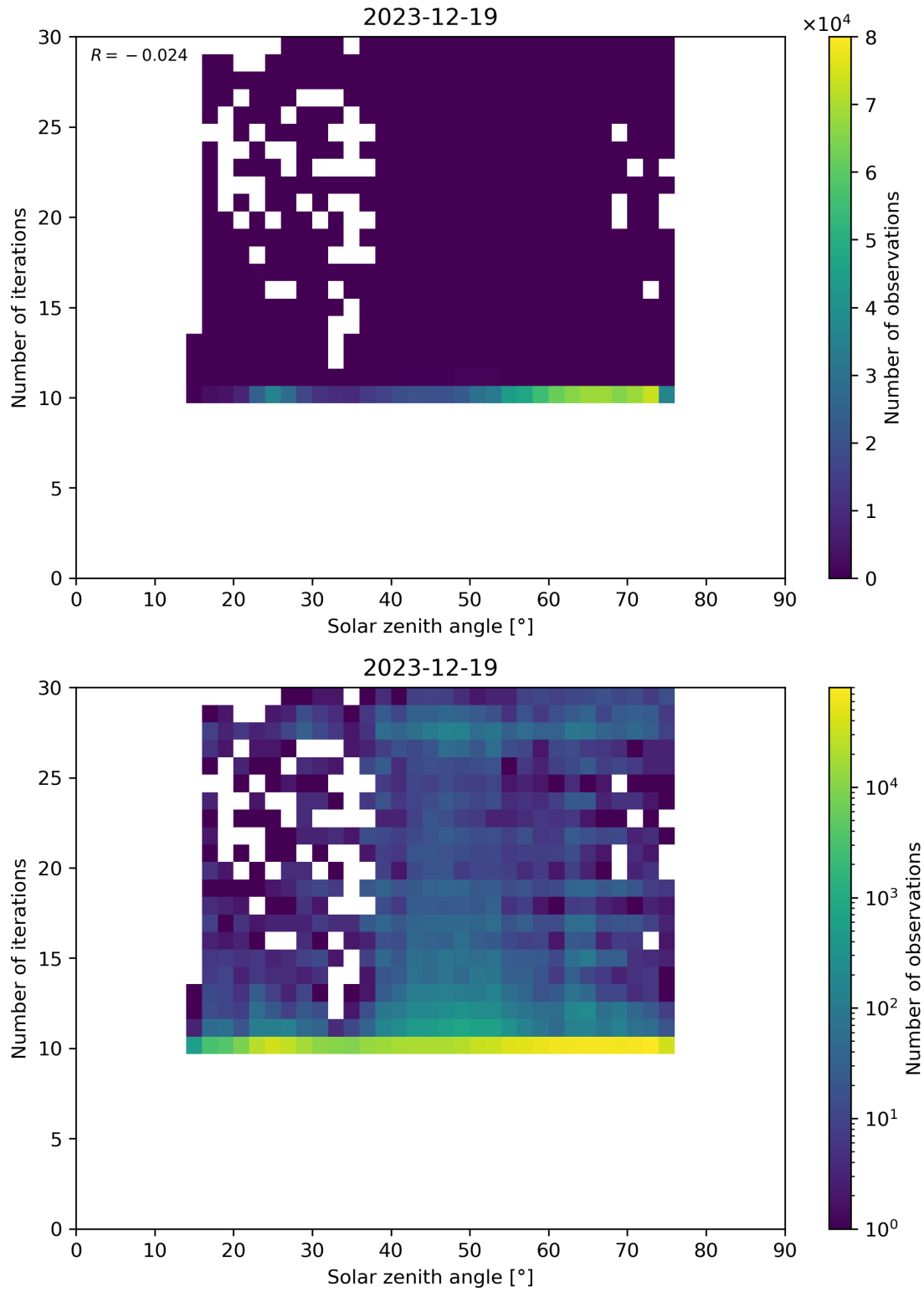
Figure 102: Scatter density plot of “Solar zenith angle” against “Number of iterations” for 2023-12-18 to 2023-12-20.
