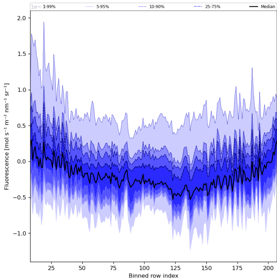
Figure 43: Along track statistics of “Fluorescence” for 2023-12-18 to 2023-12-20
