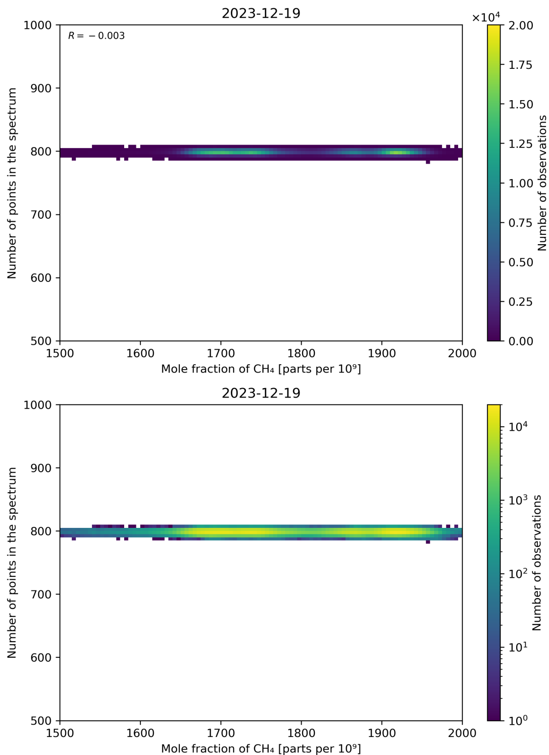
Figure 77: Scatter density plot of “Mole fraction of CH 4 ” against “Number of points in the spectrum” for 2023-12-18 to 2023-12-20.
