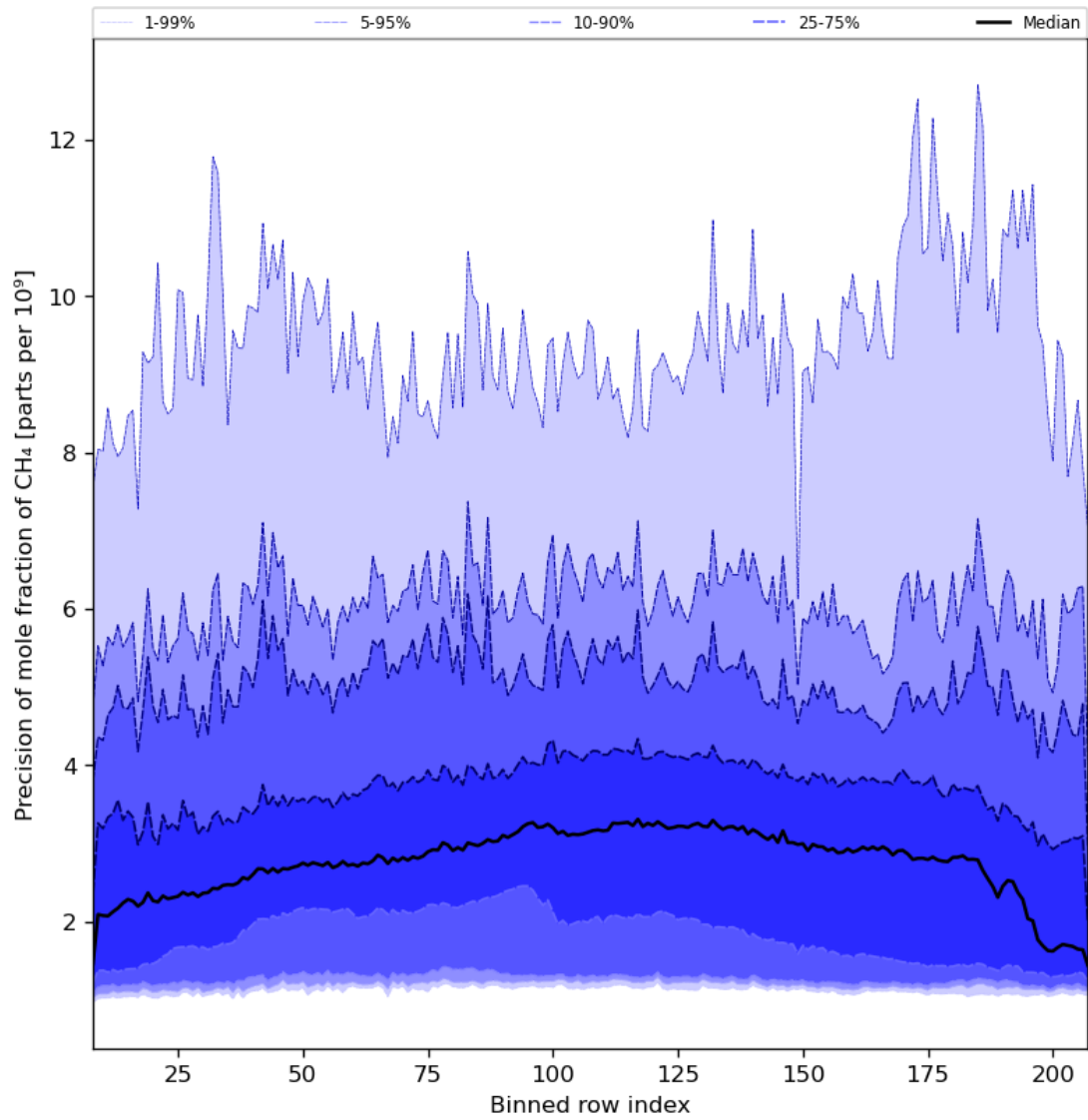
Figure 35: Along track statistics of “Precision of mole fraction of CH 4 ” for 2023-12-18 to 2023-12-20
