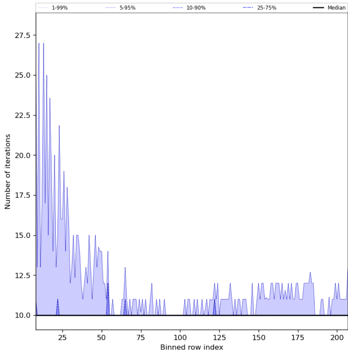
Figure 42: Along track statistics of “Number of iterations” for 2023-12-18 to 2023-12-20
