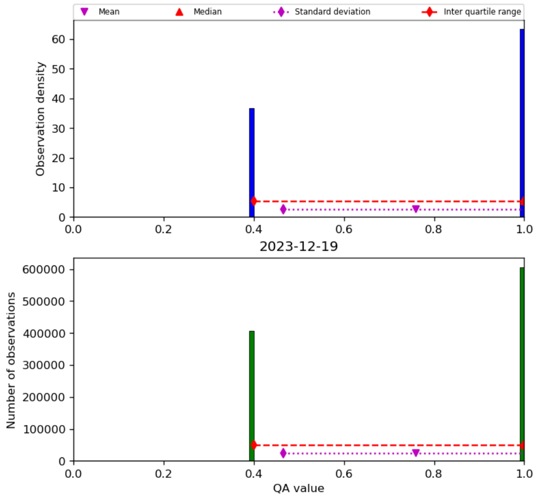
Figure 22: Histogram of “QA value” for 2023-12-18 to 2023-12-20
