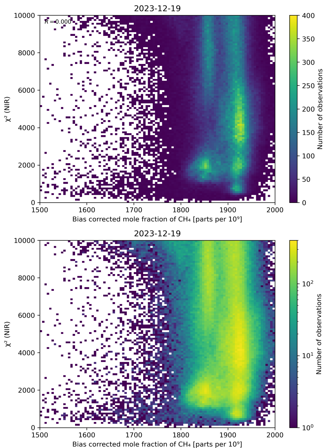
Figure 63: Scatter density plot of “Bias corrected mole fraction of \text{CH}_4 ” against “ \chi^2 (NIR)” for 2023-12-18 to 2023-12-20.
