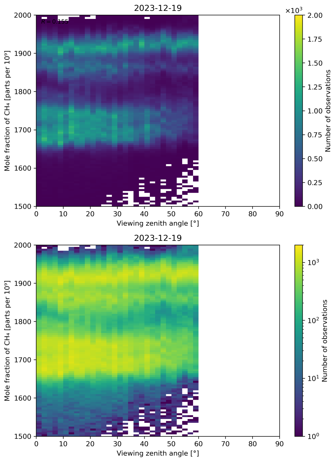
Figure 110: Scatter density plot of “Viewing zenith angle” against “Mole fraction of CH 4 ” for 2023-12-18 to 2023-12-20.
