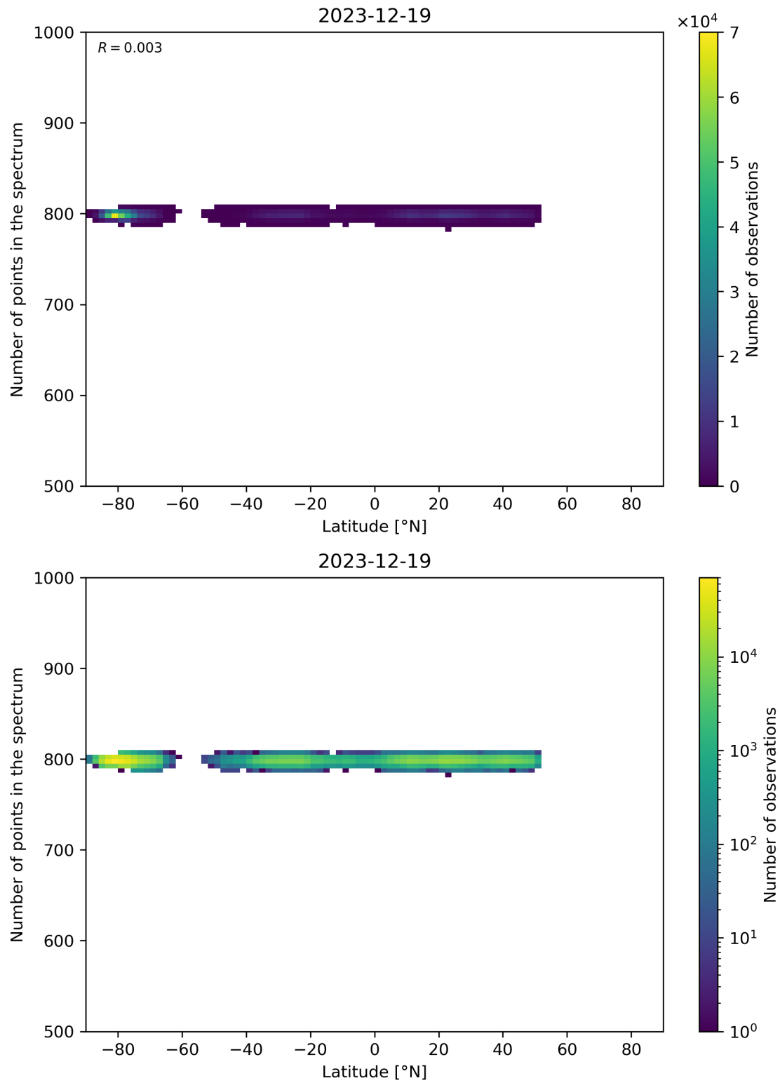
Figure 61: Scatter density plot of “Latitude” against “Number of points in the spectrum” for 2023-12-18 to 2023-12-20.
