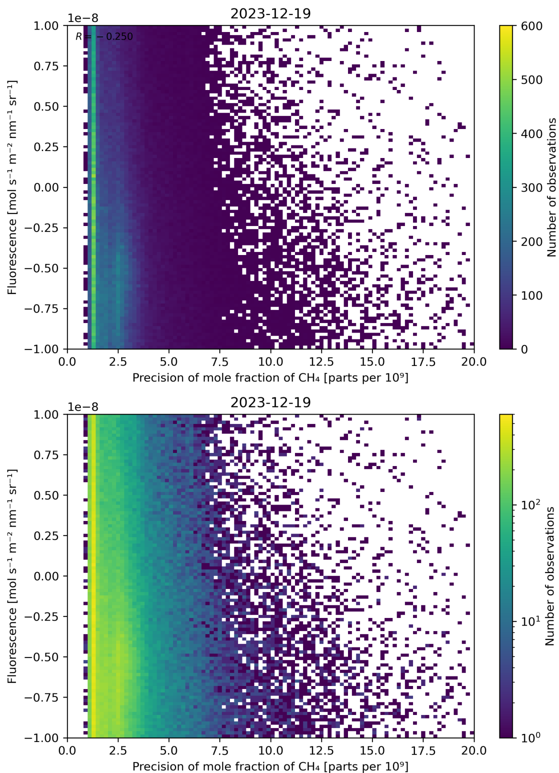
Figure 81: Scatter density plot of “Precision of mole fraction of \text{CH}_4 ” against “Fluorescence” for 2023-12-18 to 2023-12-20.
