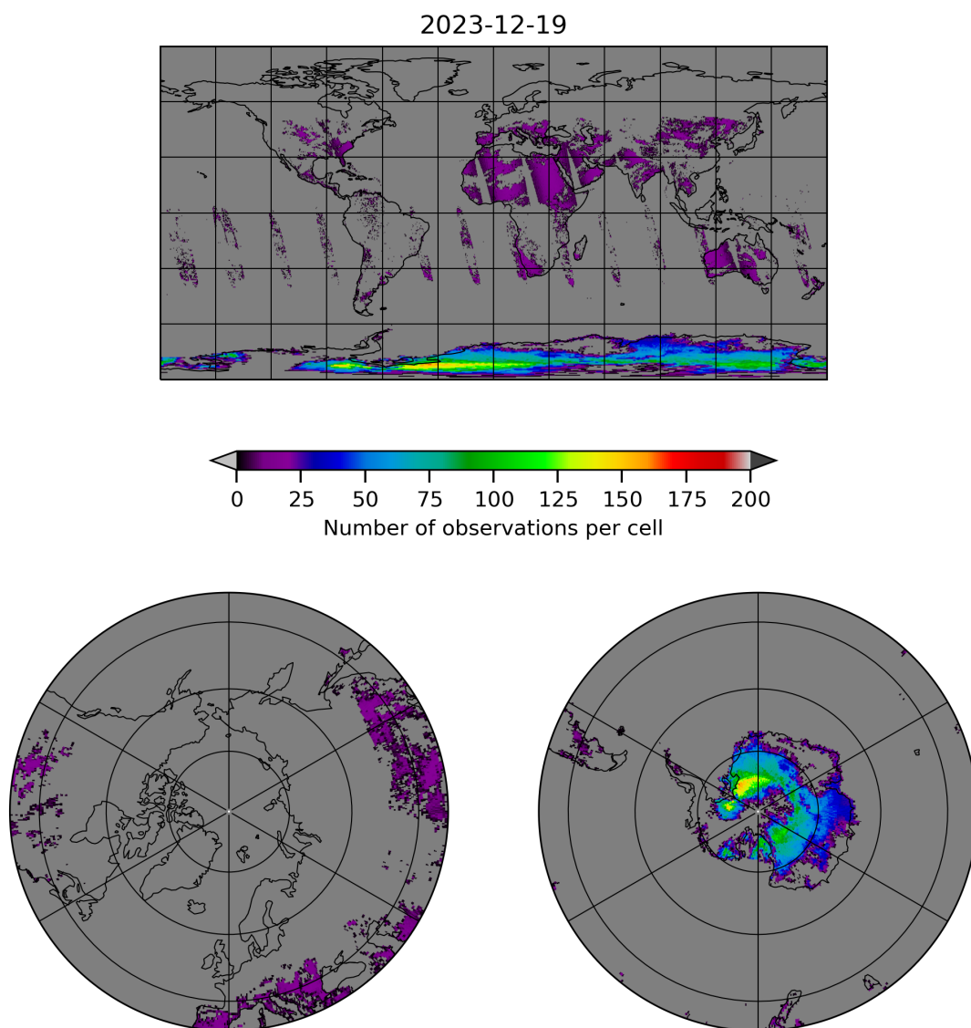
Figure 10: Map of the number of observations for 2023-12-18 to 2023-12-20
