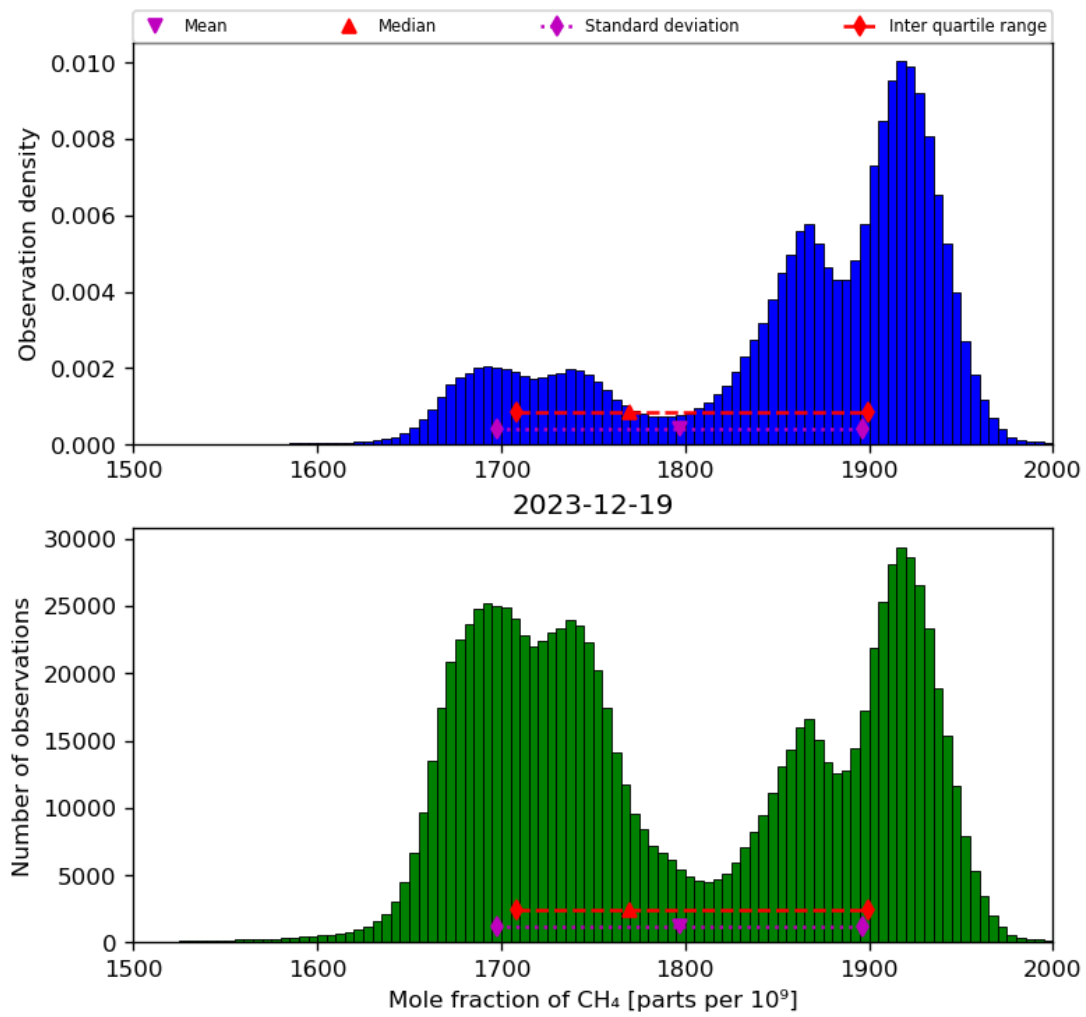
Figure 23: Histogram of “Mole fraction of CH 4 ” for 2023-12-18 to 2023-12-20
