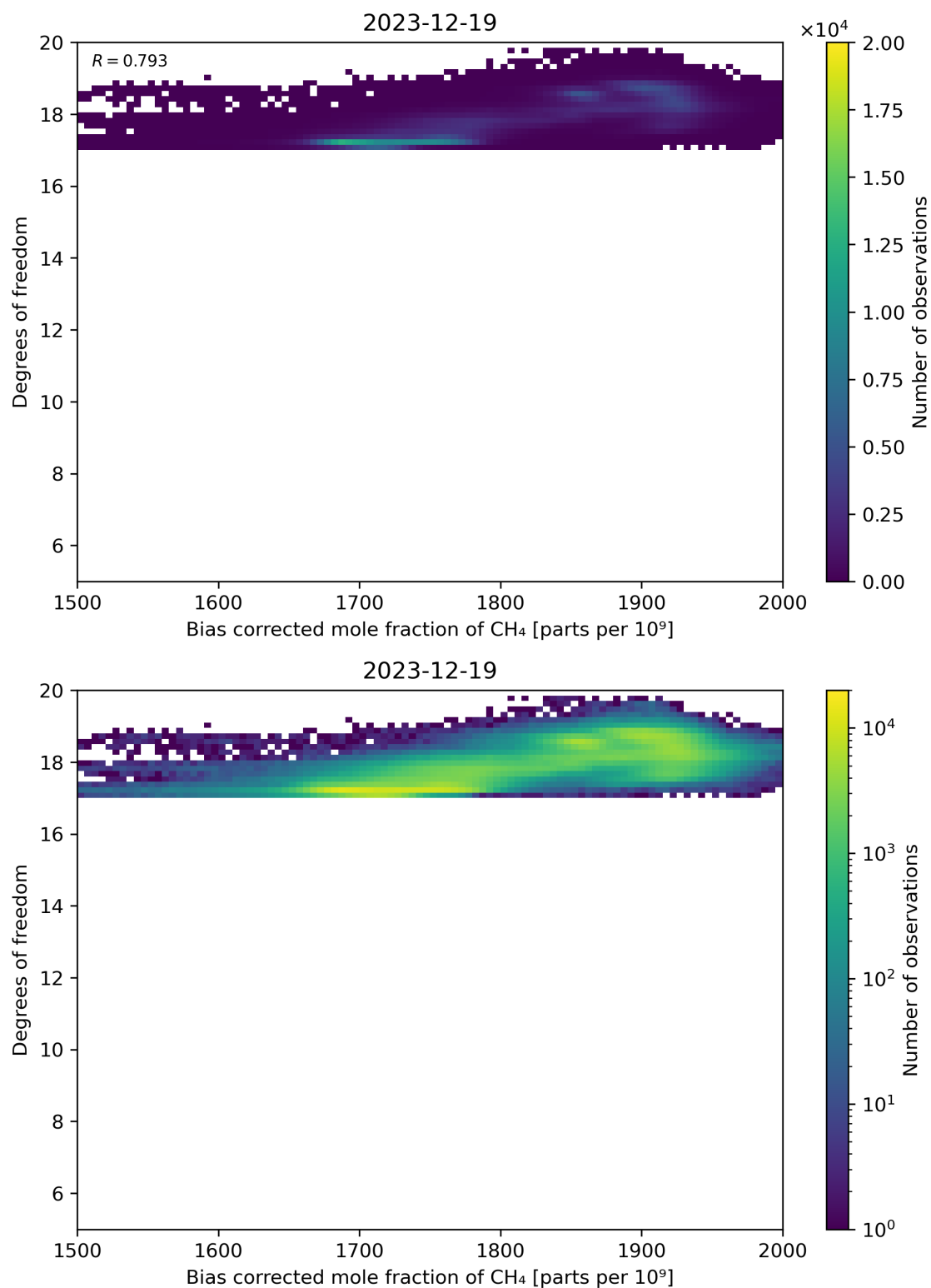
Figure 65: Scatter density plot of “Bias corrected mole fraction of CH 4 ” against “Degrees of freedom” for 2023-12-18 to 2023-12-20.
