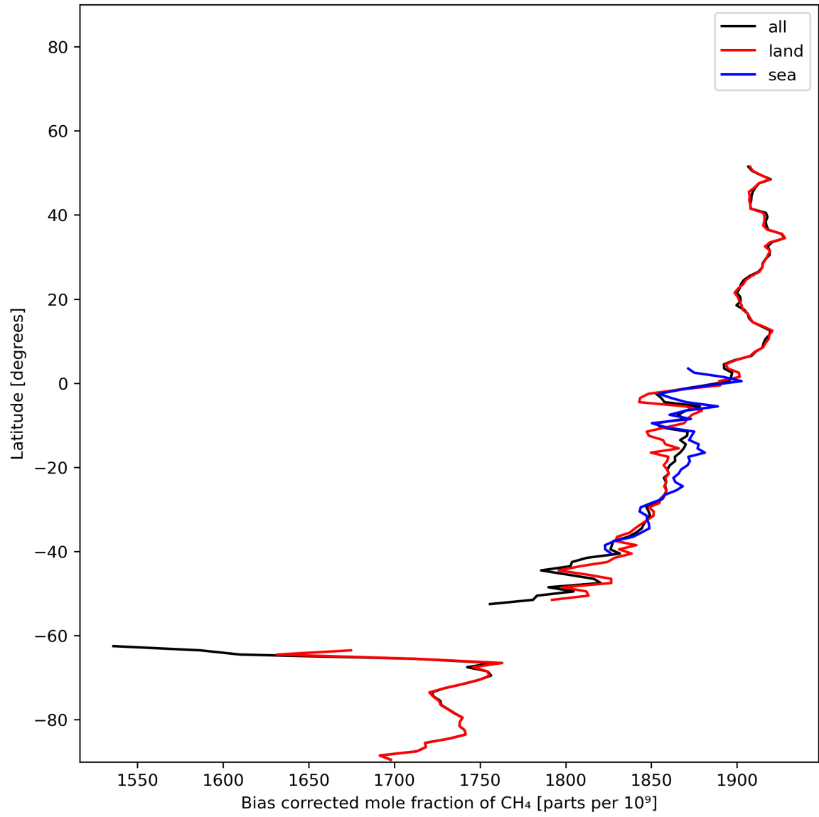
Figure 14: Zonal average of “Bias corrected mole fraction of CH 4 ” for 2023-12-18 to 2023-12-20.
