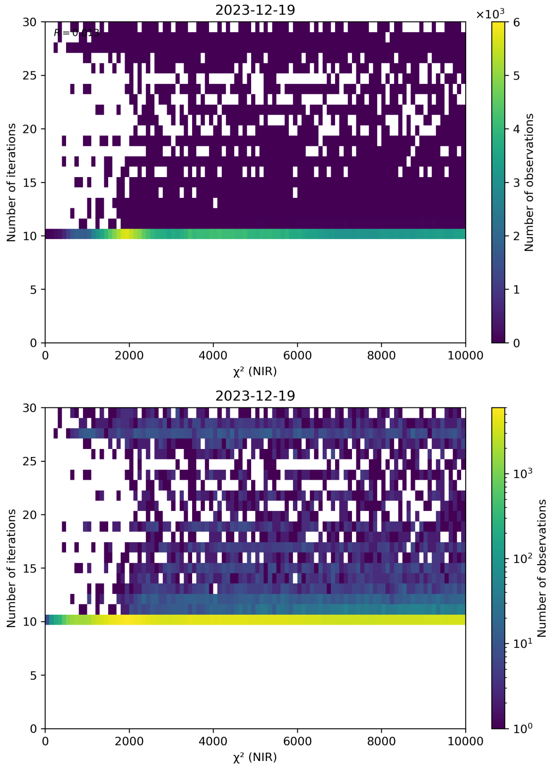
Figure 46: Scatter density plot of “ \chi^2 (NIR)” against “Number of iterations” for 2023-12-18 to 2023-12-20.
