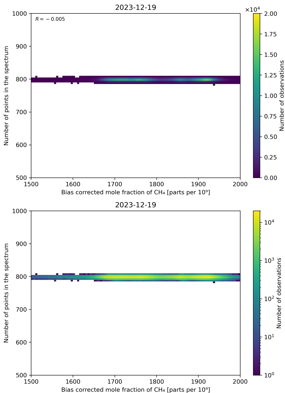
Figure 68: Scatter density plot of “Bias corrected mole fraction of CH 4 ” against “Number of points in the spectrum” for 2023-12-18 to 2023-12-20.
