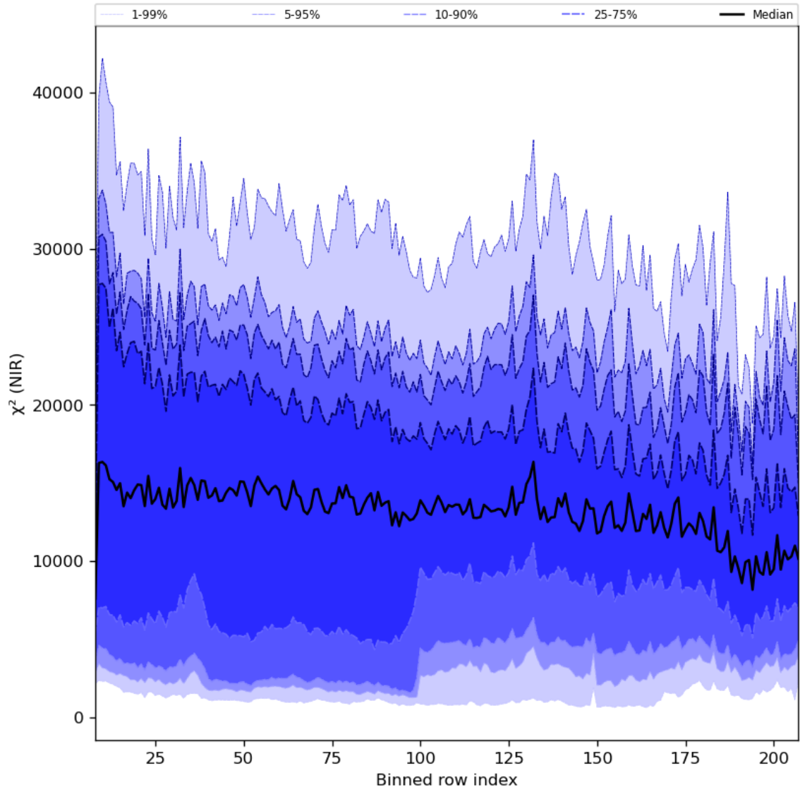
Figure 40: Along track statistics of “ \chi^2 (NIR)” for 2023-12-18 to 2023-12-20
