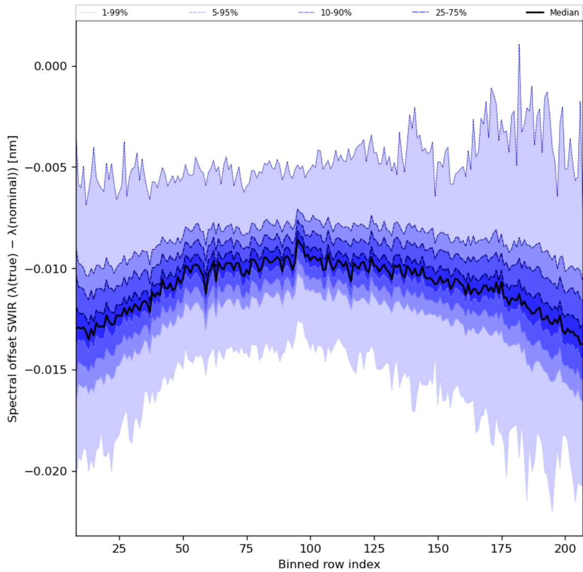
Figure 38: Along track statistics of “Spectral offset SWIR ( \lambda(\text{true}) - \lambda(\text{nominal}) )” for 2023-12-18 to 2023-12-20
