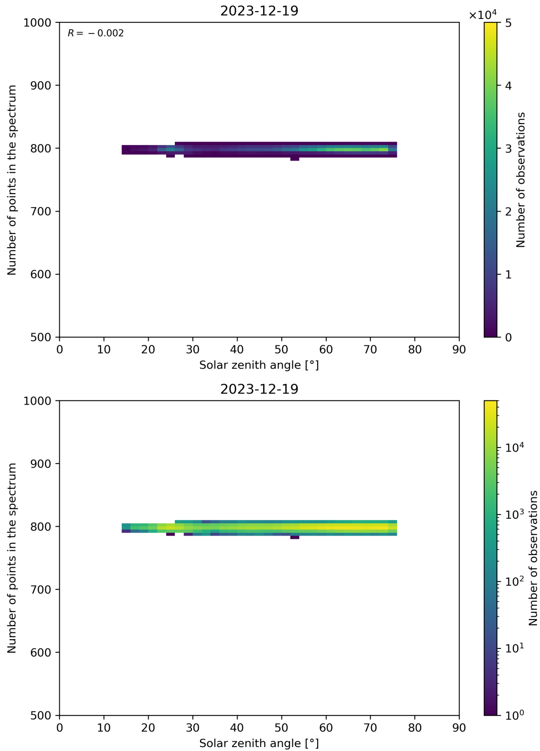
Figure 103: Scatter density plot of “Solar zenith angle” against “Number of points in the spectrum” for 2023-12-18 to 2023-12-20.
