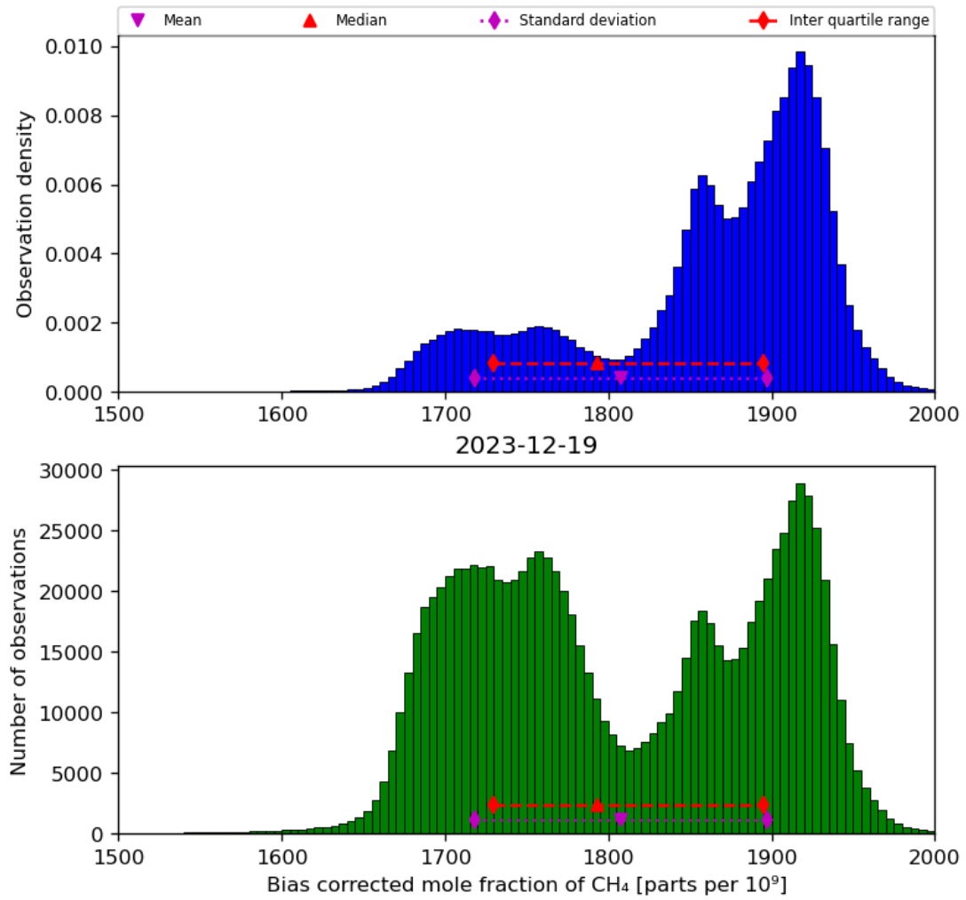
Figure 25: Histogram of “Bias corrected mole fraction of CH 4 ” for 2023-12-18 to 2023-12-20
