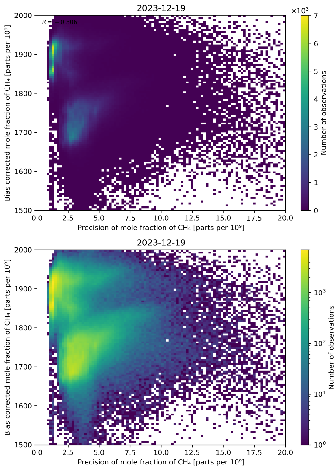
Figure 82: Scatter density plot of “Precision of mole fraction of CH 4 ” against “Bias corrected mole fraction of CH 4 ” for 2023-12-18 to 2023-12-20.
