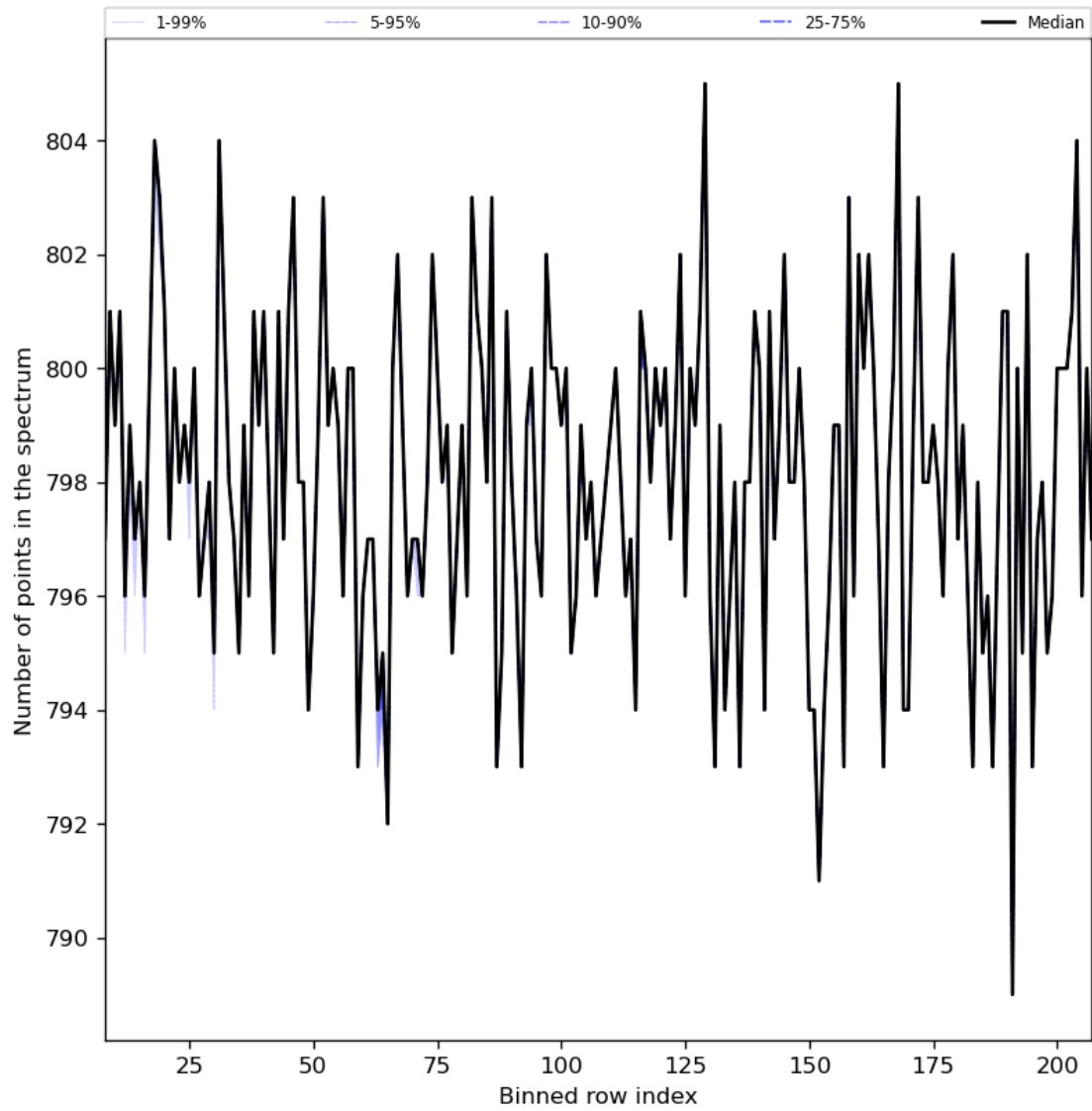
Figure 37: Along track statistics of “Number of points in the spectrum” for 2023-12-18 to 2023-12-20
