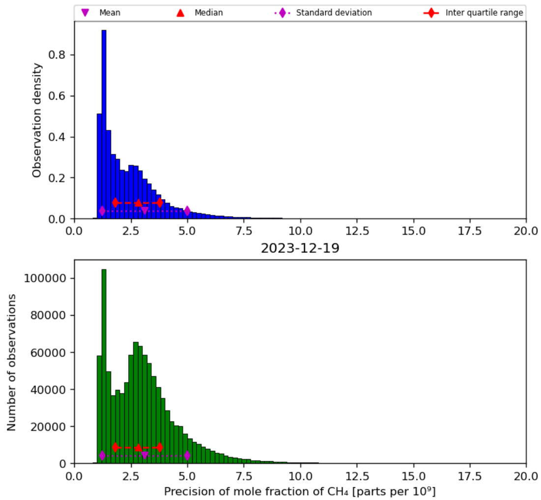
Figure 24: Histogram of “Precision of mole fraction of CH 4 ” for 2023-12-18 to 2023-12-20
