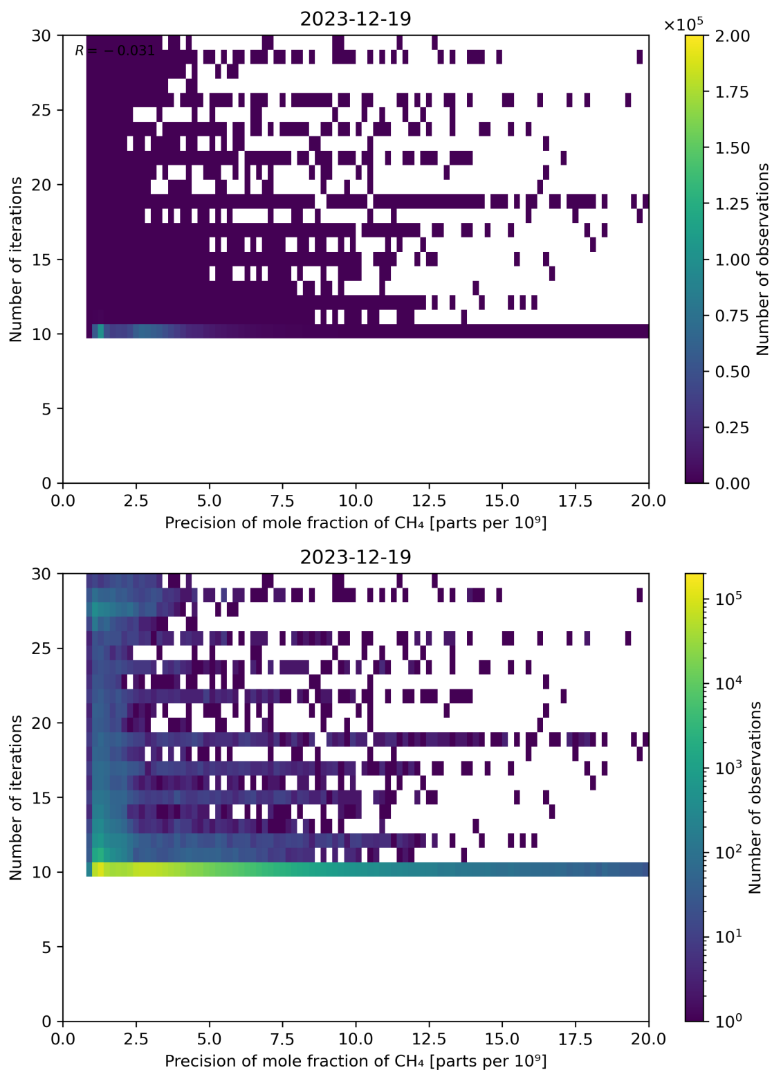
Figure 83: Scatter density plot of “Precision of mole fraction of CH 4 ” against “Number of iterations” for 2023-12-18 to 2023-12-20.
