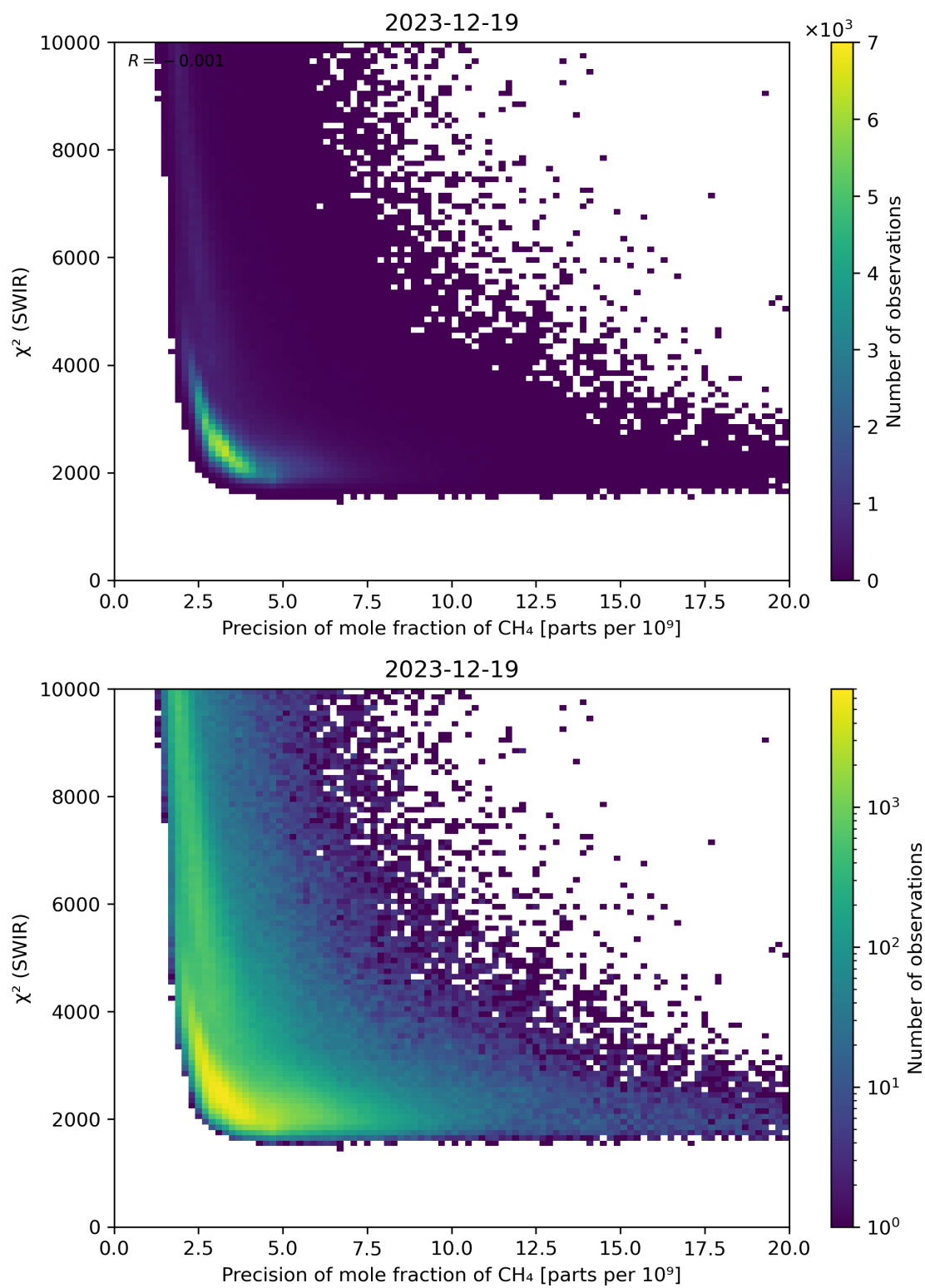
Figure 79: Scatter density plot of “Precision of mole fraction of CH 4 ” against “ \chi^2 (SWIR)” for 2023-12-18 to 2023-12-20.
