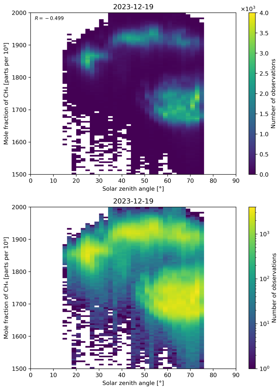
Figure 99: Scatter density plot of “Solar zenith angle” against “Mole fraction of \text{CH}_4 ” for 2023-12-18 to 2023-12-20.
