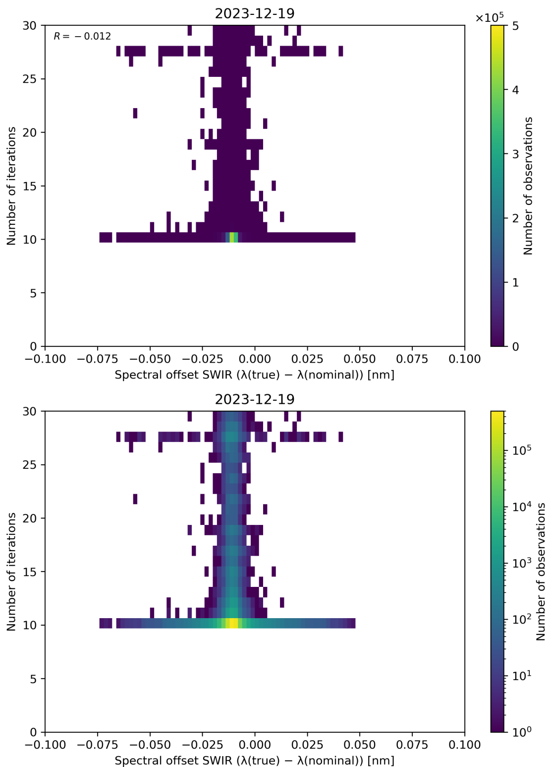
Figure 121: Scatter density plot of “Spectral offset SWIR ( \lambda(\text{true}) - \lambda(\text{nominal}) )” against “Number of iterations” for 2023-12-18 to 2023-12-20.
