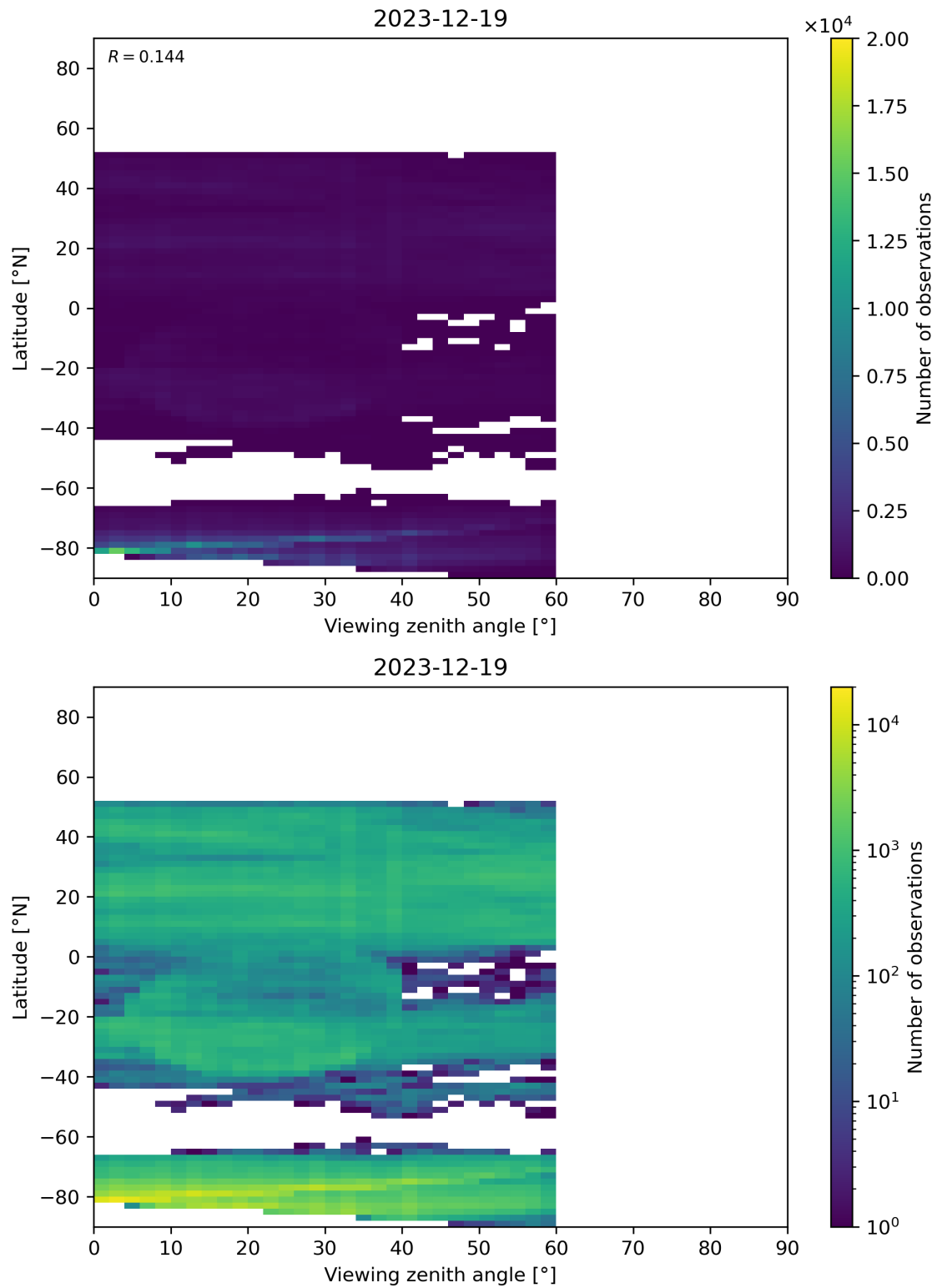
Figure 109: Scatter density plot of “Viewing zenith angle” against “Latitude” for 2023-12-18 to 2023-12-20.
