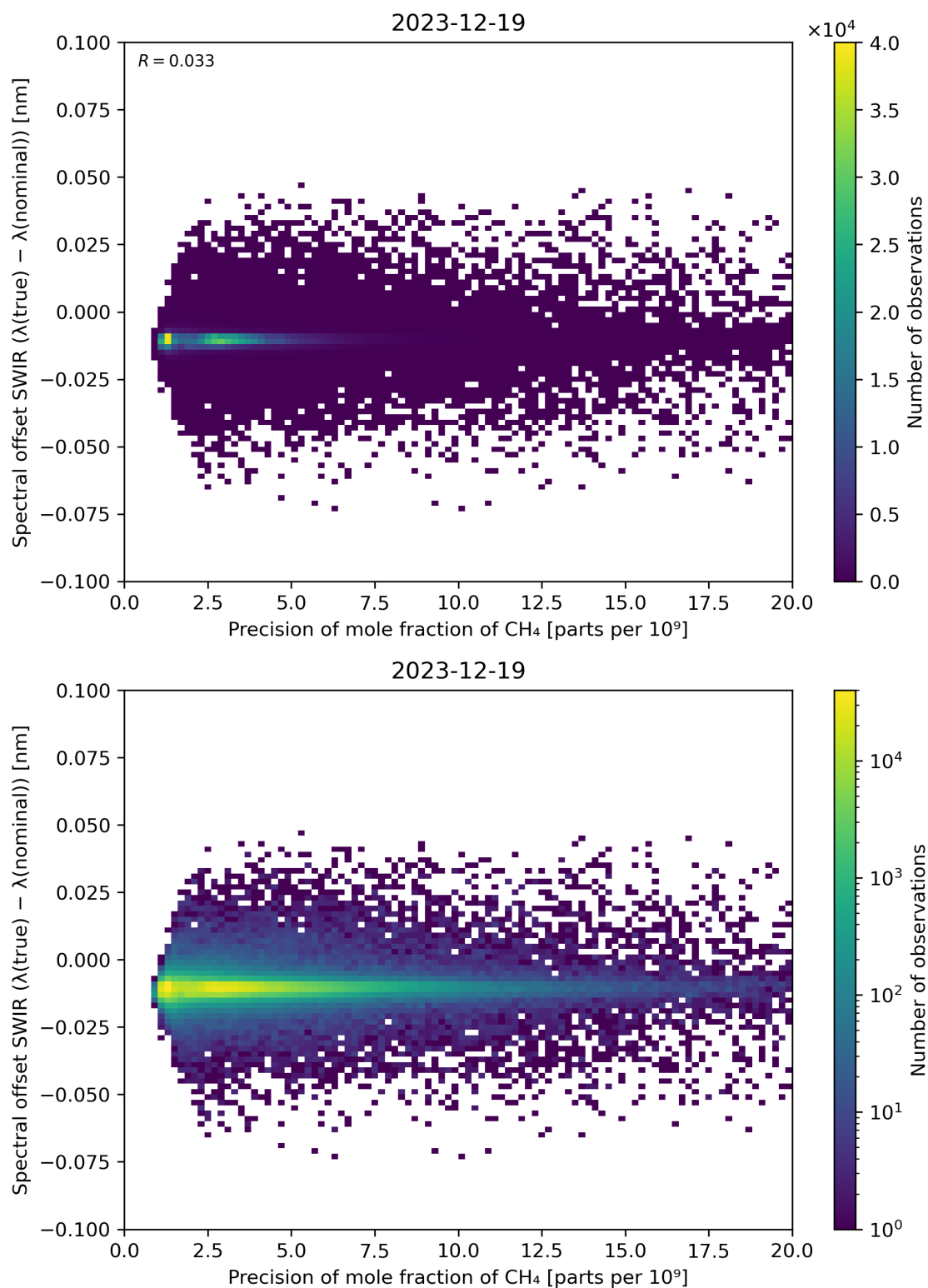
Figure 85: Scatter density plot of “Precision of mole fraction of CH 4 ” against “Spectral offset SWIR ( \lambda(\text{true}) - \lambda(\text{nominal}) )” for 2023-12-18 to 2023-12-20.
