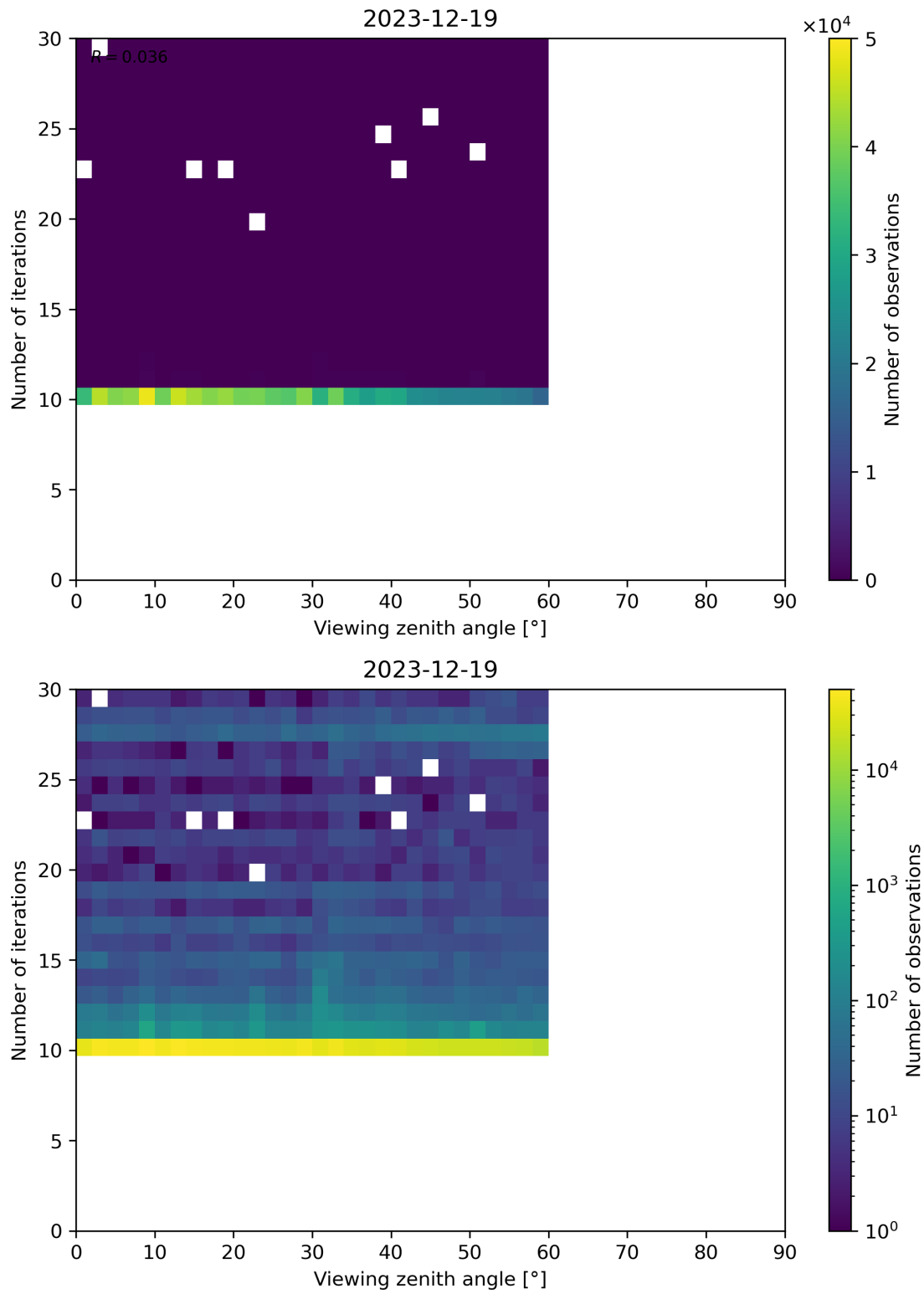
Figure 113: Scatter density plot of “Viewing zenith angle” against “Number of iterations” for 2023-12-18 to 2023-12-20.
