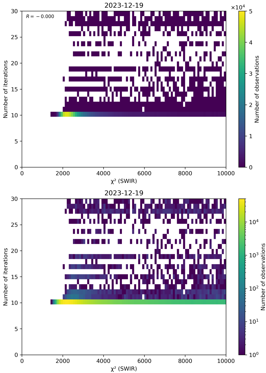
Figure 50: Scatter density plot of “ \chi^2 (SWIR)” against “Number of iterations” for 2023-12-18 to 2023-12-20.
