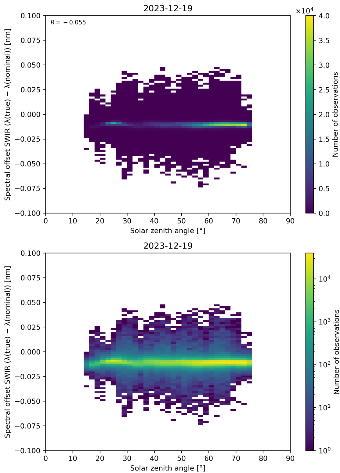
Figure 104: Scatter density plot of “Solar zenith angle” against “Spectral offset SWIR ( \lambda(\text{true}) - \lambda(\text{nominal}) )” for 2023-12-18 to 2023-12-20.
