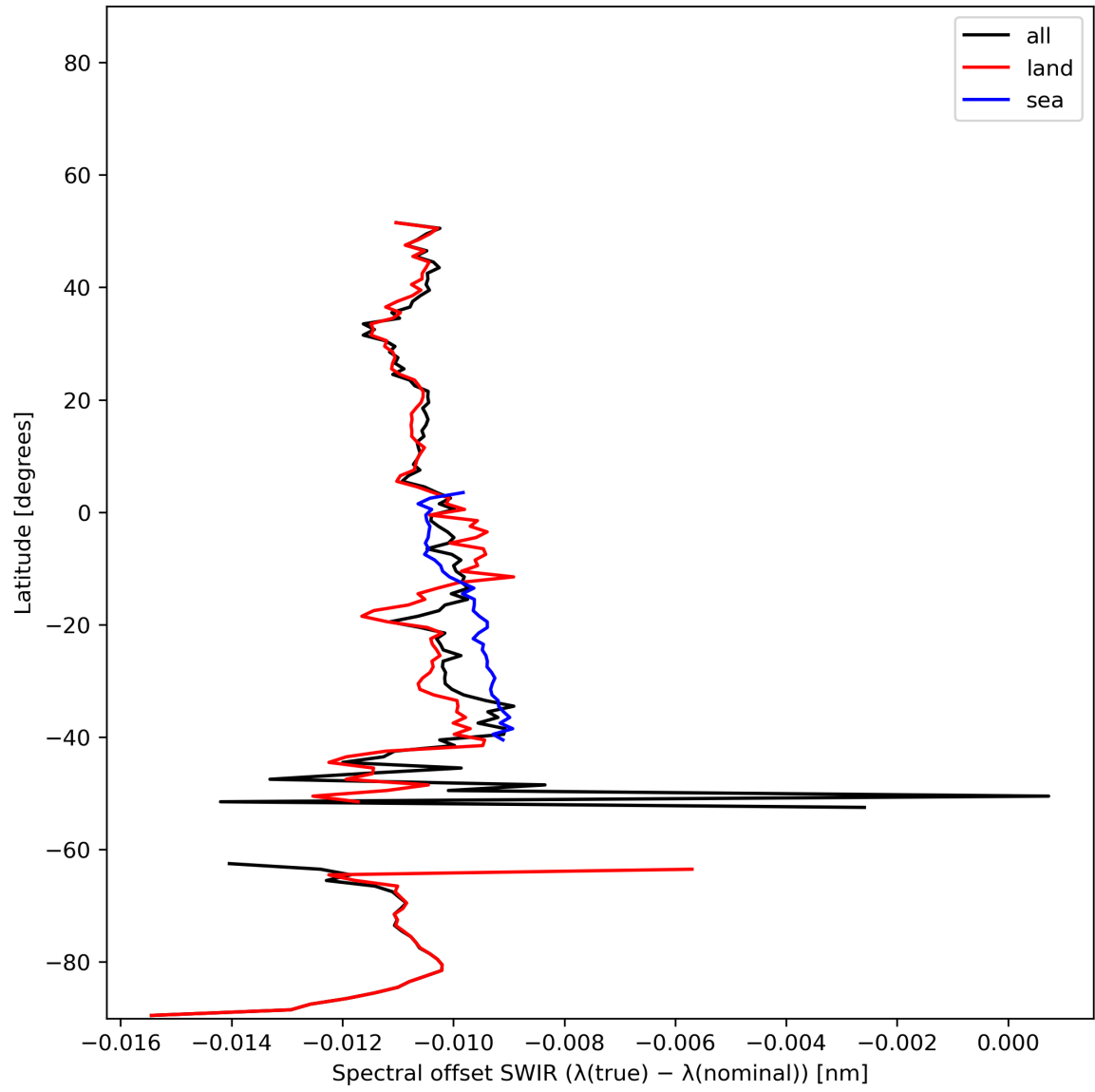
Figure 16: Zonal average of “Spectral offset SWIR ( \lambda(\text{true}) - \lambda(\text{nominal}) )” for 2023-12-18 to 2023-12-20.
