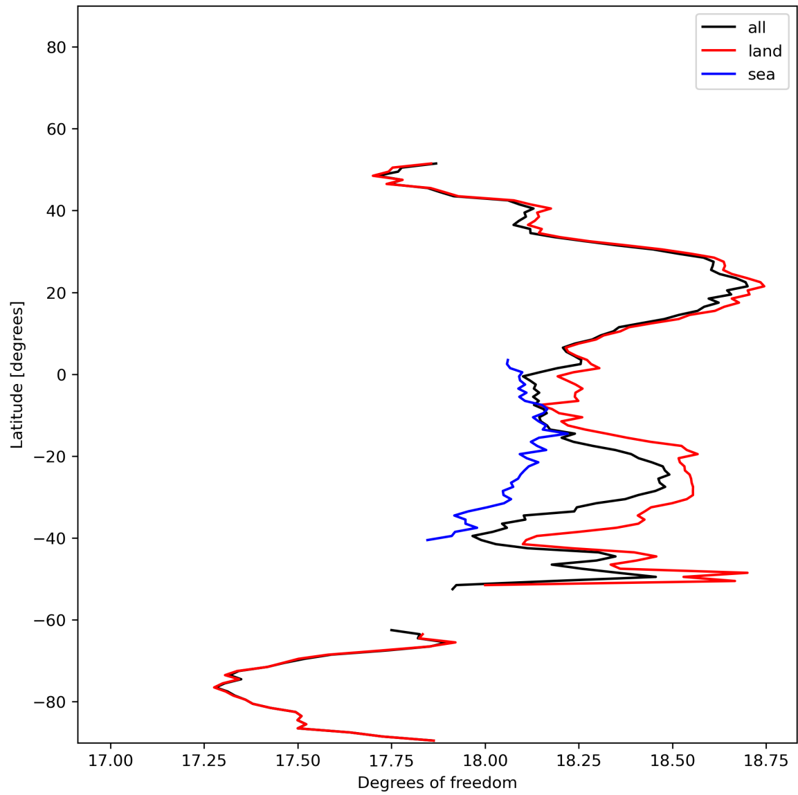
Figure 19: Zonal average of “Degrees of freedom” for 2023-12-18 to 2023-12-20.
