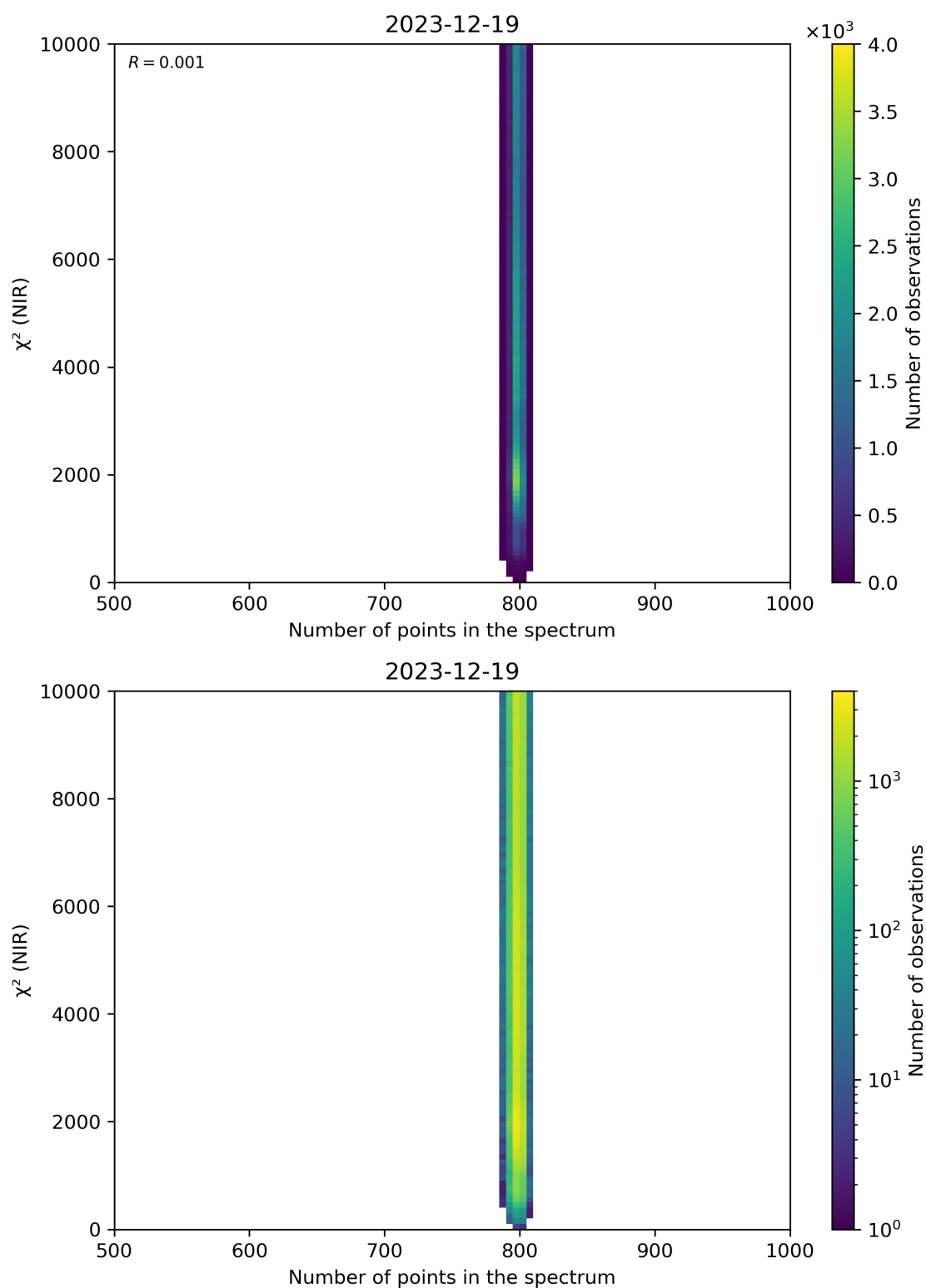
Figure 88: Scatter density plot of “Number of points in the spectrum” against “ \chi^2 (NIR)” for 2023-12-18 to 2023-12-20.
