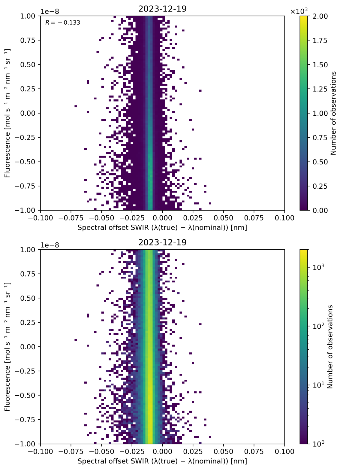
Figure 120: Scatter density plot of “Spectral offset SWIR ( \lambda(\text{true}) - \lambda(\text{nominal}) )” against “Fluorescence” for 2023-12-18 to 2023-12-20.
