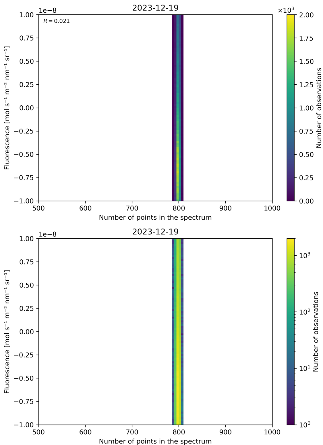
Figure 91: Scatter density plot of “Number of points in the spectrum” against “Fluorescence” for 2023-12-18 to 2023-12-20.
