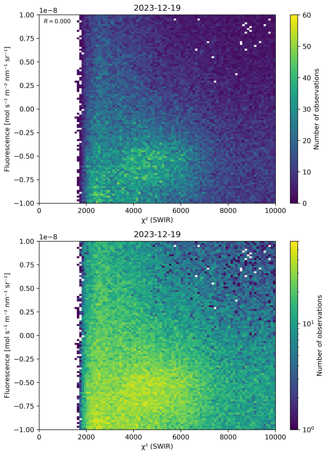
Figure 49: Scatter density plot of “ \chi^2 (SWIR)” against “Fluorescence” for 2023-12-18 to 2023-12-20.
