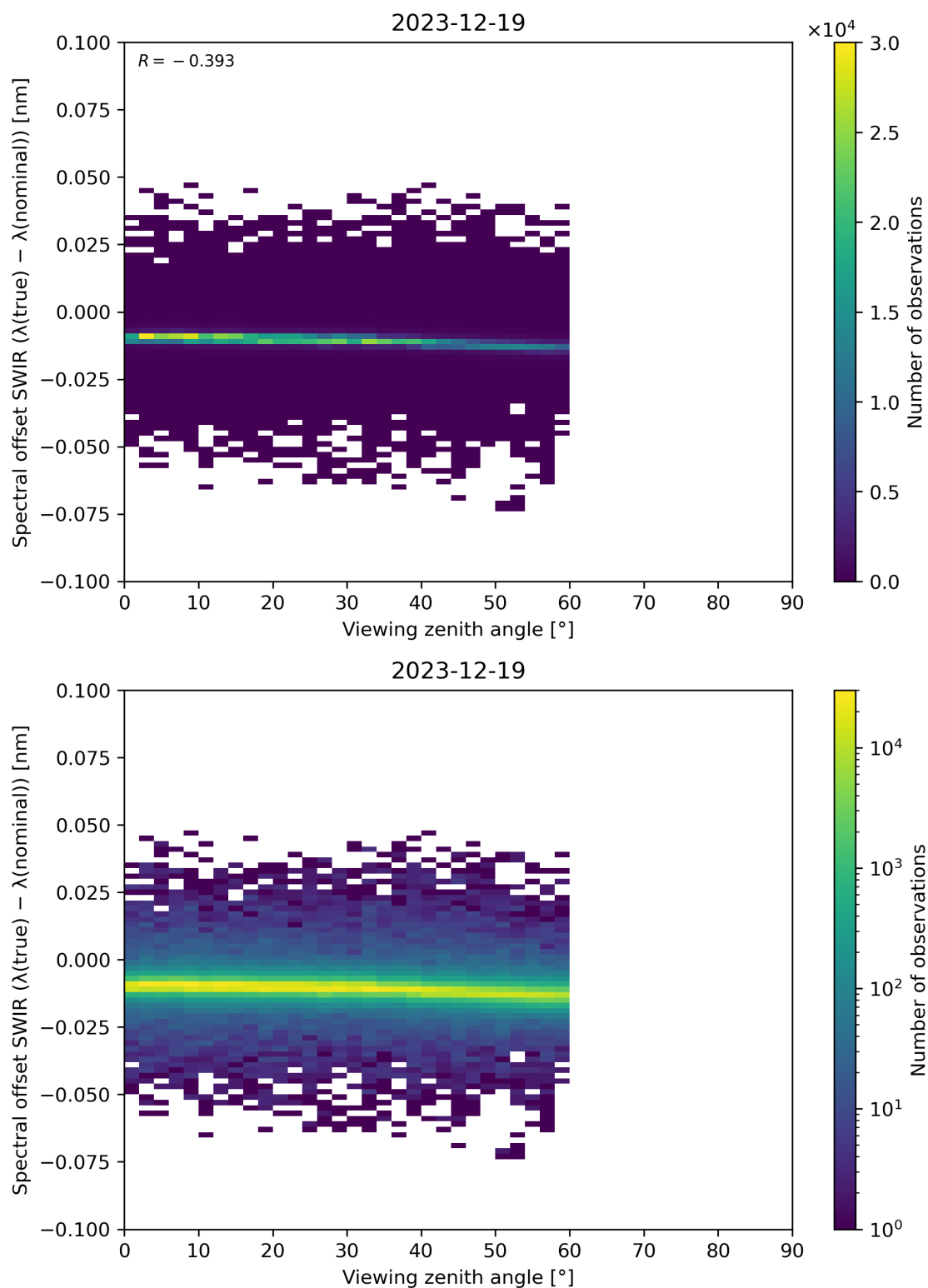
Figure 116: Scatter density plot of “Viewing zenith angle” against “Spectral offset SWIR ( \lambda(\text{true}) - \lambda(\text{nominal}) )” for 2023-12-18 to 2023-12-20.
