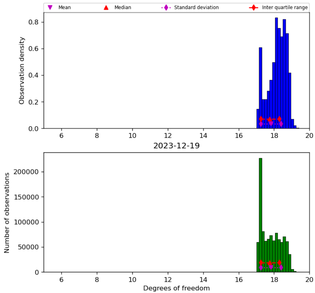
Figure 30: Histogram of “Degrees of freedom” for 2023-12-18 to 2023-12-20
