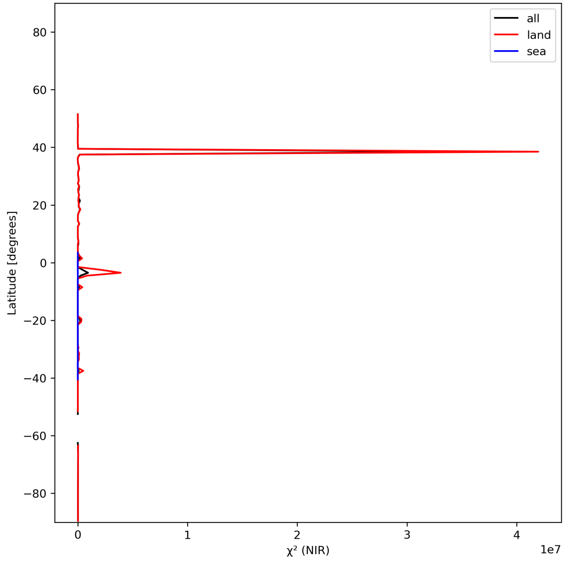
Figure 18: Zonal average of “ \chi^2 (NIR)” for 2023-12-18 to 2023-12-20.
