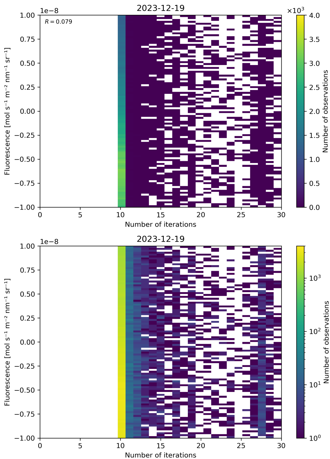
Figure 87: Scatter density plot of “Number of iterations” against “Fluorescence” for 2023-12-18 to 2023-12-20.
