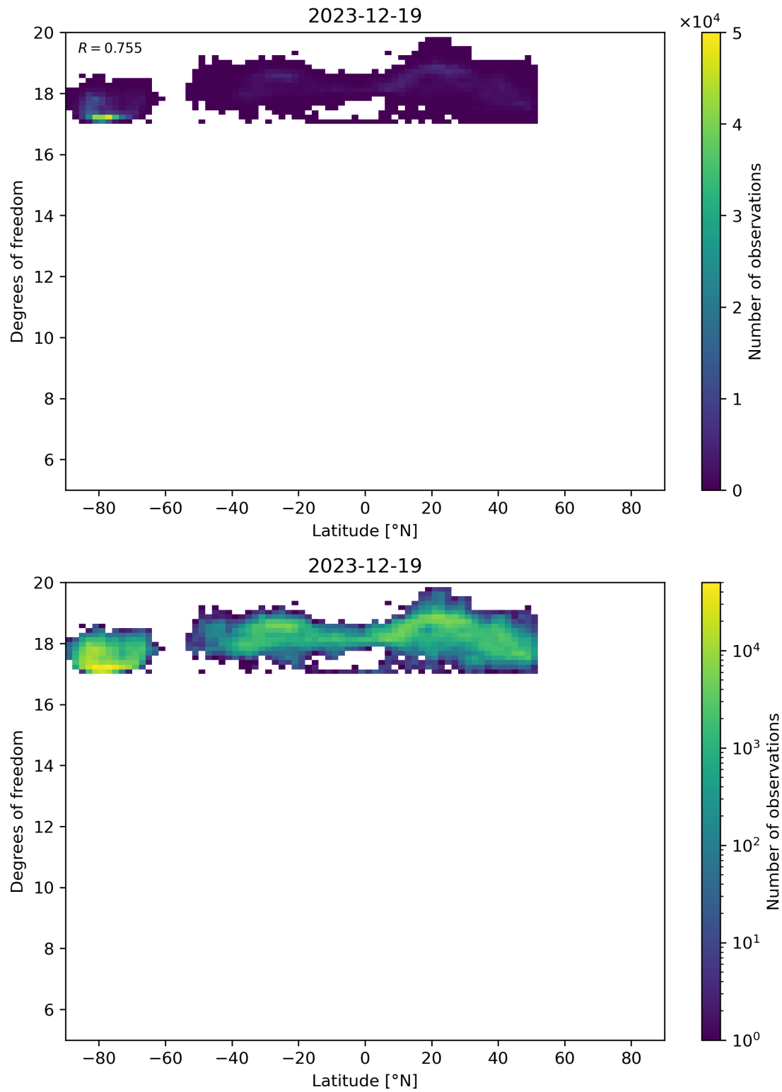
Figure 55: Scatter density plot of “Latitude” against “Degrees of freedom” for 2023-12-18 to 2023-12-20.
