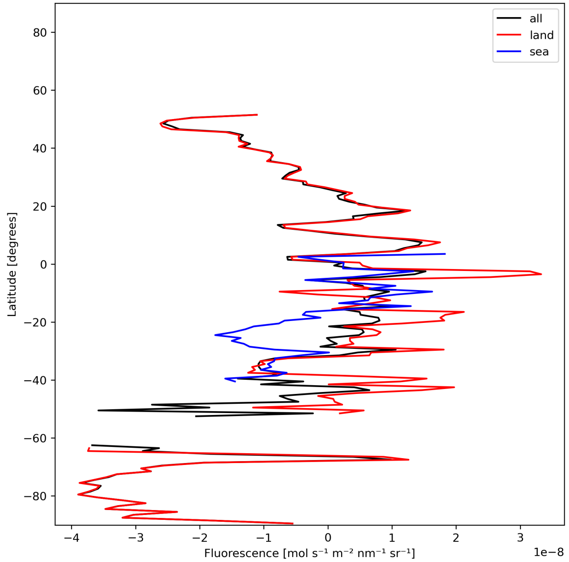
Figure 21: Zonal average of “Fluorescence” for 2023-12-18 to 2023-12-20.
