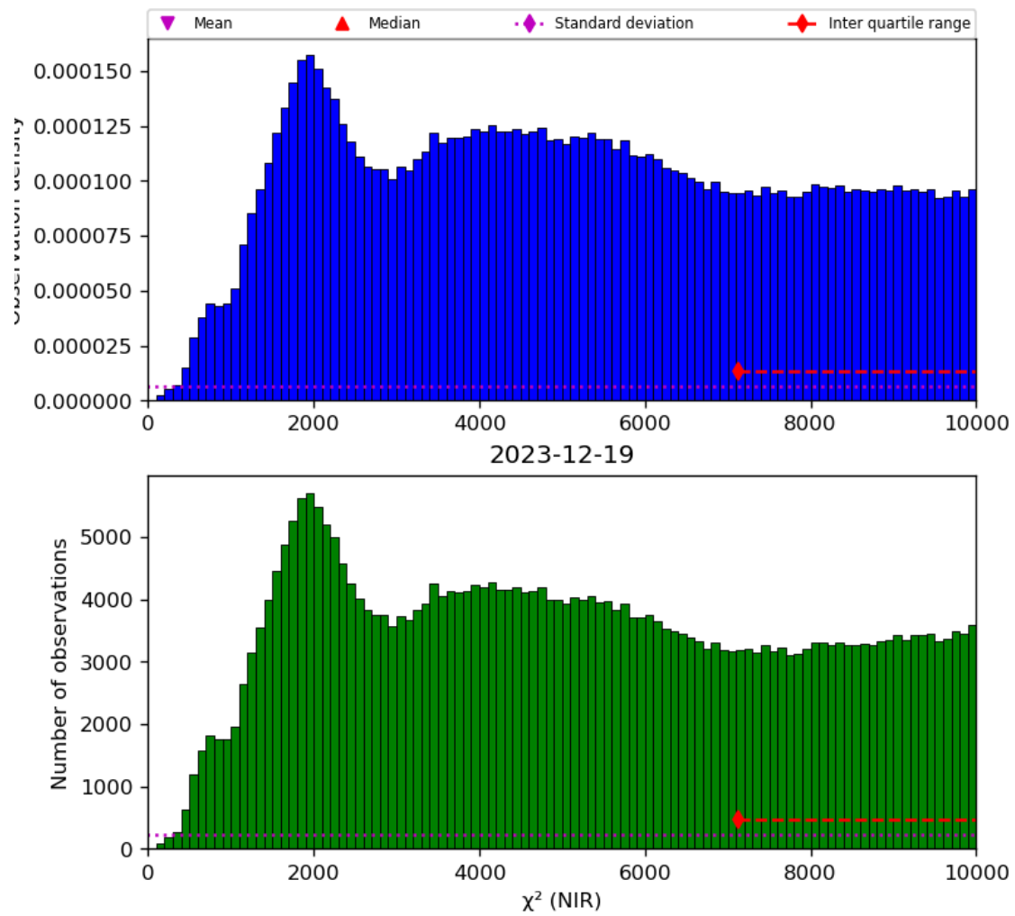
Figure 29: Histogram of “ \chi^2 (NIR)” for 2023-12-18 to 2023-12-20
