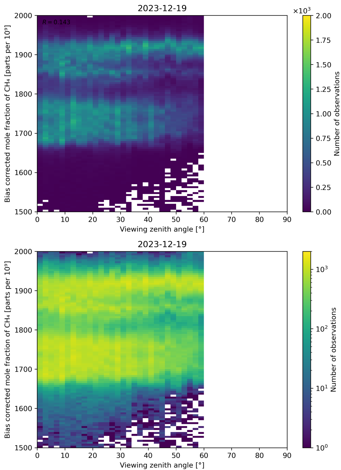
Figure 111: Scatter density plot of “Viewing zenith angle” against “Bias corrected mole fraction of CH 4 ” for 2023-12-18 to 2023-12-20.
