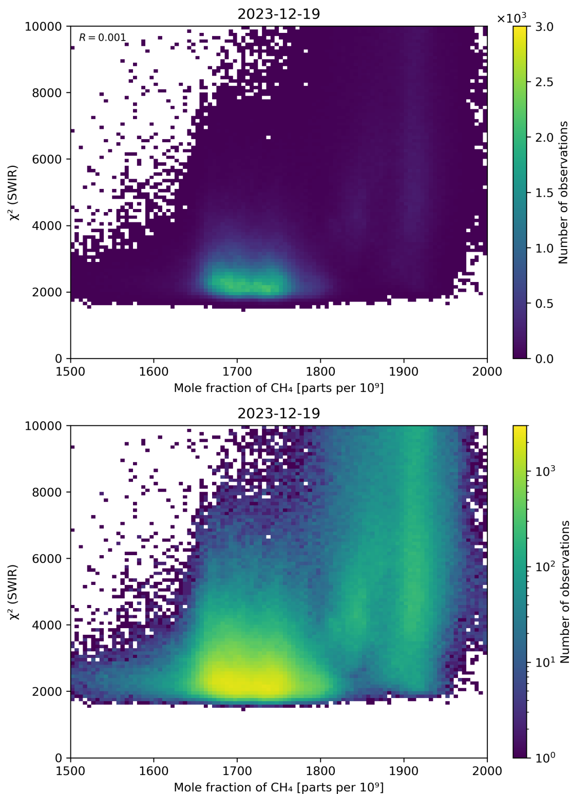
Figure 71: Scatter density plot of “Mole fraction of \text{CH}_4 ” against “ \chi^2 (SWIR)” for 2023-12-18 to 2023-12-20.
