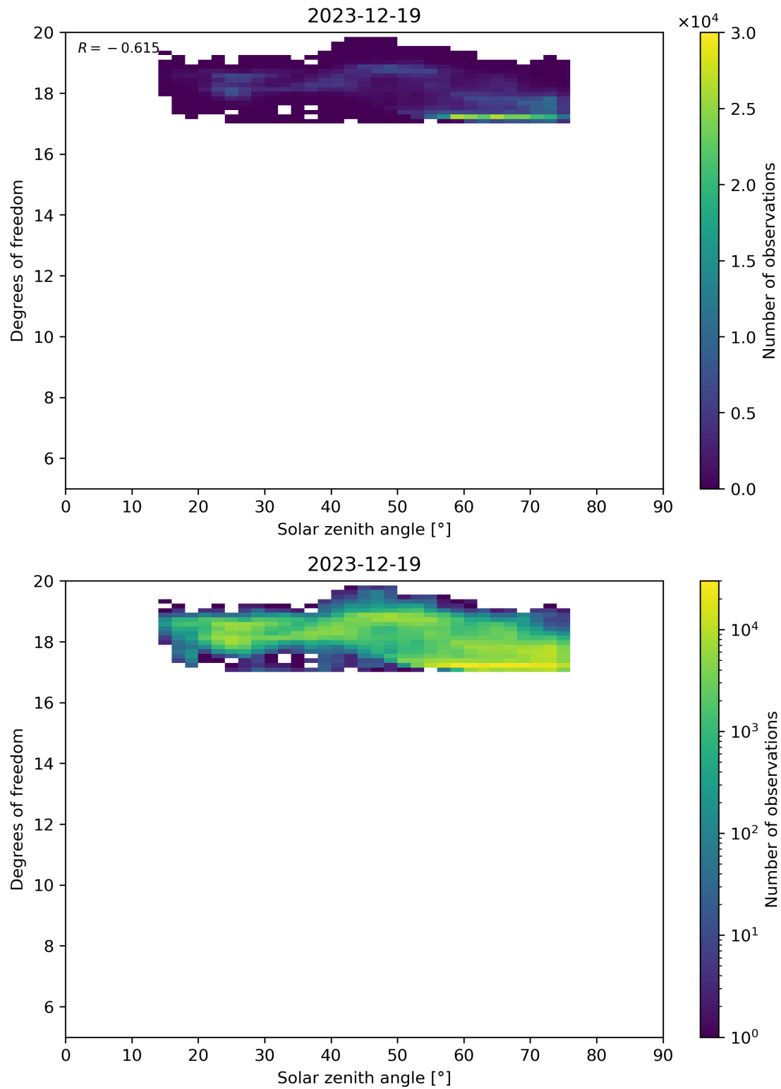
Figure 96: Scatter density plot of “Solar zenith angle” against “Degrees of freedom” for 2023-12-18 to 2023-12-20.
