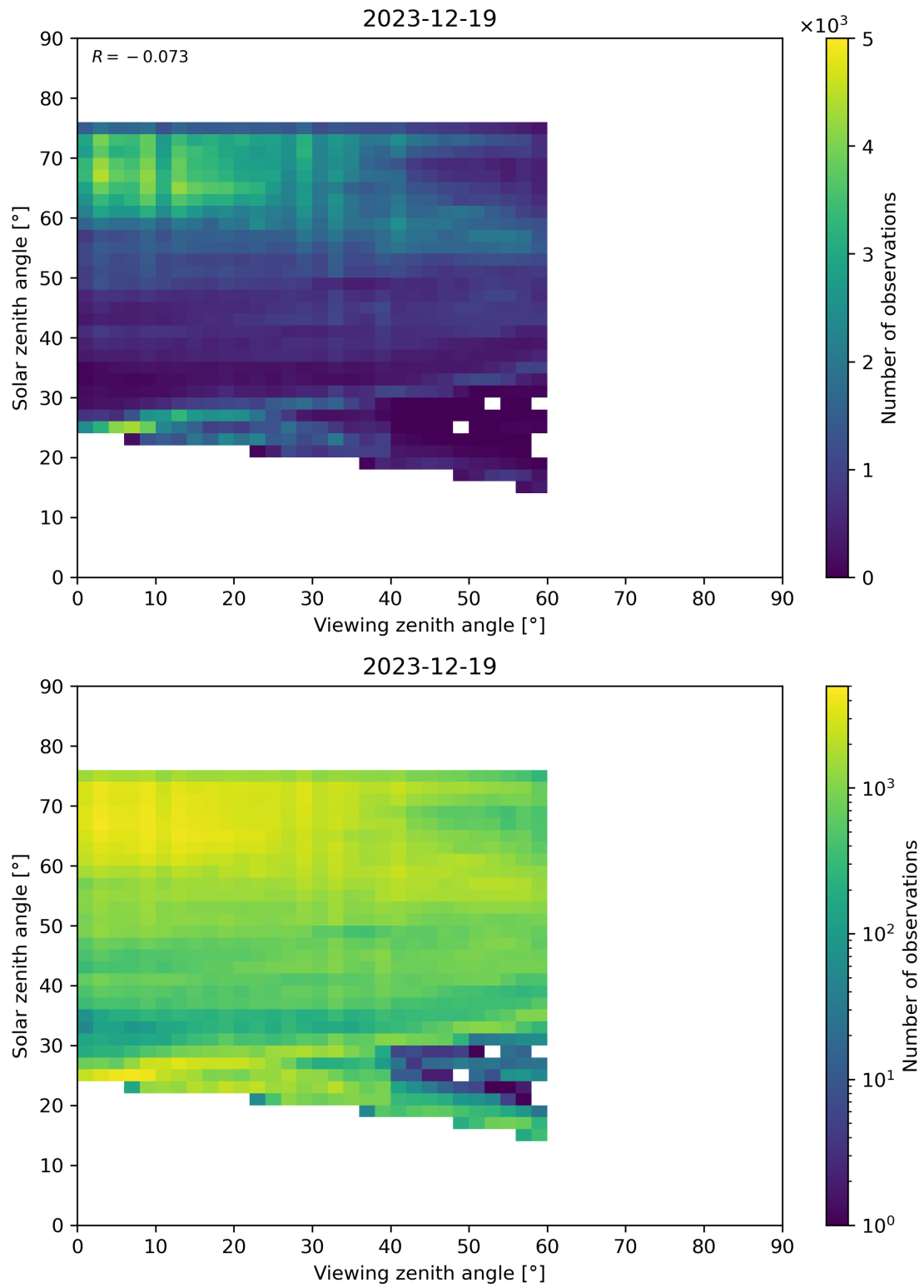
Figure 115: Scatter density plot of “Viewing zenith angle” against “Solar zenith angle” for 2023-12-18 to 2023-12-20.
