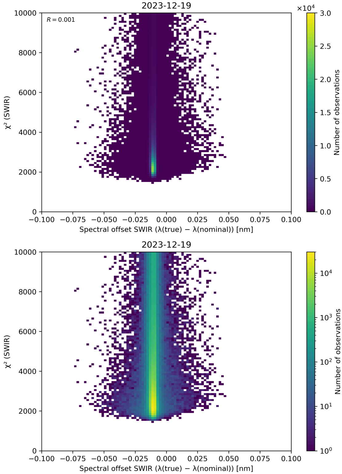
Figure 118: Scatter density plot of “Spectral offset SWIR ( \lambda(\text{true}) - \lambda(\text{nominal}) )” against “ \chi^2 (SWIR)” for 2023-12-18 to 2023-12-20.
