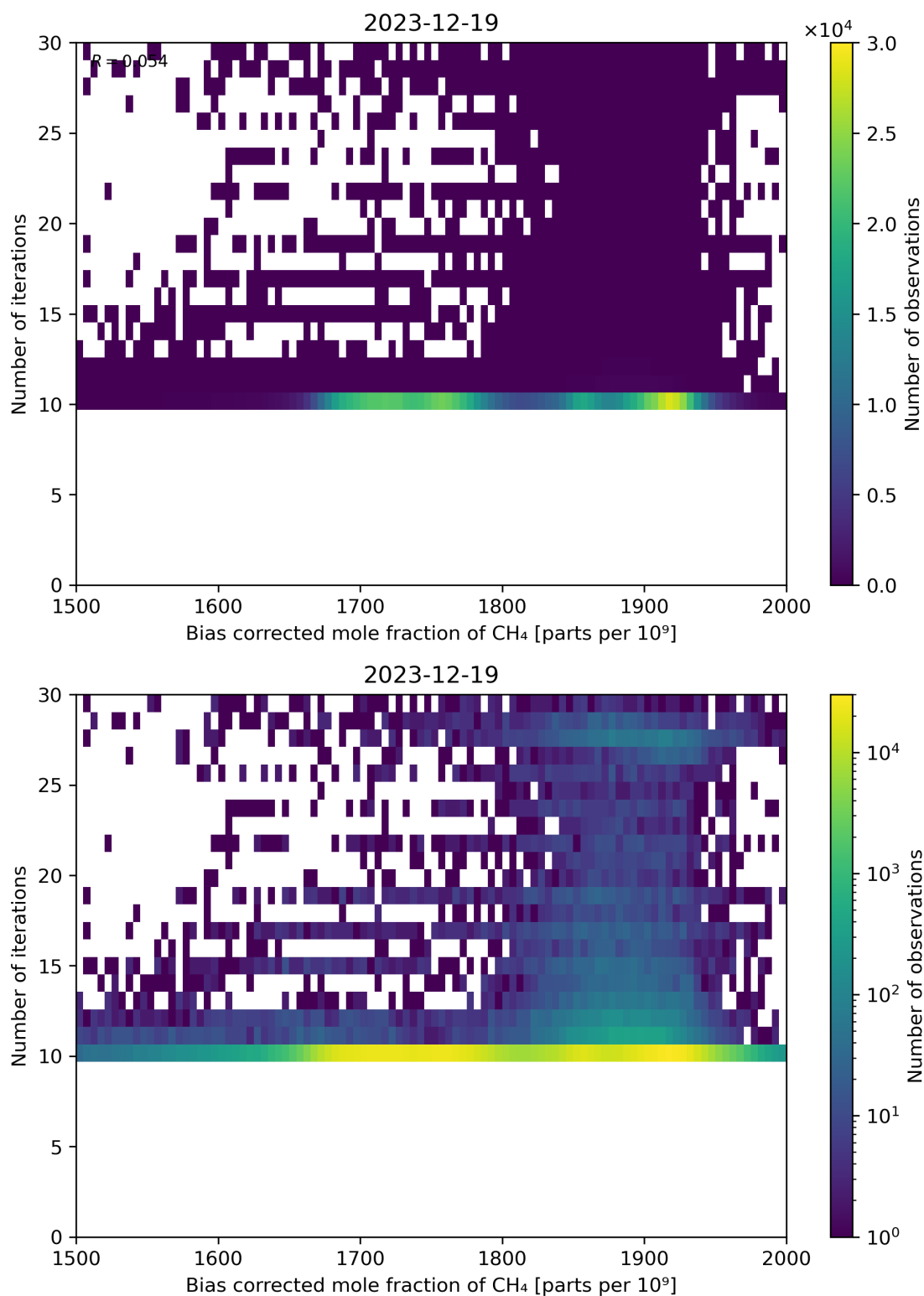
Figure 67: Scatter density plot of “Bias corrected mole fraction of \text{CH}_4 ” against “Number of iterations” for 2023-12-18 to 2023-12-20.
