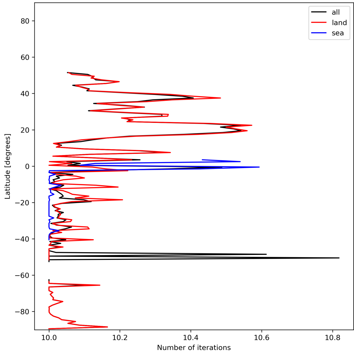
Figure 20: Zonal average of “Number of iterations” for 2023-12-18 to 2023-12-20.
