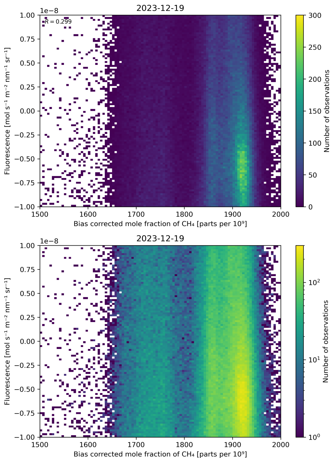
Figure 66: Scatter density plot of “Bias corrected mole fraction of \text{CH}_4 ” against “Fluorescence” for 2023-12-18 to 2023-12-20.
