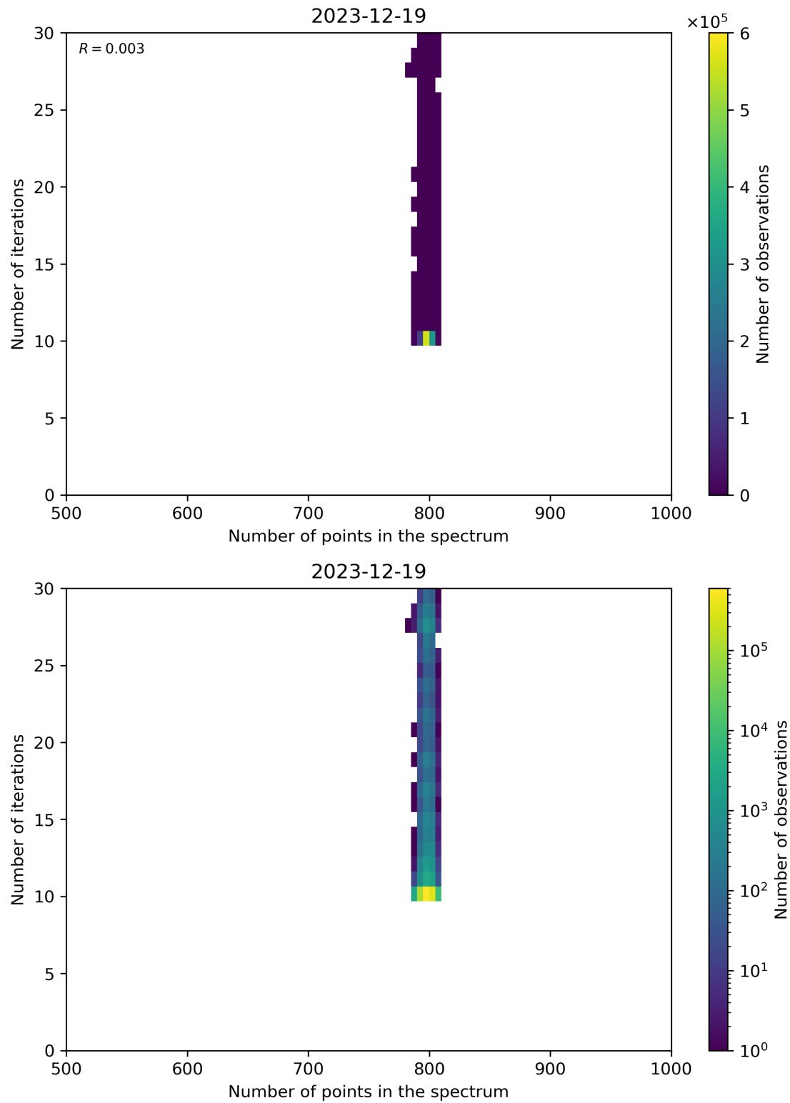
Figure 92: Scatter density plot of “Number of points in the spectrum” against “Number of iterations” for 2023-12-18 to 2023-12-20.
