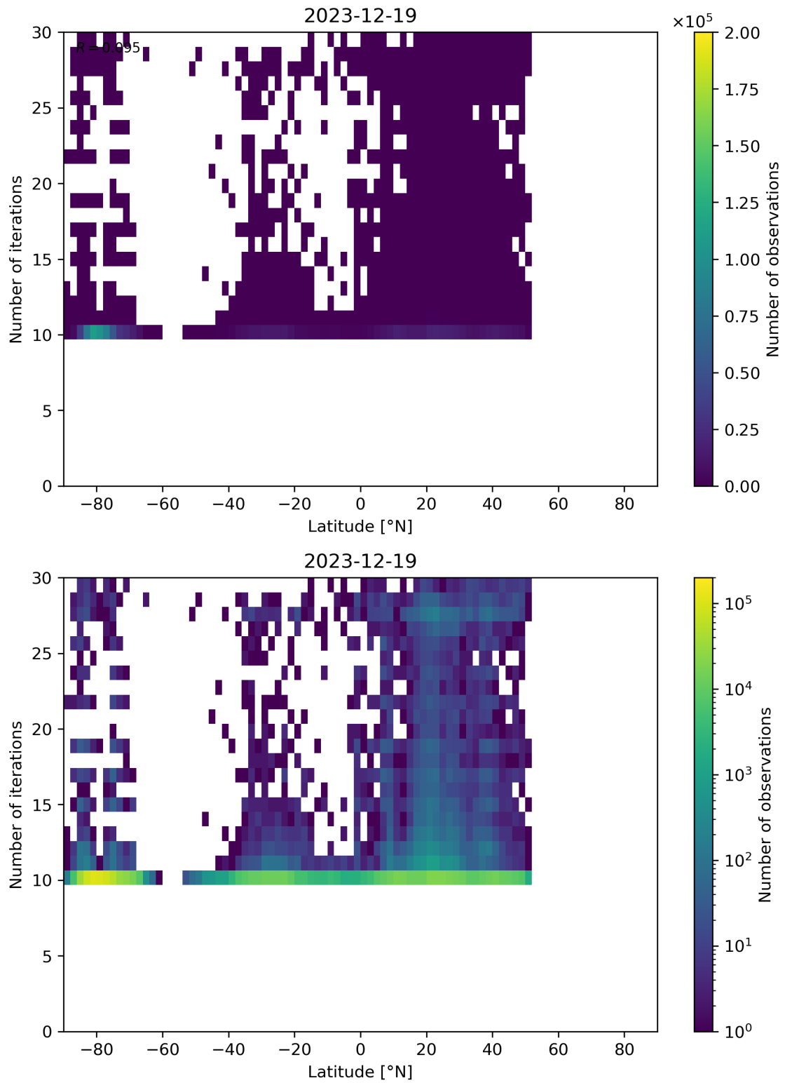
Figure 60: Scatter density plot of “Latitude” against “Number of iterations” for 2023-12-18 to 2023-12-20.
