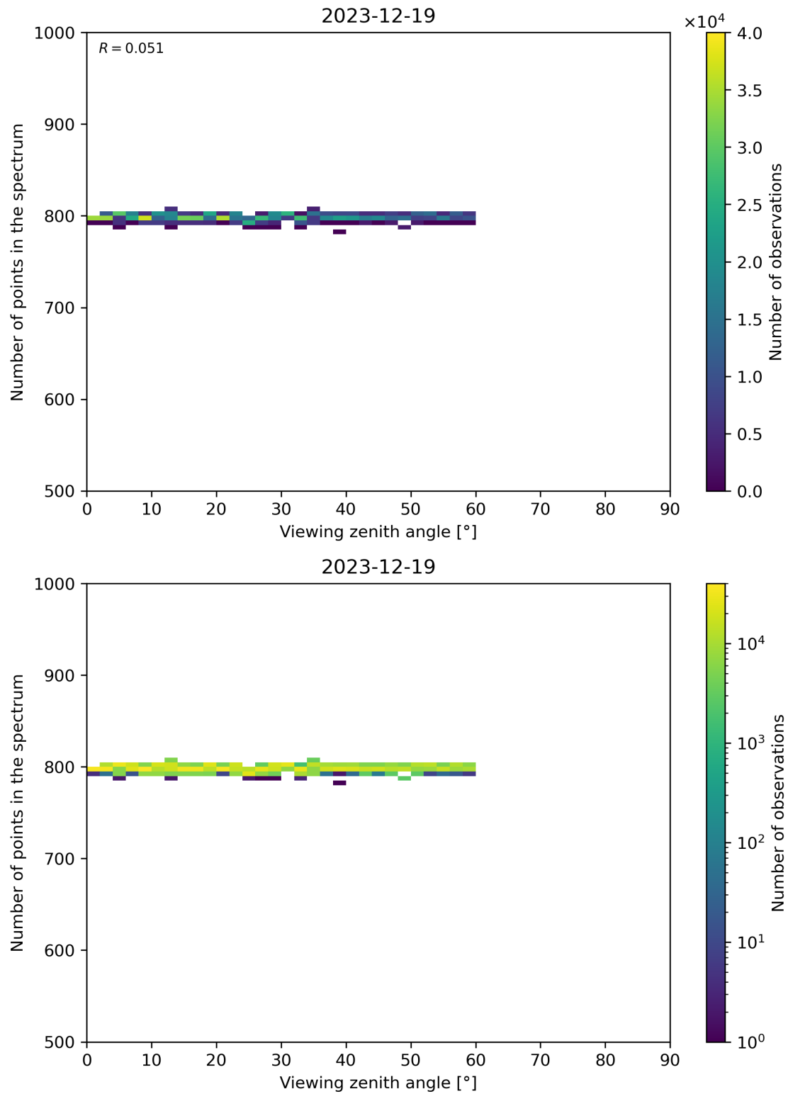
Figure 114: Scatter density plot of “Viewing zenith angle” against “Number of points in the spectrum” for 2023-12-18 to 2023-12-20.
