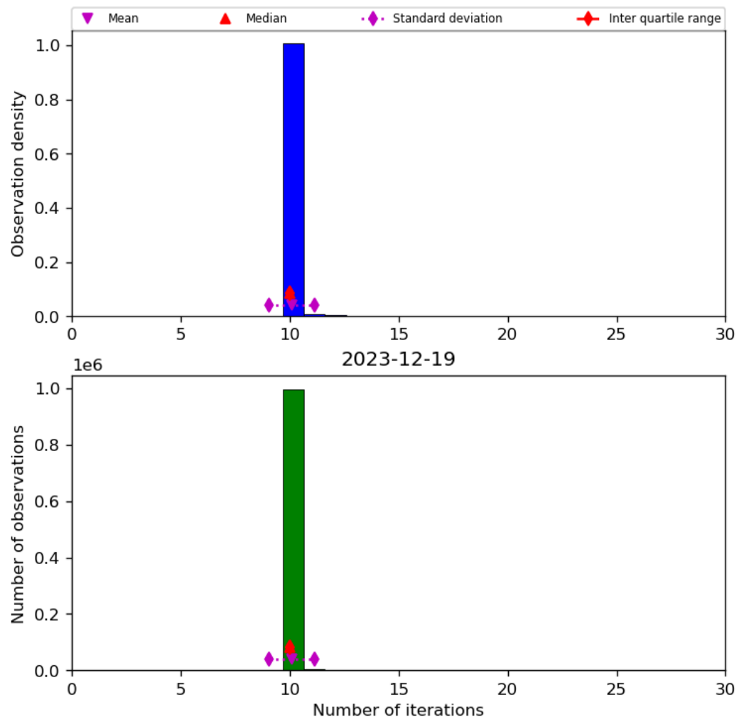
Figure 31: Histogram of “Number of iterations” for 2023-12-18 to 2023-12-20
