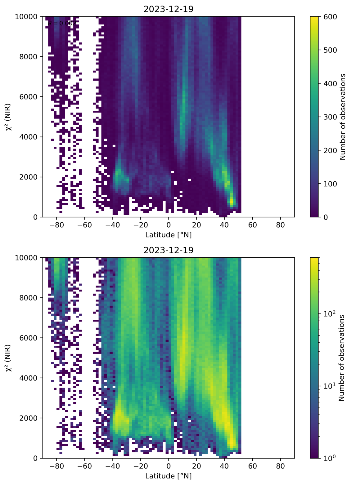
Figure 53: Scatter density plot of “Latitude” against “ \chi^2 (NIR)” for 2023-12-18 to 2023-12-20.
