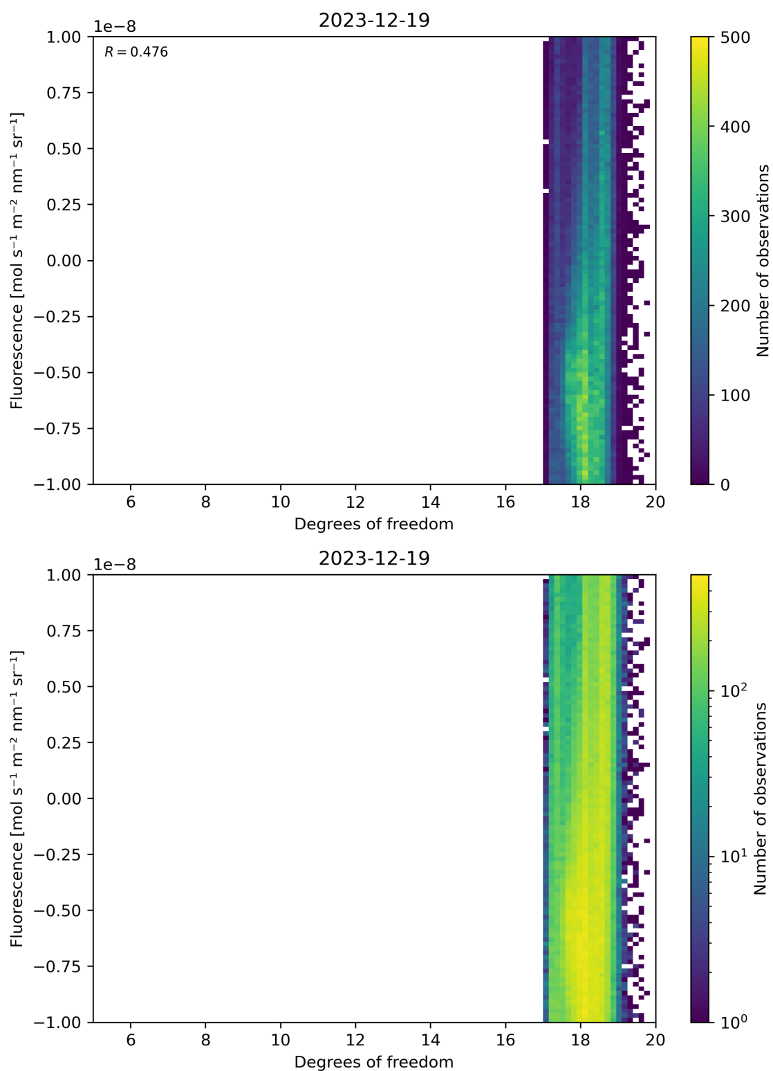
Figure 51: Scatter density plot of “Degrees of freedom” against “Fluorescence” for 2023-12-18 to 2023-12-20.
