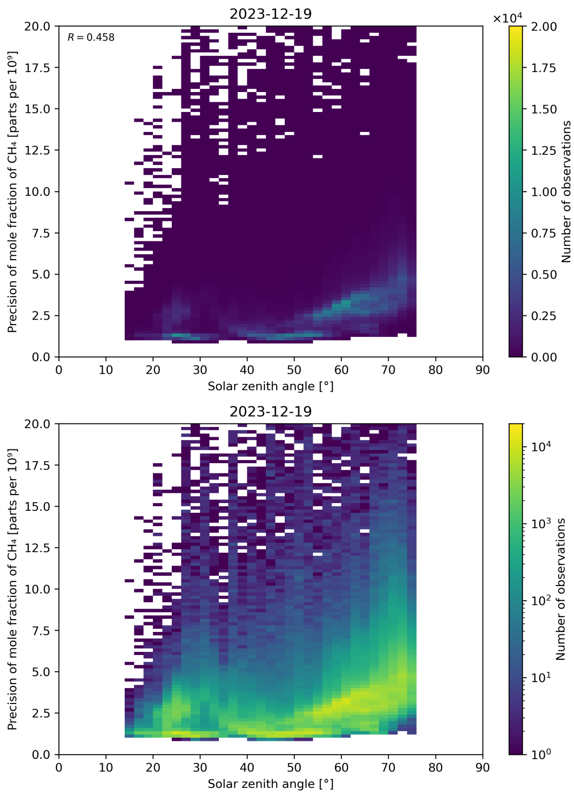
Figure 101: Scatter density plot of “Solar zenith angle” against “Precision of mole fraction of \text{CH}_4 ” for 2023-12-18 to 2023-12-20.
