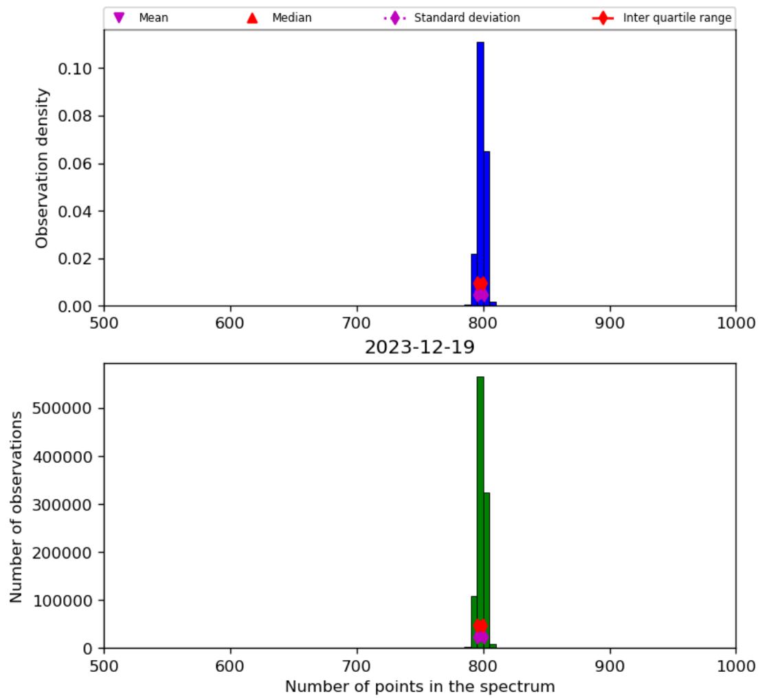
Figure 26: Histogram of “Number of points in the spectrum” for 2023-12-18 to 2023-12-20
