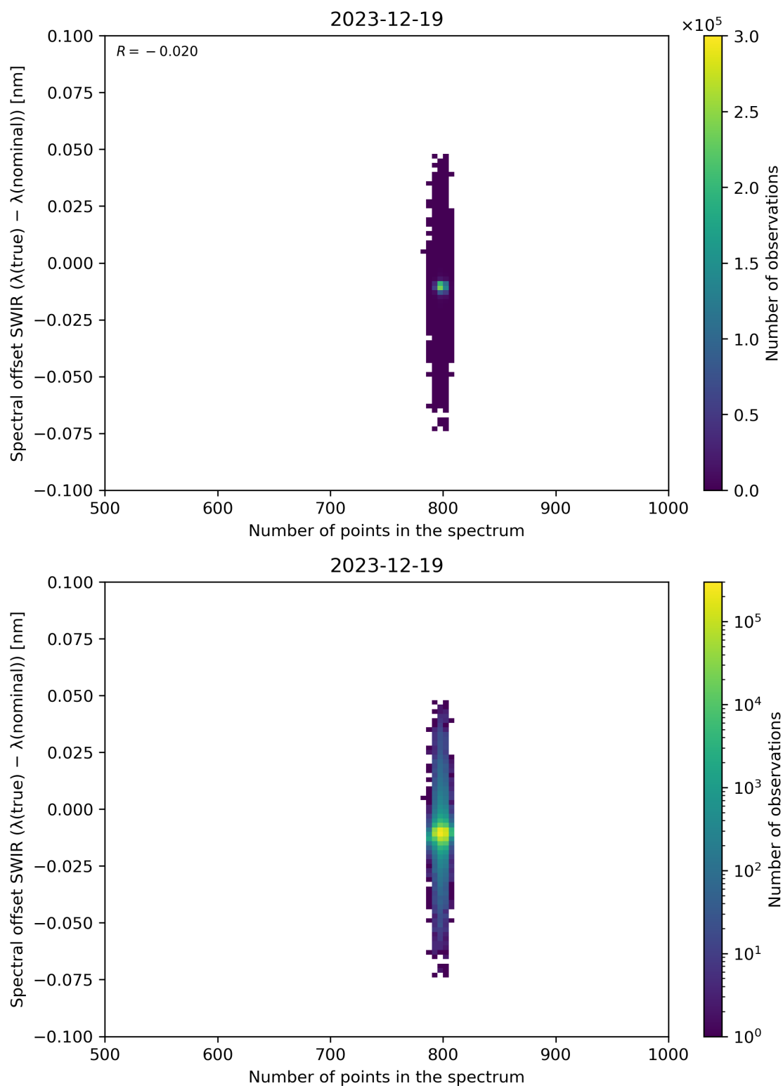
Figure 93: Scatter density plot of “Number of points in the spectrum” against “Spectral offset SWIR ( \lambda(\text{true}) - \lambda(\text{nominal}) )” for 2023-12-18 to 2023-12-20.
