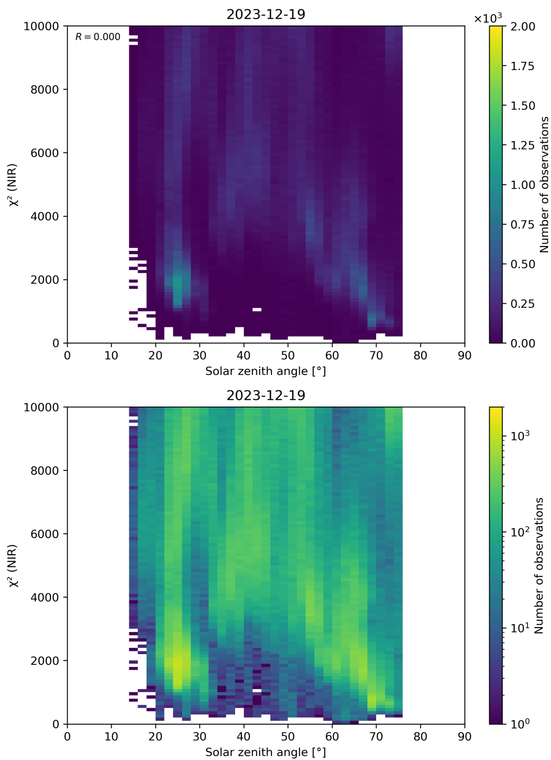
Figure 94: Scatter density plot of “Solar zenith angle” against “ \chi^2 (NIR)” for 2023-12-18 to 2023-12-20.
