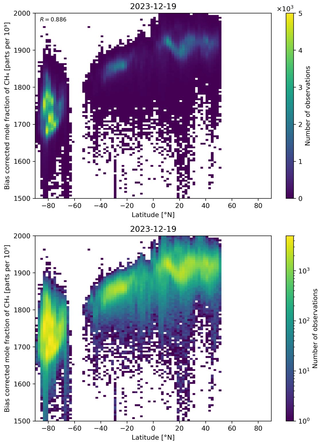
Figure 58: Scatter density plot of “Latitude” against “Bias corrected mole fraction of \text{CH}_4 ” for 2023-12-18 to 2023-12-20.
