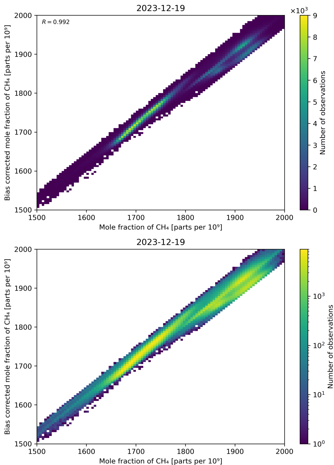
Figure 74: Scatter density plot of “Mole fraction of CH 4 ” against “Bias corrected mole fraction of CH 4 ” for 2023-12-18 to 2023-12-20.
