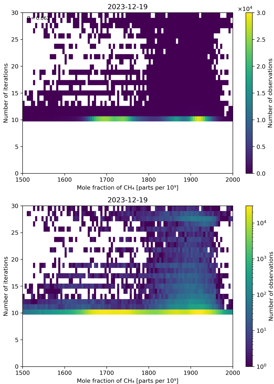
Figure 76: Scatter density plot of “Mole fraction of CH 4 ” against “Number of iterations” for 2023-12-18 to 2023-12-20.
