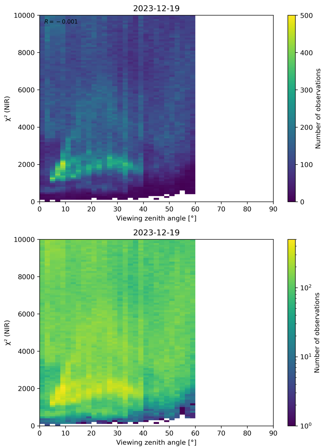
Figure 105: Scatter density plot of “Viewing zenith angle” against “ \chi^2 (NIR)” for 2023-12-18 to 2023-12-20.
