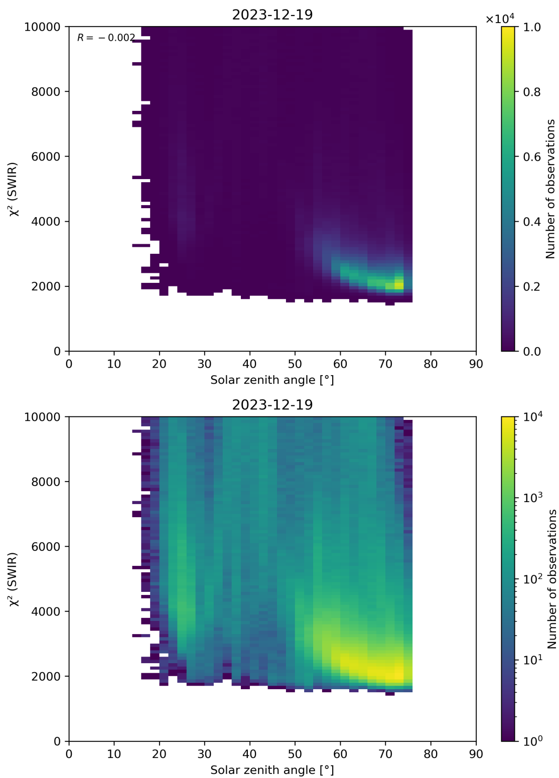
Figure 95: Scatter density plot of “Solar zenith angle” against “ \chi^2 (SWIR)” for 2023-12-18 to 2023-12-20.
