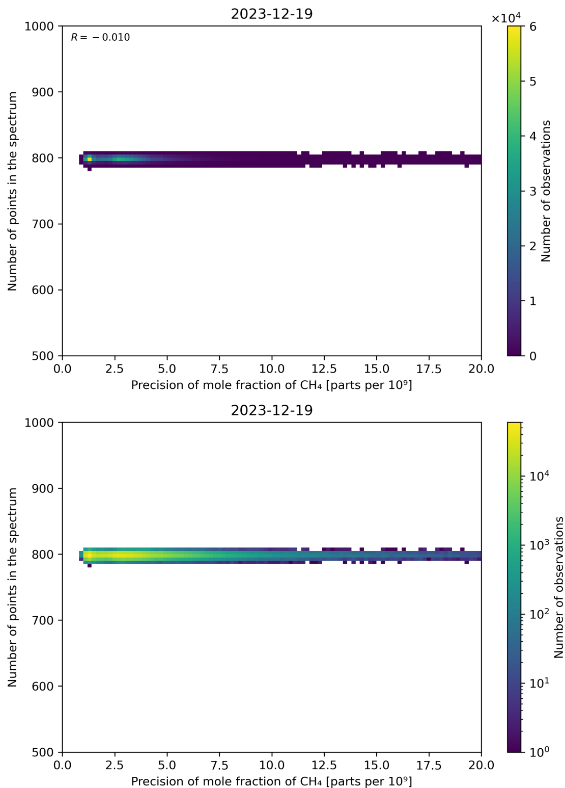
Figure 84: Scatter density plot of “Precision of mole fraction of CH 4 ” against “Number of points in the spectrum” for 2023-12-18 to 2023-12-20.
