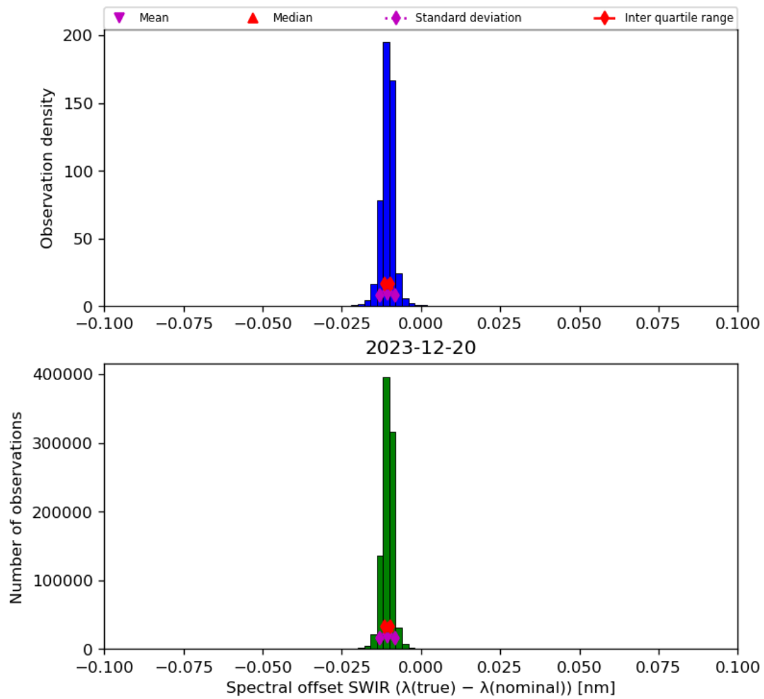
Figure 27: Histogram of “Spectral offset SWIR ( \lambda(\text{true}) - \lambda(\text{nominal}) )” for 2023-12-20 to 2023-12-21
