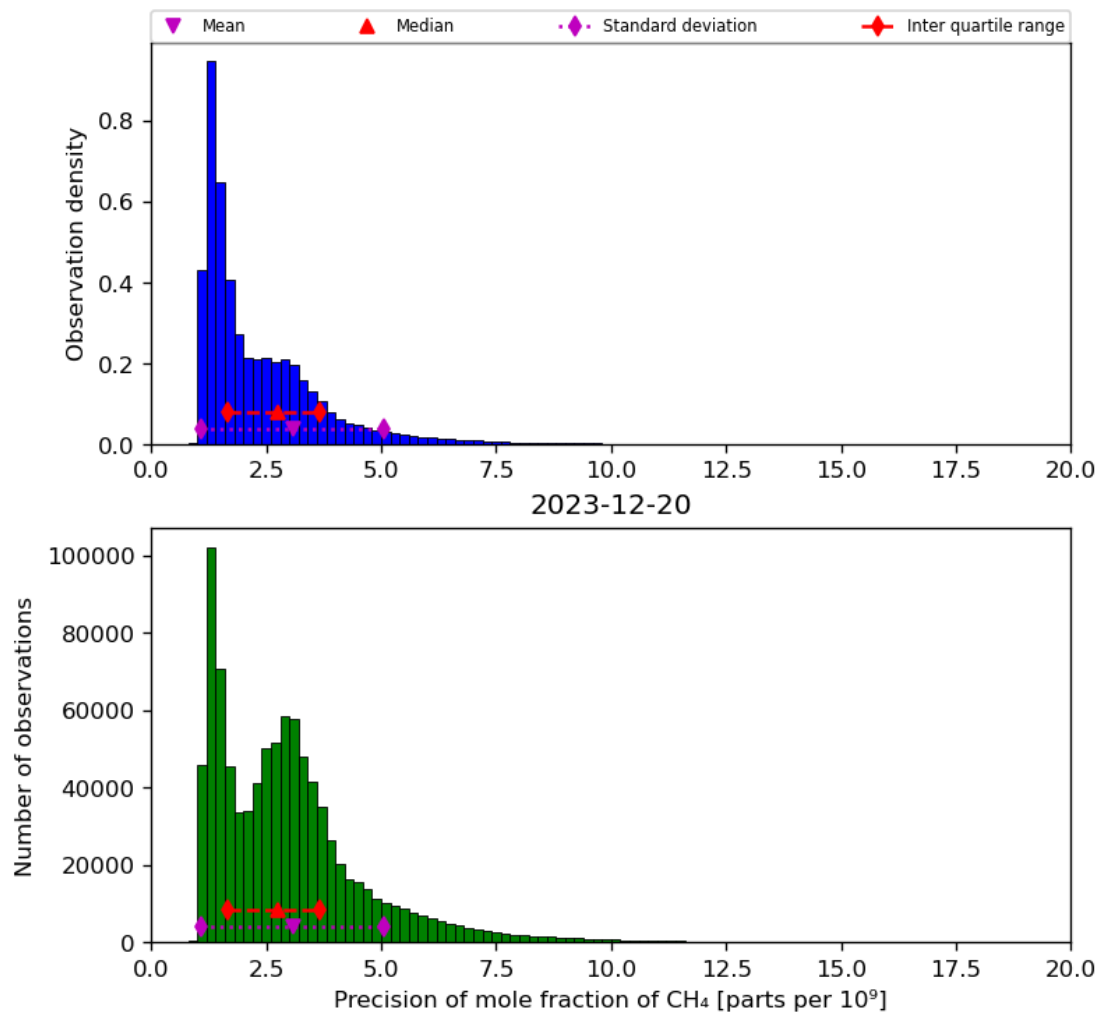
Figure 24: Histogram of “Precision of mole fraction of CH 4 ” for 2023-12-20 to 2023-12-21
