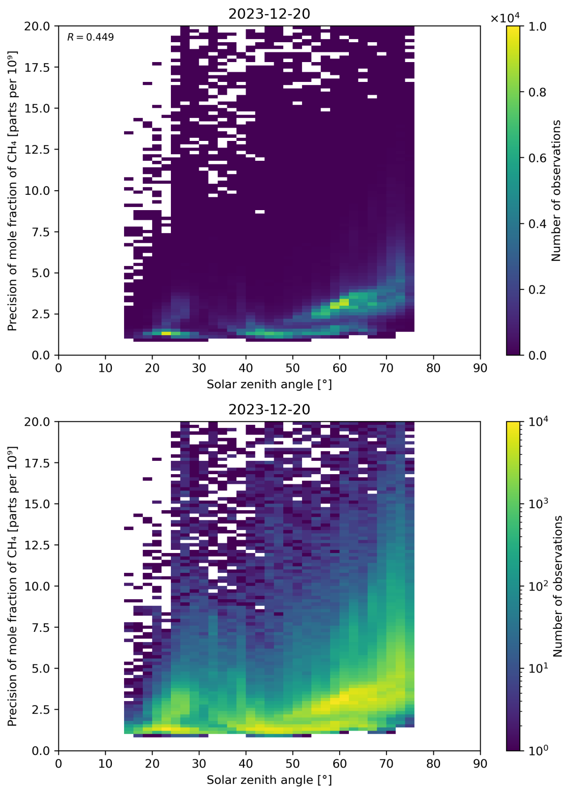
Figure 101: Scatter density plot of “Solar zenith angle” against “Precision of mole fraction of \text{CH}_4 ” for 2023-12-20 to 2023-12-21.
