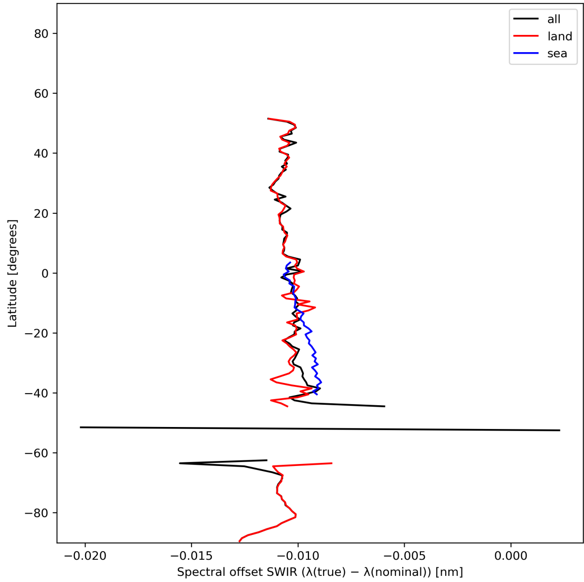
Figure 16: Zonal average of “Spectral offset SWIR ( \lambda(\text{true}) - \lambda(\text{nominal}) )” for 2023-12-20 to 2023-12-21.
