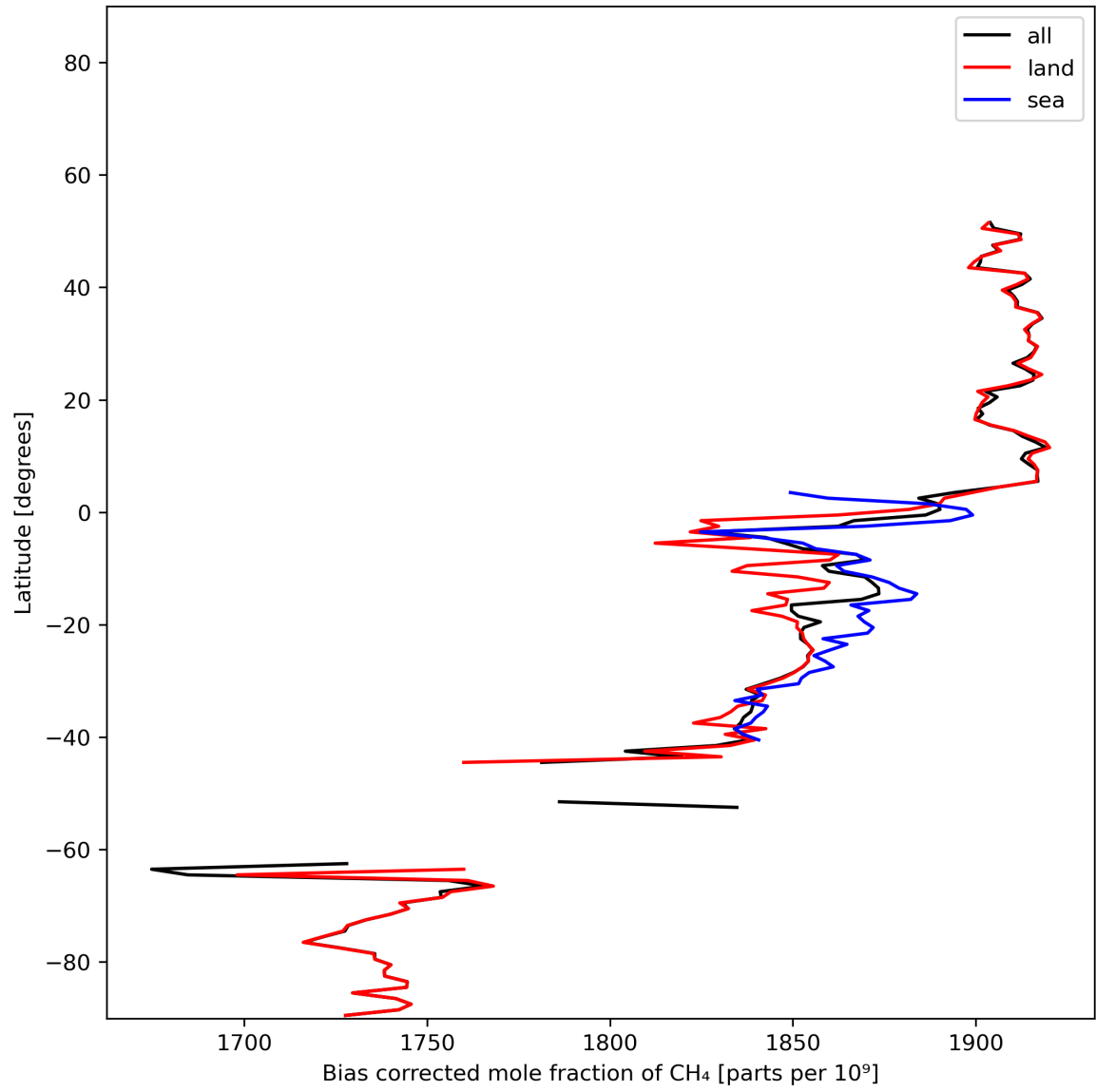
Figure 14: Zonal average of “Bias corrected mole fraction of CH 4 ” for 2023-12-20 to 2023-12-21.
