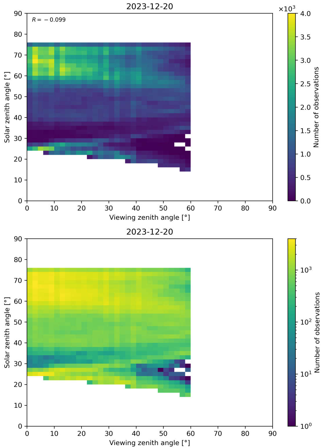
Figure 115: Scatter density plot of “Viewing zenith angle” against “Solar zenith angle” for 2023-12-20 to 2023-12-21.
