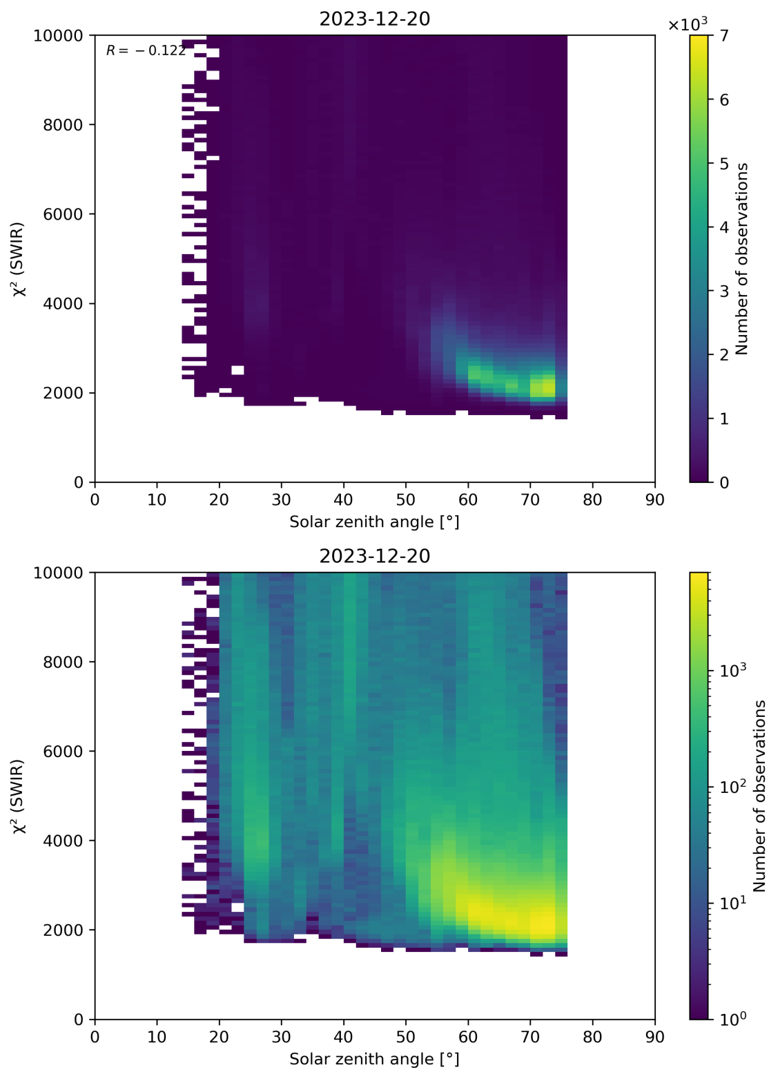
Figure 95: Scatter density plot of “Solar zenith angle” against “ \chi^2 (SWIR)” for 2023-12-20 to 2023-12-21.
