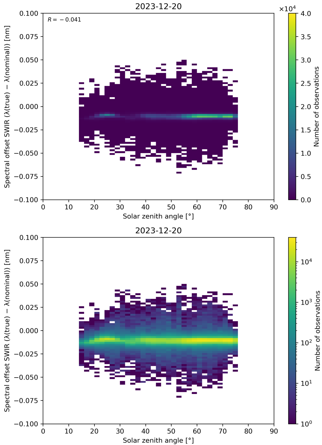
Figure 104: Scatter density plot of “Solar zenith angle” against “Spectral offset SWIR ( \lambda(\text{true}) - \lambda(\text{nominal}) )” for 2023-12-20 to 2023-12-21.
