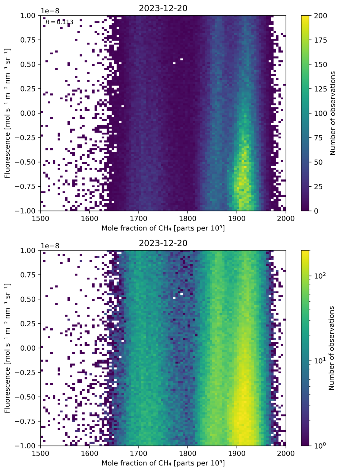
Figure 73: Scatter density plot of “Mole fraction of \text{CH}_4 ” against “Fluorescence” for 2023-12-20 to 2023-12-21.
