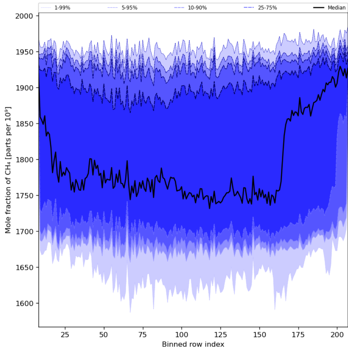
Figure 34: Along track statistics of “Mole fraction of CH 4 ” for 2023-12-20 to 2023-12-21
