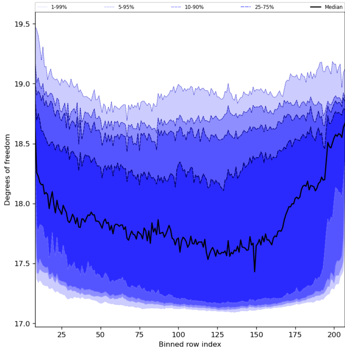
Figure 41: Along track statistics of “Degrees of freedom” for 2023-12-20 to 2023-12-21
