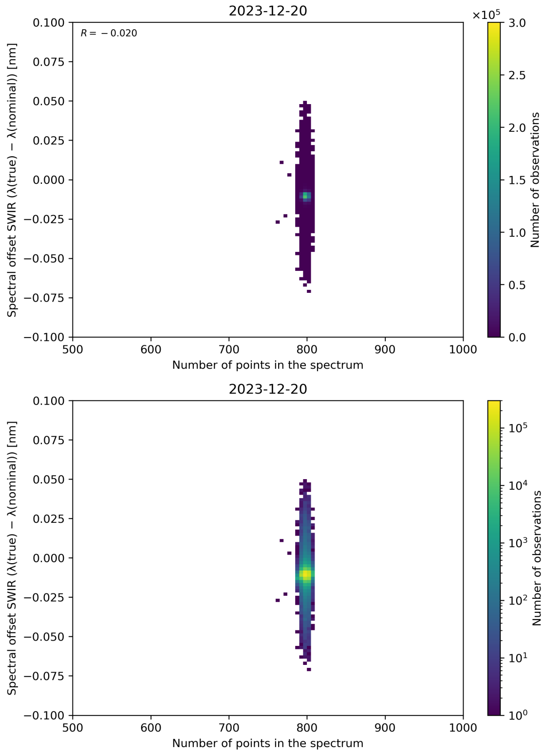
Figure 93: Scatter density plot of “Number of points in the spectrum” against “Spectral offset SWIR ( \lambda(\text{true}) - \lambda(\text{nominal}) )” for 2023-12-20 to 2023-12-21.
