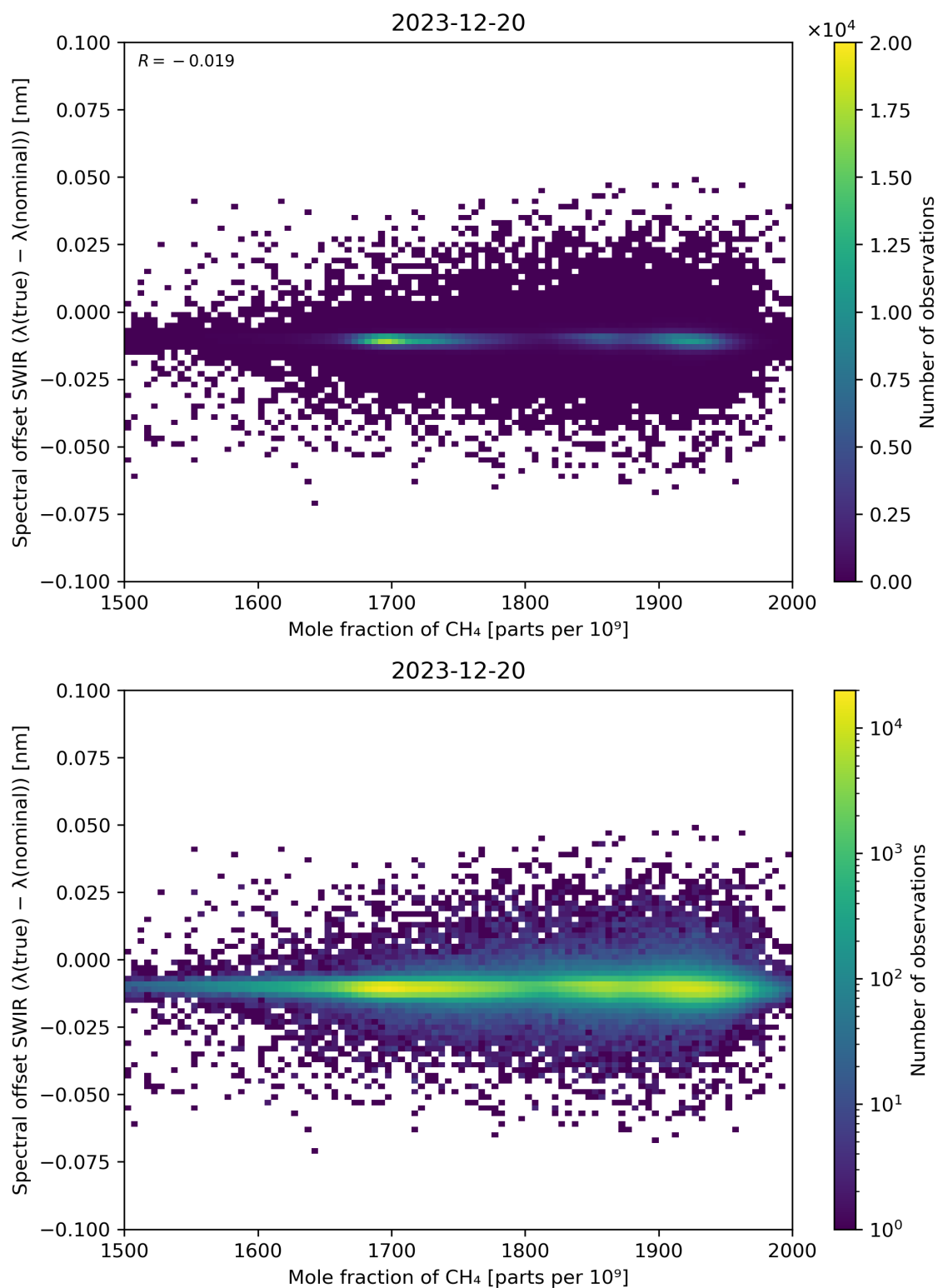
Figure 86: Scatter density plot of “Mole fraction of CH 4 ” against “Spectral offset SWIR ( \lambda(\text{true}) - \lambda(\text{nominal}) )” for 2023-12-20 to 2023-12-21.
