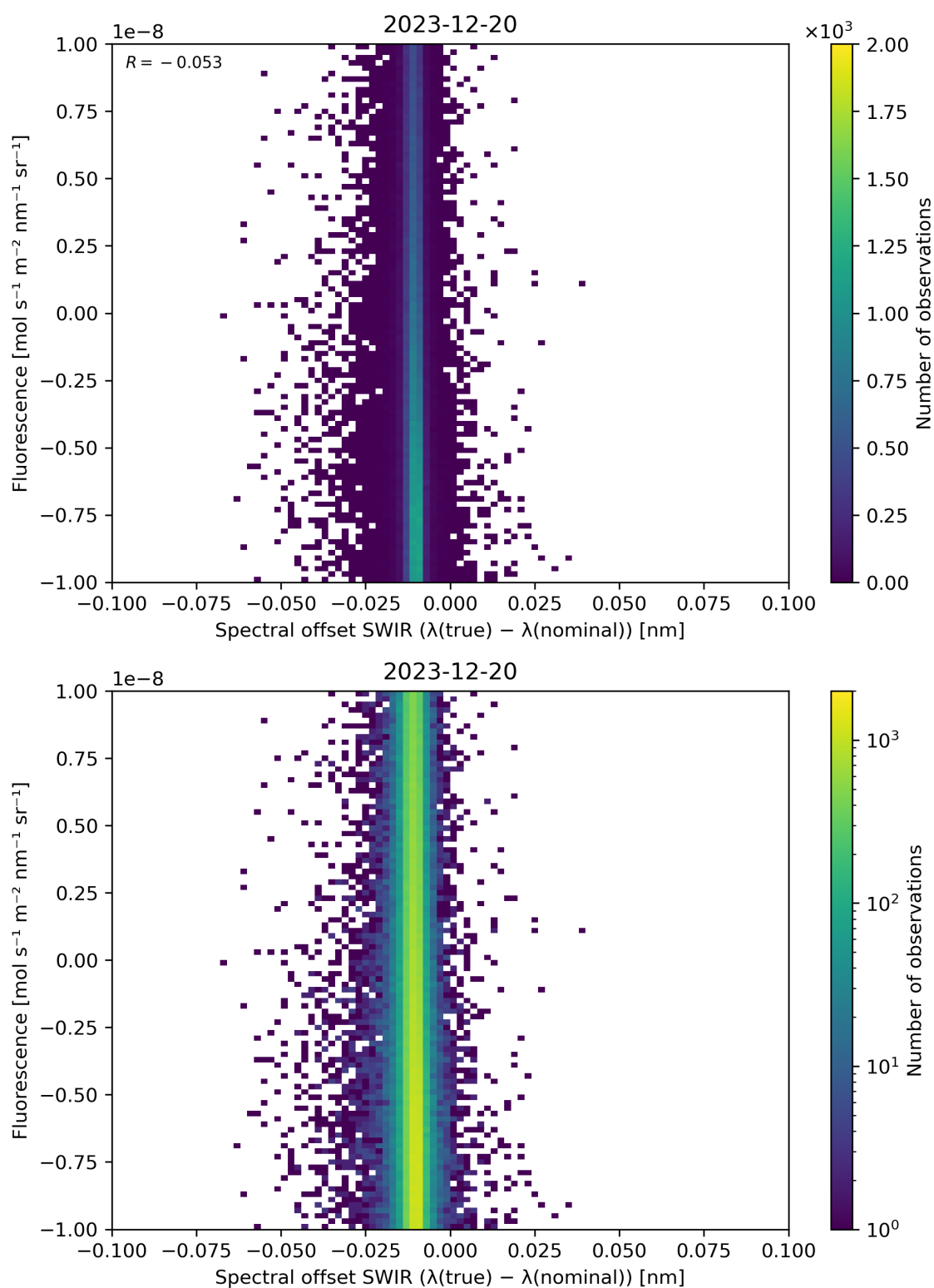
Figure 120: Scatter density plot of “Spectral offset SWIR ( \lambda(\text{true}) - \lambda(\text{nominal}) )” against “Fluorescence” for 2023-12-20 to 2023-12-21.
