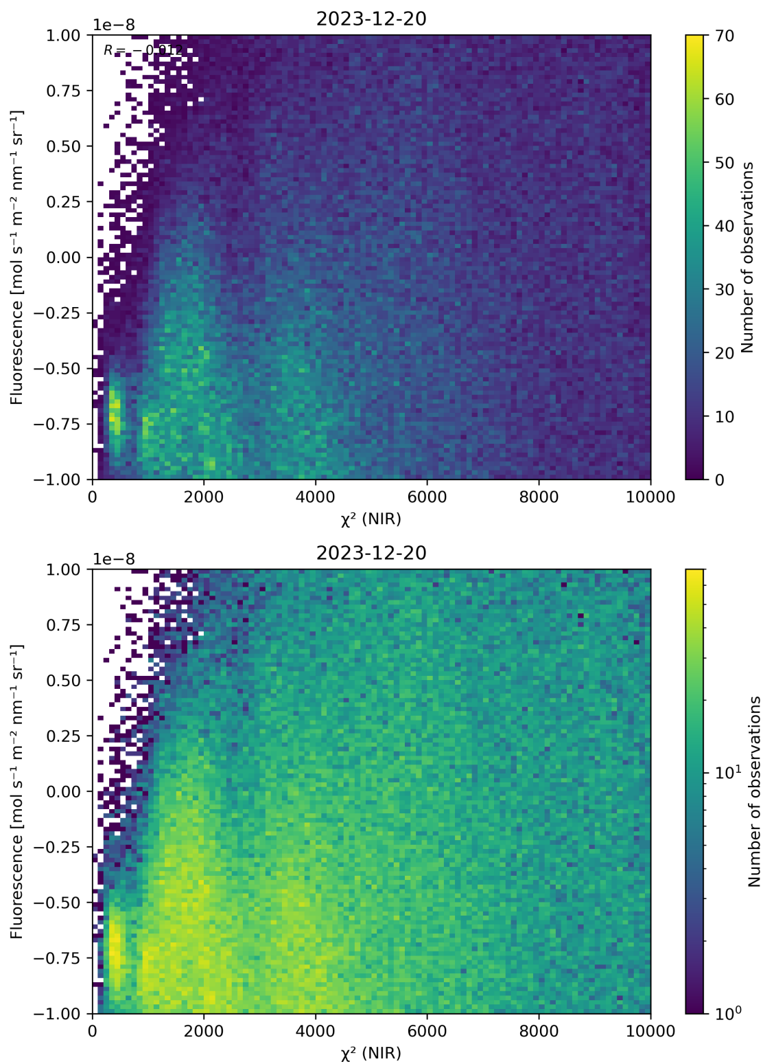
Figure 45: Scatter density plot of “ \chi^2 (NIR)” against “Fluorescence” for 2023-12-20 to 2023-12-21.
