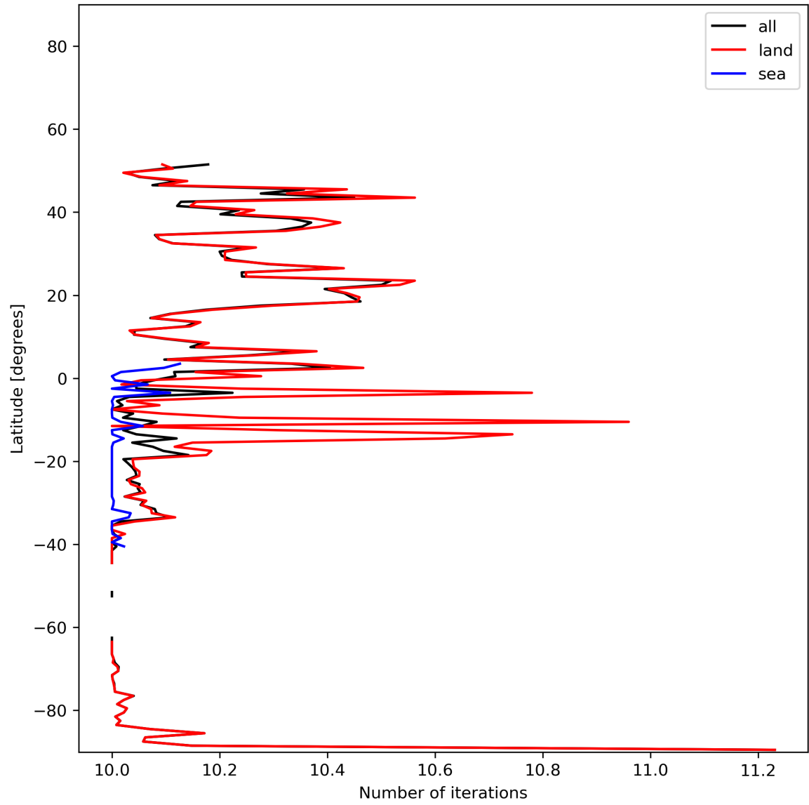
Figure 20: Zonal average of “Number of iterations” for 2023-12-20 to 2023-12-21.
