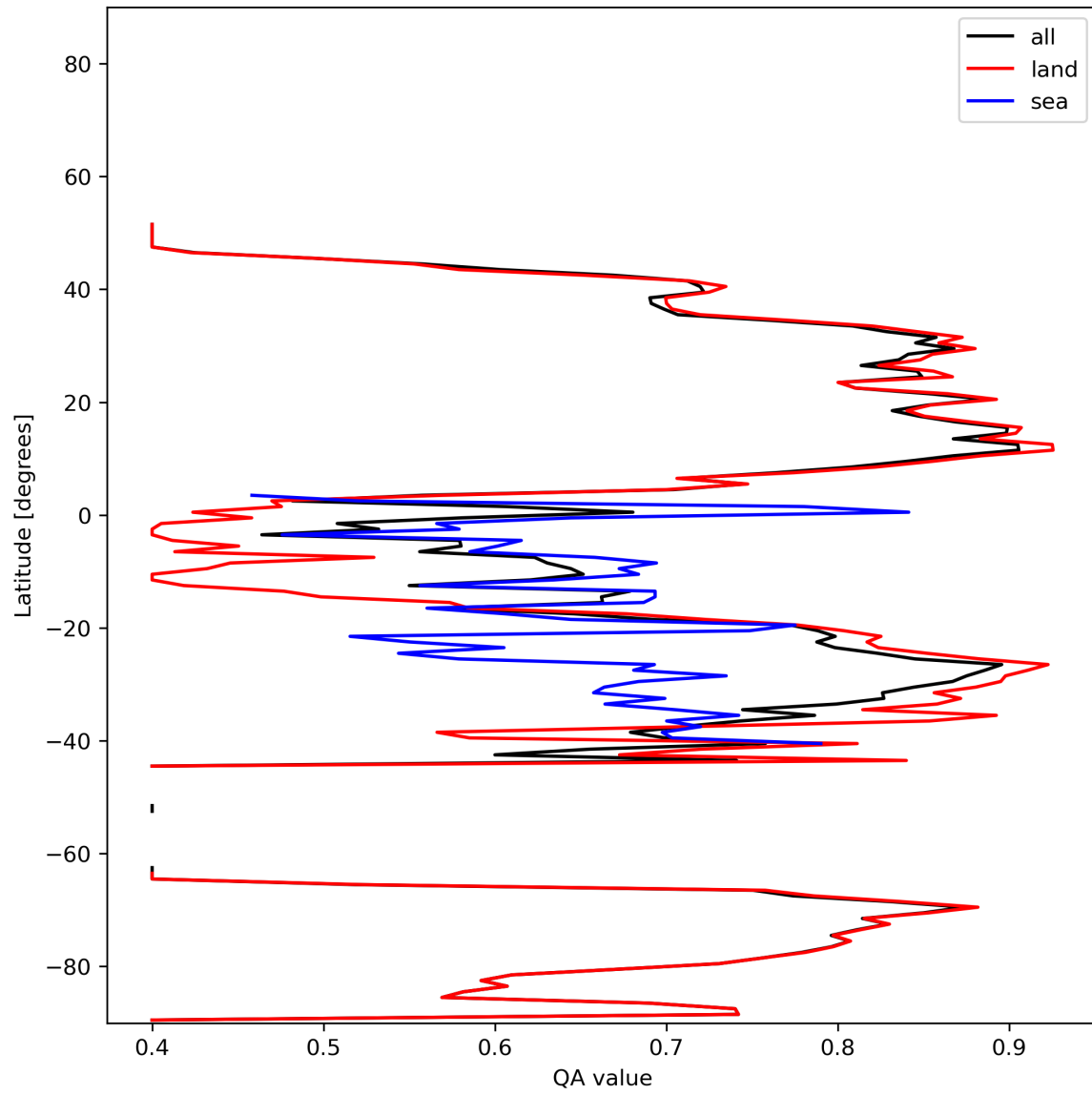
Figure 11: Zonal average of “QA value” for 2023-12-20 to 2023-12-21.
