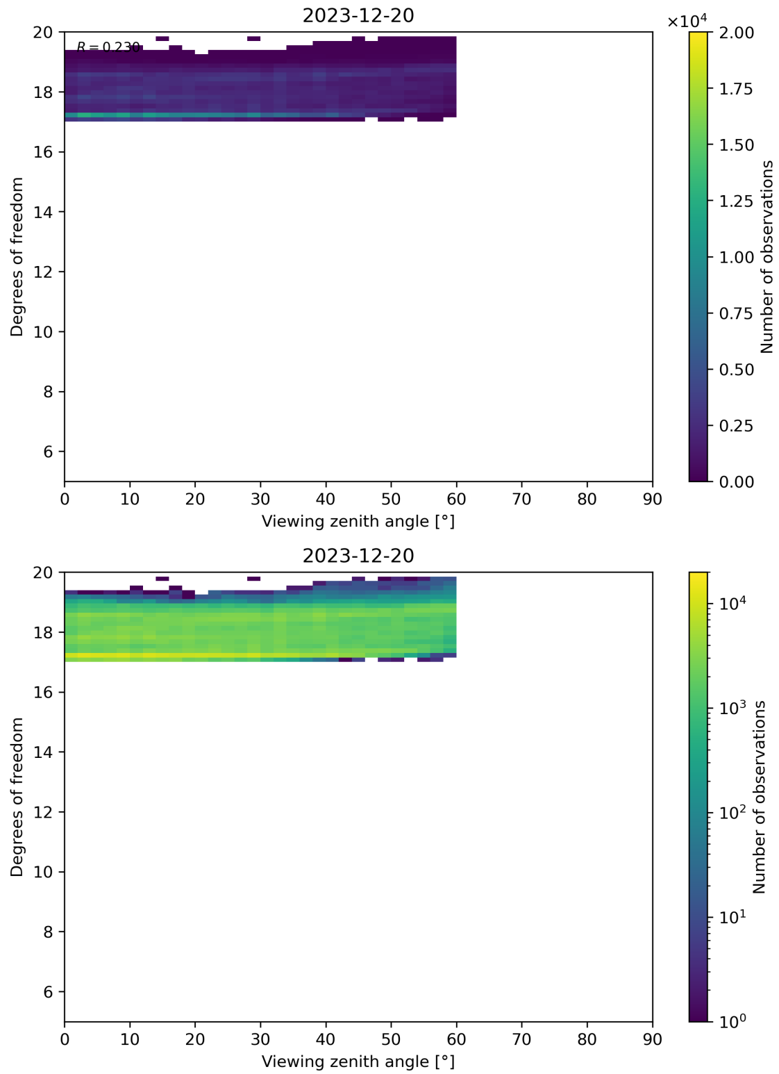
Figure 107: Scatter density plot of “Viewing zenith angle” against “Degrees of freedom” for 2023-12-20 to 2023-12-21.
