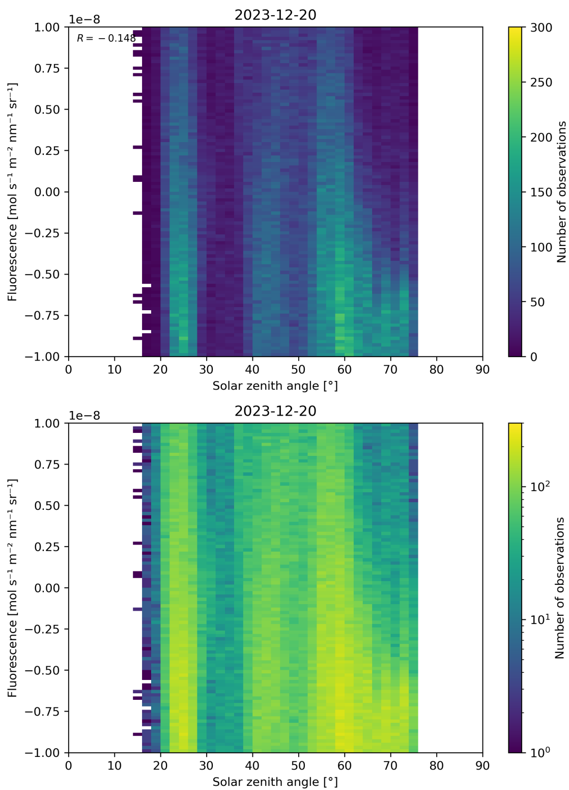
Figure 97: Scatter density plot of “Solar zenith angle” against “Fluorescence” for 2023-12-20 to 2023-12-21.
