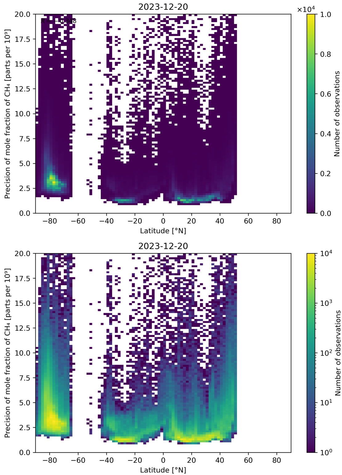
Figure 59: Scatter density plot of “Latitude” against “Precision of mole fraction of CH 4 ” for 2023-12-20 to 2023-12-21.
