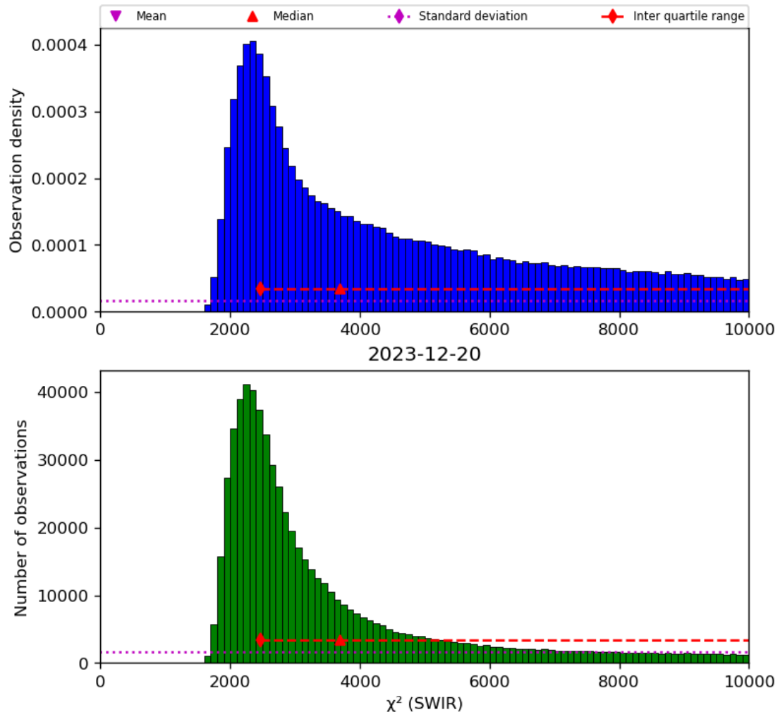
Figure 28: Histogram of “ \chi^2 (SWIR)” for 2023-12-20 to 2023-12-21
