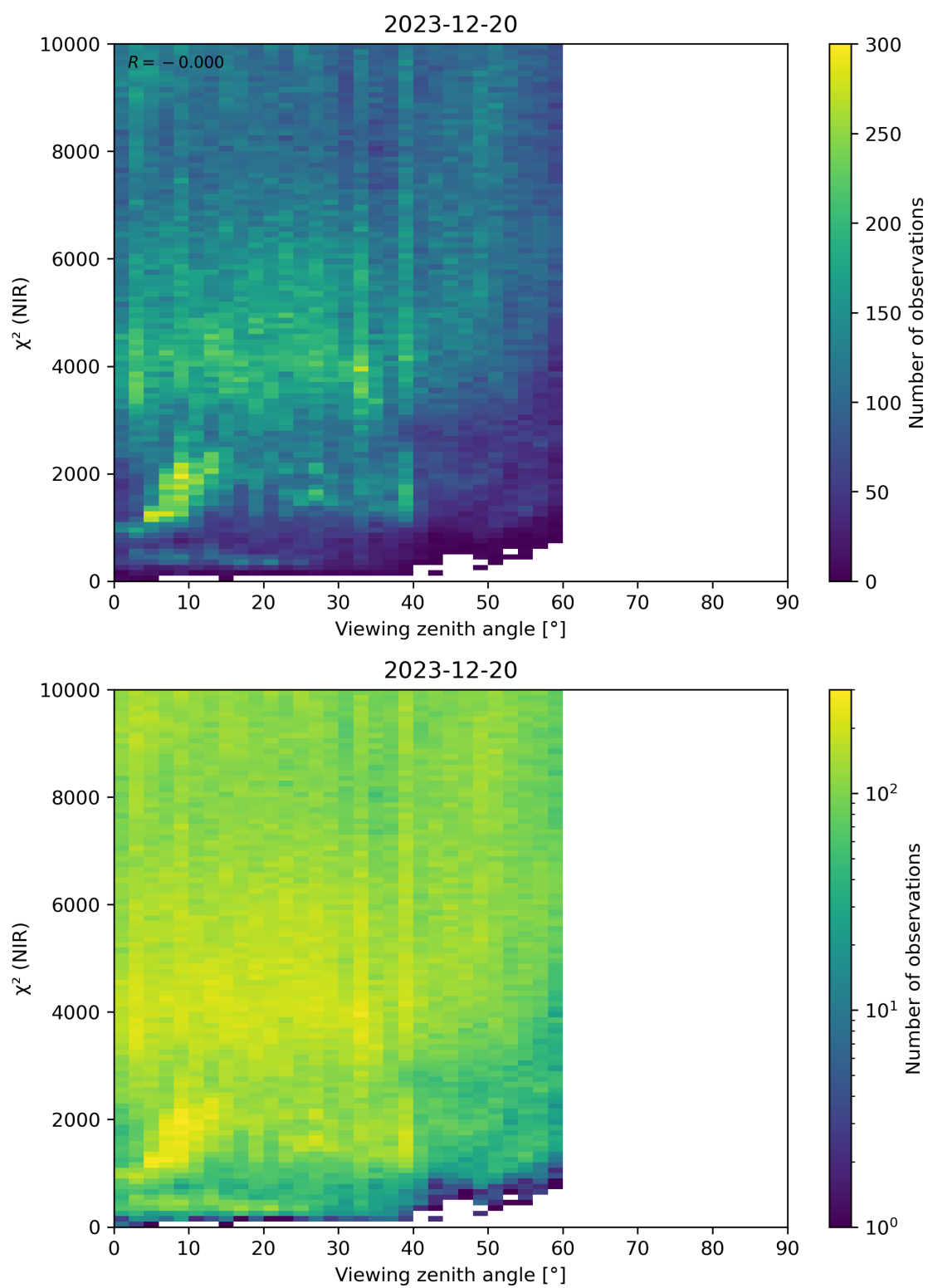
Figure 105: Scatter density plot of “Viewing zenith angle” against “ \chi^2 (NIR)” for 2023-12-20 to 2023-12-21.
