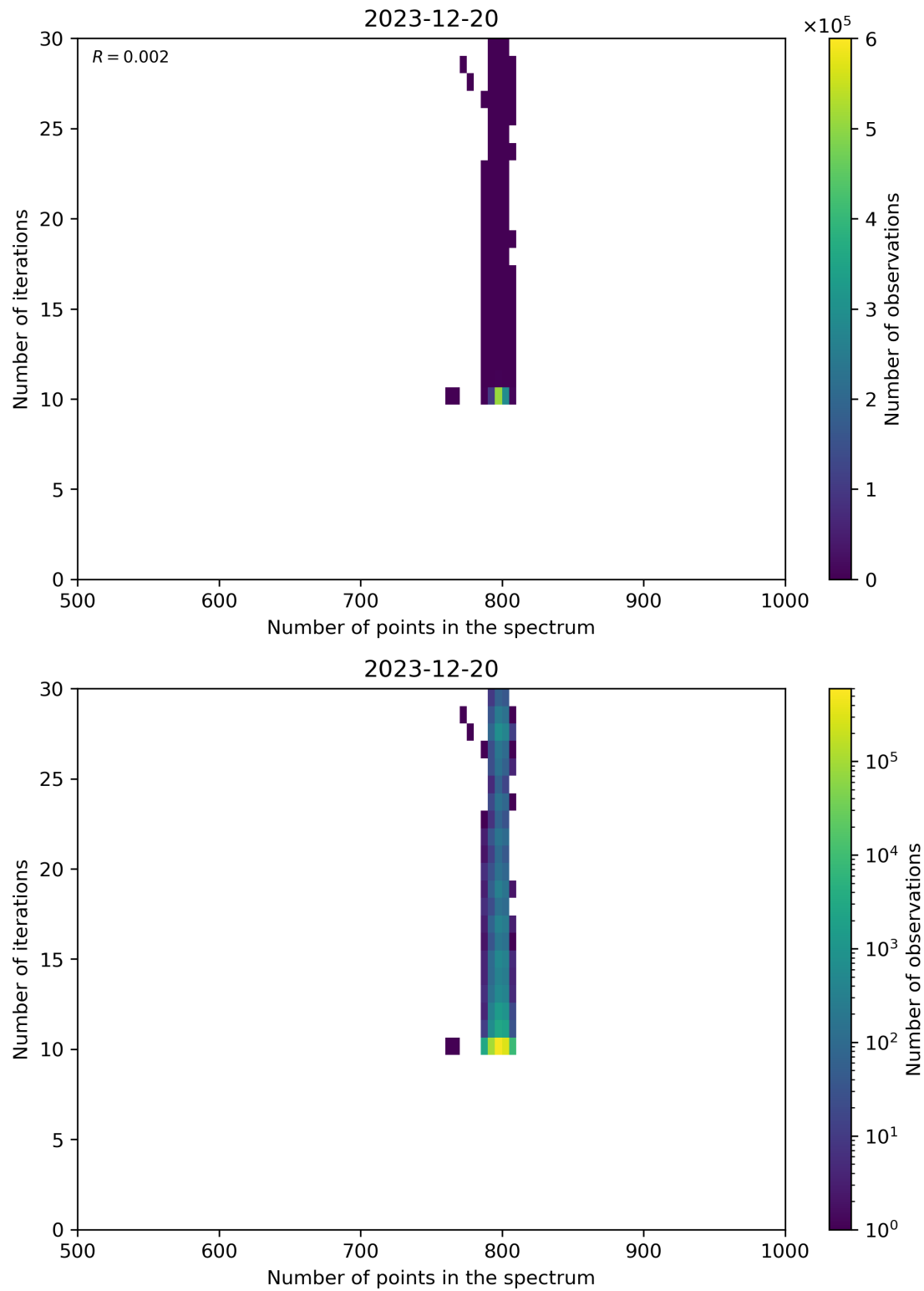
Figure 92: Scatter density plot of “Number of points in the spectrum” against “Number of iterations” for 2023-12-20 to 2023-12-21.
