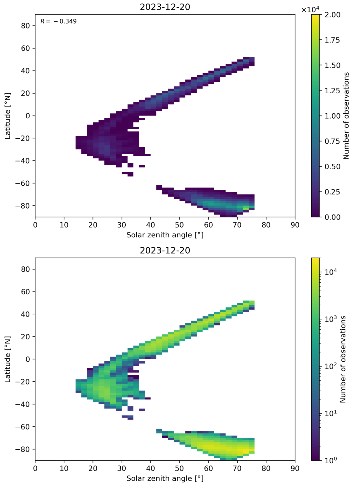
Figure 98: Scatter density plot of “Solar zenith angle” against “Latitude” for 2023-12-20 to 2023-12-21.
