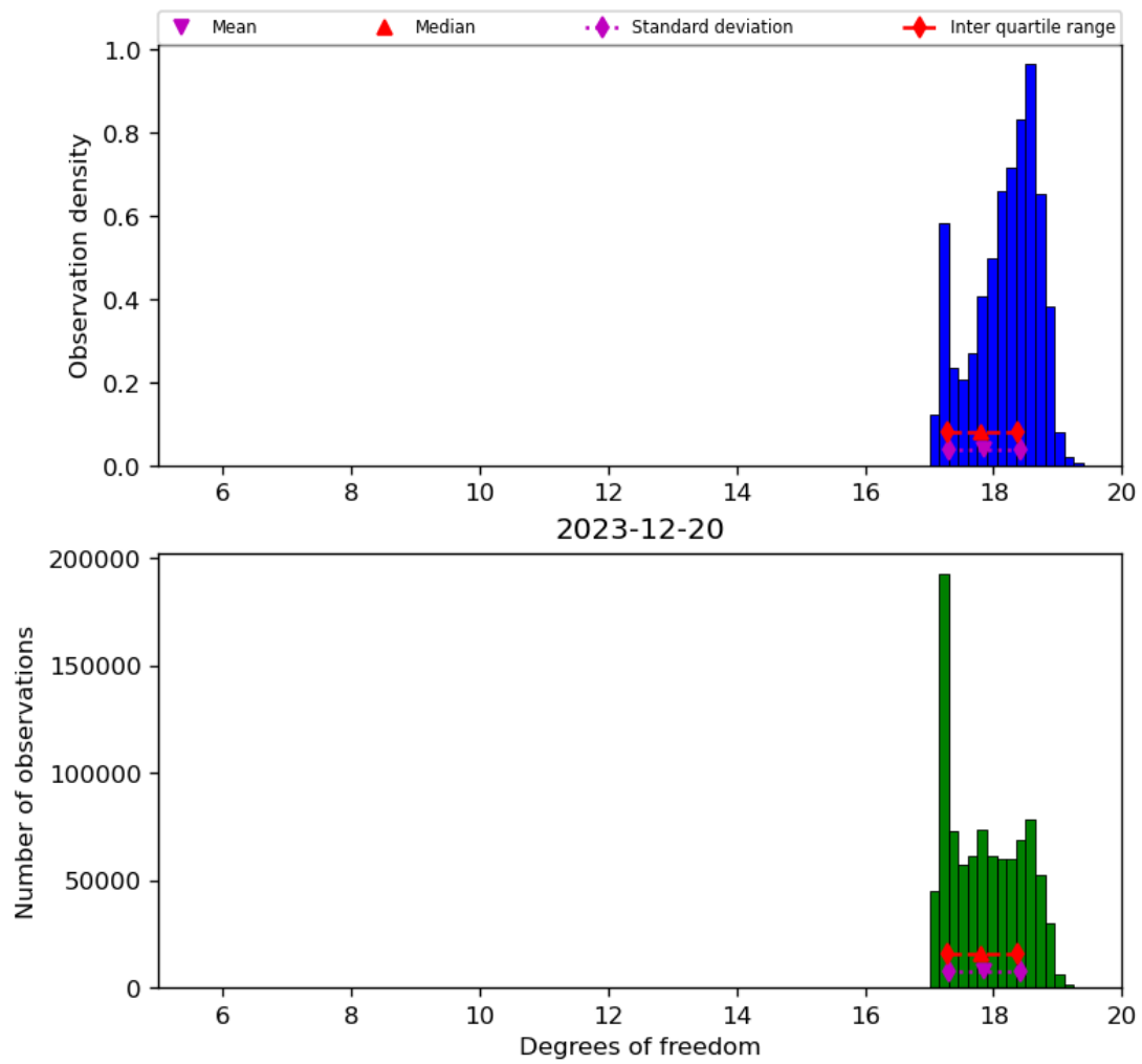
Figure 30: Histogram of “Degrees of freedom” for 2023-12-20 to 2023-12-21
