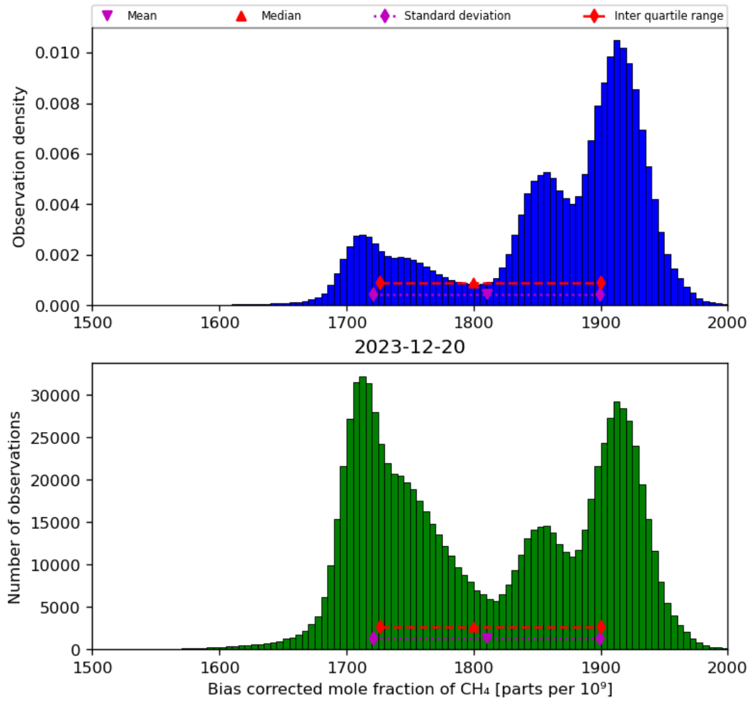
Figure 25: Histogram of “Bias corrected mole fraction of CH 4 ” for 2023-12-20 to 2023-12-21
