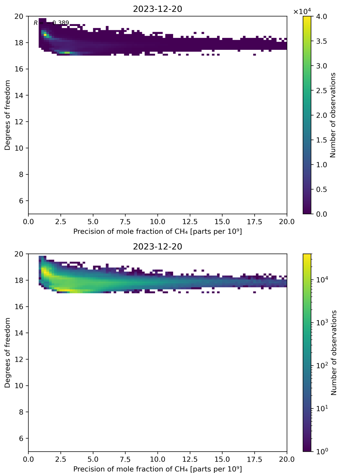
Figure 80: Scatter density plot of “Precision of mole fraction of CH 4 ” against “Degrees of freedom” for 2023-12-20 to 2023-12-21.
