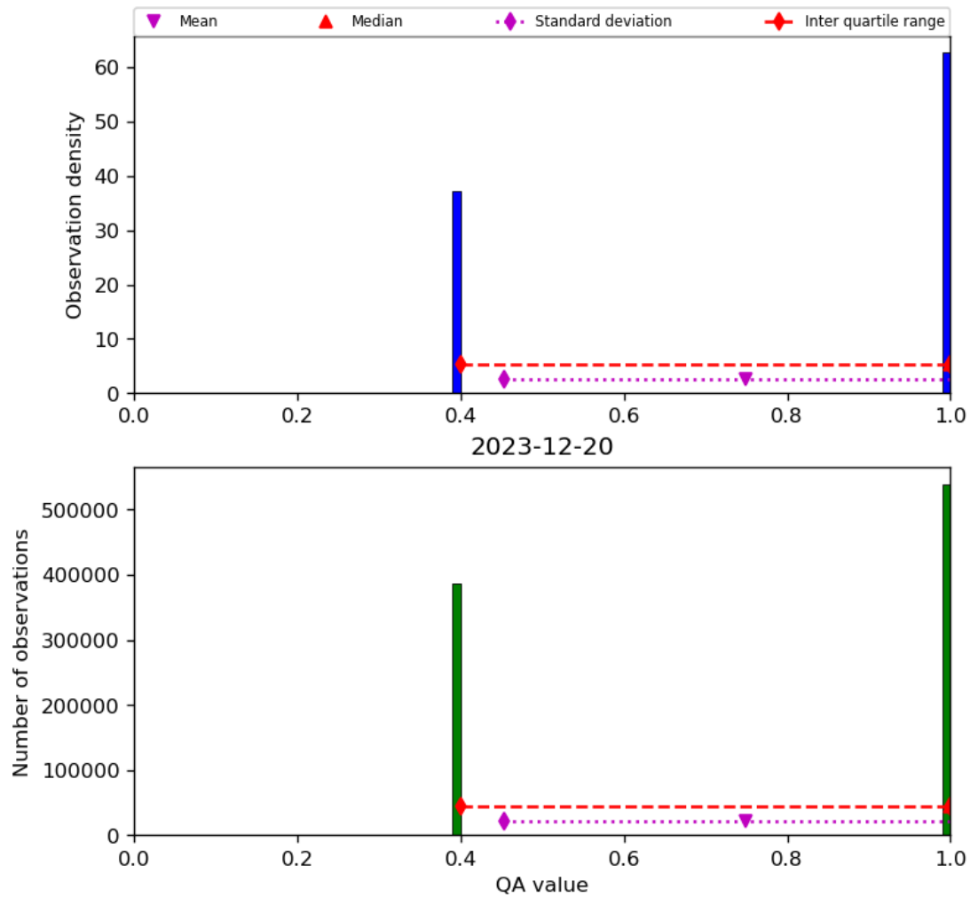
Figure 22: Histogram of “QA value” for 2023-12-20 to 2023-12-21
