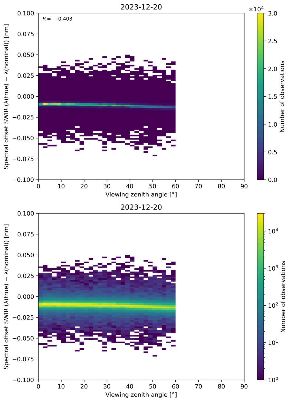
Figure 116: Scatter density plot of “Viewing zenith angle” against “Spectral offset SWIR ( \lambda(\text{true}) - \lambda(\text{nominal}) )” for 2023-12-20 to 2023-12-21.
