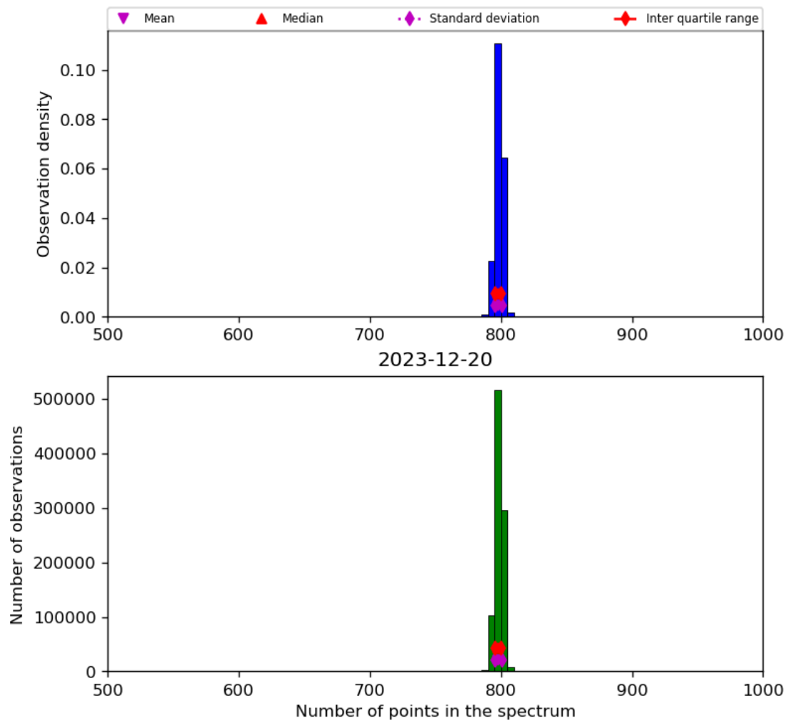
Figure 26: Histogram of “Number of points in the spectrum” for 2023-12-20 to 2023-12-21
