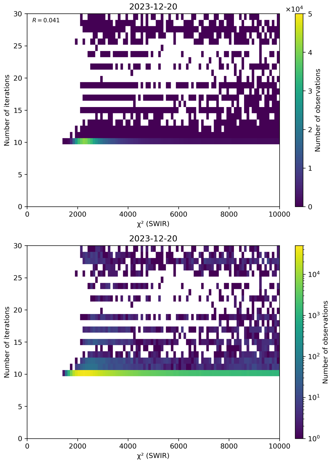
Figure 50: Scatter density plot of “ \chi^2 (SWIR)” against “Number of iterations” for 2023-12-20 to 2023-12-21.
