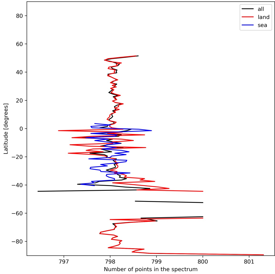
Figure 15: Zonal average of “Number of points in the spectrum” for 2023-12-20 to 2023-12-21.
