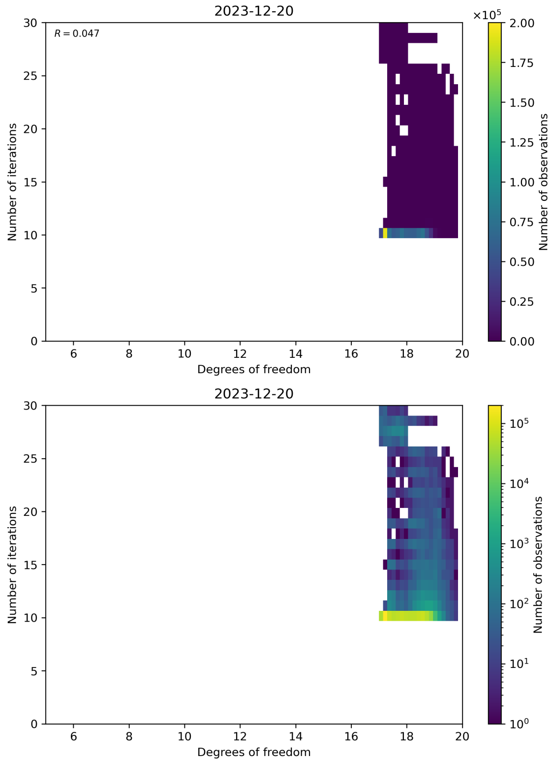
Figure 52: Scatter density plot of “Degrees of freedom” against “Number of iterations” for 2023-12-20 to 2023-12-21.
