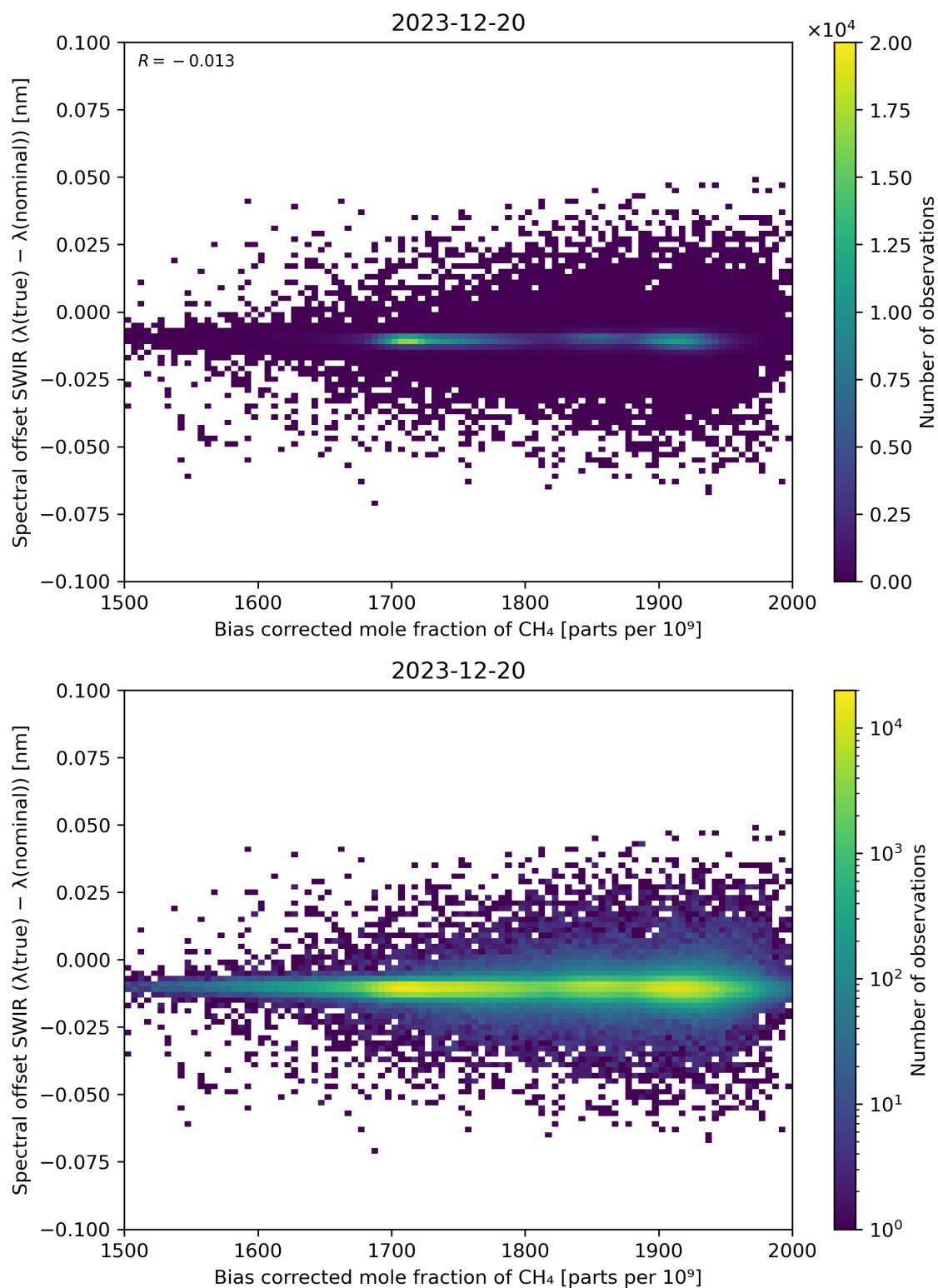
Figure 69: Scatter density plot of “Bias corrected mole fraction of \text{CH}_4 ” against “Spectral offset SWIR ( \lambda(\text{true}) - \lambda(\text{nominal}) )” for 2023-12-20 to 2023-12-21.
