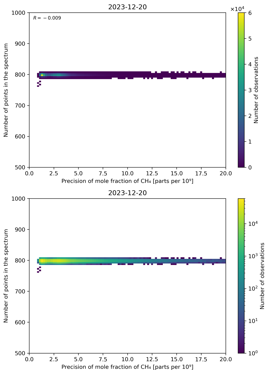
Figure 84: Scatter density plot of “Precision of mole fraction of CH 4 ” against “Number of points in the spectrum” for 2023-12-20 to 2023-12-21.
