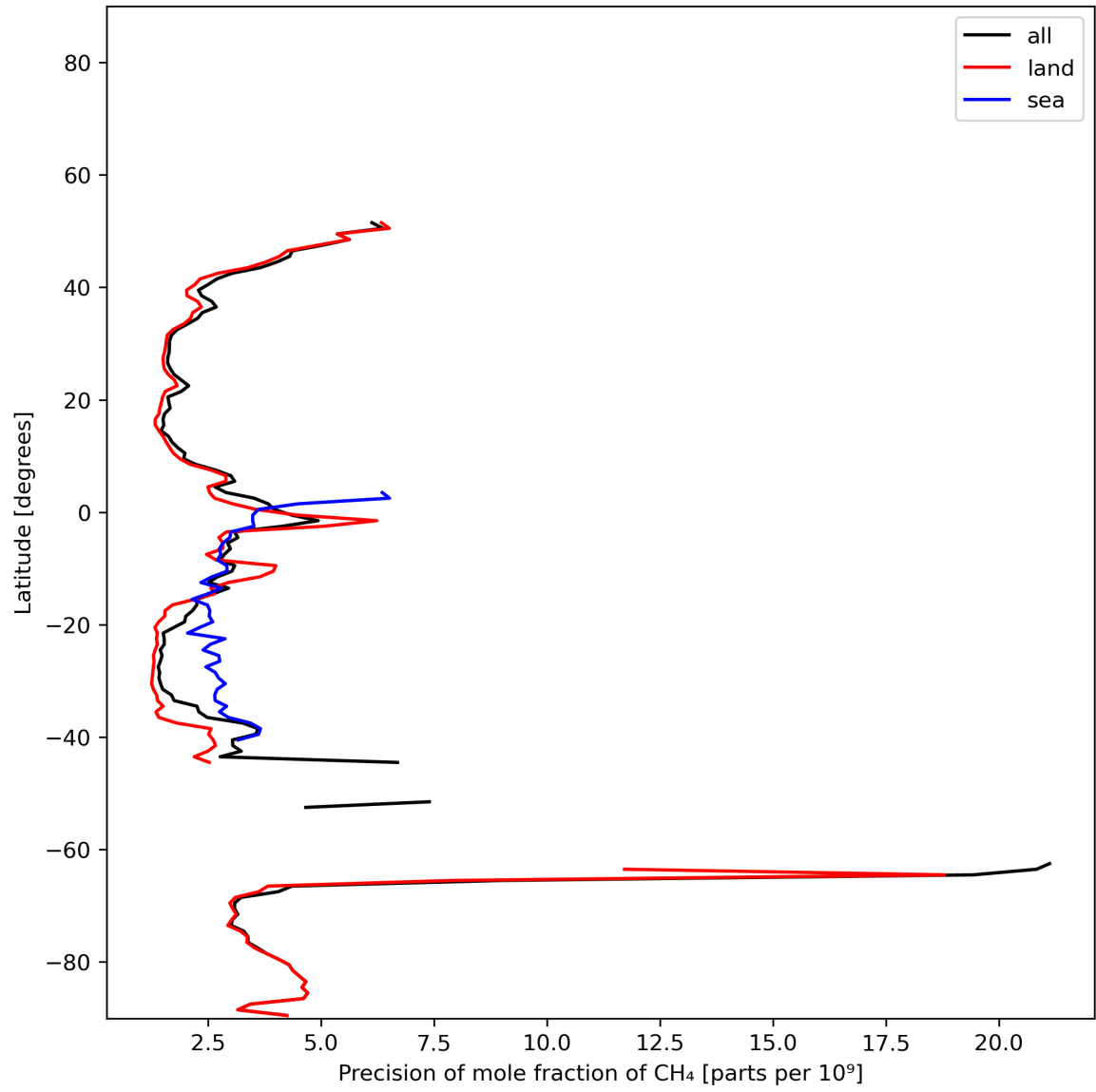
Figure 13: Zonal average of “Precision of mole fraction of CH 4 ” for 2023-12-20 to 2023-12-21.
