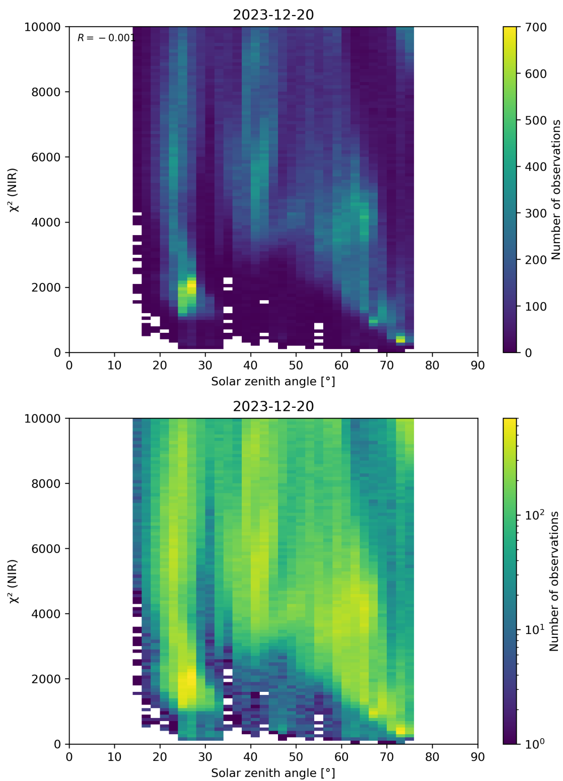
Figure 94: Scatter density plot of “Solar zenith angle” against “ \chi^2 (NIR)” for 2023-12-20 to 2023-12-21.
