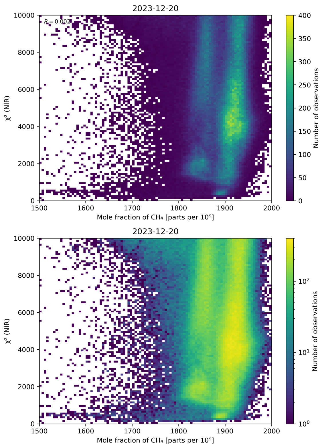
Figure 70: Scatter density plot of “Mole fraction of \text{CH}_4 ” against “ \chi^2 (NIR)” for 2023-12-20 to 2023-12-21.
