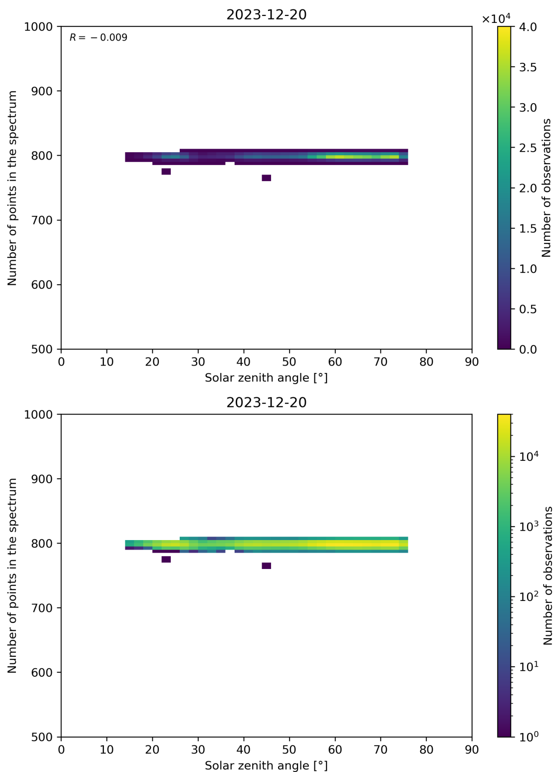
Figure 103: Scatter density plot of “Solar zenith angle” against “Number of points in the spectrum” for 2023-12-20 to 2023-12-21.
