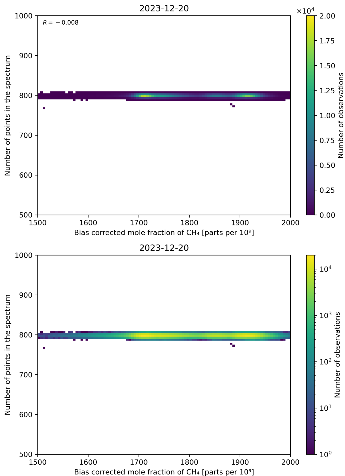
Figure 68: Scatter density plot of “Bias corrected mole fraction of CH 4 ” against “Number of points in the spectrum” for 2023-12-20 to 2023-12-21.
