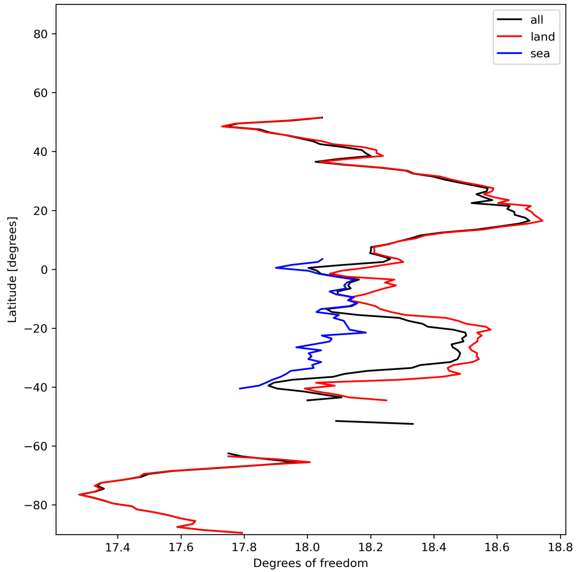
Figure 19: Zonal average of “Degrees of freedom” for 2023-12-20 to 2023-12-21.
