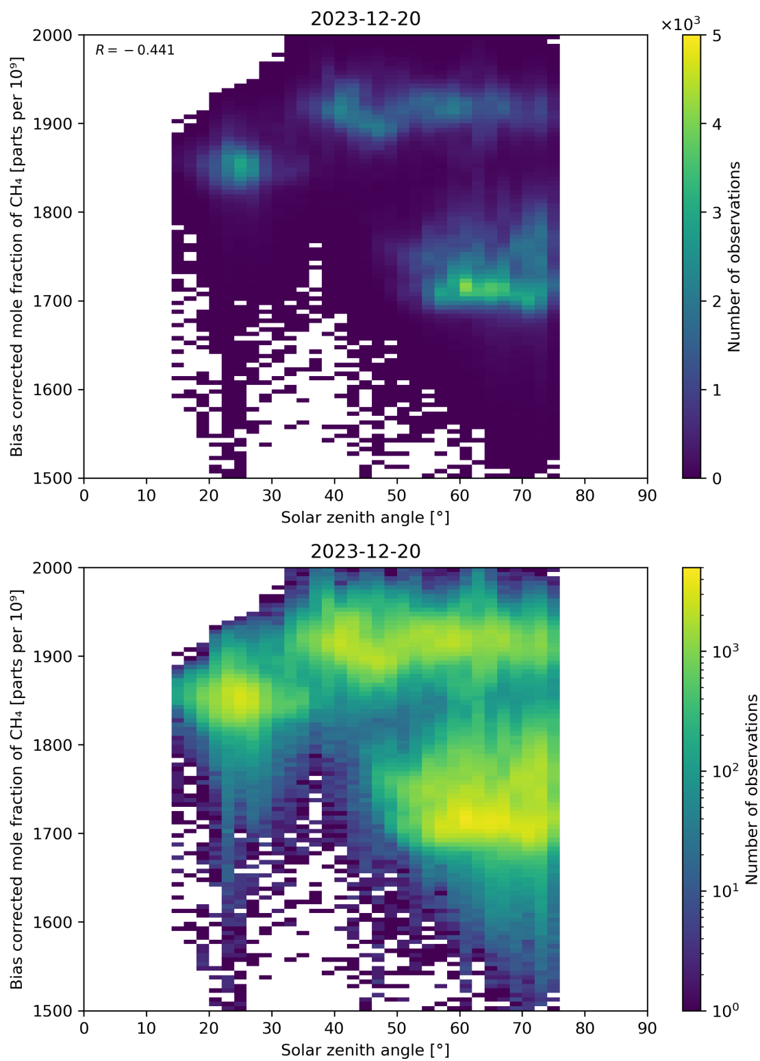
Figure 100: Scatter density plot of “Solar zenith angle” against “Bias corrected mole fraction of \text{CH}_4 ” for 2023-12-20 to 2023-12-21.
