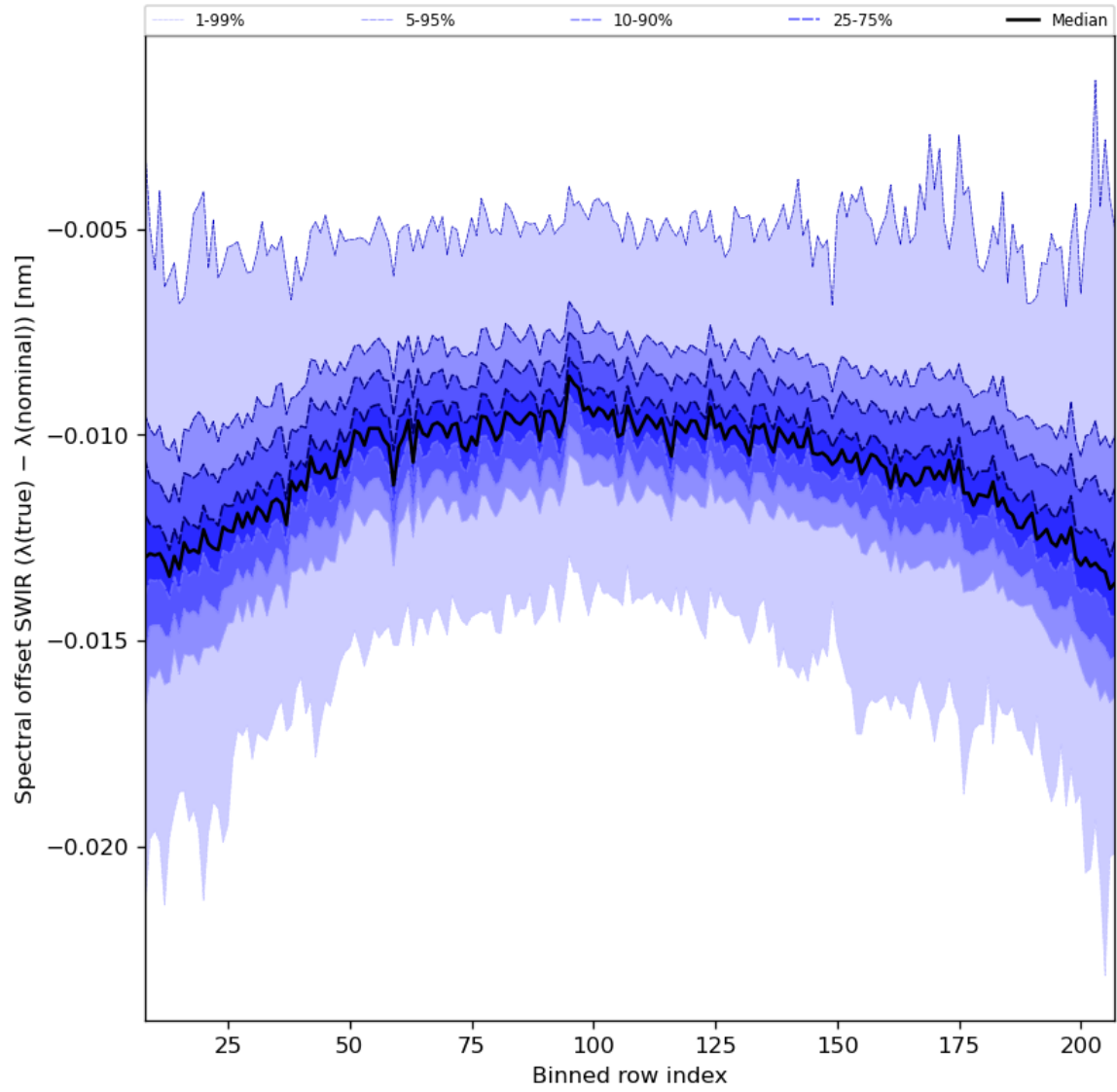
Figure 38: Along track statistics of “Spectral offset SWIR ( \lambda(\text{true}) - \lambda(\text{nominal}) )” for 2023-12-20 to 2023-12-21
