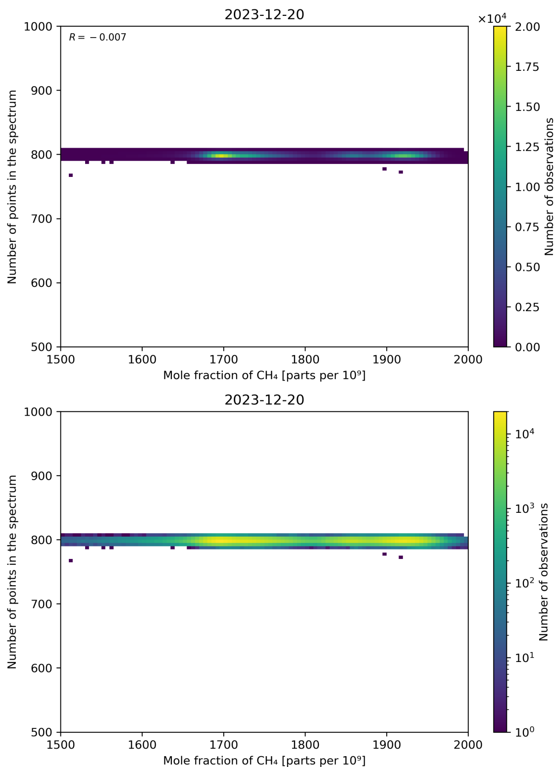
Figure 77: Scatter density plot of “Mole fraction of CH 4 ” against “Number of points in the spectrum” for 2023-12-20 to 2023-12-21.
