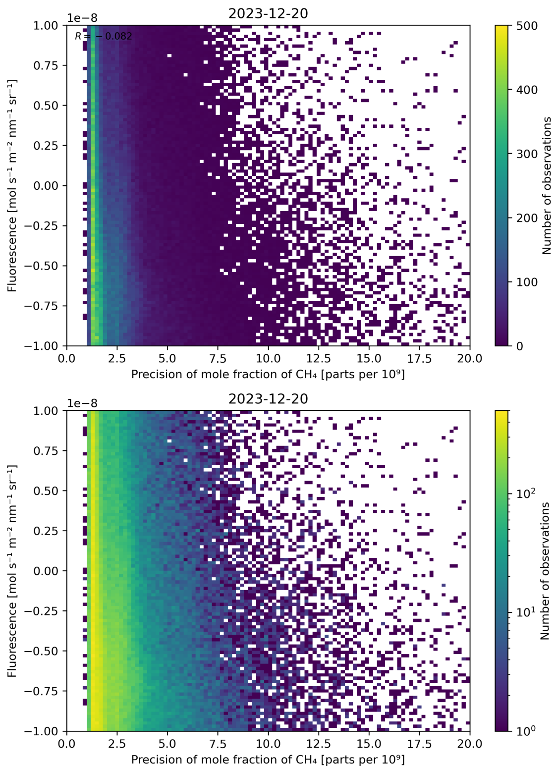
Figure 81: Scatter density plot of “Precision of mole fraction of \text{CH}_4 ” against “Fluorescence” for 2023-12-20 to 2023-12-21.
