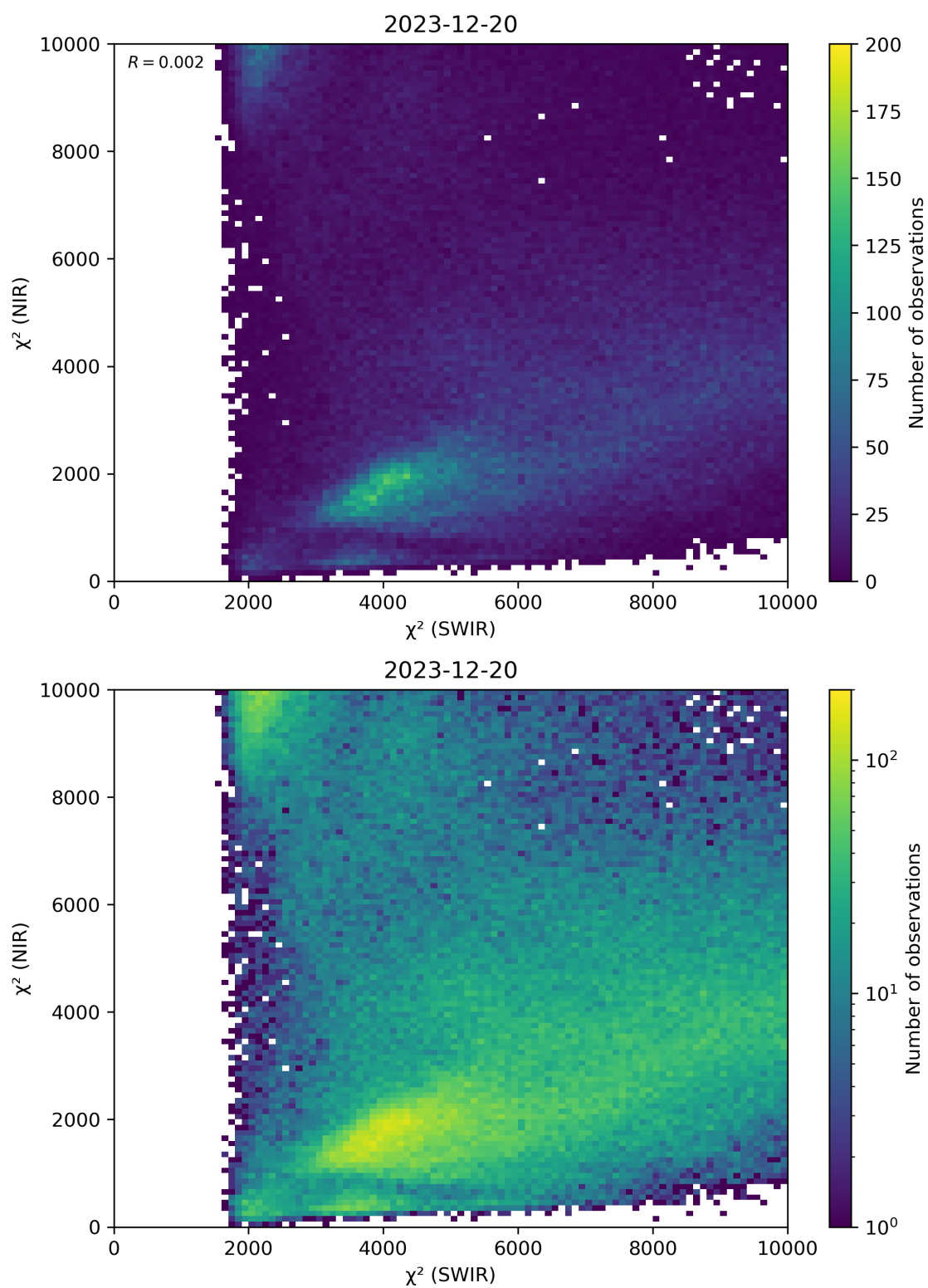
Figure 47: Scatter density plot of “ \chi^2 (SWIR)” against “ \chi^2 (NIR)” for 2023-12-20 to 2023-12-21.
