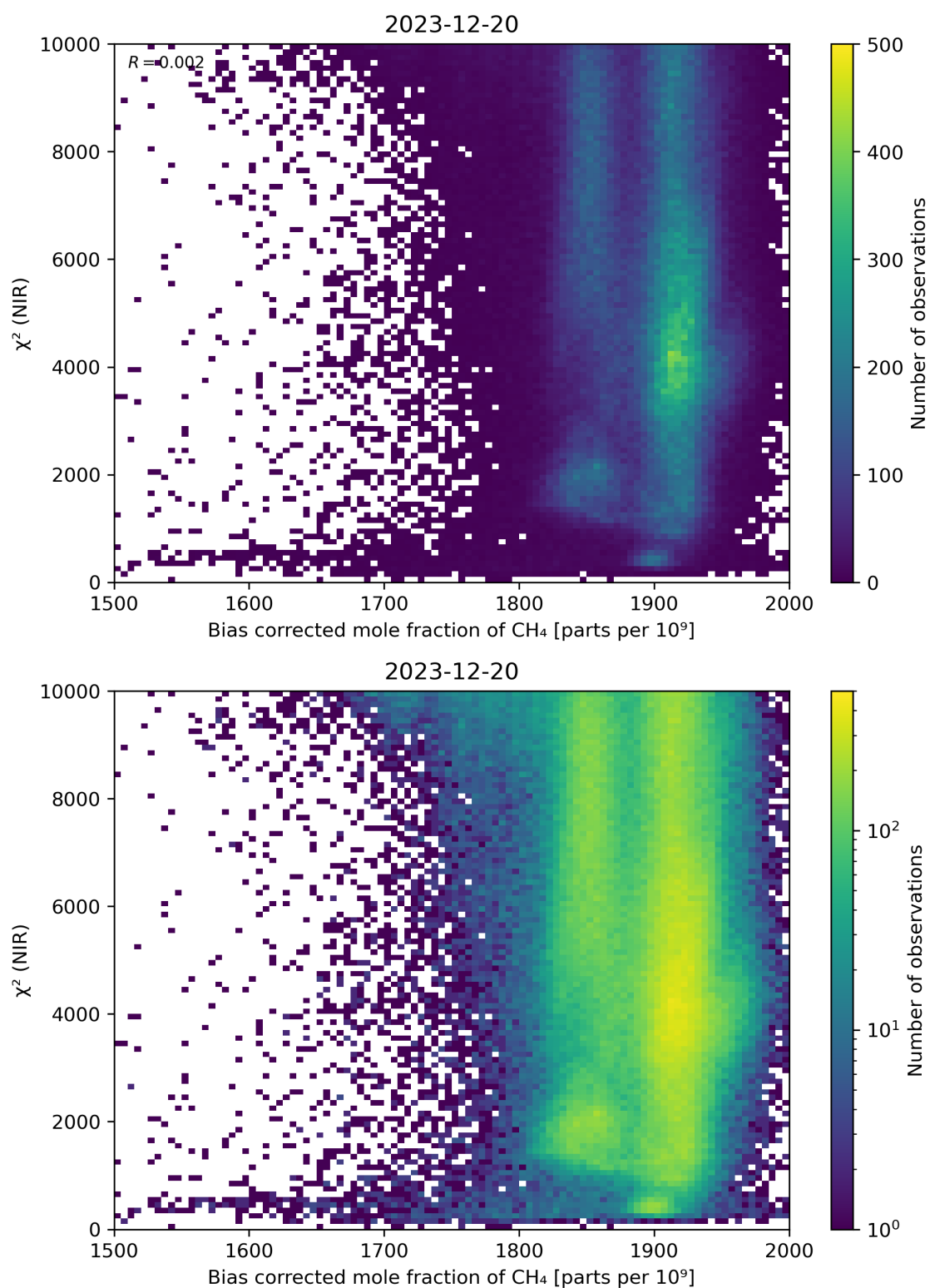
Figure 63: Scatter density plot of “Bias corrected mole fraction of CH 4 ” against “ \chi^2 (NIR)” for 2023-12-20 to 2023-12-21.
