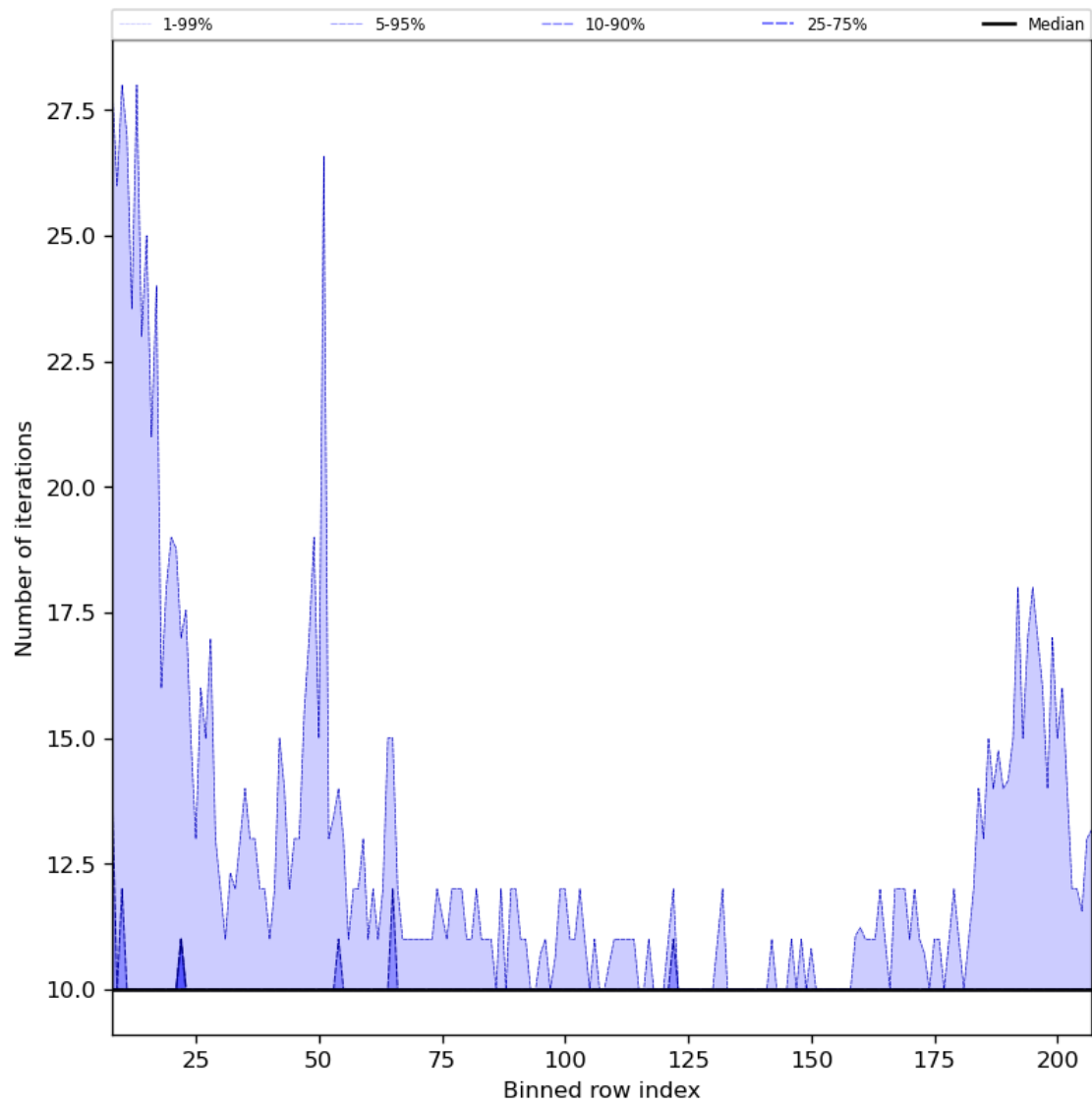
Figure 42: Along track statistics of “Number of iterations” for 2023-12-20 to 2023-12-21
