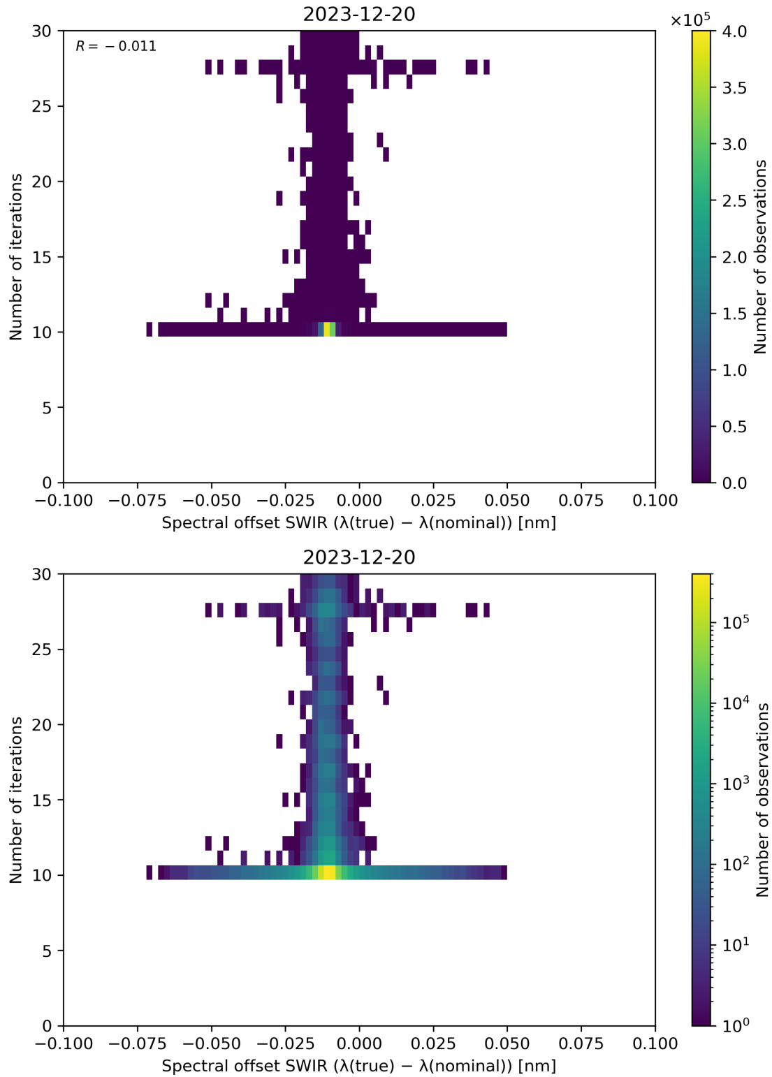
Figure 121: Scatter density plot of “Spectral offset SWIR ( \lambda(\text{true}) - \lambda(\text{nominal}) )” against “Number of iterations” for 2023-12-20 to 2023-12-21.
