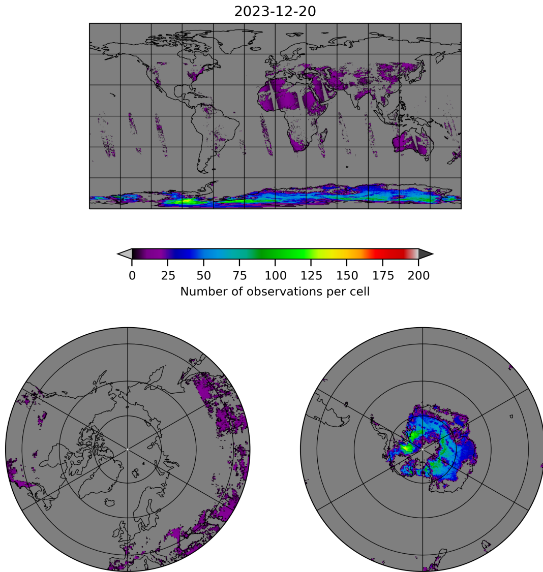
Figure 10: Map of the number of observations for 2023-12-20 to 2023-12-21
