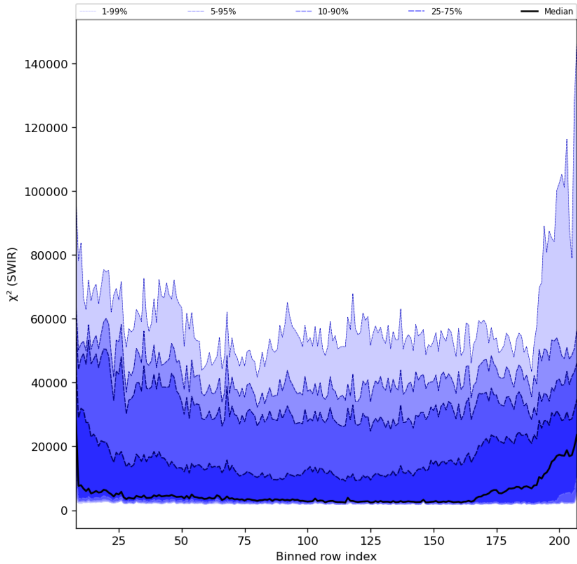
Figure 39: Along track statistics of “ \chi^2 (SWIR)” for 2023-12-20 to 2023-12-21
