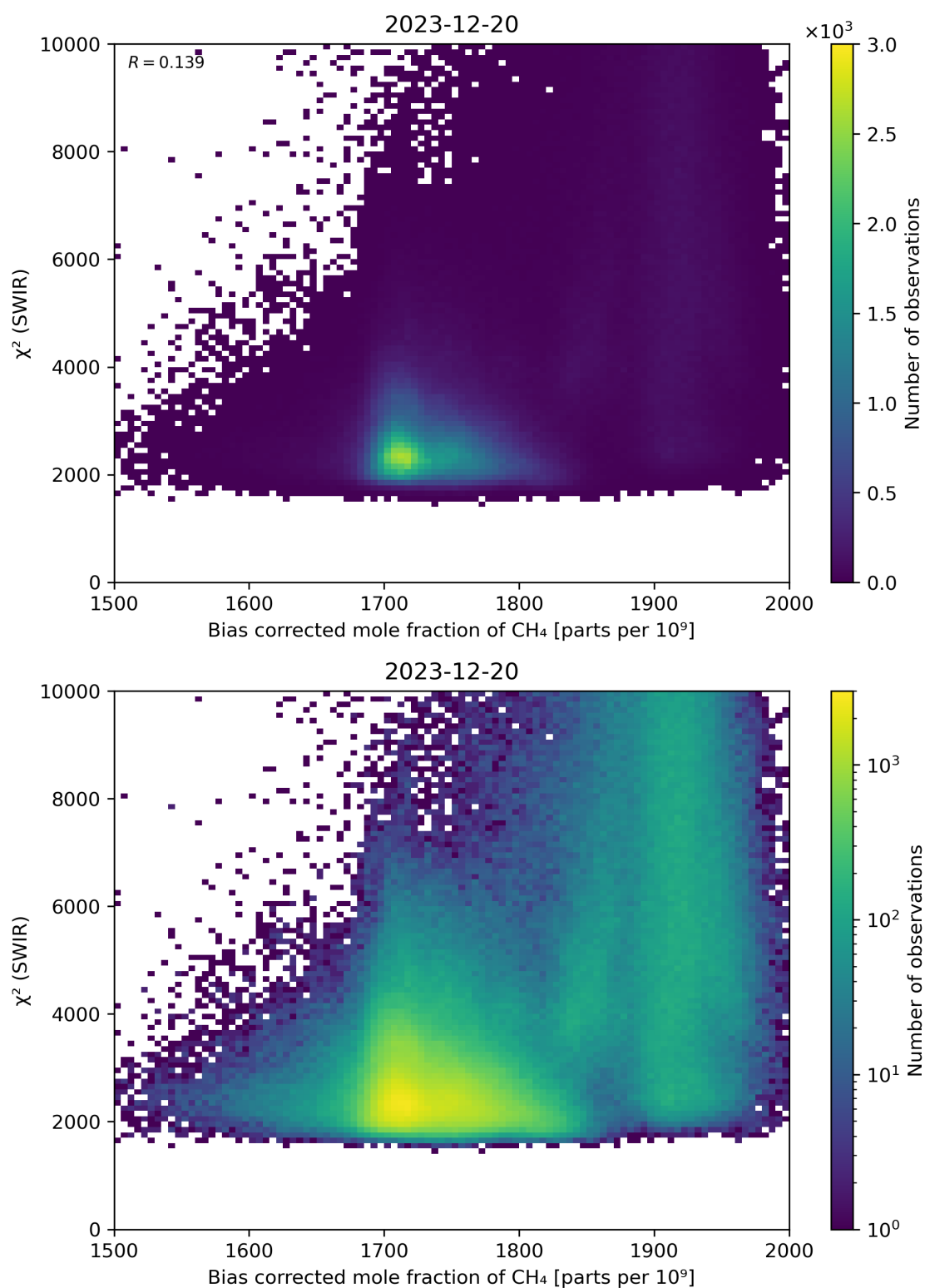
Figure 64: Scatter density plot of “Bias corrected mole fraction of \text{CH}_4 ” against “ \chi^2 (SWIR)” for 2023-12-20 to 2023-12-21.
