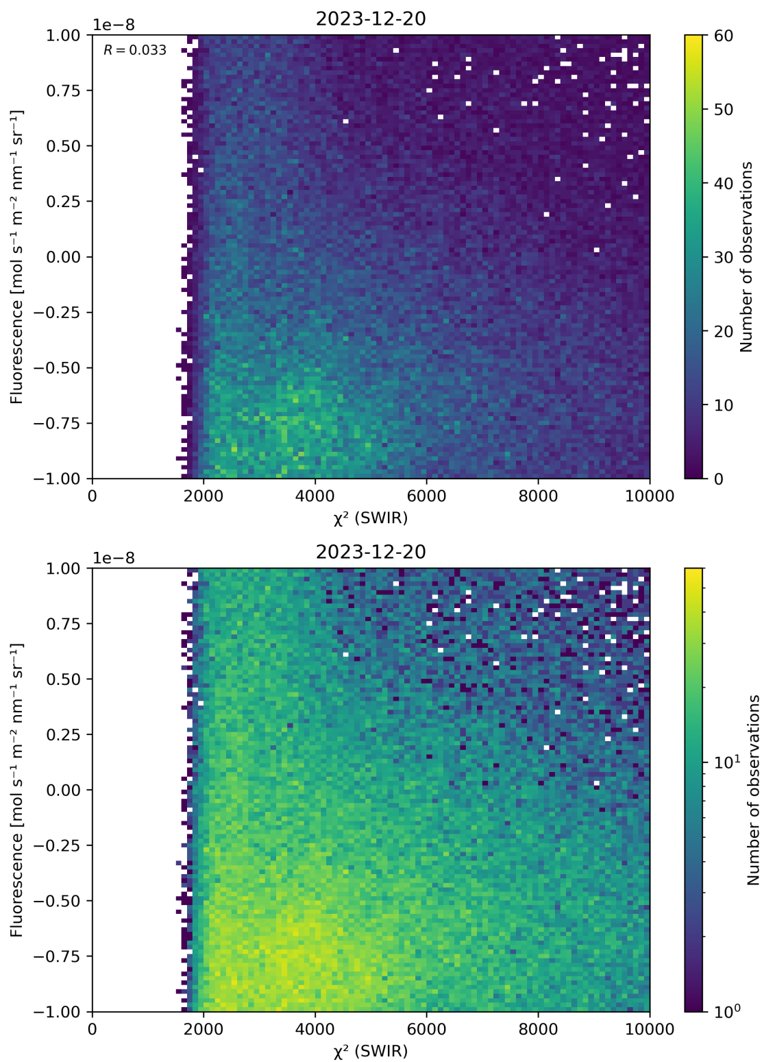
Figure 49: Scatter density plot of “ \chi^2 (SWIR)” against “Fluorescence” for 2023-12-20 to 2023-12-21.
