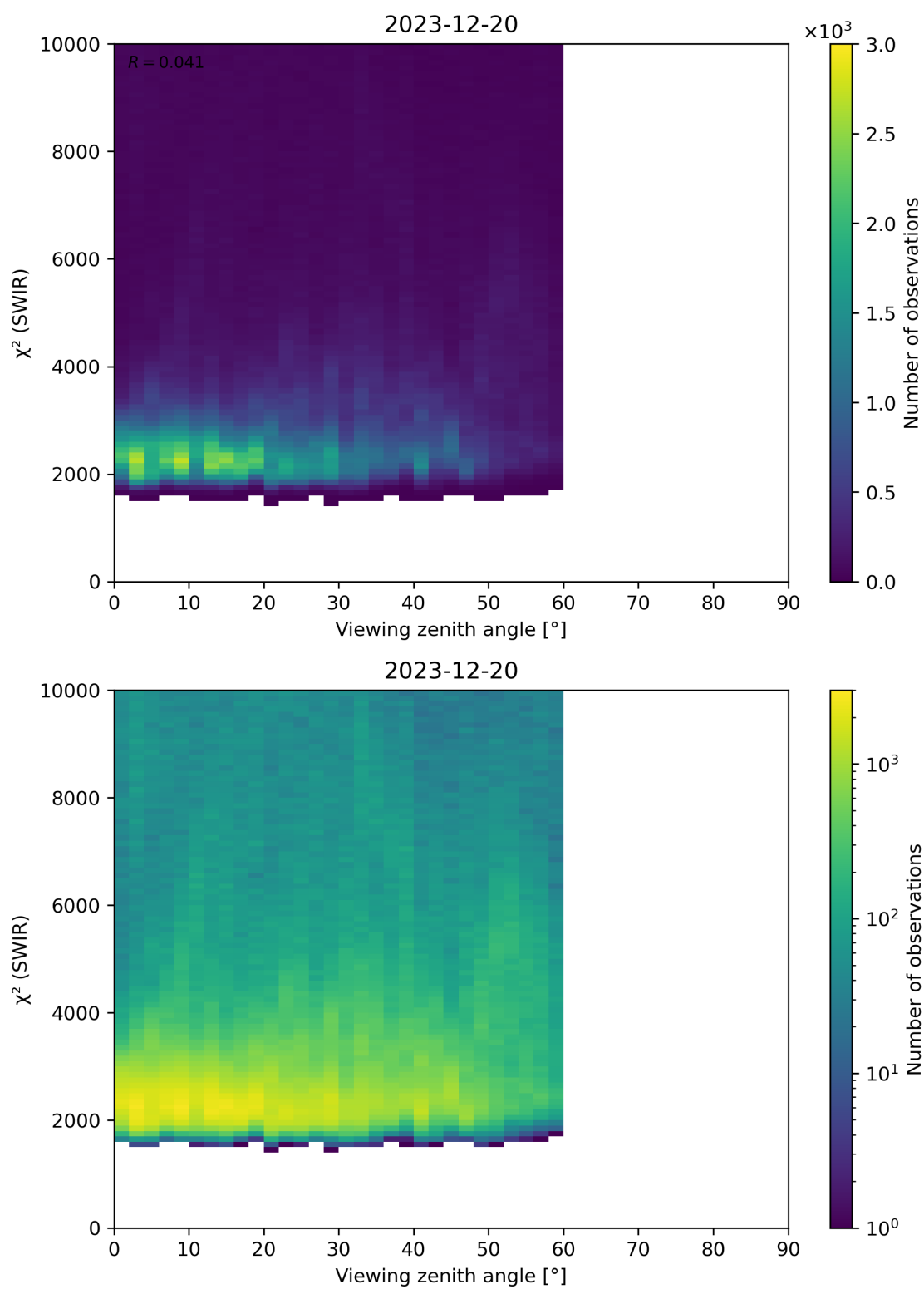
Figure 106: Scatter density plot of “Viewing zenith angle” against “ \chi^2 (SWIR)” for 2023-12-20 to 2023-12-21.
