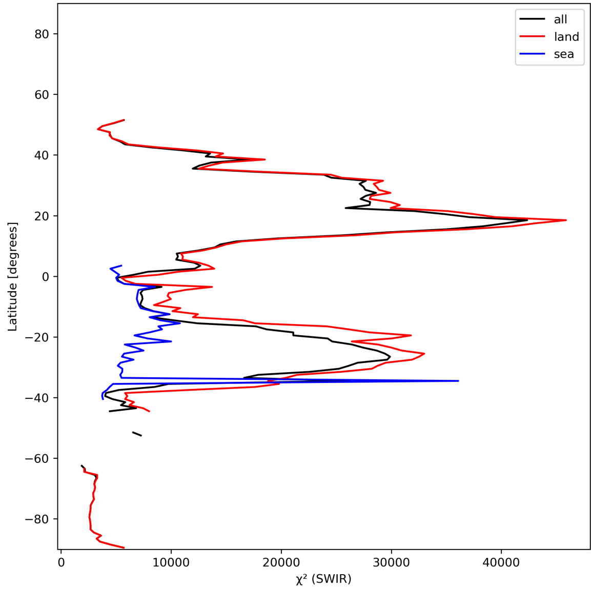
Figure 17: Zonal average of “ \chi^2 (SWIR)” for 2023-12-20 to 2023-12-21.
