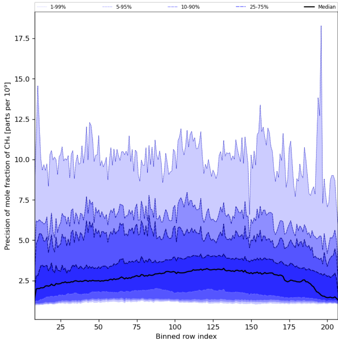
Figure 35: Along track statistics of “Precision of mole fraction of CH 4 ” for 2023-12-20 to 2023-12-21
