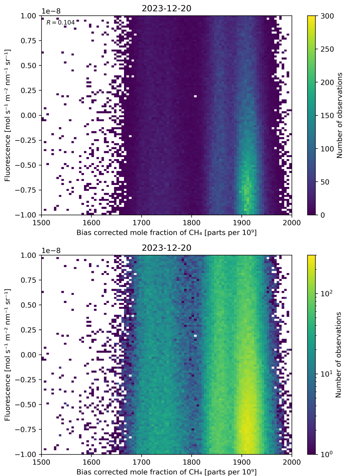
Figure 66: Scatter density plot of “Bias corrected mole fraction of \text{CH}_4 ” against “Fluorescence” for 2023-12-20 to 2023-12-21.
