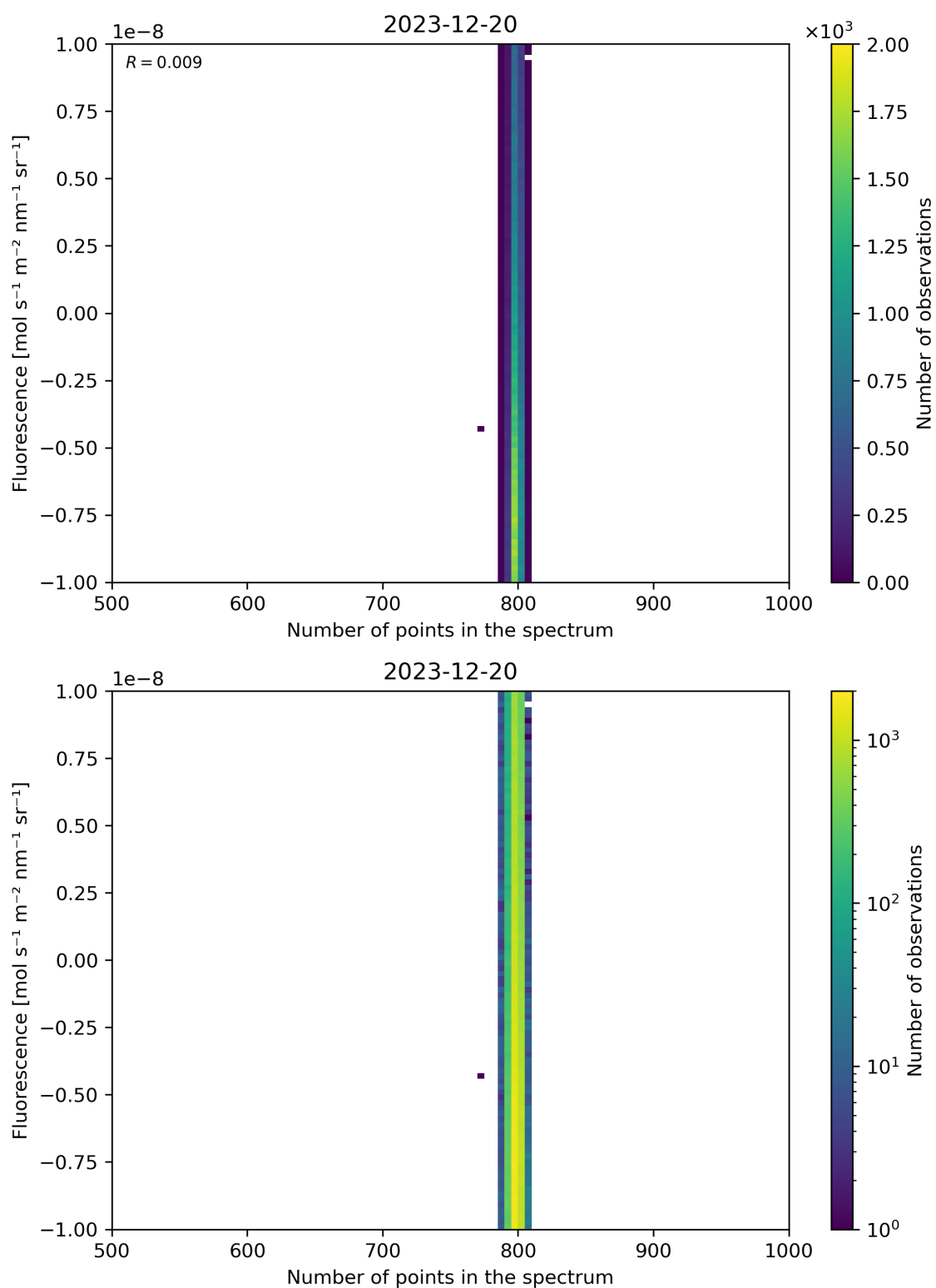
Figure 91: Scatter density plot of “Number of points in the spectrum” against “Fluorescence” for 2023-12-20 to 2023-12-21.
