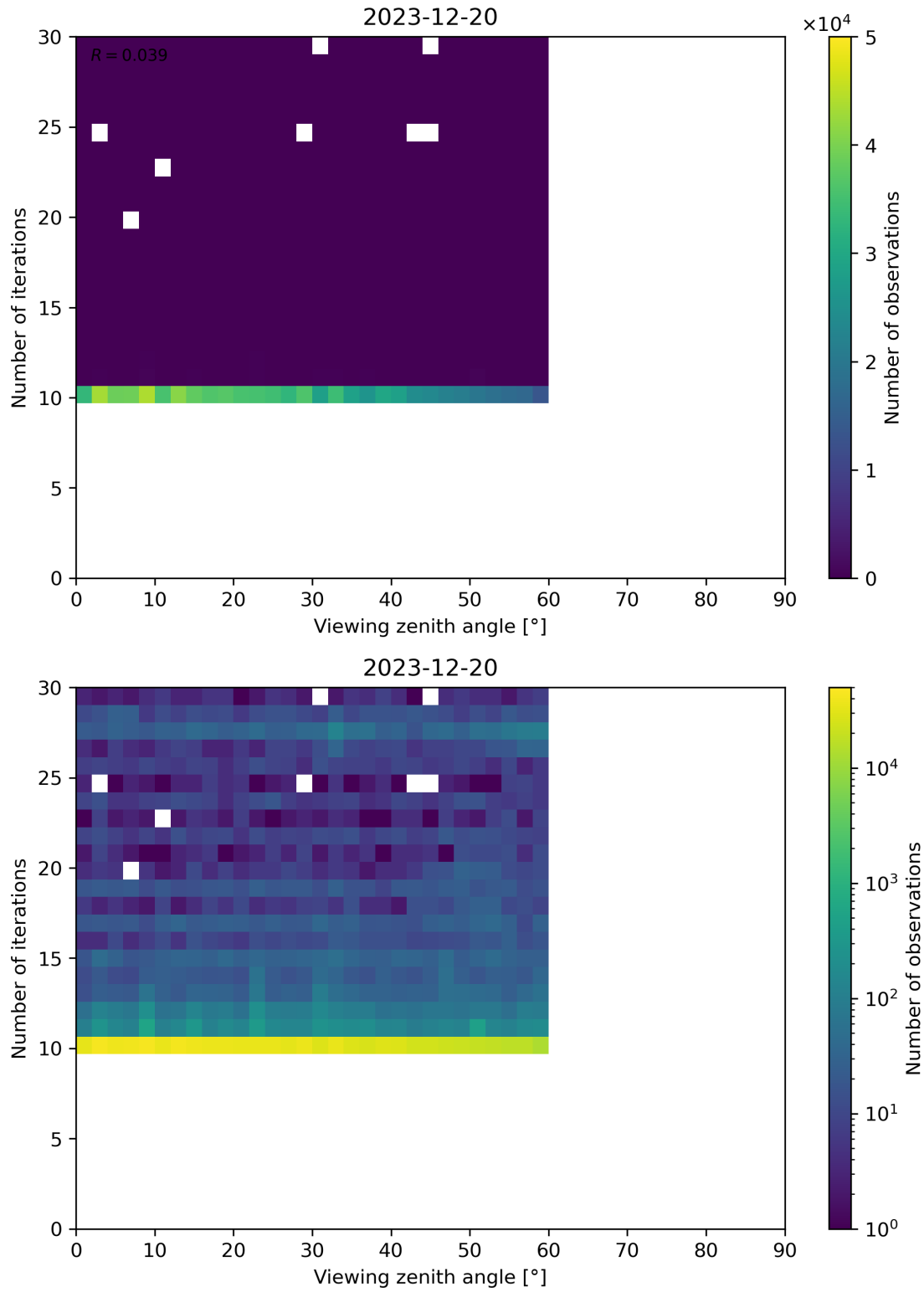
Figure 113: Scatter density plot of “Viewing zenith angle” against “Number of iterations” for 2023-12-20 to 2023-12-21.
