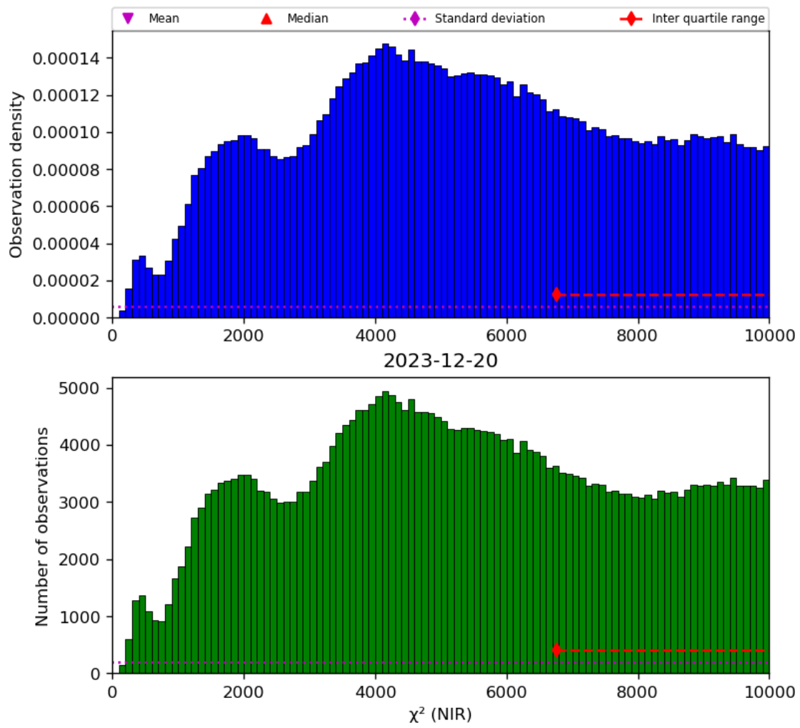
Figure 29: Histogram of “ \chi^2 (NIR)” for 2023-12-20 to 2023-12-21
