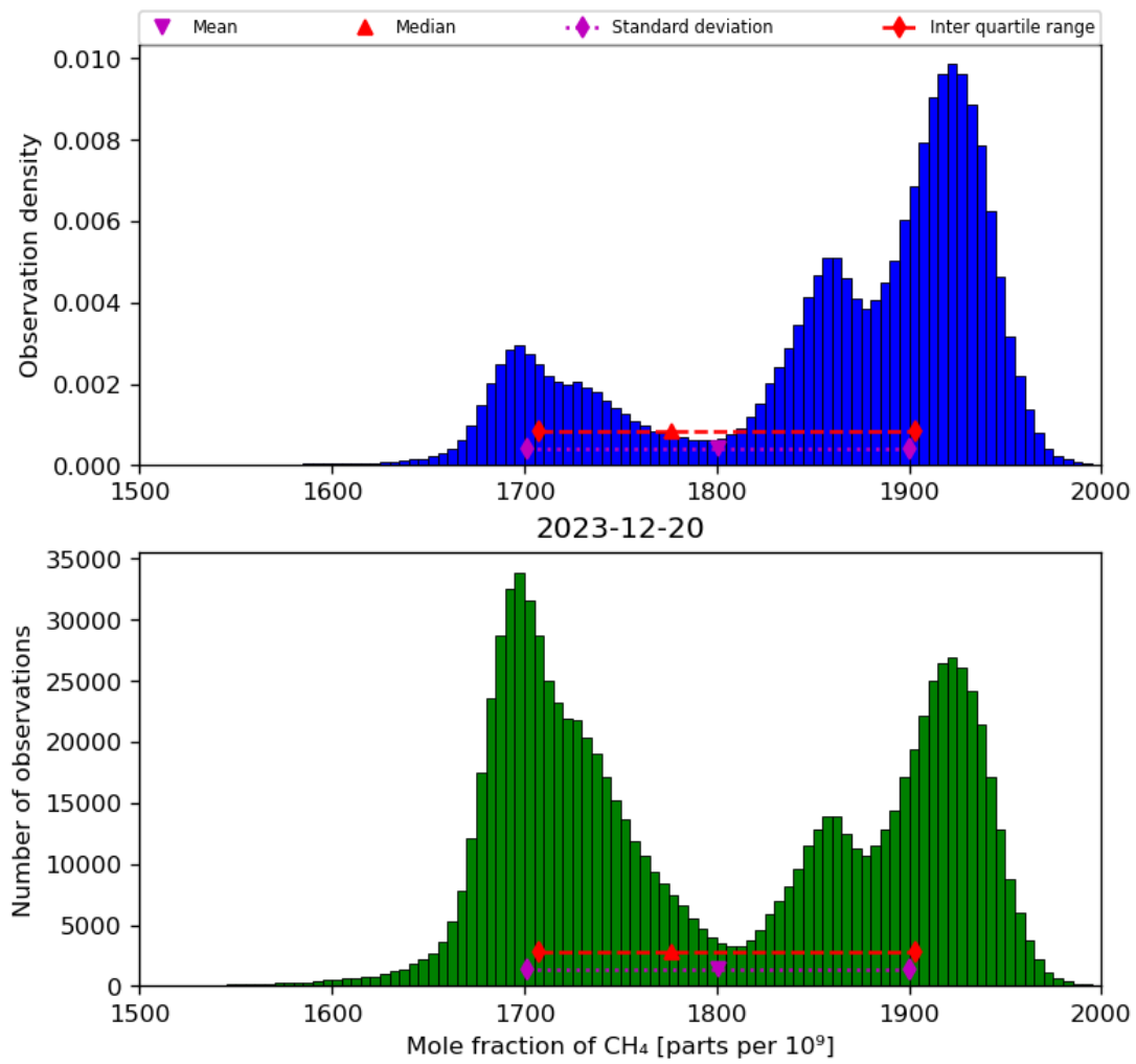
Figure 23: Histogram of “Mole fraction of CH 4 ” for 2023-12-20 to 2023-12-21
