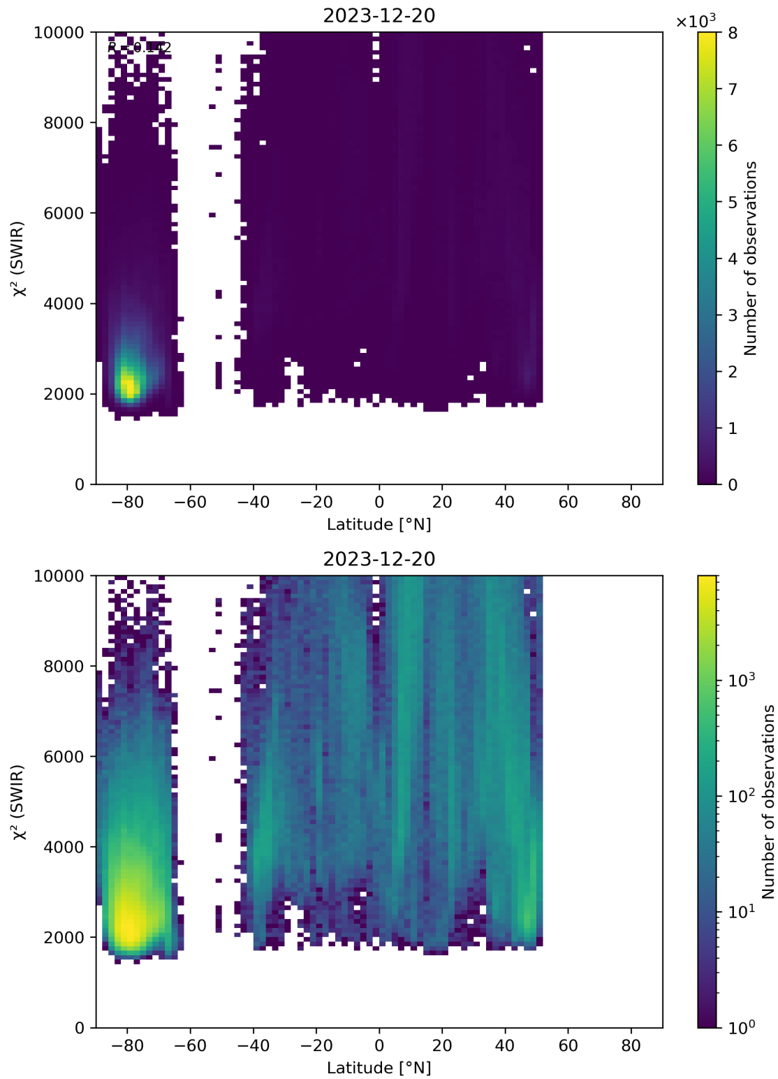
Figure 54: Scatter density plot of “Latitude” against “ \chi^2 (SWIR)” for 2023-12-20 to 2023-12-21.
