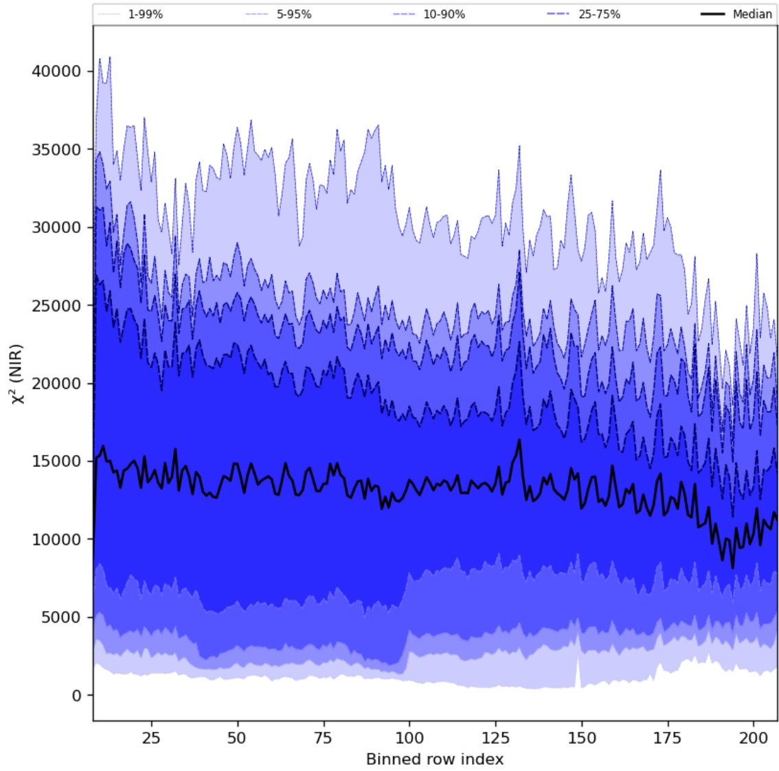
Figure 40: Along track statistics of " \chi^2 (NIR)" for 2023-12-20 to 2023-12-21
