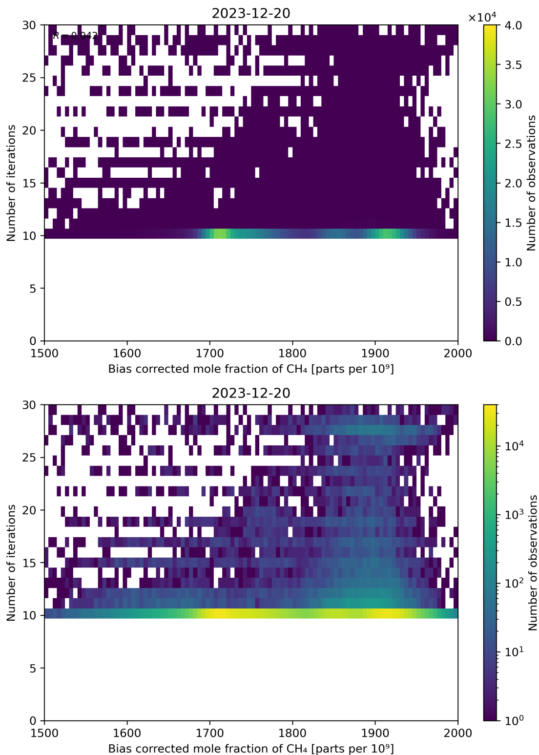
Figure 67: Scatter density plot of “Bias corrected mole fraction of \text{CH}_4 ” against “Number of iterations” for 2023-12-20 to 2023-12-21.
