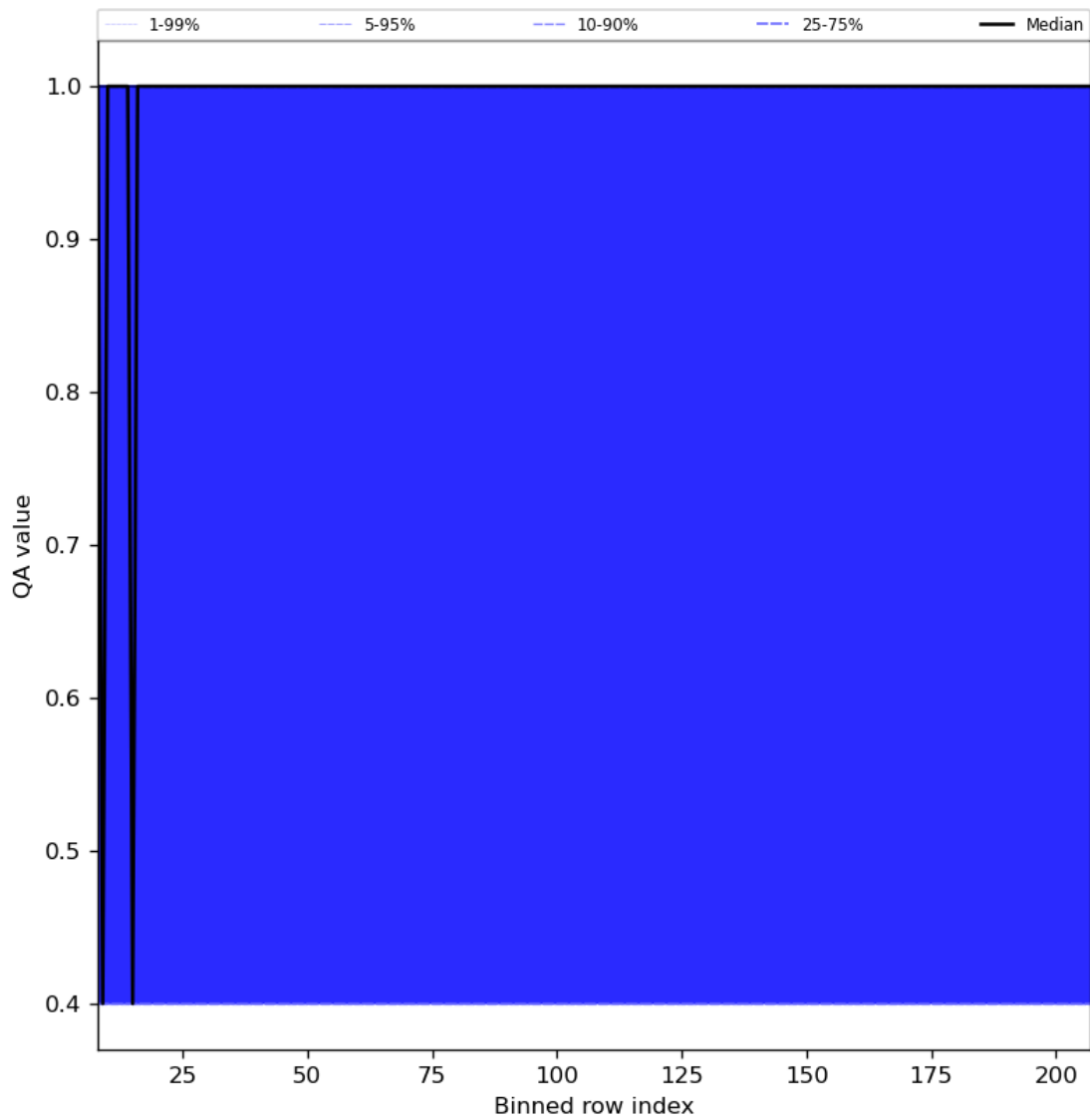
Figure 33: Along track statistics of “QA value” for 2023-12-20 to 2023-12-21
