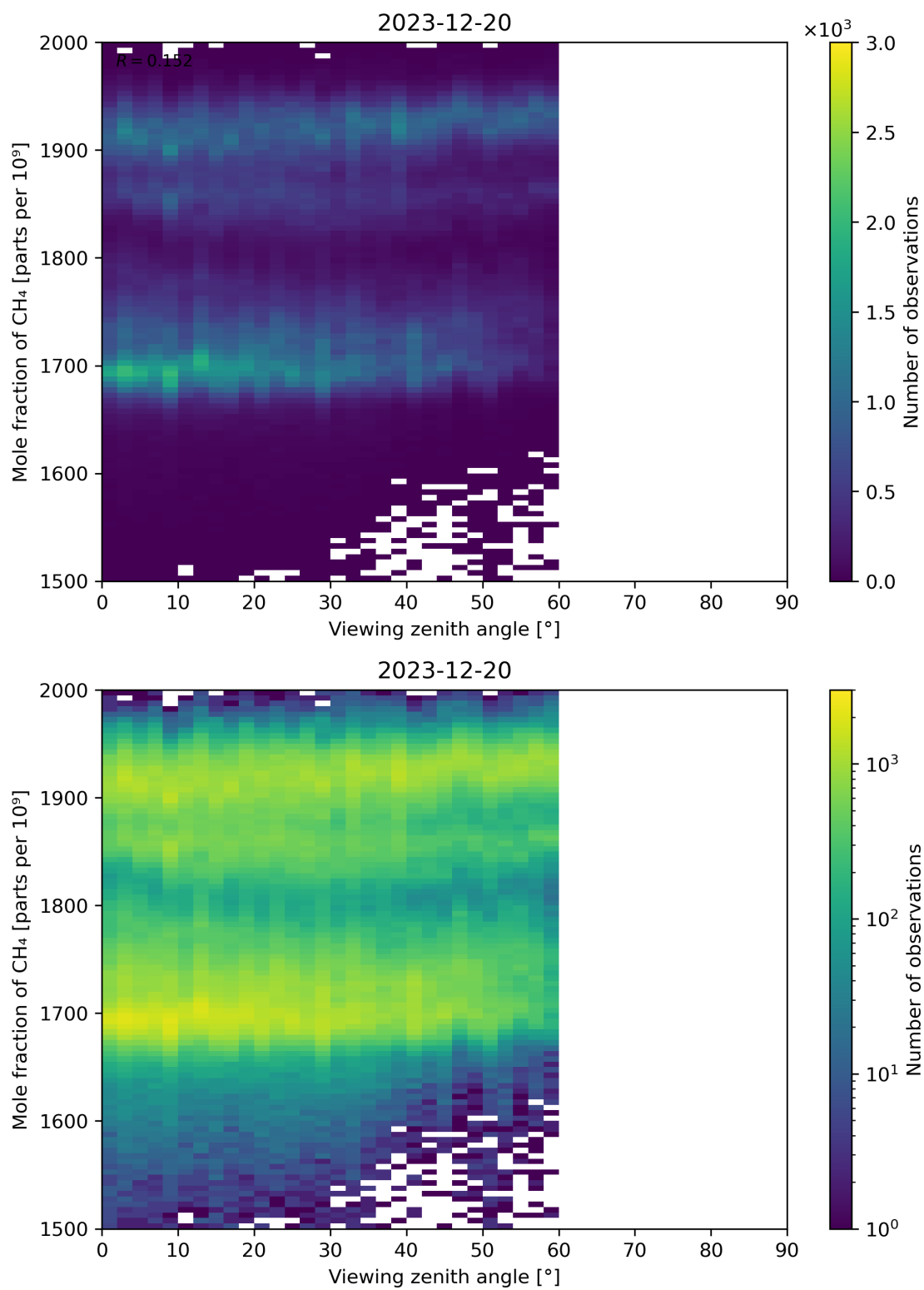
Figure 110: Scatter density plot of “Viewing zenith angle” against “Mole fraction of CH 4 ” for 2023-12-20 to 2023-12-21.
