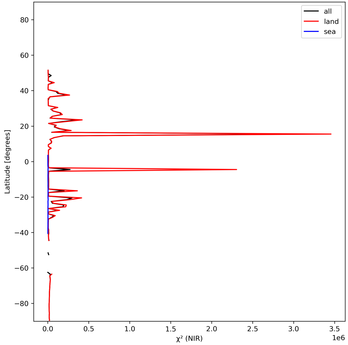
Figure 18: Zonal average of “ \chi^2 (NIR)” for 2023-12-20 to 2023-12-21.
