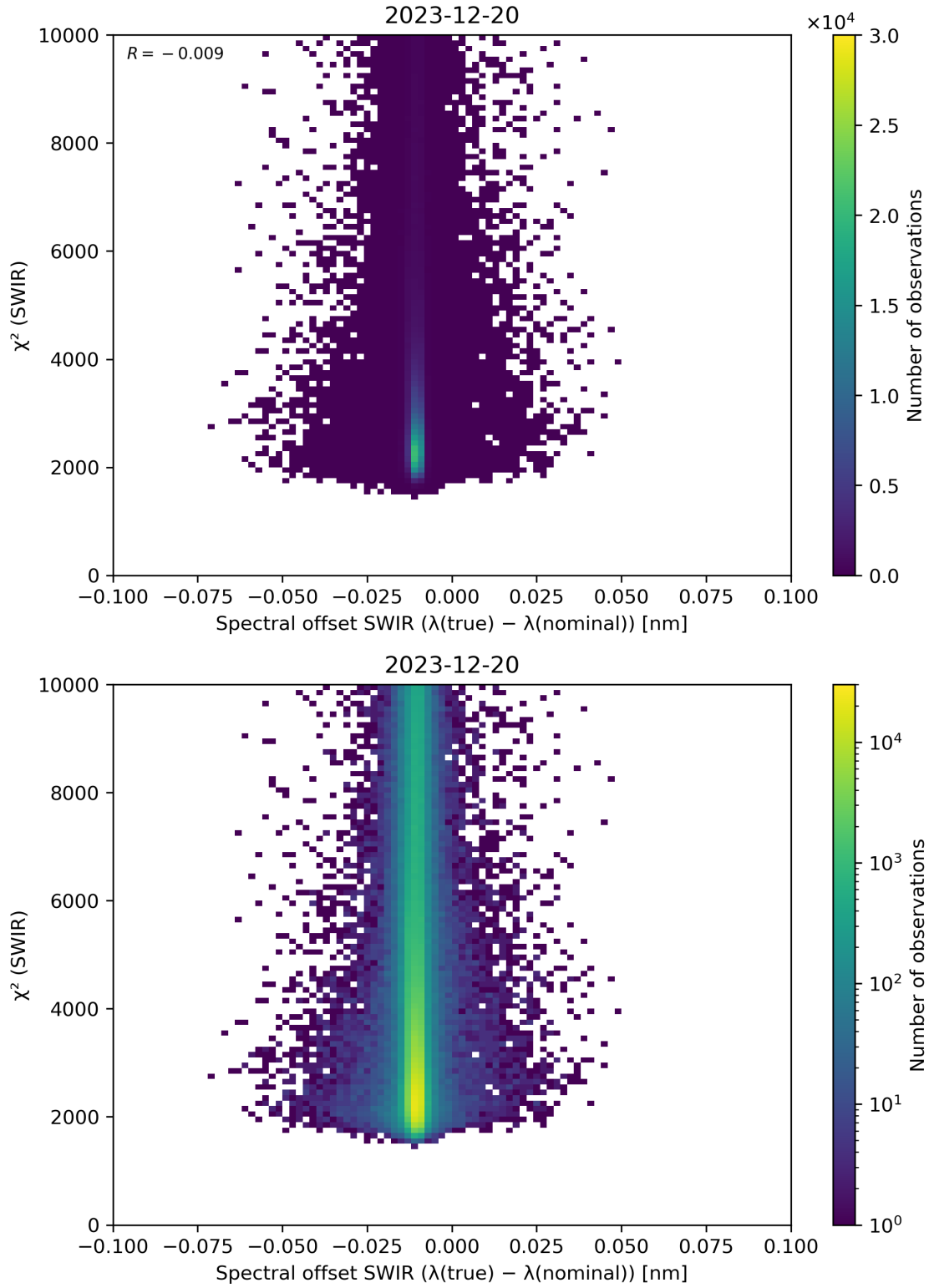
Figure 118: Scatter density plot of “Spectral offset SWIR ( \lambda(\text{true}) - \lambda(\text{nominal}) )” against “ \chi^2 (SWIR)” for 2023-12-20 to 2023-12-21.
