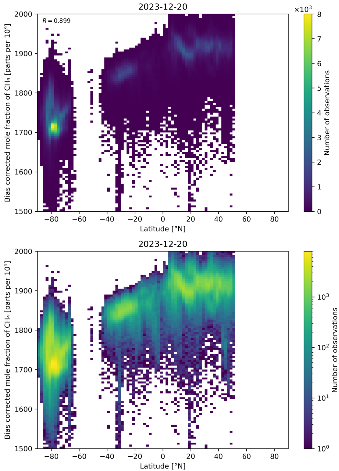
Figure 58: Scatter density plot of “Latitude” against “Bias corrected mole fraction of CH 4 ” for 2023-12-20 to 2023-12-21.
