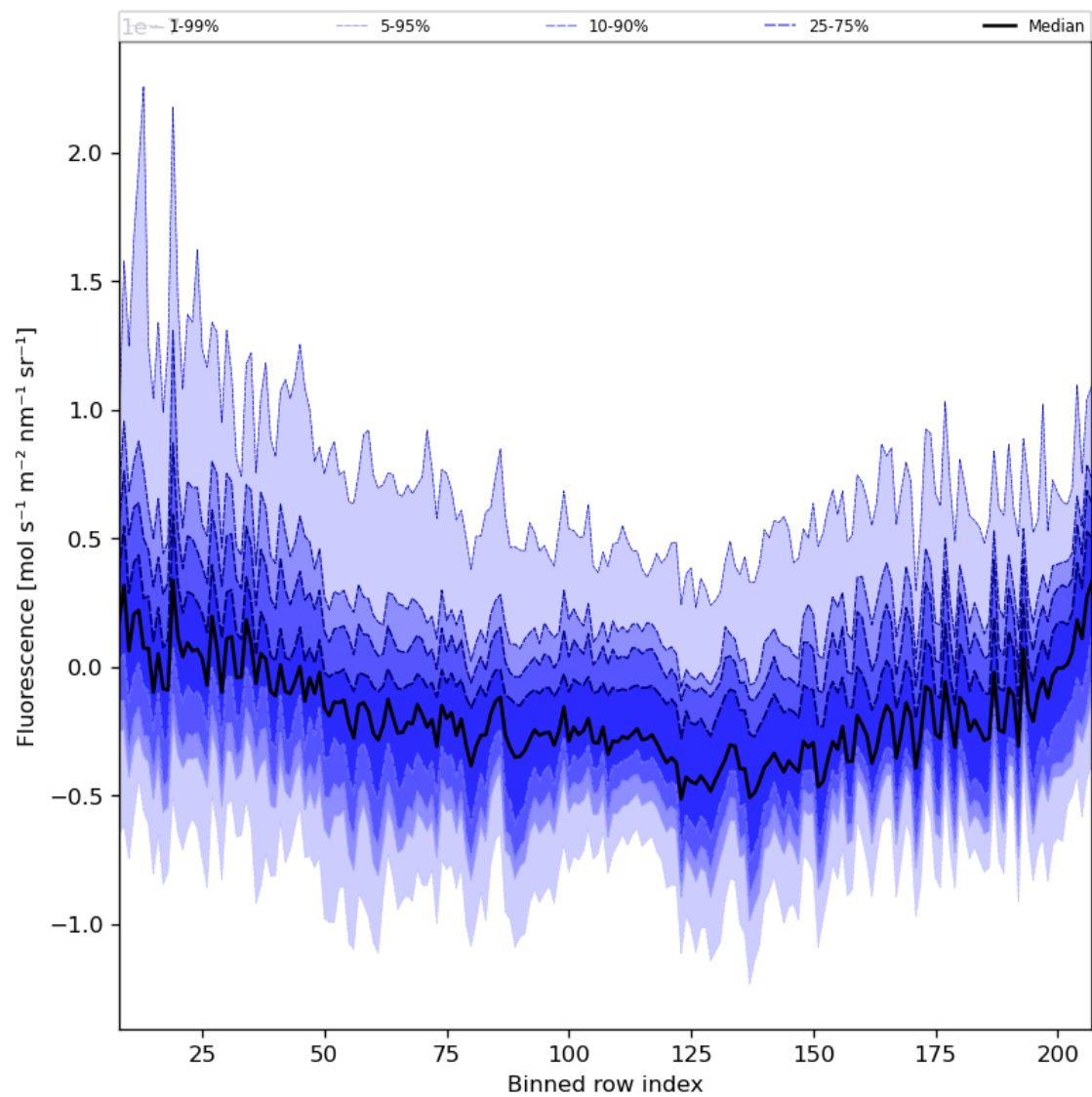
Figure 43: Along track statistics of “Fluorescence” for 2023-12-20 to 2023-12-21
