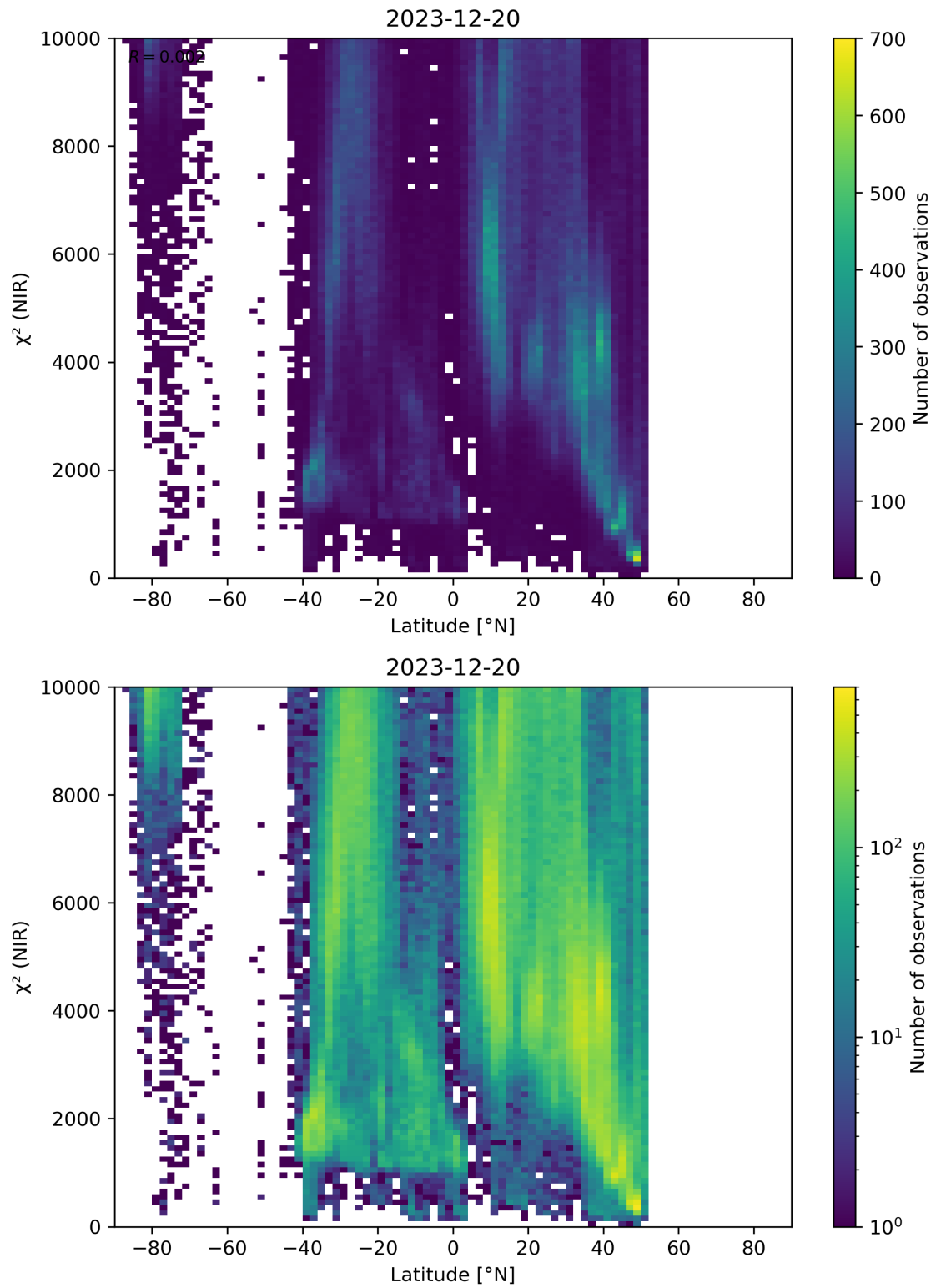
Figure 53: Scatter density plot of “Latitude” against “ \chi^2 (NIR)” for 2023-12-20 to 2023-12-21.
