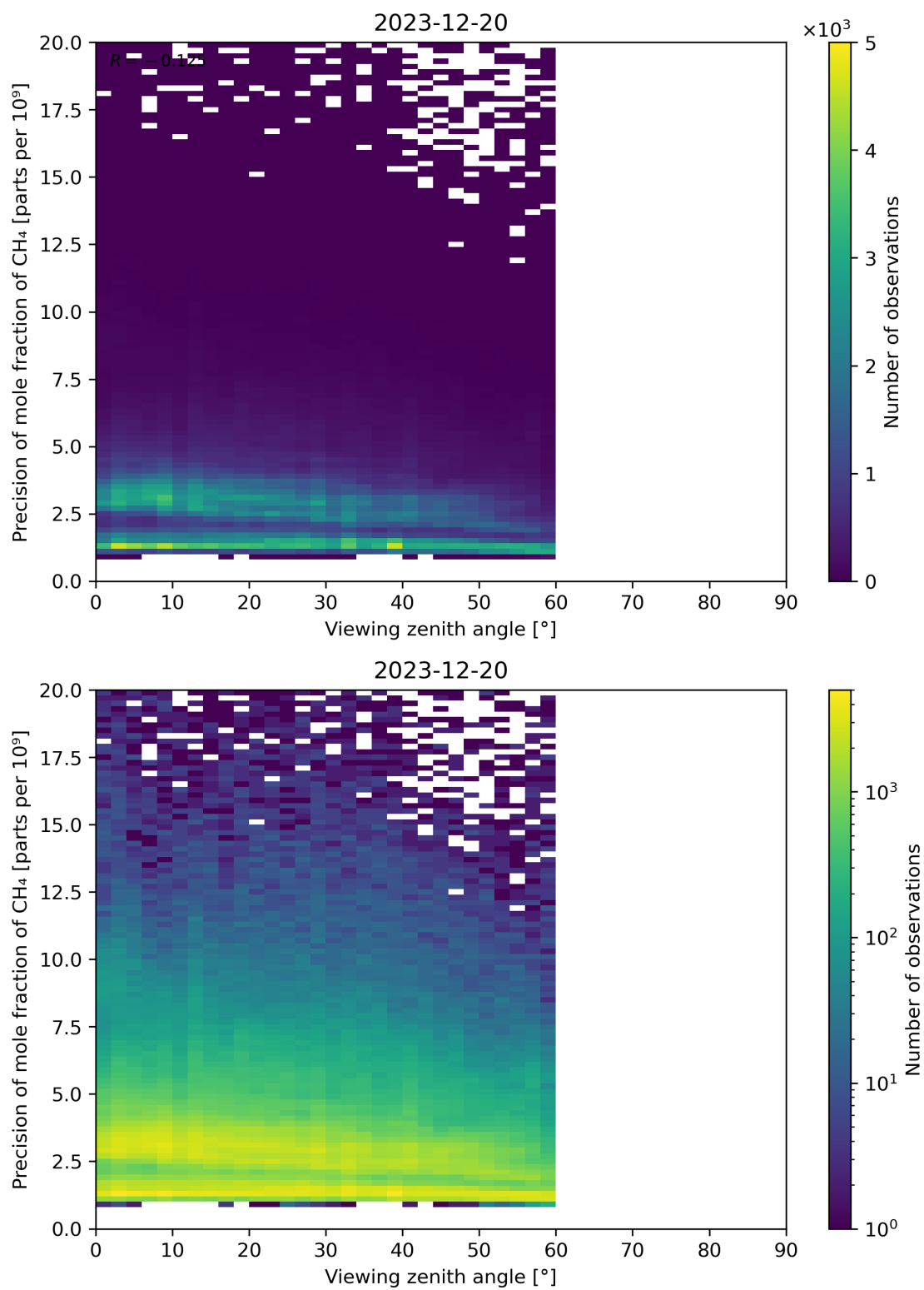
Figure 112: Scatter density plot of “Viewing zenith angle” against “Precision of mole fraction of CH 4 ” for 2023-12-20 to 2023-12-21.
