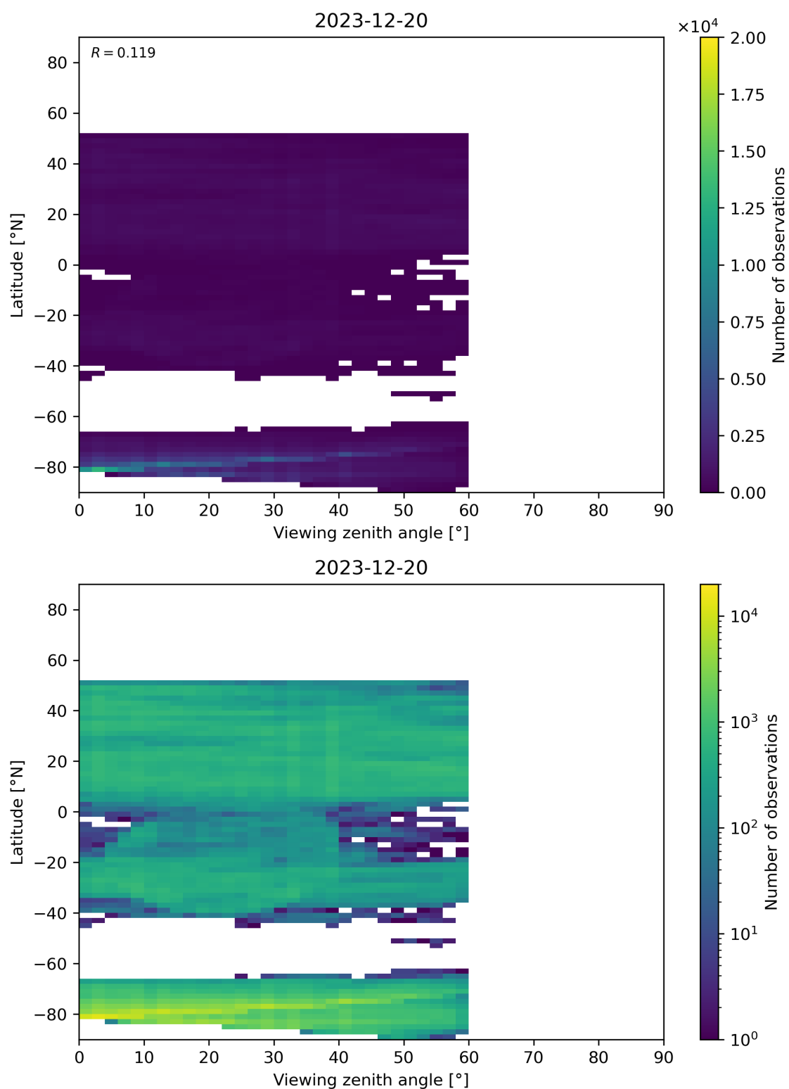
Figure 109: Scatter density plot of “Viewing zenith angle” against “Latitude” for 2023-12-20 to 2023-12-21.
