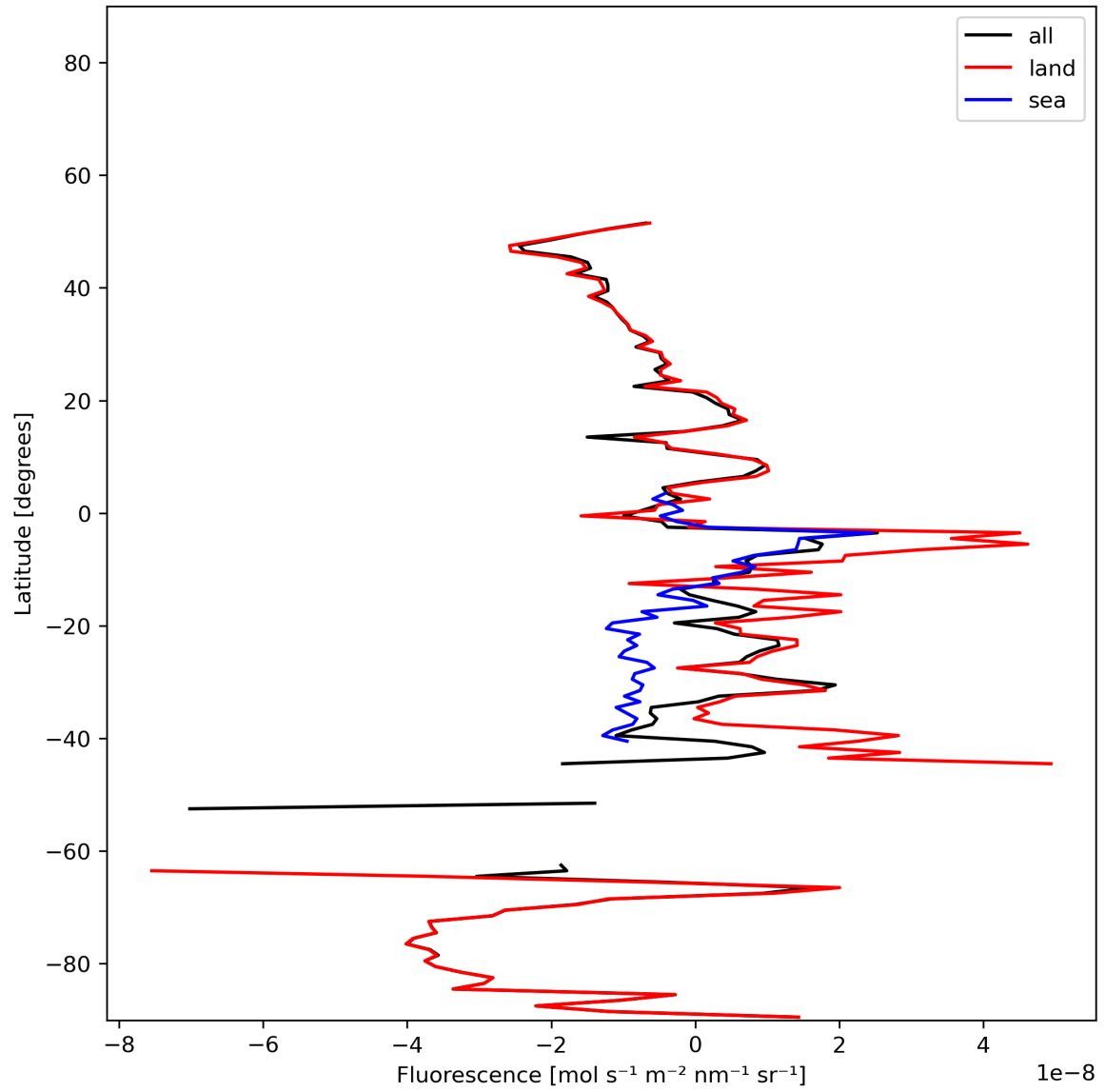
Figure 21: Zonal average of “Fluorescence” for 2023-12-20 to 2023-12-21.
