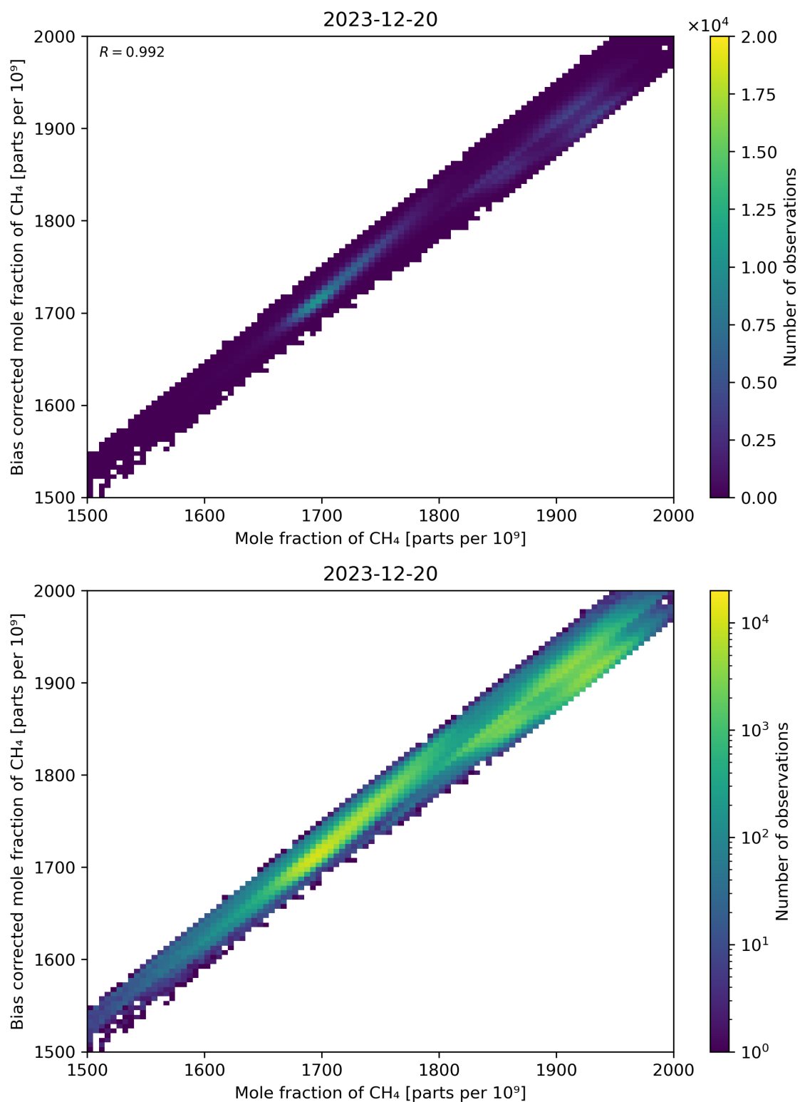
Figure 74: Scatter density plot of “Mole fraction of CH 4 ” against “Bias corrected mole fraction of CH 4 ” for 2023-12-20 to 2023-12-21.
