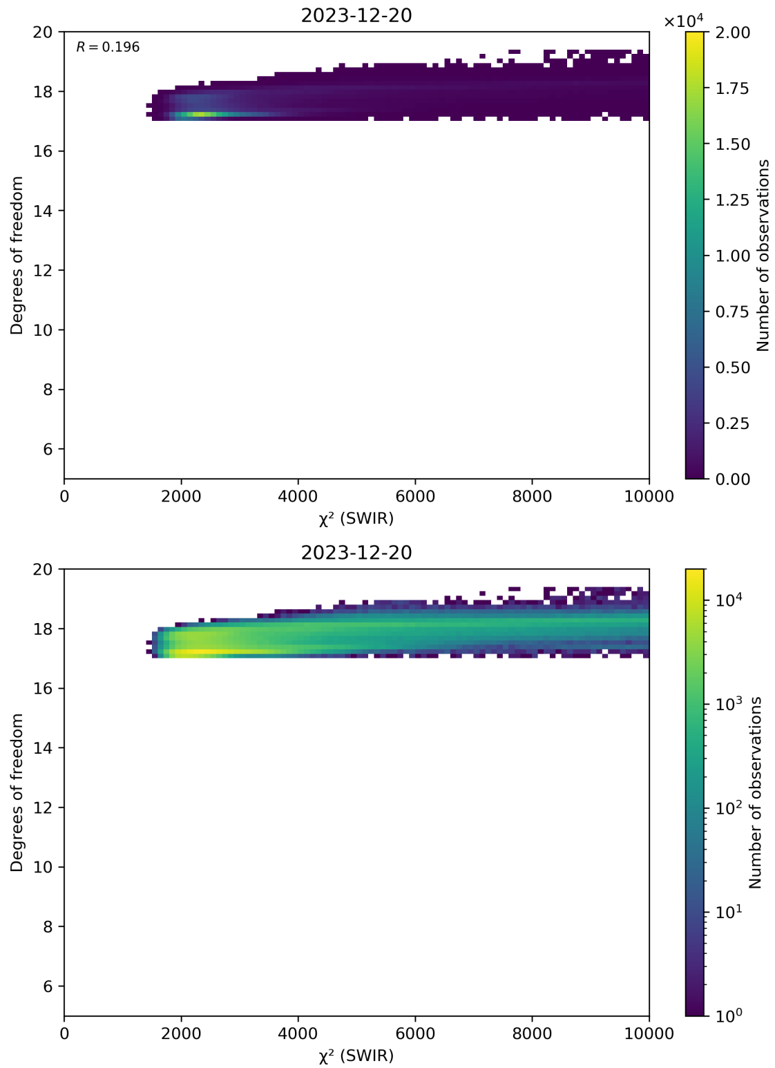
Figure 48: Scatter density plot of “ \chi^2 (SWIR)” against “Degrees of freedom” for 2023-12-20 to 2023-12-21.
