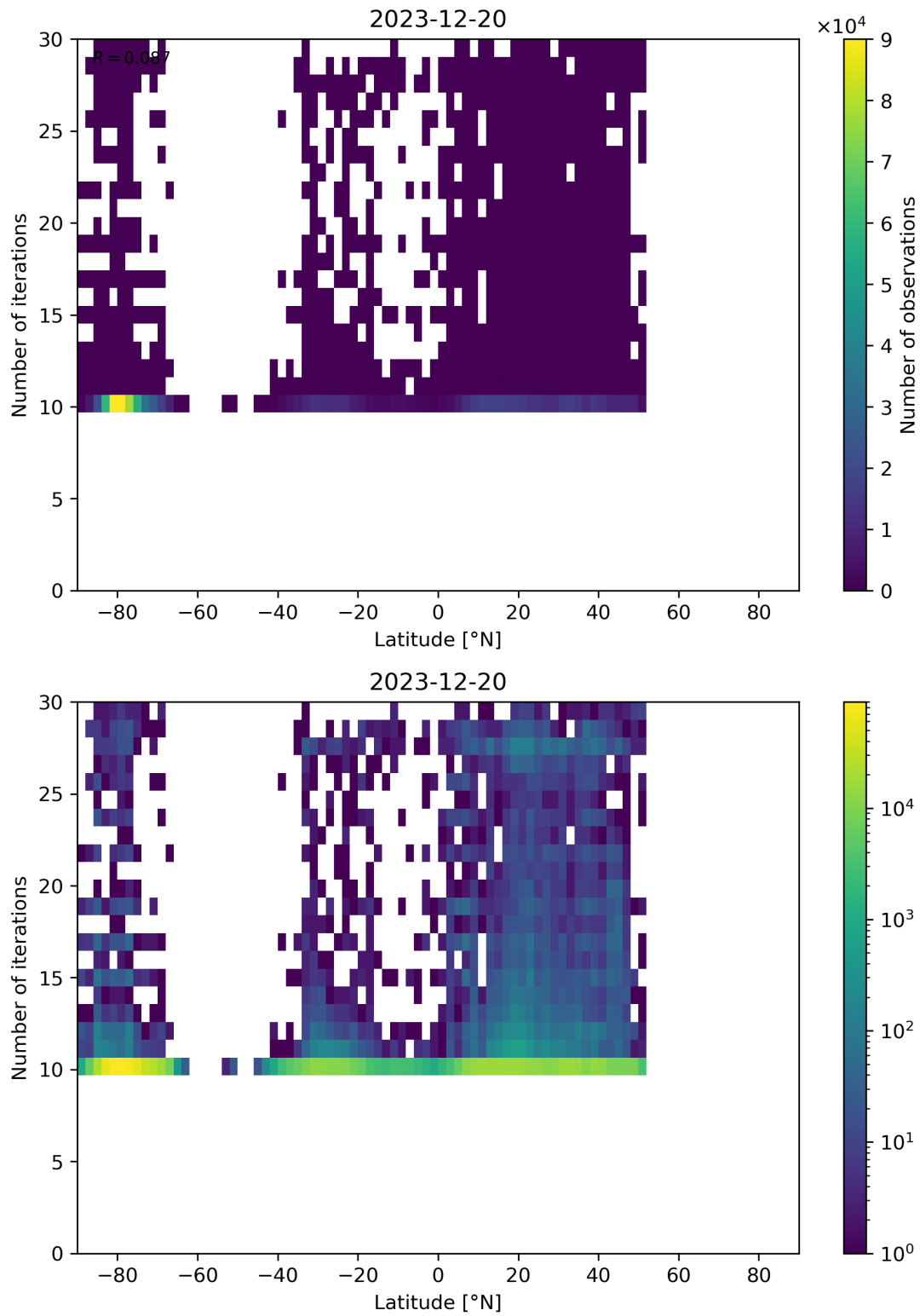
Figure 60: Scatter density plot of “Latitude” against “Number of iterations” for 2023-12-20 to 2023-12-21.
