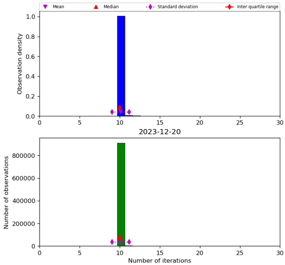
Figure 31: Histogram of “Number of iterations” for 2023-12-20 to 2023-12-21
