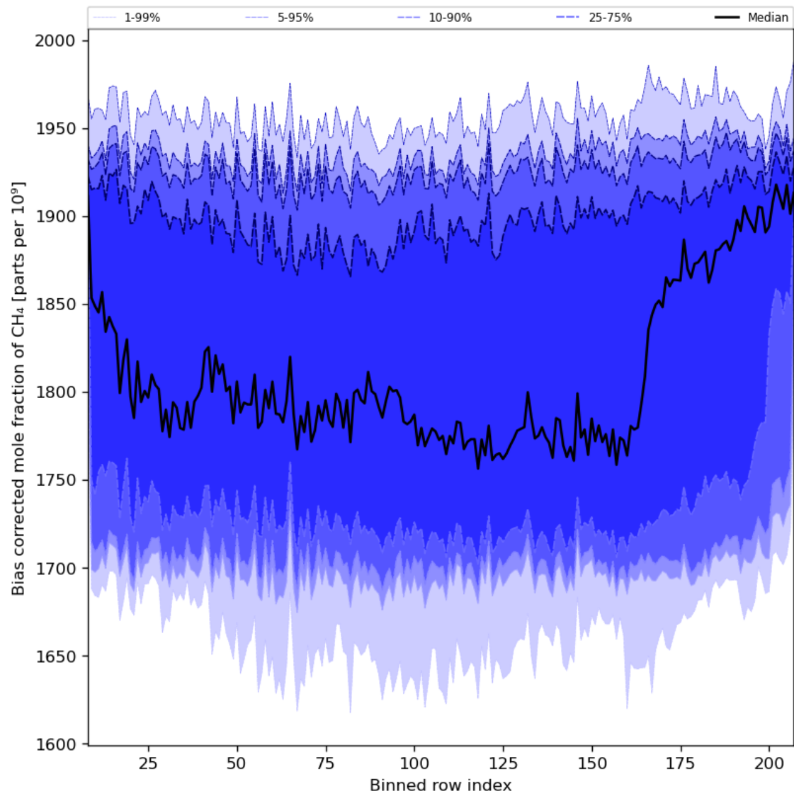
Figure 36: Along track statistics of “Bias corrected mole fraction of CH 4 ” for 2023-12-20 to 2023-12-21
