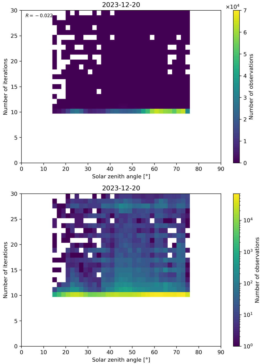
Figure 102: Scatter density plot of “Solar zenith angle” against “Number of iterations” for 2023-12-20 to 2023-12-21.
