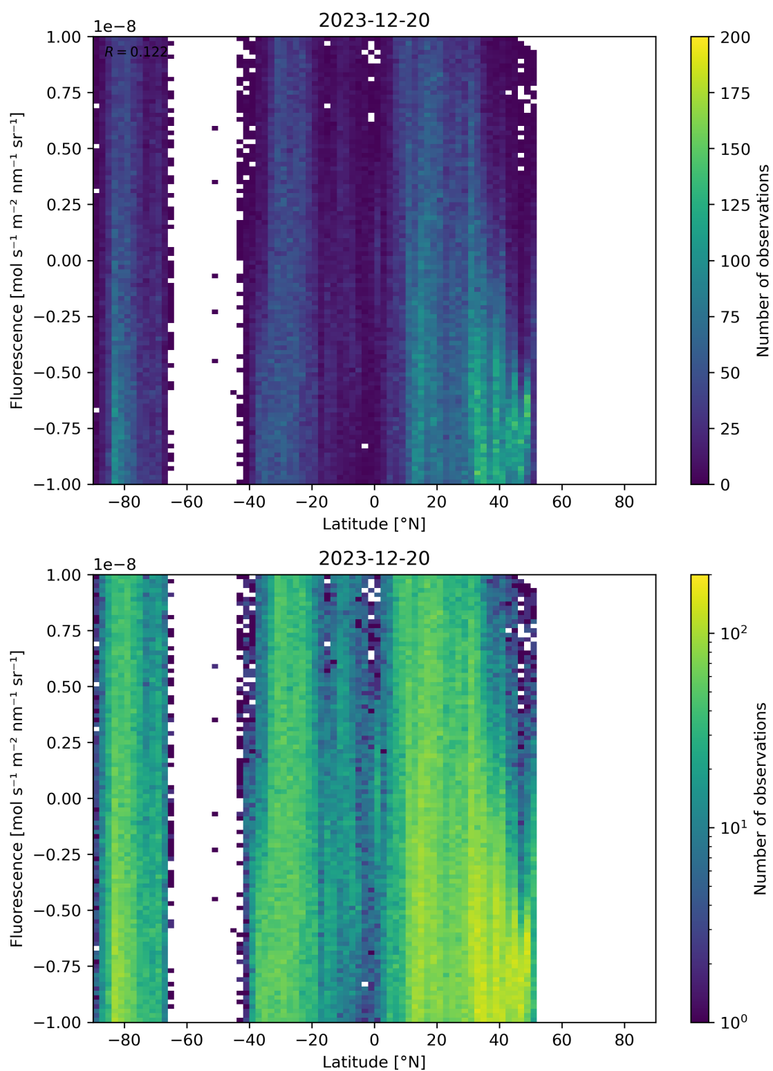
Figure 56: Scatter density plot of “Latitude” against “Fluorescence” for 2023-12-20 to 2023-12-21.
