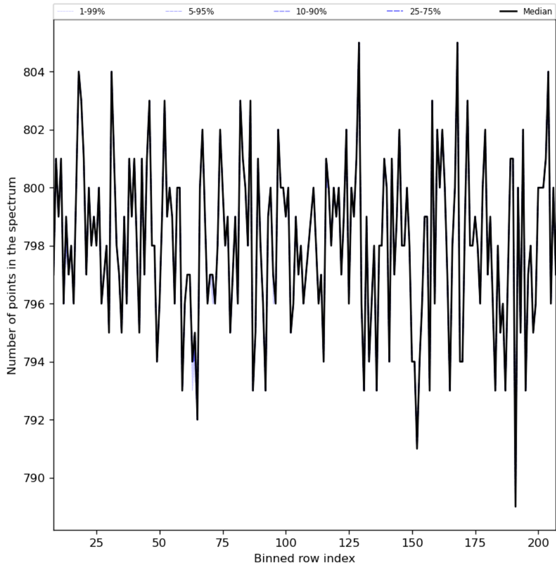
Figure 37: Along track statistics of “Number of points in the spectrum” for 2023-12-20 to 2023-12-21
