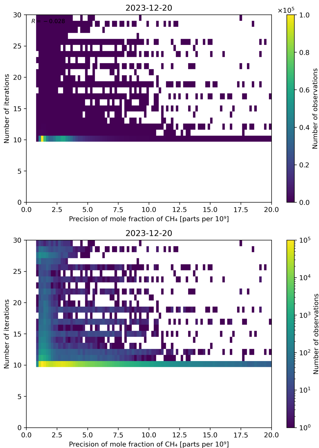
Figure 83: Scatter density plot of “Precision of mole fraction of CH 4 ” against “Number of iterations” for 2023-12-20 to 2023-12-21.
