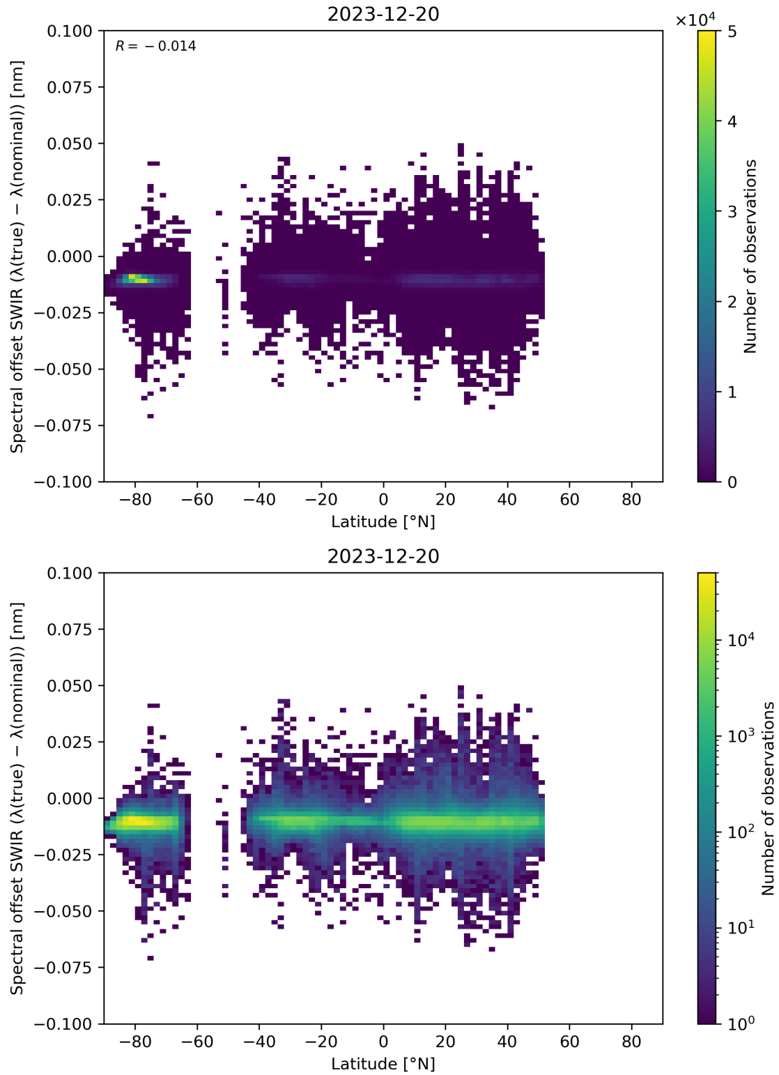
Figure 62: Scatter density plot of “Latitude” against “Spectral offset SWIR ( \lambda(\text{true}) - \lambda(\text{nominal}) )” for 2023-12-20 to 2023-12-21.
