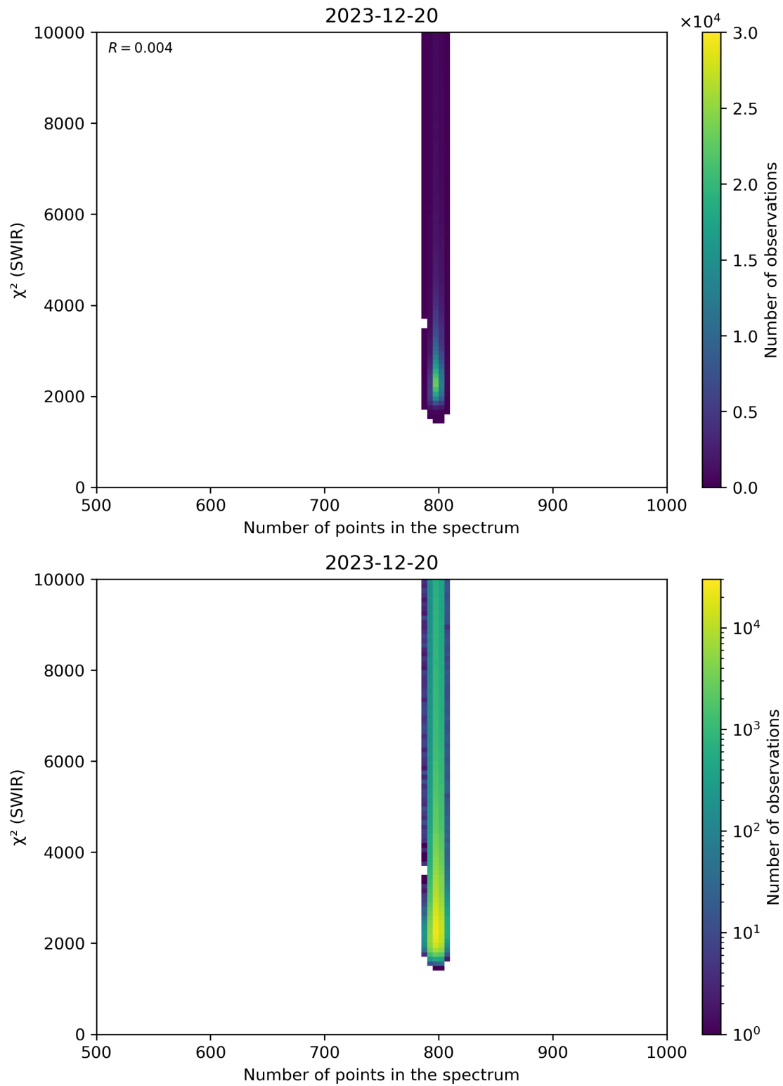
Figure 89: Scatter density plot of “Number of points in the spectrum” against “ \chi^2 (SWIR)” for 2023-12-20 to 2023-12-21.
