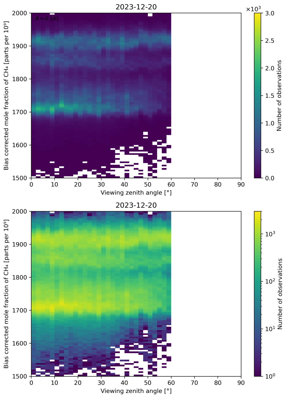
Figure 111: Scatter density plot of “Viewing zenith angle” against “Bias corrected mole fraction of CH 4 ” for 2023-12-20 to 2023-12-21.
