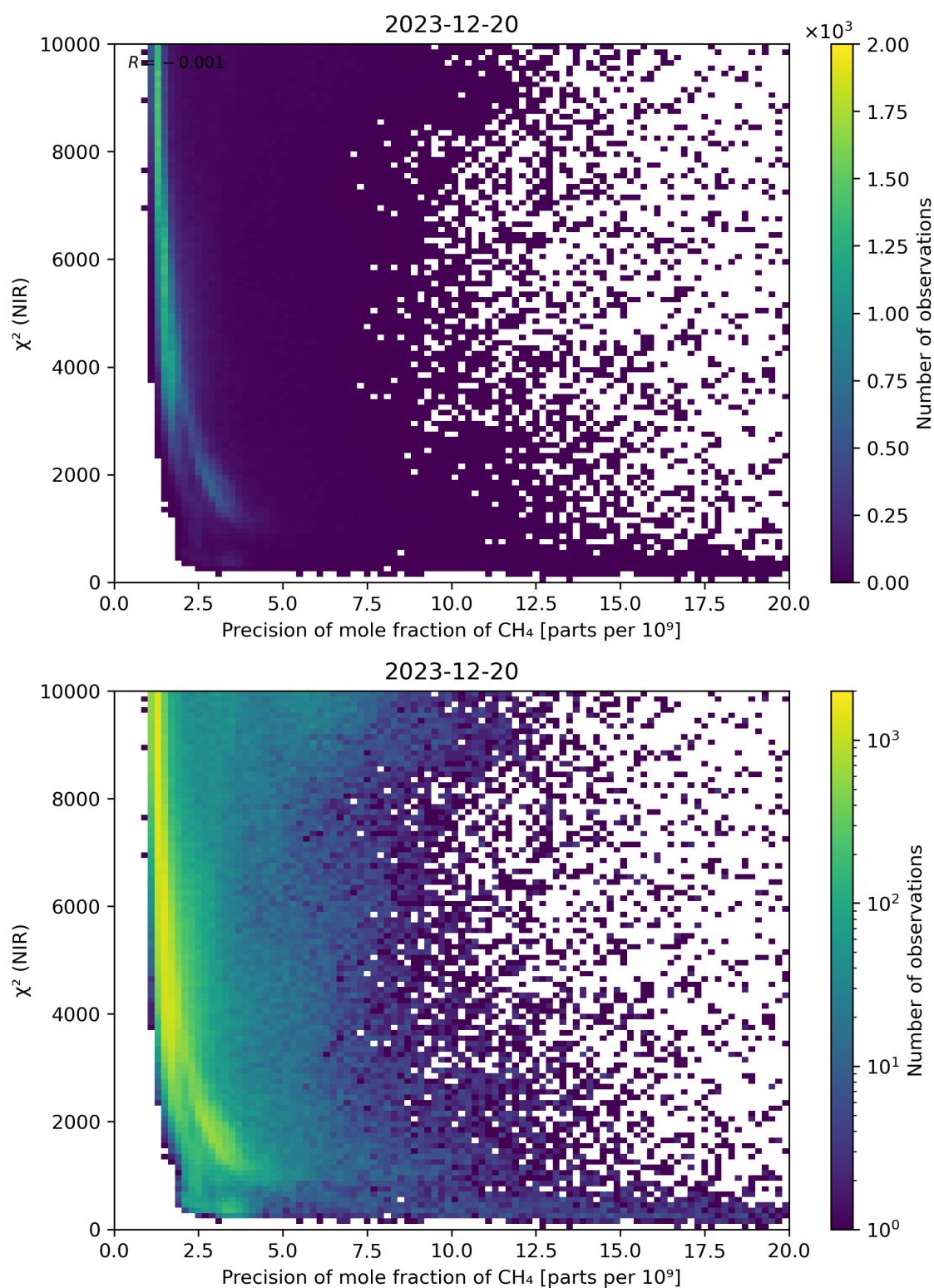
Figure 78: Scatter density plot of “Precision of mole fraction of CH 4 ” against “ \chi^2 (NIR)” for 2023-12-20 to 2023-12-21.
