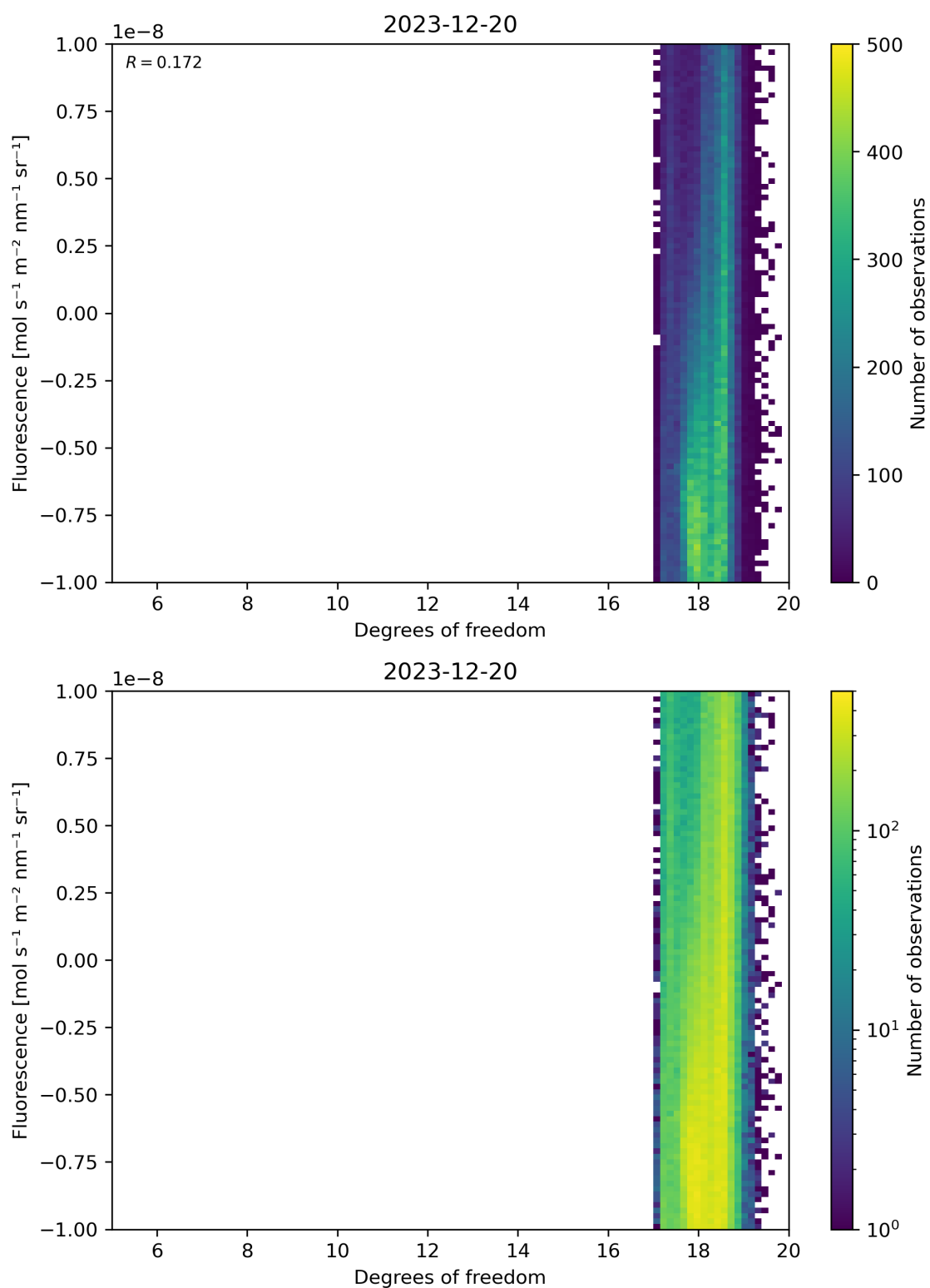
Figure 51: Scatter density plot of “Degrees of freedom” against “Fluorescence” for 2023-12-20 to 2023-12-21.
