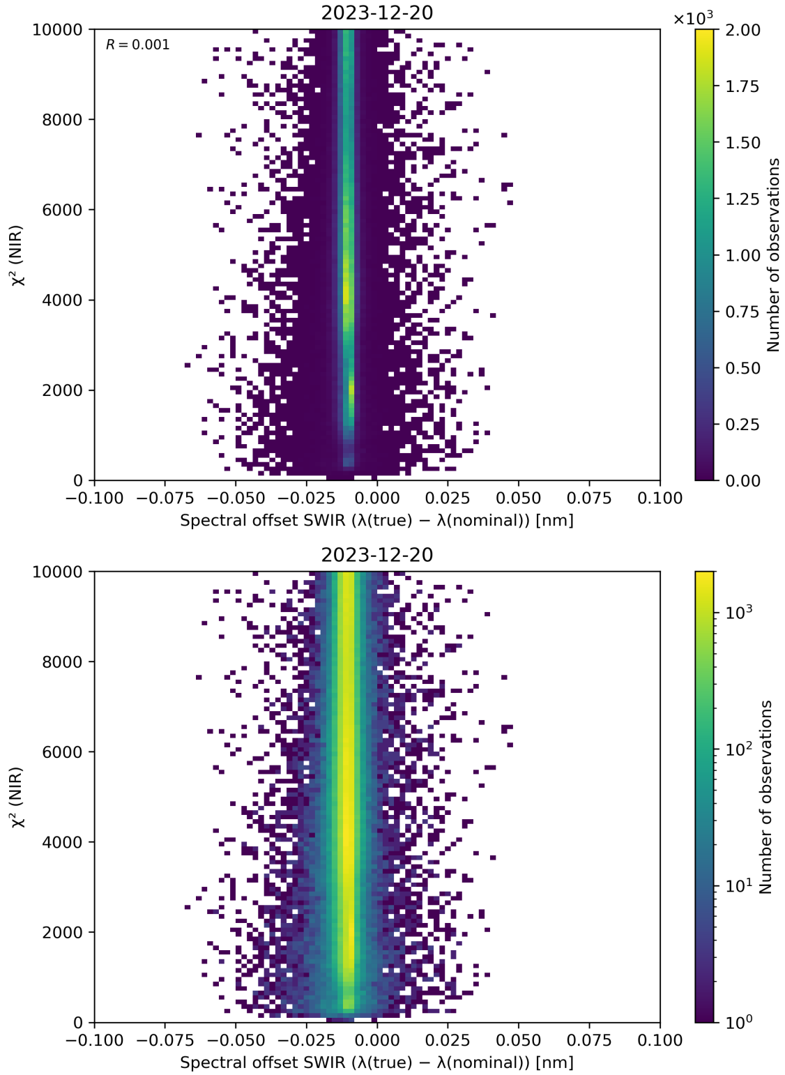
Figure 117: Scatter density plot of “Spectral offset SWIR ( \lambda(\text{true}) - \lambda(\text{nominal}) )” against “ \chi^2 (NIR)” for 2023-12-20 to 2023-12-21.
