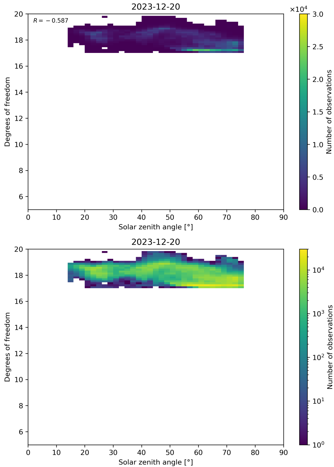
Figure 96: Scatter density plot of “Solar zenith angle” against “Degrees of freedom” for 2023-12-20 to 2023-12-21.
