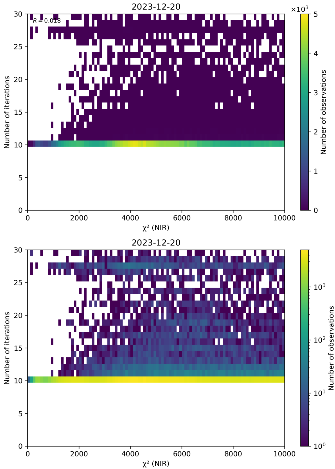
Figure 46: Scatter density plot of “ \chi^2 (NIR)” against “Number of iterations” for 2023-12-20 to 2023-12-21.
