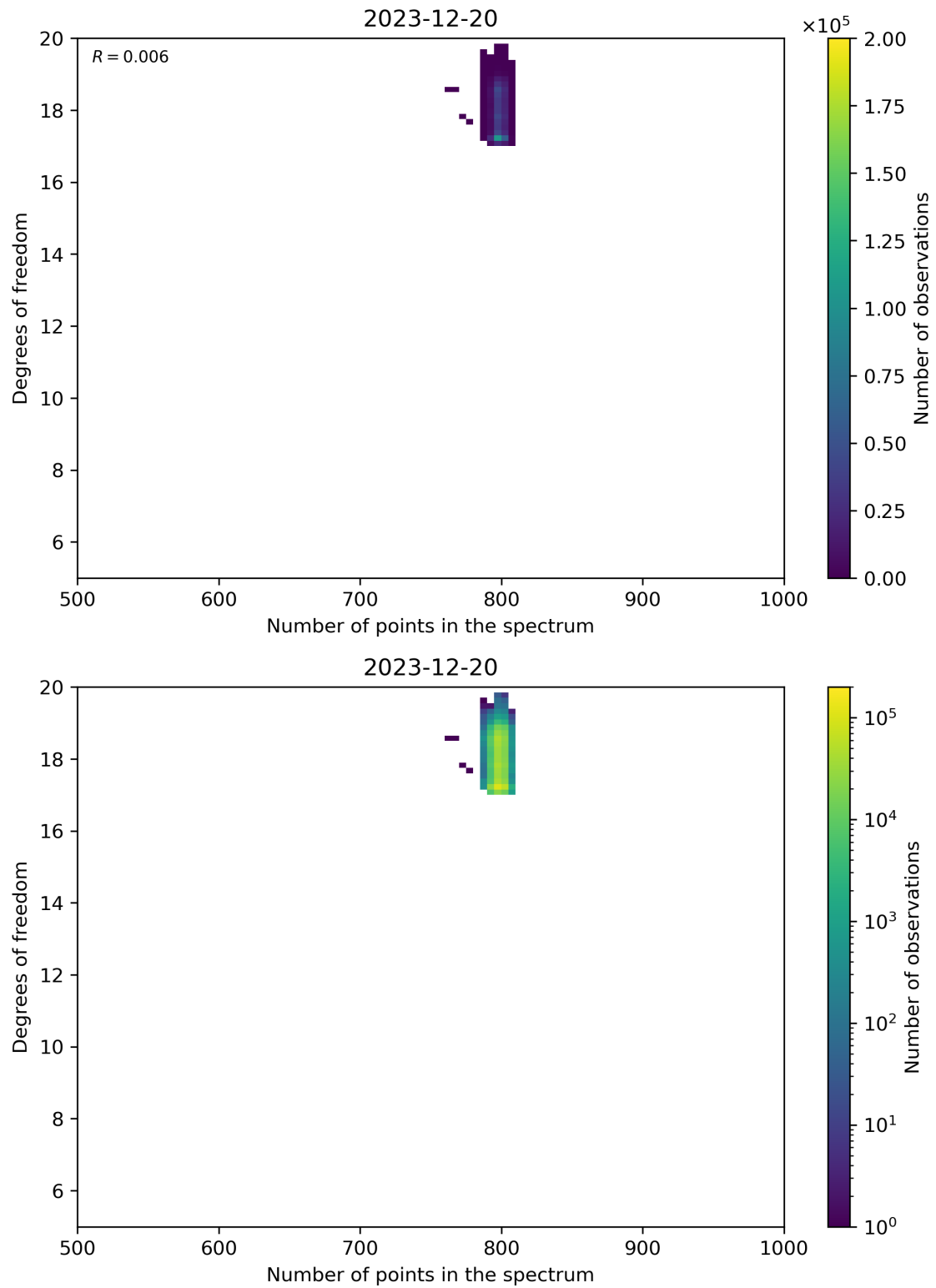
Figure 90: Scatter density plot of “Number of points in the spectrum” against “Degrees of freedom” for 2023-12-20 to 2023-12-21.
