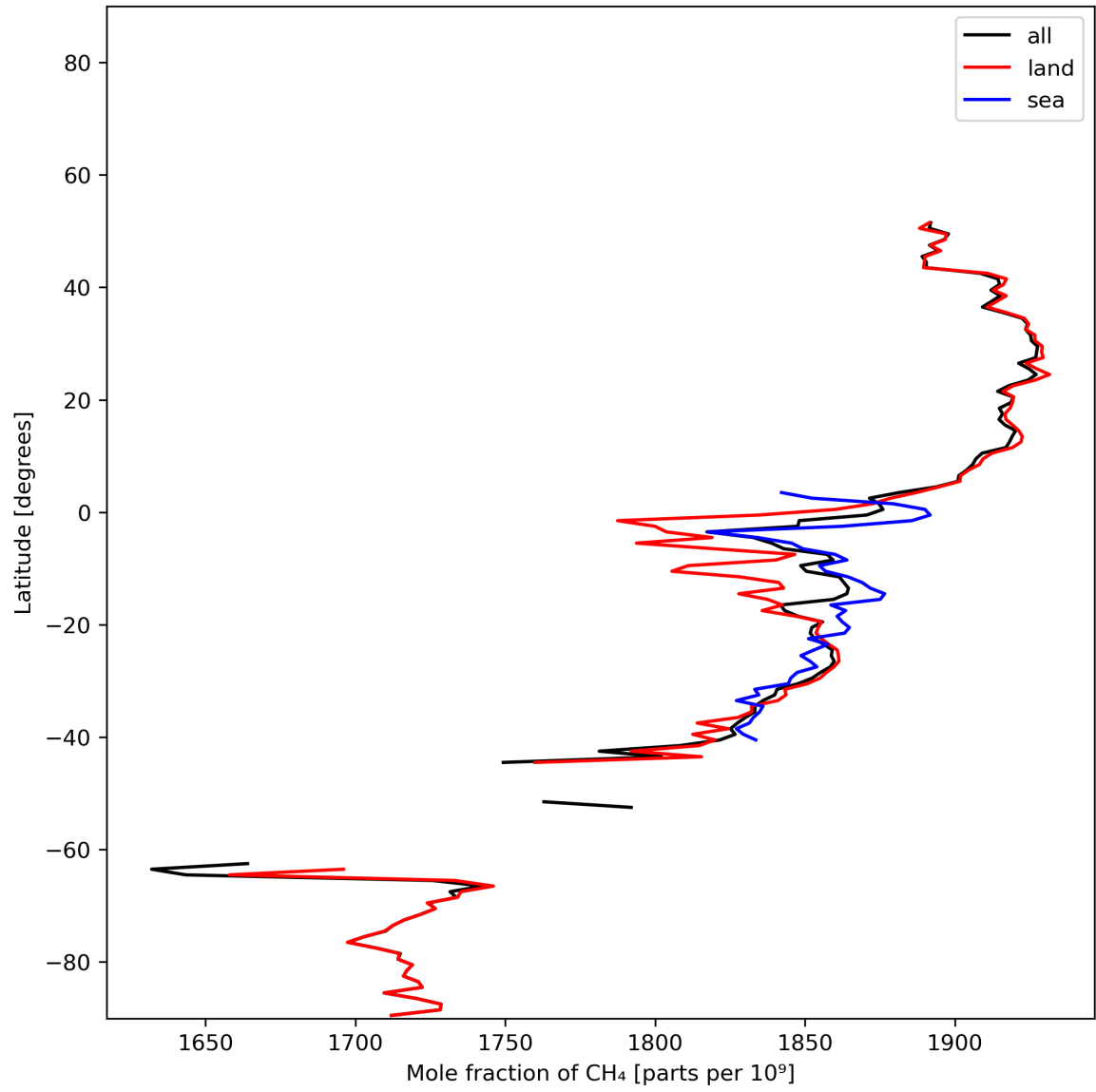
Figure 12: Zonal average of “Mole fraction of \text{CH}_4 ” for 2023-12-20 to 2023-12-21.
