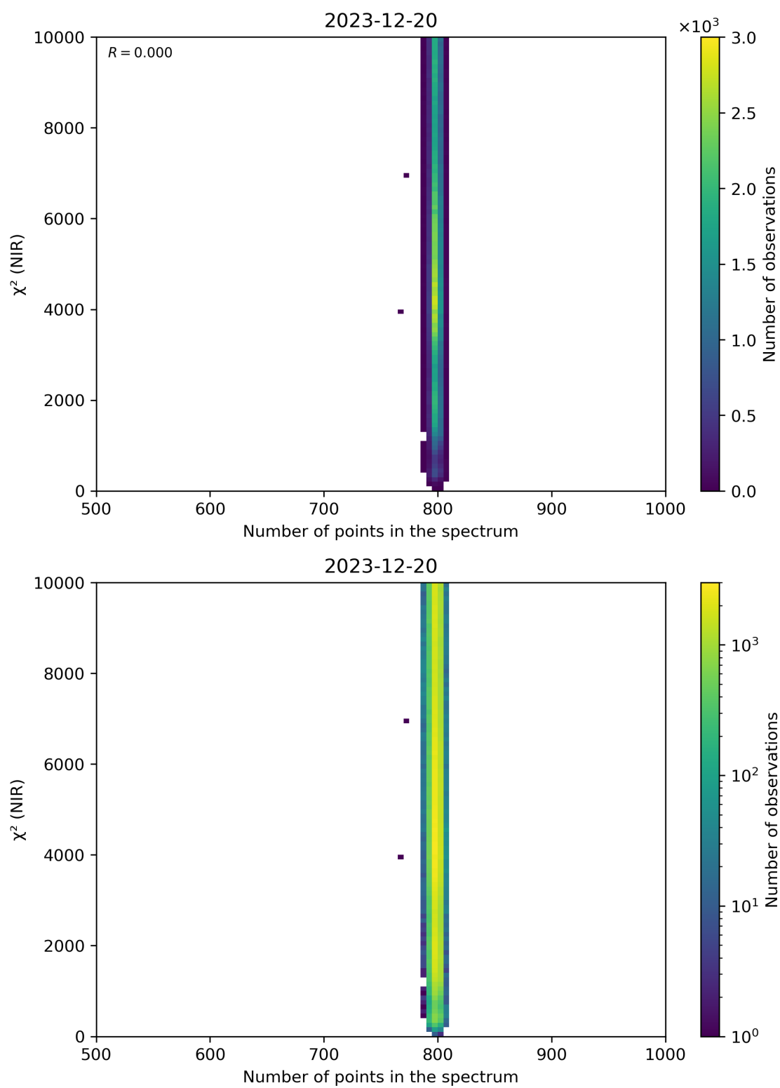
Figure 88: Scatter density plot of “Number of points in the spectrum” against “ \chi^2 (NIR)” for 2023-12-20 to 2023-12-21.
