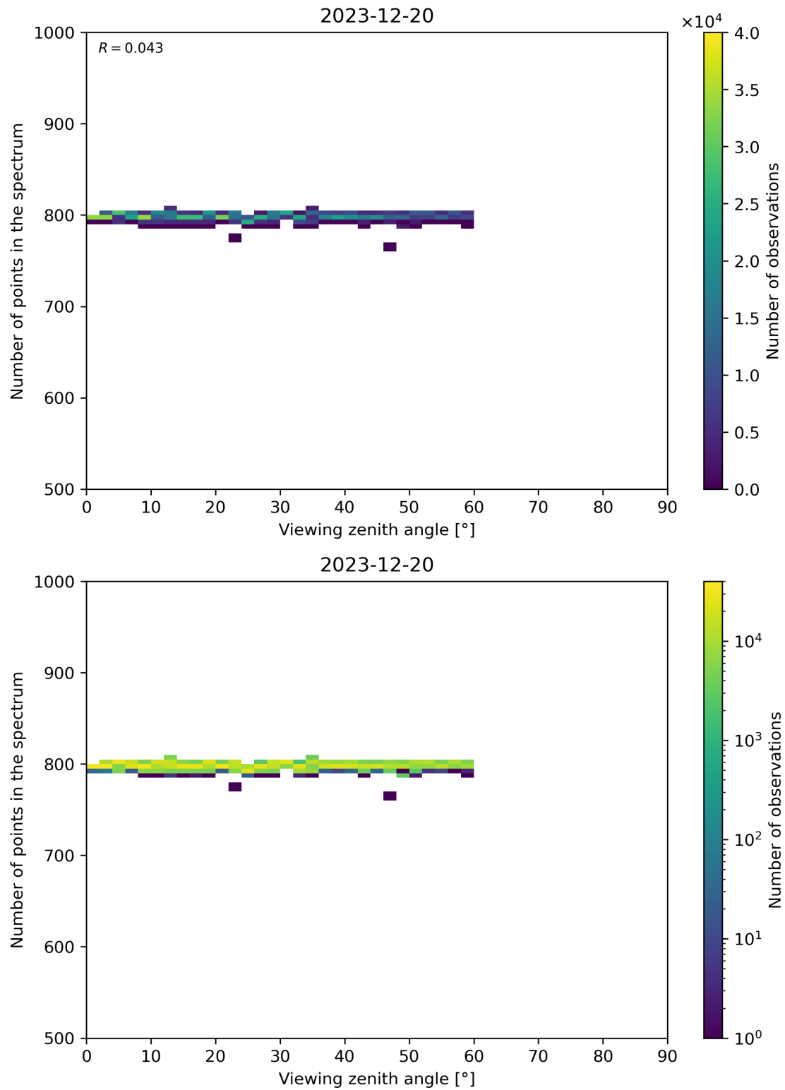
Figure 114: Scatter density plot of “Viewing zenith angle” against “Number of points in the spectrum” for 2023-12-20 to 2023-12-21.
