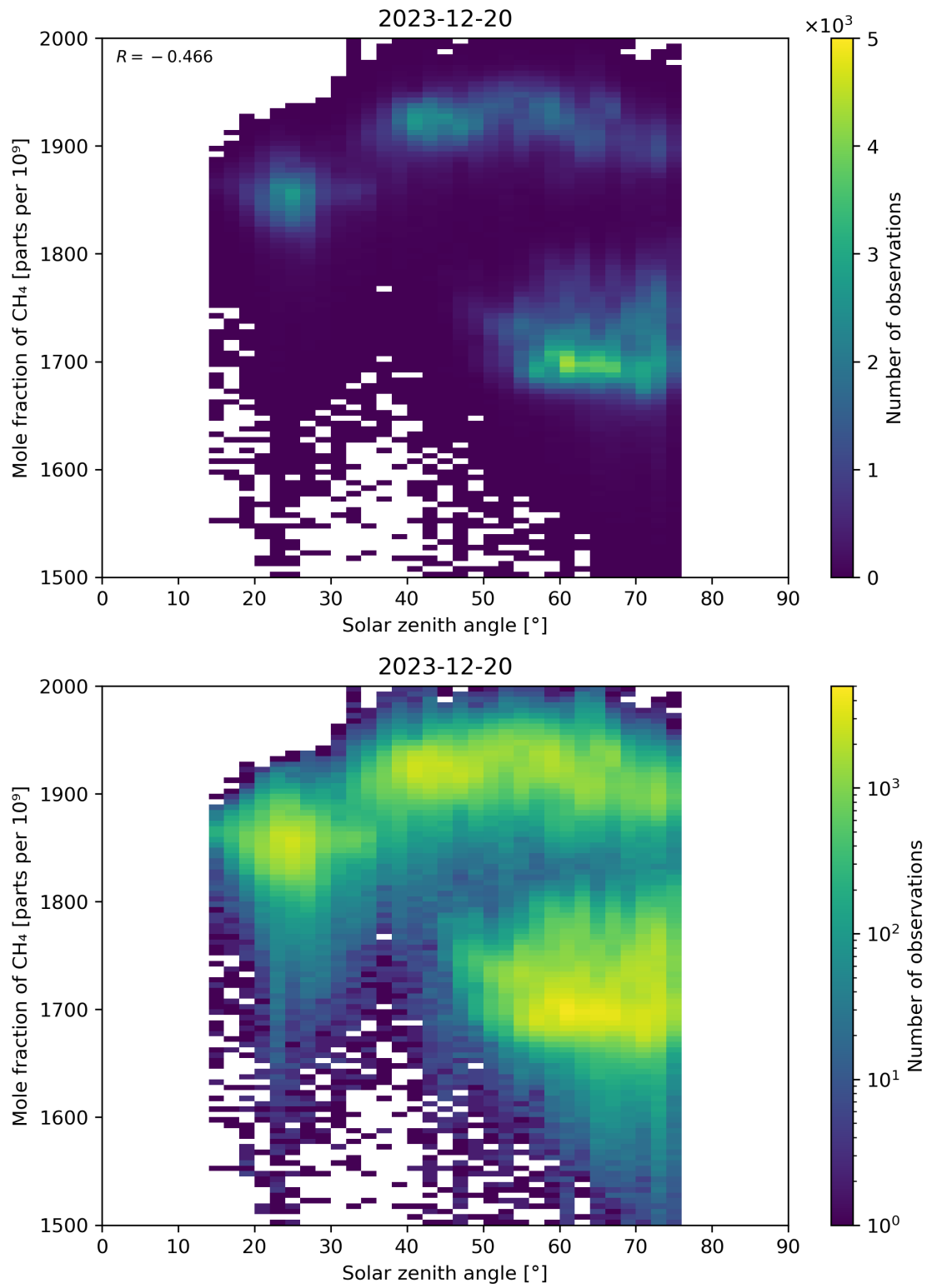
Figure 99: Scatter density plot of “Solar zenith angle” against “Mole fraction of CH 4 ” for 2023-12-20 to 2023-12-21.
