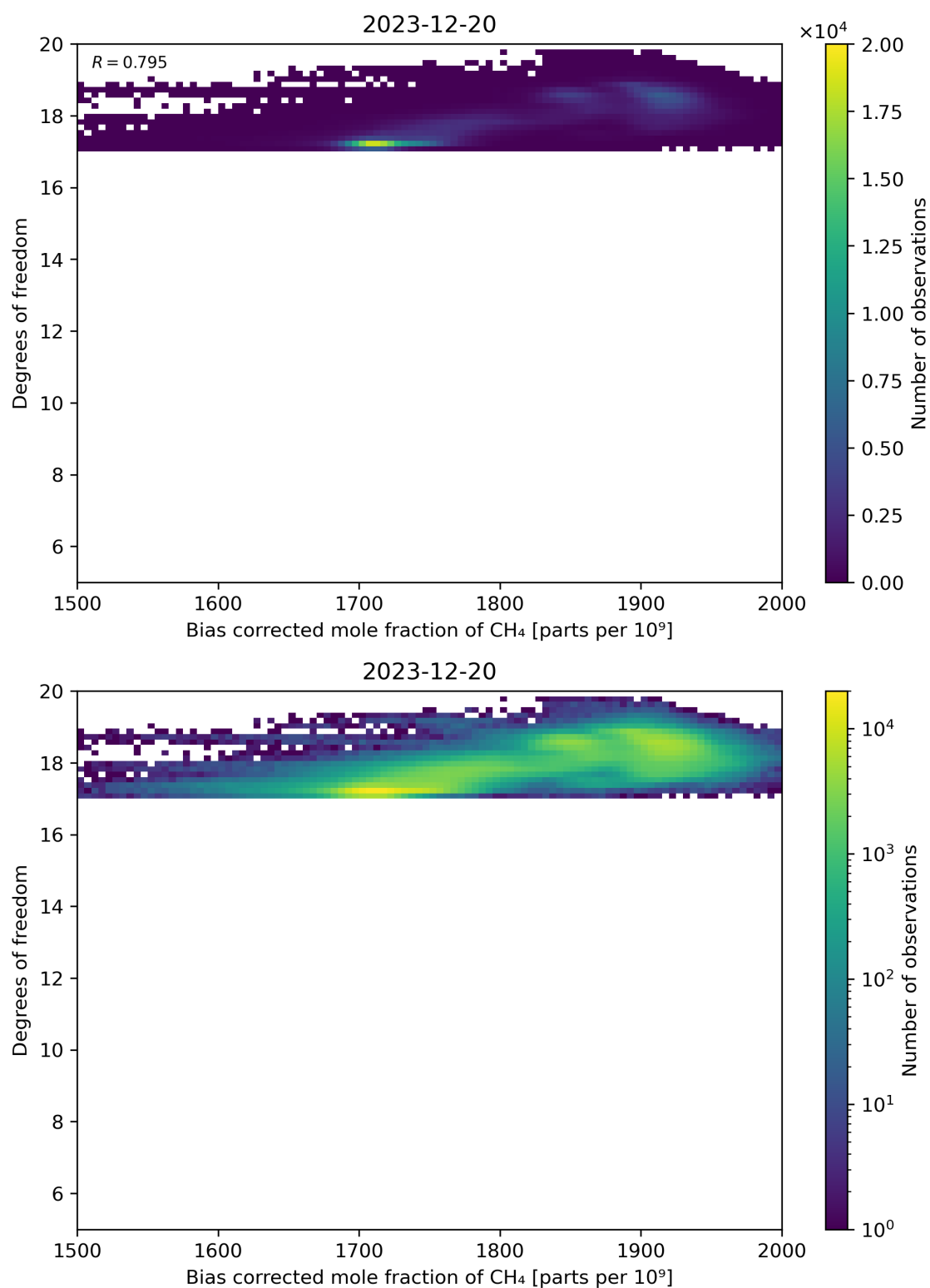
Figure 65: Scatter density plot of “Bias corrected mole fraction of CH 4 ” against “Degrees of freedom” for 2023-12-20 to 2023-12-21.
