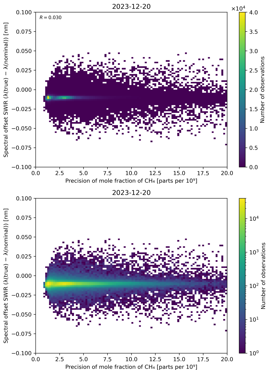
Figure 85: Scatter density plot of “Precision of mole fraction of CH 4 ” against “Spectral offset SWIR ( \lambda(\text{true}) - \lambda(\text{nominal}) )” for 2023-12-20 to 2023-12-21.
