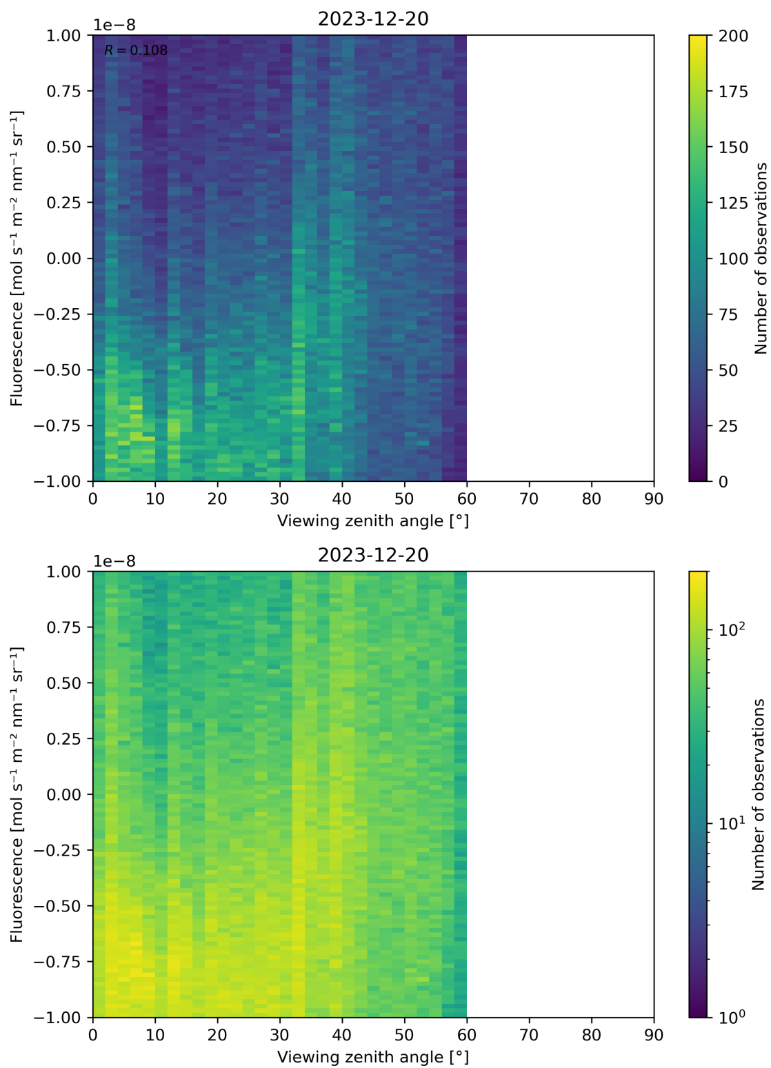
Figure 108: Scatter density plot of “Viewing zenith angle” against “Fluorescence” for 2023-12-20 to 2023-12-21.
