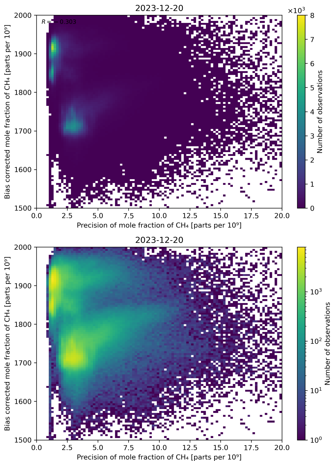
Figure 82: Scatter density plot of “Precision of mole fraction of \text{CH}_4 ” against “Bias corrected mole fraction of \text{CH}_4 ” for 2023-12-20 to 2023-12-21.
