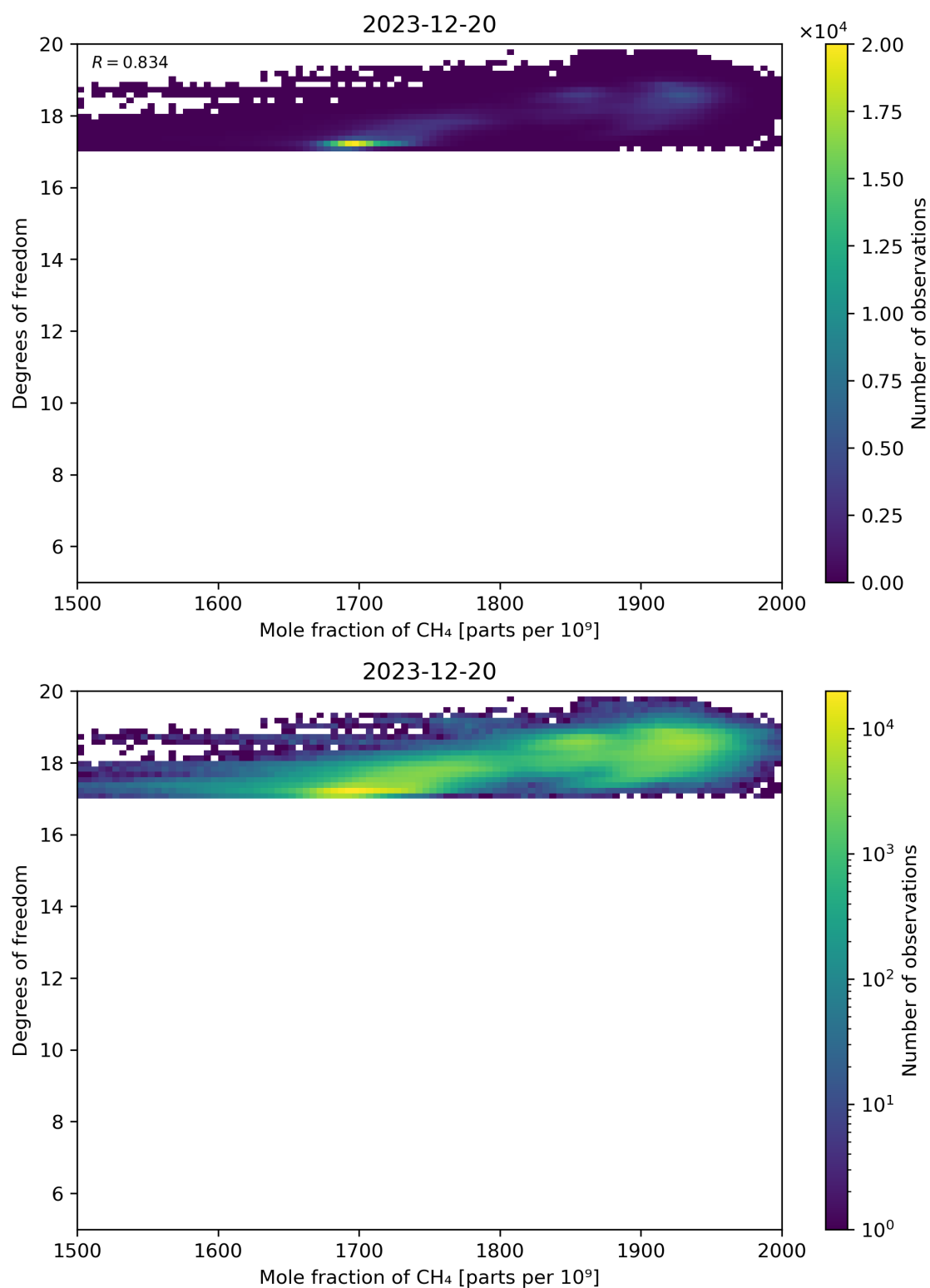
Figure 72: Scatter density plot of “Mole fraction of CH 4 ” against “Degrees of freedom” for 2023-12-20 to 2023-12-21.
