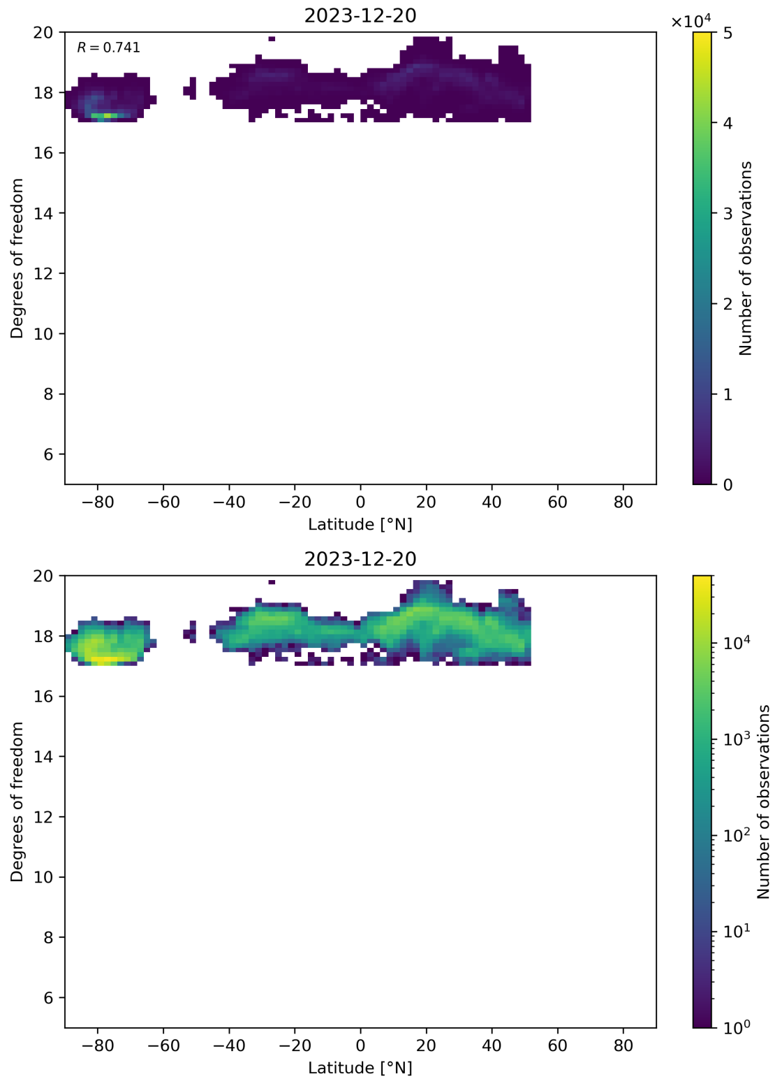
Figure 55: Scatter density plot of “Latitude” against “Degrees of freedom” for 2023-12-20 to 2023-12-21.
