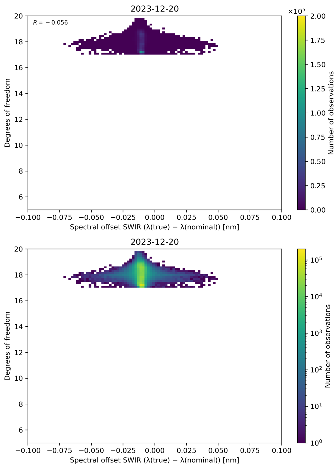
Figure 119: Scatter density plot of “Spectral offset SWIR ( \lambda(\text{true}) - \lambda(\text{nominal}) )” against “Degrees of freedom” for 2023-12-20 to 2023-12-21.
