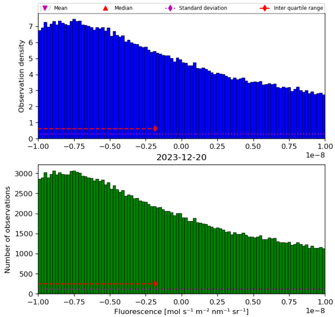
Figure 32: Histogram of “Fluorescence” for 2023-12-20 to 2023-12-21
