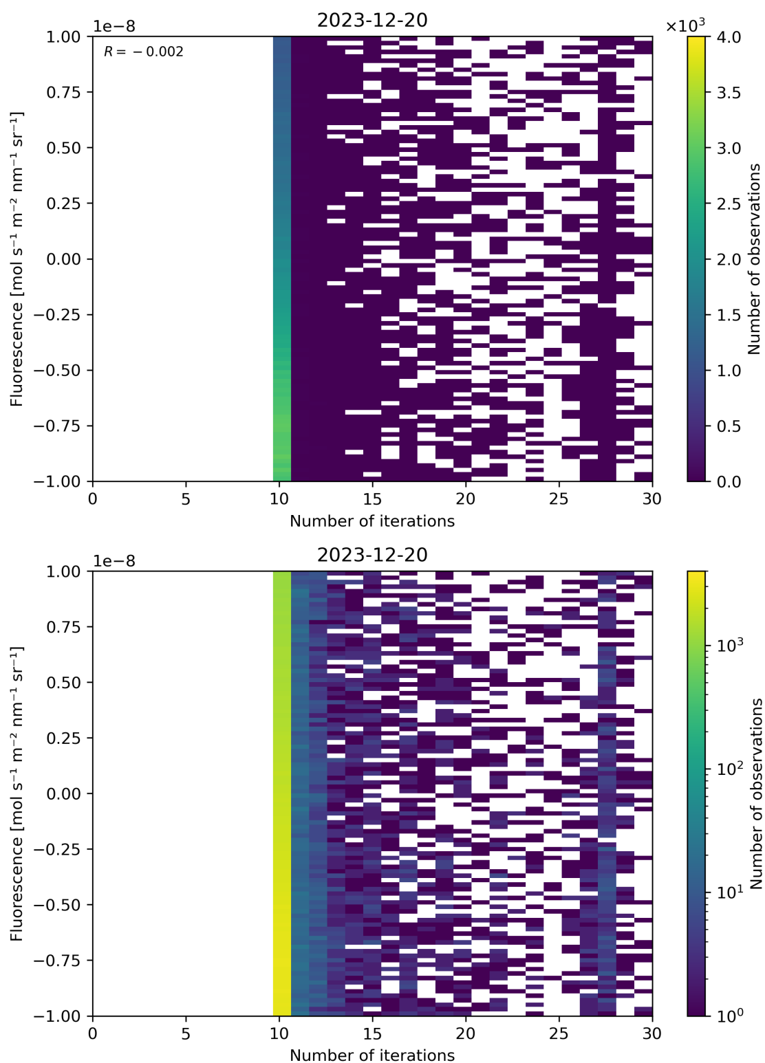
Figure 87: Scatter density plot of “Number of iterations” against “Fluorescence” for 2023-12-20 to 2023-12-21.
