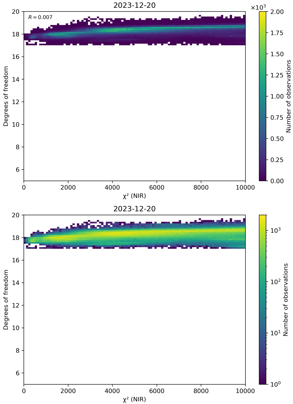
Figure 44: Scatter density plot of “ \chi^2 (NIR)” against “Degrees of freedom” for 2023-12-20 to 2023-12-21.
