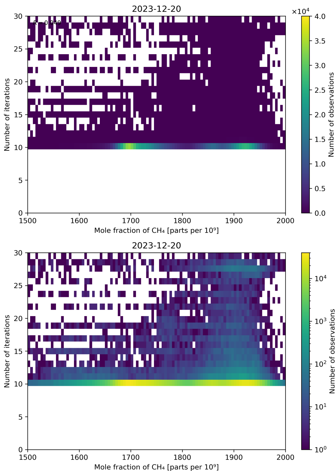
Figure 76: Scatter density plot of “Mole fraction of CH 4 ” against “Number of iterations” for 2023-12-20 to 2023-12-21.
