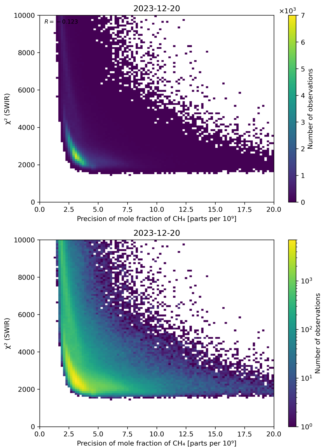
Figure 79: Scatter density plot of “Precision of mole fraction of CH 4 ” against “ \chi^2 (SWIR)” for 2023-12-20 to 2023-12-21.
