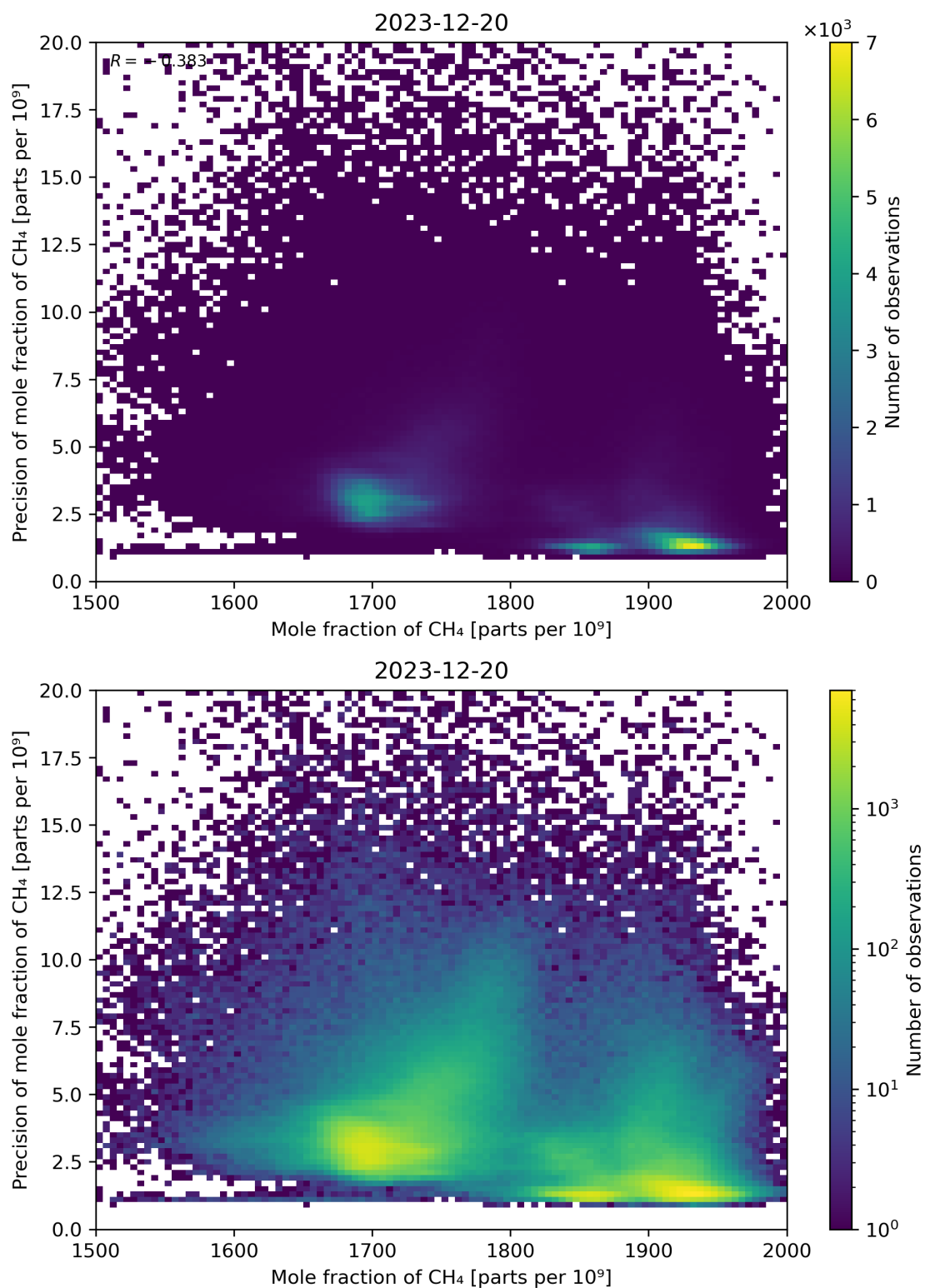
Figure 75: Scatter density plot of “Mole fraction of CH 4 ” against “Precision of mole fraction of CH 4 ” for 2023-12-20 to 2023-12-21.
