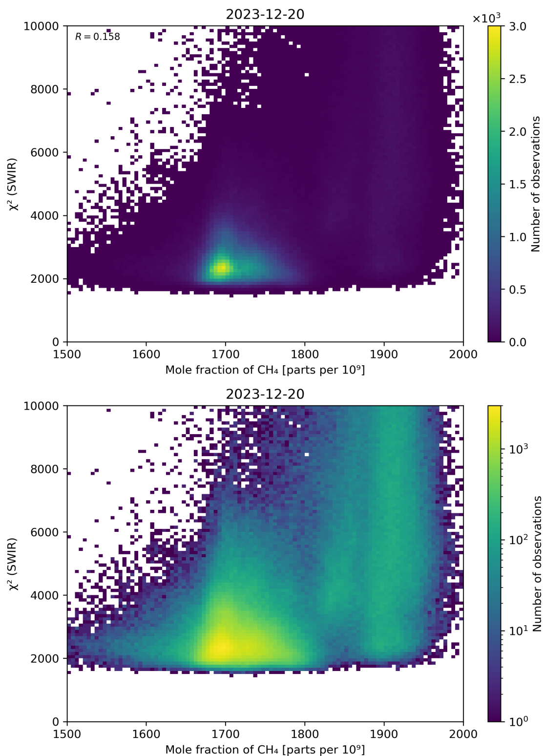
Figure 71: Scatter density plot of “Mole fraction of \text{CH}_4 ” against “ \chi^2 (SWIR)” for 2023-12-20 to 2023-12-21.
