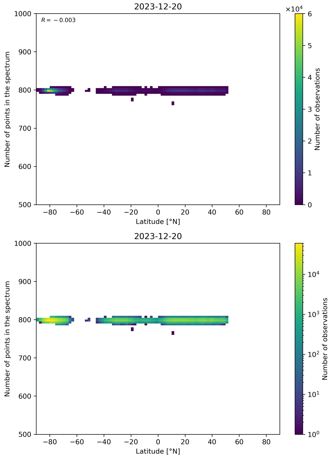
Figure 61: Scatter density plot of “Latitude” against “Number of points in the spectrum” for 2023-12-20 to 2023-12-21.
