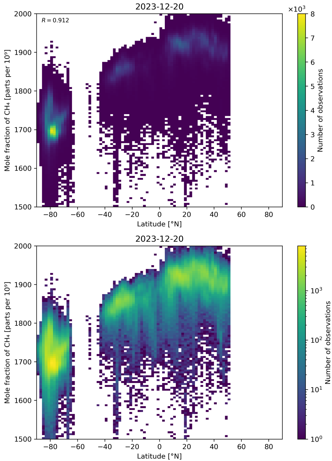
Figure 57: Scatter density plot of “Latitude” against “Mole fraction of CH 4 ” for 2023-12-20 to 2023-12-21.
