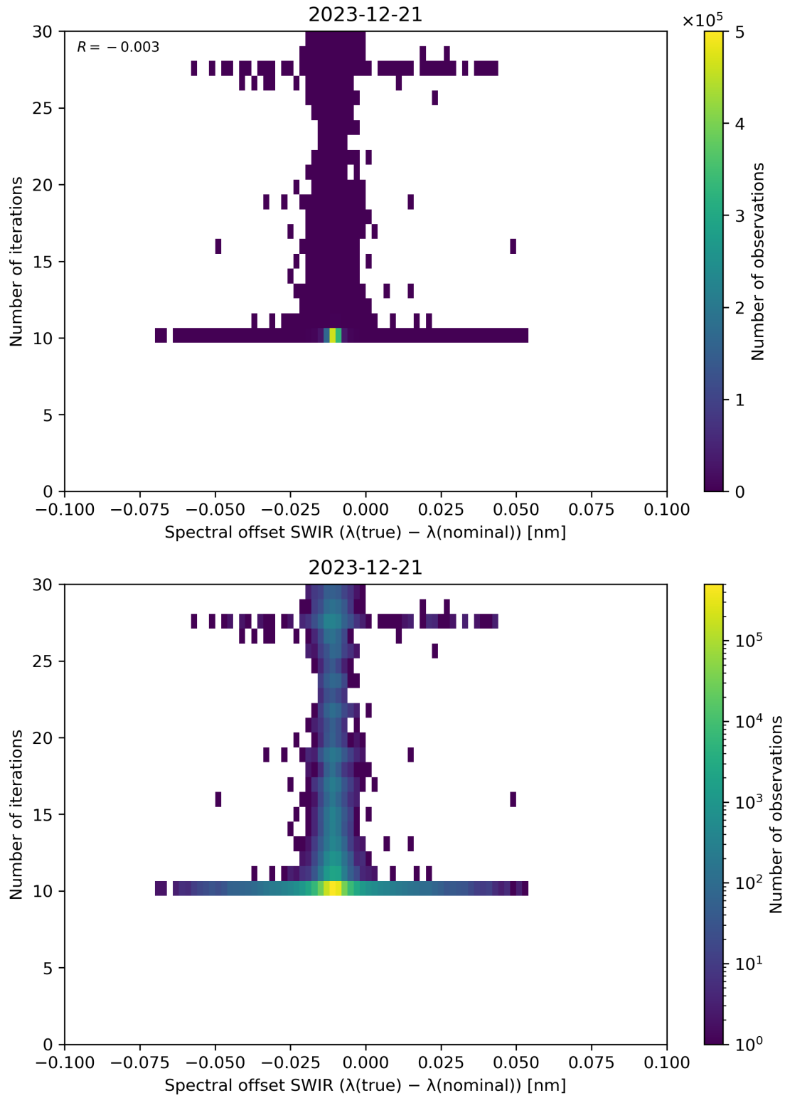
Figure 121: Scatter density plot of “Spectral offset SWIR ( \lambda(\text{true}) - \lambda(\text{nominal}) )” against “Number of iterations” for 2023-12-20 to 2023-12-22.
