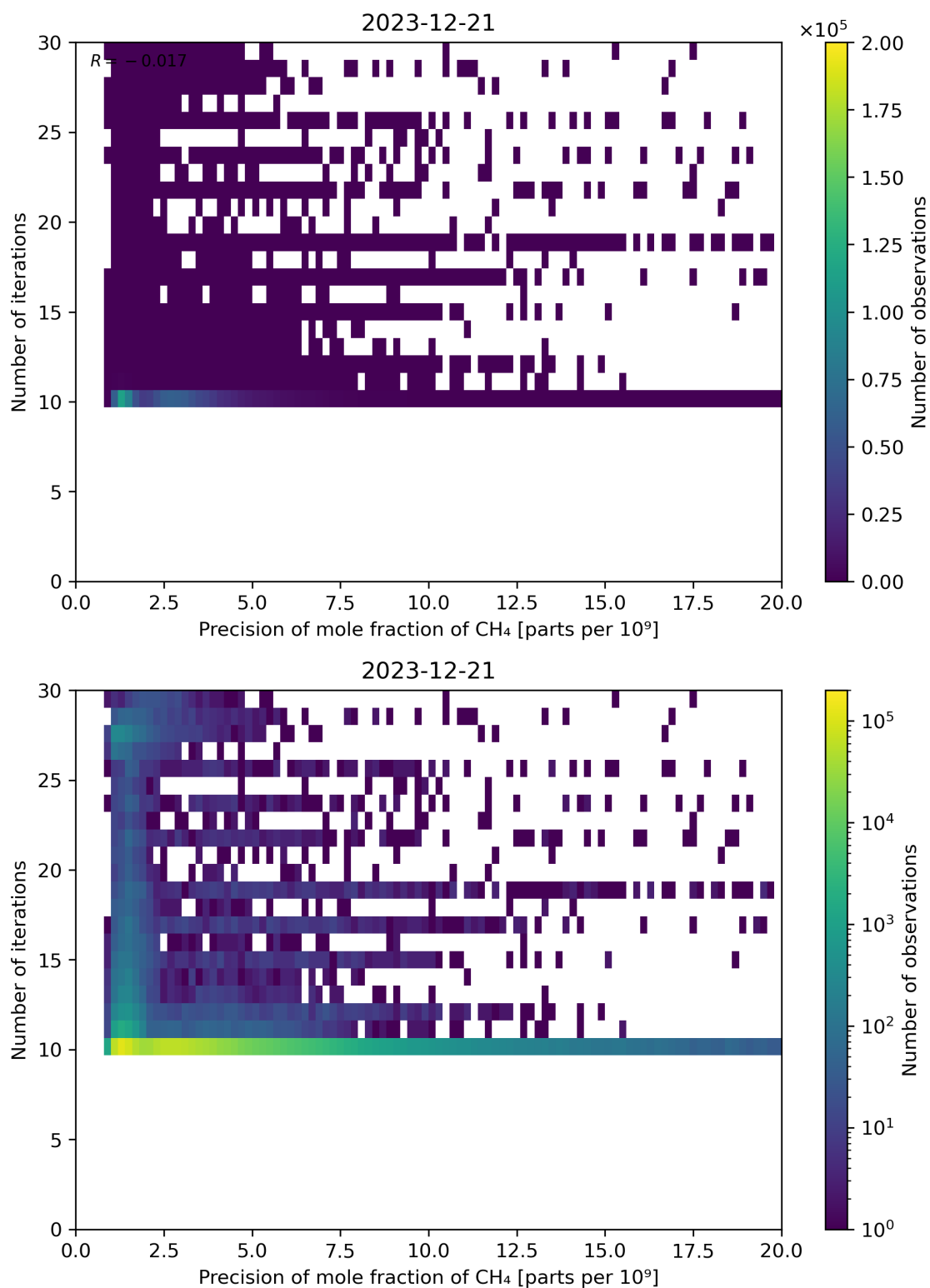
Figure 83: Scatter density plot of “Precision of mole fraction of CH 4 ” against “Number of iterations” for 2023-12-20 to 2023-12-22.
