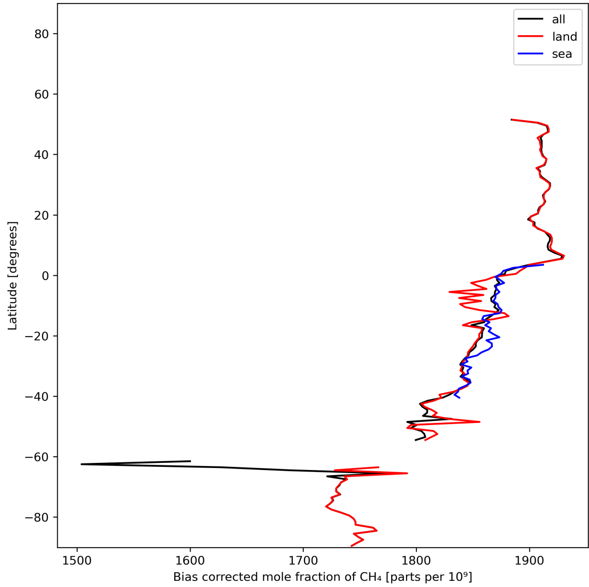
Figure 14: Zonal average of “Bias corrected mole fraction of CH 4 ” for 2023-12-20 to 2023-12-22.
