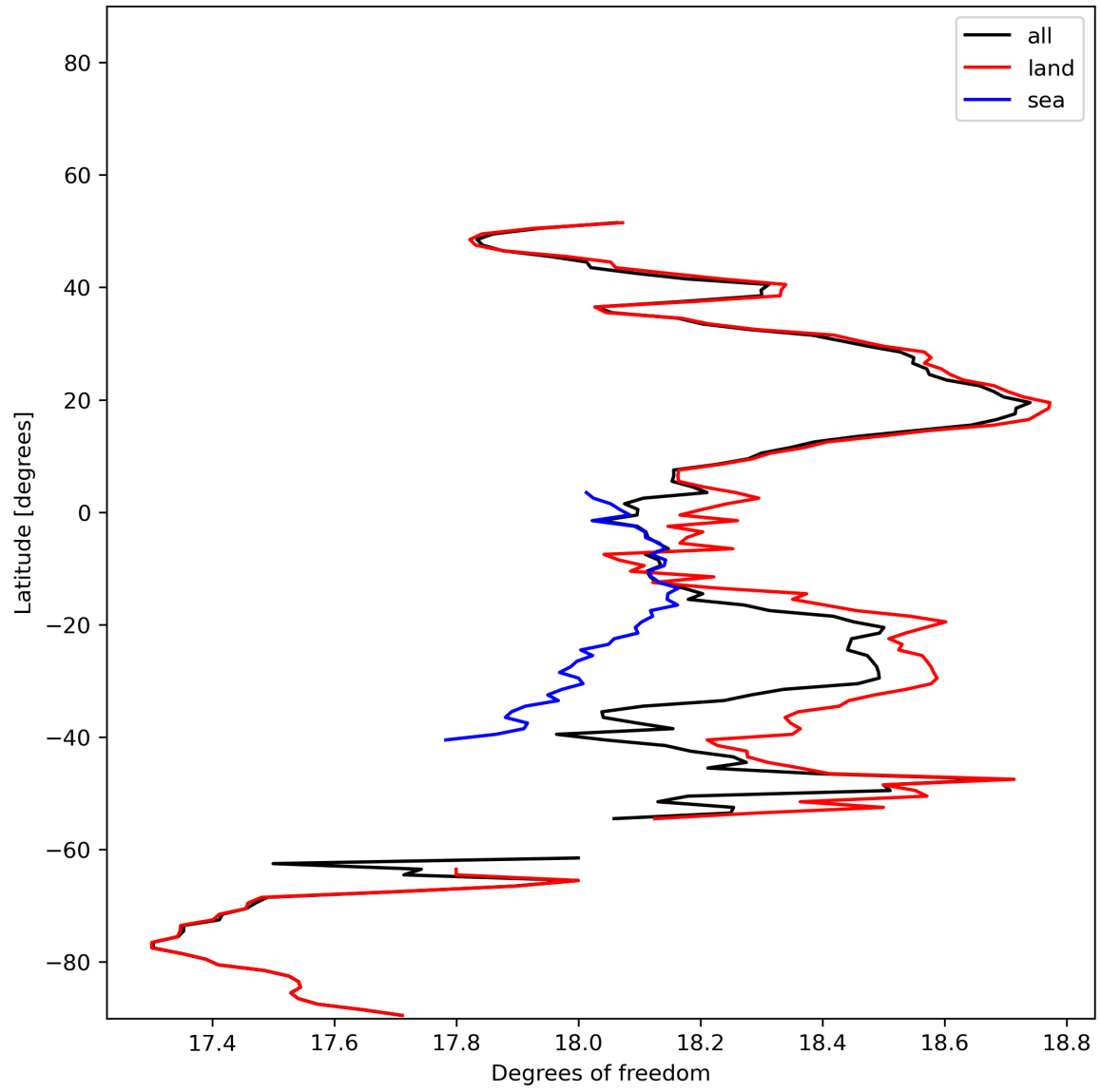
Figure 19: Zonal average of “Degrees of freedom” for 2023-12-20 to 2023-12-22.
