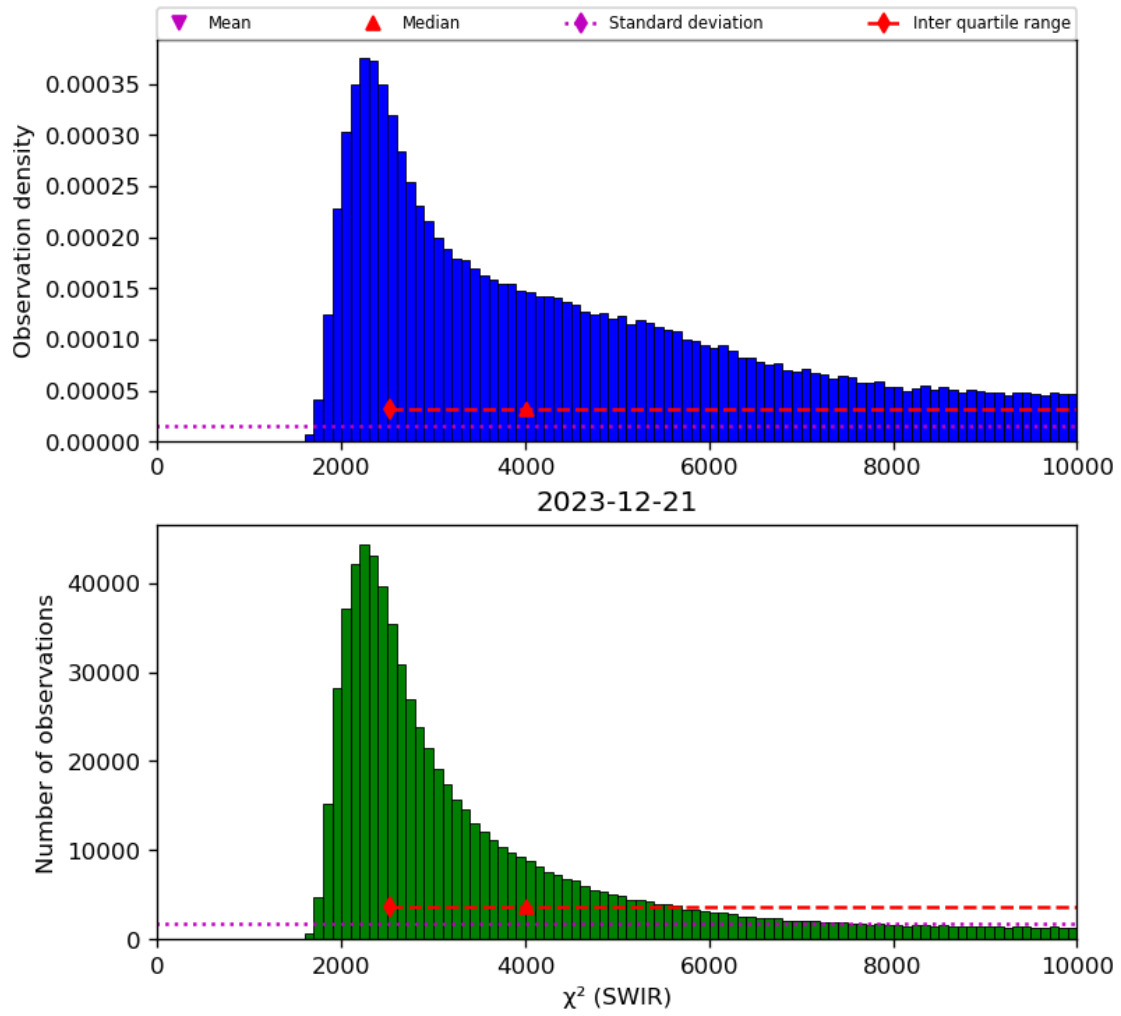
Figure 28: Histogram of “ \chi^2 (SWIR)” for 2023-12-20 to 2023-12-22
