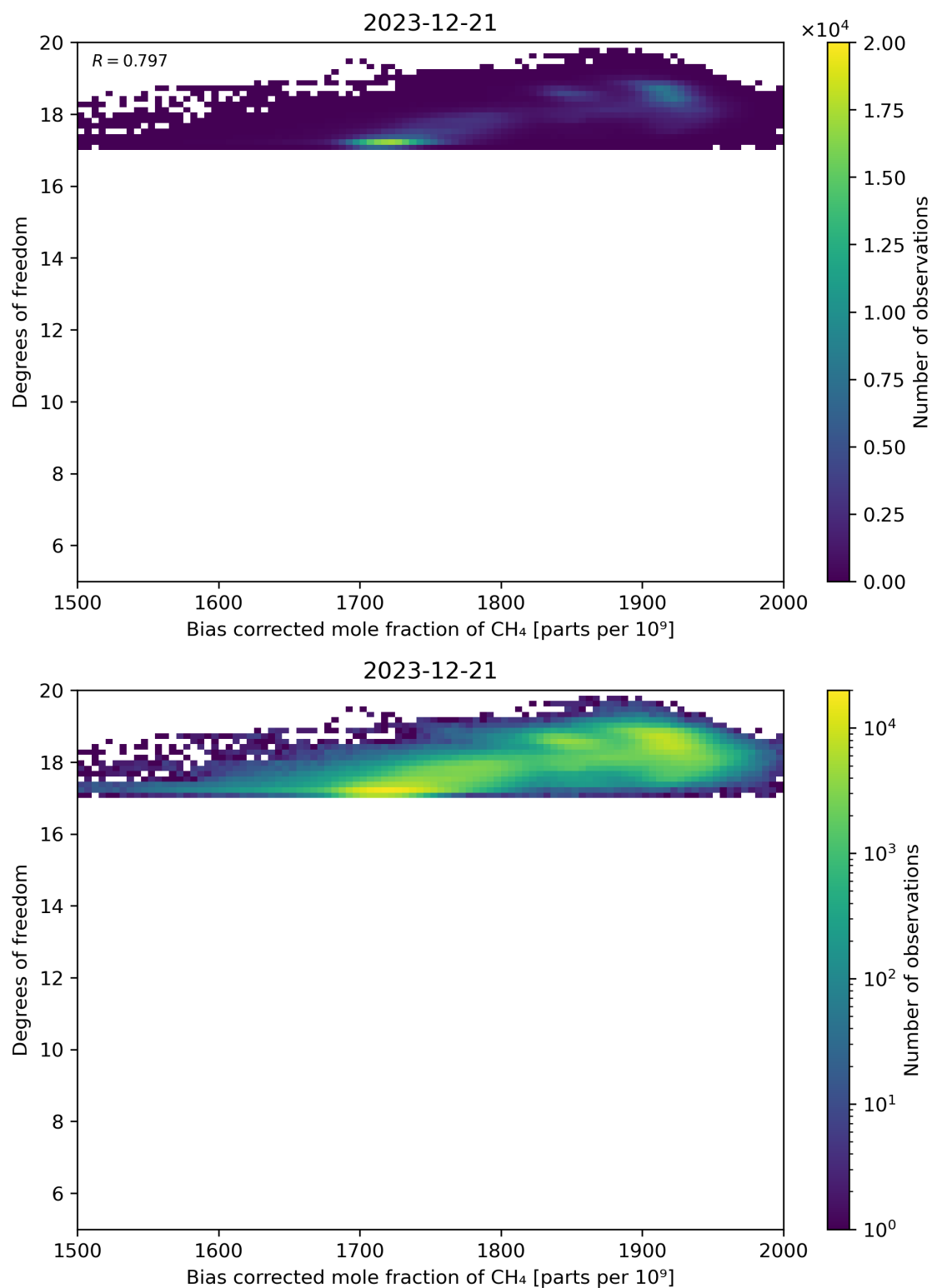
Figure 65: Scatter density plot of “Bias corrected mole fraction of CH 4 ” against “Degrees of freedom” for 2023-12-20 to 2023-12-22.
