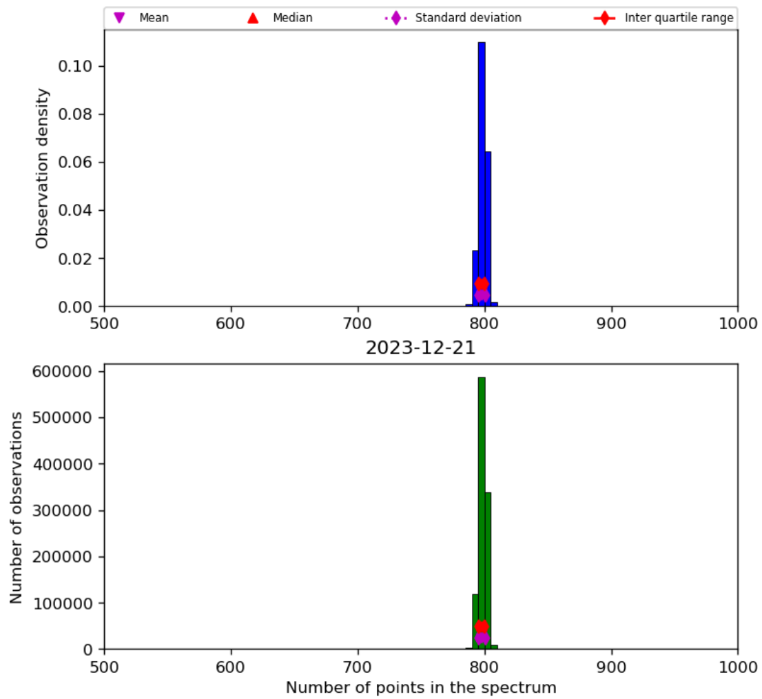
Figure 26: Histogram of “Number of points in the spectrum” for 2023-12-20 to 2023-12-22
