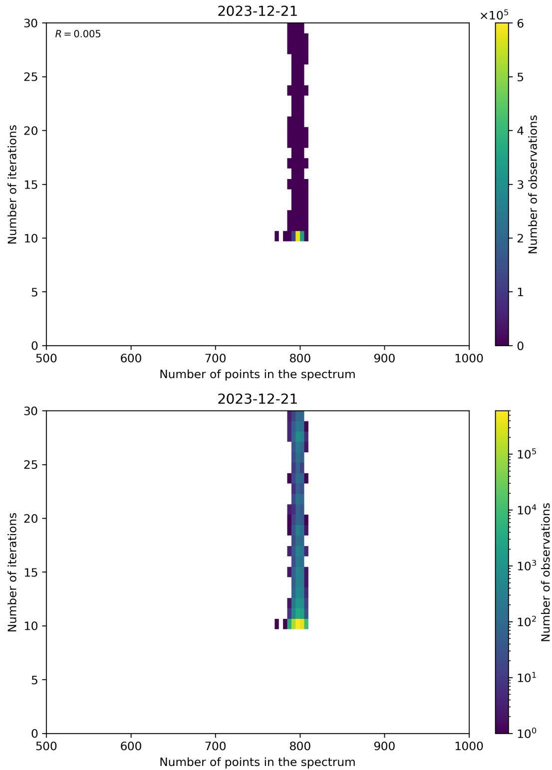
Figure 92: Scatter density plot of “Number of points in the spectrum” against “Number of iterations” for 2023-12-20 to 2023-12-22.
