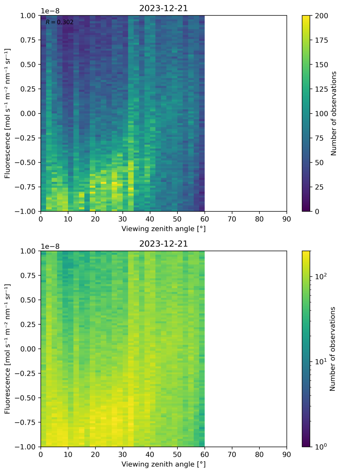
Figure 108: Scatter density plot of “Viewing zenith angle” against “Fluorescence” for 2023-12-20 to 2023-12-22.
