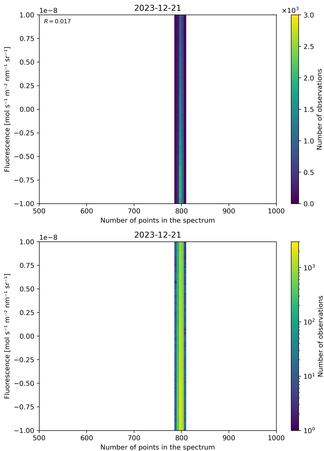
Figure 91: Scatter density plot of “Number of points in the spectrum” against “Fluorescence” for 2023-12-20 to 2023-12-22.
