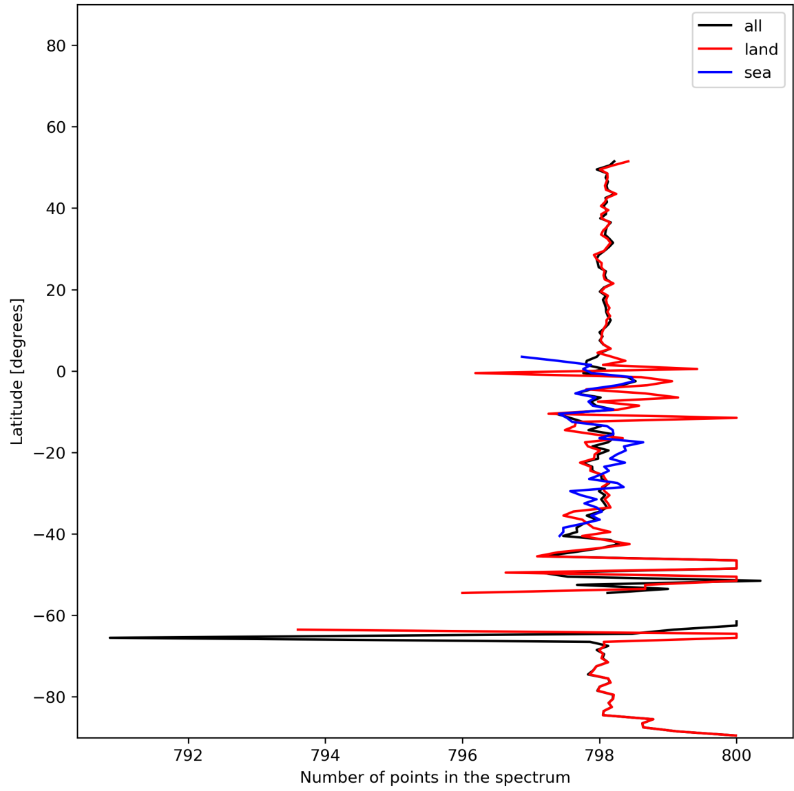
Figure 15: Zonal average of “Number of points in the spectrum” for 2023-12-20 to 2023-12-22.
