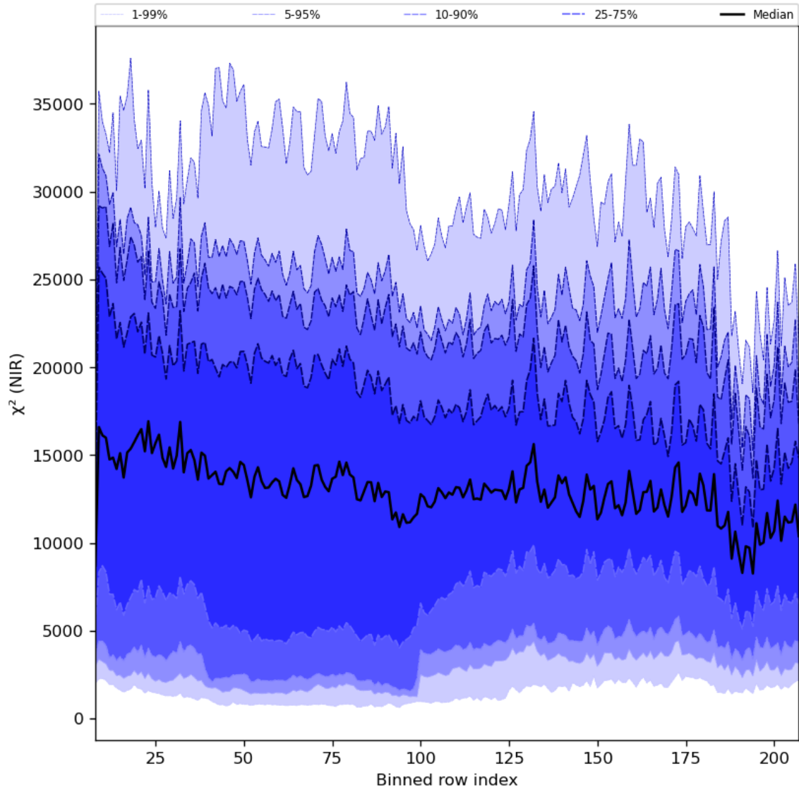
Figure 40: Along track statistics of “ \chi^2 (NIR)” for 2023-12-20 to 2023-12-22
