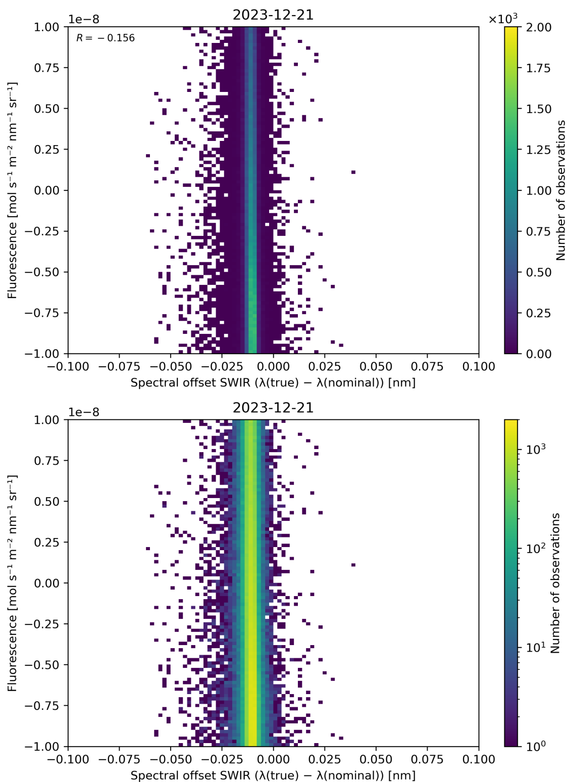
Figure 120: Scatter density plot of “Spectral offset SWIR ( \lambda(\text{true}) - \lambda(\text{nominal}) )” against “Fluorescence” for 2023-12-20 to 2023-12-22.
