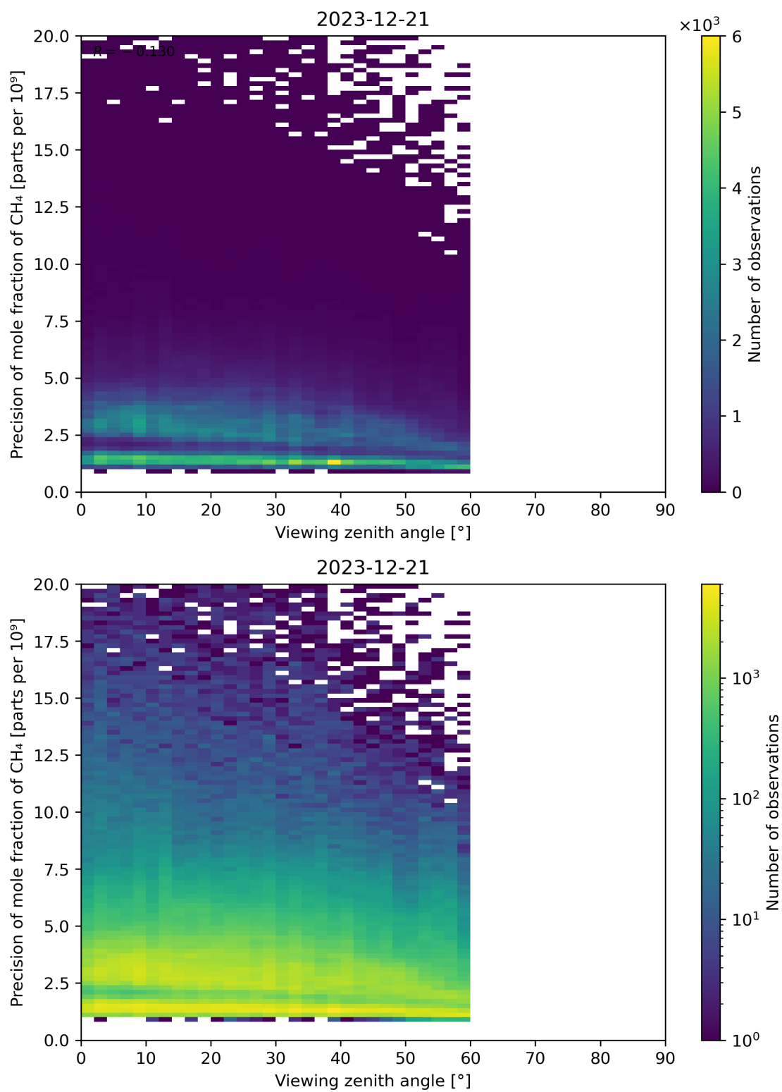
Figure 112: Scatter density plot of “Viewing zenith angle” against “Precision of mole fraction of CH 4 ” for 2023-12-20 to 2023-12-22.
