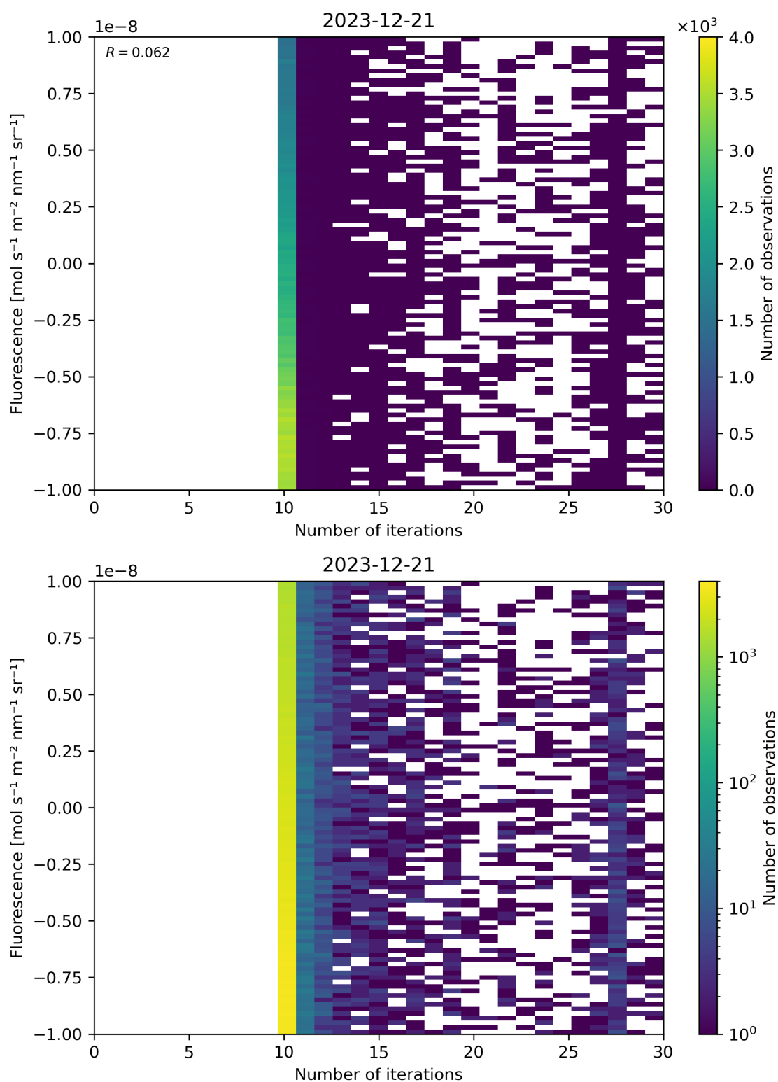
Figure 87: Scatter density plot of “Number of iterations” against “Fluorescence” for 2023-12-20 to 2023-12-22.
