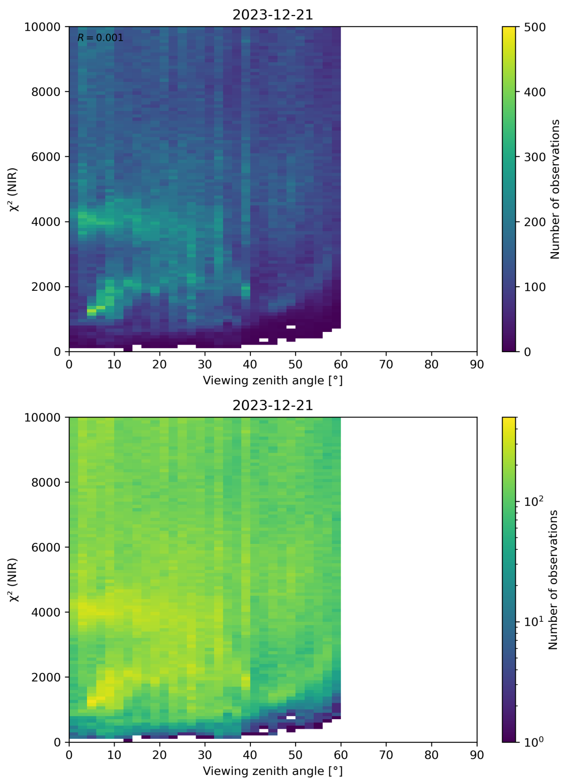
Figure 105: Scatter density plot of “Viewing zenith angle” against “ \chi^2 (NIR)” for 2023-12-20 to 2023-12-22.
