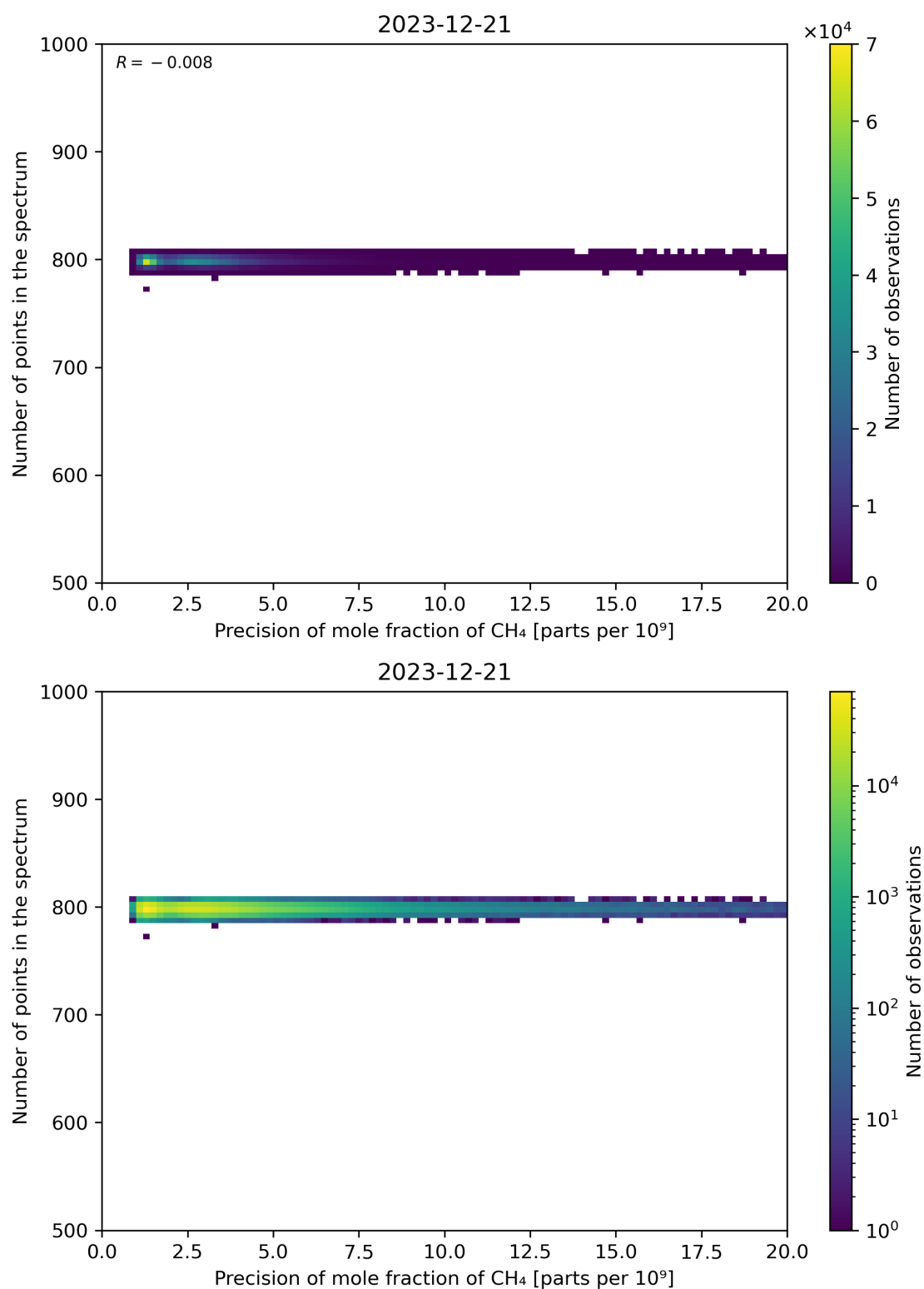
Figure 84: Scatter density plot of “Precision of mole fraction of CH 4 ” against “Number of points in the spectrum” for 2023-12-20 to 2023-12-22.
