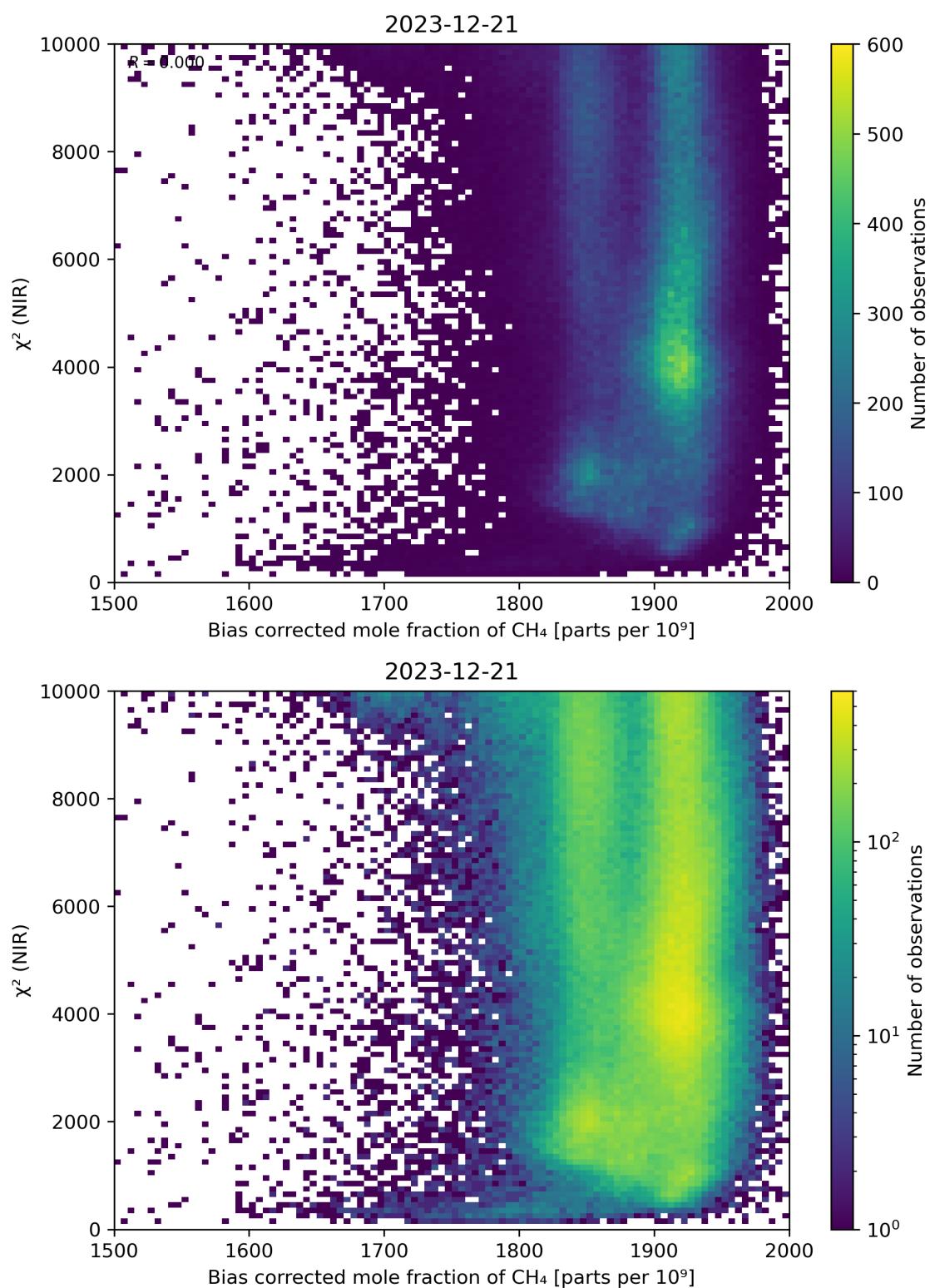
Figure 63: Scatter density plot of “Bias corrected mole fraction of \text{CH}_4 ” against “ \chi^2 (NIR)” for 2023-12-20 to 2023-12-22.
