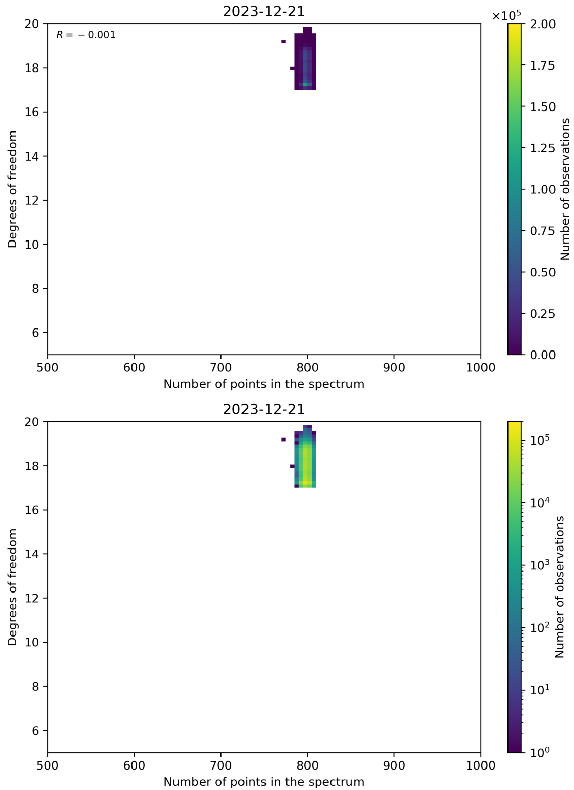
Figure 90: Scatter density plot of “Number of points in the spectrum” against “Degrees of freedom” for 2023-12-20 to 2023-12-22.
