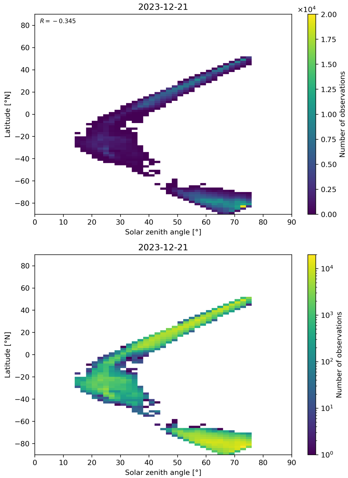
Figure 98: Scatter density plot of “Solar zenith angle” against “Latitude” for 2023-12-20 to 2023-12-22.
