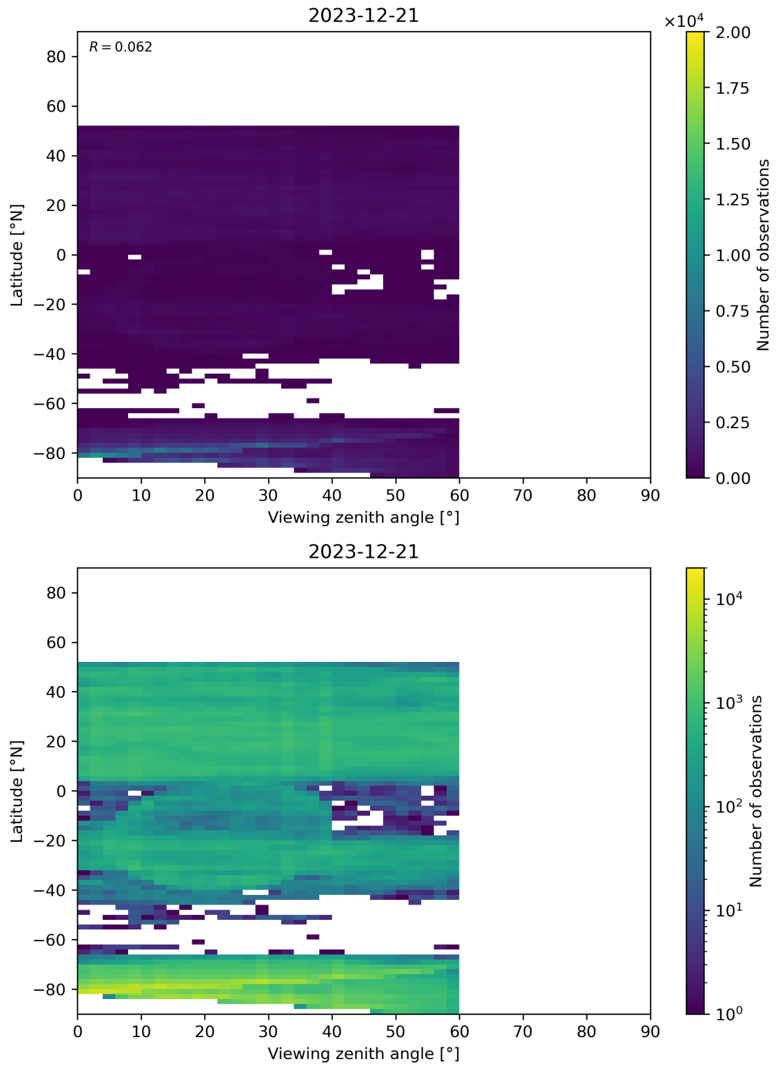
Figure 109: Scatter density plot of “Viewing zenith angle” against “Latitude” for 2023-12-20 to 2023-12-22.
