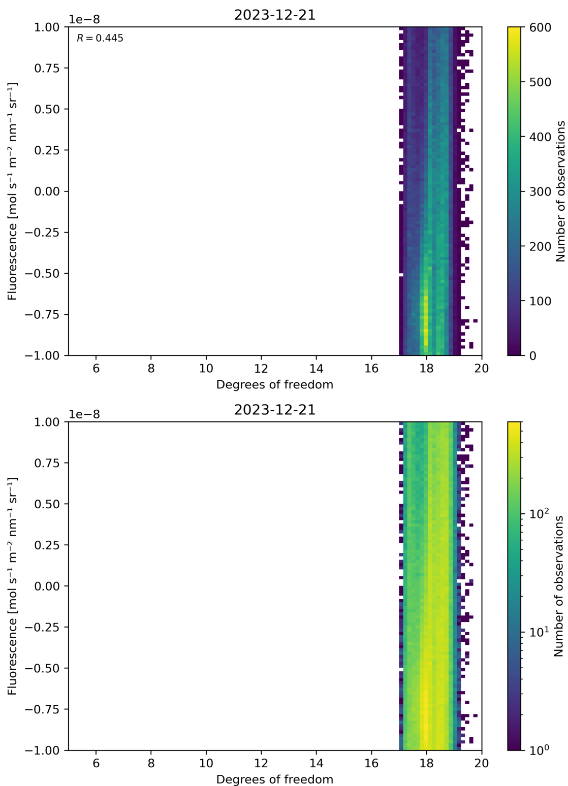
Figure 51: Scatter density plot of “Degrees of freedom” against “Fluorescence” for 2023-12-20 to 2023-12-22.
