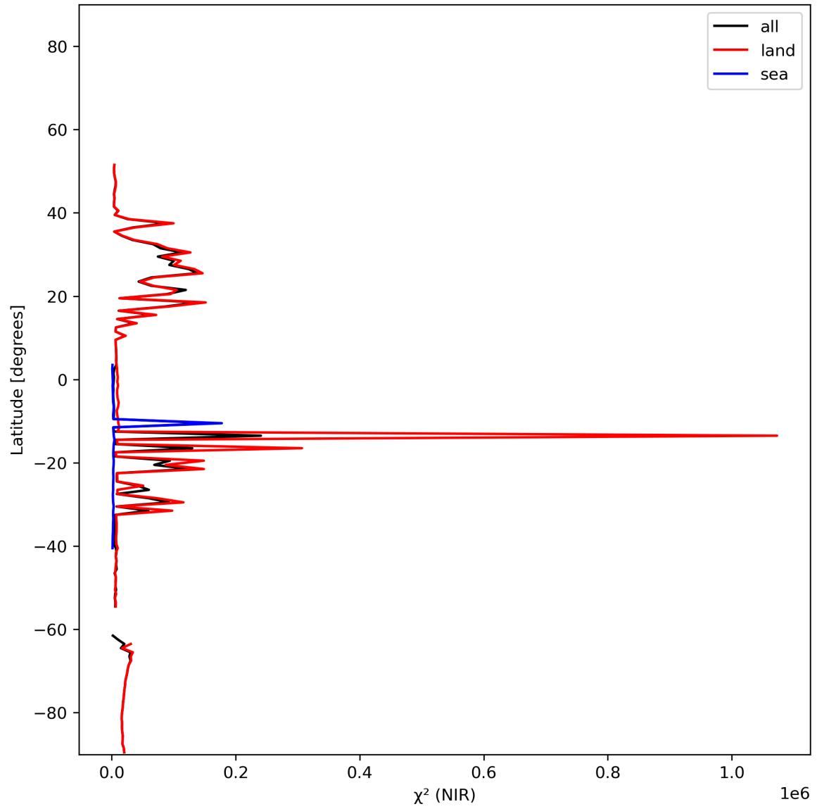
Figure 18: Zonal average of “ \chi^2 (NIR)” for 2023-12-20 to 2023-12-22.
