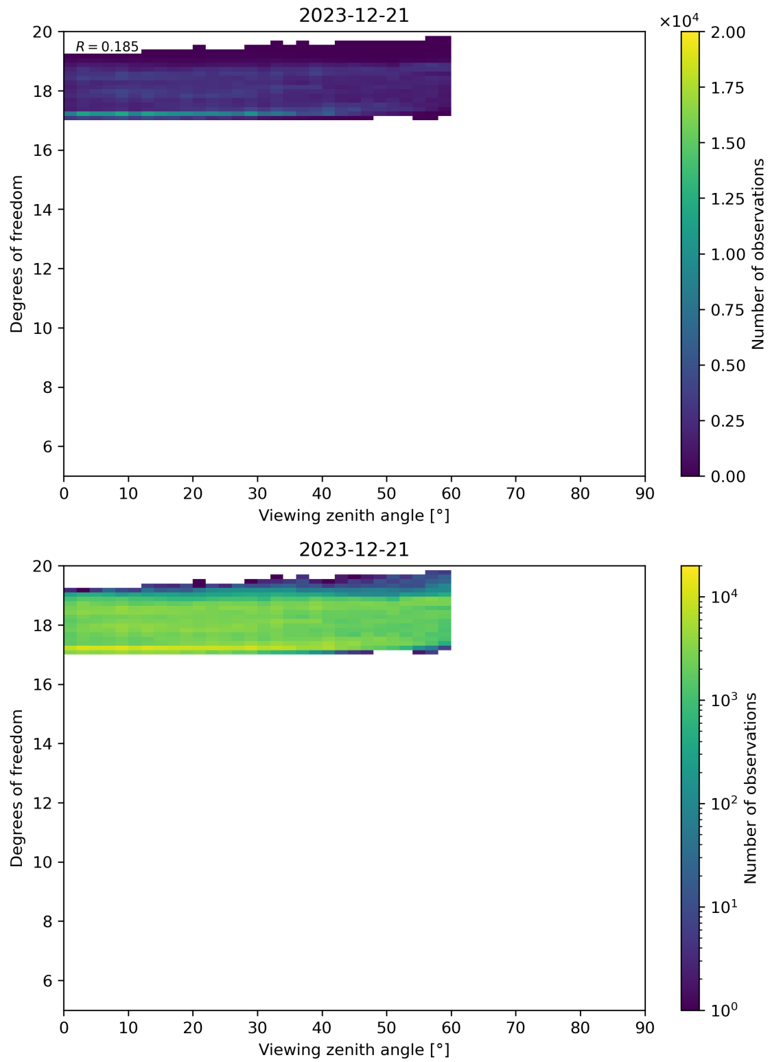
Figure 107: Scatter density plot of “Viewing zenith angle” against “Degrees of freedom” for 2023-12-20 to 2023-12-22.
