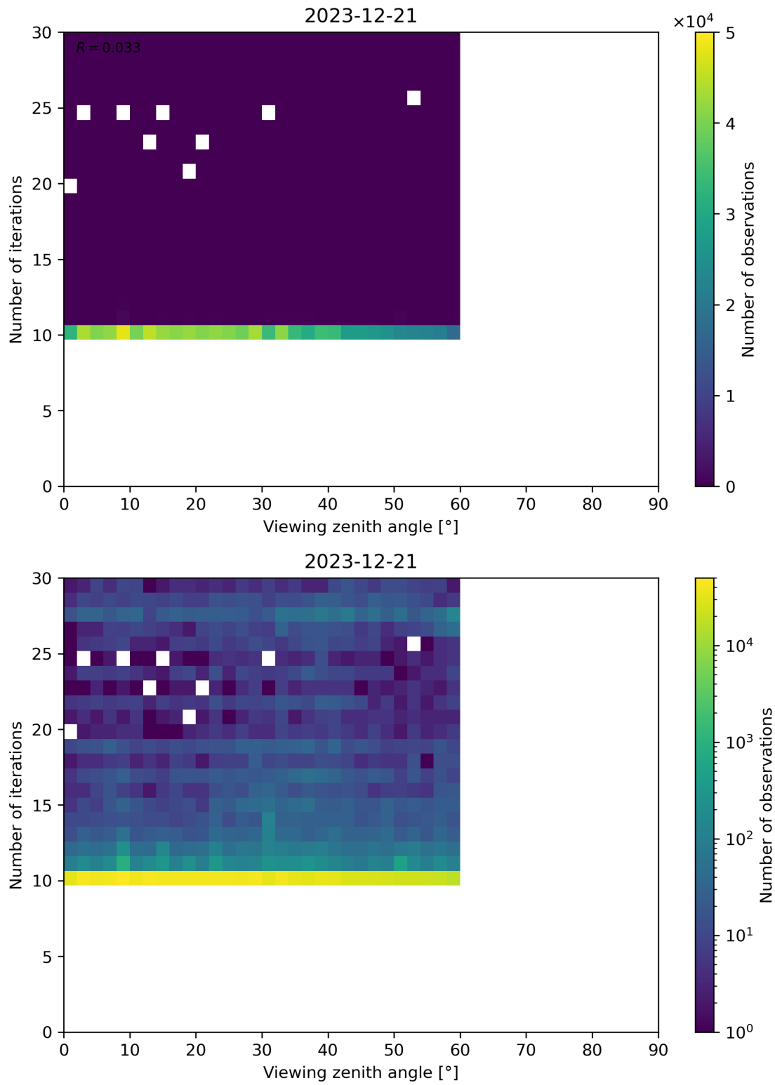
Figure 113: Scatter density plot of “Viewing zenith angle” against “Number of iterations” for 2023-12-20 to 2023-12-22.
