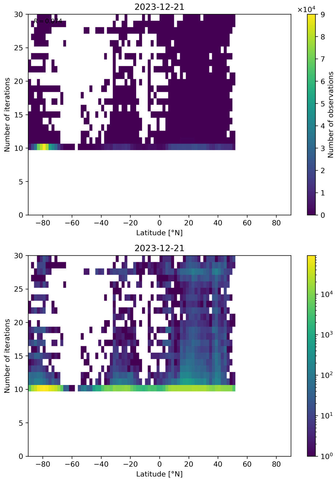
Figure 60: Scatter density plot of “Latitude” against “Number of iterations” for 2023-12-20 to 2023-12-22.
