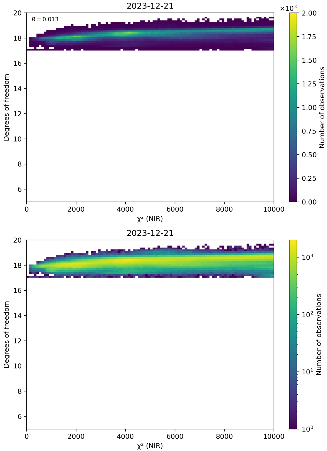
Figure 44: Scatter density plot of “ \chi^2 (NIR)” against “Degrees of freedom” for 2023-12-20 to 2023-12-22.
