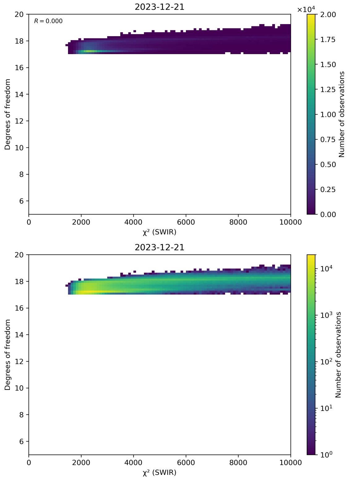
Figure 48: Scatter density plot of “ \chi^2 (SWIR)” against “Degrees of freedom” for 2023-12-20 to 2023-12-22.
