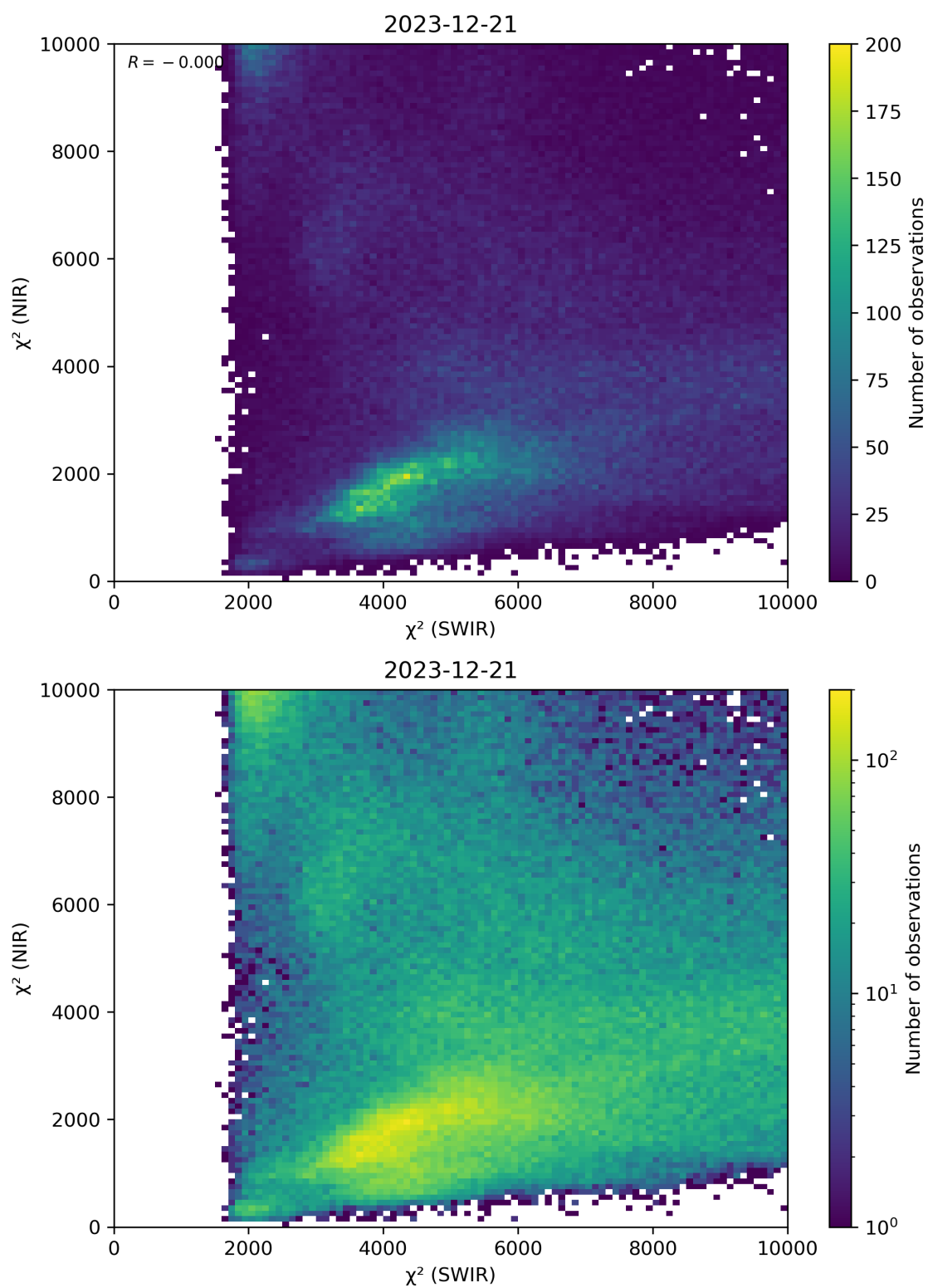
Figure 47: Scatter density plot of “ \chi^2 (SWIR)” against “ \chi^2 (NIR)” for 2023-12-20 to 2023-12-22.
