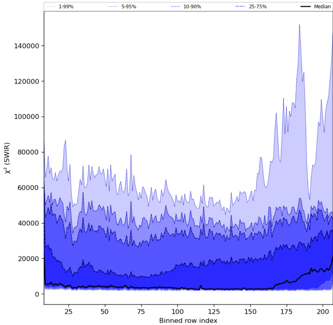
Figure 39: Along track statistics of “ \chi^2 (SWIR)” for 2023-12-20 to 2023-12-22
