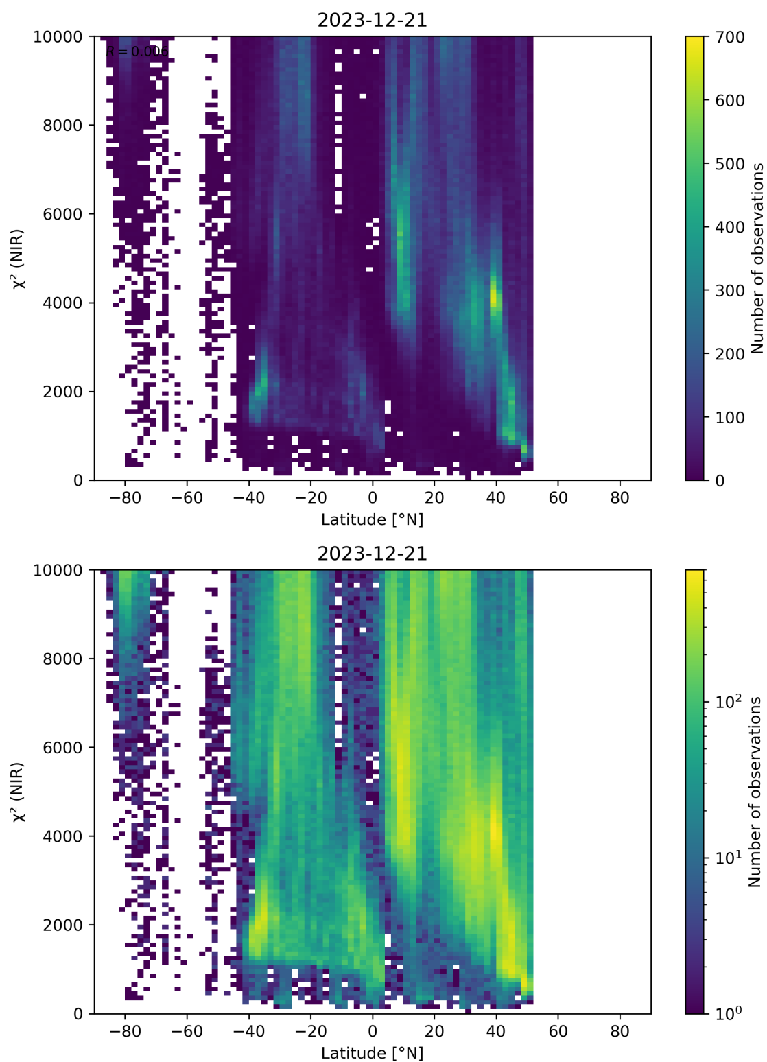
Figure 53: Scatter density plot of “Latitude” against “ \chi^2 (NIR)” for 2023-12-20 to 2023-12-22.
