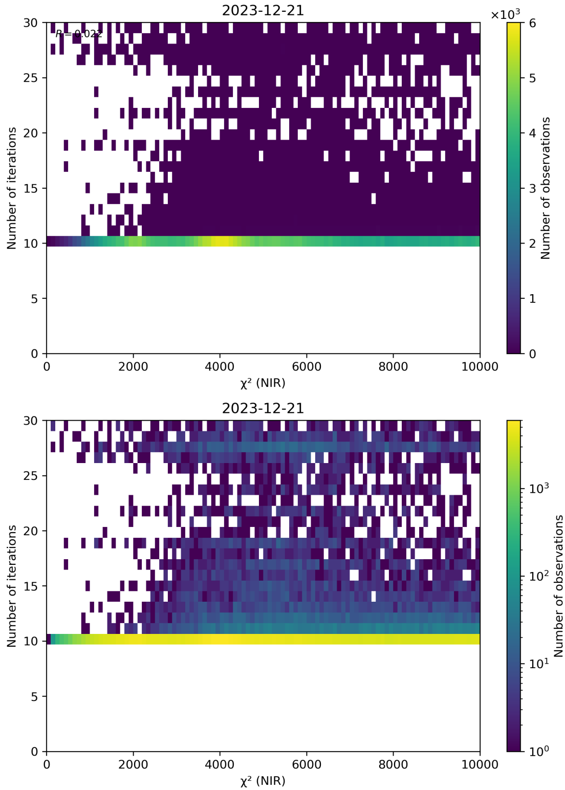
Figure 46: Scatter density plot of “ \chi^2 (NIR)” against “Number of iterations” for 2023-12-20 to 2023-12-22.
