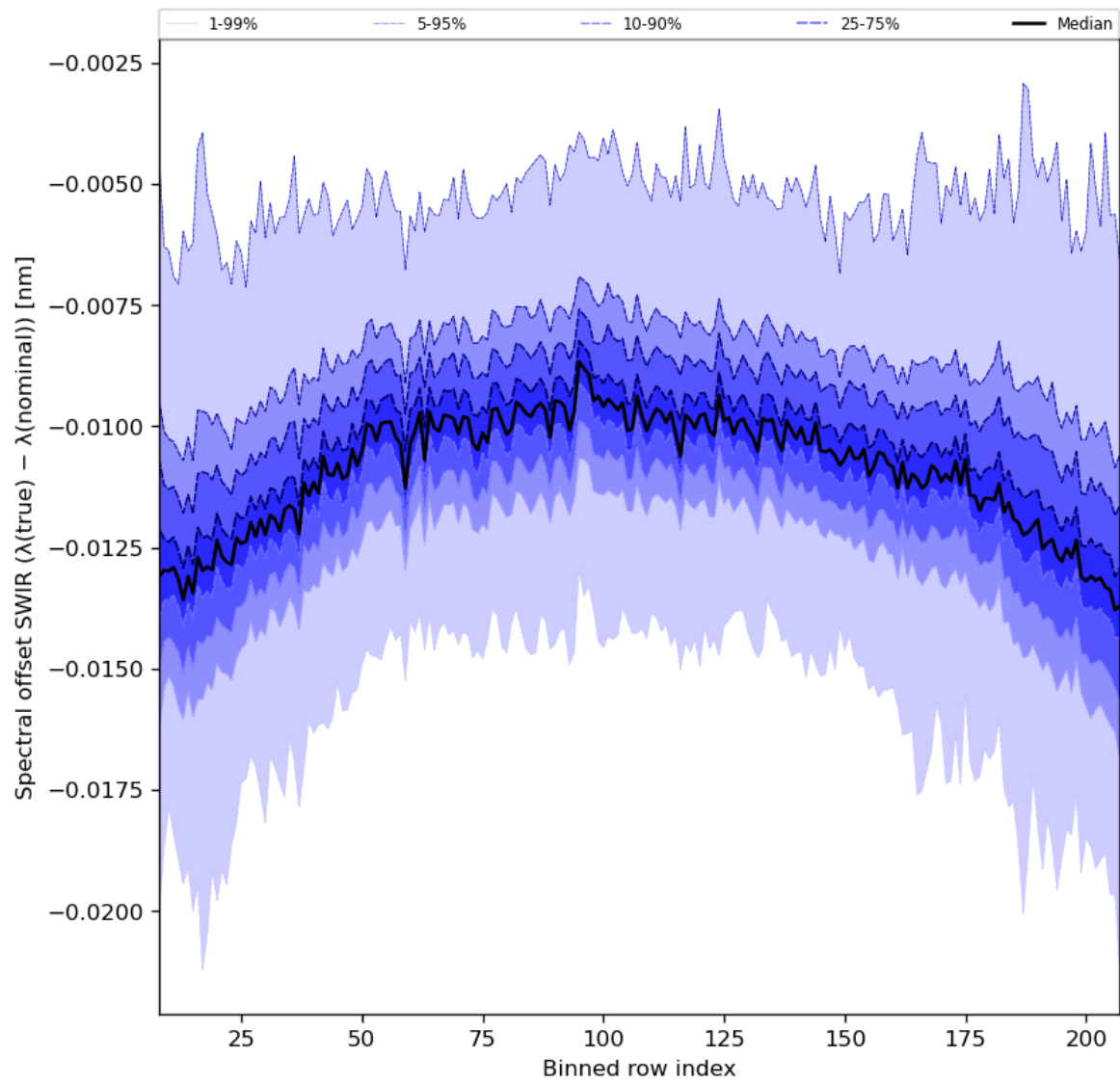
Figure 38: Along track statistics of “Spectral offset SWIR ( \lambda(\text{true}) - \lambda(\text{nominal}) )” for 2023-12-20 to 2023-12-22
