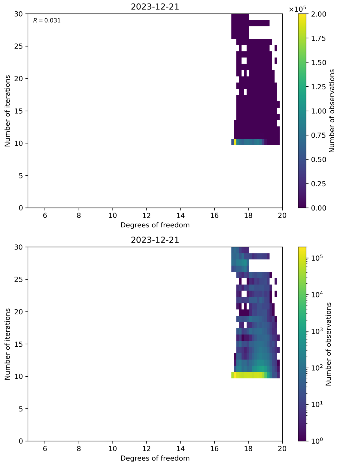
Figure 52: Scatter density plot of “Degrees of freedom” against “Number of iterations” for 2023-12-20 to 2023-12-22.
