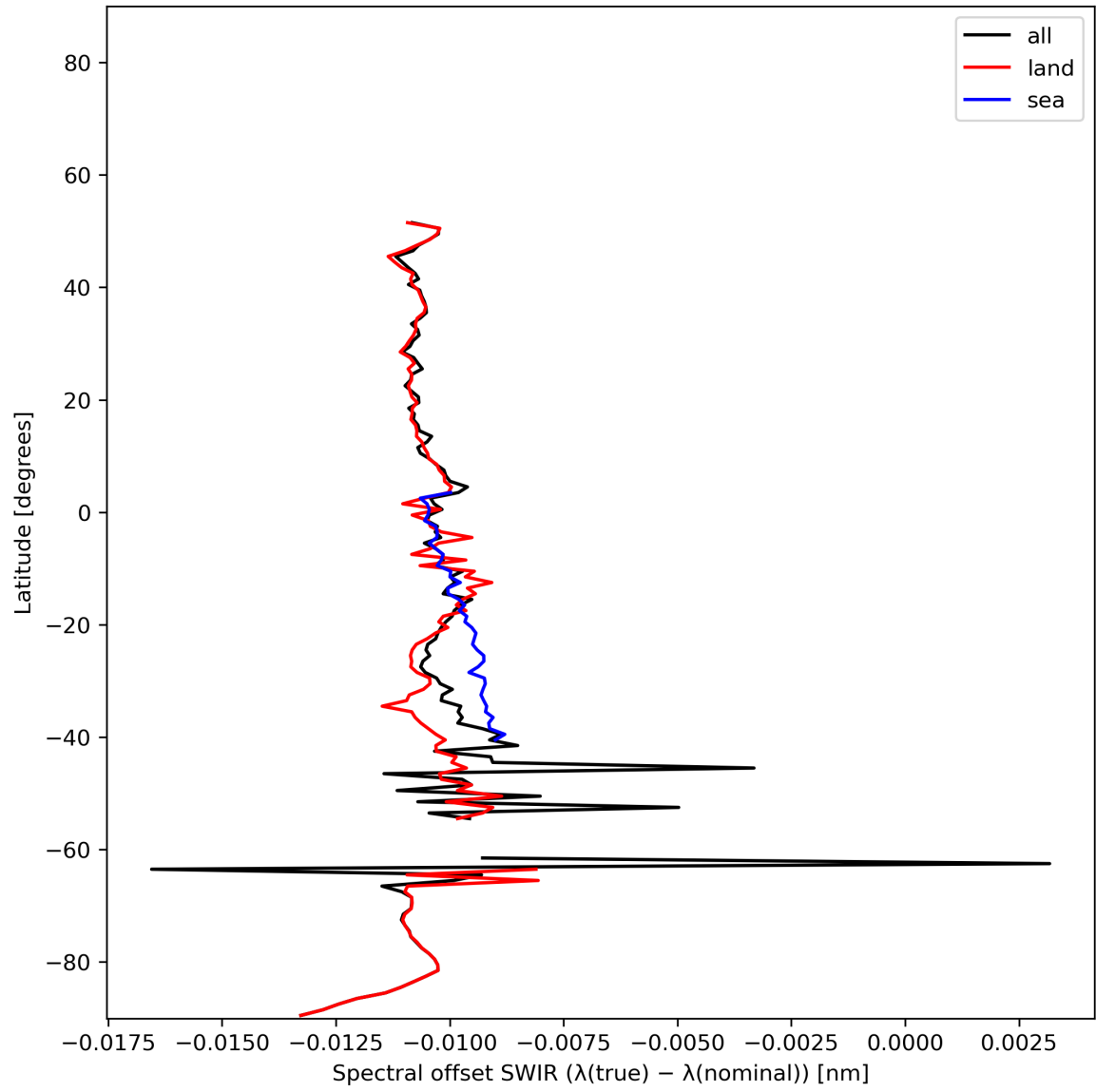
Figure 16: Zonal average of “Spectral offset SWIR ( \lambda(\text{true}) - \lambda(\text{nominal}) )” for 2023-12-20 to 2023-12-22.
