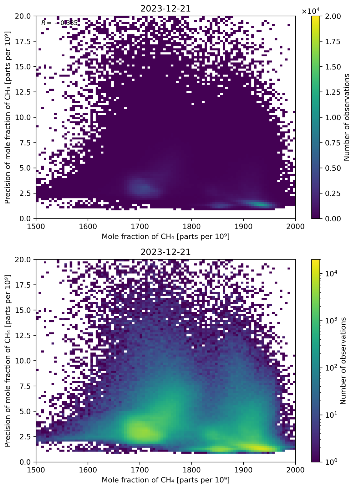
Figure 75: Scatter density plot of “Mole fraction of CH 4 ” against “Precision of mole fraction of CH 4 ” for 2023-12-20 to 2023-12-22.
