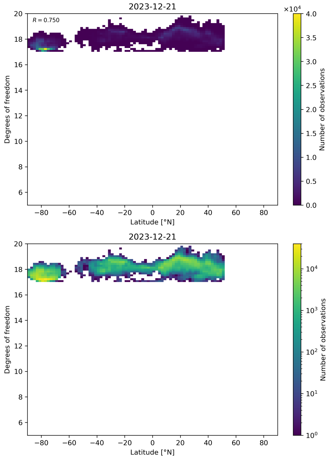
Figure 55: Scatter density plot of “Latitude” against “Degrees of freedom” for 2023-12-20 to 2023-12-22.
