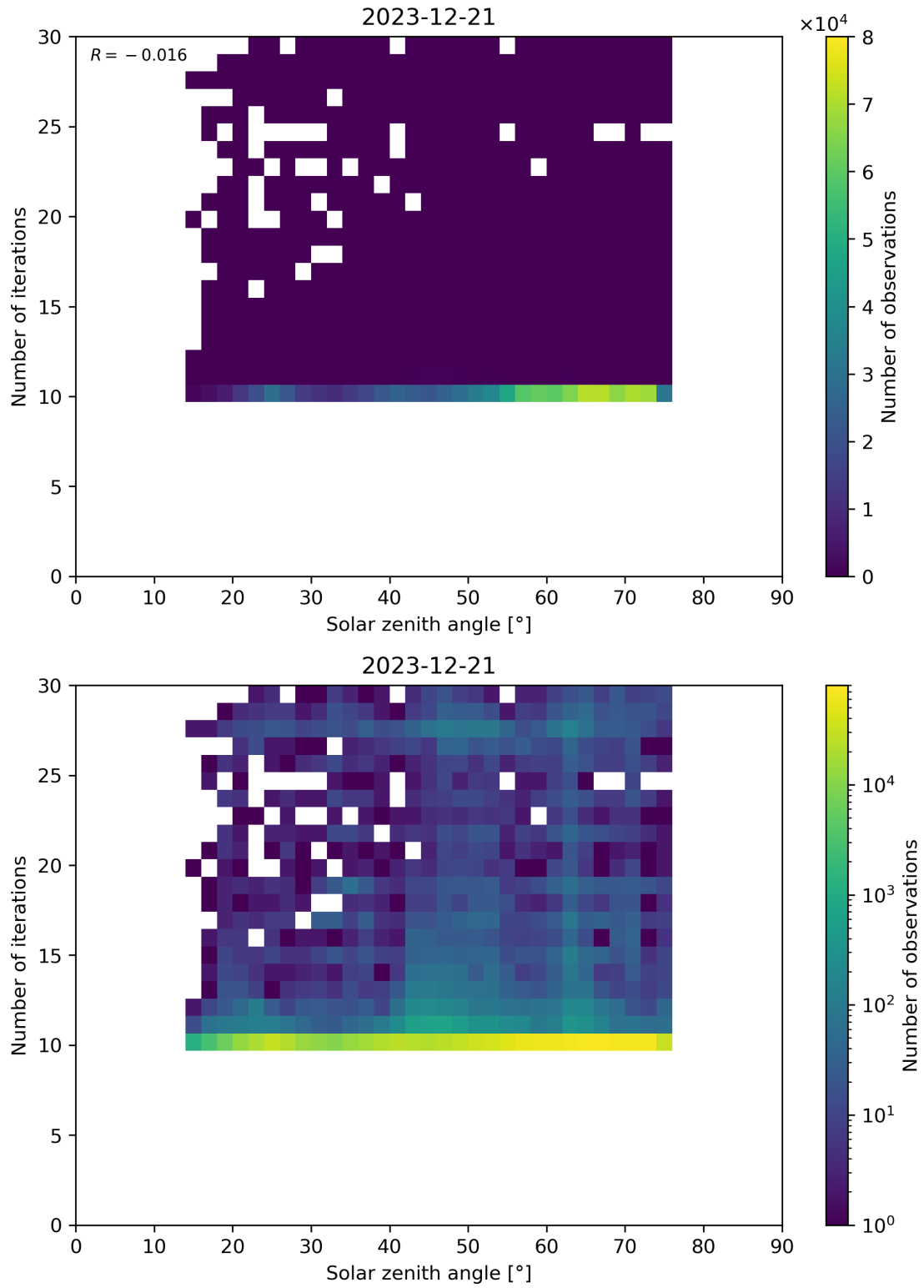
Figure 102: Scatter density plot of “Solar zenith angle” against “Number of iterations” for 2023-12-20 to 2023-12-22.
