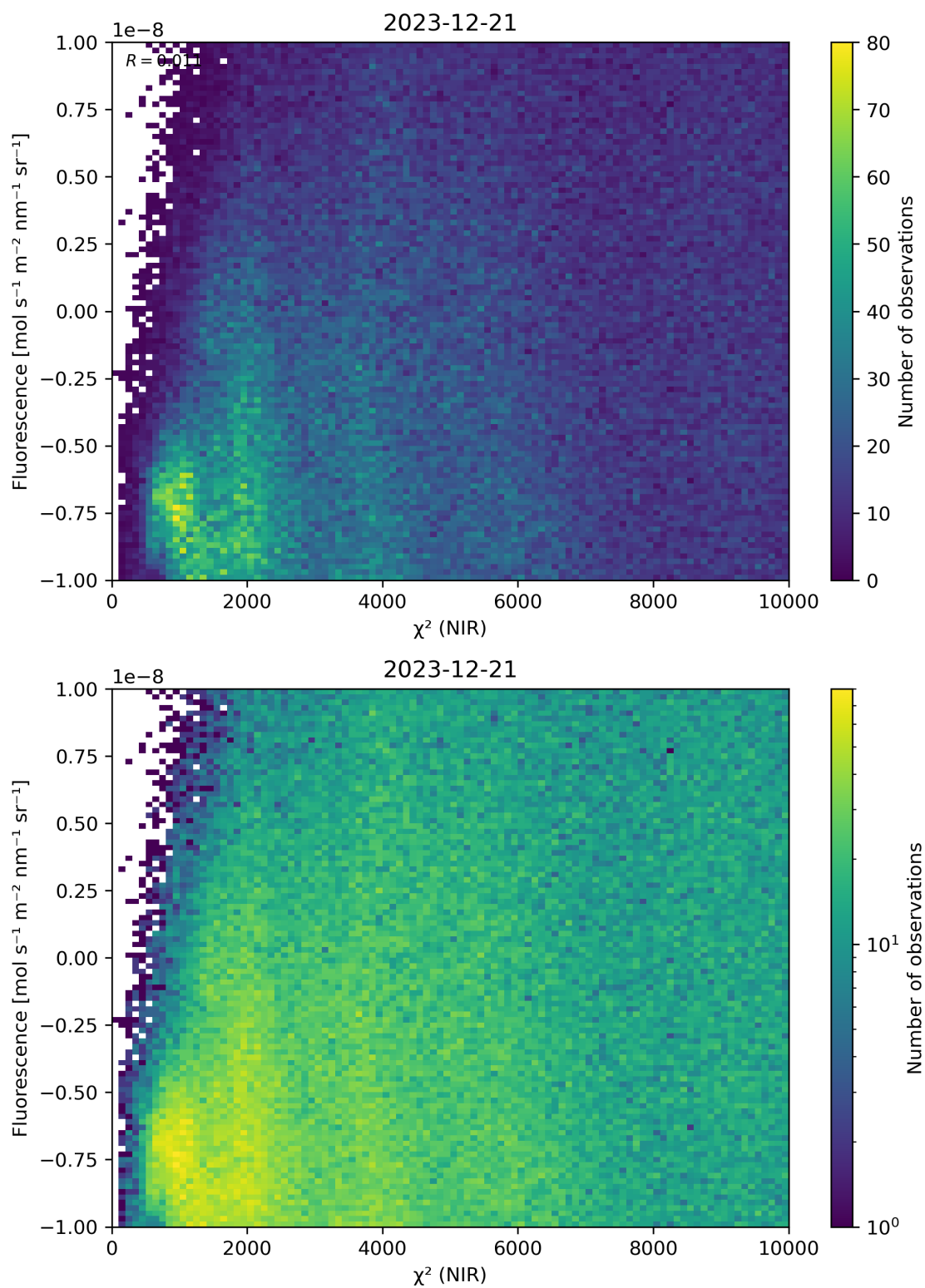
Figure 45: Scatter density plot of “ \chi^2 (NIR)” against “Fluorescence” for 2023-12-20 to 2023-12-22.
