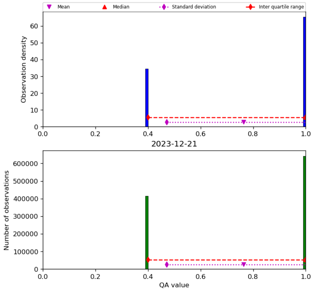
Figure 22: Histogram of “QA value” for 2023-12-20 to 2023-12-22
