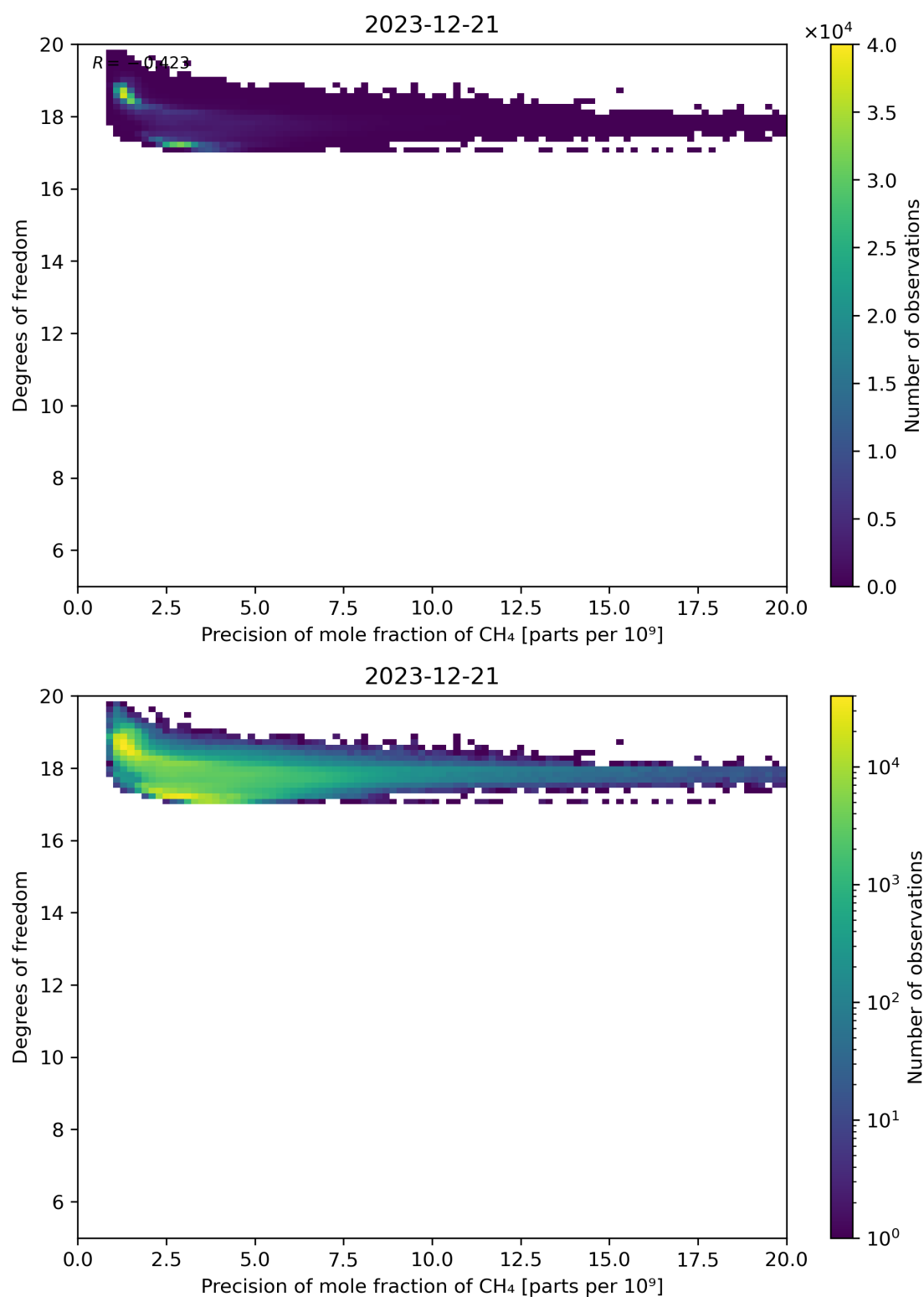
Figure 80: Scatter density plot of “Precision of mole fraction of CH 4 ” against “Degrees of freedom” for 2023-12-20 to 2023-12-22.
