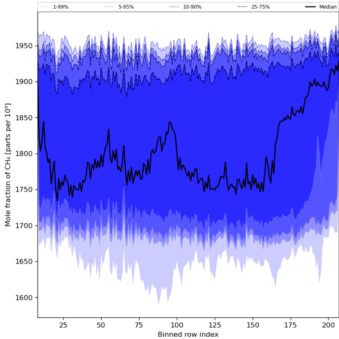
Figure 34: Along track statistics of “Mole fraction of CH 4 ” for 2023-12-20 to 2023-12-22
