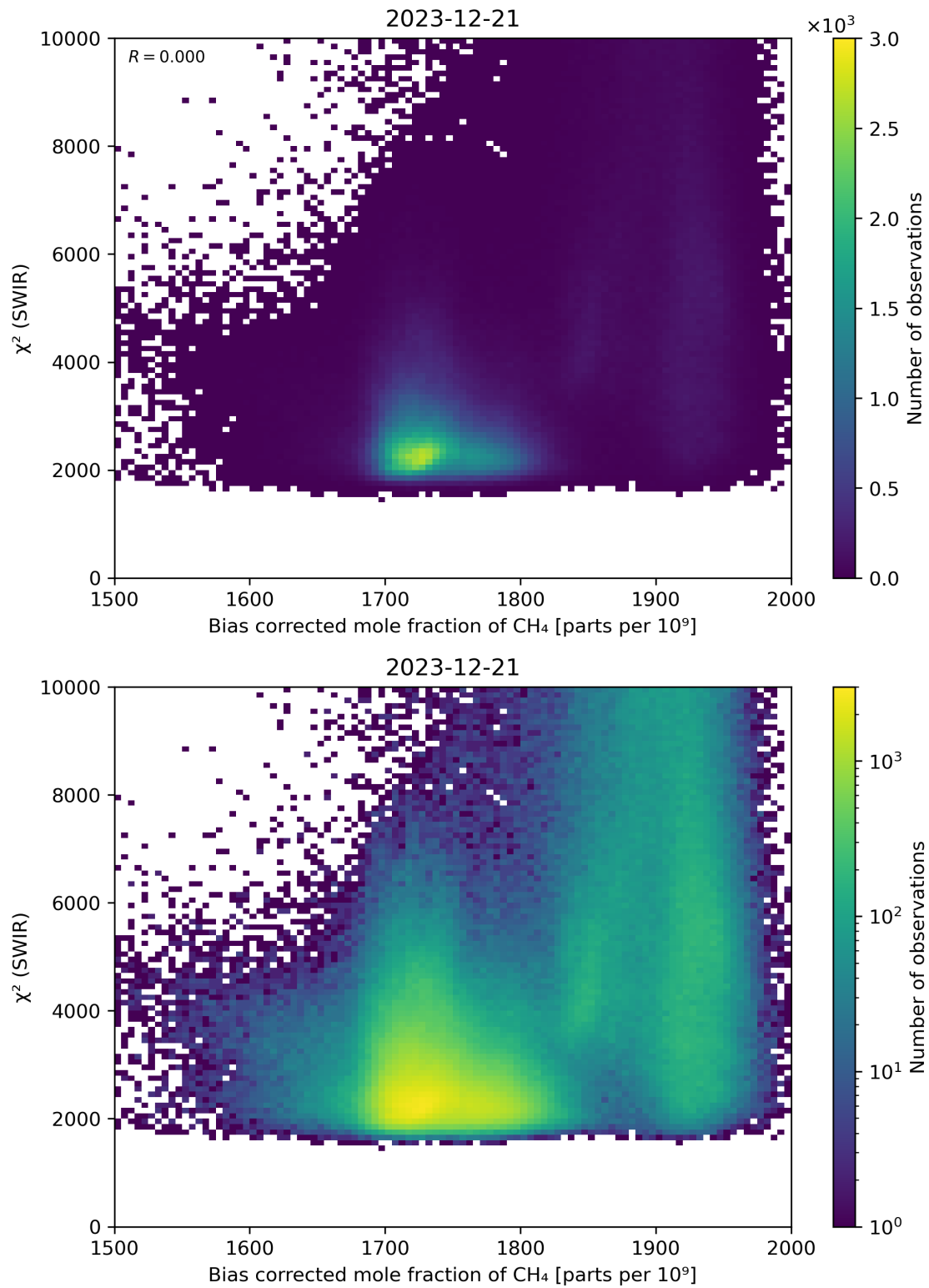
Figure 64: Scatter density plot of “Bias corrected mole fraction of \text{CH}_4 ” against “ \chi^2 (SWIR)” for 2023-12-20 to 2023-12-22.
