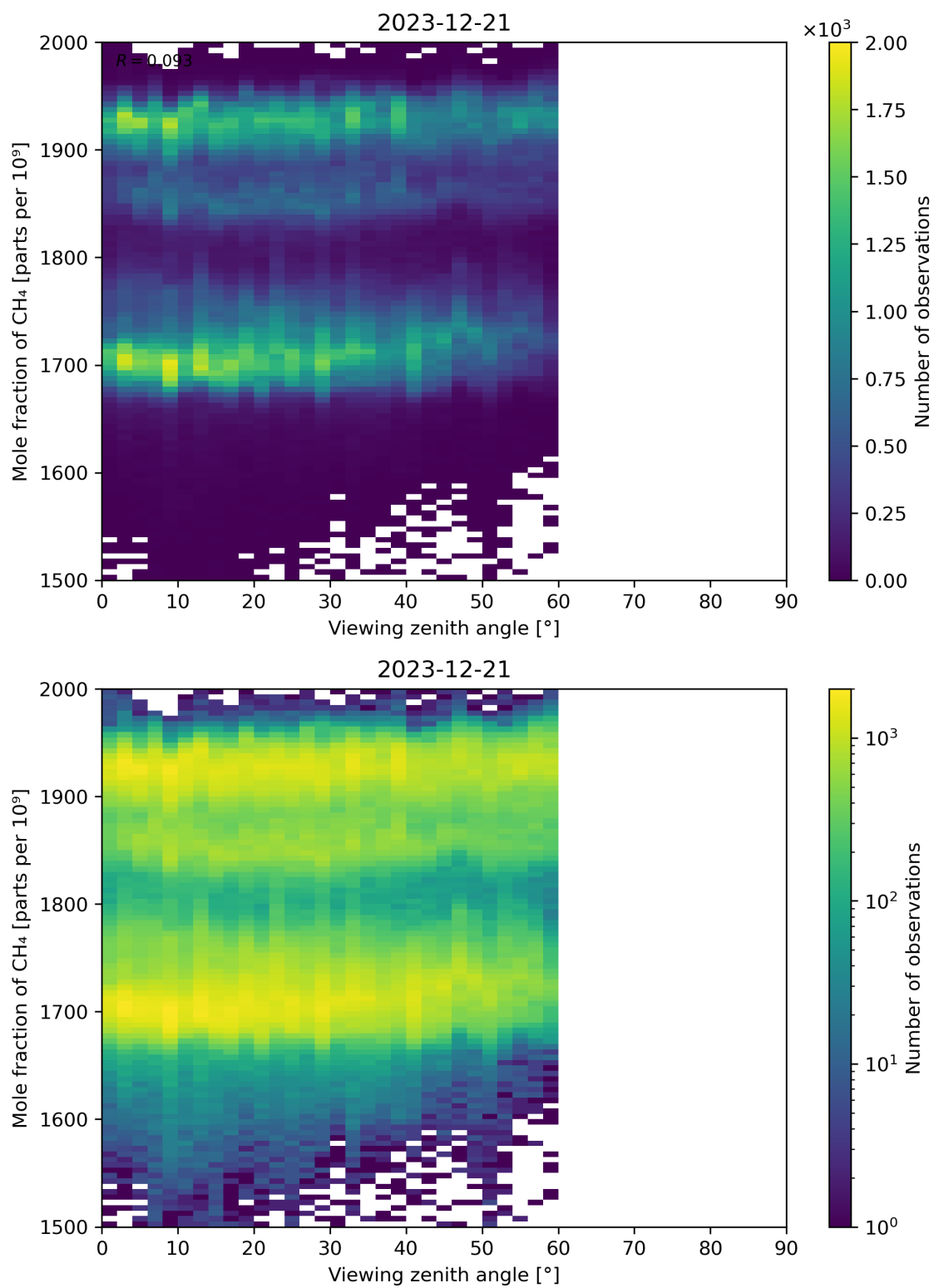
Figure 110: Scatter density plot of “Viewing zenith angle” against “Mole fraction of CH 4 ” for 2023-12-20 to 2023-12-22.
