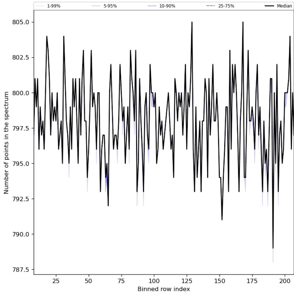
Figure 37: Along track statistics of “Number of points in the spectrum” for 2023-12-20 to 2023-12-22
