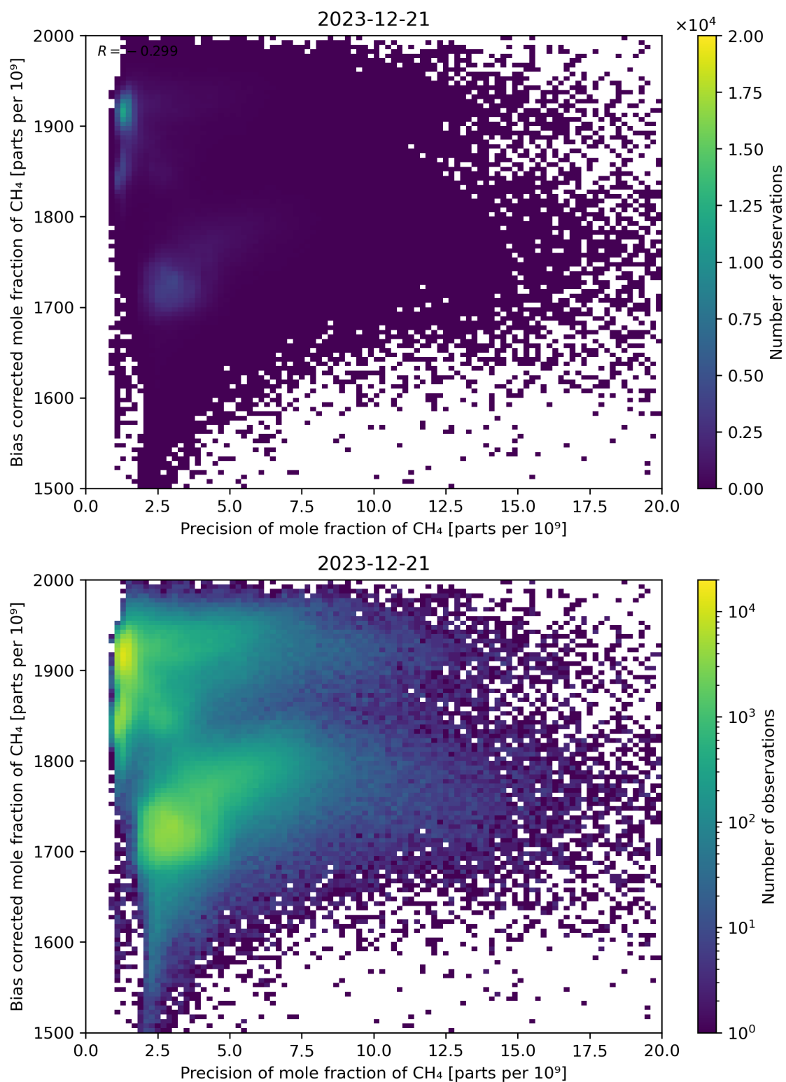
Figure 82: Scatter density plot of “Precision of mole fraction of CH 4 ” against “Bias corrected mole fraction of CH 4 ” for 2023-12-20 to 2023-12-22.
