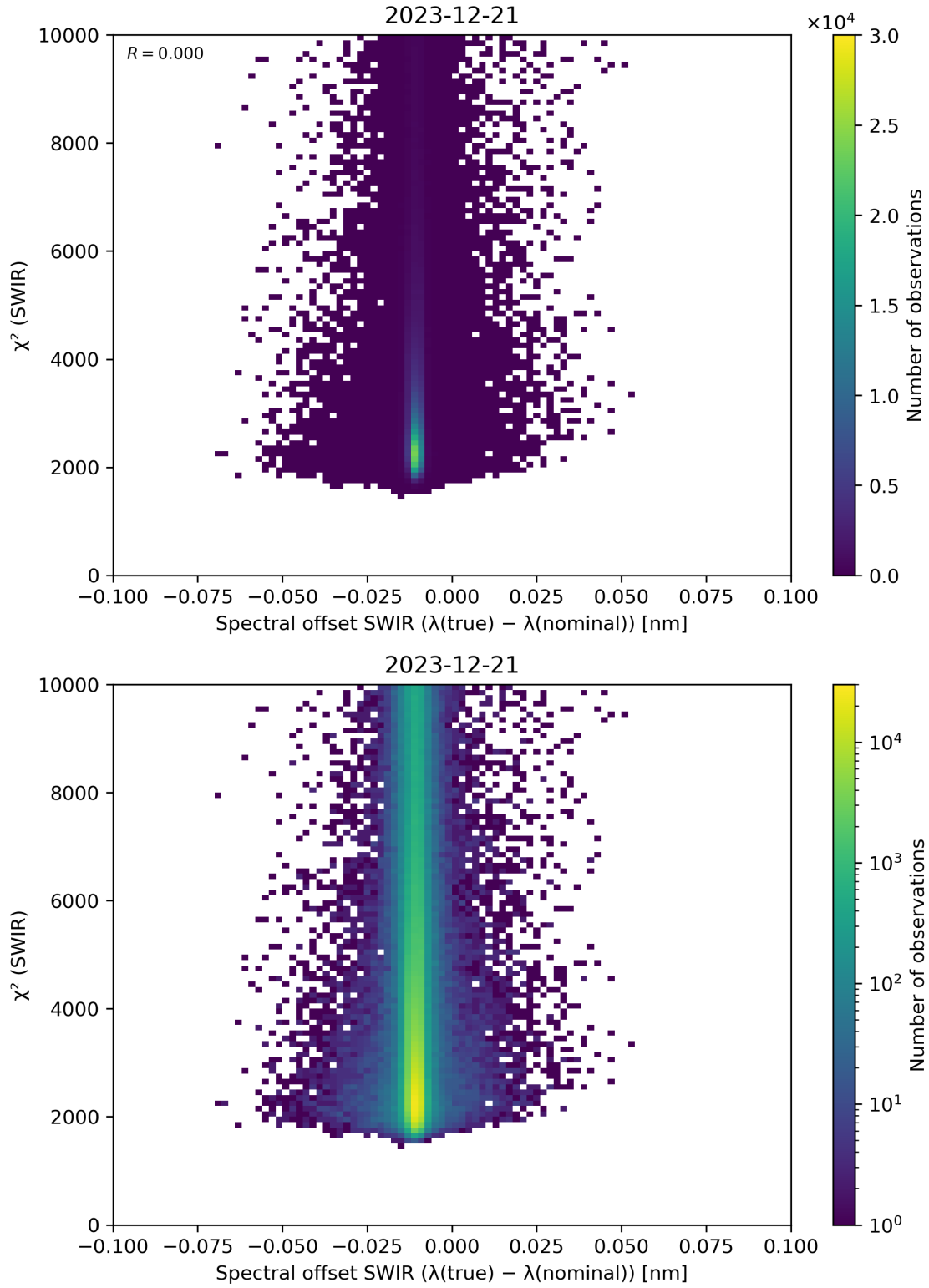
Figure 118: Scatter density plot of “Spectral offset SWIR ( \lambda(\text{true}) - \lambda(\text{nominal}) )” against “ \chi^2 (SWIR)” for 2023-12-20 to 2023-12-22.
