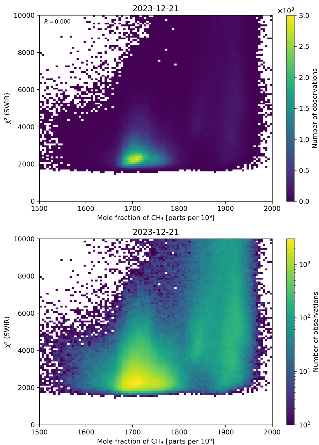
Figure 71: Scatter density plot of “Mole fraction of \text{CH}_4 ” against “ \chi^2 (SWIR)” for 2023-12-20 to 2023-12-22.
