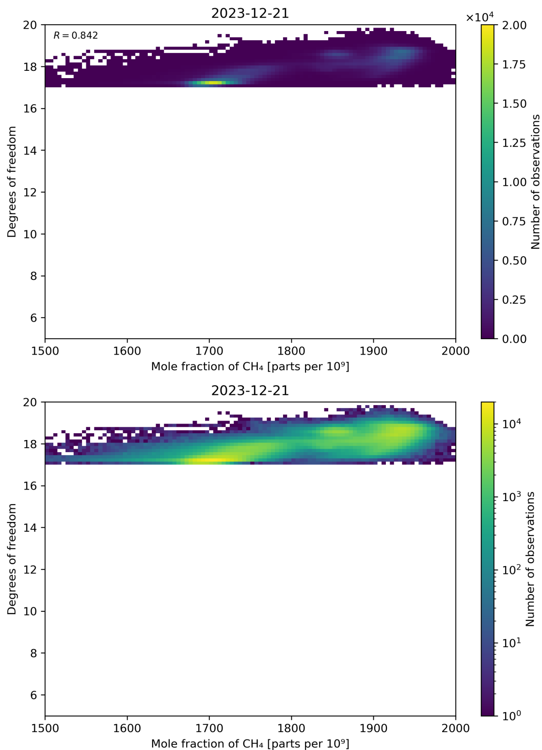
Figure 72: Scatter density plot of “Mole fraction of CH 4 ” against “Degrees of freedom” for 2023-12-20 to 2023-12-22.
