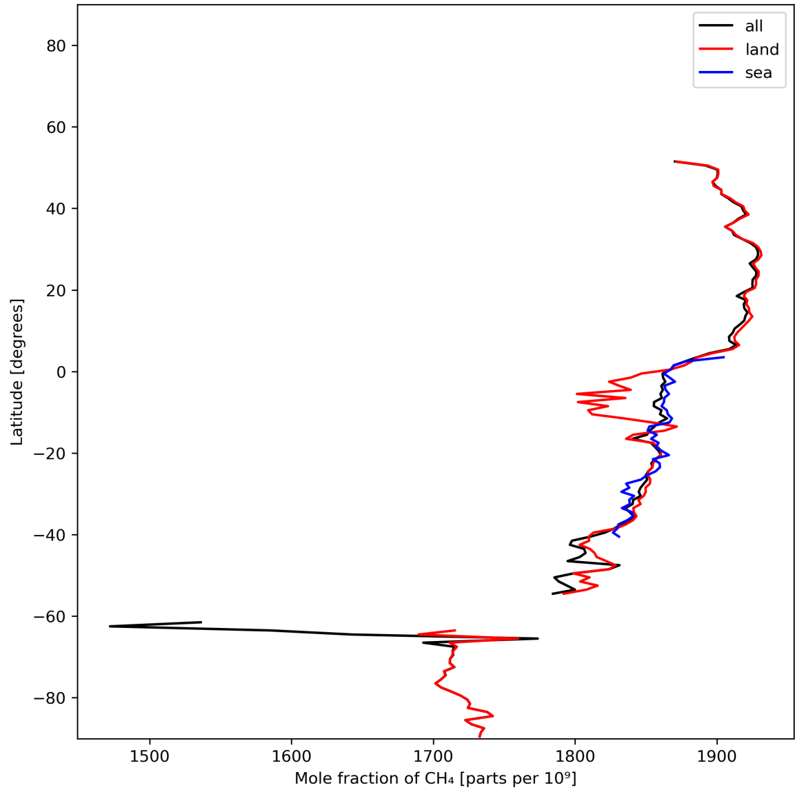
Figure 12: Zonal average of “Mole fraction of CH 4 ” for 2023-12-20 to 2023-12-22.
