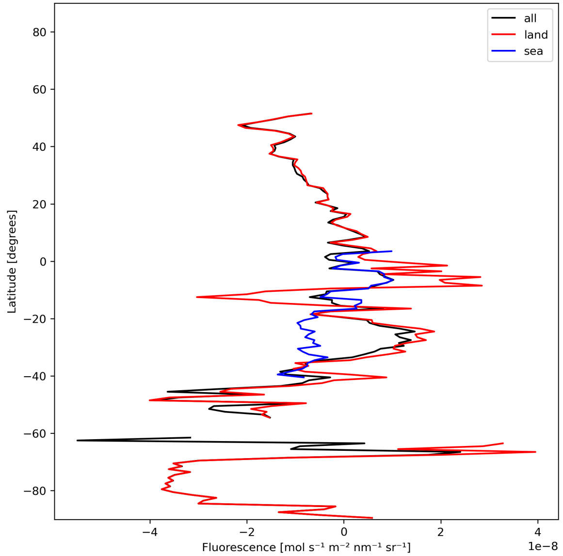
Figure 21: Zonal average of “Fluorescence” for 2023-12-20 to 2023-12-22.
