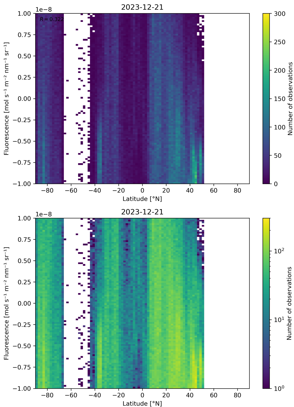
Figure 56: Scatter density plot of “Latitude” against “Fluorescence” for 2023-12-20 to 2023-12-22.
