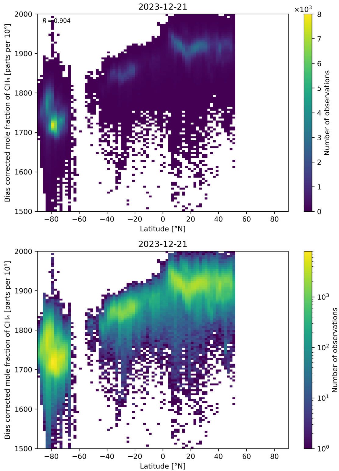
Figure 58: Scatter density plot of “Latitude” against “Bias corrected mole fraction of CH 4 ” for 2023-12-20 to 2023-12-22.
