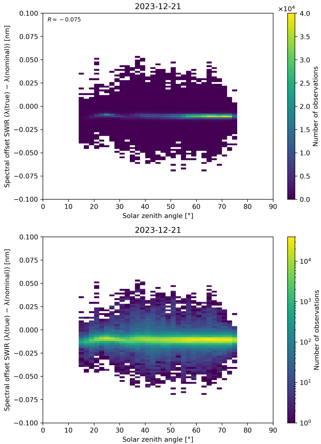
Figure 104: Scatter density plot of “Solar zenith angle” against “Spectral offset SWIR ( \lambda(\text{true}) - \lambda(\text{nominal}) )” for 2023-12-20 to 2023-12-22.
