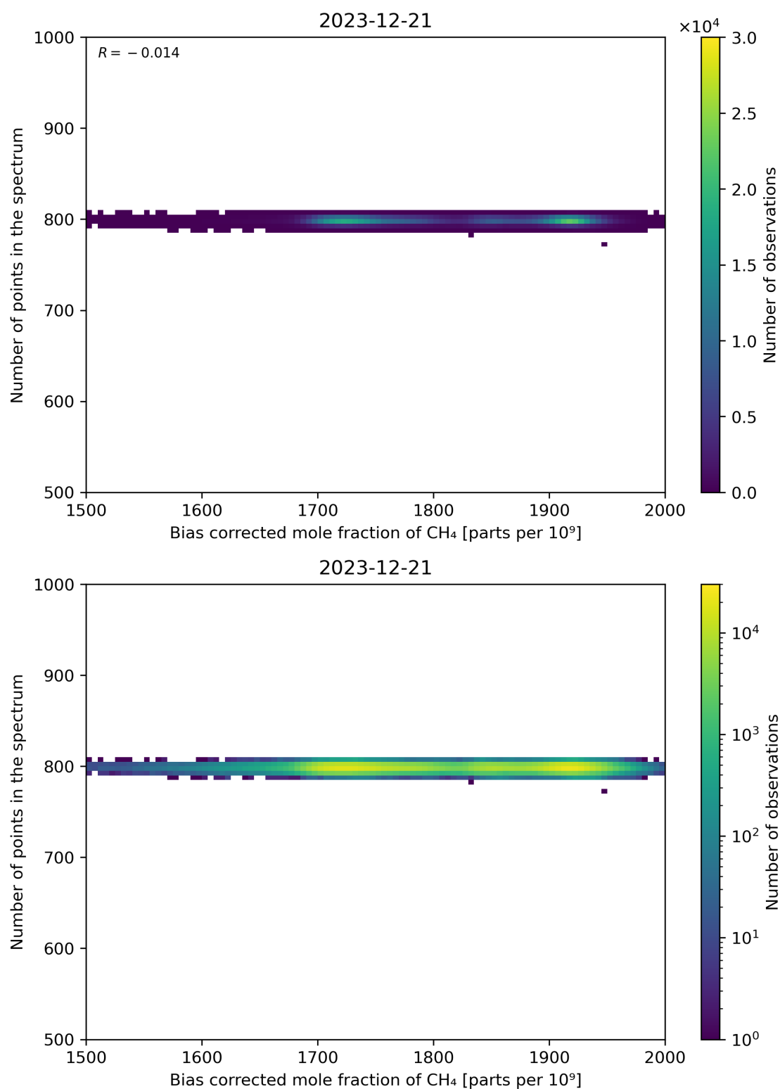
Figure 68: Scatter density plot of “Bias corrected mole fraction of CH 4 ” against “Number of points in the spectrum” for 2023-12-20 to 2023-12-22.
