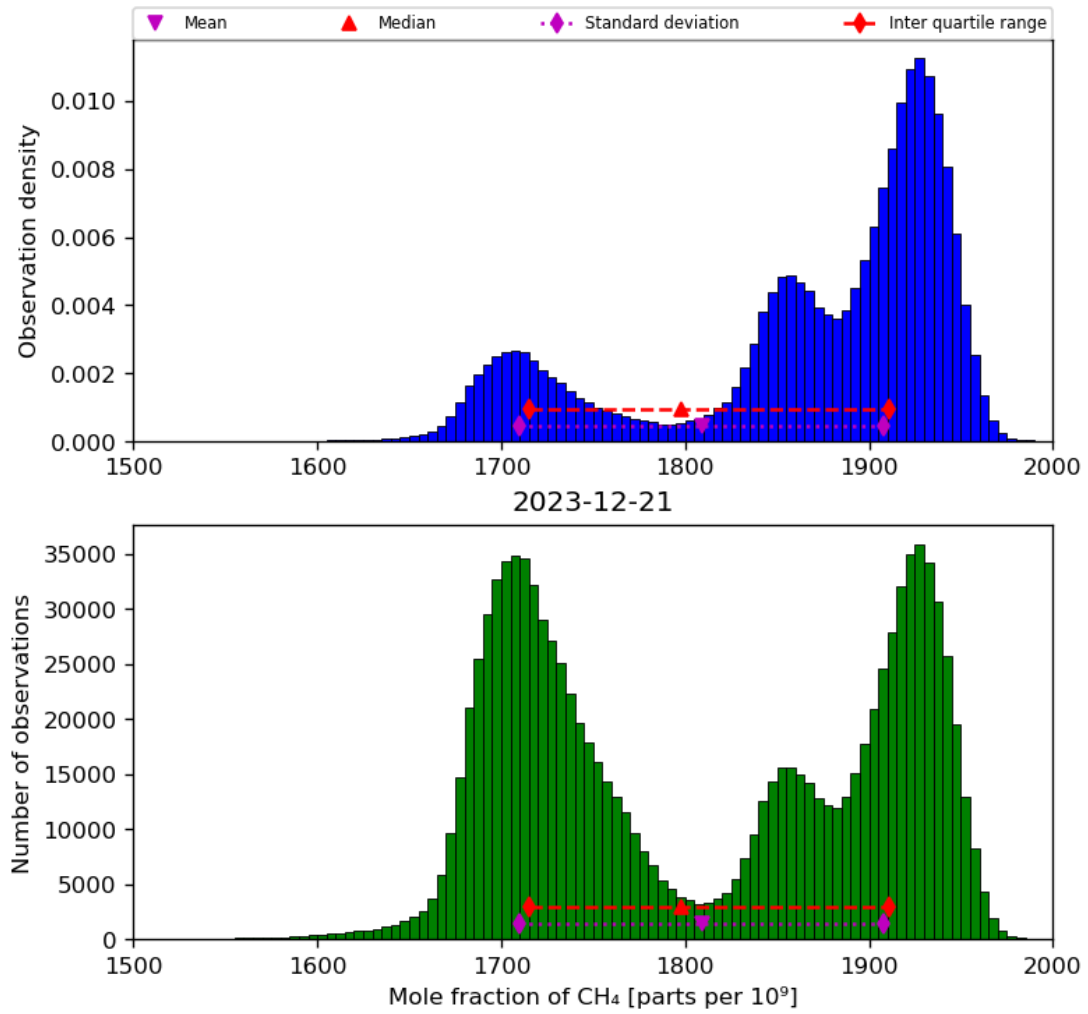
Figure 23: Histogram of “Mole fraction of CH 4 ” for 2023-12-20 to 2023-12-22
