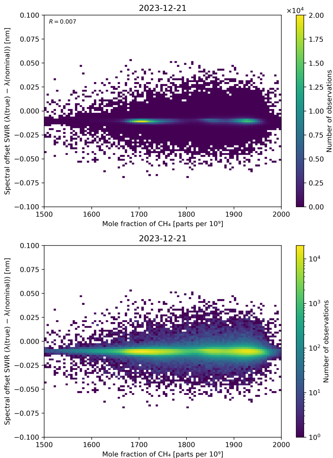
Figure 86: Scatter density plot of “Mole fraction of CH 4 ” against “Spectral offset SWIR ( \lambda(\text{true}) - \lambda(\text{nominal}) )” for 2023-12-20 to 2023-12-22.
