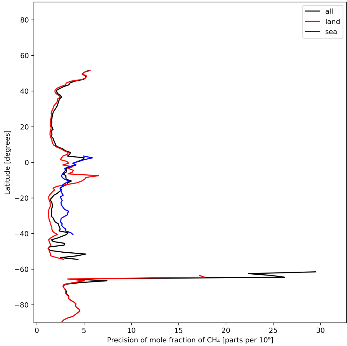
Figure 13: Zonal average of “Precision of mole fraction of CH 4 ” for 2023-12-20 to 2023-12-22.
