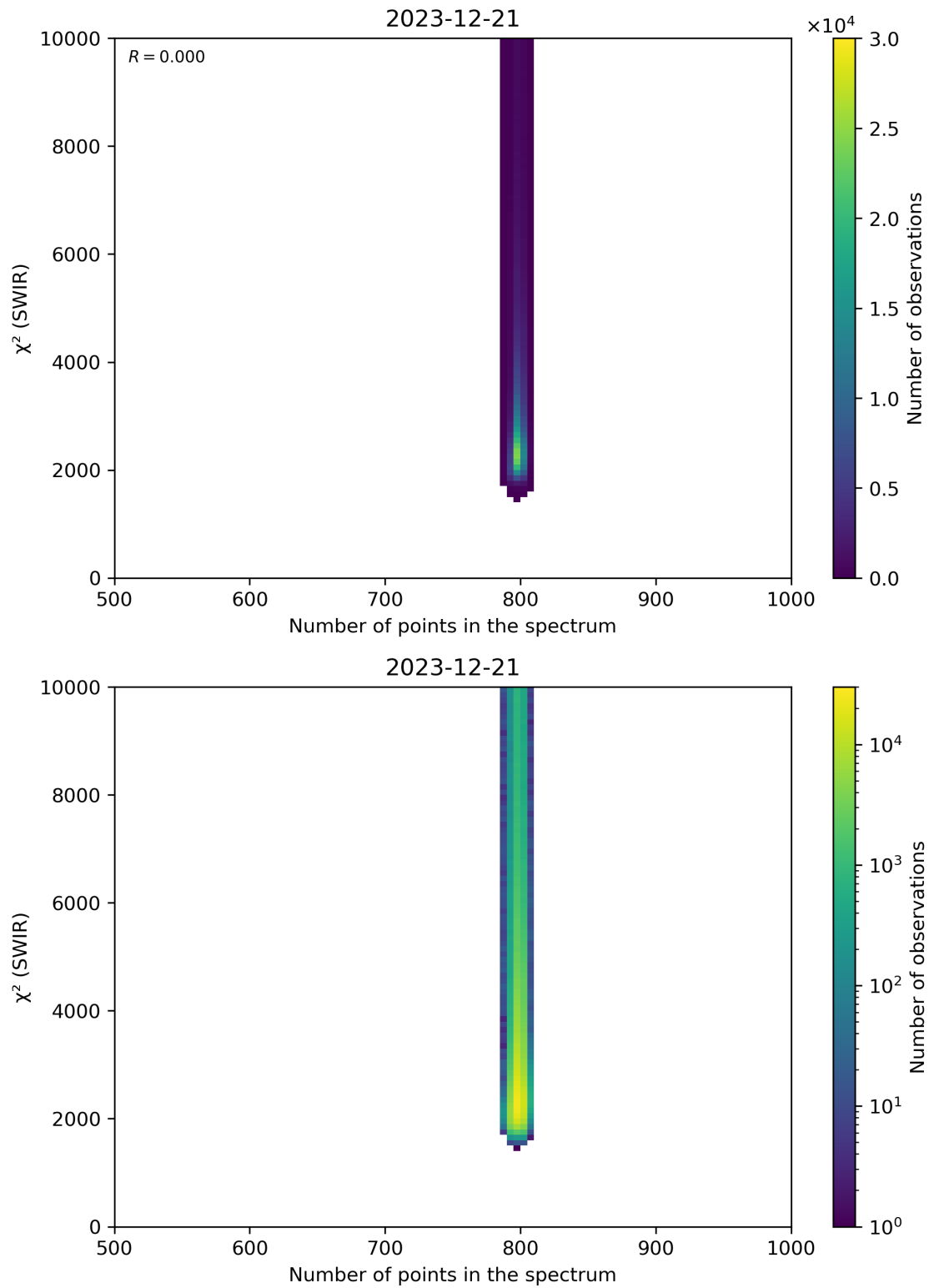
Figure 89: Scatter density plot of “Number of points in the spectrum” against “ \chi^2 (SWIR)” for 2023-12-20 to 2023-12-22.
