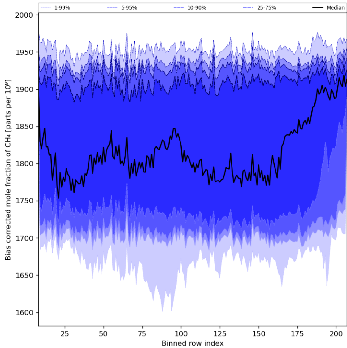
Figure 36: Along track statistics of “Bias corrected mole fraction of CH 4 ” for 2023-12-20 to 2023-12-22
