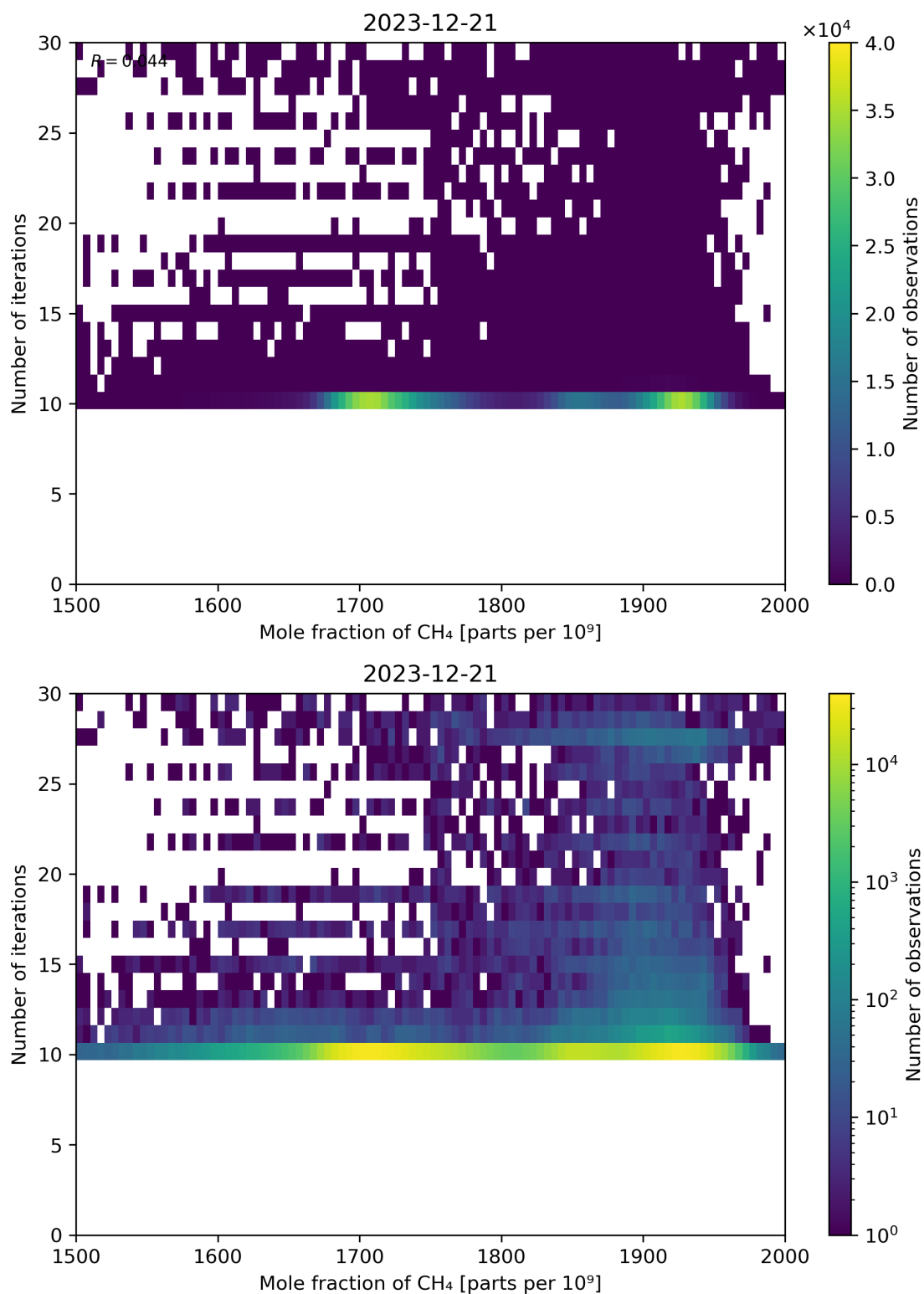
Figure 76: Scatter density plot of “Mole fraction of CH 4 ” against “Number of iterations” for 2023-12-20 to 2023-12-22.
