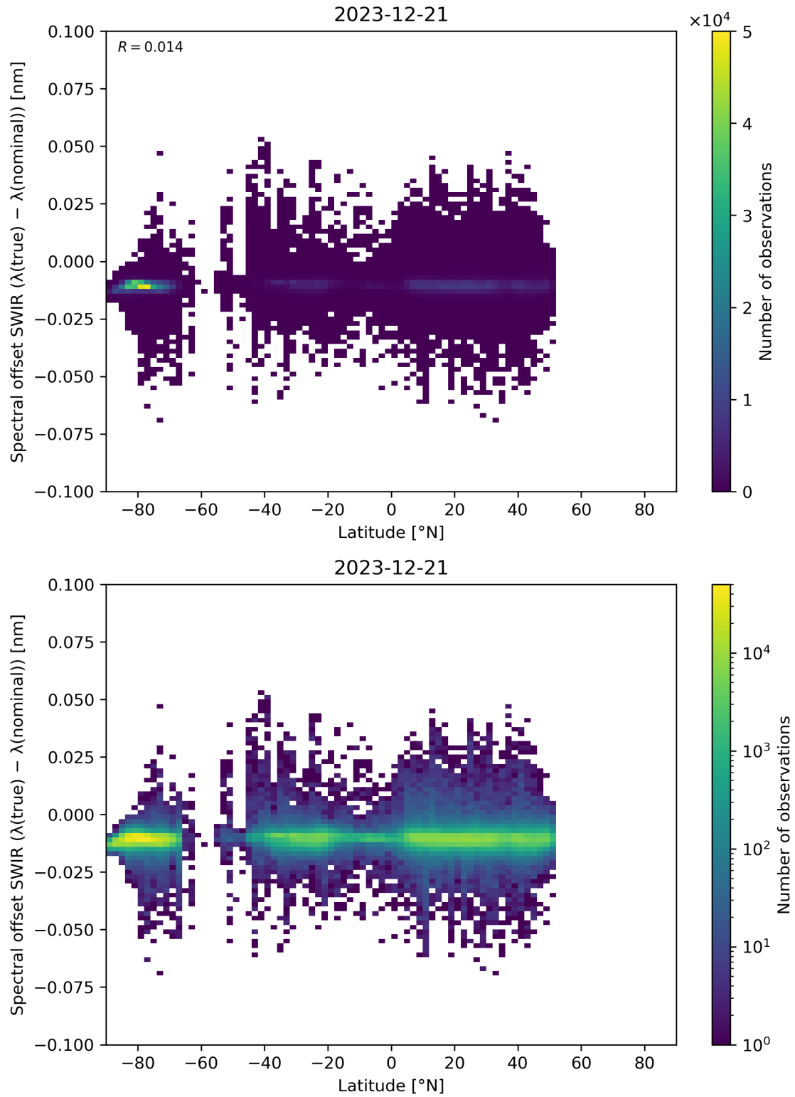
Figure 62: Scatter density plot of “Latitude” against “Spectral offset SWIR ( \lambda(\text{true}) - \lambda(\text{nominal}) )” for 2023-12-20 to 2023-12-22.
