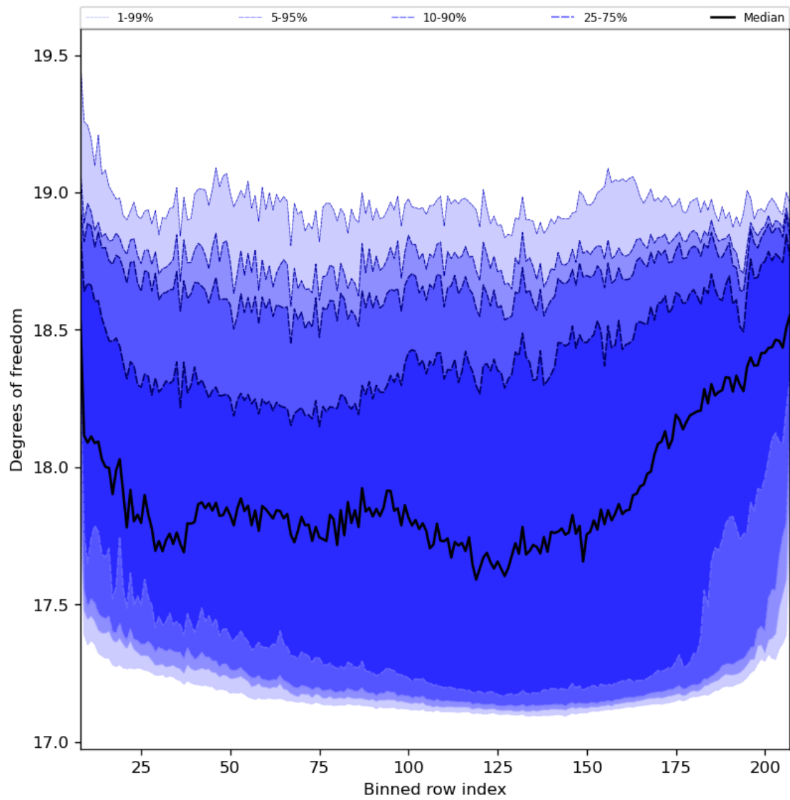
Figure 41: Along track statistics of “Degrees of freedom” for 2023-12-20 to 2023-12-22
