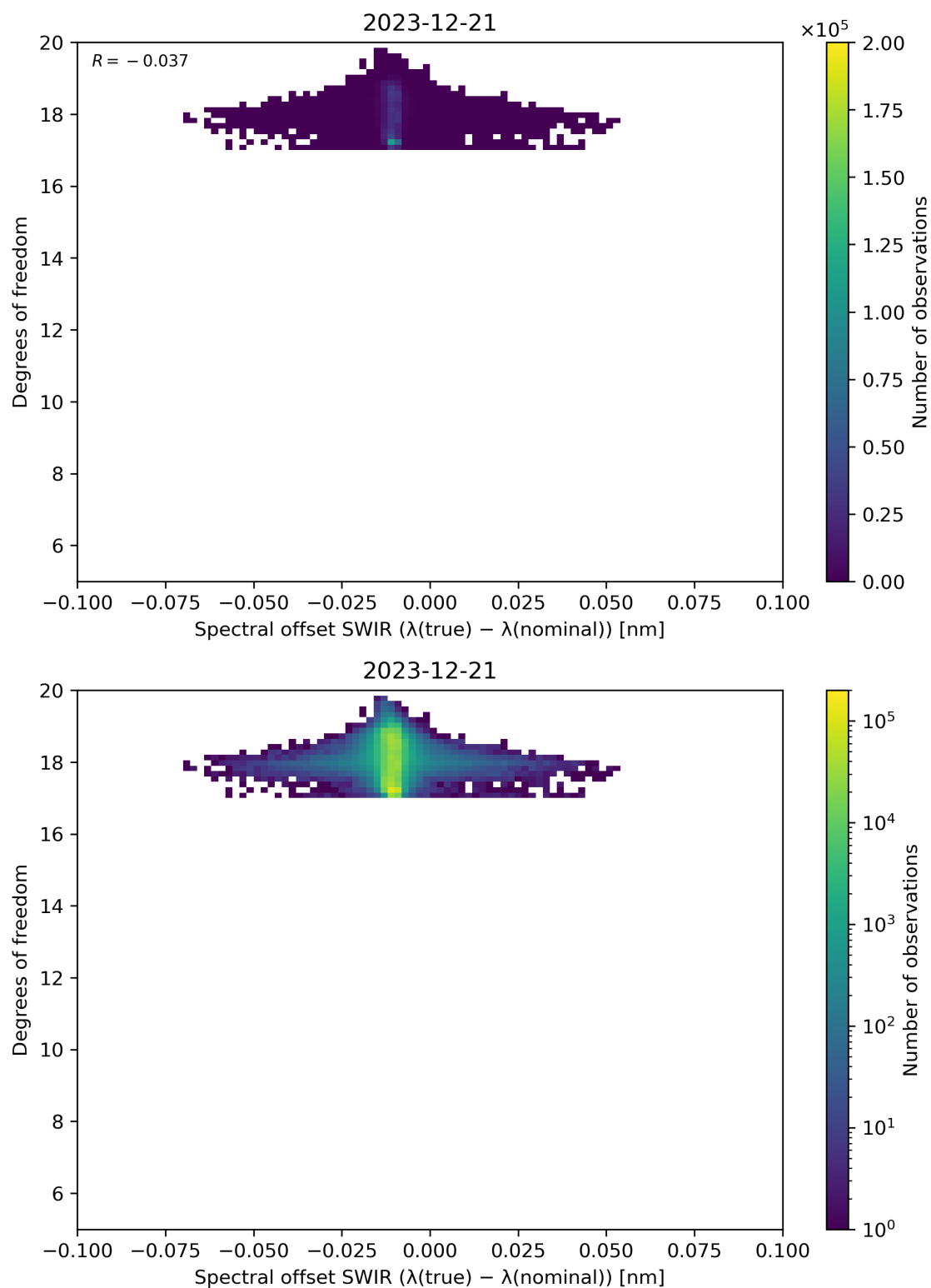
Figure 119: Scatter density plot of “Spectral offset SWIR ( \lambda(\text{true}) - \lambda(\text{nominal}) )” against “Degrees of freedom” for 2023-12-20 to 2023-12-22.
