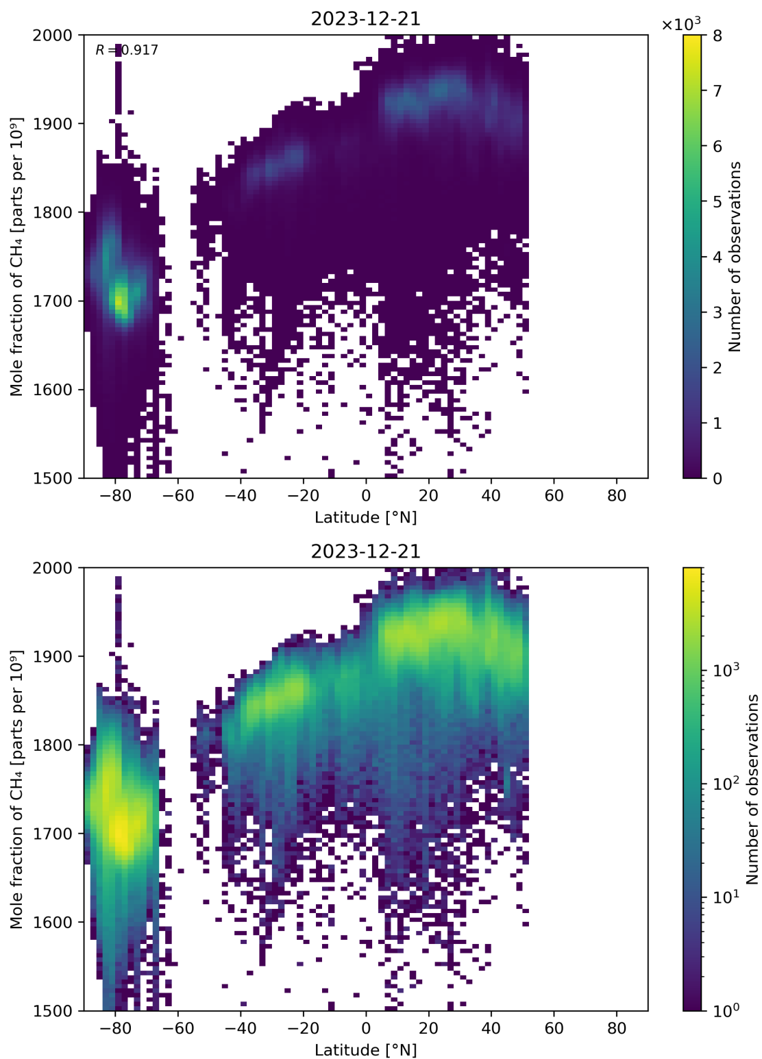
Figure 57: Scatter density plot of “Latitude” against “Mole fraction of CH 4 ” for 2023-12-20 to 2023-12-22.
