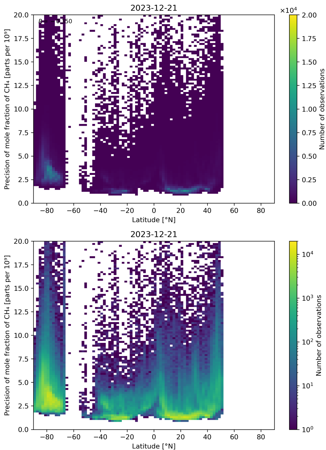
Figure 59: Scatter density plot of “Latitude” against “Precision of mole fraction of CH 4 ” for 2023-12-20 to 2023-12-22.
