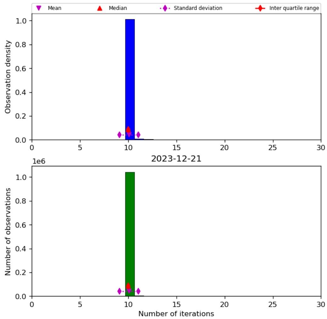
Figure 31: Histogram of “Number of iterations” for 2023-12-20 to 2023-12-22
