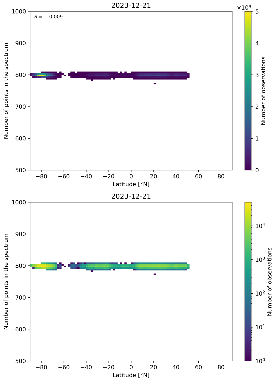
Figure 61: Scatter density plot of “Latitude” against “Number of points in the spectrum” for 2023-12-20 to 2023-12-22.
