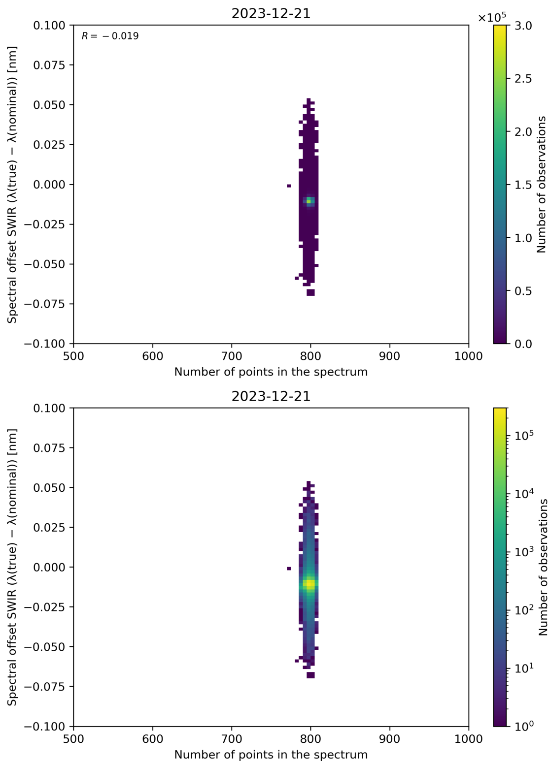
Figure 93: Scatter density plot of “Number of points in the spectrum” against “Spectral offset SWIR ( \lambda(\text{true}) - \lambda(\text{nominal}) )” for 2023-12-20 to 2023-12-22.
