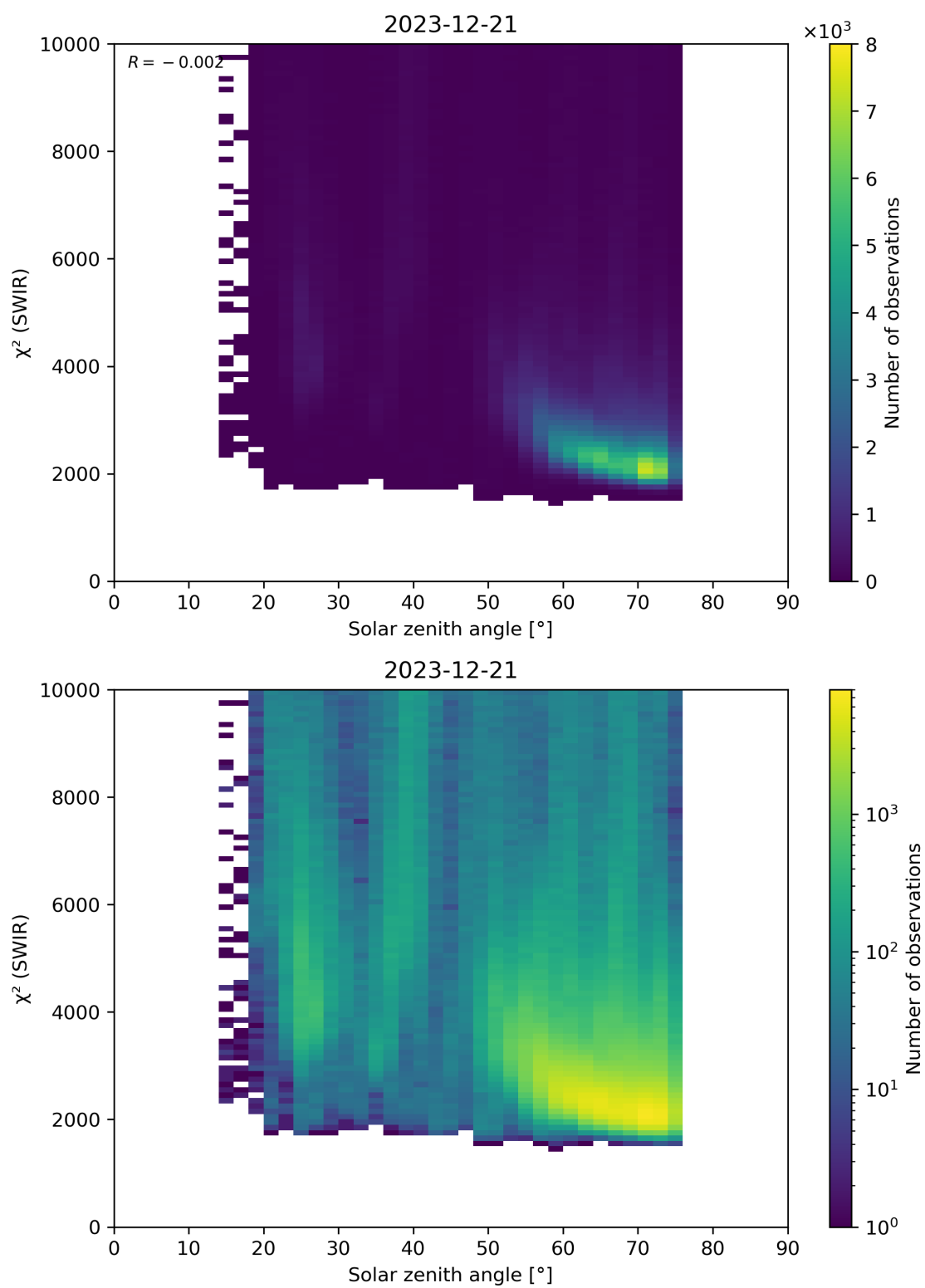
Figure 95: Scatter density plot of “Solar zenith angle” against “ \chi^2 (SWIR)” for 2023-12-20 to 2023-12-22.
