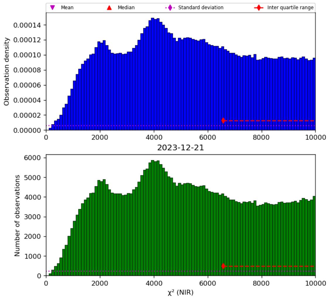
Figure 29: Histogram of “ \chi^2 (NIR)” for 2023-12-20 to 2023-12-22
