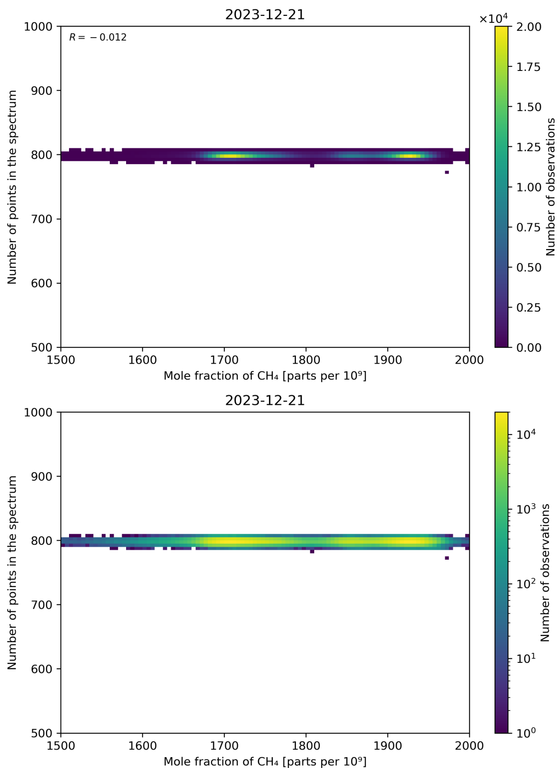
Figure 77: Scatter density plot of “Mole fraction of CH 4 ” against “Number of points in the spectrum” for 2023-12-20 to 2023-12-22.
