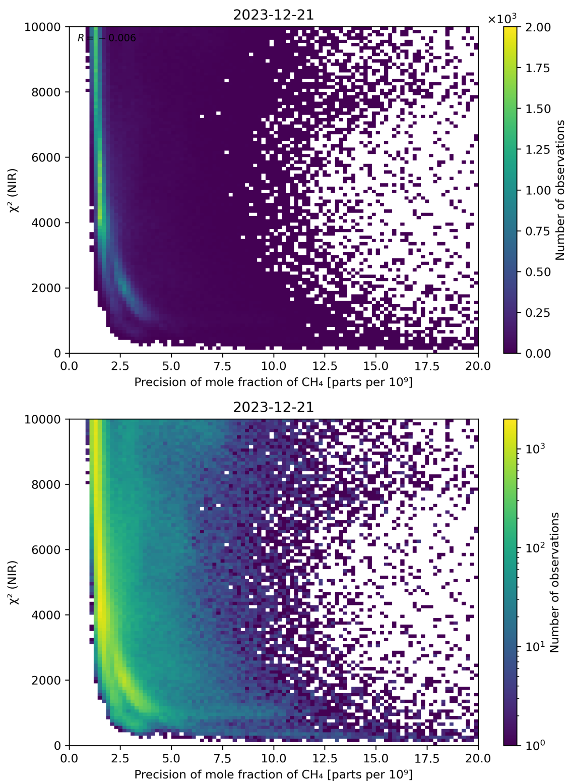
Figure 78: Scatter density plot of “Precision of mole fraction of \text{CH}_4 ” against “ \chi^2 (NIR)” for 2023-12-20 to 2023-12-22.
