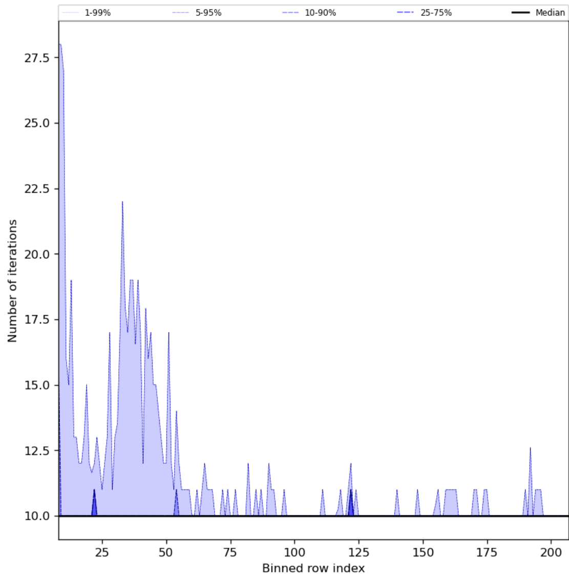
Figure 42: Along track statistics of “Number of iterations” for 2023-12-20 to 2023-12-22
