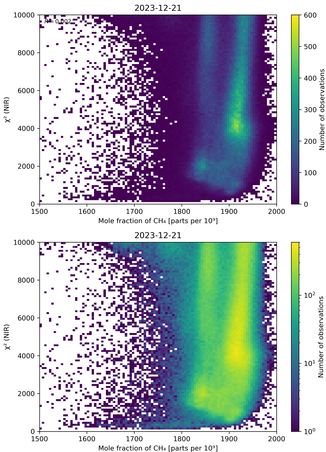
Figure 70: Scatter density plot of “Mole fraction of CH 4 ” against “ \chi^2 (NIR)” for 2023-12-20 to 2023-12-22.
