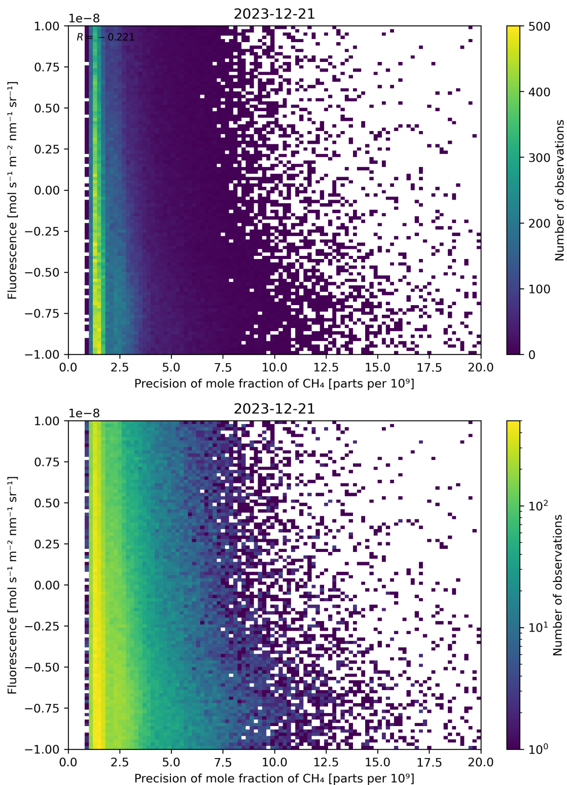
Figure 81: Scatter density plot of “Precision of mole fraction of \text{CH}_4 ” against “Fluorescence” for 2023-12-20 to 2023-12-22.
