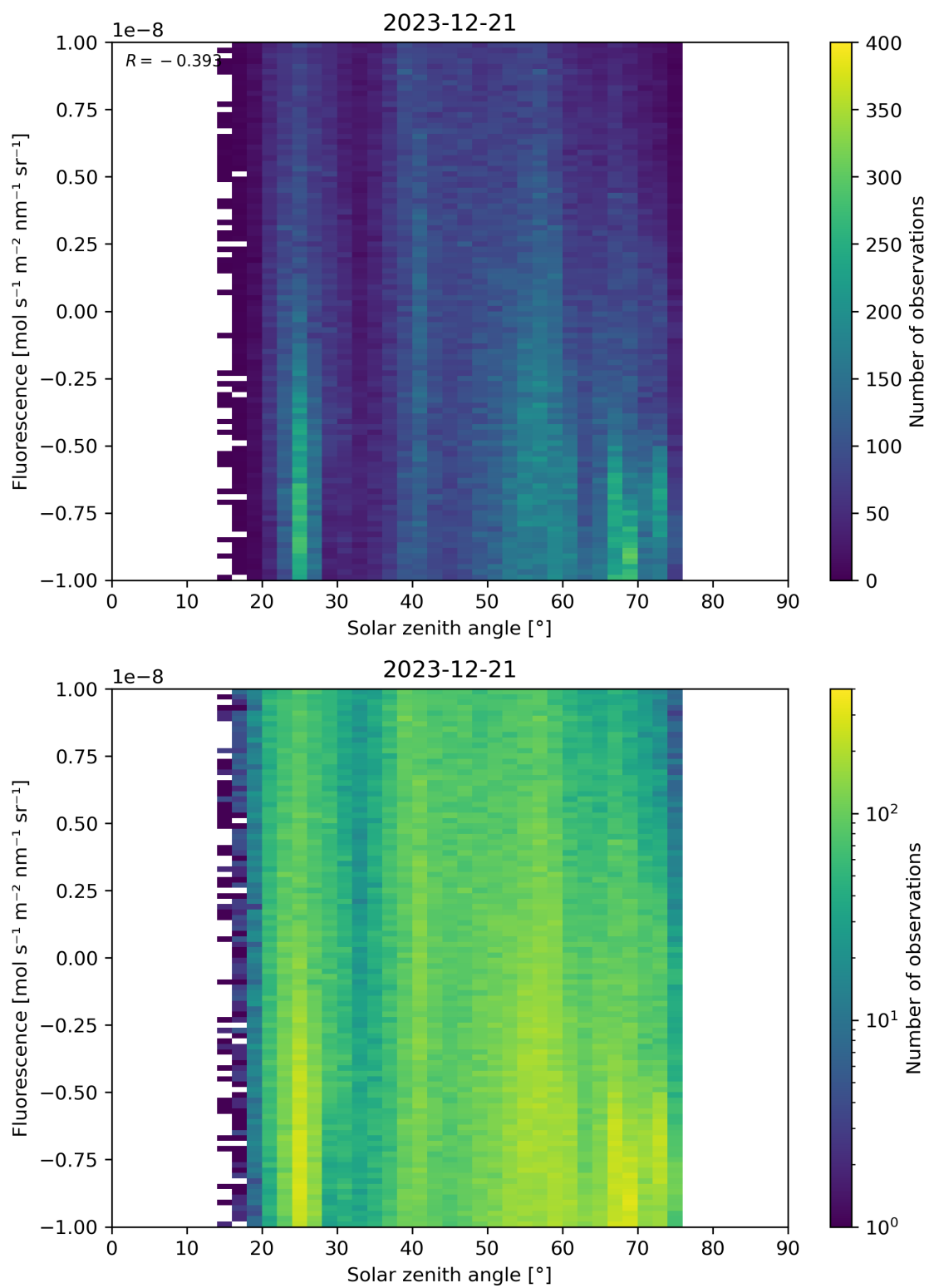
Figure 97: Scatter density plot of “Solar zenith angle” against “Fluorescence” for 2023-12-20 to 2023-12-22.
