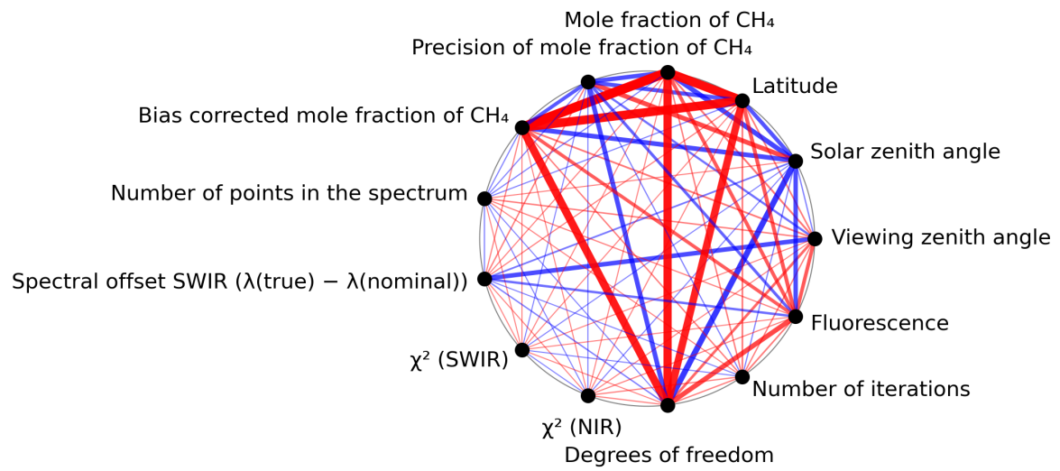
Figure 1: Map of correlation graph for 2023-12-20 to 2023-12-22.
