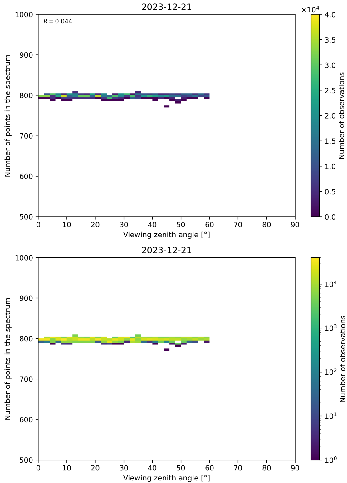
Figure 114: Scatter density plot of “Viewing zenith angle” against “Number of points in the spectrum” for 2023-12-20 to 2023-12-22.
