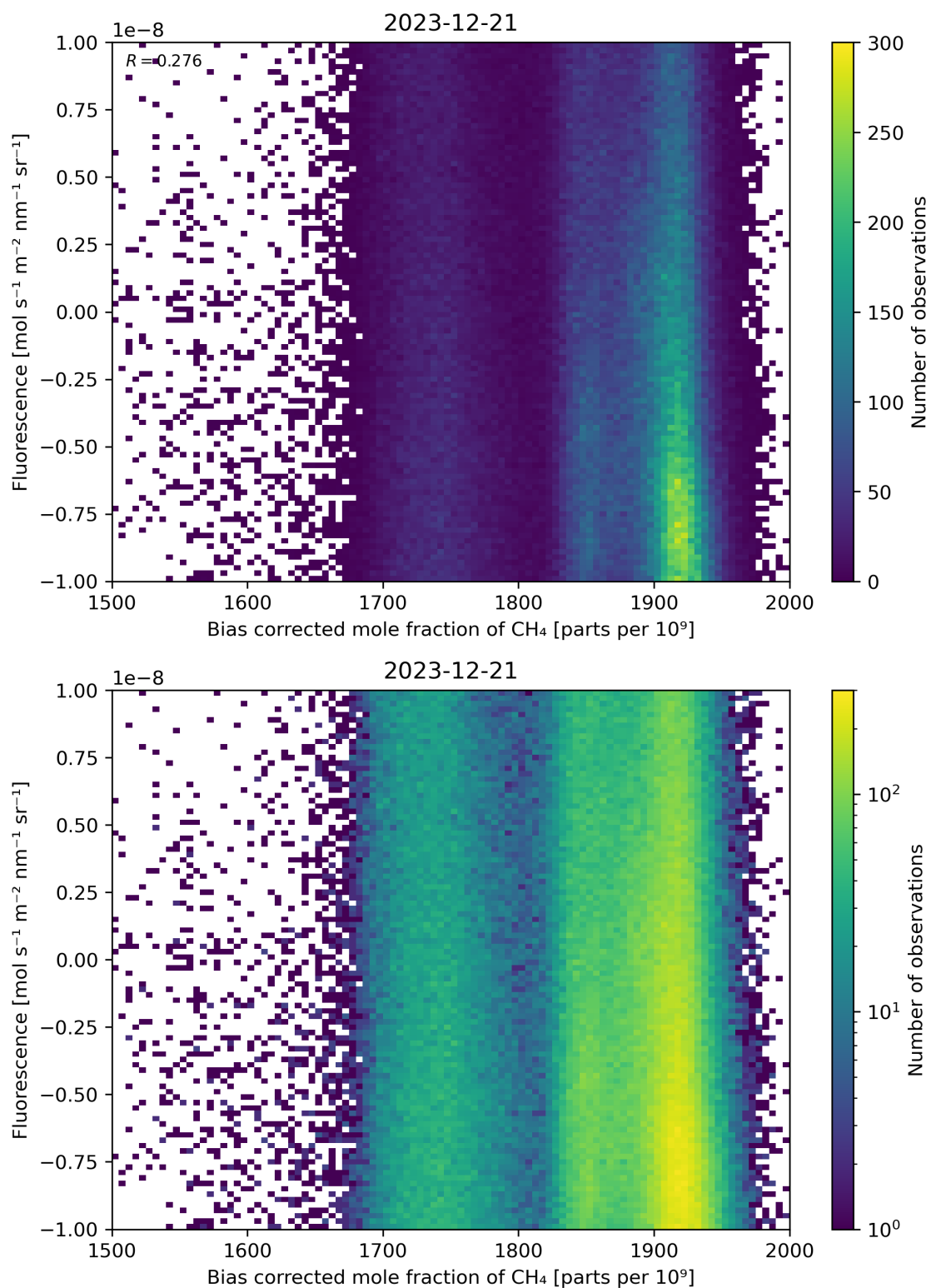
Figure 66: Scatter density plot of “Bias corrected mole fraction of \text{CH}_4 ” against “Fluorescence” for 2023-12-20 to 2023-12-22.
