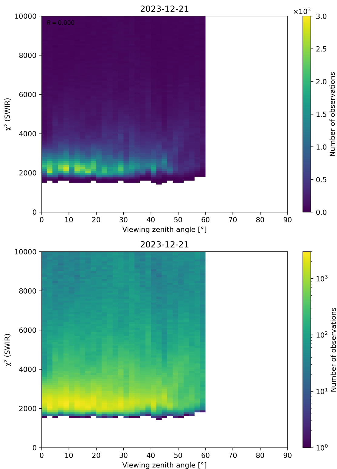
Figure 106: Scatter density plot of “Viewing zenith angle” against “ \chi^2 (SWIR)” for 2023-12-20 to 2023-12-22.
