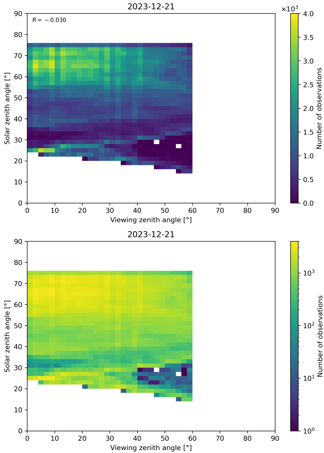
Figure 115: Scatter density plot of “Viewing zenith angle” against “Solar zenith angle” for 2023-12-20 to 2023-12-22.
