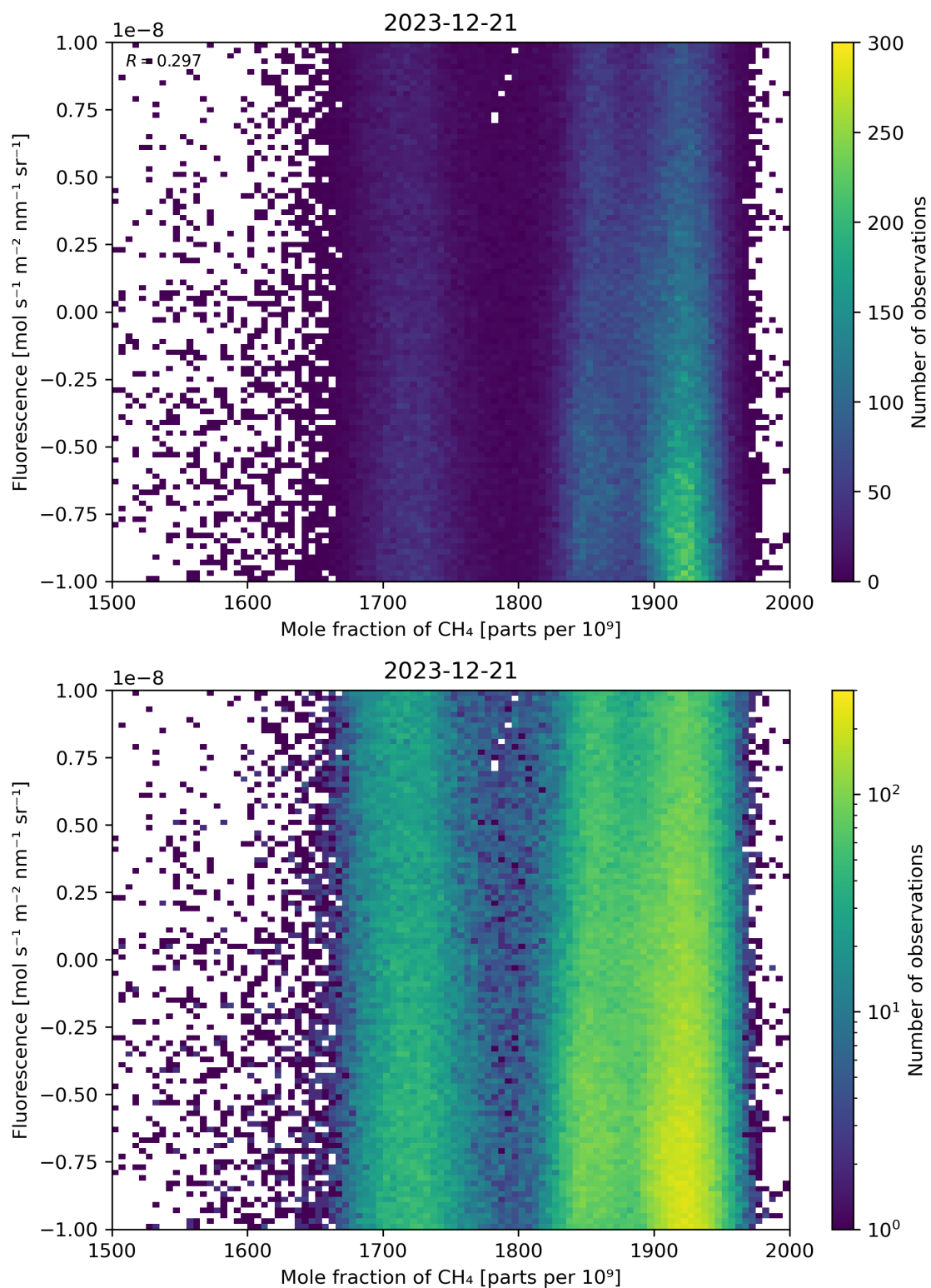
Figure 73: Scatter density plot of “Mole fraction of CH 4 ” against “Fluorescence” for 2023-12-20 to 2023-12-22.
