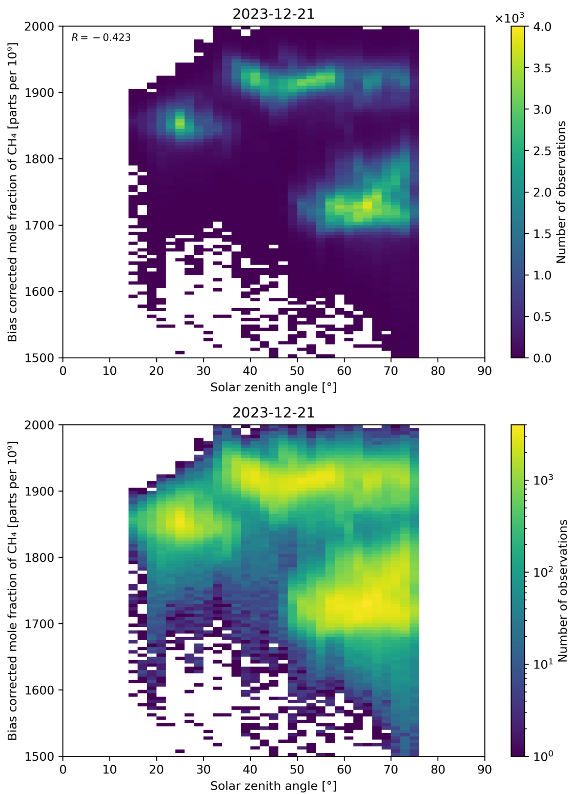
Figure 100: Scatter density plot of “Solar zenith angle” against “Bias corrected mole fraction of \text{CH}_4 ” for 2023-12-20 to 2023-12-22.
