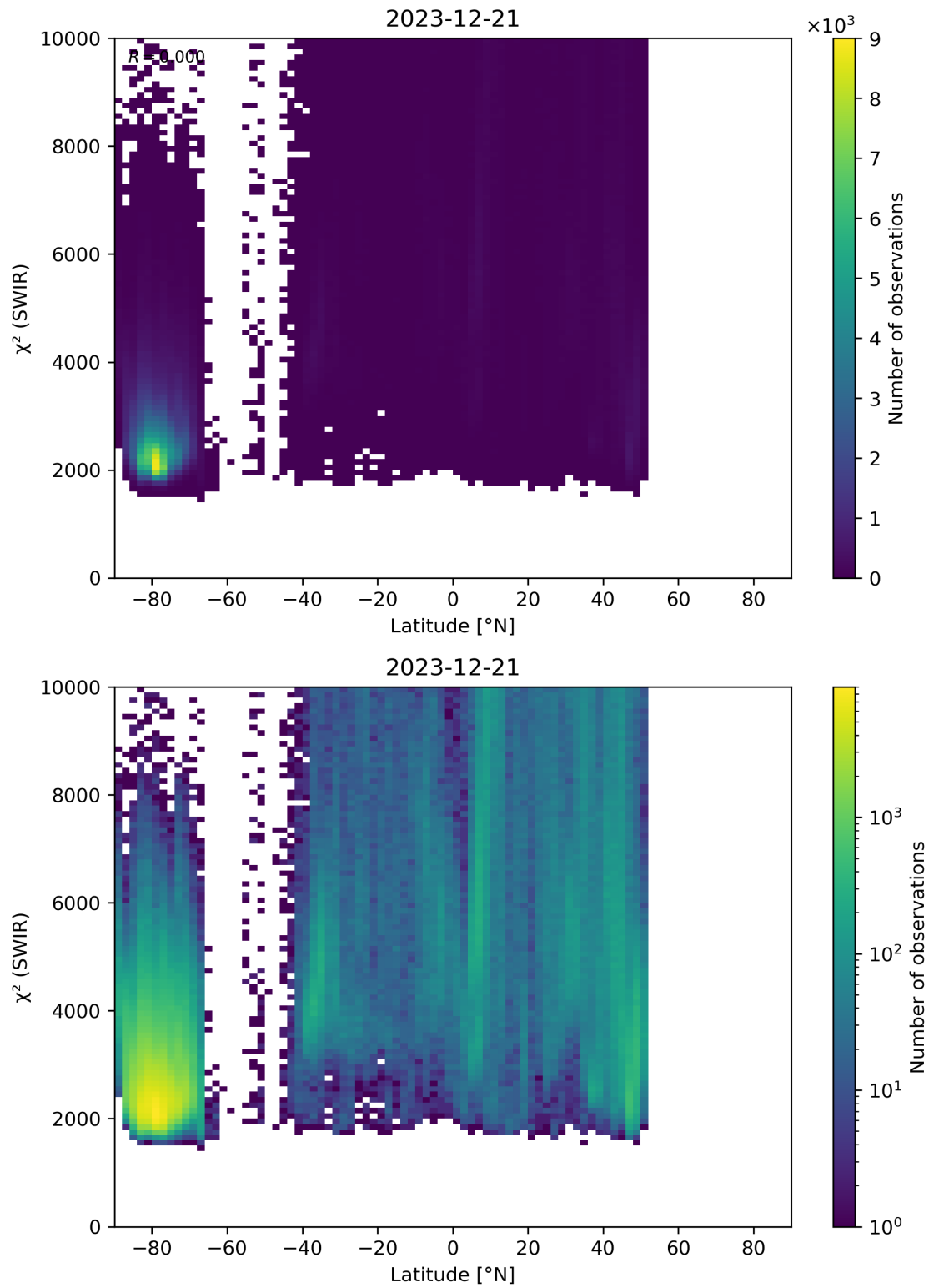
Figure 54: Scatter density plot of “Latitude” against “ \chi^2 (SWIR)” for 2023-12-20 to 2023-12-22.
