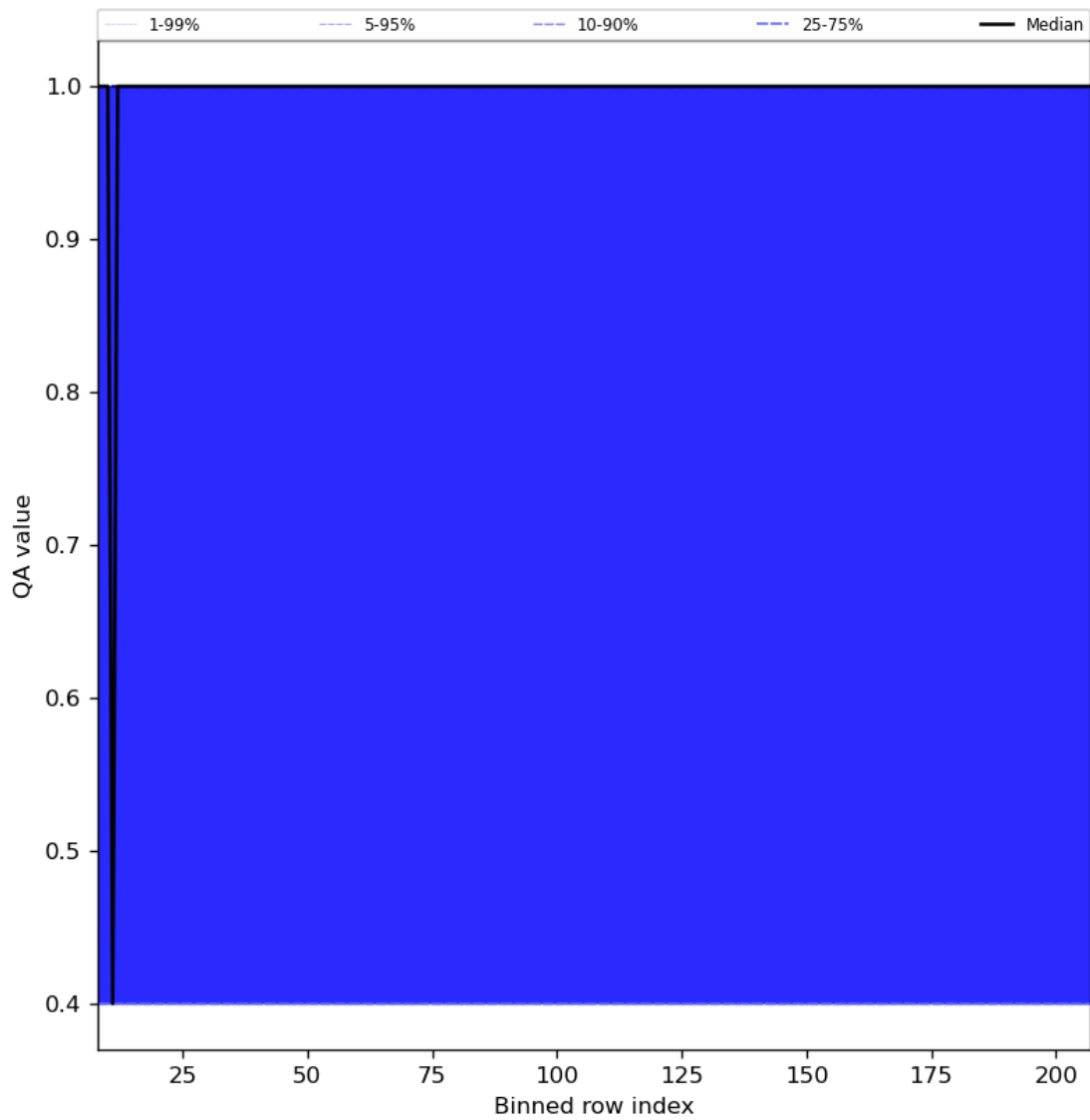
Figure 33: Along track statistics of “QA value” for 2023-12-20 to 2023-12-22
