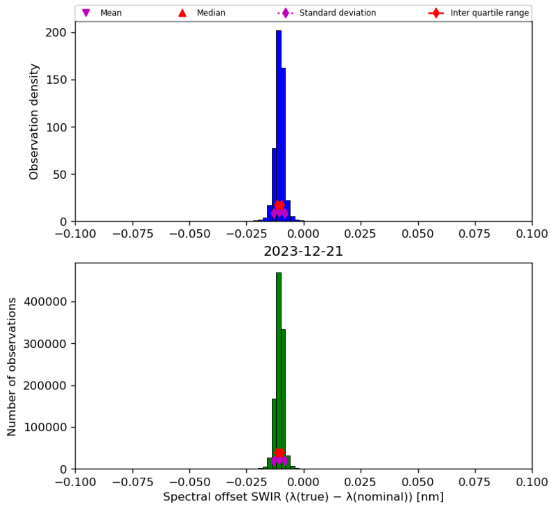
Figure 27: Histogram of “Spectral offset SWIR ( \lambda(\text{true}) - \lambda(\text{nominal}) )” for 2023-12-20 to 2023-12-22
