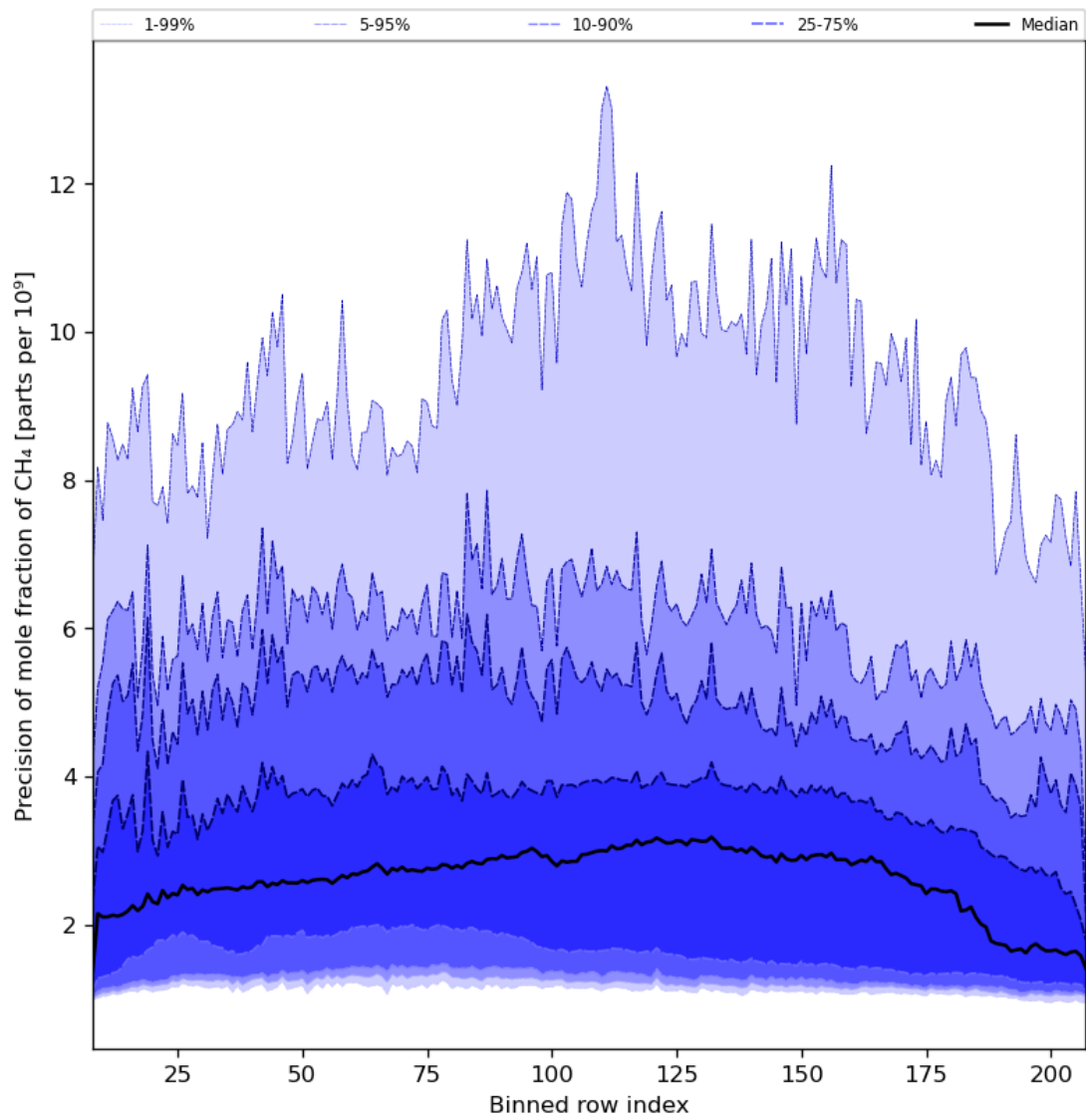
Figure 35: Along track statistics of “Precision of mole fraction of CH 4 ” for 2023-12-20 to 2023-12-22
