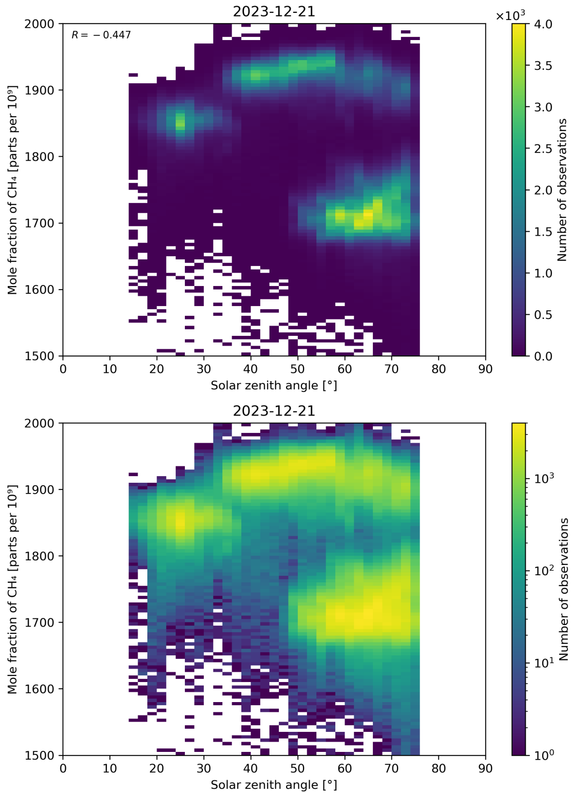
Figure 99: Scatter density plot of “Solar zenith angle” against “Mole fraction of CH 4 ” for 2023-12-20 to 2023-12-22.
