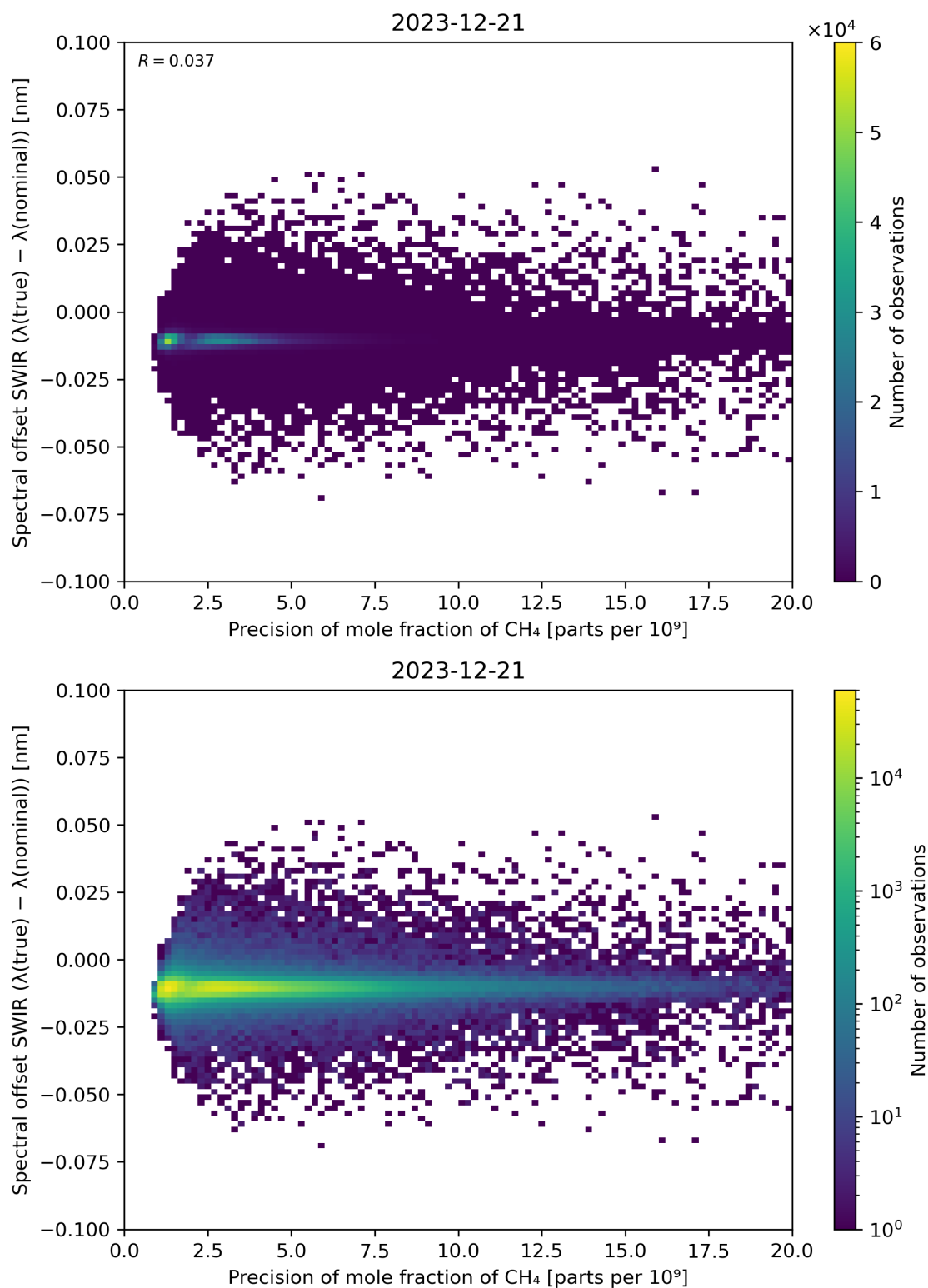
Figure 85: Scatter density plot of “Precision of mole fraction of CH 4 ” against “Spectral offset SWIR ( \lambda(\text{true}) - \lambda(\text{nominal}) )” for 2023-12-20 to 2023-12-22.
