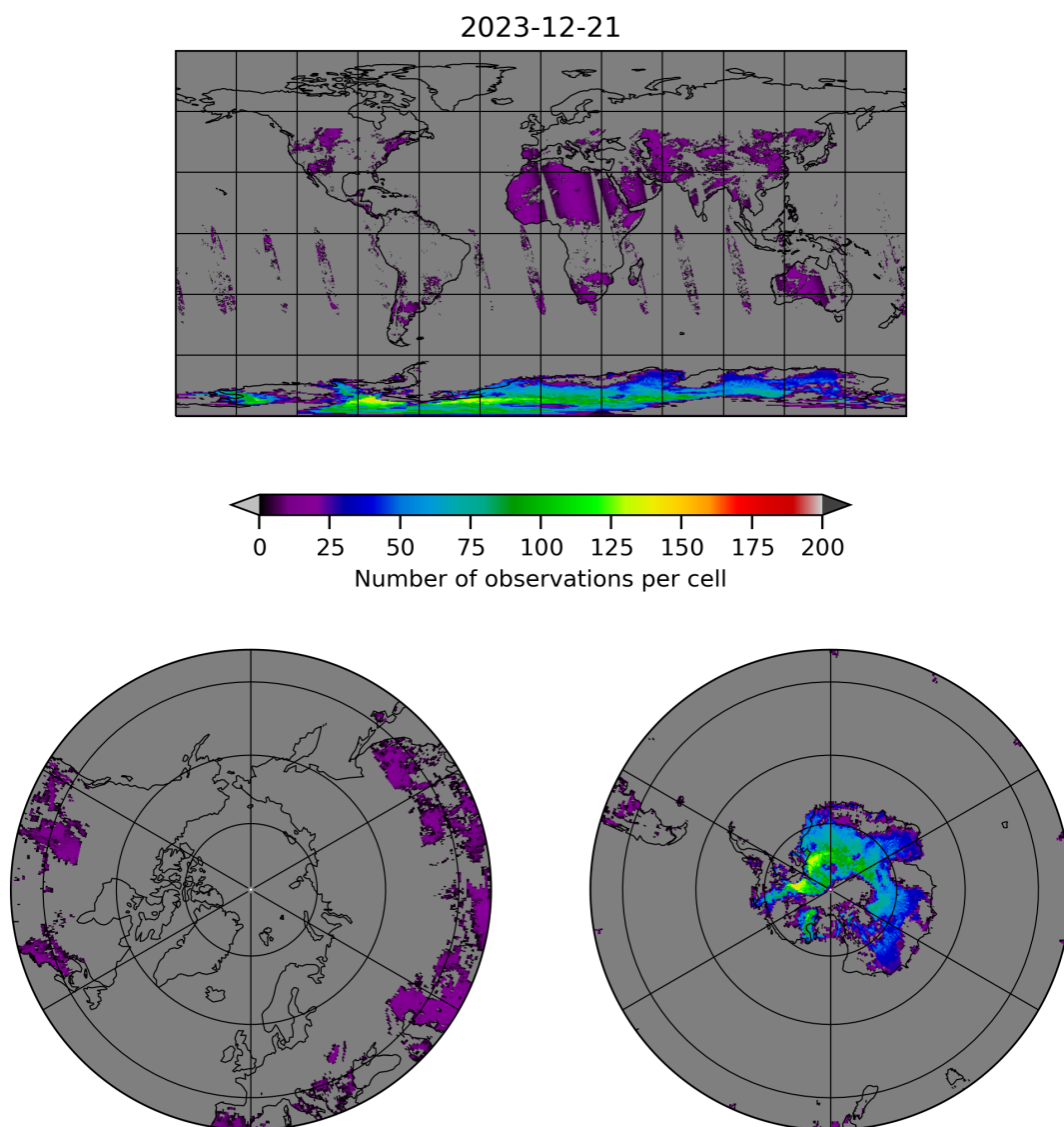
Figure 10: Map of the number of observations for 2023-12-20 to 2023-12-22
