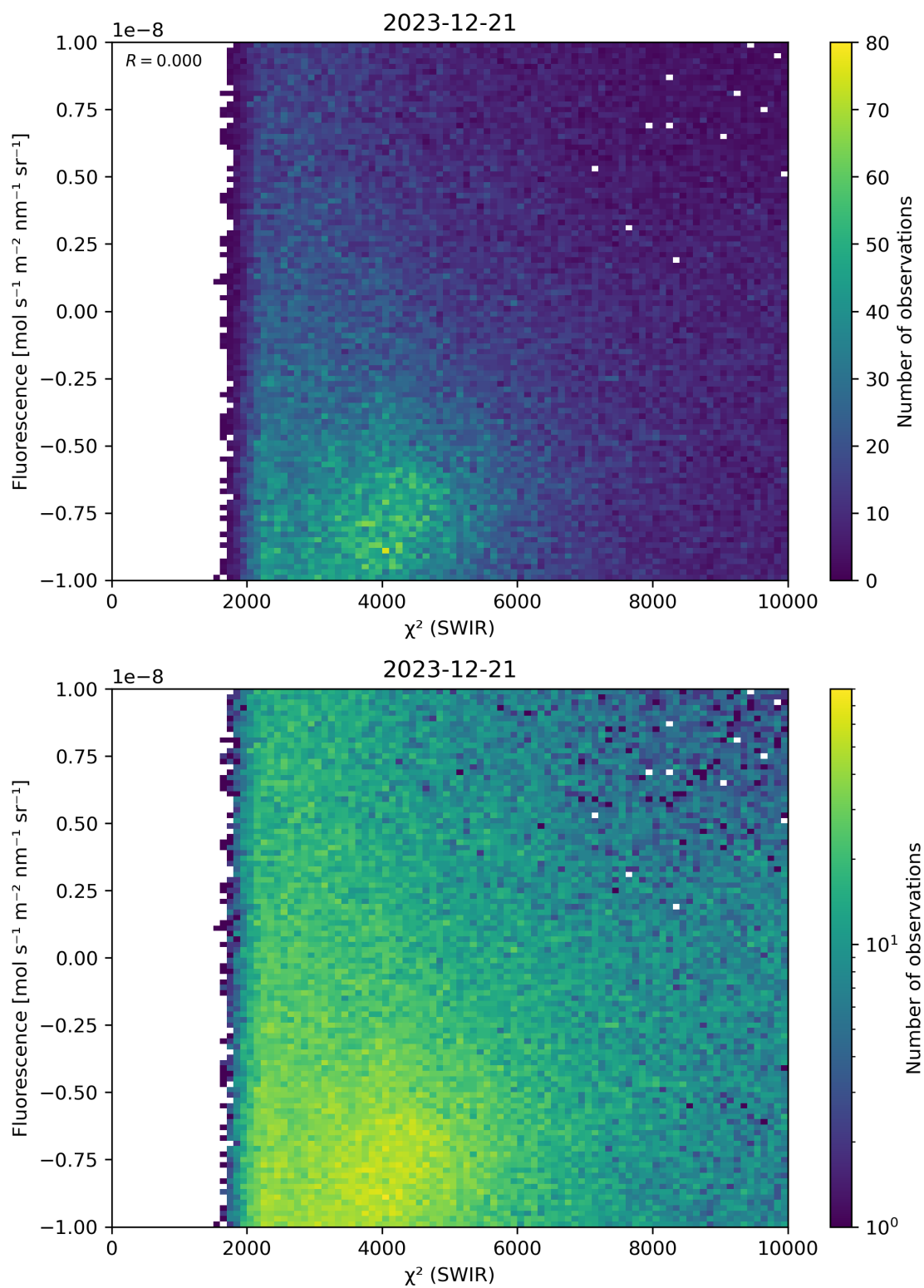
Figure 49: Scatter density plot of “ \chi^2 (SWIR)” against “Fluorescence” for 2023-12-20 to 2023-12-22.
