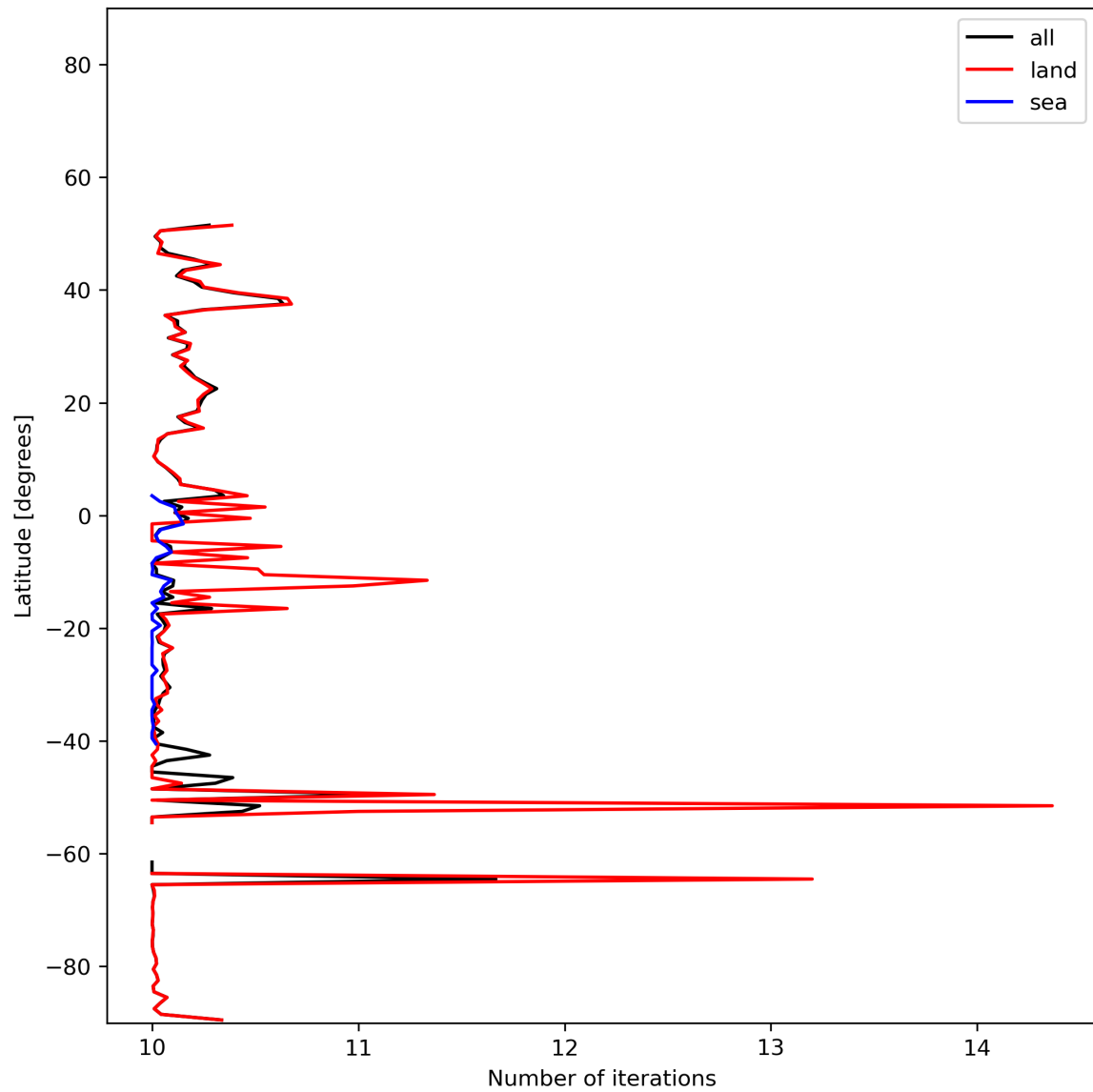
Figure 20: Zonal average of “Number of iterations” for 2023-12-20 to 2023-12-22.
