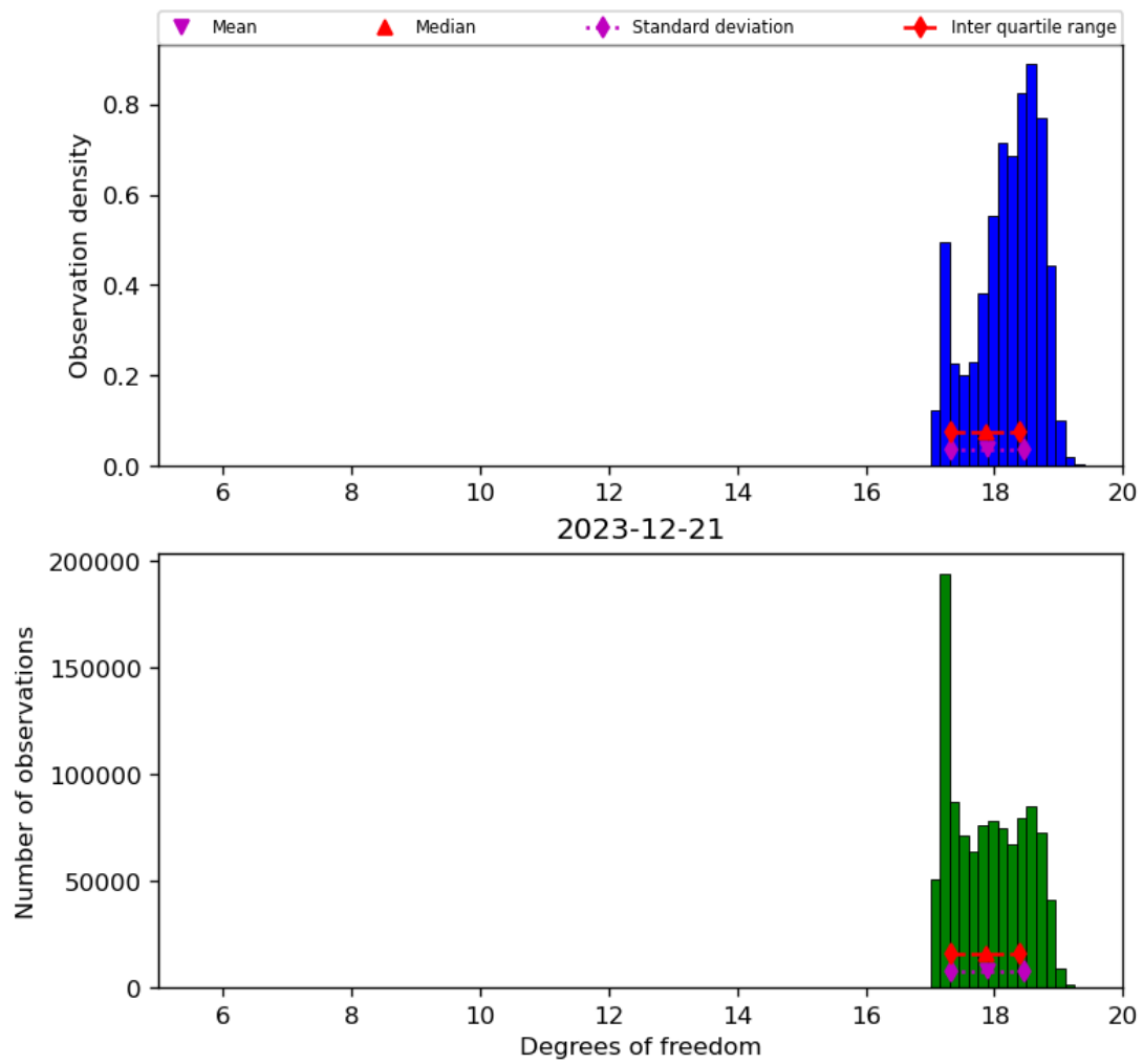
Figure 30: Histogram of “Degrees of freedom” for 2023-12-20 to 2023-12-22
