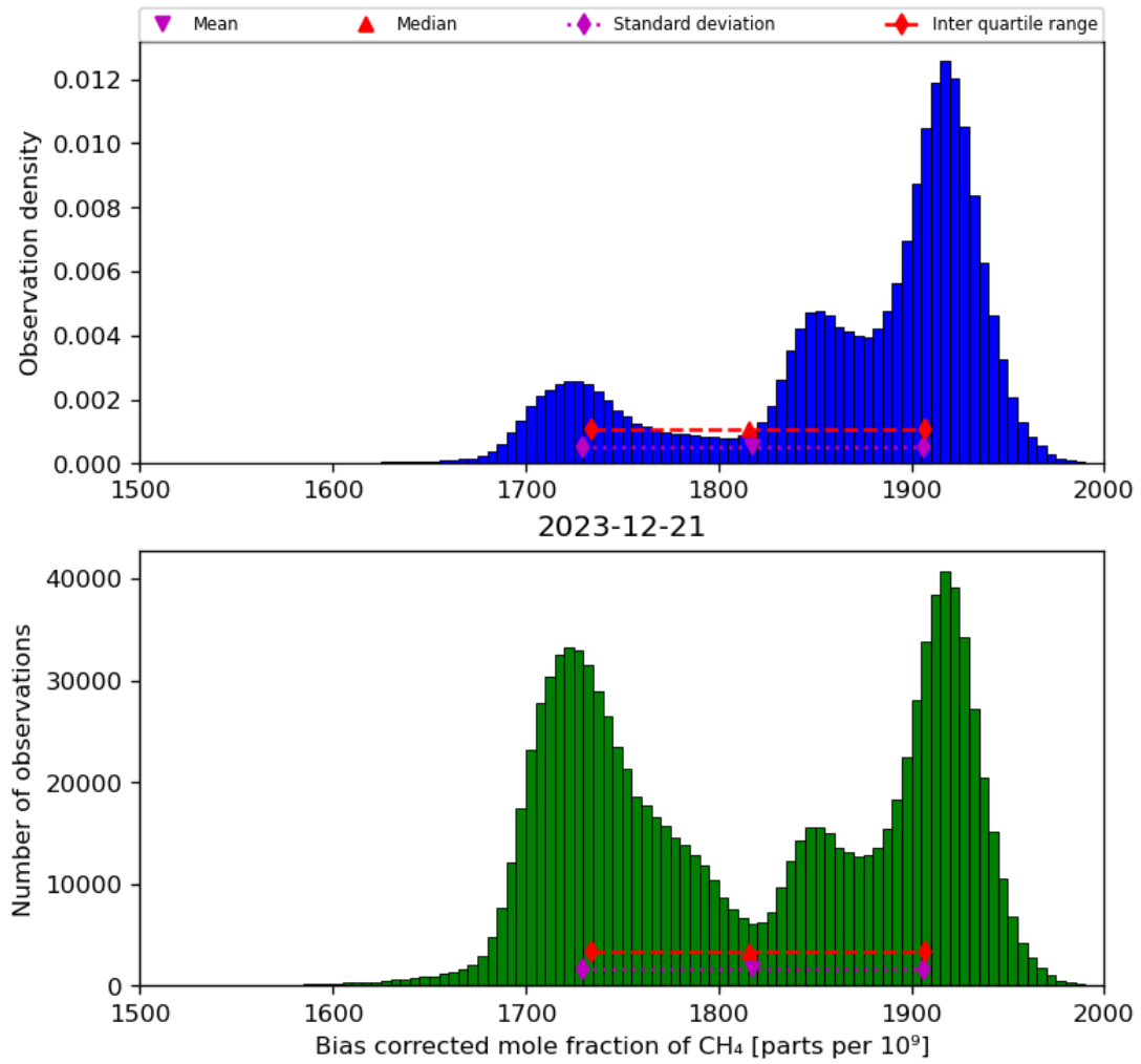
Figure 25: Histogram of “Bias corrected mole fraction of CH 4 ” for 2023-12-20 to 2023-12-22
