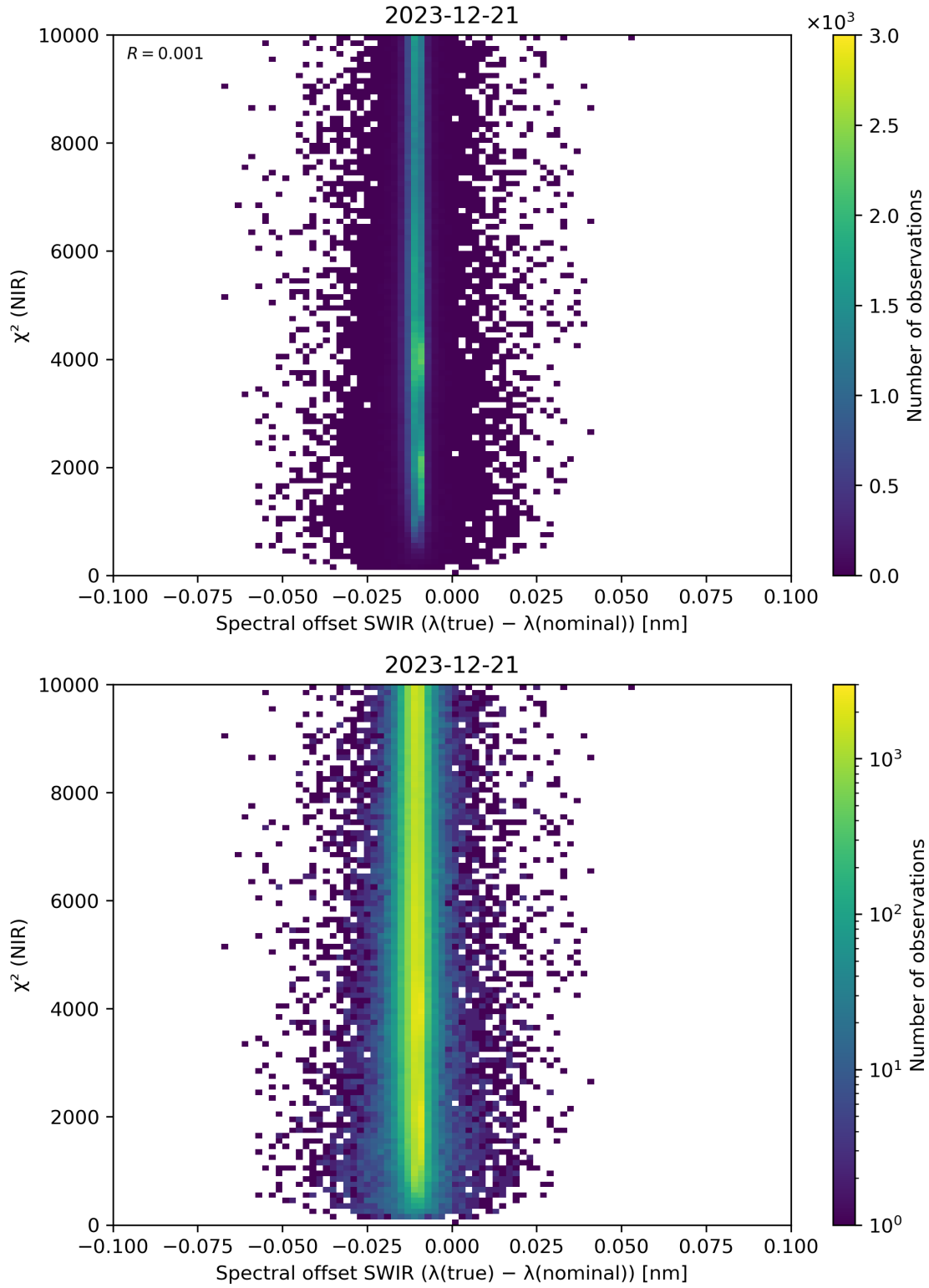
Figure 117: Scatter density plot of “Spectral offset SWIR ( \lambda(\text{true}) - \lambda(\text{nominal}) )” against “ \chi^2 (NIR)” for 2023-12-20 to 2023-12-22.
