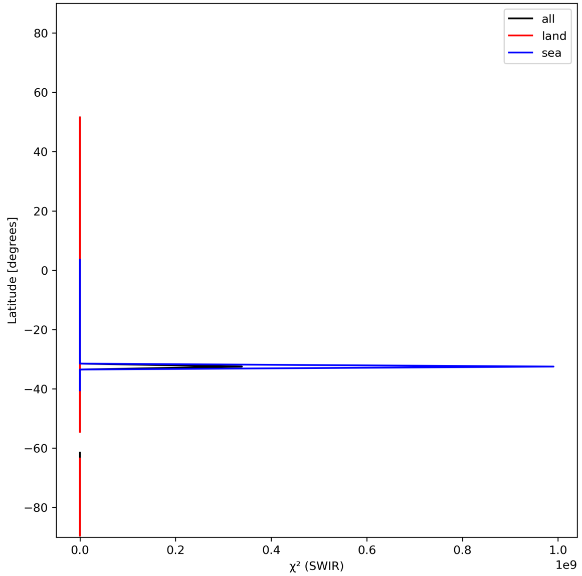
Figure 17: Zonal average of “ \chi^2 (SWIR)” for 2023-12-20 to 2023-12-22.
