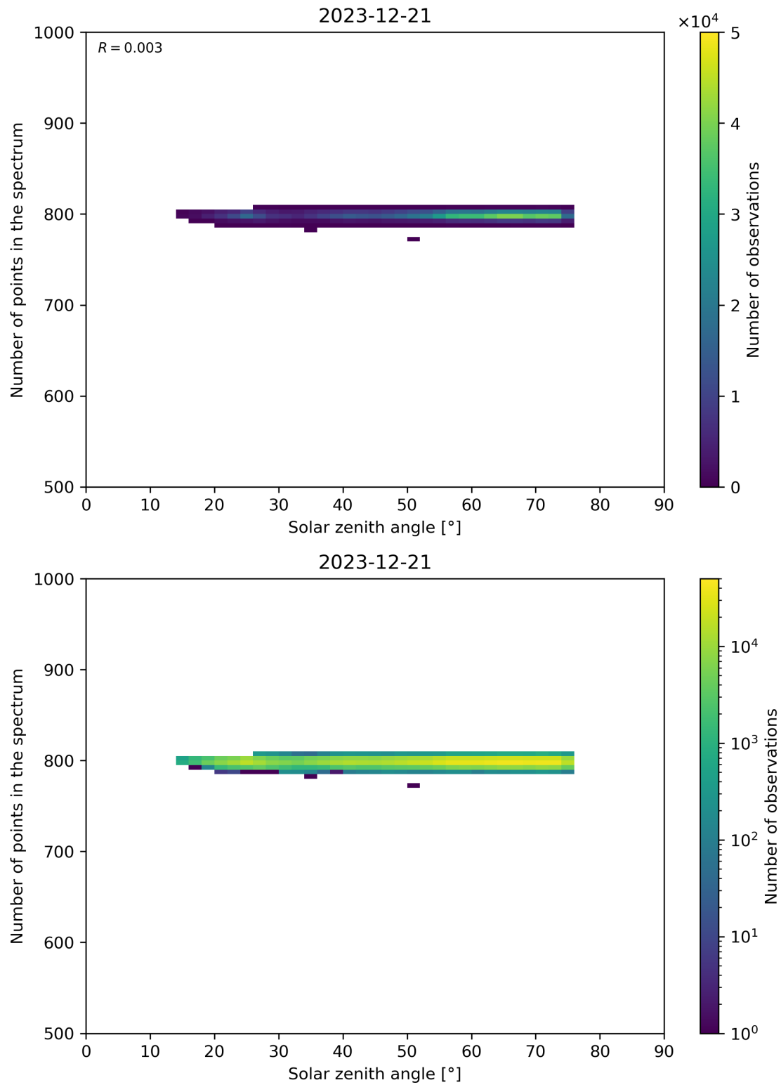
Figure 103: Scatter density plot of “Solar zenith angle” against “Number of points in the spectrum” for 2023-12-20 to 2023-12-22.
