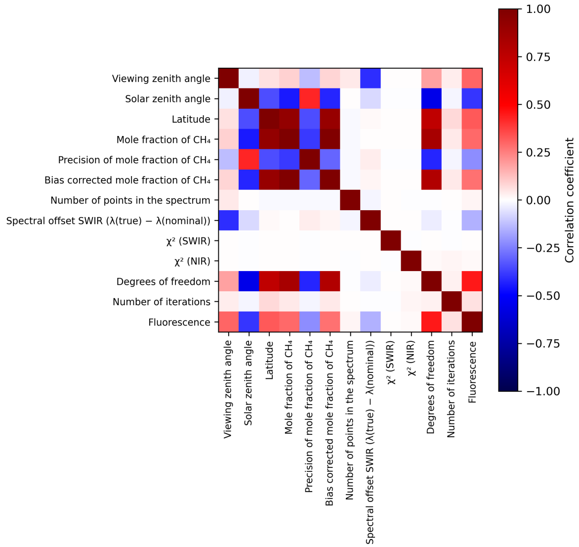
Figure 2: Map of correlation matrix for 2023-12-20 to 2023-12-22.
