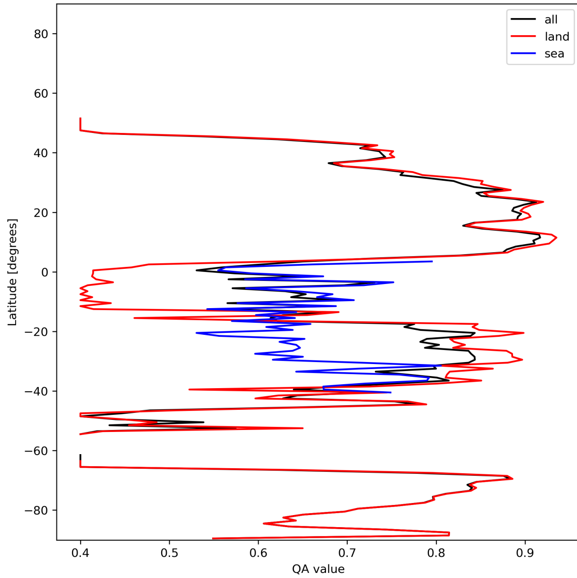
Figure 11: Zonal average of “QA value” for 2023-12-20 to 2023-12-22.
