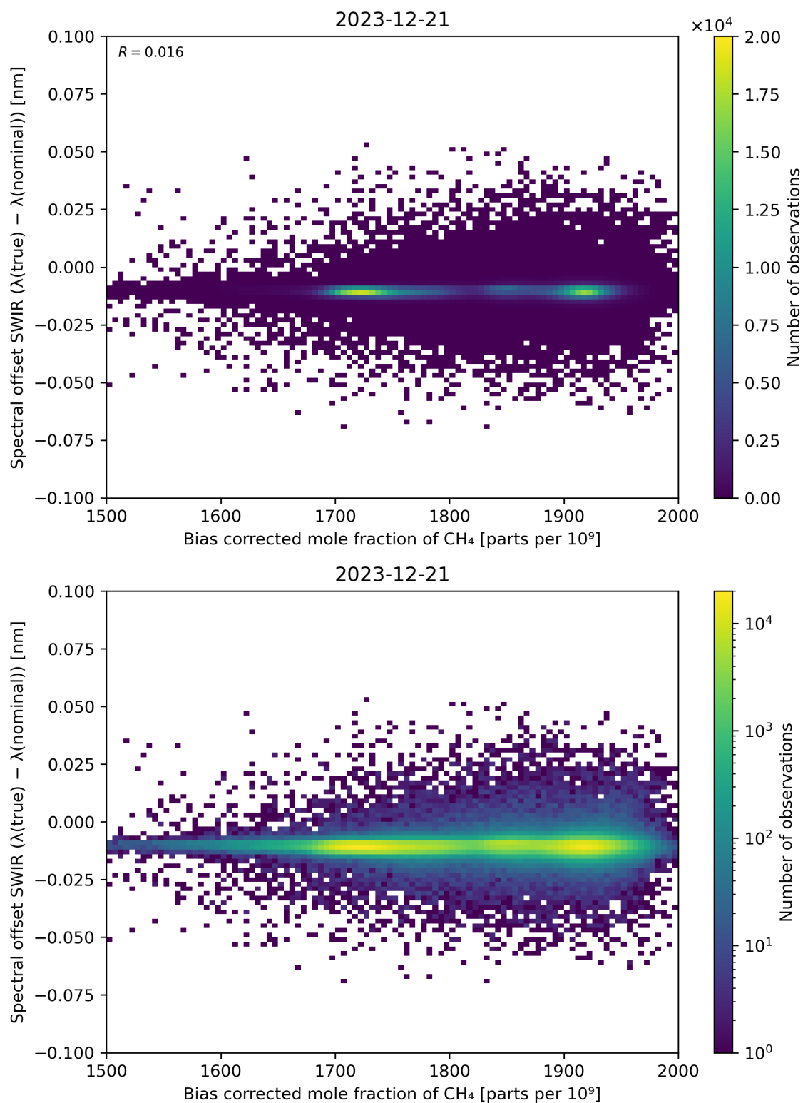
Figure 69: Scatter density plot of “Bias corrected mole fraction of \text{CH}_4 ” against “Spectral offset SWIR ( \lambda(\text{true}) - \lambda(\text{nominal}) )” for 2023-12-20 to 2023-12-22.
