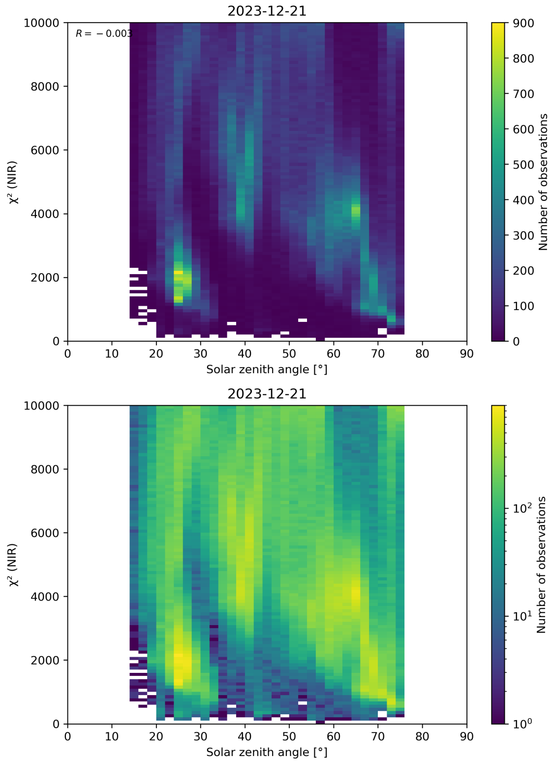
Figure 94: Scatter density plot of “Solar zenith angle” against “ \chi^2 (NIR)” for 2023-12-20 to 2023-12-22.
