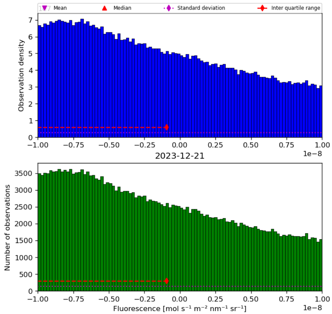
Figure 32: Histogram of “Fluorescence” for 2023-12-20 to 2023-12-22
