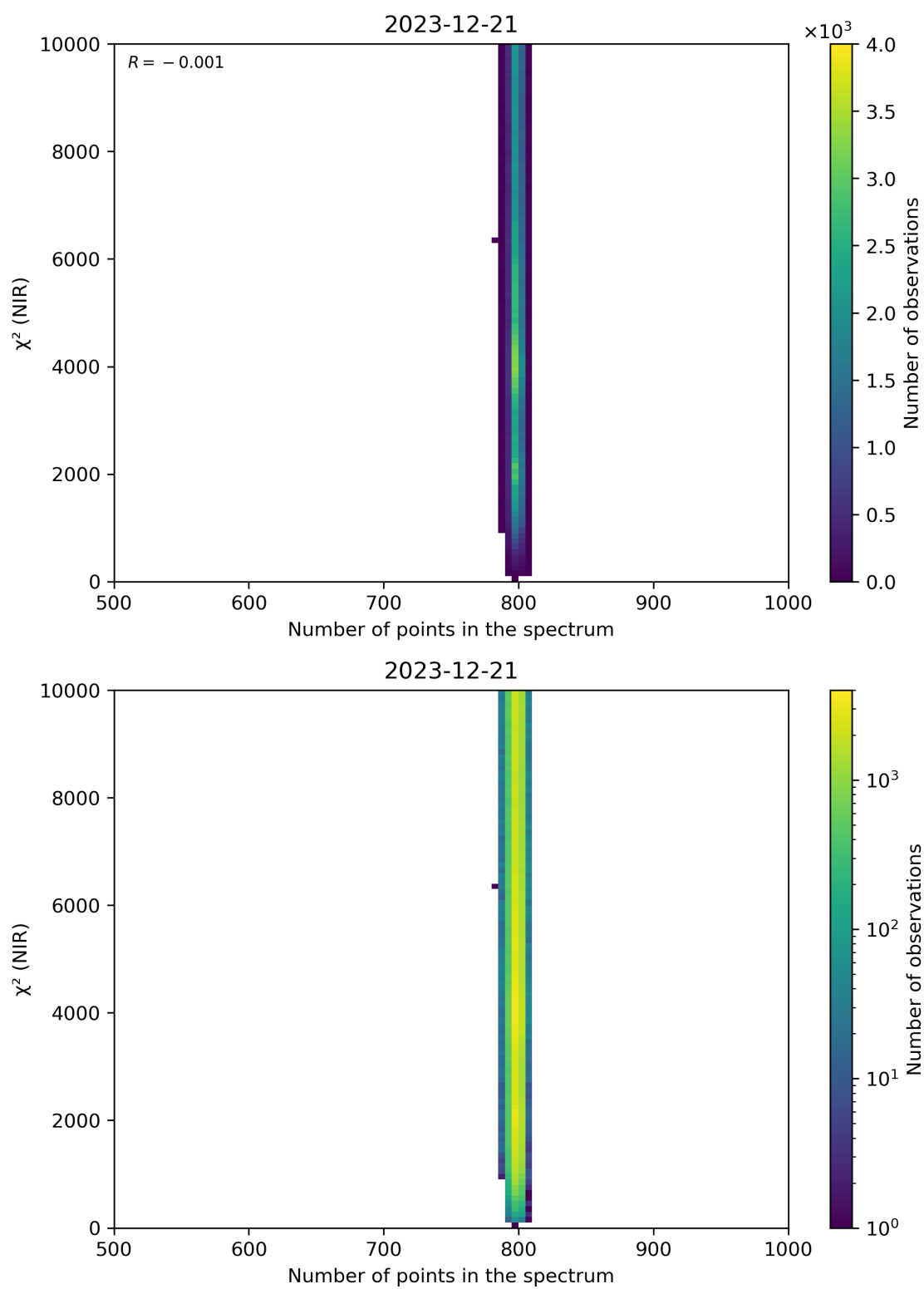
Figure 88: Scatter density plot of “Number of points in the spectrum” against “ \chi^2 (NIR)” for 2023-12-20 to 2023-12-22.
