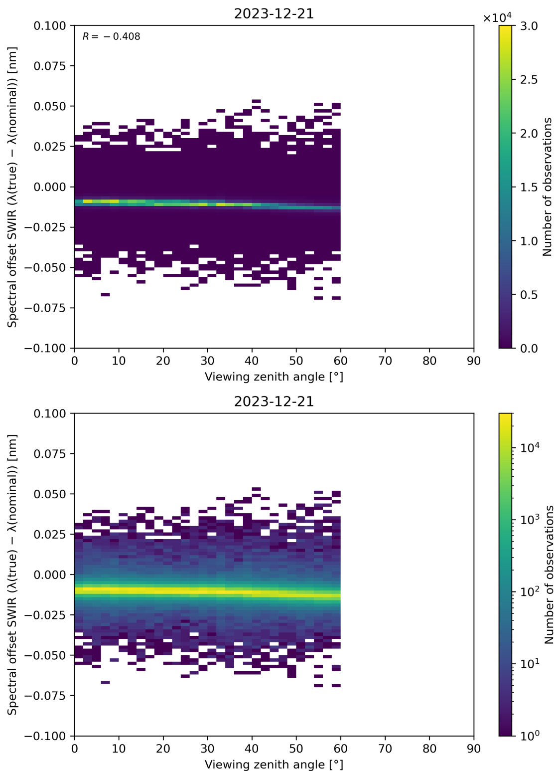
Figure 116: Scatter density plot of “Viewing zenith angle” against “Spectral offset SWIR ( \lambda(\text{true}) - \lambda(\text{nominal}) )” for 2023-12-20 to 2023-12-22.
