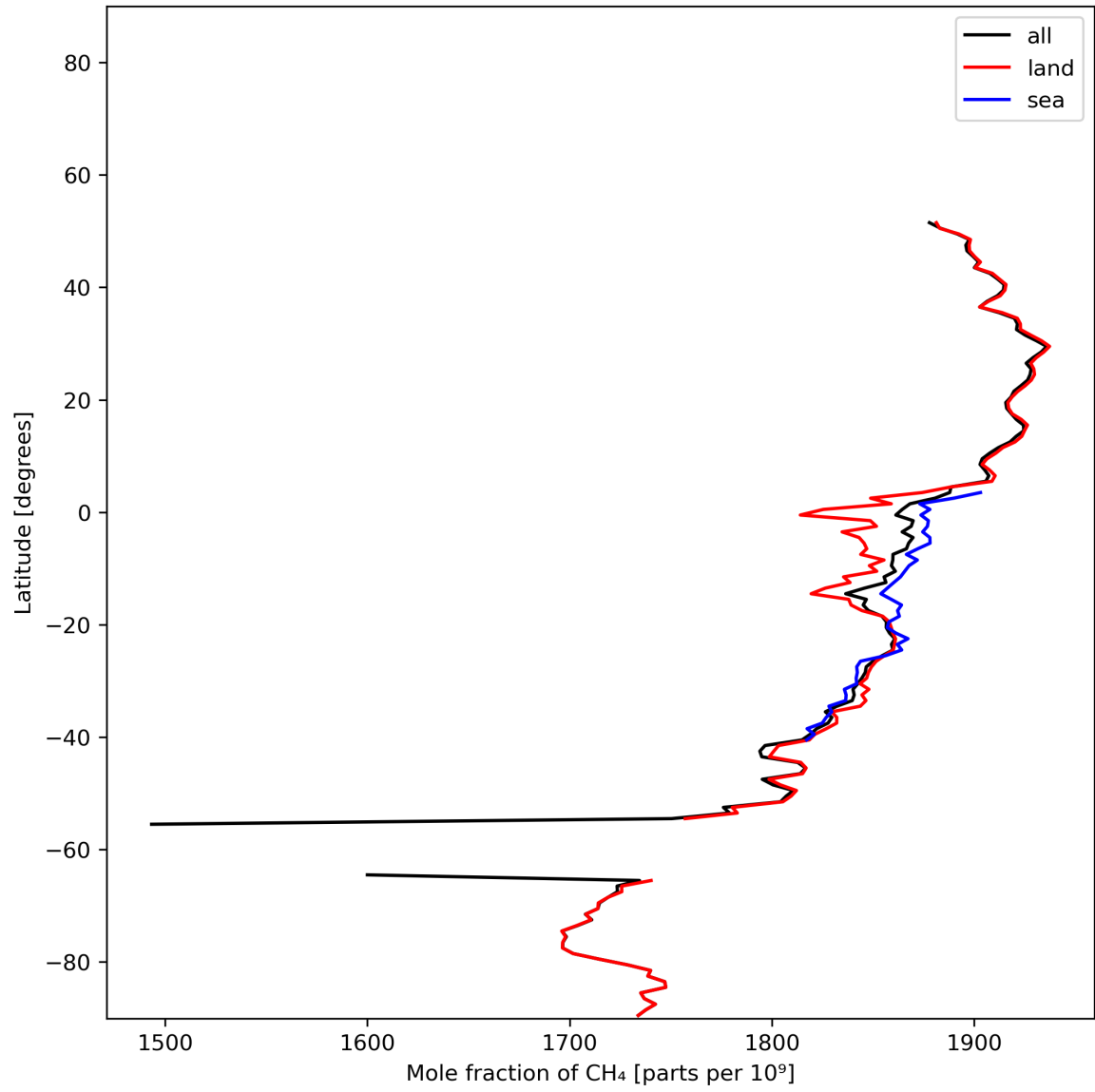
Figure 12: Zonal average of “Mole fraction of \text{CH}_4 ” for 2023-12-21 to 2023-12-23.
