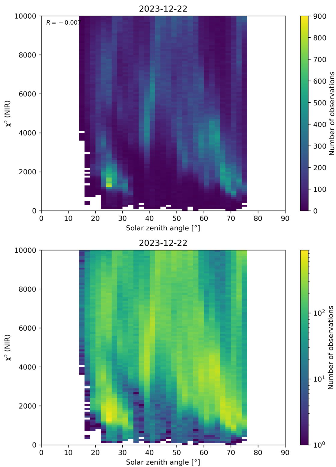
Figure 94: Scatter density plot of “Solar zenith angle” against “ \chi^2 (NIR)” for 2023-12-21 to 2023-12-23.
