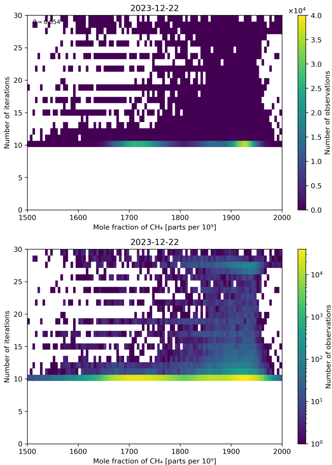
Figure 76: Scatter density plot of “Mole fraction of CH 4 ” against “Number of iterations” for 2023-12-21 to 2023-12-23.
