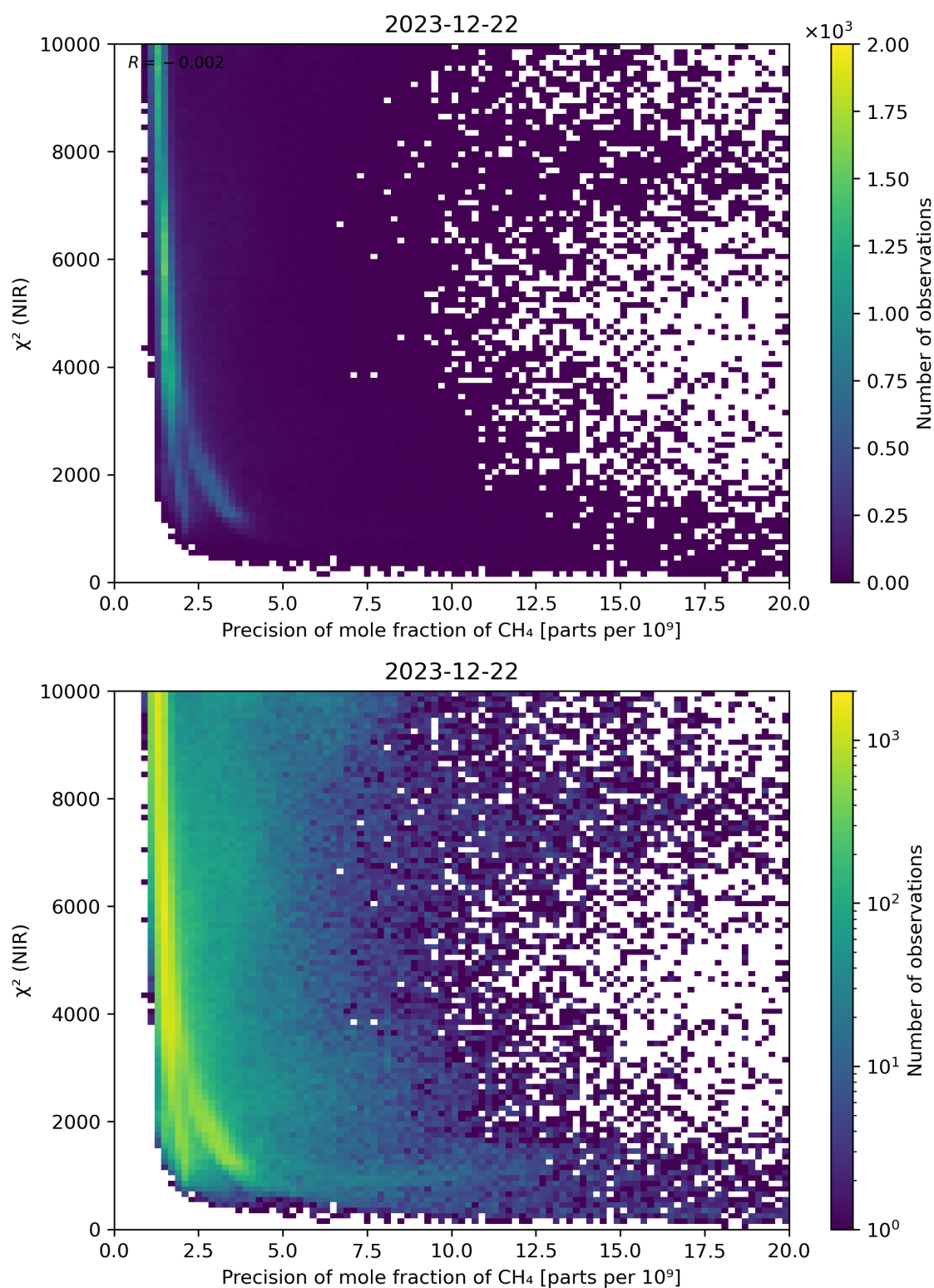
Figure 78: Scatter density plot of “Precision of mole fraction of \text{CH}_4 ” against “ \chi^2 (NIR)” for 2023-12-21 to 2023-12-23.
