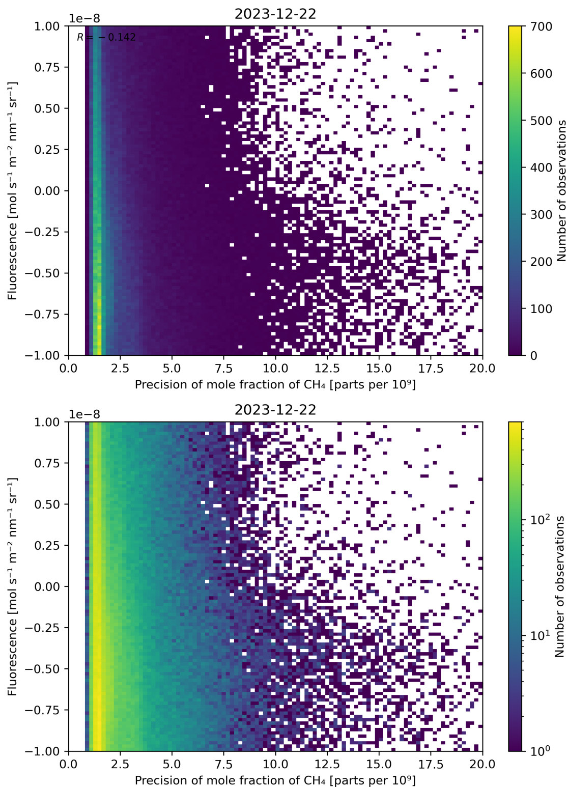
Figure 81: Scatter density plot of “Precision of mole fraction of CH 4 ” against “Fluorescence” for 2023-12-21 to 2023-12-23.
