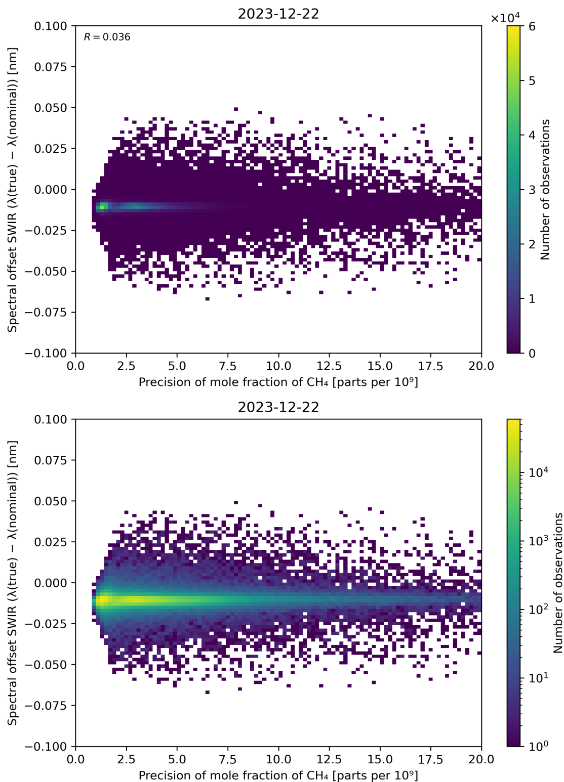
Figure 85: Scatter density plot of “Precision of mole fraction of \text{CH}_4 ” against “Spectral offset SWIR ( \lambda(\text{true}) - \lambda(\text{nominal}) )” for 2023-12-21 to 2023-12-23.
