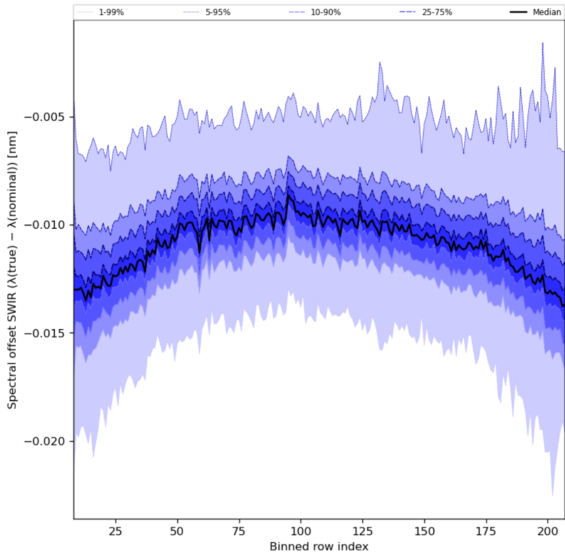
Figure 38: Along track statistics of “Spectral offset SWIR ( \lambda(\text{true}) - \lambda(\text{nominal}) )” for 2023-12-21 to 2023-12-23
