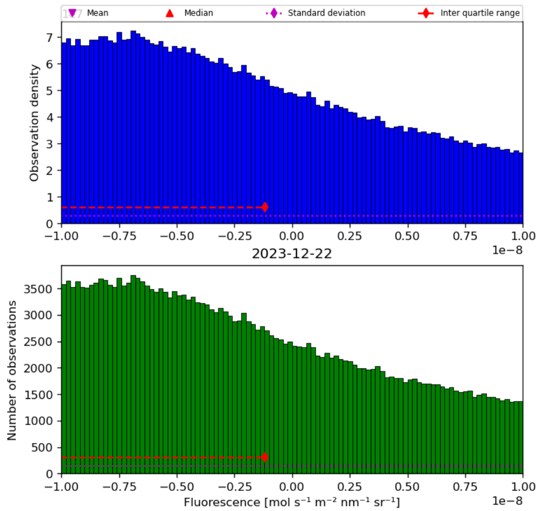
Figure 32: Histogram of “Fluorescence” for 2023-12-21 to 2023-12-23
