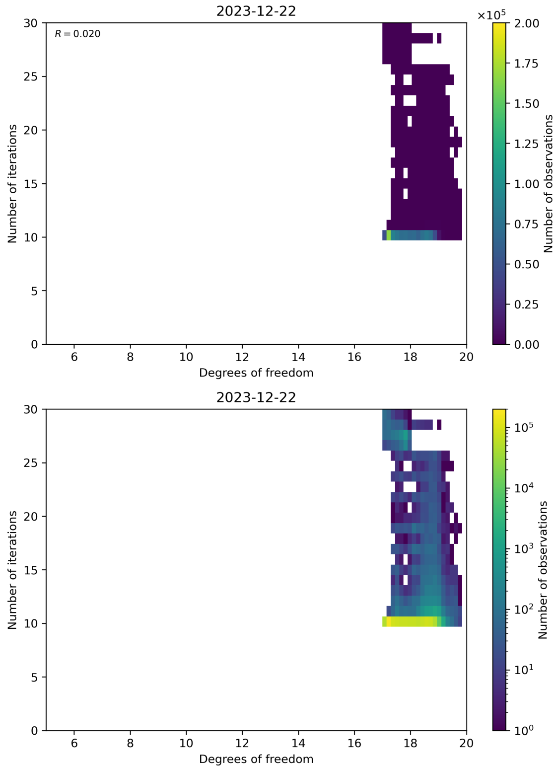
Figure 52: Scatter density plot of “Degrees of freedom” against “Number of iterations” for 2023-12-21 to 2023-12-23.
