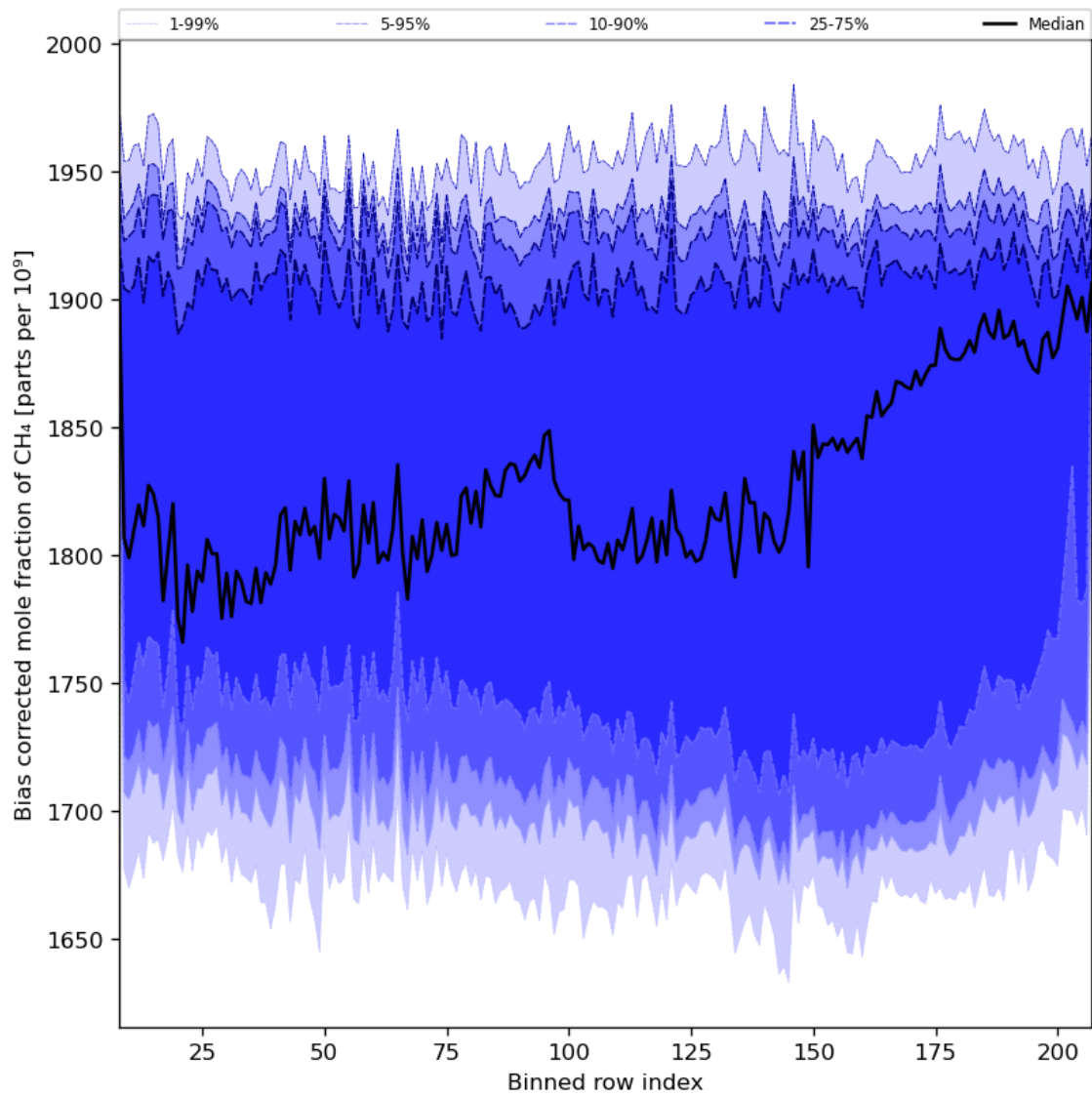
Figure 36: Along track statistics of “Bias corrected mole fraction of CH 4 ” for 2023-12-21 to 2023-12-23
