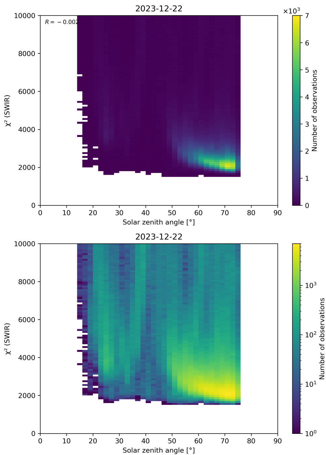
Figure 95: Scatter density plot of “Solar zenith angle” against “ \chi^2 (SWIR)” for 2023-12-21 to 2023-12-23.
