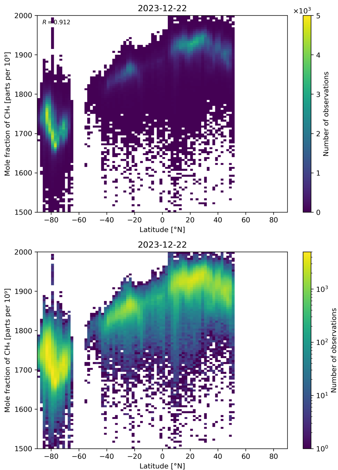
Figure 57: Scatter density plot of “Latitude” against “Mole fraction of CH 4 ” for 2023-12-21 to 2023-12-23.
