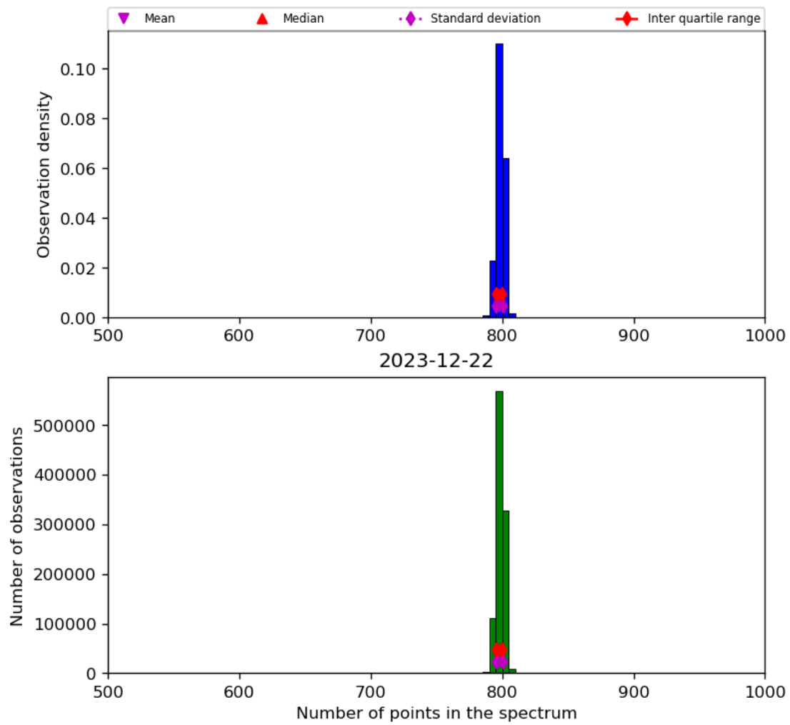
Figure 26: Histogram of “Number of points in the spectrum” for 2023-12-21 to 2023-12-23
