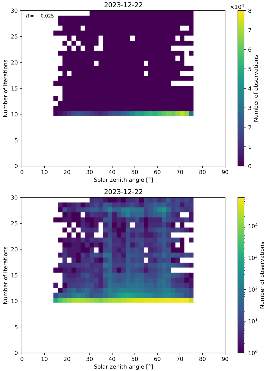
Figure 102: Scatter density plot of “Solar zenith angle” against “Number of iterations” for 2023-12-21 to 2023-12-23.
