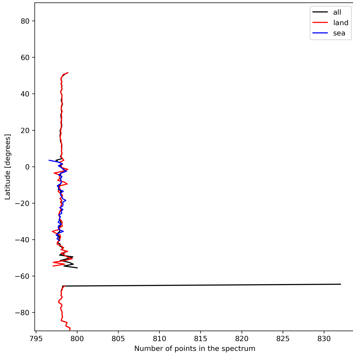
Figure 15: Zonal average of “Number of points in the spectrum” for 2023-12-21 to 2023-12-23.
