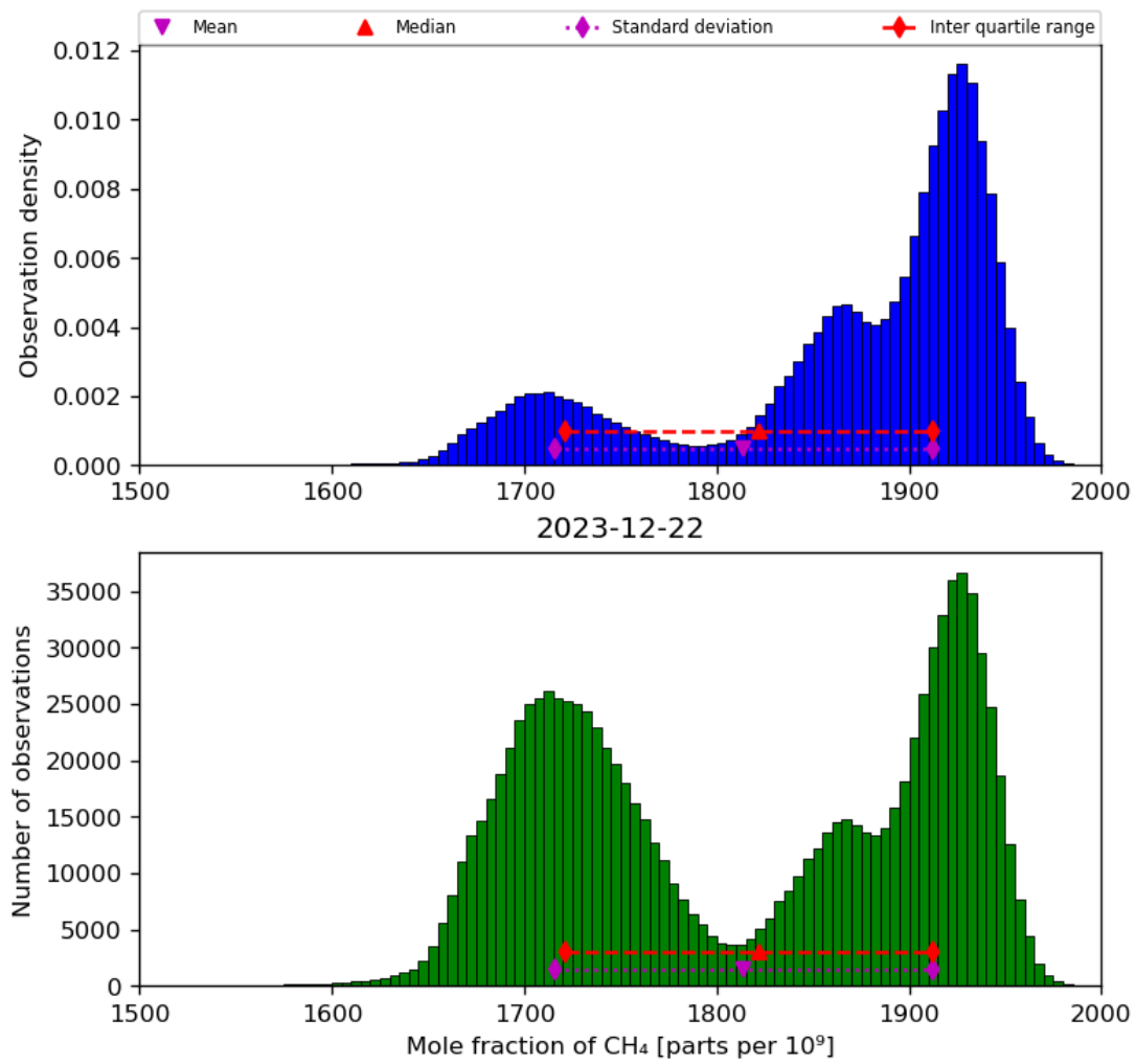
Figure 23: Histogram of “Mole fraction of CH 4 ” for 2023-12-21 to 2023-12-23
