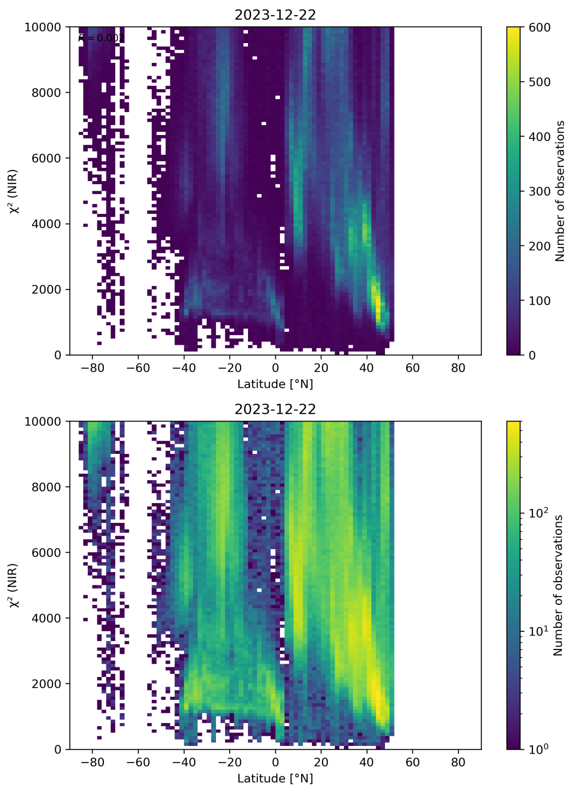
Figure 53: Scatter density plot of “Latitude” against “ \chi^2 (NIR)” for 2023-12-21 to 2023-12-23.
