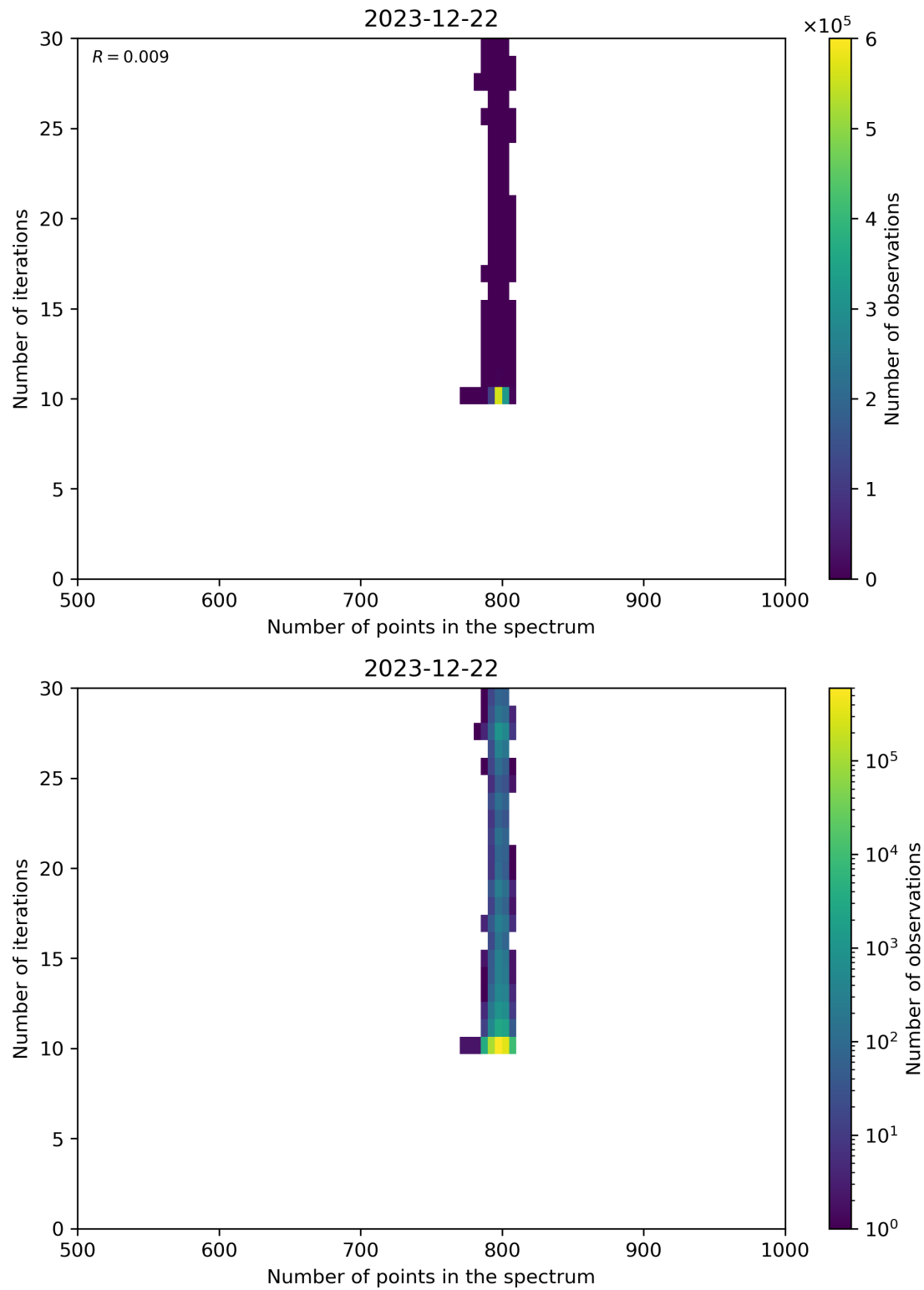
Figure 92: Scatter density plot of “Number of points in the spectrum” against “Number of iterations” for 2023-12-21 to 2023-12-23.
