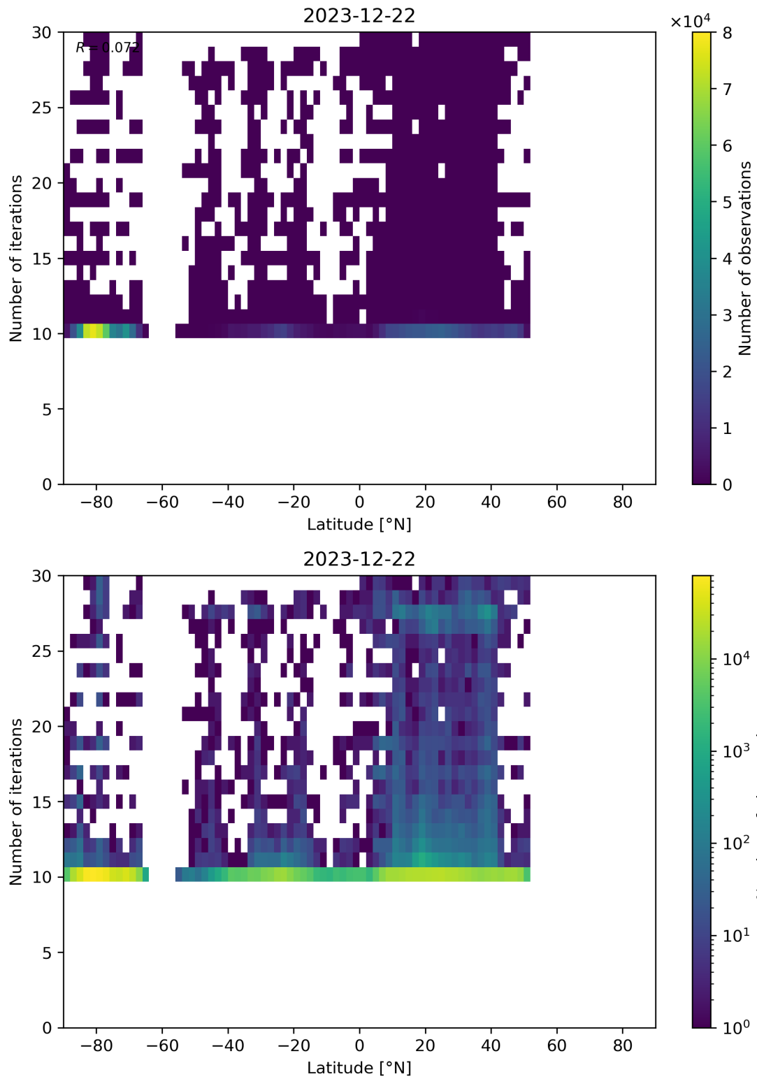
Figure 60: Scatter density plot of “Latitude” against “Number of iterations” for 2023-12-21 to 2023-12-23.
