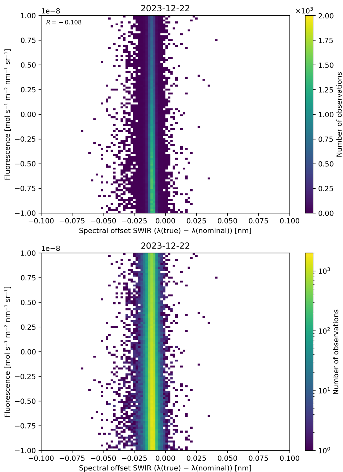
Figure 120: Scatter density plot of “Spectral offset SWIR ( \lambda(\text{true}) - \lambda(\text{nominal}) )” against “Fluorescence” for 2023-12-21 to 2023-12-23.
