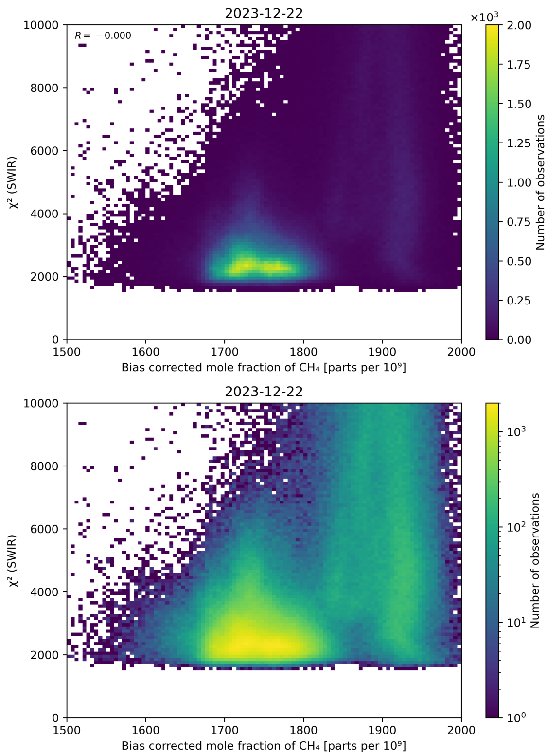
Figure 64: Scatter density plot of “Bias corrected mole fraction of CH 4 ” against “ \chi^2 (SWIR)” for 2023-12-21 to 2023-12-23.
