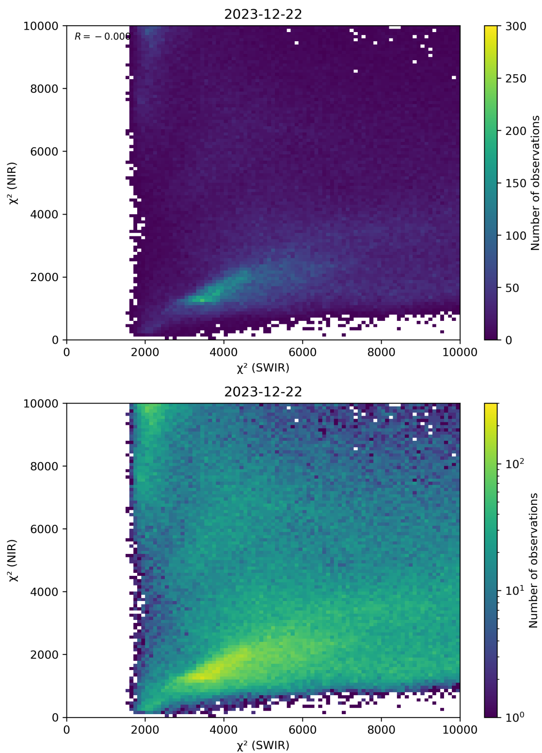
Figure 47: Scatter density plot of “ \chi^2 (SWIR)” against “ \chi^2 (NIR)” for 2023-12-21 to 2023-12-23.
