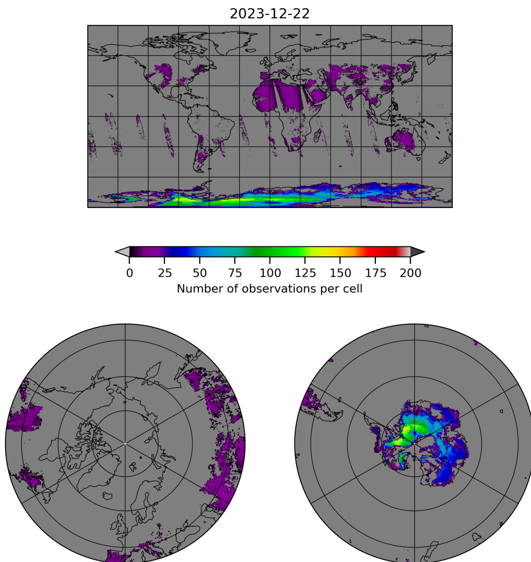
Figure 10: Map of the number of observations for 2023-12-21 to 2023-12-23
