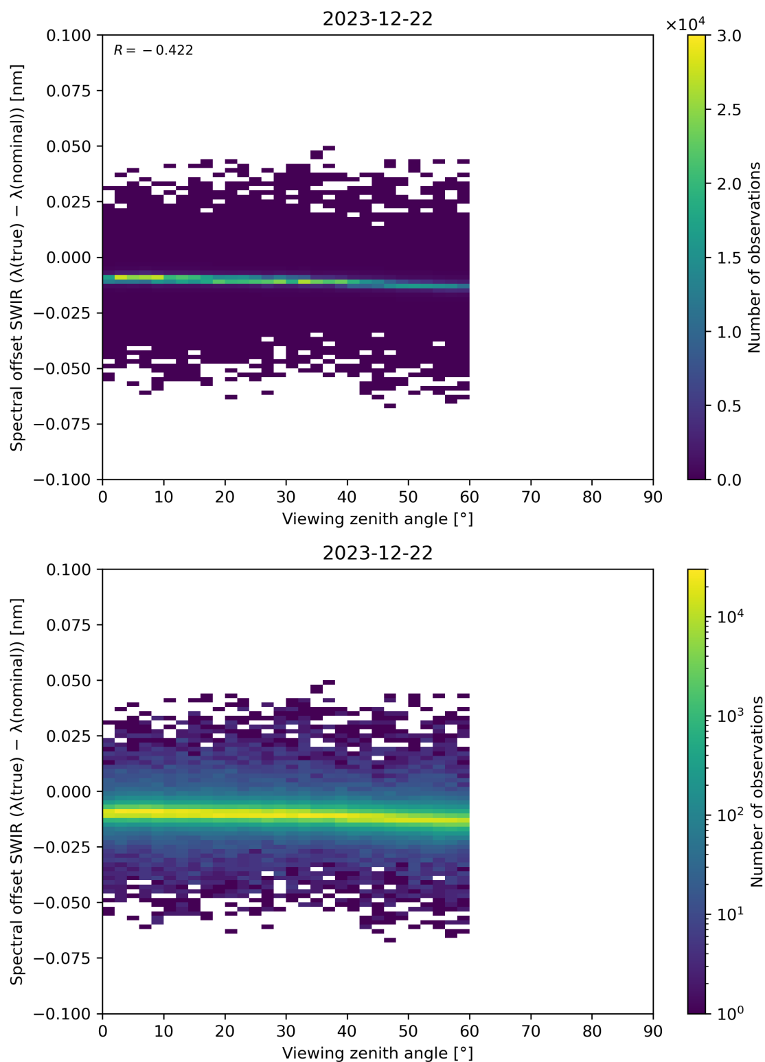
Figure 116: Scatter density plot of “Viewing zenith angle” against “Spectral offset SWIR ( \lambda(\text{true}) - \lambda(\text{nominal}) )” for 2023-12-21 to 2023-12-23.
