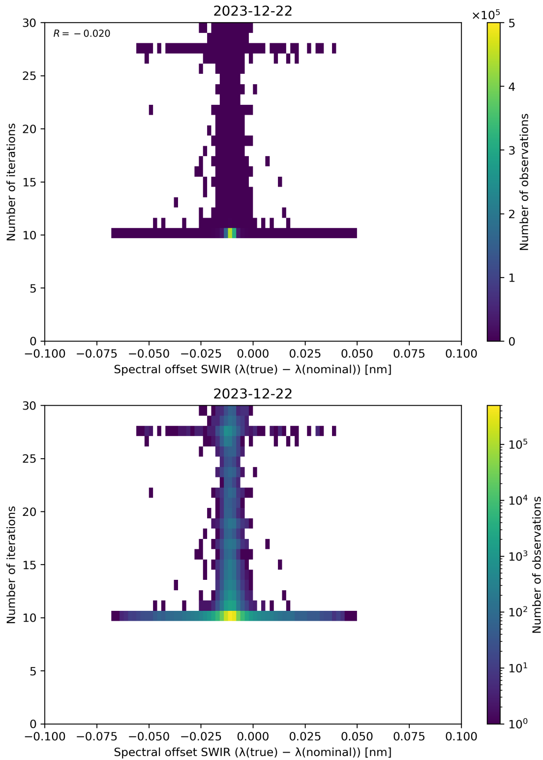
Figure 121: Scatter density plot of “Spectral offset SWIR ( \lambda(\text{true}) - \lambda(\text{nominal}) )” against “Number of iterations” for 2023-12-21 to 2023-12-23.
