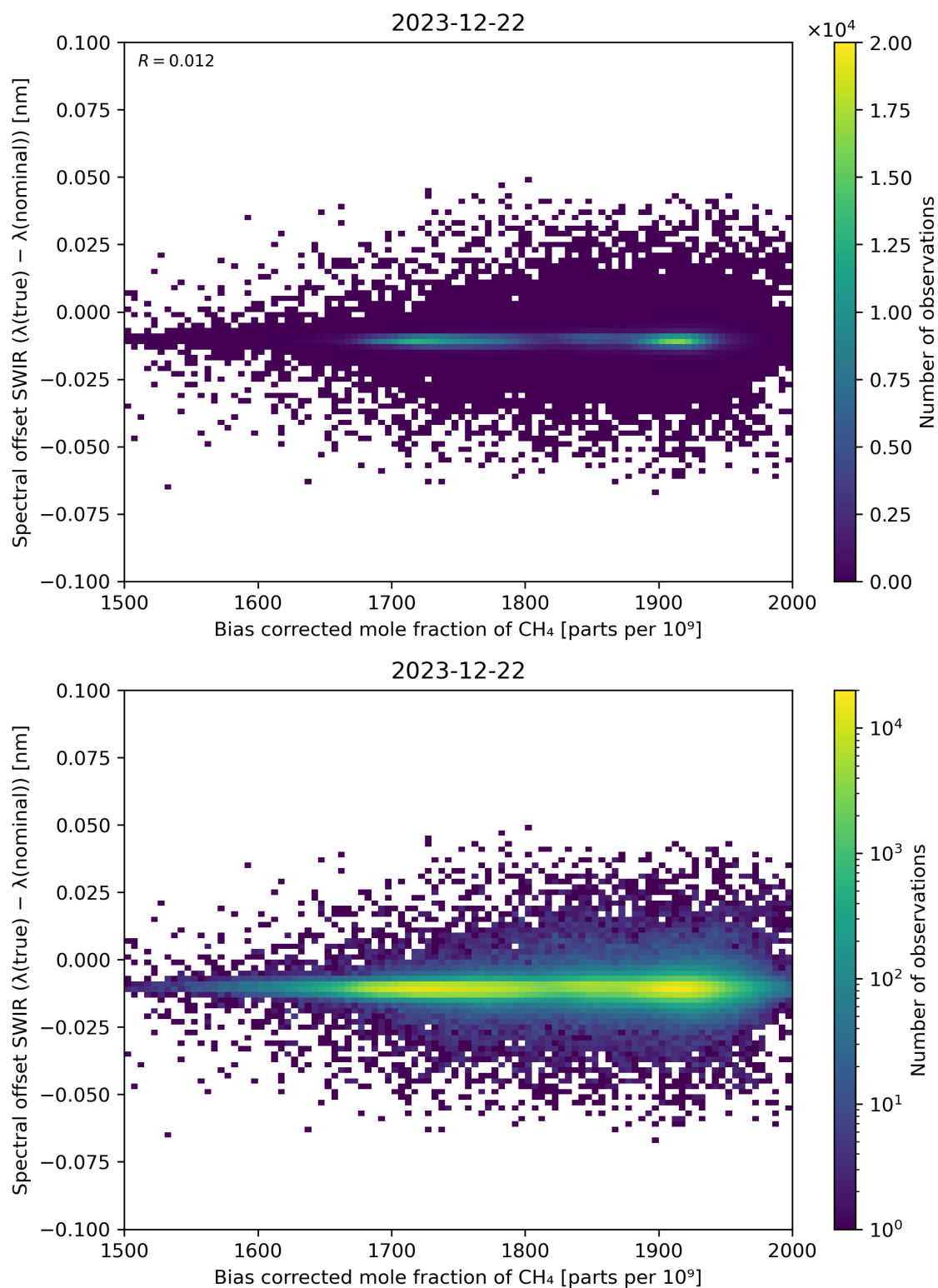
Figure 69: Scatter density plot of “Bias corrected mole fraction of \text{CH}_4 ” against “Spectral offset SWIR ( \lambda(\text{true}) - \lambda(\text{nominal}) )” for 2023-12-21 to 2023-12-23.
