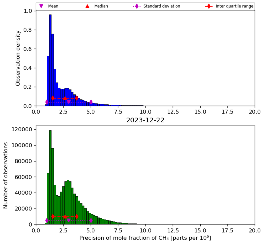
Figure 24: Histogram of “Precision of mole fraction of CH 4 ” for 2023-12-21 to 2023-12-23
