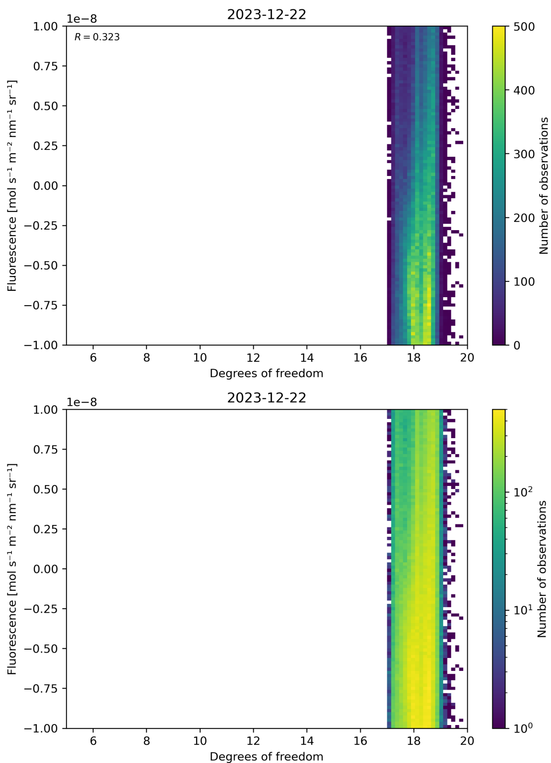
Figure 51: Scatter density plot of “Degrees of freedom” against “Fluorescence” for 2023-12-21 to 2023-12-23.
