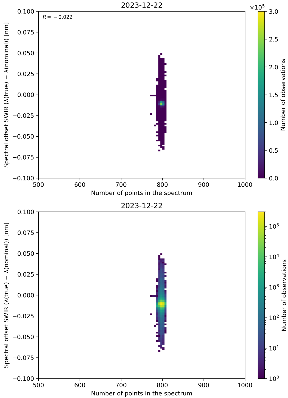
Figure 93: Scatter density plot of “Number of points in the spectrum” against “Spectral offset SWIR ( \lambda(\text{true}) - \lambda(\text{nominal}) )” for 2023-12-21 to 2023-12-23.
