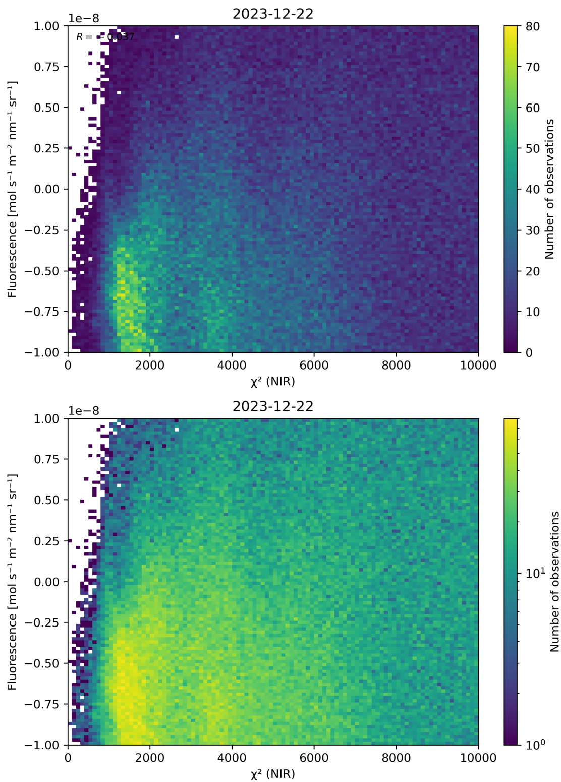
Figure 45: Scatter density plot of “ \chi^2 (NIR)” against “Fluorescence” for 2023-12-21 to 2023-12-23.
