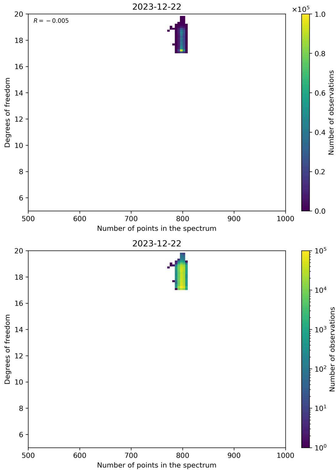
Figure 90: Scatter density plot of “Number of points in the spectrum” against “Degrees of freedom” for 2023-12-21 to 2023-12-23.
