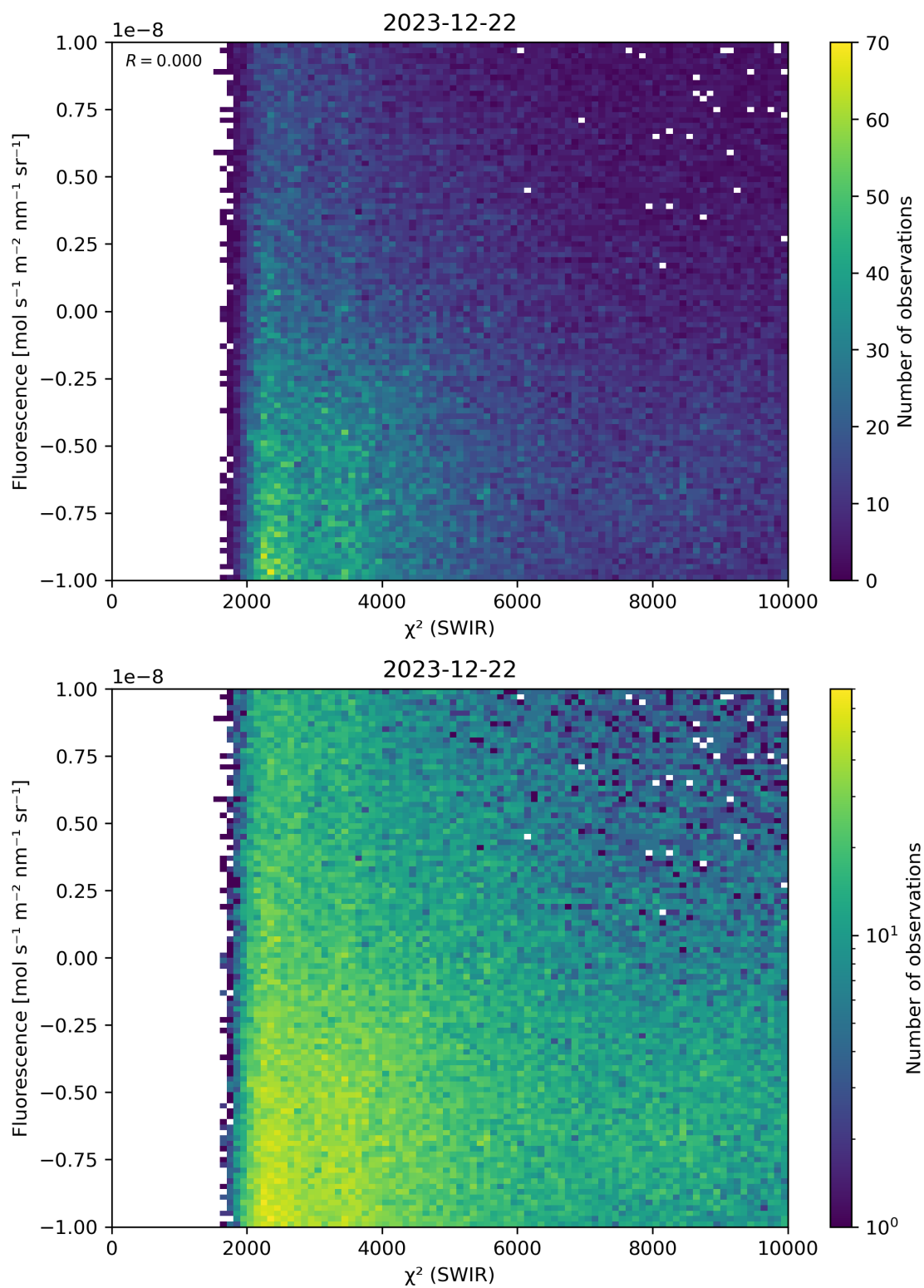
Figure 49: Scatter density plot of “ \chi^2 (SWIR)” against “Fluorescence” for 2023-12-21 to 2023-12-23.
