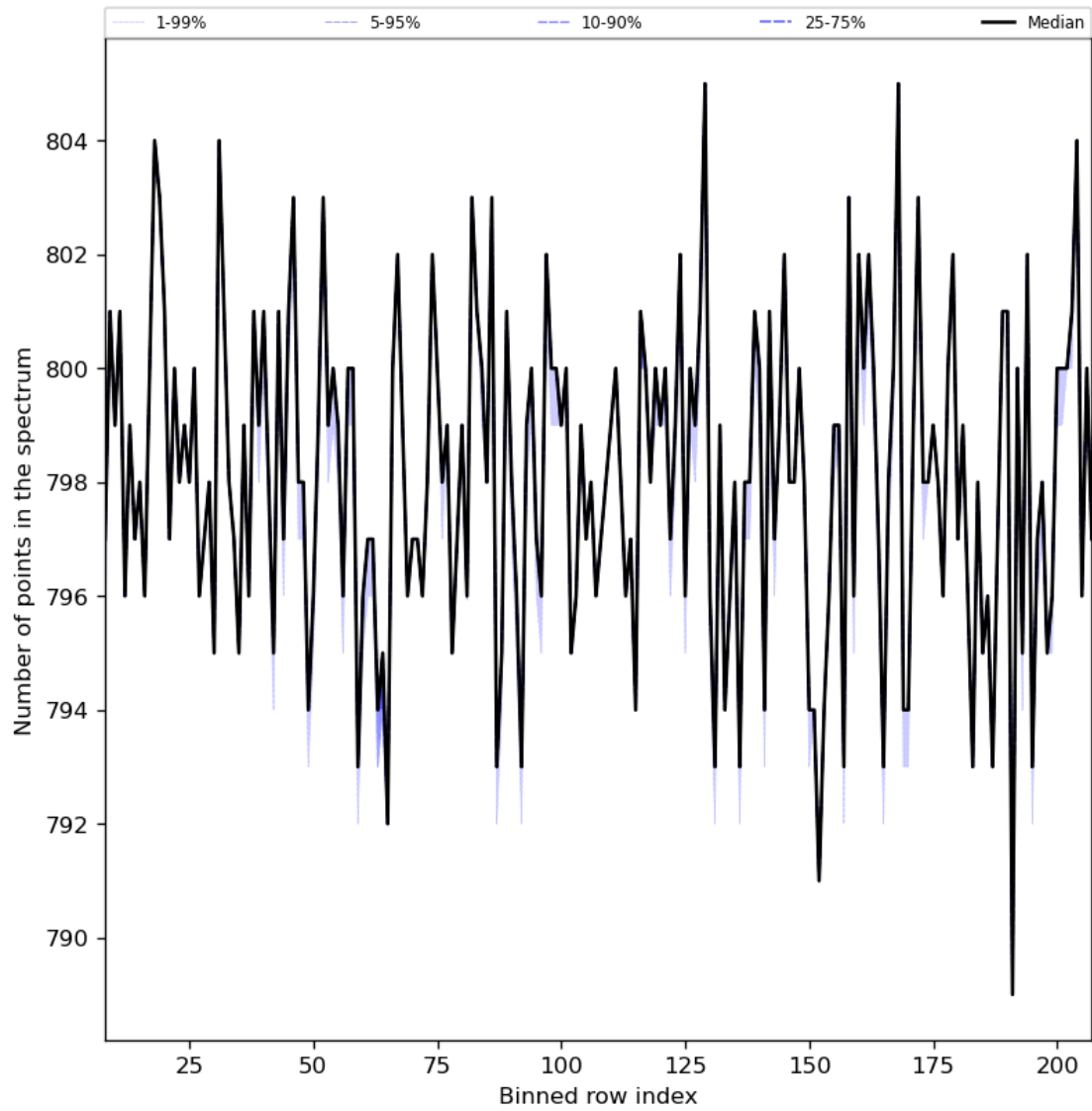
Figure 37: Along track statistics of “Number of points in the spectrum” for 2023-12-21 to 2023-12-23
