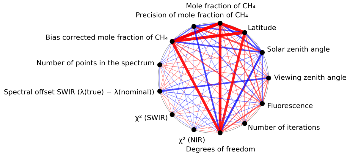
Figure 1: Map of correlation graph for 2023-12-21 to 2023-12-23.
