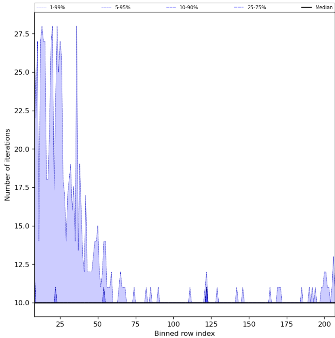
Figure 42: Along track statistics of “Number of iterations” for 2023-12-21 to 2023-12-23
