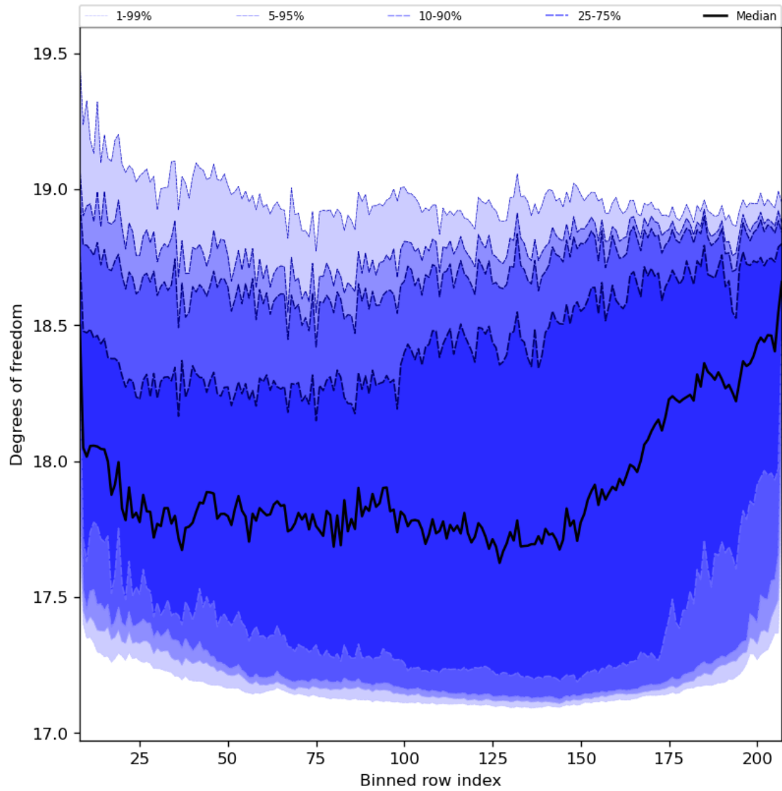
Figure 41: Along track statistics of “Degrees of freedom” for 2023-12-21 to 2023-12-23
