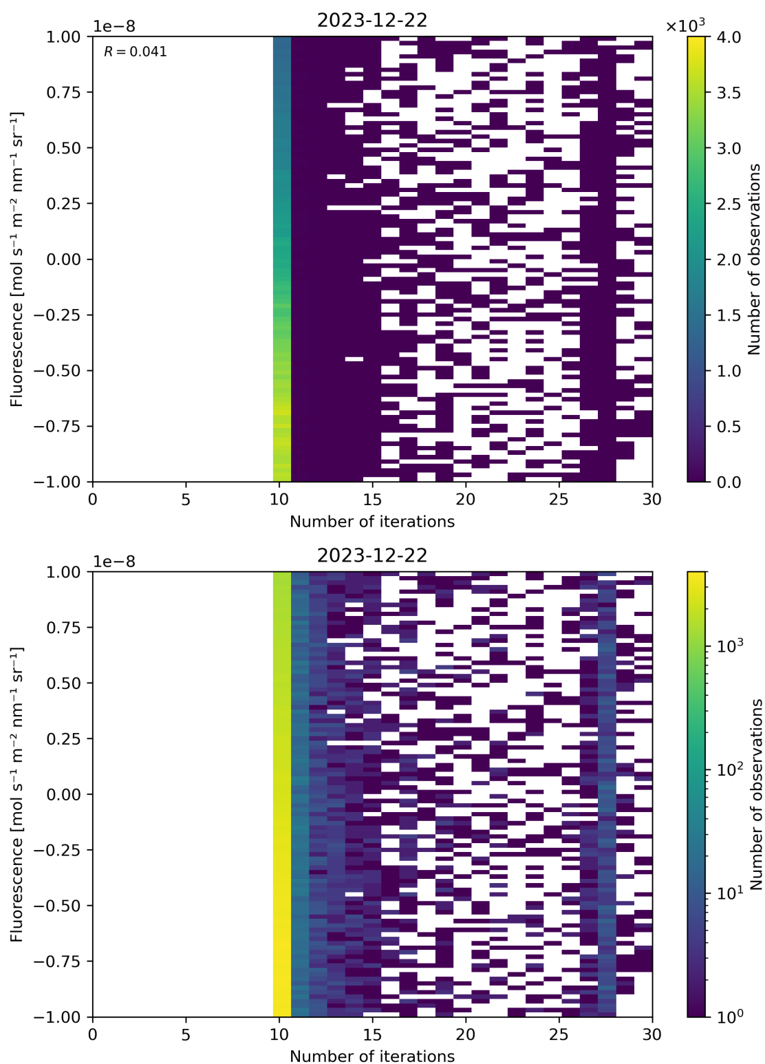
Figure 87: Scatter density plot of “Number of iterations” against “Fluorescence” for 2023-12-21 to 2023-12-23.
