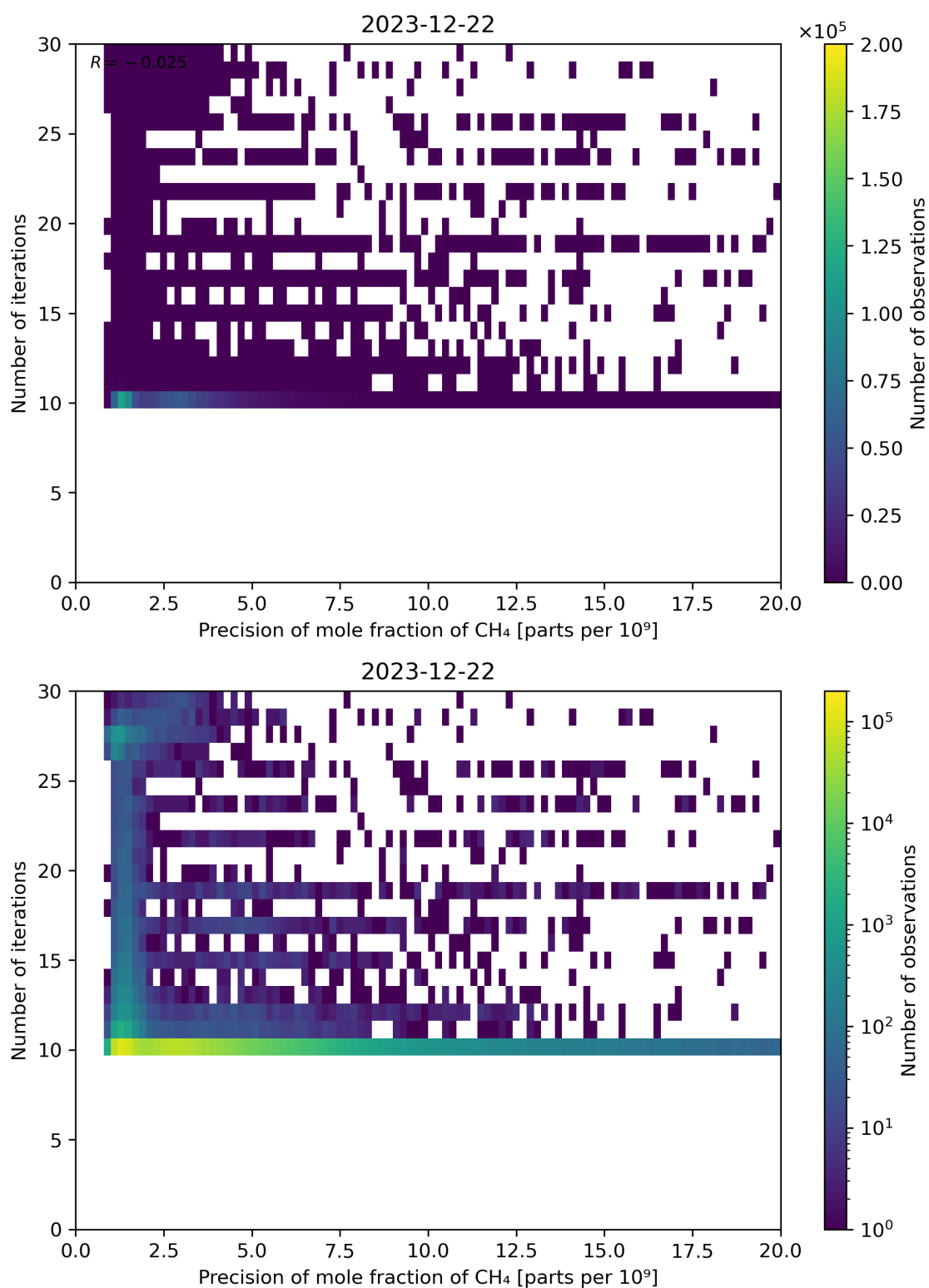
Figure 83: Scatter density plot of “Precision of mole fraction of CH 4 ” against “Number of iterations” for 2023-12-21 to 2023-12-23.
