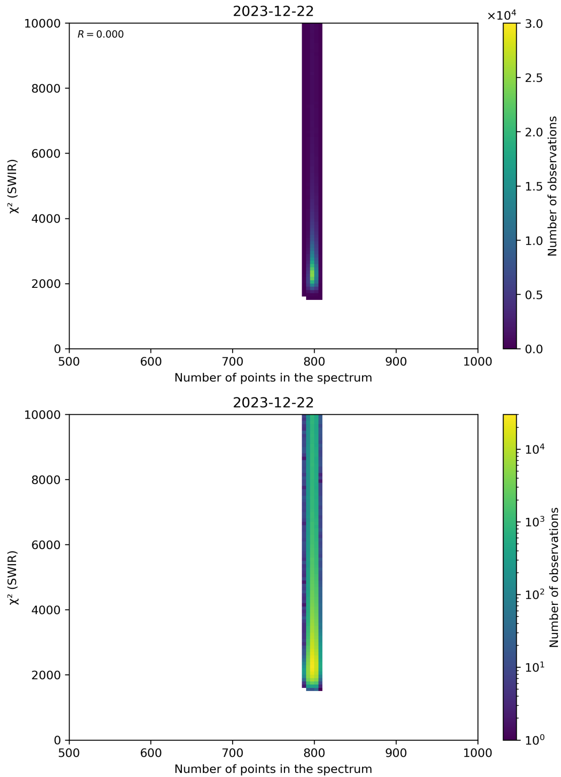
Figure 89: Scatter density plot of “Number of points in the spectrum” against “ \chi^2 (SWIR)” for 2023-12-21 to 2023-12-23.
