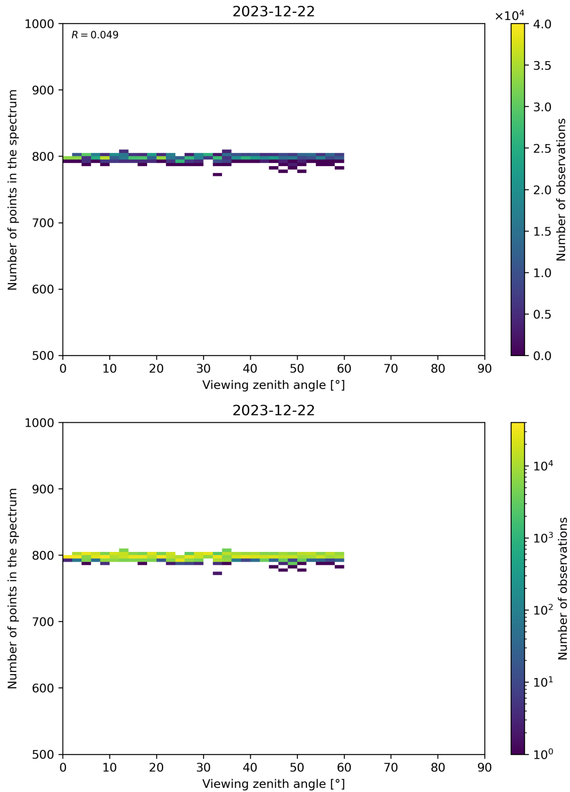
Figure 114: Scatter density plot of “Viewing zenith angle” against “Number of points in the spectrum” for 2023-12-21 to 2023-12-23.
