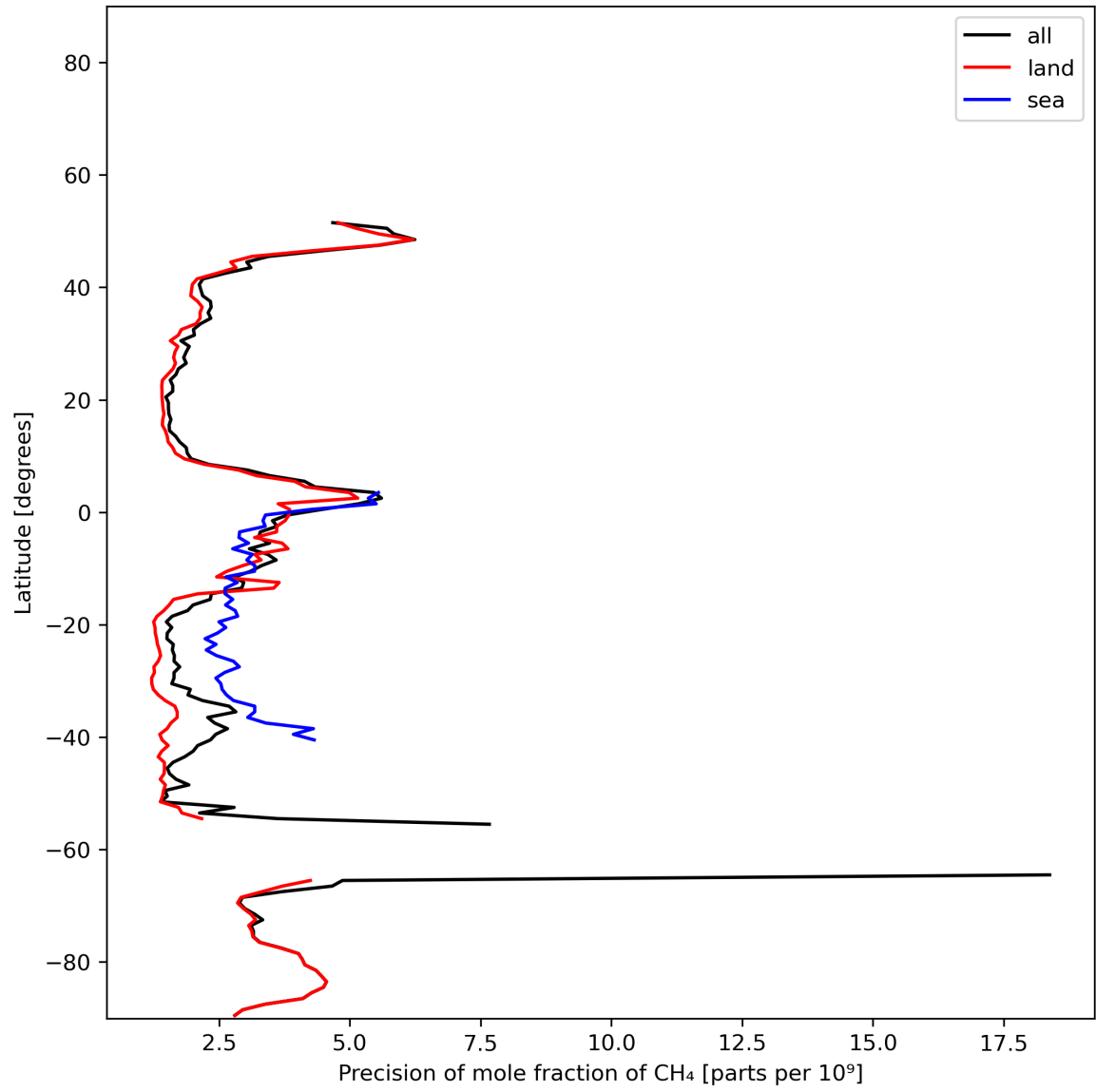
Figure 13: Zonal average of “Precision of mole fraction of CH 4 ” for 2023-12-21 to 2023-12-23.
