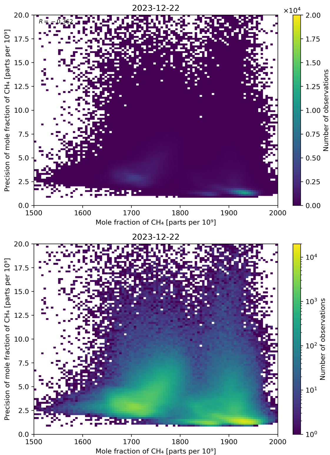
Figure 75: Scatter density plot of “Mole fraction of CH 4 ” against “Precision of mole fraction of CH 4 ” for 2023-12-21 to 2023-12-23.
