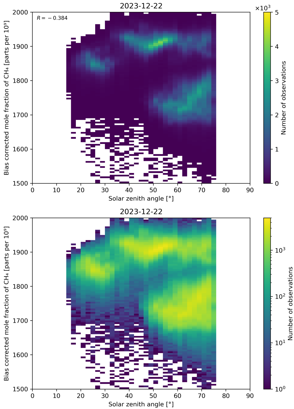
Figure 100: Scatter density plot of “Solar zenith angle” against “Bias corrected mole fraction of \text{CH}_4 ” for 2023-12-21 to 2023-12-23.
