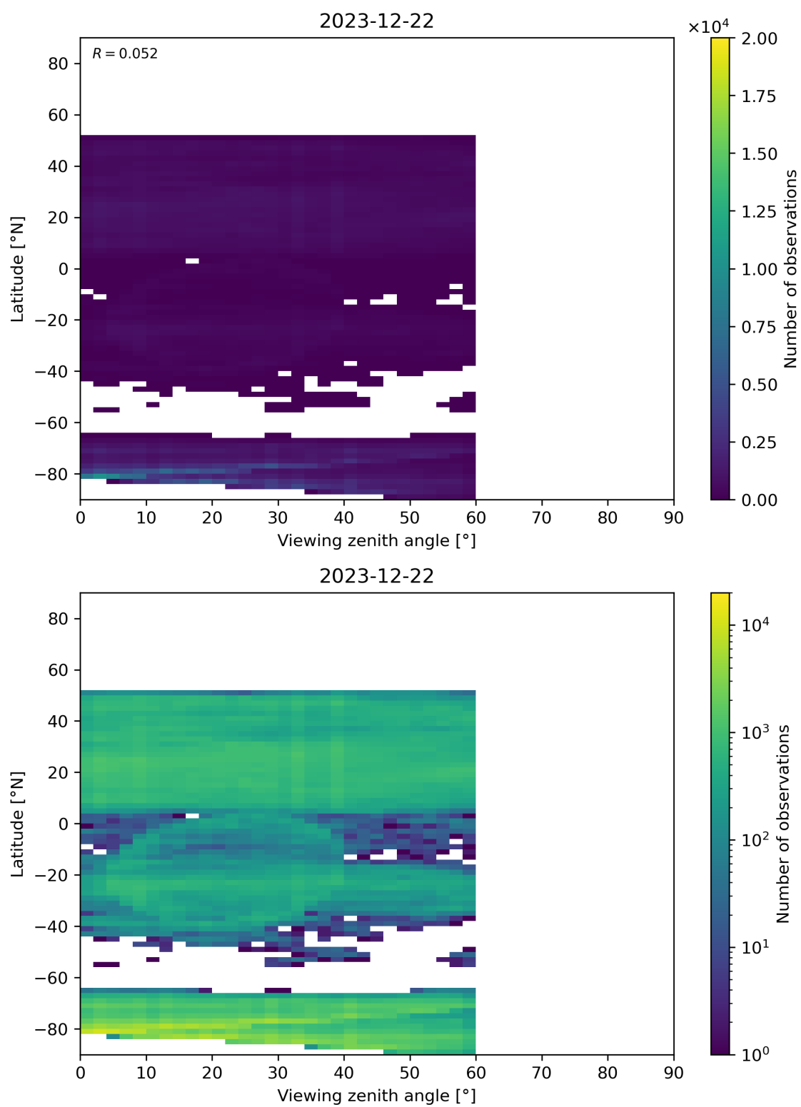
Figure 109: Scatter density plot of “Viewing zenith angle” against “Latitude” for 2023-12-21 to 2023-12-23.
