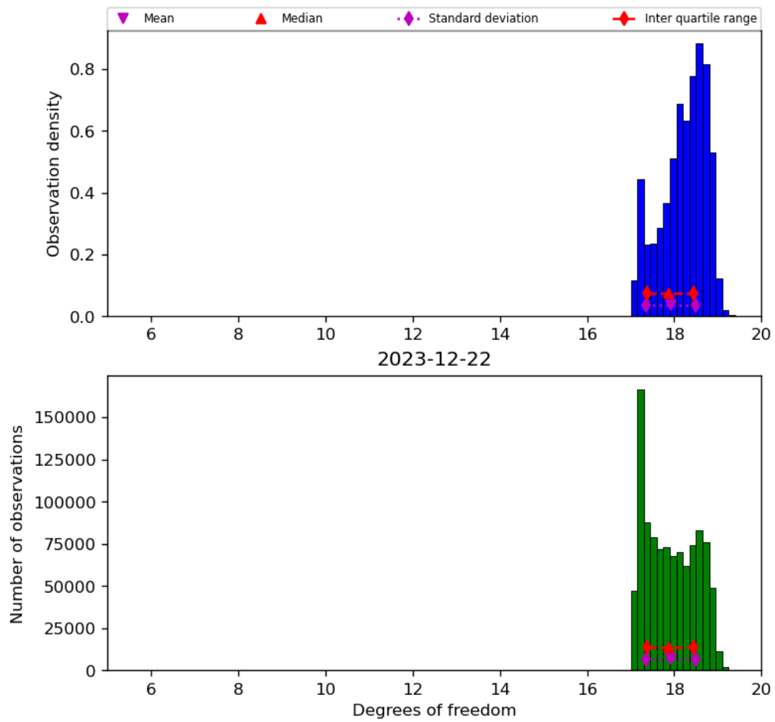
Figure 30: Histogram of “Degrees of freedom” for 2023-12-21 to 2023-12-23
