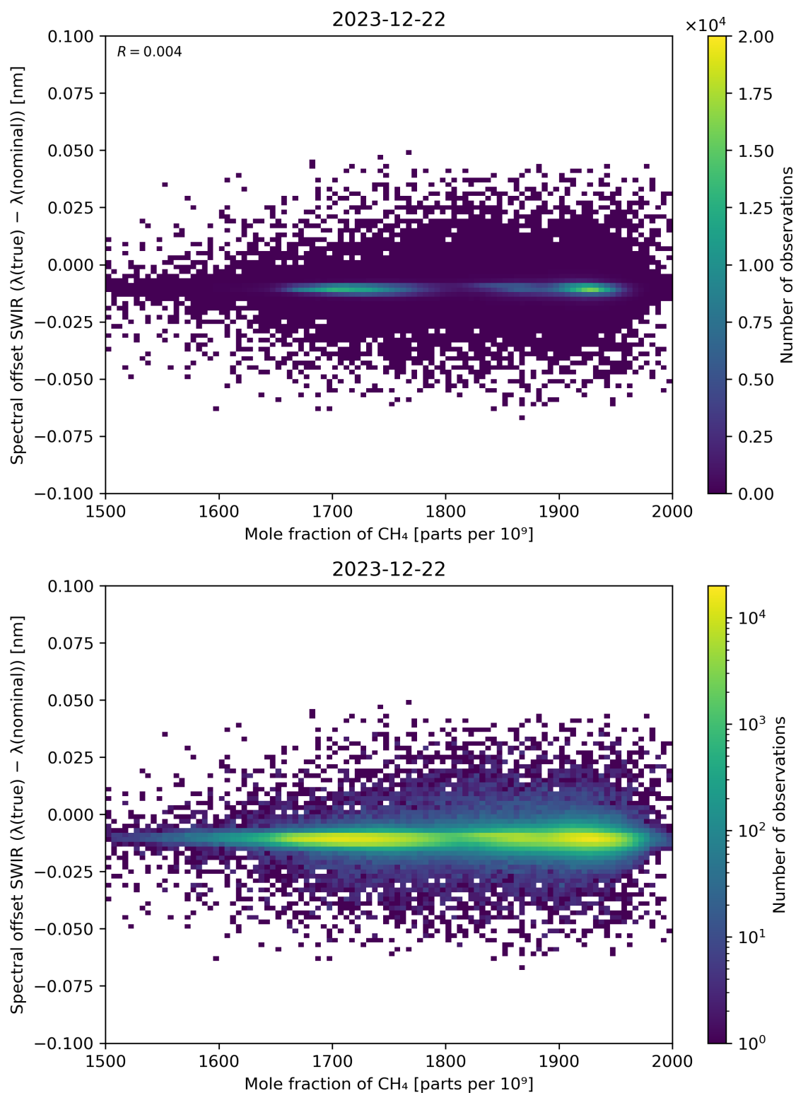
Figure 86: Scatter density plot of “Mole fraction of CH 4 ” against “Spectral offset SWIR ( \lambda(\text{true}) - \lambda(\text{nominal}) )” for 2023-12-21 to 2023-12-23.
