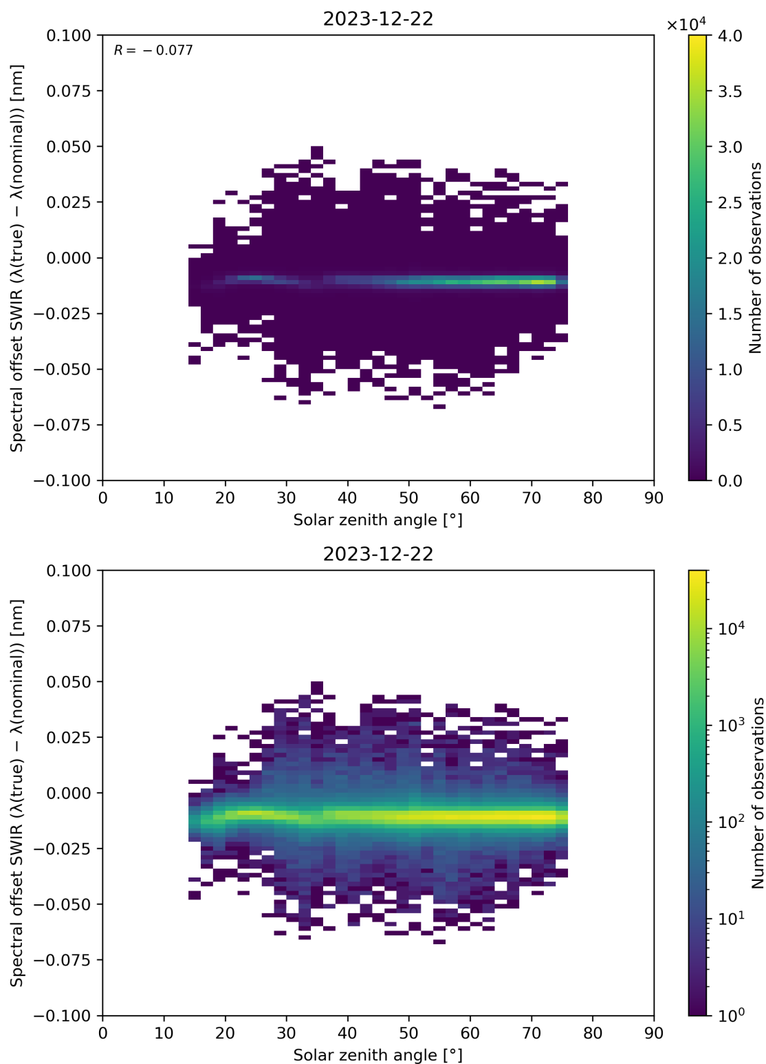
Figure 104: Scatter density plot of “Solar zenith angle” against “Spectral offset SWIR ( \lambda(\text{true}) - \lambda(\text{nominal}) )” for 2023-12-21 to 2023-12-23.
