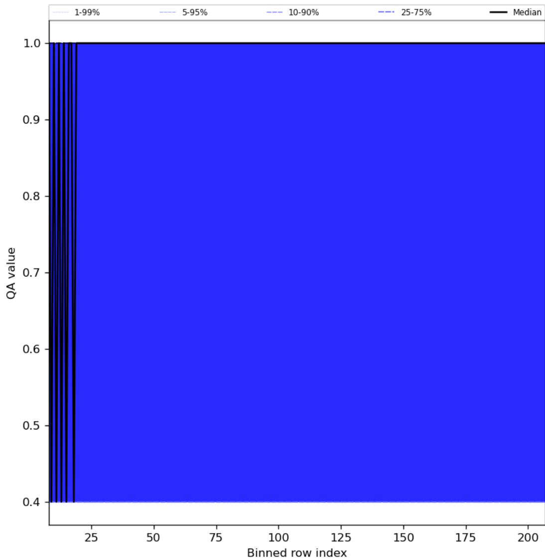
Figure 33: Along track statistics of “QA value” for 2023-12-21 to 2023-12-23
