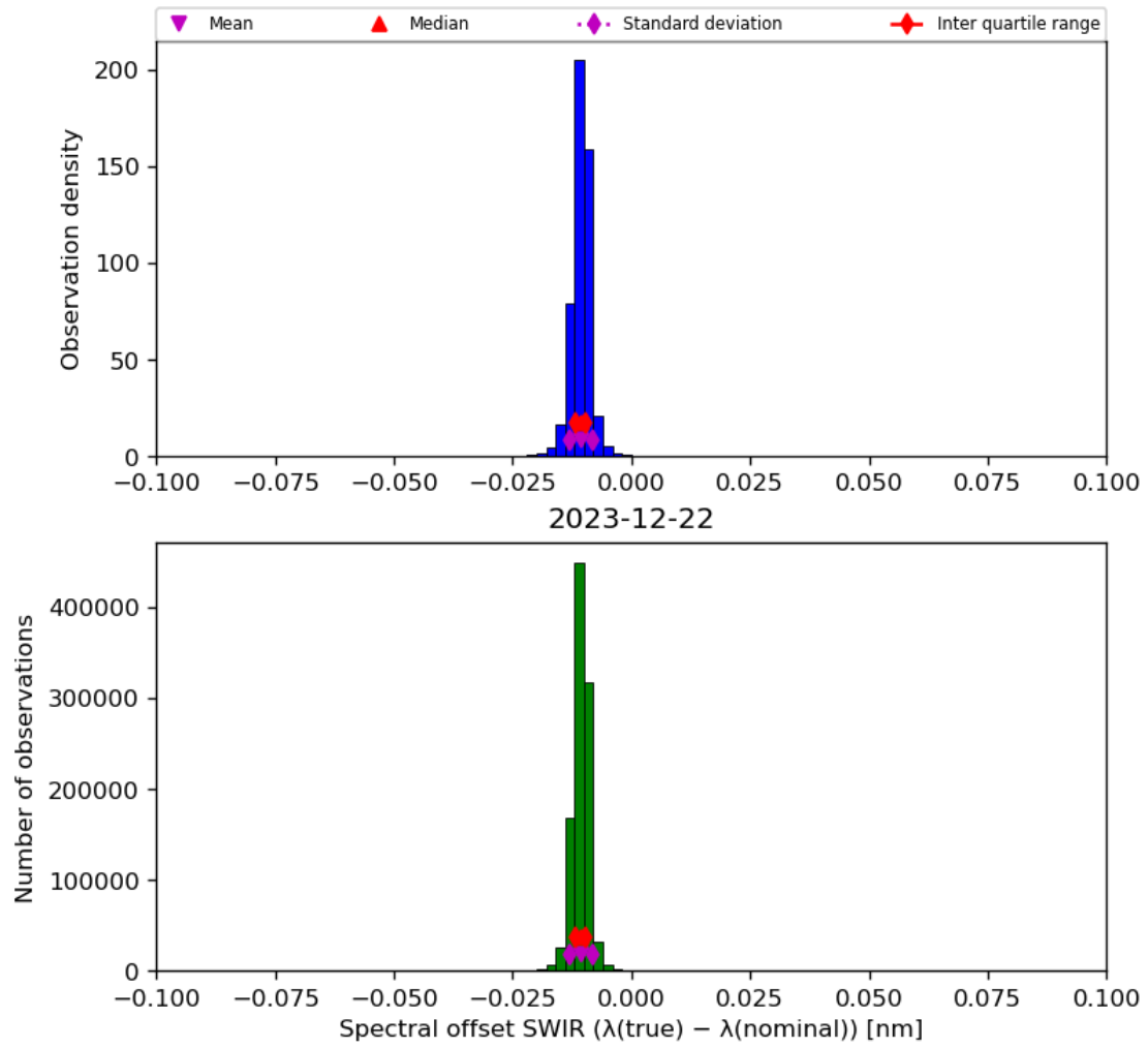
Figure 27: Histogram of “Spectral offset SWIR ( \lambda(\text{true}) - \lambda(\text{nominal}) )” for 2023-12-21 to 2023-12-23
