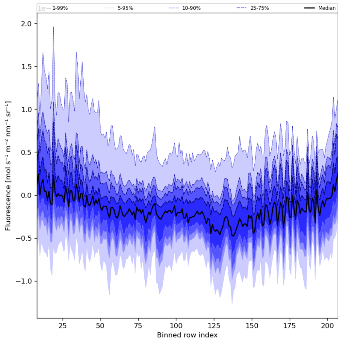
Figure 43: Along track statistics of “Fluorescence” for 2023-12-21 to 2023-12-23
