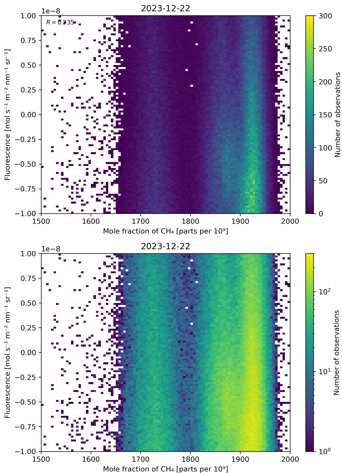
Figure 73: Scatter density plot of “Mole fraction of \text{CH}_4 ” against “Fluorescence” for 2023-12-21 to 2023-12-23.
