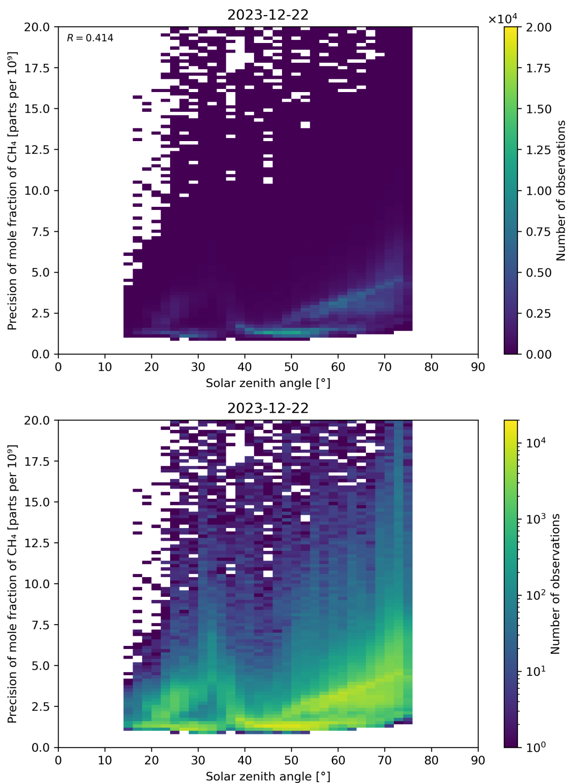
Figure 101: Scatter density plot of “Solar zenith angle” against “Precision of mole fraction of CH 4 ” for 2023-12-21 to 2023-12-23.
