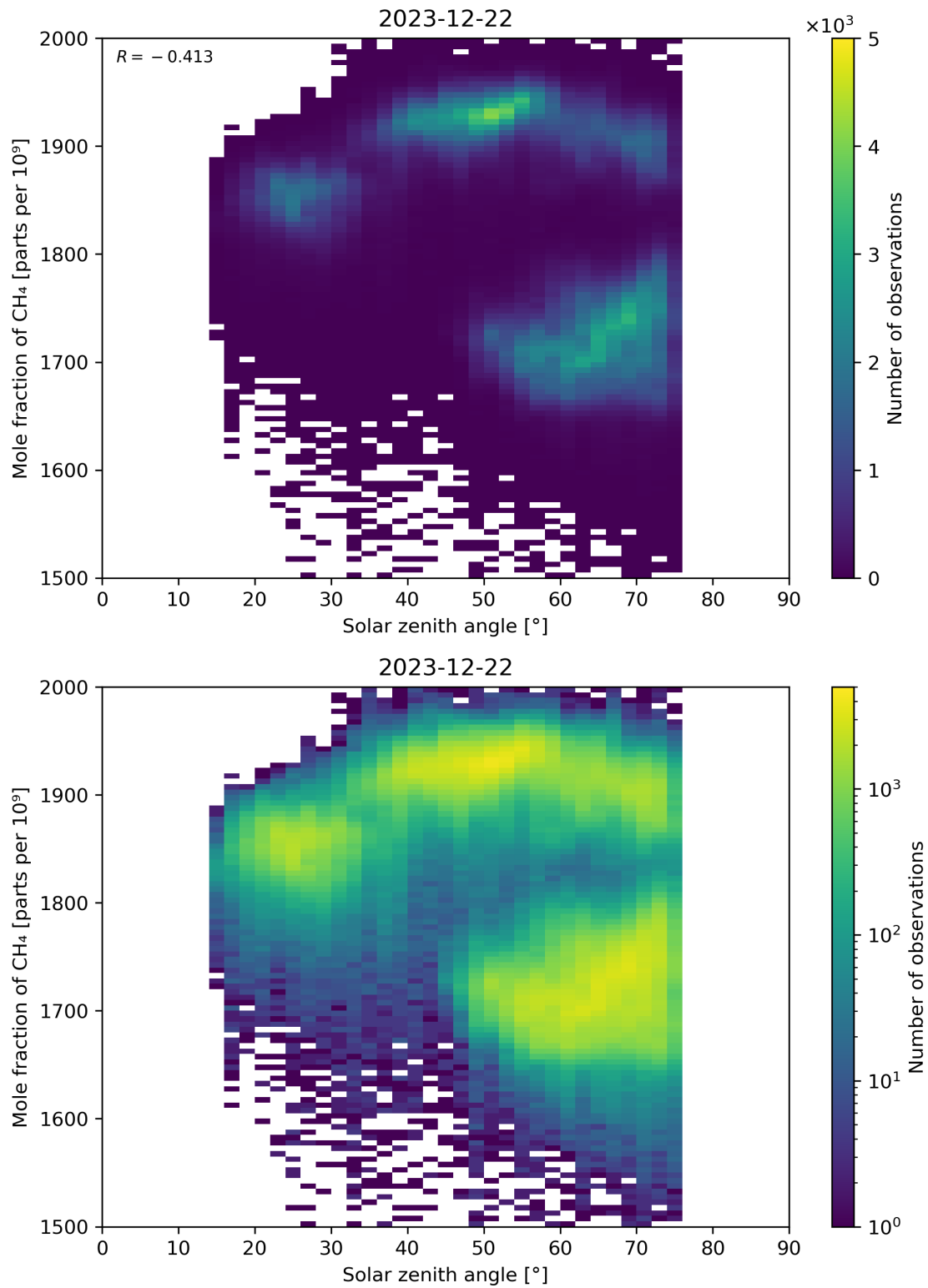
Figure 99: Scatter density plot of “Solar zenith angle” against “Mole fraction of \text{CH}_4 ” for 2023-12-21 to 2023-12-23.
