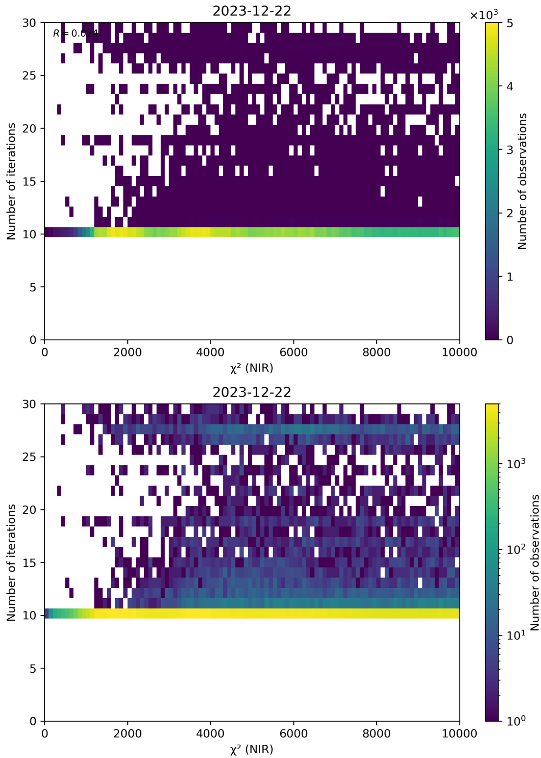
Figure 46: Scatter density plot of “ \chi^2 (NIR)” against “Number of iterations” for 2023-12-21 to 2023-12-23.
