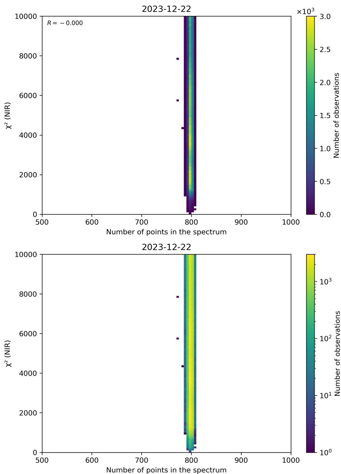
Figure 88: Scatter density plot of “Number of points in the spectrum” against “ \chi^2 (NIR)” for 2023-12-21 to 2023-12-23.
