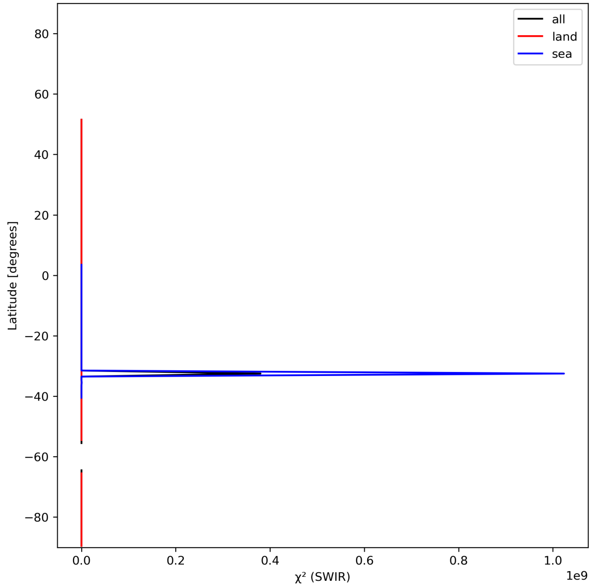
Figure 17: Zonal average of “ \chi^2 (SWIR)” for 2023-12-21 to 2023-12-23.
