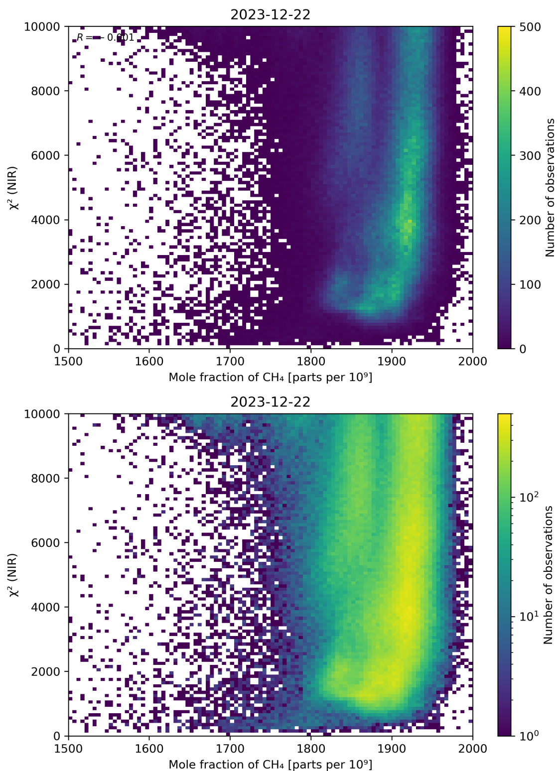
Figure 70: Scatter density plot of “Mole fraction of \text{CH}_4 ” against “ \chi^2 (NIR)” for 2023-12-21 to 2023-12-23.
