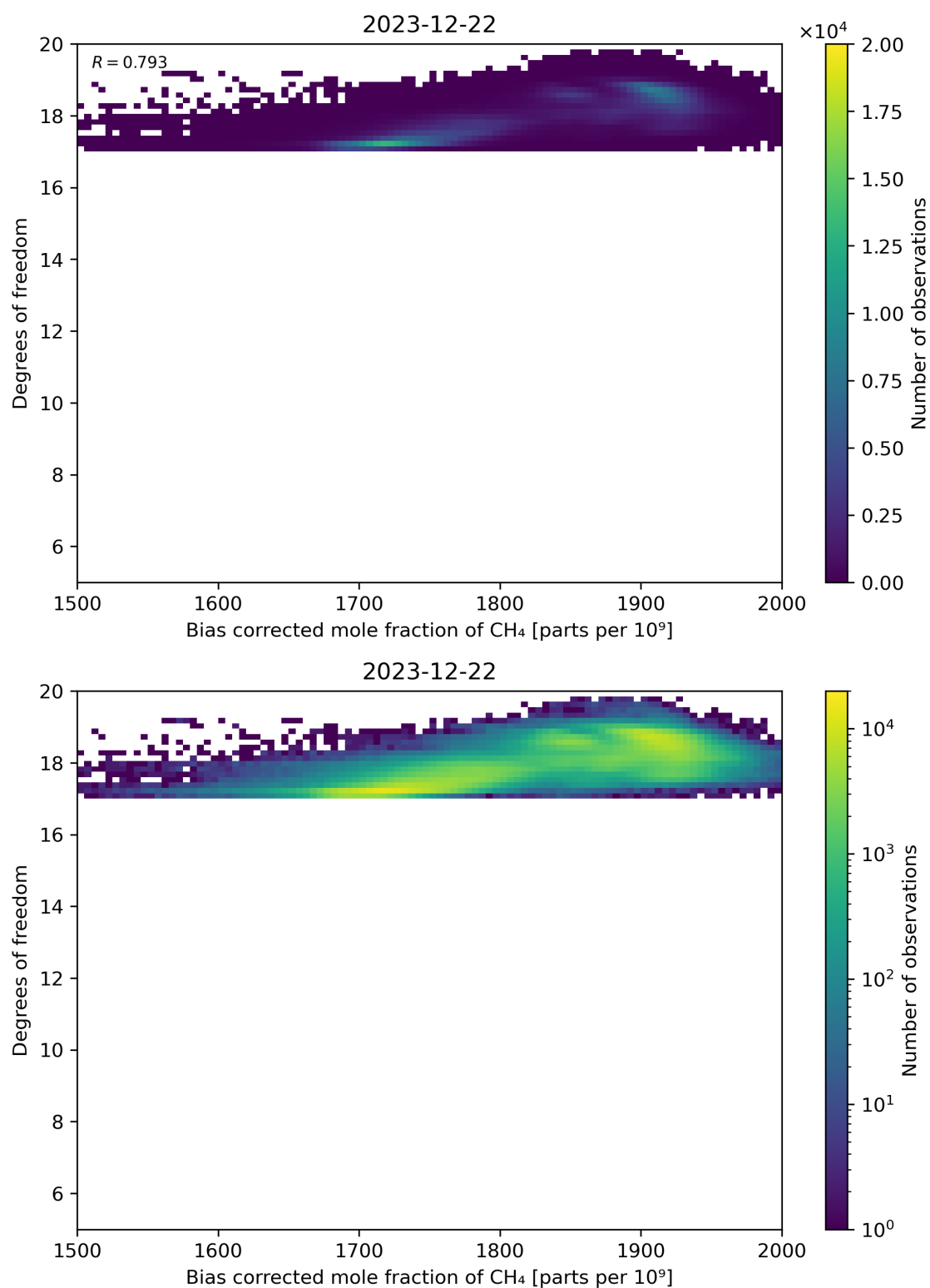
Figure 65: Scatter density plot of “Bias corrected mole fraction of CH 4 ” against “Degrees of freedom” for 2023-12-21 to 2023-12-23.
