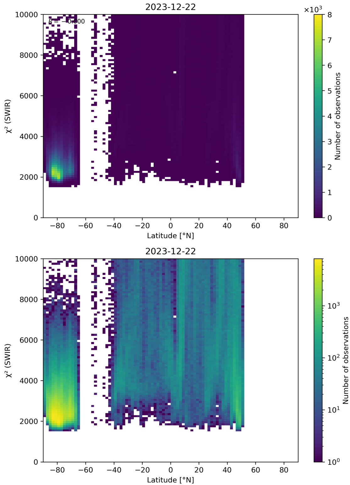
Figure 54: Scatter density plot of “Latitude” against “ \chi^2 (SWIR)” for 2023-12-21 to 2023-12-23.
