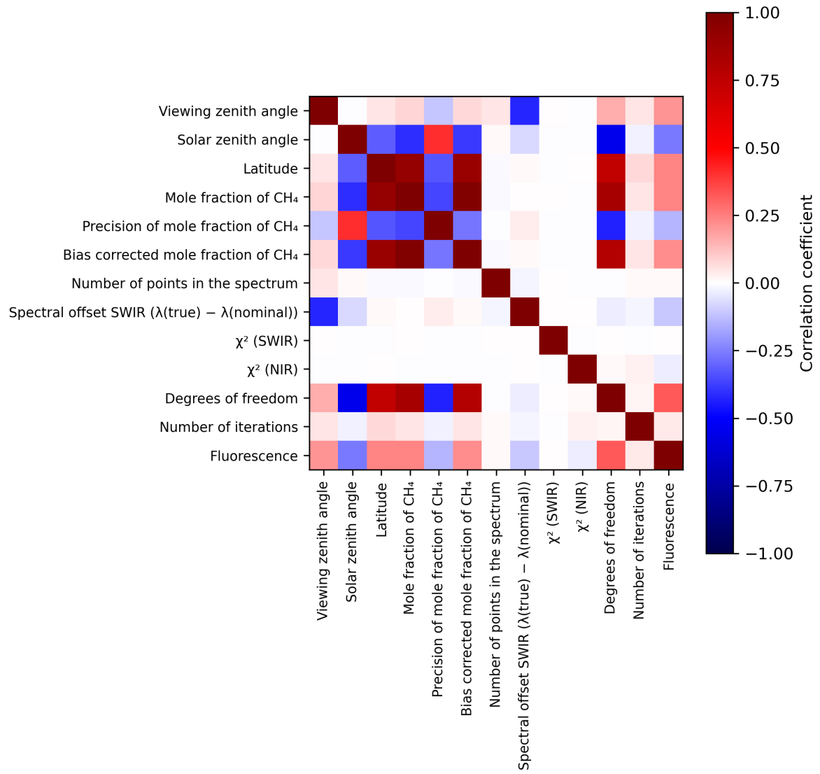
Figure 2: Map of correlation matrix for 2023-12-21 to 2023-12-23.
