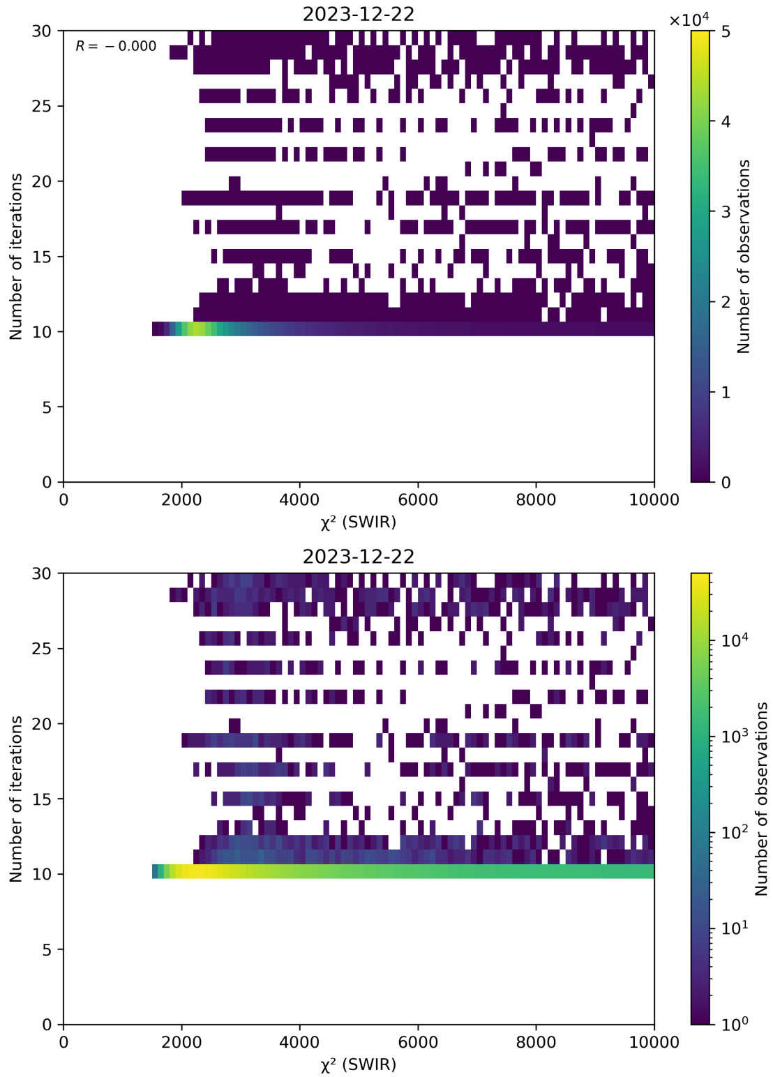
Figure 50: Scatter density plot of “ \chi^2 (SWIR)” against “Number of iterations” for 2023-12-21 to 2023-12-23.
