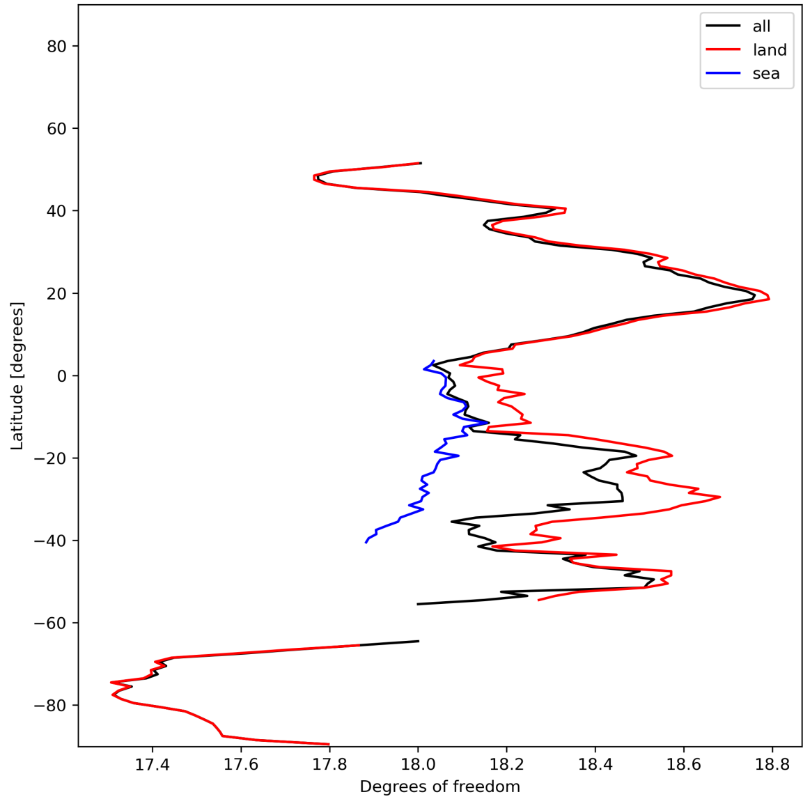
Figure 19: Zonal average of “Degrees of freedom” for 2023-12-21 to 2023-12-23.
