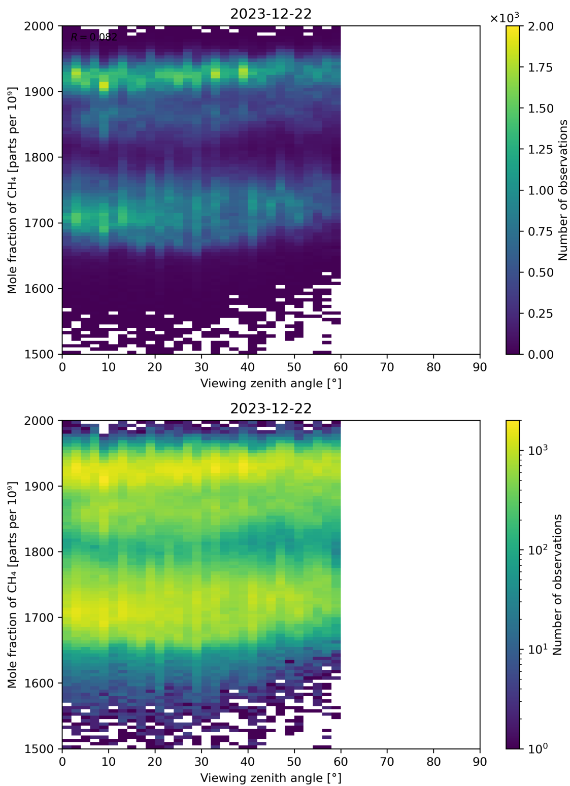
Figure 110: Scatter density plot of “Viewing zenith angle” against “Mole fraction of CH 4 ” for 2023-12-21 to 2023-12-23.
