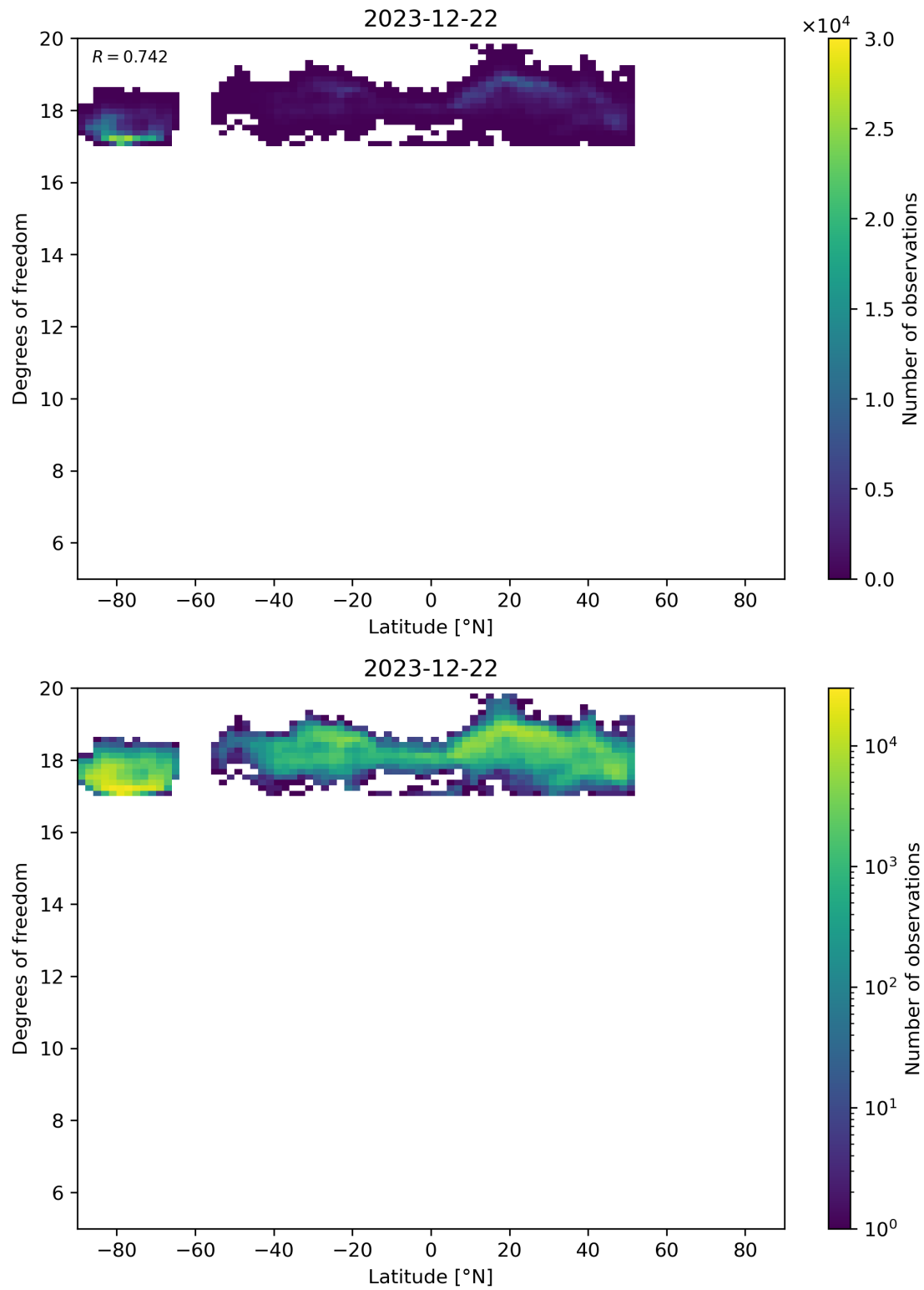
Figure 55: Scatter density plot of “Latitude” against “Degrees of freedom” for 2023-12-21 to 2023-12-23.
