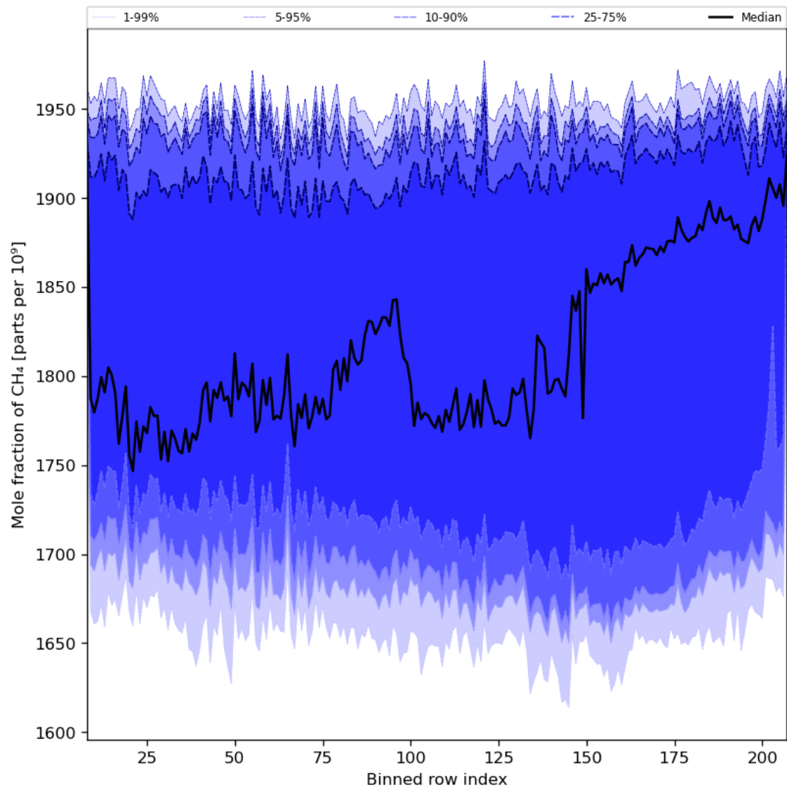
Figure 34: Along track statistics of “Mole fraction of CH 4 ” for 2023-12-21 to 2023-12-23
