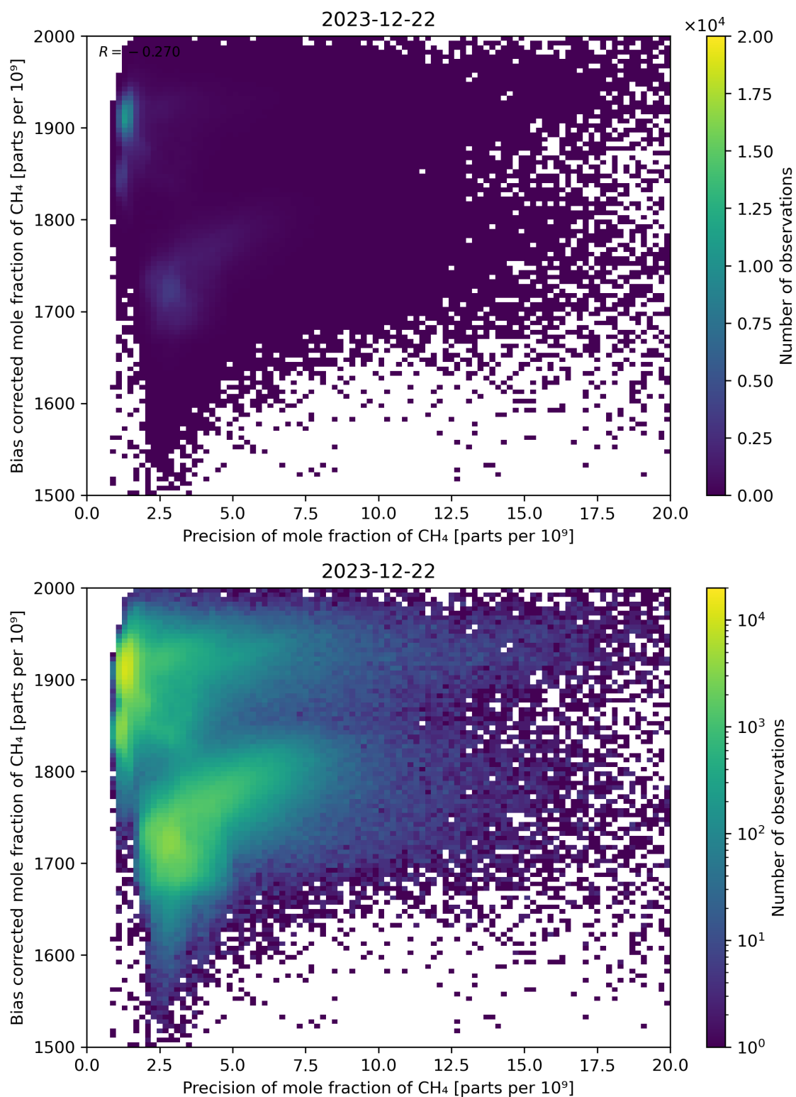
Figure 82: Scatter density plot of “Precision of mole fraction of CH 4 ” against “Bias corrected mole fraction of CH 4 ” for 2023-12-21 to 2023-12-23.
