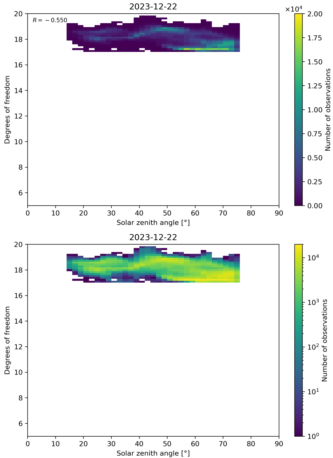
Figure 96: Scatter density plot of “Solar zenith angle” against “Degrees of freedom” for 2023-12-21 to 2023-12-23.
