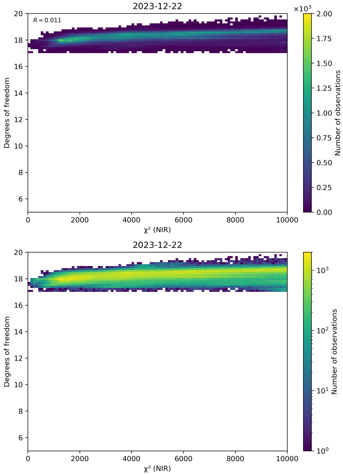
Figure 44: Scatter density plot of “ \chi^2 (NIR)” against “Degrees of freedom” for 2023-12-21 to 2023-12-23.
