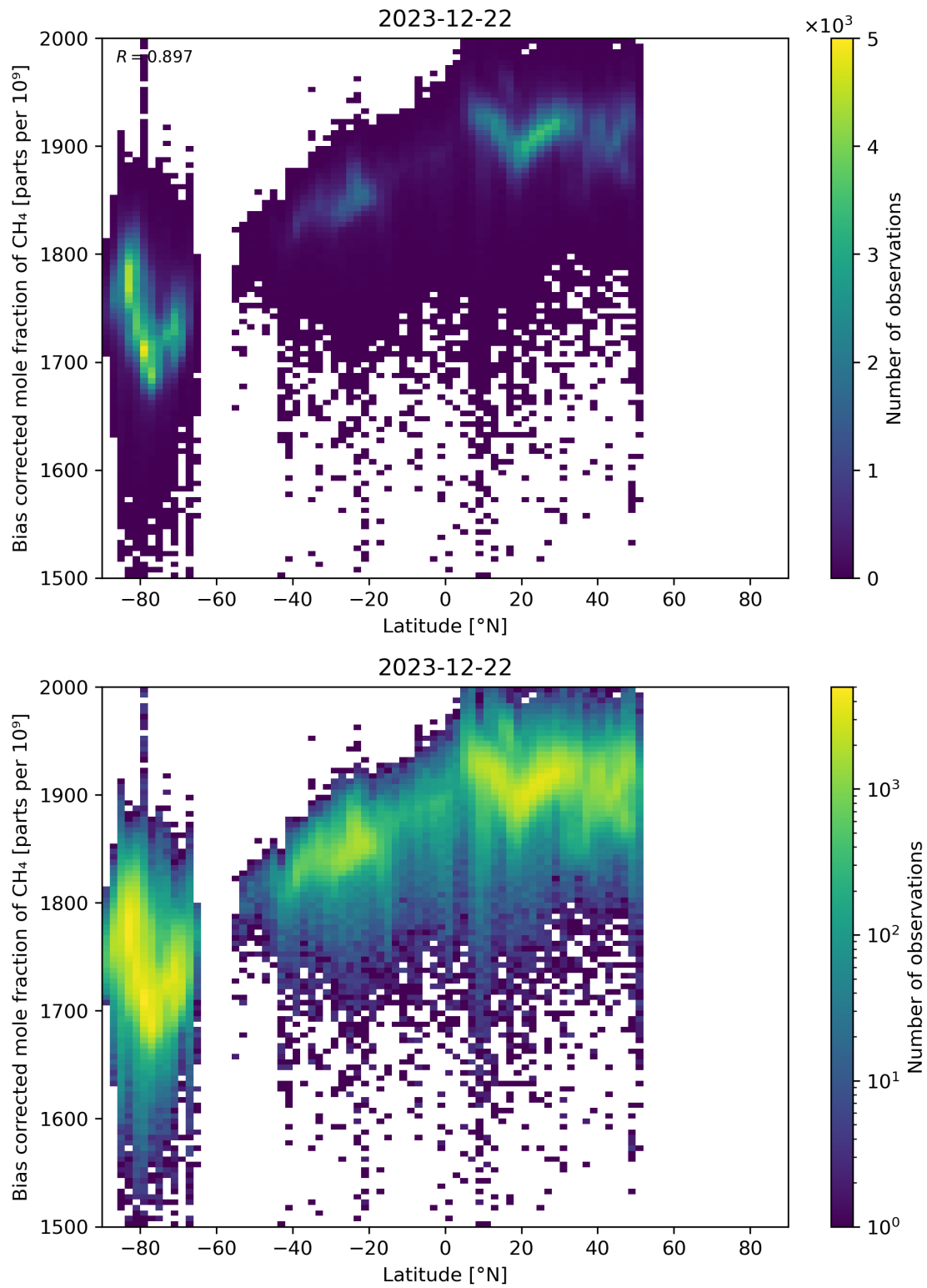
Figure 58: Scatter density plot of “Latitude” against “Bias corrected mole fraction of CH 4 ” for 2023-12-21 to 2023-12-23.
