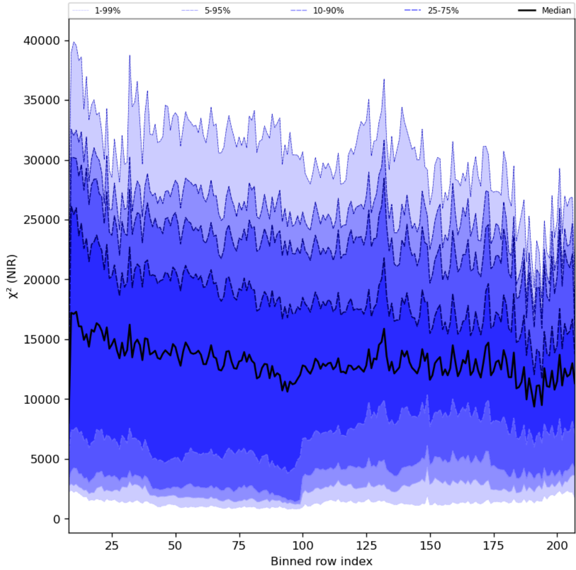
Figure 40: Along track statistics of “ \chi^2 (NIR)” for 2023-12-21 to 2023-12-23
