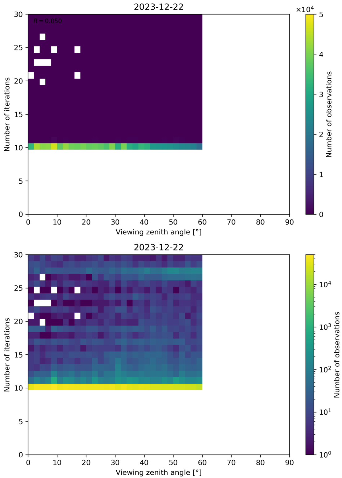
Figure 113: Scatter density plot of “Viewing zenith angle” against “Number of iterations” for 2023-12-21 to 2023-12-23.
