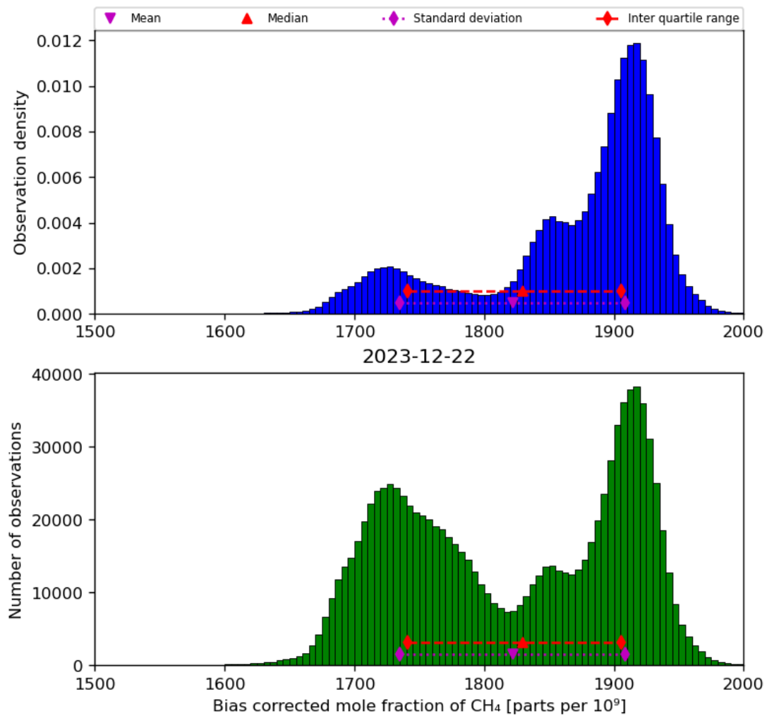
Figure 25: Histogram of “Bias corrected mole fraction of CH 4 ” for 2023-12-21 to 2023-12-23
