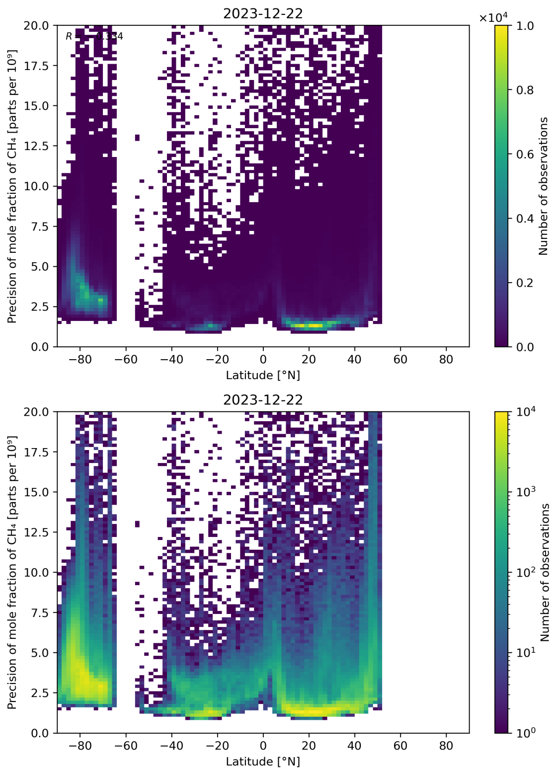
Figure 59: Scatter density plot of “Latitude” against “Precision of mole fraction of CH 4 ” for 2023-12-21 to 2023-12-23.
