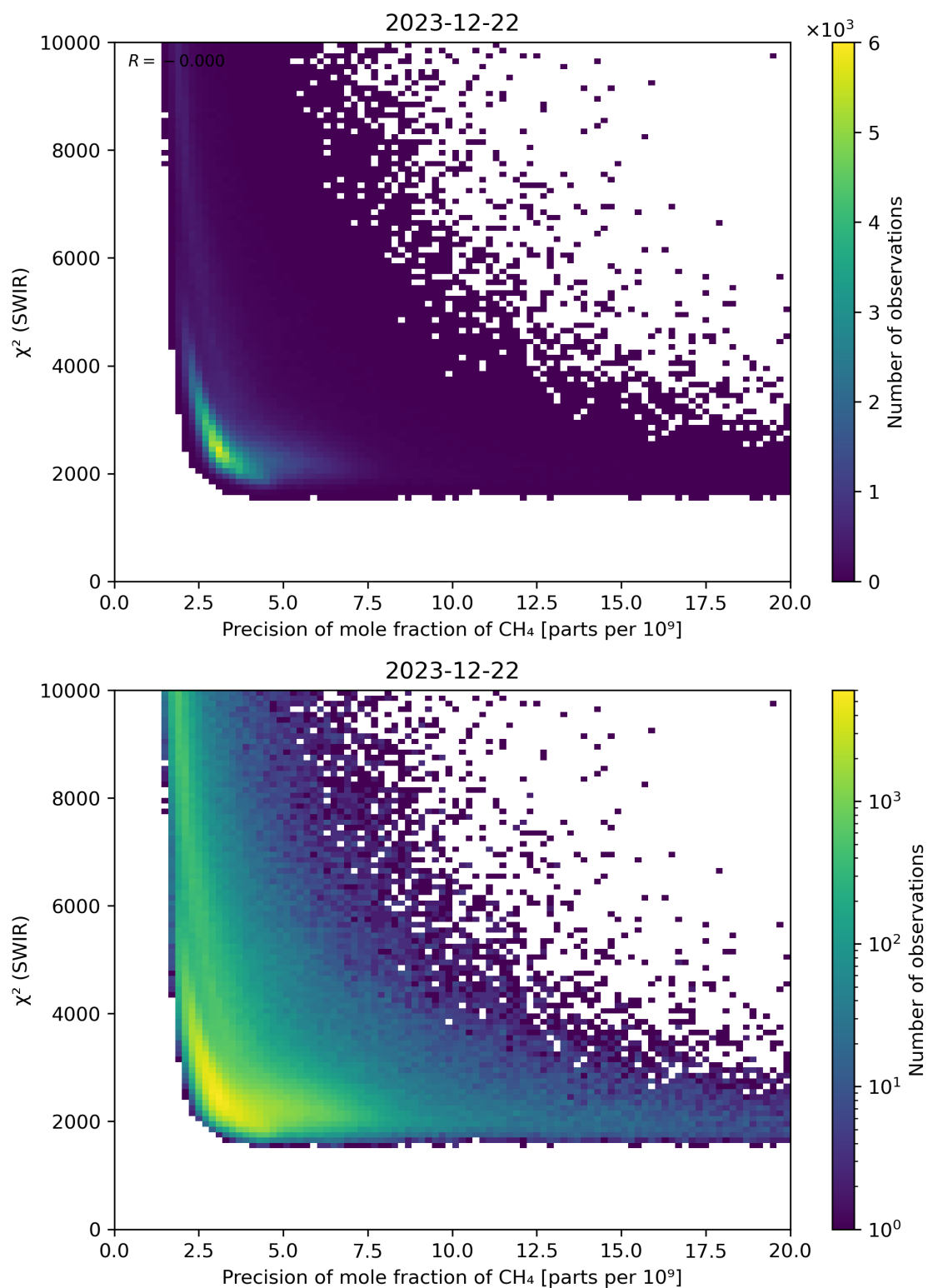
Figure 79: Scatter density plot of “Precision of mole fraction of CH 4 ” against “ \chi^2 (SWIR)” for 2023-12-21 to 2023-12-23.
