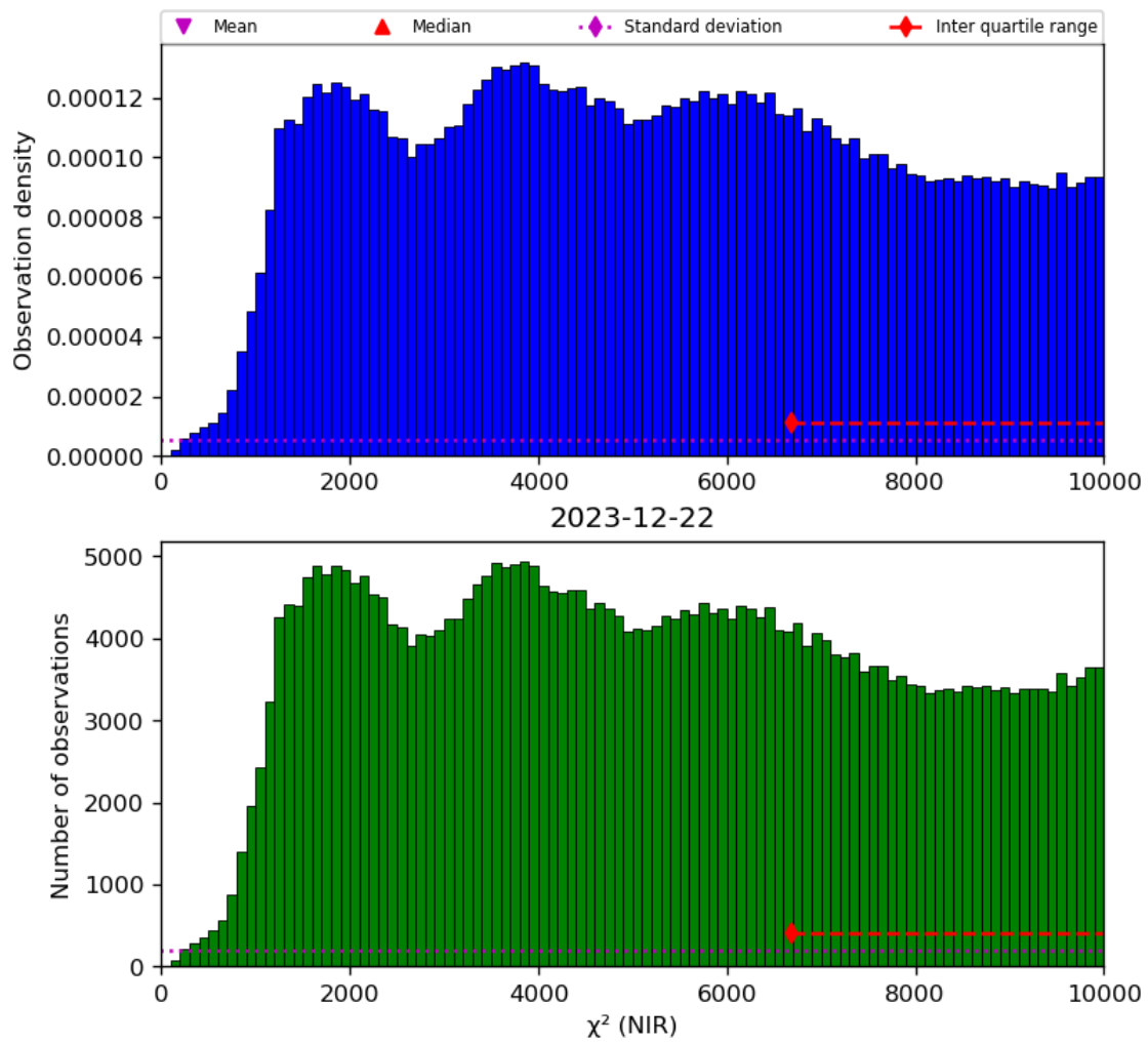
Figure 29: Histogram of " \chi^2 (NIR)" for 2023-12-21 to 2023-12-23
