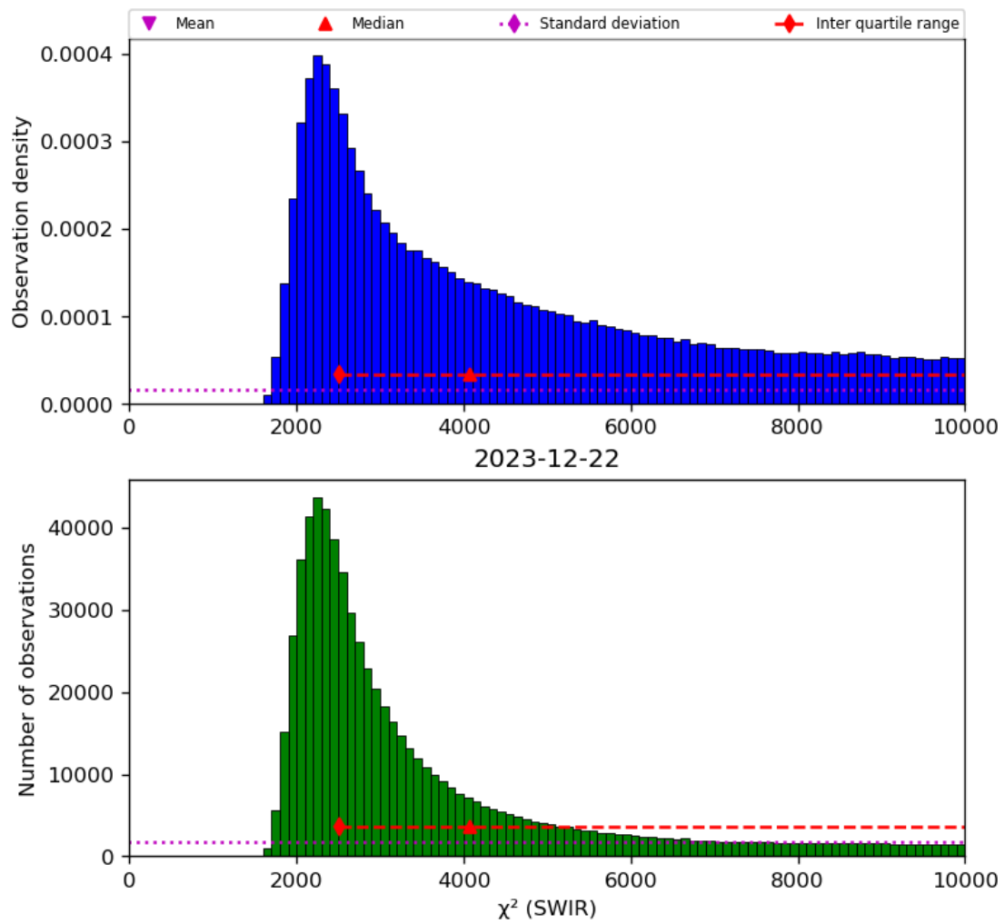
Figure 28: Histogram of “ \chi^2 (SWIR)” for 2023-12-21 to 2023-12-23
