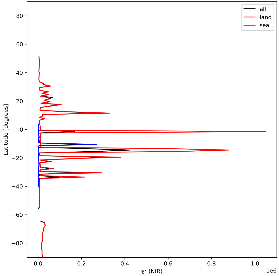
Figure 18: Zonal average of “ \chi^2 (NIR)” for 2023-12-21 to 2023-12-23.
