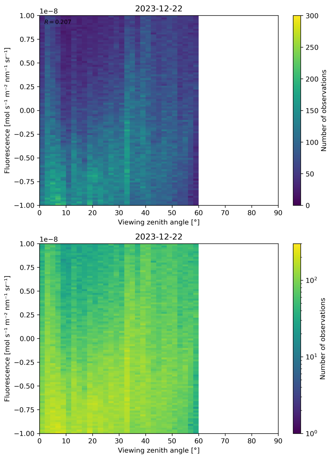
Figure 108: Scatter density plot of “Viewing zenith angle” against “Fluorescence” for 2023-12-21 to 2023-12-23.
