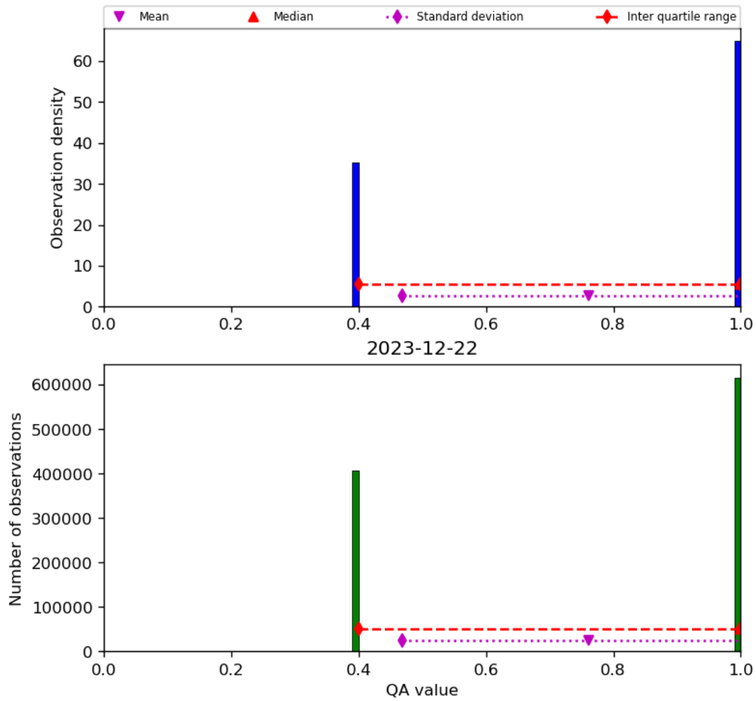
Figure 22: Histogram of “QA value” for 2023-12-21 to 2023-12-23
