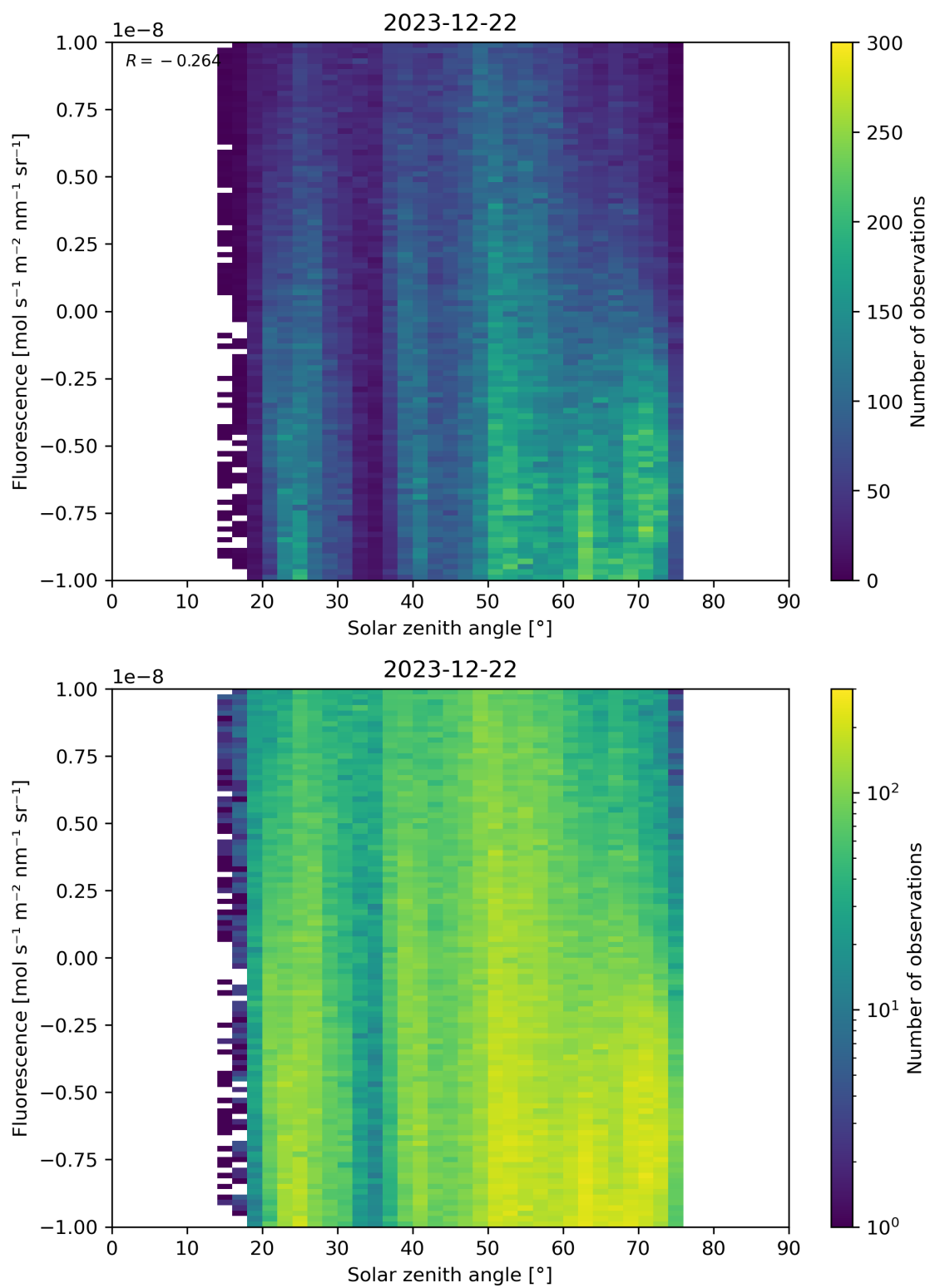
Figure 97: Scatter density plot of “Solar zenith angle” against “Fluorescence” for 2023-12-21 to 2023-12-23.
