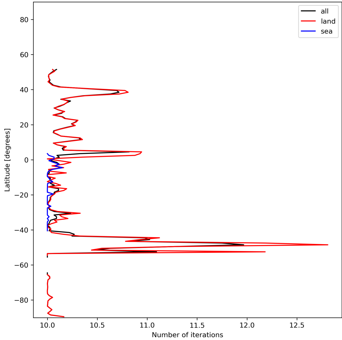
Figure 20: Zonal average of “Number of iterations” for 2023-12-21 to 2023-12-23.
