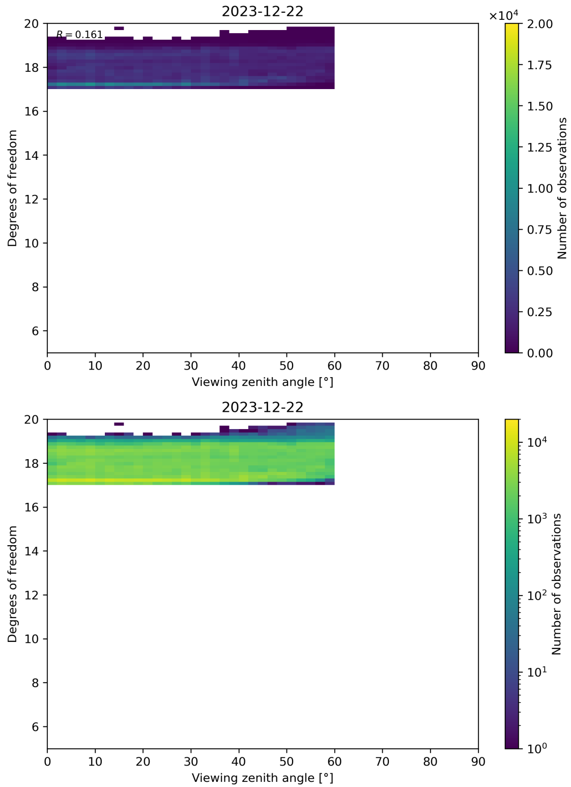
Figure 107: Scatter density plot of “Viewing zenith angle” against “Degrees of freedom” for 2023-12-21 to 2023-12-23.
