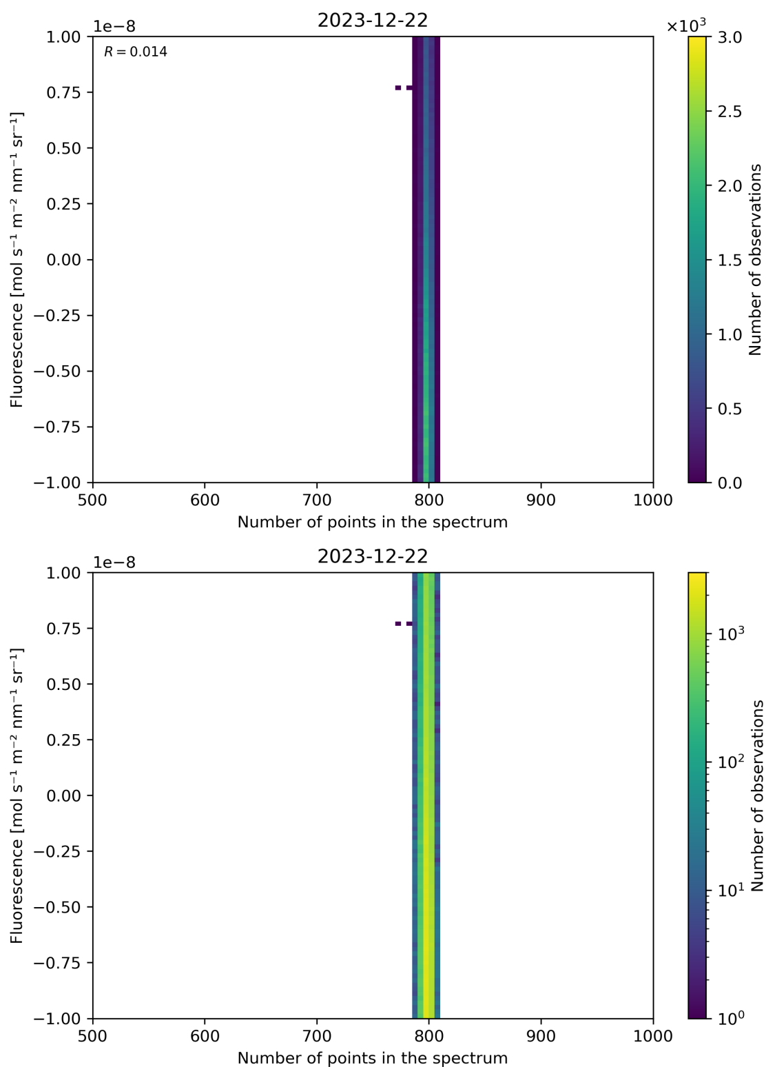
Figure 91: Scatter density plot of “Number of points in the spectrum” against “Fluorescence” for 2023-12-21 to 2023-12-23.
