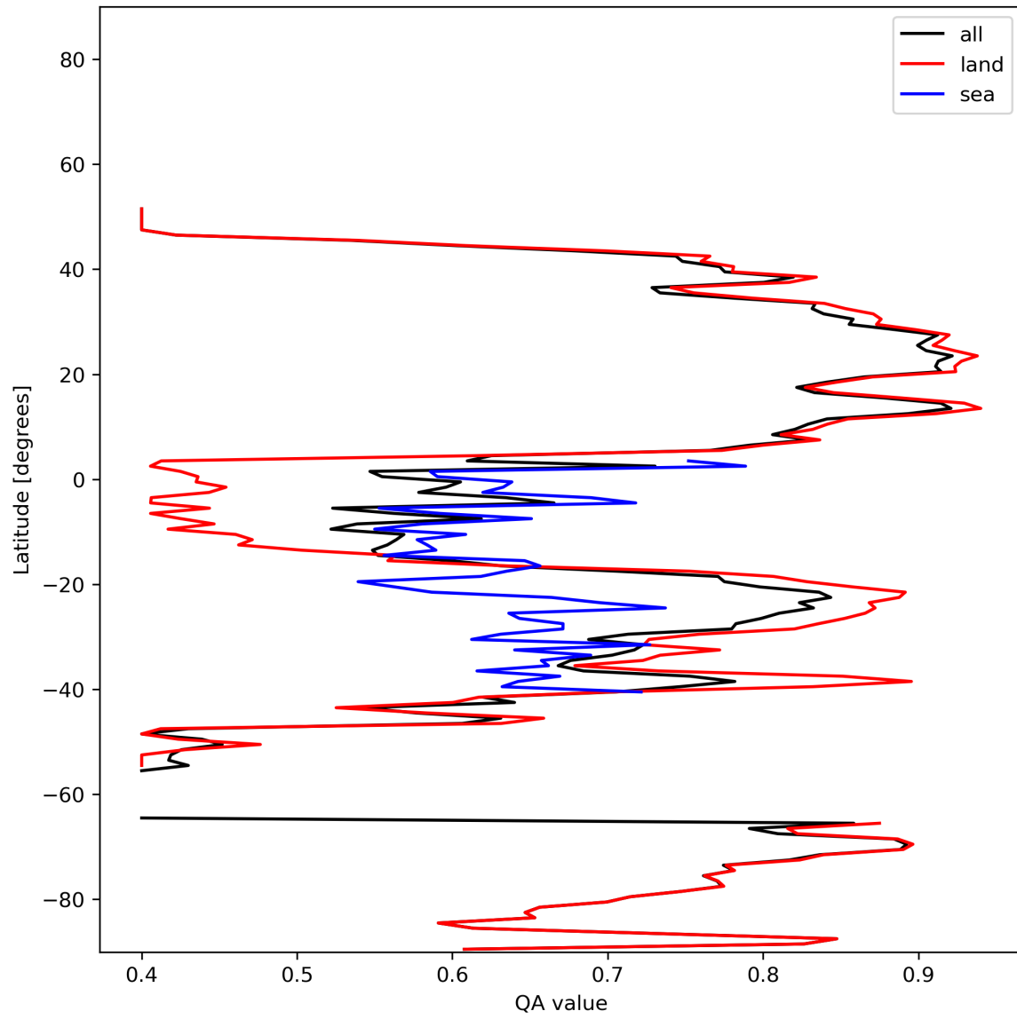
Figure 11: Zonal average of “QA value” for 2023-12-21 to 2023-12-23.
