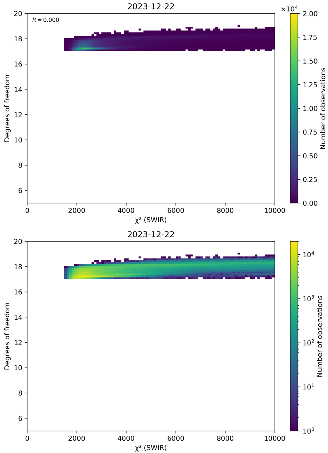
Figure 48: Scatter density plot of “ \chi^2 (SWIR)” against “Degrees of freedom” for 2023-12-21 to 2023-12-23.
