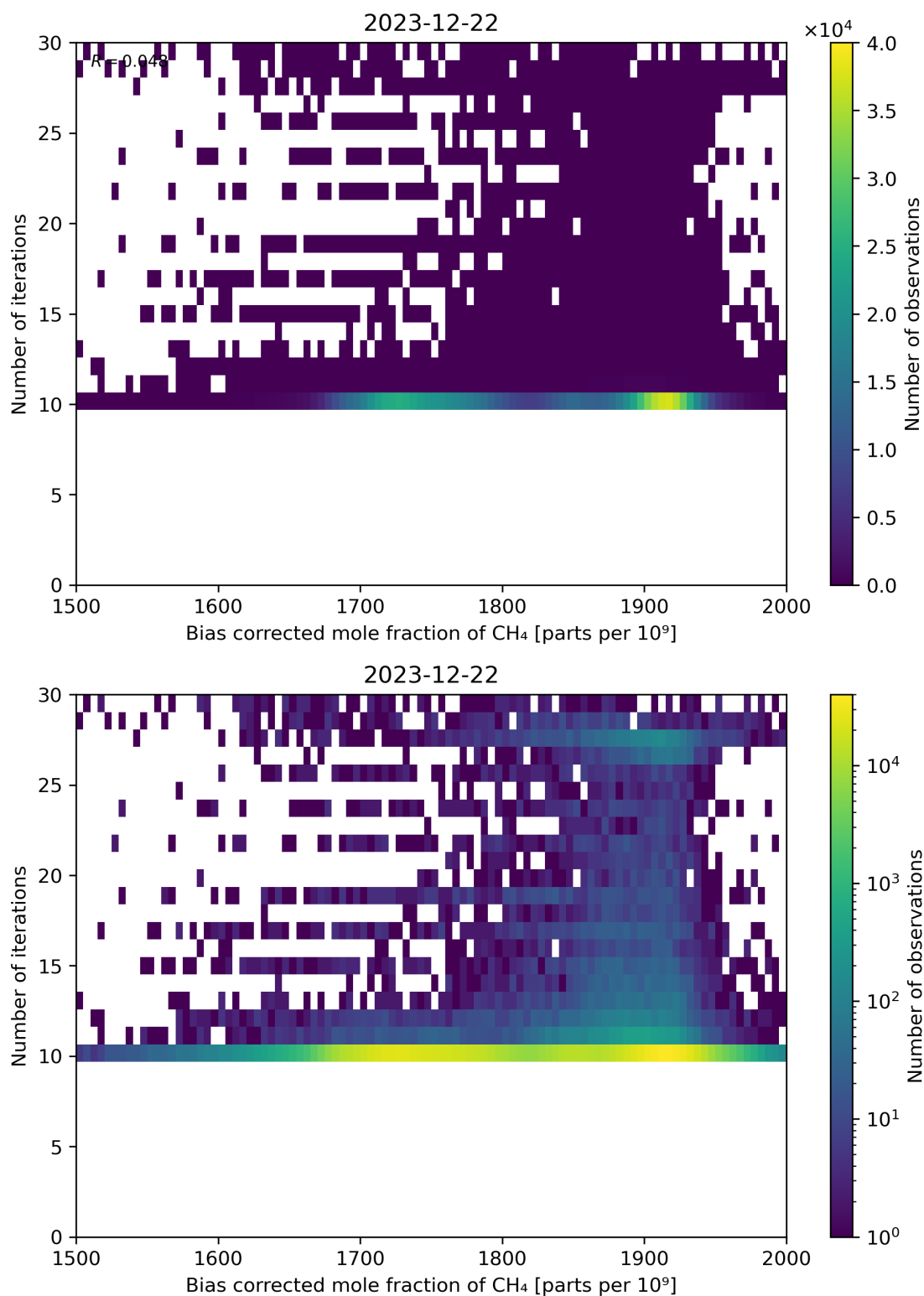
Figure 67: Scatter density plot of “Bias corrected mole fraction of \text{CH}_4 ” against “Number of iterations” for 2023-12-21 to 2023-12-23.
