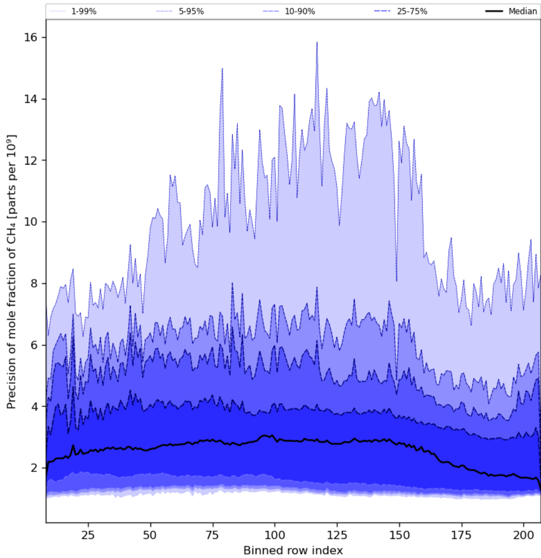
Figure 35: Along track statistics of “Precision of mole fraction of CH 4 ” for 2023-12-21 to 2023-12-23
