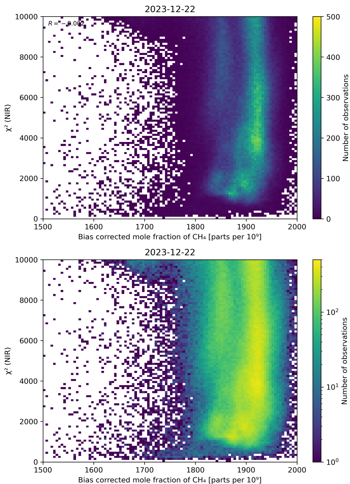
Figure 63: Scatter density plot of “Bias corrected mole fraction of CH 4 ” against “ \chi^2 (NIR)” for 2023-12-21 to 2023-12-23.
