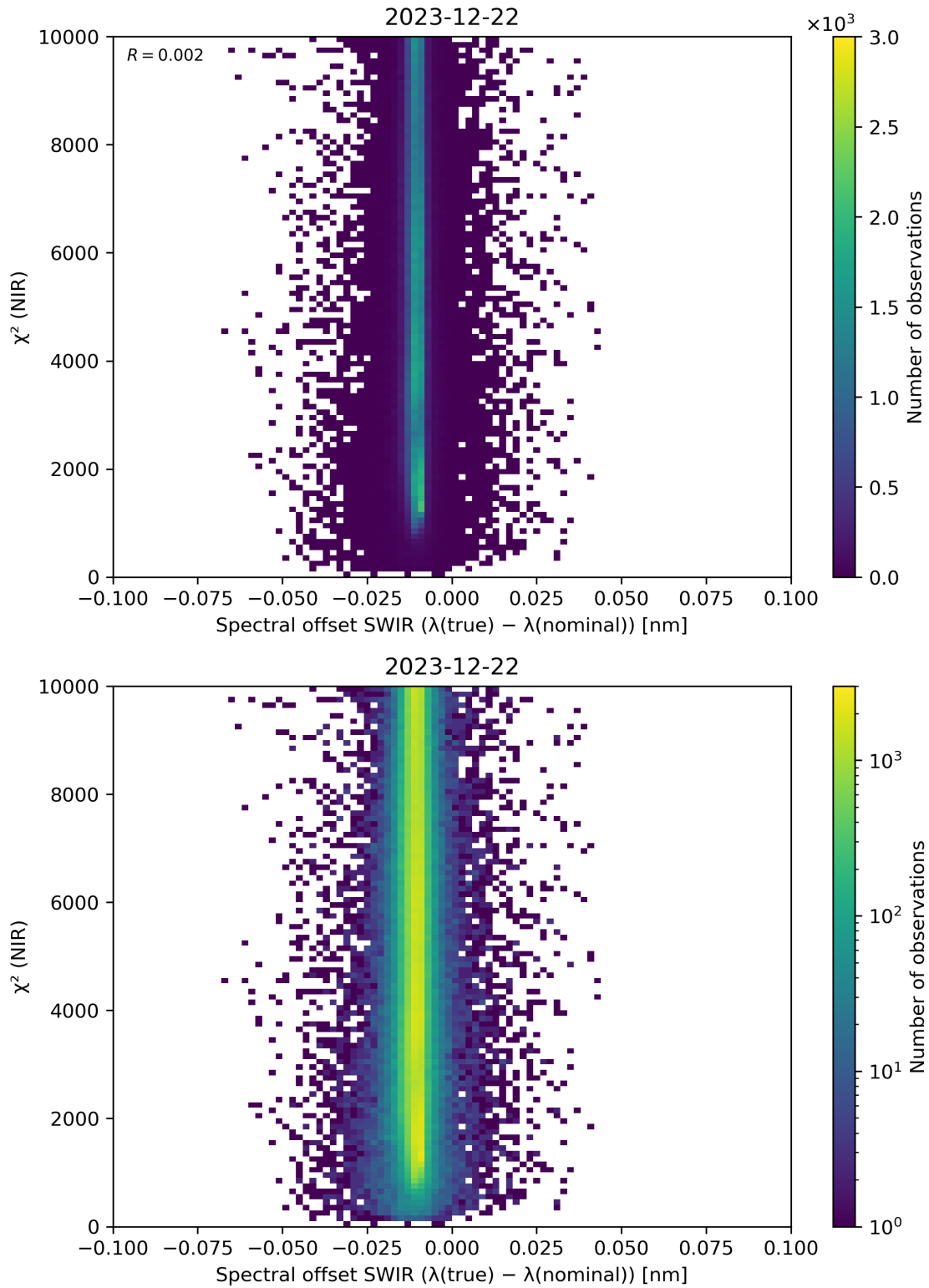
Figure 117: Scatter density plot of “Spectral offset SWIR ( \lambda(\text{true}) - \lambda(\text{nominal}) )” against “ \chi^2 (NIR)” for 2023-12-21 to 2023-12-23.
