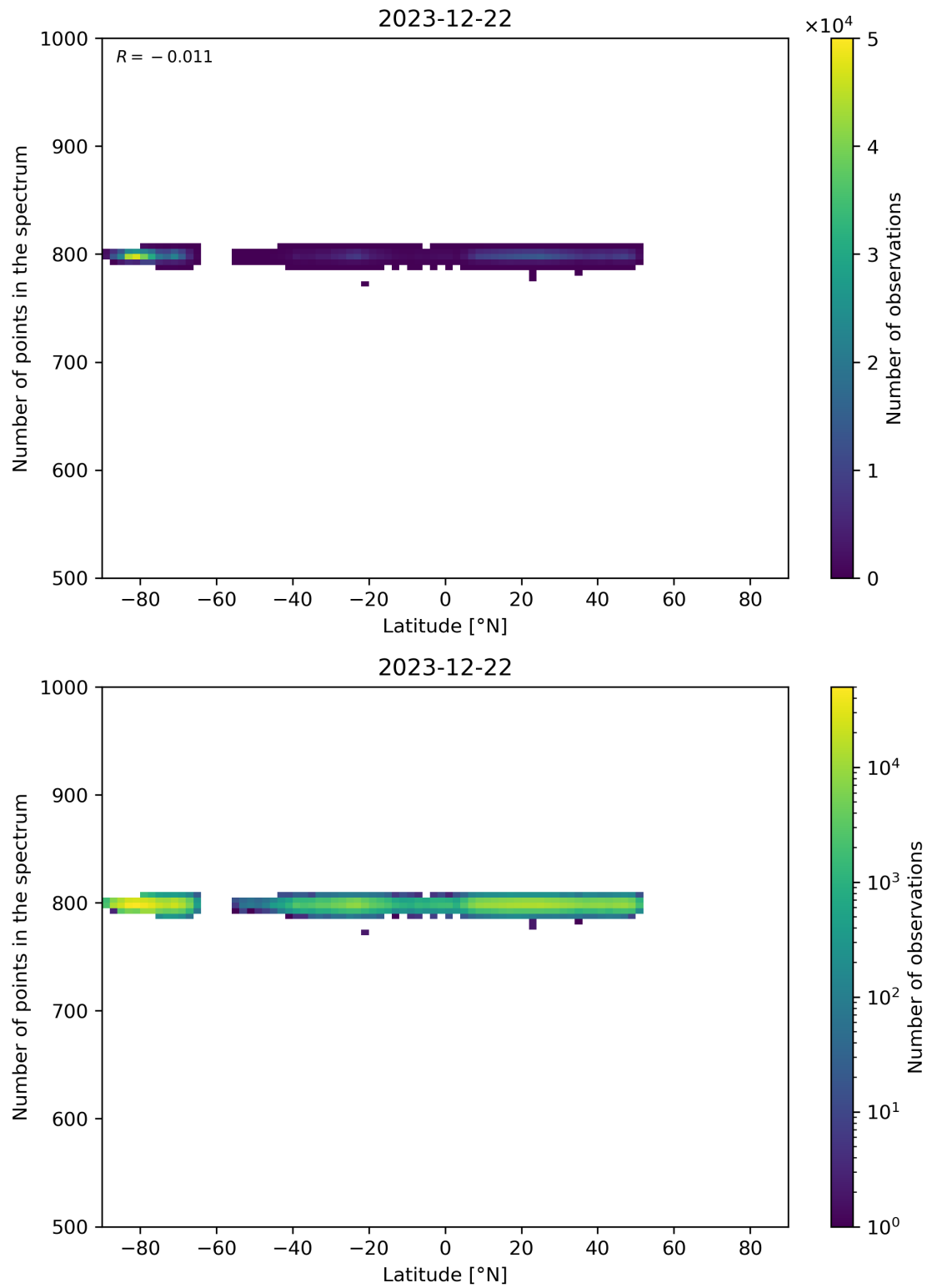
Figure 61: Scatter density plot of “Latitude” against “Number of points in the spectrum” for 2023-12-21 to 2023-12-23.
