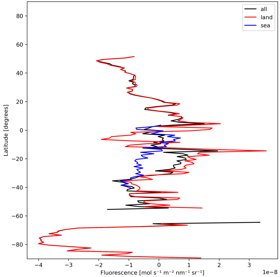
Figure 21: Zonal average of “Fluorescence” for 2023-12-21 to 2023-12-23.
