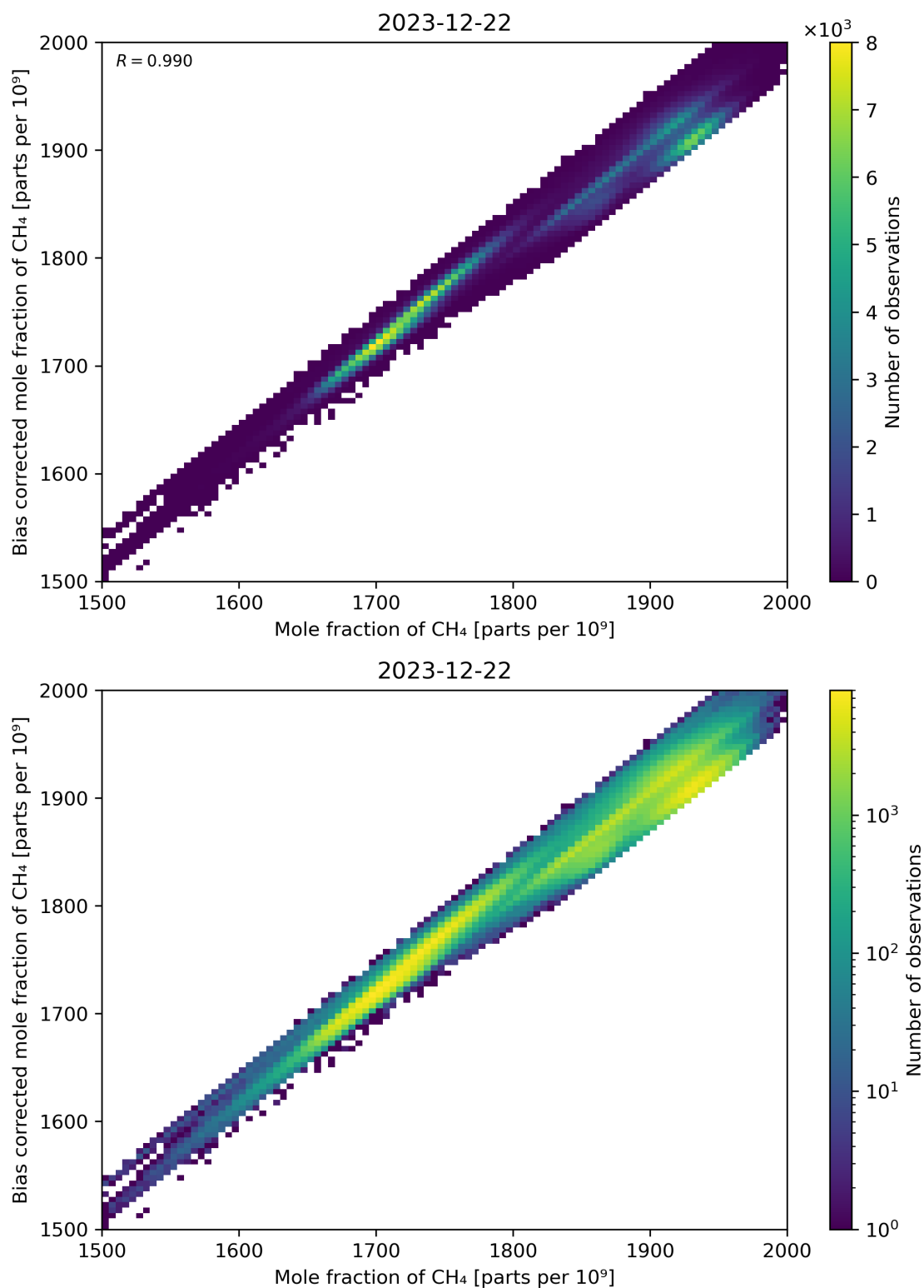
Figure 74: Scatter density plot of “Mole fraction of CH 4 ” against “Bias corrected mole fraction of CH 4 ” for 2023-12-21 to 2023-12-23.
