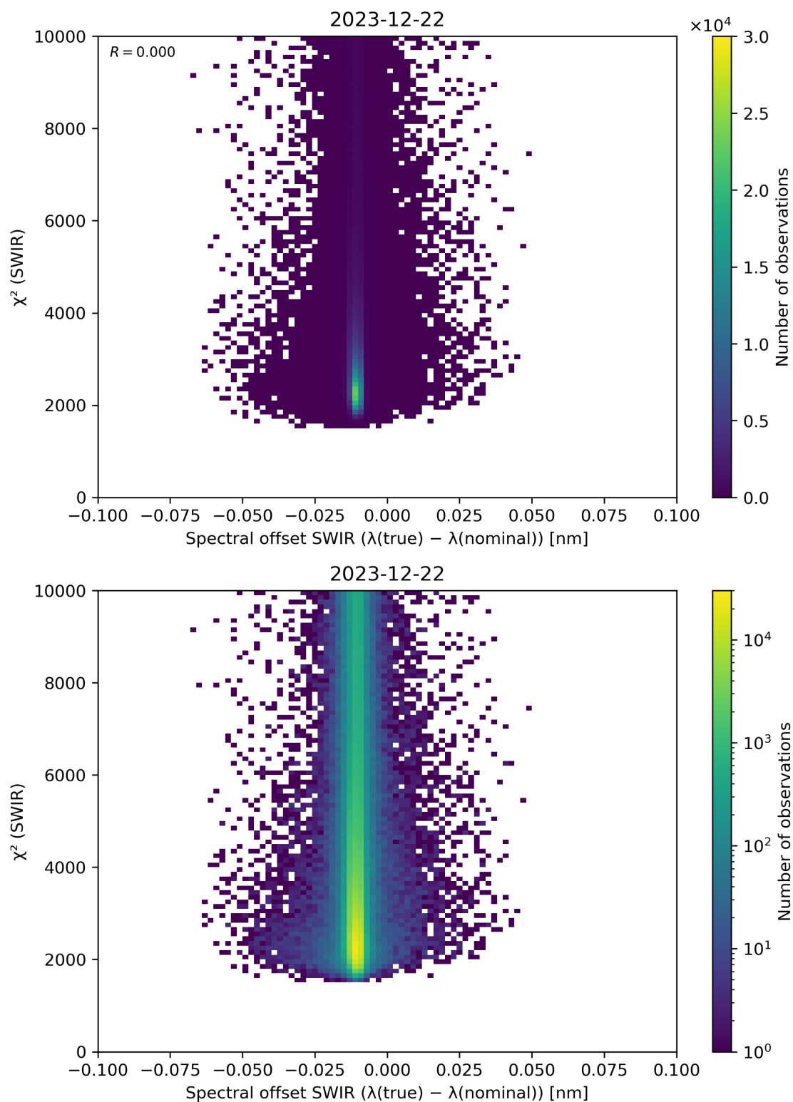
Figure 118: Scatter density plot of “Spectral offset SWIR ( \lambda(\text{true}) - \lambda(\text{nominal}) )” against “ \chi^2 (SWIR)” for 2023-12-21 to 2023-12-23.
