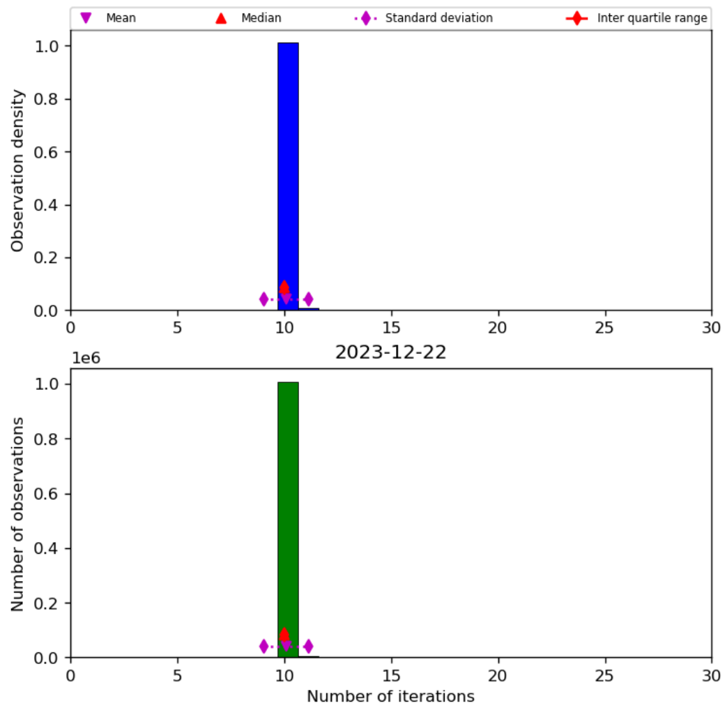
Figure 31: Histogram of “Number of iterations” for 2023-12-21 to 2023-12-23
