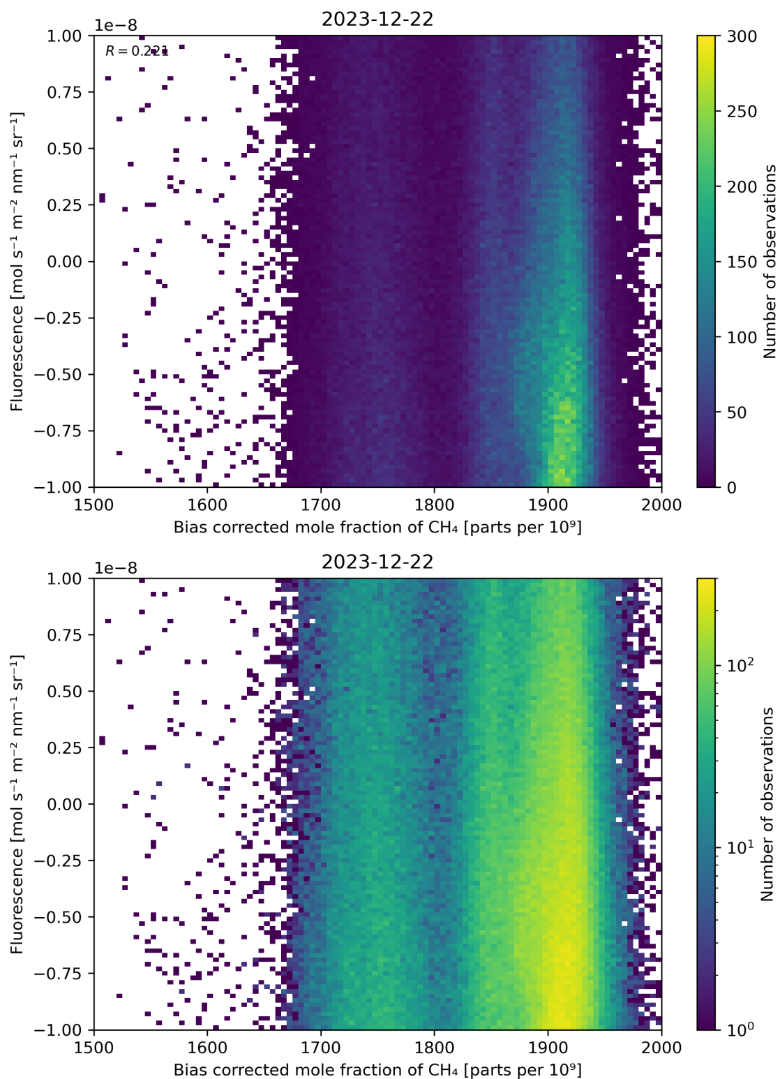
Figure 66: Scatter density plot of “Bias corrected mole fraction of \text{CH}_4 ” against “Fluorescence” for 2023-12-21 to 2023-12-23.
