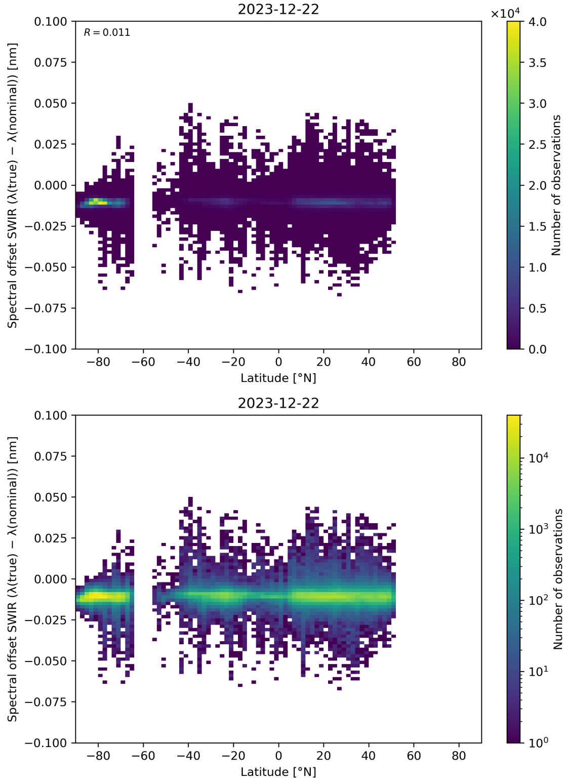
Figure 62: Scatter density plot of “Latitude” against “Spectral offset SWIR ( \lambda(\text{true}) - \lambda(\text{nominal}) )” for 2023-12-21 to 2023-12-23.
