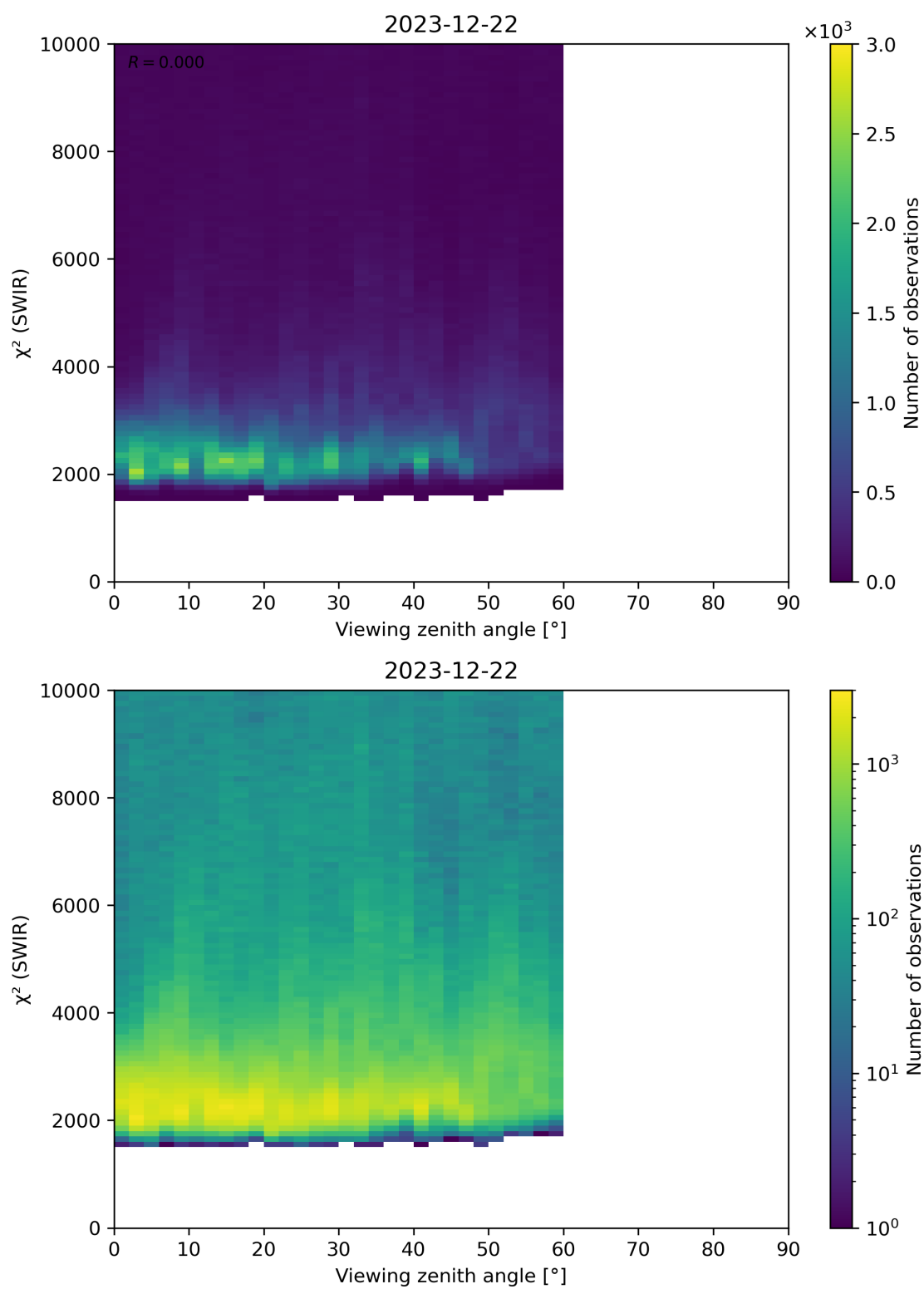
Figure 106: Scatter density plot of “Viewing zenith angle” against “ \chi^2 (SWIR)” for 2023-12-21 to 2023-12-23.
