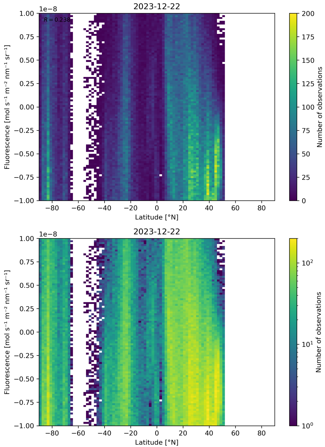
Figure 56: Scatter density plot of “Latitude” against “Fluorescence” for 2023-12-21 to 2023-12-23.
