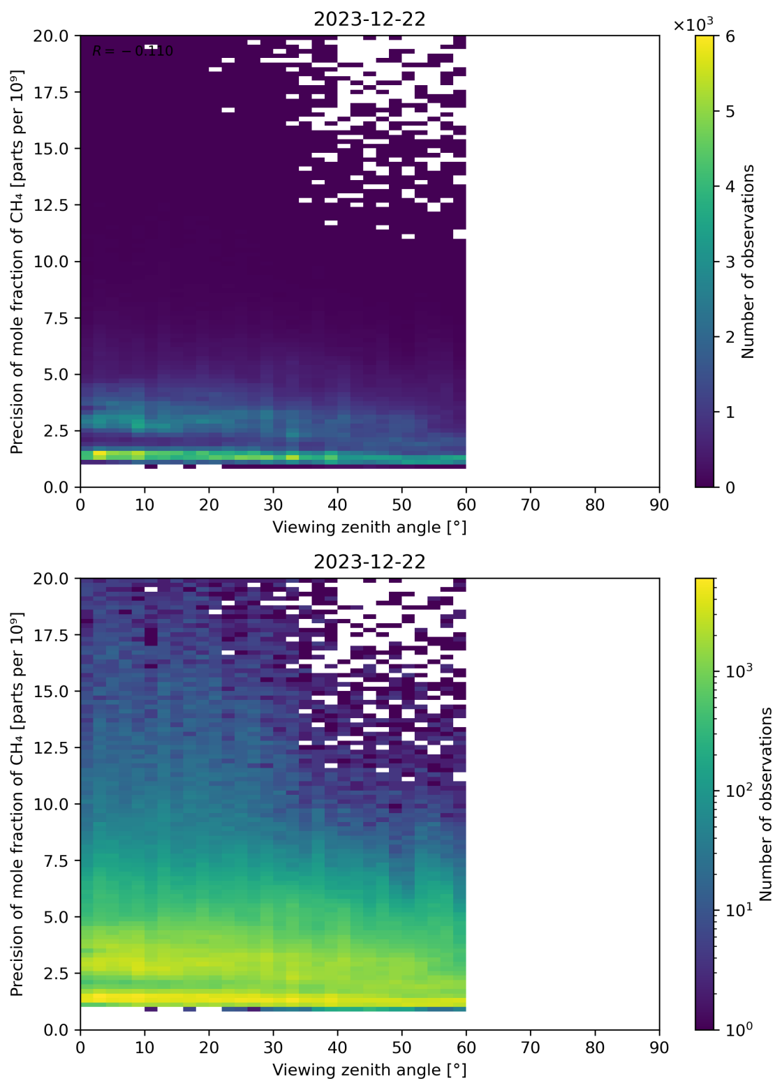
Figure 112: Scatter density plot of “Viewing zenith angle” against “Precision of mole fraction of CH 4 ” for 2023-12-21 to 2023-12-23.
