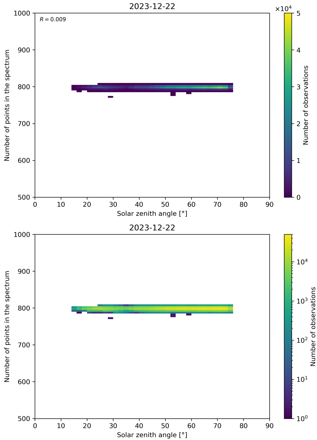
Figure 103: Scatter density plot of “Solar zenith angle” against “Number of points in the spectrum” for 2023-12-21 to 2023-12-23.
