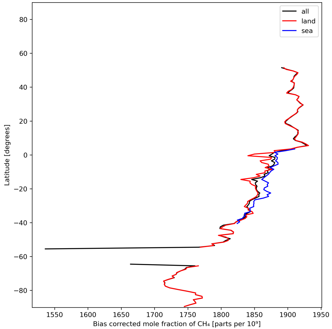
Figure 14: Zonal average of “Bias corrected mole fraction of CH 4 ” for 2023-12-21 to 2023-12-23.
