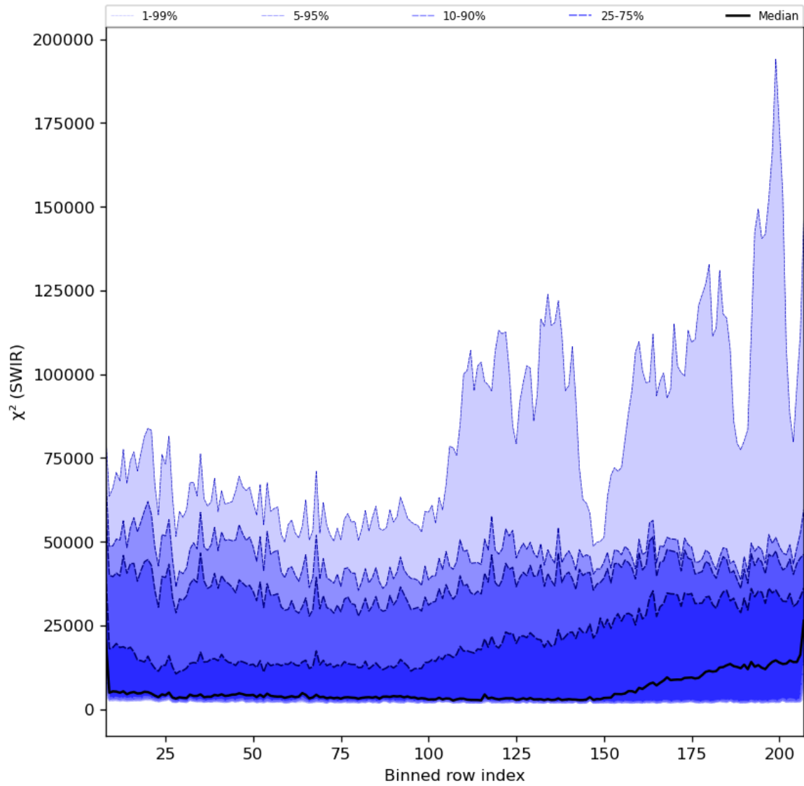
Figure 39: Along track statistics of “ \chi^2 (SWIR)” for 2023-12-21 to 2023-12-23
