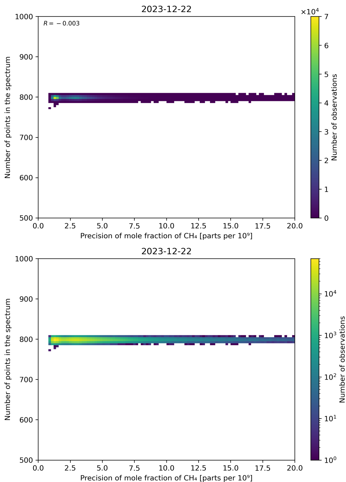
Figure 84: Scatter density plot of “Precision of mole fraction of CH 4 ” against “Number of points in the spectrum” for 2023-12-21 to 2023-12-23.
