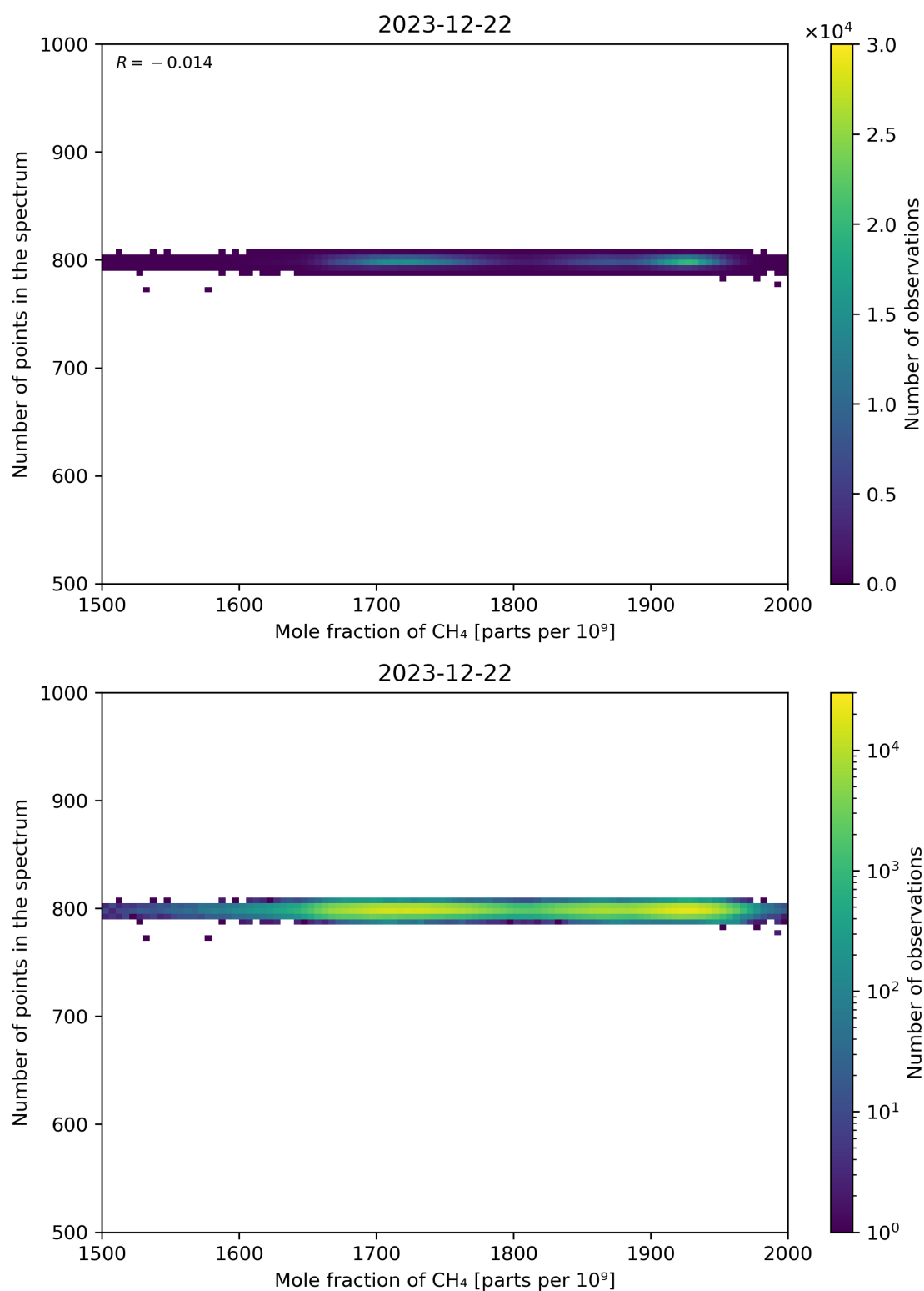
Figure 77: Scatter density plot of “Mole fraction of CH 4 ” against “Number of points in the spectrum” for 2023-12-21 to 2023-12-23.
