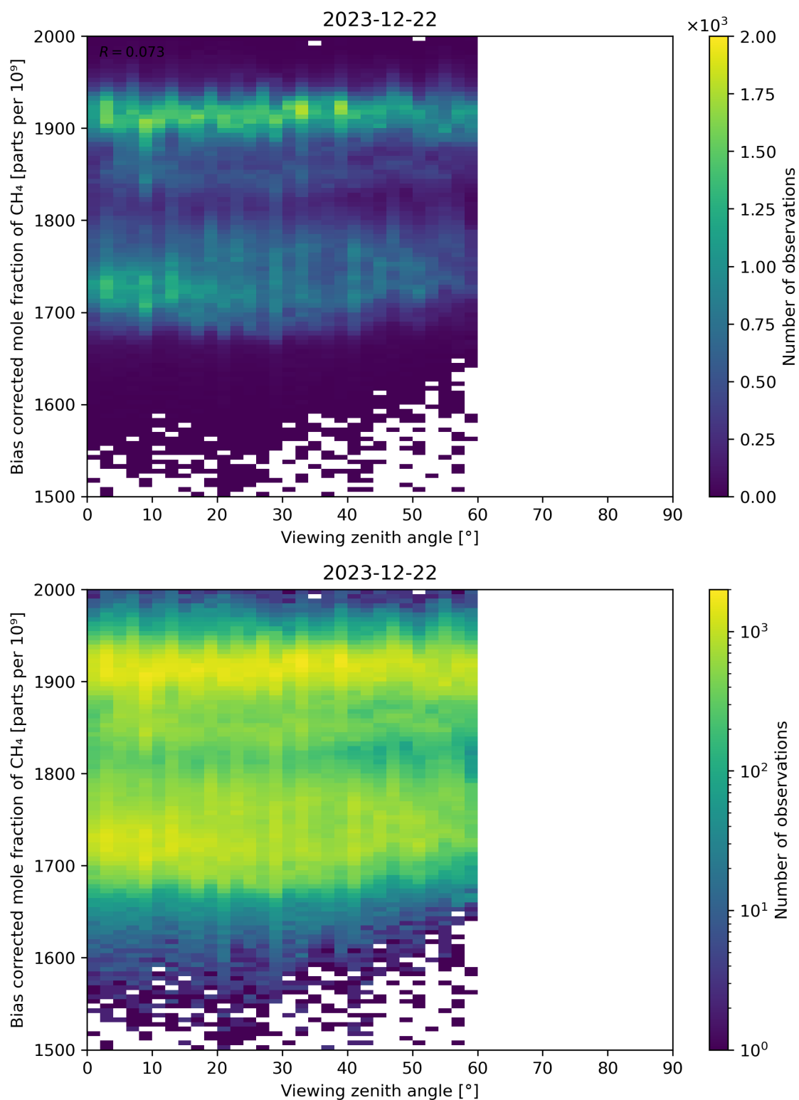
Figure 111: Scatter density plot of “Viewing zenith angle” against “Bias corrected mole fraction of CH 4 ” for 2023-12-21 to 2023-12-23.
