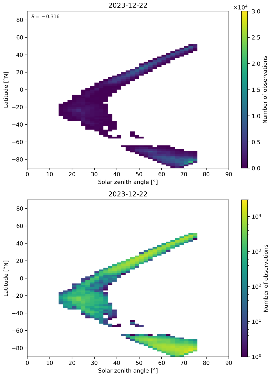
Figure 98: Scatter density plot of “Solar zenith angle” against “Latitude” for 2023-12-21 to 2023-12-23.
