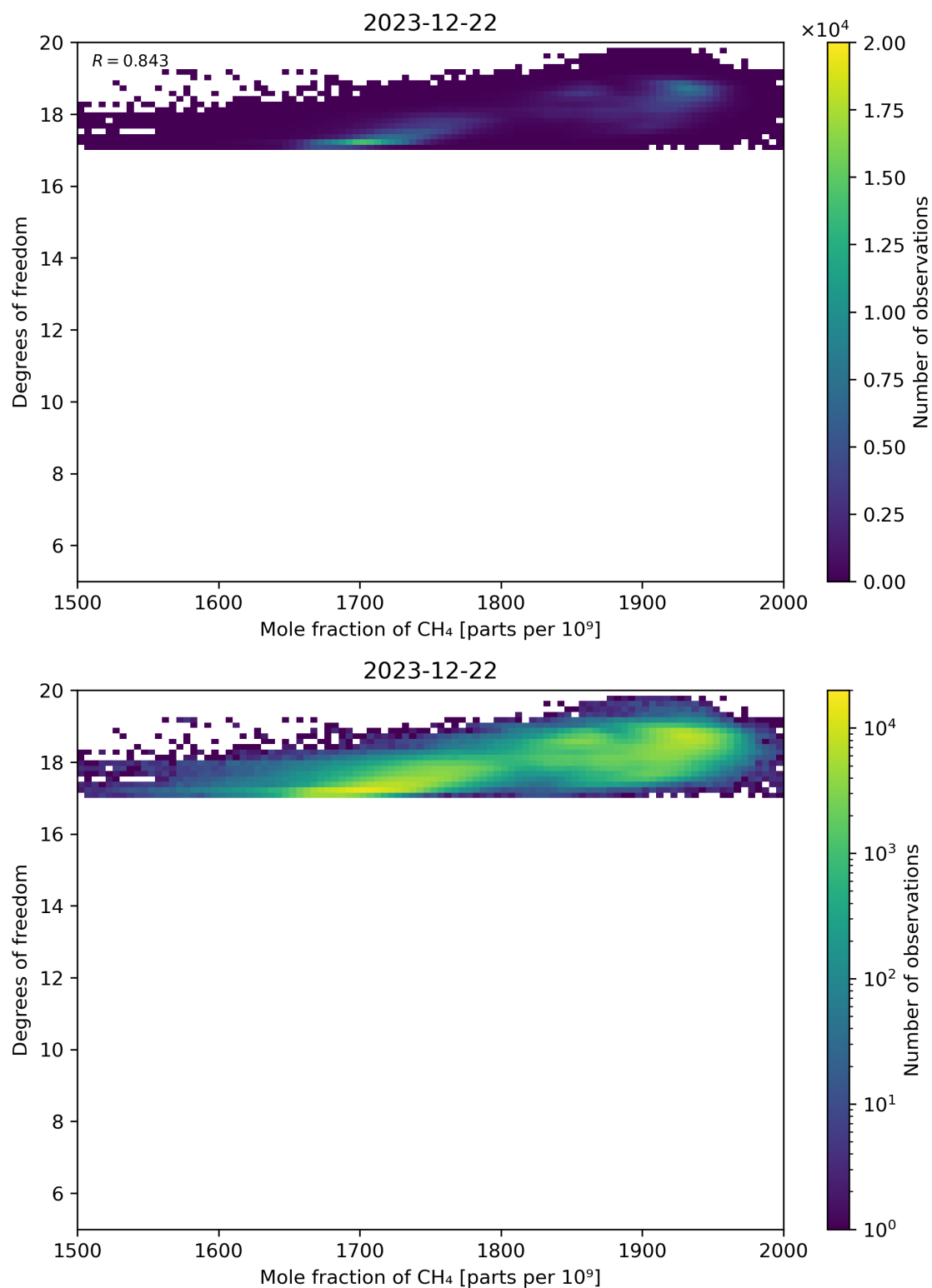
Figure 72: Scatter density plot of “Mole fraction of CH 4 ” against “Degrees of freedom” for 2023-12-21 to 2023-12-23.
