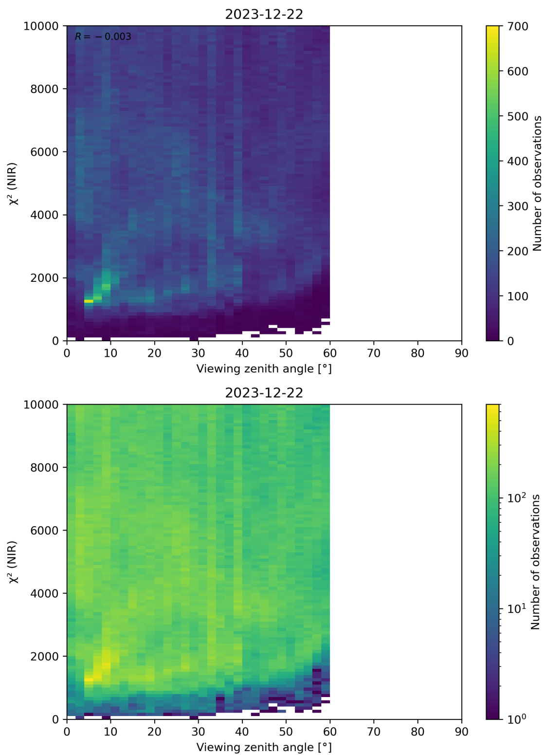
Figure 105: Scatter density plot of “Viewing zenith angle” against “ \chi^2 (NIR)” for 2023-12-21 to 2023-12-23.
