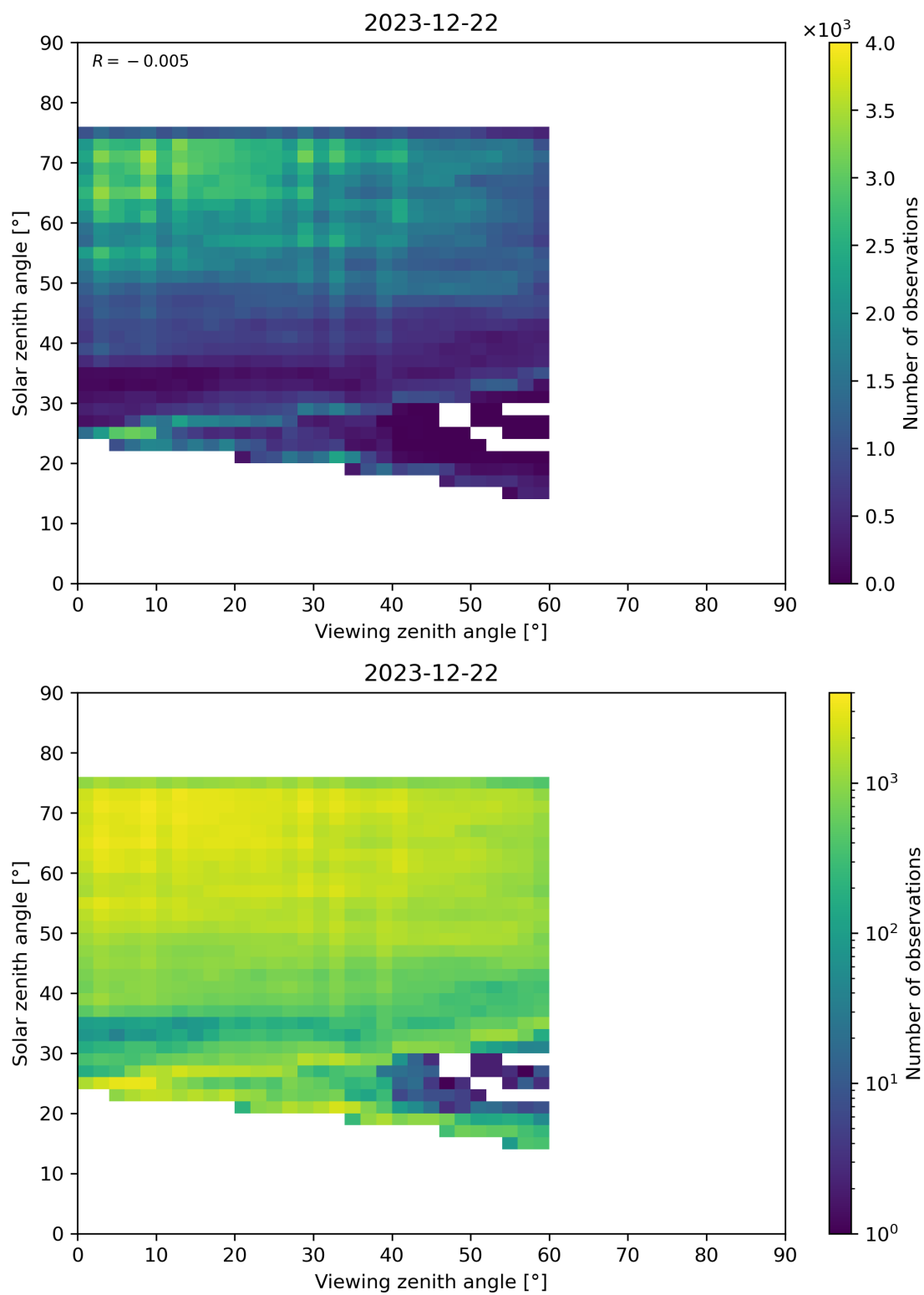
Figure 115: Scatter density plot of “Viewing zenith angle” against “Solar zenith angle” for 2023-12-21 to 2023-12-23.
