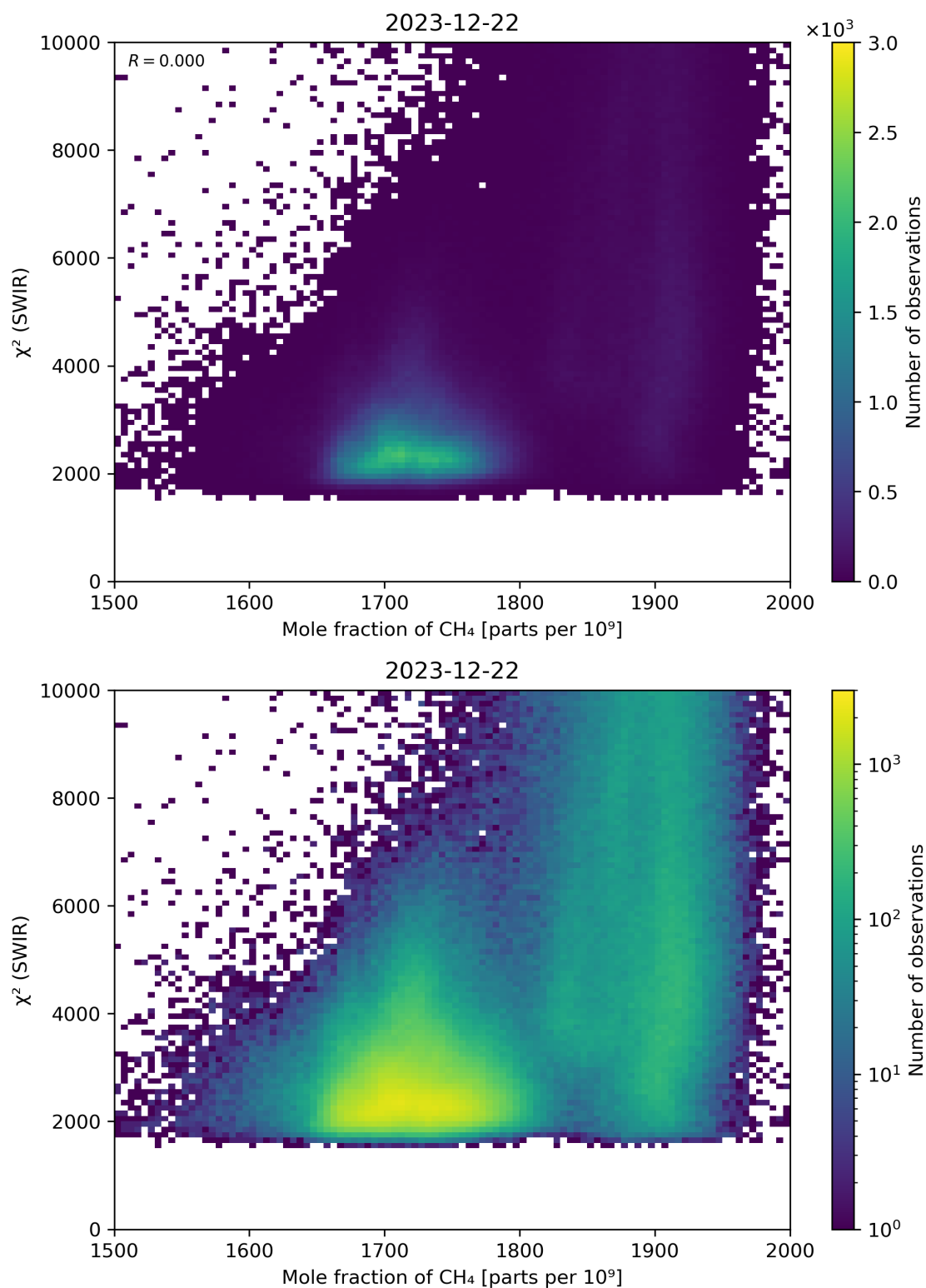
Figure 71: Scatter density plot of “Mole fraction of \text{CH}_4 ” against “ \chi^2 (SWIR)” for 2023-12-21 to 2023-12-23.
