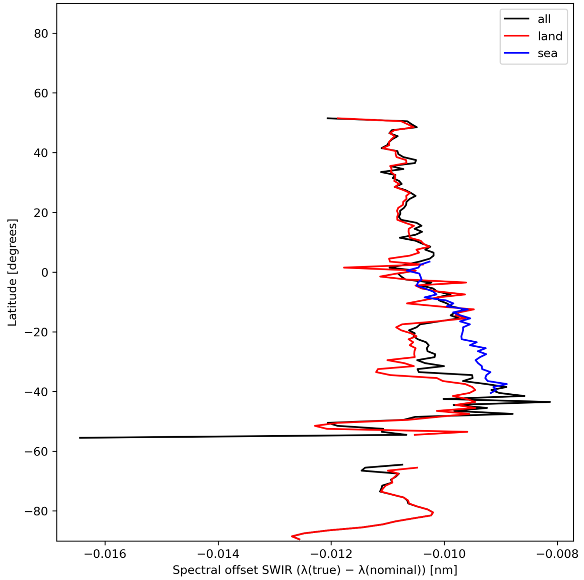
Figure 16: Zonal average of “Spectral offset SWIR ( \lambda(\text{true}) - \lambda(\text{nominal}) )” for 2023-12-21 to 2023-12-23.
