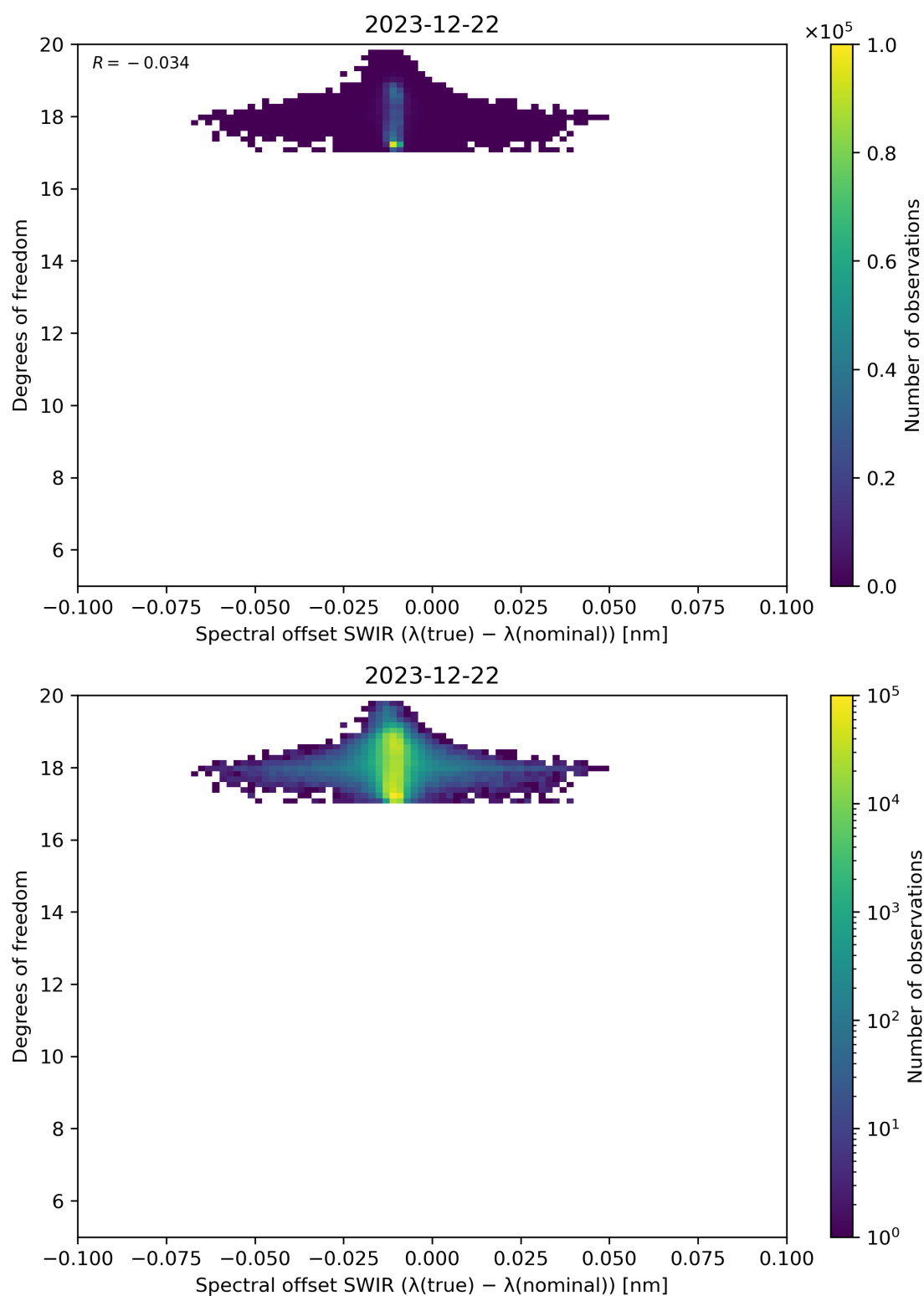
Figure 119: Scatter density plot of “Spectral offset SWIR ( \lambda(\text{true}) - \lambda(\text{nominal}) )” against “Degrees of freedom” for 2023-12-21 to 2023-12-23.
