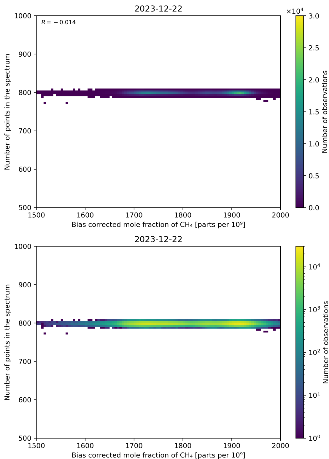
Figure 68: Scatter density plot of “Bias corrected mole fraction of CH 4 ” against “Number of points in the spectrum” for 2023-12-21 to 2023-12-23.
