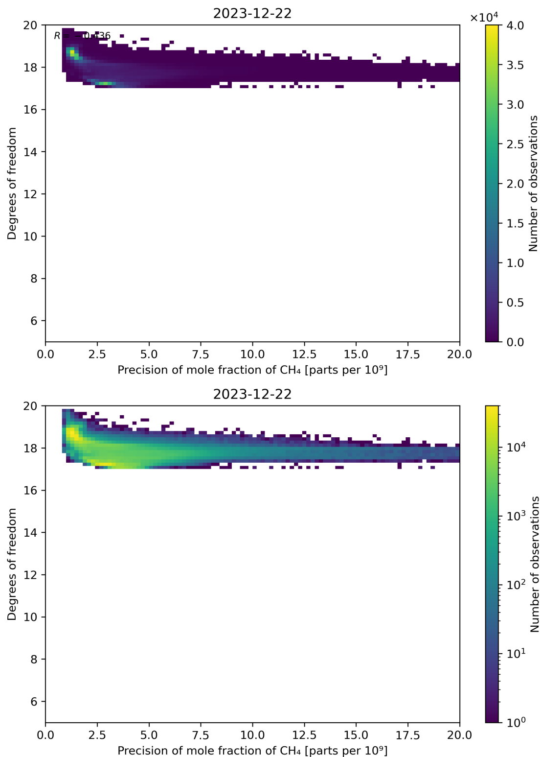
Figure 80: Scatter density plot of “Precision of mole fraction of CH 4 ” against “Degrees of freedom” for 2023-12-21 to 2023-12-23.
