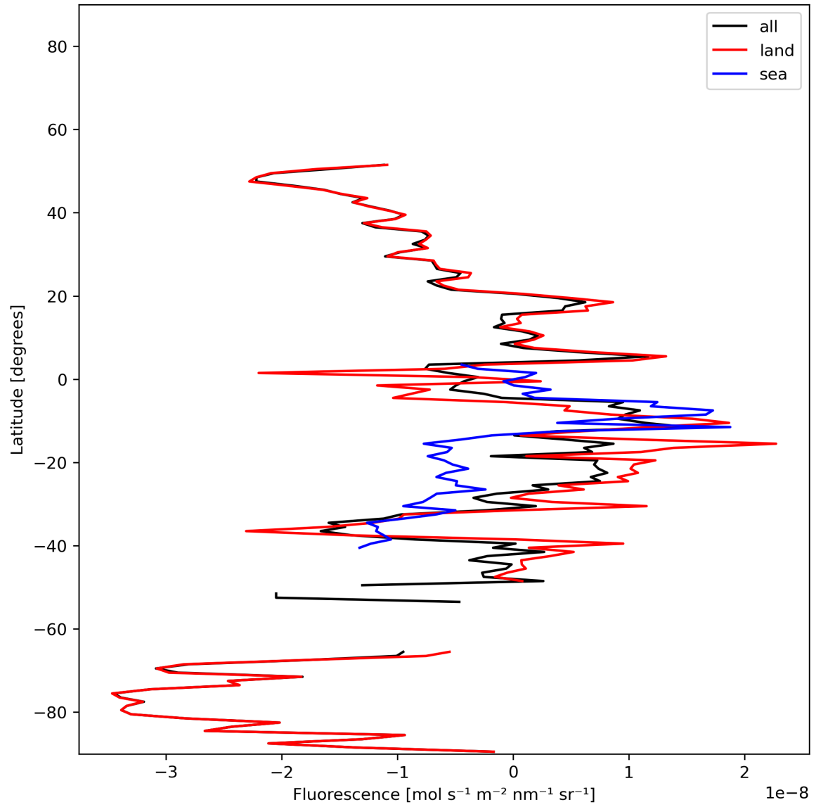
Figure 21: Zonal average of “Fluorescence” for 2023-12-22 to 2023-12-24.
