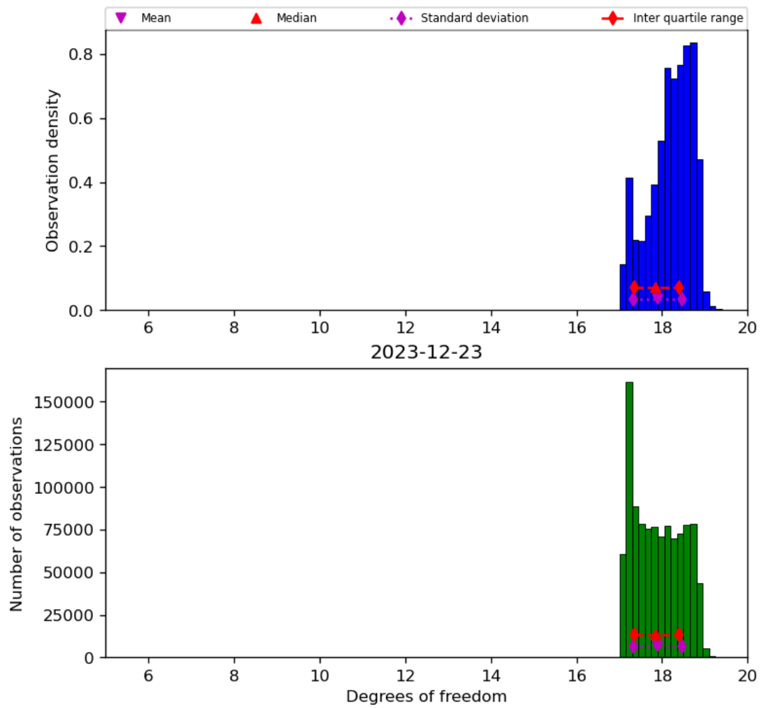
Figure 30: Histogram of “Degrees of freedom” for 2023-12-22 to 2023-12-24
