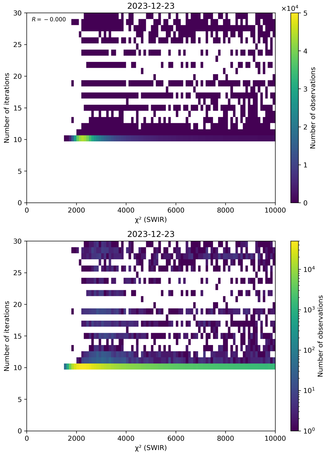
Figure 50: Scatter density plot of “ \chi^2 (SWIR)” against “Number of iterations” for 2023-12-22 to 2023-12-24.
