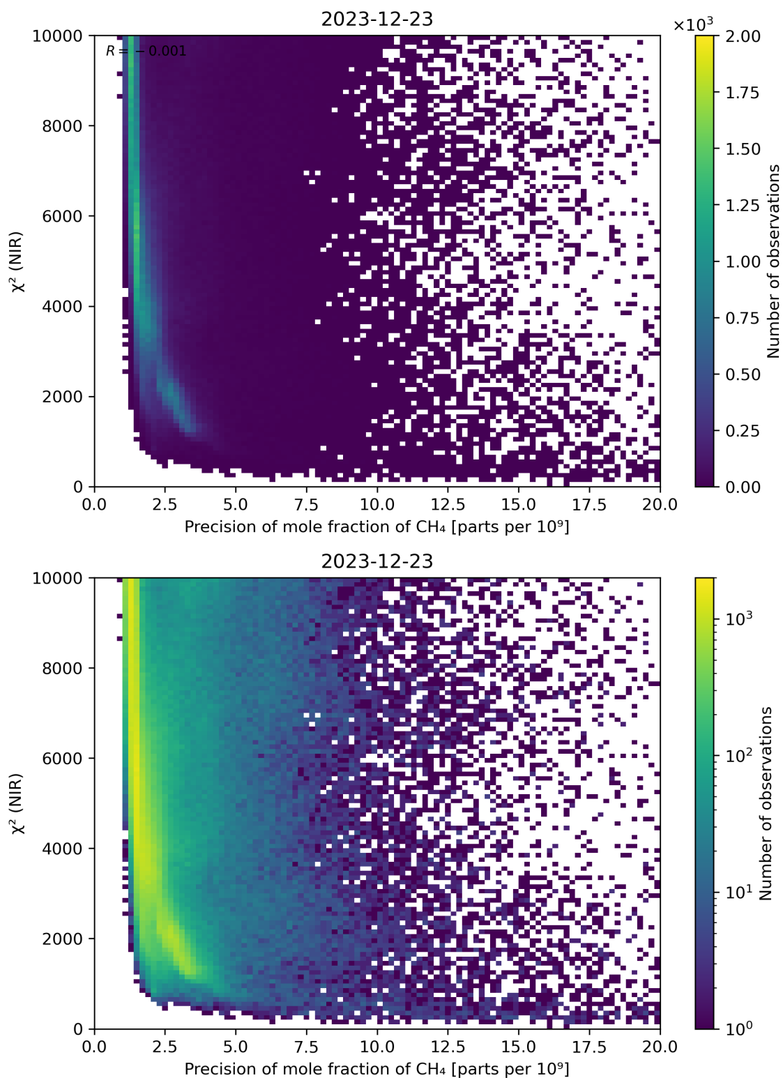
Figure 78: Scatter density plot of “Precision of mole fraction of CH 4 ” against “ \chi^2 (NIR)” for 2023-12-22 to 2023-12-24.
