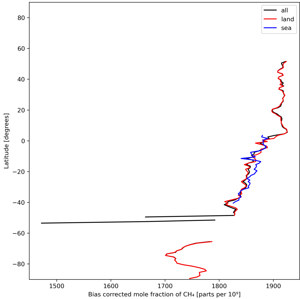
Figure 14: Zonal average of “Bias corrected mole fraction of CH 4 ” for 2023-12-22 to 2023-12-24.
