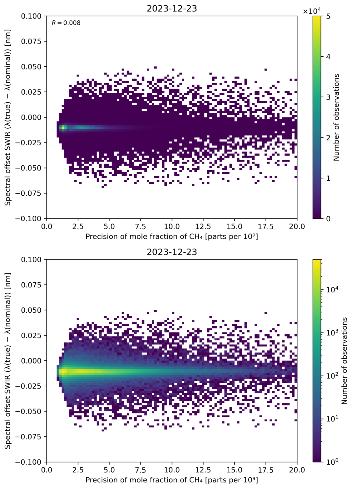
Figure 85: Scatter density plot of “Precision of mole fraction of \text{CH}_4 ” against “Spectral offset SWIR ( \lambda(\text{true}) - \lambda(\text{nominal}) )” for 2023-12-22 to 2023-12-24.
