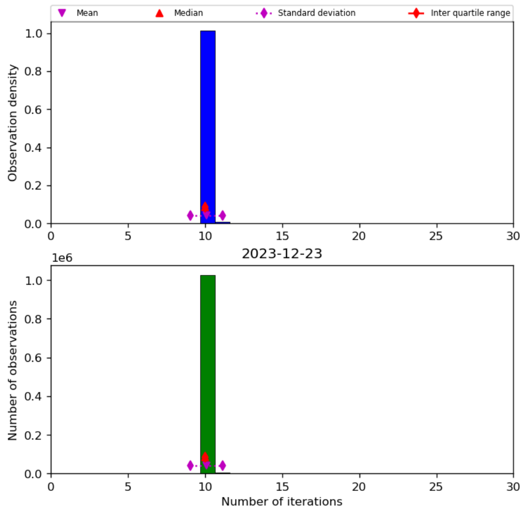
Figure 31: Histogram of “Number of iterations” for 2023-12-22 to 2023-12-24
