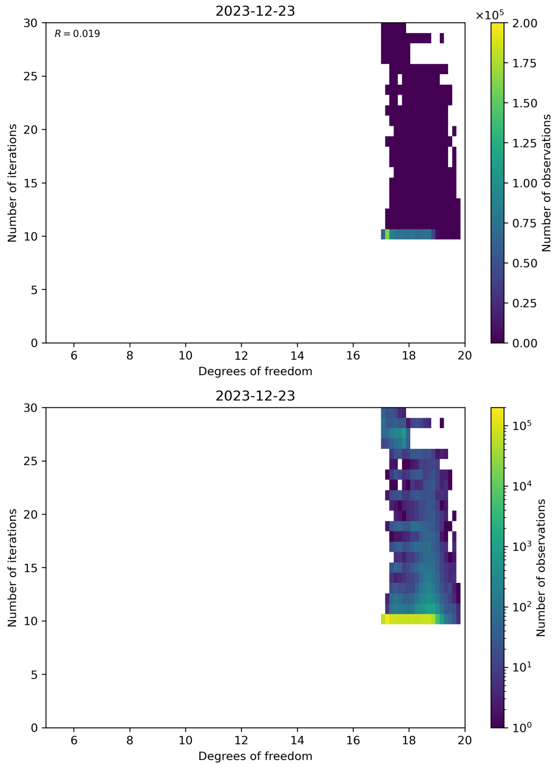
Figure 52: Scatter density plot of “Degrees of freedom” against “Number of iterations” for 2023-12-22 to 2023-12-24.
