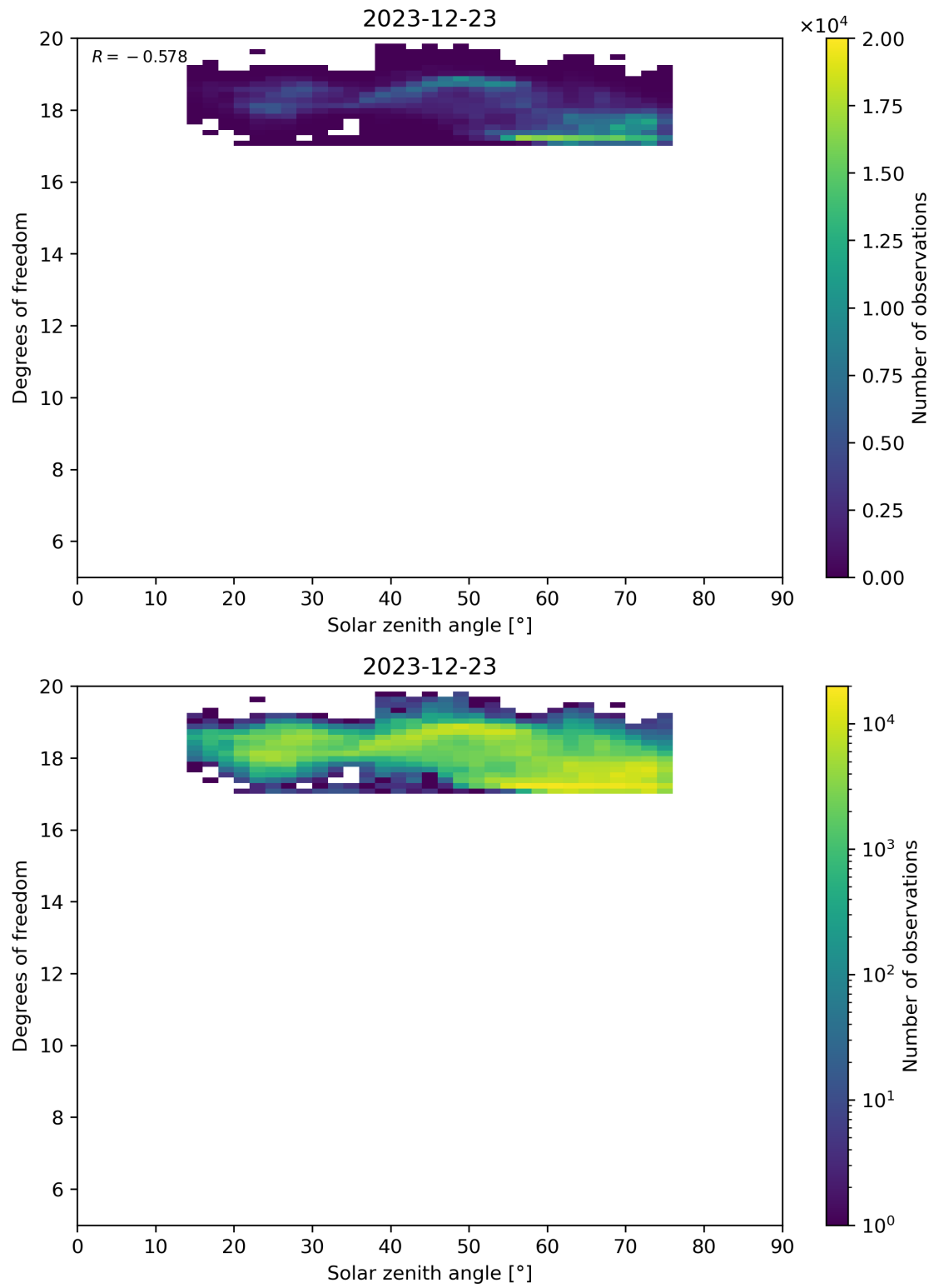
Figure 96: Scatter density plot of “Solar zenith angle” against “Degrees of freedom” for 2023-12-22 to 2023-12-24.
