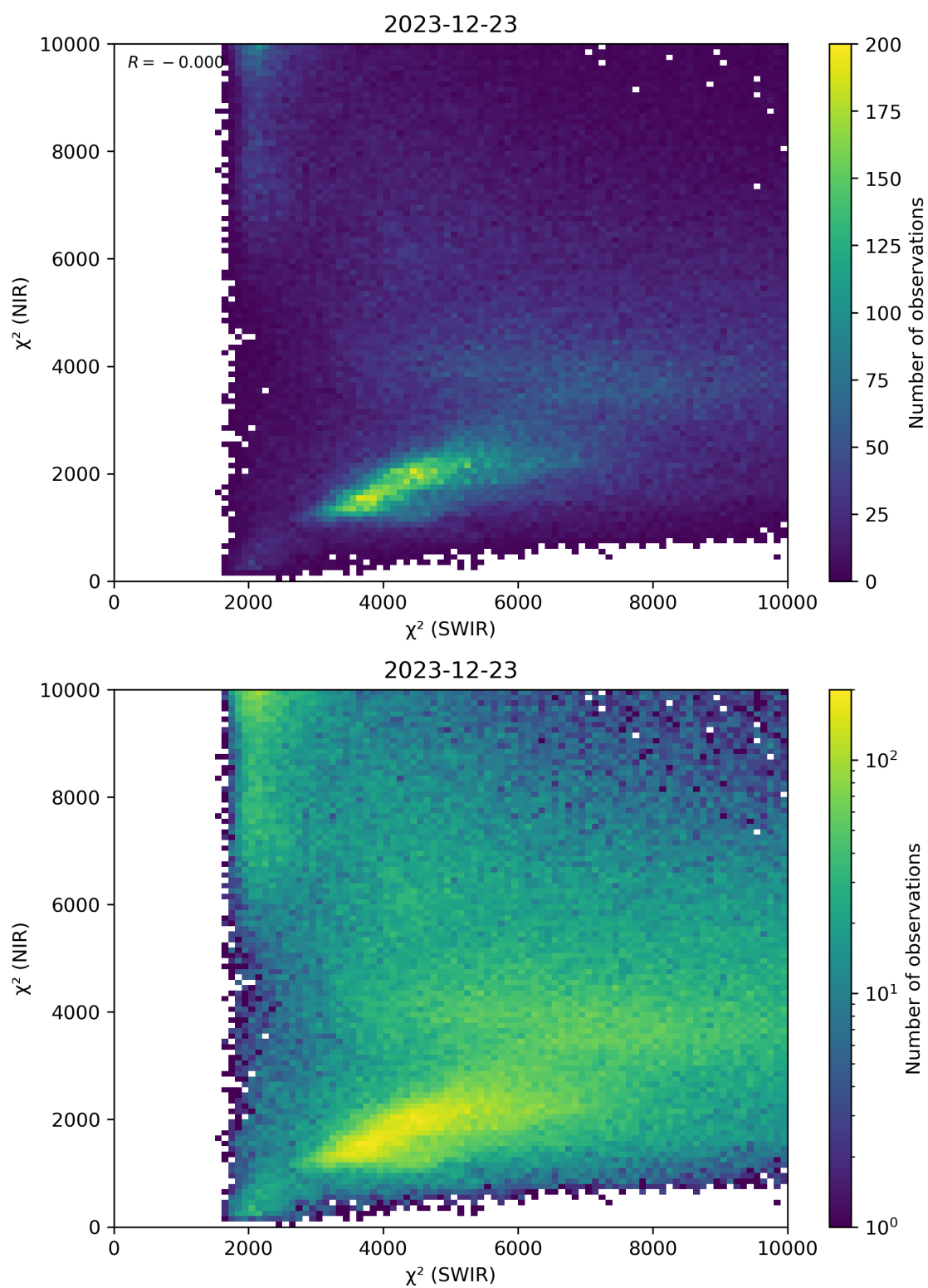
Figure 47: Scatter density plot of “ \chi^2 (SWIR)” against “ \chi^2 (NIR)” for 2023-12-22 to 2023-12-24.
