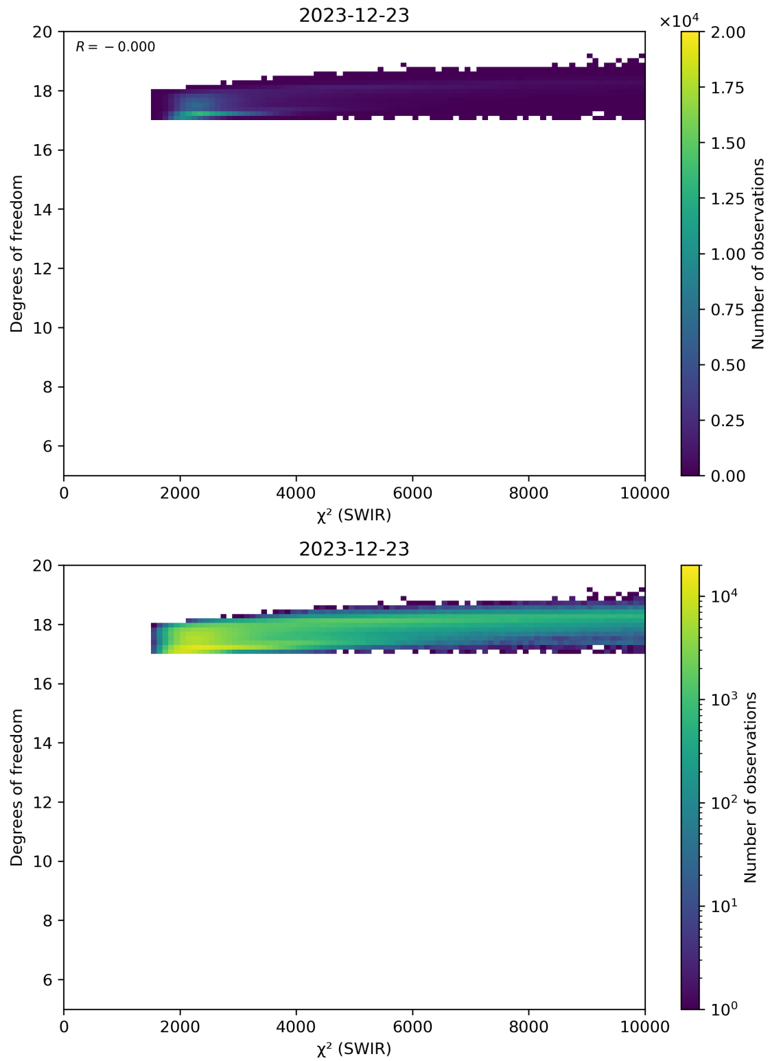
Figure 48: Scatter density plot of “ \chi^2 (SWIR)” against “Degrees of freedom” for 2023-12-22 to 2023-12-24.
