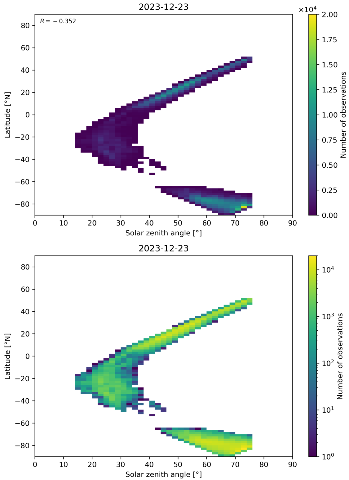
Figure 98: Scatter density plot of “Solar zenith angle” against “Latitude” for 2023-12-22 to 2023-12-24.
