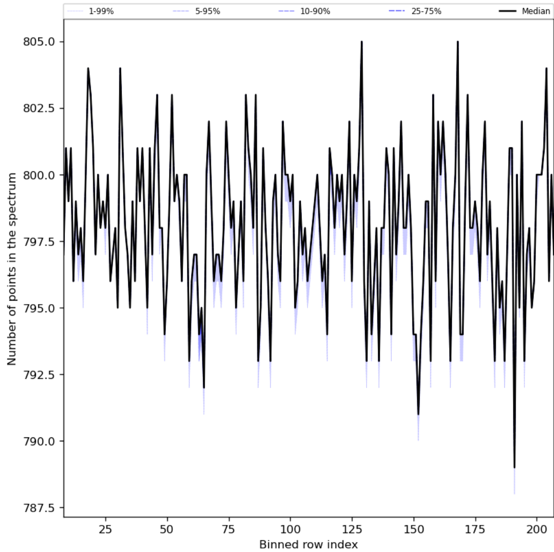
Figure 37: Along track statistics of “Number of points in the spectrum” for 2023-12-22 to 2023-12-24
