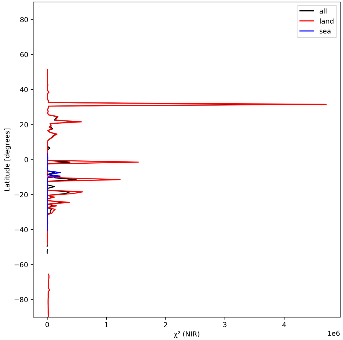
Figure 18: Zonal average of “ \chi^2 (NIR)” for 2023-12-22 to 2023-12-24.
