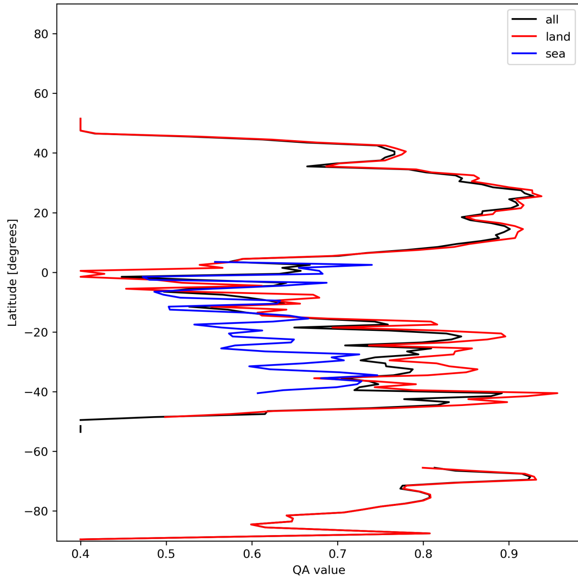
Figure 11: Zonal average of “QA value” for 2023-12-22 to 2023-12-24.
