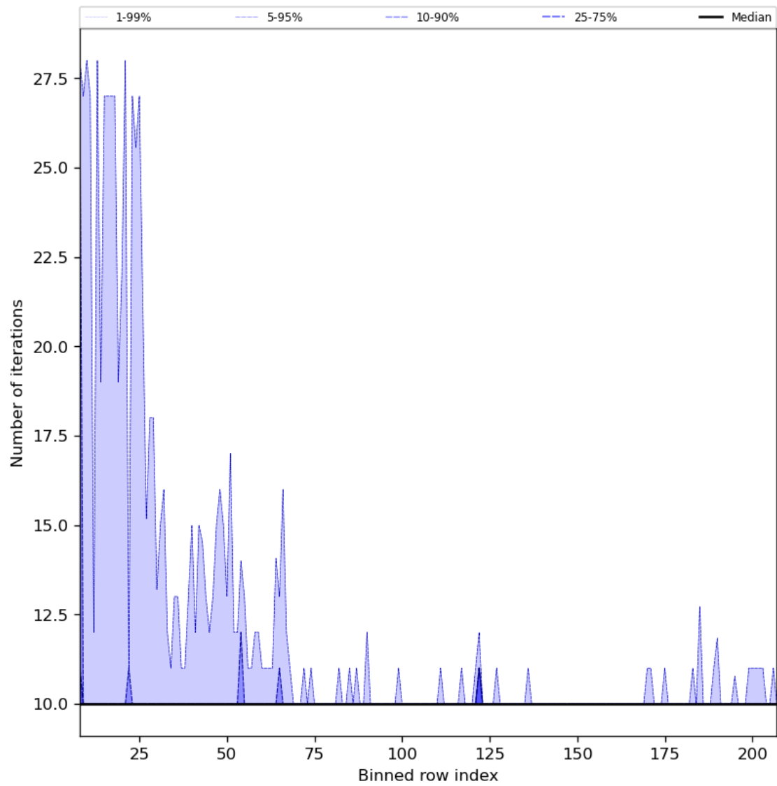
Figure 42: Along track statistics of “Number of iterations” for 2023-12-22 to 2023-12-24
