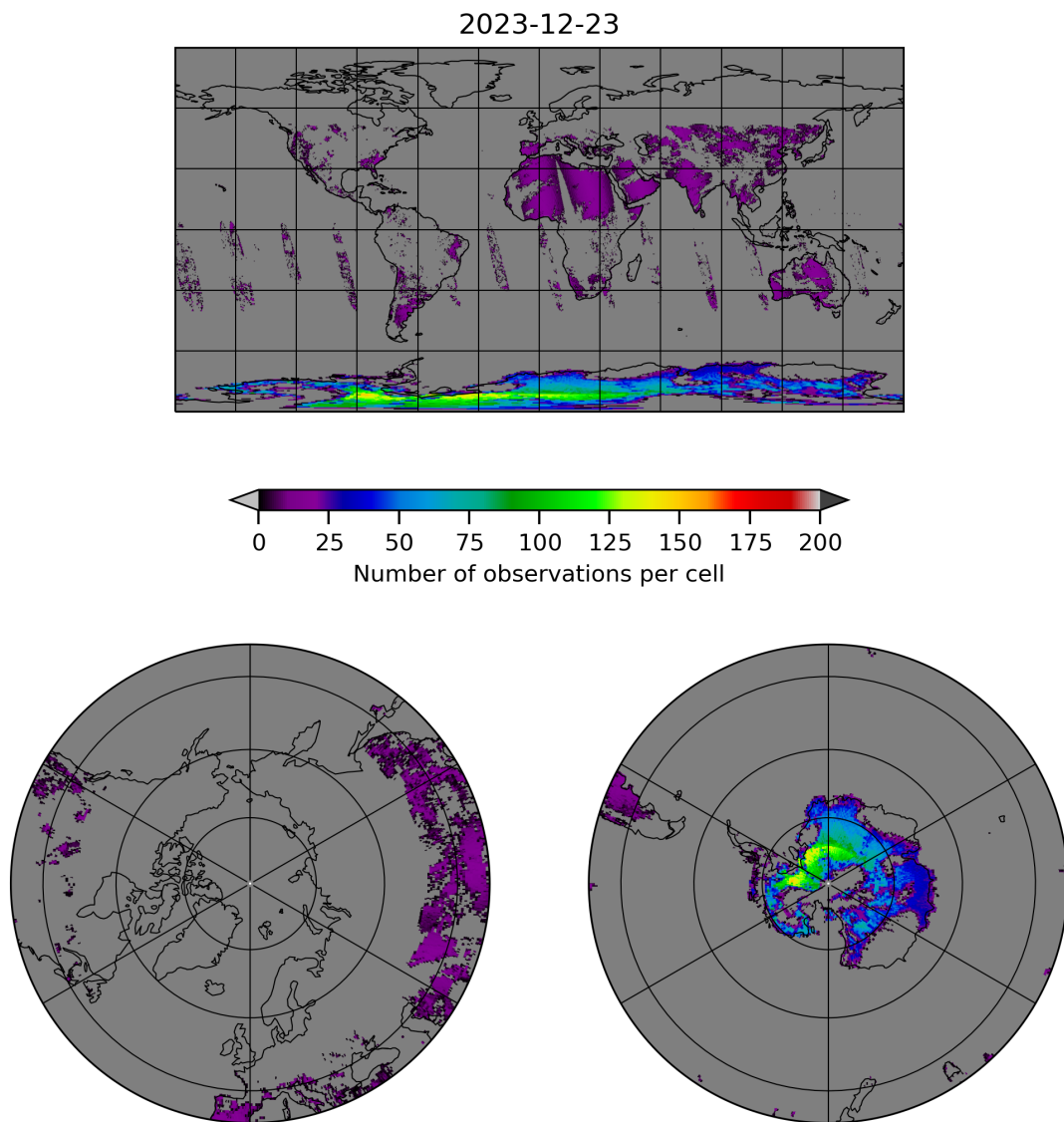
Figure 10: Map of the number of observations for 2023-12-22 to 2023-12-24
