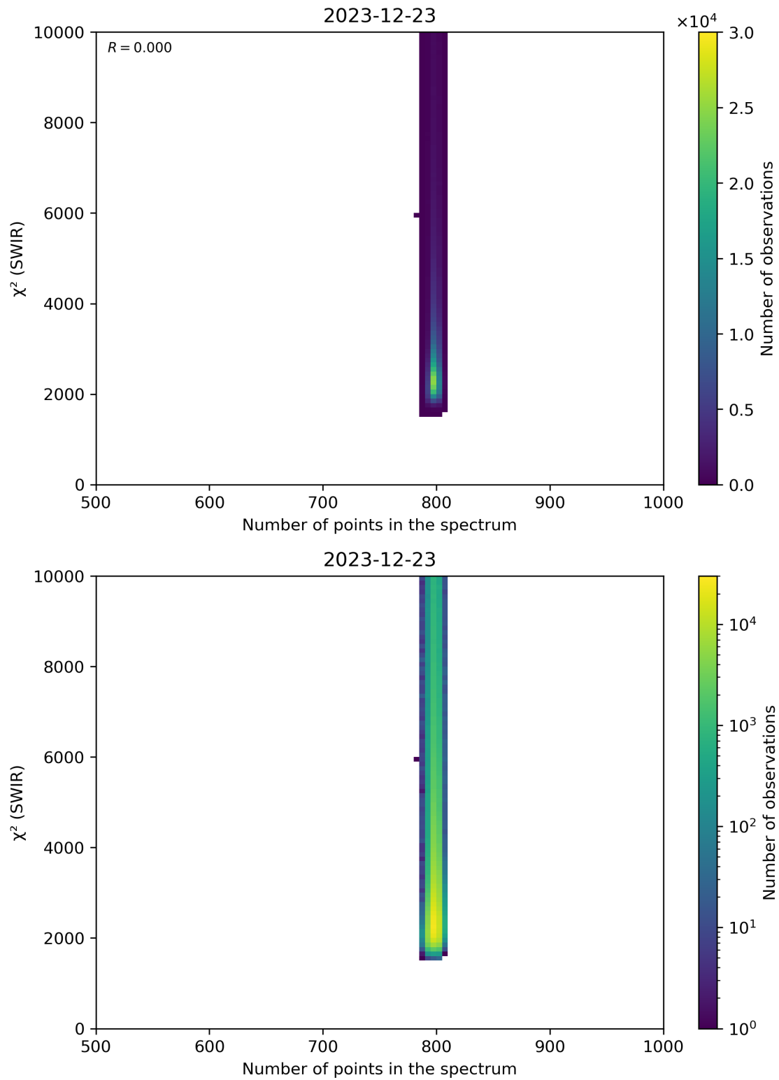
Figure 89: Scatter density plot of “Number of points in the spectrum” against “ \chi^2 (SWIR)” for 2023-12-22 to 2023-12-24.
