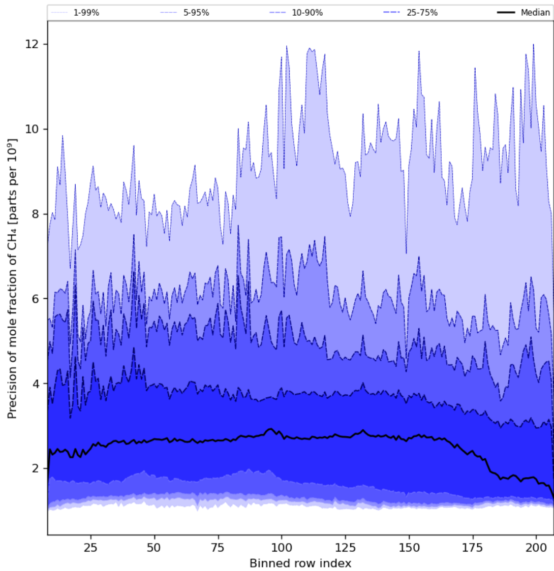
Figure 35: Along track statistics of “Precision of mole fraction of CH 4 ” for 2023-12-22 to 2023-12-24
