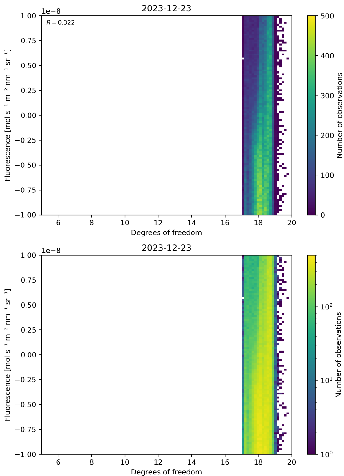
Figure 51: Scatter density plot of “Degrees of freedom” against “Fluorescence” for 2023-12-22 to 2023-12-24.
