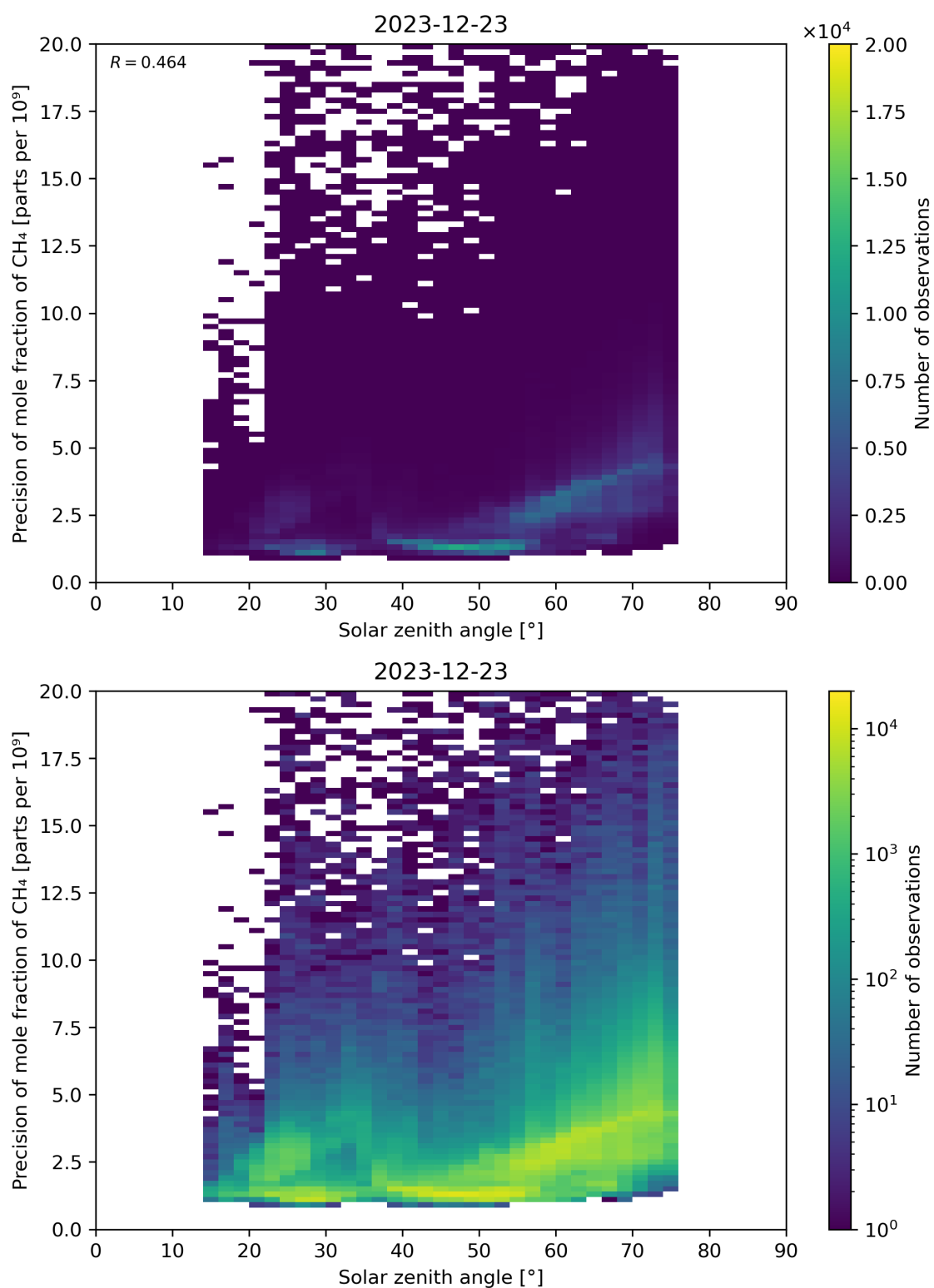
Figure 101: Scatter density plot of “Solar zenith angle” against “Precision of mole fraction of CH 4 ” for 2023-12-22 to 2023-12-24.
