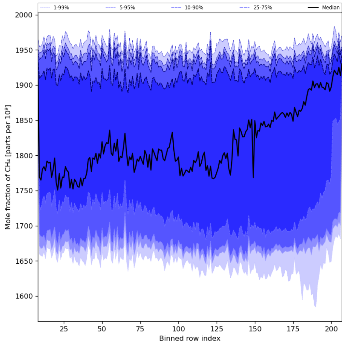
Figure 34: Along track statistics of “Mole fraction of CH 4 ” for 2023-12-22 to 2023-12-24
