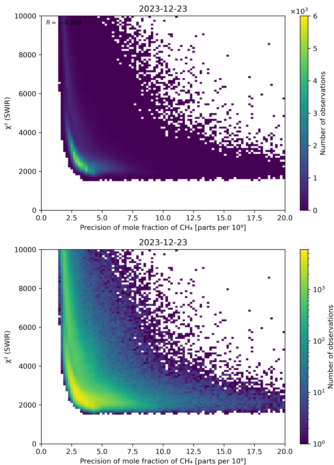
Figure 79: Scatter density plot of “Precision of mole fraction of CH 4 ” against “ \chi^2 (SWIR)” for 2023-12-22 to 2023-12-24.
