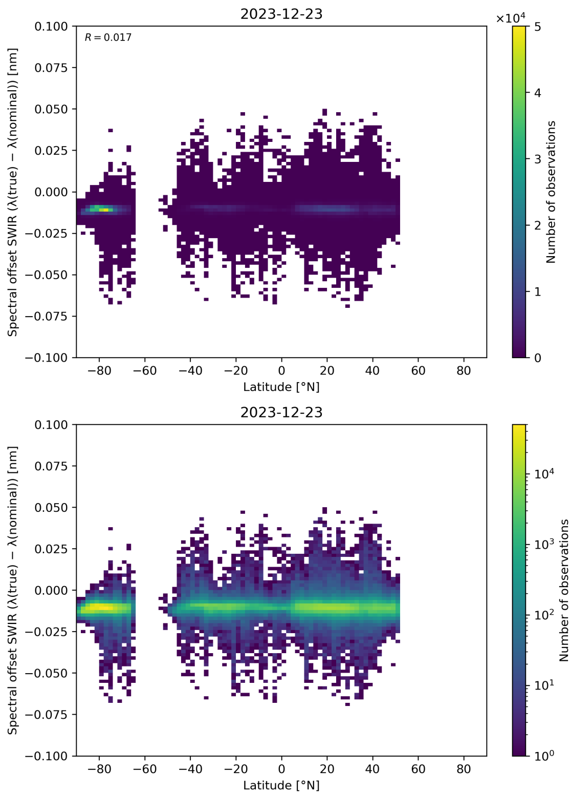
Figure 62: Scatter density plot of “Latitude” against “Spectral offset SWIR ( \lambda(\text{true}) - \lambda(\text{nominal}) )” for 2023-12-22 to 2023-12-24.
