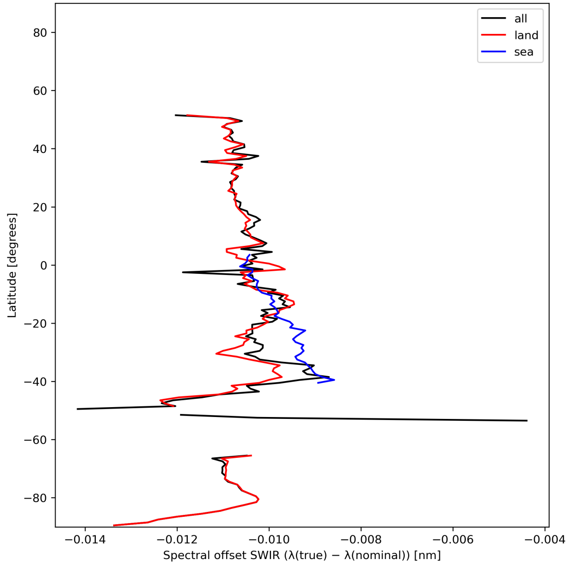
Figure 16: Zonal average of “Spectral offset SWIR ( \lambda(\text{true}) - \lambda(\text{nominal}) )” for 2023-12-22 to 2023-12-24.
