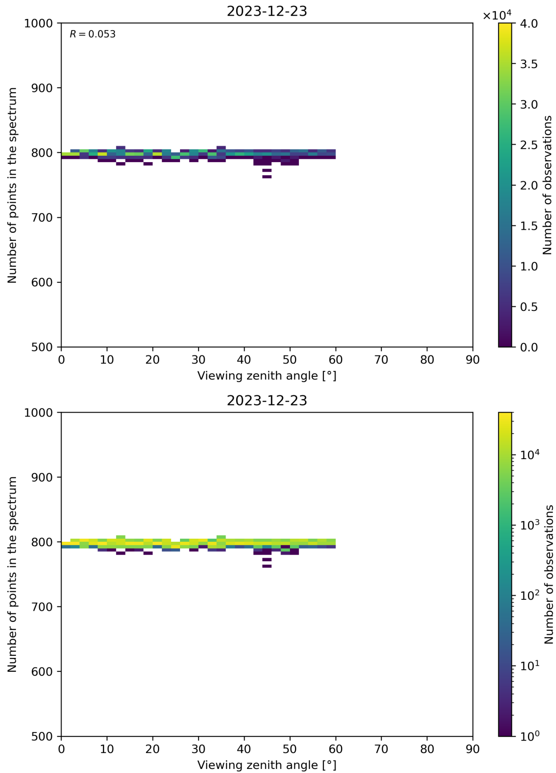
Figure 114: Scatter density plot of “Viewing zenith angle” against “Number of points in the spectrum” for 2023-12-22 to 2023-12-24.
