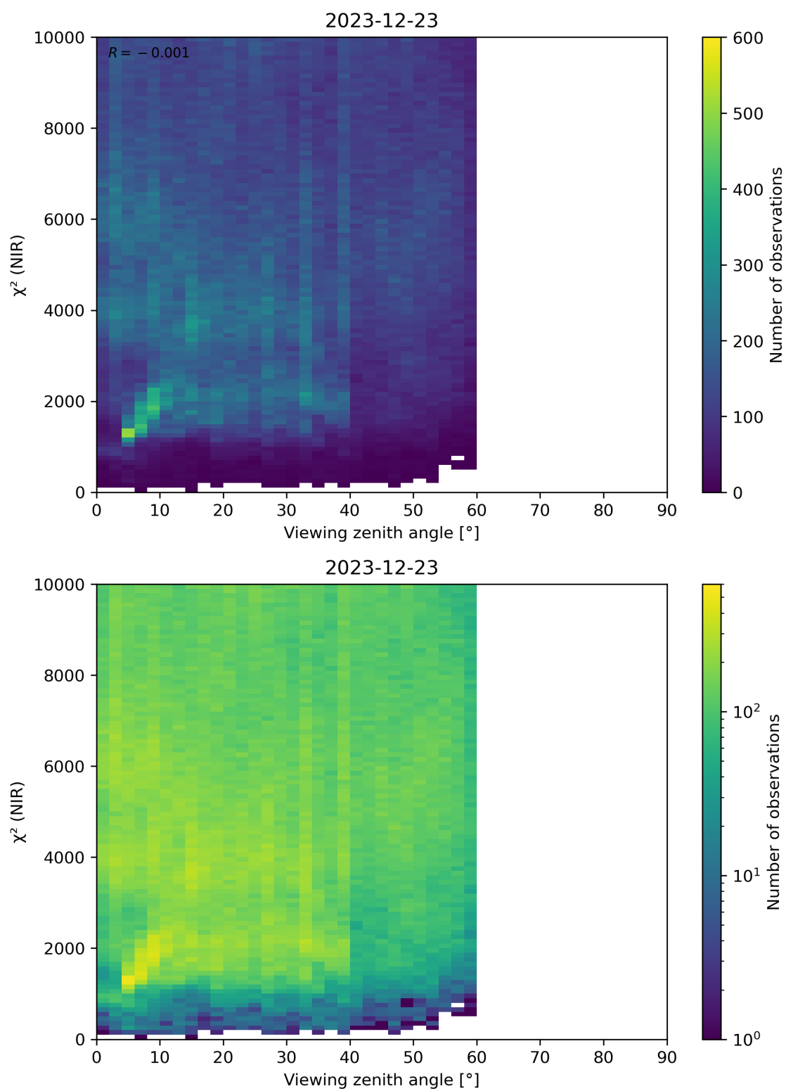
Figure 105: Scatter density plot of “Viewing zenith angle” against “ \chi^2 (NIR)” for 2023-12-22 to 2023-12-24.
