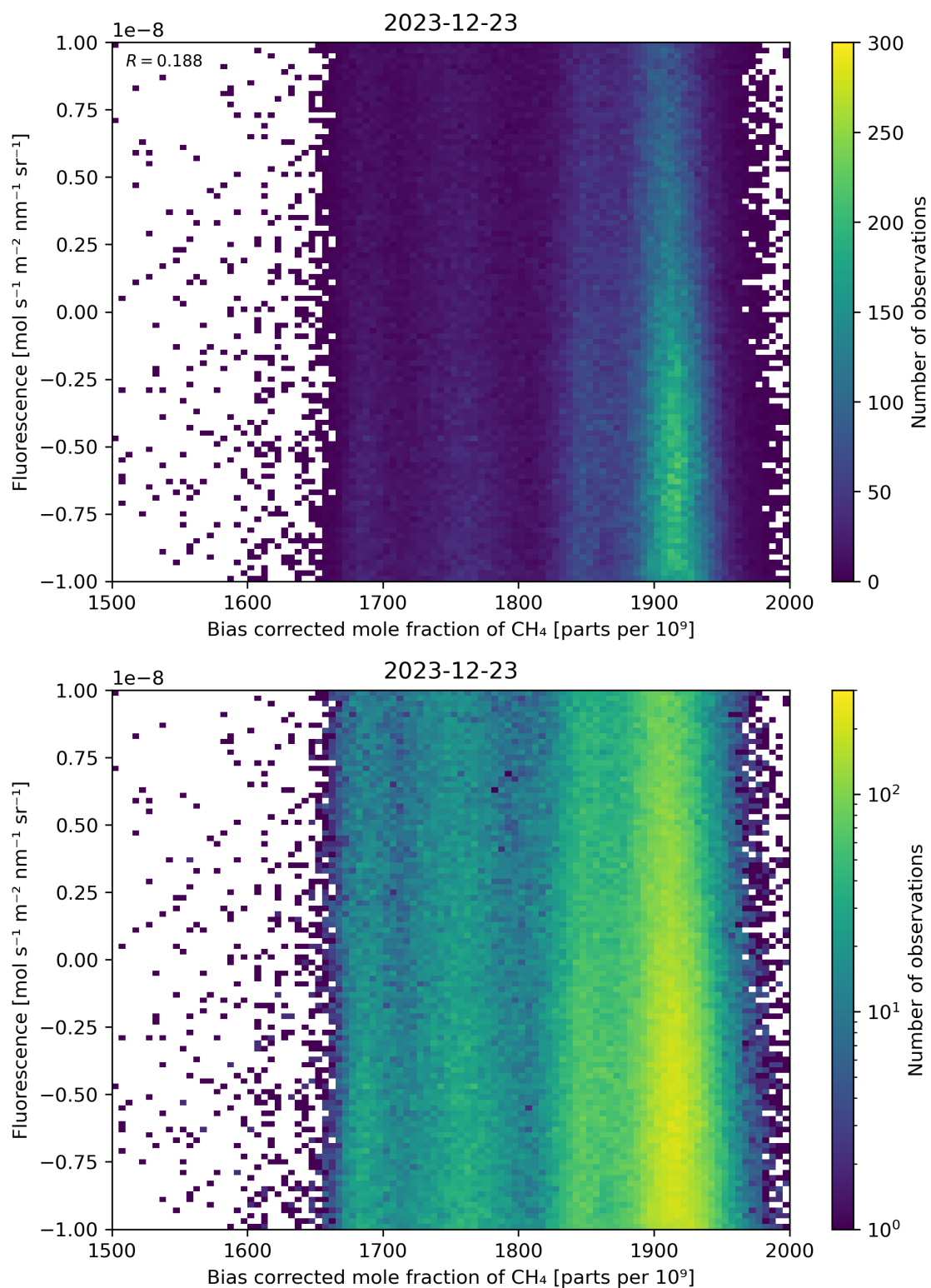
Figure 66: Scatter density plot of “Bias corrected mole fraction of \text{CH}_4 ” against “Fluorescence” for 2023-12-22 to 2023-12-24.
