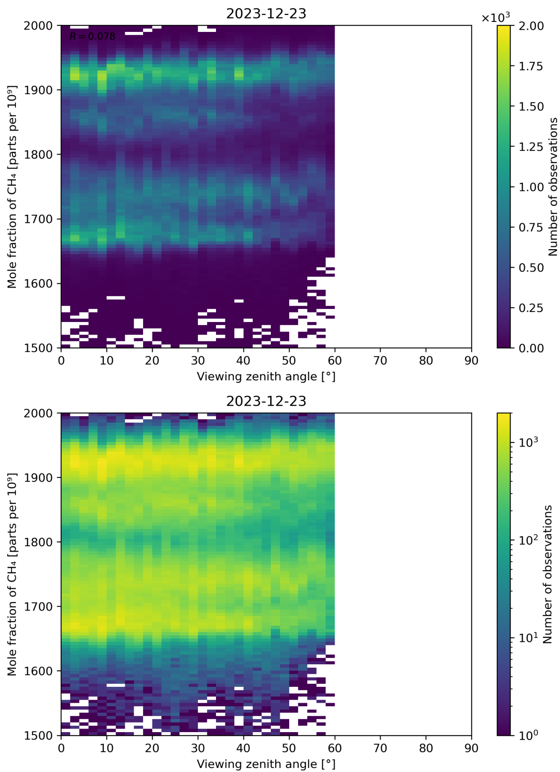
Figure 110: Scatter density plot of “Viewing zenith angle” against “Mole fraction of \text{CH}_4 ” for 2023-12-22 to 2023-12-24.
