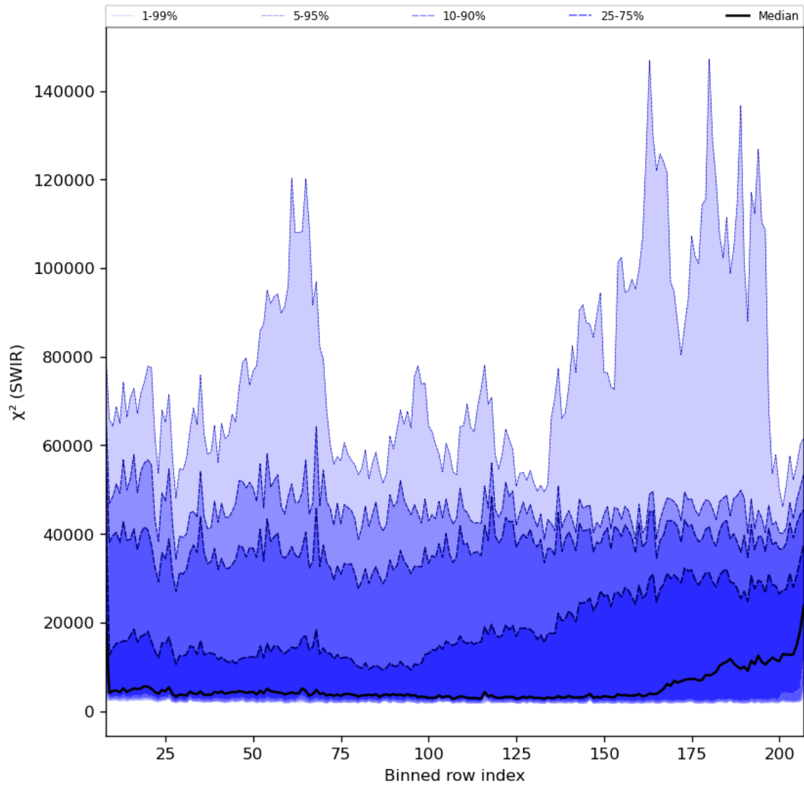
Figure 39: Along track statistics of " \chi^2 (SWIR)" for 2023-12-22 to 2023-12-24
