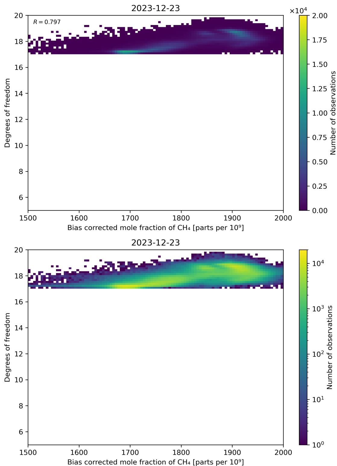
Figure 65: Scatter density plot of “Bias corrected mole fraction of CH 4 ” against “Degrees of freedom” for 2023-12-22 to 2023-12-24.
