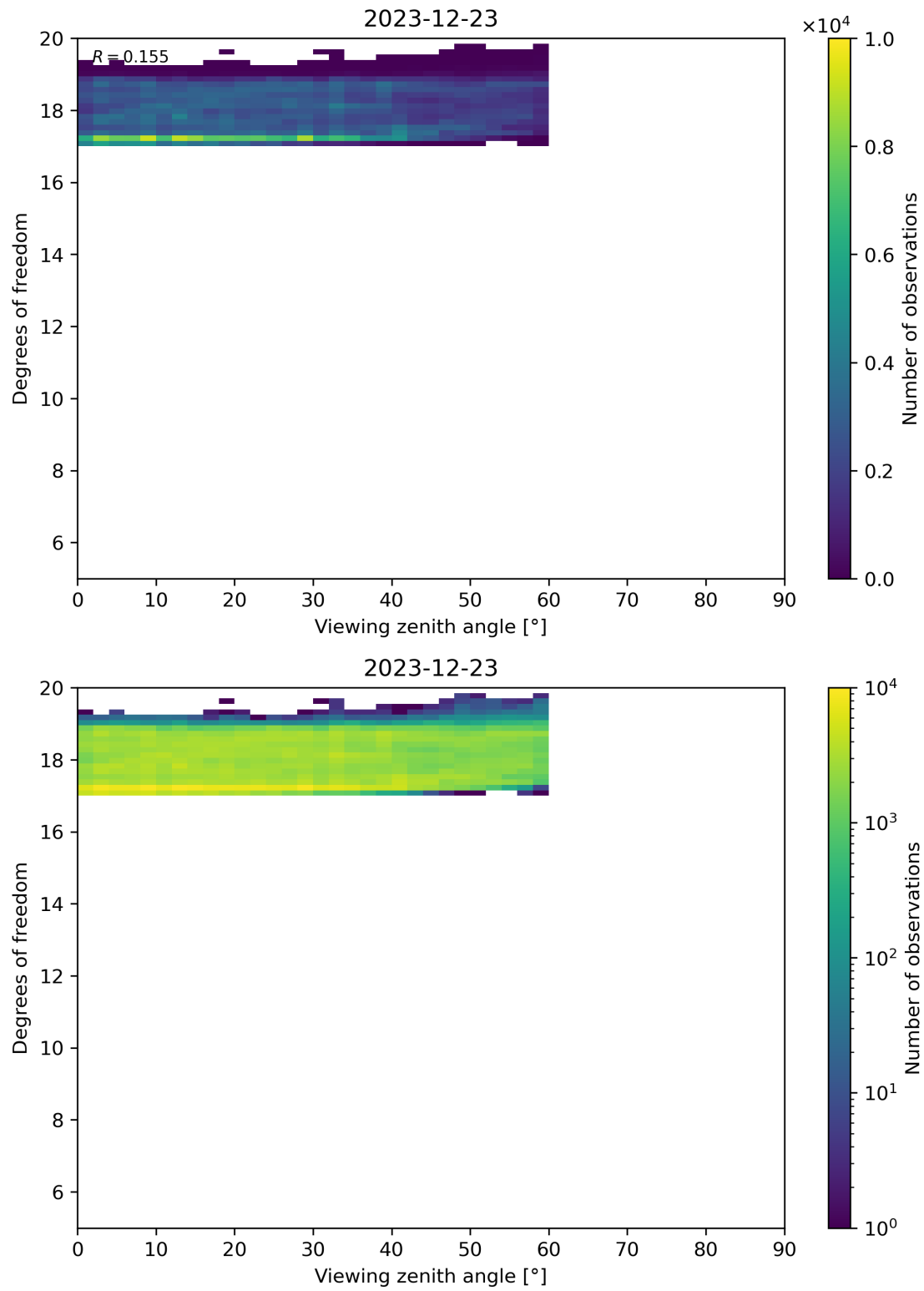
Figure 107: Scatter density plot of “Viewing zenith angle” against “Degrees of freedom” for 2023-12-22 to 2023-12-24.
