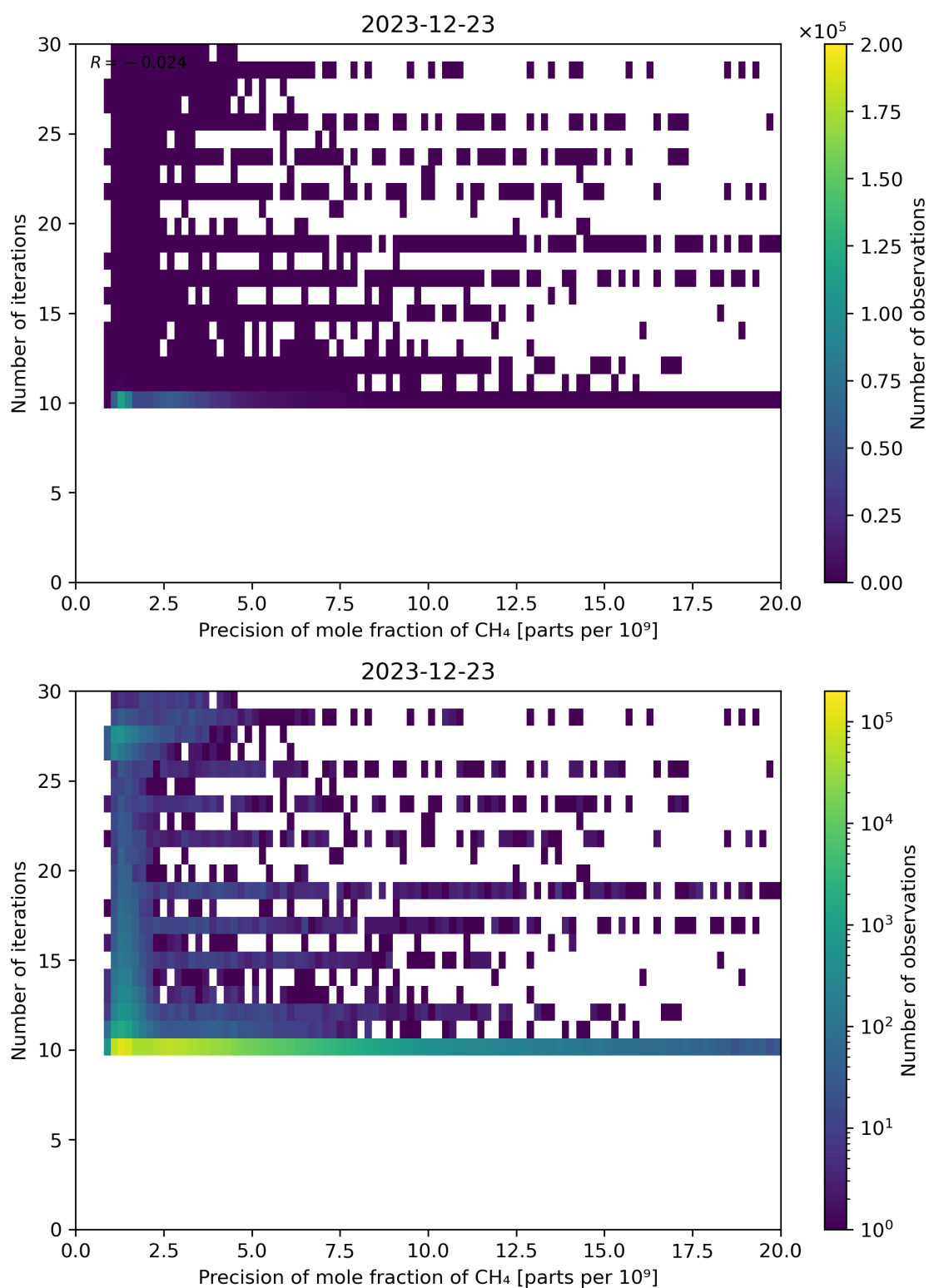
Figure 83: Scatter density plot of “Precision of mole fraction of CH 4 ” against “Number of iterations” for 2023-12-22 to 2023-12-24.
