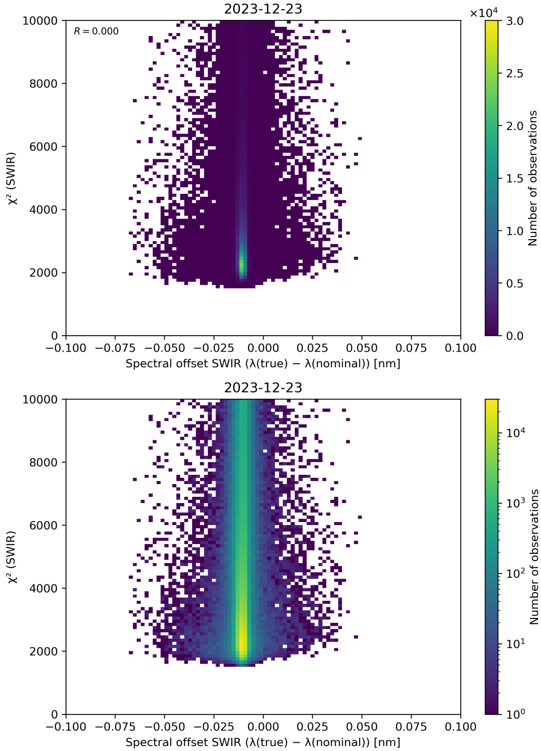
Figure 118: Scatter density plot of “Spectral offset SWIR ( \lambda(\text{true}) - \lambda(\text{nominal}) )” against “ \chi^2 (SWIR)” for 2023-12-22 to 2023-12-24.
