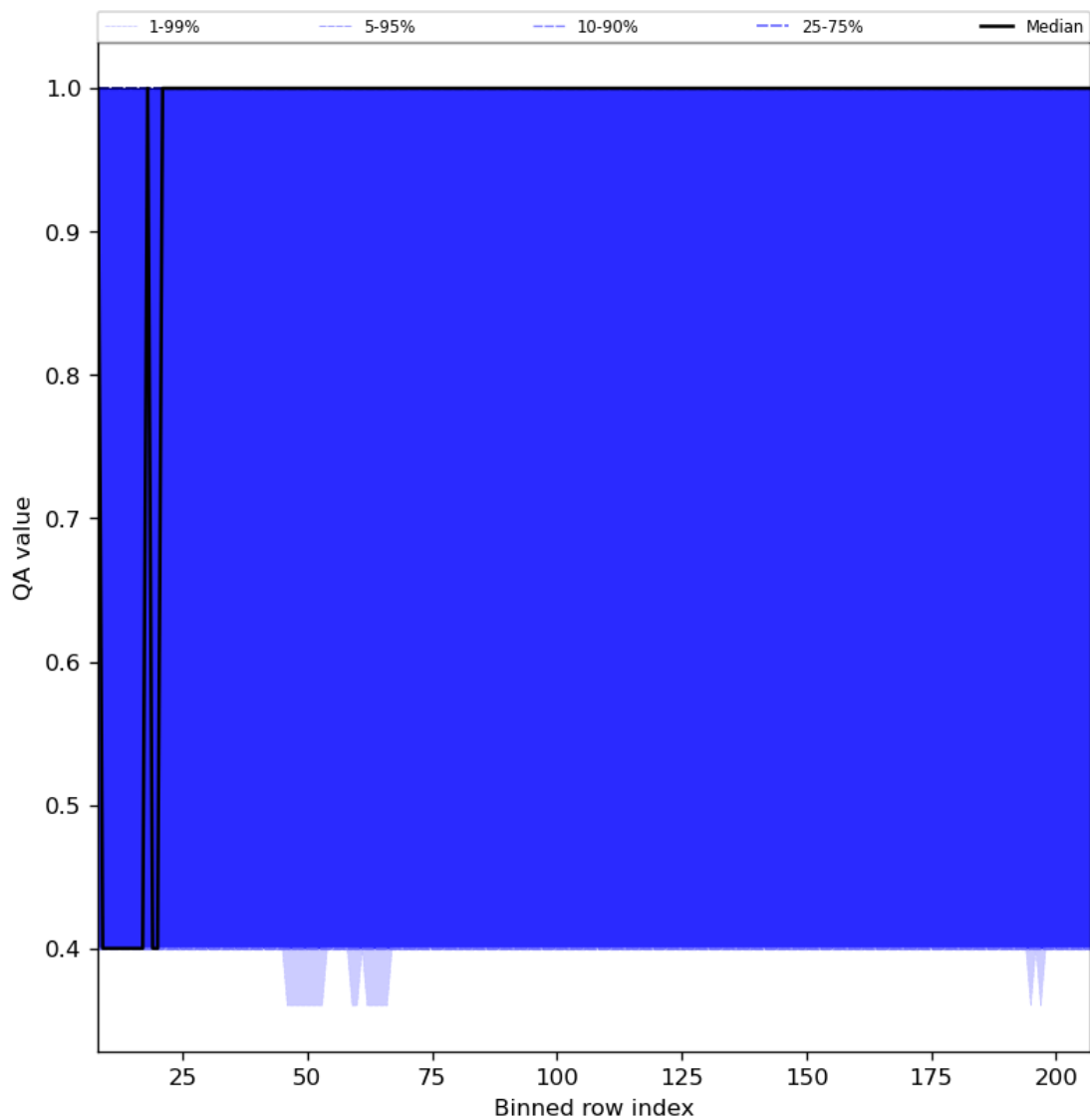
Figure 33: Along track statistics of “QA value” for 2023-12-22 to 2023-12-24
