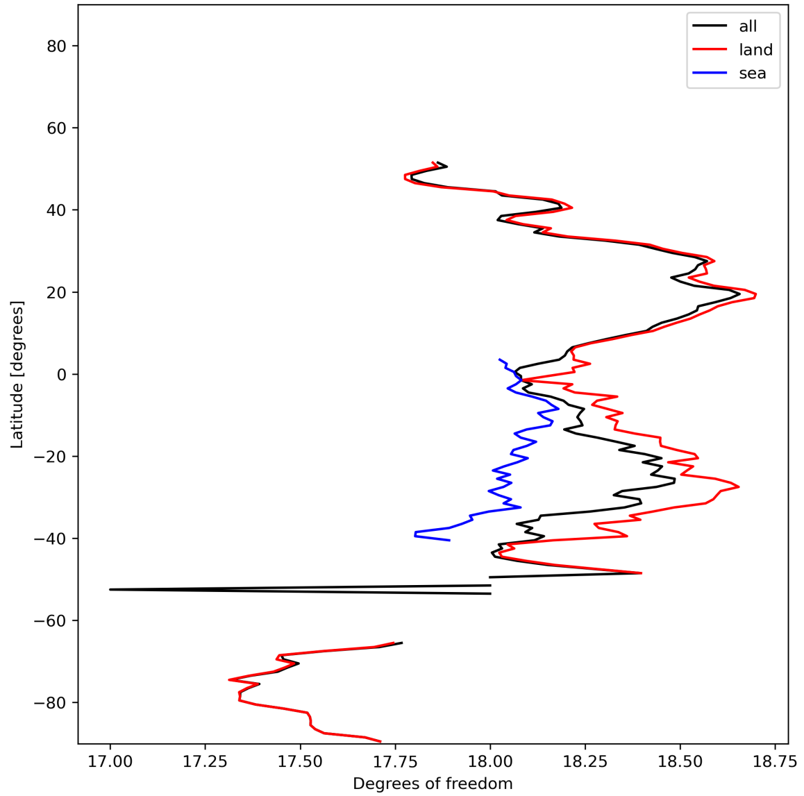
Figure 19: Zonal average of “Degrees of freedom” for 2023-12-22 to 2023-12-24.
