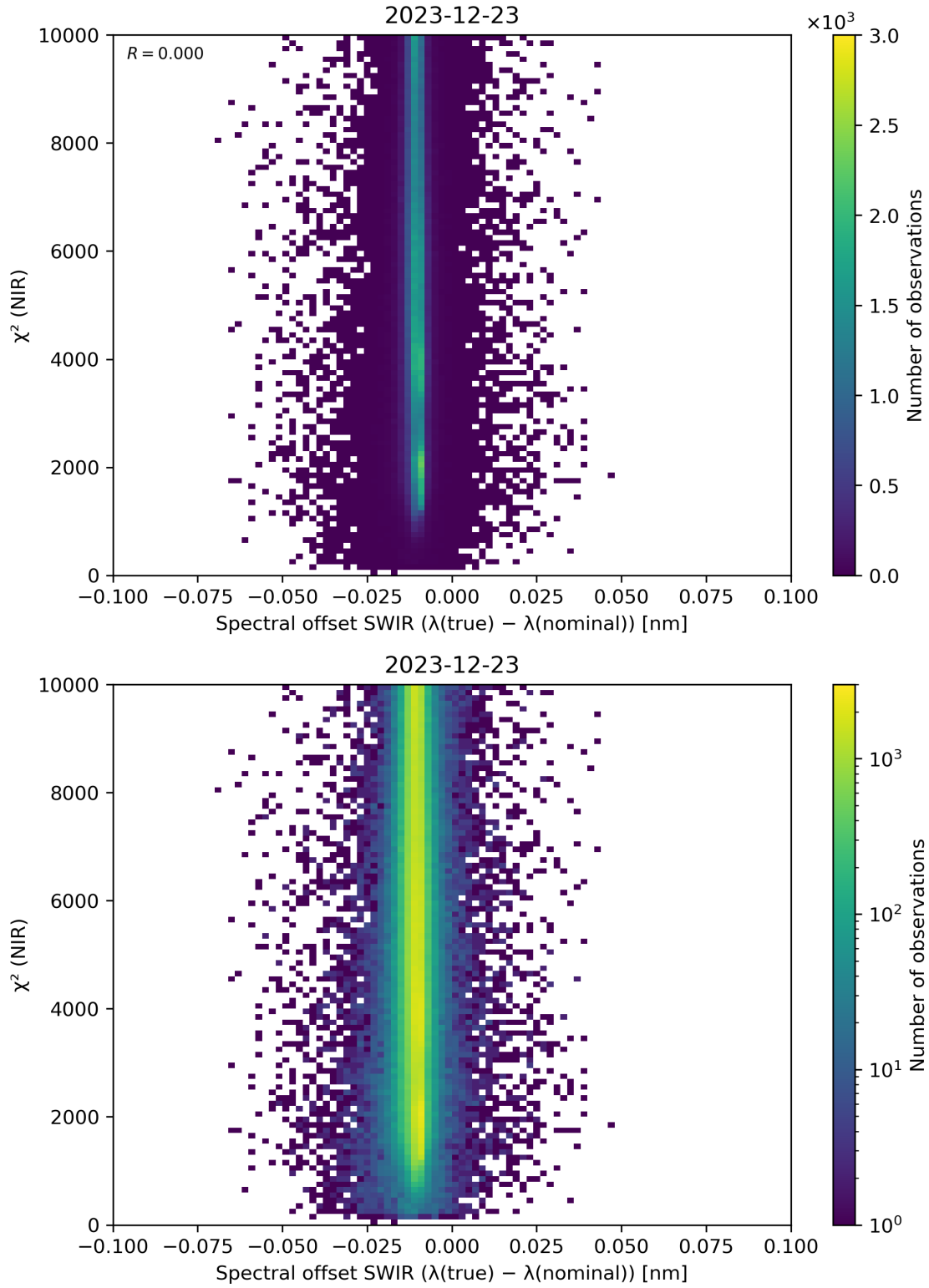
Figure 117: Scatter density plot of “Spectral offset SWIR ( \lambda(\text{true}) - \lambda(\text{nominal}) )” against “ \chi^2 (NIR)” for 2023-12-22 to 2023-12-24.
