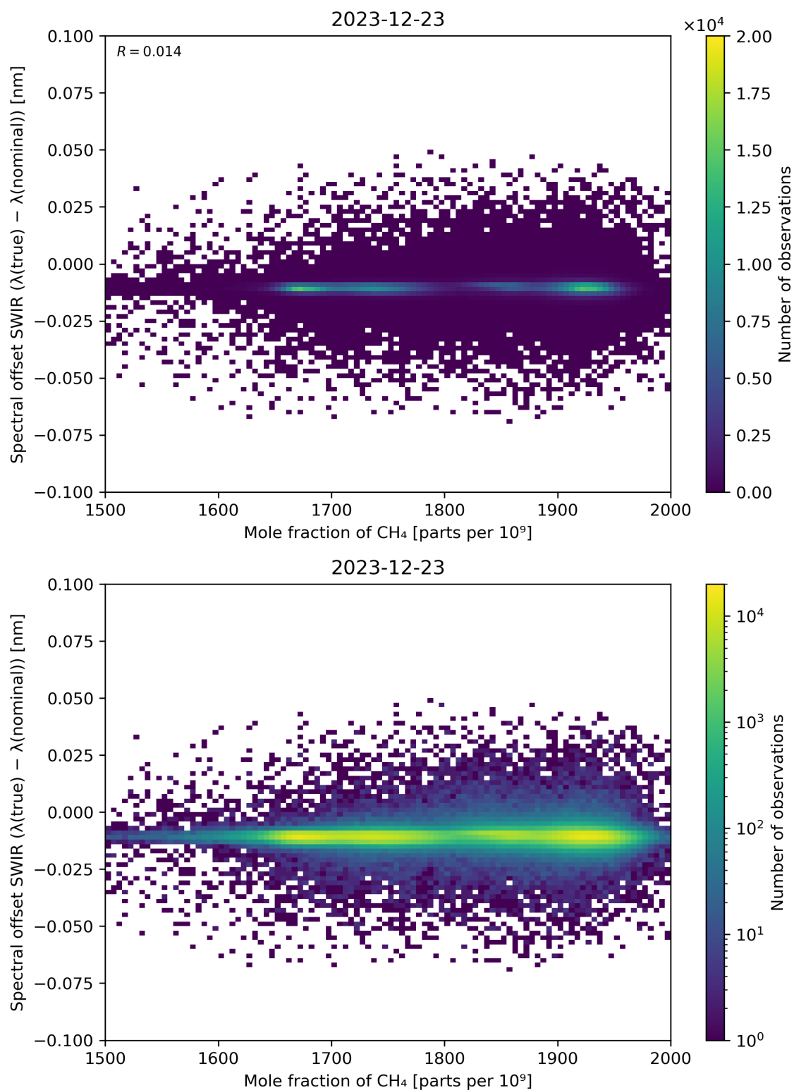
Figure 86: Scatter density plot of “Mole fraction of CH 4 ” against “Spectral offset SWIR ( \lambda(\text{true}) - \lambda(\text{nominal}) )” for 2023-12-22 to 2023-12-24.
