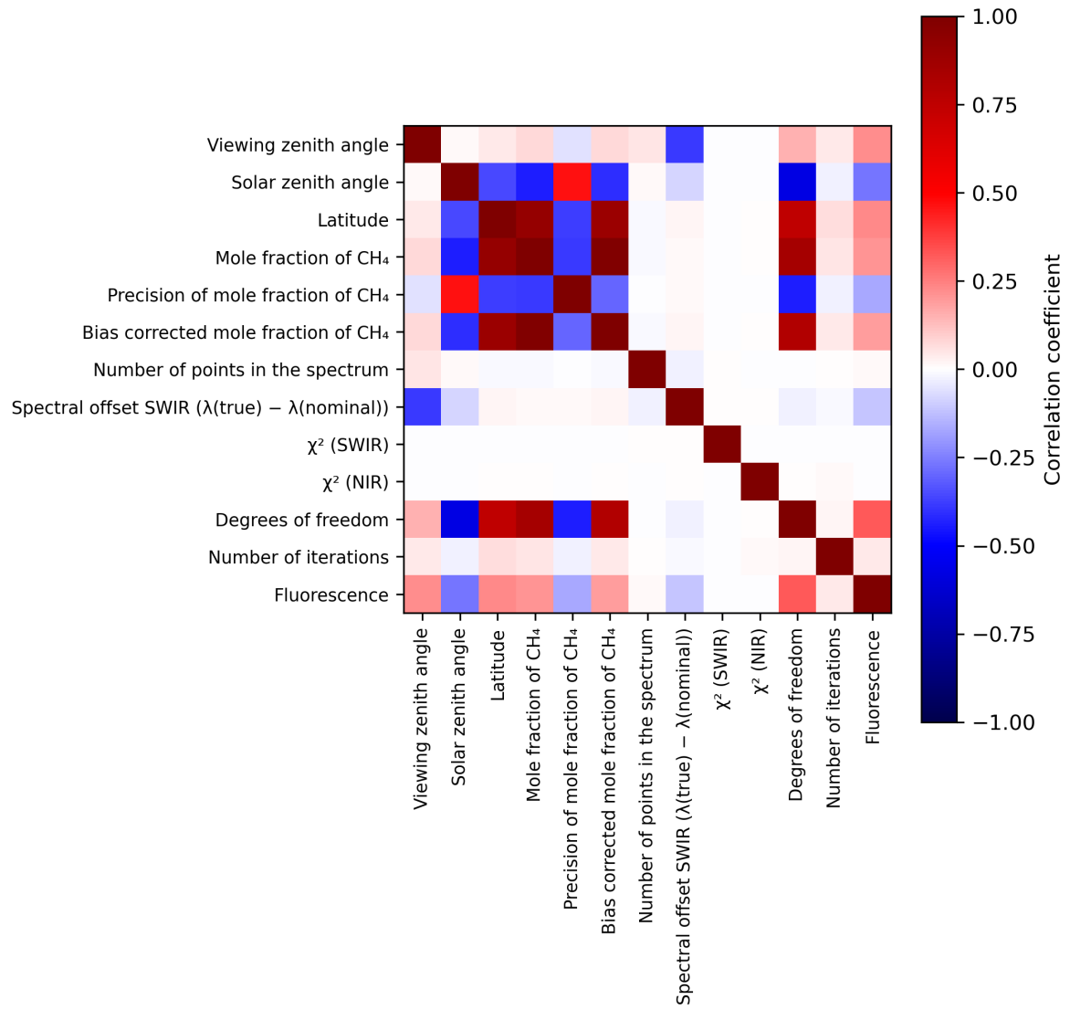
Figure 2: Map of correlation matrix for 2023-12-22 to 2023-12-24.
