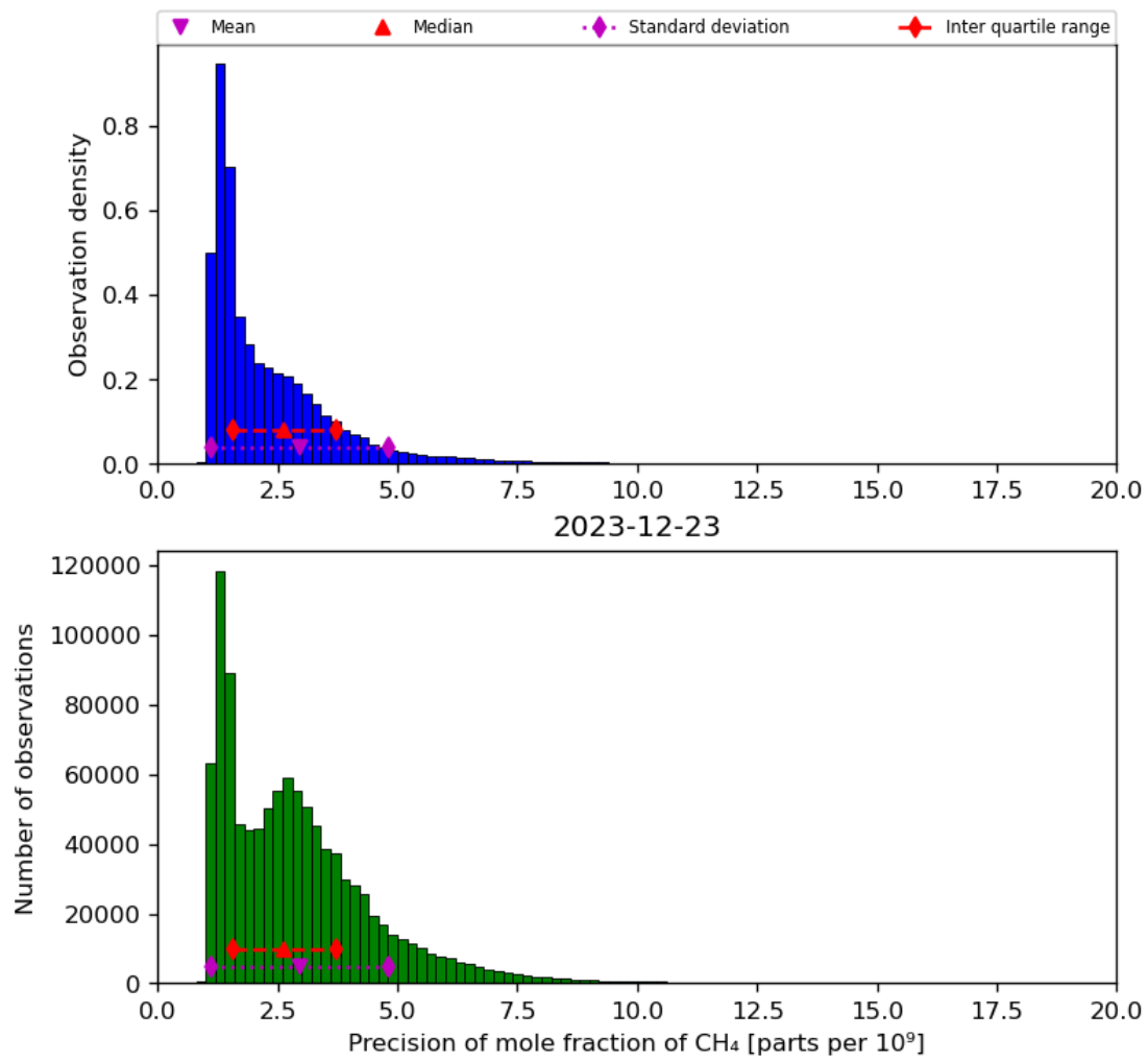
Figure 24: Histogram of “Precision of mole fraction of CH 4 ” for 2023-12-22 to 2023-12-24
