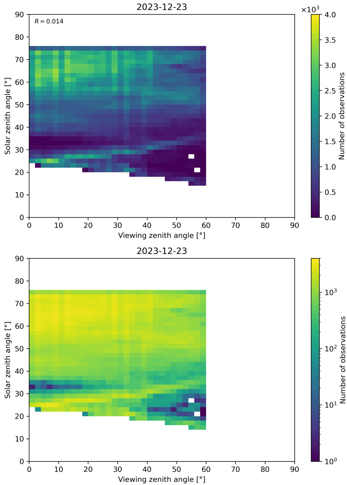
Figure 115: Scatter density plot of “Viewing zenith angle” against “Solar zenith angle” for 2023-12-22 to 2023-12-24.
