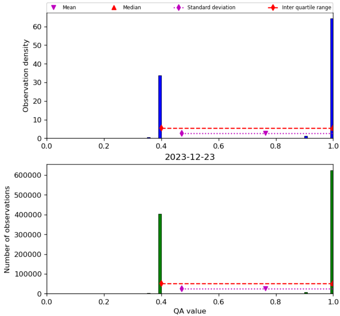
Figure 22: Histogram of “QA value” for 2023-12-22 to 2023-12-24
