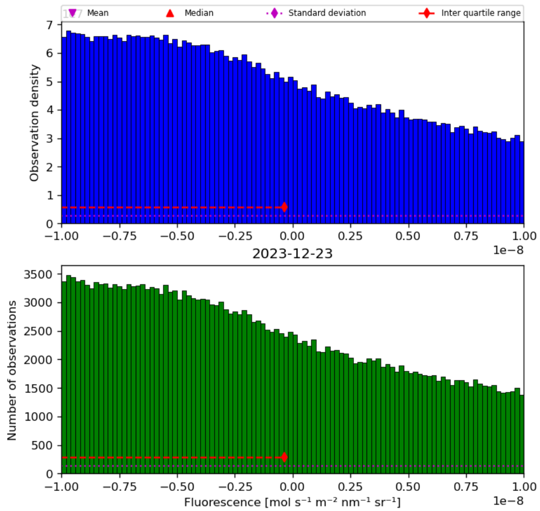
Figure 32: Histogram of “Fluorescence” for 2023-12-22 to 2023-12-24
