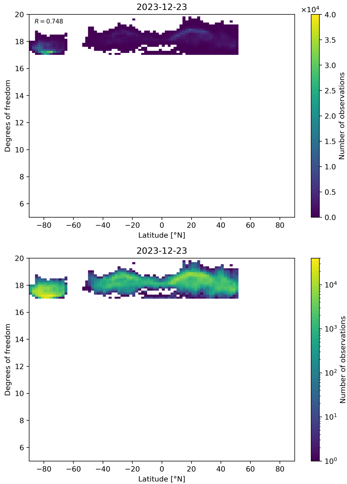
Figure 55: Scatter density plot of “Latitude” against “Degrees of freedom” for 2023-12-22 to 2023-12-24.
