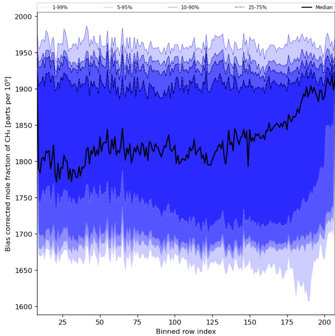
Figure 36: Along track statistics of “Bias corrected mole fraction of CH 4 ” for 2023-12-22 to 2023-12-24
