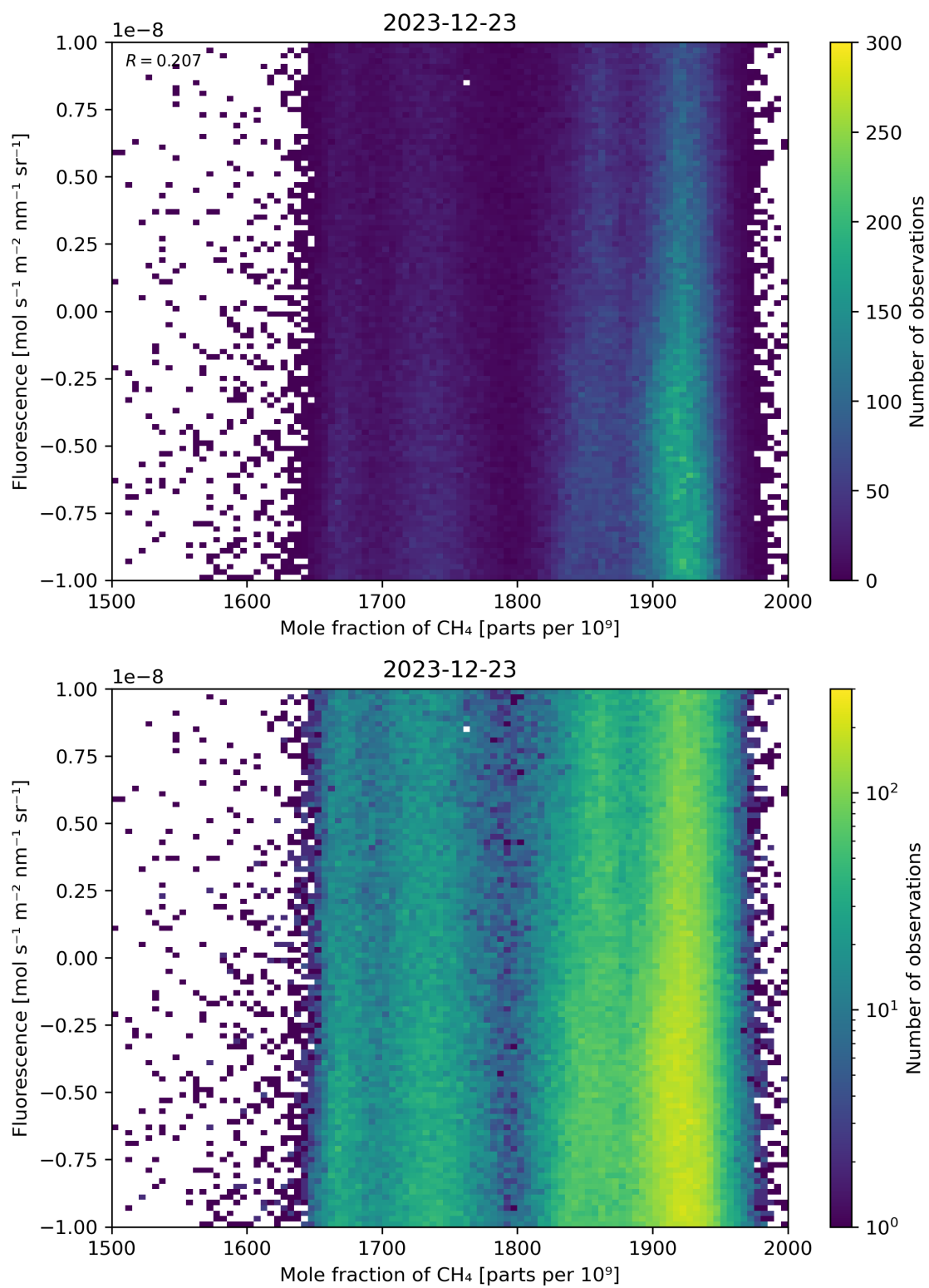
Figure 73: Scatter density plot of “Mole fraction of \text{CH}_4 ” against “Fluorescence” for 2023-12-22 to 2023-12-24.
