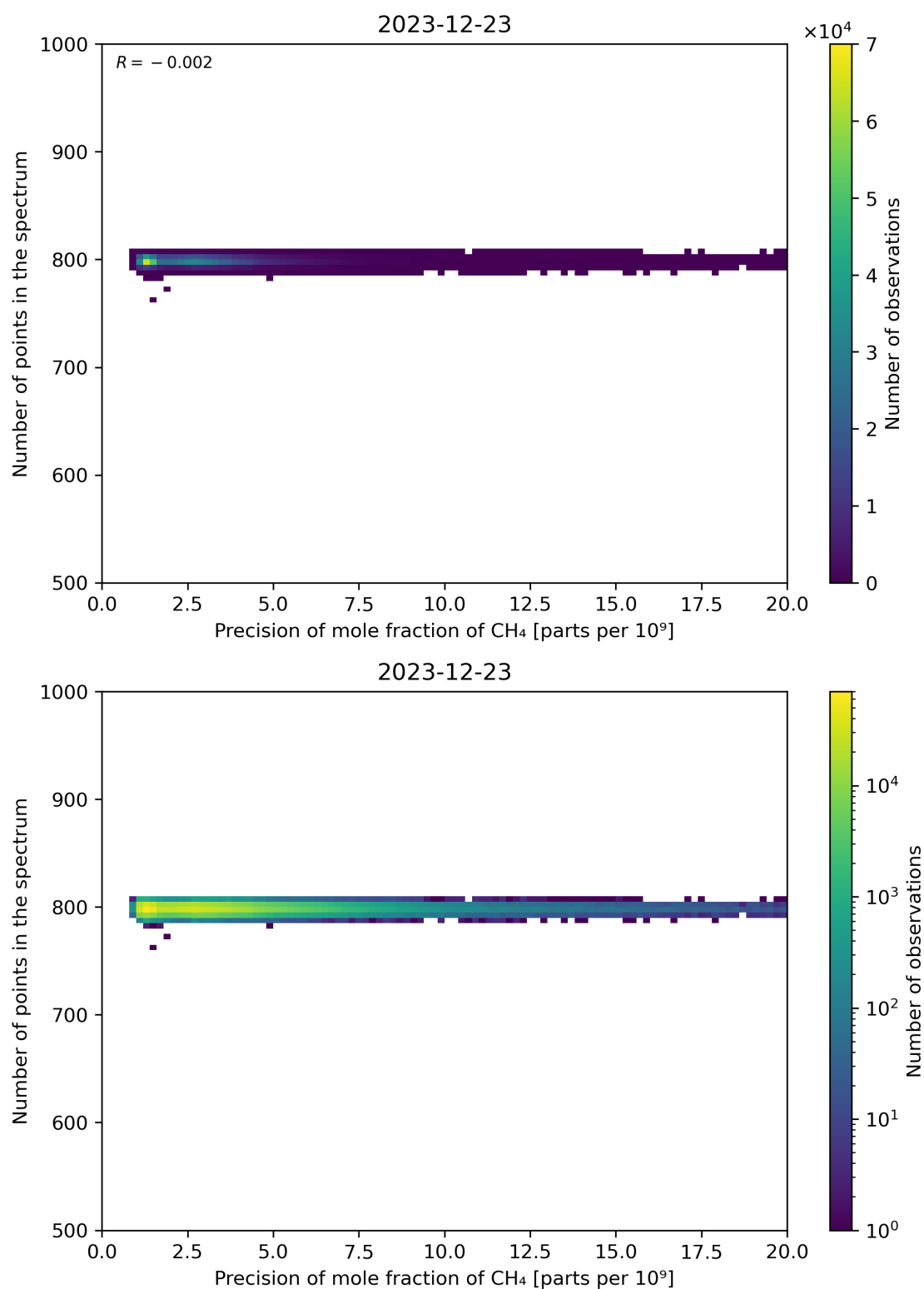
Figure 84: Scatter density plot of “Precision of mole fraction of CH 4 ” against “Number of points in the spectrum” for 2023-12-22 to 2023-12-24.
