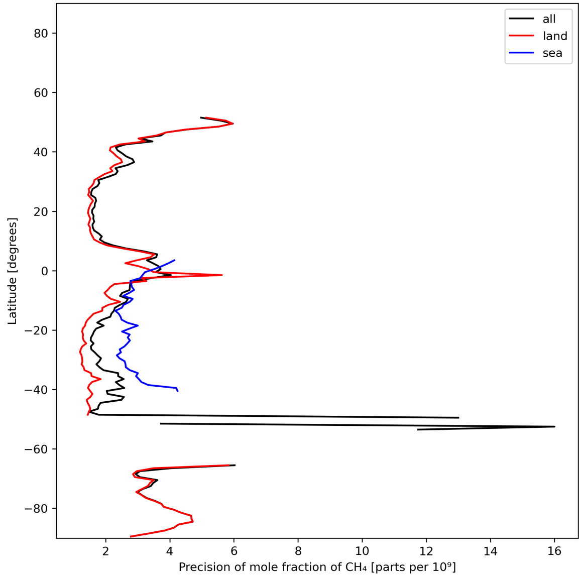
Figure 13: Zonal average of “Precision of mole fraction of CH 4 ” for 2023-12-22 to 2023-12-24.
