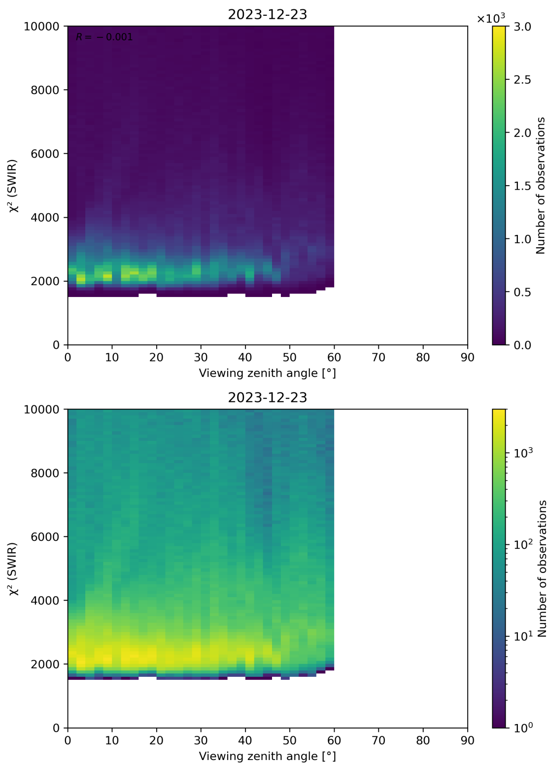
Figure 106: Scatter density plot of “Viewing zenith angle” against “ \chi^2 (SWIR)” for 2023-12-22 to 2023-12-24.
