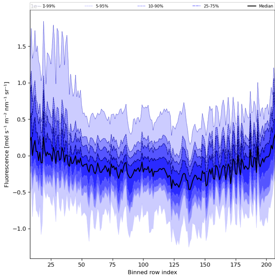
Figure 43: Along track statistics of “Fluorescence” for 2023-12-22 to 2023-12-24
