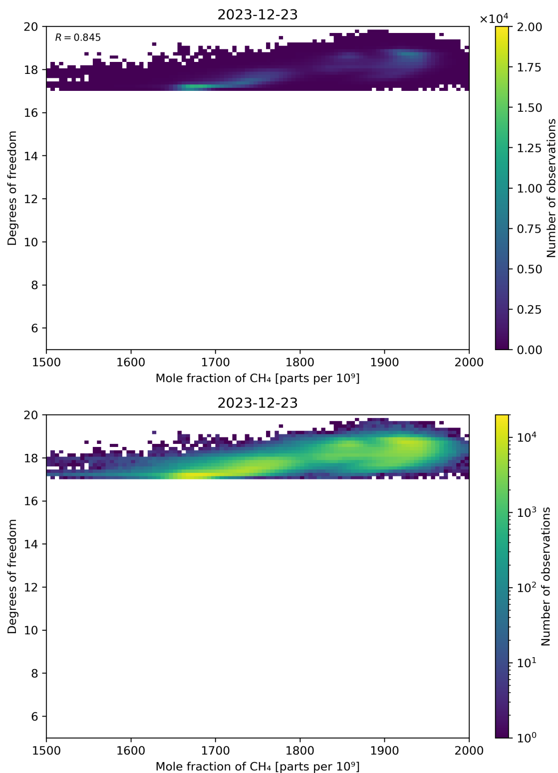
Figure 72: Scatter density plot of “Mole fraction of CH 4 ” against “Degrees of freedom” for 2023-12-22 to 2023-12-24.
