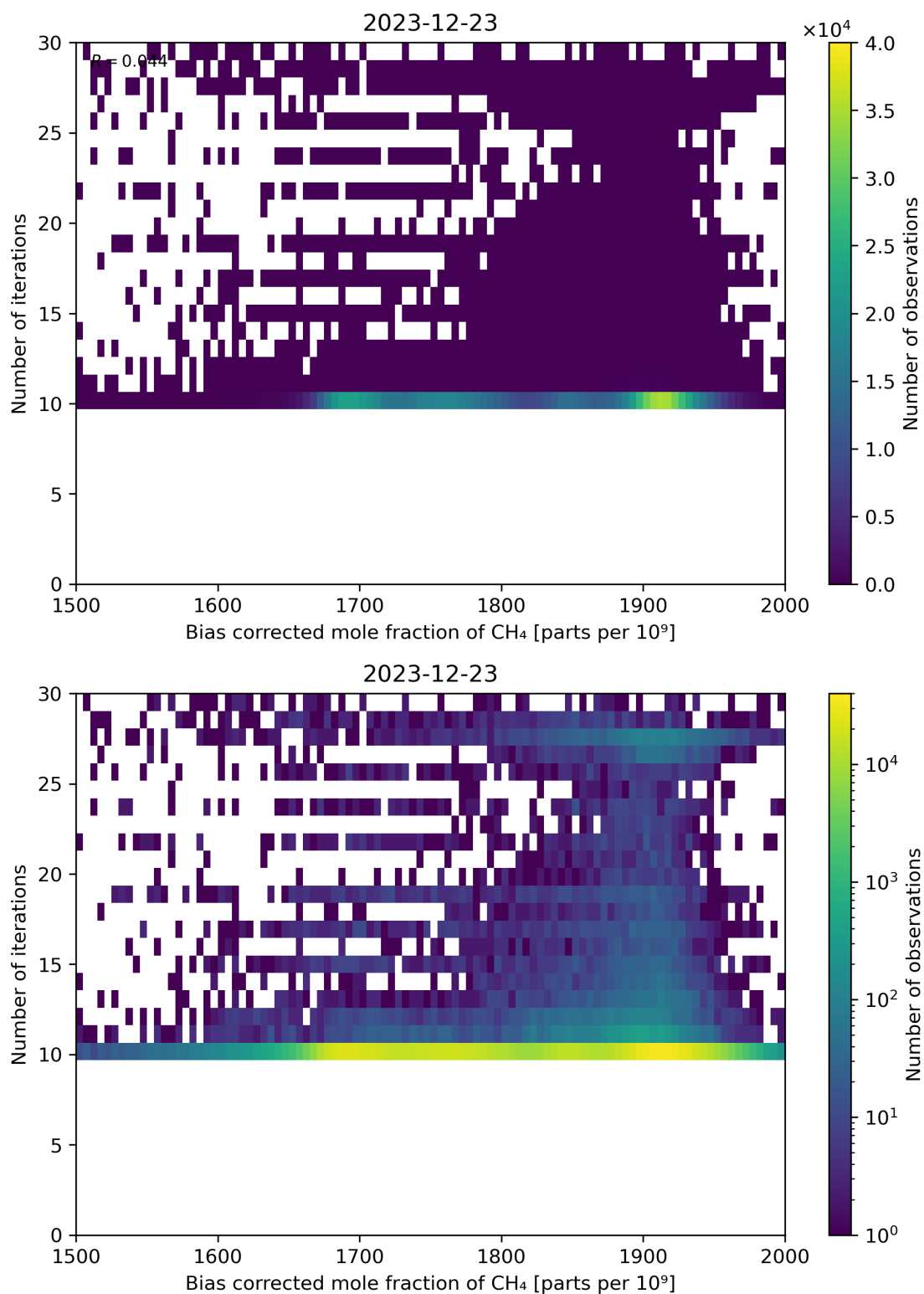
Figure 67: Scatter density plot of “Bias corrected mole fraction of \text{CH}_4 ” against “Number of iterations” for 2023-12-22 to 2023-12-24.
