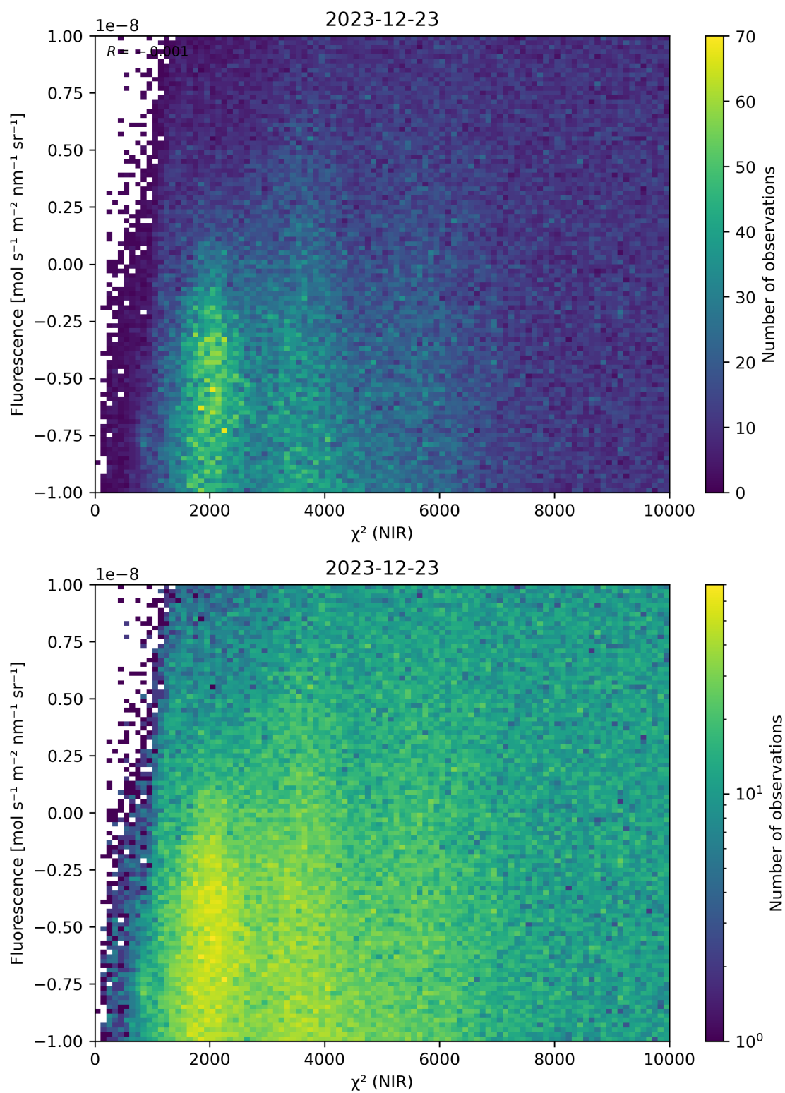
Figure 45: Scatter density plot of “ \chi^2 (NIR)” against “Fluorescence” for 2023-12-22 to 2023-12-24.
