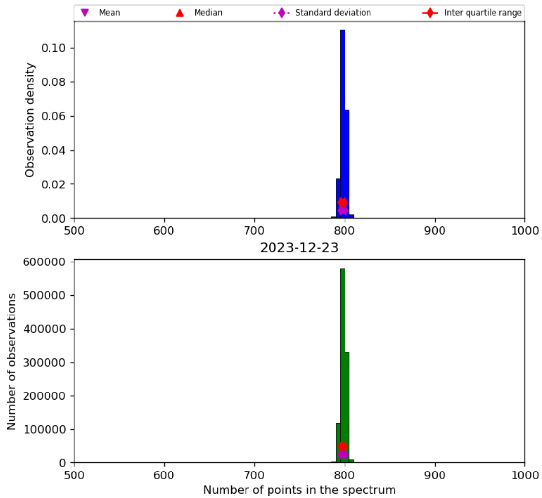
Figure 26: Histogram of “Number of points in the spectrum” for 2023-12-22 to 2023-12-24
