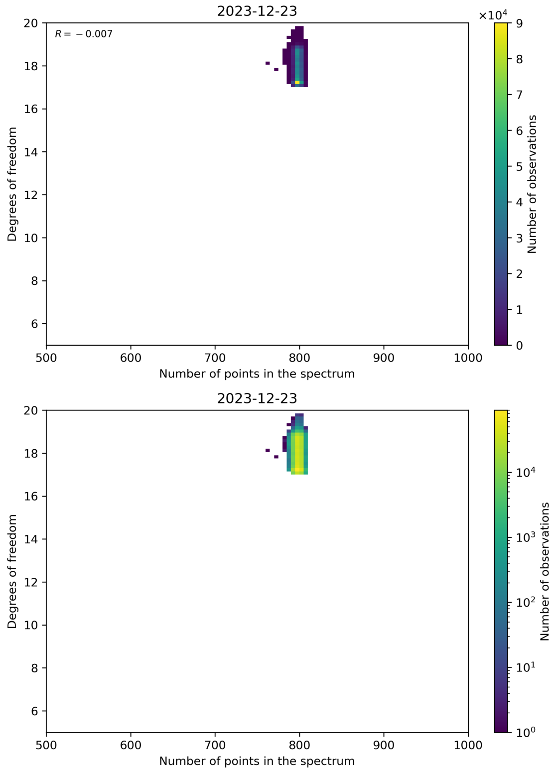
Figure 90: Scatter density plot of “Number of points in the spectrum” against “Degrees of freedom” for 2023-12-22 to 2023-12-24.
