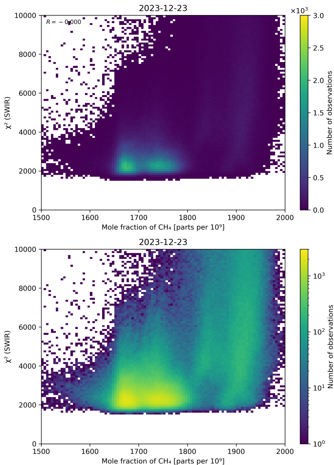
Figure 71: Scatter density plot of “Mole fraction of \text{CH}_4 ” against “ \chi^2 (SWIR)” for 2023-12-22 to 2023-12-24.
