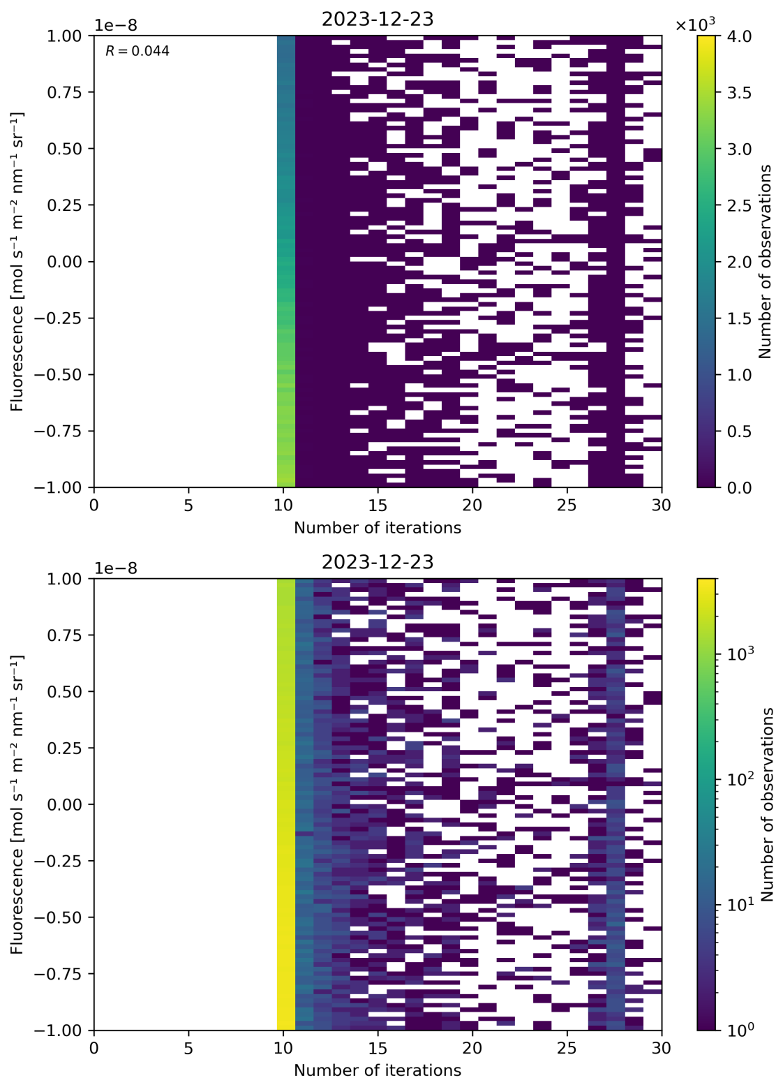
Figure 87: Scatter density plot of “Number of iterations” against “Fluorescence” for 2023-12-22 to 2023-12-24.
