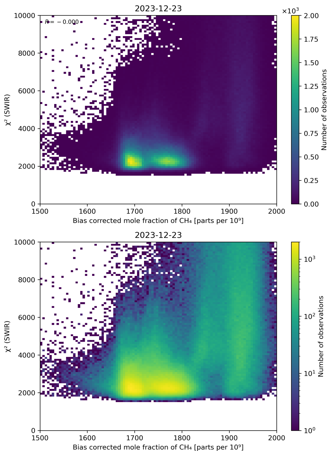
Figure 64: Scatter density plot of “Bias corrected mole fraction of CH 4 ” against “ \chi^2 (SWIR)” for 2023-12-22 to 2023-12-24.
