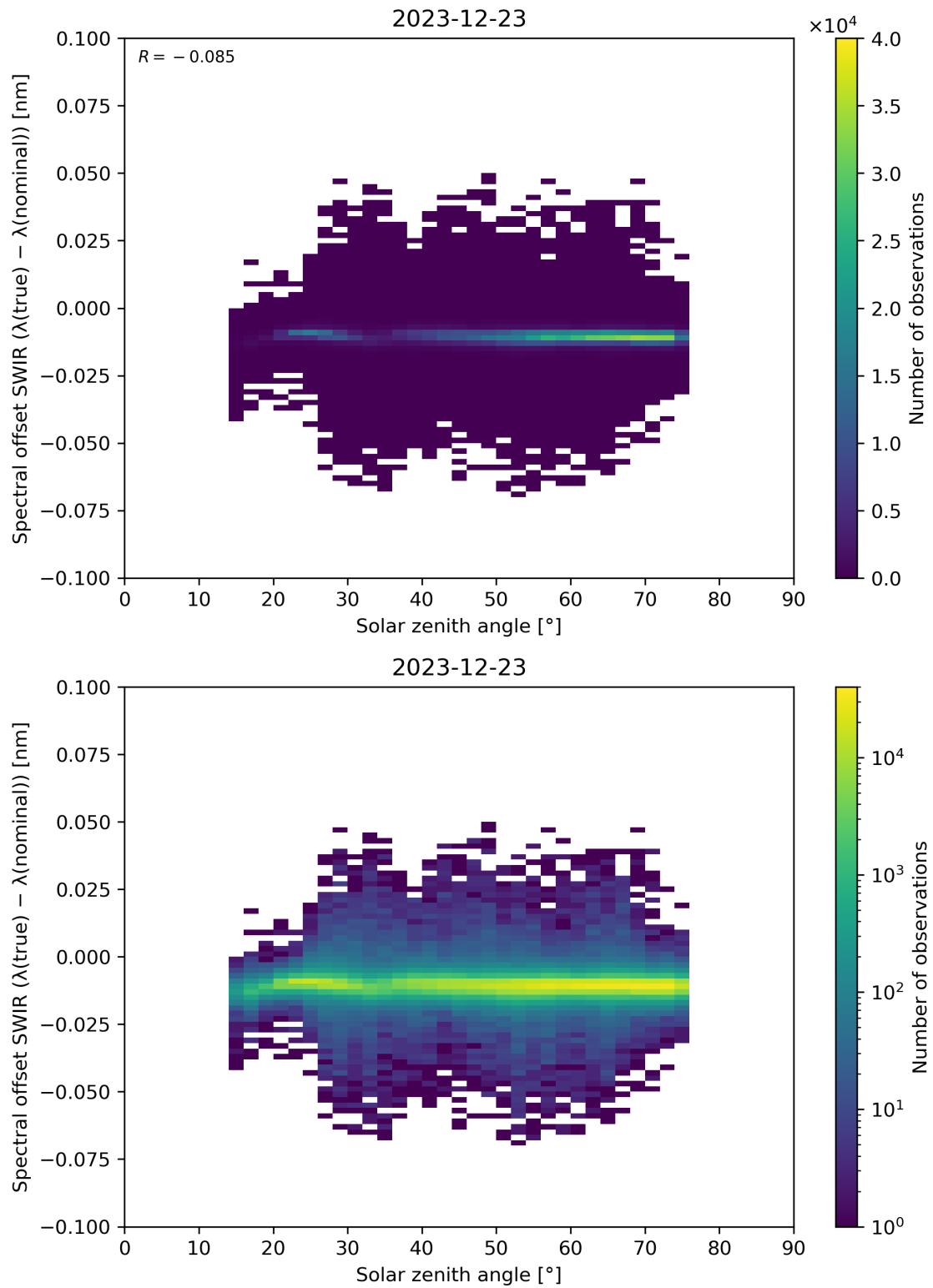
Figure 104: Scatter density plot of “Solar zenith angle” against “Spectral offset SWIR ( \lambda(\text{true}) - \lambda(\text{nominal}) )” for 2023-12-22 to 2023-12-24.
