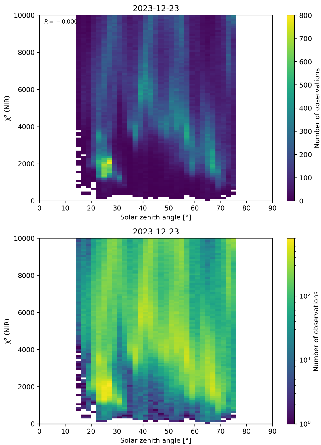
Figure 94: Scatter density plot of “Solar zenith angle” against “ \chi^2 (NIR)” for 2023-12-22 to 2023-12-24.
