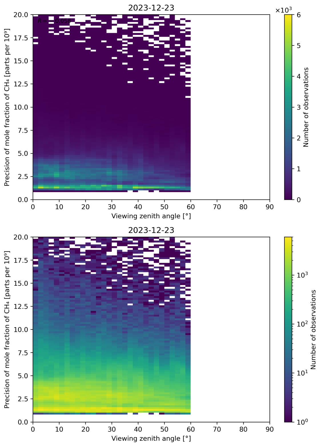
Figure 112: Scatter density plot of “Viewing zenith angle” against “Precision of mole fraction of CH 4 ” for 2023-12-22 to 2023-12-24.
