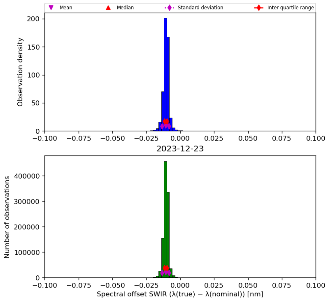
Figure 27: Histogram of “Spectral offset SWIR ( \lambda(\text{true}) - \lambda(\text{nominal}) )” for 2023-12-22 to 2023-12-24
