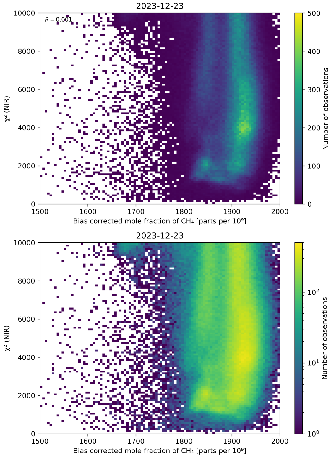
Figure 63: Scatter density plot of “Bias corrected mole fraction of CH 4 ” against “ \chi^2 (NIR)” for 2023-12-22 to 2023-12-24.
