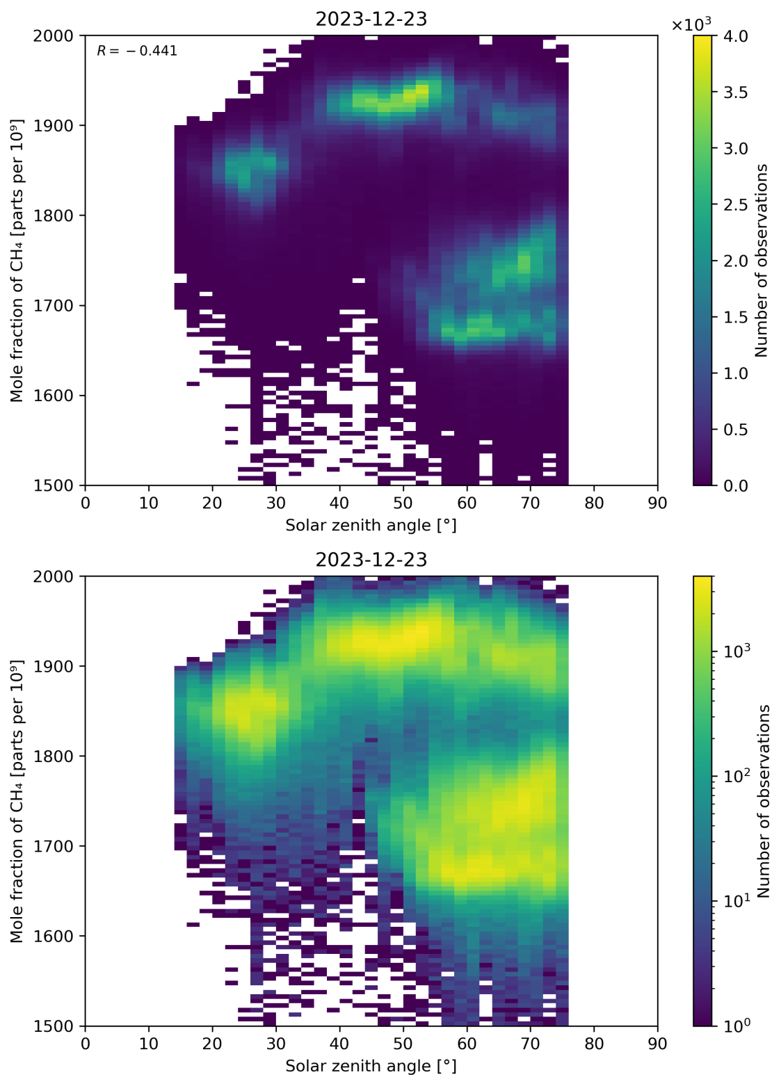
Figure 99: Scatter density plot of “Solar zenith angle” against “Mole fraction of CH 4 ” for 2023-12-22 to 2023-12-24.
