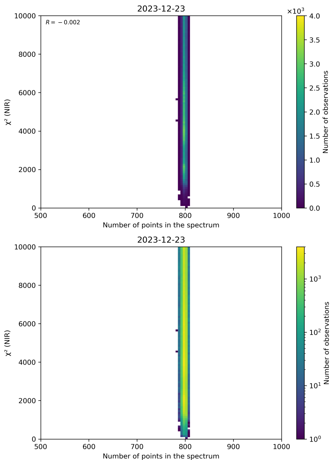
Figure 88: Scatter density plot of “Number of points in the spectrum” against “ \chi^2 (NIR)” for 2023-12-22 to 2023-12-24.
