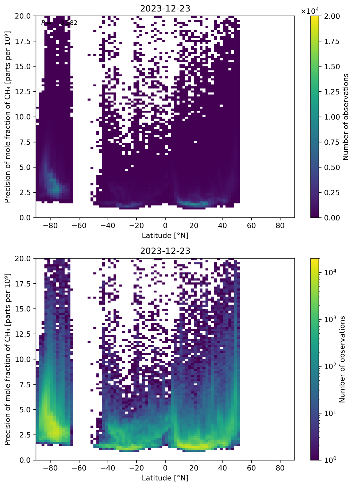
Figure 59: Scatter density plot of “Latitude” against “Precision of mole fraction of CH 4 ” for 2023-12-22 to 2023-12-24.
