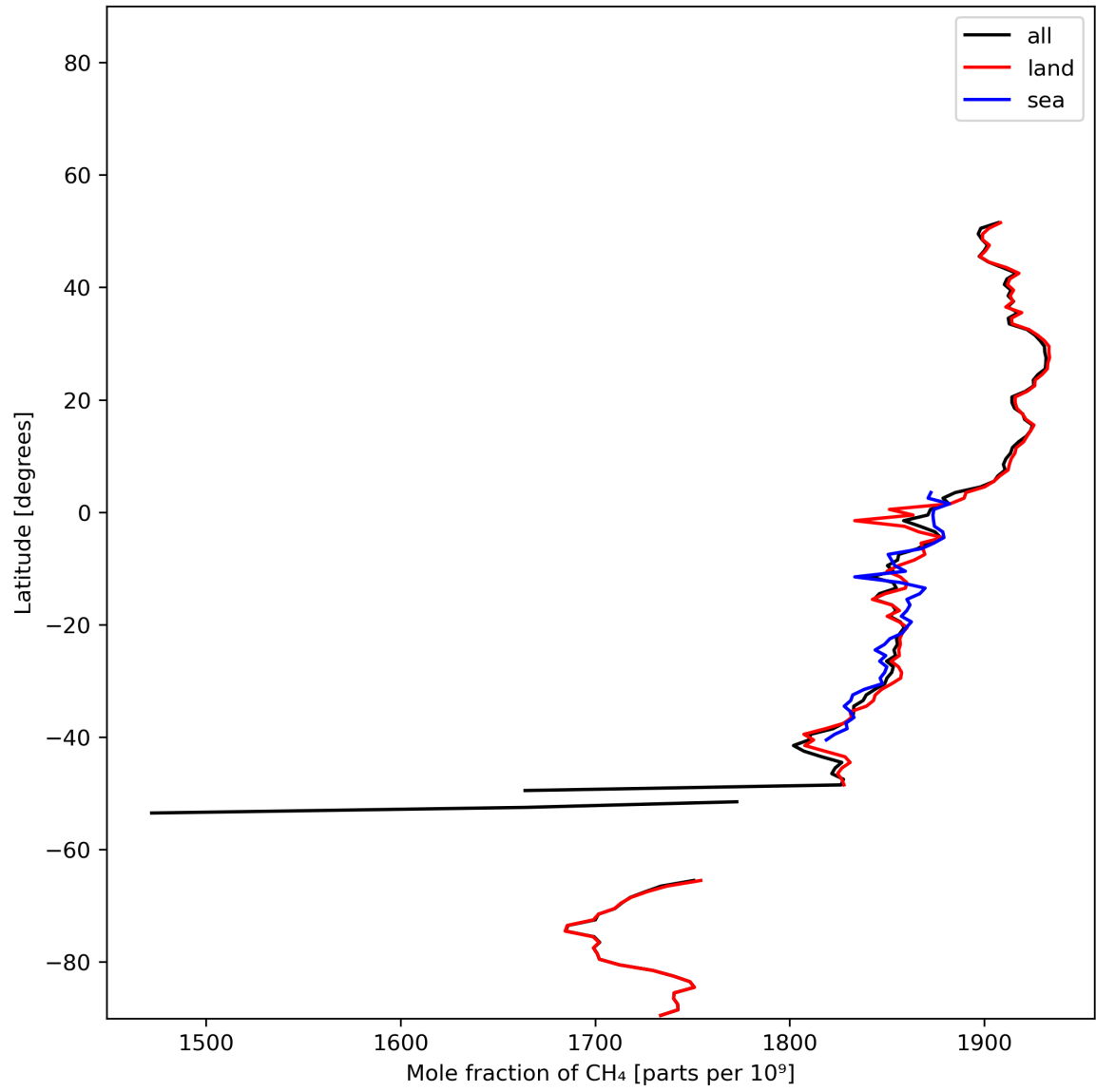
Figure 12: Zonal average of “Mole fraction of CH 4 ” for 2023-12-22 to 2023-12-24.
