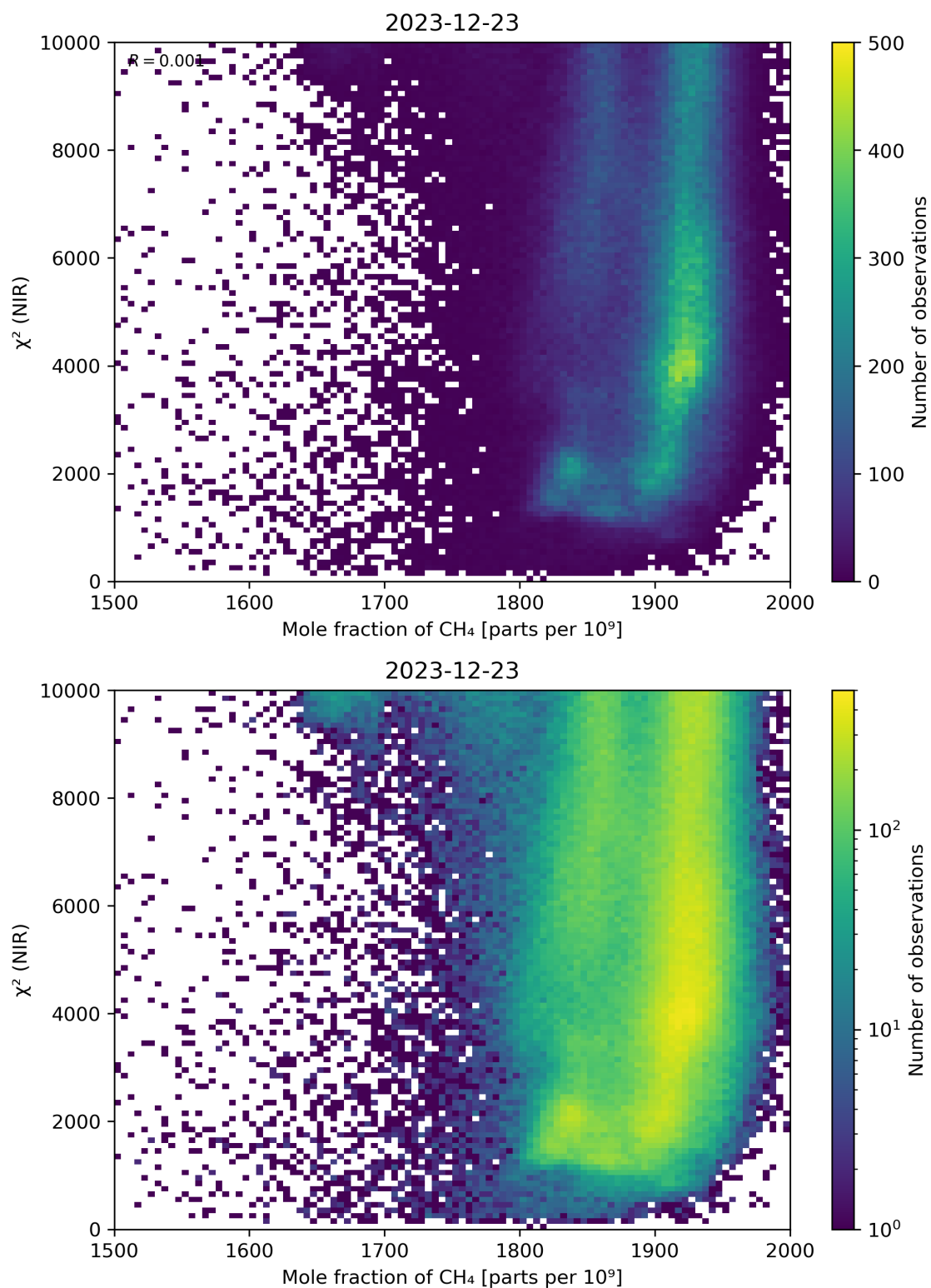
Figure 70: Scatter density plot of “Mole fraction of \text{CH}_4 ” against “ \chi^2 (NIR)” for 2023-12-22 to 2023-12-24.
