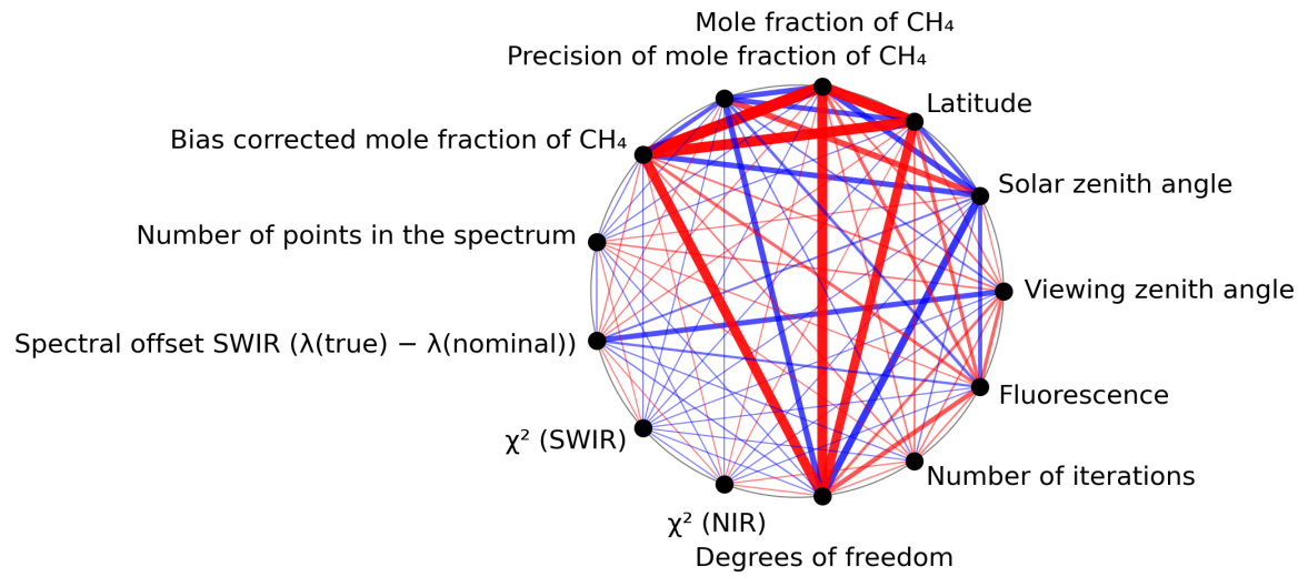
Figure 1: Map of correlation graph for 2023-12-22 to 2023-12-24.
