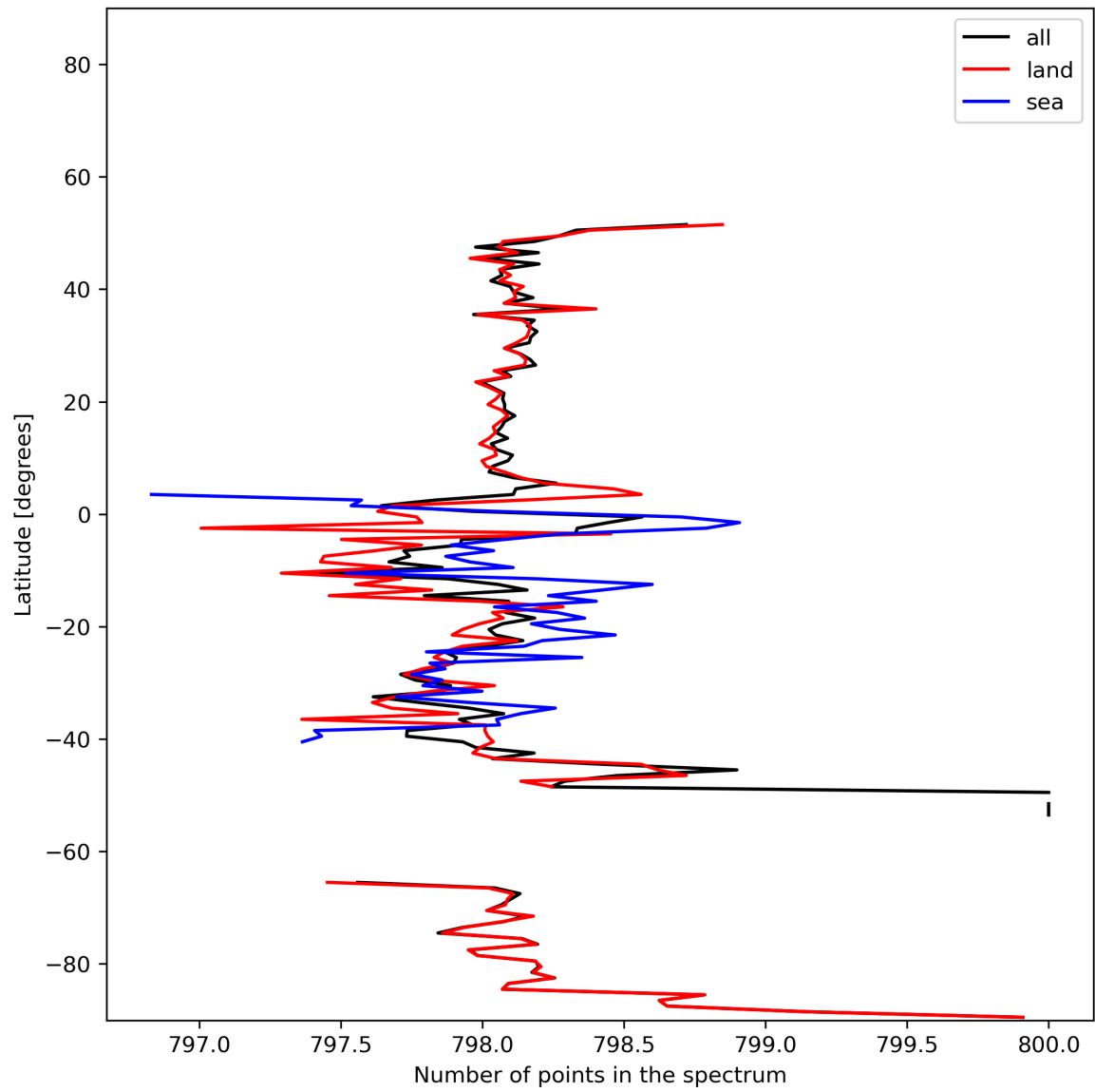
Figure 15: Zonal average of “Number of points in the spectrum” for 2023-12-22 to 2023-12-24.
