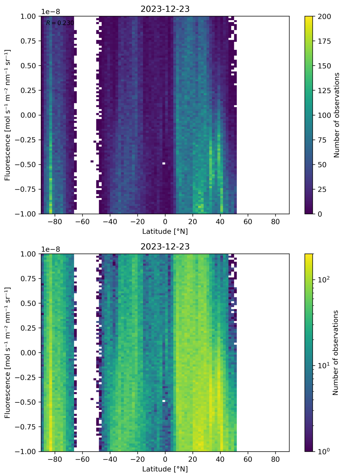
Figure 56: Scatter density plot of “Latitude” against “Fluorescence” for 2023-12-22 to 2023-12-24.
