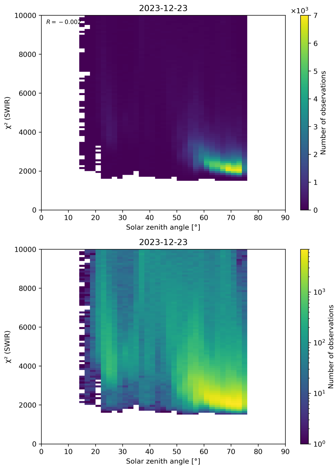
Figure 95: Scatter density plot of “Solar zenith angle” against “ \chi^2 (SWIR)” for 2023-12-22 to 2023-12-24.
