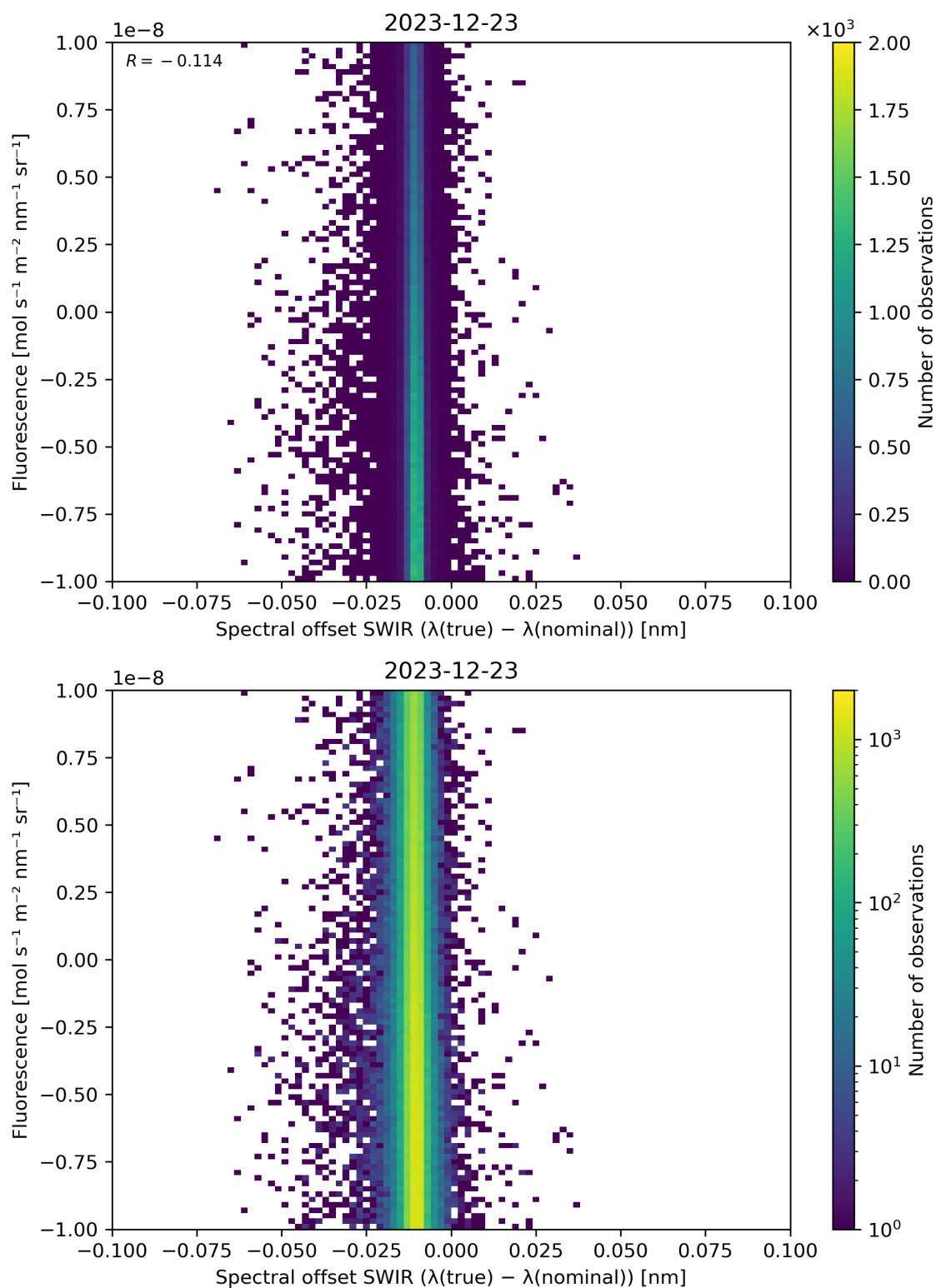
Figure 120: Scatter density plot of “Spectral offset SWIR ( \lambda(\text{true}) - \lambda(\text{nominal}) )” against “Fluorescence” for 2023-12-22 to 2023-12-24.
