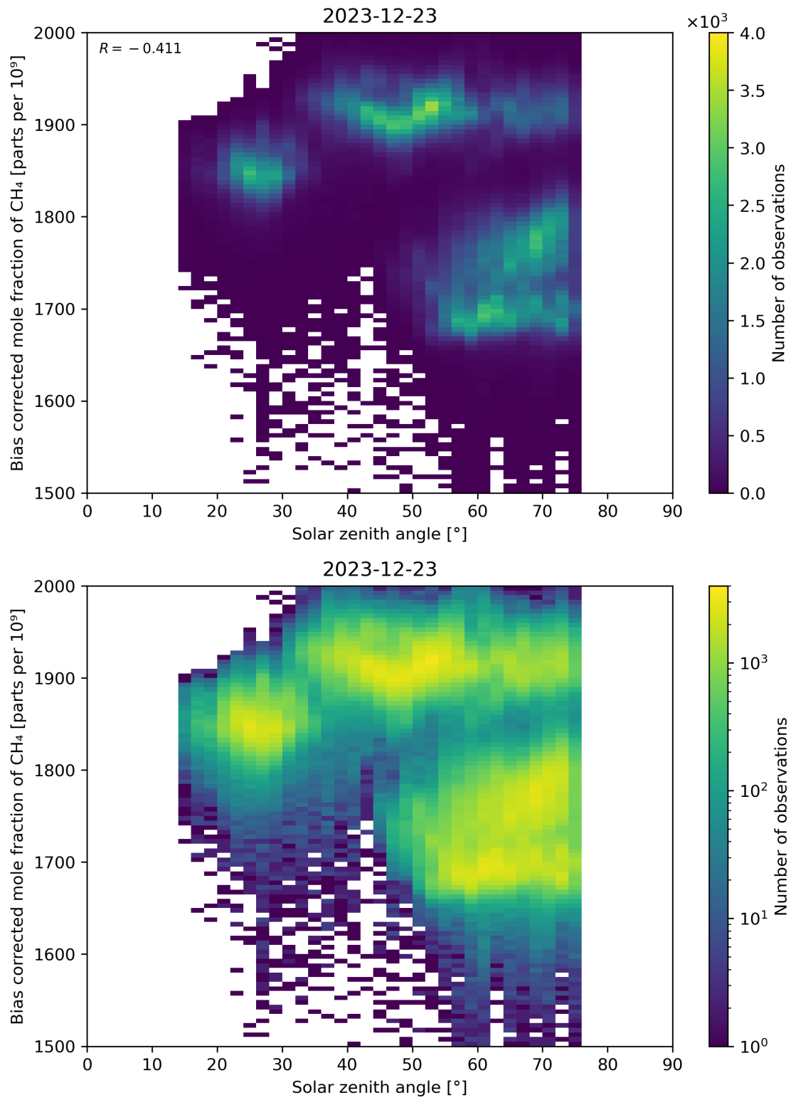
Figure 100: Scatter density plot of “Solar zenith angle” against “Bias corrected mole fraction of \text{CH}_4 ” for 2023-12-22 to 2023-12-24.
