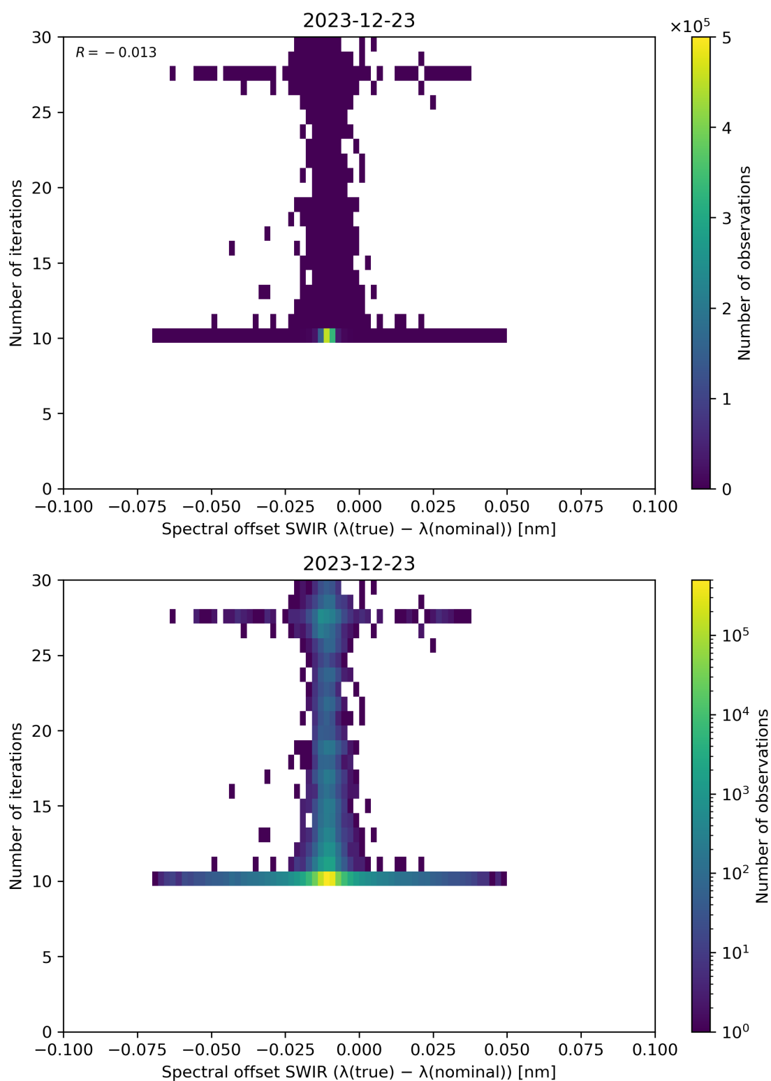
Figure 121: Scatter density plot of “Spectral offset SWIR ( \lambda(\text{true}) - \lambda(\text{nominal}) )” against “Number of iterations” for 2023-12-22 to 2023-12-24.
