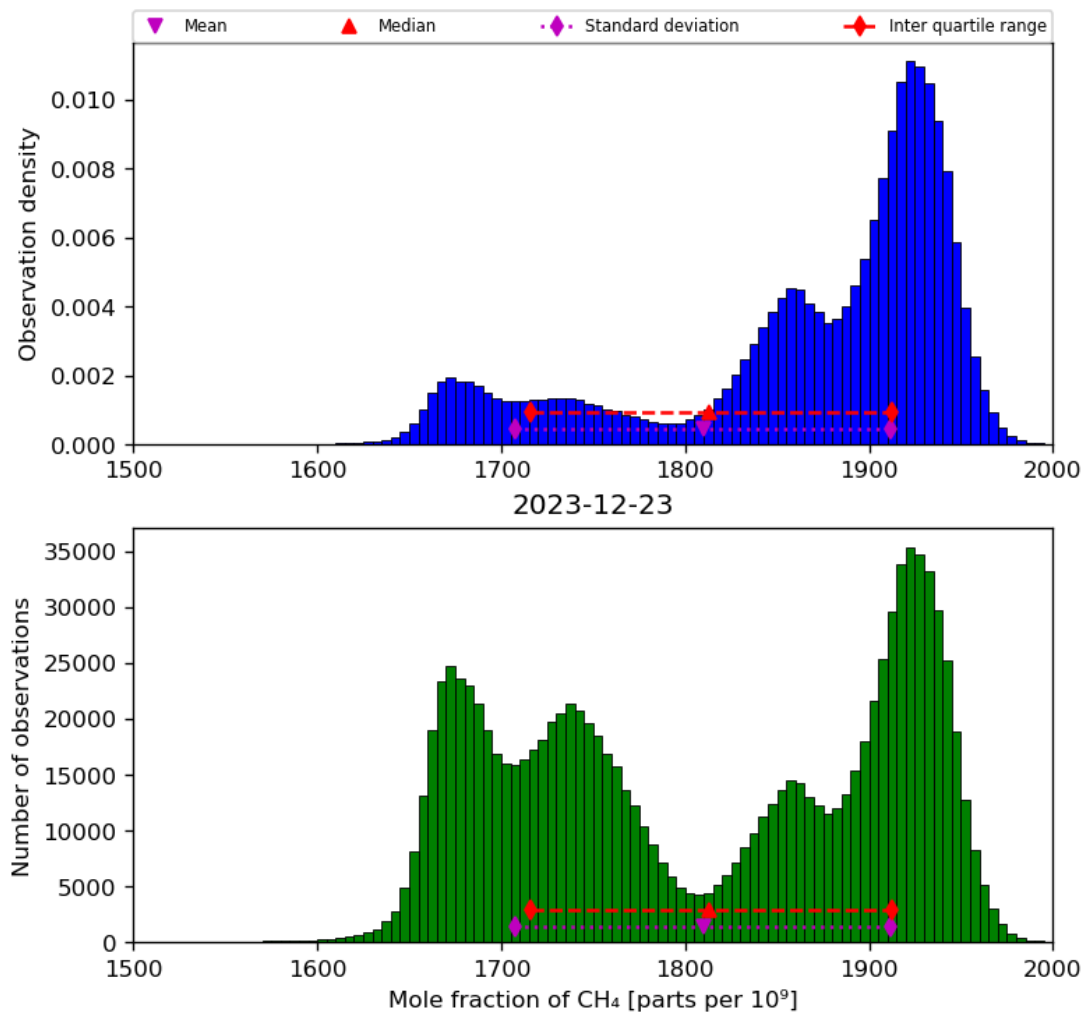
Figure 23: Histogram of “Mole fraction of CH 4 ” for 2023-12-22 to 2023-12-24
