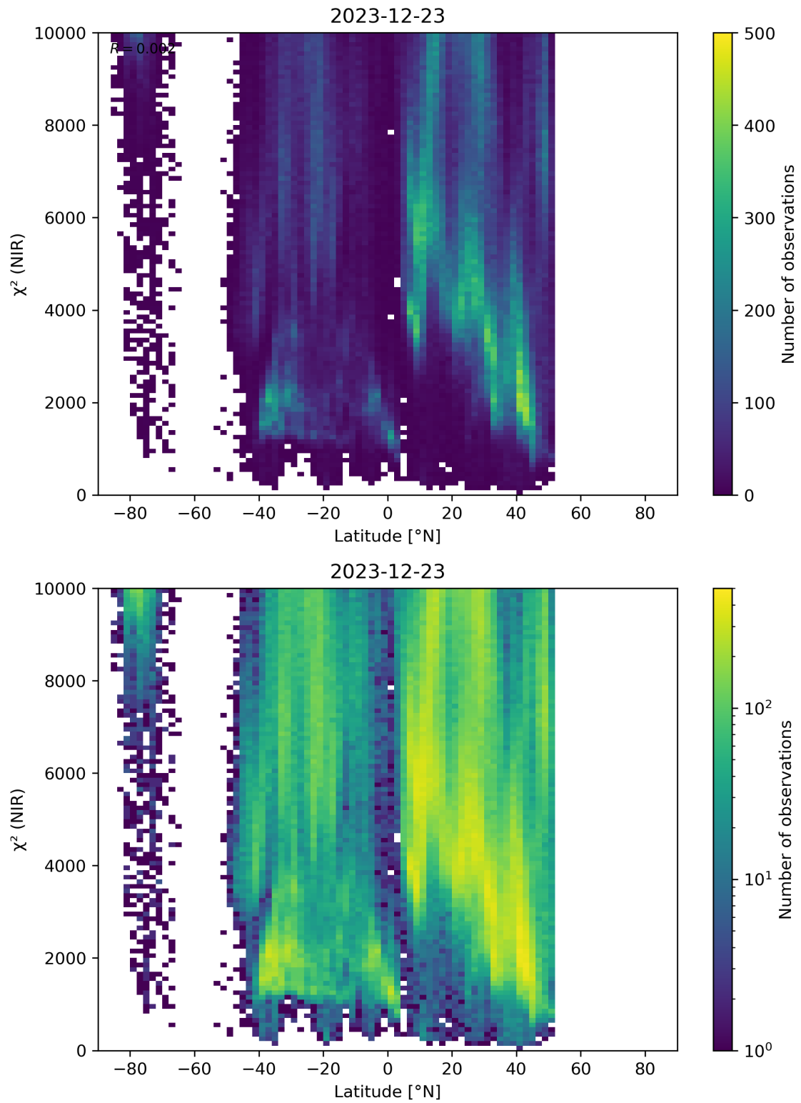
Figure 53: Scatter density plot of “Latitude” against “ \chi^2 (NIR)” for 2023-12-22 to 2023-12-24.
