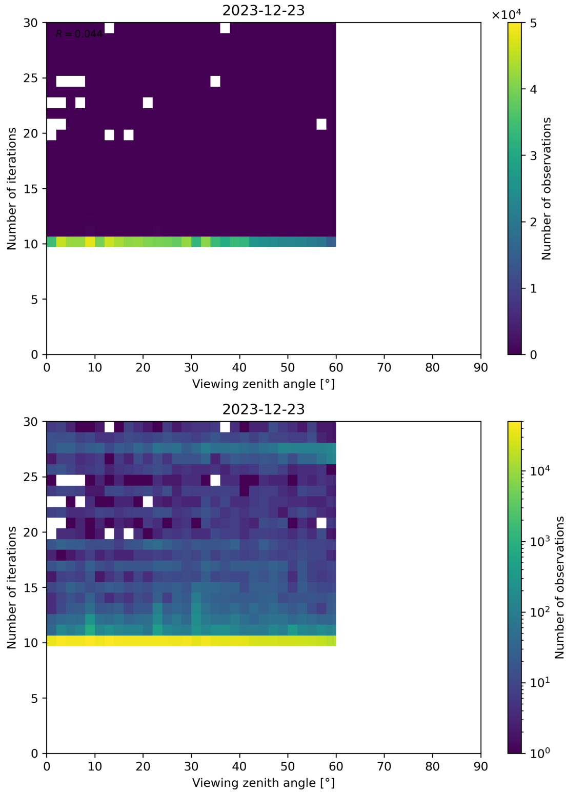
Figure 113: Scatter density plot of “Viewing zenith angle” against “Number of iterations” for 2023-12-22 to 2023-12-24.
