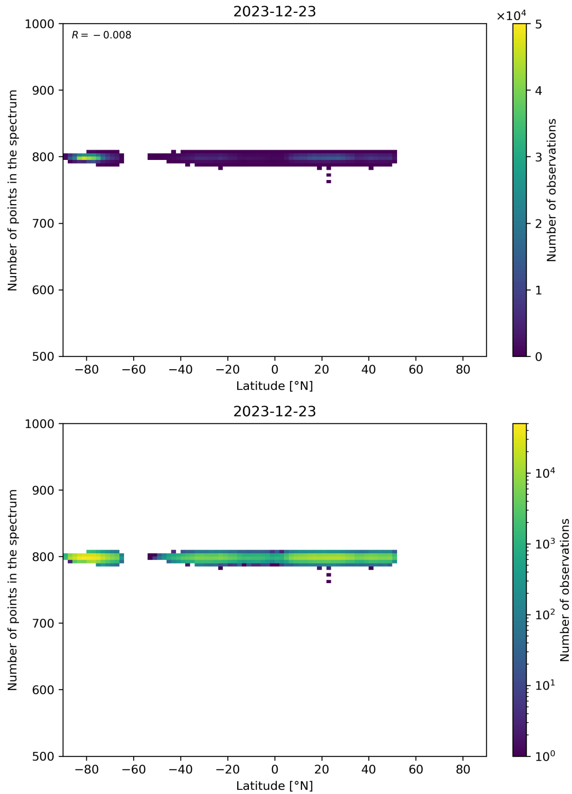
Figure 61: Scatter density plot of “Latitude” against “Number of points in the spectrum” for 2023-12-22 to 2023-12-24.
