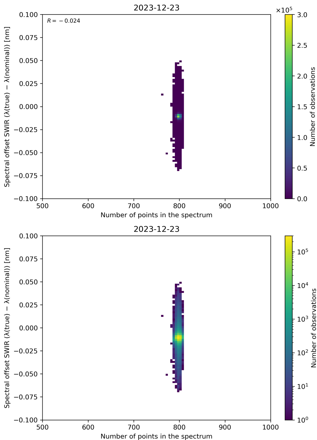
Figure 93: Scatter density plot of “Number of points in the spectrum” against “Spectral offset SWIR ( \lambda(\text{true}) - \lambda(\text{nominal}) )” for 2023-12-22 to 2023-12-24.
