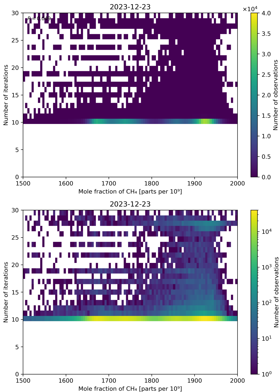
Figure 76: Scatter density plot of “Mole fraction of CH 4 ” against “Number of iterations” for 2023-12-22 to 2023-12-24.
