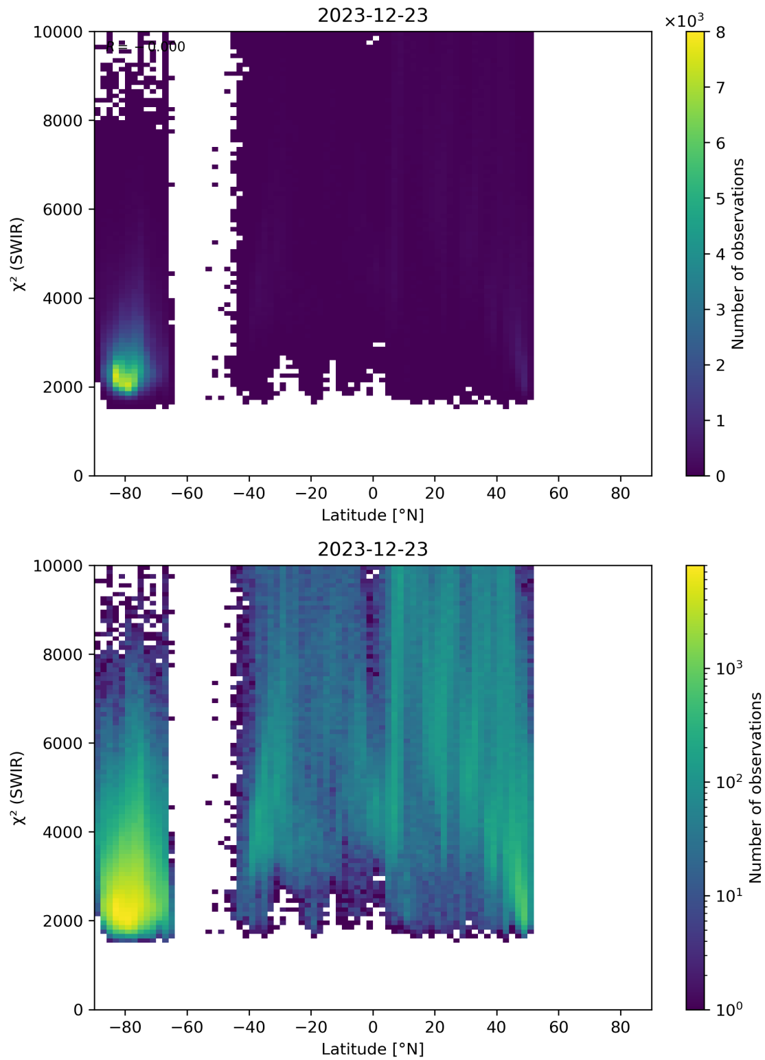
Figure 54: Scatter density plot of “Latitude” against “ \chi^2 (SWIR)” for 2023-12-22 to 2023-12-24.
