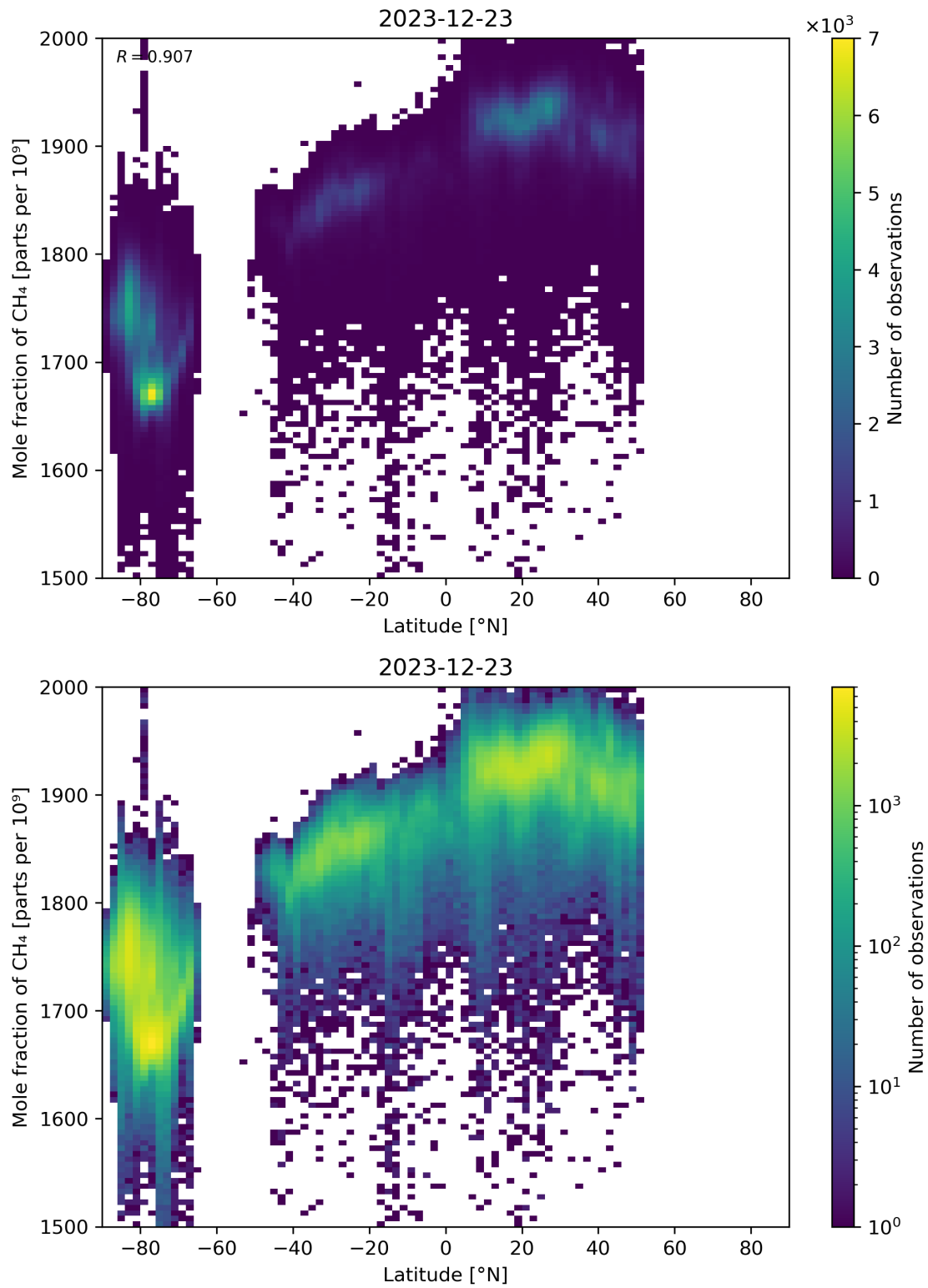
Figure 57: Scatter density plot of “Latitude” against “Mole fraction of CH 4 ” for 2023-12-22 to 2023-12-24.
