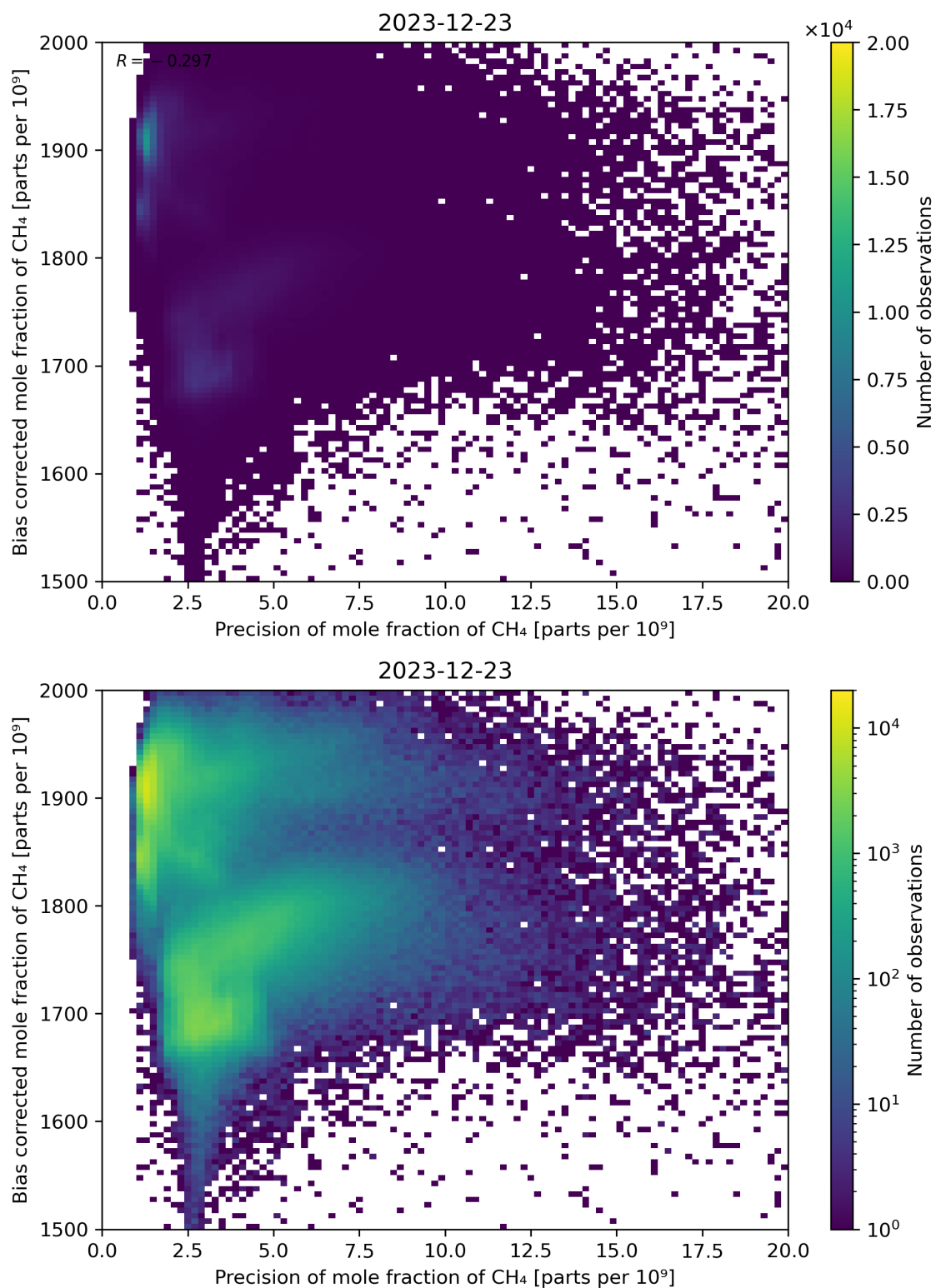
Figure 82: Scatter density plot of “Precision of mole fraction of CH 4 ” against “Bias corrected mole fraction of CH 4 ” for 2023-12-22 to 2023-12-24.
