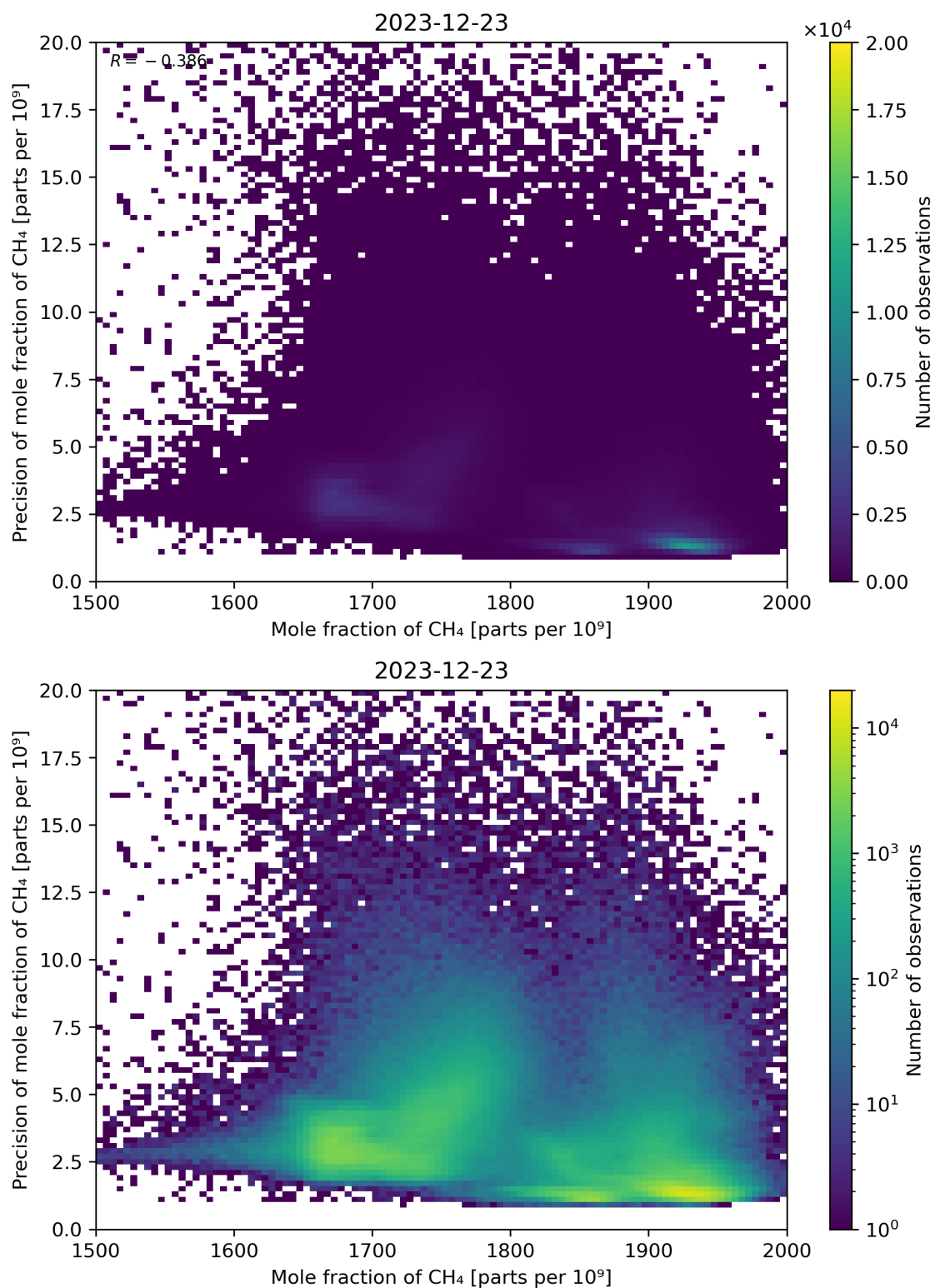
Figure 75: Scatter density plot of “Mole fraction of CH 4 ” against “Precision of mole fraction of CH 4 ” for 2023-12-22 to 2023-12-24.
