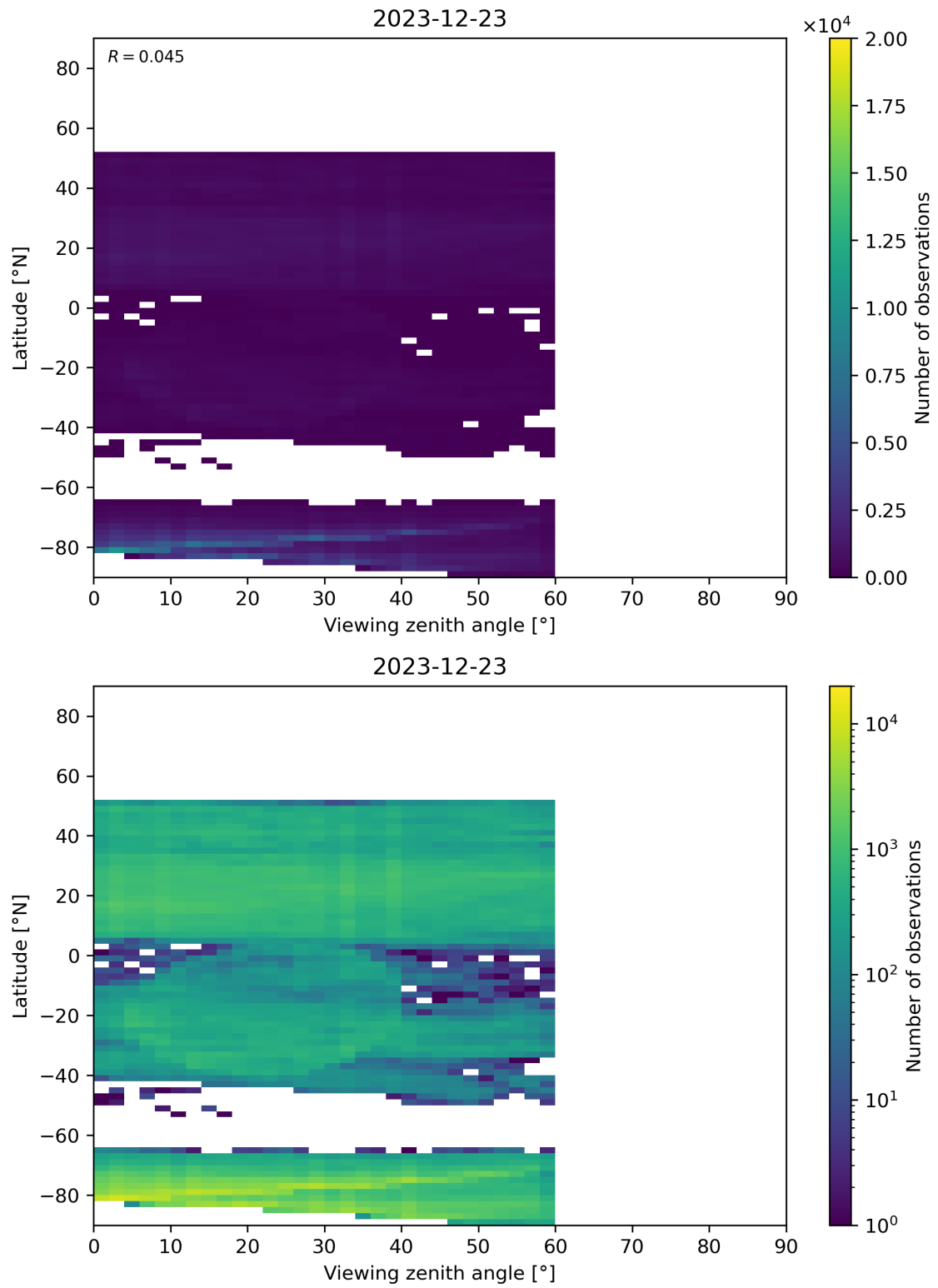
Figure 109: Scatter density plot of “Viewing zenith angle” against “Latitude” for 2023-12-22 to 2023-12-24.
