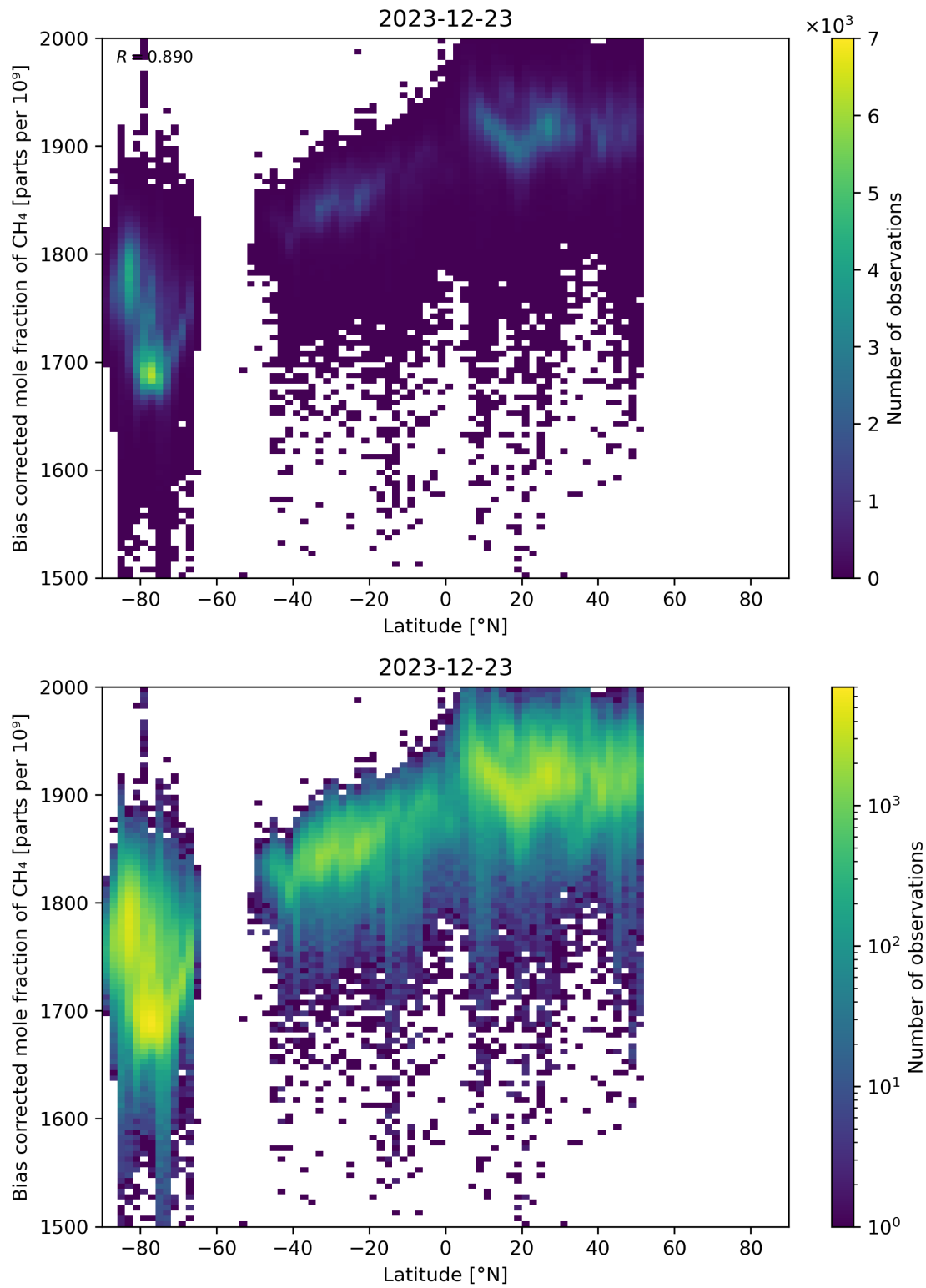
Figure 58: Scatter density plot of “Latitude” against “Bias corrected mole fraction of CH 4 ” for 2023-12-22 to 2023-12-24.
