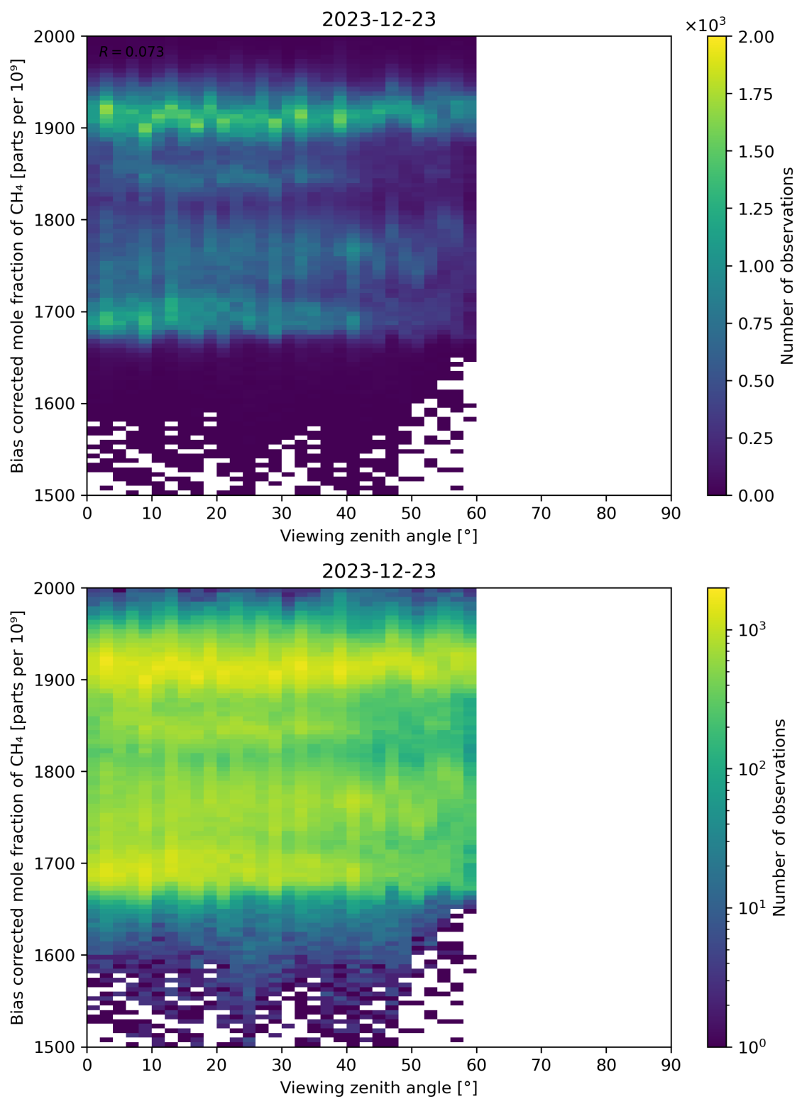
Figure 111: Scatter density plot of “Viewing zenith angle” against “Bias corrected mole fraction of CH 4 ” for 2023-12-22 to 2023-12-24.
