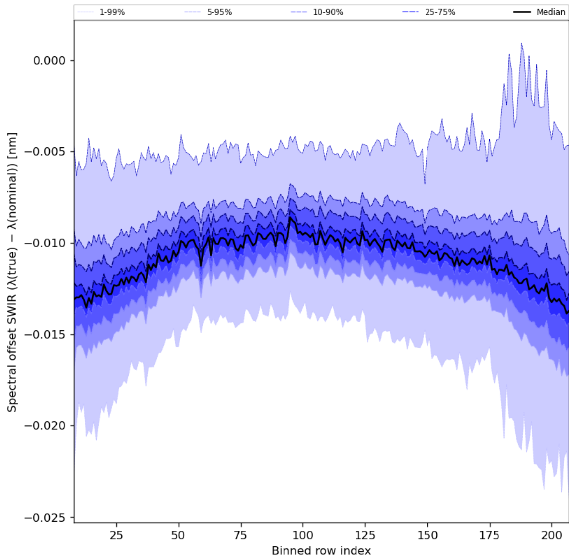
Figure 38: Along track statistics of “Spectral offset SWIR ( \lambda(\text{true}) - \lambda(\text{nominal}) )” for 2023-12-22 to 2023-12-24
