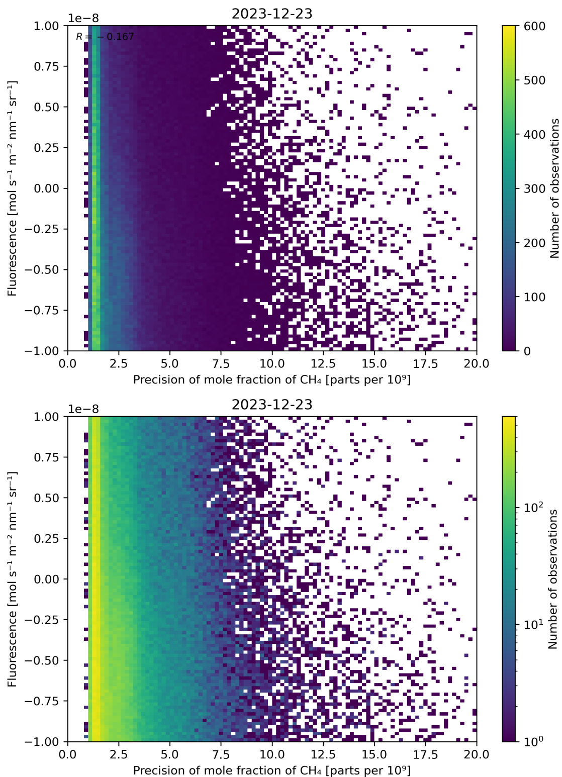
Figure 81: Scatter density plot of “Precision of mole fraction of \text{CH}_4 ” against “Fluorescence” for 2023-12-22 to 2023-12-24.
