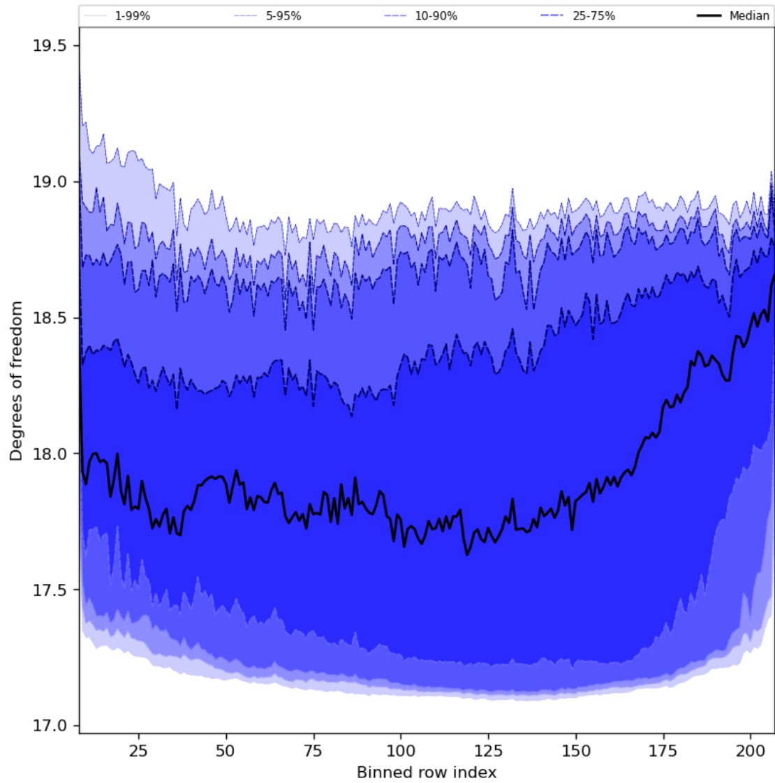
Figure 41: Along track statistics of “Degrees of freedom” for 2023-12-22 to 2023-12-24
