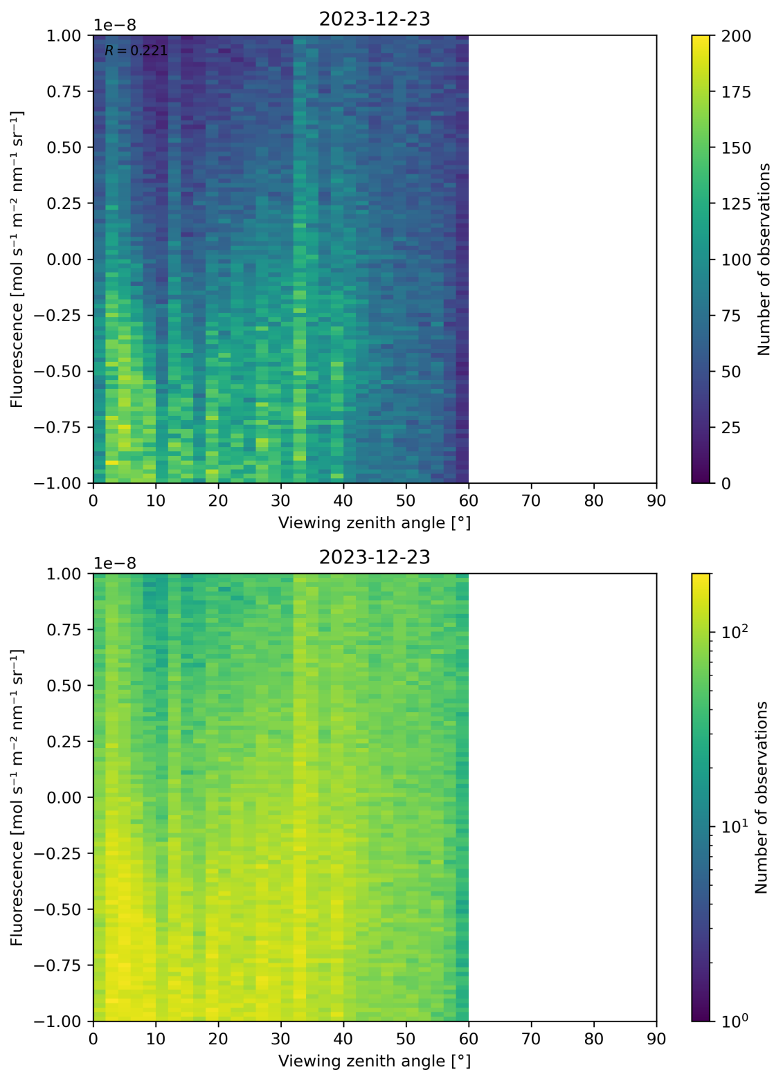
Figure 108: Scatter density plot of “Viewing zenith angle” against “Fluorescence” for 2023-12-22 to 2023-12-24.
