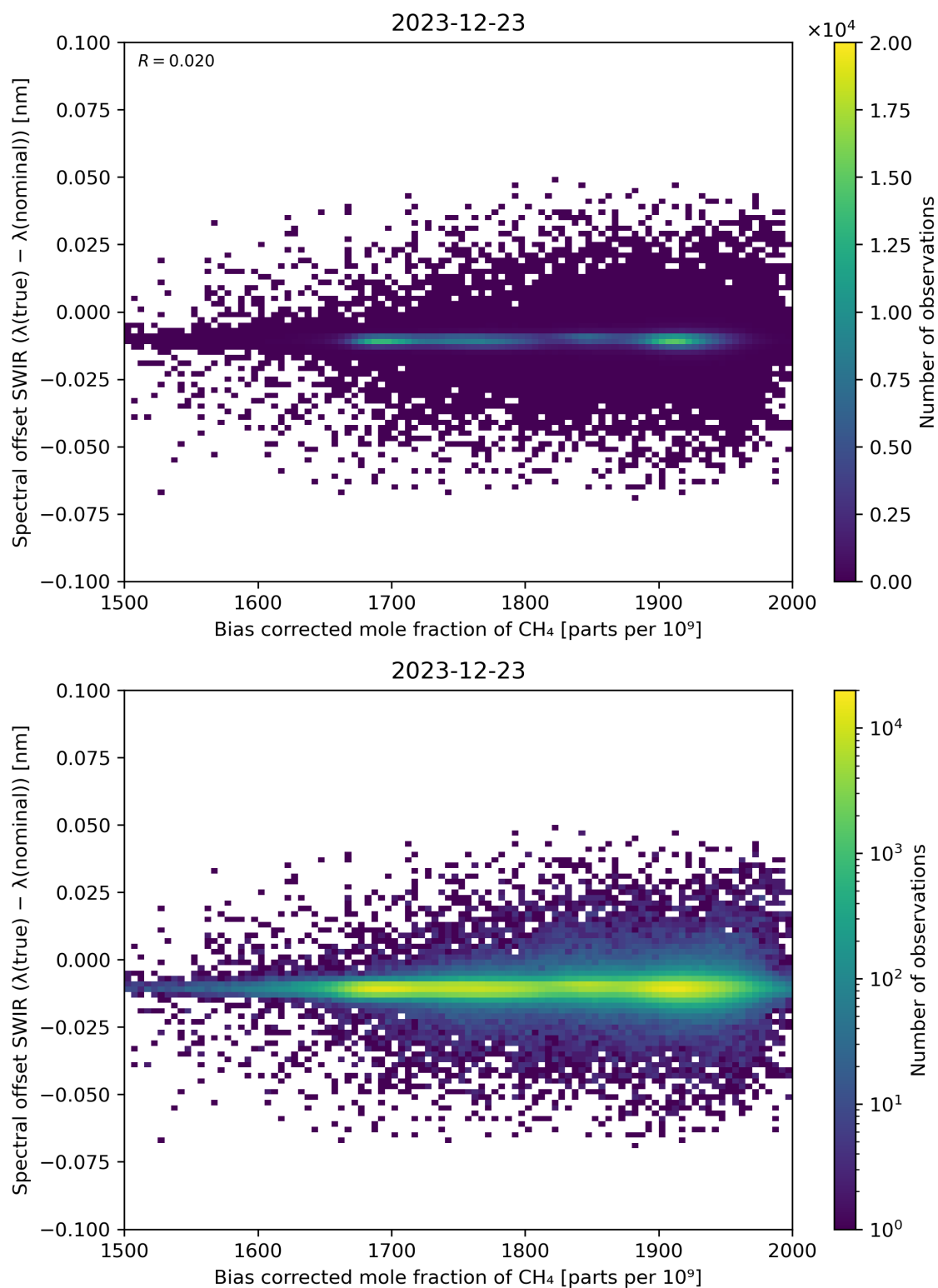
Figure 69: Scatter density plot of “Bias corrected mole fraction of \text{CH}_4 ” against “Spectral offset SWIR ( \lambda(\text{true}) - \lambda(\text{nominal}) )” for 2023-12-22 to 2023-12-24.
