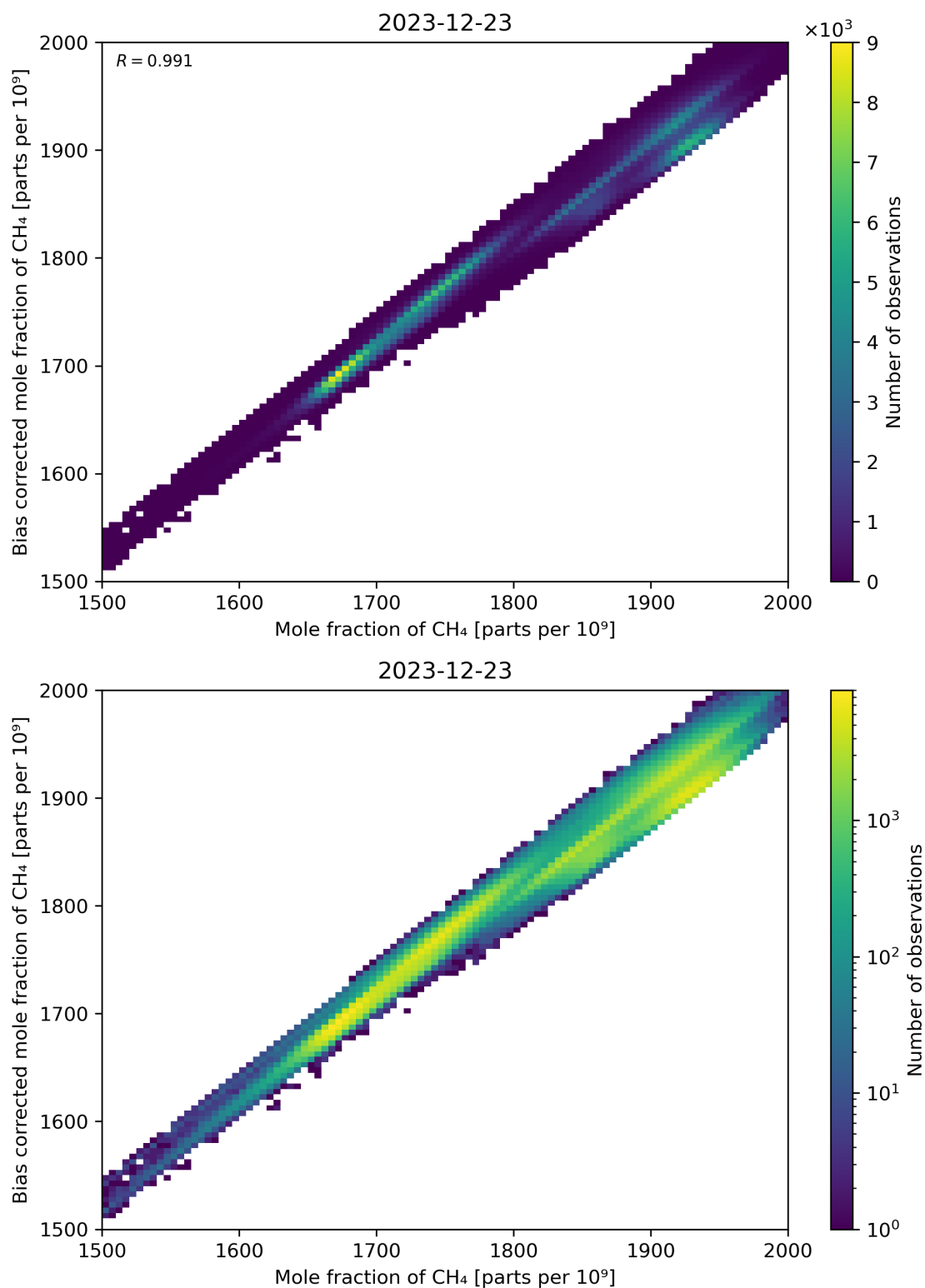
Figure 74: Scatter density plot of “Mole fraction of CH 4 ” against “Bias corrected mole fraction of CH 4 ” for 2023-12-22 to 2023-12-24.
