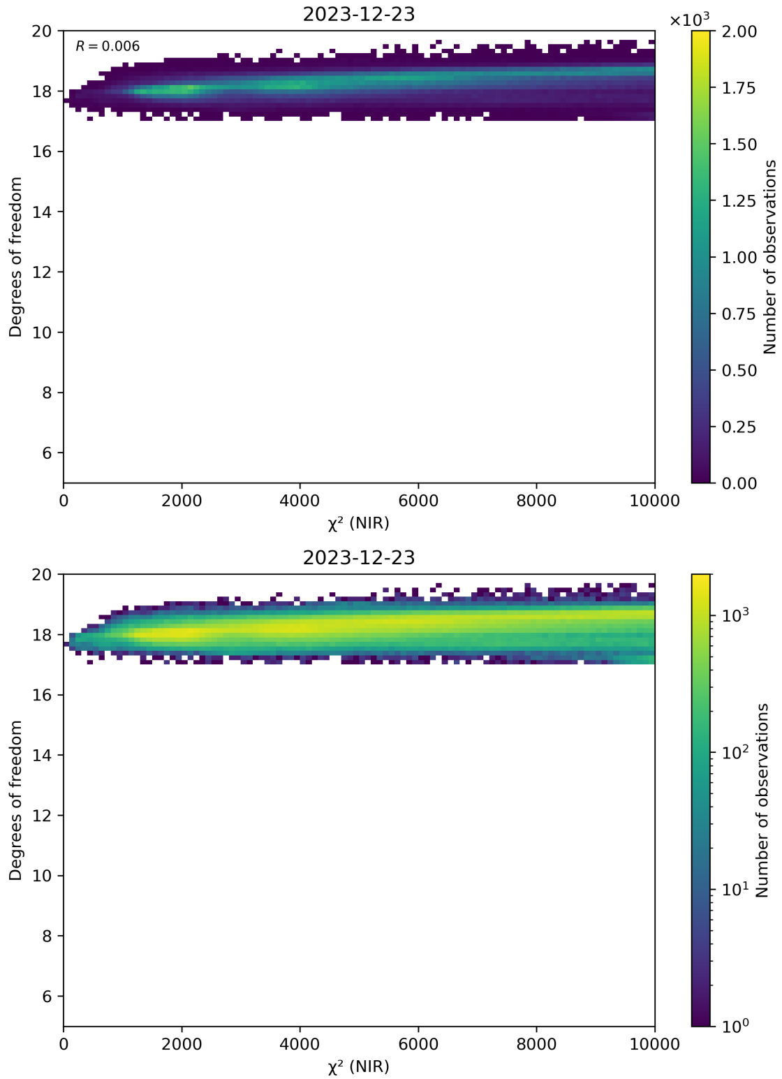
Figure 44: Scatter density plot of “ \chi^2 (NIR)” against “Degrees of freedom” for 2023-12-22 to 2023-12-24.
