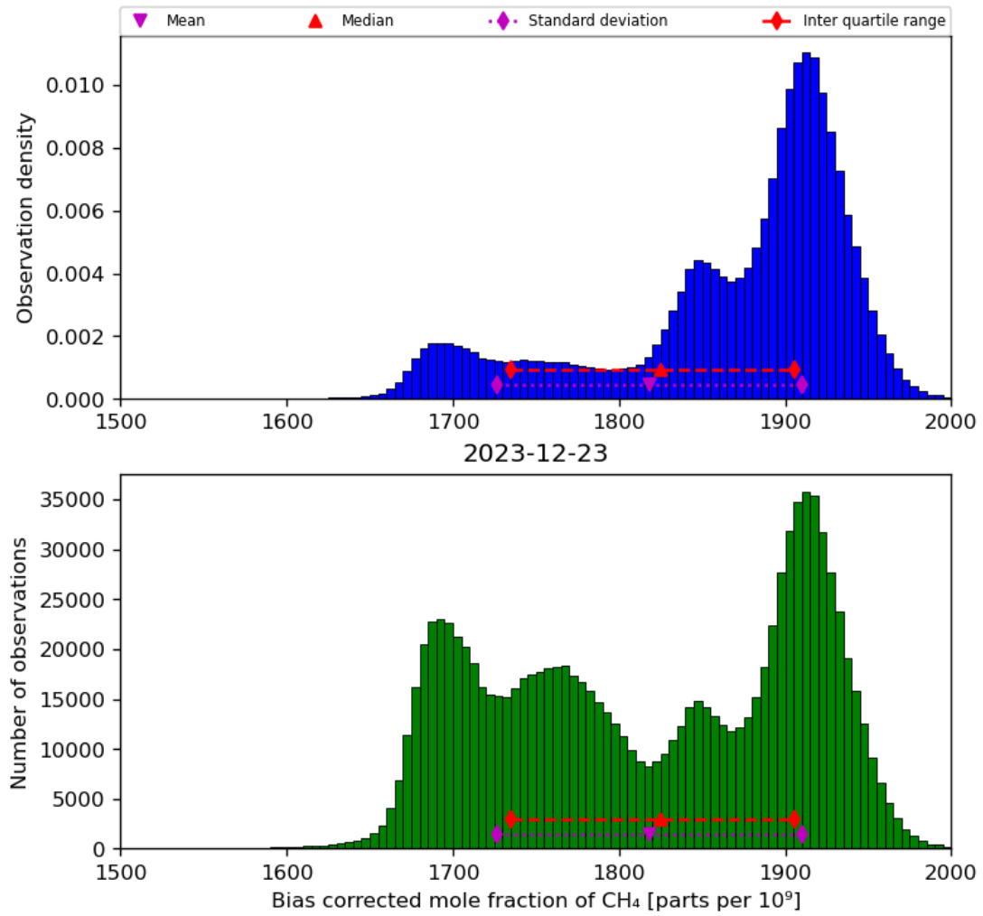
Figure 25: Histogram of “Bias corrected mole fraction of CH 4 ” for 2023-12-22 to 2023-12-24
