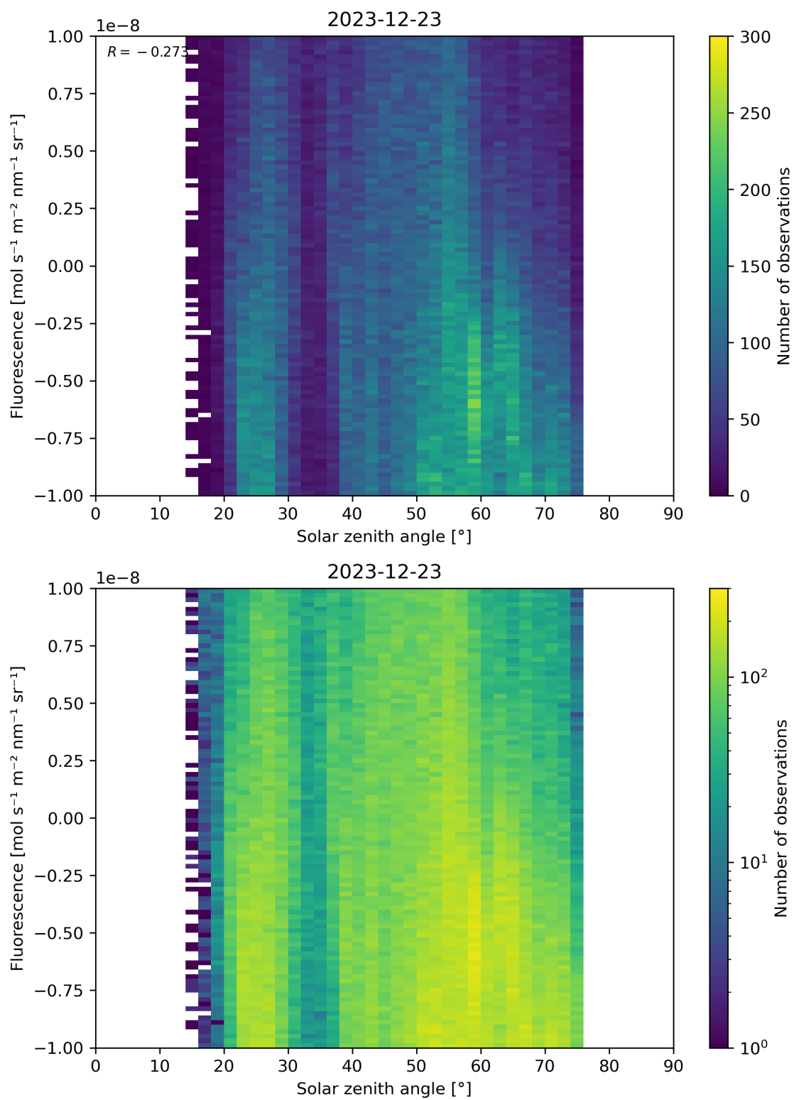
Figure 97: Scatter density plot of “Solar zenith angle” against “Fluorescence” for 2023-12-22 to 2023-12-24.
