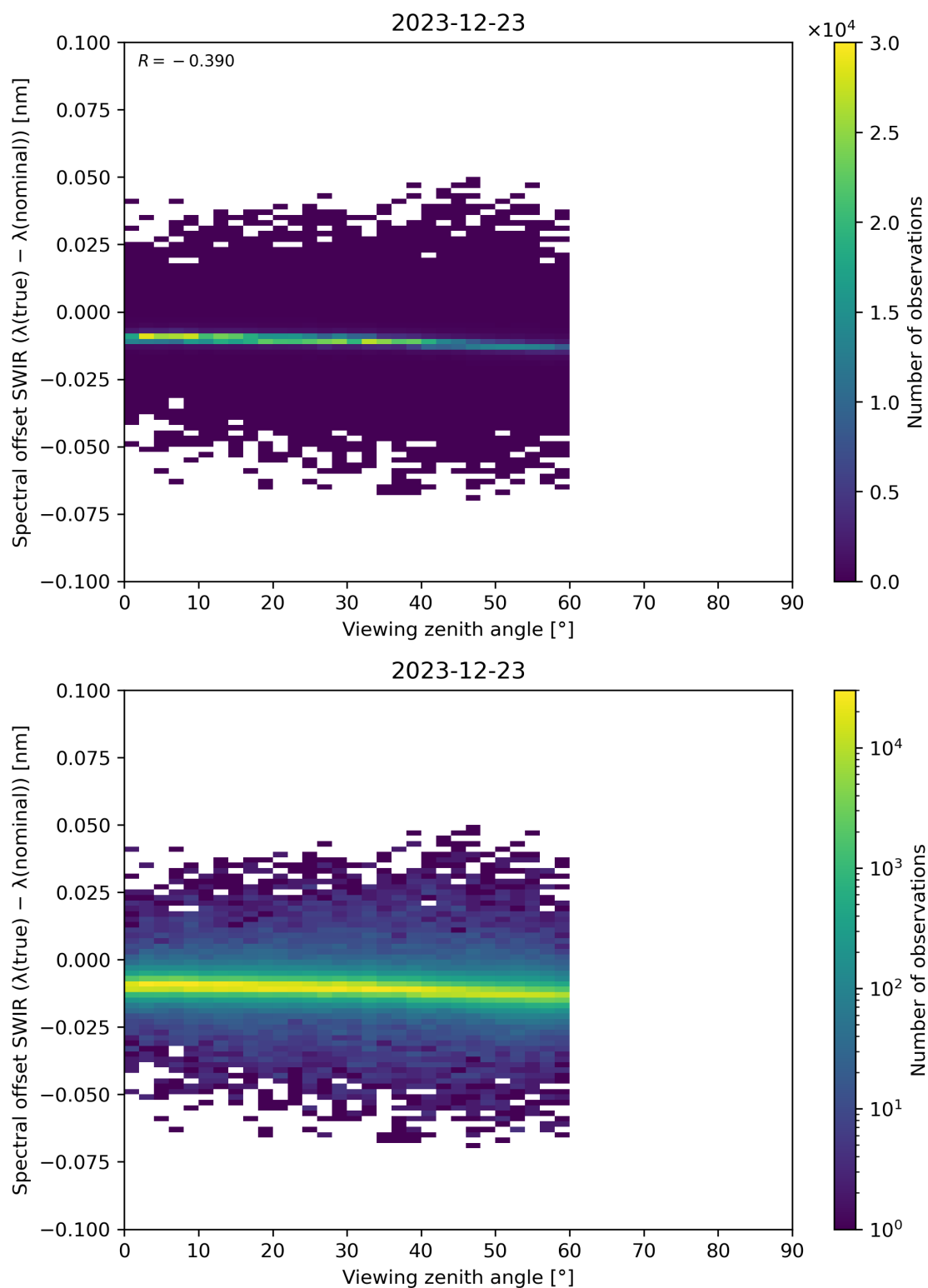
Figure 116: Scatter density plot of “Viewing zenith angle” against “Spectral offset SWIR ( \lambda(\text{true}) - \lambda(\text{nominal}) )” for 2023-12-22 to 2023-12-24.
