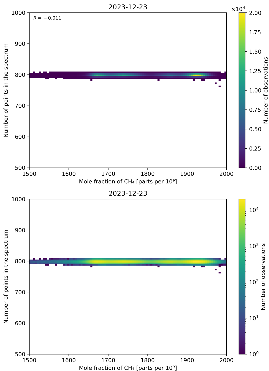
Figure 77: Scatter density plot of “Mole fraction of CH 4 ” against “Number of points in the spectrum” for 2023-12-22 to 2023-12-24.
