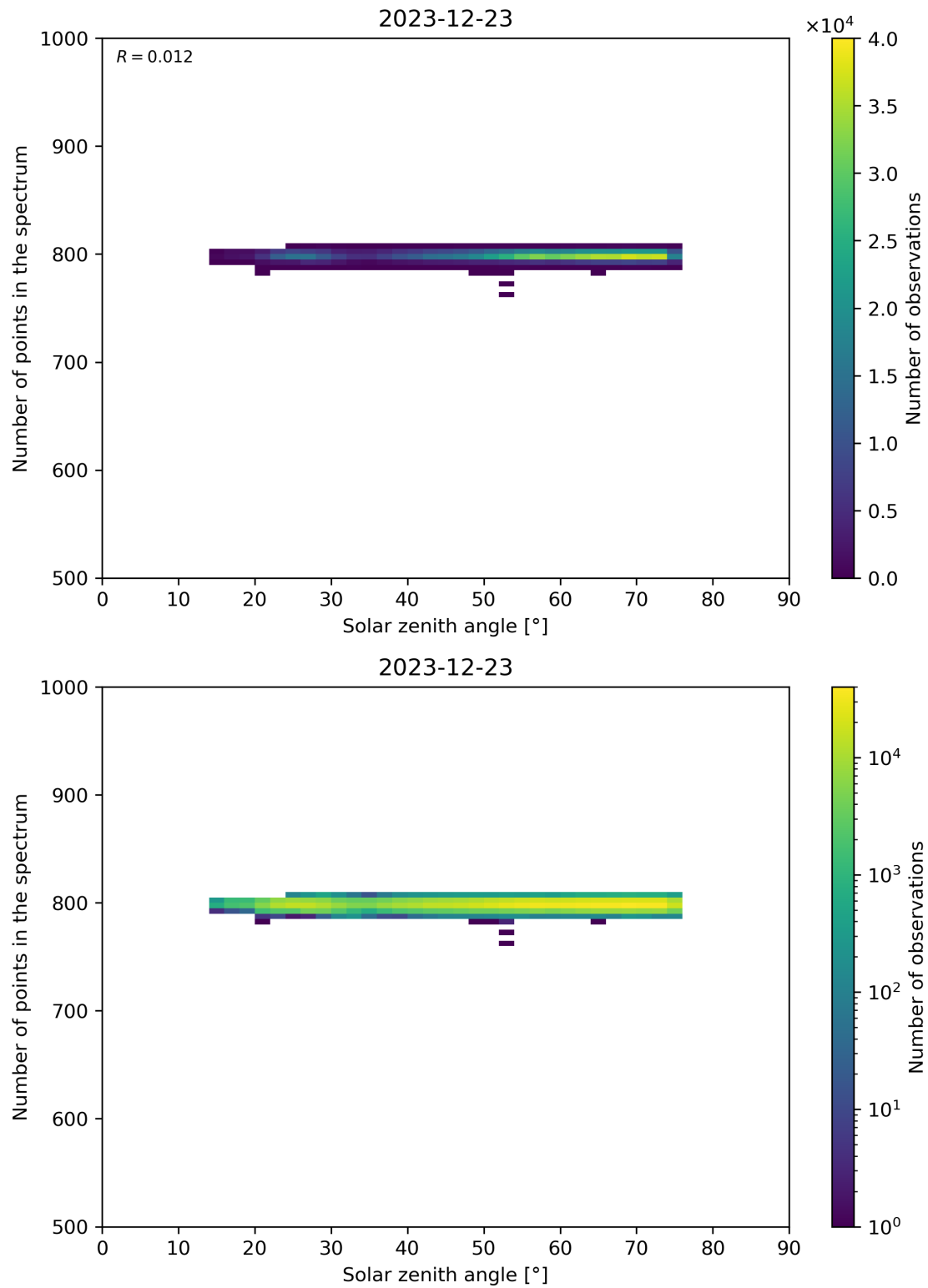
Figure 103: Scatter density plot of “Solar zenith angle” against “Number of points in the spectrum” for 2023-12-22 to 2023-12-24.
