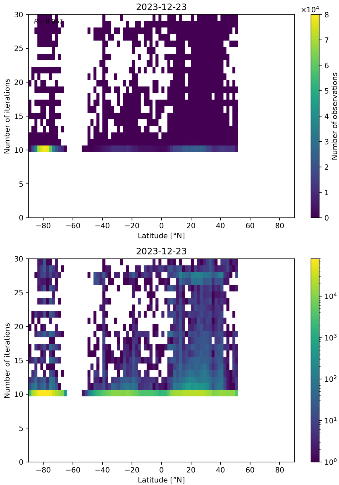
Figure 60: Scatter density plot of “Latitude” against “Number of iterations” for 2023-12-22 to 2023-12-24.
