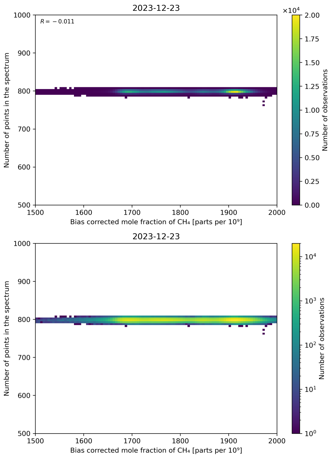
Figure 68: Scatter density plot of “Bias corrected mole fraction of CH 4 ” against “Number of points in the spectrum” for 2023-12-22 to 2023-12-24.
