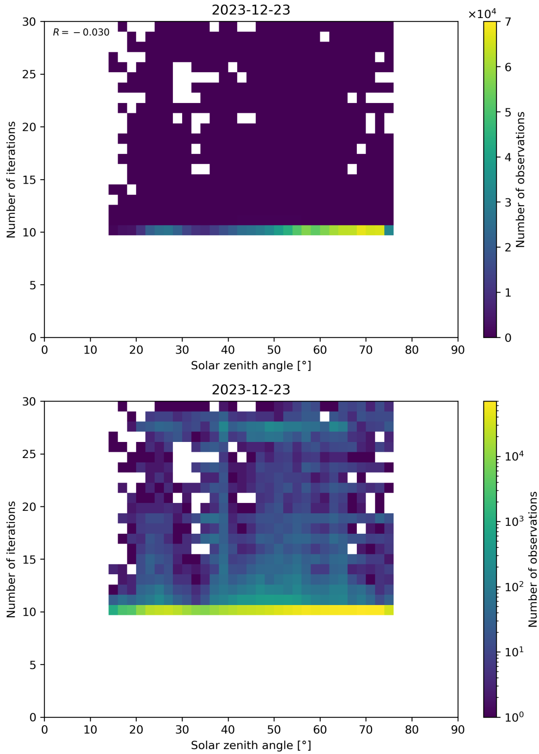
Figure 102: Scatter density plot of “Solar zenith angle” against “Number of iterations” for 2023-12-22 to 2023-12-24.
