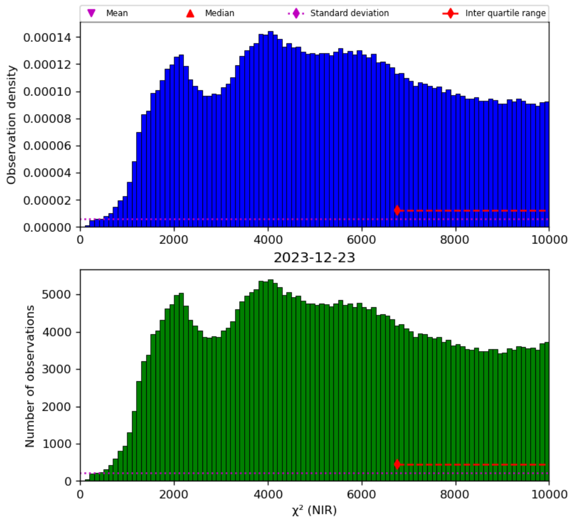
Figure 29: Histogram of “ \chi^2 (NIR)” for 2023-12-22 to 2023-12-24
