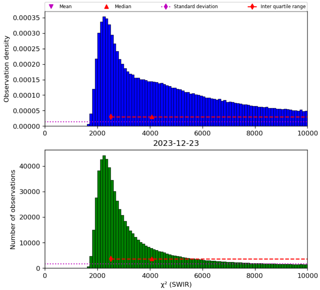
Figure 28: Histogram of “ \chi^2 (SWIR)” for 2023-12-22 to 2023-12-24
