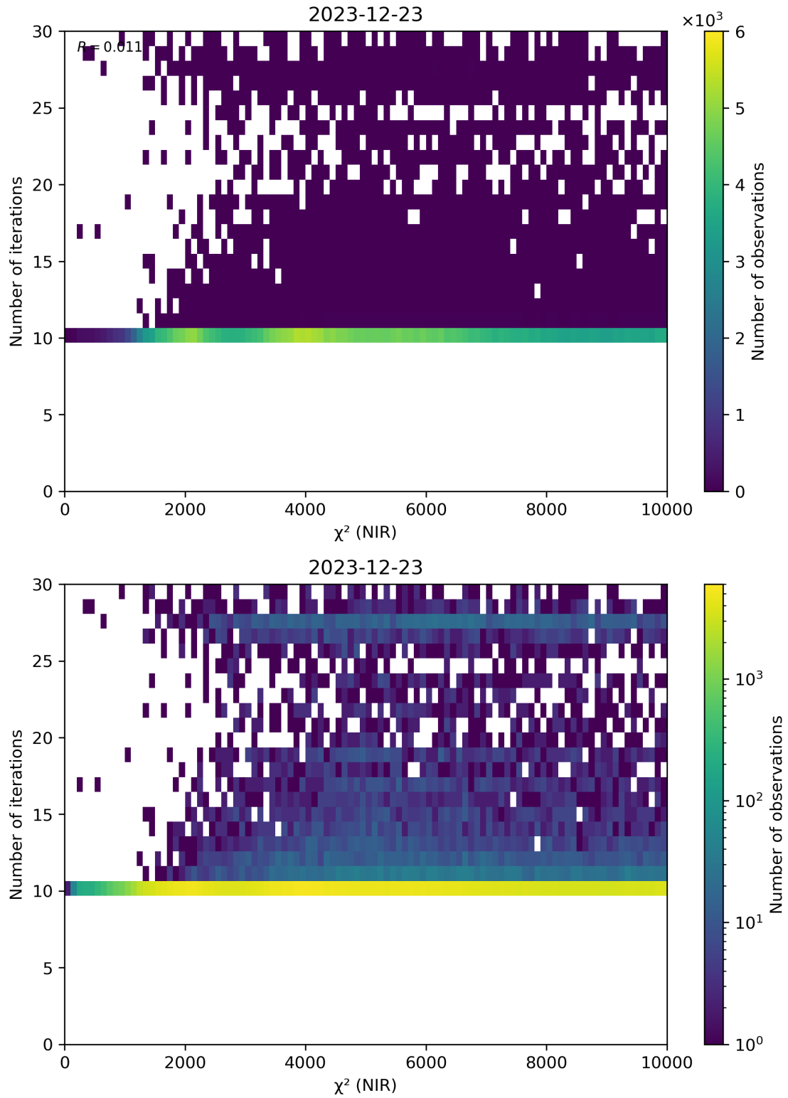
Figure 46: Scatter density plot of “ \chi^2 (NIR)” against “Number of iterations” for 2023-12-22 to 2023-12-24.
