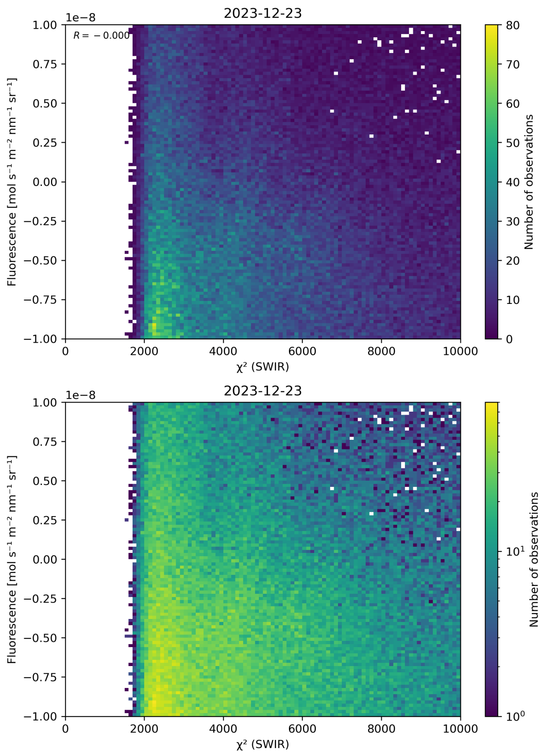
Figure 49: Scatter density plot of “ \chi^2 (SWIR)” against “Fluorescence” for 2023-12-22 to 2023-12-24.
