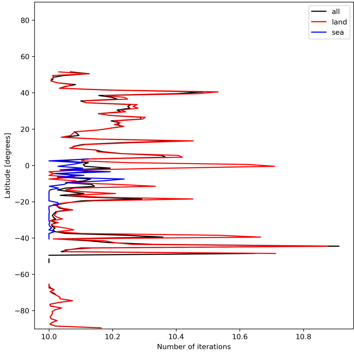
Figure 20: Zonal average of “Number of iterations” for 2023-12-22 to 2023-12-24.
