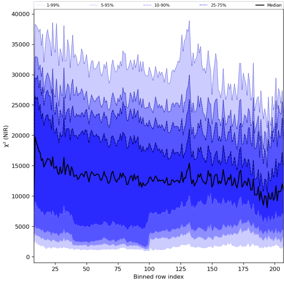
Figure 40: Along track statistics of “ \chi^2 (NIR)” for 2023-12-22 to 2023-12-24
