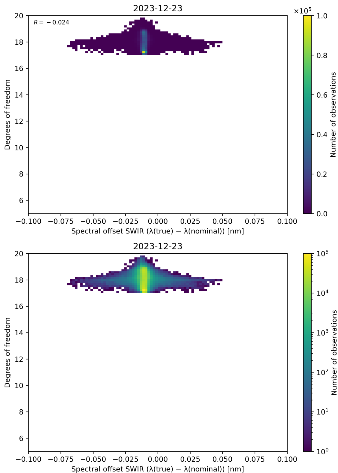
Figure 119: Scatter density plot of “Spectral offset SWIR ( \lambda(\text{true}) - \lambda(\text{nominal}) )” against “Degrees of freedom” for 2023-12-22 to 2023-12-24.
