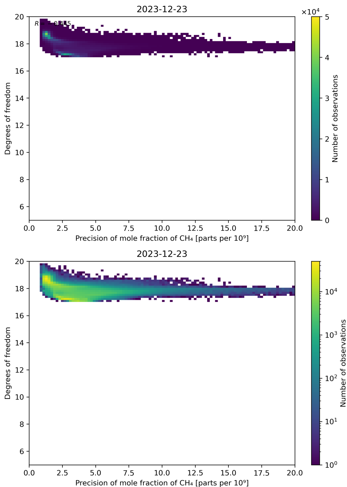
Figure 80: Scatter density plot of “Precision of mole fraction of CH 4 ” against “Degrees of freedom” for 2023-12-22 to 2023-12-24.
