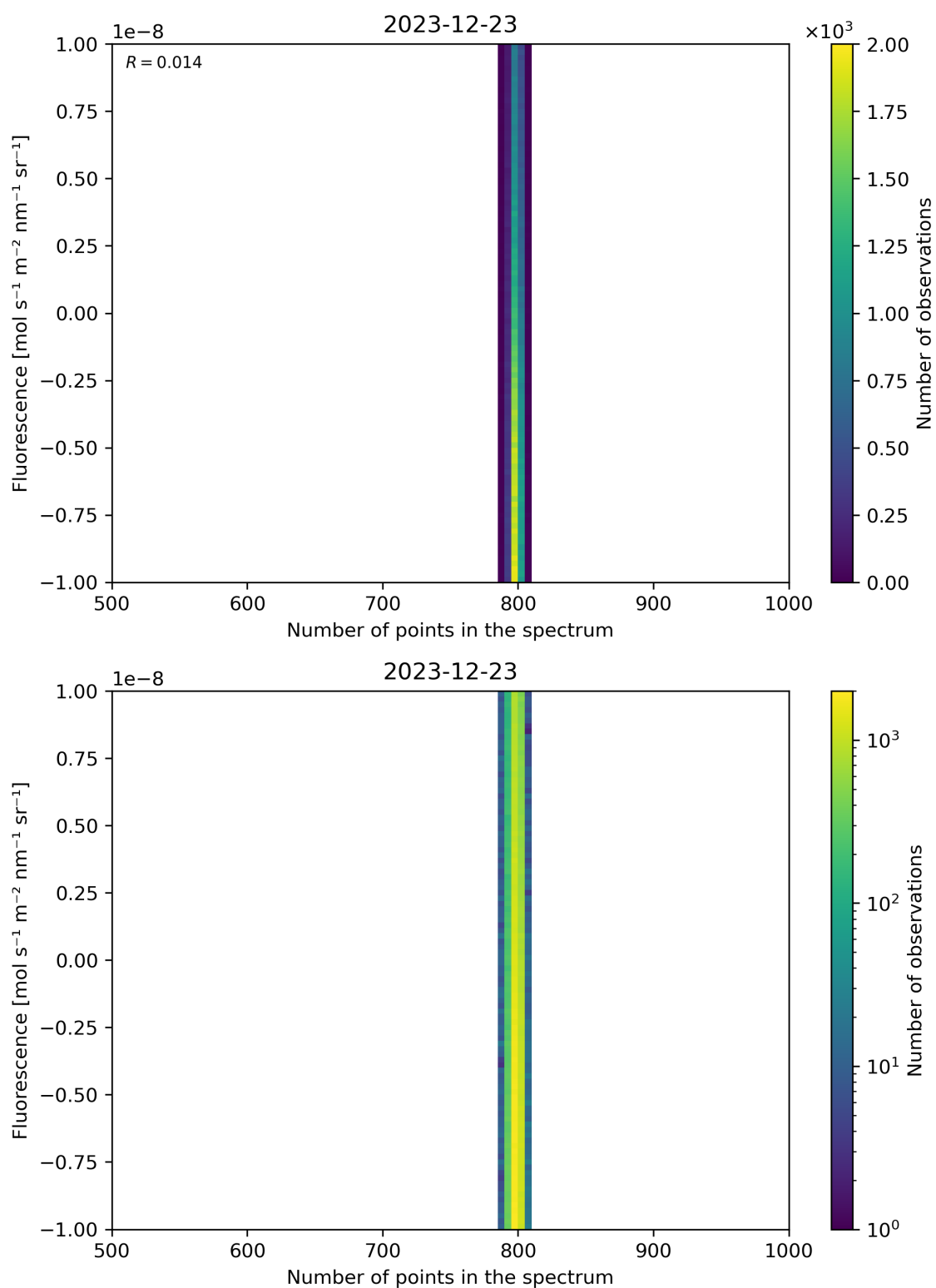
Figure 91: Scatter density plot of “Number of points in the spectrum” against “Fluorescence” for 2023-12-22 to 2023-12-24.
