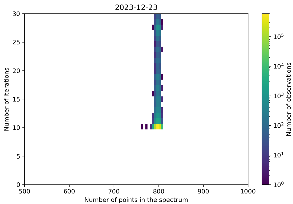
Figure 92: Scatter density plot of “Number of points in the spectrum” against “Number of iterations” for 2023-12-22 to 2023-12-24.
