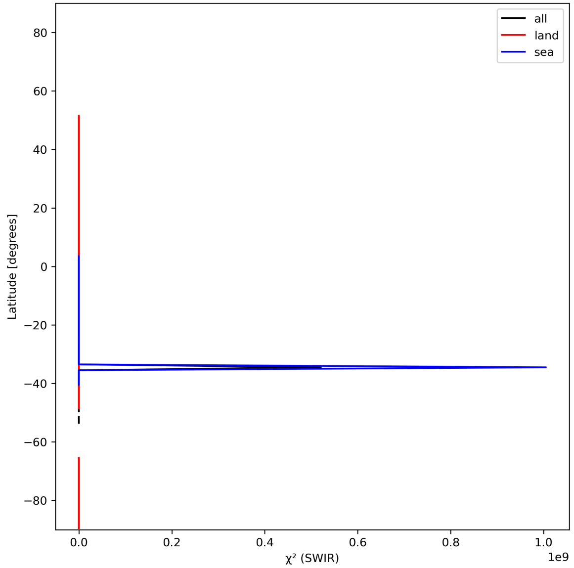
Figure 17: Zonal average of “ \chi^2 (SWIR)” for 2023-12-22 to 2023-12-24.
