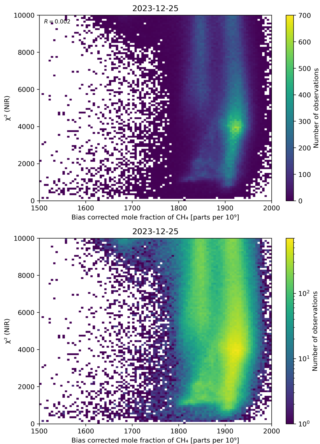
Figure 63: Scatter density plot of “Bias corrected mole fraction of CH 4 ” against “ \chi^2 (NIR)” for 2023-12-25 to 2023-12-26.
