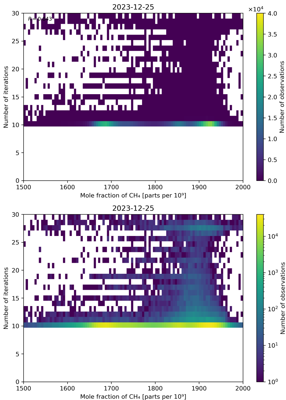
Figure 76: Scatter density plot of “Mole fraction of CH 4 ” against “Number of iterations” for 2023-12-25 to 2023-12-26.
