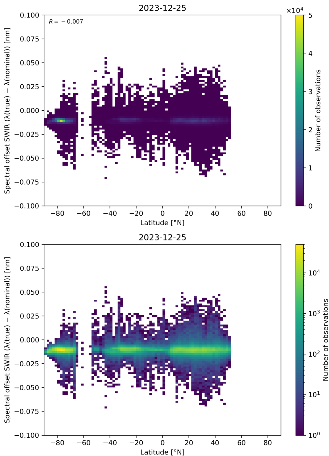
Figure 62: Scatter density plot of “Latitude” against “Spectral offset SWIR ( \lambda(\text{true}) - \lambda(\text{nominal}) )” for 2023-12-25 to 2023-12-26.
