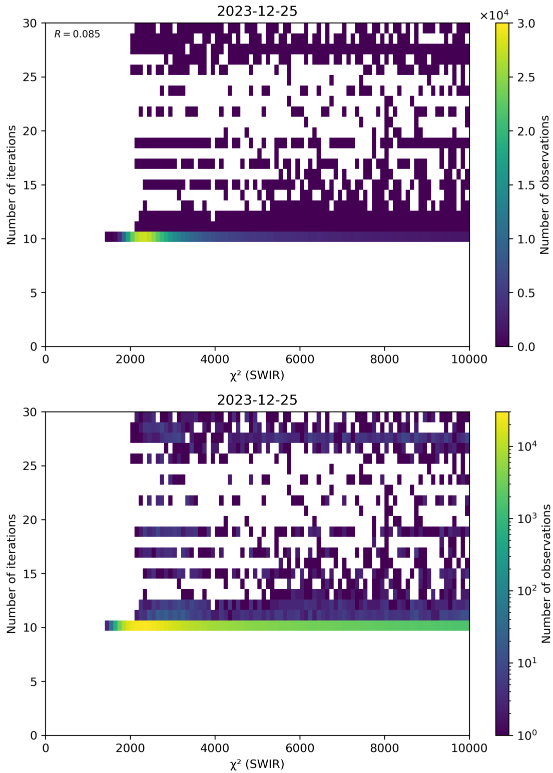
Figure 50: Scatter density plot of “ \chi^2 (SWIR)” against “Number of iterations” for 2023-12-25 to 2023-12-26.
