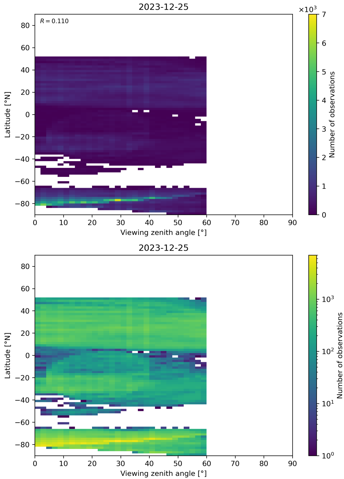
Figure 109: Scatter density plot of “Viewing zenith angle” against “Latitude” for 2023-12-25 to 2023-12-26.
