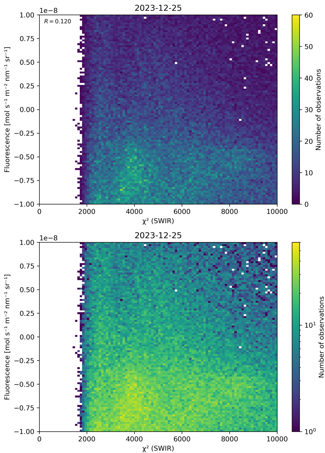
Figure 49: Scatter density plot of “ \chi^2 (SWIR)” against “Fluorescence” for 2023-12-25 to 2023-12-26.
