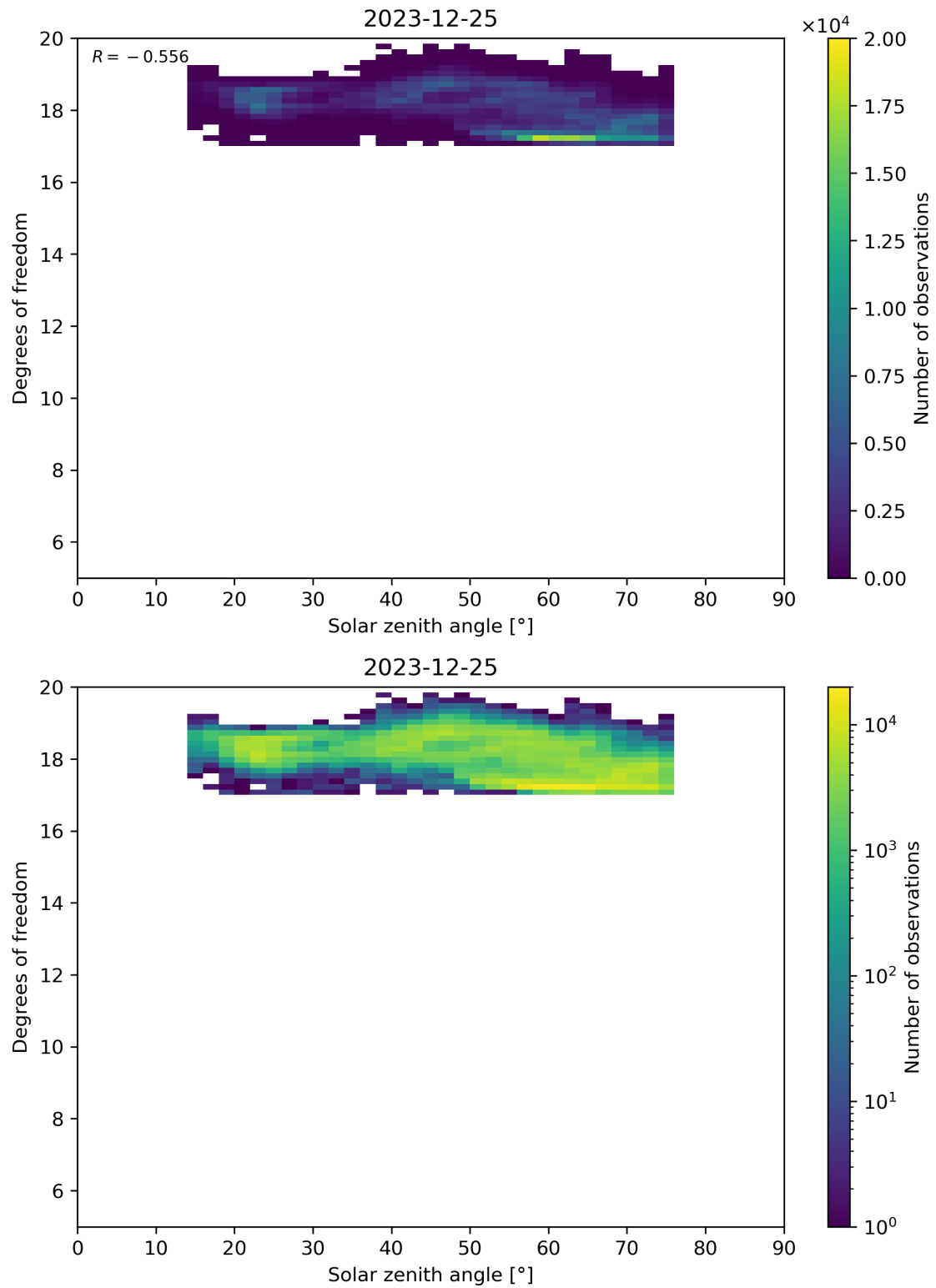
Figure 96: Scatter density plot of “Solar zenith angle” against “Degrees of freedom” for 2023-12-25 to 2023-12-26.
