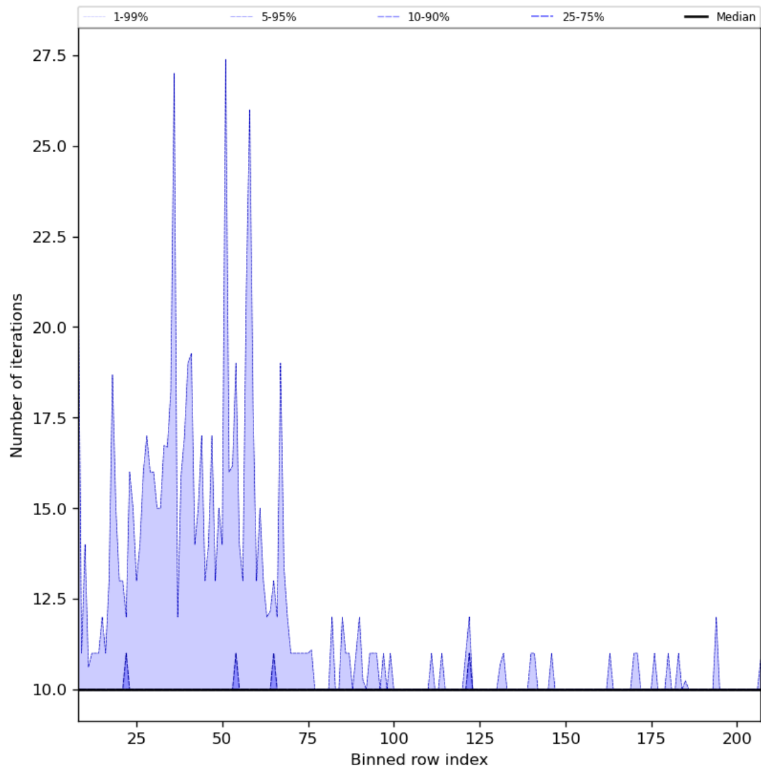
Figure 42: Along track statistics of “Number of iterations” for 2023-12-25 to 2023-12-26
