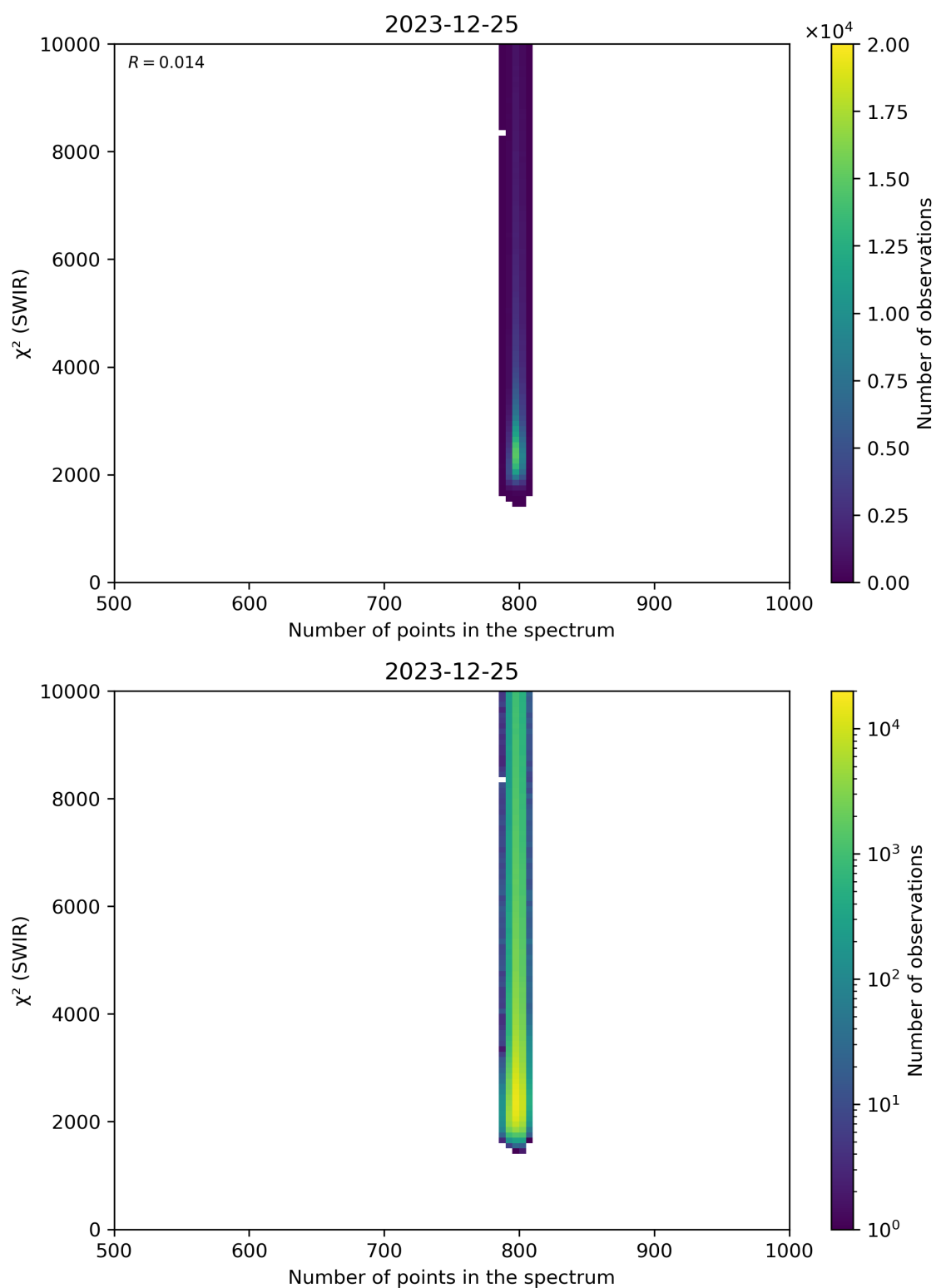
Figure 89: Scatter density plot of “Number of points in the spectrum” against “ \chi^2 (SWIR)” for 2023-12-25 to 2023-12-26.
