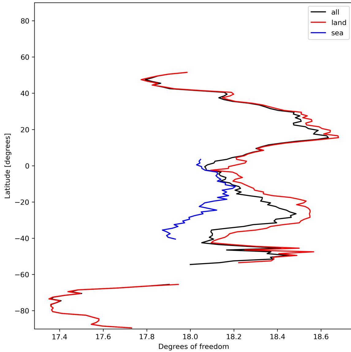
Figure 19: Zonal average of “Degrees of freedom” for 2023-12-25 to 2023-12-26.
