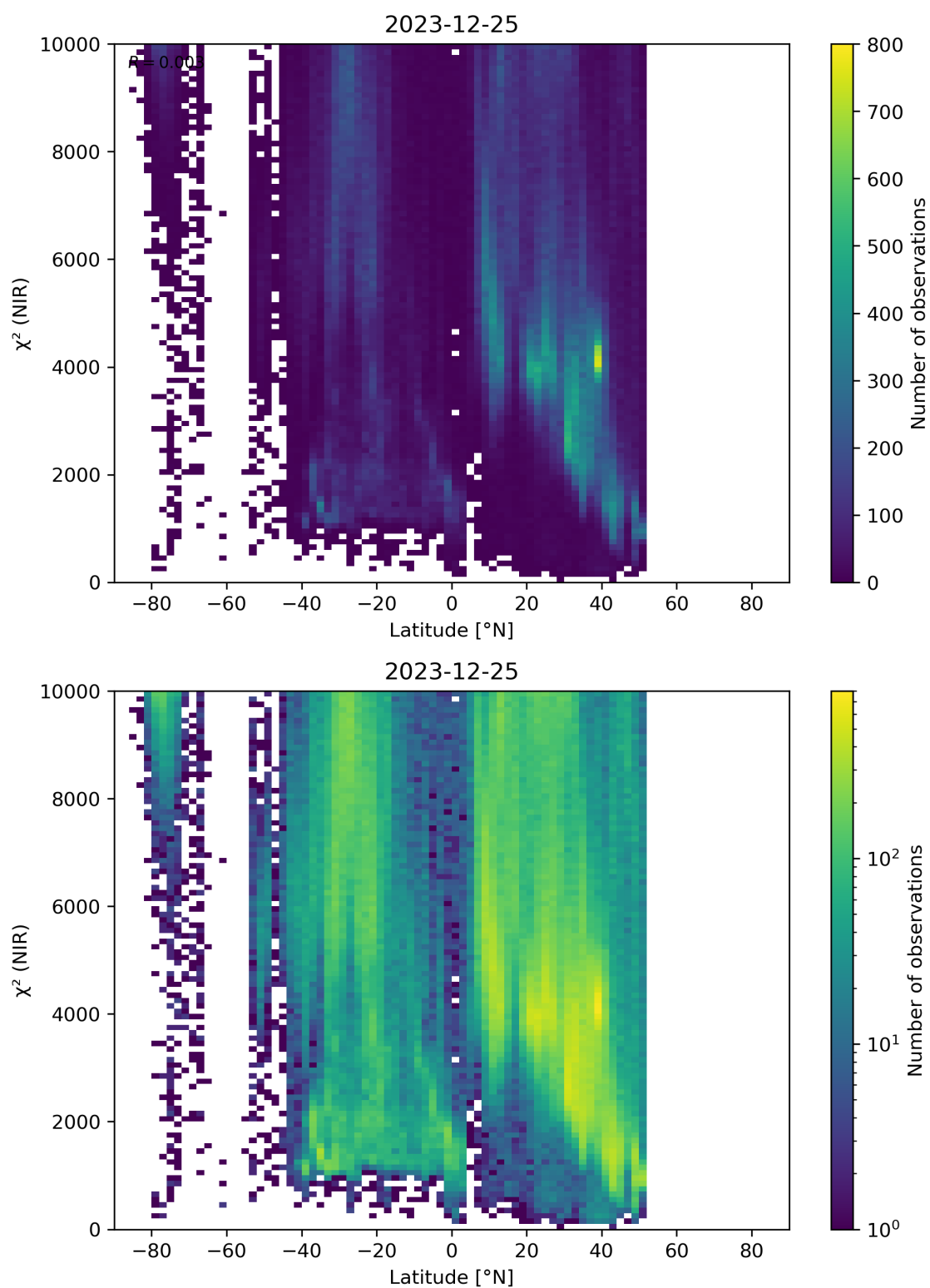
Figure 53: Scatter density plot of “Latitude” against “ \chi^2 (NIR)” for 2023-12-25 to 2023-12-26.
