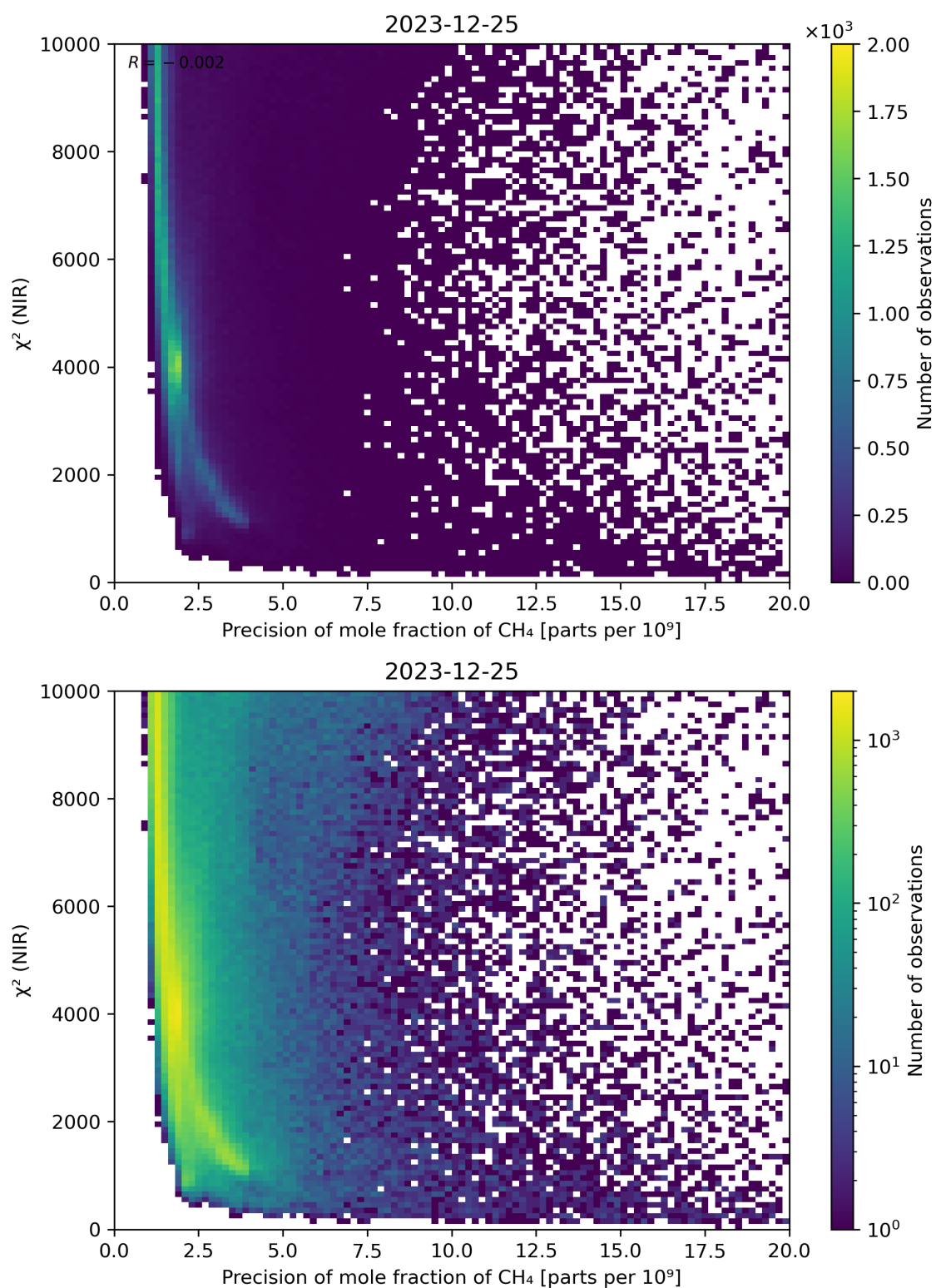
Figure 78: Scatter density plot of “Precision of mole fraction of \text{CH}_4 ” against “ \chi^2 (NIR)” for 2023-12-25 to 2023-12-26.
