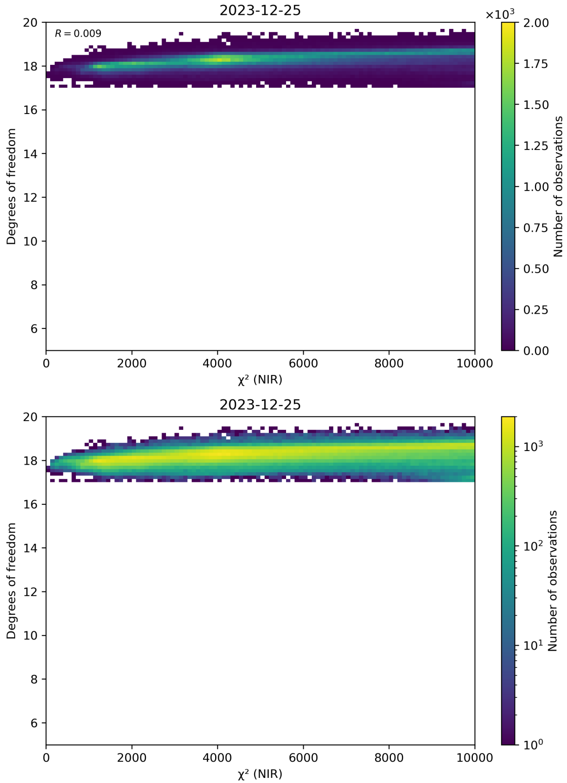
Figure 44: Scatter density plot of “ \chi^2 (NIR)” against “Degrees of freedom” for 2023-12-25 to 2023-12-26.
