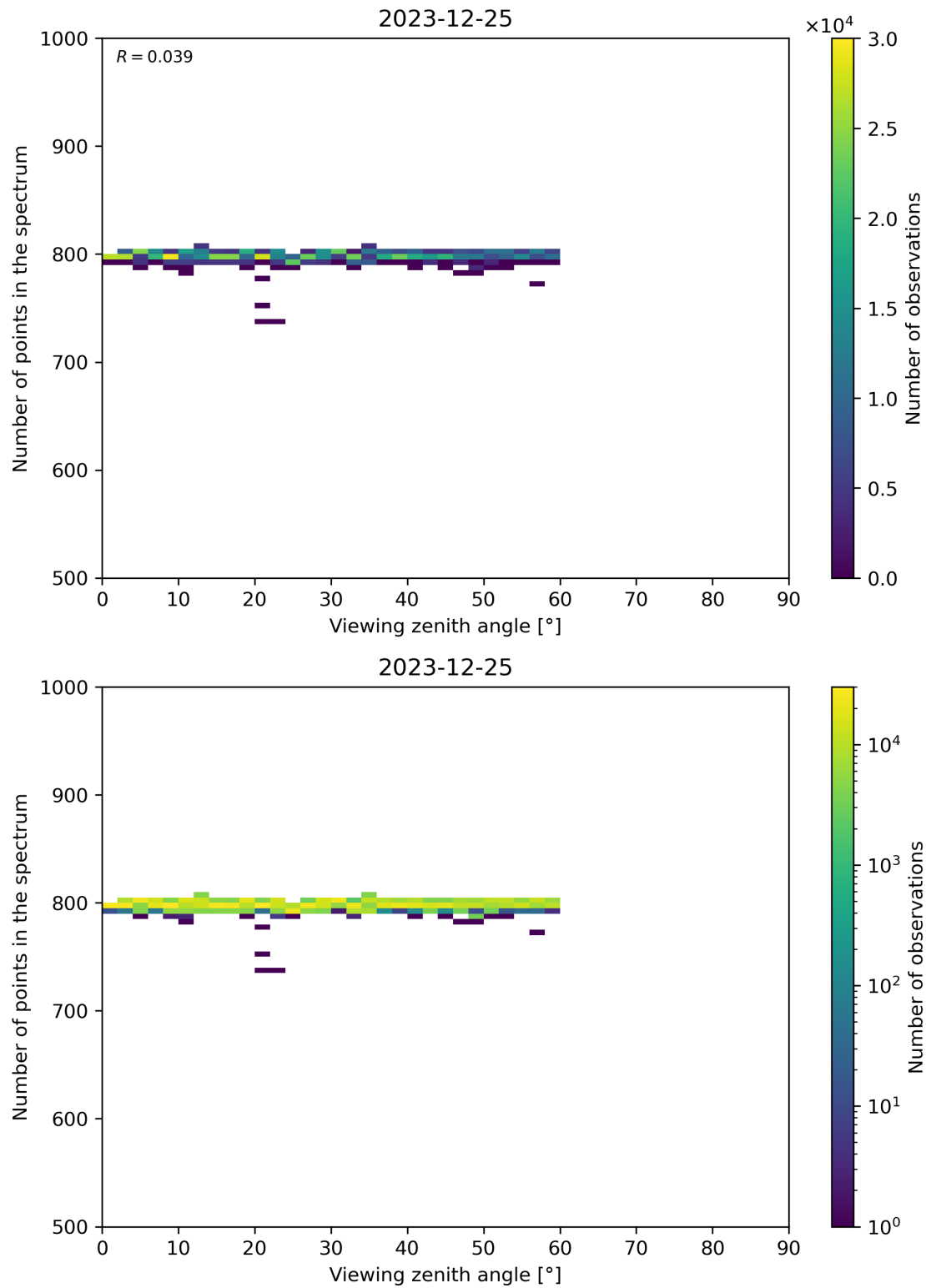
Figure 114: Scatter density plot of “Viewing zenith angle” against “Number of points in the spectrum” for 2023-12-25 to 2023-12-26.
