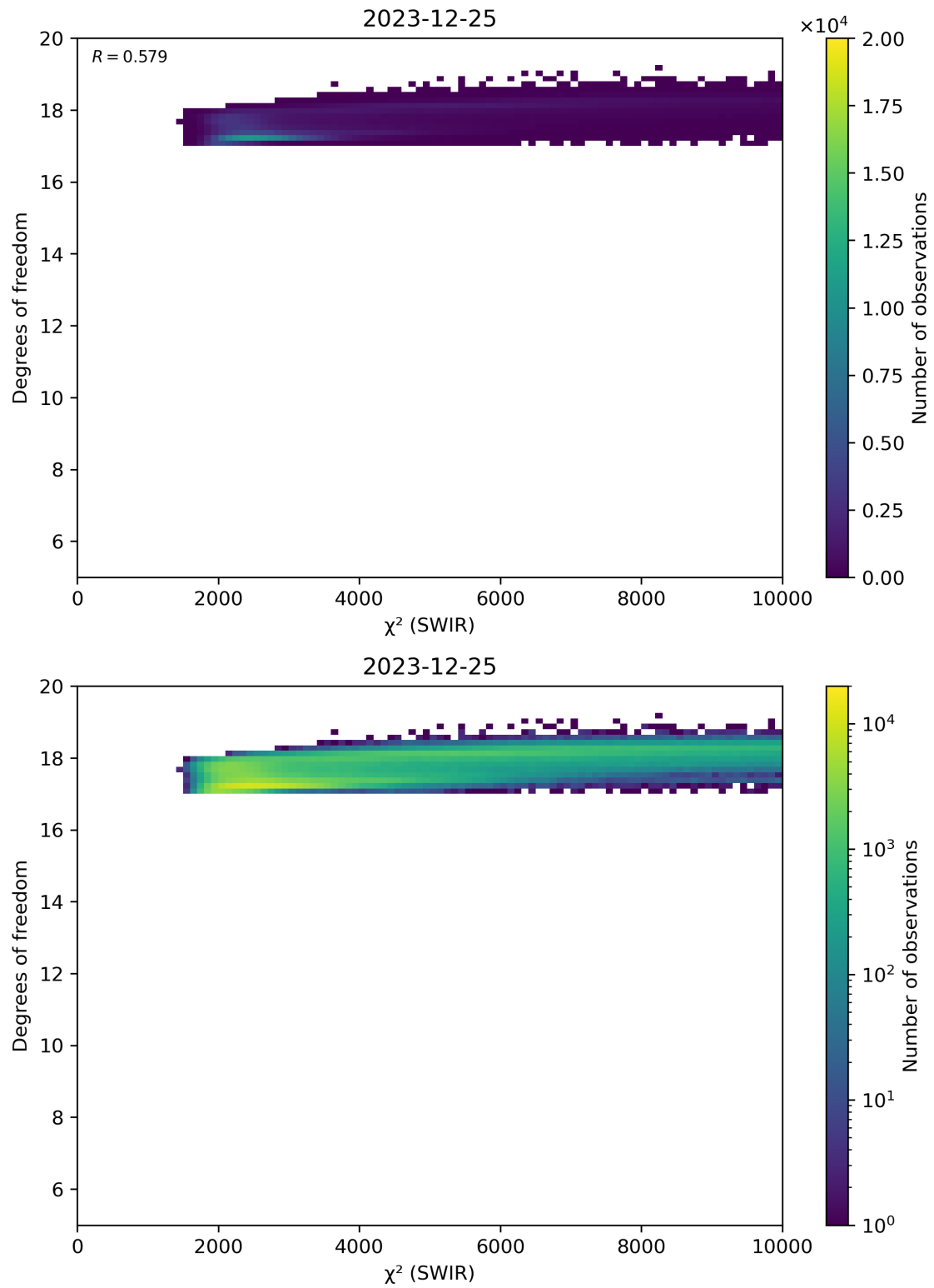
Figure 48: Scatter density plot of “ \chi^2 (SWIR)” against “Degrees of freedom” for 2023-12-25 to 2023-12-26.
