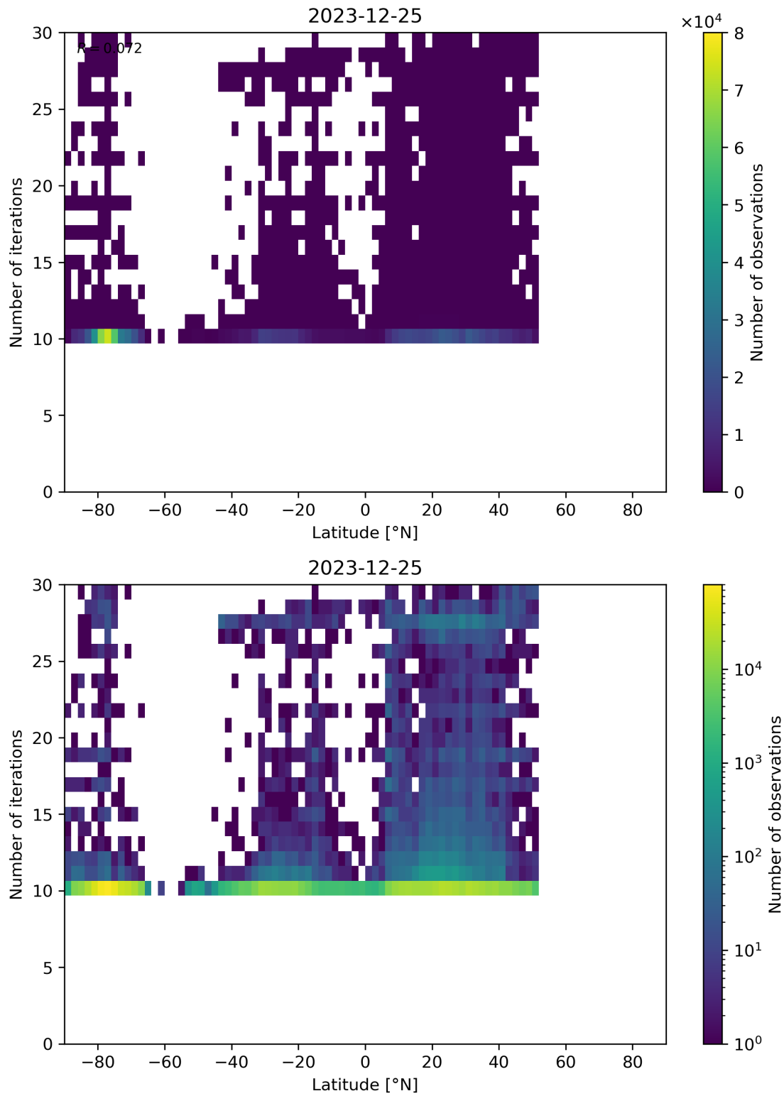
Figure 60: Scatter density plot of “Latitude” against “Number of iterations” for 2023-12-25 to 2023-12-26.
