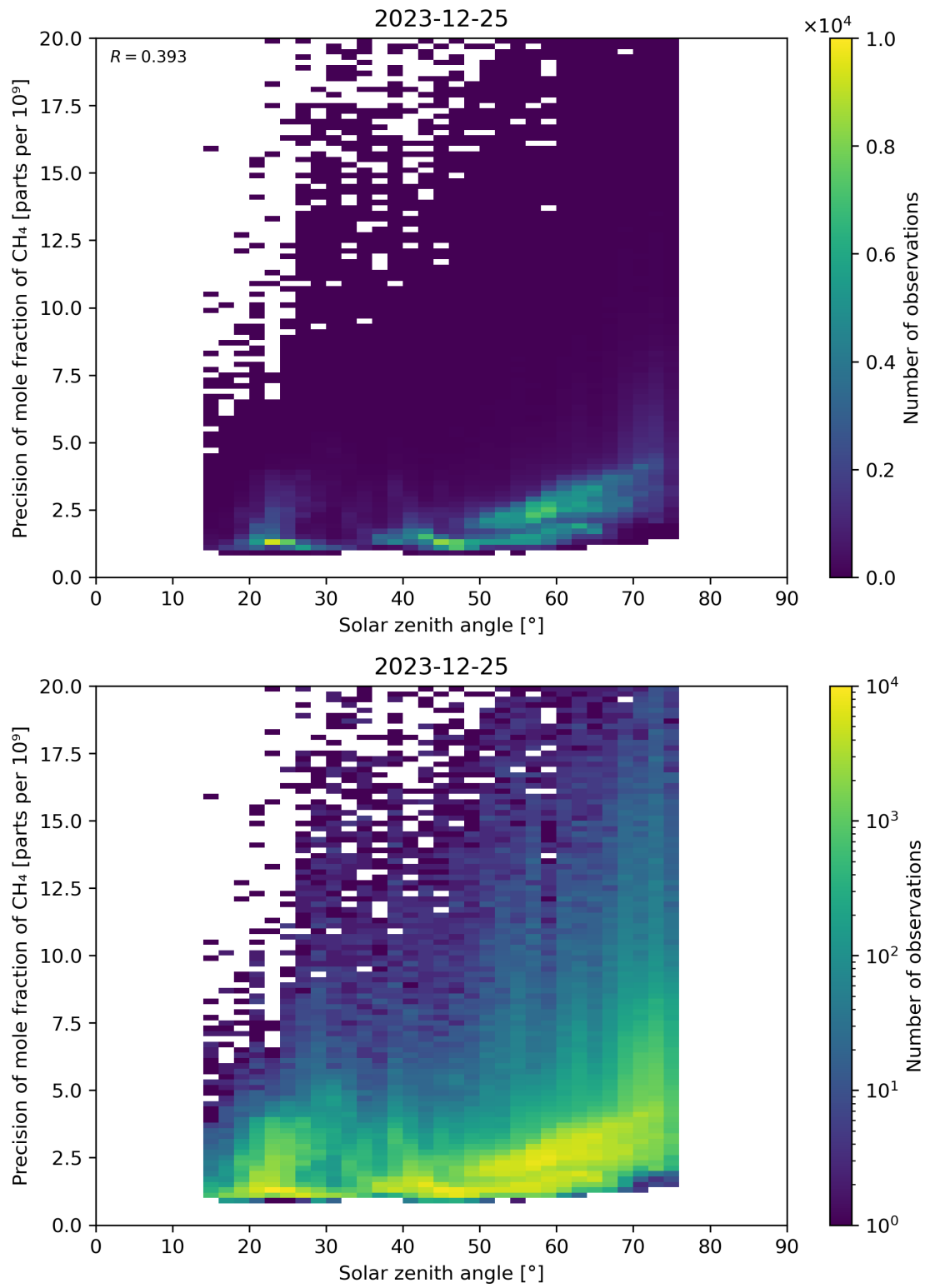
Figure 101: Scatter density plot of “Solar zenith angle” against “Precision of mole fraction of \text{CH}_4 ” for 2023-12-25 to 2023-12-26.
