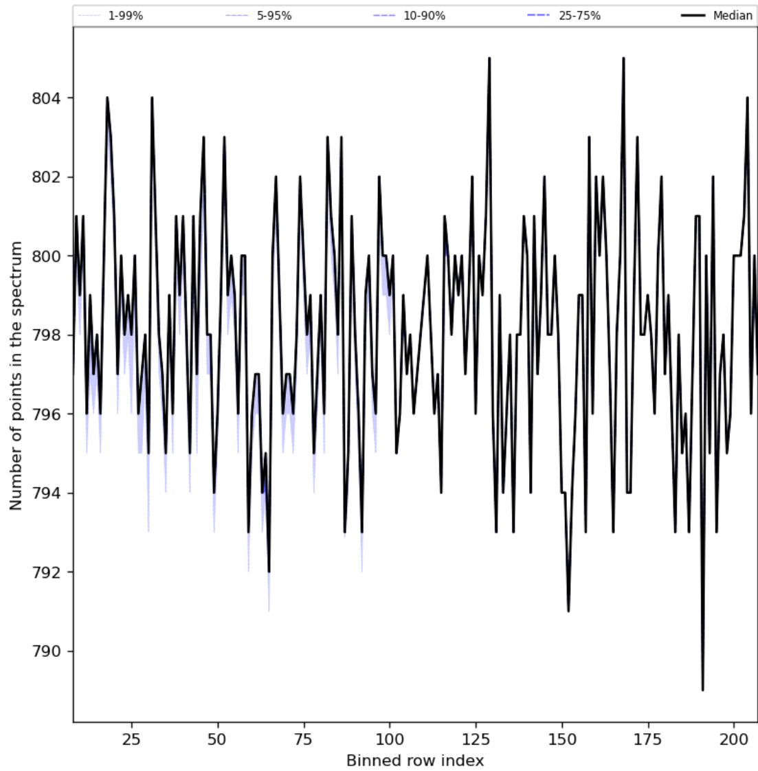
Figure 37: Along track statistics of “Number of points in the spectrum” for 2023-12-25 to 2023-12-26
