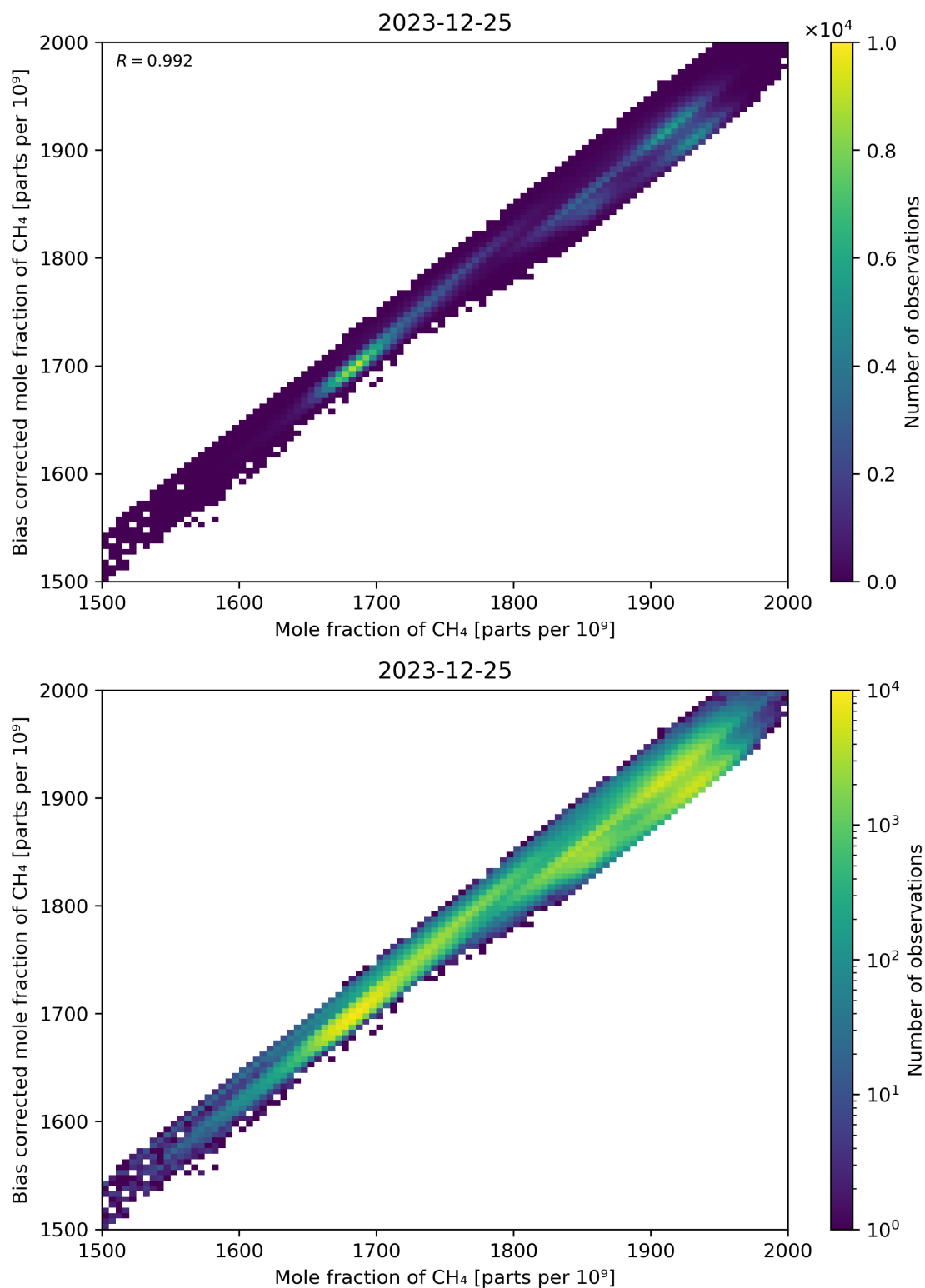
Figure 74: Scatter density plot of “Mole fraction of CH 4 ” against “Bias corrected mole fraction of CH 4 ” for 2023-12-25 to 2023-12-26.
