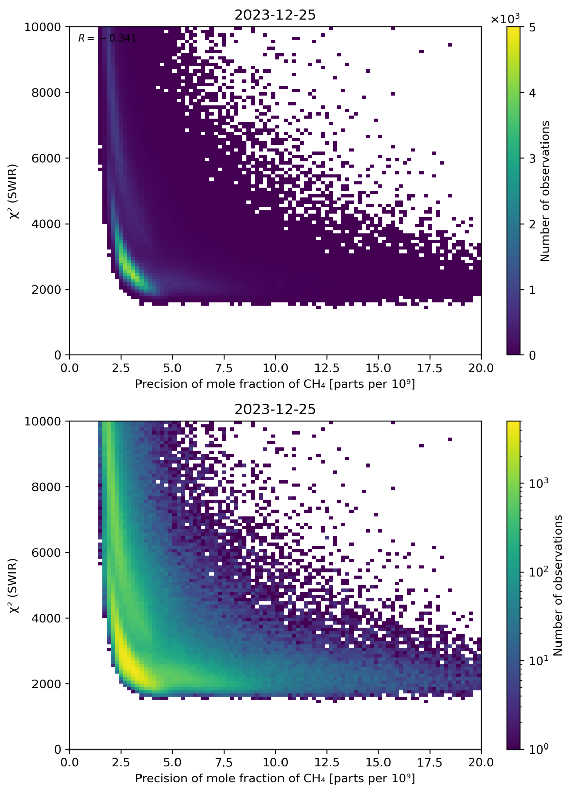
Figure 79: Scatter density plot of “Precision of mole fraction of \text{CH}_4 ” against “ \chi^2 (SWIR)” for 2023-12-25 to 2023-12-26.
