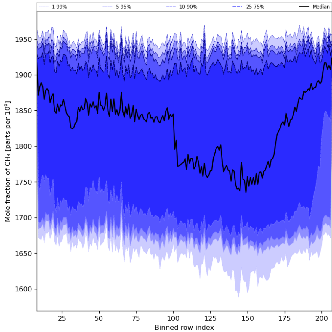
Figure 34: Along track statistics of “Mole fraction of CH 4 ” for 2023-12-25 to 2023-12-26
