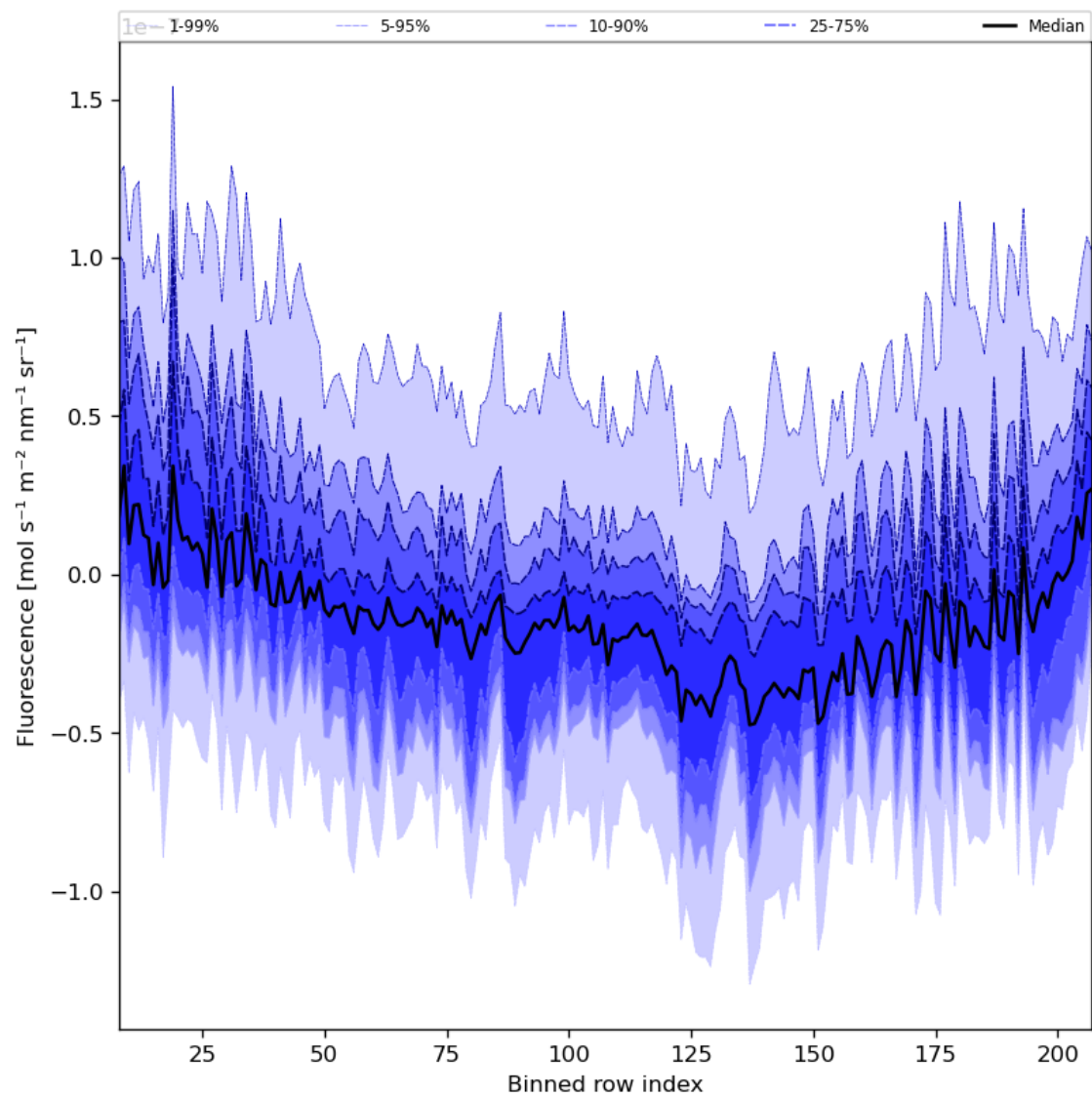
Figure 43: Along track statistics of “Fluorescence” for 2023-12-25 to 2023-12-26
