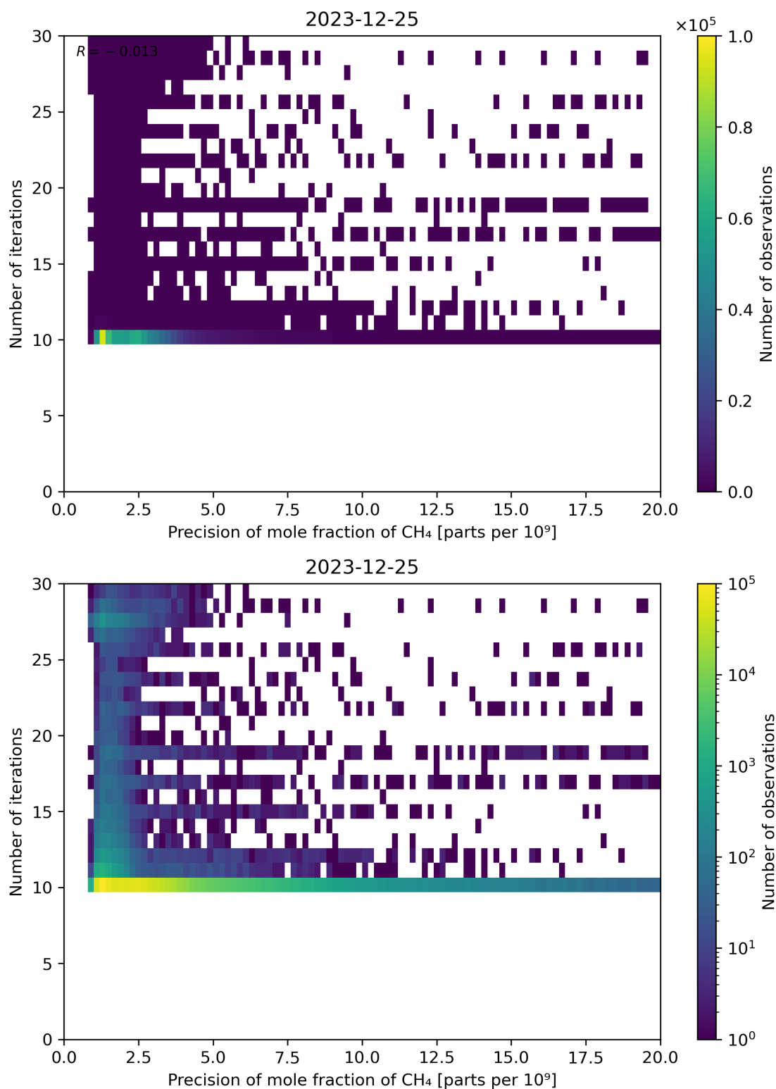
Figure 83: Scatter density plot of “Precision of mole fraction of CH 4 ” against “Number of iterations” for 2023-12-25 to 2023-12-26.
