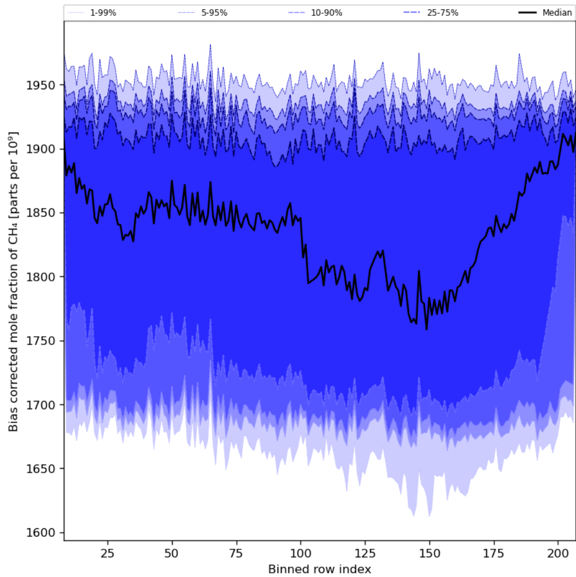
Figure 36: Along track statistics of “Bias corrected mole fraction of CH 4 ” for 2023-12-25 to 2023-12-26
