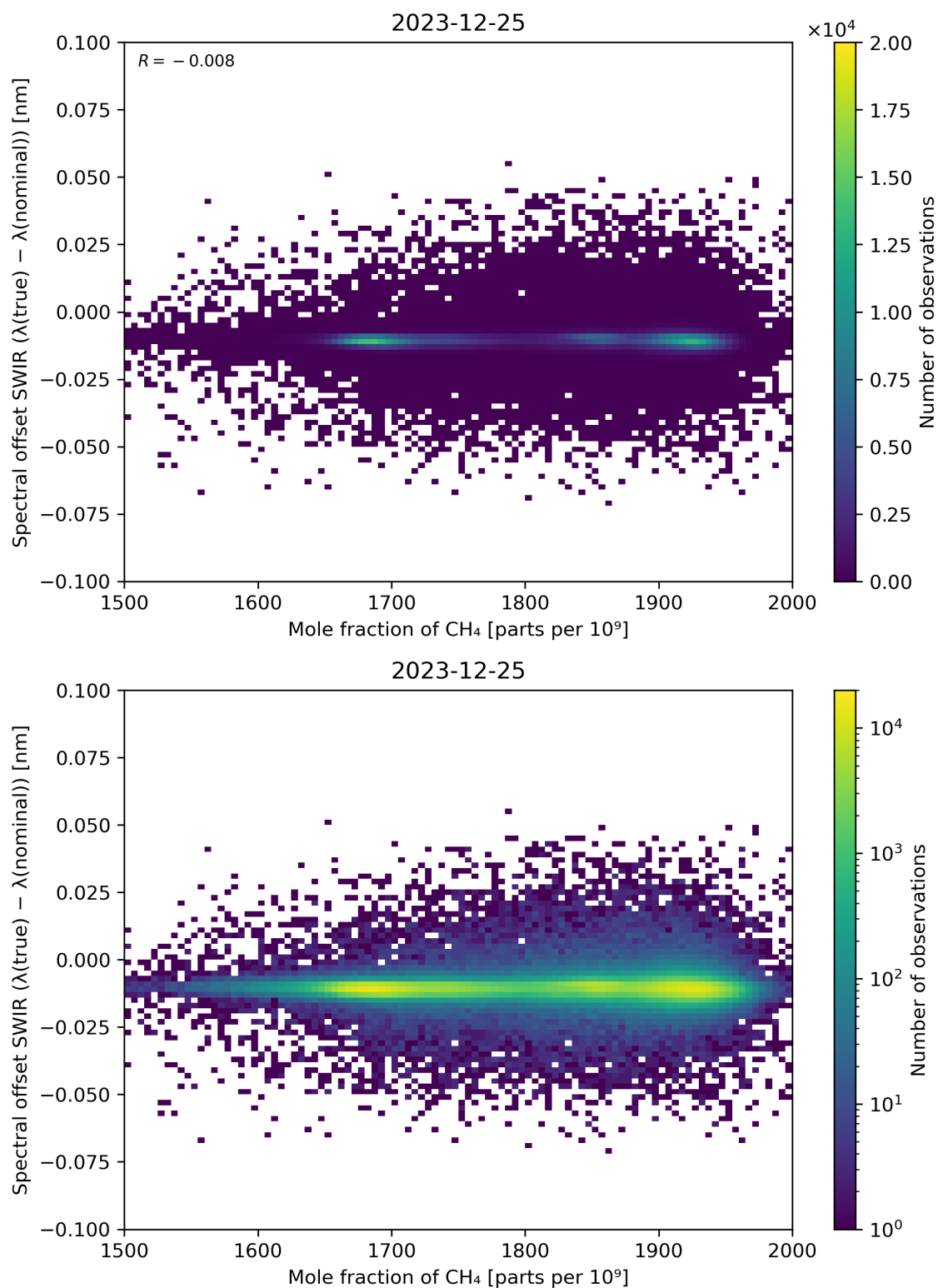
Figure 86: Scatter density plot of “Mole fraction of CH 4 ” against “Spectral offset SWIR ( \lambda(\text{true}) - \lambda(\text{nominal}) )” for 2023-12-25 to 2023-12-26.
