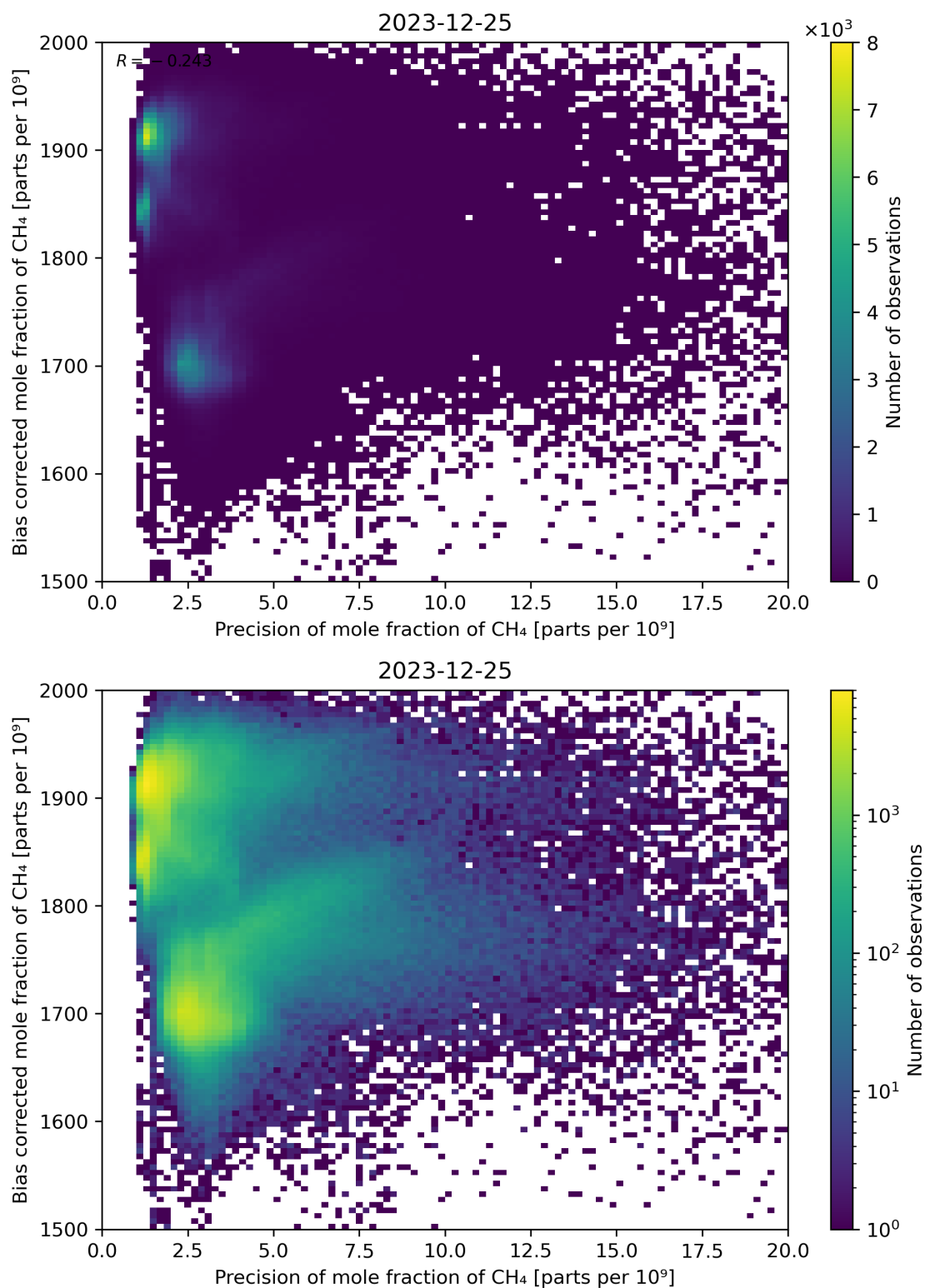
Figure 82: Scatter density plot of “Precision of mole fraction of CH 4 ” against “Bias corrected mole fraction of CH 4 ” for 2023-12-25 to 2023-12-26.
