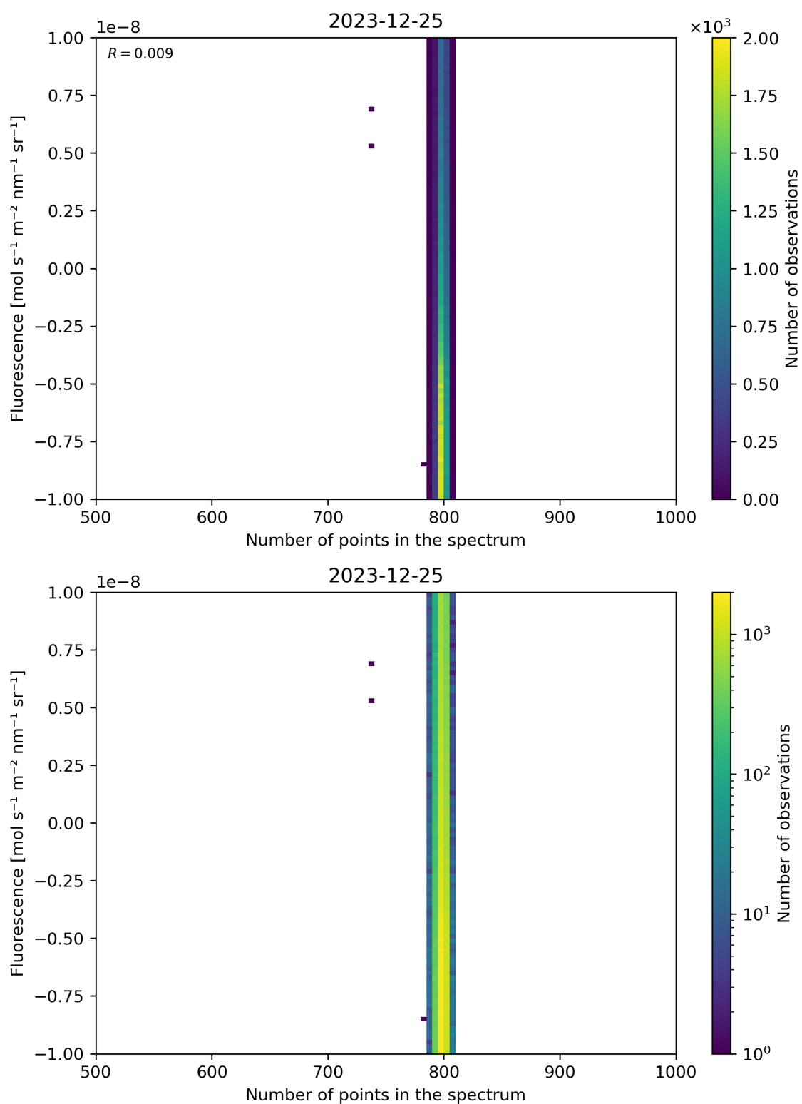
Figure 91: Scatter density plot of “Number of points in the spectrum” against “Fluorescence” for 2023-12-25 to 2023-12-26.
