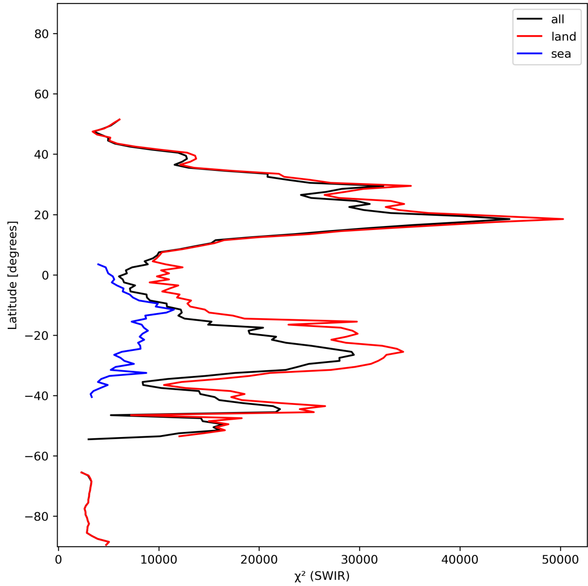
Figure 17: Zonal average of “ \chi^2 (SWIR)” for 2023-12-25 to 2023-12-26.
