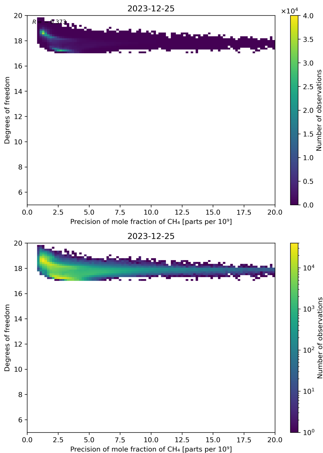
Figure 80: Scatter density plot of “Precision of mole fraction of CH 4 ” against “Degrees of freedom” for 2023-12-25 to 2023-12-26.
