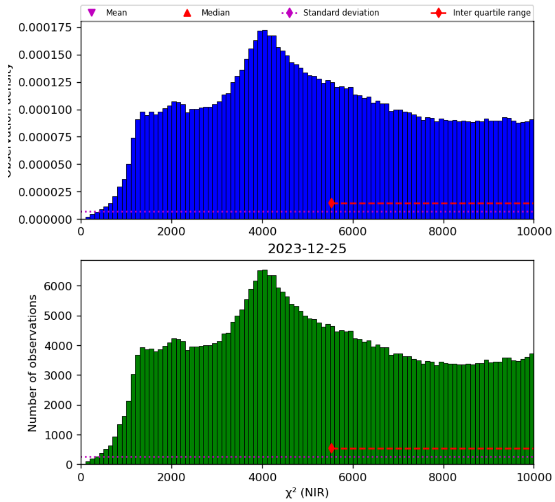
Figure 29: Histogram of “ \chi^2 (NIR)” for 2023-12-25 to 2023-12-26
