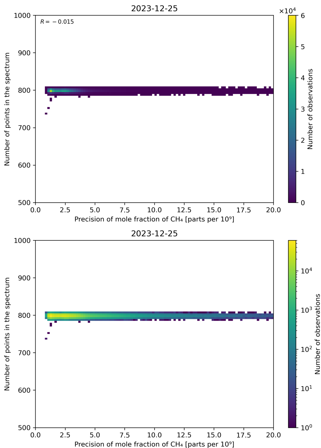
Figure 84: Scatter density plot of “Precision of mole fraction of CH 4 ” against “Number of points in the spectrum” for 2023-12-25 to 2023-12-26.
