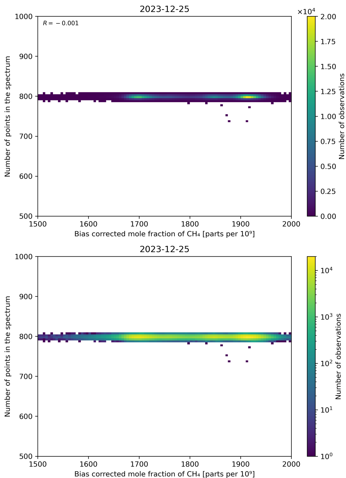
Figure 68: Scatter density plot of “Bias corrected mole fraction of CH 4 ” against “Number of points in the spectrum” for 2023-12-25 to 2023-12-26.
