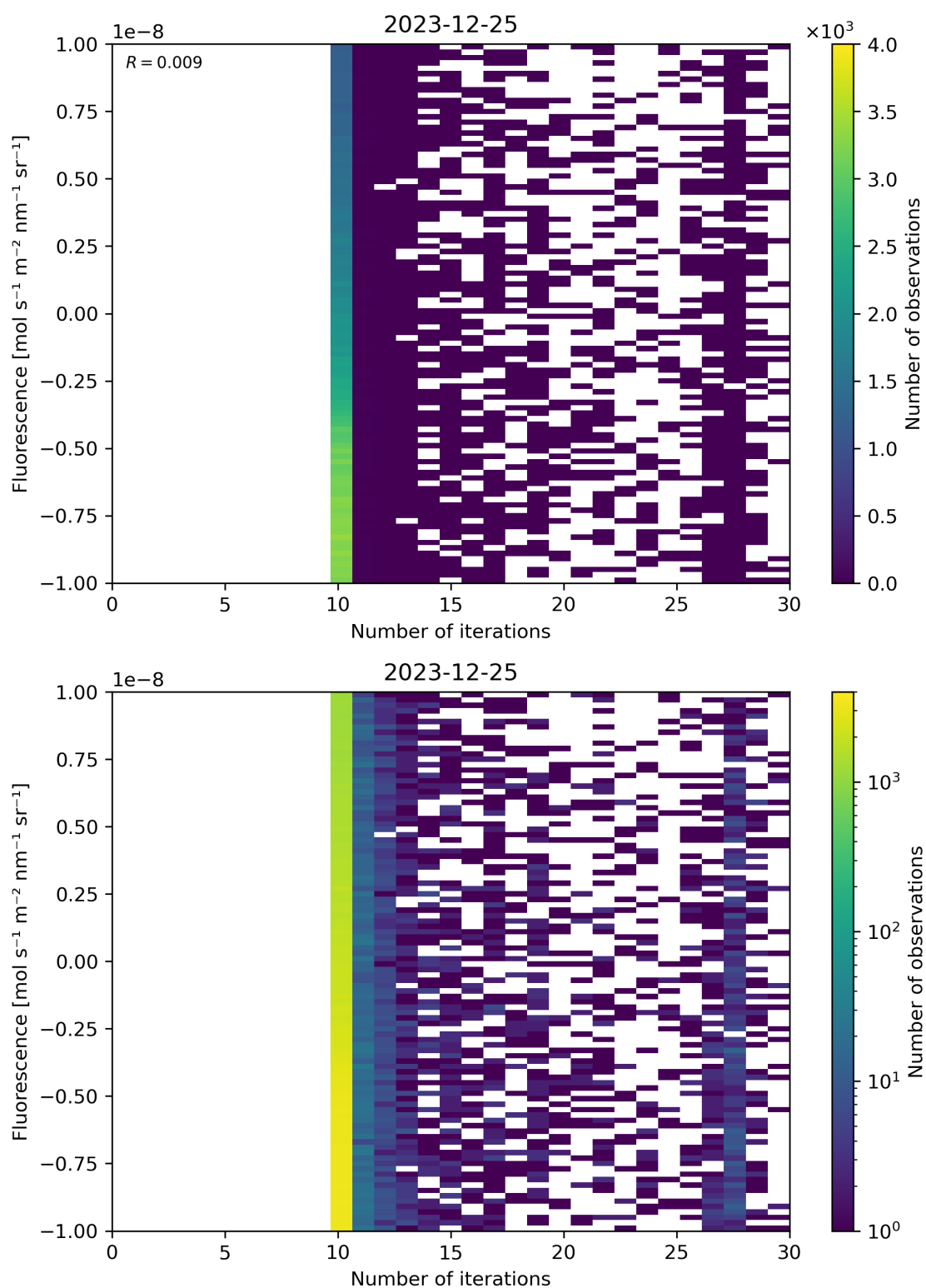
Figure 87: Scatter density plot of “Number of iterations” against “Fluorescence” for 2023-12-25 to 2023-12-26.
