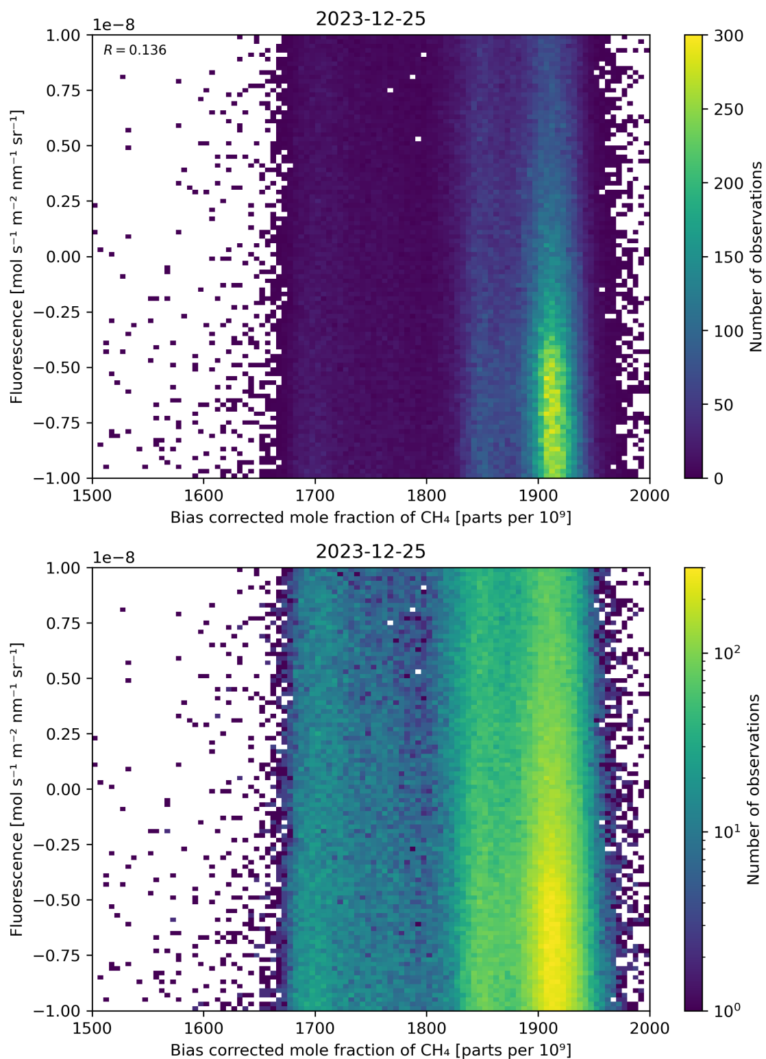
Figure 66: Scatter density plot of “Bias corrected mole fraction of \text{CH}_4 ” against “Fluorescence” for 2023-12-25 to 2023-12-26.
