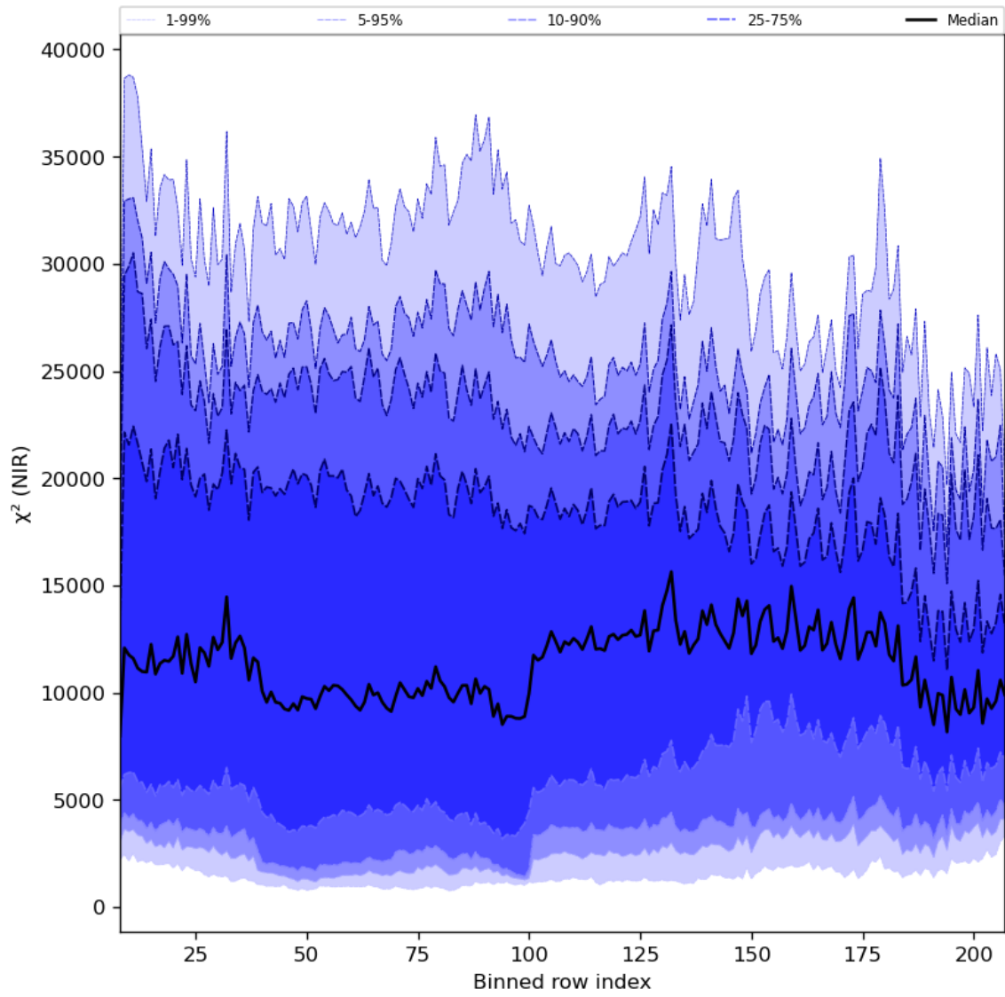
Figure 40: Along track statistics of “ \chi^2 (NIR)” for 2023-12-25 to 2023-12-26
