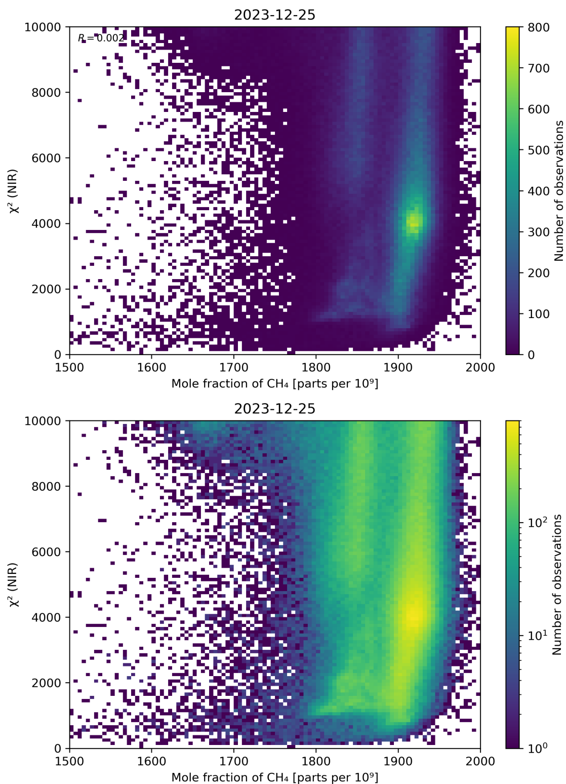
Figure 70: Scatter density plot of “Mole fraction of CH 4 ” against “ \chi^2 (NIR)” for 2023-12-25 to 2023-12-26.
