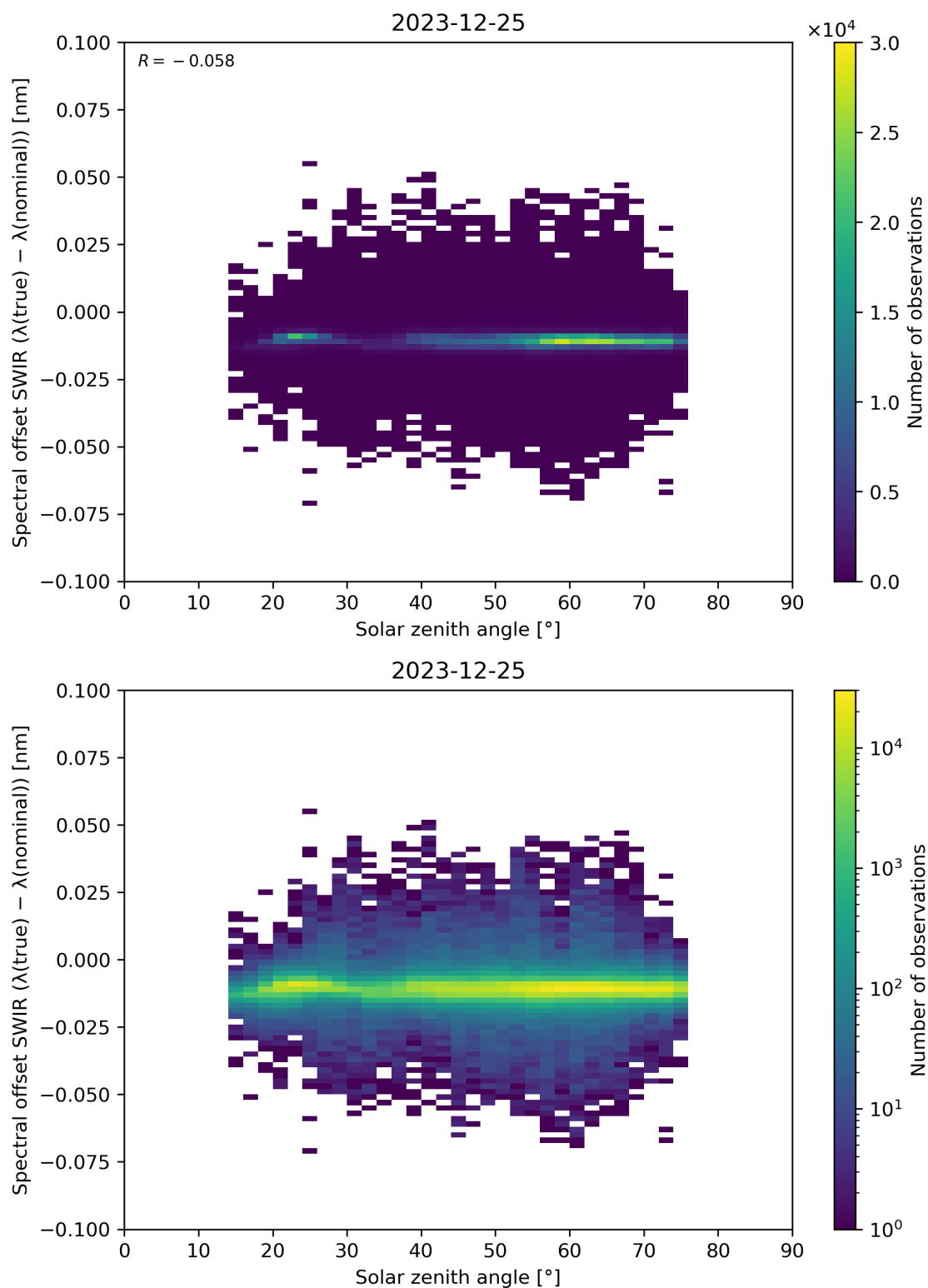
Figure 104: Scatter density plot of “Solar zenith angle” against “Spectral offset SWIR ( \lambda(\text{true}) - \lambda(\text{nominal}) )” for 2023-12-25 to 2023-12-26.
