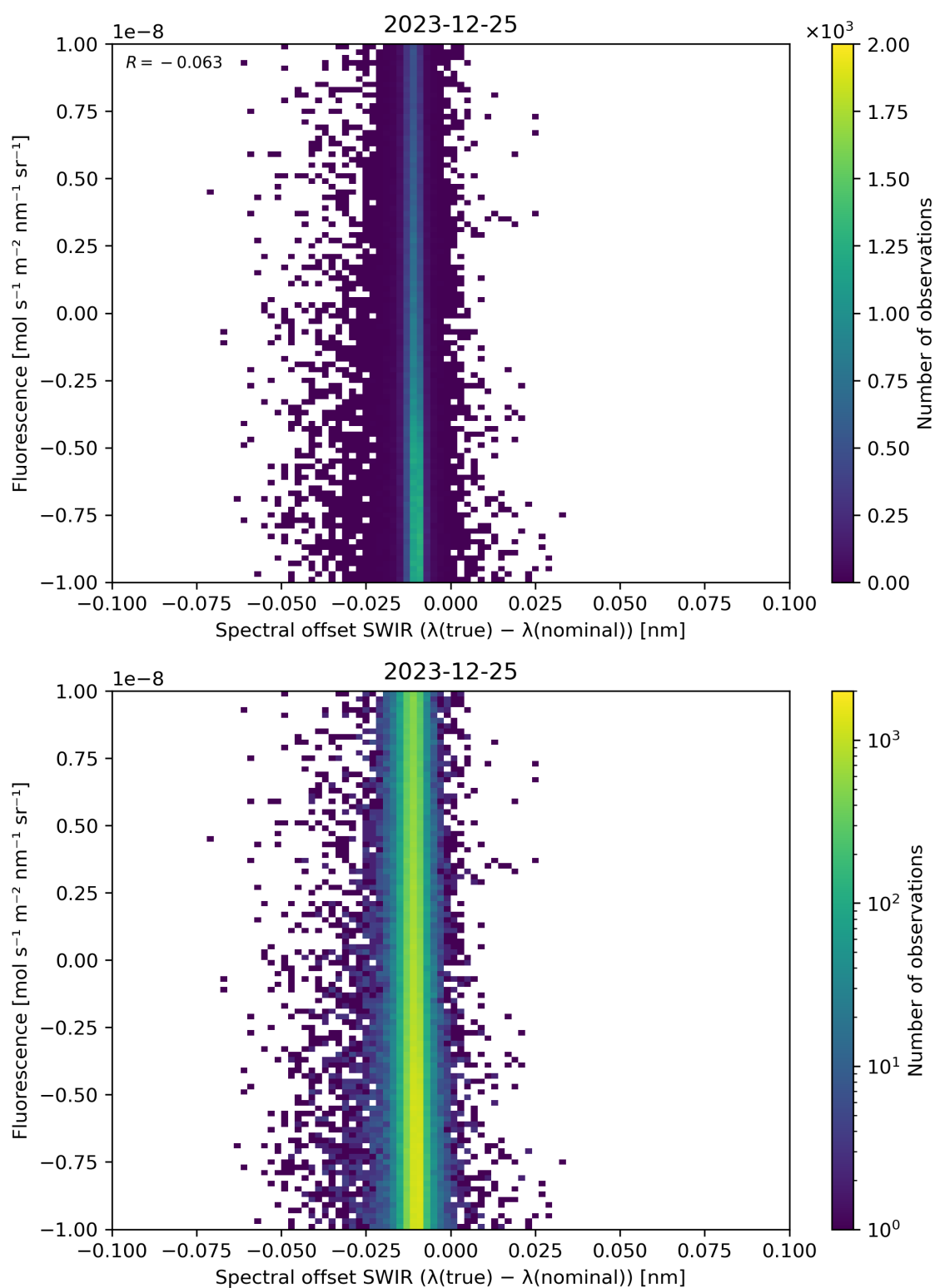
Figure 120: Scatter density plot of “Spectral offset SWIR ( \lambda(\text{true}) - \lambda(\text{nominal}) )” against “Fluorescence” for 2023-12-25 to 2023-12-26.
