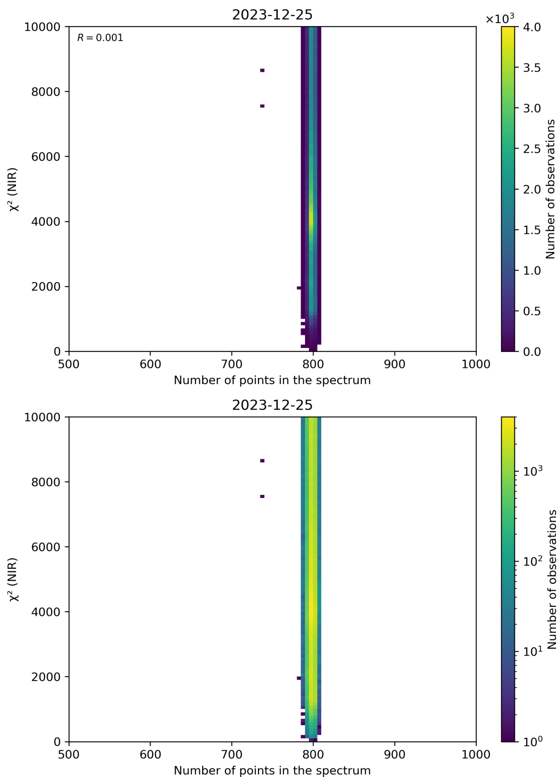
Figure 88: Scatter density plot of “Number of points in the spectrum” against “ \chi^2 (NIR)” for 2023-12-25 to 2023-12-26.
