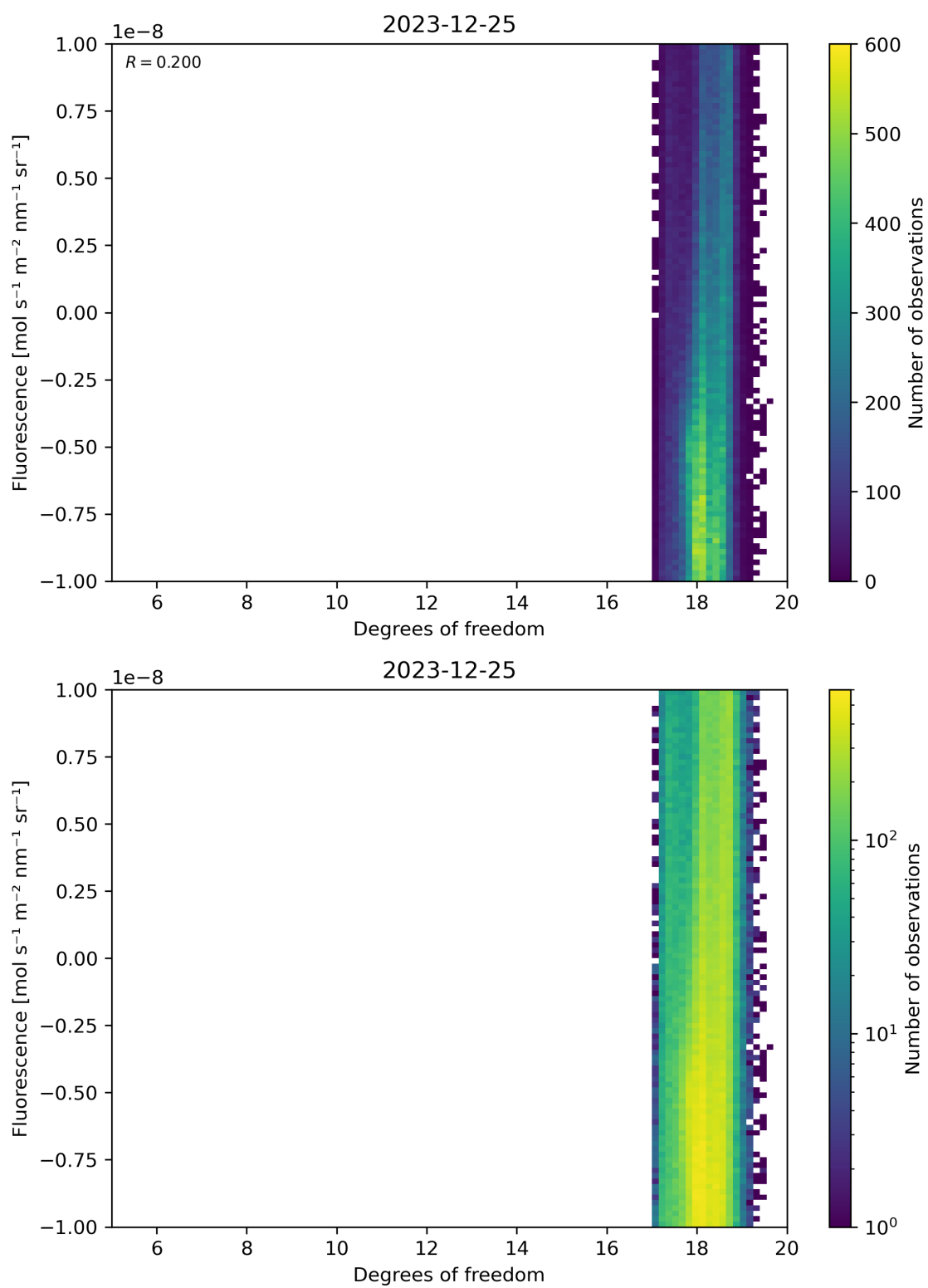
Figure 51: Scatter density plot of “Degrees of freedom” against “Fluorescence” for 2023-12-25 to 2023-12-26.
