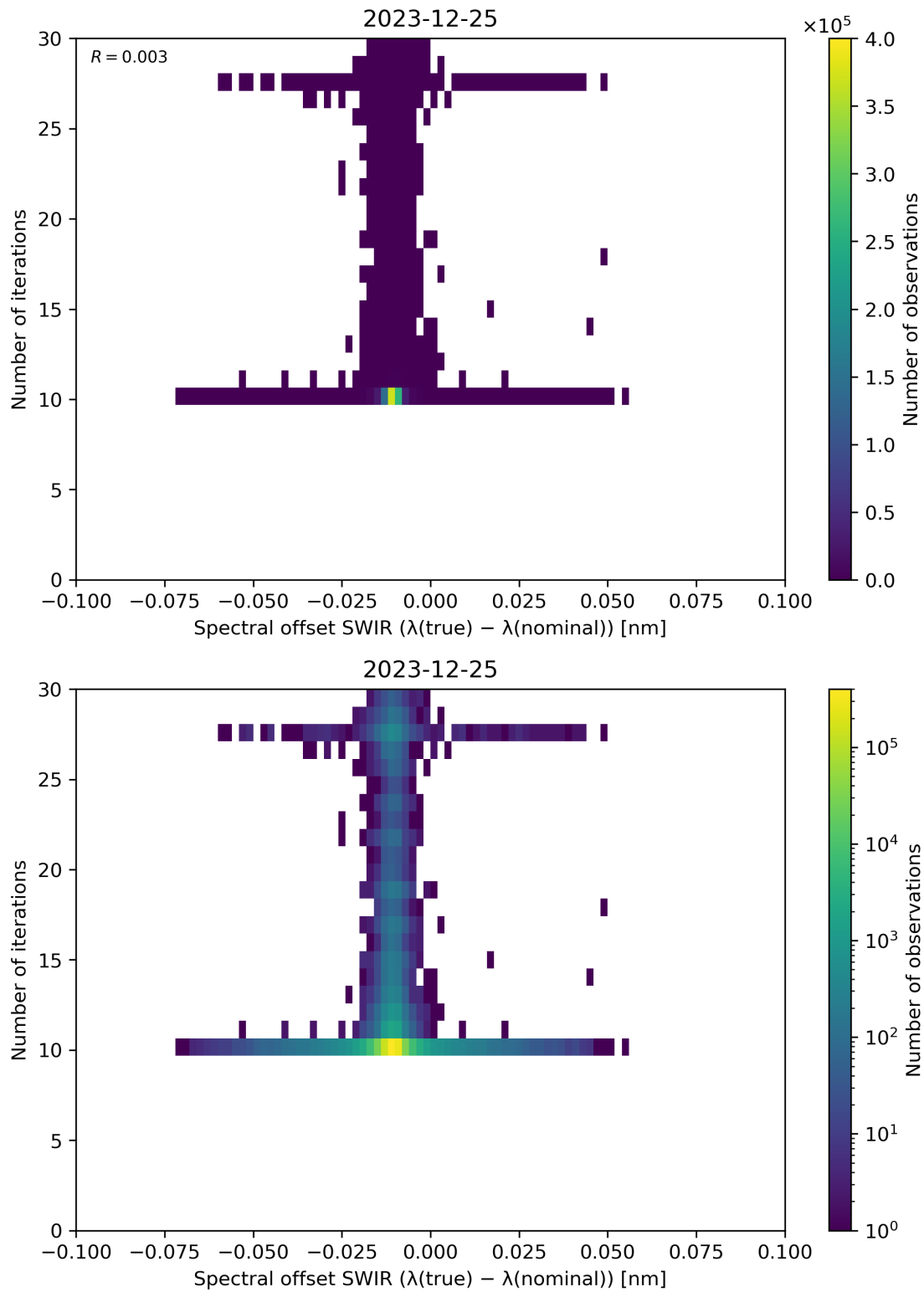
Figure 121: Scatter density plot of “Spectral offset SWIR ( \lambda(\text{true}) - \lambda(\text{nominal}) )” against “Number of iterations” for 2023-12-25 to 2023-12-26.
