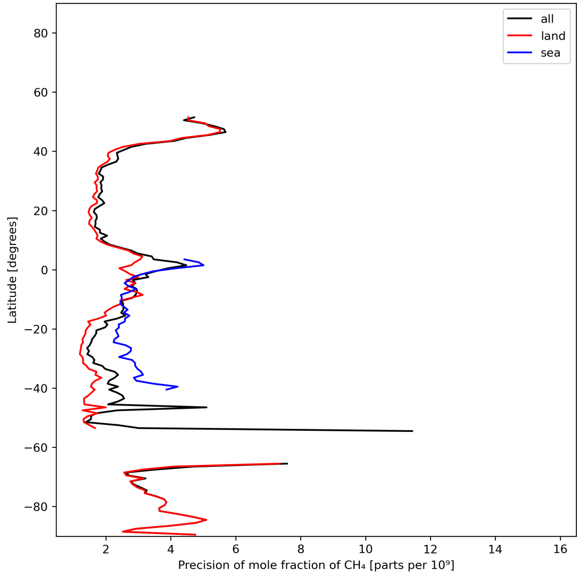
Figure 13: Zonal average of “Precision of mole fraction of \text{CH}_4 ” for 2023-12-25 to 2023-12-26.
