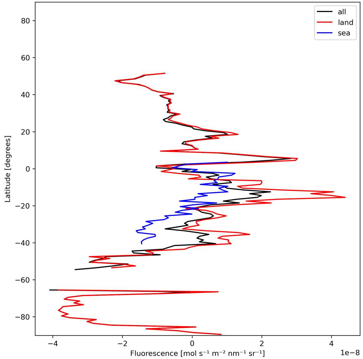
Figure 21: Zonal average of “Fluorescence” for 2023-12-25 to 2023-12-26.
