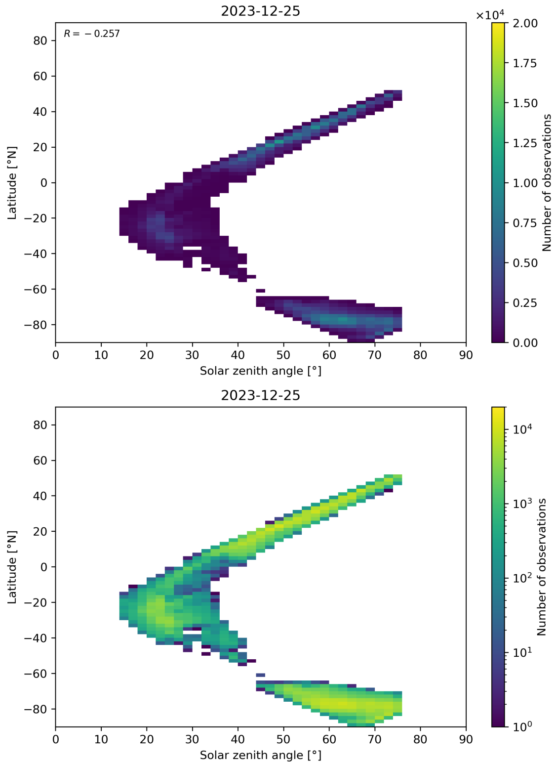
Figure 98: Scatter density plot of “Solar zenith angle” against “Latitude” for 2023-12-25 to 2023-12-26.
