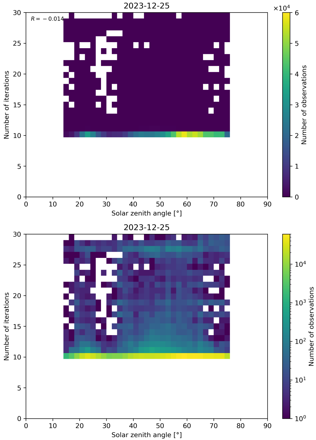
Figure 102: Scatter density plot of “Solar zenith angle” against “Number of iterations” for 2023-12-25 to 2023-12-26.
