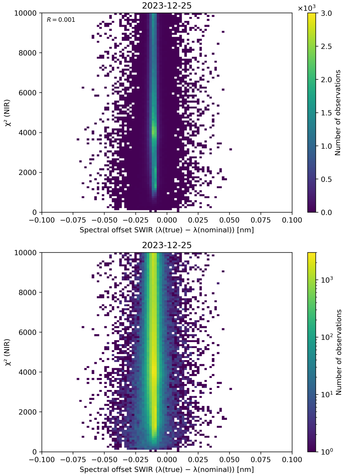
Figure 117: Scatter density plot of “Spectral offset SWIR ( \lambda(\text{true}) - \lambda(\text{nominal}) )” against “ \chi^2 (NIR)” for 2023-12-25 to 2023-12-26.
