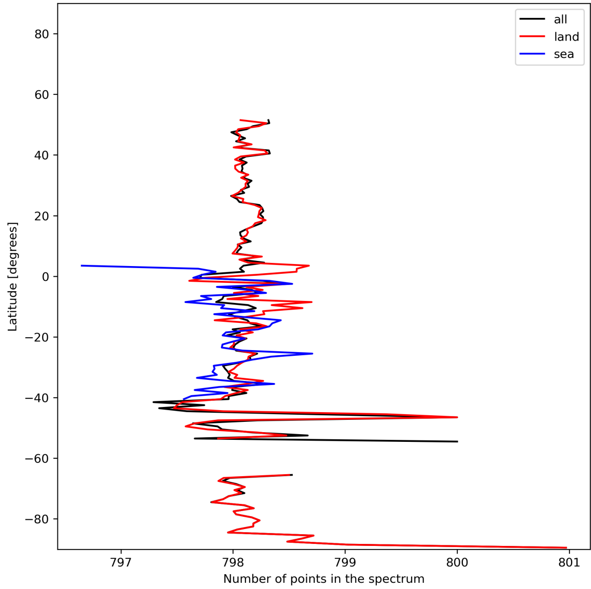
Figure 15: Zonal average of “Number of points in the spectrum” for 2023-12-25 to 2023-12-26.
