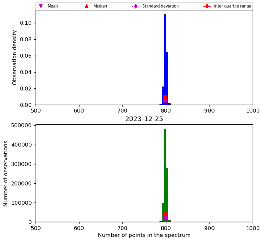
Figure 26: Histogram of “Number of points in the spectrum” for 2023-12-25 to 2023-12-26
