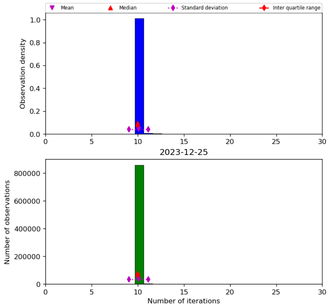
Figure 31: Histogram of “Number of iterations” for 2023-12-25 to 2023-12-26
