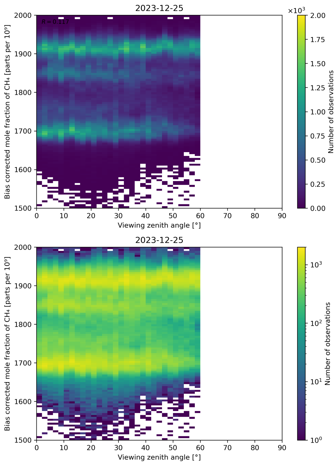
Figure 111: Scatter density plot of “Viewing zenith angle” against “Bias corrected mole fraction of CH 4 ” for 2023-12-25 to 2023-12-26.
