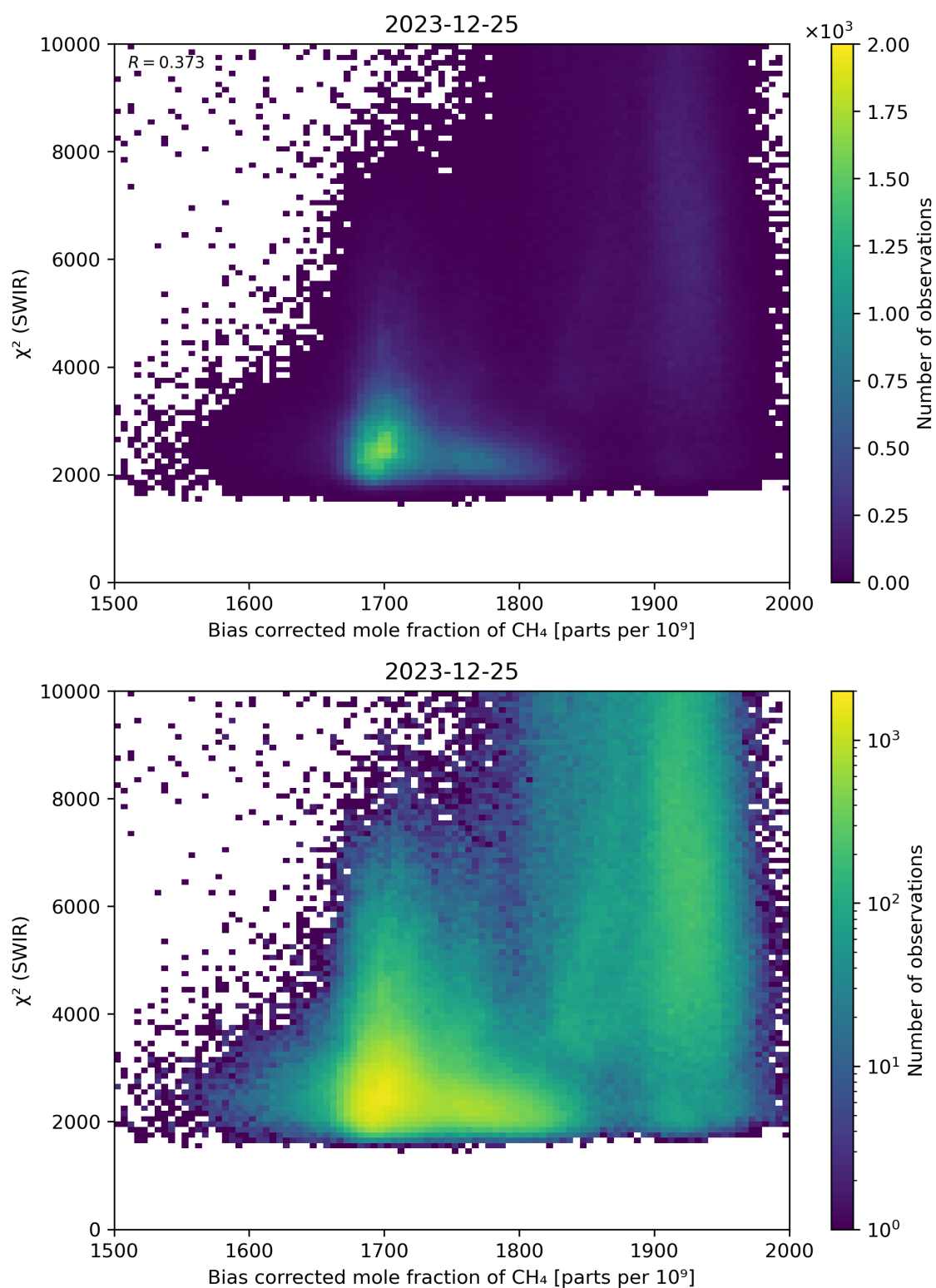
Figure 64: Scatter density plot of “Bias corrected mole fraction of \text{CH}_4 ” against “ \chi^2 (SWIR)” for 2023-12-25 to 2023-12-26.
