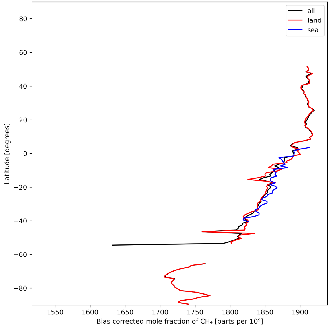
Figure 14: Zonal average of “Bias corrected mole fraction of CH 4 ” for 2023-12-25 to 2023-12-26.
