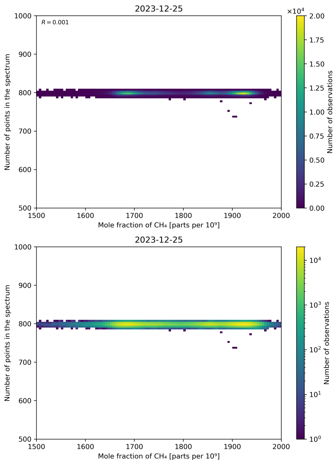
Figure 77: Scatter density plot of “Mole fraction of CH 4 ” against “Number of points in the spectrum” for 2023-12-25 to 2023-12-26.
