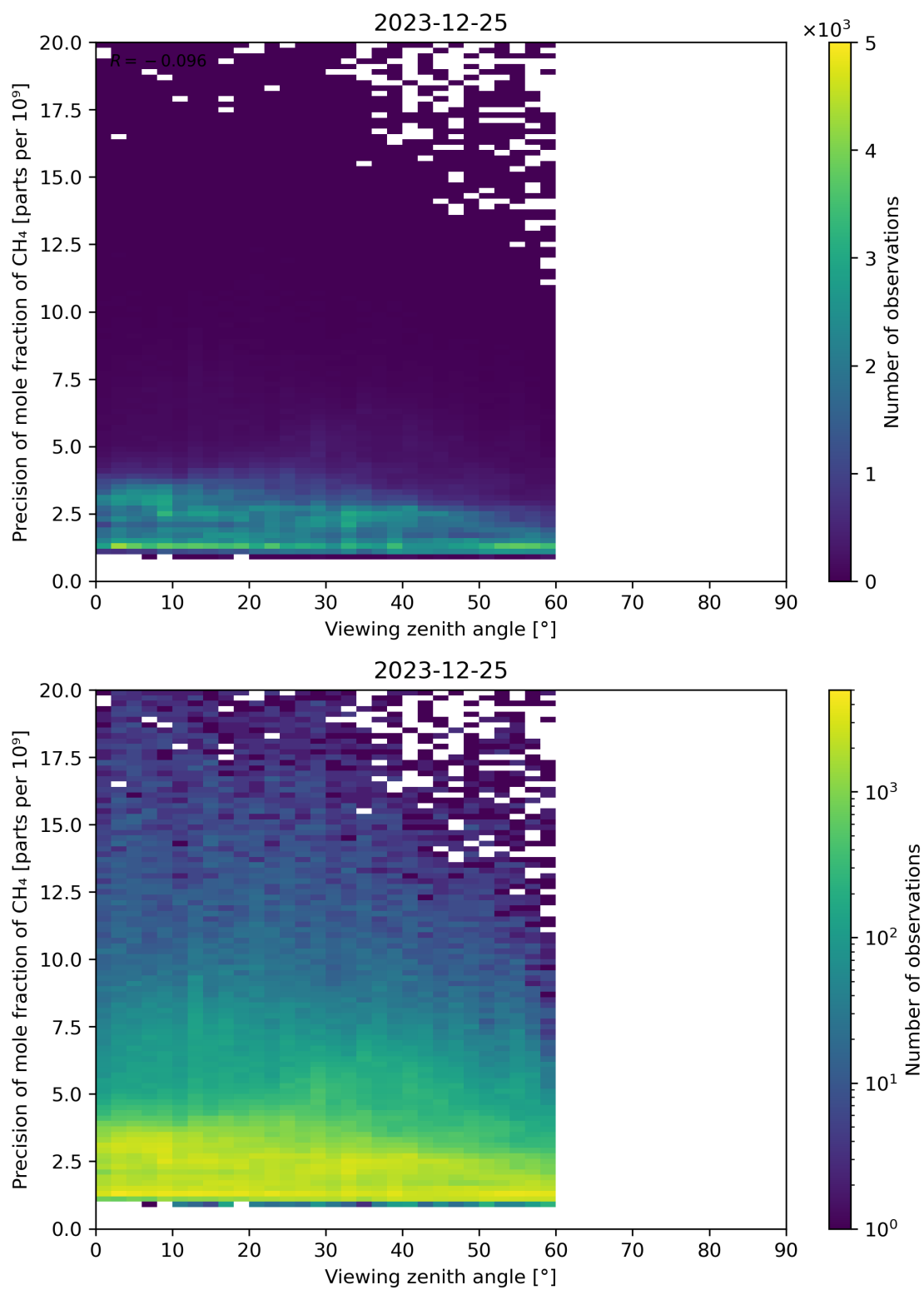
Figure 112: Scatter density plot of “Viewing zenith angle” against “Precision of mole fraction of CH 4 ” for 2023-12-25 to 2023-12-26.
