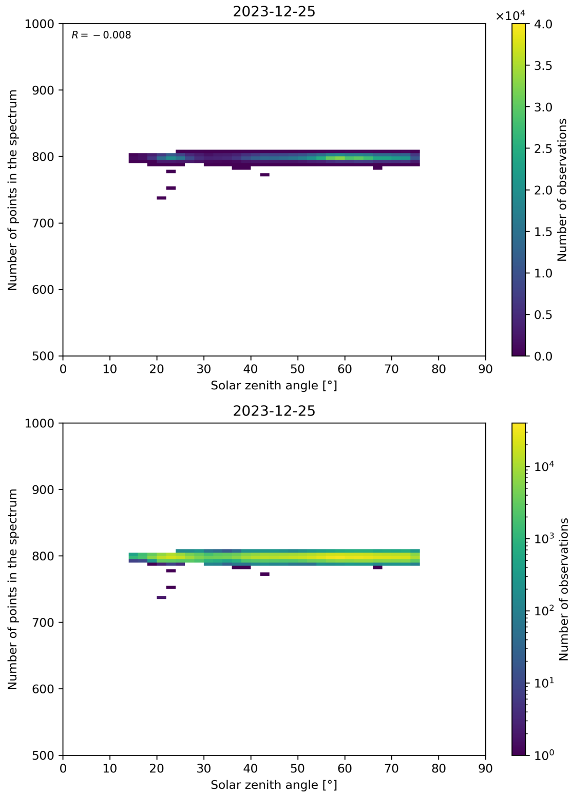
Figure 103: Scatter density plot of “Solar zenith angle” against “Number of points in the spectrum” for 2023-12-25 to 2023-12-26.
