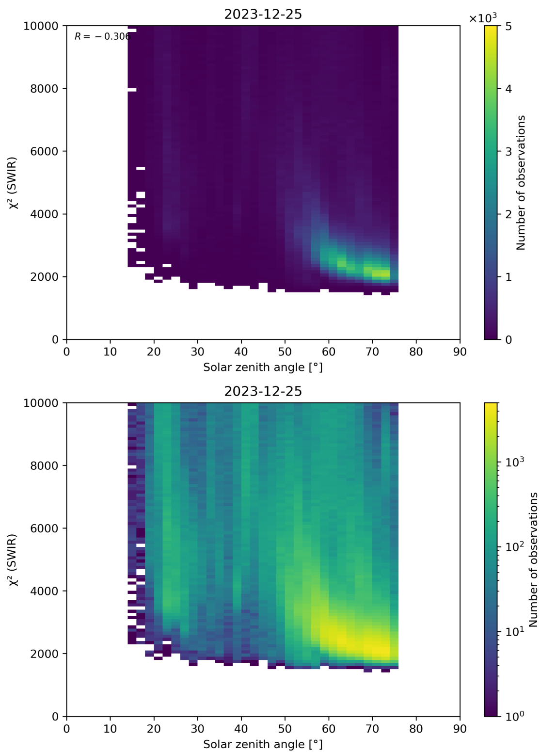
Figure 95: Scatter density plot of “Solar zenith angle” against “ \chi^2 (SWIR)” for 2023-12-25 to 2023-12-26.
