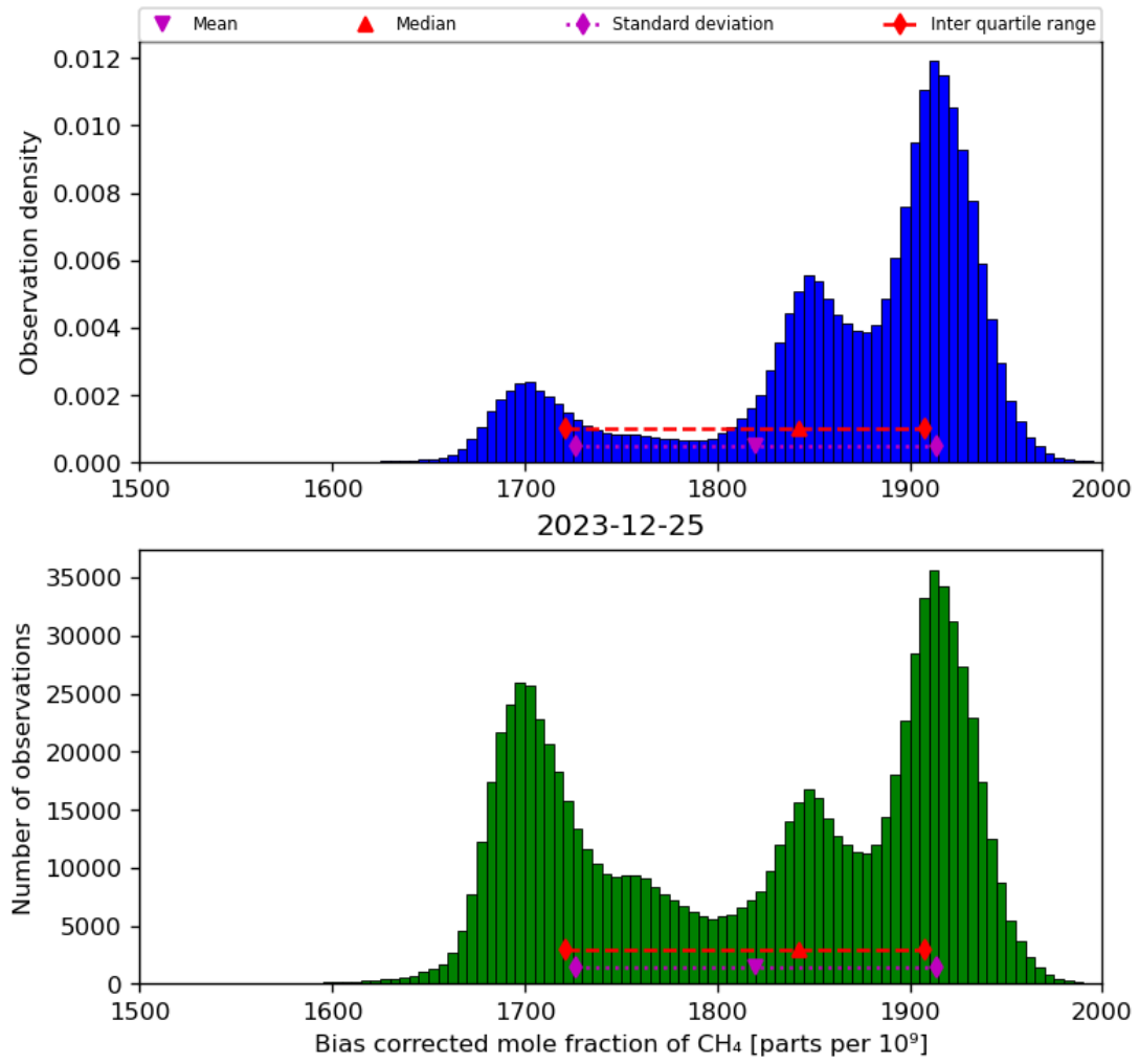
Figure 25: Histogram of “Bias corrected mole fraction of CH 4 ” for 2023-12-25 to 2023-12-26
