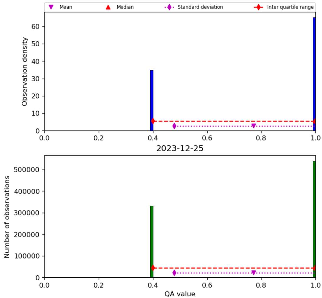
Figure 22: Histogram of “QA value” for 2023-12-25 to 2023-12-26
