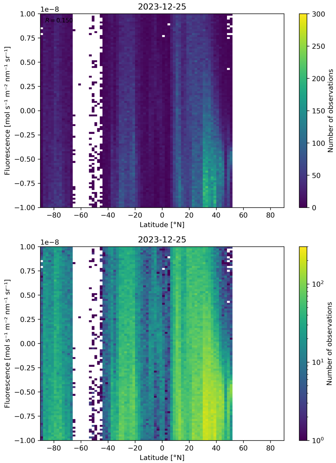
Figure 56: Scatter density plot of “Latitude” against “Fluorescence” for 2023-12-25 to 2023-12-26.
