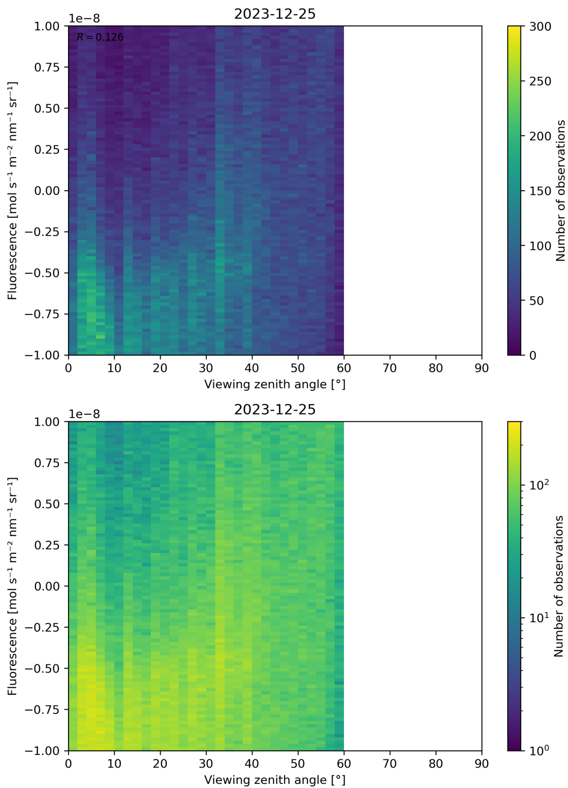
Figure 108: Scatter density plot of “Viewing zenith angle” against “Fluorescence” for 2023-12-25 to 2023-12-26.
