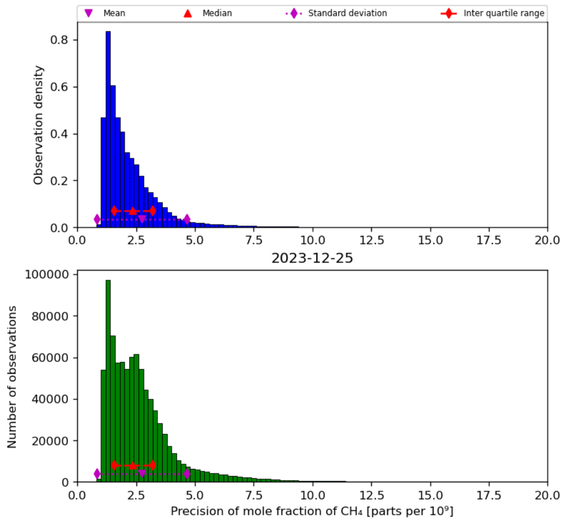
Figure 24: Histogram of “Precision of mole fraction of CH 4 ” for 2023-12-25 to 2023-12-26
