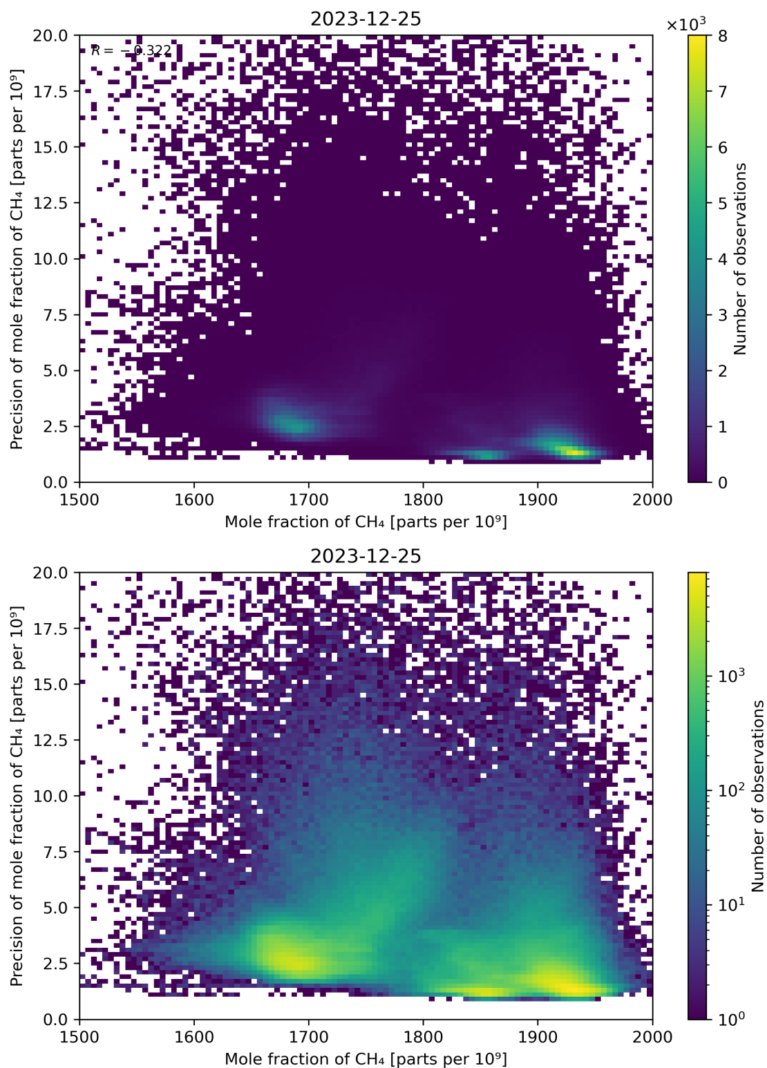
Figure 75: Scatter density plot of “Mole fraction of CH 4 ” against “Precision of mole fraction of CH 4 ” for 2023-12-25 to 2023-12-26.
