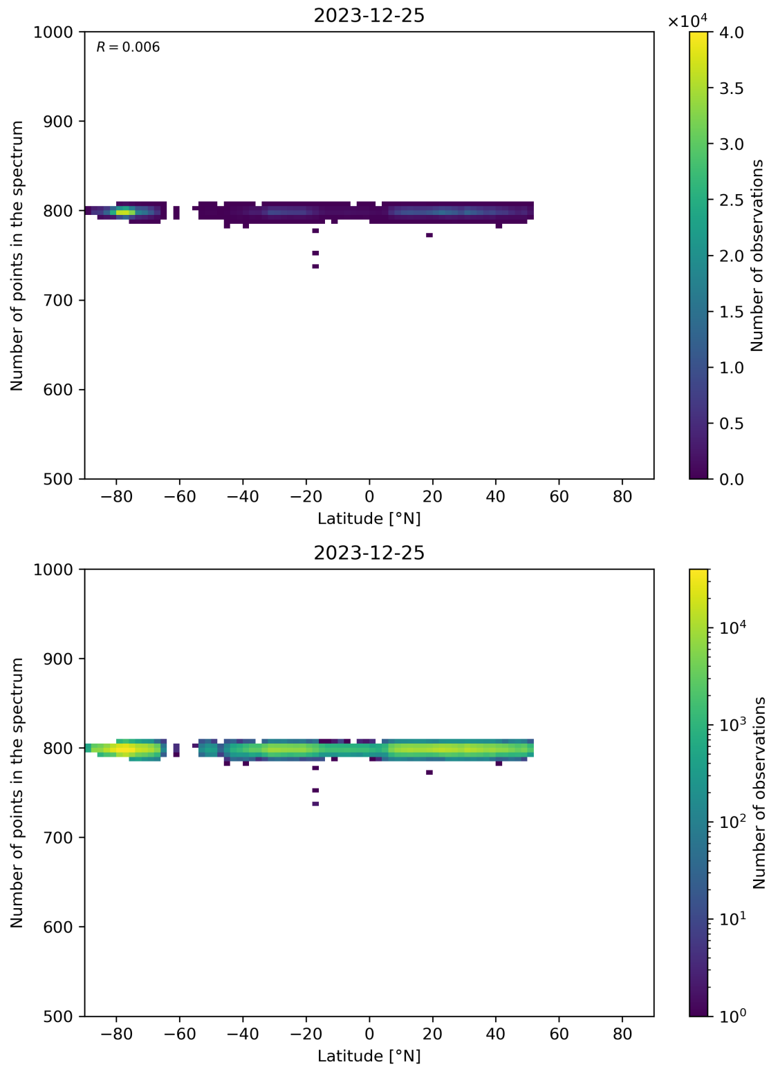
Figure 61: Scatter density plot of “Latitude” against “Number of points in the spectrum” for 2023-12-25 to 2023-12-26.
