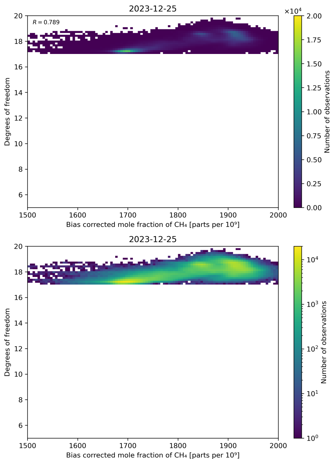
Figure 65: Scatter density plot of “Bias corrected mole fraction of CH 4 ” against “Degrees of freedom” for 2023-12-25 to 2023-12-26.
