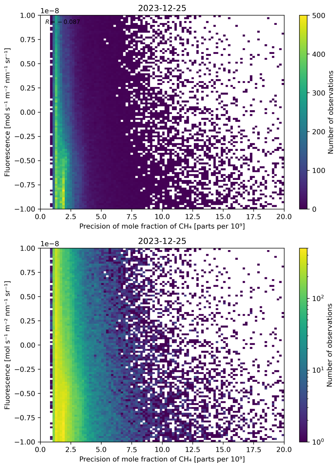
Figure 81: Scatter density plot of “Precision of mole fraction of CH 4 ” against “Fluorescence” for 2023-12-25 to 2023-12-26.
