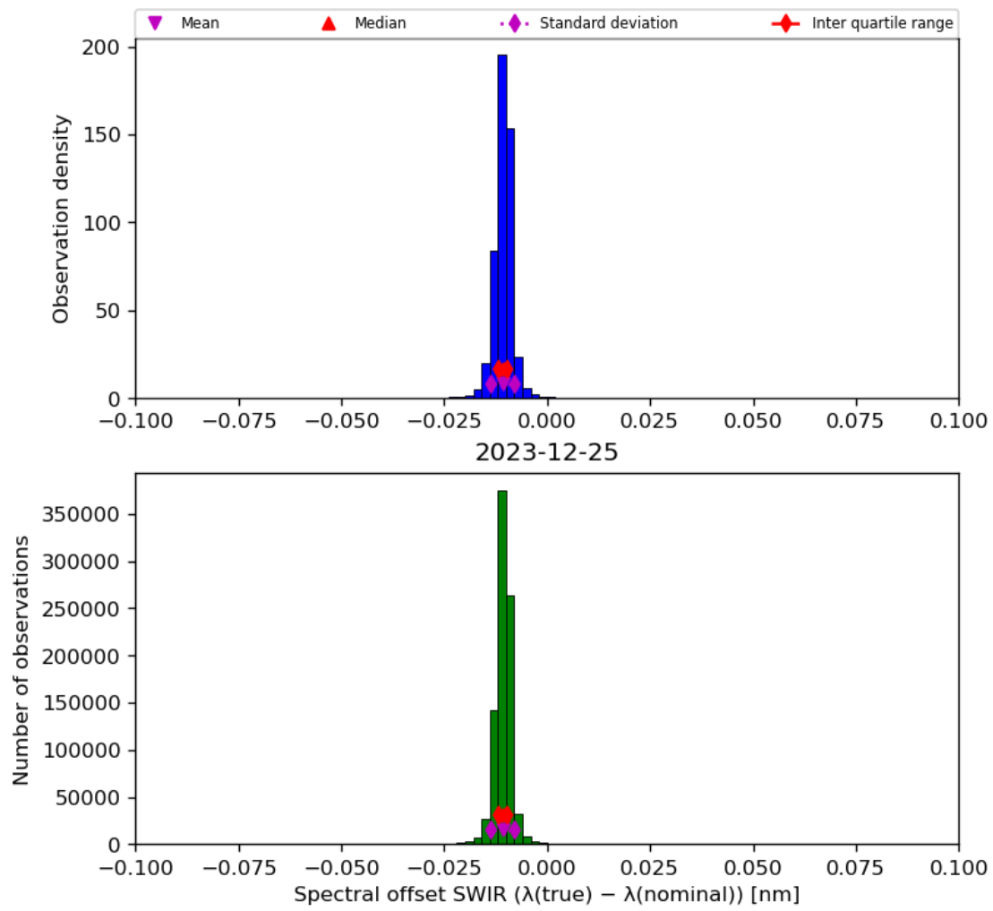
Figure 27: Histogram of “Spectral offset SWIR ( \lambda(\text{true}) - \lambda(\text{nominal}) )” for 2023-12-25 to 2023-12-26
