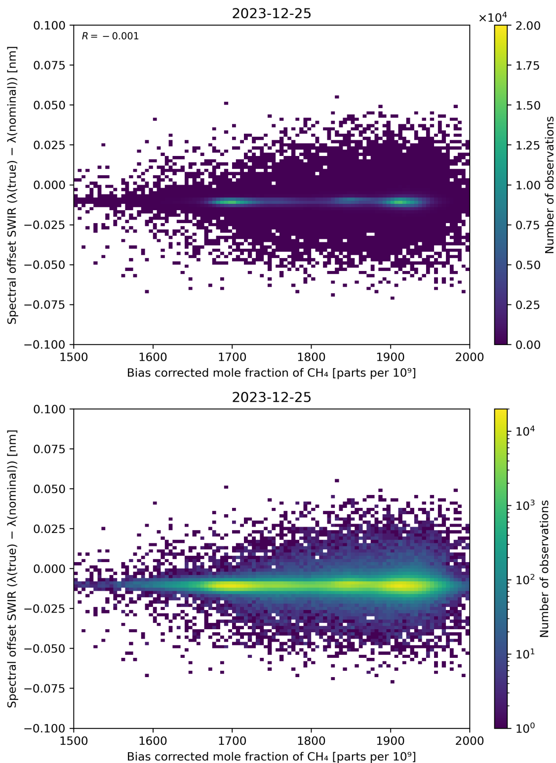
Figure 69: Scatter density plot of “Bias corrected mole fraction of \text{CH}_4 ” against “Spectral offset SWIR ( \lambda(\text{true}) - \lambda(\text{nominal}) )” for 2023-12-25 to 2023-12-26.
