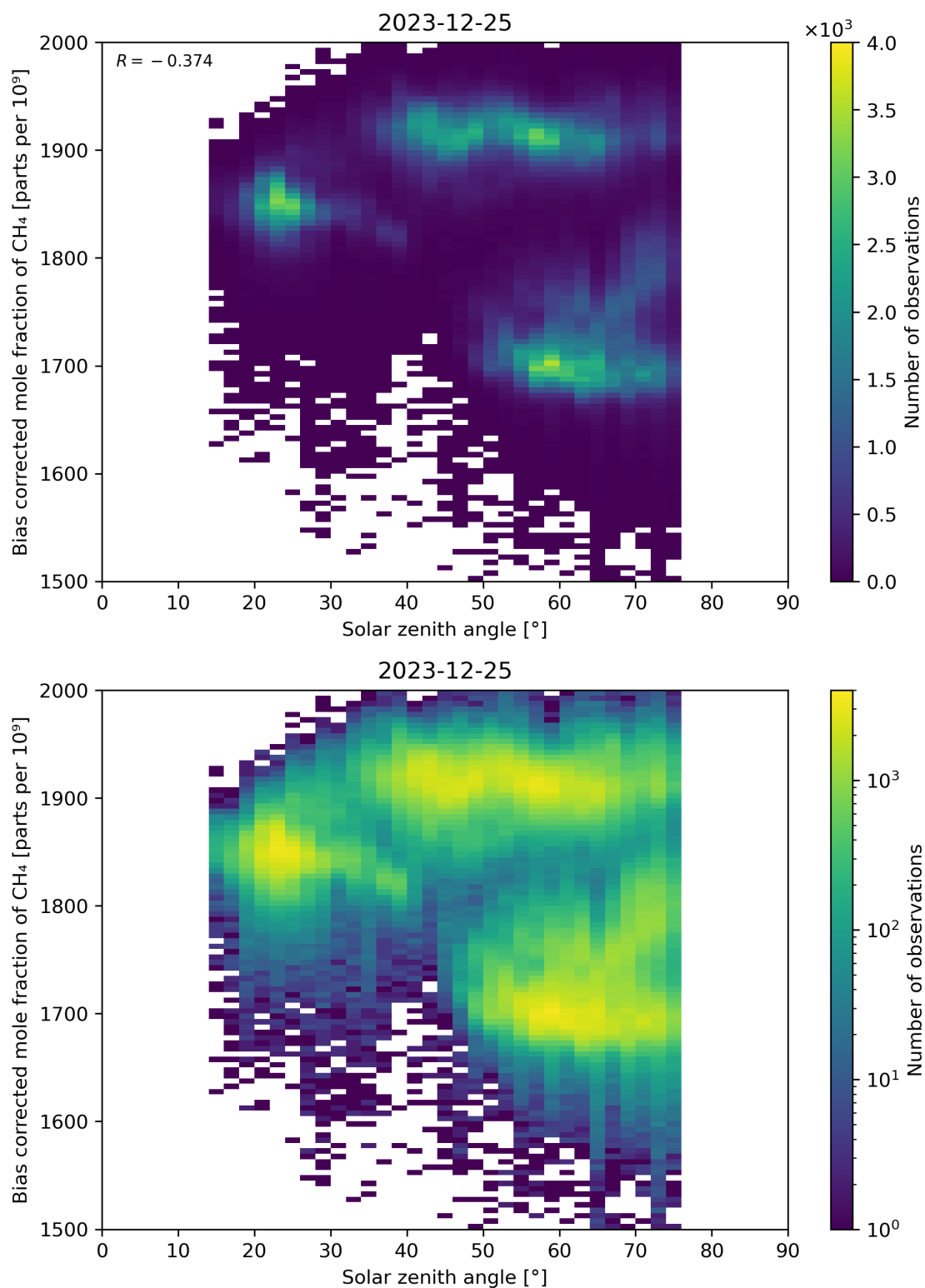
Figure 100: Scatter density plot of “Solar zenith angle” against “Bias corrected mole fraction of CH 4 ” for 2023-12-25 to 2023-12-26.
