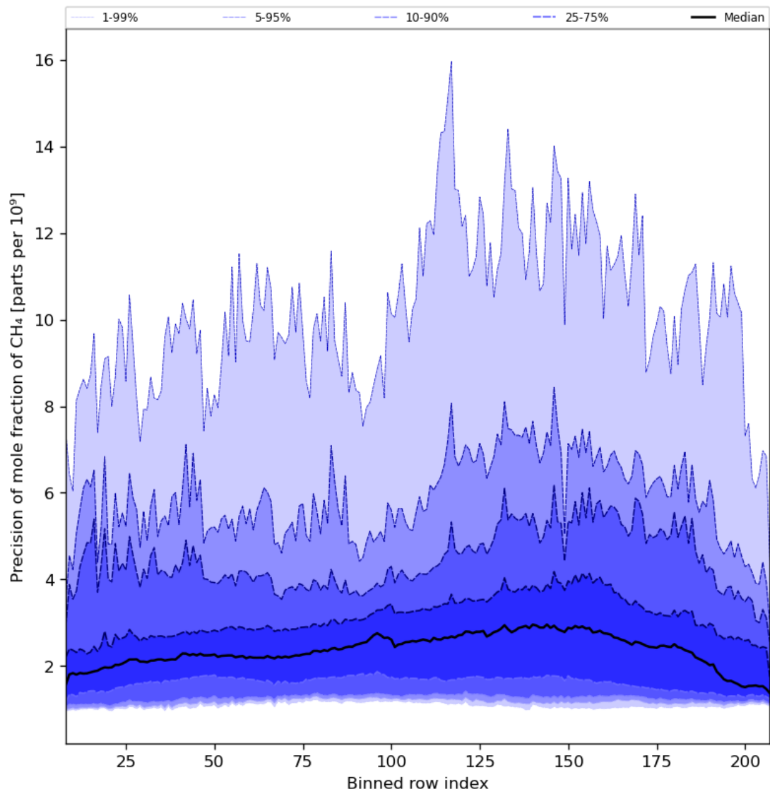
Figure 35: Along track statistics of "Precision of mole fraction of CH 4 " for 2023-12-25 to 2023-12-26
