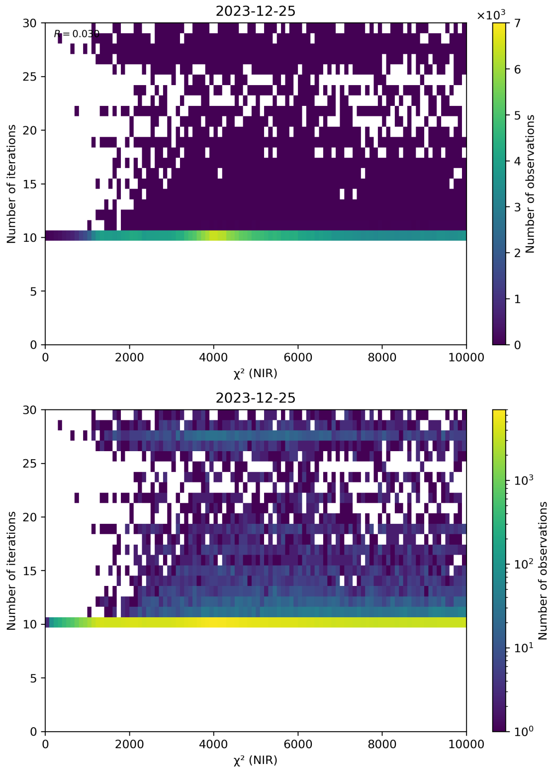
Figure 46: Scatter density plot of “ \chi^2 (NIR)” against “Number of iterations” for 2023-12-25 to 2023-12-26.
