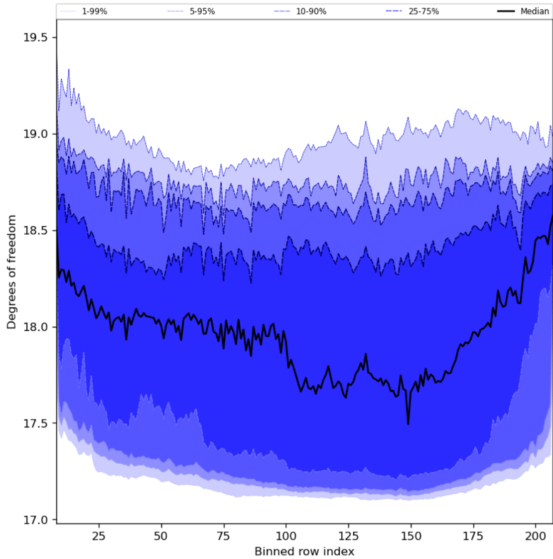
Figure 41: Along track statistics of “Degrees of freedom” for 2023-12-25 to 2023-12-26
