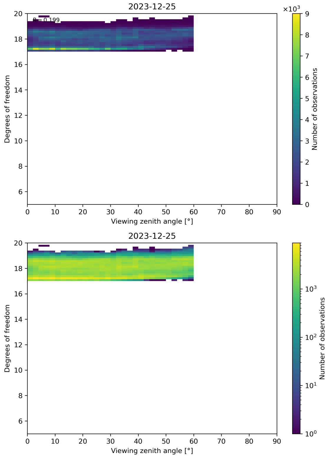
Figure 107: Scatter density plot of “Viewing zenith angle” against “Degrees of freedom” for 2023-12-25 to 2023-12-26.
