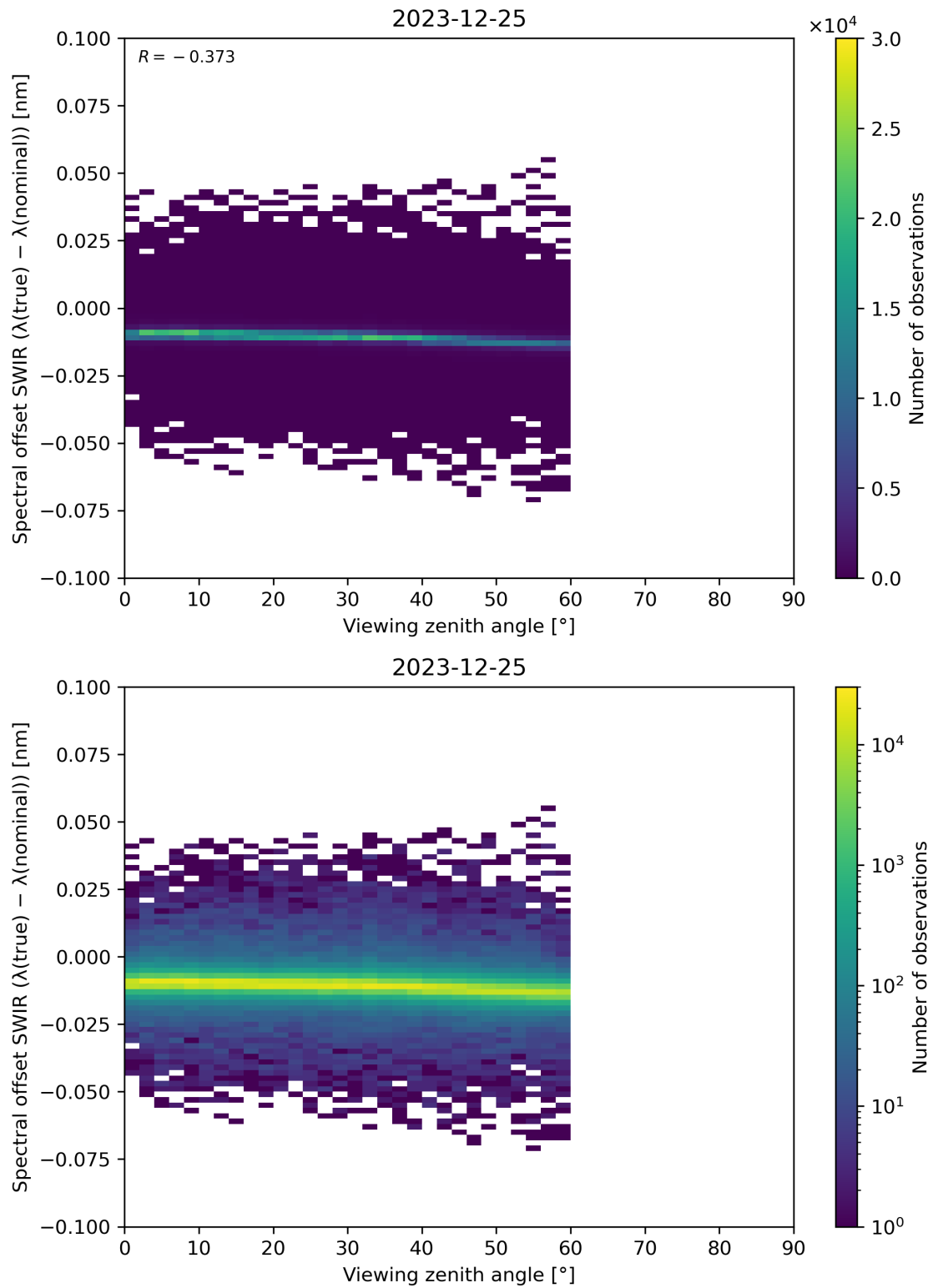
Figure 116: Scatter density plot of “Viewing zenith angle” against “Spectral offset SWIR ( \lambda(\text{true}) - \lambda(\text{nominal}) )” for 2023-12-25 to 2023-12-26.
