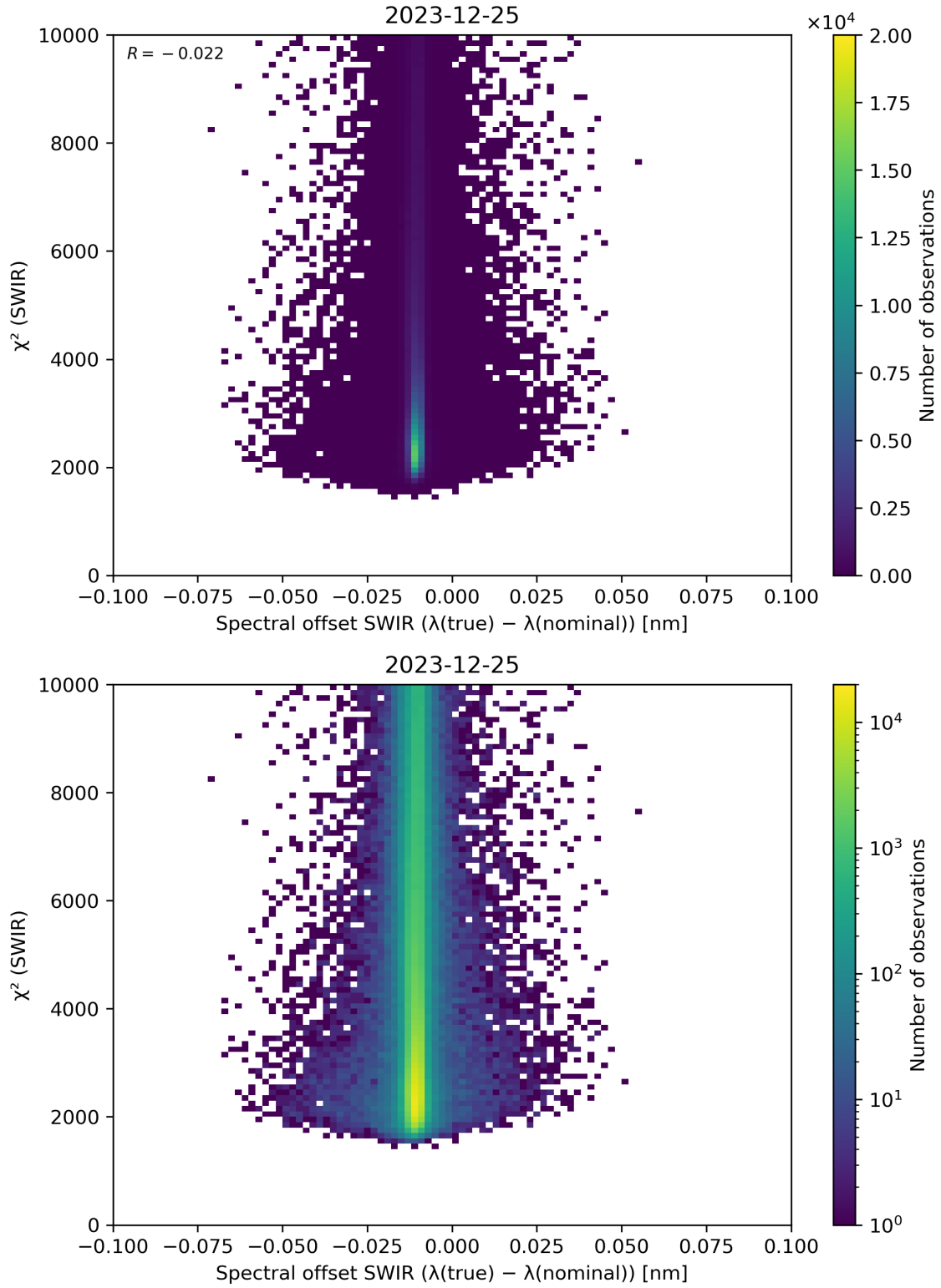
Figure 118: Scatter density plot of “Spectral offset SWIR ( \lambda(\text{true}) - \lambda(\text{nominal}) )” against “ \chi^2 (SWIR)” for 2023-12-25 to 2023-12-26.
