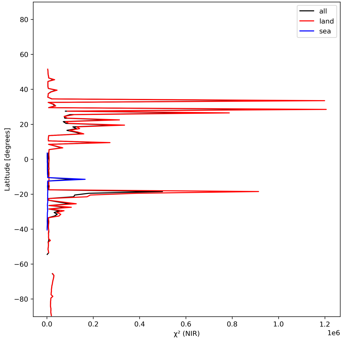
Figure 18: Zonal average of “ \chi^2 (NIR)” for 2023-12-25 to 2023-12-26.
