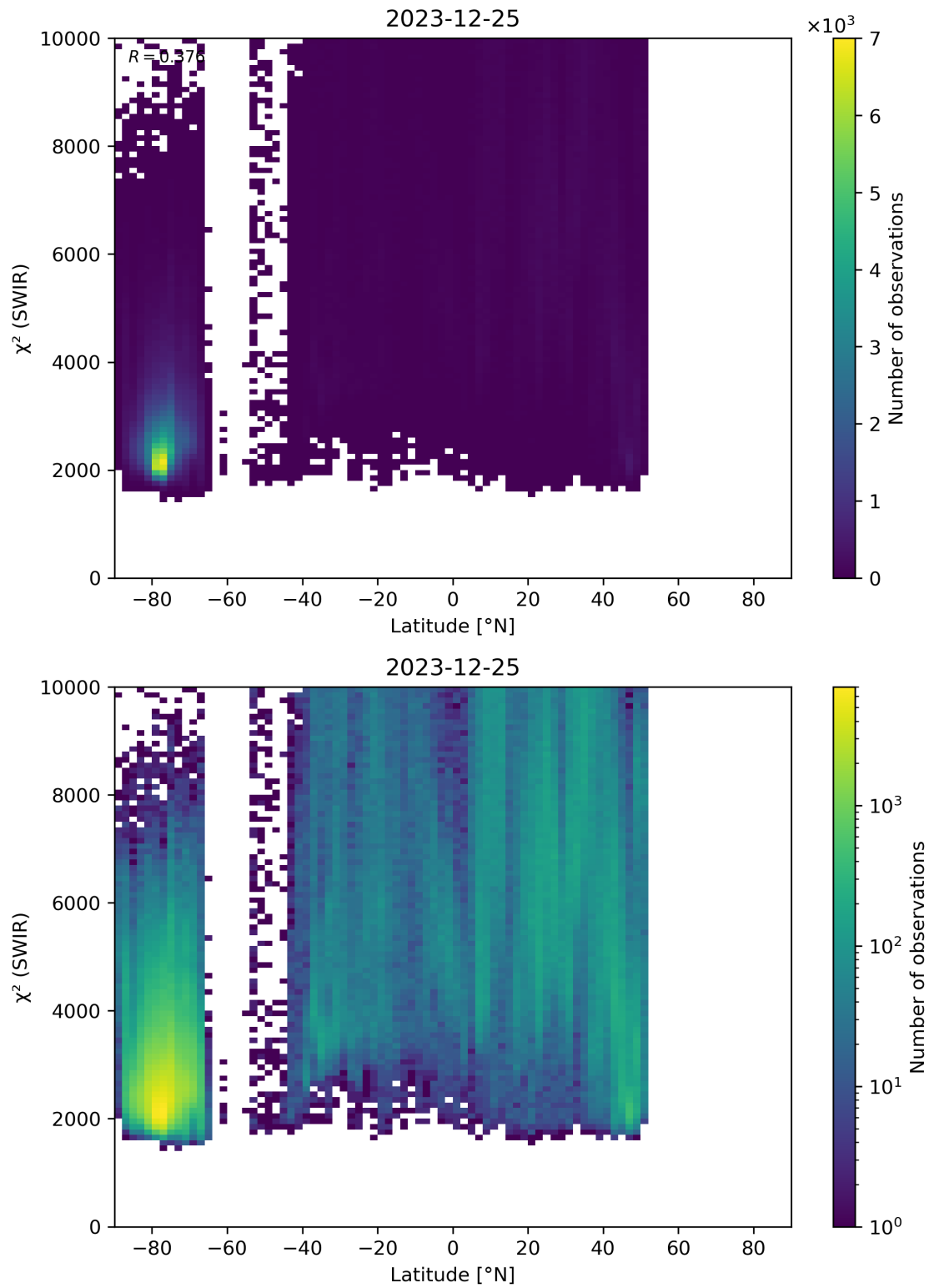
Figure 54: Scatter density plot of “Latitude” against “ \chi^2 (SWIR)” for 2023-12-25 to 2023-12-26.
