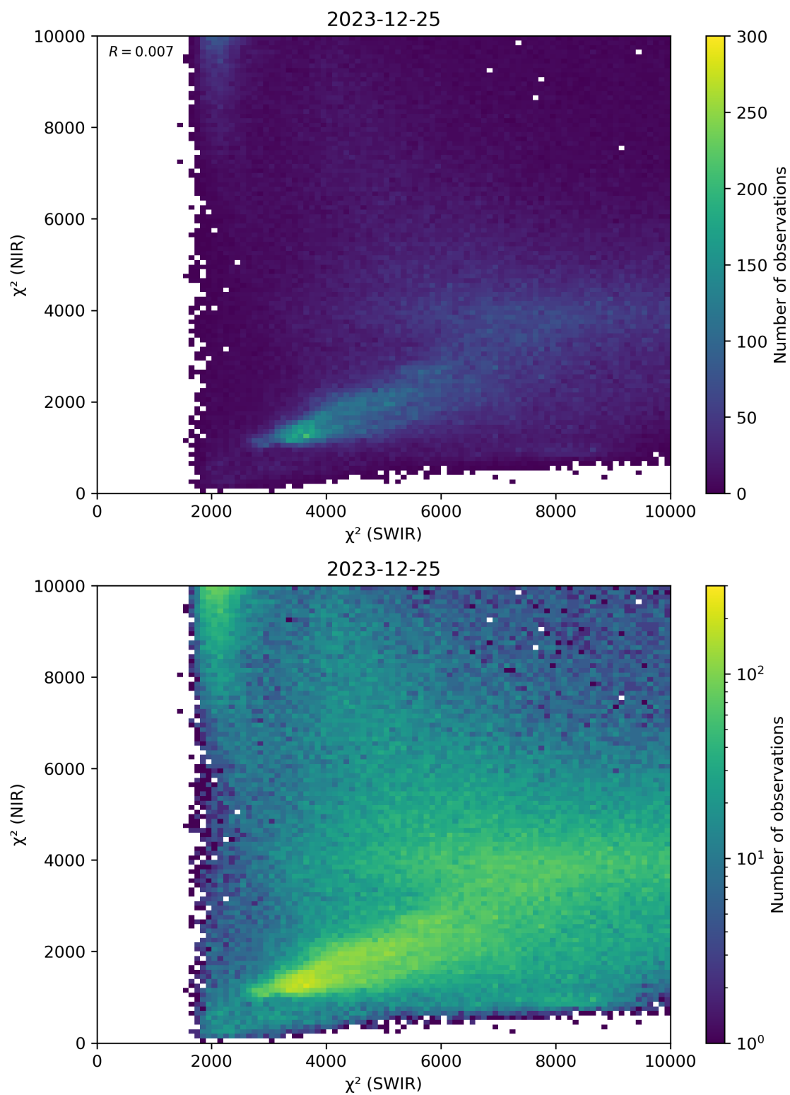
Figure 47: Scatter density plot of “ \chi^2 (SWIR)” against “ \chi^2 (NIR)” for 2023-12-25 to 2023-12-26.
