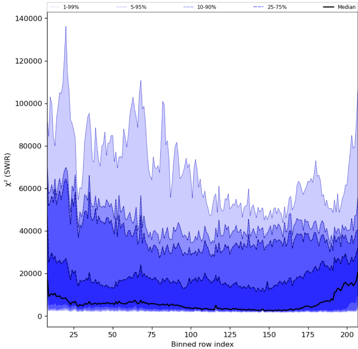
Figure 39: Along track statistics of “ \chi^2 (SWIR)” for 2023-12-25 to 2023-12-26
