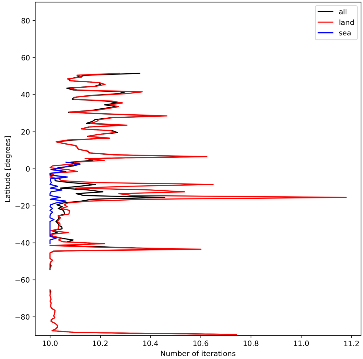
Figure 20: Zonal average of “Number of iterations” for 2023-12-25 to 2023-12-26.
