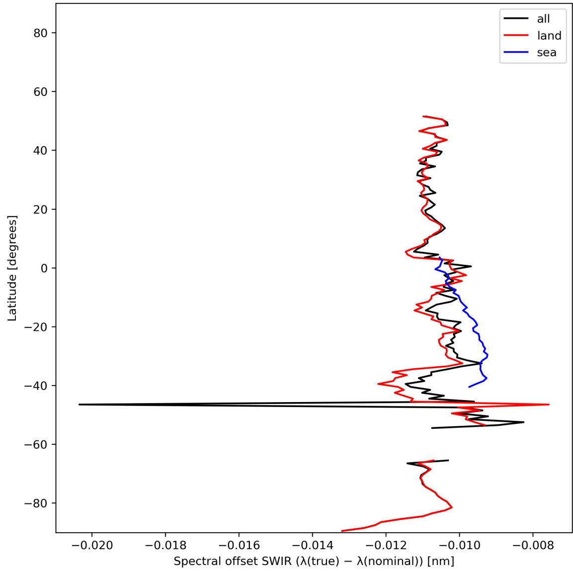
Figure 16: Zonal average of “Spectral offset SWIR ( \lambda(\text{true}) - \lambda(\text{nominal}) )” for 2023-12-25 to 2023-12-26.
