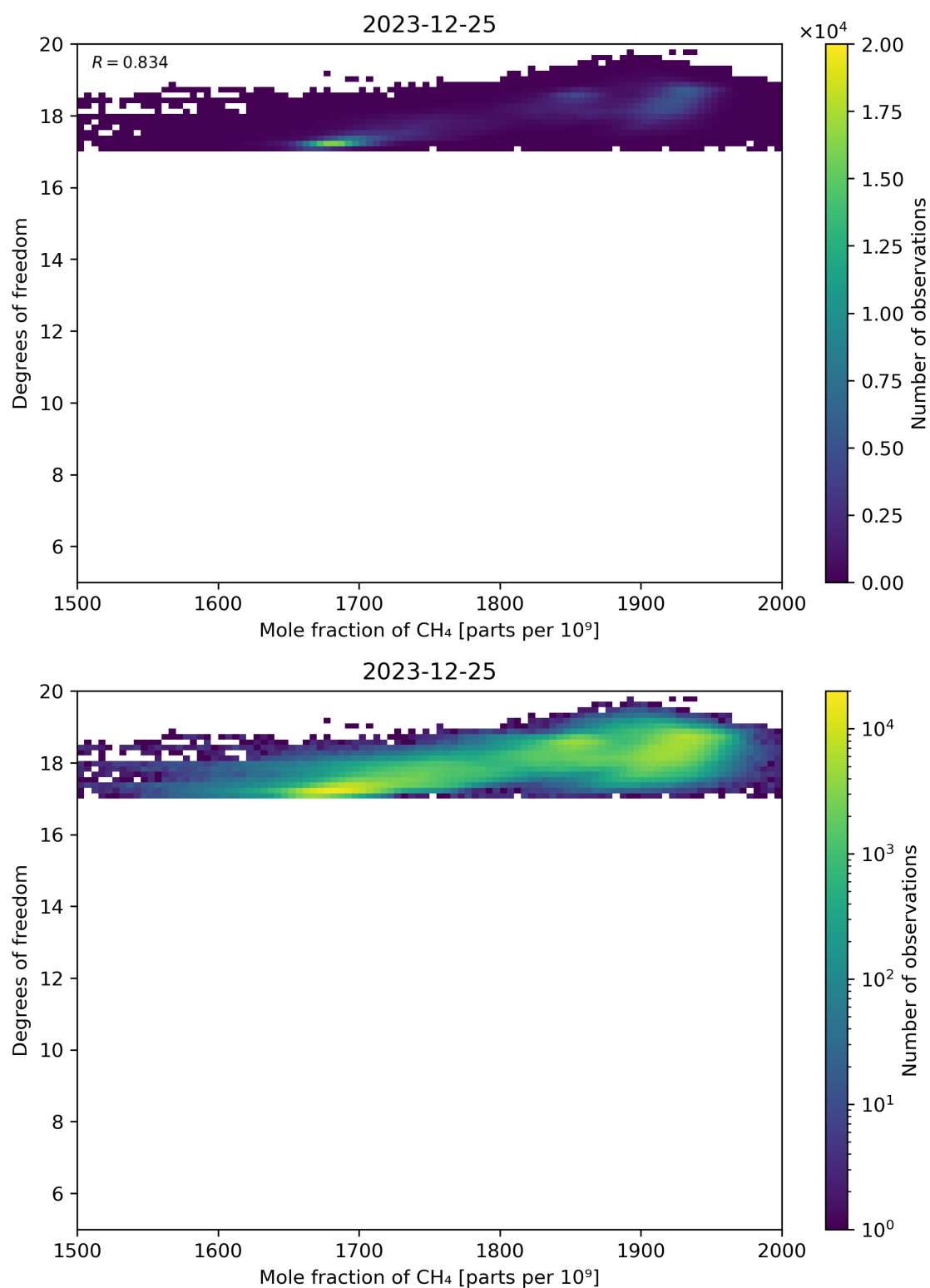
Figure 72: Scatter density plot of “Mole fraction of CH 4 ” against “Degrees of freedom” for 2023-12-25 to 2023-12-26.
