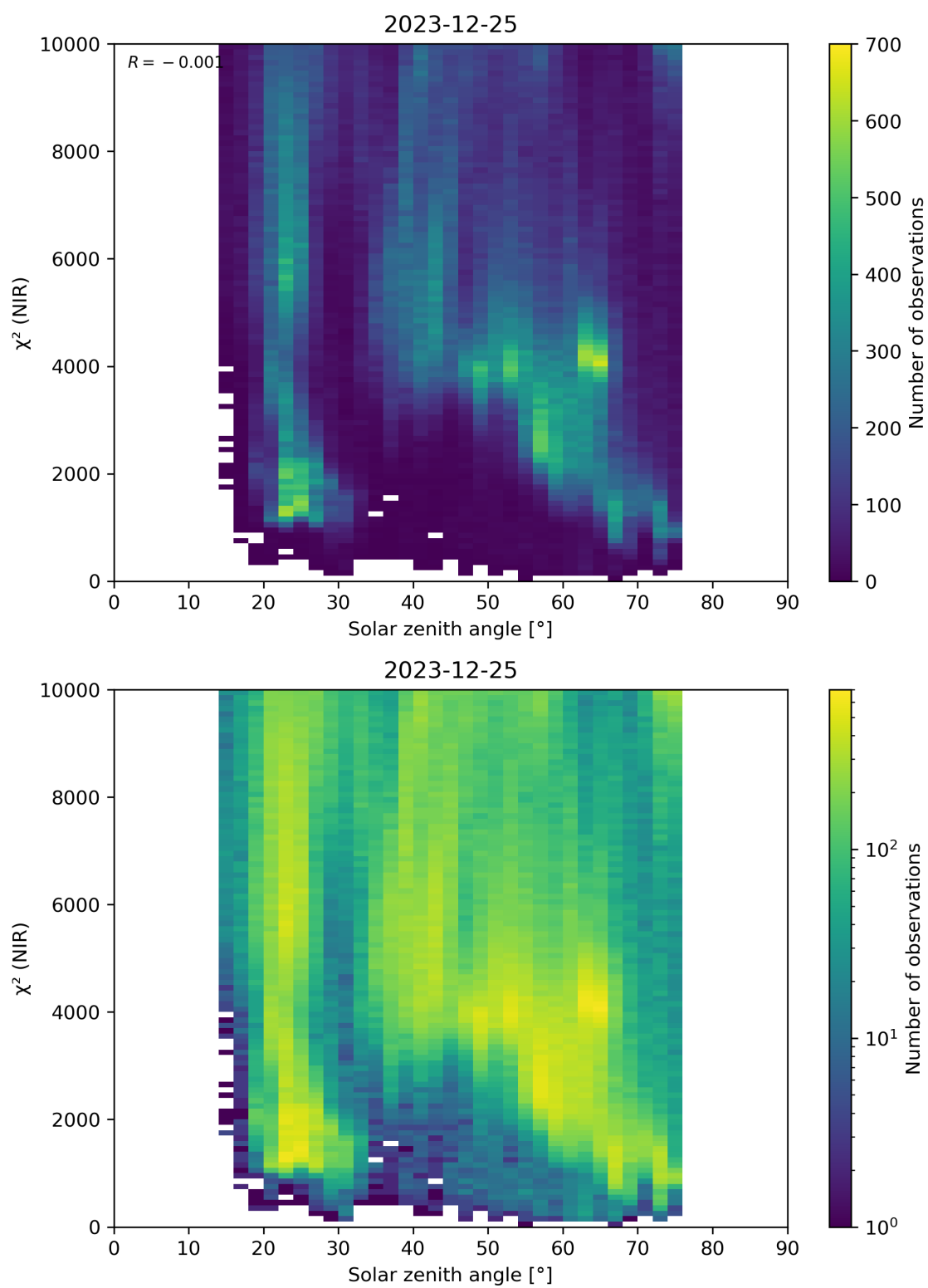
Figure 94: Scatter density plot of “Solar zenith angle” against “ \chi^2 (NIR)” for 2023-12-25 to 2023-12-26.
