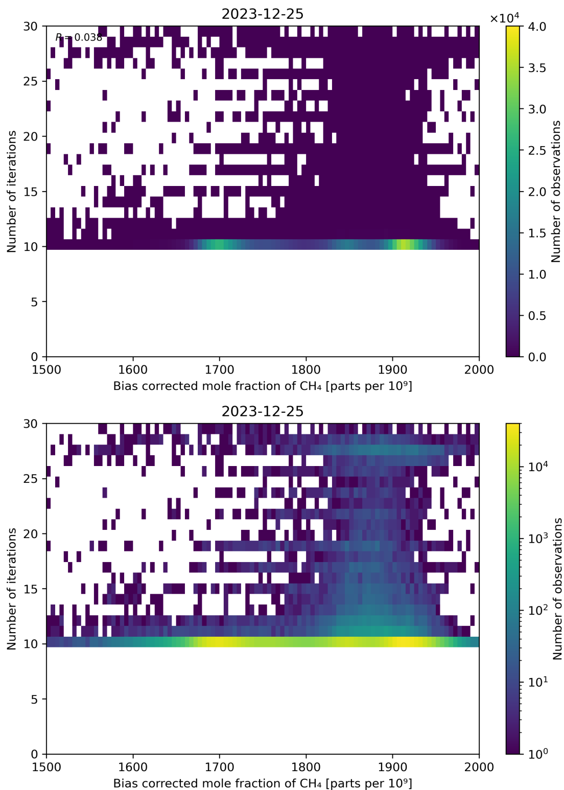
Figure 67: Scatter density plot of “Bias corrected mole fraction of \text{CH}_4 ” against “Number of iterations” for 2023-12-25 to 2023-12-26.
