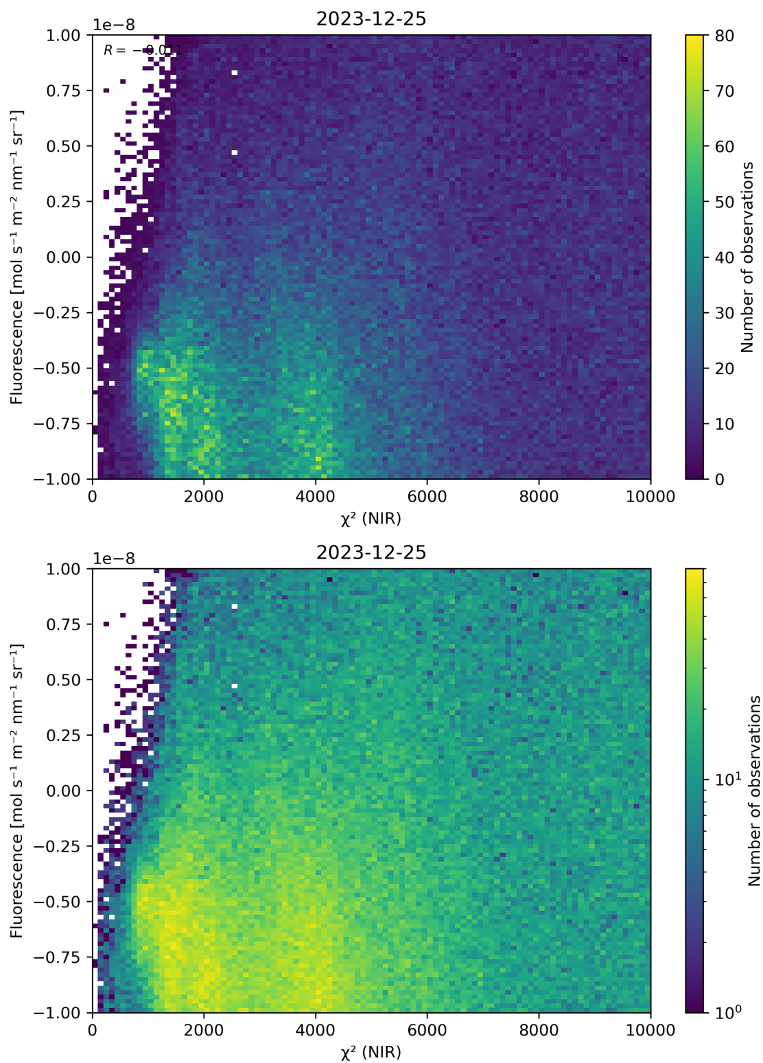
Figure 45: Scatter density plot of “ \chi^2 (NIR)” against “Fluorescence” for 2023-12-25 to 2023-12-26.
