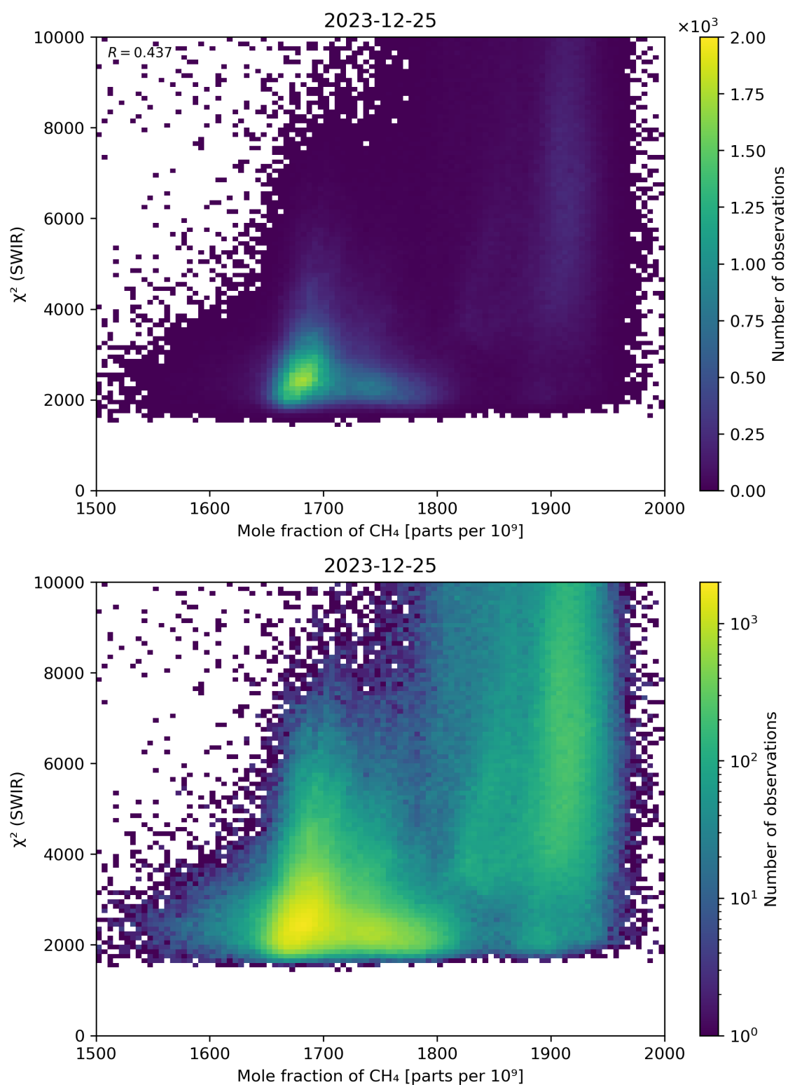
Figure 71: Scatter density plot of “Mole fraction of \text{CH}_4 ” against “ \chi^2 (SWIR)” for 2023-12-25 to 2023-12-26.
