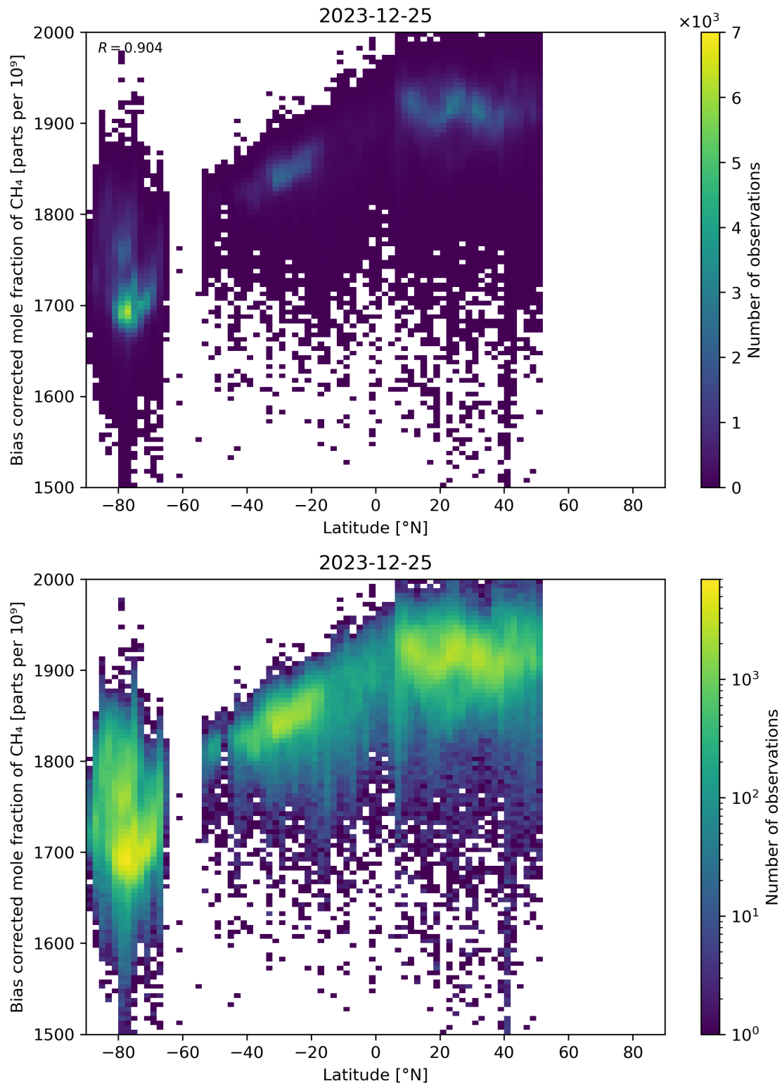
Figure 58: Scatter density plot of “Latitude” against “Bias corrected mole fraction of CH 4 ” for 2023-12-25 to 2023-12-26.
