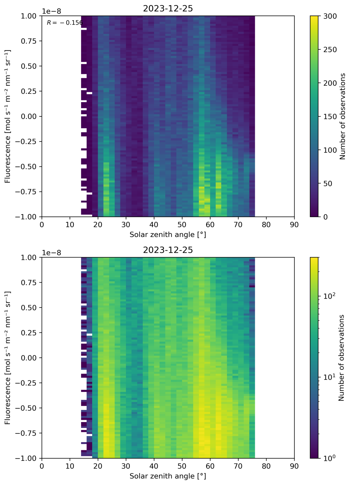
Figure 97: Scatter density plot of “Solar zenith angle” against “Fluorescence” for 2023-12-25 to 2023-12-26.
