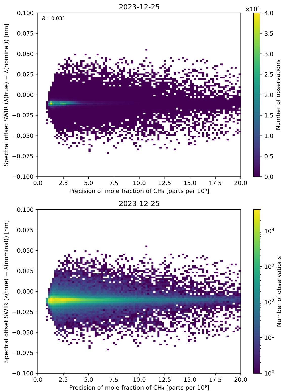
Figure 85: Scatter density plot of “Precision of mole fraction of \text{CH}_4 ” against “Spectral offset SWIR ( \lambda(\text{true}) - \lambda(\text{nominal}) )” for 2023-12-25 to 2023-12-26.
