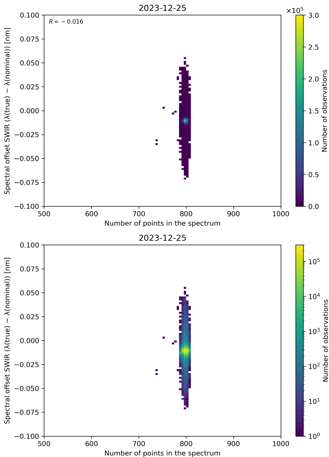
Figure 93: Scatter density plot of “Number of points in the spectrum” against “Spectral offset SWIR ( \lambda(\text{true}) - \lambda(\text{nominal}) )” for 2023-12-25 to 2023-12-26.
