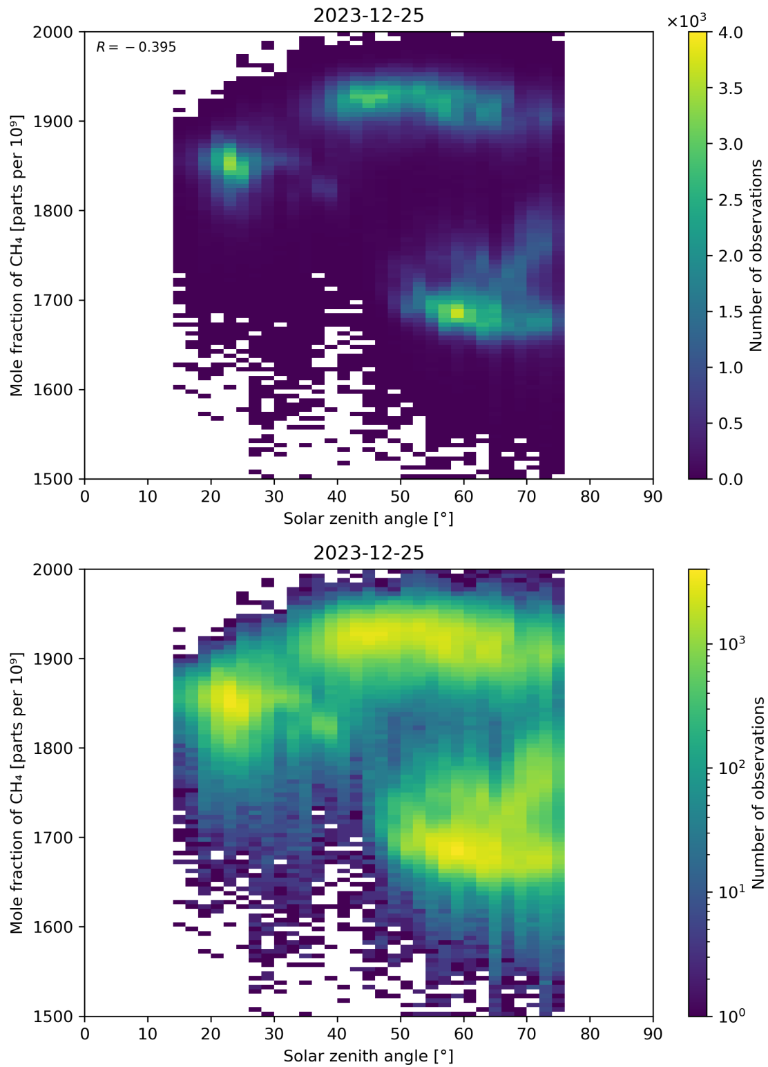
Figure 99: Scatter density plot of “Solar zenith angle” against “Mole fraction of CH 4 ” for 2023-12-25 to 2023-12-26.
