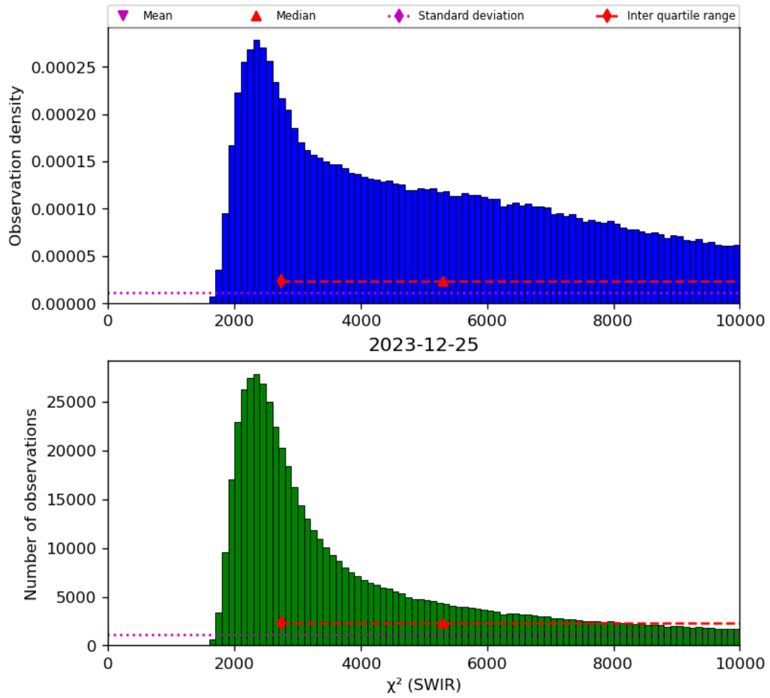
Figure 28: Histogram of “ \chi^2 (SWIR)” for 2023-12-25 to 2023-12-26
