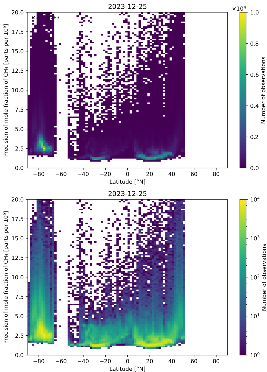
Figure 59: Scatter density plot of “Latitude” against “Precision of mole fraction of CH 4 ” for 2023-12-25 to 2023-12-26.
