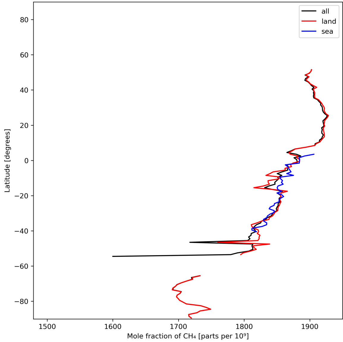
Figure 12: Zonal average of “Mole fraction of CH 4 ” for 2023-12-25 to 2023-12-26.
