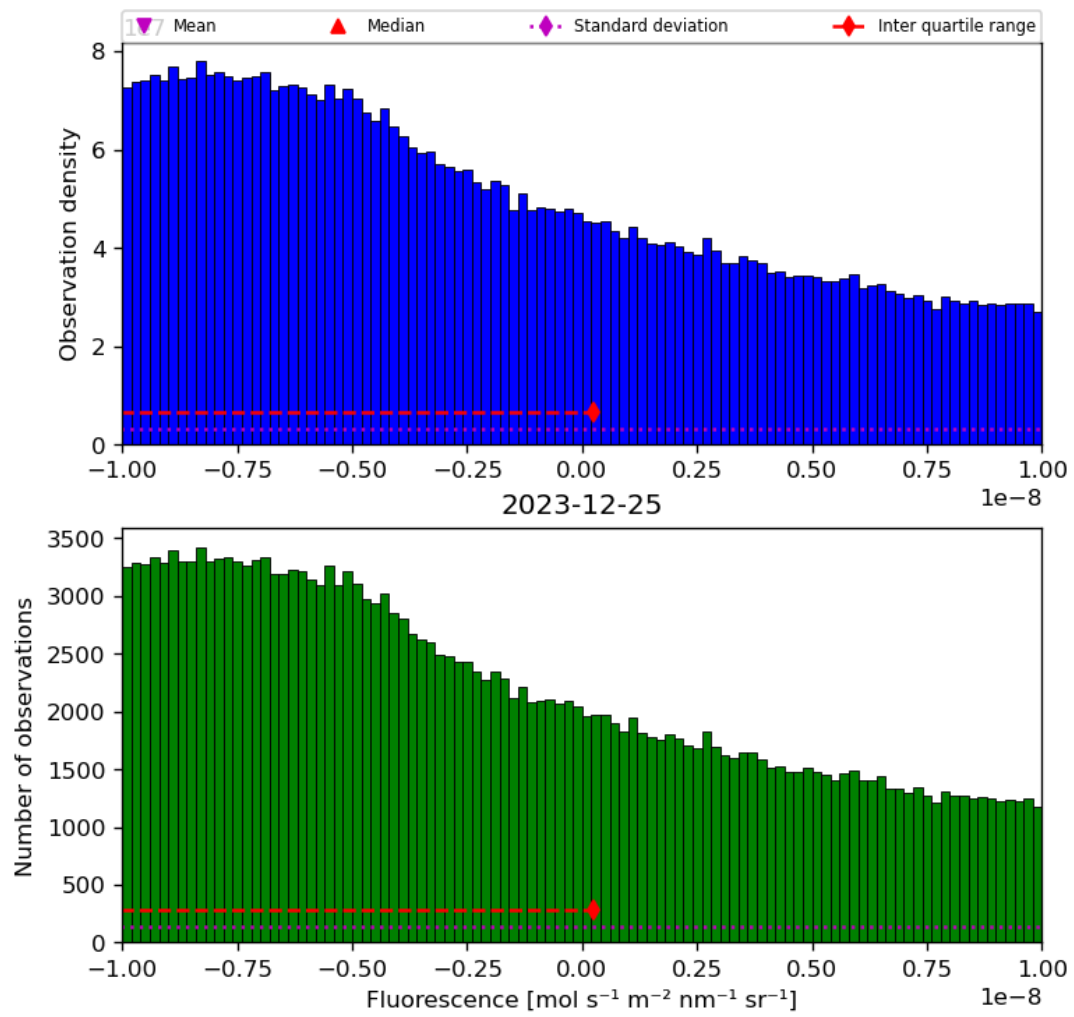
Figure 32: Histogram of “Fluorescence” for 2023-12-25 to 2023-12-26
