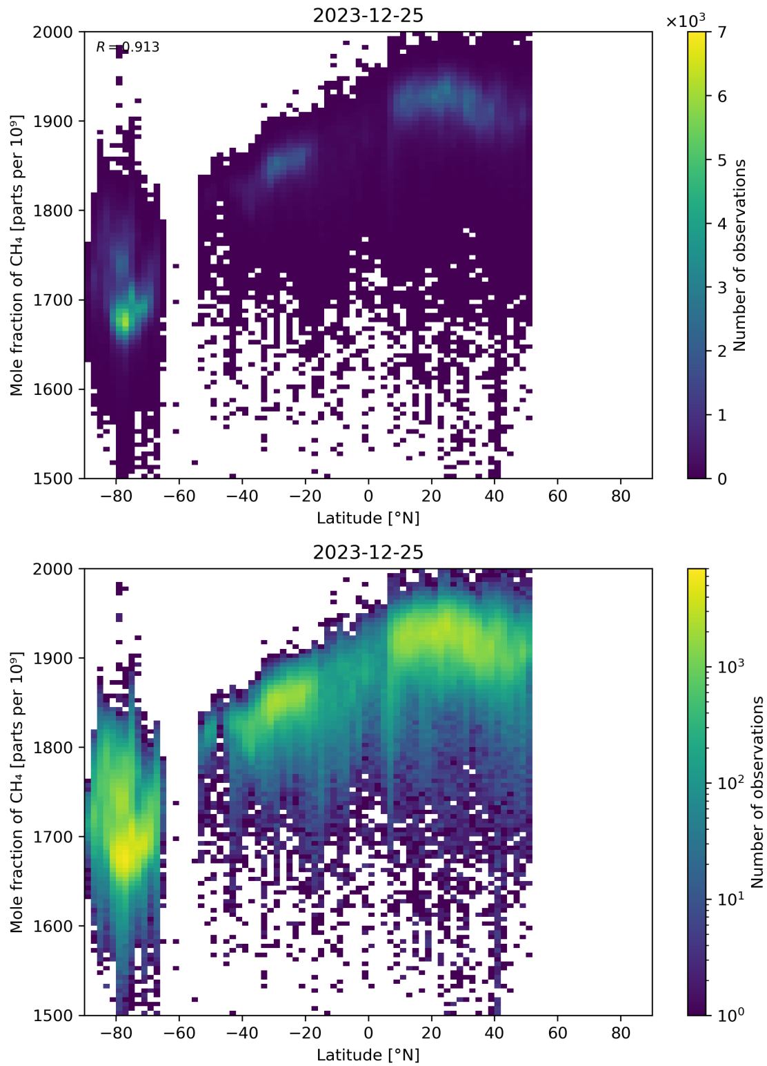
Figure 57: Scatter density plot of “Latitude” against “Mole fraction of CH 4 ” for 2023-12-25 to 2023-12-26.
