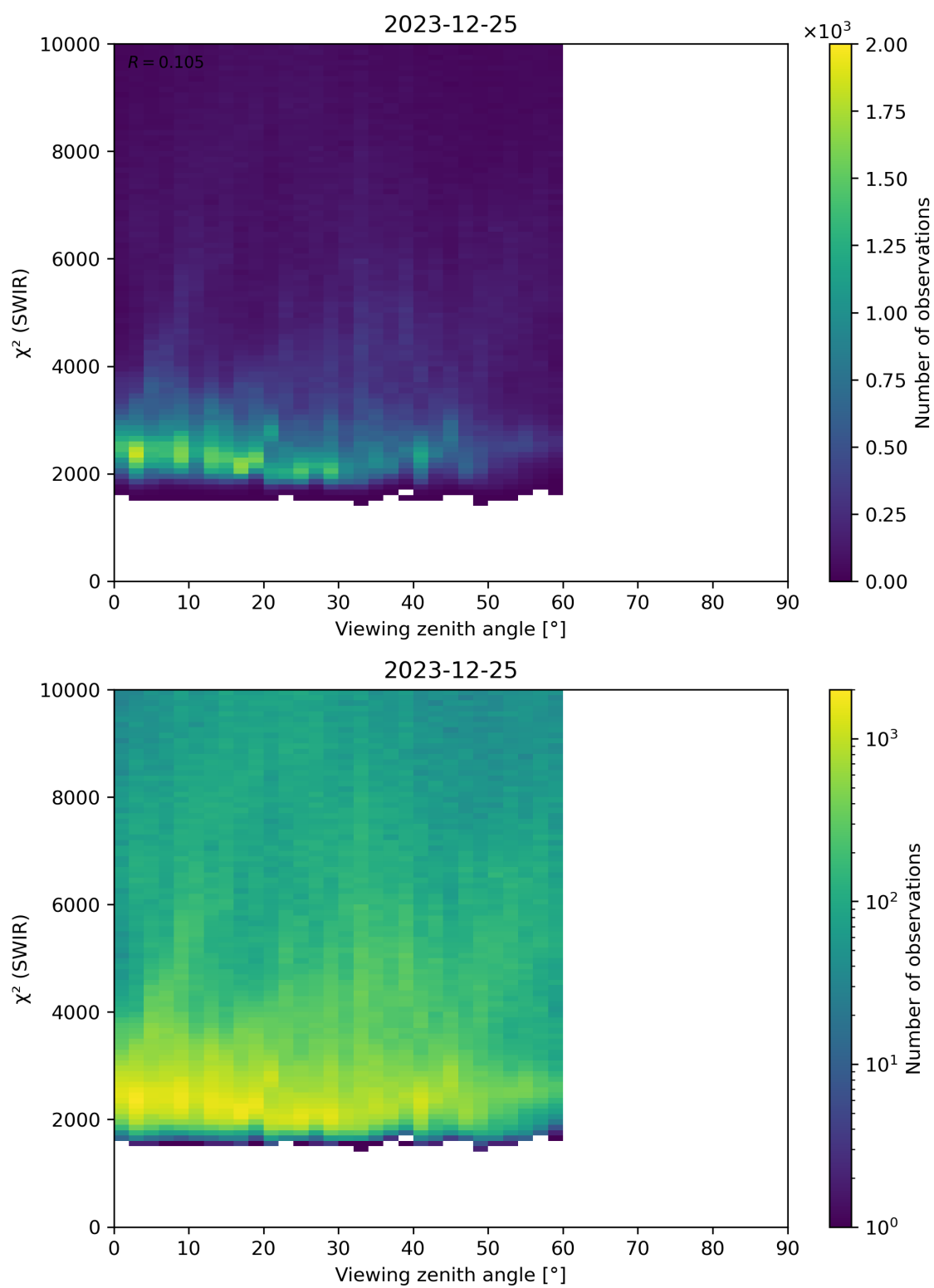
Figure 106: Scatter density plot of “Viewing zenith angle” against “ \chi^2 (SWIR)” for 2023-12-25 to 2023-12-26.
