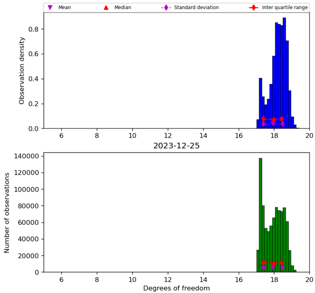
Figure 30: Histogram of “Degrees of freedom” for 2023-12-25 to 2023-12-26
