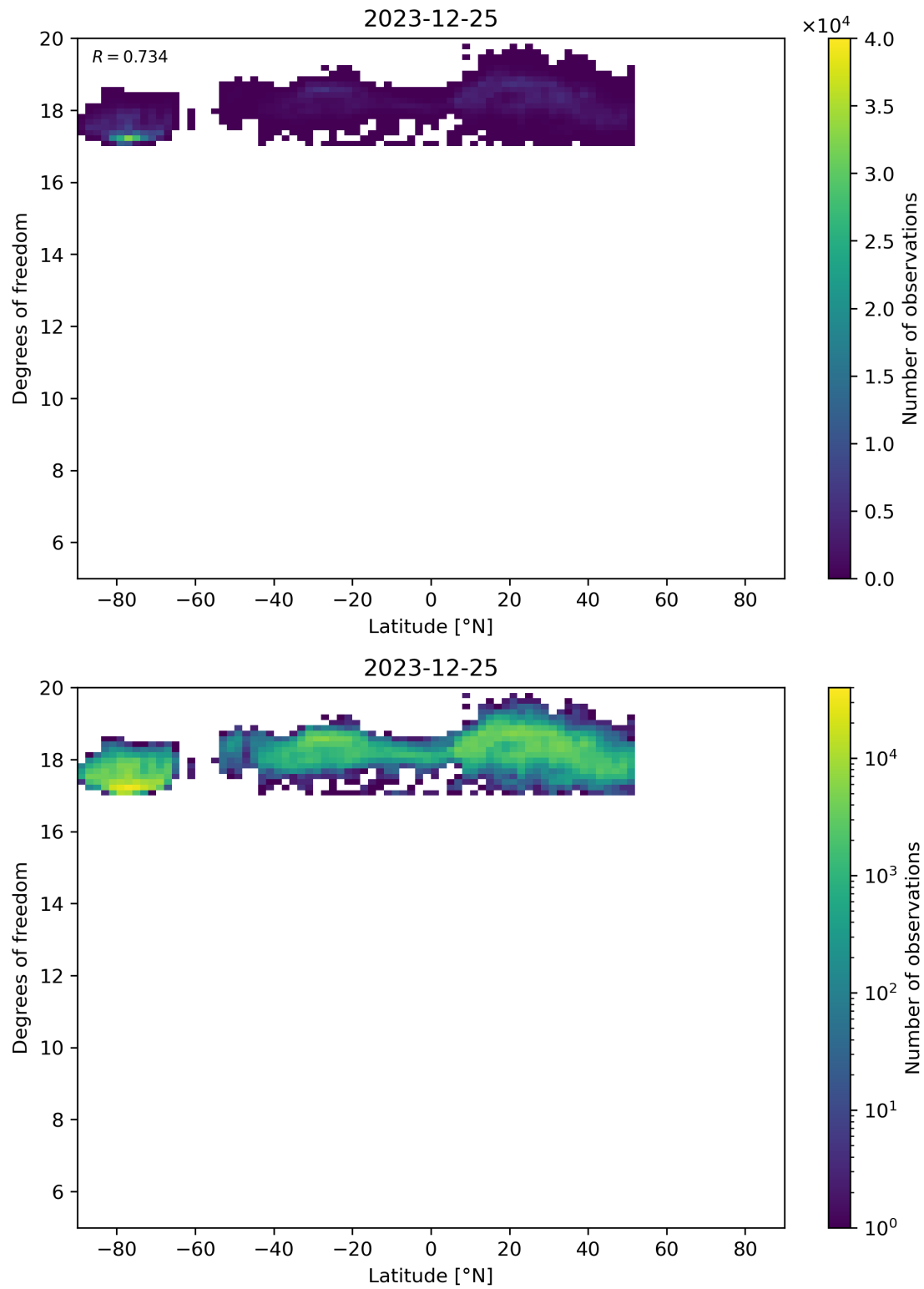
Figure 55: Scatter density plot of “Latitude” against “Degrees of freedom” for 2023-12-25 to 2023-12-26.
