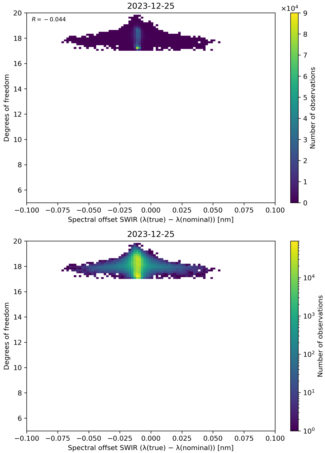
Figure 119: Scatter density plot of “Spectral offset SWIR ( \lambda(\text{true}) - \lambda(\text{nominal}) )” against “Degrees of freedom” for 2023-12-25 to 2023-12-26.
