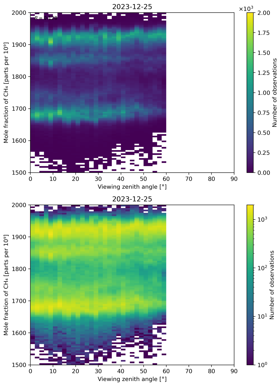
Figure 110: Scatter density plot of “Viewing zenith angle” against “Mole fraction of CH 4 ” for 2023-12-25 to 2023-12-26.
