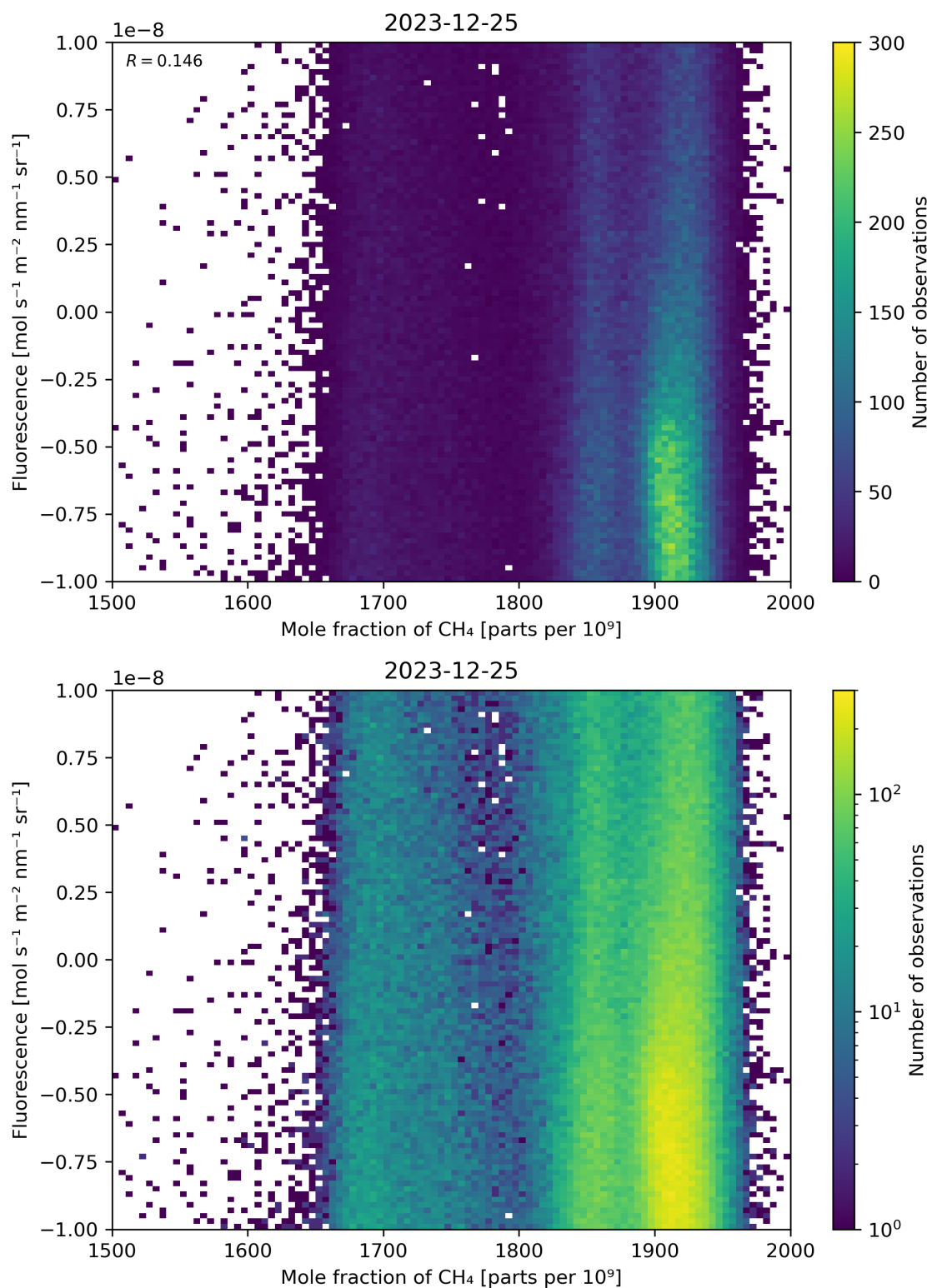
Figure 73: Scatter density plot of “Mole fraction of \text{CH}_4 ” against “Fluorescence” for 2023-12-25 to 2023-12-26.
