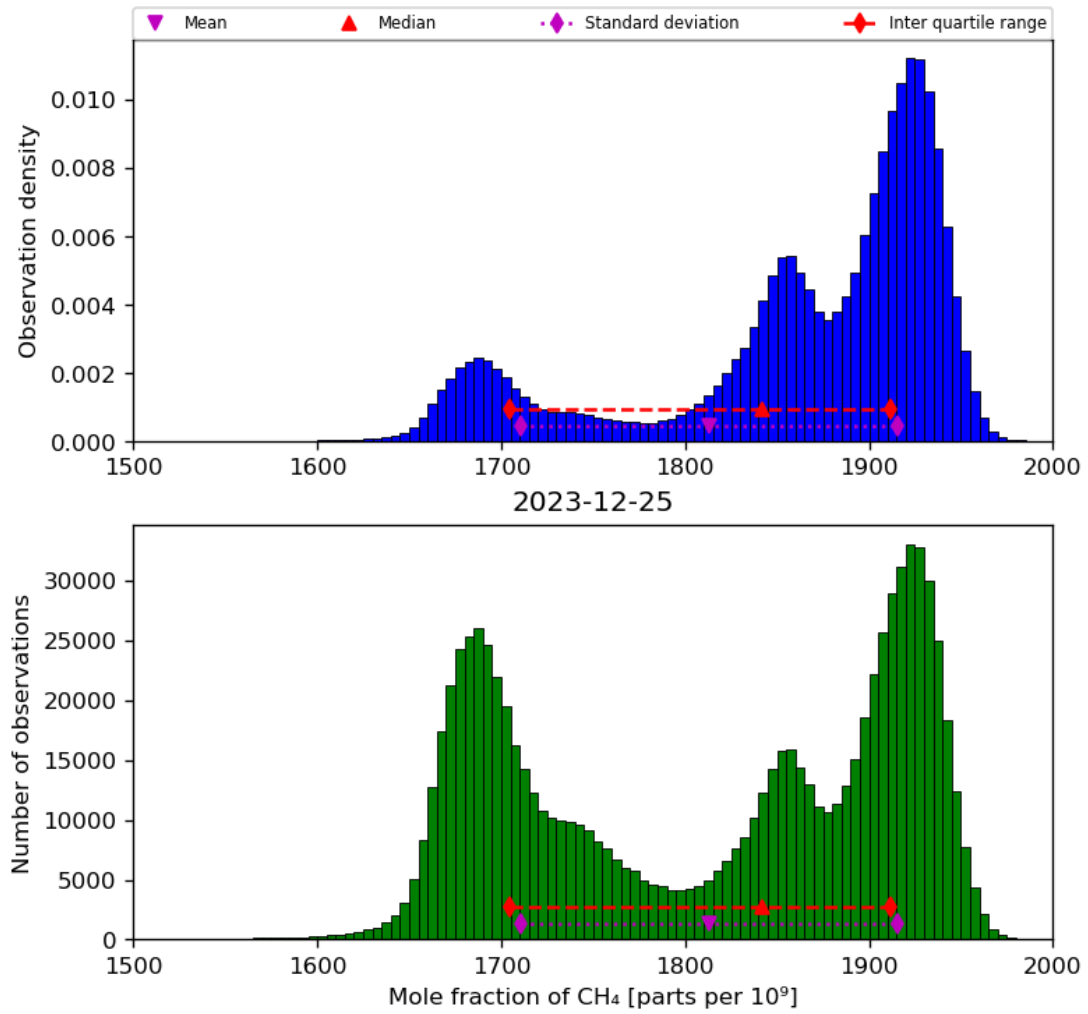
Figure 23: Histogram of “Mole fraction of CH 4 ” for 2023-12-25 to 2023-12-26
