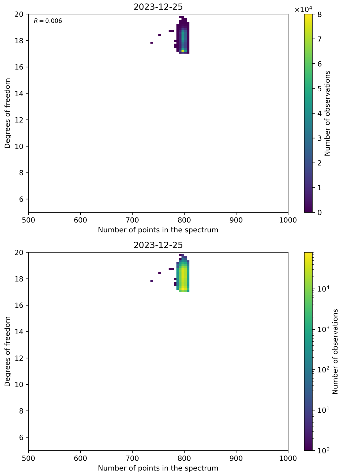
Figure 90: Scatter density plot of “Number of points in the spectrum” against “Degrees of freedom” for 2023-12-25 to 2023-12-26.
