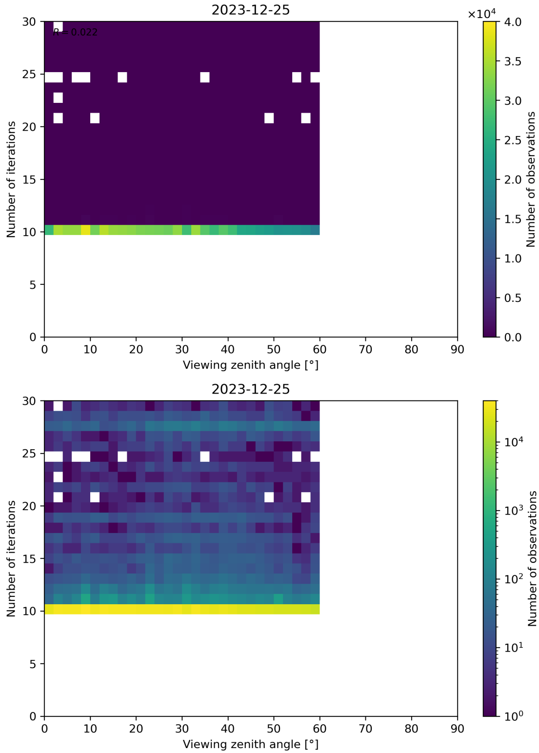
Figure 113: Scatter density plot of “Viewing zenith angle” against “Number of iterations” for 2023-12-25 to 2023-12-26.
