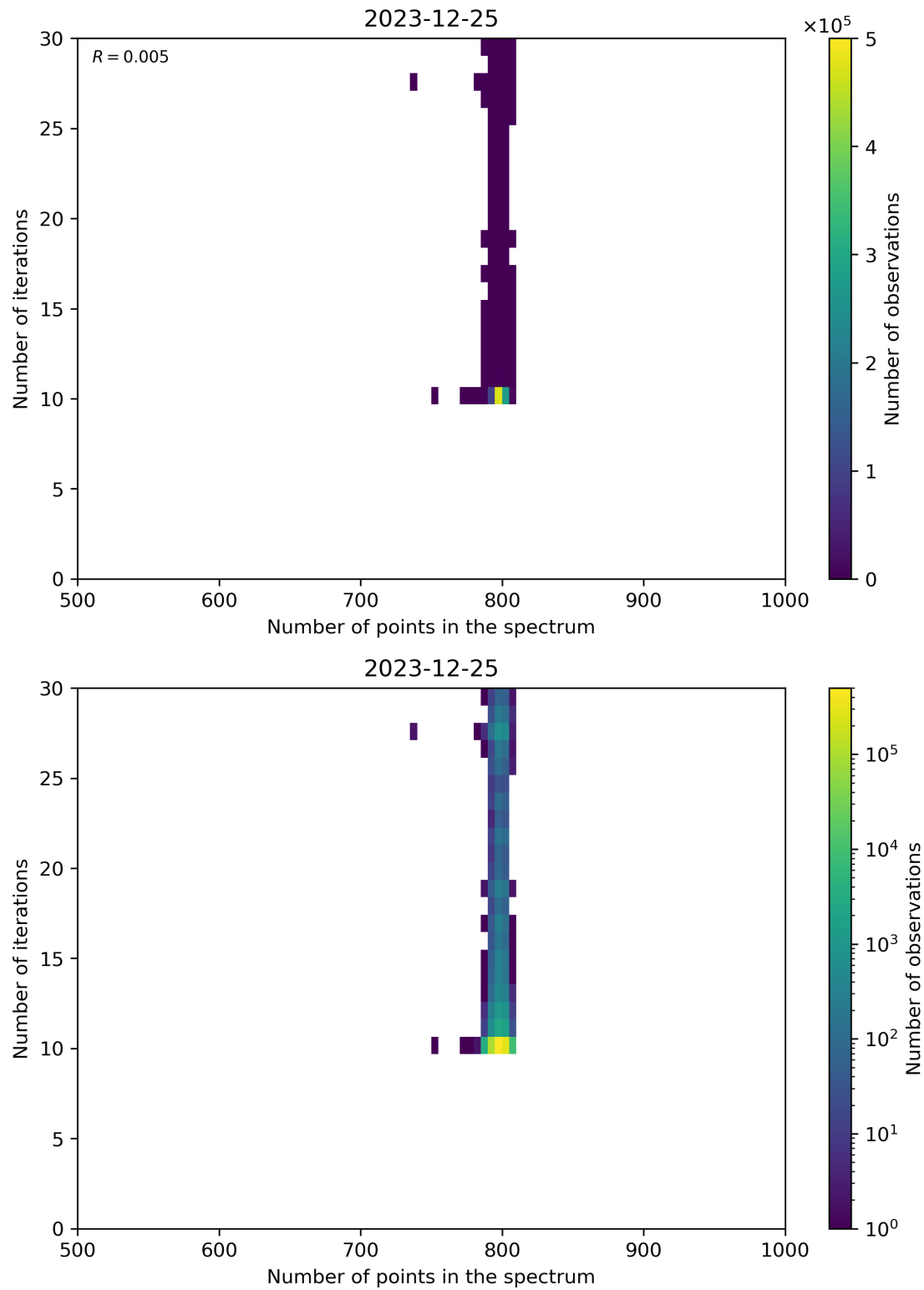
Figure 92: Scatter density plot of “Number of points in the spectrum” against “Number of iterations” for 2023-12-25 to 2023-12-26.
