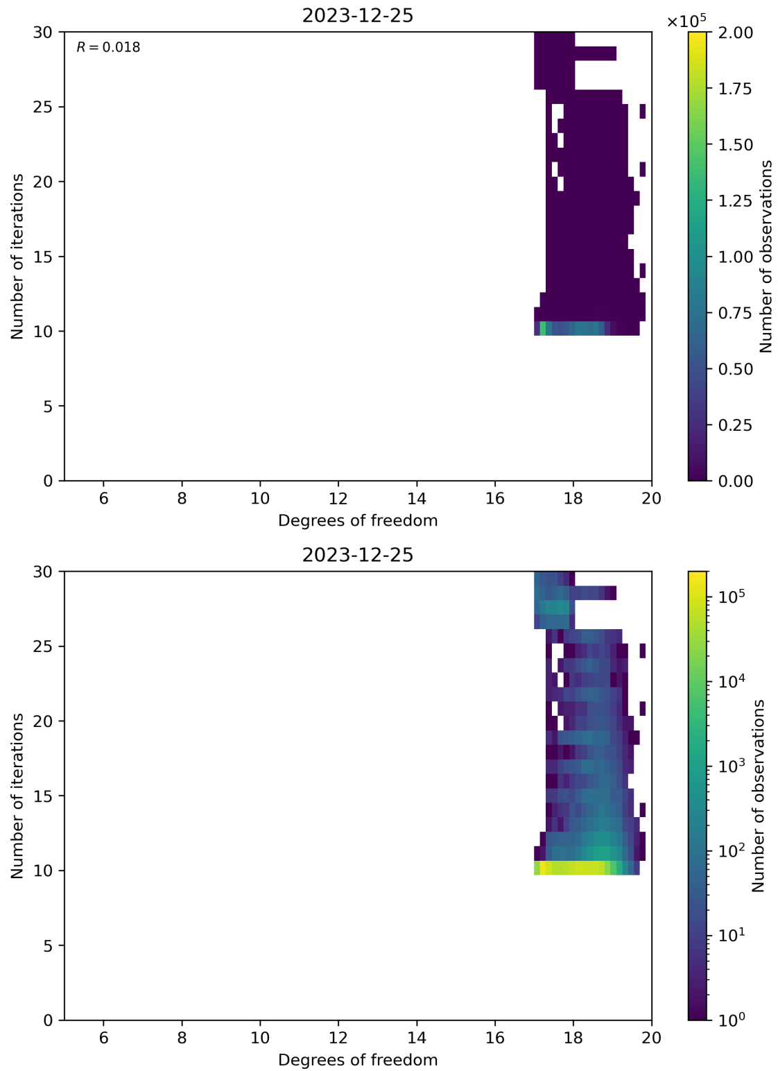
Figure 52: Scatter density plot of “Degrees of freedom” against “Number of iterations” for 2023-12-25 to 2023-12-26.
