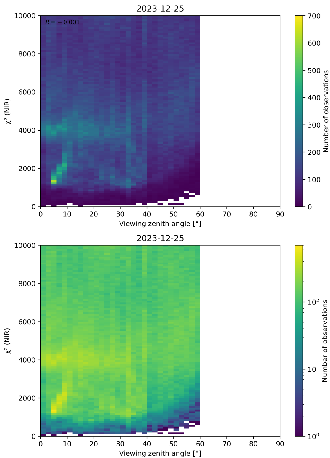
Figure 105: Scatter density plot of “Viewing zenith angle” against “ \chi^2 (NIR)” for 2023-12-25 to 2023-12-26.
