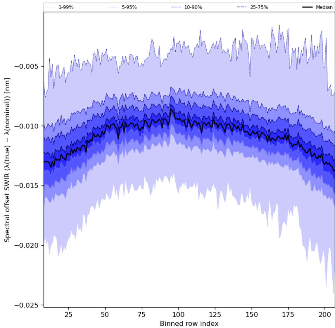
Figure 38: Along track statistics of “Spectral offset SWIR ( \lambda(\text{true}) - \lambda(\text{nominal}) )” for 2023-12-25 to 2023-12-26
