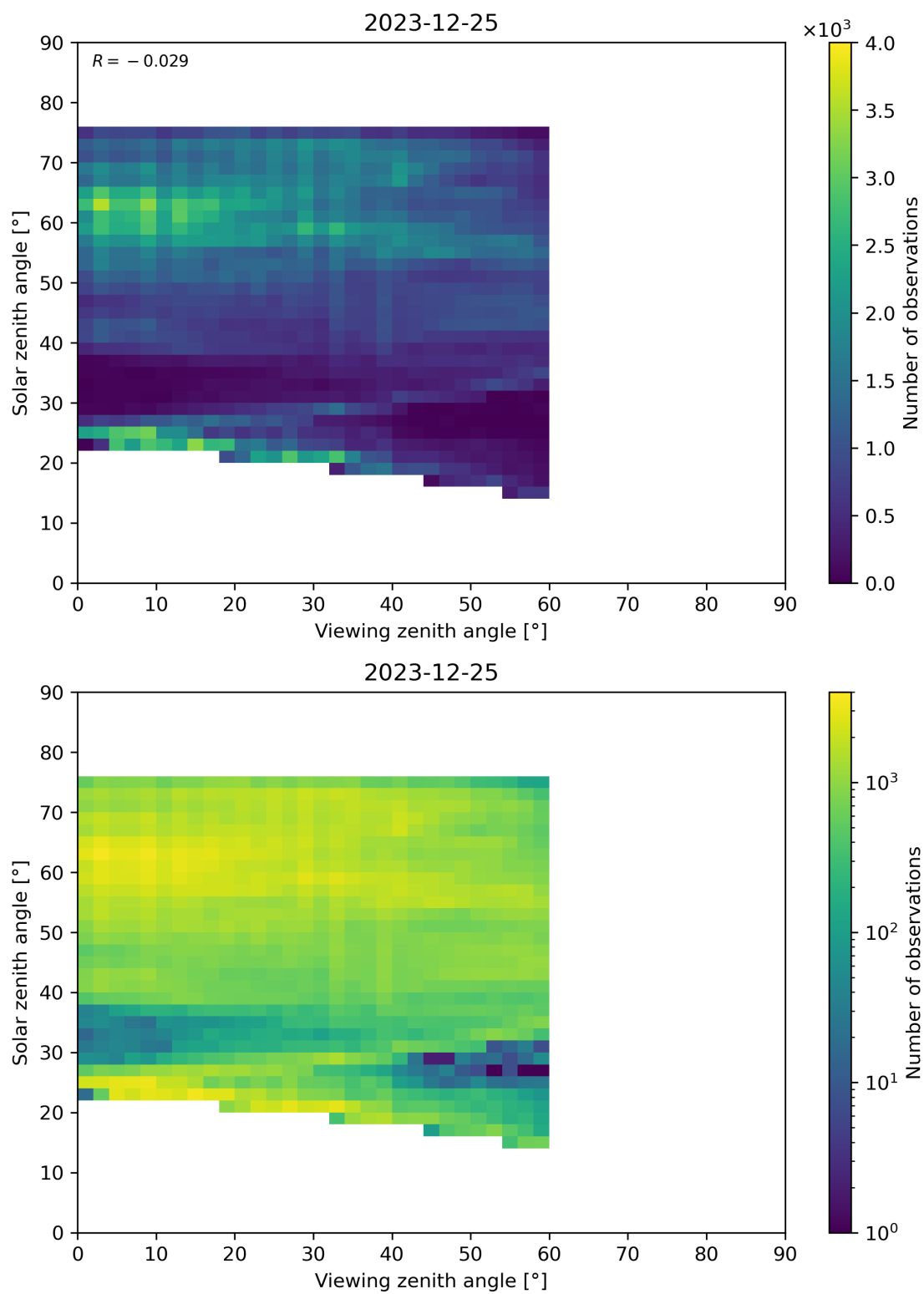
Figure 115: Scatter density plot of “Viewing zenith angle” against “Solar zenith angle” for 2023-12-25 to 2023-12-26.
