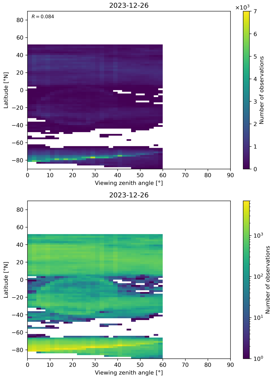
Figure 109: Scatter density plot of “Viewing zenith angle” against “Latitude” for 2023-12-25 to 2023-12-27.
