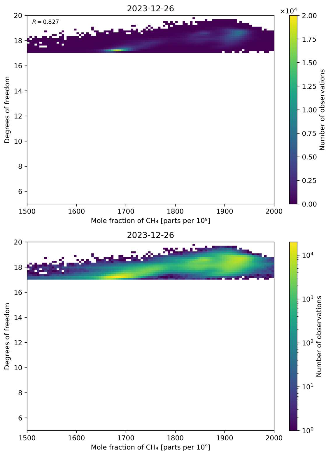
Figure 72: Scatter density plot of “Mole fraction of CH 4 ” against “Degrees of freedom” for 2023-12-25 to 2023-12-27.
