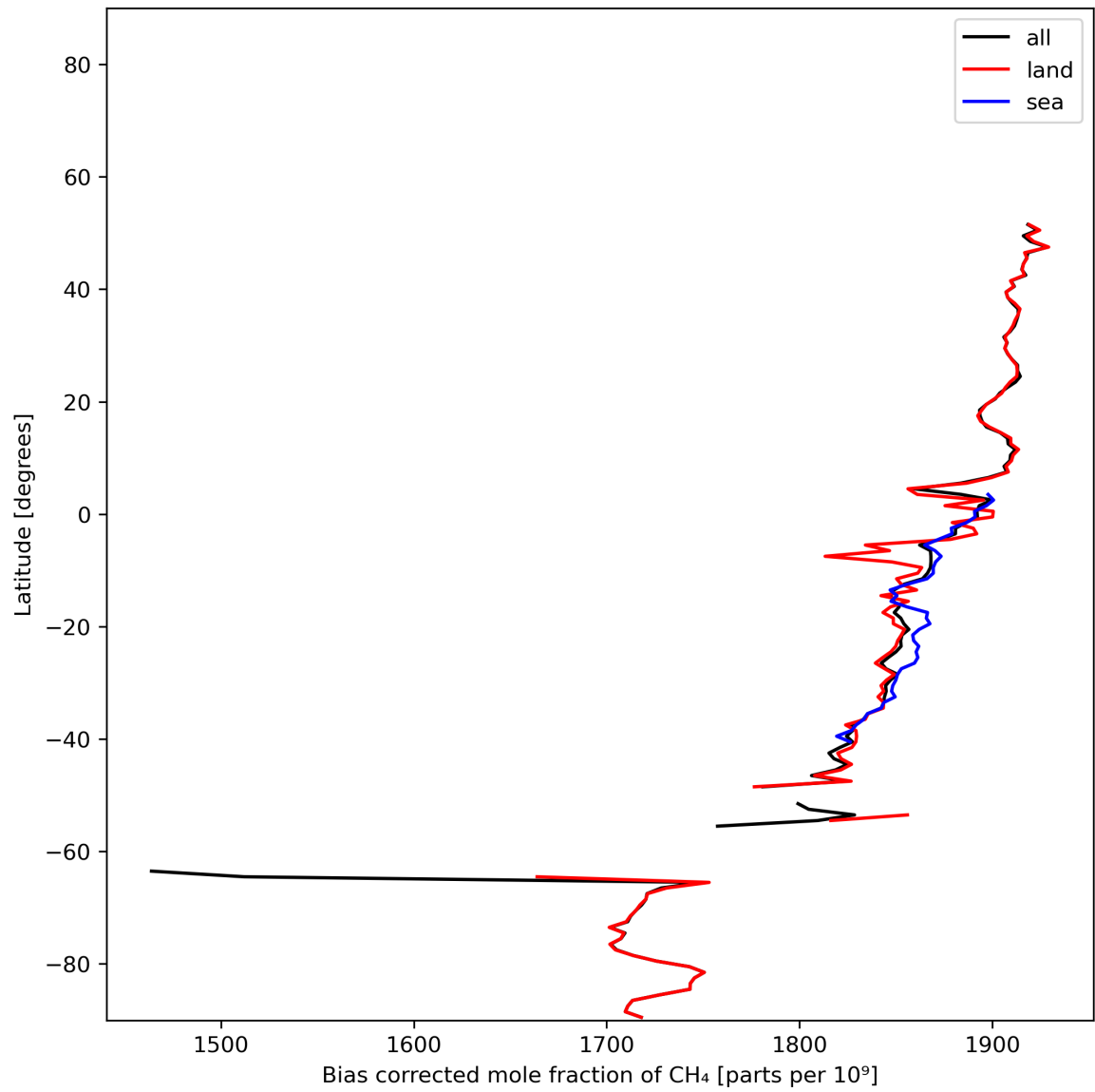
Figure 14: Zonal average of “Bias corrected mole fraction of CH 4 ” for 2023-12-25 to 2023-12-27.
