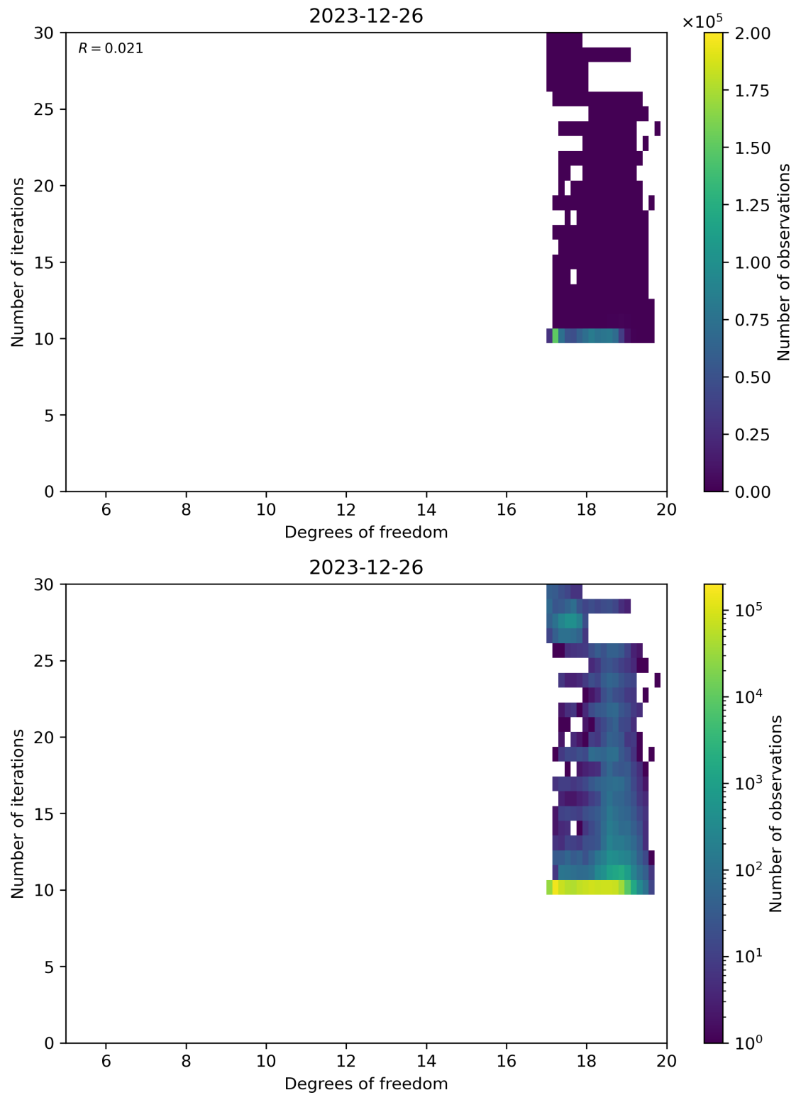
Figure 52: Scatter density plot of “Degrees of freedom” against “Number of iterations” for 2023-12-25 to 2023-12-27.
