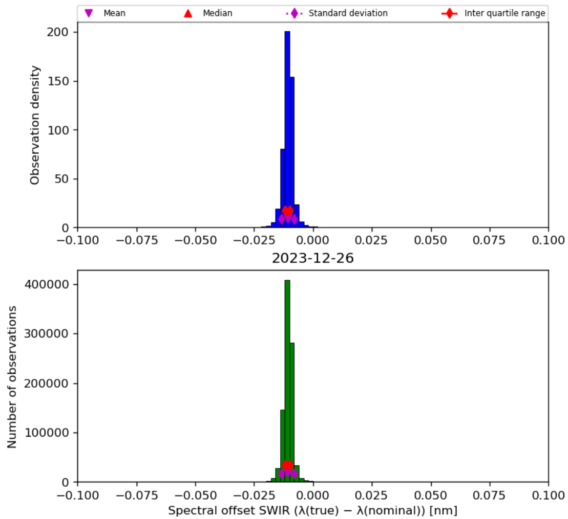
Figure 27: Histogram of “Spectral offset SWIR ( \lambda(\text{true}) - \lambda(\text{nominal}) )” for 2023-12-25 to 2023-12-27
