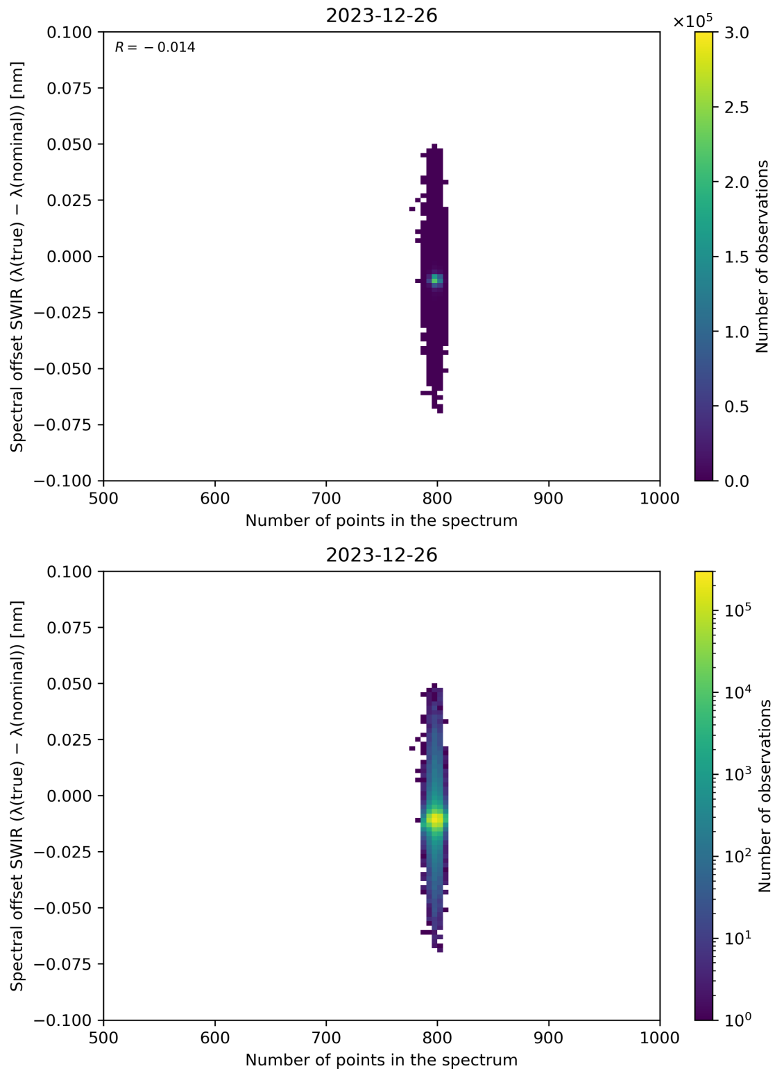
Figure 93: Scatter density plot of “Number of points in the spectrum” against “Spectral offset SWIR ( \lambda(\text{true}) - \lambda(\text{nominal}) )” for 2023-12-25 to 2023-12-27.
