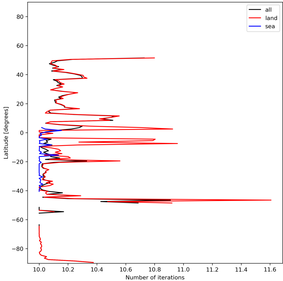
Figure 20: Zonal average of “Number of iterations” for 2023-12-25 to 2023-12-27.
