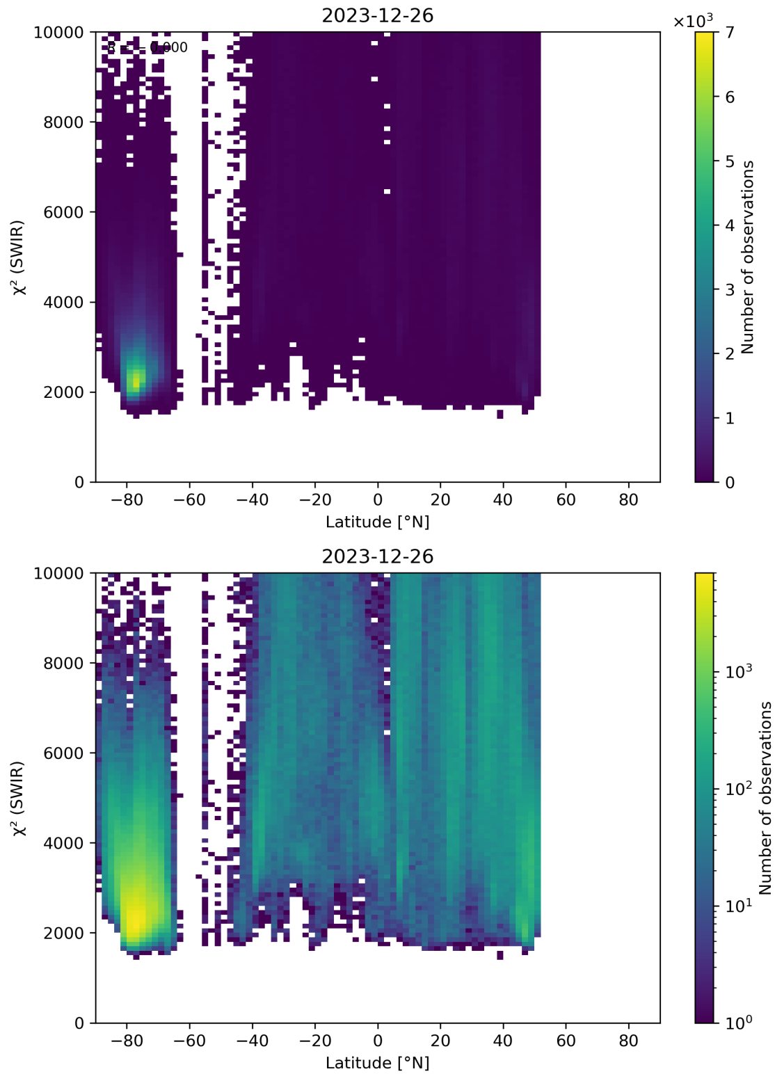
Figure 54: Scatter density plot of “Latitude” against “ \chi^2 (SWIR)” for 2023-12-25 to 2023-12-27.
