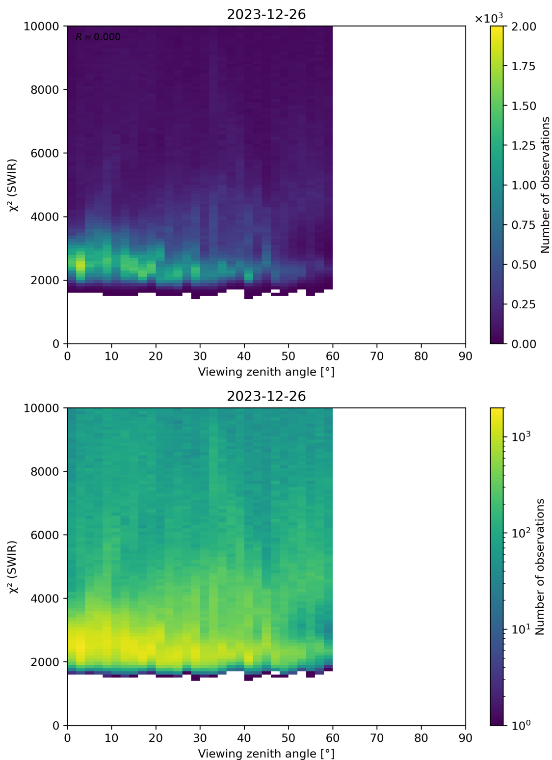
Figure 106: Scatter density plot of “Viewing zenith angle” against “ \chi^2 (SWIR)” for 2023-12-25 to 2023-12-27.
