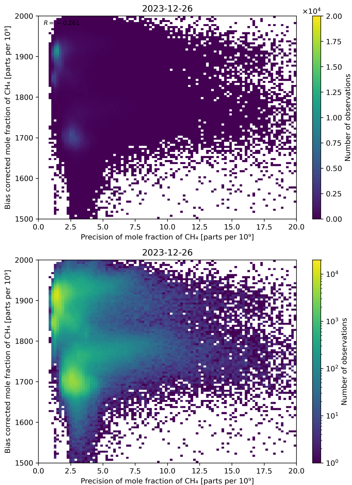
Figure 82: Scatter density plot of “Precision of mole fraction of CH 4 ” against “Bias corrected mole fraction of CH 4 ” for 2023-12-25 to 2023-12-27.
