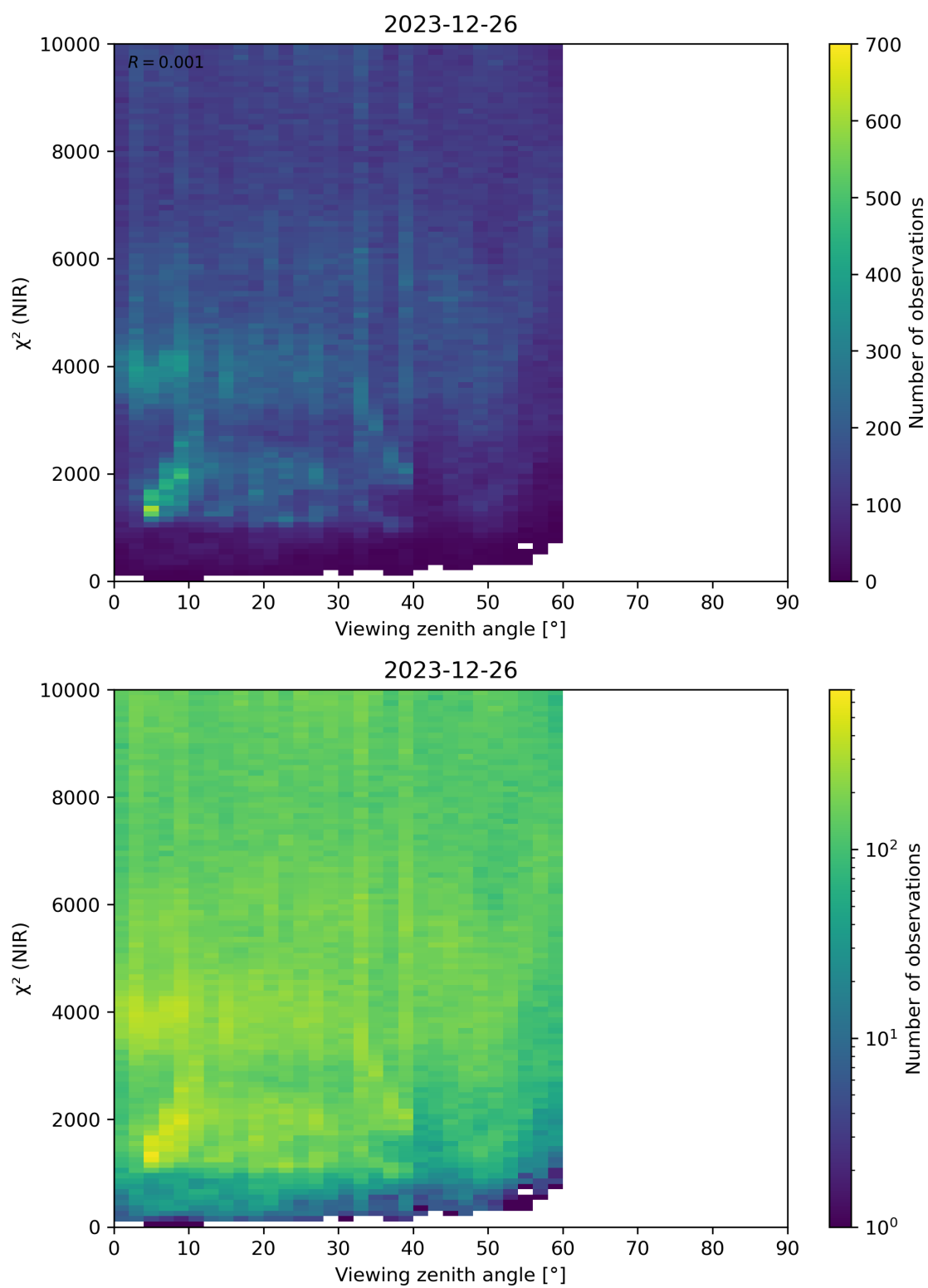
Figure 105: Scatter density plot of “Viewing zenith angle” against “ \chi^2 (NIR)” for 2023-12-25 to 2023-12-27.
