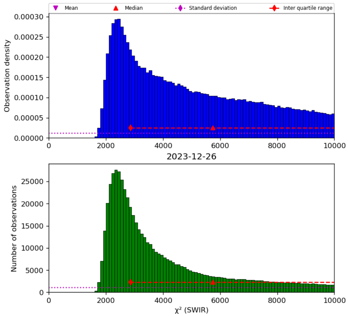
Figure 28: Histogram of “ \chi^2 (SWIR)” for 2023-12-25 to 2023-12-27
