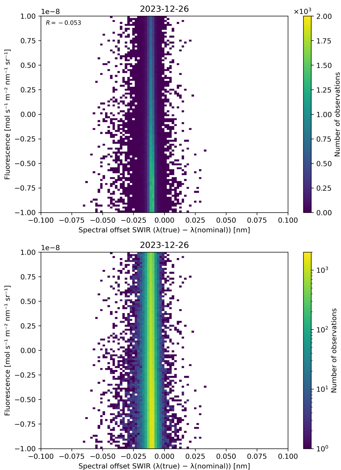
Figure 120: Scatter density plot of “Spectral offset SWIR ( \lambda(\text{true}) - \lambda(\text{nominal}) )” against “Fluorescence” for 2023-12-25 to 2023-12-27.
