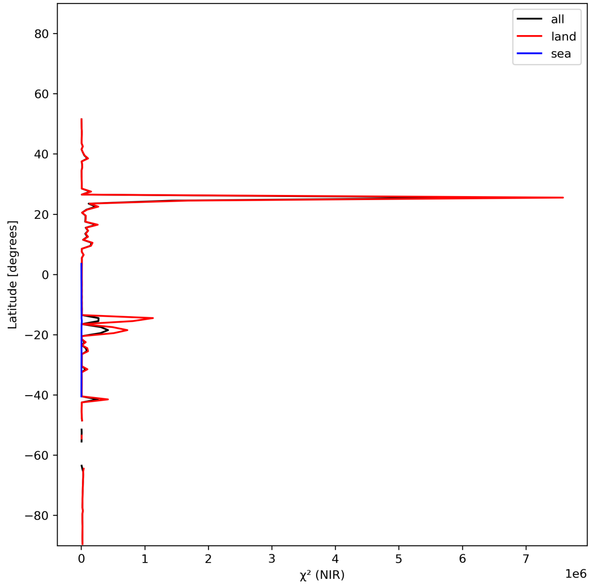
Figure 18: Zonal average of “ \chi^2 (NIR)” for 2023-12-25 to 2023-12-27.
