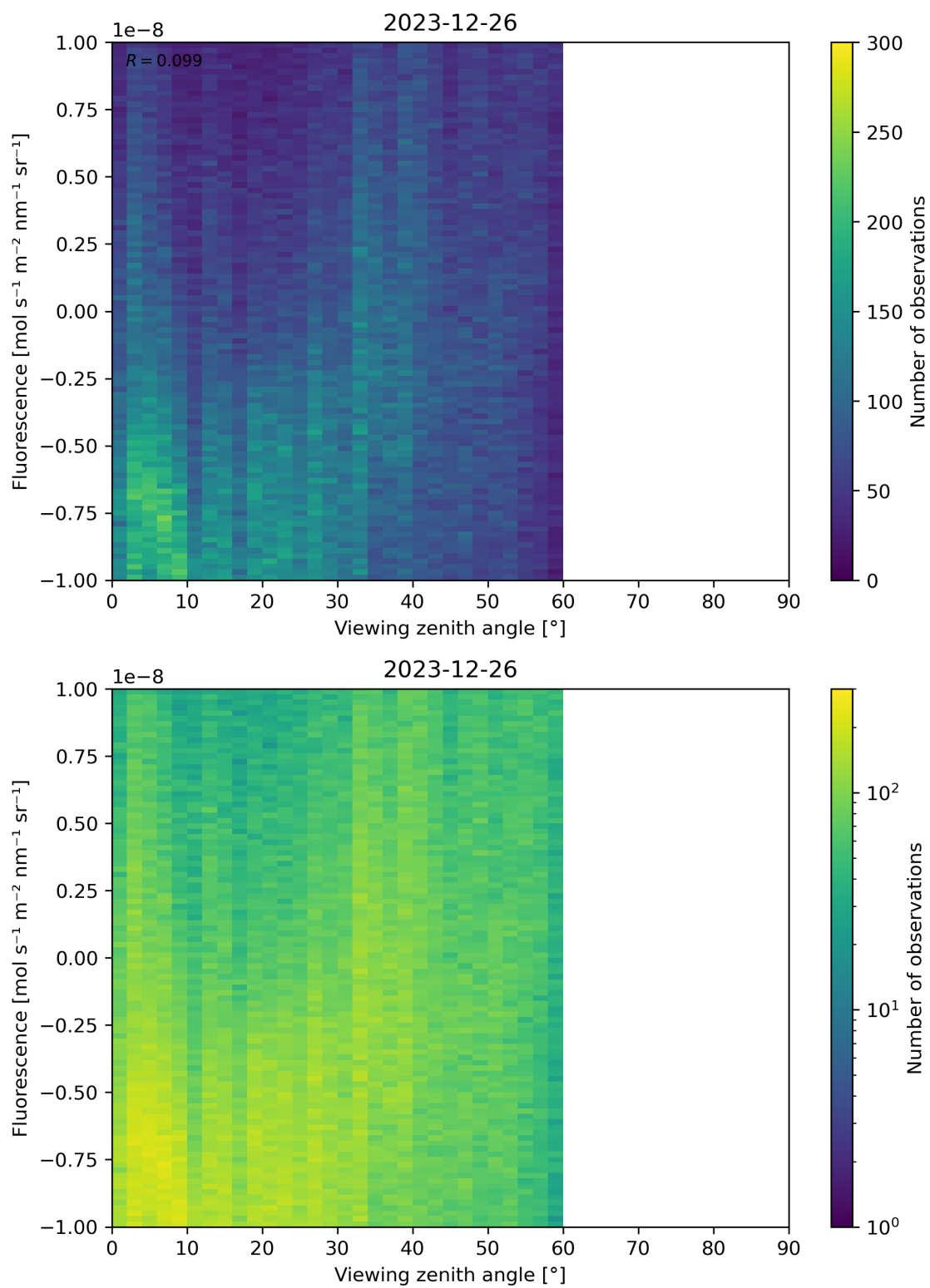
Figure 108: Scatter density plot of “Viewing zenith angle” against “Fluorescence” for 2023-12-25 to 2023-12-27.
