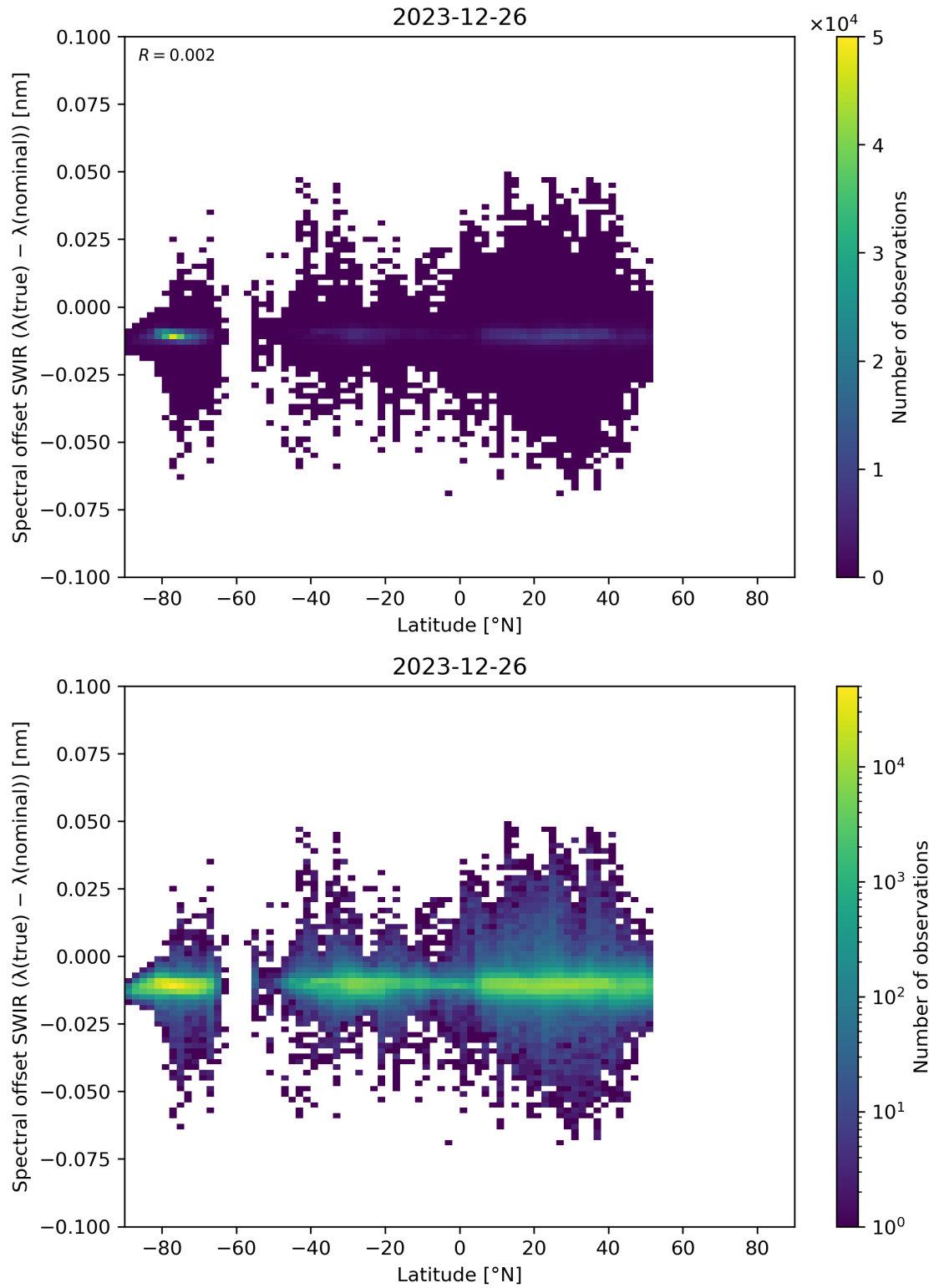
Figure 62: Scatter density plot of “Latitude” against “Spectral offset SWIR ( \lambda(\text{true}) - \lambda(\text{nominal}) )” for 2023-12-25 to 2023-12-27.
