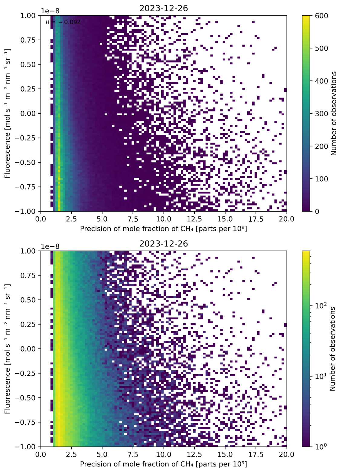
Figure 81: Scatter density plot of “Precision of mole fraction of \text{CH}_4 ” against “Fluorescence” for 2023-12-25 to 2023-12-27.
