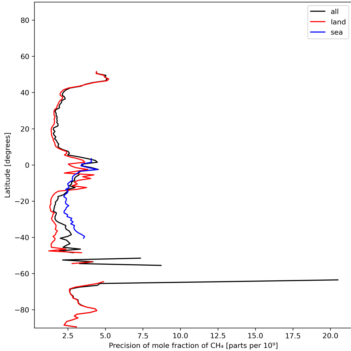
Figure 13: Zonal average of “Precision of mole fraction of CH 4 ” for 2023-12-25 to 2023-12-27.
