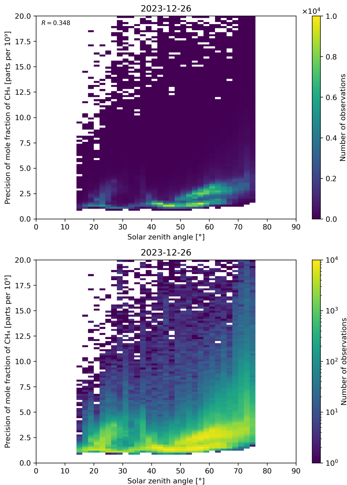
Figure 101: Scatter density plot of “Solar zenith angle” against “Precision of mole fraction of \text{CH}_4 ” for 2023-12-25 to 2023-12-27.
