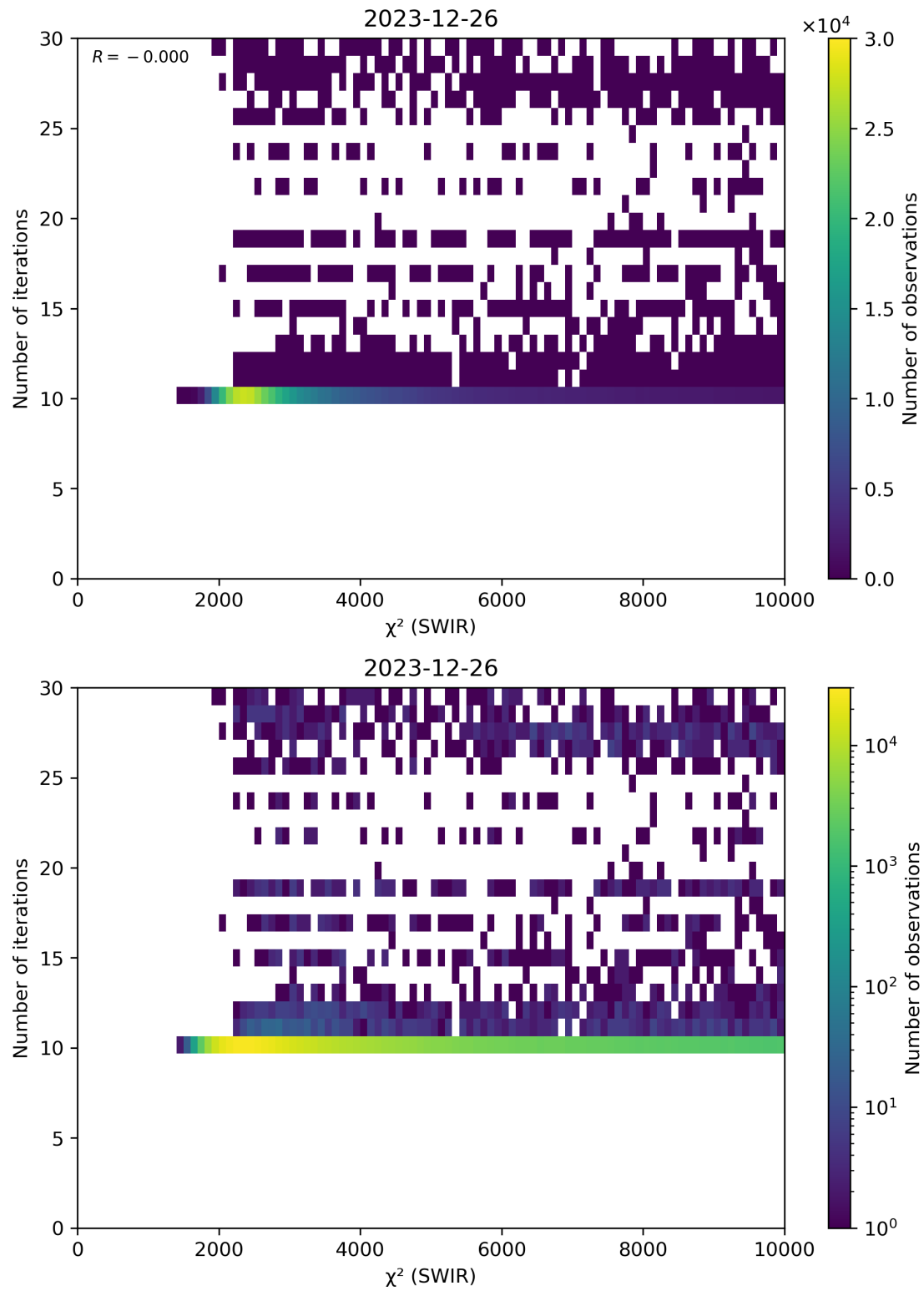
Figure 50: Scatter density plot of “ \chi^2 (SWIR)” against “Number of iterations” for 2023-12-25 to 2023-12-27.
