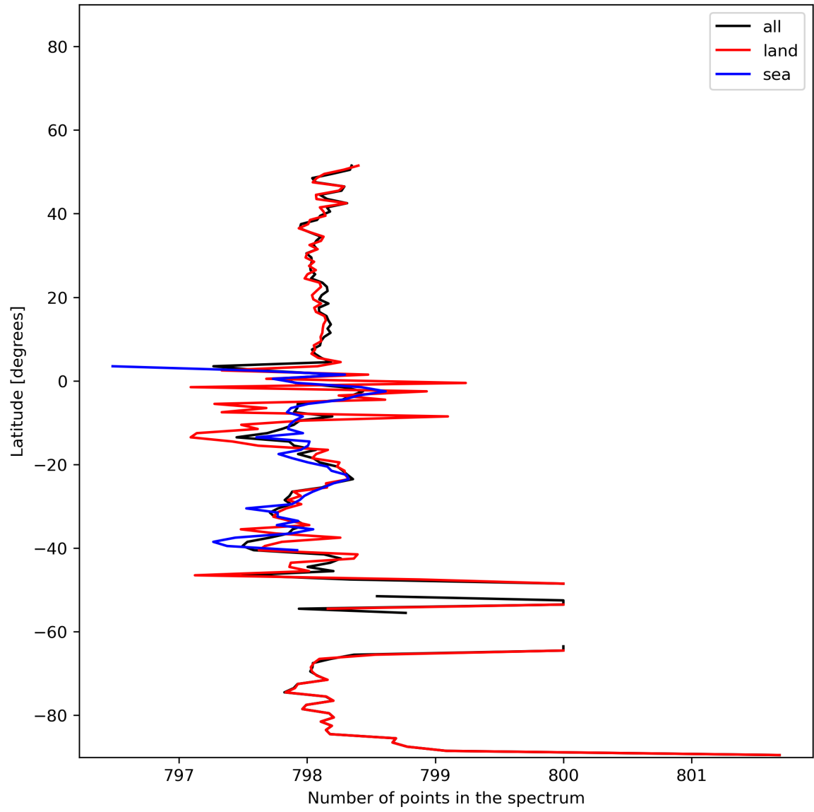
Figure 15: Zonal average of “Number of points in the spectrum” for 2023-12-25 to 2023-12-27.
