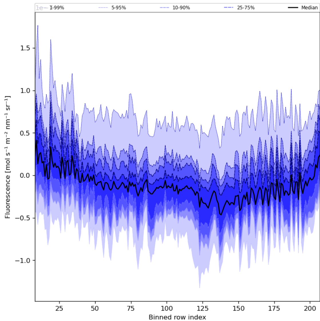
Figure 43: Along track statistics of “Fluorescence” for 2023-12-25 to 2023-12-27
