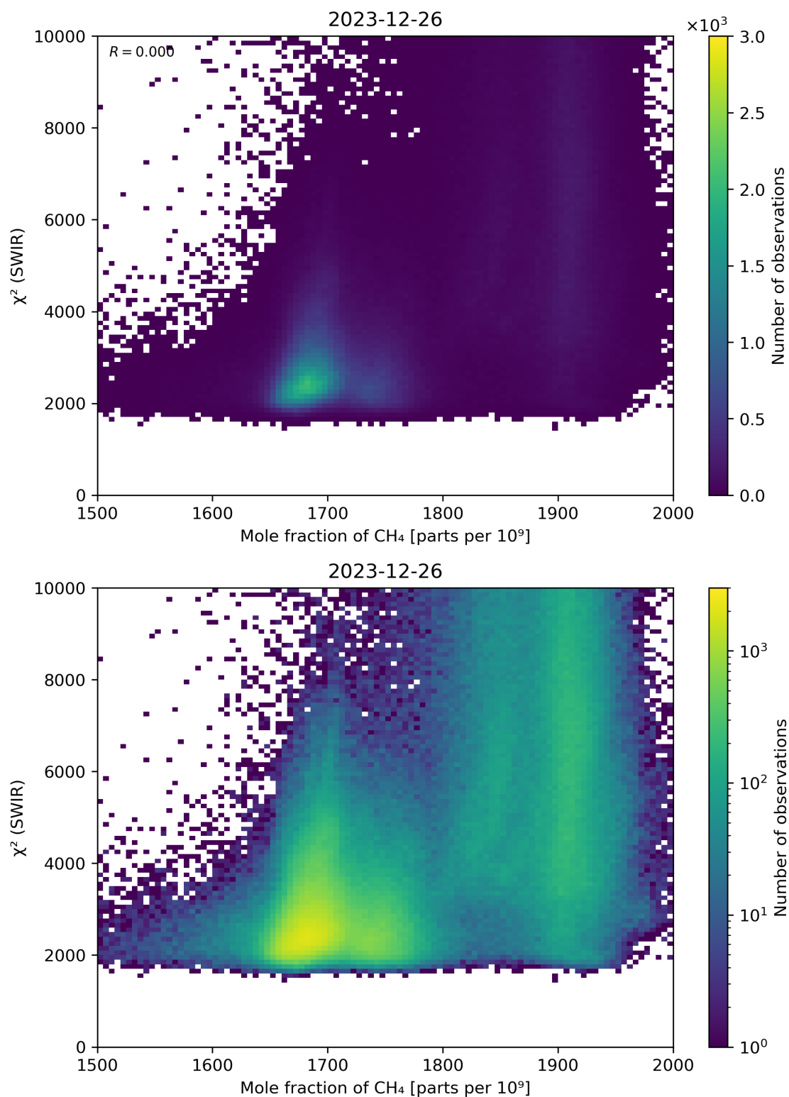
Figure 71: Scatter density plot of “Mole fraction of \text{CH}_4 ” against “ \chi^2 (SWIR)” for 2023-12-25 to 2023-12-27.
