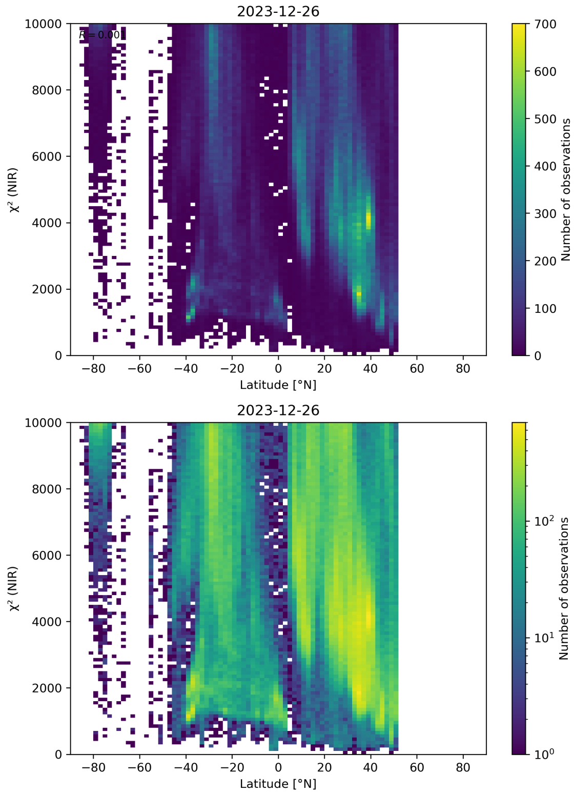
Figure 53: Scatter density plot of “Latitude” against “ \chi^2 (NIR)” for 2023-12-25 to 2023-12-27.
