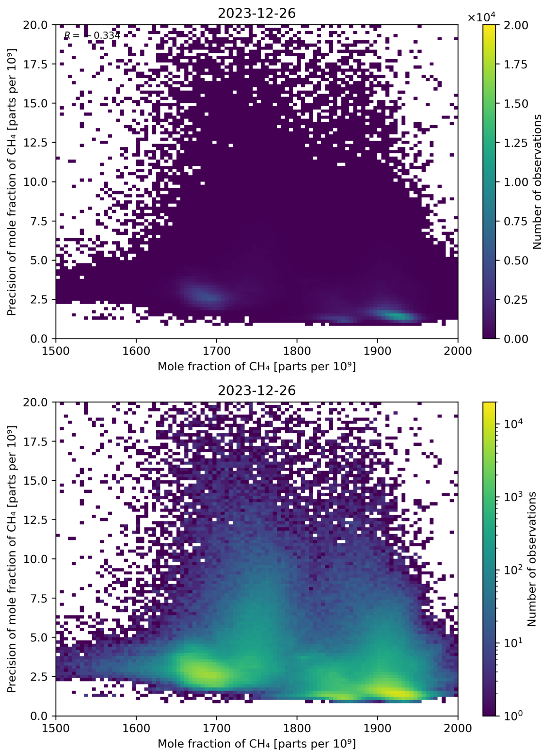
Figure 75: Scatter density plot of “Mole fraction of CH 4 ” against “Precision of mole fraction of CH 4 ” for 2023-12-25 to 2023-12-27.
