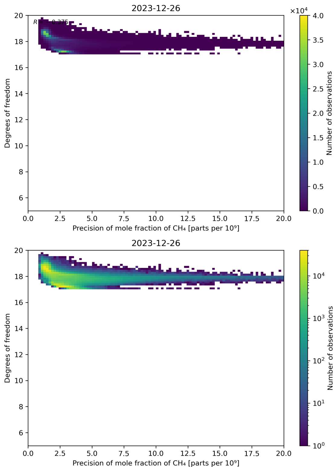
Figure 80: Scatter density plot of “Precision of mole fraction of CH 4 ” against “Degrees of freedom” for 2023-12-25 to 2023-12-27.
