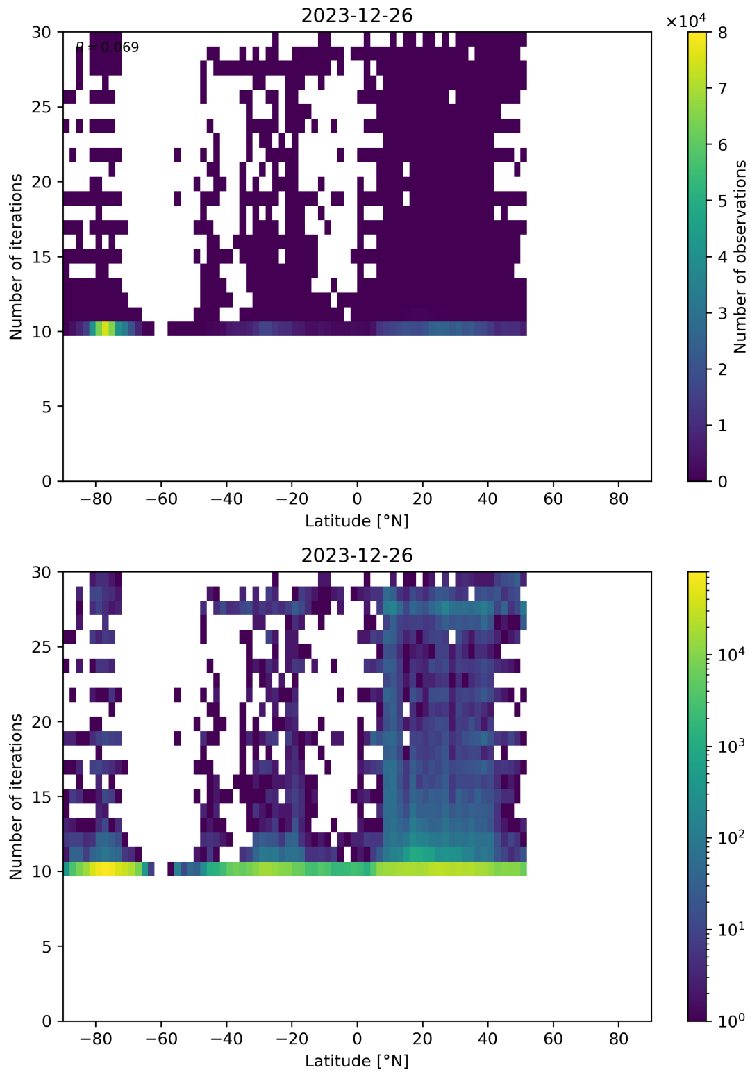
Figure 60: Scatter density plot of “Latitude” against “Number of iterations” for 2023-12-25 to 2023-12-27.
