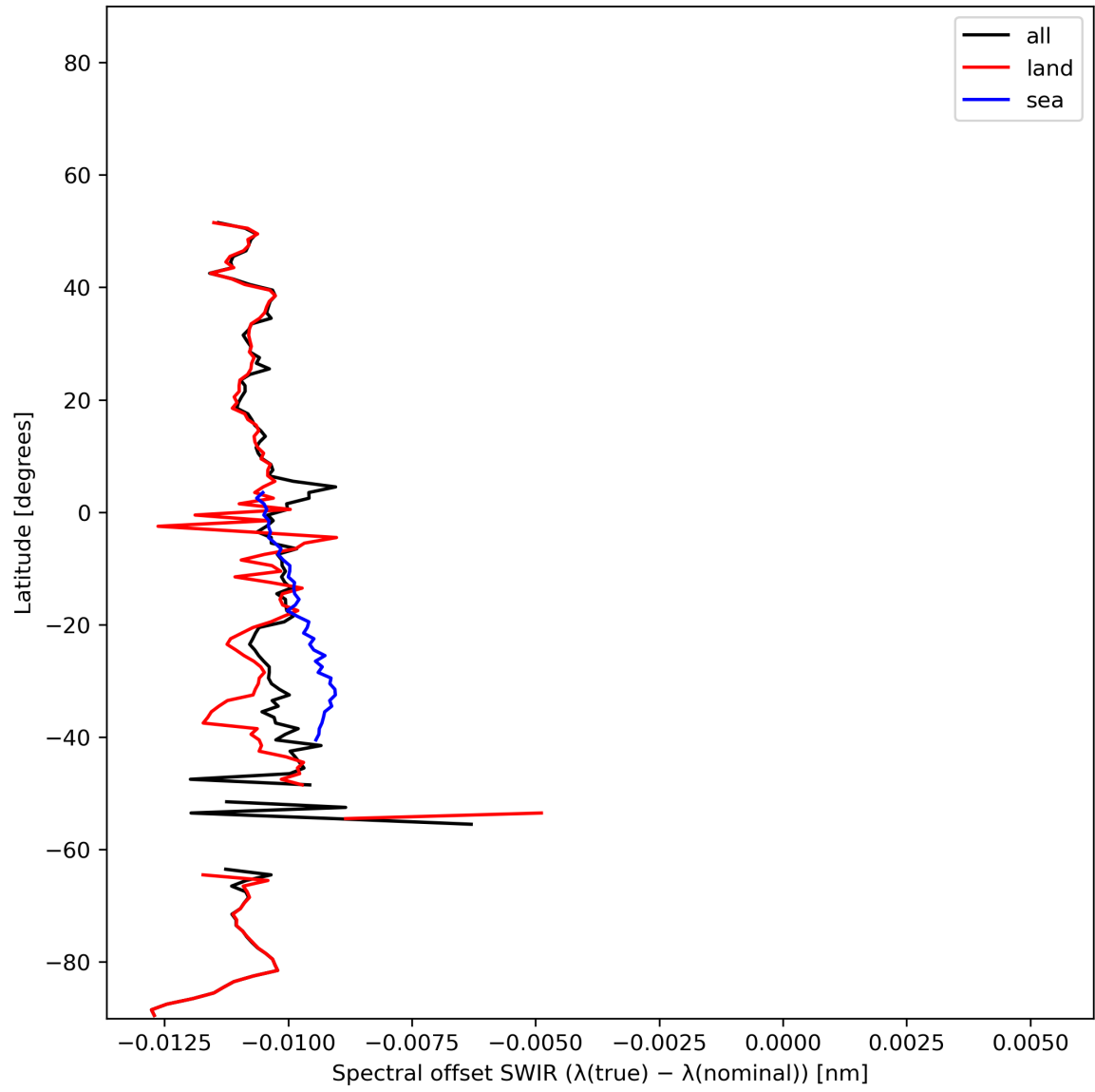
Figure 16: Zonal average of “Spectral offset SWIR ( \lambda(\text{true}) - \lambda(\text{nominal}) )” for 2023-12-25 to 2023-12-27.
