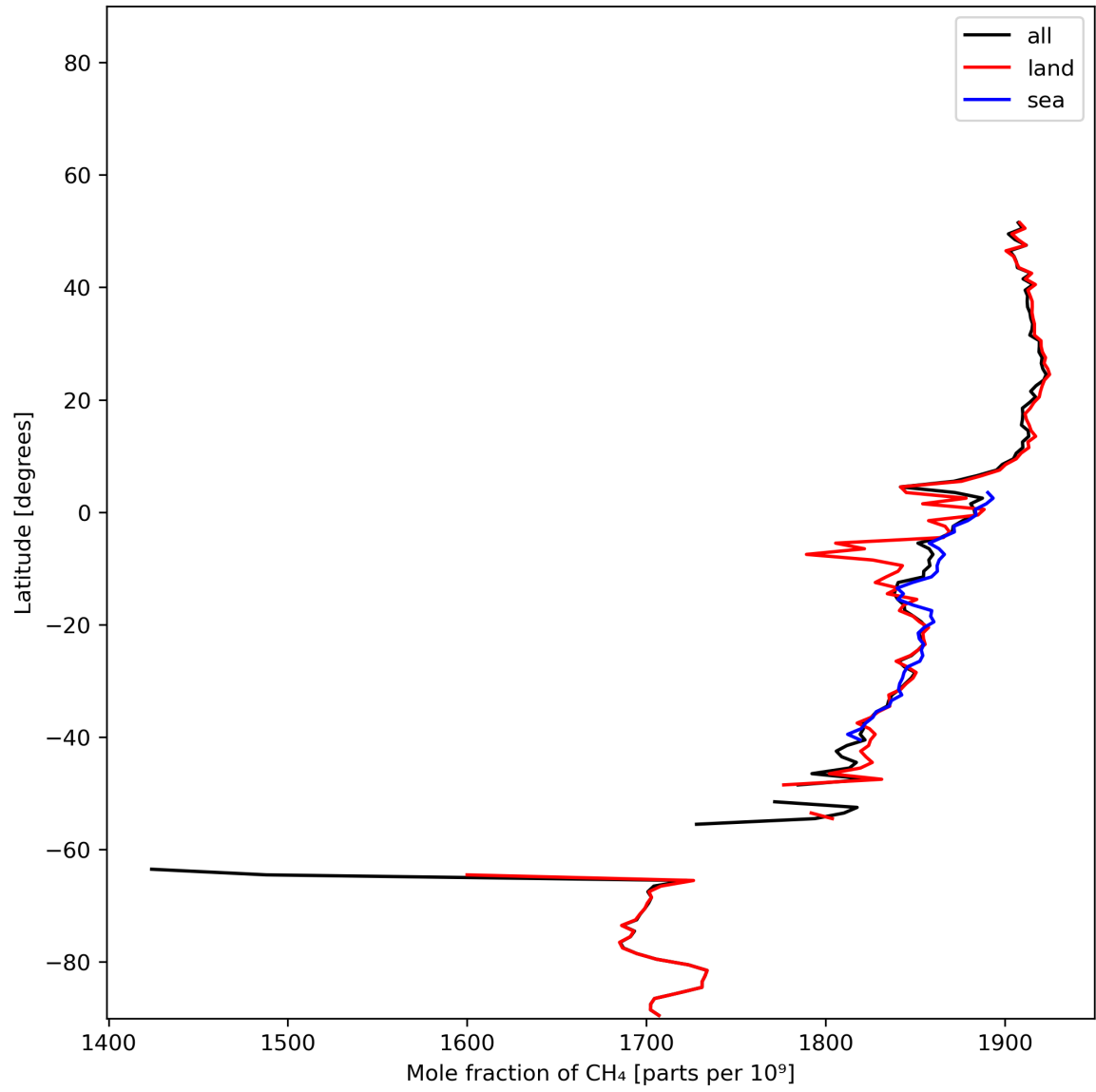
Figure 12: Zonal average of “Mole fraction of \text{CH}_4 ” for 2023-12-25 to 2023-12-27.
