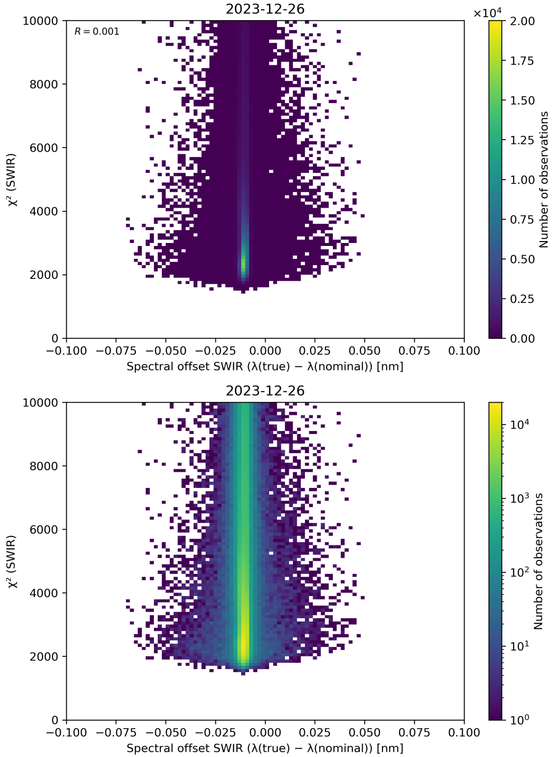
Figure 118: Scatter density plot of “Spectral offset SWIR ( \lambda(\text{true}) - \lambda(\text{nominal}) )” against “ \chi^2 (SWIR)” for 2023-12-25 to 2023-12-27.
