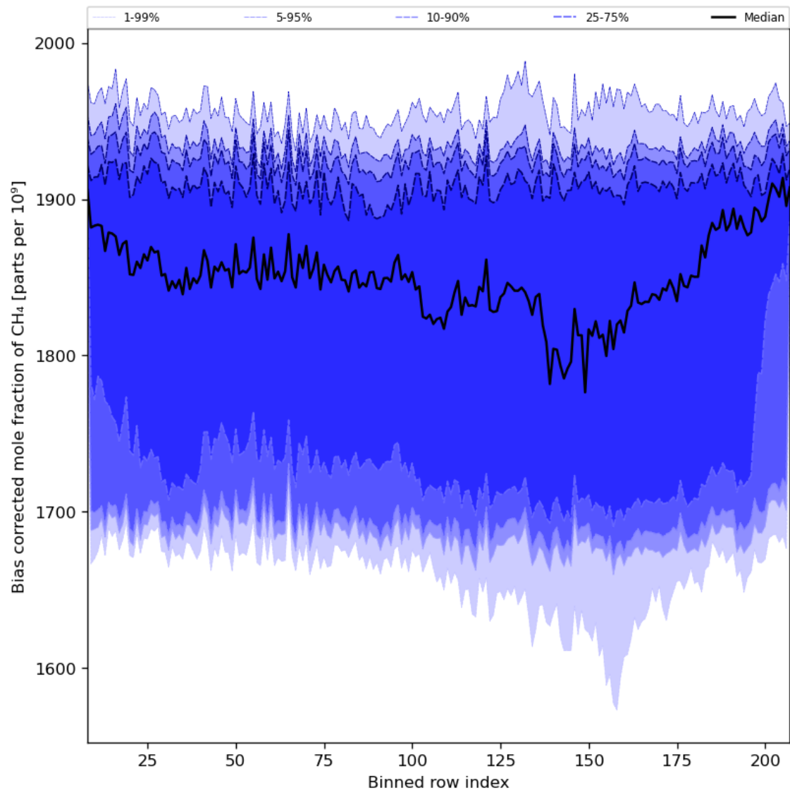
Figure 36: Along track statistics of “Bias corrected mole fraction of CH 4 ” for 2023-12-25 to 2023-12-27
