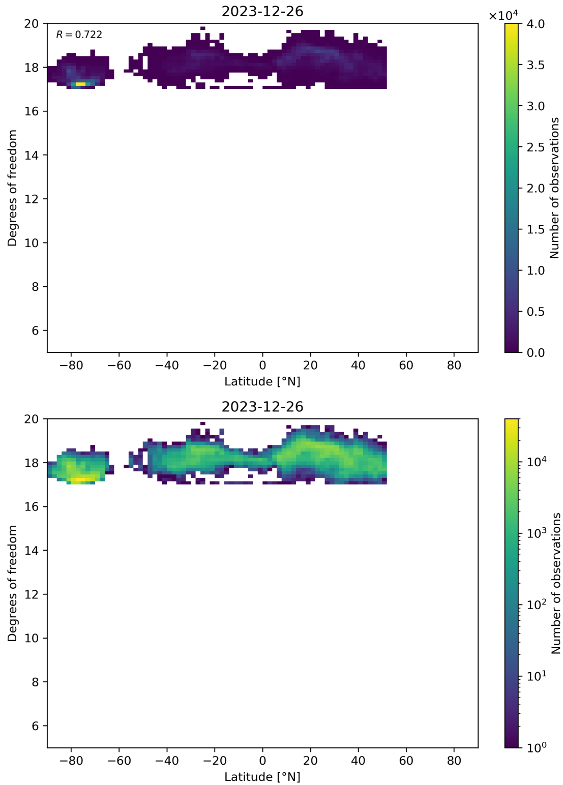
Figure 55: Scatter density plot of “Latitude” against “Degrees of freedom” for 2023-12-25 to 2023-12-27.
