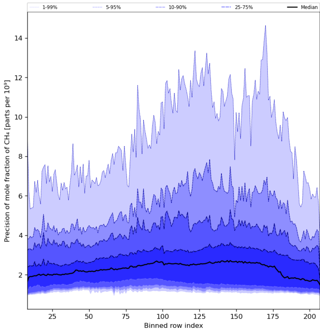
Figure 35: Along track statistics of “Precision of mole fraction of CH 4 ” for 2023-12-25 to 2023-12-27
