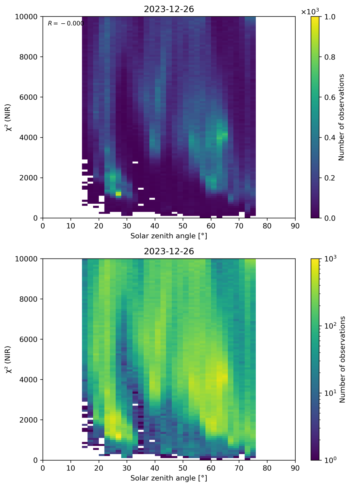
Figure 94: Scatter density plot of “Solar zenith angle” against “ \chi^2 (NIR)” for 2023-12-25 to 2023-12-27.
