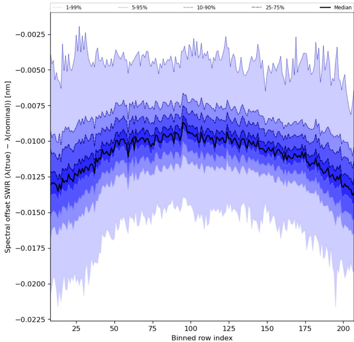
Figure 38: Along track statistics of “Spectral offset SWIR ( \lambda(\text{true}) - \lambda(\text{nominal}) )” for 2023-12-25 to 2023-12-27
