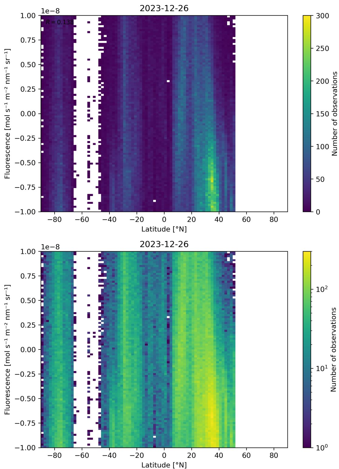
Figure 56: Scatter density plot of “Latitude” against “Fluorescence” for 2023-12-25 to 2023-12-27.
