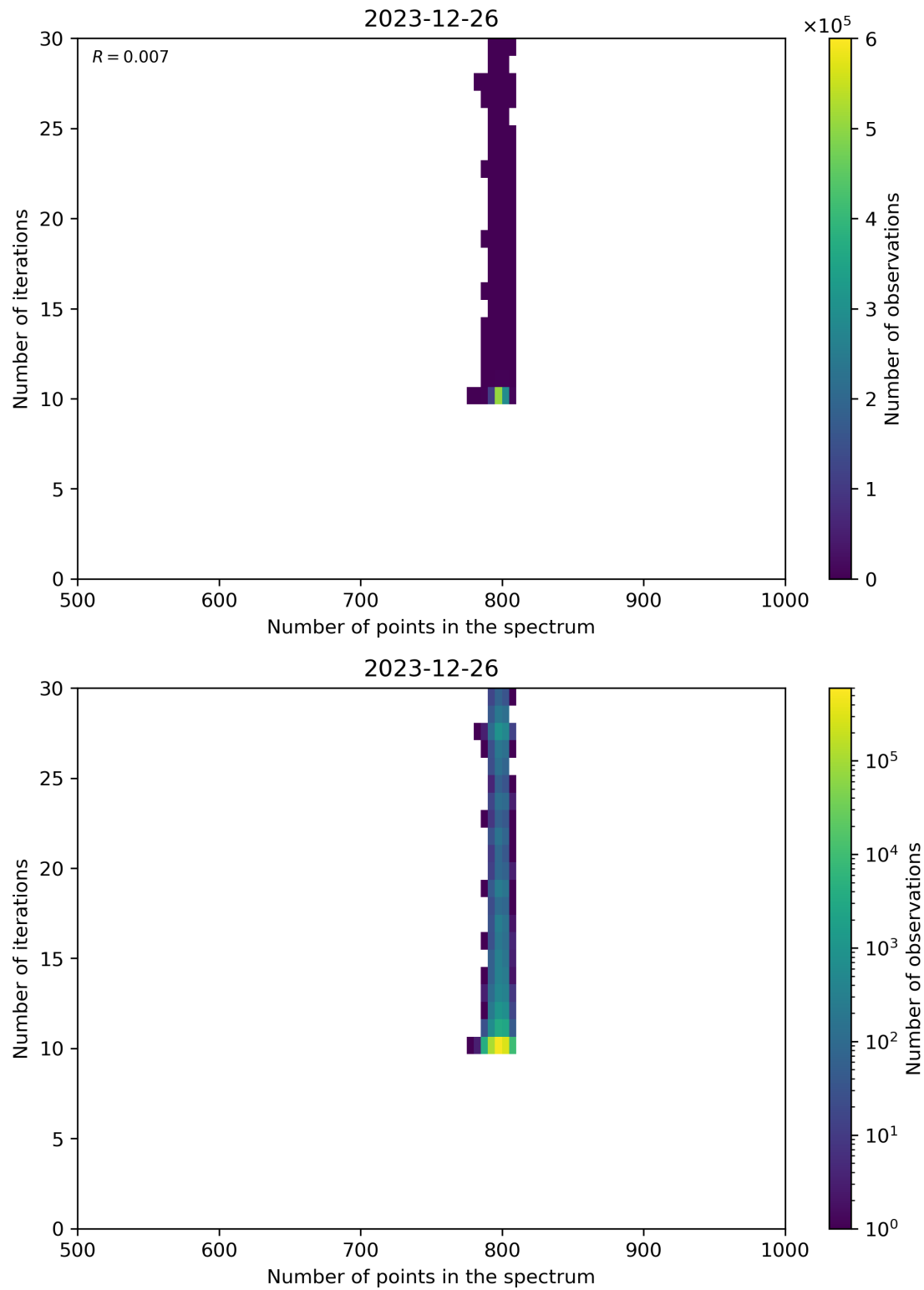
Figure 92: Scatter density plot of “Number of points in the spectrum” against “Number of iterations” for 2023-12-25 to 2023-12-27.
