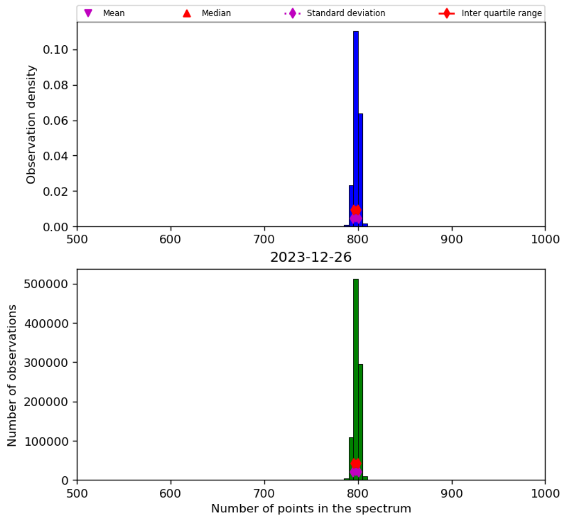
Figure 26: Histogram of “Number of points in the spectrum” for 2023-12-25 to 2023-12-27
