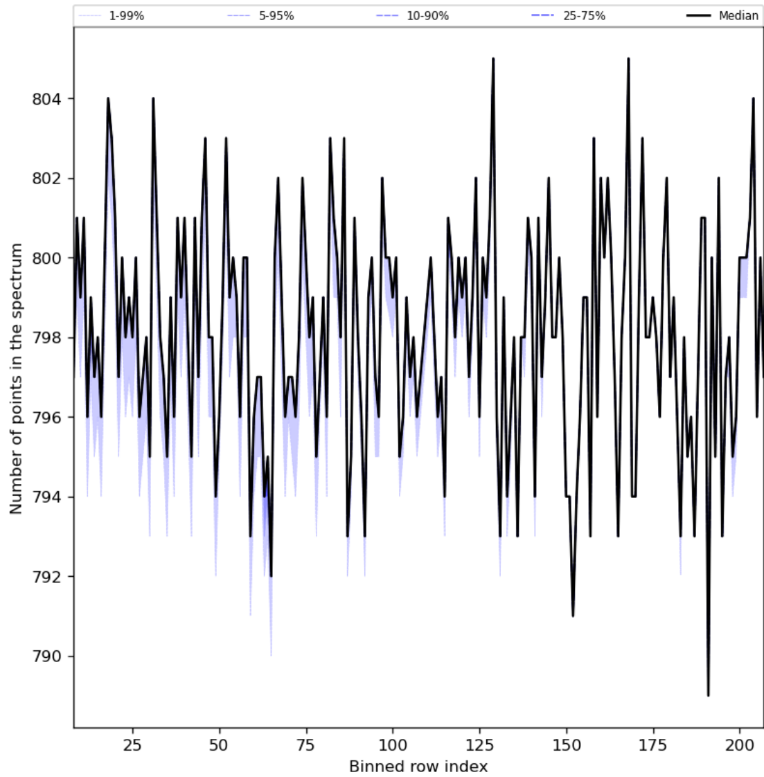
Figure 37: Along track statistics of “Number of points in the spectrum” for 2023-12-25 to 2023-12-27
