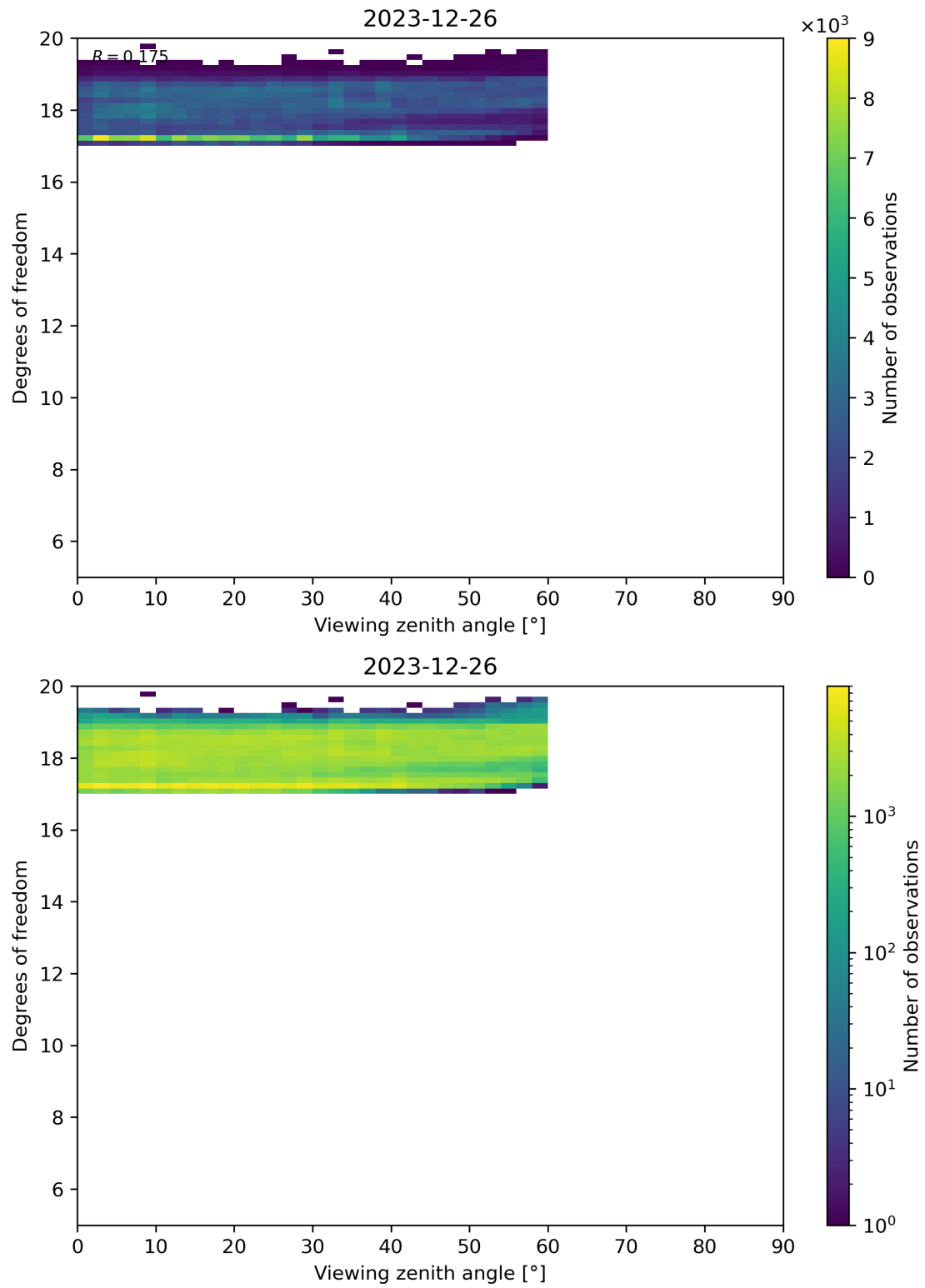
Figure 107: Scatter density plot of “Viewing zenith angle” against “Degrees of freedom” for 2023-12-25 to 2023-12-27.
