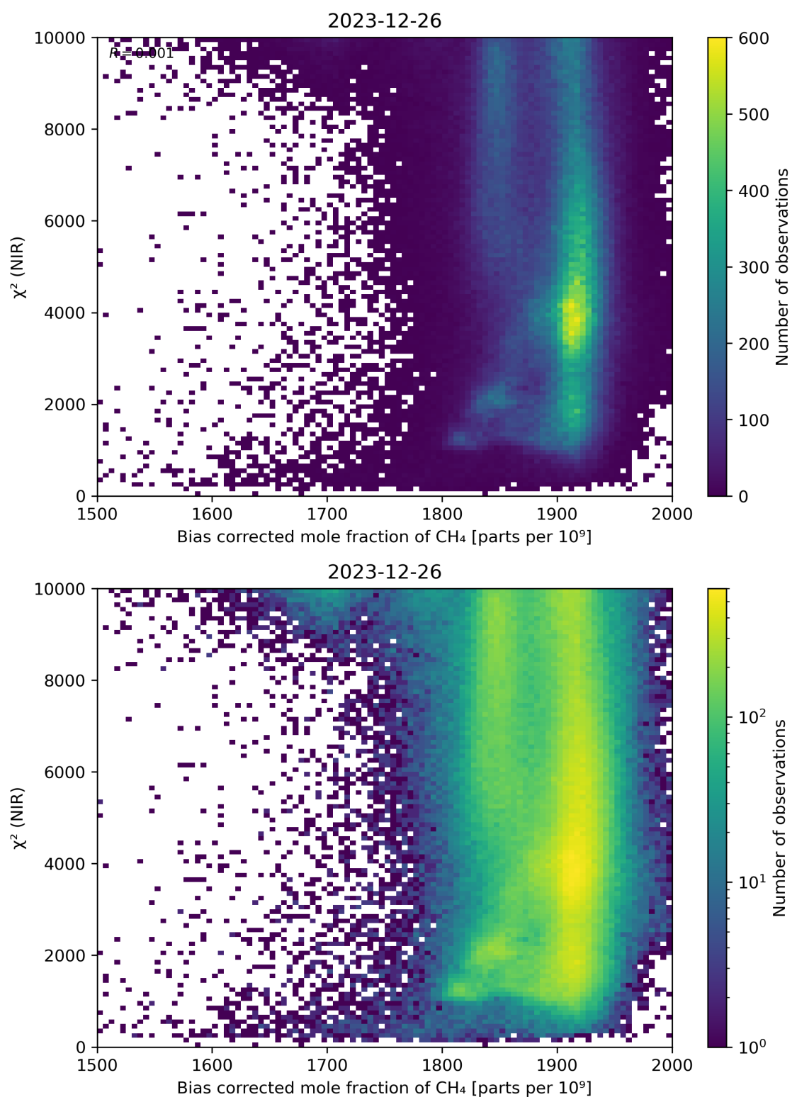
Figure 63: Scatter density plot of “Bias corrected mole fraction of \text{CH}_4 ” against “ \chi^2 (NIR)” for 2023-12-25 to 2023-12-27.
