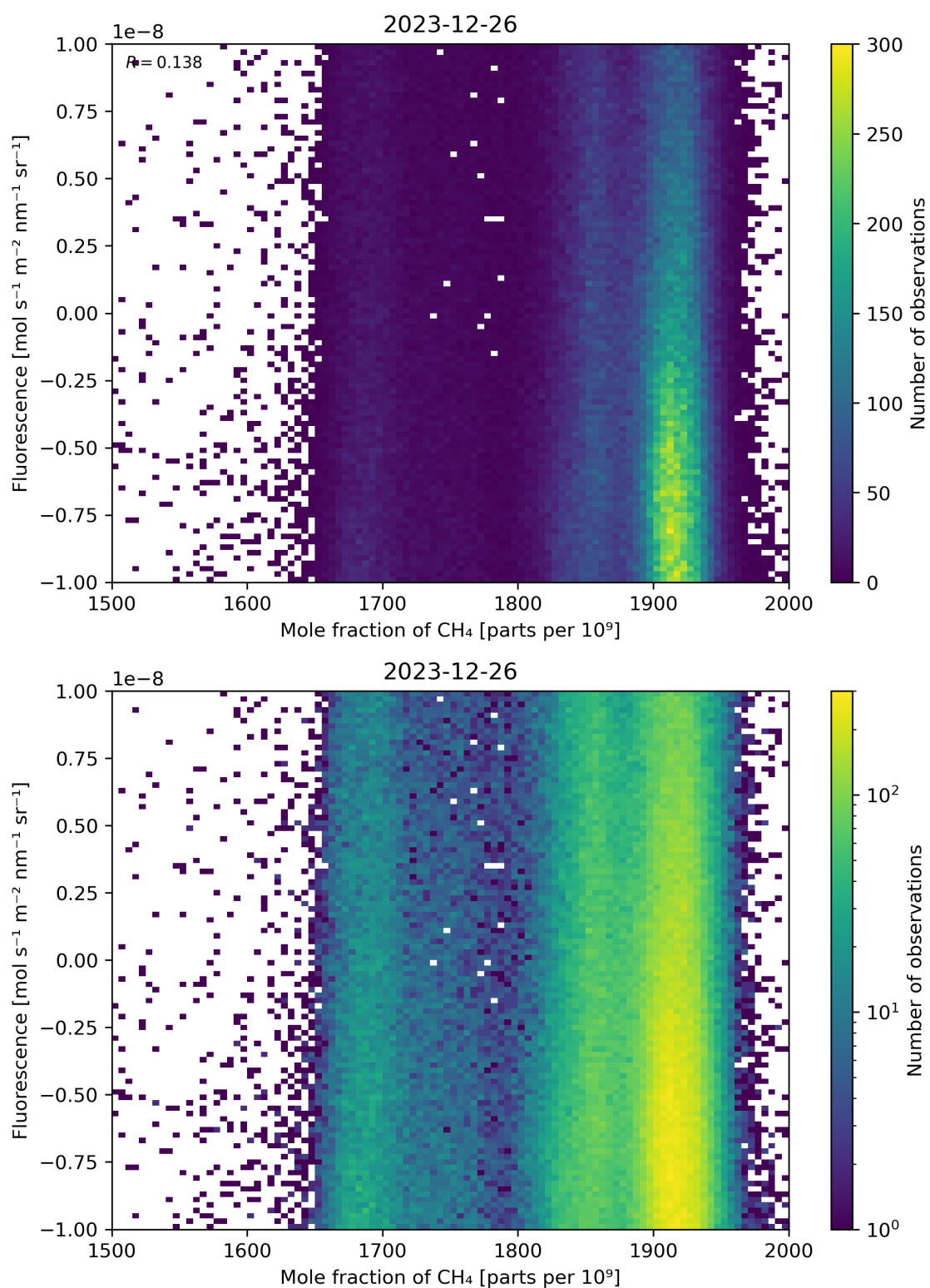
Figure 73: Scatter density plot of “Mole fraction of \text{CH}_4 ” against “Fluorescence” for 2023-12-25 to 2023-12-27.
