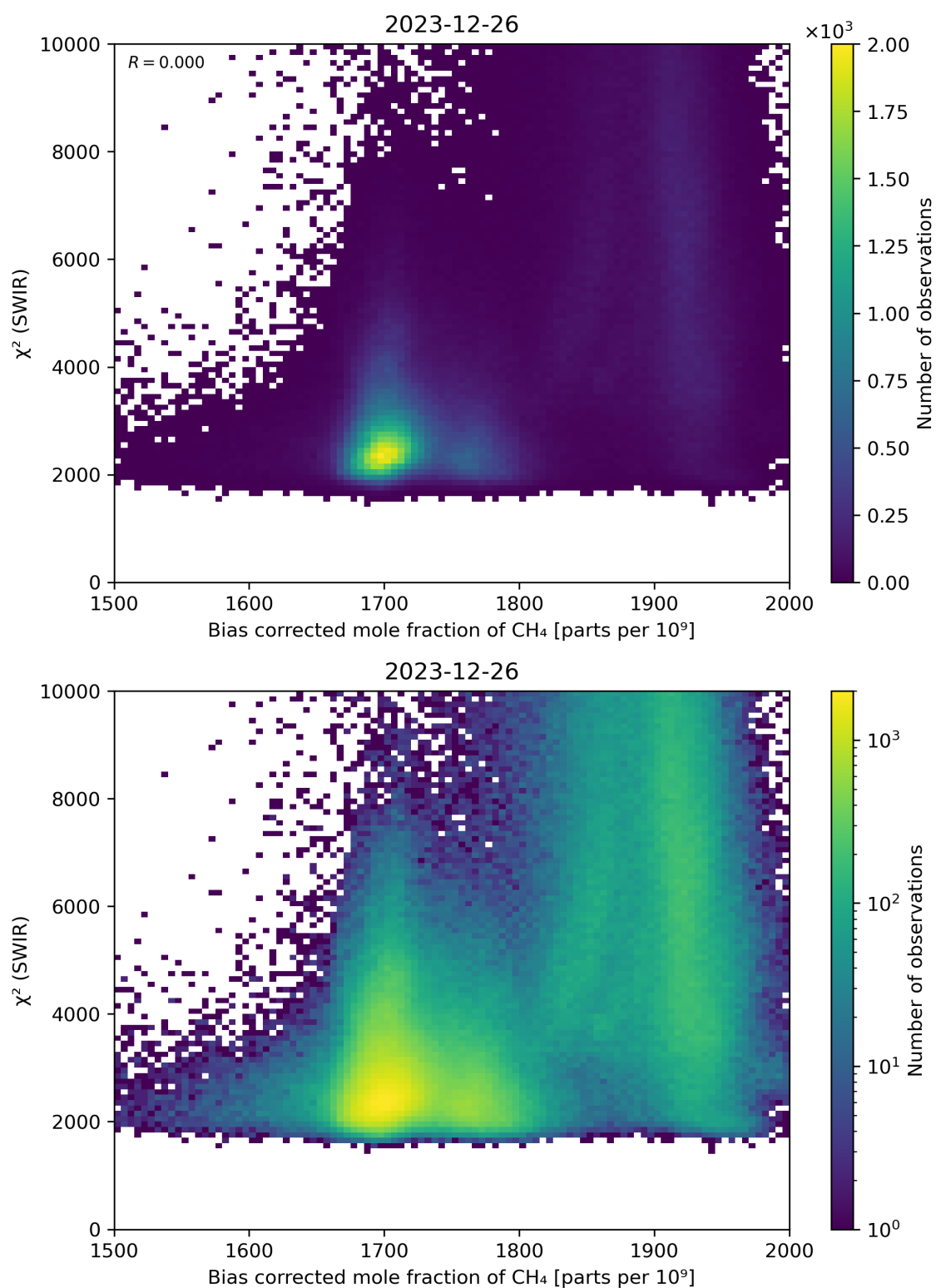
Figure 64: Scatter density plot of “Bias corrected mole fraction of CH 4 ” against “ \chi^2 (SWIR)” for 2023-12-25 to 2023-12-27.
