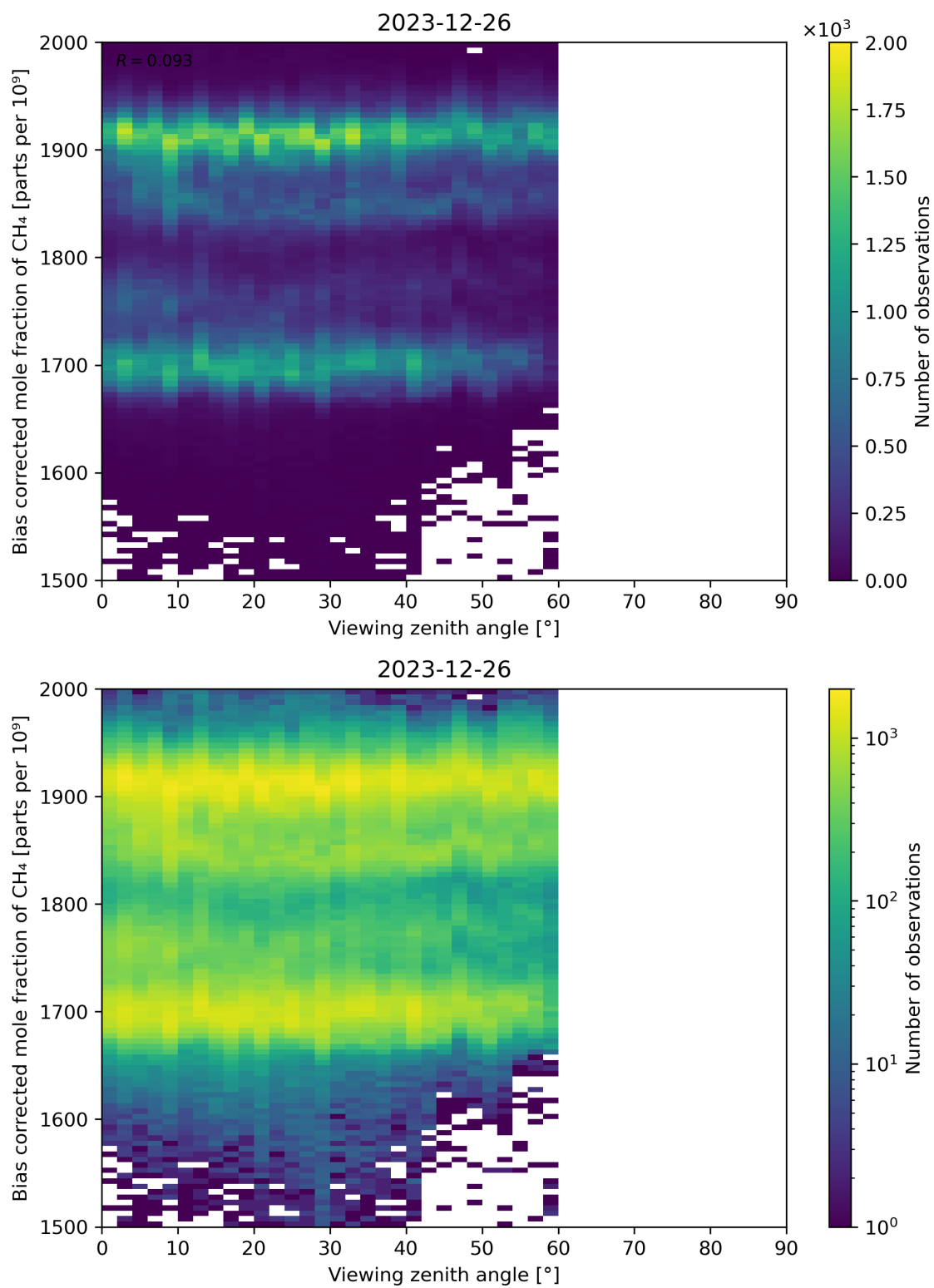
Figure 111: Scatter density plot of “Viewing zenith angle” against “Bias corrected mole fraction of CH 4 ” for 2023-12-25 to 2023-12-27.
