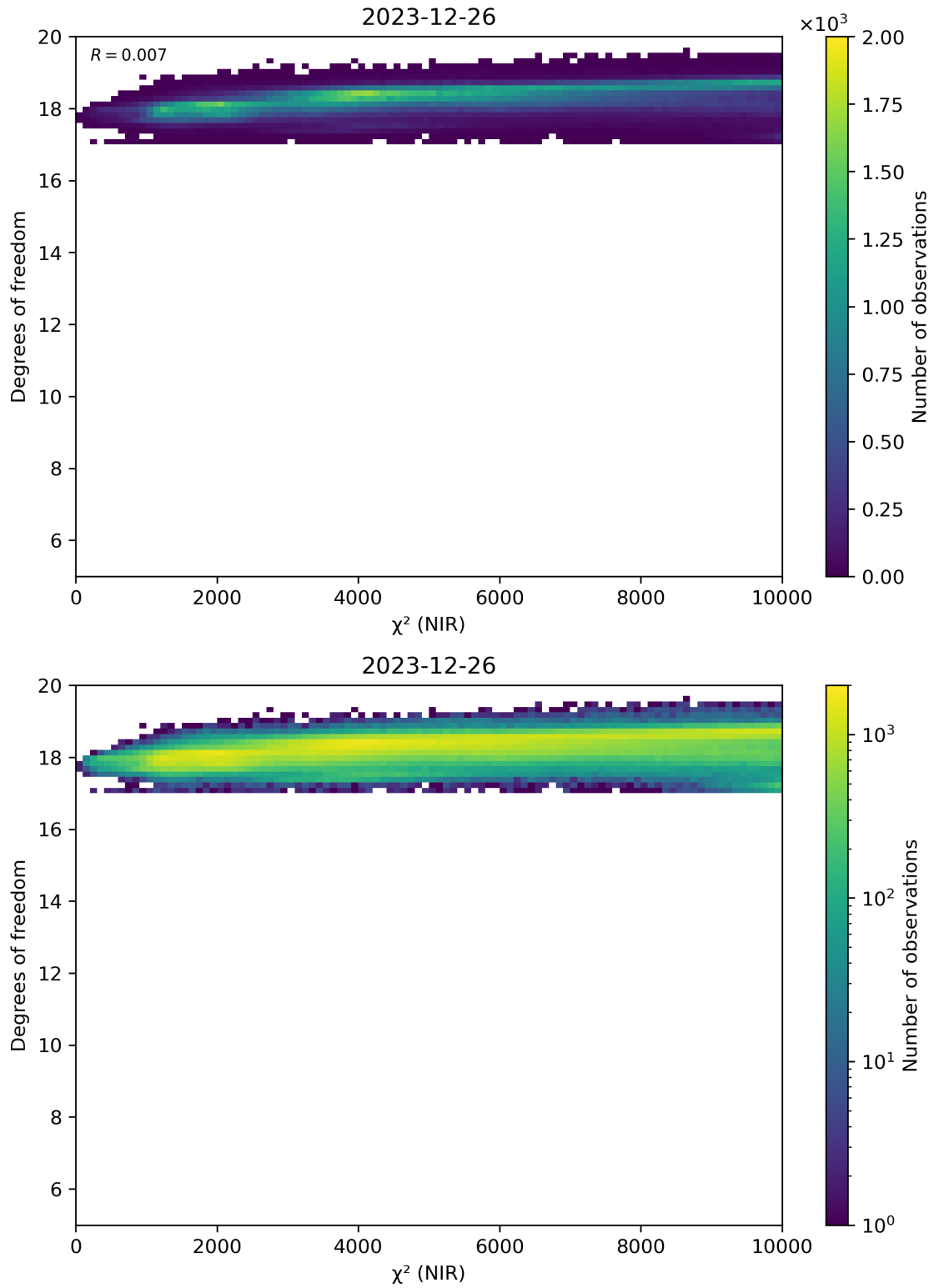
Figure 44: Scatter density plot of “ \chi^2 (NIR)” against “Degrees of freedom” for 2023-12-25 to 2023-12-27.
