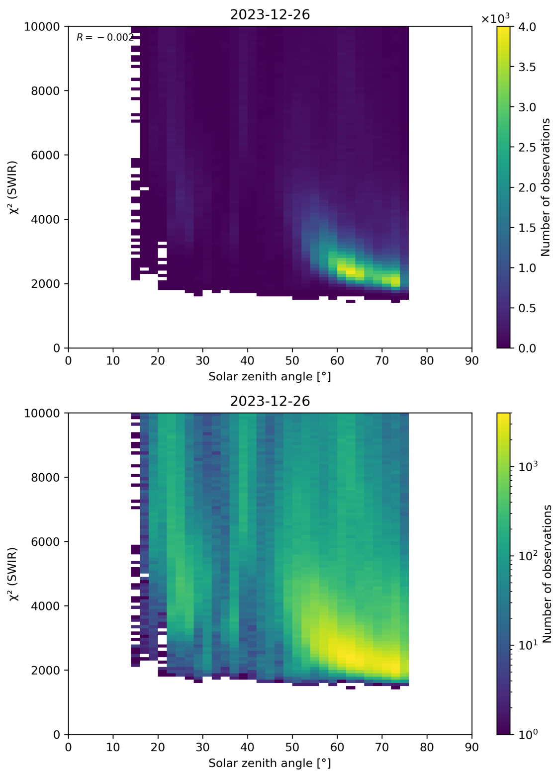
Figure 95: Scatter density plot of “Solar zenith angle” against “ \chi^2 (SWIR)” for 2023-12-25 to 2023-12-27.
