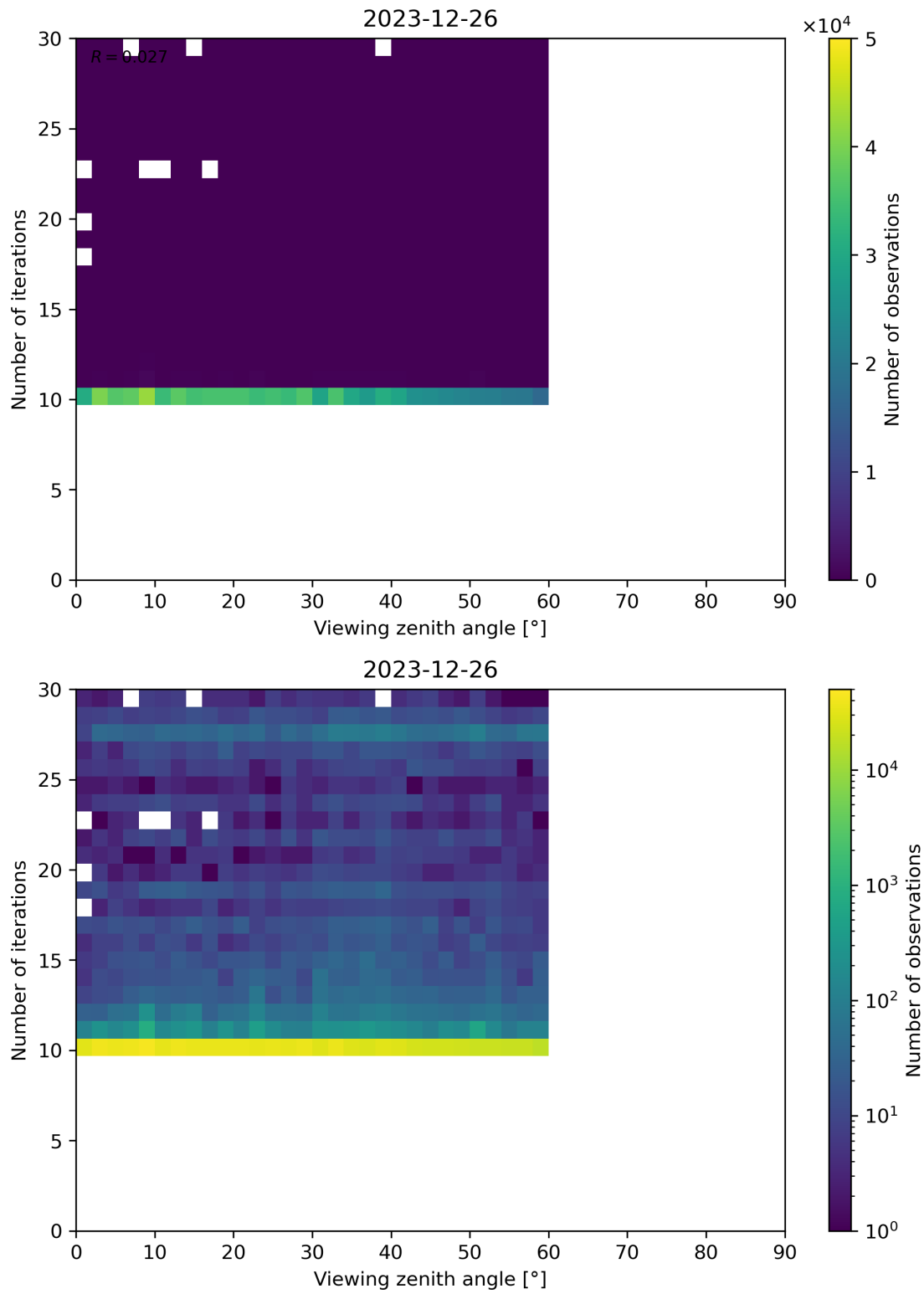
Figure 113: Scatter density plot of “Viewing zenith angle” against “Number of iterations” for 2023-12-25 to 2023-12-27.
