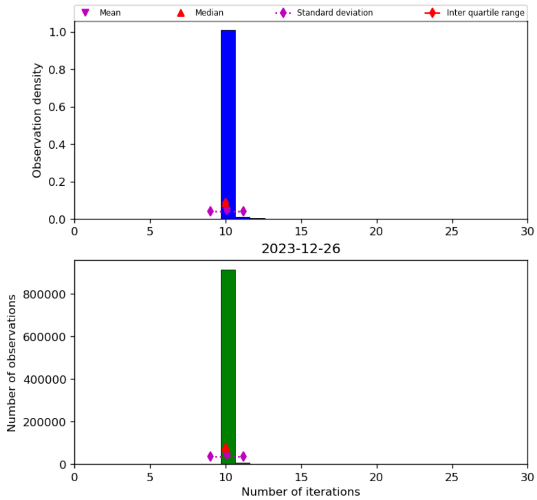
Figure 31: Histogram of “Number of iterations” for 2023-12-25 to 2023-12-27
