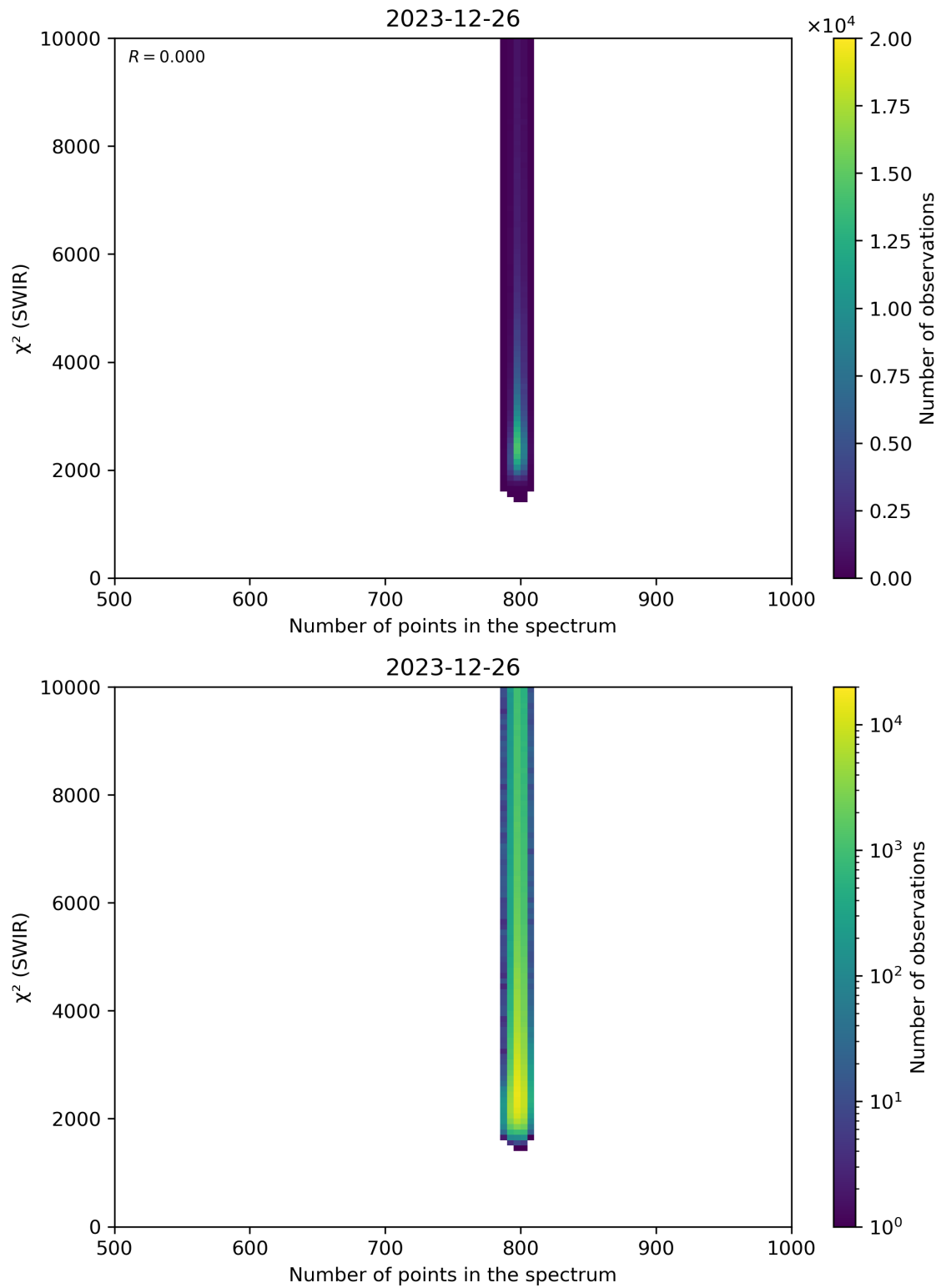
Figure 89: Scatter density plot of “Number of points in the spectrum” against “ \chi^2 (SWIR)” for 2023-12-25 to 2023-12-27.
