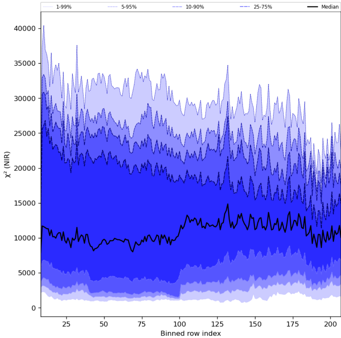
Figure 40: Along track statistics of “ \chi^2 (NIR)” for 2023-12-25 to 2023-12-27
