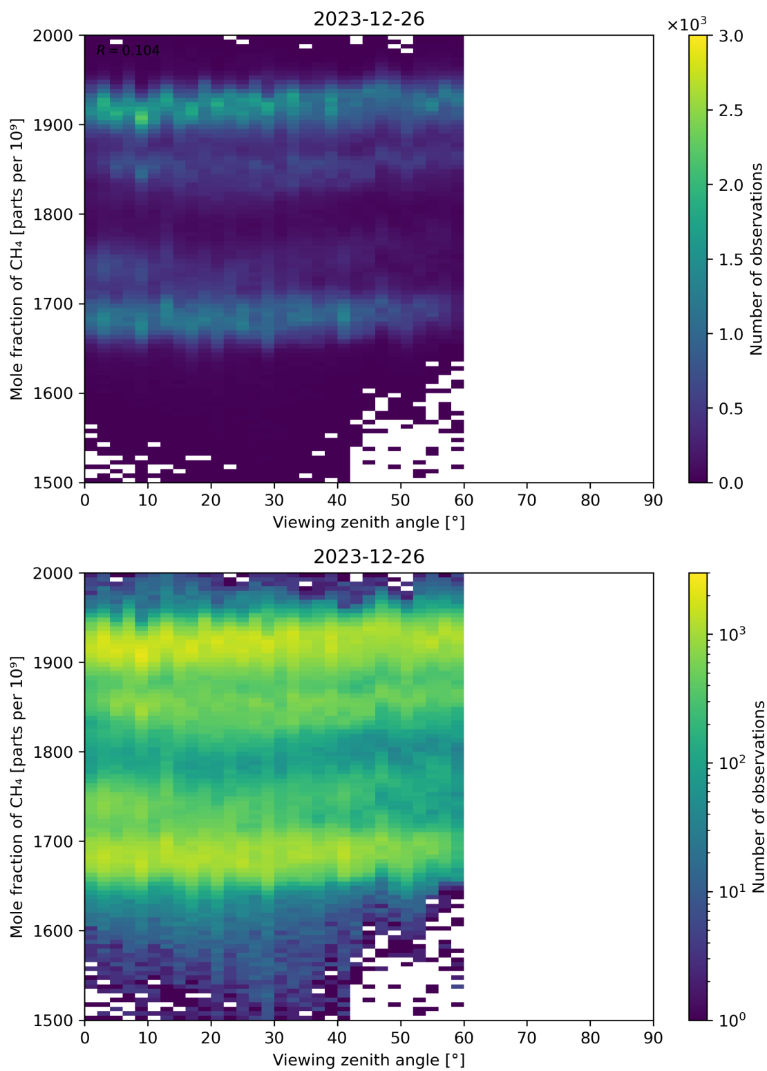
Figure 110: Scatter density plot of “Viewing zenith angle” against “Mole fraction of CH 4 ” for 2023-12-25 to 2023-12-27.
