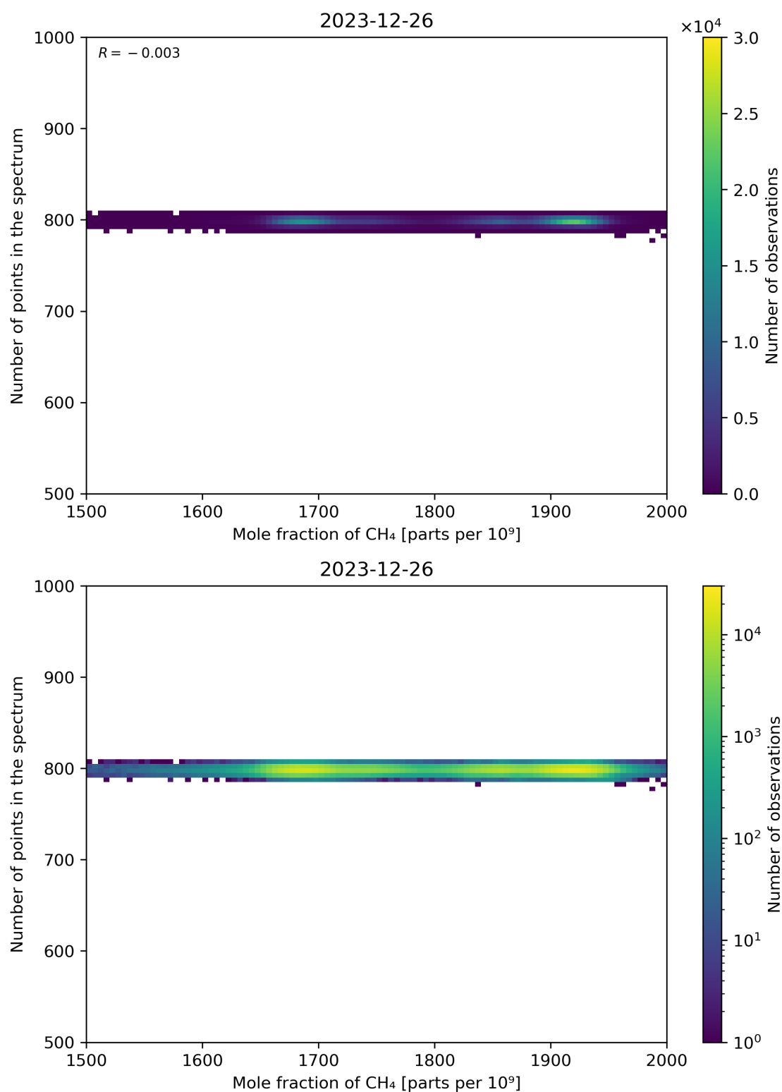
Figure 77: Scatter density plot of “Mole fraction of CH 4 ” against “Number of points in the spectrum” for 2023-12-25 to 2023-12-27.
