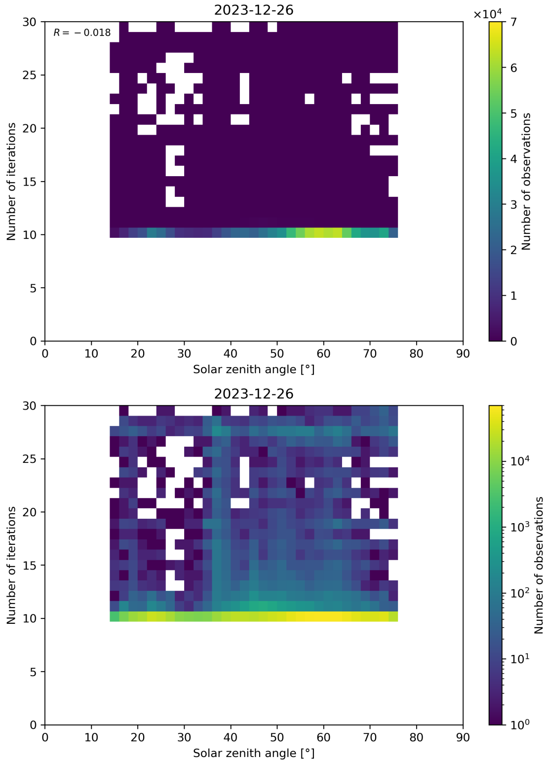
Figure 102: Scatter density plot of “Solar zenith angle” against “Number of iterations” for 2023-12-25 to 2023-12-27.
