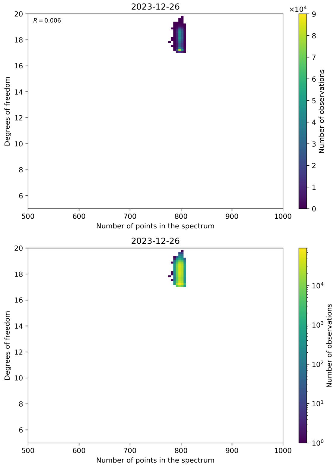
Figure 90: Scatter density plot of “Number of points in the spectrum” against “Degrees of freedom” for 2023-12-25 to 2023-12-27.
