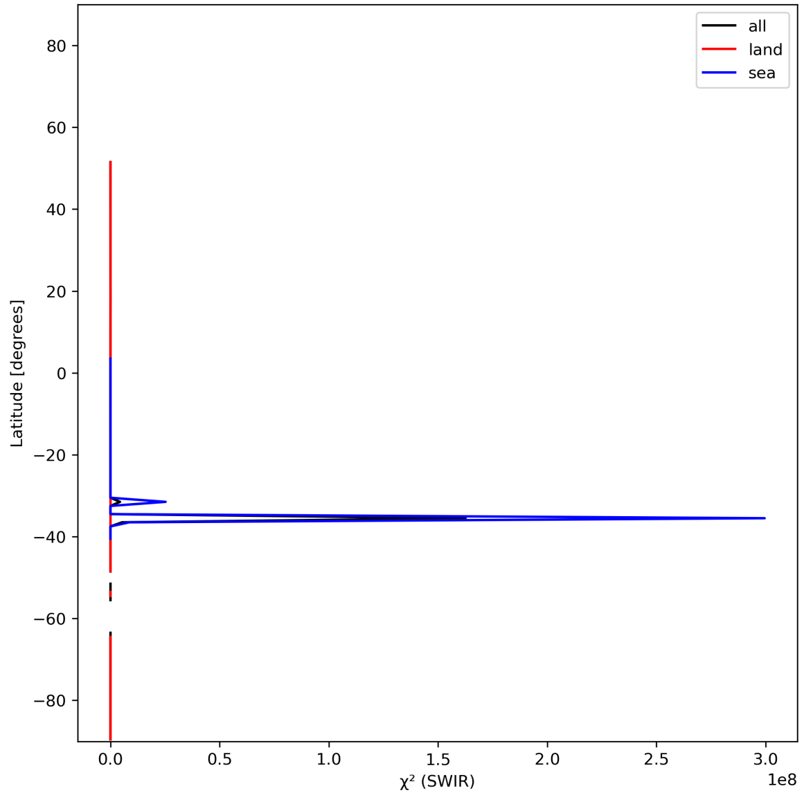
Figure 17: Zonal average of “ \chi^2 (SWIR)” for 2023-12-25 to 2023-12-27.
