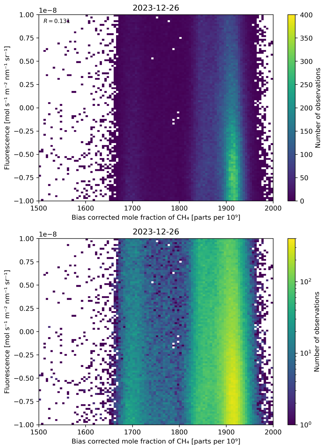
Figure 66: Scatter density plot of “Bias corrected mole fraction of \text{CH}_4 ” against “Fluorescence” for 2023-12-25 to 2023-12-27.
