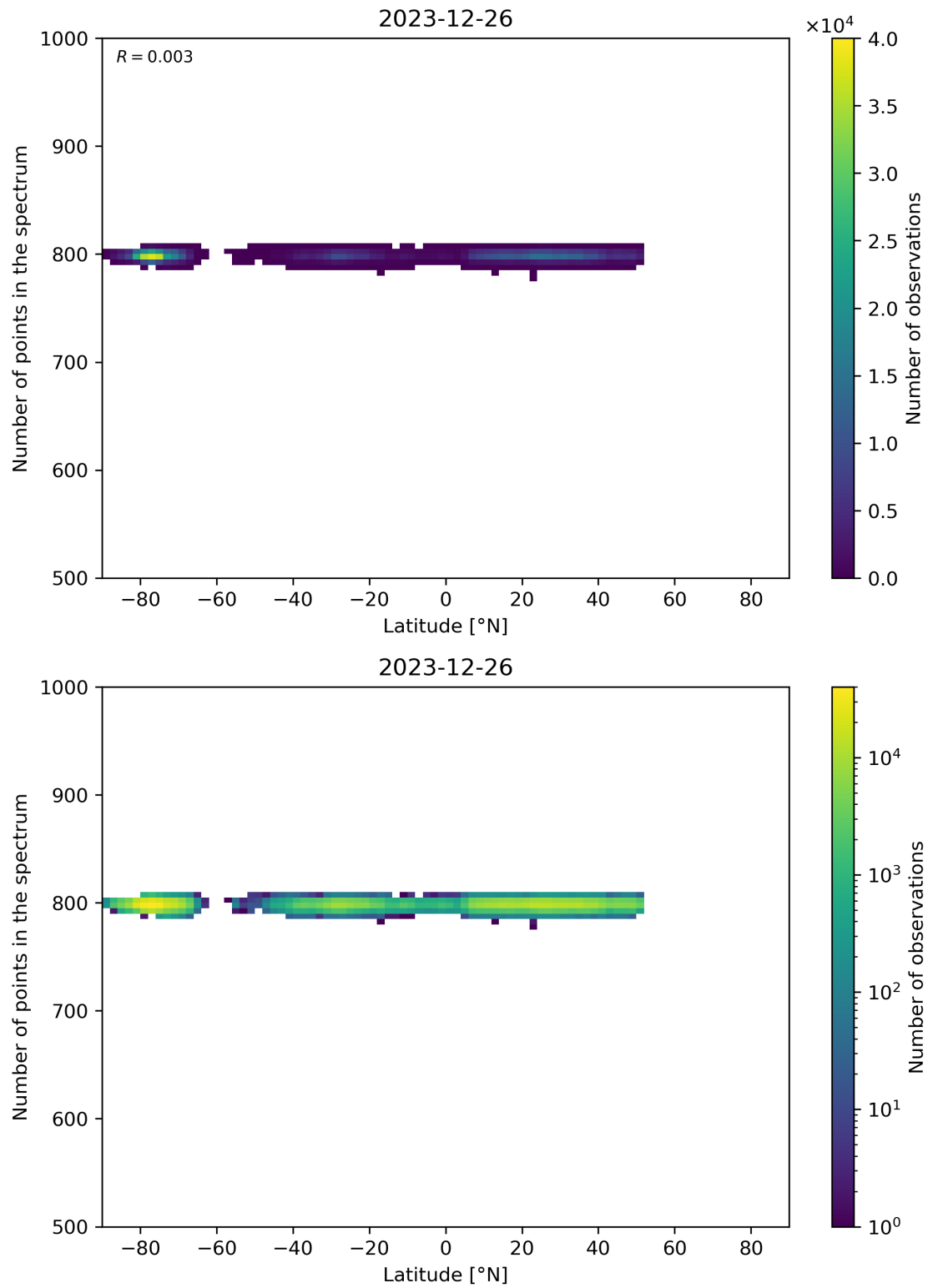
Figure 61: Scatter density plot of “Latitude” against “Number of points in the spectrum” for 2023-12-25 to 2023-12-27.
