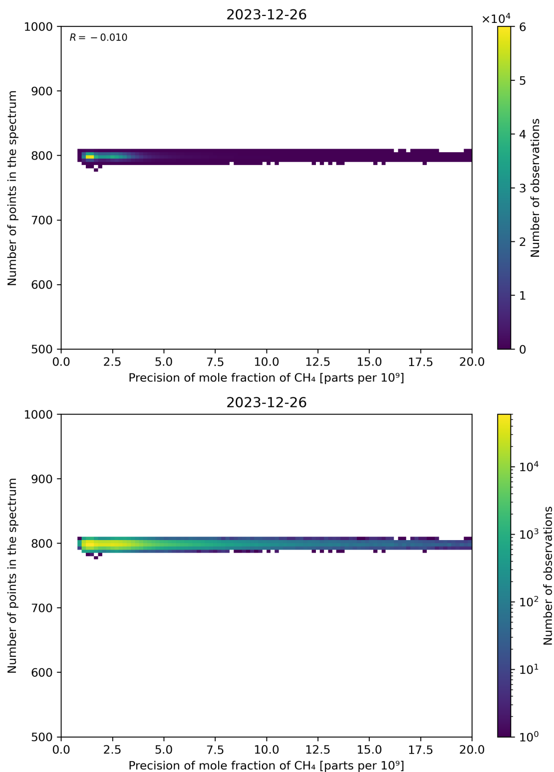
Figure 84: Scatter density plot of “Precision of mole fraction of CH 4 ” against “Number of points in the spectrum” for 2023-12-25 to 2023-12-27.
