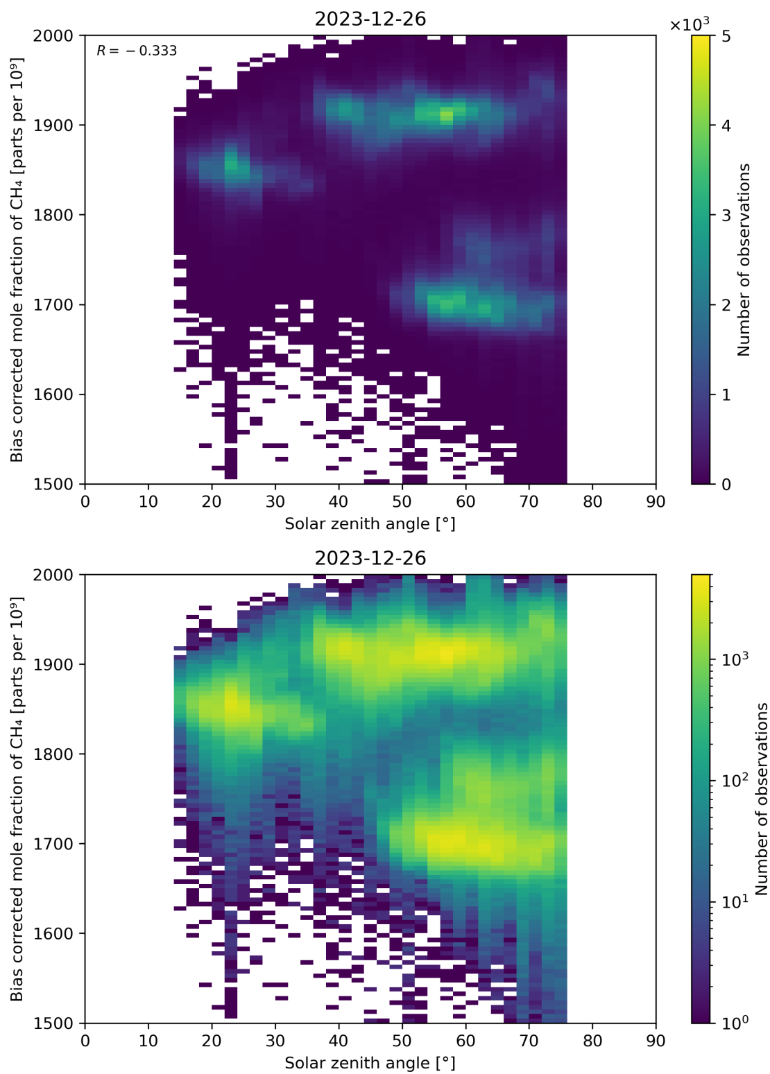
Figure 100: Scatter density plot of “Solar zenith angle” against “Bias corrected mole fraction of CH 4 ” for 2023-12-25 to 2023-12-27.
