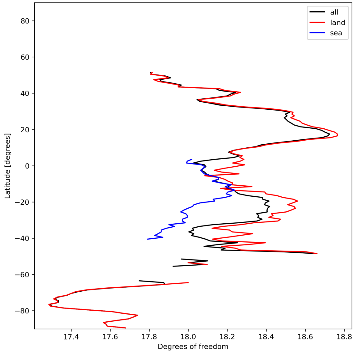
Figure 19: Zonal average of “Degrees of freedom” for 2023-12-25 to 2023-12-27.
