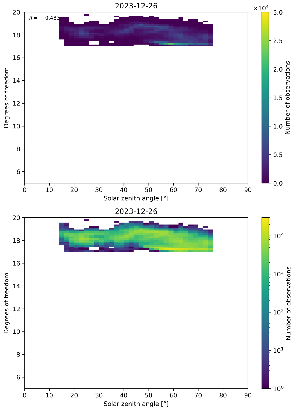
Figure 96: Scatter density plot of “Solar zenith angle” against “Degrees of freedom” for 2023-12-25 to 2023-12-27.
