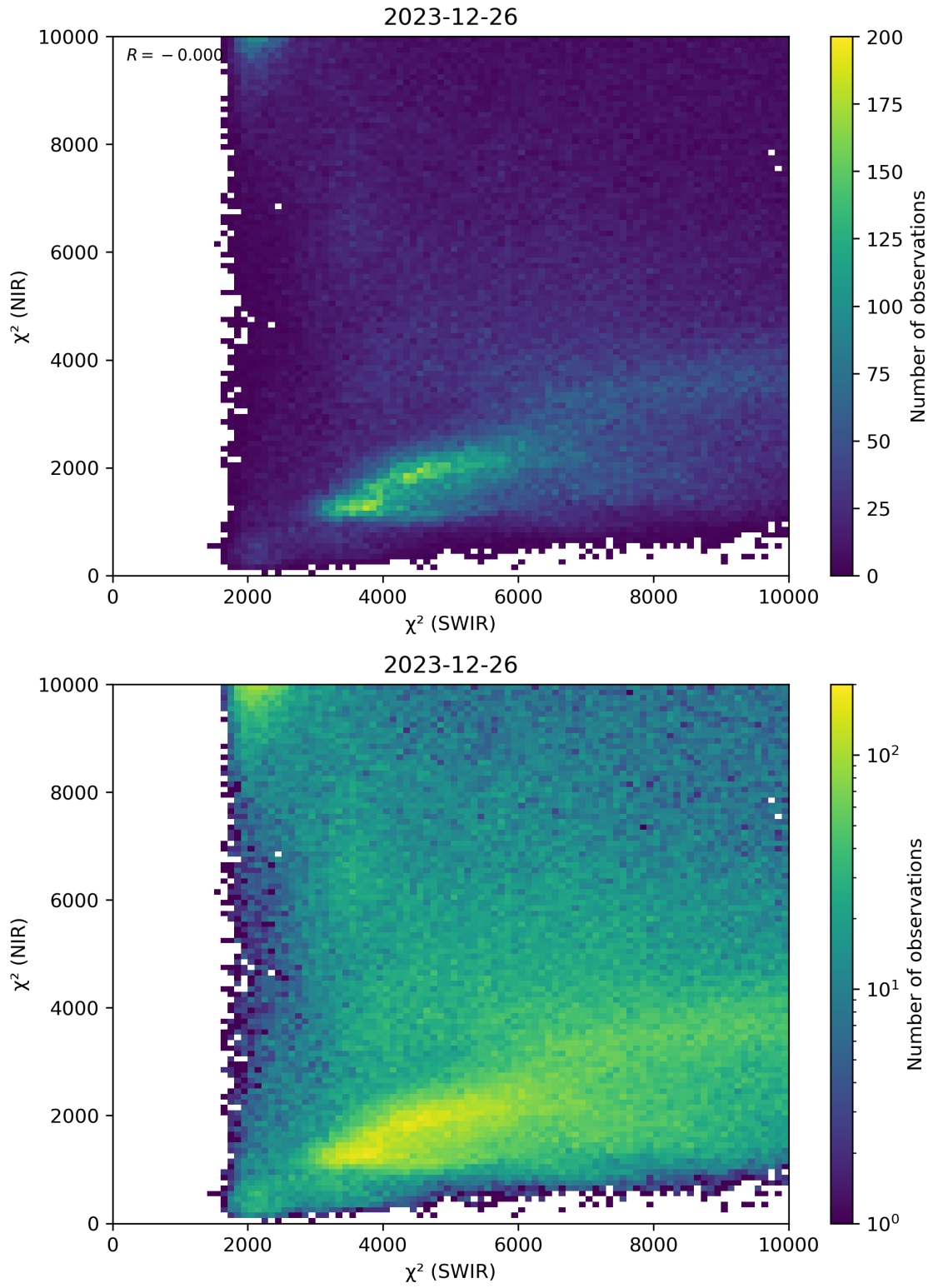
Figure 47: Scatter density plot of “ \chi^2 (SWIR)” against “ \chi^2 (NIR)” for 2023-12-25 to 2023-12-27.
