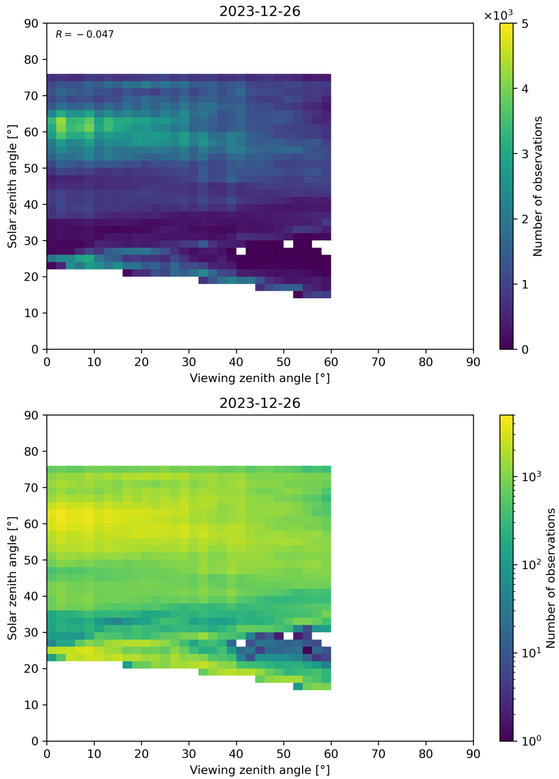
Figure 115: Scatter density plot of “Viewing zenith angle” against “Solar zenith angle” for 2023-12-25 to 2023-12-27.
