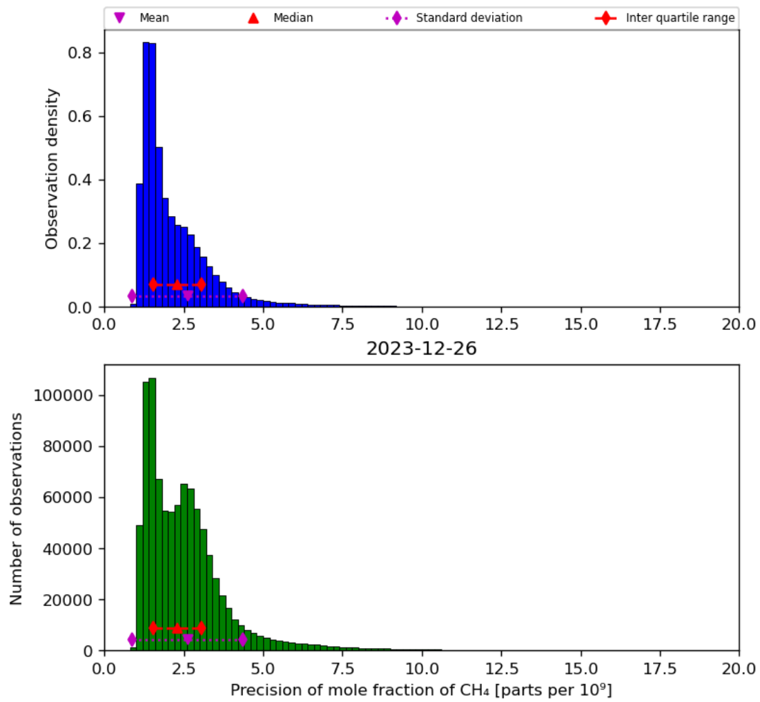
Figure 24: Histogram of “Precision of mole fraction of CH 4 ” for 2023-12-25 to 2023-12-27
