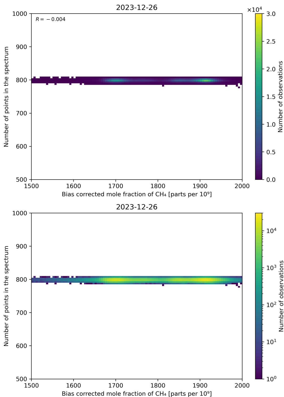
Figure 68: Scatter density plot of “Bias corrected mole fraction of CH 4 ” against “Number of points in the spectrum” for 2023-12-25 to 2023-12-27.
