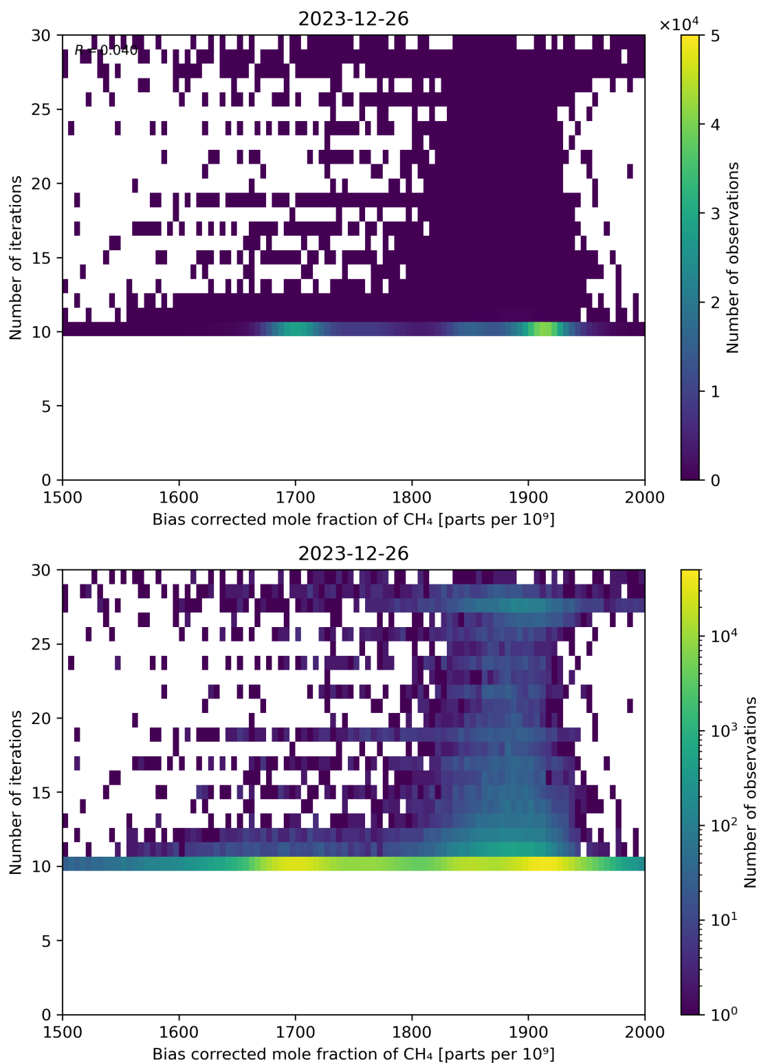
Figure 67: Scatter density plot of “Bias corrected mole fraction of CH 4 ” against “Number of iterations” for 2023-12-25 to 2023-12-27.
