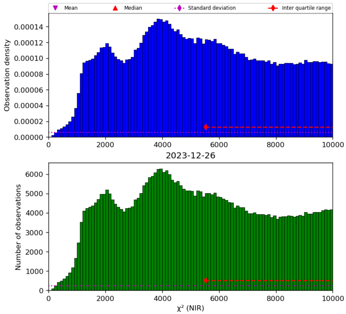
Figure 29: Histogram of “ \chi^2 (NIR)” for 2023-12-25 to 2023-12-27
