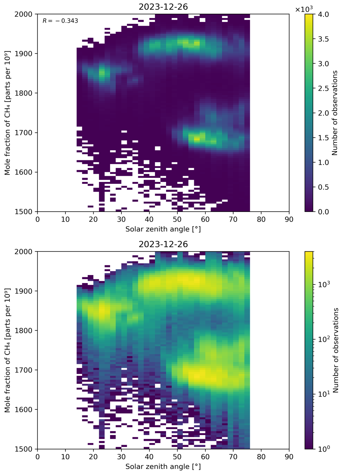
Figure 99: Scatter density plot of “Solar zenith angle” against “Mole fraction of \text{CH}_4 ” for 2023-12-25 to 2023-12-27.
