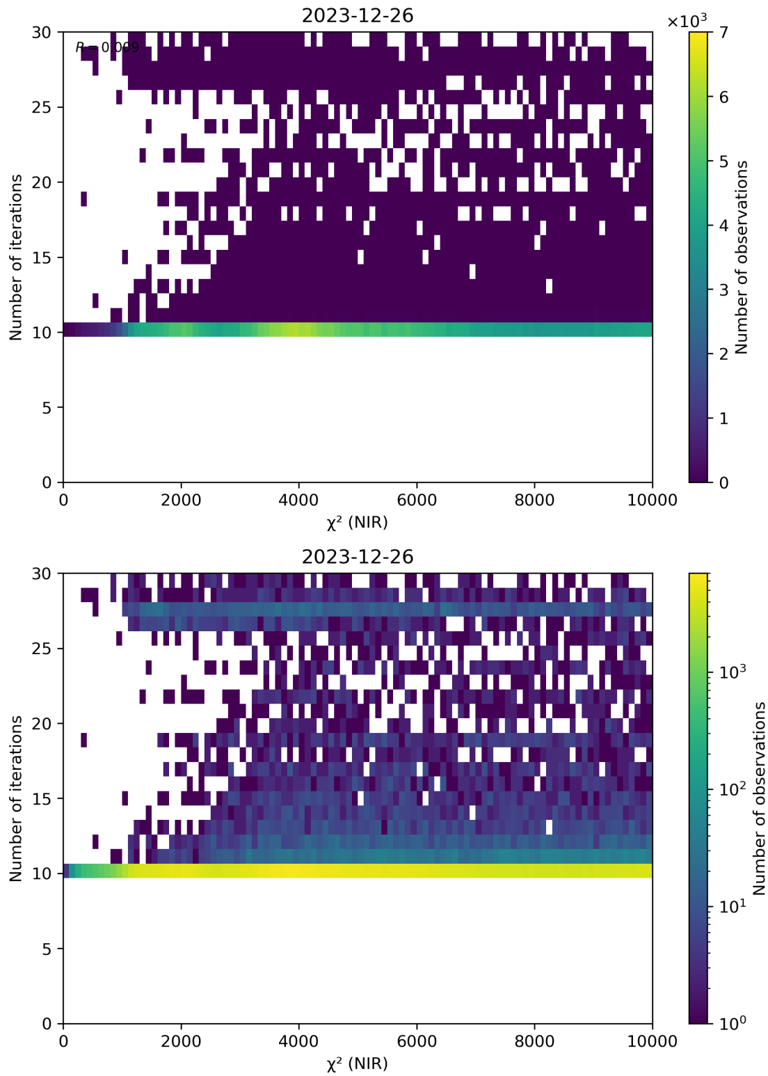
Figure 46: Scatter density plot of “ \chi^2 (NIR)” against “Number of iterations” for 2023-12-25 to 2023-12-27.
