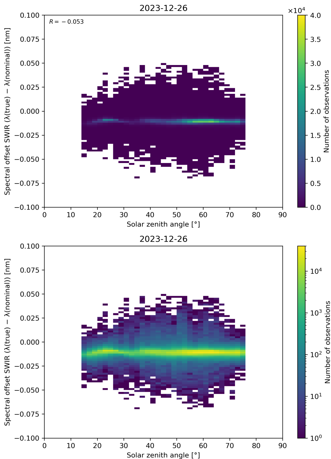
Figure 104: Scatter density plot of “Solar zenith angle” against “Spectral offset SWIR ( \lambda(\text{true}) - \lambda(\text{nominal}) )” for 2023-12-25 to 2023-12-27.
