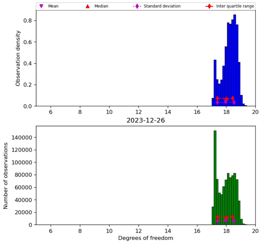
Figure 30: Histogram of “Degrees of freedom” for 2023-12-25 to 2023-12-27
