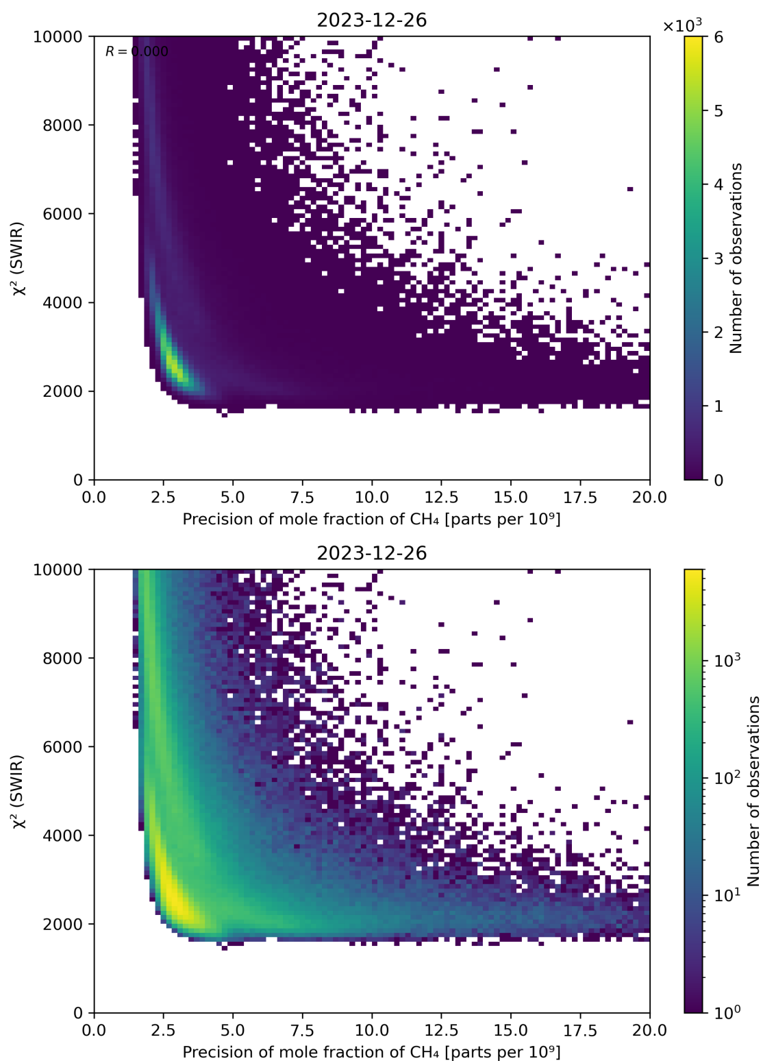
Figure 79: Scatter density plot of “Precision of mole fraction of CH 4 ” against “ \chi^2 (SWIR)” for 2023-12-25 to 2023-12-27.
