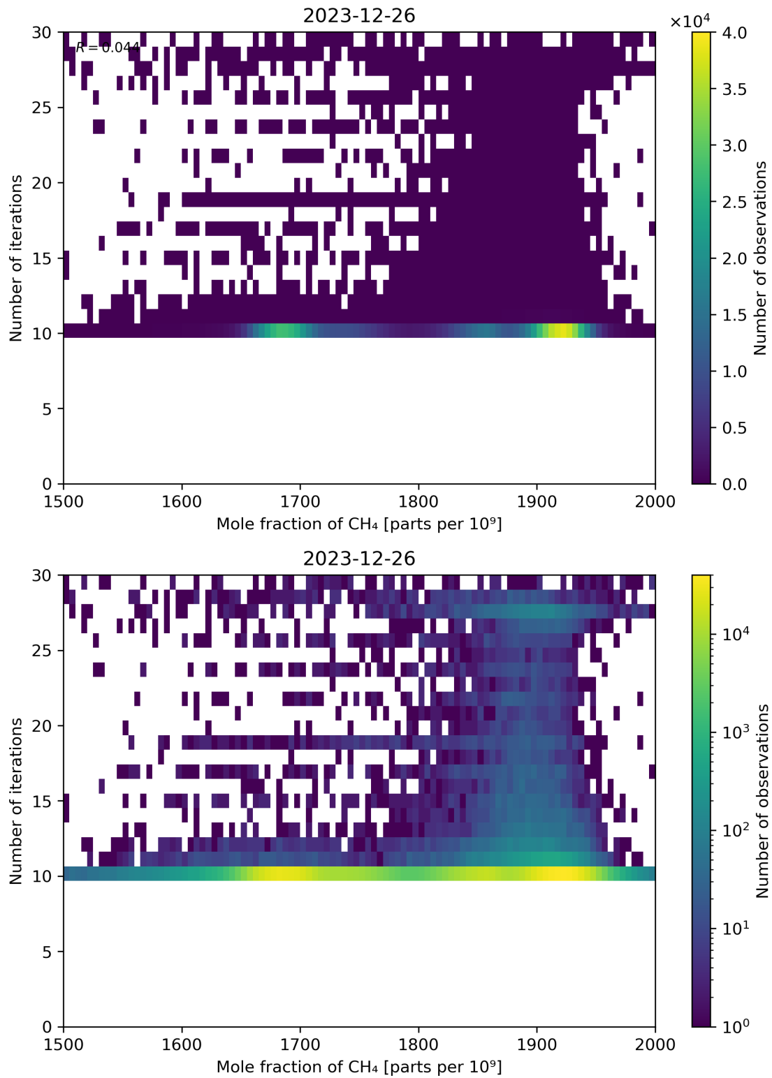
Figure 76: Scatter density plot of “Mole fraction of CH 4 ” against “Number of iterations” for 2023-12-25 to 2023-12-27.
