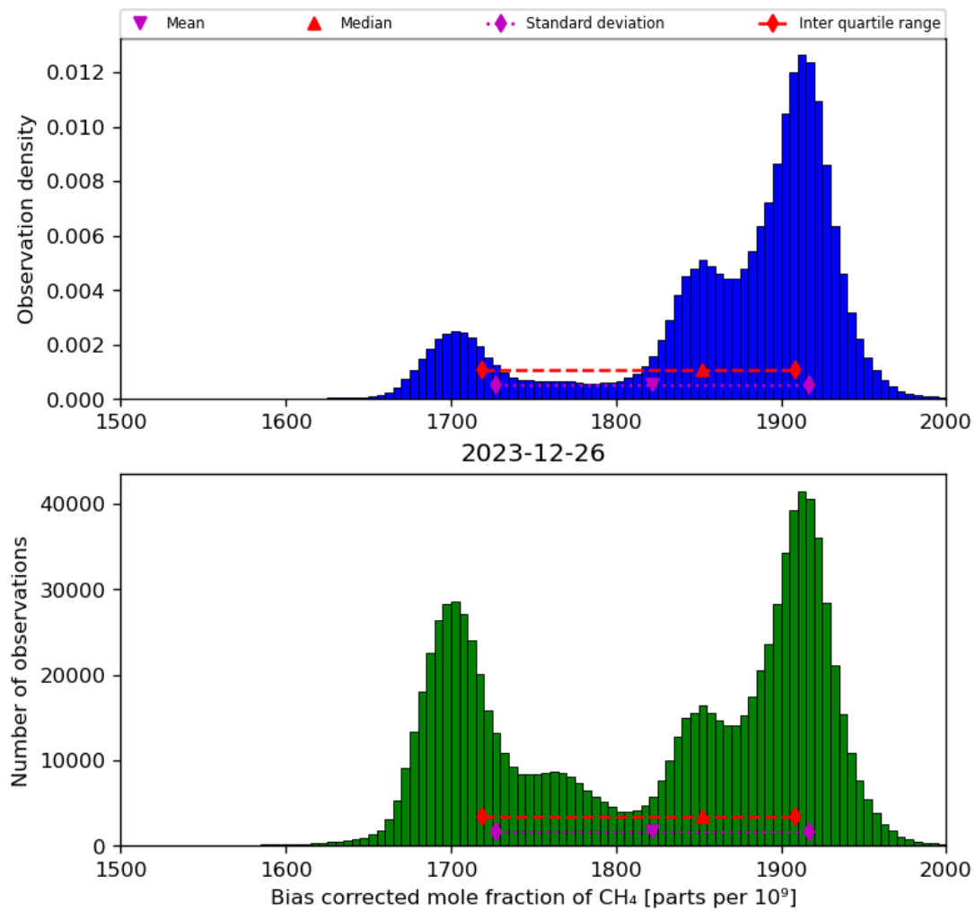
Figure 25: Histogram of “Bias corrected mole fraction of CH 4 ” for 2023-12-25 to 2023-12-27
