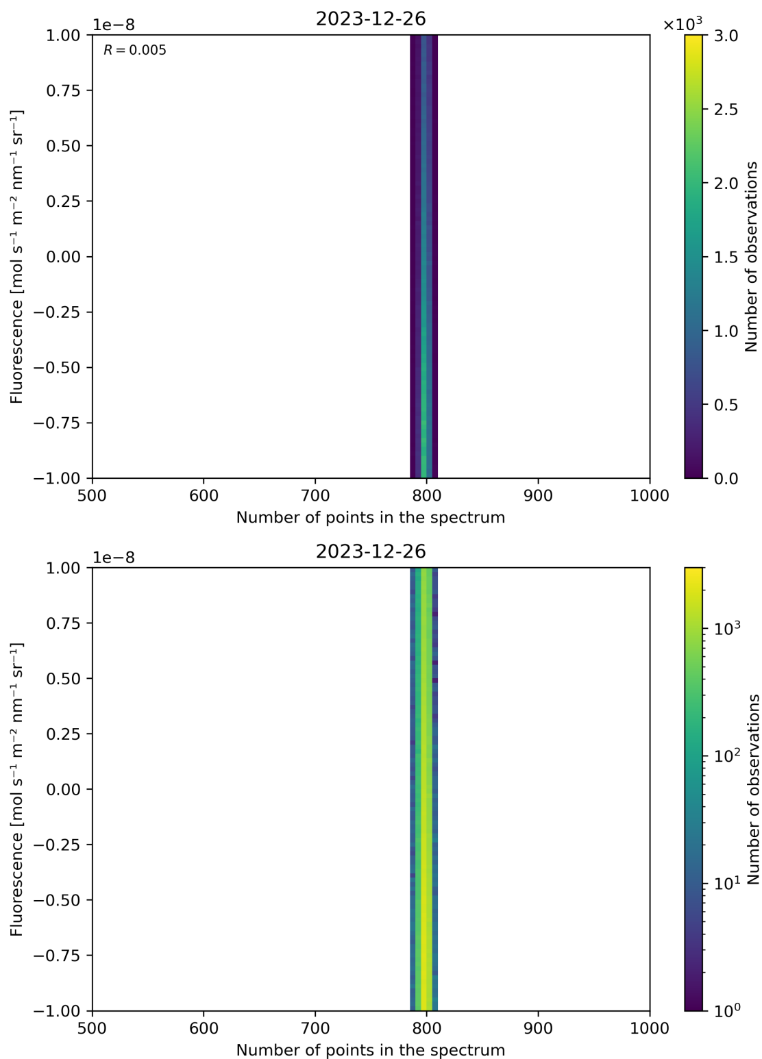
Figure 91: Scatter density plot of “Number of points in the spectrum” against “Fluorescence” for 2023-12-25 to 2023-12-27.
