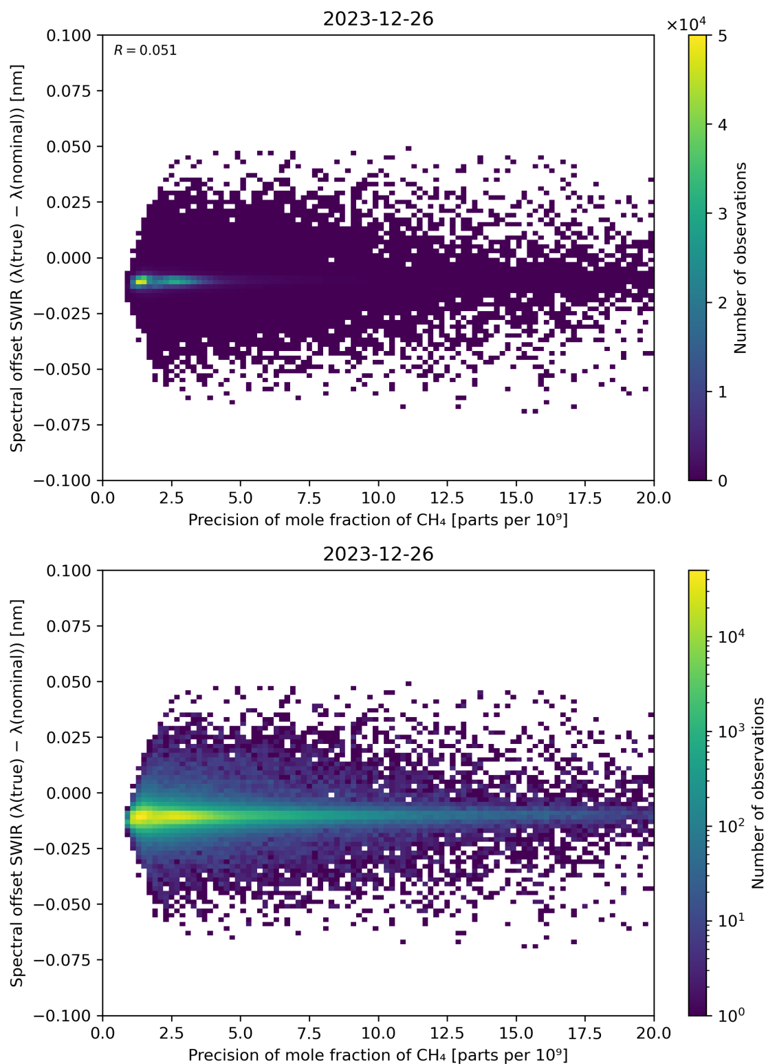
Figure 85: Scatter density plot of “Precision of mole fraction of CH 4 ” against “Spectral offset SWIR ( \lambda(\text{true}) - \lambda(\text{nominal}) )” for 2023-12-25 to 2023-12-27.
