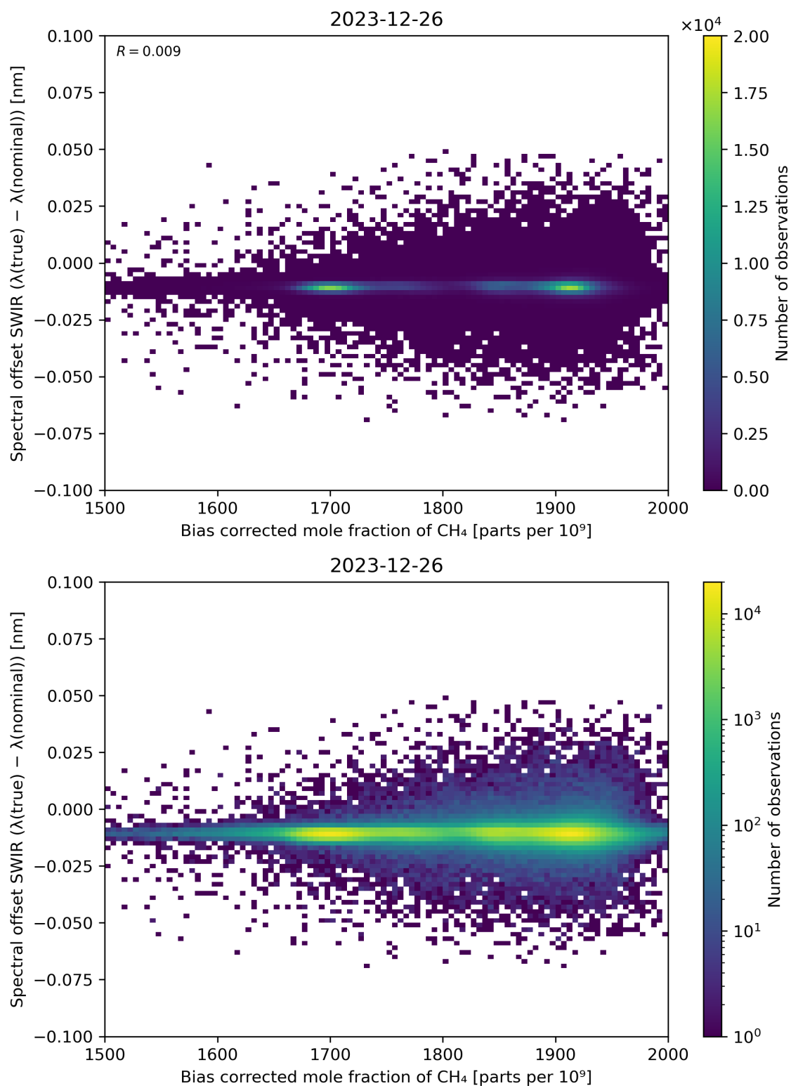
Figure 69: Scatter density plot of “Bias corrected mole fraction of \text{CH}_4 ” against “Spectral offset SWIR ( \lambda(\text{true}) - \lambda(\text{nominal}) )” for 2023-12-25 to 2023-12-27.
