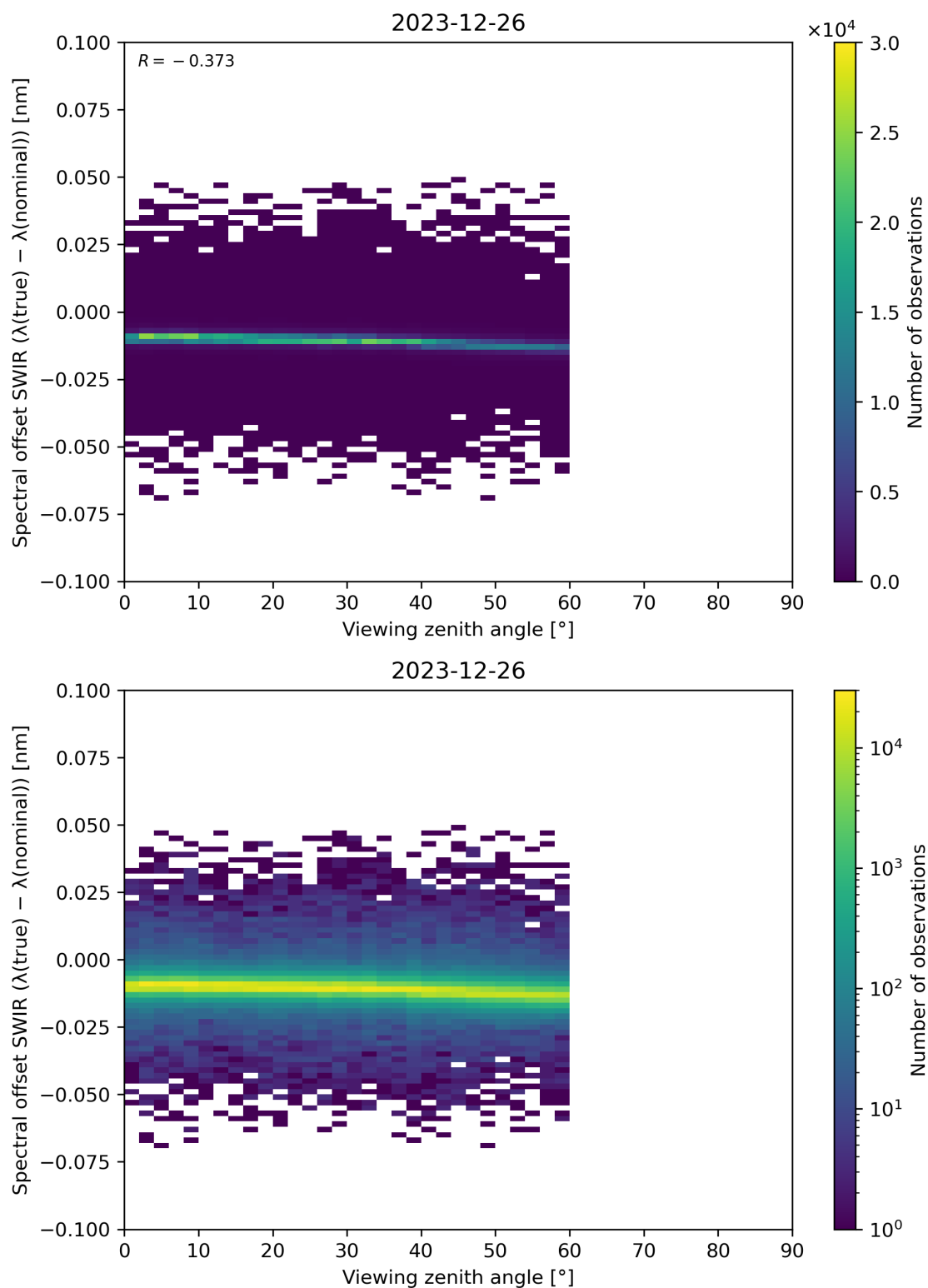
Figure 116: Scatter density plot of “Viewing zenith angle” against “Spectral offset SWIR ( \lambda(\text{true}) - \lambda(\text{nominal}) )” for 2023-12-25 to 2023-12-27.
