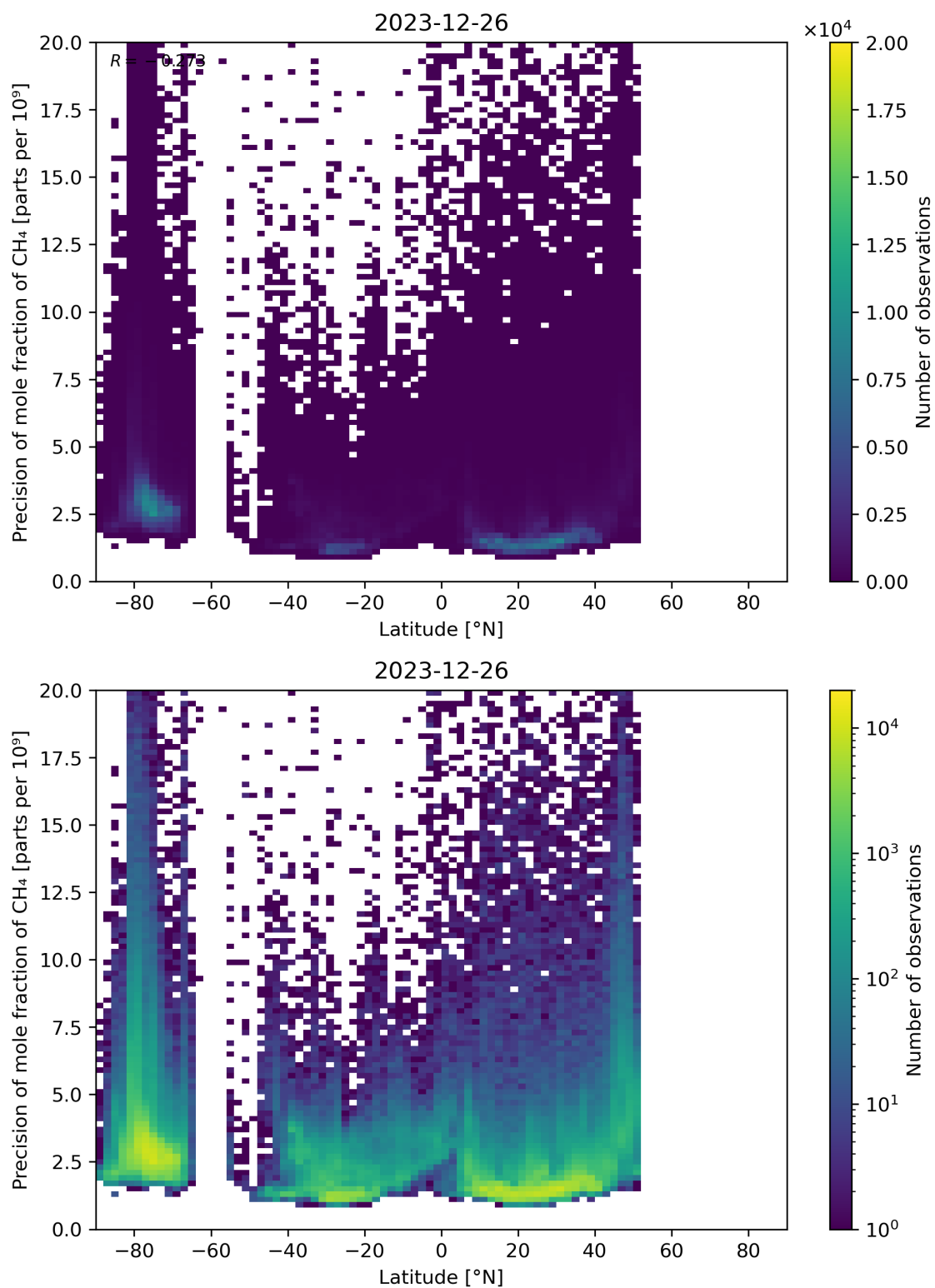
Figure 59: Scatter density plot of “Latitude” against “Precision of mole fraction of CH 4 ” for 2023-12-25 to 2023-12-27.
