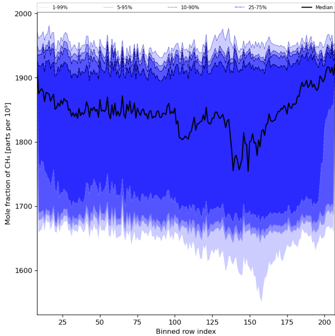
Figure 34: Along track statistics of “Mole fraction of CH 4 ” for 2023-12-25 to 2023-12-27
