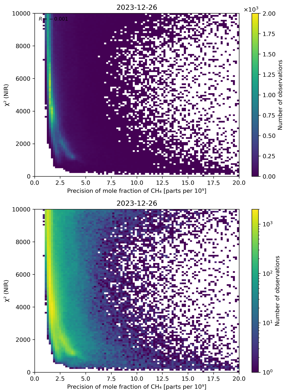
Figure 78: Scatter density plot of “Precision of mole fraction of \text{CH}_4 ” against “ \chi^2 (NIR)” for 2023-12-25 to 2023-12-27.
