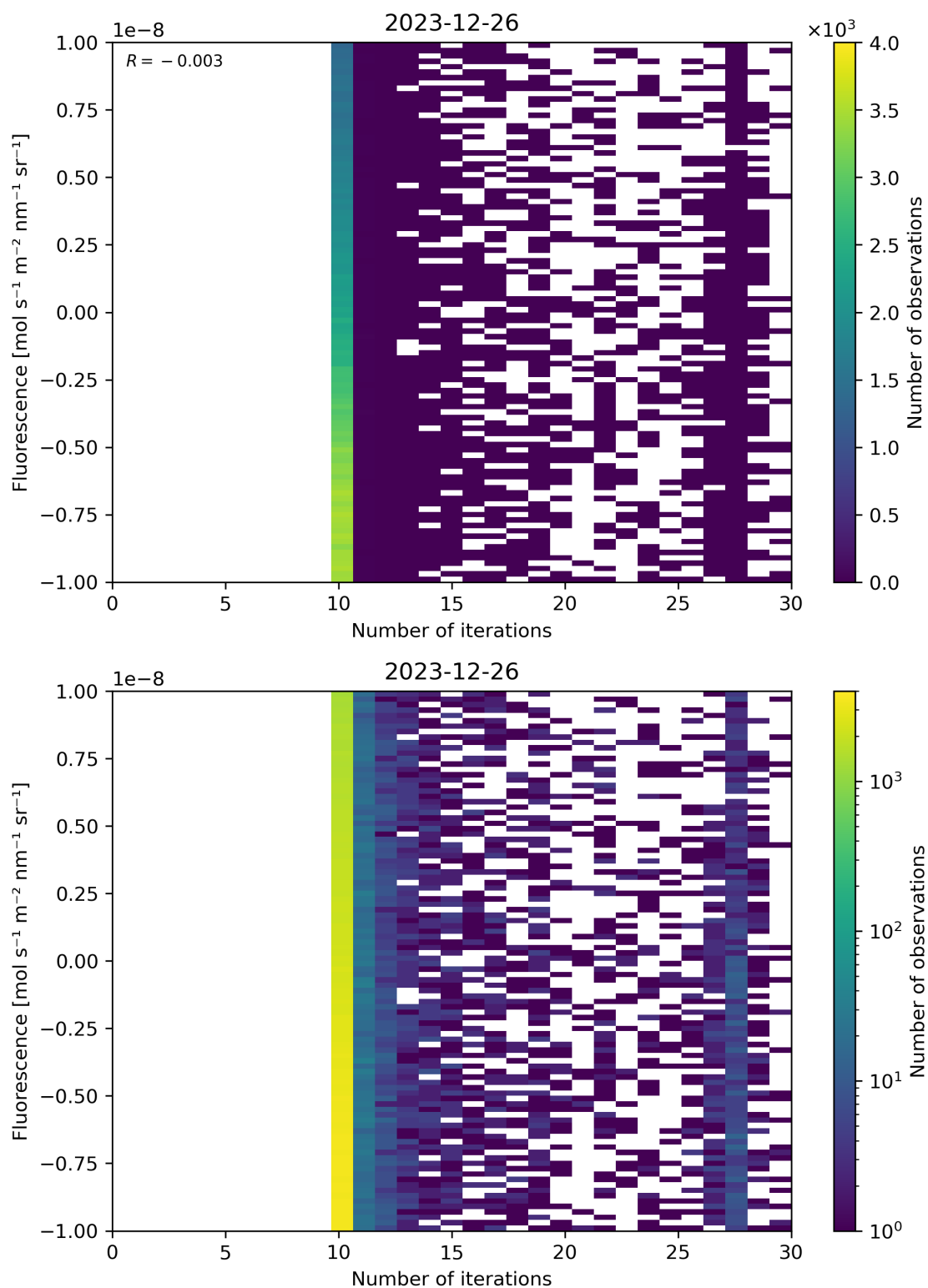
Figure 87: Scatter density plot of “Number of iterations” against “Fluorescence” for 2023-12-25 to 2023-12-27.
