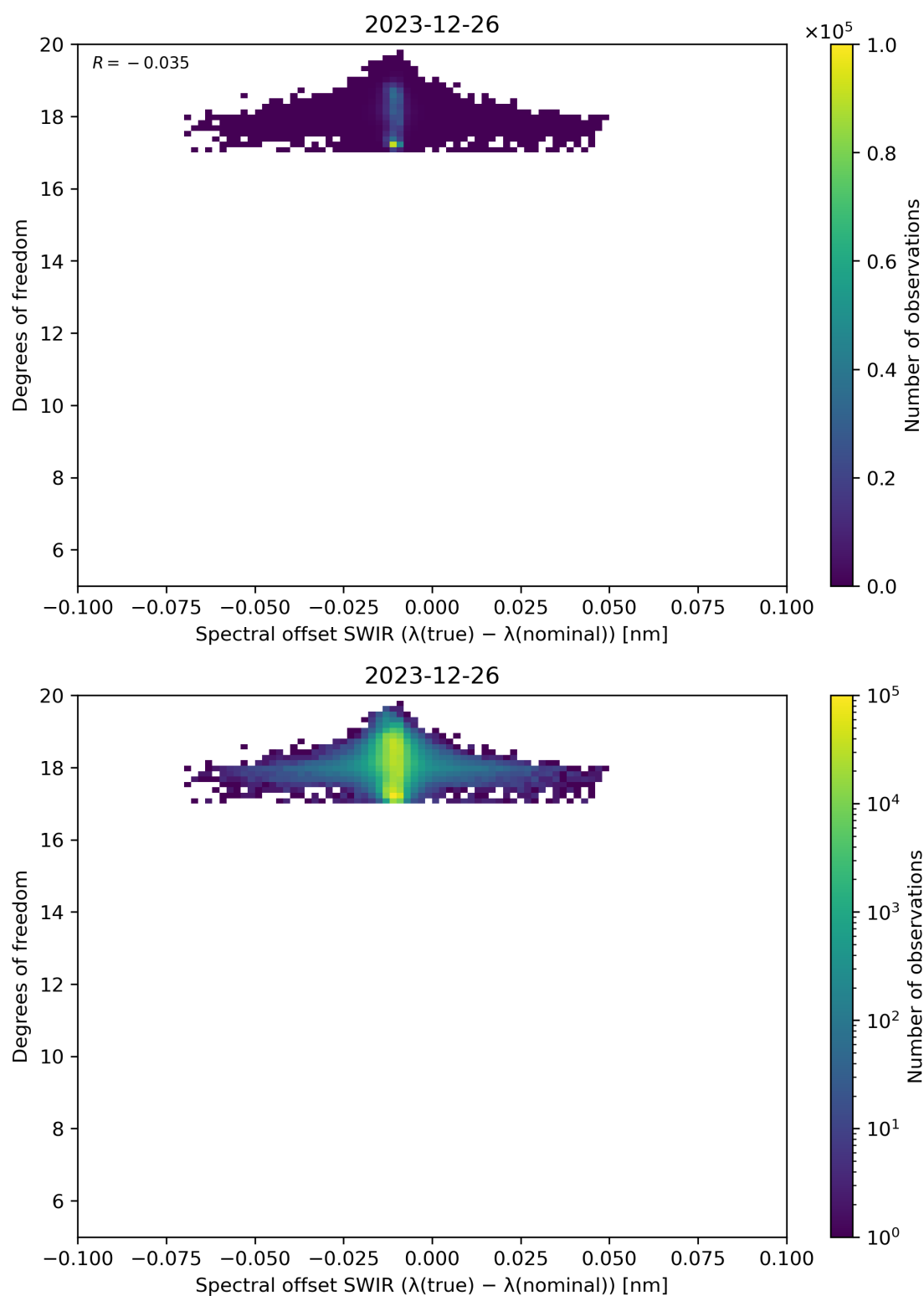
Figure 119: Scatter density plot of “Spectral offset SWIR ( \lambda(\text{true}) - \lambda(\text{nominal}) )” against “Degrees of freedom” for 2023-12-25 to 2023-12-27.
