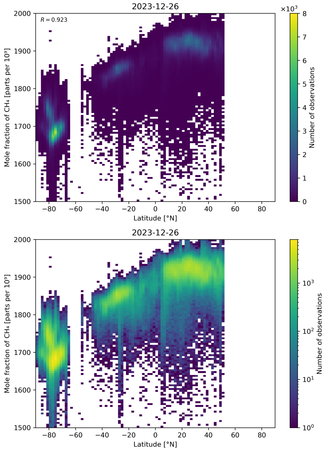
Figure 57: Scatter density plot of “Latitude” against “Mole fraction of CH 4 ” for 2023-12-25 to 2023-12-27.
