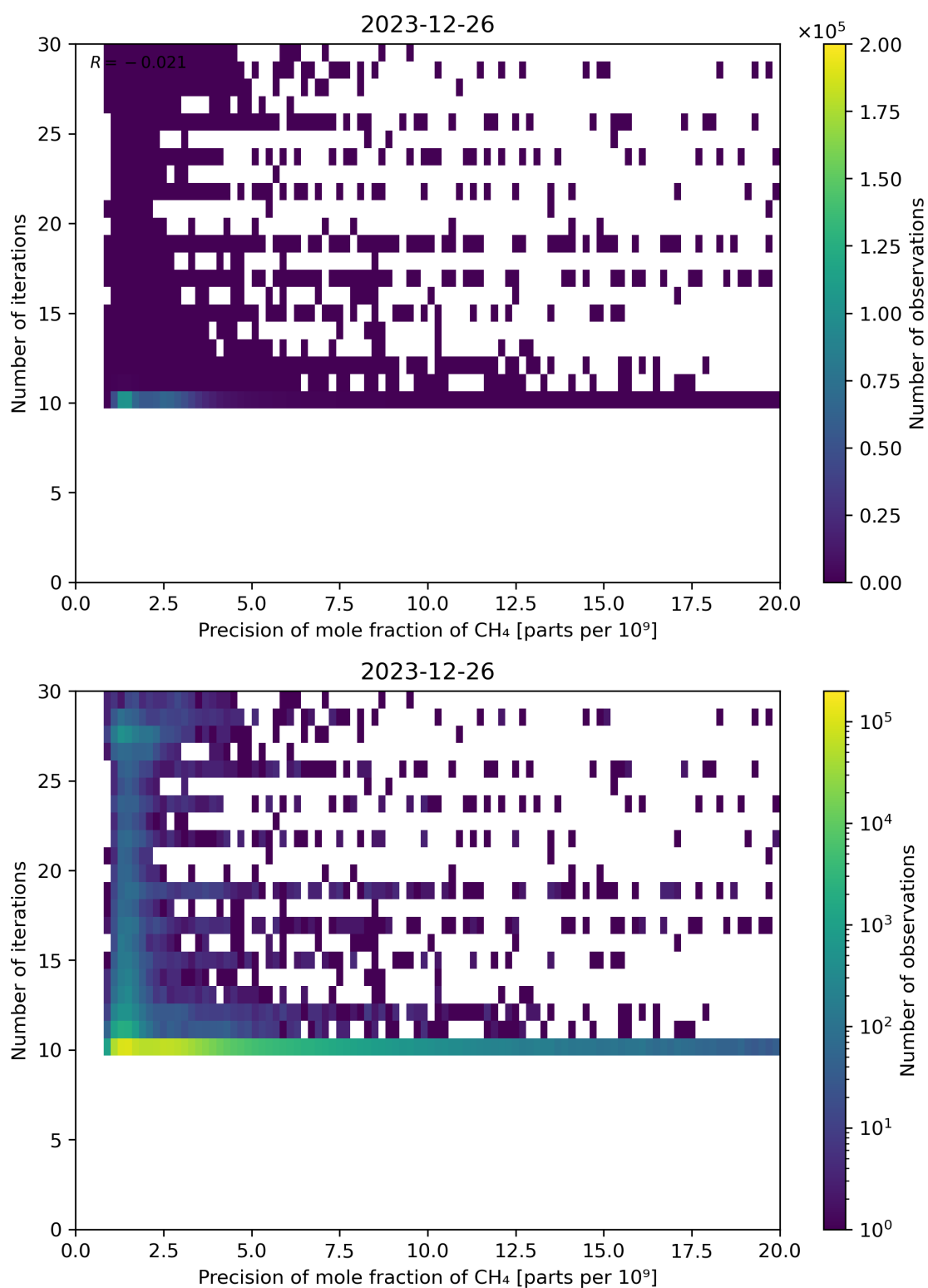
Figure 83: Scatter density plot of “Precision of mole fraction of CH 4 ” against “Number of iterations” for 2023-12-25 to 2023-12-27.
