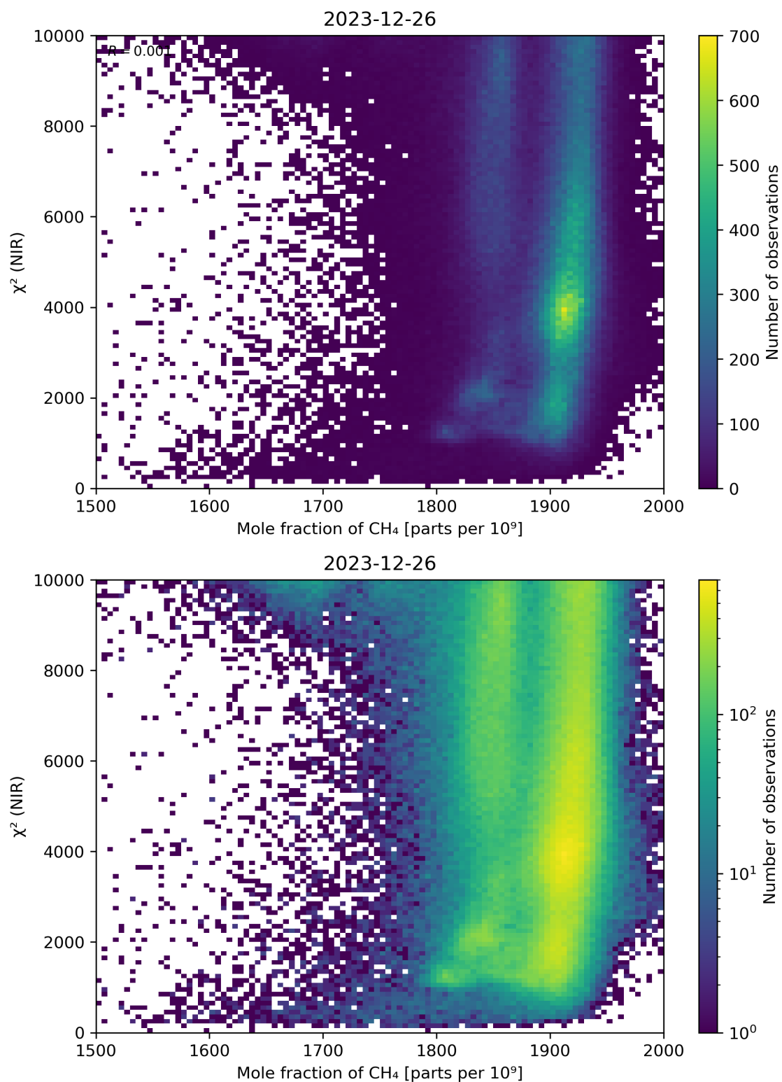
Figure 70: Scatter density plot of “Mole fraction of \text{CH}_4 ” against “ \chi^2 (NIR)” for 2023-12-25 to 2023-12-27.
