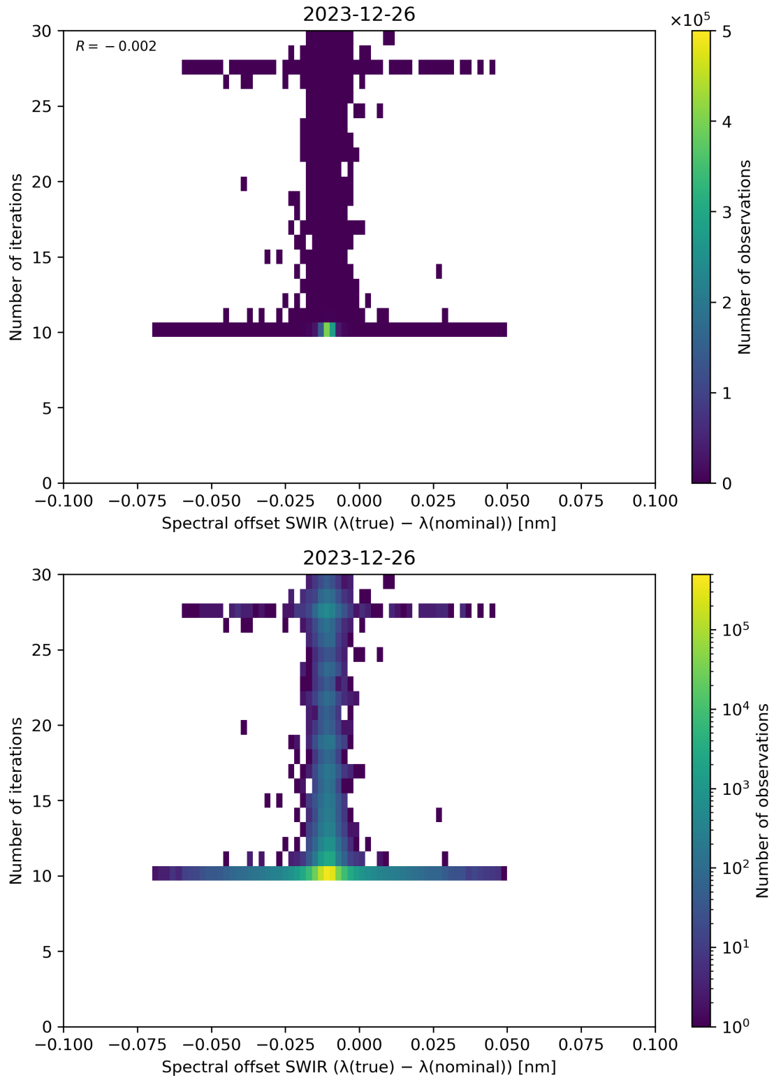
Figure 121: Scatter density plot of “Spectral offset SWIR ( \lambda(\text{true}) - \lambda(\text{nominal}) )” against “Number of iterations” for 2023-12-25 to 2023-12-27.
