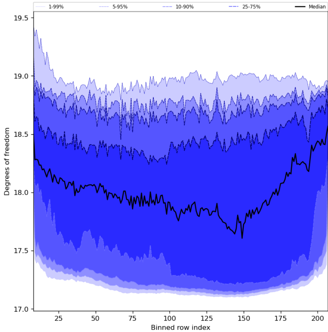
Figure 41: Along track statistics of “Degrees of freedom” for 2023-12-25 to 2023-12-27
