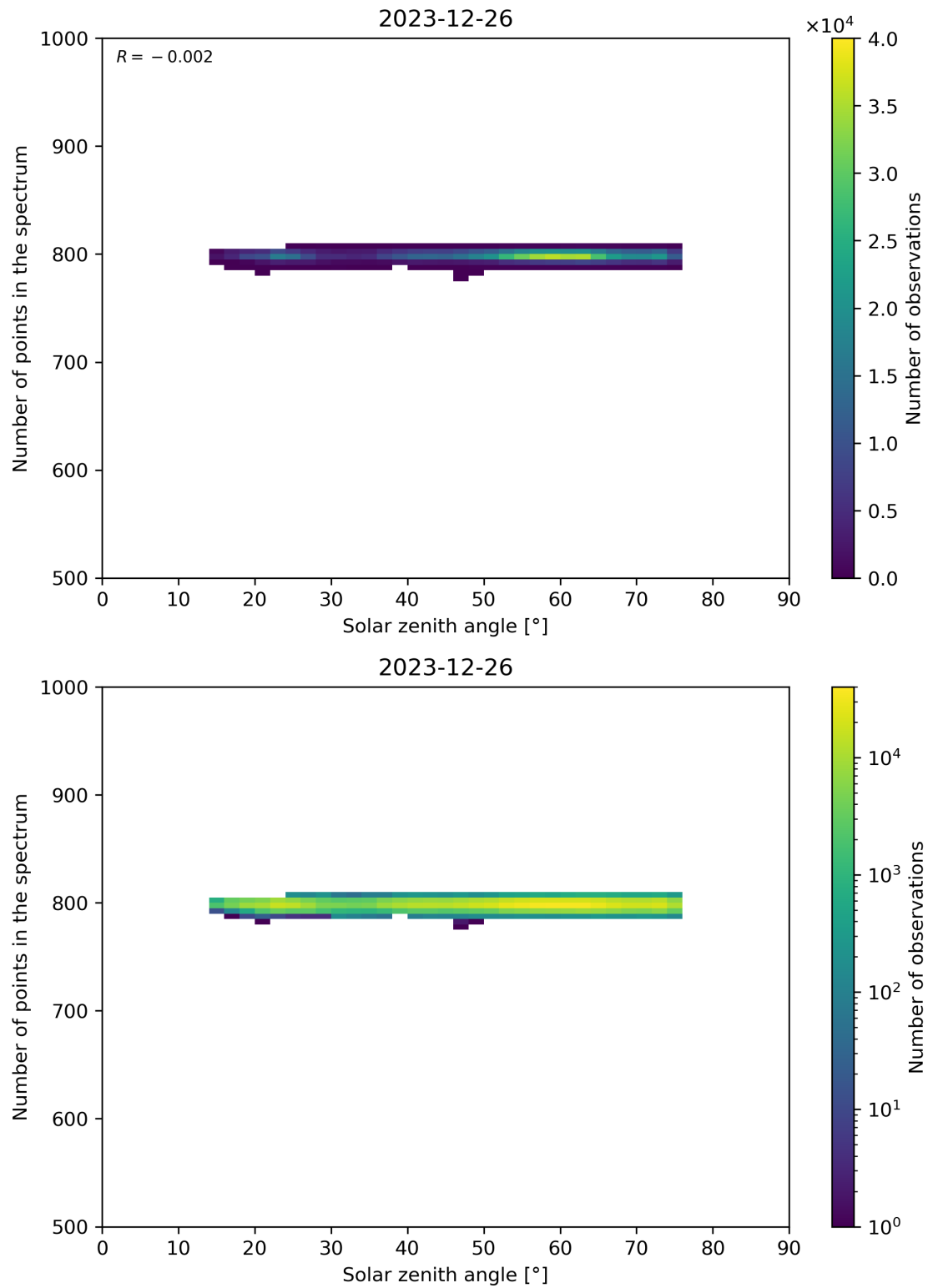
Figure 103: Scatter density plot of “Solar zenith angle” against “Number of points in the spectrum” for 2023-12-25 to 2023-12-27.
