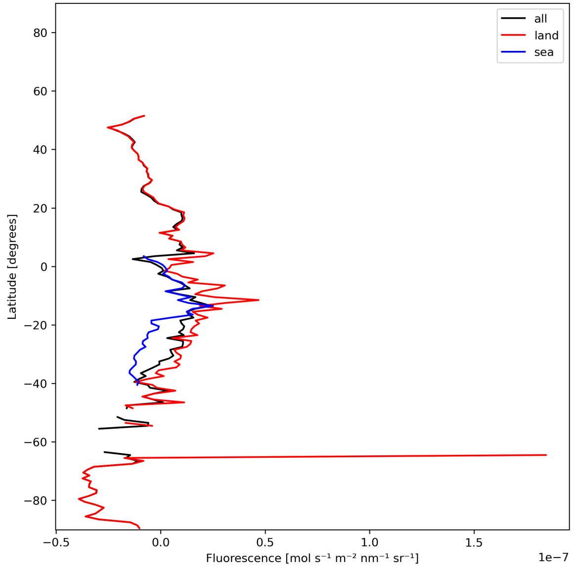
Figure 21: Zonal average of “Fluorescence” for 2023-12-25 to 2023-12-27.
