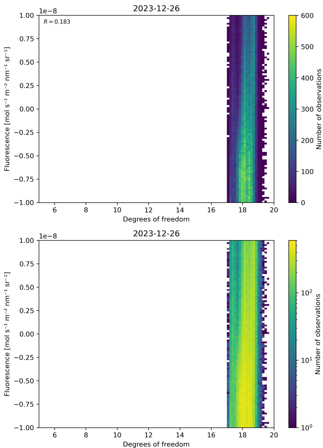
Figure 51: Scatter density plot of “Degrees of freedom” against “Fluorescence” for 2023-12-25 to 2023-12-27.
