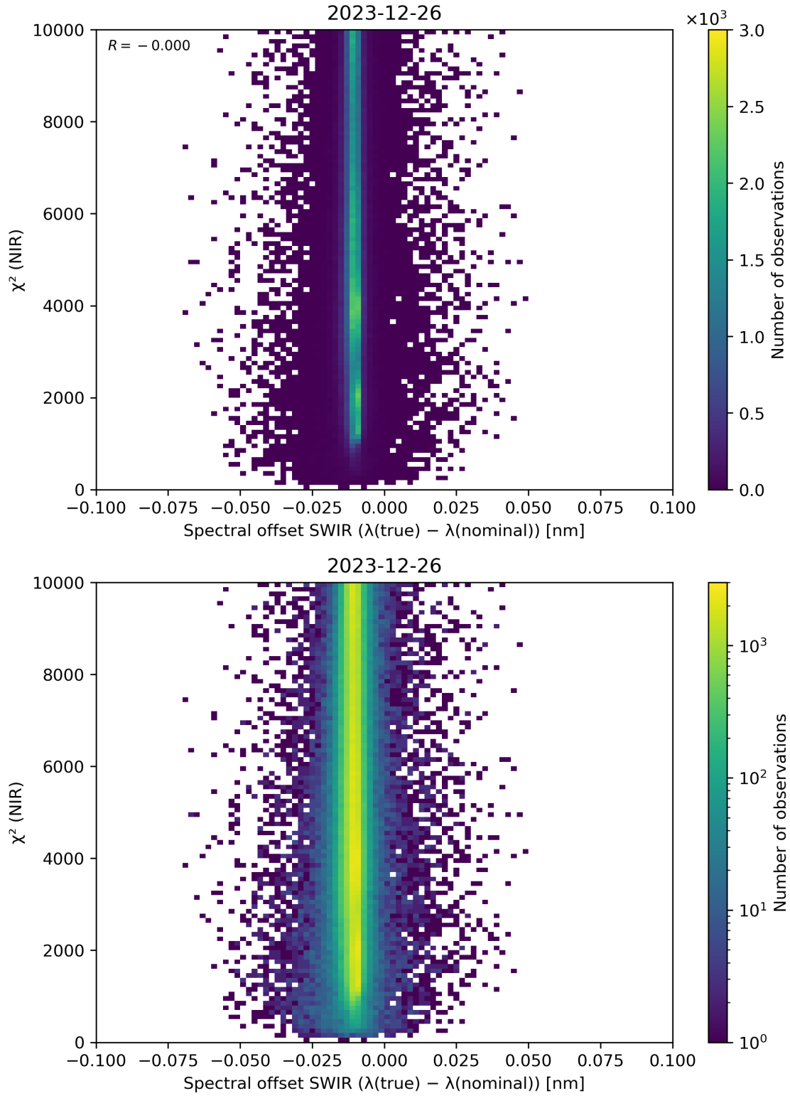
Figure 117: Scatter density plot of “Spectral offset SWIR ( \lambda(\text{true}) - \lambda(\text{nominal}) )” against “ \chi^2 (NIR)” for 2023-12-25 to 2023-12-27.
