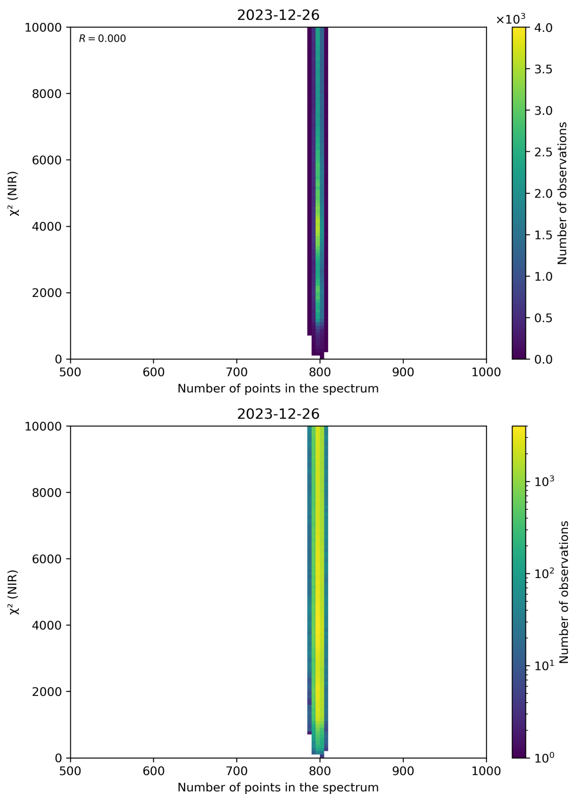
Figure 88: Scatter density plot of “Number of points in the spectrum” against “ \chi^2 (NIR)” for 2023-12-25 to 2023-12-27.
