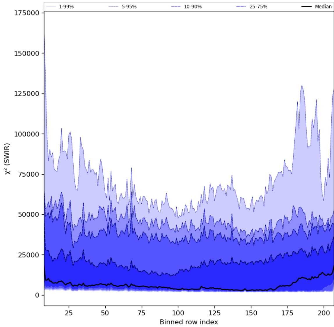
Figure 39: Along track statistics of “ \chi^2 (SWIR)” for 2023-12-25 to 2023-12-27
