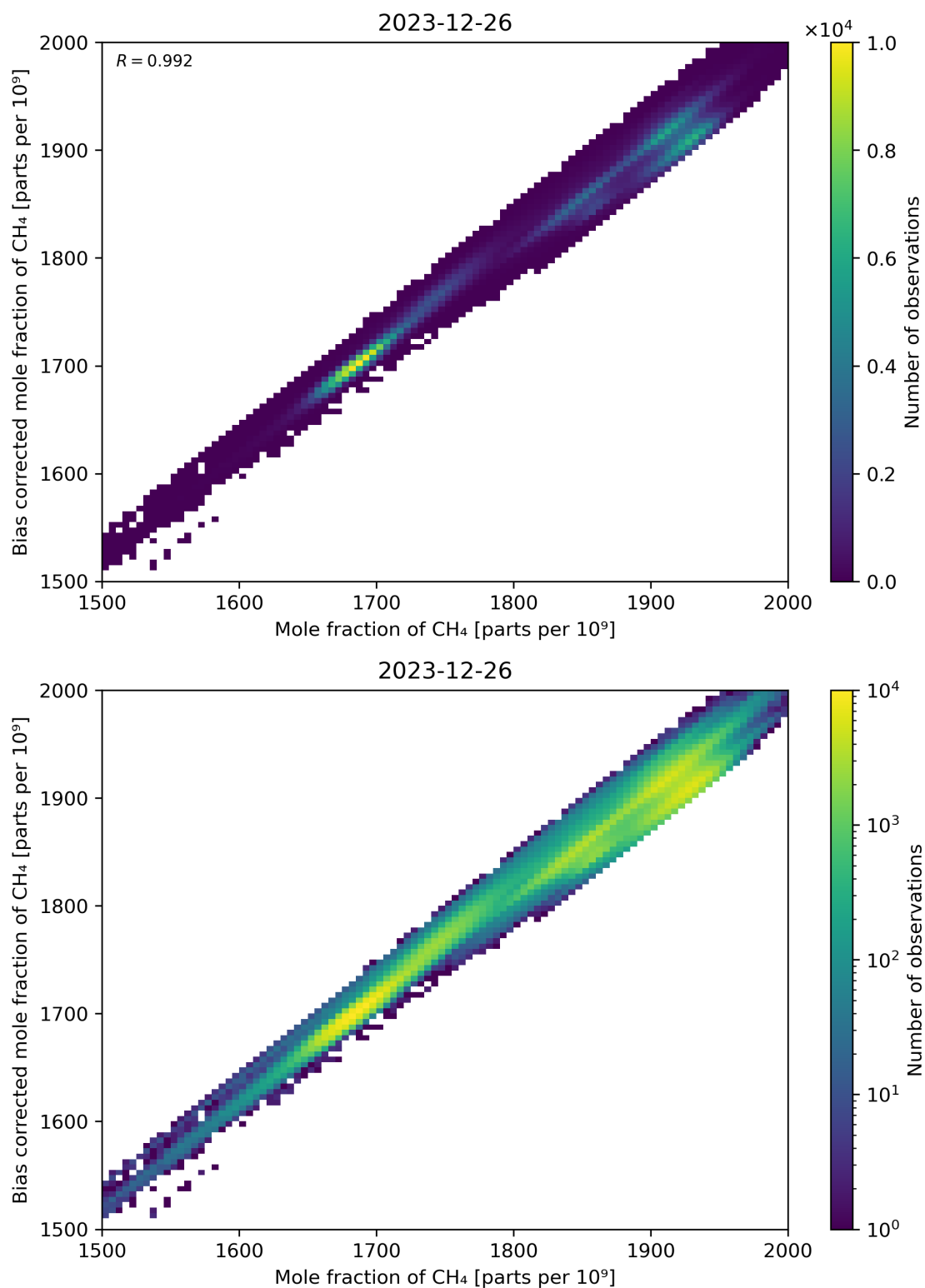
Figure 74: Scatter density plot of “Mole fraction of CH 4 ” against “Bias corrected mole fraction of CH 4 ” for 2023-12-25 to 2023-12-27.
