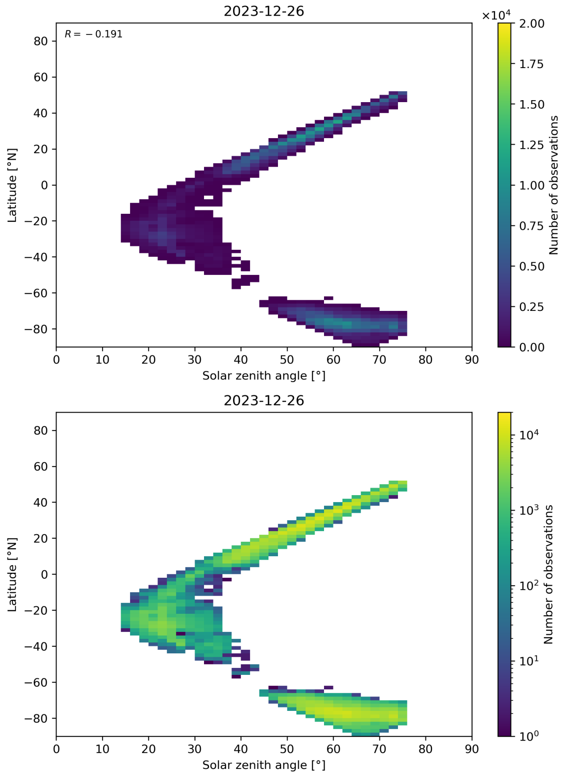
Figure 98: Scatter density plot of “Solar zenith angle” against “Latitude” for 2023-12-25 to 2023-12-27.
