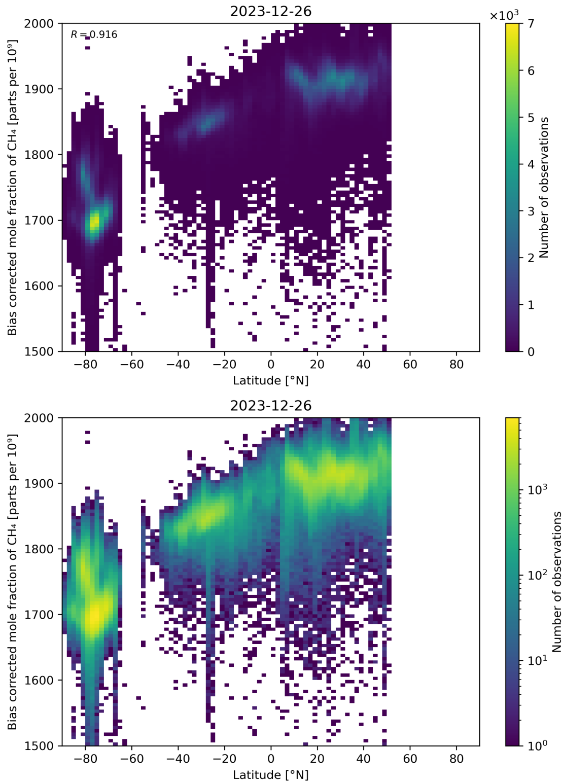
Figure 58: Scatter density plot of “Latitude” against “Bias corrected mole fraction of CH 4 ” for 2023-12-25 to 2023-12-27.
