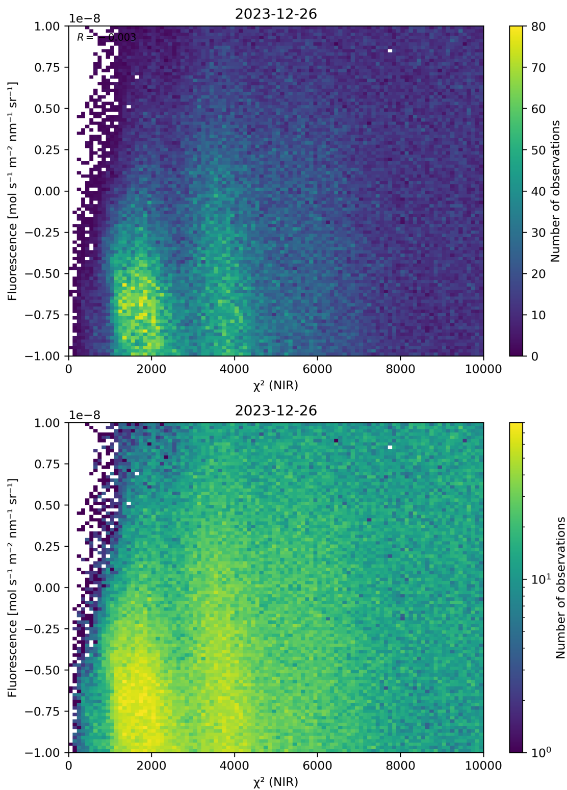
Figure 45: Scatter density plot of “ \chi^2 (NIR)” against “Fluorescence” for 2023-12-25 to 2023-12-27.
