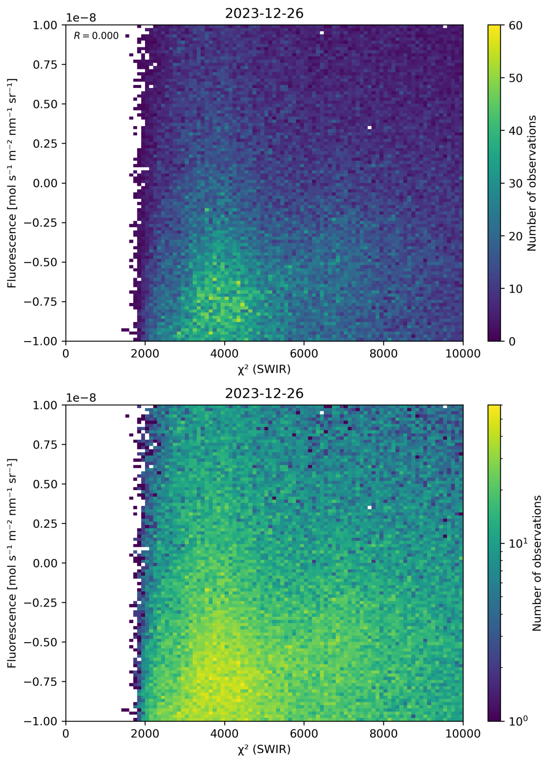
Figure 49: Scatter density plot of “ \chi^2 (SWIR)” against “Fluorescence” for 2023-12-25 to 2023-12-27.
