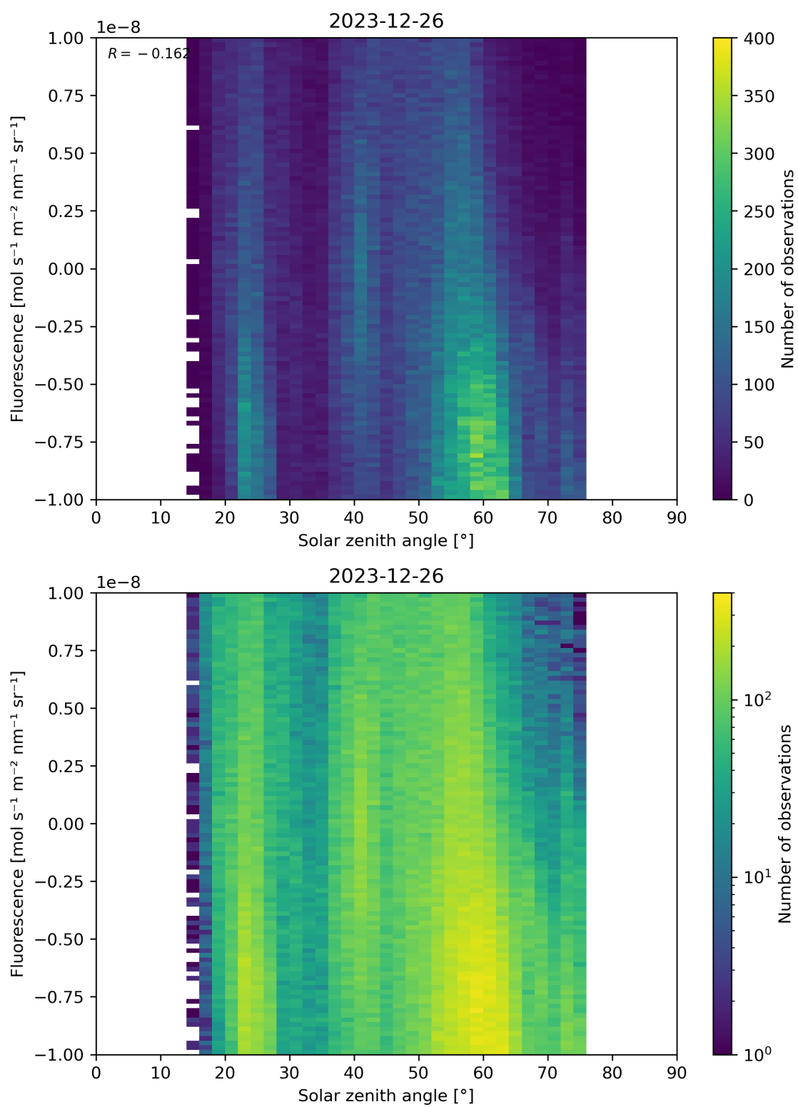
Figure 97: Scatter density plot of “Solar zenith angle” against “Fluorescence” for 2023-12-25 to 2023-12-27.
