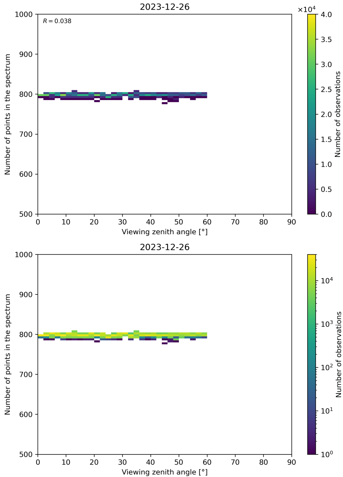
Figure 114: Scatter density plot of “Viewing zenith angle” against “Number of points in the spectrum” for 2023-12-25 to 2023-12-27.
