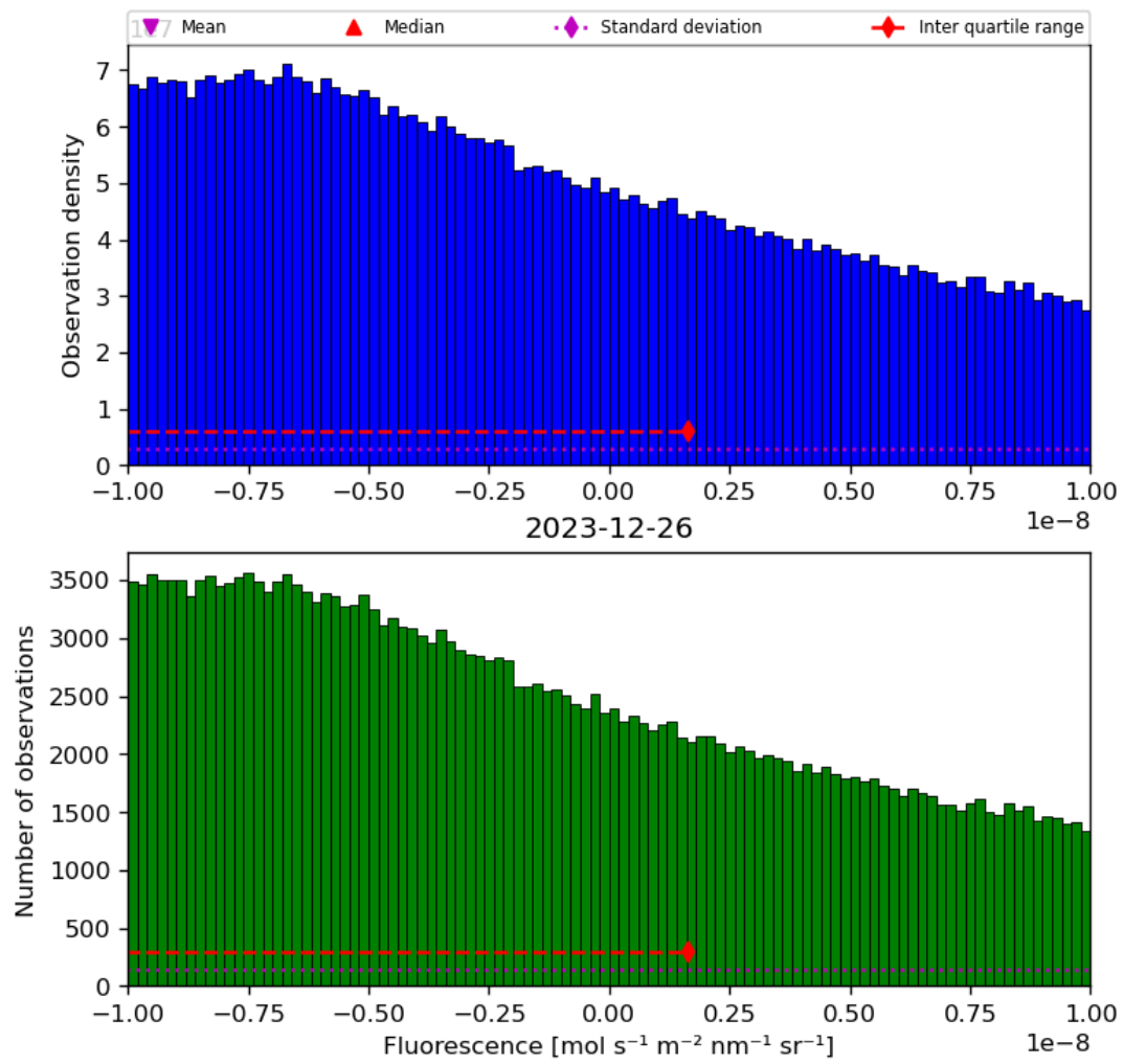
Figure 32: Histogram of “Fluorescence” for 2023-12-25 to 2023-12-27
