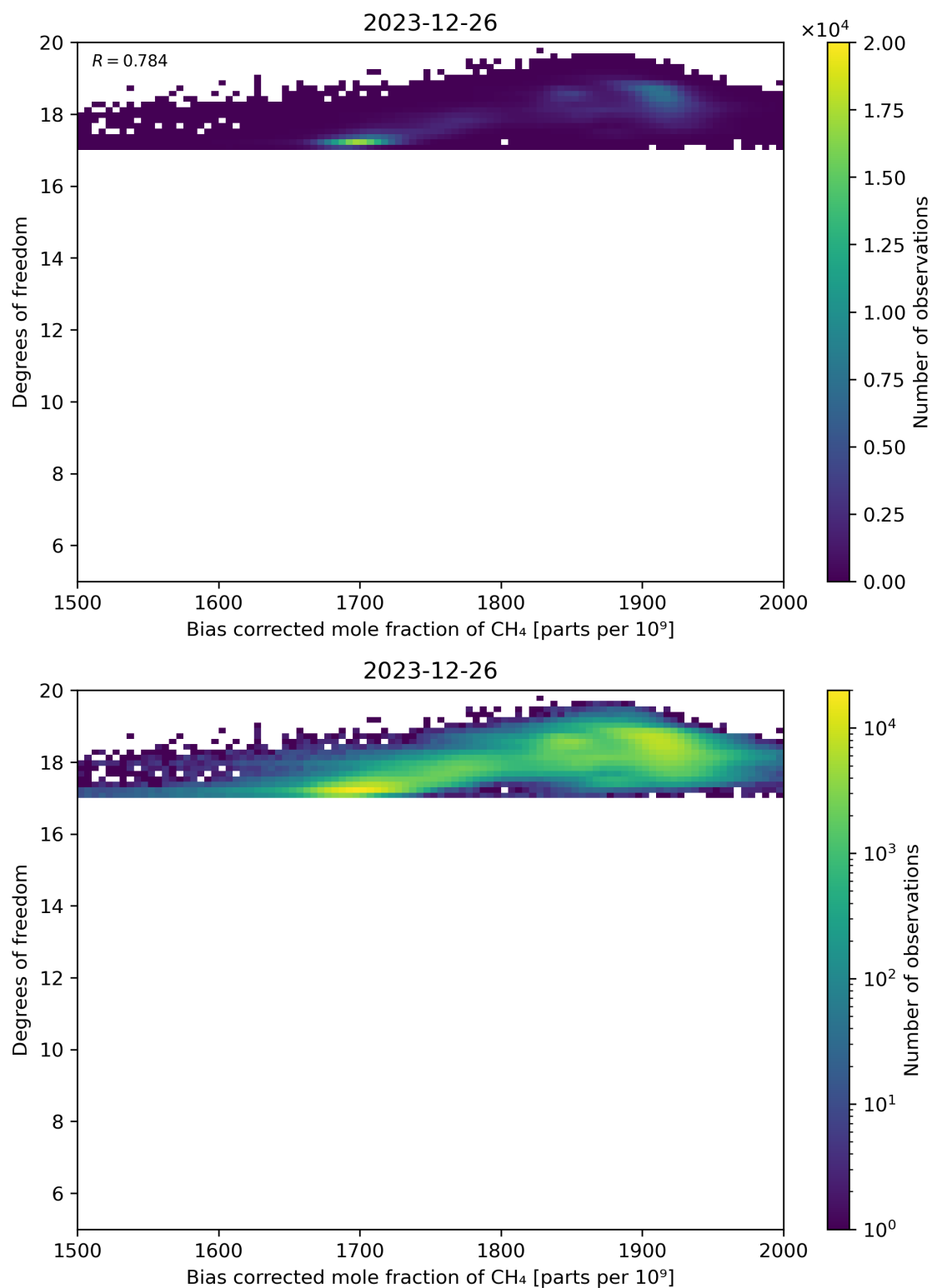
Figure 65: Scatter density plot of “Bias corrected mole fraction of CH 4 ” against “Degrees of freedom” for 2023-12-25 to 2023-12-27.
