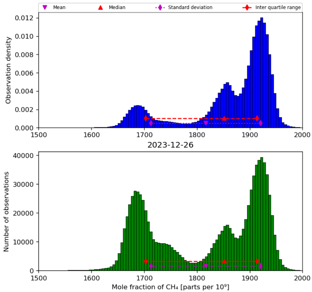
Figure 23: Histogram of “Mole fraction of CH 4 ” for 2023-12-25 to 2023-12-27
