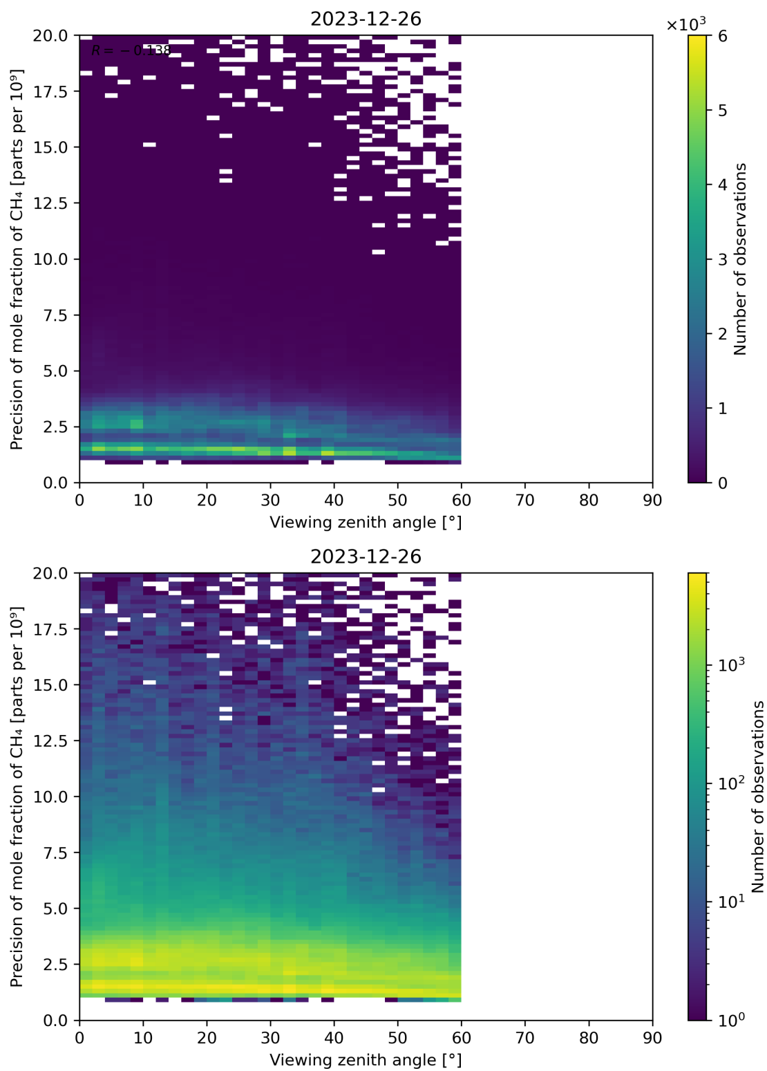
Figure 112: Scatter density plot of “Viewing zenith angle” against “Precision of mole fraction of CH 4 ” for 2023-12-25 to 2023-12-27.
