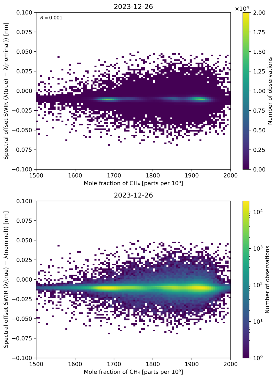
Figure 86: Scatter density plot of “Mole fraction of CH 4 ” against “Spectral offset SWIR ( \lambda(\text{true}) - \lambda(\text{nominal}) )” for 2023-12-25 to 2023-12-27.
