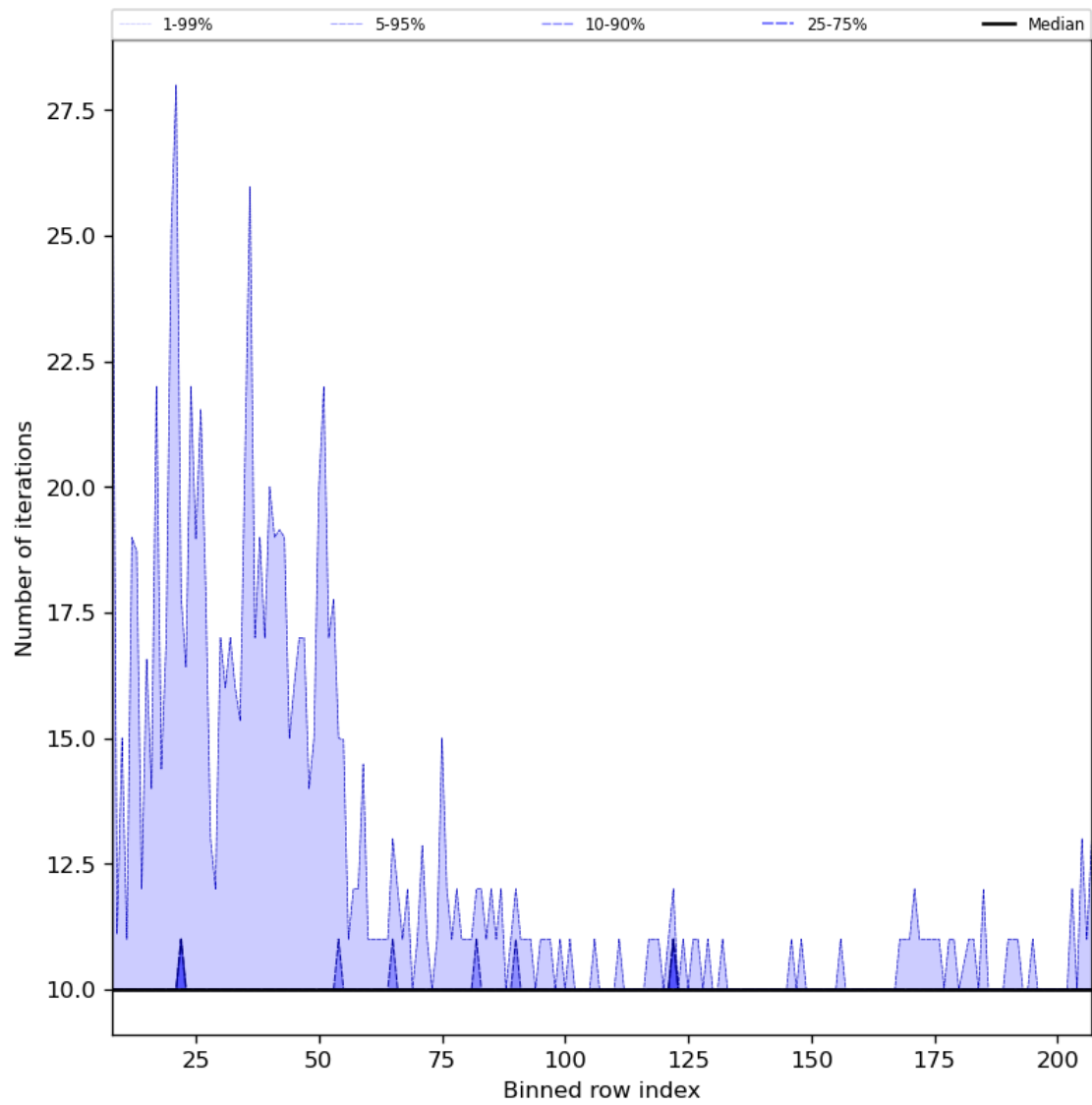
Figure 42: Along track statistics of “Number of iterations” for 2023-12-25 to 2023-12-27
