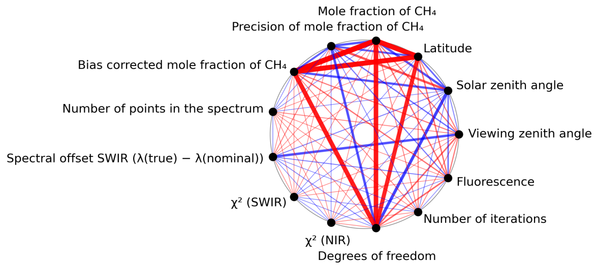
Figure 1: Map of correlation graph for 2023-12-25 to 2023-12-27.
