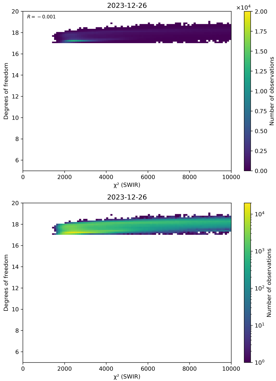
Figure 48: Scatter density plot of “ \chi^2 (SWIR)” against “Degrees of freedom” for 2023-12-25 to 2023-12-27.
