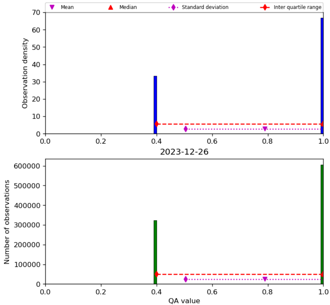
Figure 22: Histogram of “QA value” for 2023-12-25 to 2023-12-27
