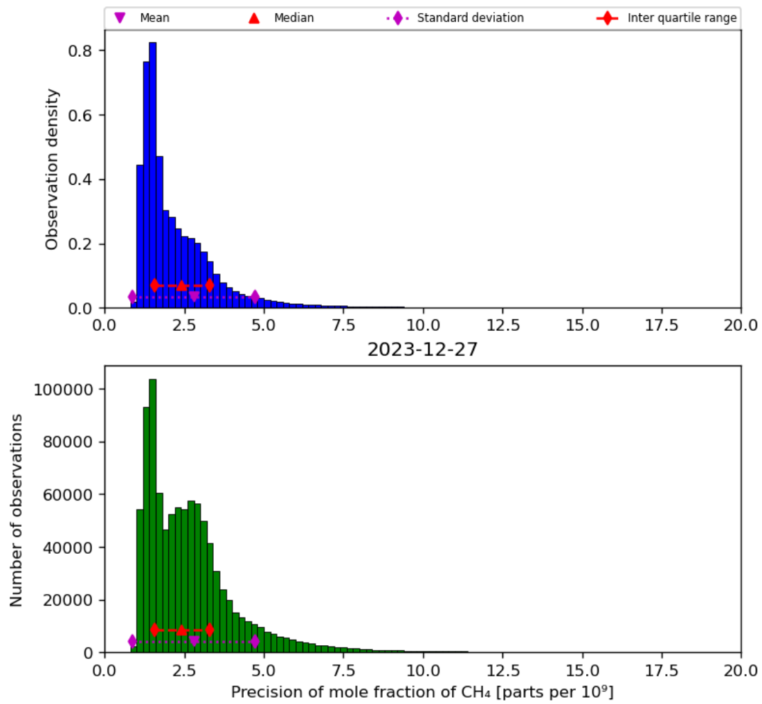
Figure 24: Histogram of “Precision of mole fraction of CH 4 ” for 2023-12-26 to 2023-12-28
