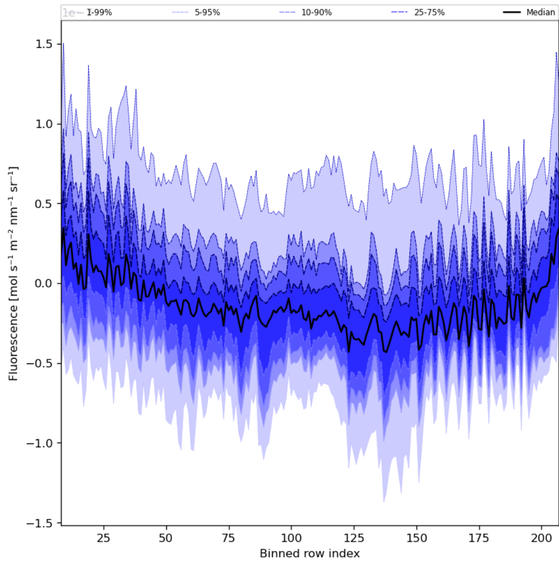
Figure 43: Along track statistics of “Fluorescence” for 2023-12-26 to 2023-12-28
