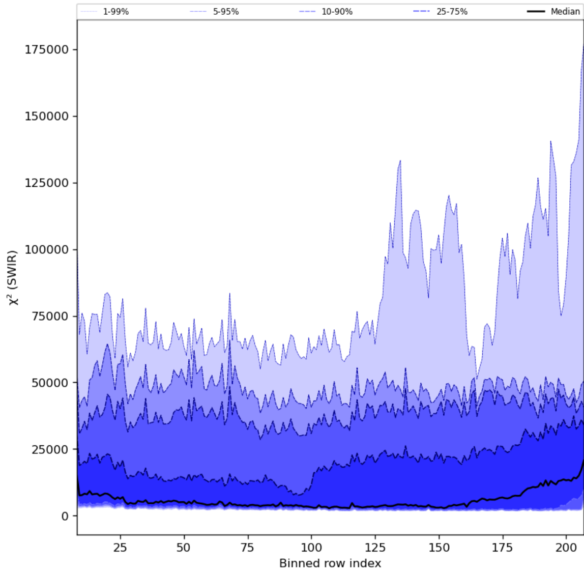
Figure 39: Along track statistics of “ \chi^2 (SWIR)” for 2023-12-26 to 2023-12-28
