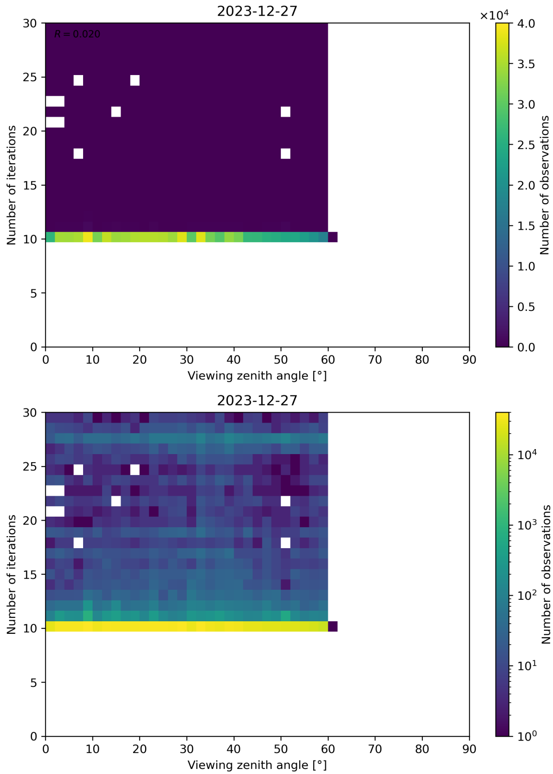
Figure 113: Scatter density plot of “Viewing zenith angle” against “Number of iterations” for 2023-12-26 to 2023-12-28.
