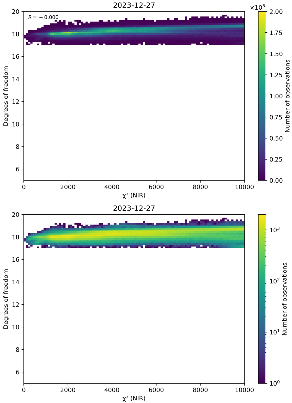
Figure 44: Scatter density plot of “ \chi^2 (NIR)” against “Degrees of freedom” for 2023-12-26 to 2023-12-28.
