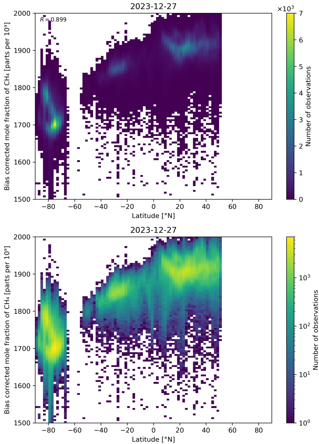
Figure 58: Scatter density plot of “Latitude” against “Bias corrected mole fraction of CH 4 ” for 2023-12-26 to 2023-12-28.
