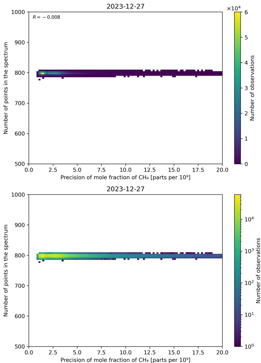
Figure 84: Scatter density plot of “Precision of mole fraction of CH 4 ” against “Number of points in the spectrum” for 2023-12-26 to 2023-12-28.
