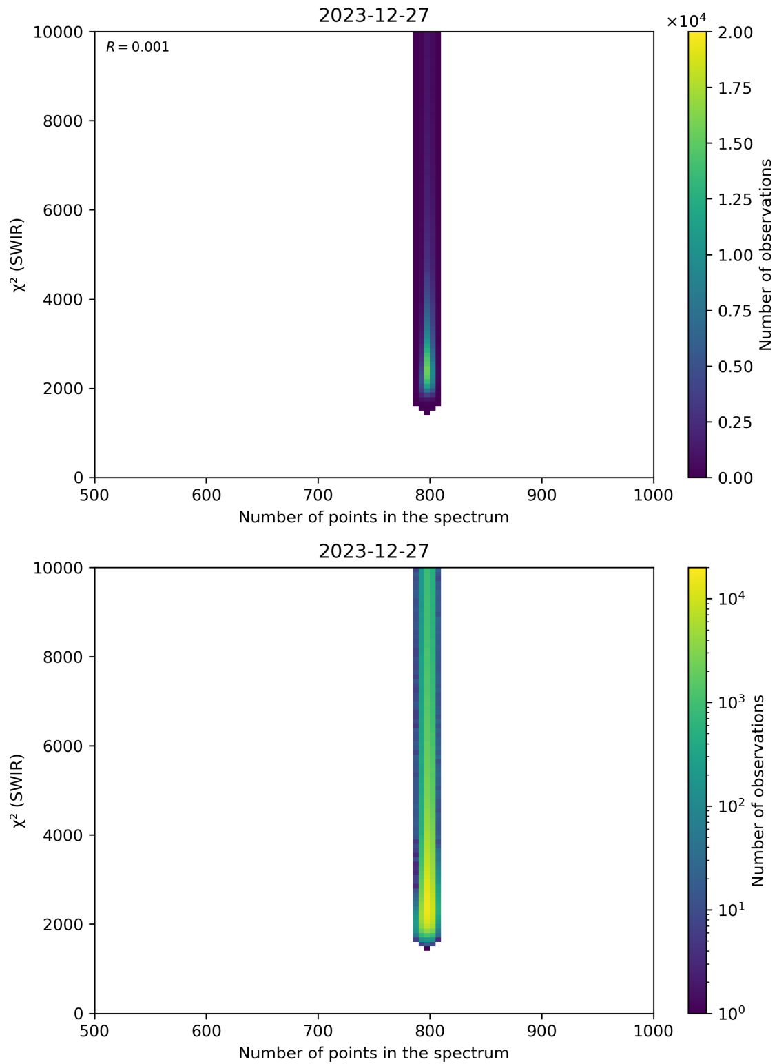
Figure 89: Scatter density plot of “Number of points in the spectrum” against “ \chi^2 (SWIR)” for 2023-12-26 to 2023-12-28.
