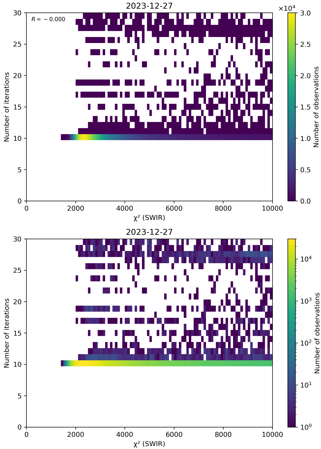
Figure 50: Scatter density plot of “ \chi^2 (SWIR)” against “Number of iterations” for 2023-12-26 to 2023-12-28.
