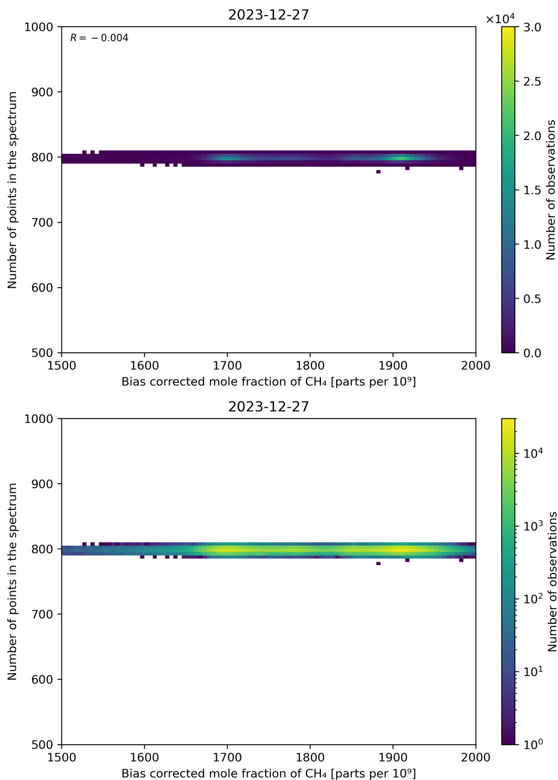
Figure 68: Scatter density plot of “Bias corrected mole fraction of CH 4 ” against “Number of points in the spectrum” for 2023-12-26 to 2023-12-28.
