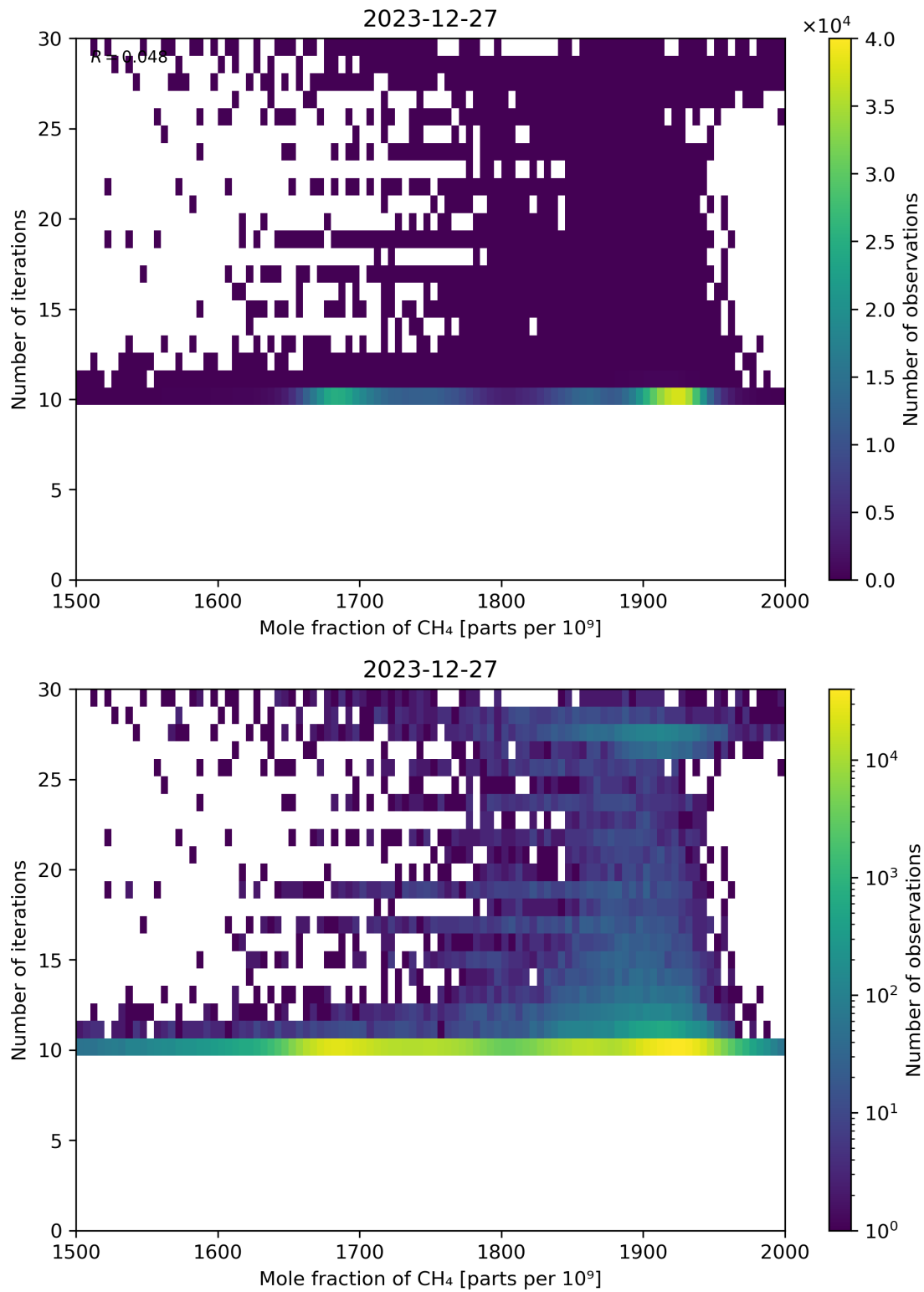
Figure 76: Scatter density plot of “Mole fraction of CH 4 ” against “Number of iterations” for 2023-12-26 to 2023-12-28.
