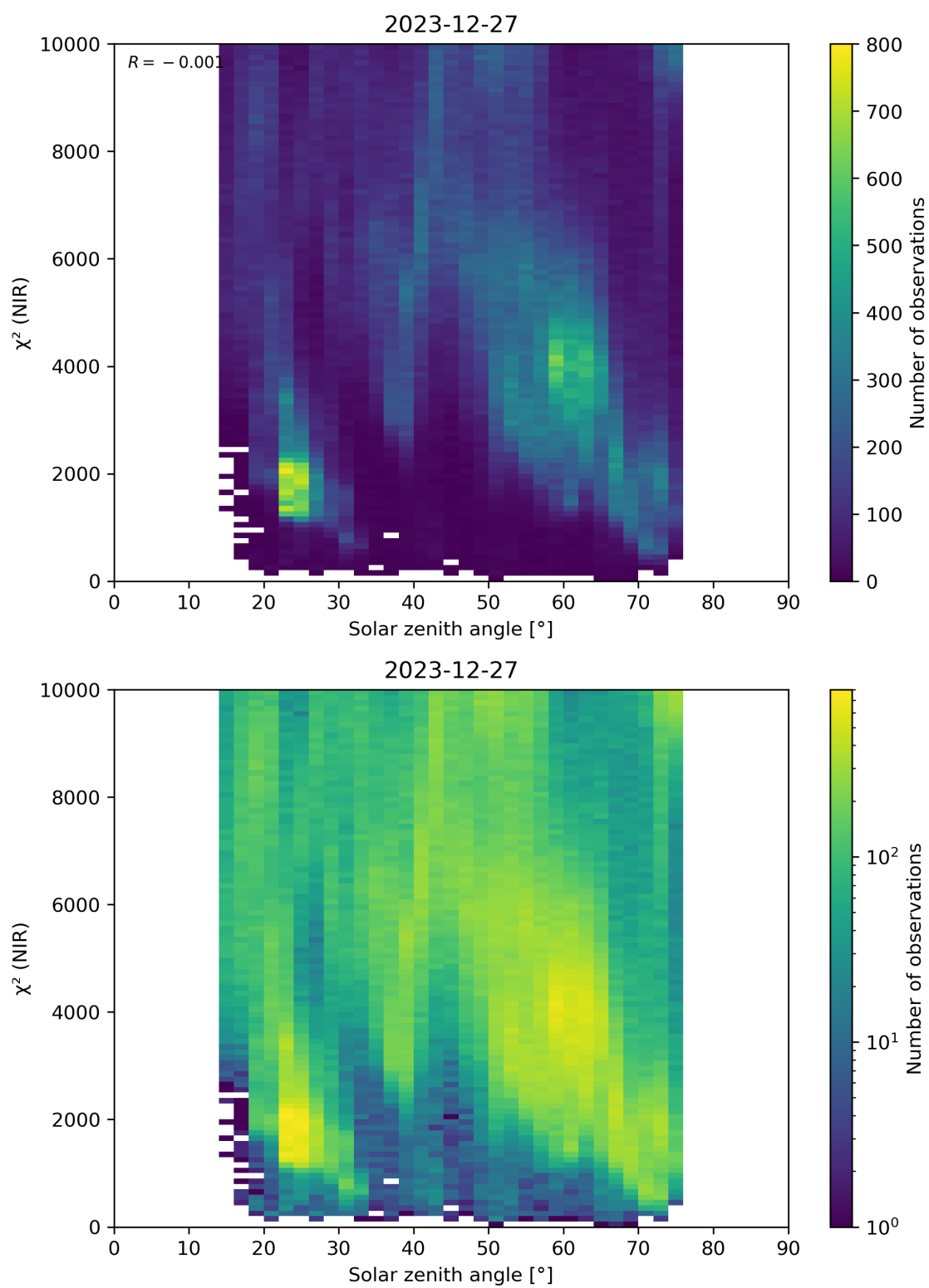
Figure 94: Scatter density plot of “Solar zenith angle” against “ \chi^2 (NIR)” for 2023-12-26 to 2023-12-28.
