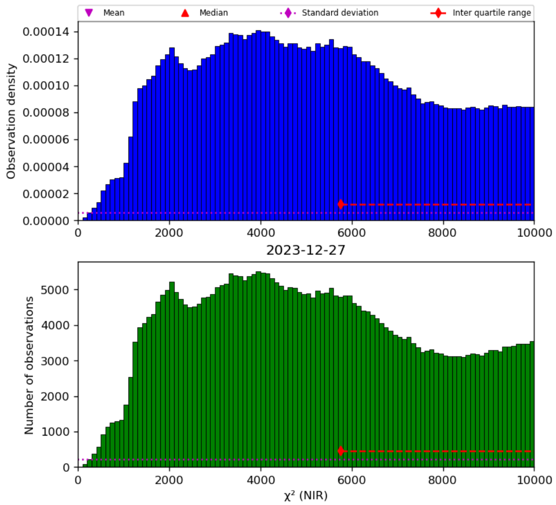
Figure 29: Histogram of " \chi^2 (NIR)" for 2023-12-26 to 2023-12-28
