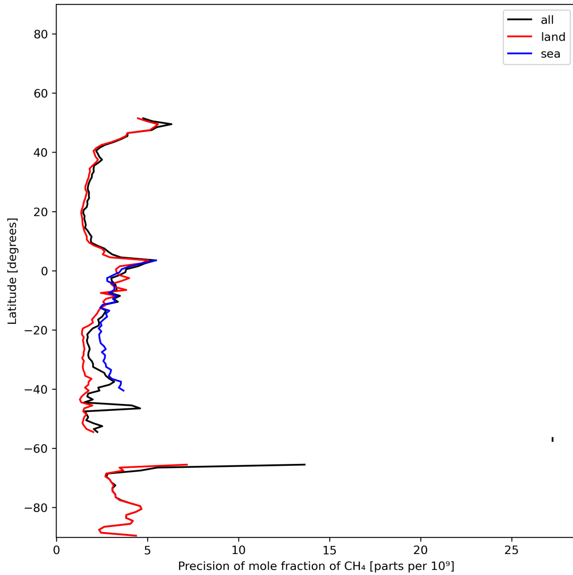
Figure 13: Zonal average of “Precision of mole fraction of \text{CH}_4 ” for 2023-12-26 to 2023-12-28.
