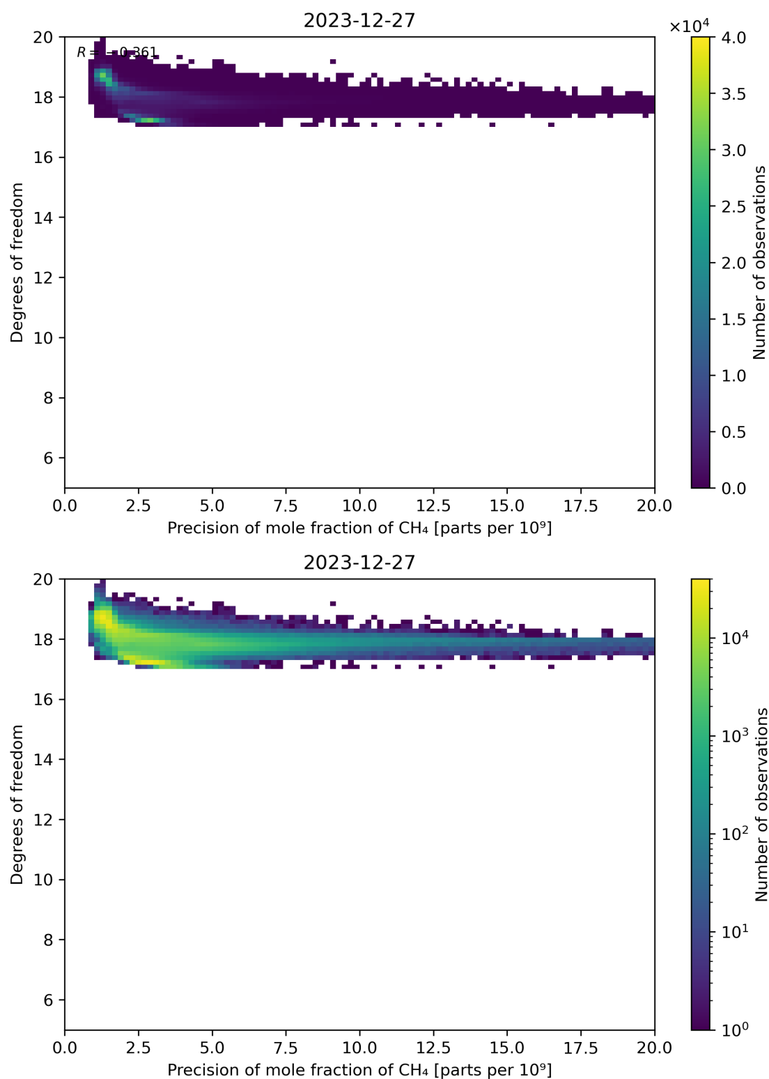
Figure 80: Scatter density plot of “Precision of mole fraction of CH 4 ” against “Degrees of freedom” for 2023-12-26 to 2023-12-28.
