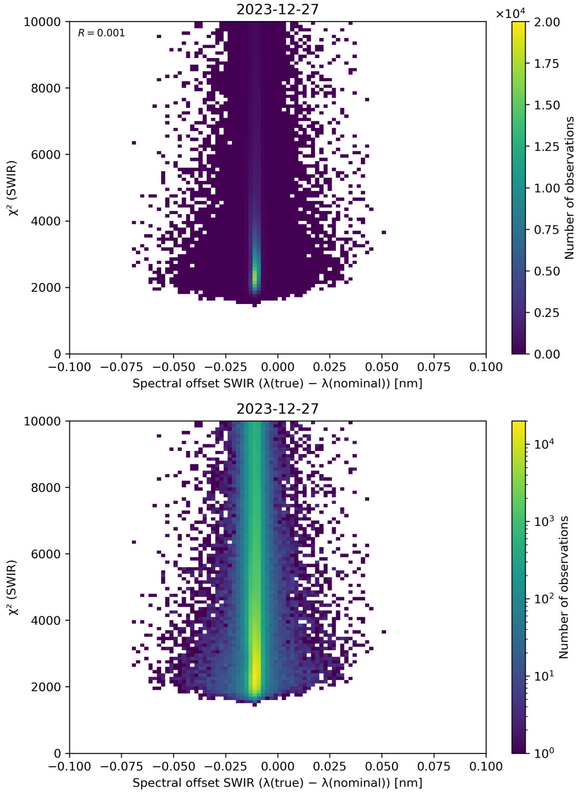
Figure 118: Scatter density plot of “Spectral offset SWIR ( \lambda(\text{true}) - \lambda(\text{nominal}) )” against “ \chi^2 (SWIR)” for 2023-12-26 to 2023-12-28.
