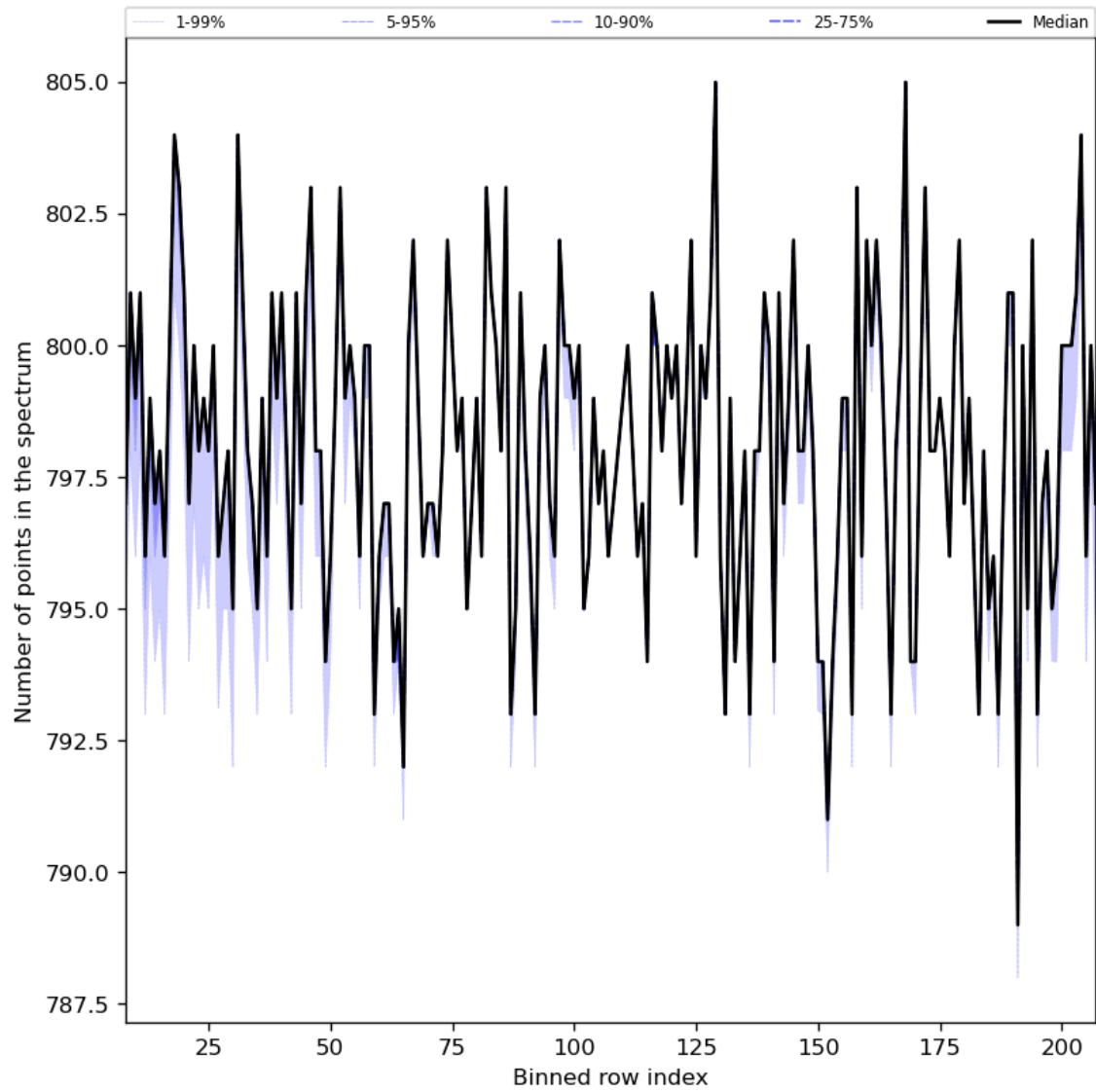
Figure 37: Along track statistics of “Number of points in the spectrum” for 2023-12-26 to 2023-12-28
