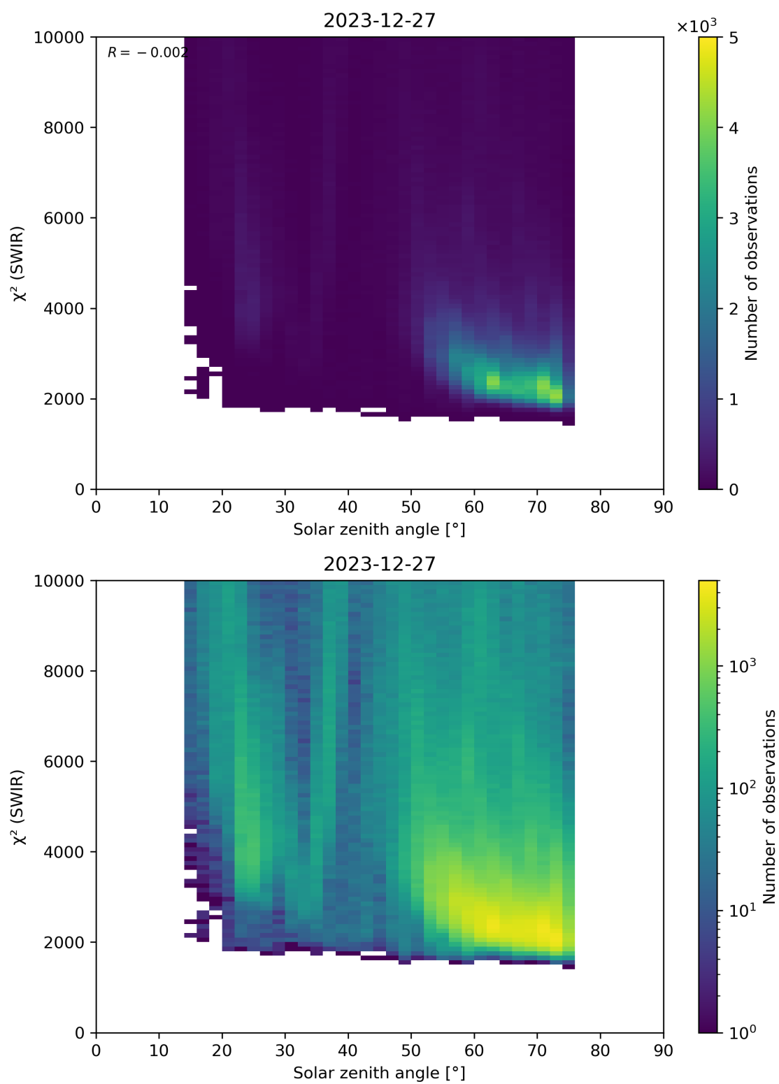
Figure 95: Scatter density plot of “Solar zenith angle” against “ \chi^2 (SWIR)” for 2023-12-26 to 2023-12-28.
