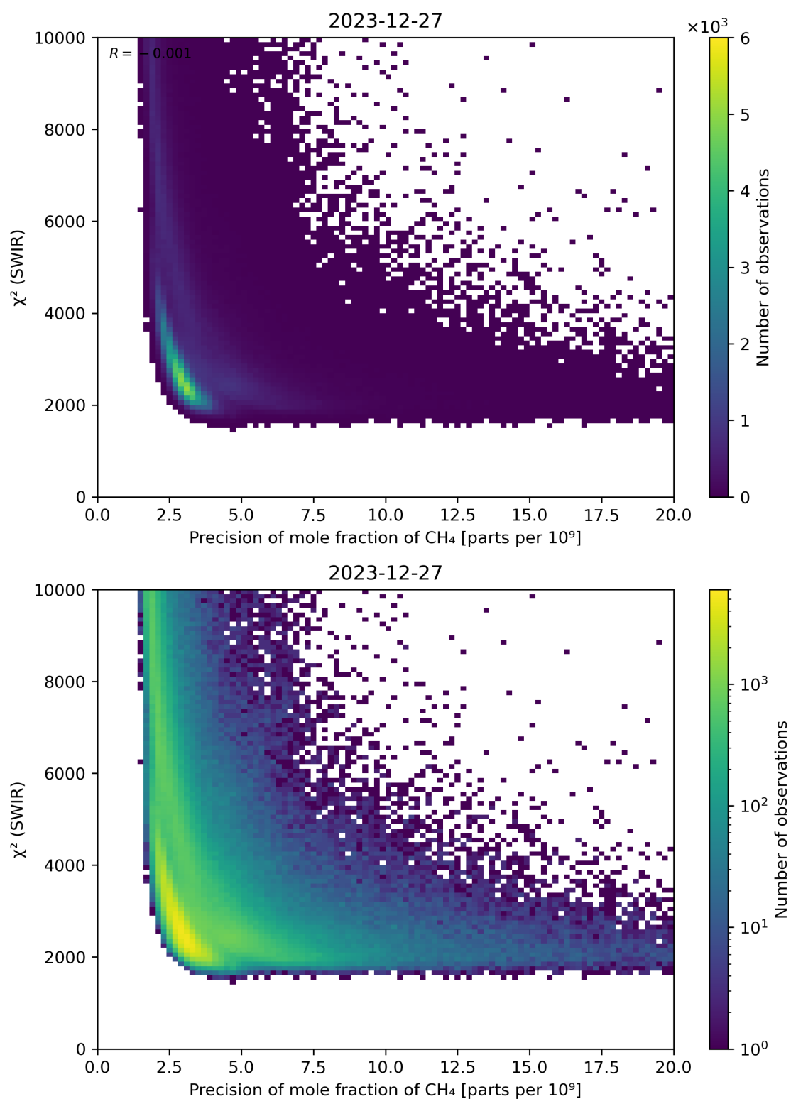
Figure 79: Scatter density plot of “Precision of mole fraction of CH 4 ” against “ \chi^2 (SWIR)” for 2023-12-26 to 2023-12-28.
