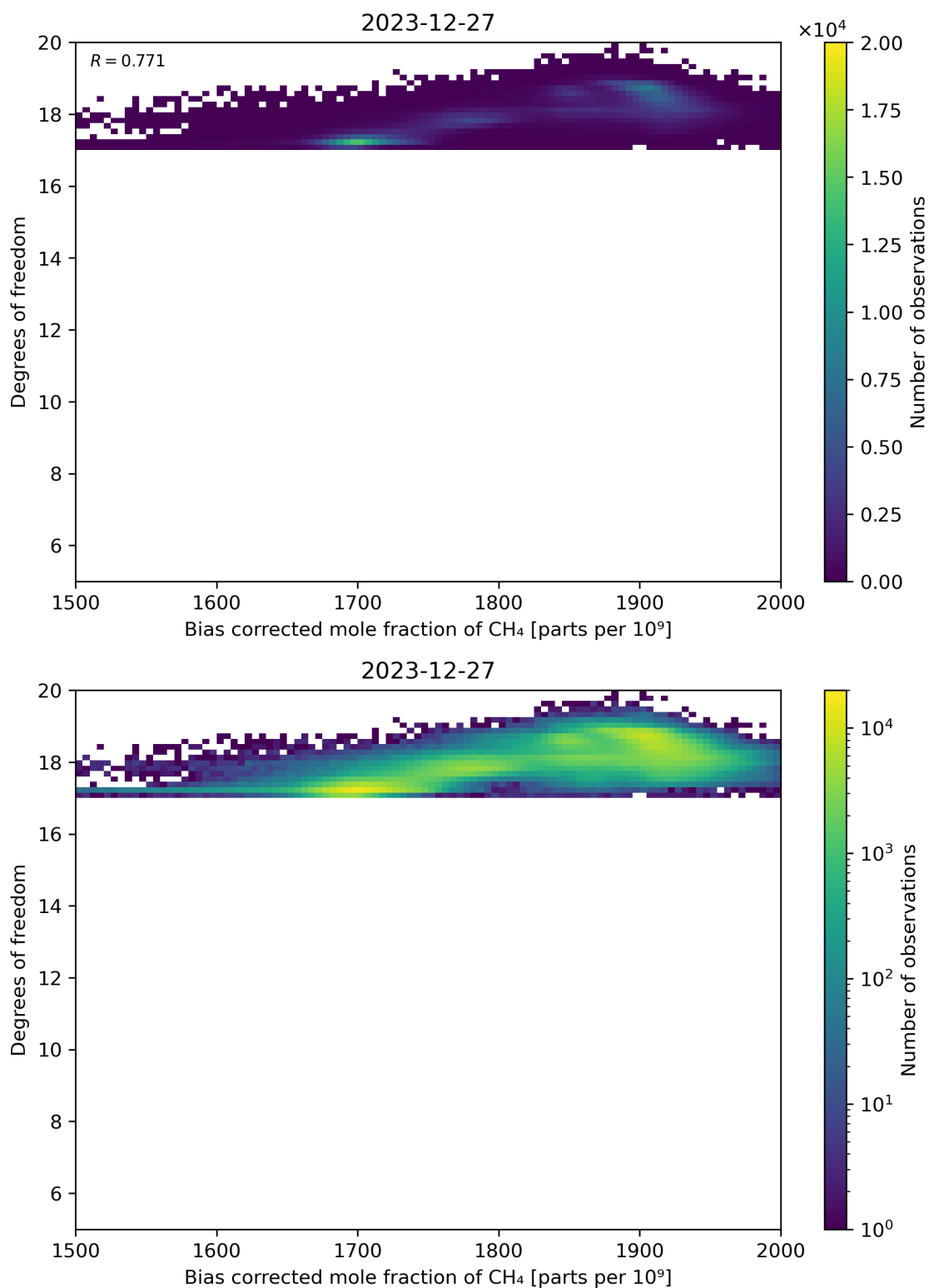
Figure 65: Scatter density plot of “Bias corrected mole fraction of CH 4 ” against “Degrees of freedom” for 2023-12-26 to 2023-12-28.
