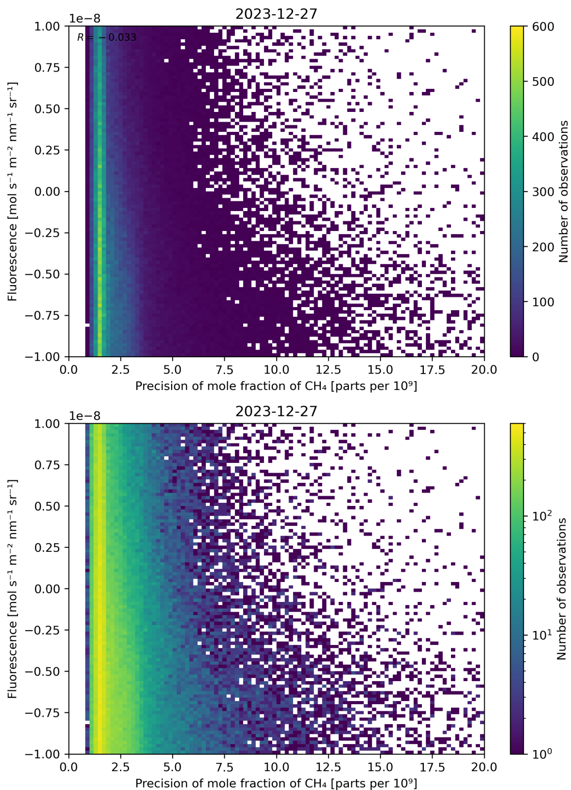
Figure 81: Scatter density plot of “Precision of mole fraction of \text{CH}_4 ” against “Fluorescence” for 2023-12-26 to 2023-12-28.
