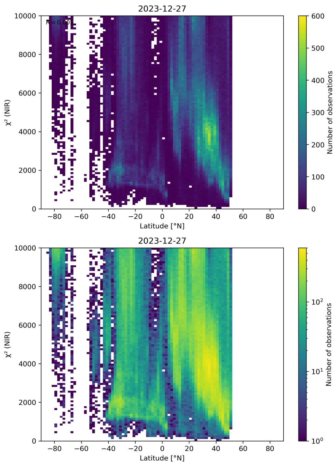
Figure 53: Scatter density plot of “Latitude” against “ \chi^2 (NIR)” for 2023-12-26 to 2023-12-28.
