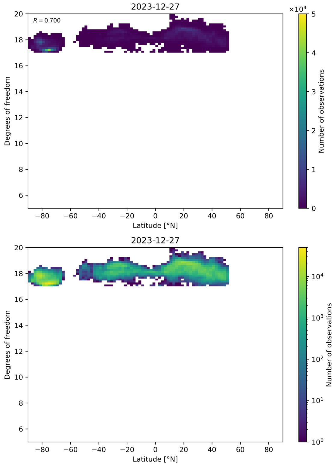
Figure 55: Scatter density plot of “Latitude” against “Degrees of freedom” for 2023-12-26 to 2023-12-28.
