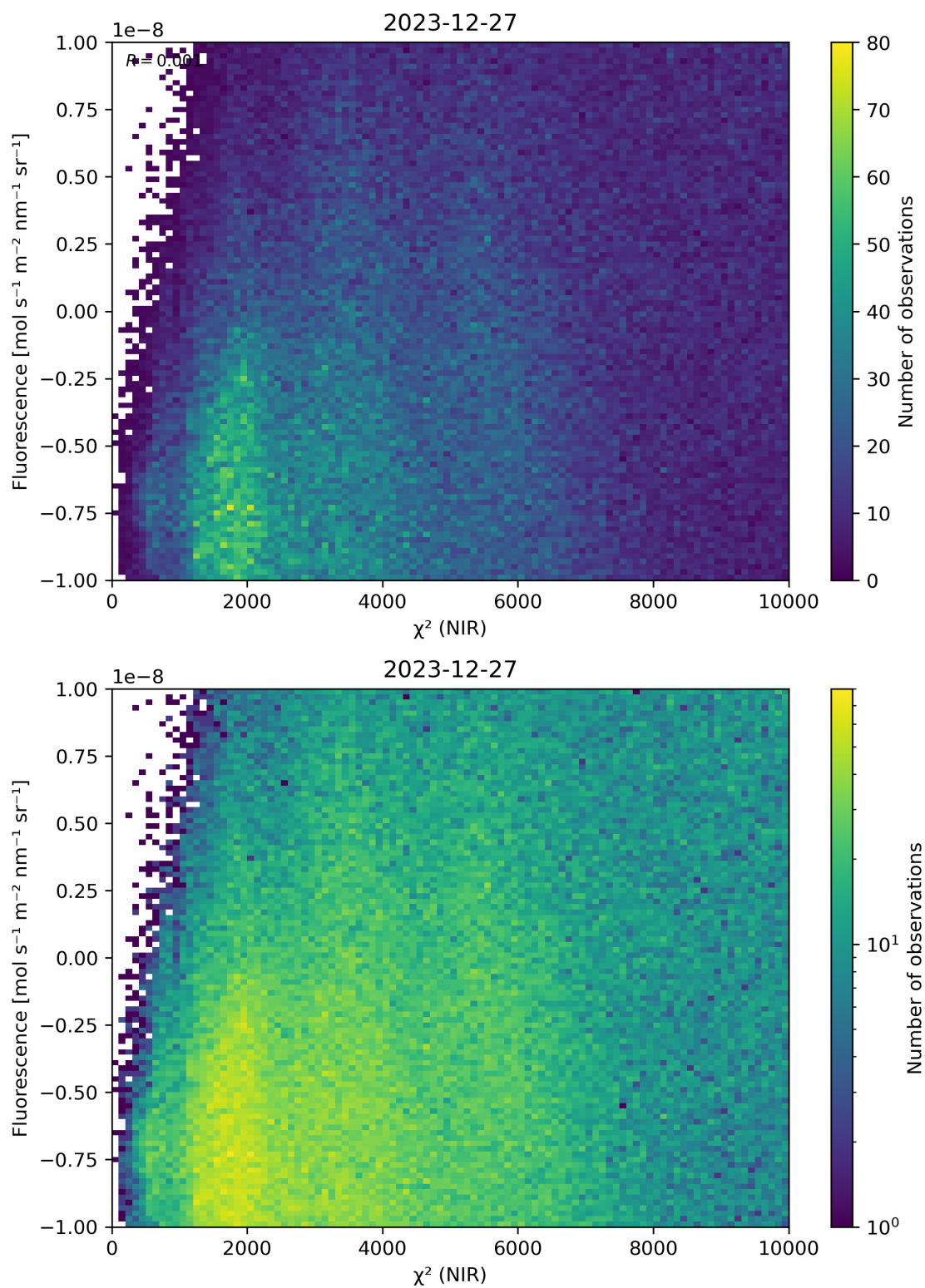
Figure 45: Scatter density plot of “ \chi^2 (NIR)” against “Fluorescence” for 2023-12-26 to 2023-12-28.
