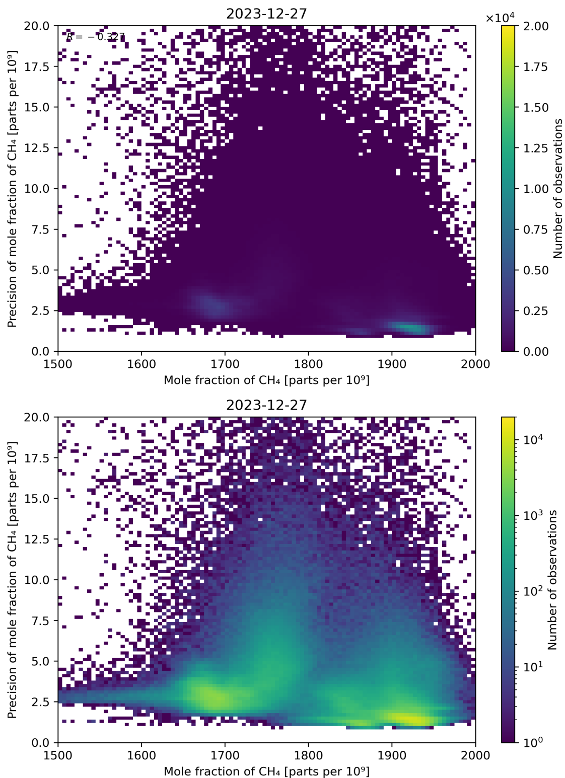
Figure 75: Scatter density plot of “Mole fraction of CH 4 ” against “Precision of mole fraction of CH 4 ” for 2023-12-26 to 2023-12-28.
