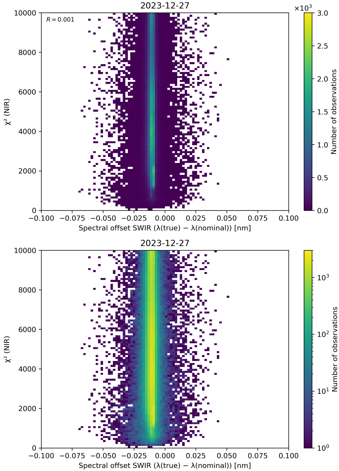
Figure 117: Scatter density plot of “Spectral offset SWIR ( \lambda(\text{true}) - \lambda(\text{nominal}) )” against “ \chi^2 (NIR)” for 2023-12-26 to 2023-12-28.
