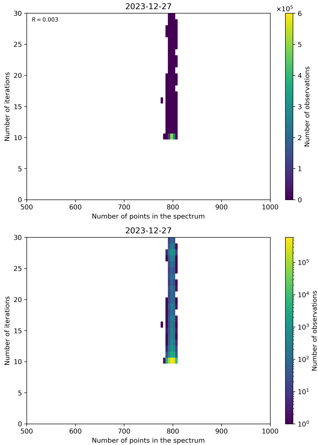
Figure 92: Scatter density plot of “Number of points in the spectrum” against “Number of iterations” for 2023-12-26 to 2023-12-28.
