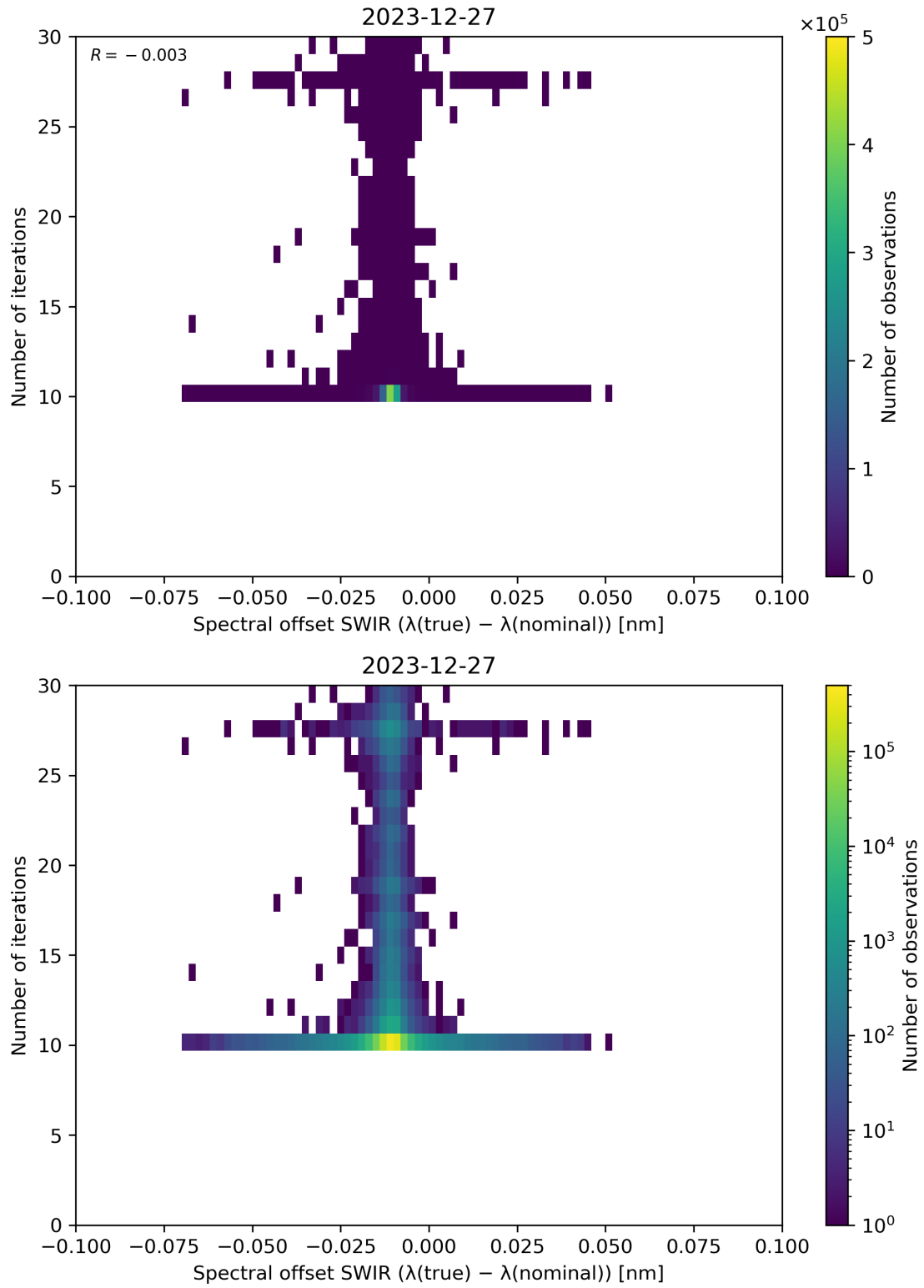
Figure 121: Scatter density plot of “Spectral offset SWIR ( \lambda(\text{true}) - \lambda(\text{nominal}) )” against “Number of iterations” for 2023-12-26 to 2023-12-28.
