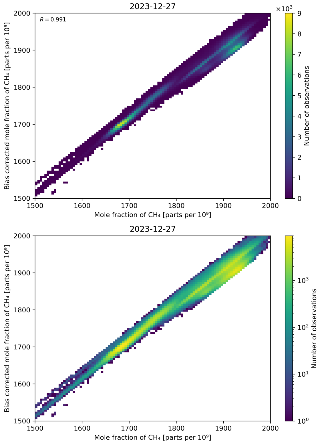
Figure 74: Scatter density plot of “Mole fraction of CH 4 ” against “Bias corrected mole fraction of CH 4 ” for 2023-12-26 to 2023-12-28.
