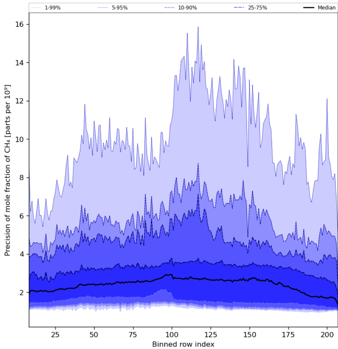
Figure 35: Along track statistics of “Precision of mole fraction of CH 4 ” for 2023-12-26 to 2023-12-28
