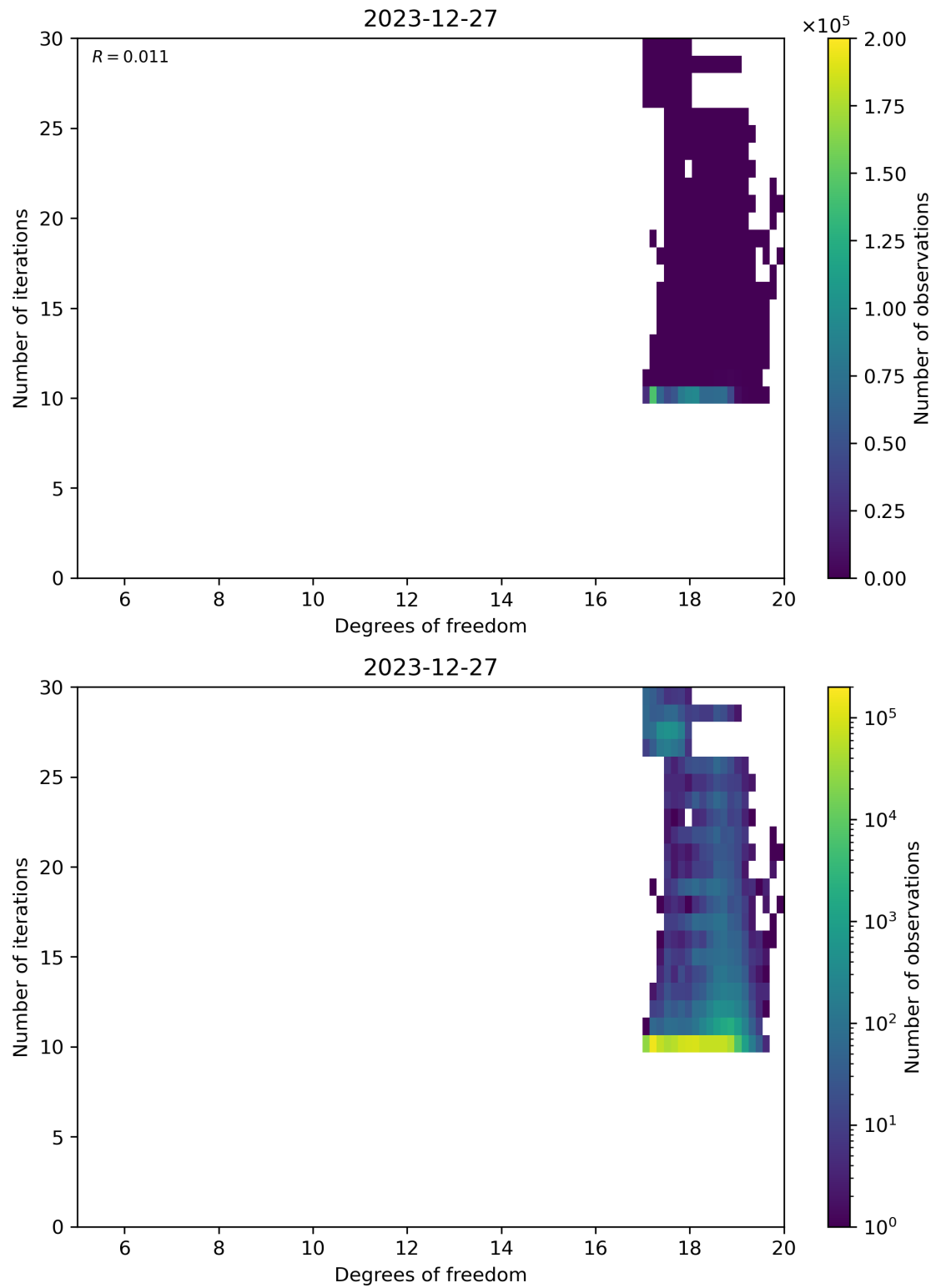
Figure 52: Scatter density plot of “Degrees of freedom” against “Number of iterations” for 2023-12-26 to 2023-12-28.
