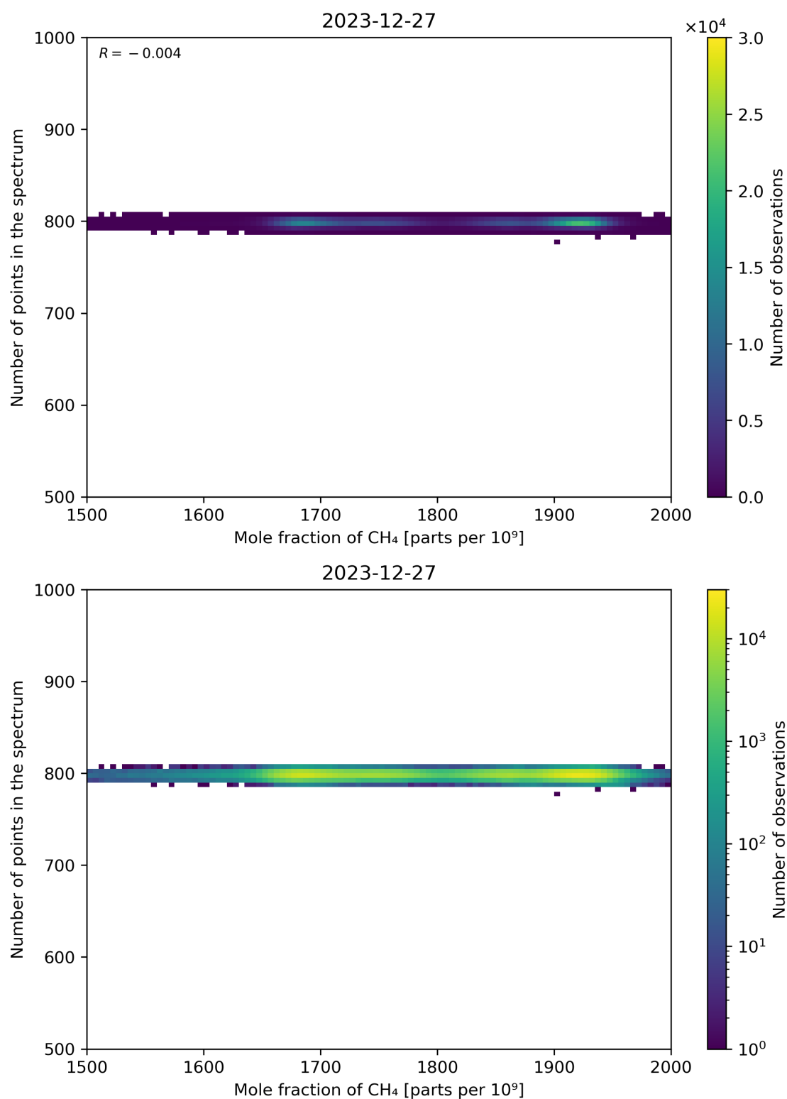
Figure 77: Scatter density plot of “Mole fraction of CH 4 ” against “Number of points in the spectrum” for 2023-12-26 to 2023-12-28.
