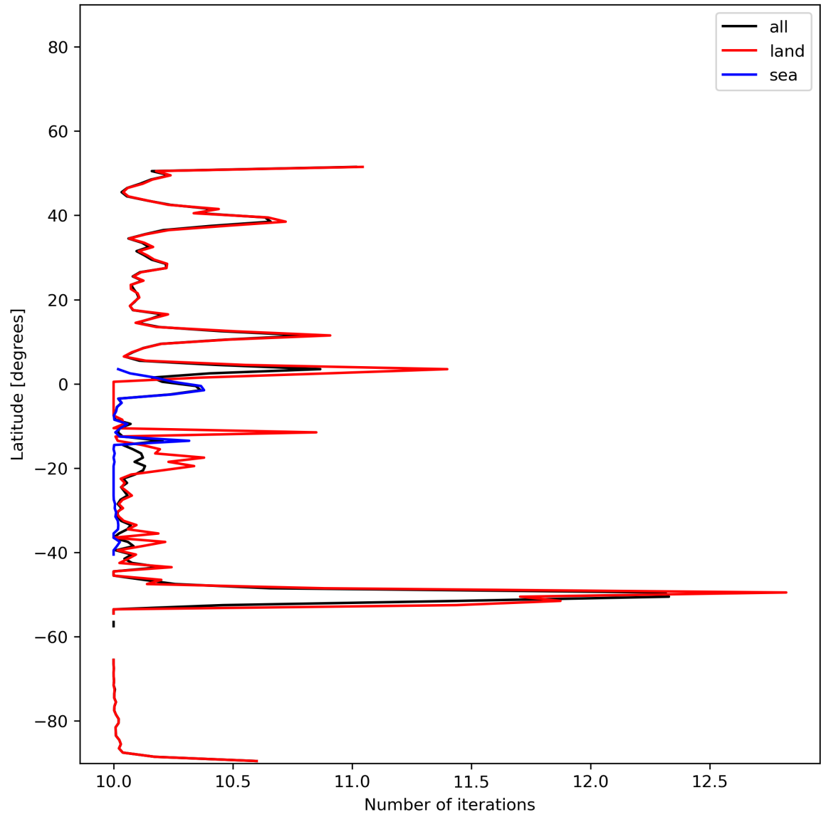
Figure 20: Zonal average of “Number of iterations” for 2023-12-26 to 2023-12-28.
