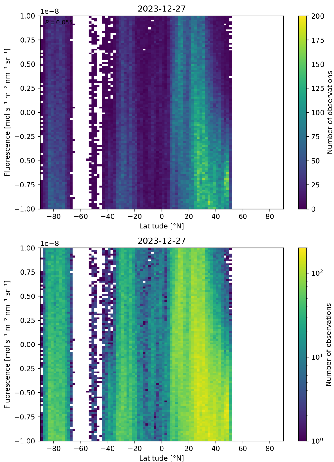
Figure 56: Scatter density plot of “Latitude” against “Fluorescence” for 2023-12-26 to 2023-12-28.
