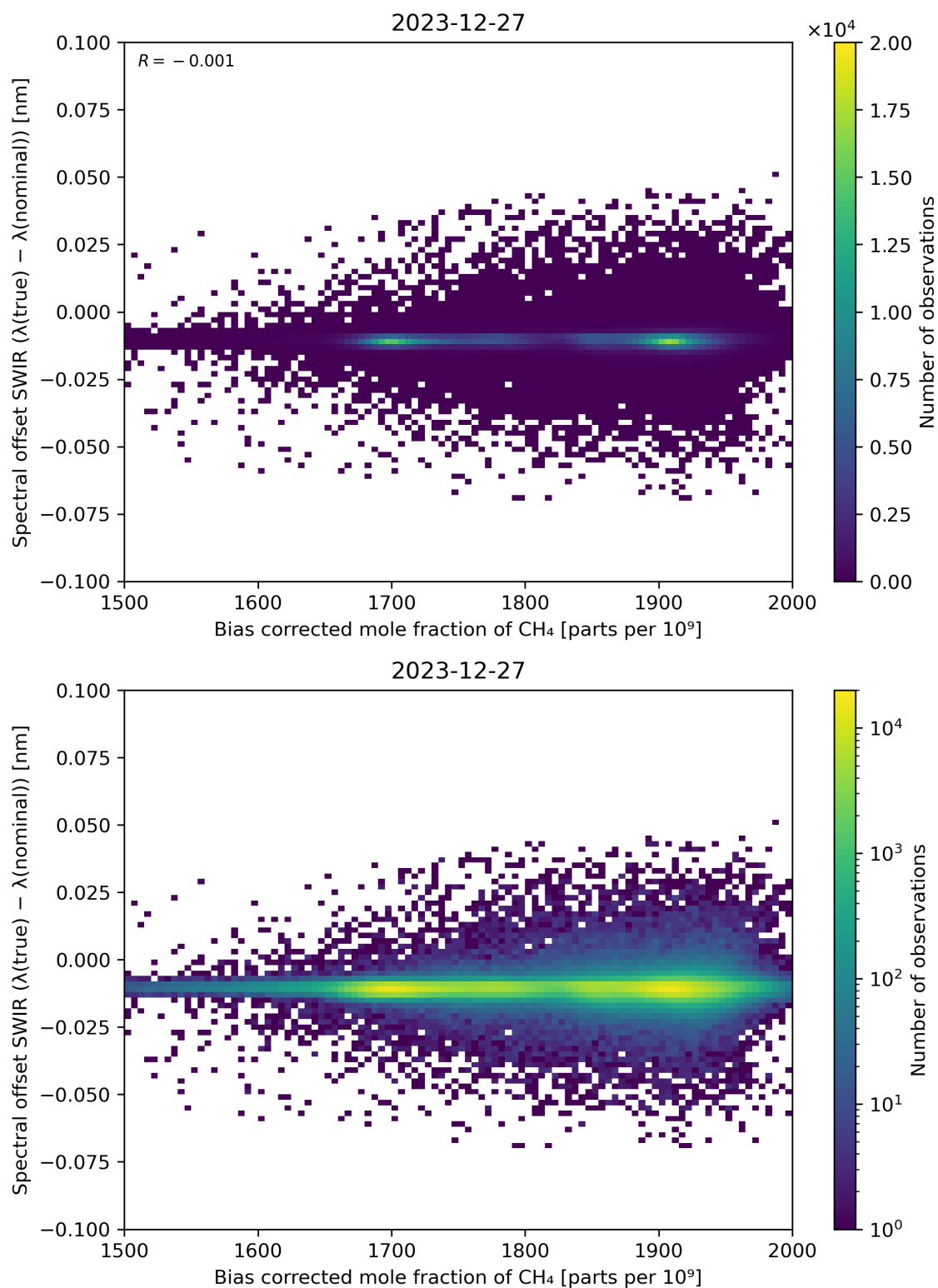
Figure 69: Scatter density plot of “Bias corrected mole fraction of \text{CH}_4 ” against “Spectral offset SWIR ( \lambda(\text{true}) - \lambda(\text{nominal}) )” for 2023-12-26 to 2023-12-28.
