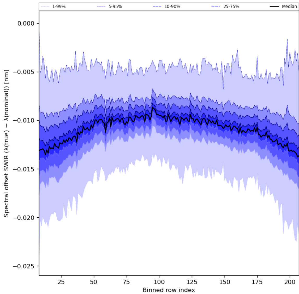
Figure 38: Along track statistics of “Spectral offset SWIR ( \lambda(\text{true}) - \lambda(\text{nominal}) )” for 2023-12-26 to 2023-12-28
