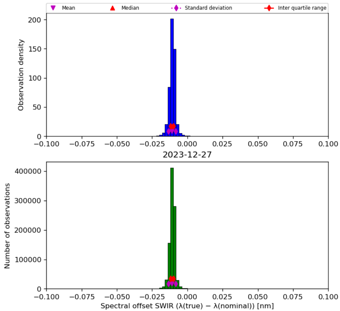
Figure 27: Histogram of “Spectral offset SWIR ( \lambda(\text{true}) - \lambda(\text{nominal}) )” for 2023-12-26 to 2023-12-28
