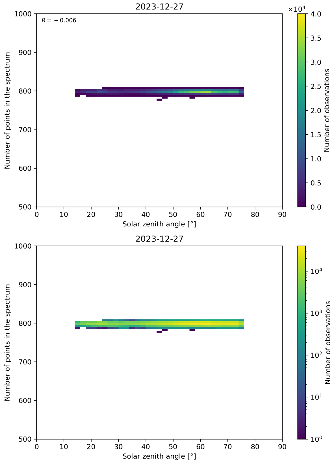
Figure 103: Scatter density plot of “Solar zenith angle” against “Number of points in the spectrum” for 2023-12-26 to 2023-12-28.
