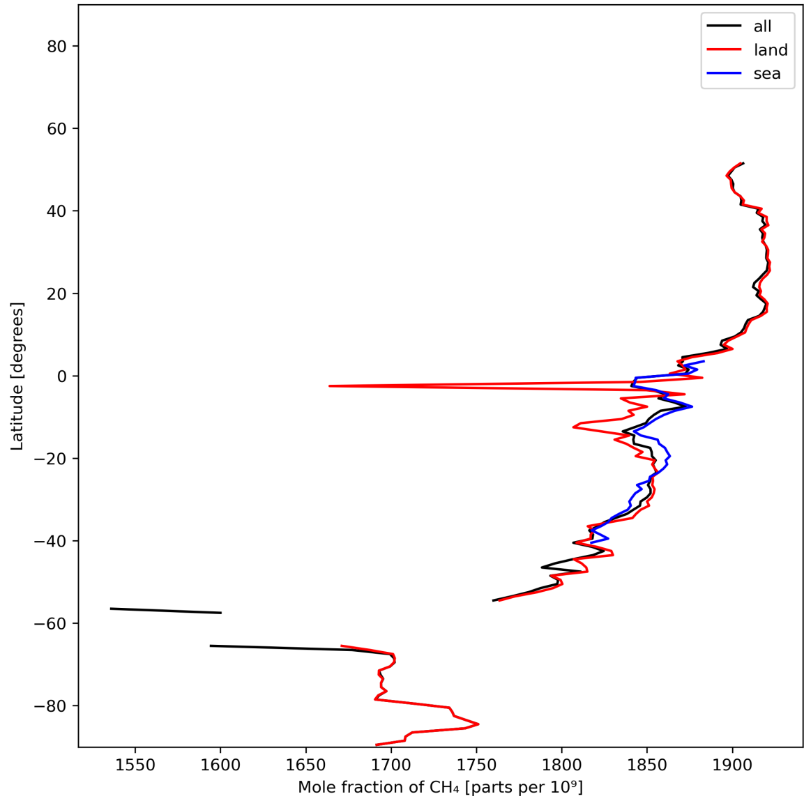
Figure 12: Zonal average of “Mole fraction of \text{CH}_4 ” for 2023-12-26 to 2023-12-28.
