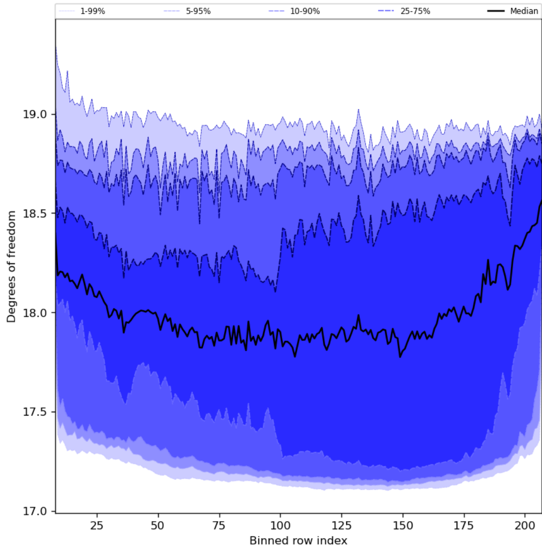
Figure 41: Along track statistics of “Degrees of freedom” for 2023-12-26 to 2023-12-28
