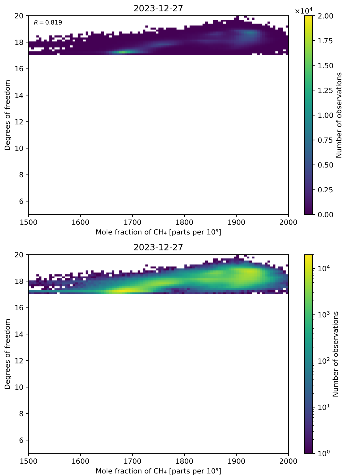
Figure 72: Scatter density plot of “Mole fraction of CH 4 ” against “Degrees of freedom” for 2023-12-26 to 2023-12-28.
