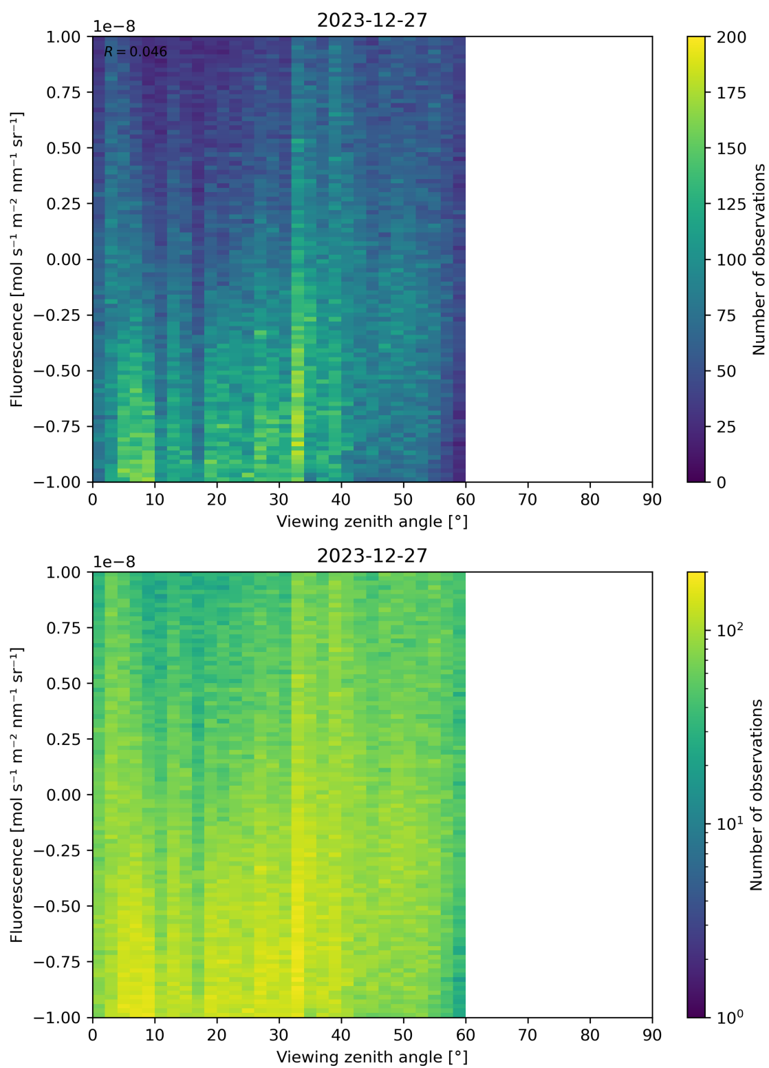
Figure 108: Scatter density plot of “Viewing zenith angle” against “Fluorescence” for 2023-12-26 to 2023-12-28.
