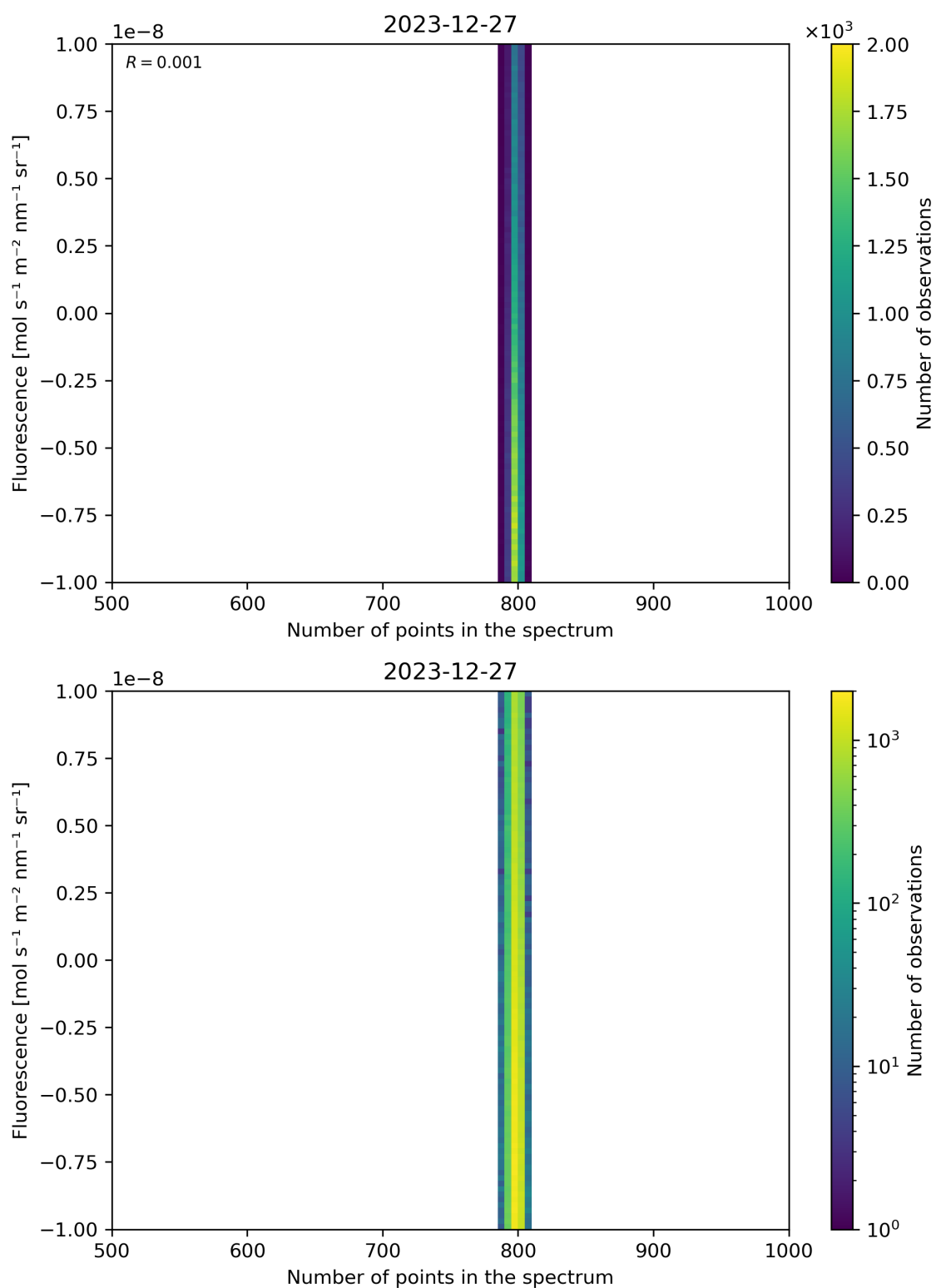
Figure 91: Scatter density plot of “Number of points in the spectrum” against “Fluorescence” for 2023-12-26 to 2023-12-28.
