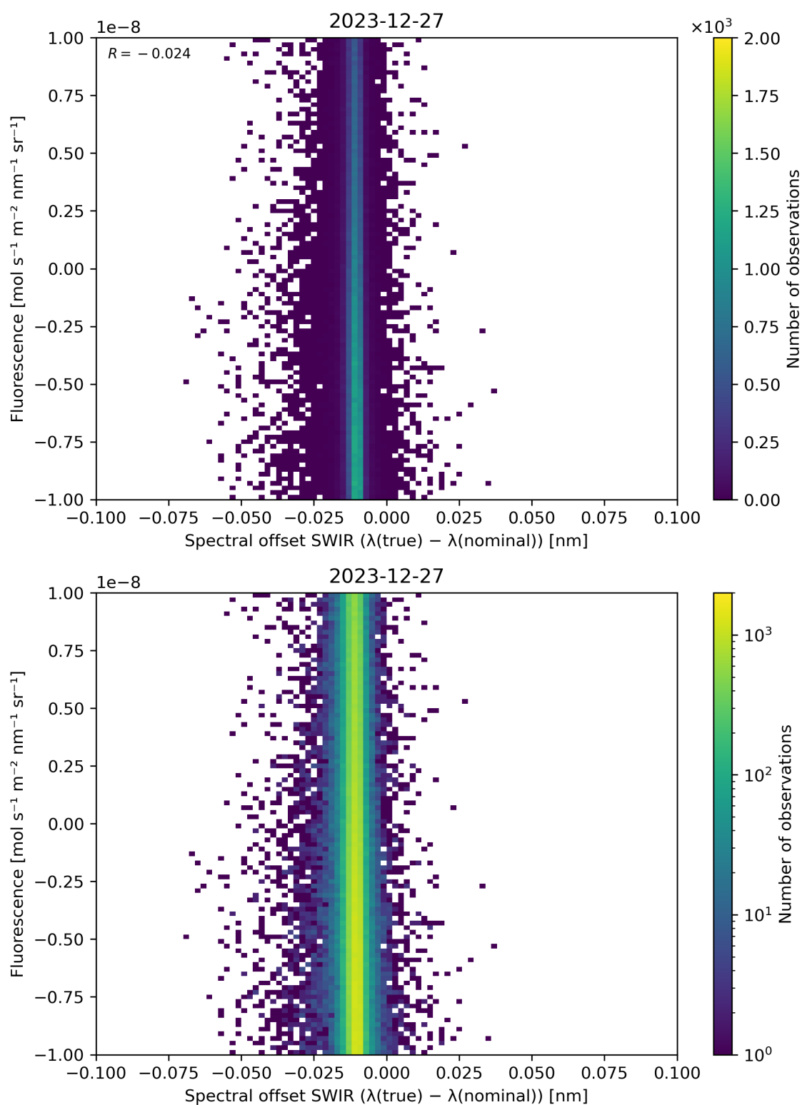
Figure 120: Scatter density plot of “Spectral offset SWIR ( \lambda(\text{true}) - \lambda(\text{nominal}) )” against “Fluorescence” for 2023-12-26 to 2023-12-28.
