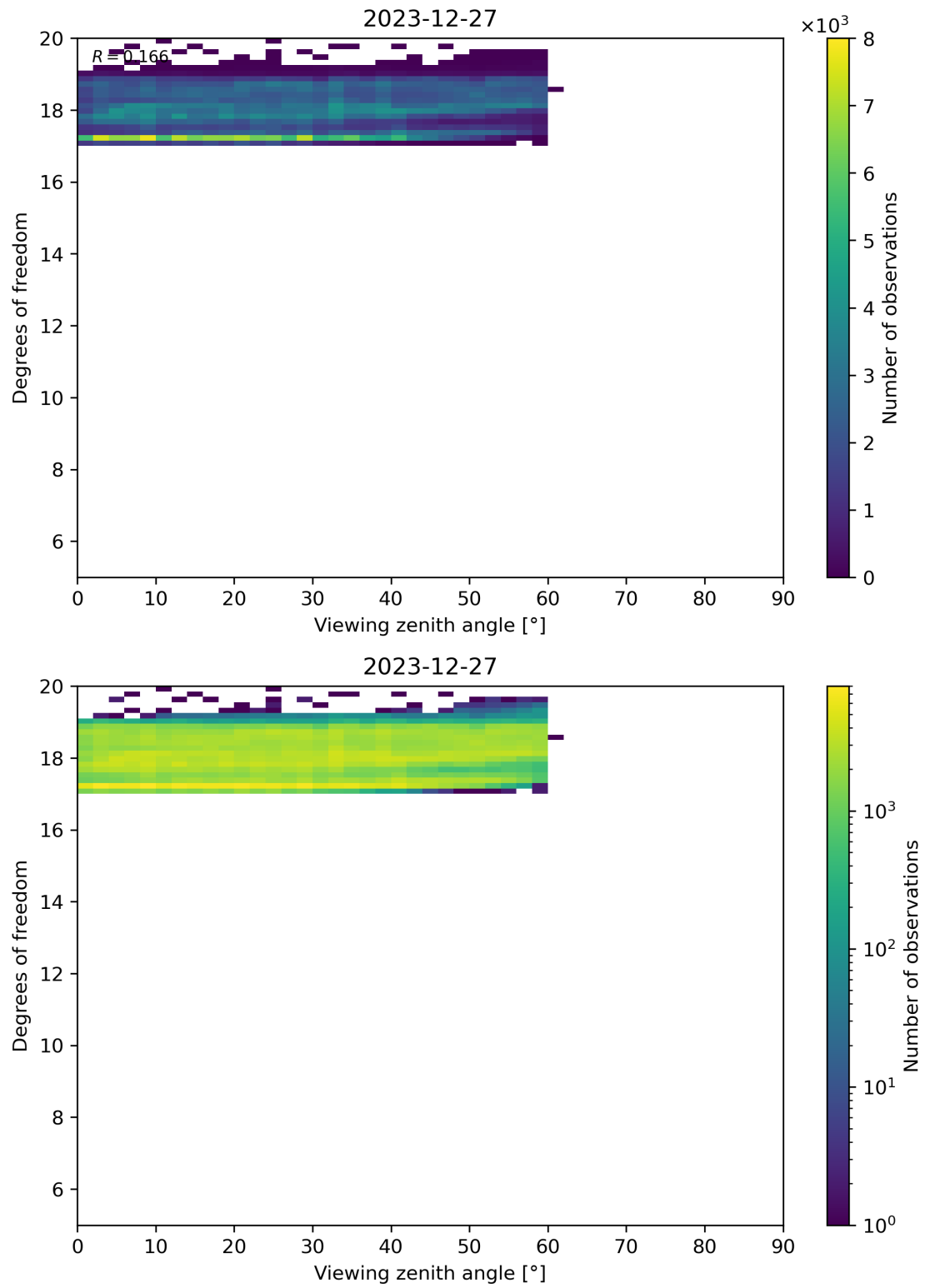
Figure 107: Scatter density plot of “Viewing zenith angle” against “Degrees of freedom” for 2023-12-26 to 2023-12-28.
