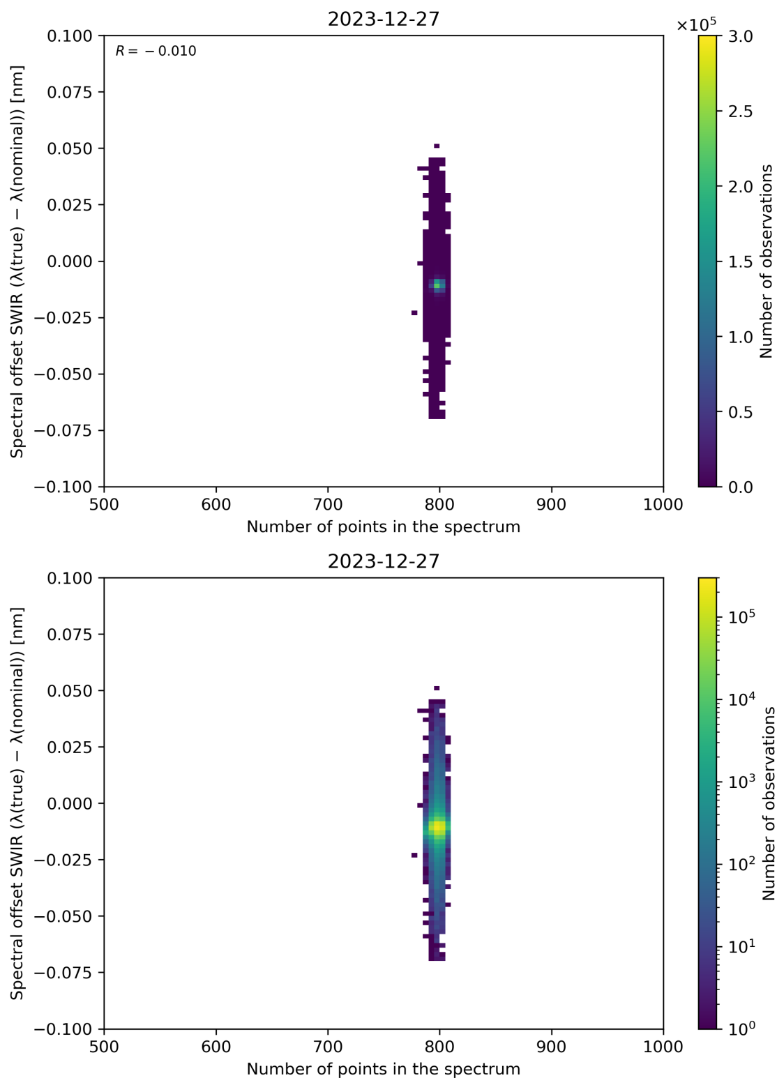
Figure 93: Scatter density plot of “Number of points in the spectrum” against “Spectral offset SWIR ( \lambda(\text{true}) - \lambda(\text{nominal}) )” for 2023-12-26 to 2023-12-28.
