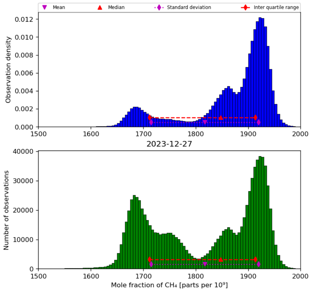
Figure 23: Histogram of “Mole fraction of CH 4 ” for 2023-12-26 to 2023-12-28
