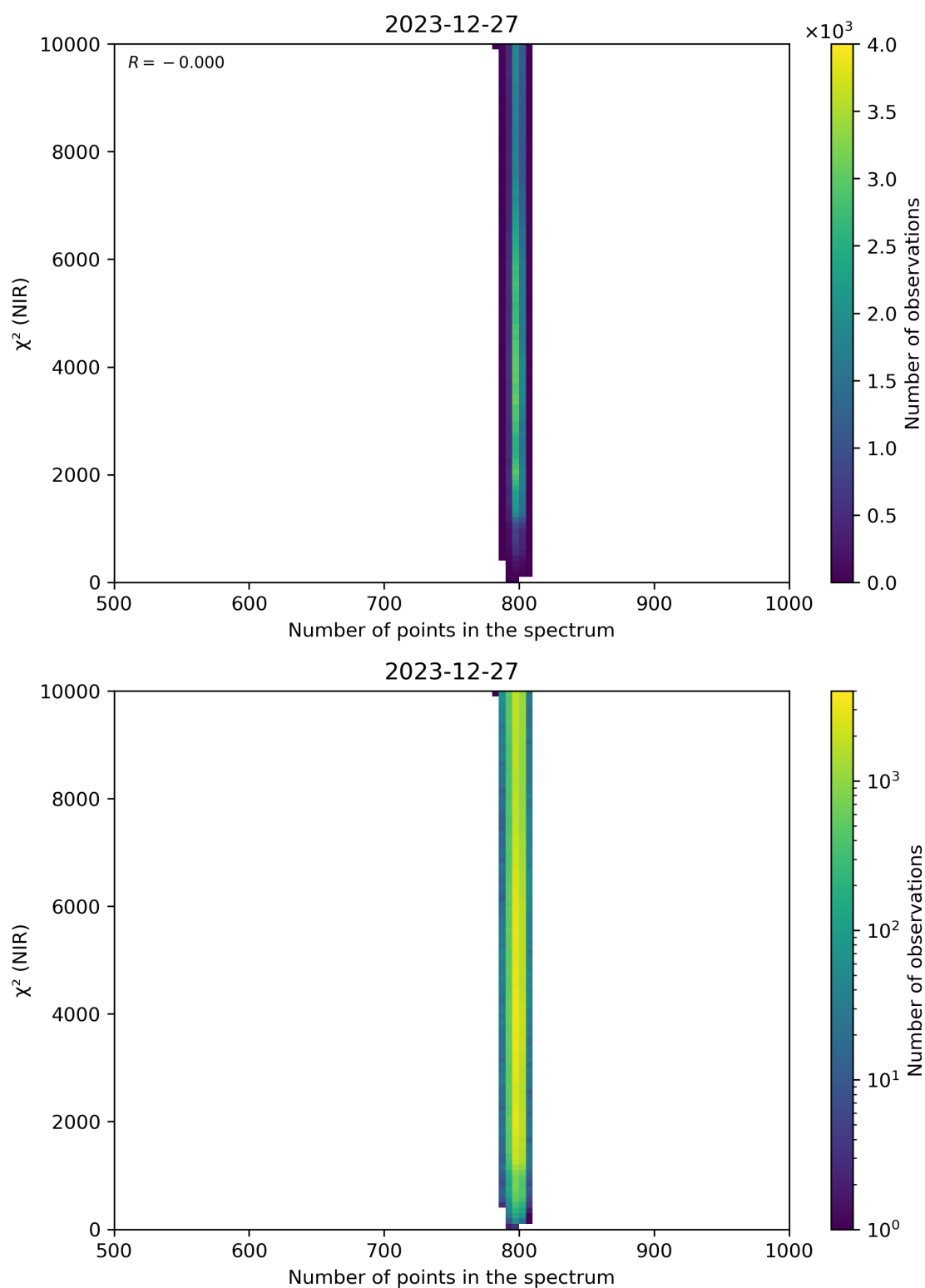
Figure 88: Scatter density plot of “Number of points in the spectrum” against “ \chi^2 (NIR)” for 2023-12-26 to 2023-12-28.
