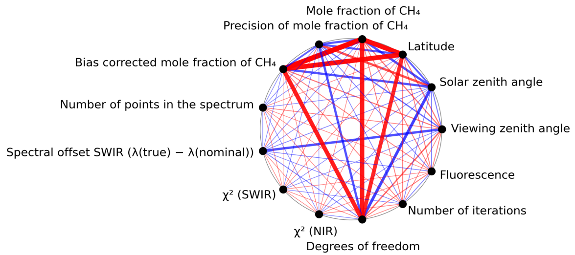
Figure 1: Map of correlation graph for 2023-12-26 to 2023-12-28.
