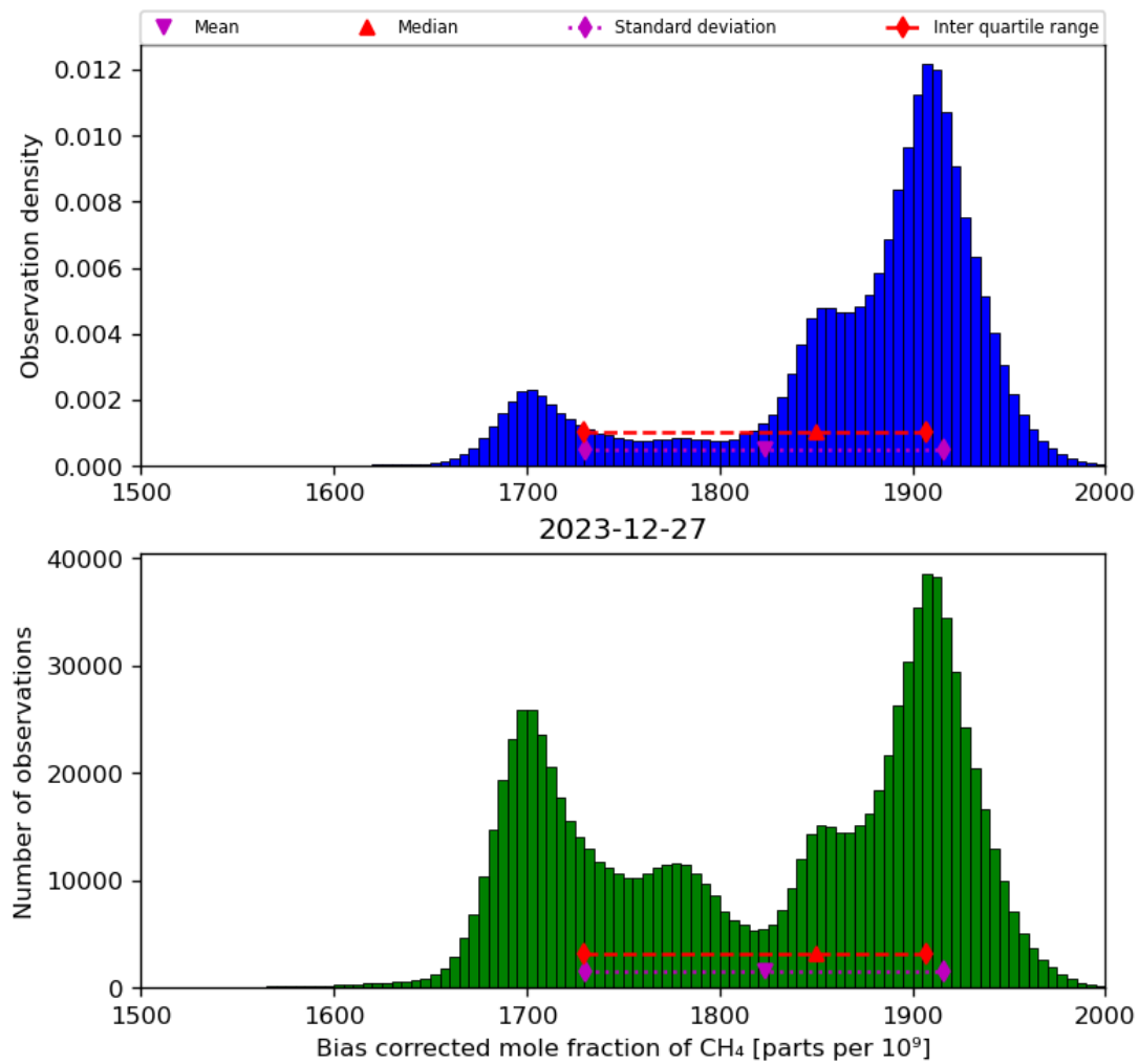
Figure 25: Histogram of “Bias corrected mole fraction of CH 4 ” for 2023-12-26 to 2023-12-28
