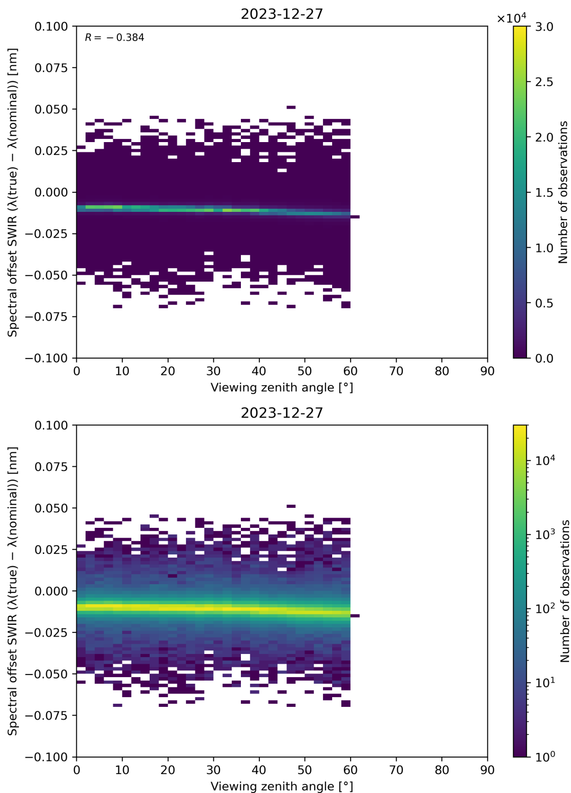
Figure 116: Scatter density plot of “Viewing zenith angle” against “Spectral offset SWIR ( \lambda(\text{true}) - \lambda(\text{nominal}) )” for 2023-12-26 to 2023-12-28.
