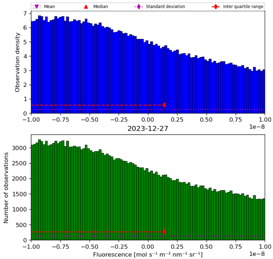
Figure 32: Histogram of “Fluorescence” for 2023-12-26 to 2023-12-28
