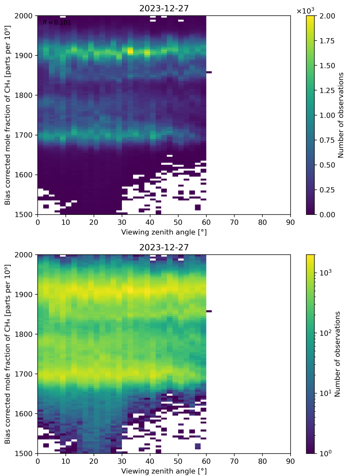
Figure 111: Scatter density plot of “Viewing zenith angle” against “Bias corrected mole fraction of \text{CH}_4 ” for 2023-12-26 to 2023-12-28.
