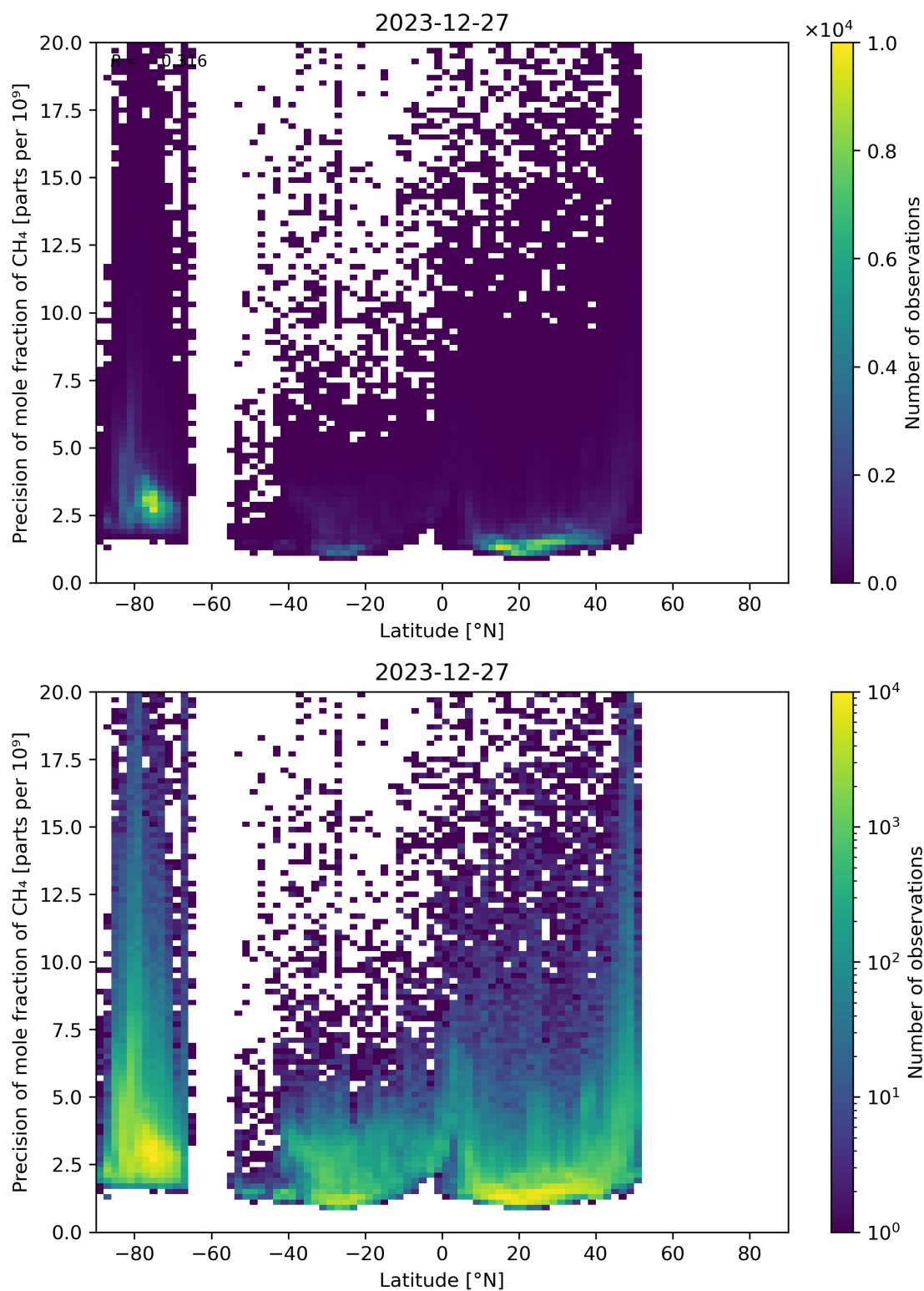
Figure 59: Scatter density plot of “Latitude” against “Precision of mole fraction of CH 4 ” for 2023-12-26 to 2023-12-28.
