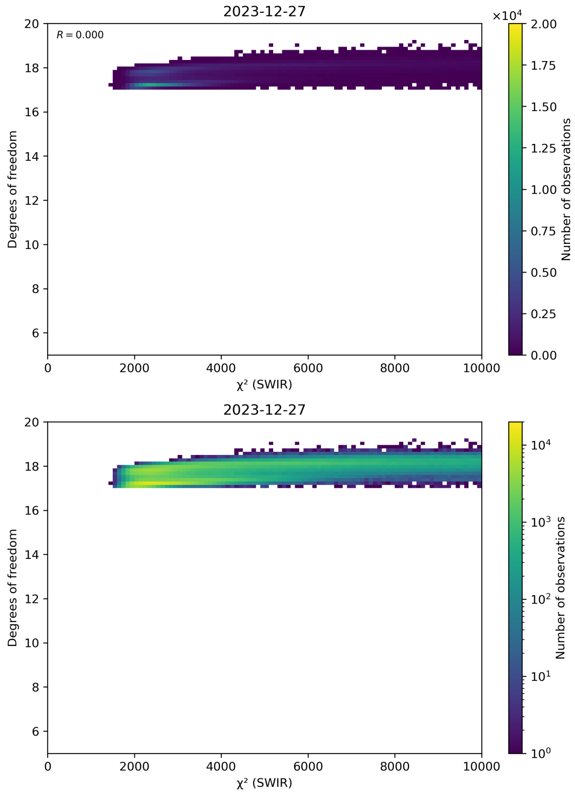
Figure 48: Scatter density plot of “ \chi^2 (SWIR)” against “Degrees of freedom” for 2023-12-26 to 2023-12-28.
