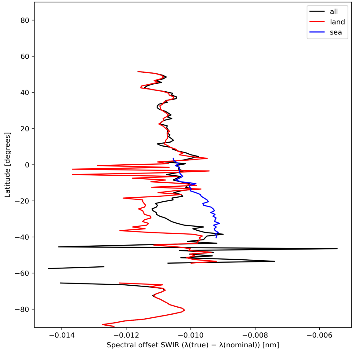
Figure 16: Zonal average of “Spectral offset SWIR ( \lambda(\text{true}) - \lambda(\text{nominal}) )” for 2023-12-26 to 2023-12-28.
