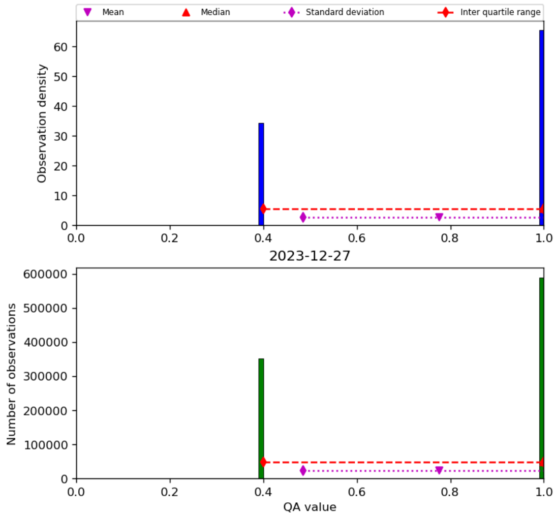
Figure 22: Histogram of “QA value” for 2023-12-26 to 2023-12-28
