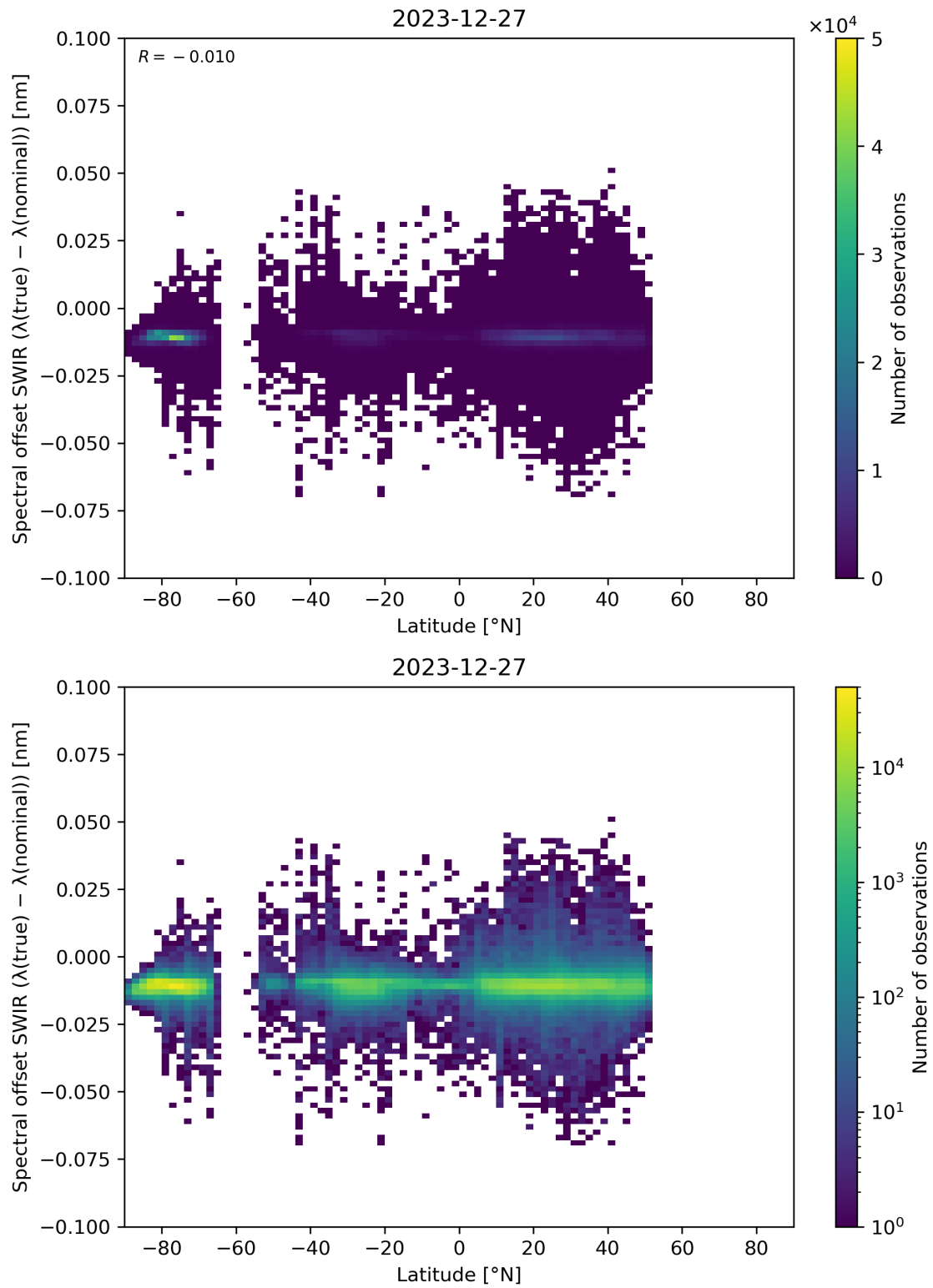
Figure 62: Scatter density plot of “Latitude” against “Spectral offset SWIR ( \lambda(\text{true}) - \lambda(\text{nominal}) )” for 2023-12-26 to 2023-12-28.
