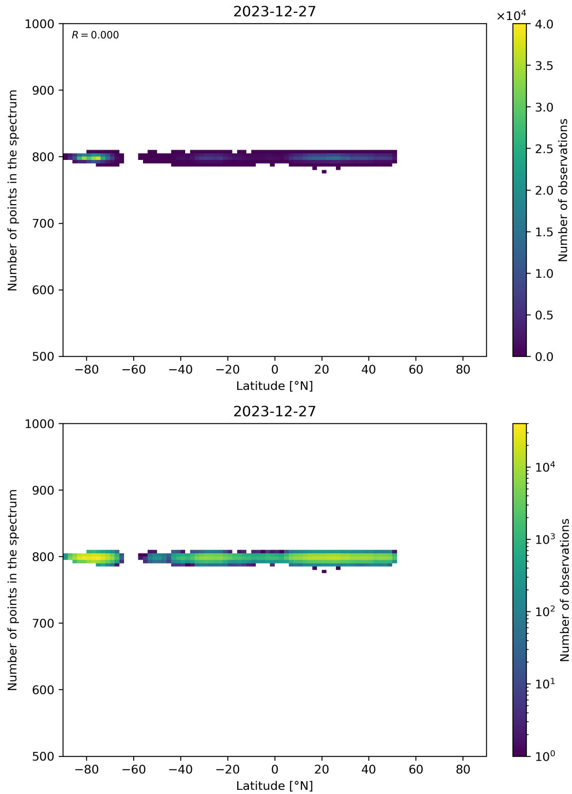
Figure 61: Scatter density plot of “Latitude” against “Number of points in the spectrum” for 2023-12-26 to 2023-12-28.
