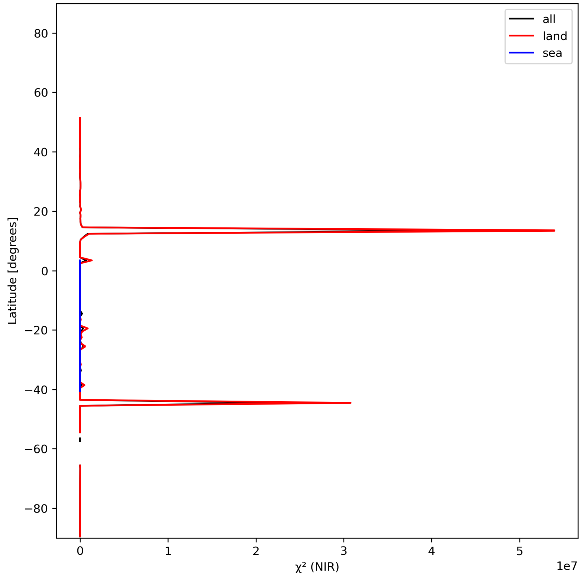
Figure 18: Zonal average of “ \chi^2 (NIR)” for 2023-12-26 to 2023-12-28.
