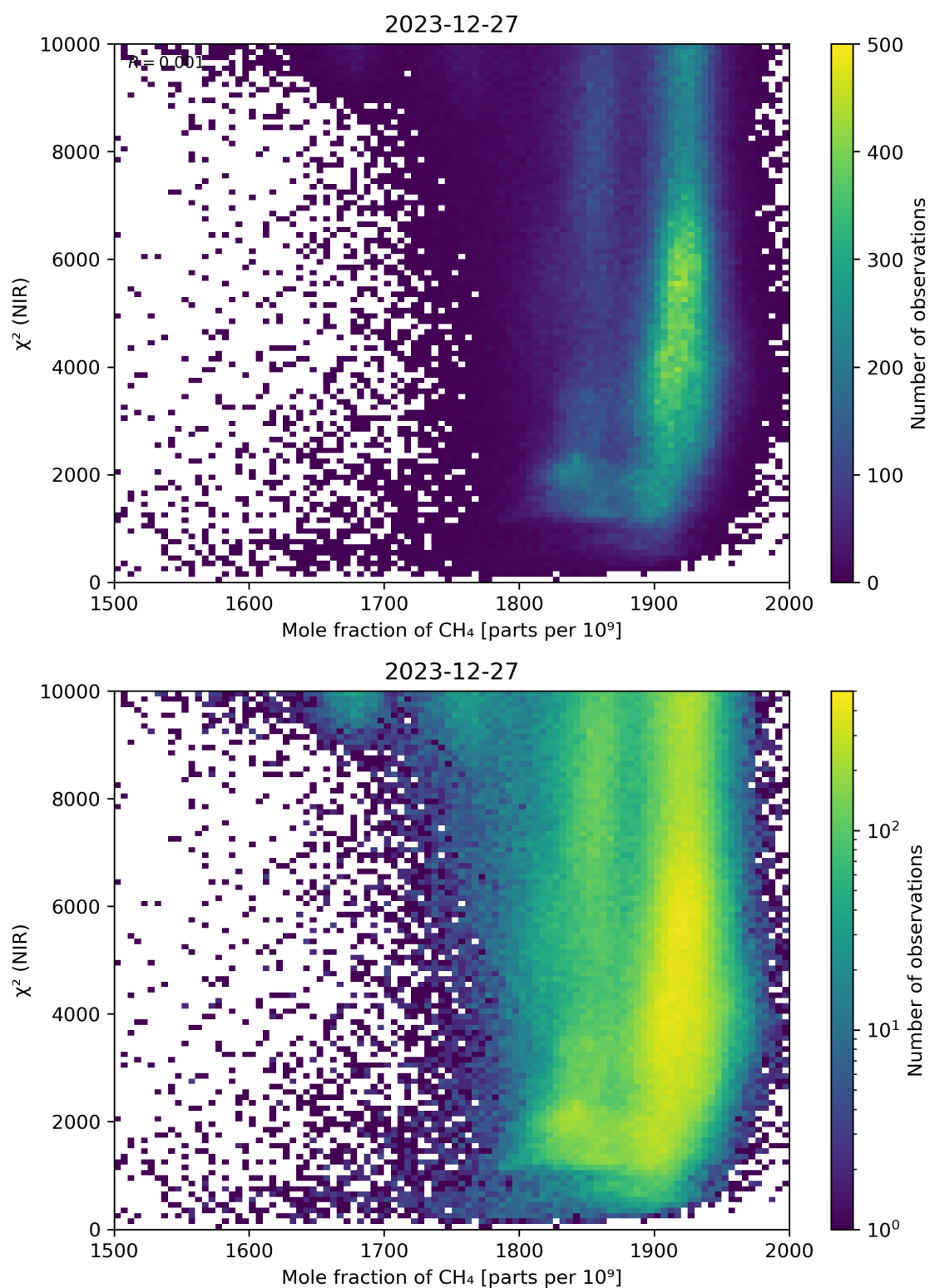
Figure 70: Scatter density plot of “Mole fraction of \text{CH}_4 ” against “ \chi^2 (NIR)” for 2023-12-26 to 2023-12-28.
