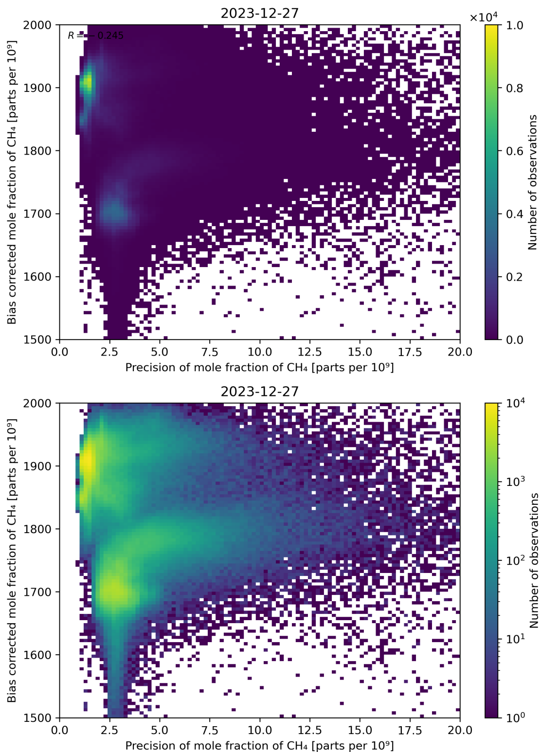
Figure 82: Scatter density plot of “Precision of mole fraction of CH 4 ” against “Bias corrected mole fraction of CH 4 ” for 2023-12-26 to 2023-12-28.
