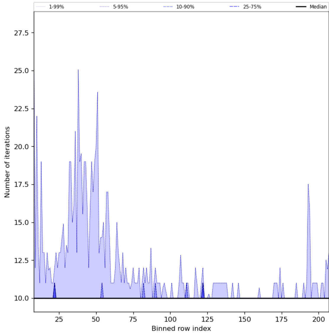
Figure 42: Along track statistics of “Number of iterations” for 2023-12-26 to 2023-12-28
