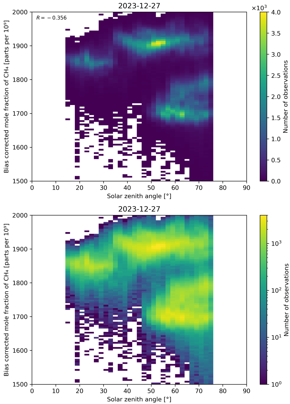
Figure 100: Scatter density plot of “Solar zenith angle” against “Bias corrected mole fraction of CH 4 ” for 2023-12-26 to 2023-12-28.
