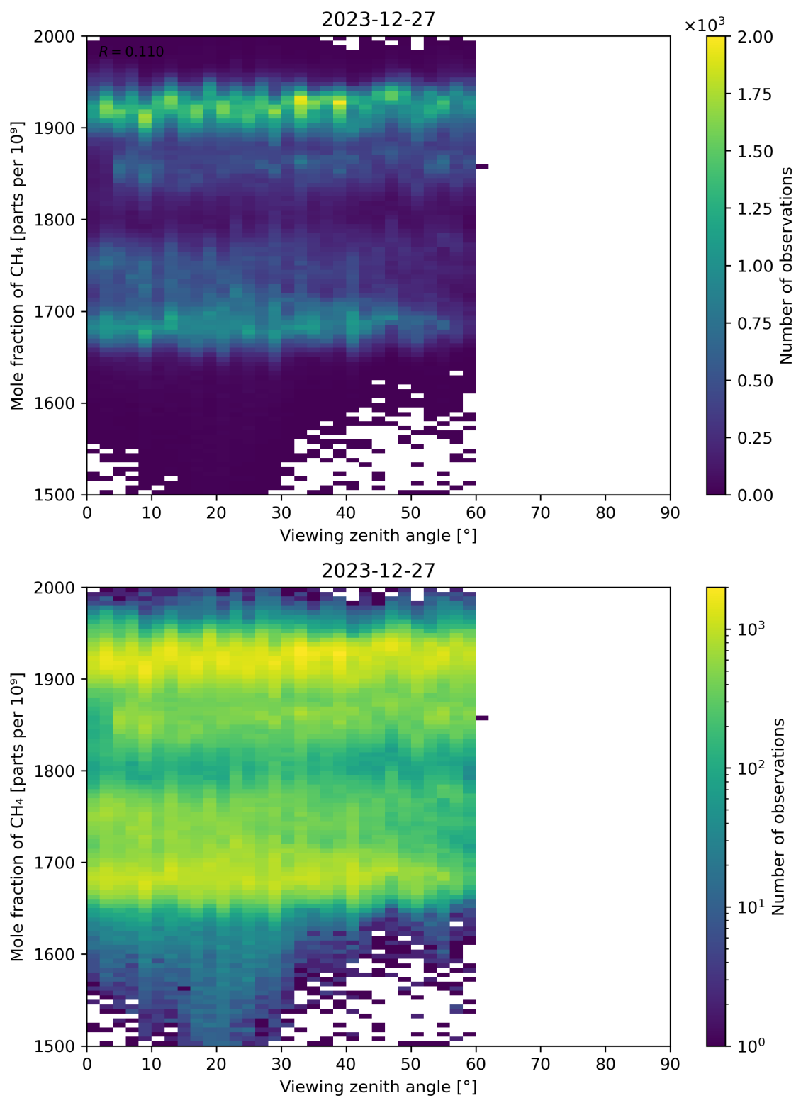
Figure 110: Scatter density plot of “Viewing zenith angle” against “Mole fraction of CH 4 ” for 2023-12-26 to 2023-12-28.
