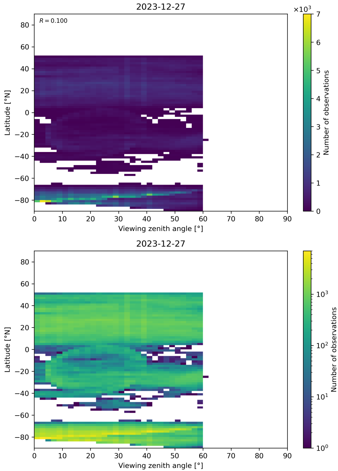
Figure 109: Scatter density plot of “Viewing zenith angle” against “Latitude” for 2023-12-26 to 2023-12-28.
