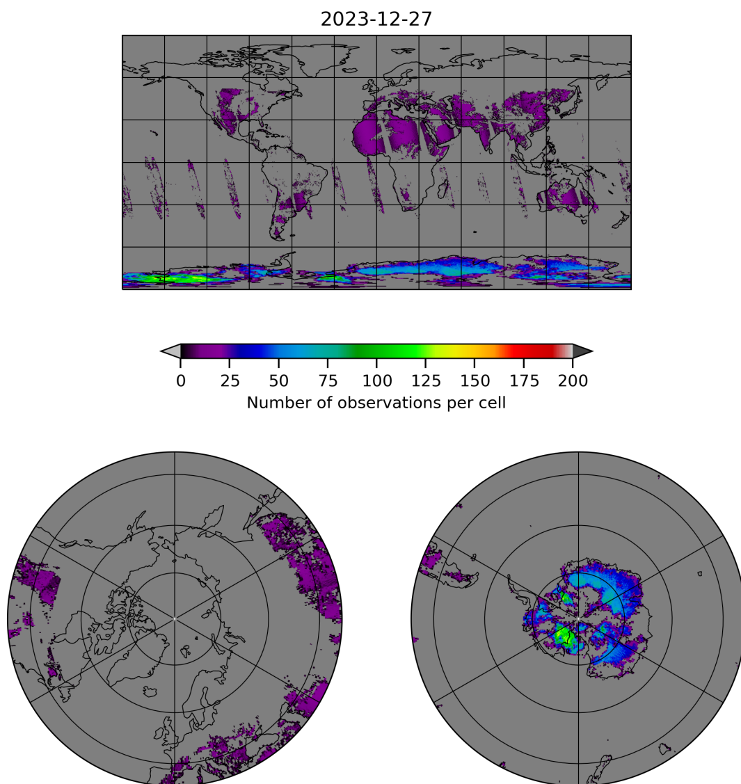
Figure 10: Map of the number of observations for 2023-12-26 to 2023-12-28
