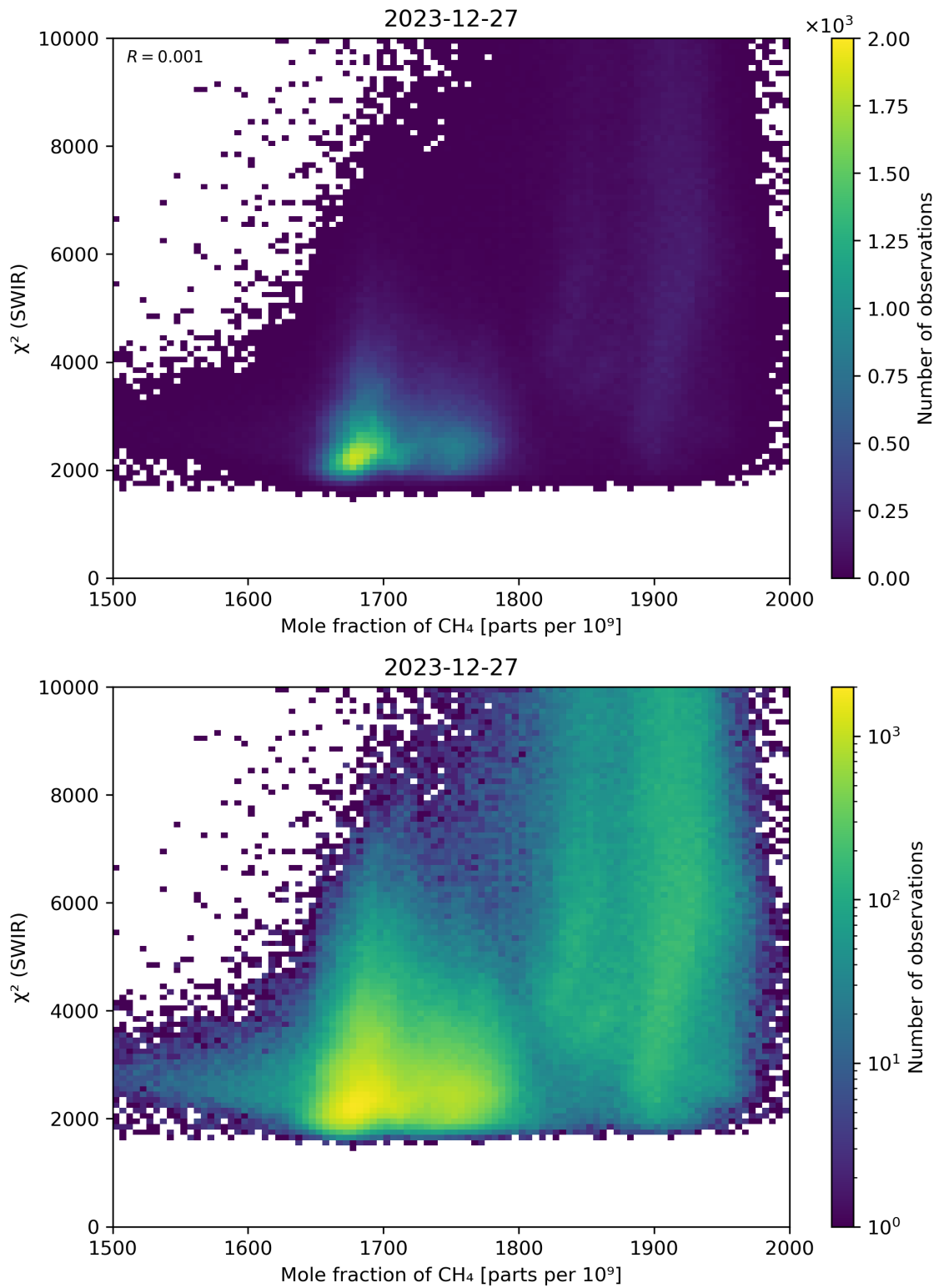
Figure 71: Scatter density plot of “Mole fraction of \text{CH}_4 ” against “ \chi^2 (SWIR)” for 2023-12-26 to 2023-12-28.
