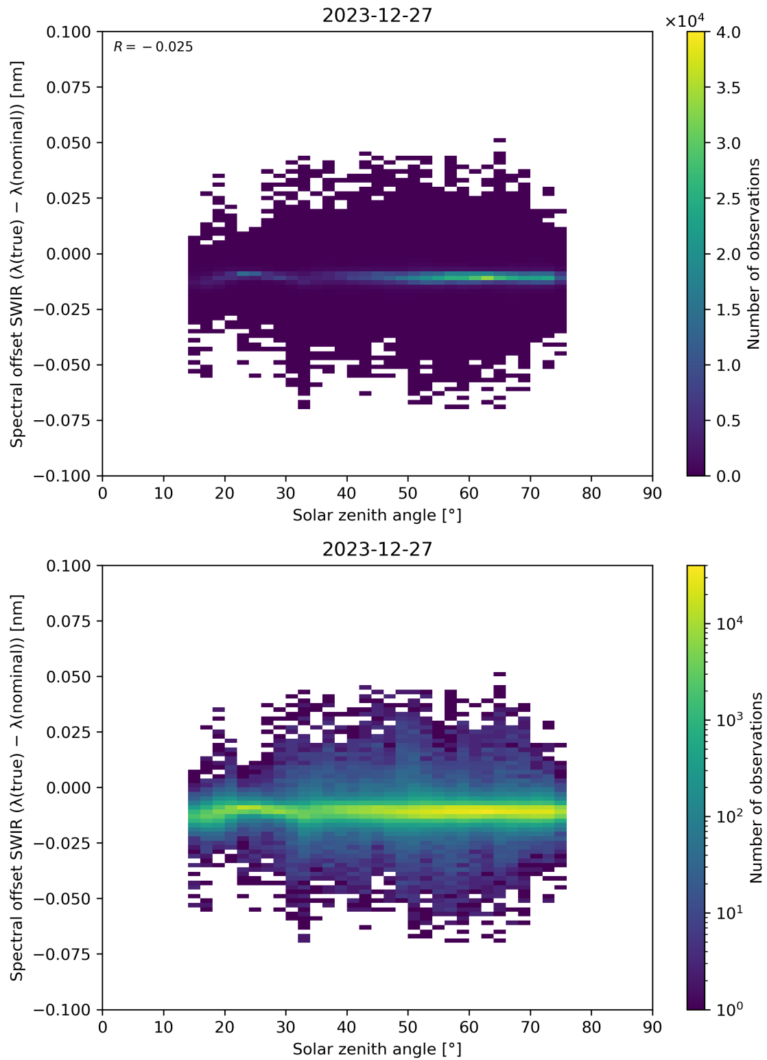
Figure 104: Scatter density plot of “Solar zenith angle” against “Spectral offset SWIR ( \lambda(\text{true}) - \lambda(\text{nominal}) )” for 2023-12-26 to 2023-12-28.
