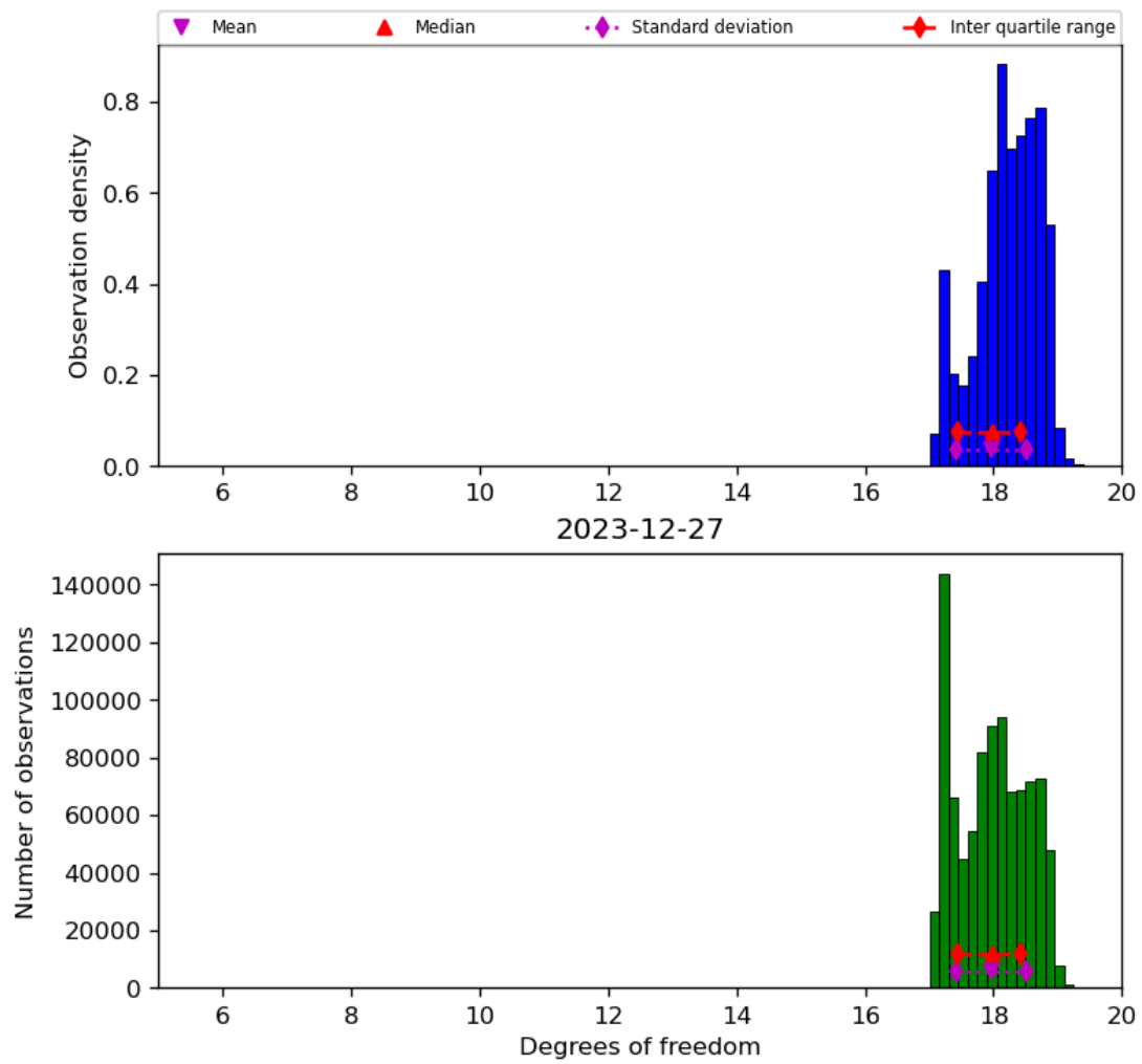
Figure 30: Histogram of “Degrees of freedom” for 2023-12-26 to 2023-12-28
