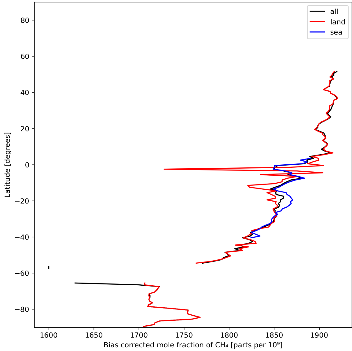
Figure 14: Zonal average of “Bias corrected mole fraction of CH 4 ” for 2023-12-26 to 2023-12-28.
