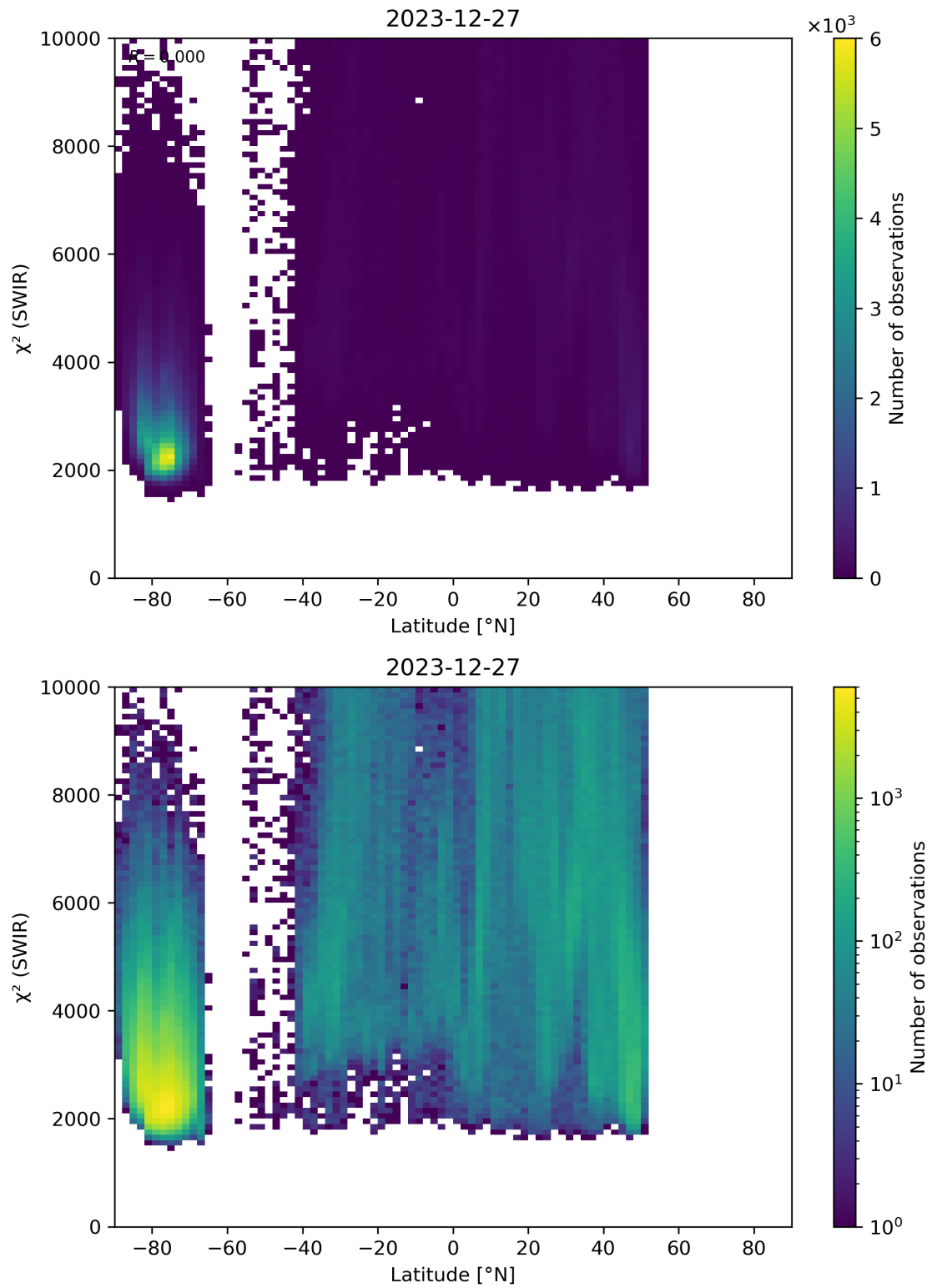
Figure 54: Scatter density plot of “Latitude” against “ \chi^2 (SWIR)” for 2023-12-26 to 2023-12-28.
