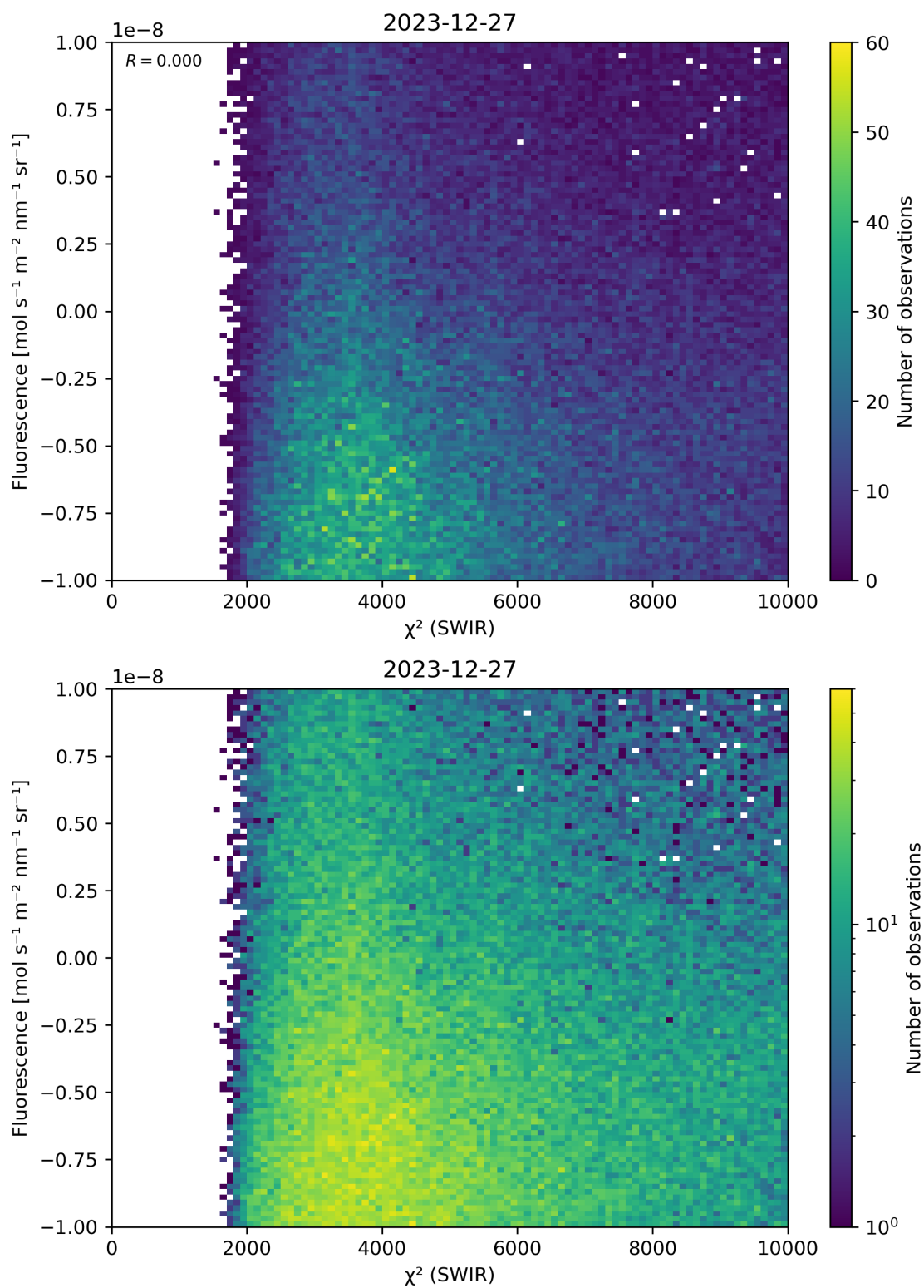
Figure 49: Scatter density plot of “ \chi^2 (SWIR)” against “Fluorescence” for 2023-12-26 to 2023-12-28.
