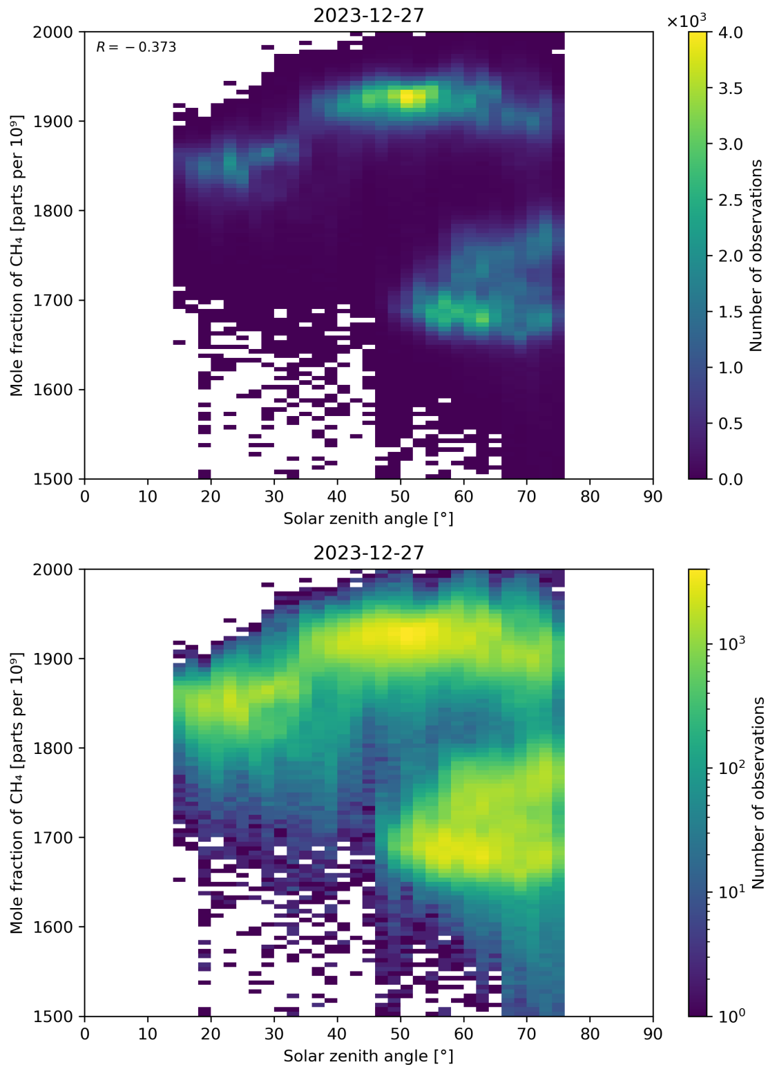
Figure 99: Scatter density plot of “Solar zenith angle” against “Mole fraction of CH 4 ” for 2023-12-26 to 2023-12-28.
