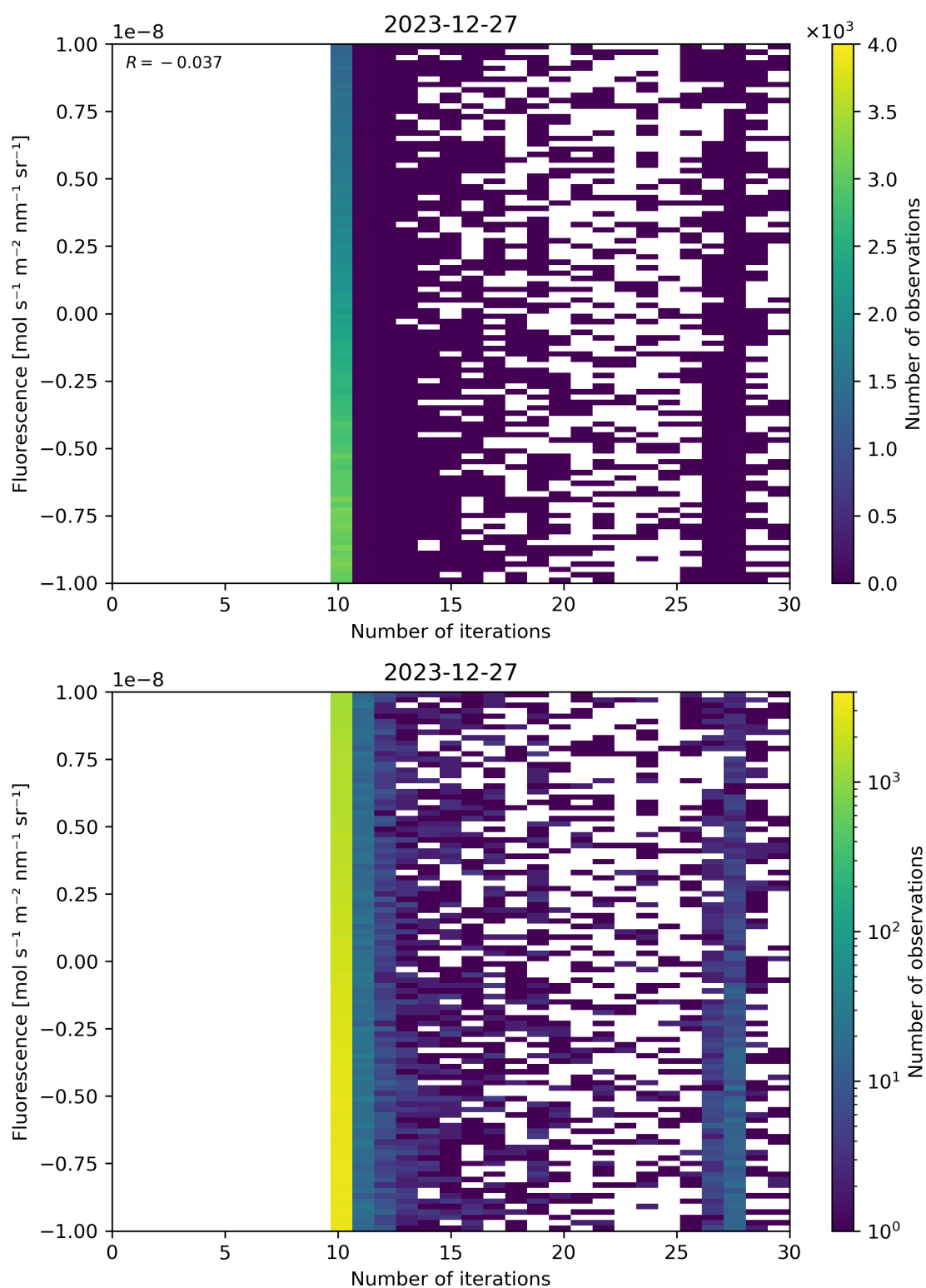
Figure 87: Scatter density plot of “Number of iterations” against “Fluorescence” for 2023-12-26 to 2023-12-28.
