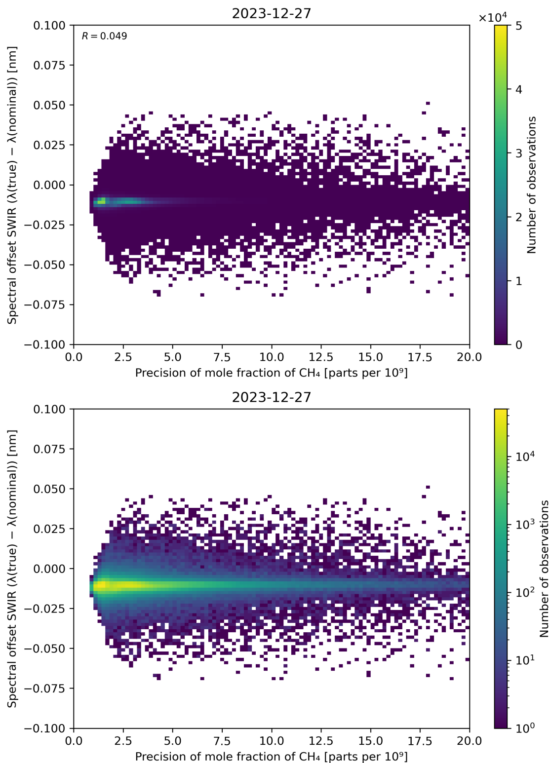
Figure 85: Scatter density plot of “Precision of mole fraction of CH 4 ” against “Spectral offset SWIR ( \lambda(\text{true}) - \lambda(\text{nominal}) )” for 2023-12-26 to 2023-12-28.
