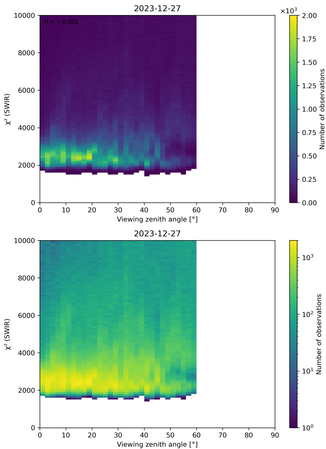
Figure 106: Scatter density plot of “Viewing zenith angle” against “ \chi^2 (SWIR)” for 2023-12-26 to 2023-12-28.
