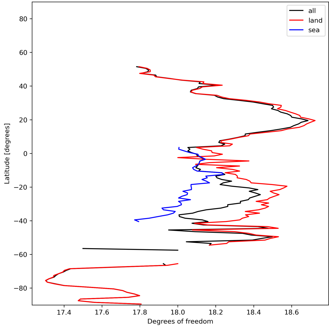
Figure 19: Zonal average of “Degrees of freedom” for 2023-12-26 to 2023-12-28.
