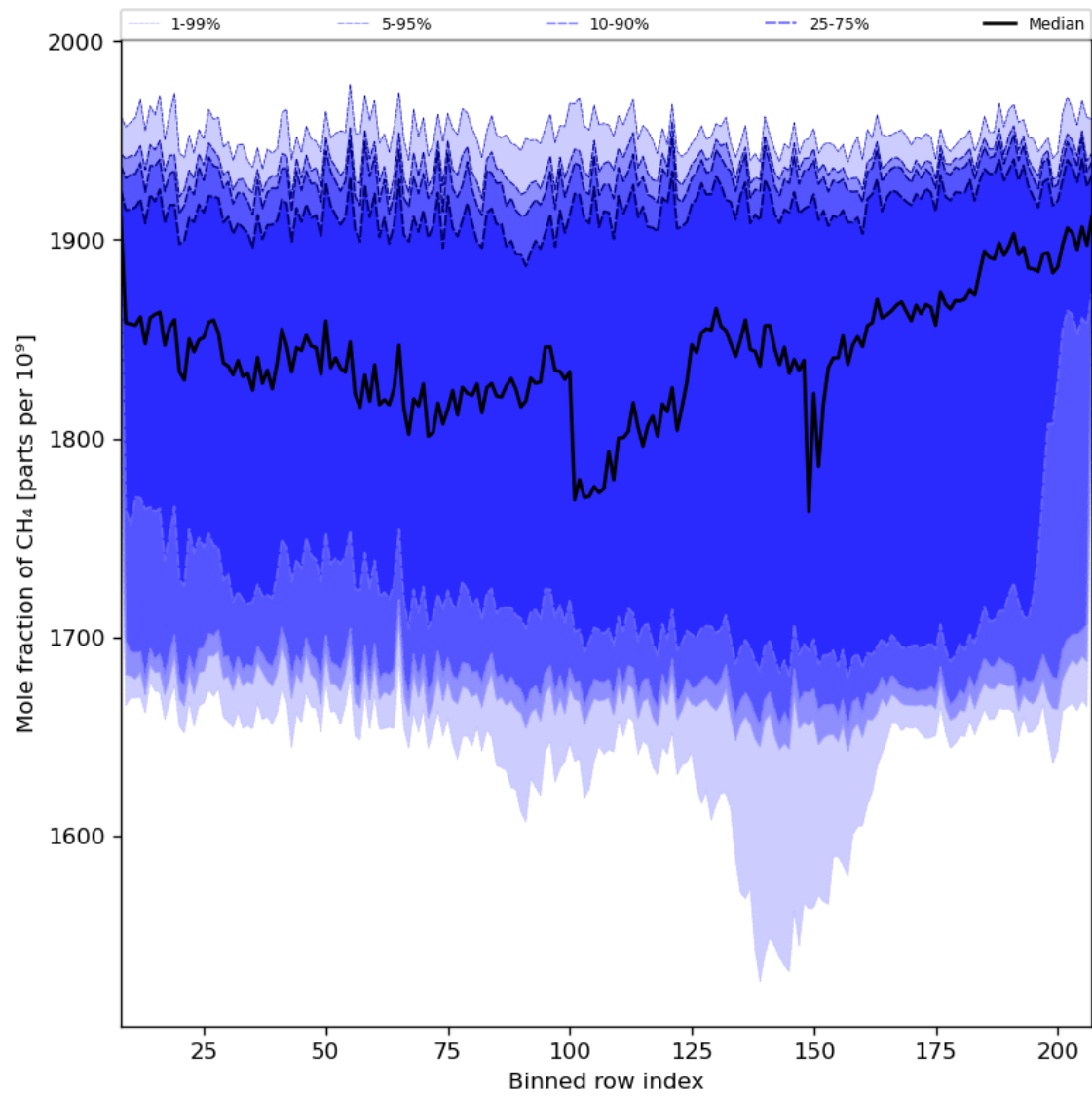
Figure 34: Along track statistics of “Mole fraction of CH 4 ” for 2023-12-26 to 2023-12-28
