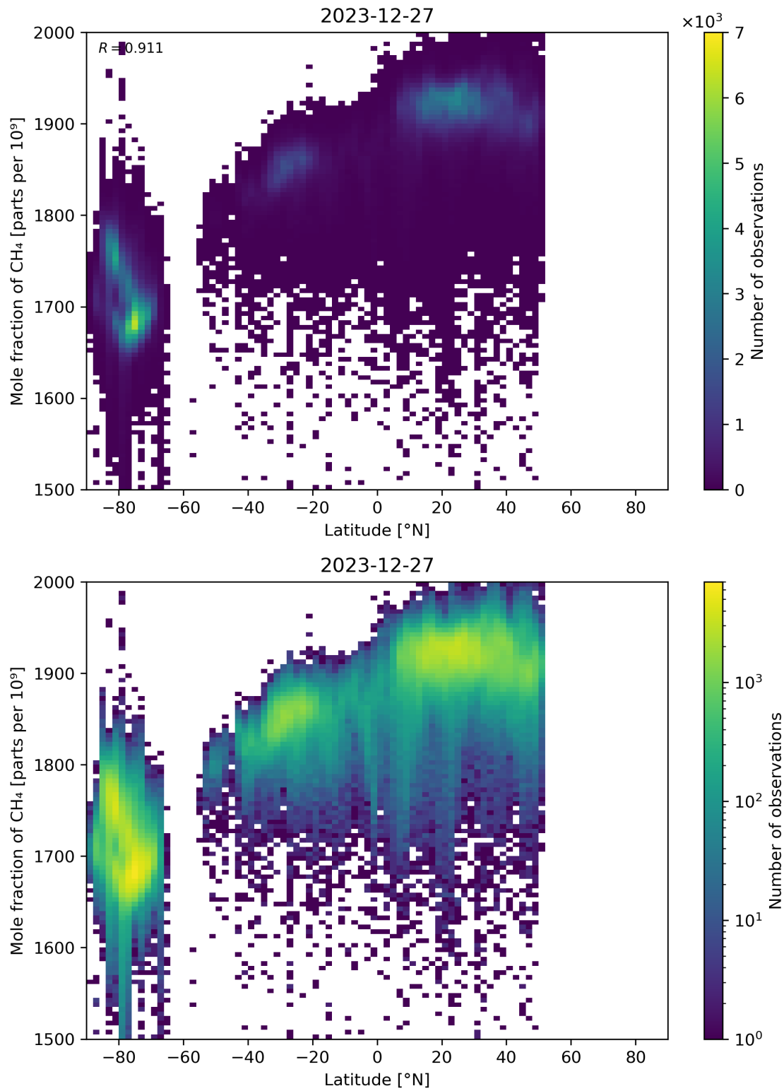
Figure 57: Scatter density plot of “Latitude” against “Mole fraction of CH 4 ” for 2023-12-26 to 2023-12-28.
