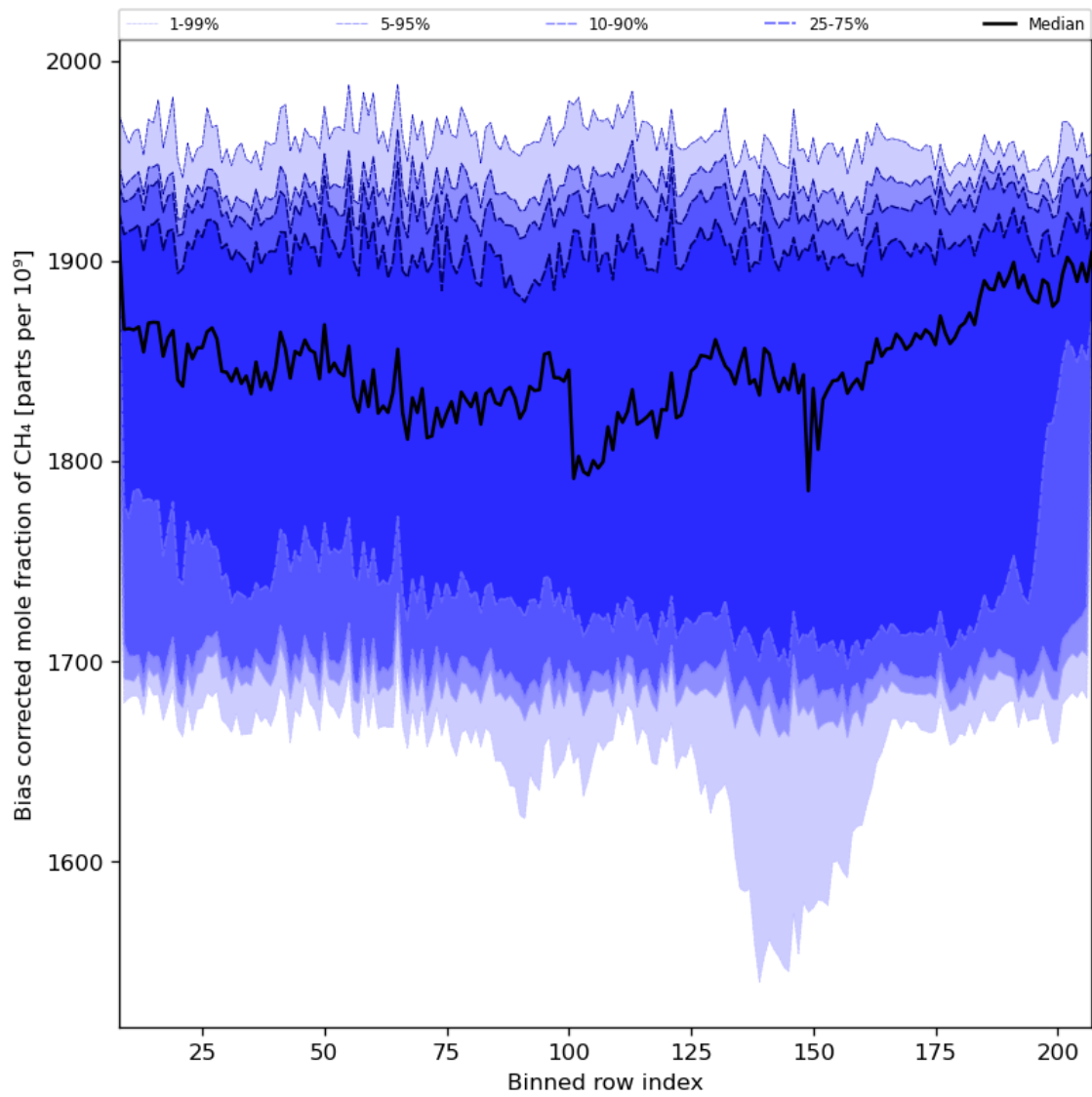
Figure 36: Along track statistics of “Bias corrected mole fraction of CH 4 ” for 2023-12-26 to 2023-12-28
