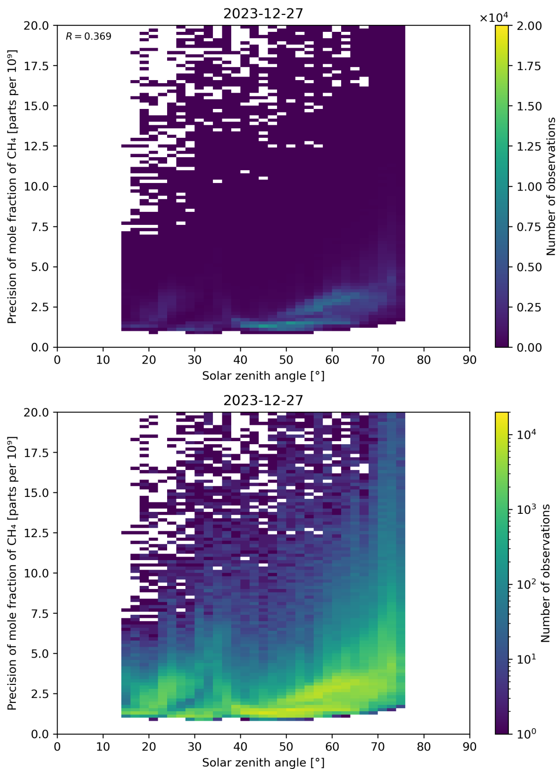
Figure 101: Scatter density plot of “Solar zenith angle” against “Precision of mole fraction of CH 4 ” for 2023-12-26 to 2023-12-28.
