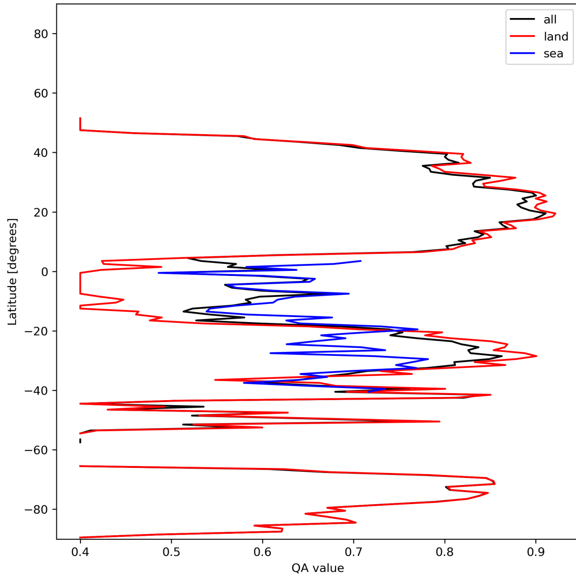
Figure 11: Zonal average of “QA value” for 2023-12-26 to 2023-12-28.
