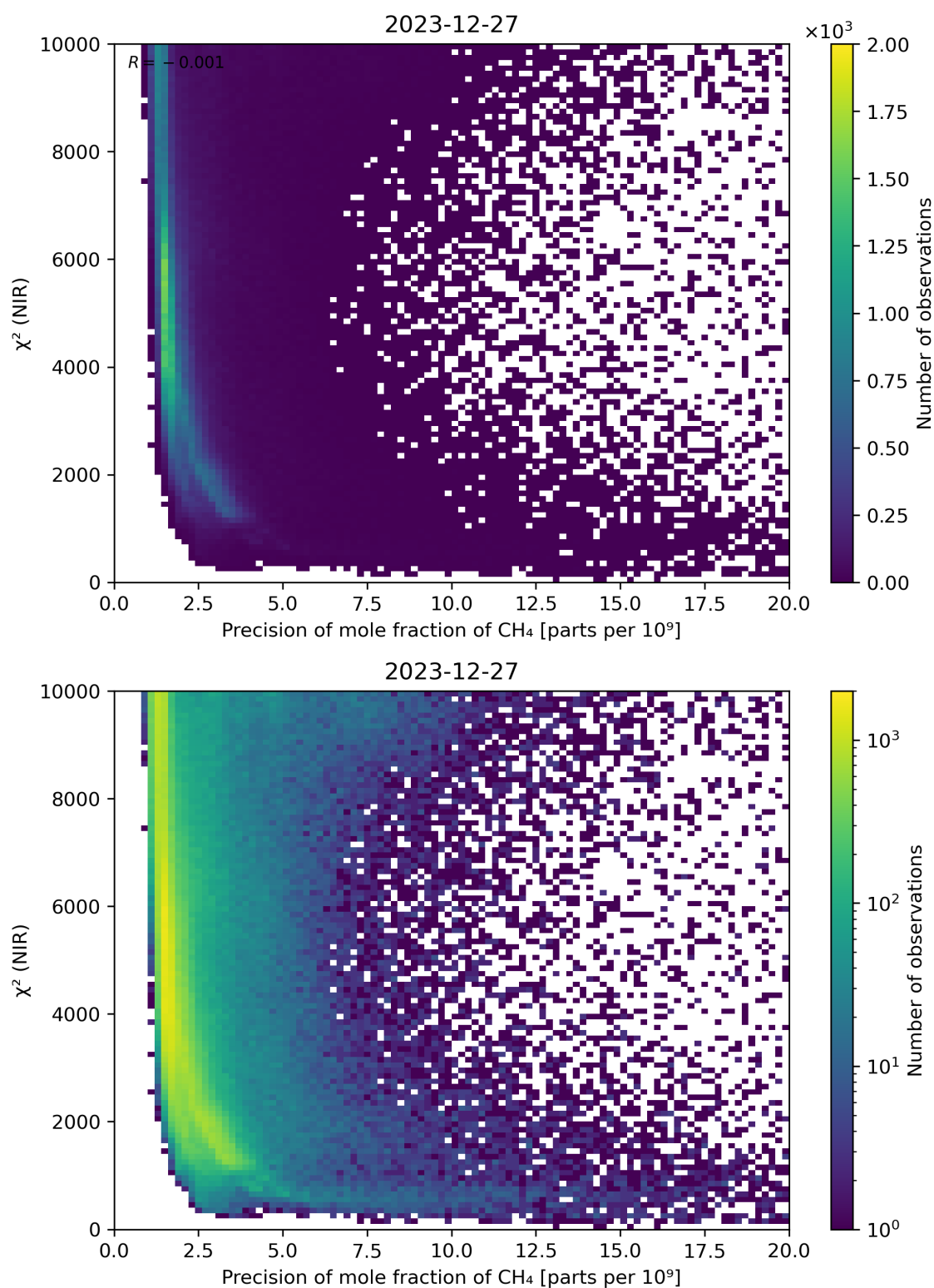
Figure 78: Scatter density plot of “Precision of mole fraction of CH 4 ” against “ \chi^2 (NIR)” for 2023-12-26 to 2023-12-28.
