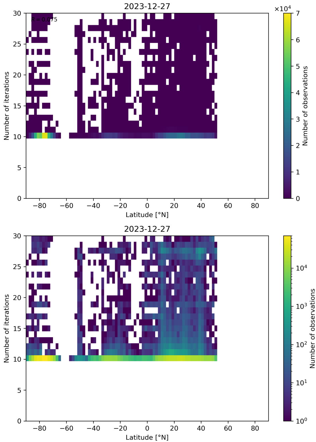
Figure 60: Scatter density plot of “Latitude” against “Number of iterations” for 2023-12-26 to 2023-12-28.
