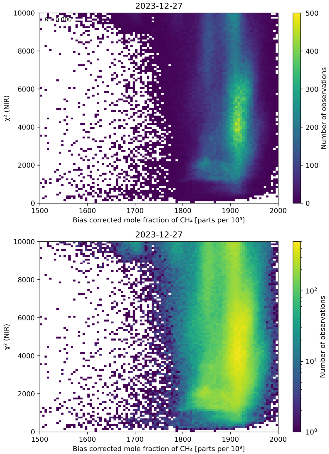
Figure 63: Scatter density plot of “Bias corrected mole fraction of \text{CH}_4 ” against “ \chi^2 (NIR)” for 2023-12-26 to 2023-12-28.
