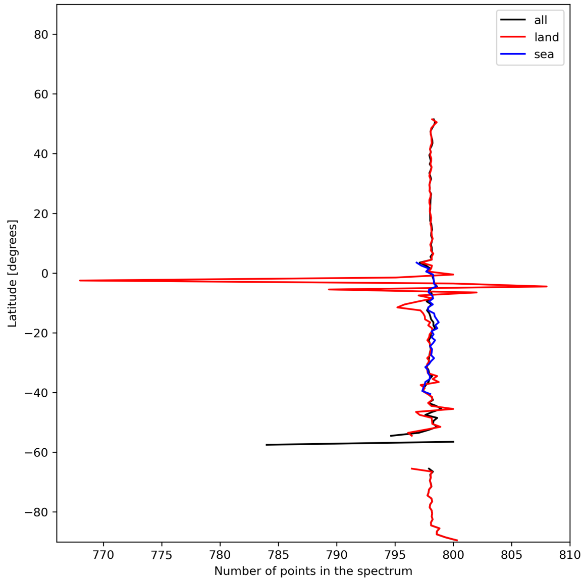
Figure 15: Zonal average of “Number of points in the spectrum” for 2023-12-26 to 2023-12-28.
