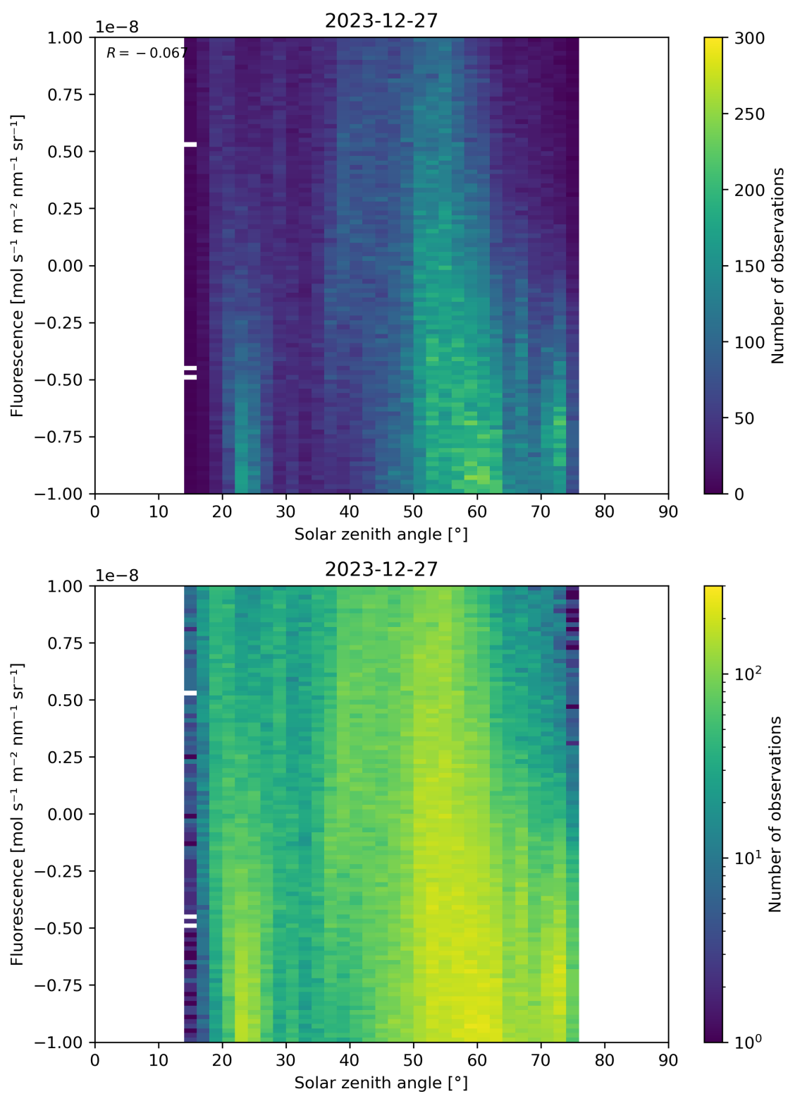
Figure 97: Scatter density plot of “Solar zenith angle” against “Fluorescence” for 2023-12-26 to 2023-12-28.
