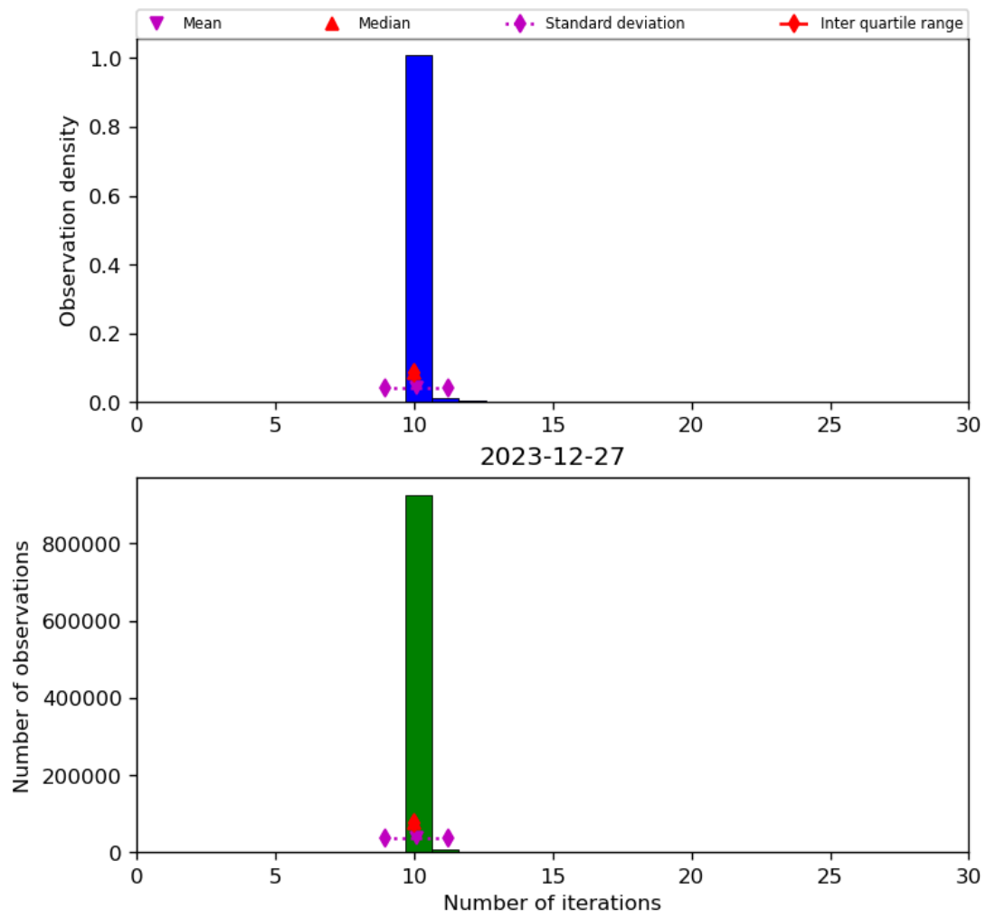
Figure 31: Histogram of “Number of iterations” for 2023-12-26 to 2023-12-28
