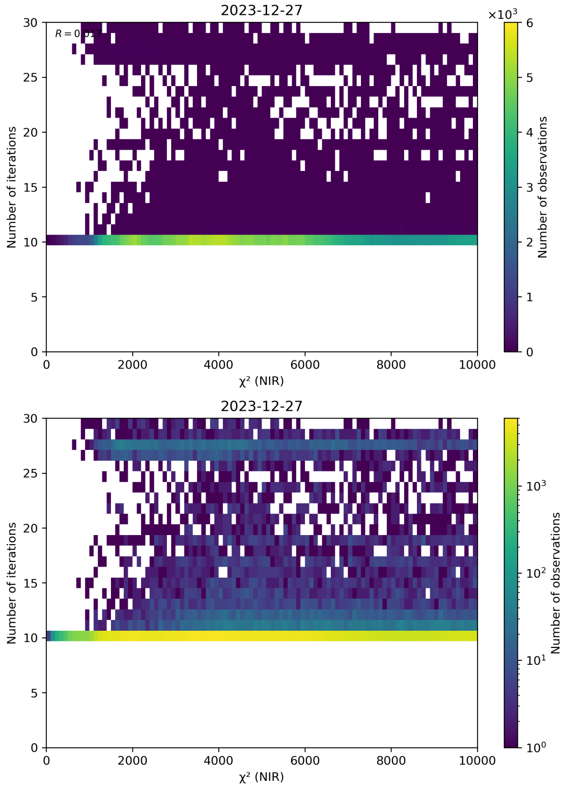
Figure 46: Scatter density plot of “ \chi^2 (NIR)” against “Number of iterations” for 2023-12-26 to 2023-12-28.
