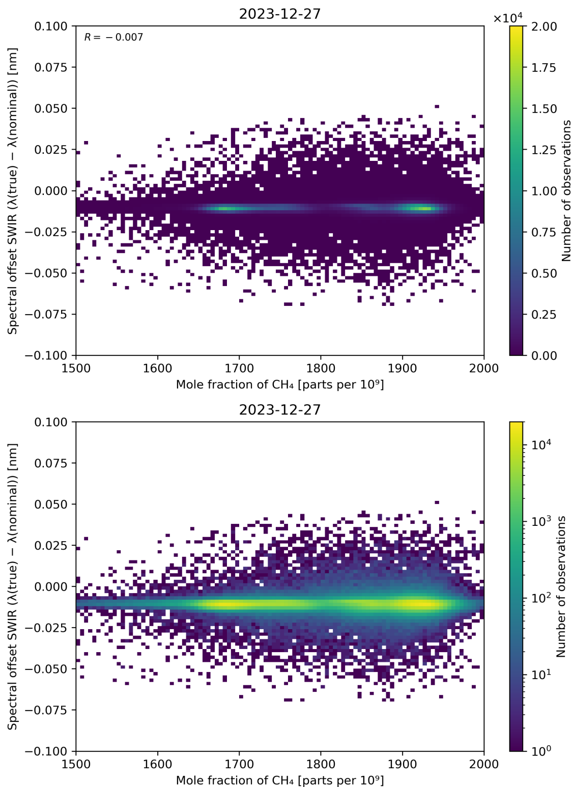
Figure 86: Scatter density plot of “Mole fraction of CH 4 ” against “Spectral offset SWIR ( \lambda(\text{true}) - \lambda(\text{nominal}) )” for 2023-12-26 to 2023-12-28.
