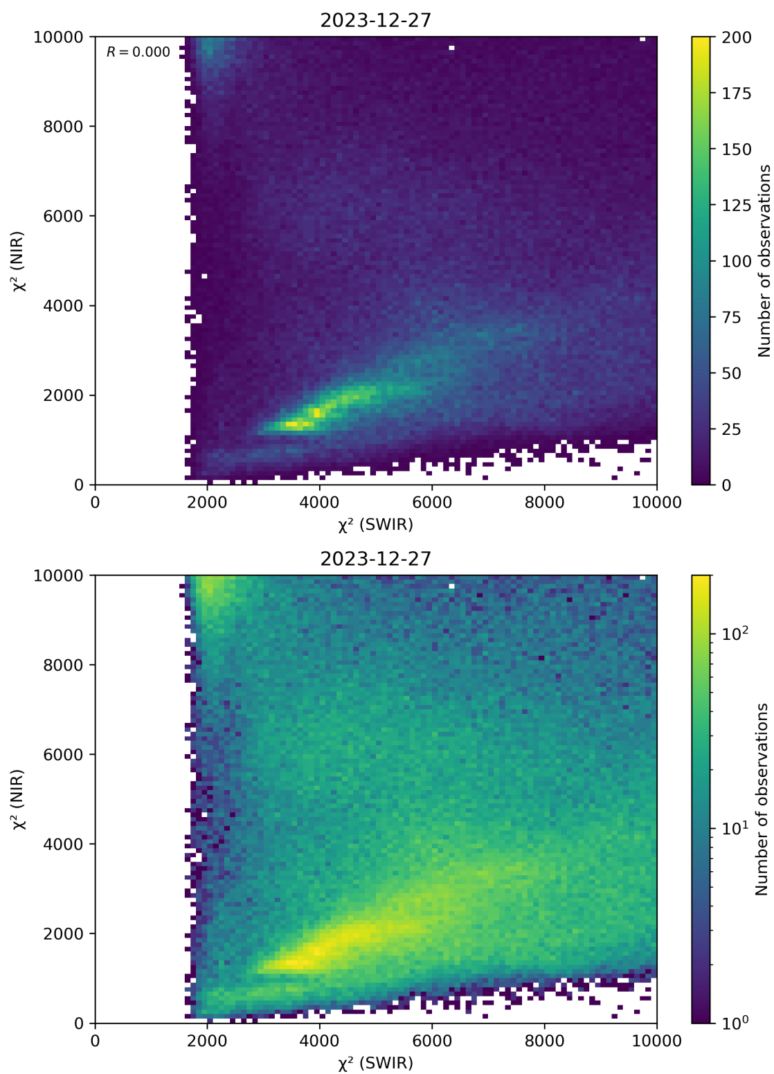
Figure 47: Scatter density plot of “ \chi^2 (SWIR)” against “ \chi^2 (NIR)” for 2023-12-26 to 2023-12-28.
