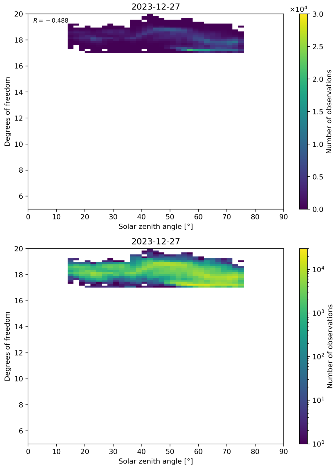
Figure 96: Scatter density plot of “Solar zenith angle” against “Degrees of freedom” for 2023-12-26 to 2023-12-28.
