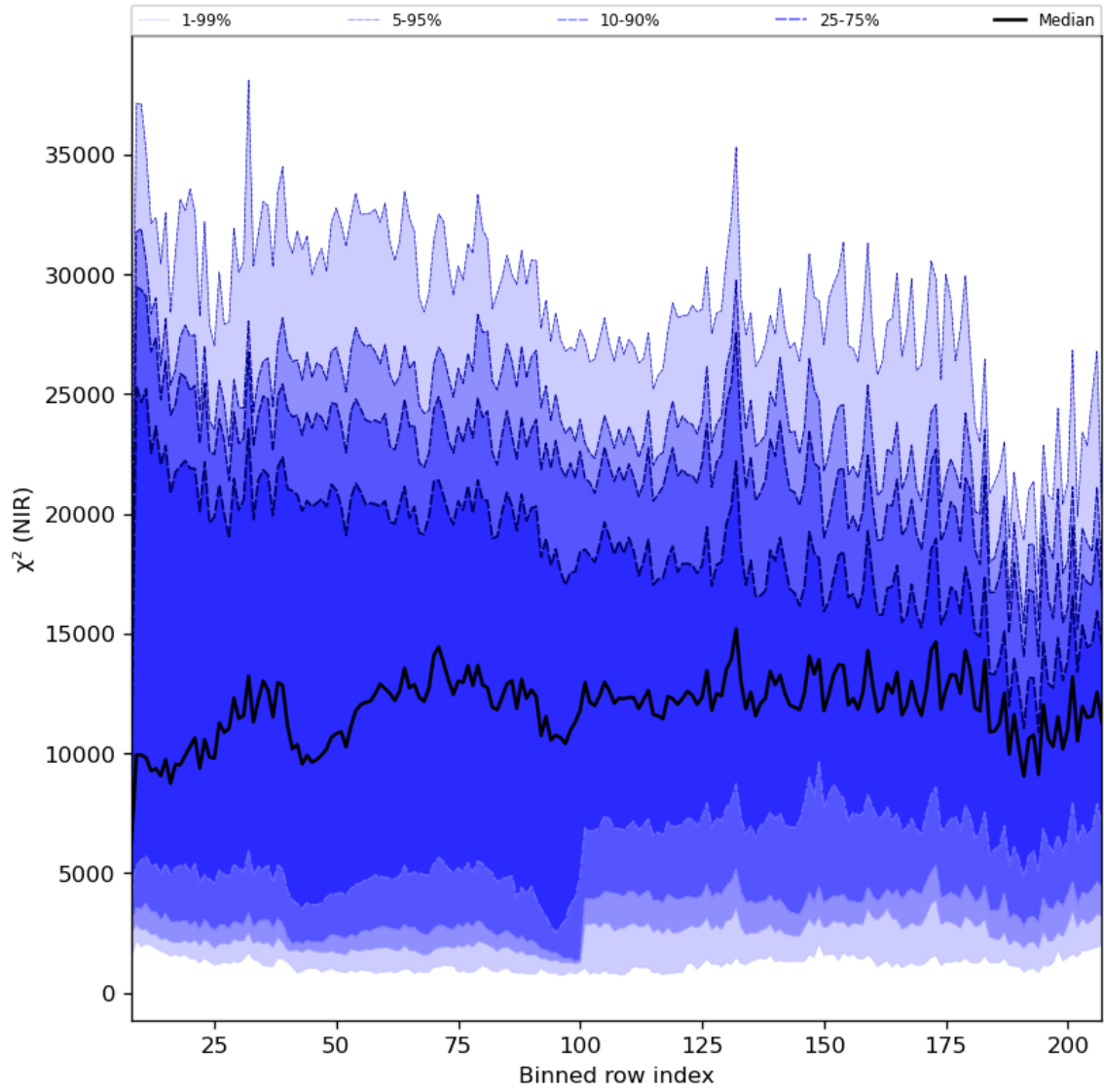
Figure 40: Along track statistics of " \chi^2 (NIR)" for 2023-12-26 to 2023-12-28
