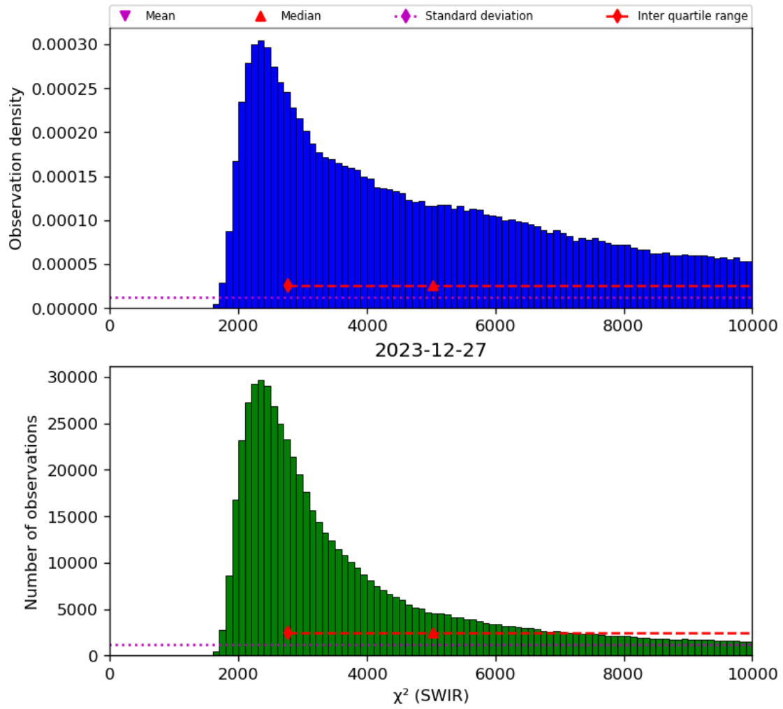
Figure 28: Histogram of “ \chi^2 (SWIR)” for 2023-12-26 to 2023-12-28
