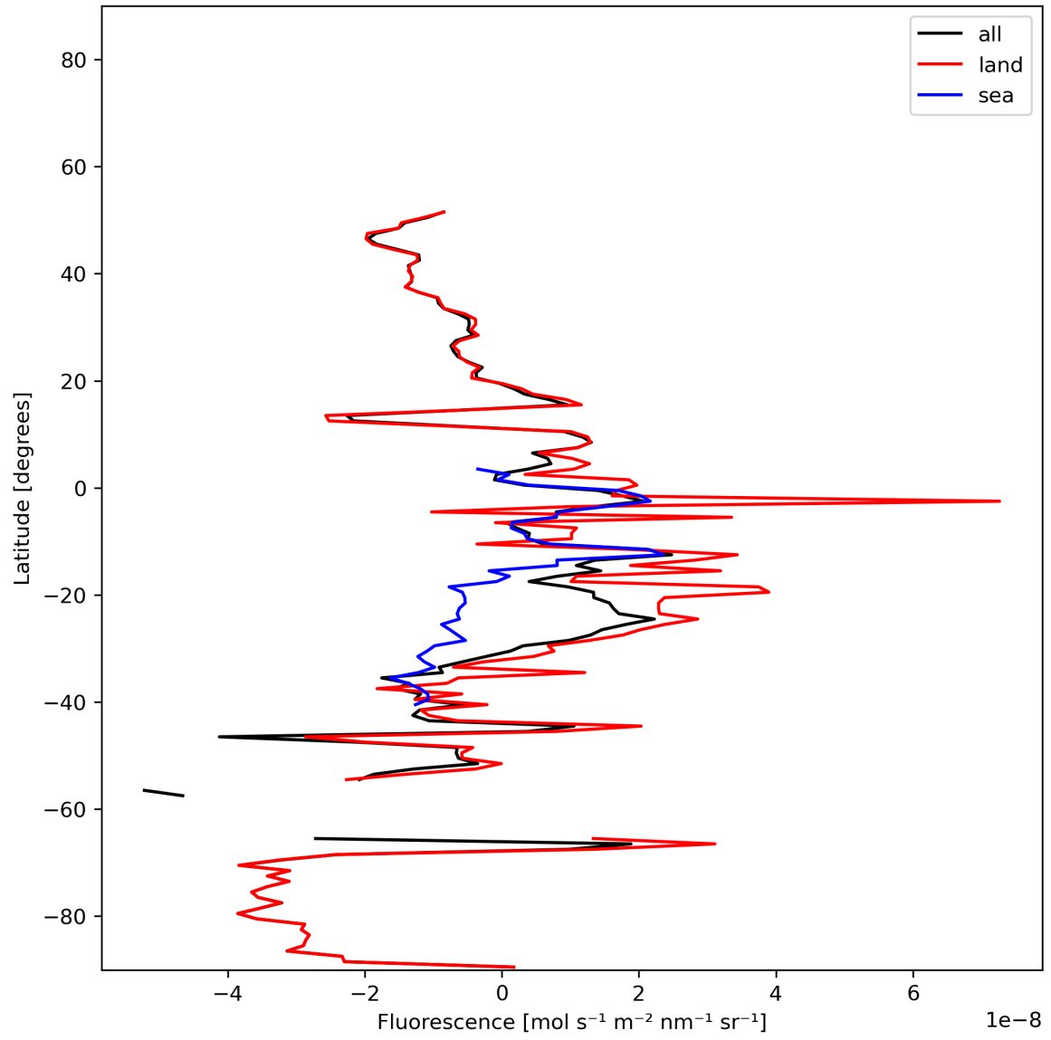
Figure 21: Zonal average of “Fluorescence” for 2023-12-26 to 2023-12-28.
