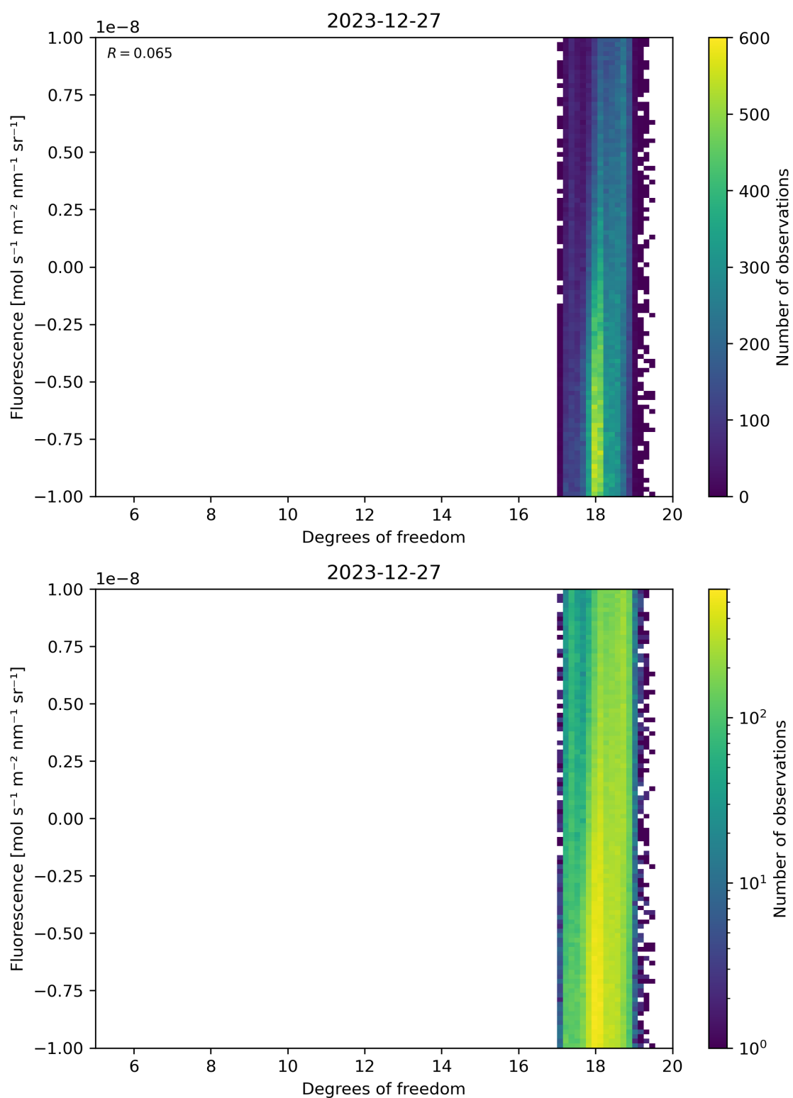
Figure 51: Scatter density plot of “Degrees of freedom” against “Fluorescence” for 2023-12-26 to 2023-12-28.
