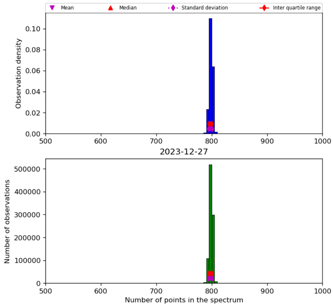
Figure 26: Histogram of “Number of points in the spectrum” for 2023-12-26 to 2023-12-28
