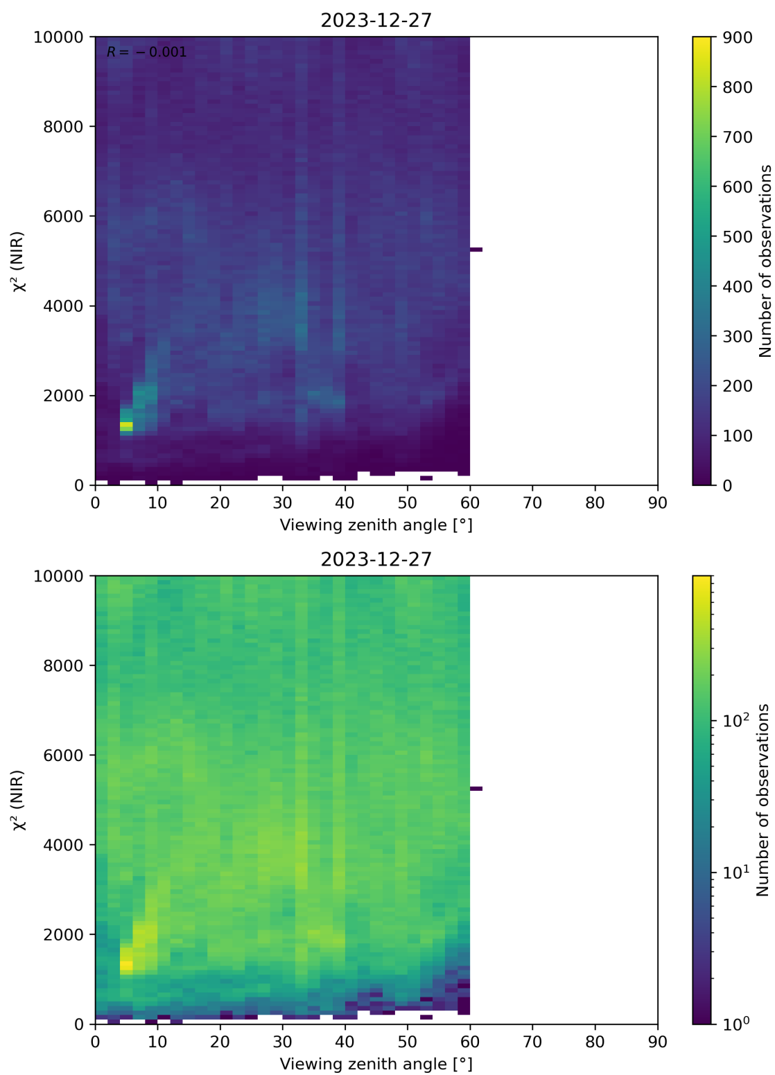
Figure 105: Scatter density plot of “Viewing zenith angle” against “ \chi^2 (NIR)” for 2023-12-26 to 2023-12-28.
