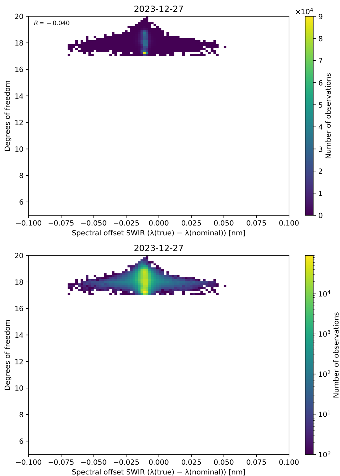
Figure 119: Scatter density plot of “Spectral offset SWIR ( \lambda(\text{true}) - \lambda(\text{nominal}) )” against “Degrees of freedom” for 2023-12-26 to 2023-12-28.
