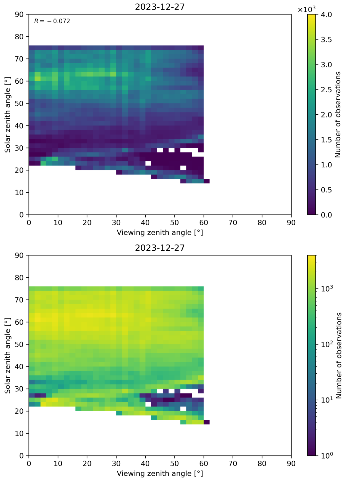
Figure 115: Scatter density plot of “Viewing zenith angle” against “Solar zenith angle” for 2023-12-26 to 2023-12-28.
