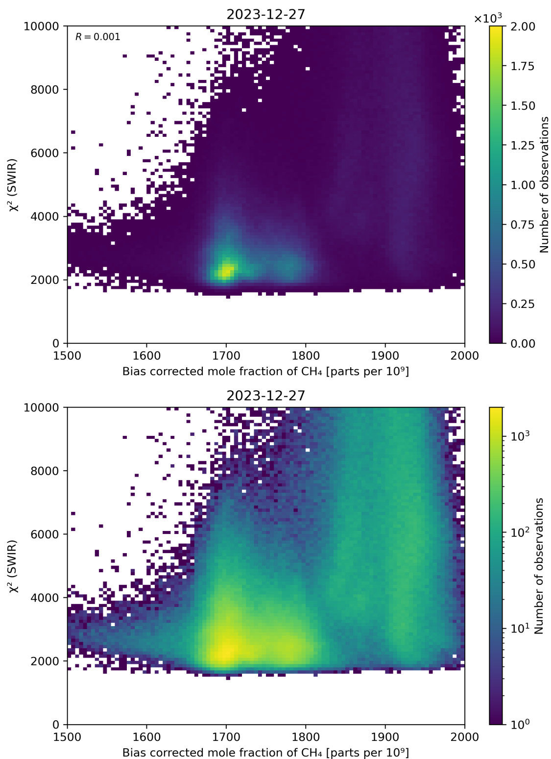
Figure 64: Scatter density plot of “Bias corrected mole fraction of CH 4 ” against “ \chi^2 (SWIR)” for 2023-12-26 to 2023-12-28.
