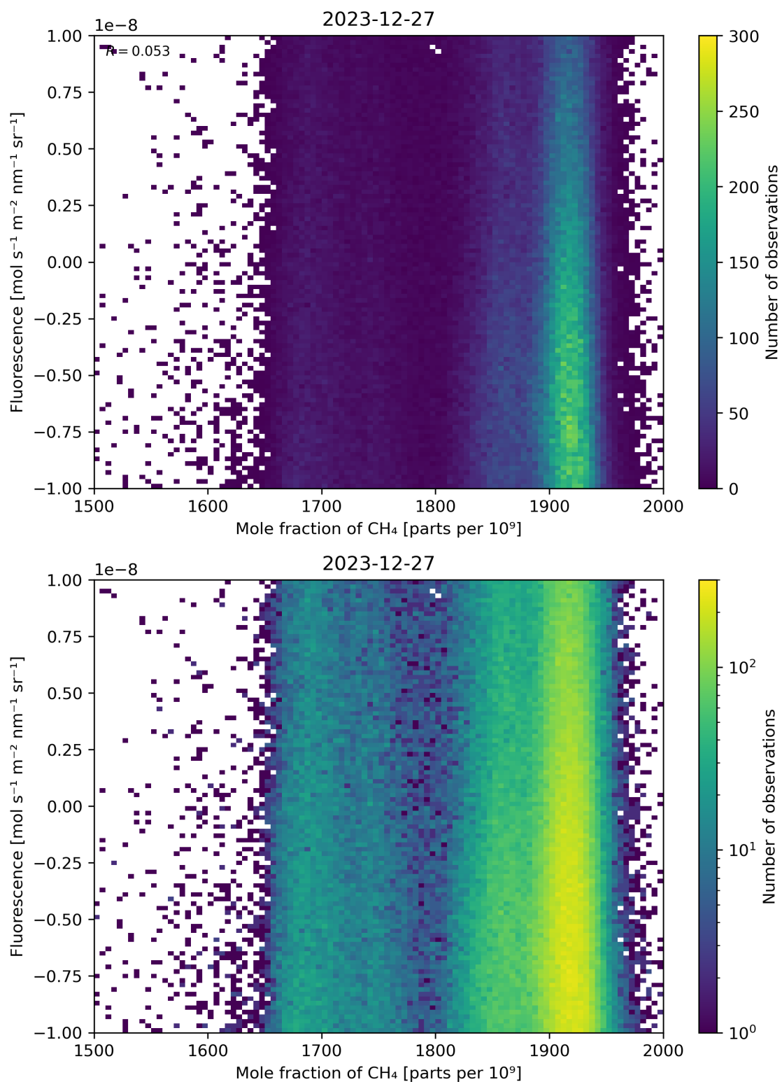
Figure 73: Scatter density plot of “Mole fraction of \text{CH}_4 ” against “Fluorescence” for 2023-12-26 to 2023-12-28.
