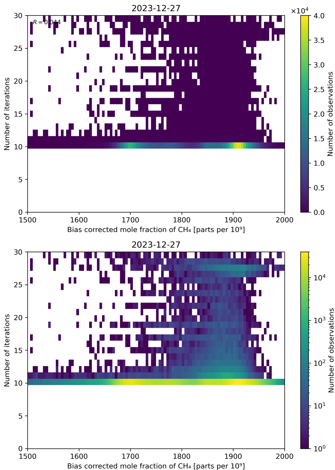
Figure 67: Scatter density plot of “Bias corrected mole fraction of CH 4 ” against “Number of iterations” for 2023-12-26 to 2023-12-28.
