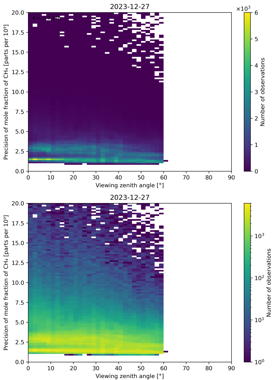
Figure 112: Scatter density plot of “Viewing zenith angle” against “Precision of mole fraction of CH 4 ” for 2023-12-26 to 2023-12-28.
