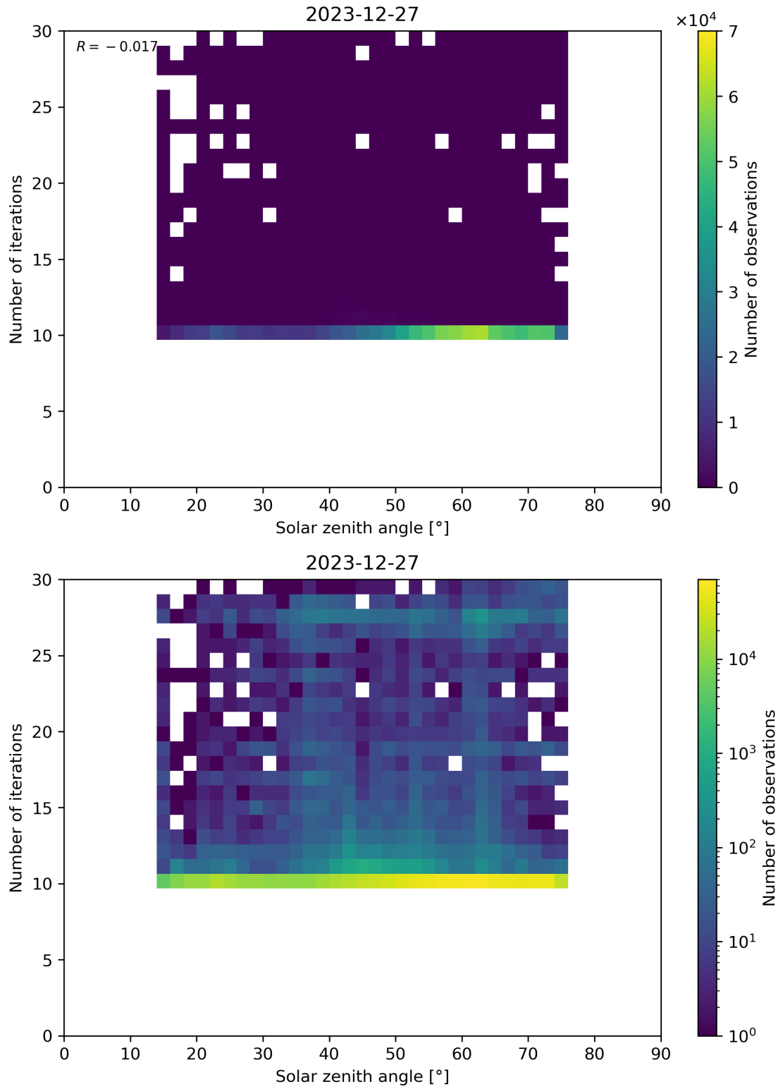
Figure 102: Scatter density plot of “Solar zenith angle” against “Number of iterations” for 2023-12-26 to 2023-12-28.
