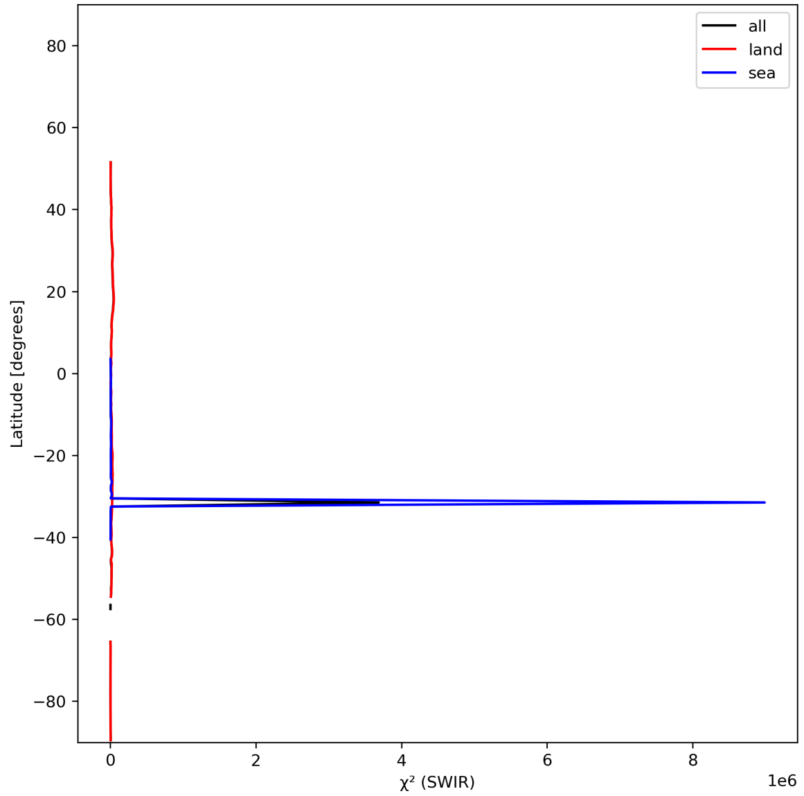
Figure 17: Zonal average of “ \chi^2 (SWIR)” for 2023-12-26 to 2023-12-28.
