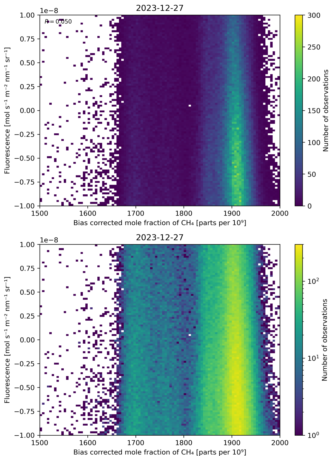
Figure 66: Scatter density plot of “Bias corrected mole fraction of \text{CH}_4 ” against “Fluorescence” for 2023-12-26 to 2023-12-28.
