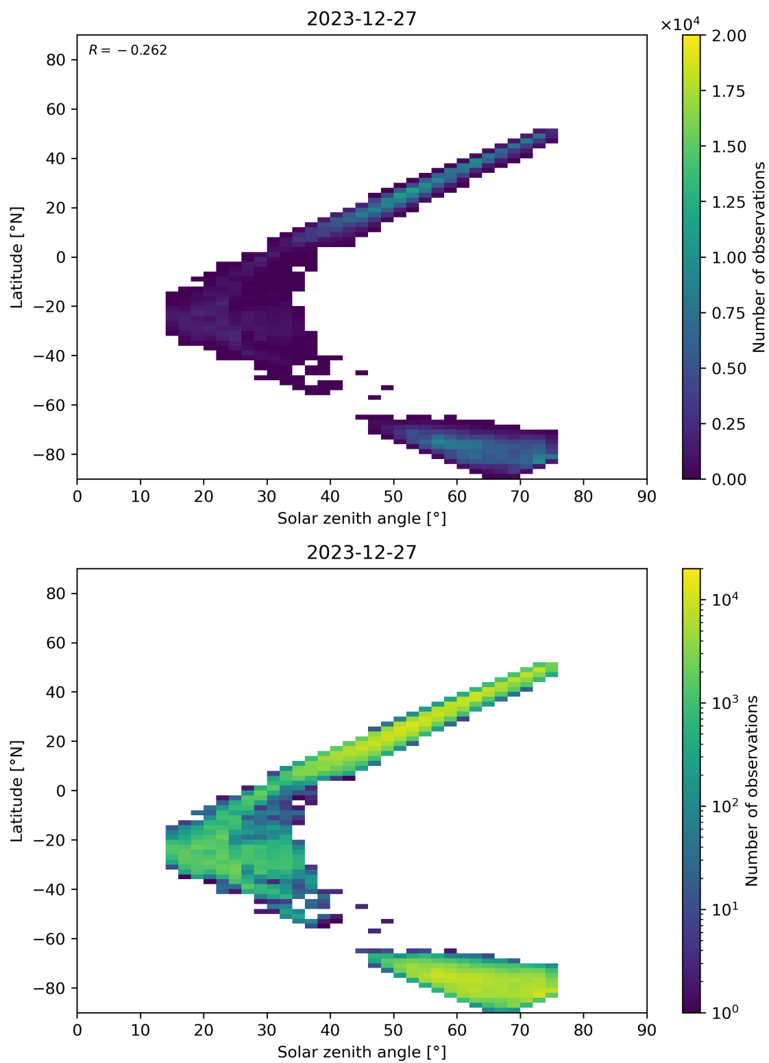
Figure 98: Scatter density plot of “Solar zenith angle” against “Latitude” for 2023-12-26 to 2023-12-28.
