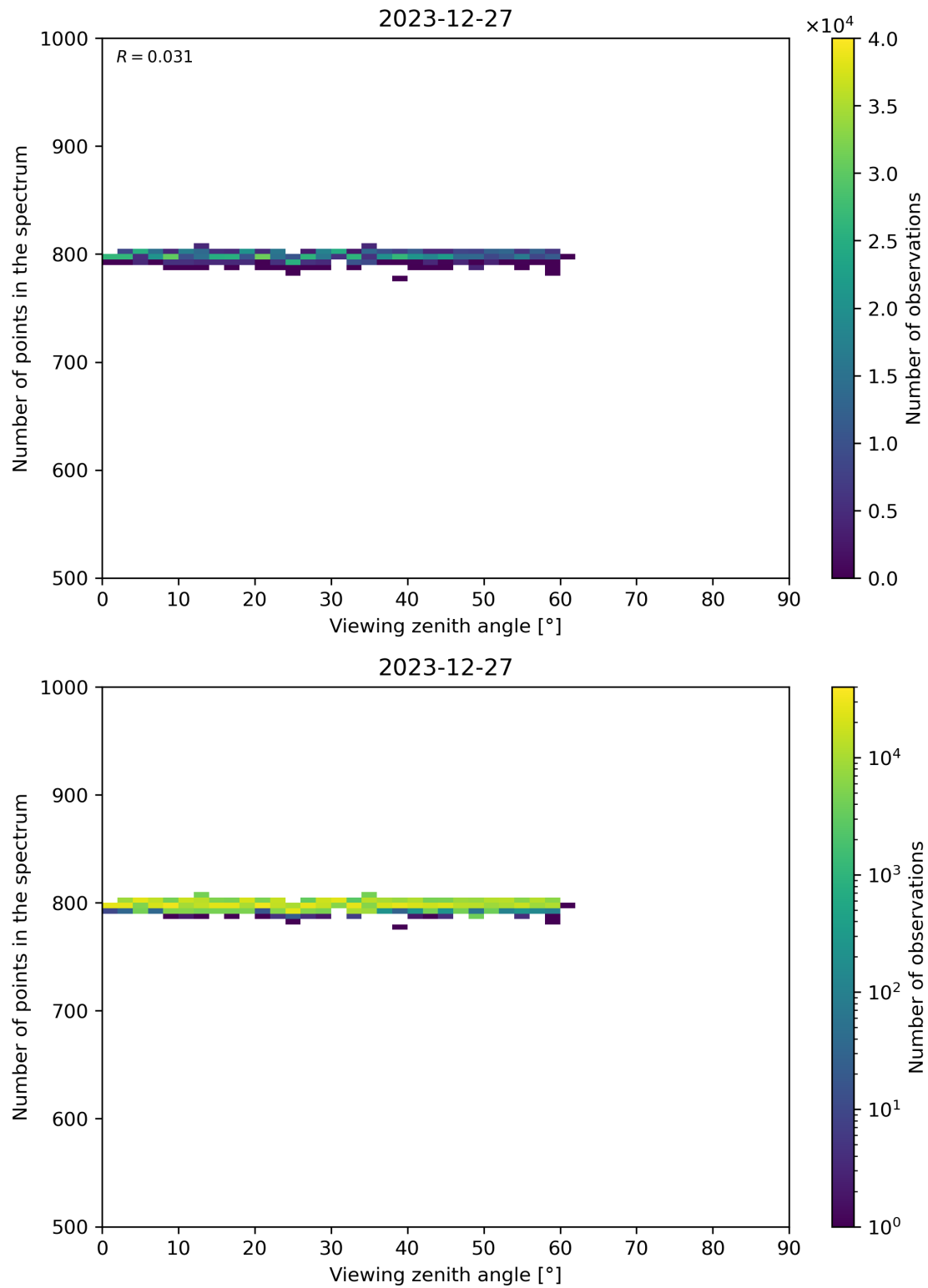
Figure 114: Scatter density plot of “Viewing zenith angle” against “Number of points in the spectrum” for 2023-12-26 to 2023-12-28.
