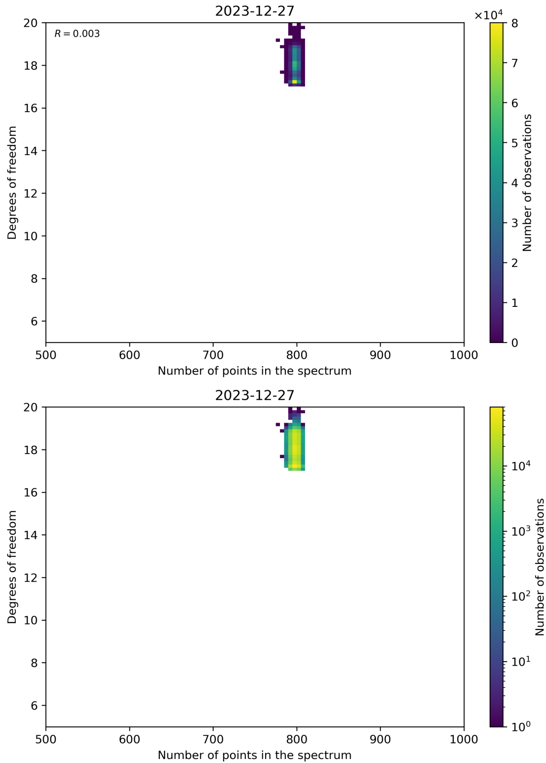
Figure 90: Scatter density plot of “Number of points in the spectrum” against “Degrees of freedom” for 2023-12-26 to 2023-12-28.
