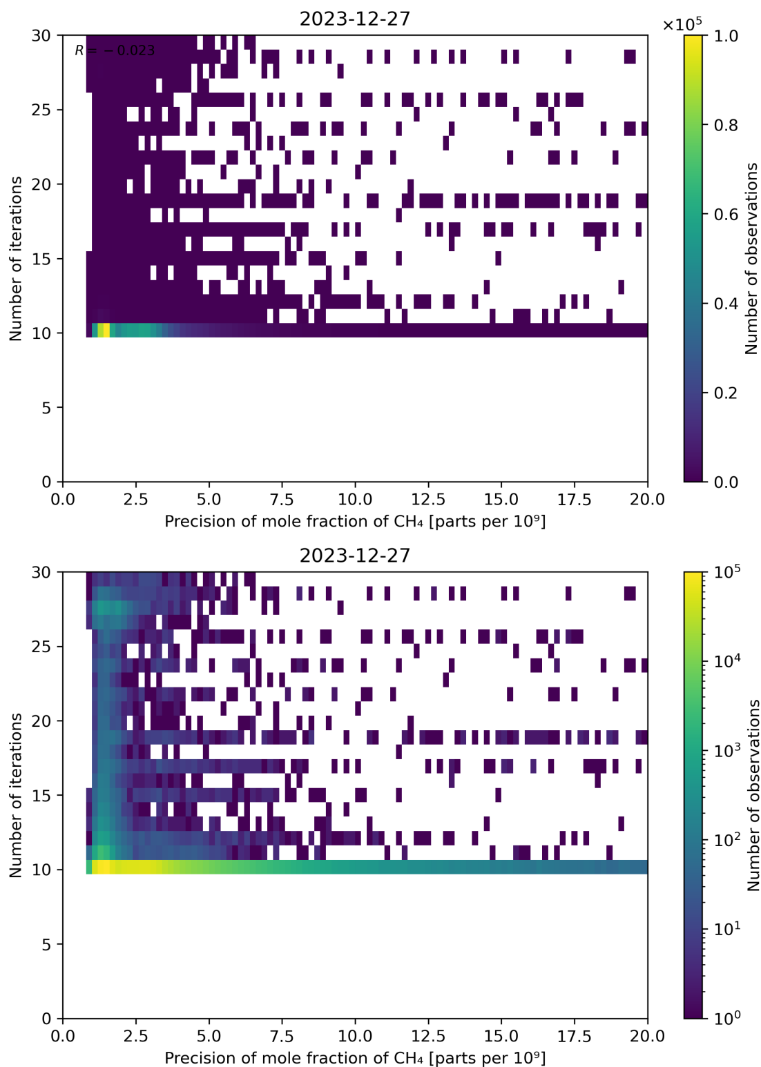
Figure 83: Scatter density plot of “Precision of mole fraction of CH 4 ” against “Number of iterations” for 2023-12-26 to 2023-12-28.
