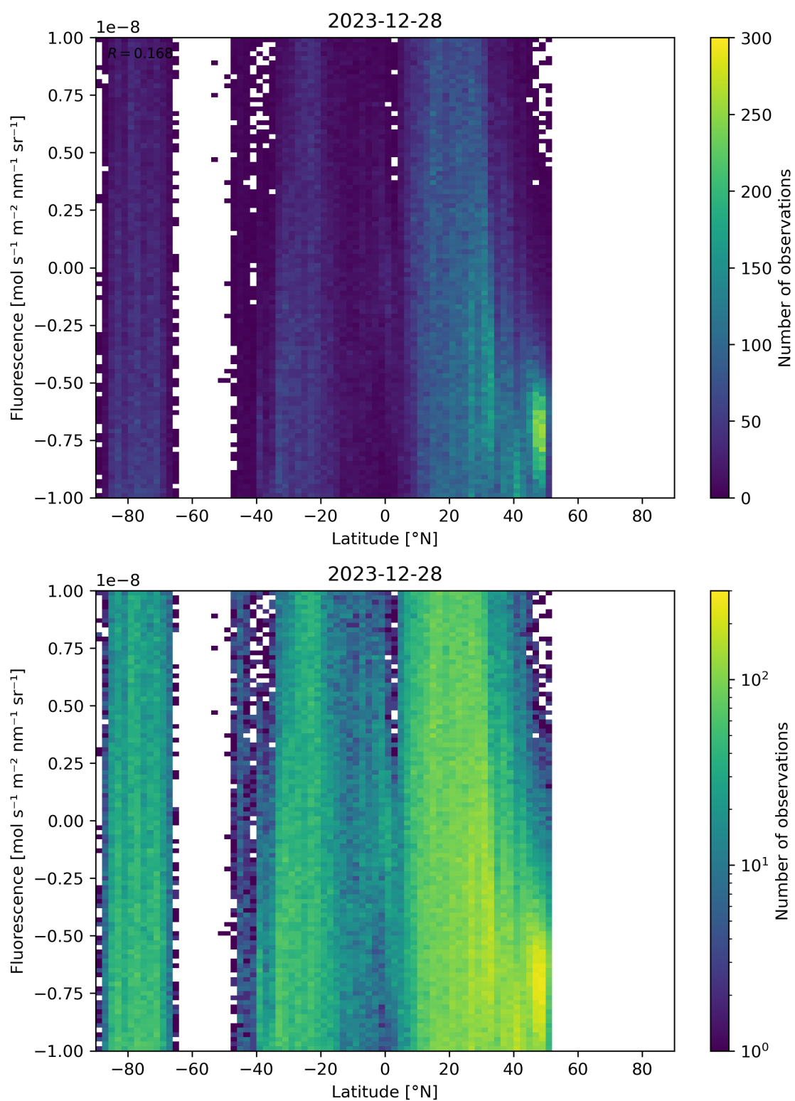
Figure 56: Scatter density plot of “Latitude” against “Fluorescence” for 2023-12-27 to 2023-12-29.
