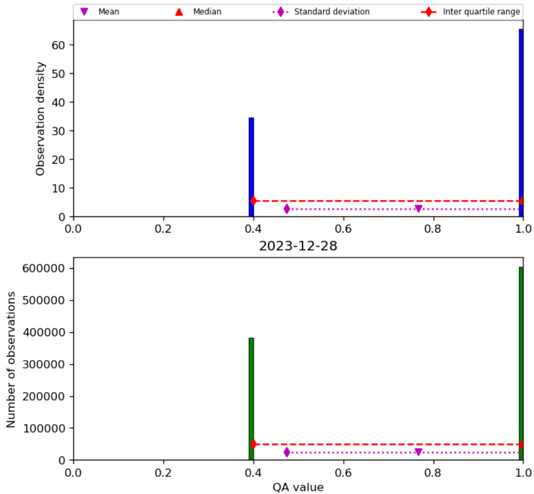
Figure 22: Histogram of “QA value” for 2023-12-27 to 2023-12-29
