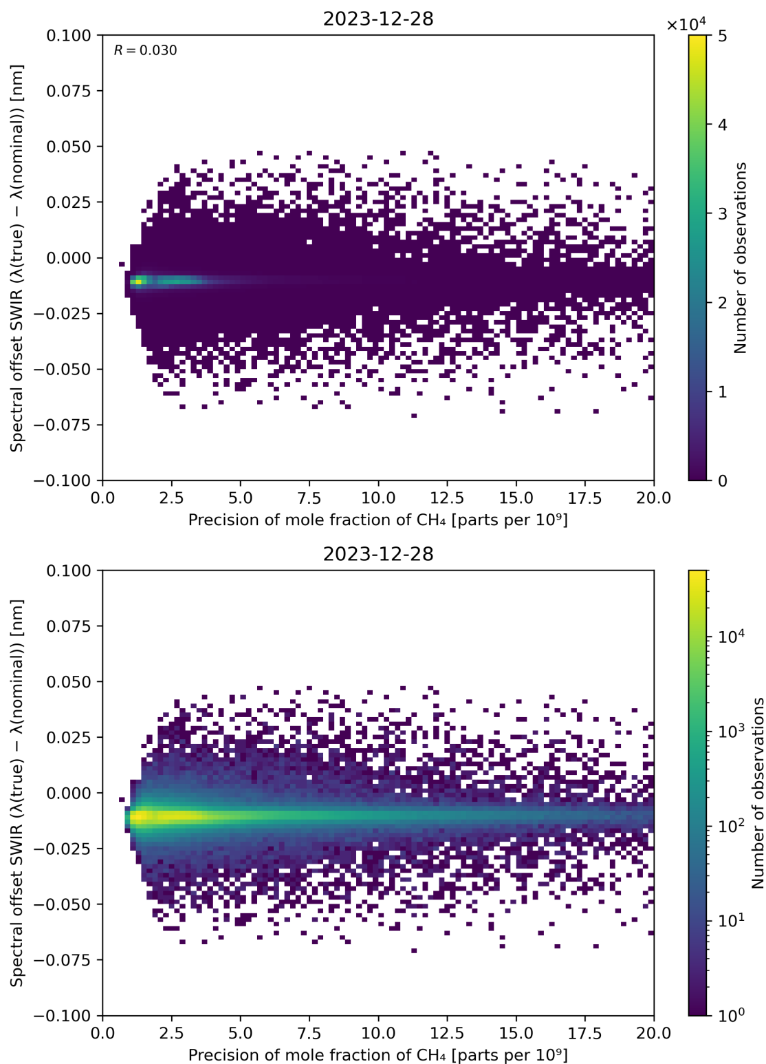
Figure 85: Scatter density plot of “Precision of mole fraction of CH 4 ” against “Spectral offset SWIR ( \lambda(\text{true}) - \lambda(\text{nominal}) )” for 2023-12-27 to 2023-12-29.
