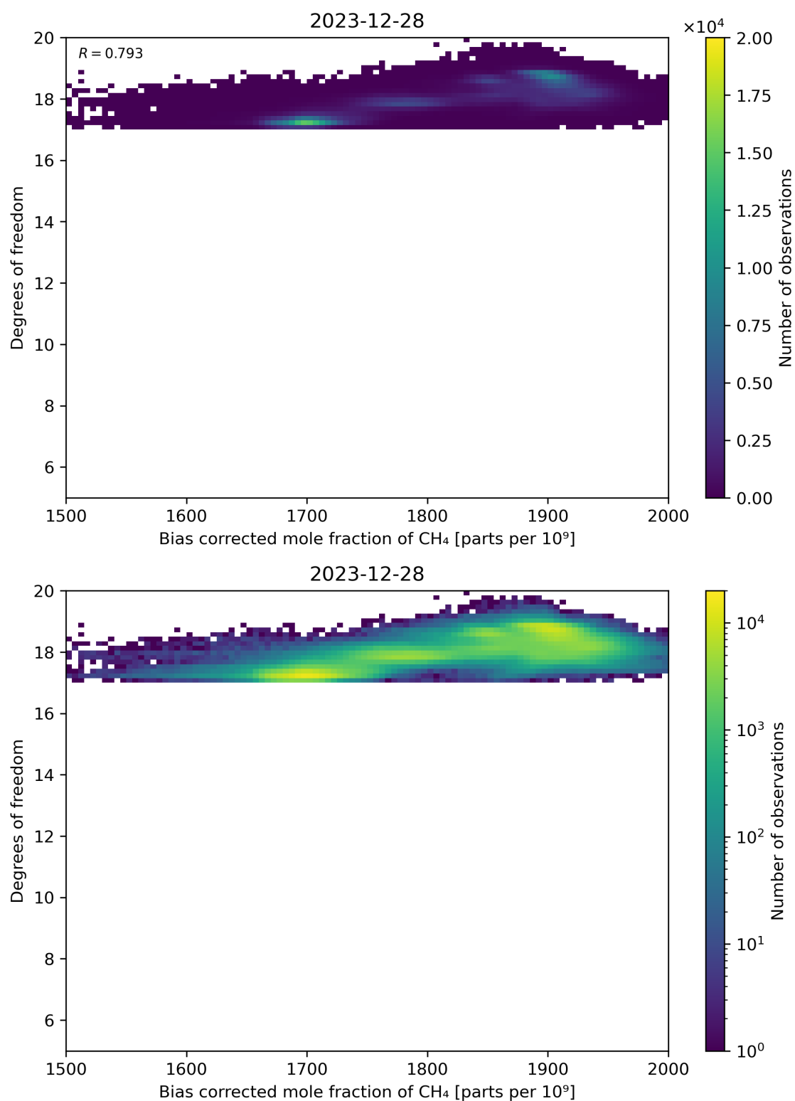
Figure 65: Scatter density plot of “Bias corrected mole fraction of CH 4 ” against “Degrees of freedom” for 2023-12-27 to 2023-12-29.
