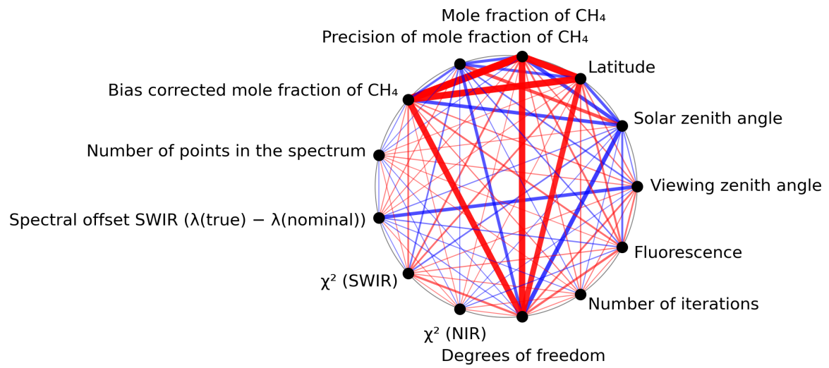
Figure 1: Map of correlation graph for 2023-12-27 to 2023-12-29.
