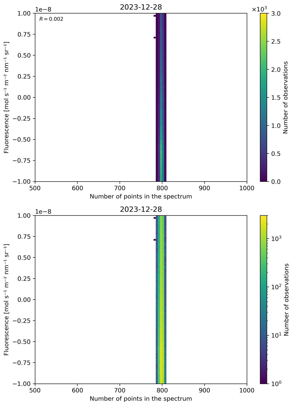
Figure 91: Scatter density plot of “Number of points in the spectrum” against “Fluorescence” for 2023-12-27 to 2023-12-29.
