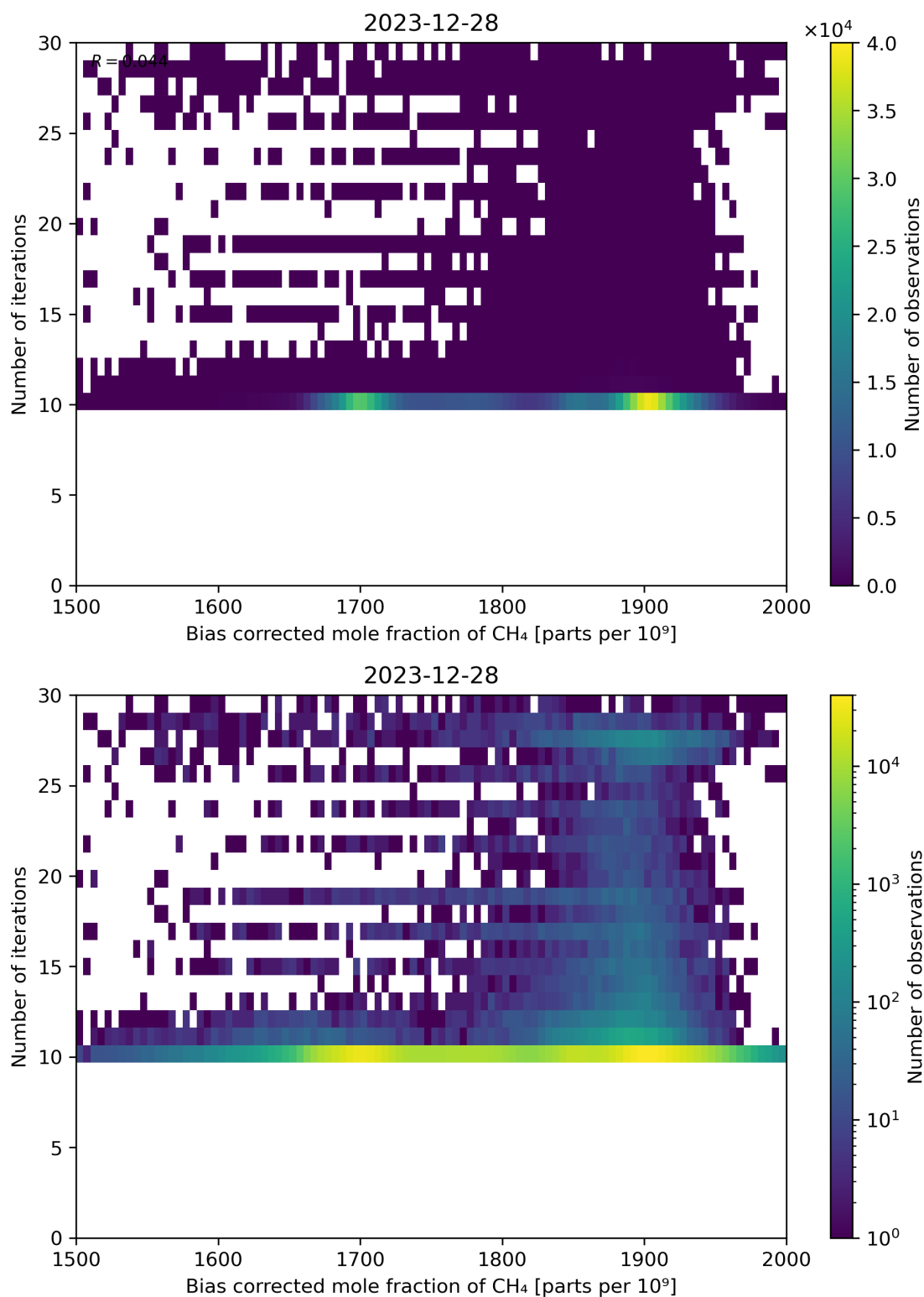
Figure 67: Scatter density plot of “Bias corrected mole fraction of CH 4 ” against “Number of iterations” for 2023-12-27 to 2023-12-29.
