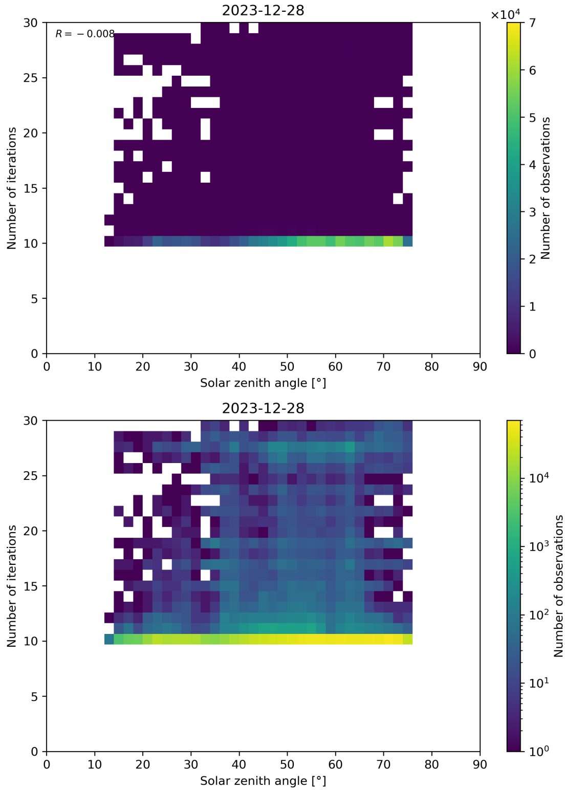
Figure 102: Scatter density plot of “Solar zenith angle” against “Number of iterations” for 2023-12-27 to 2023-12-29.
