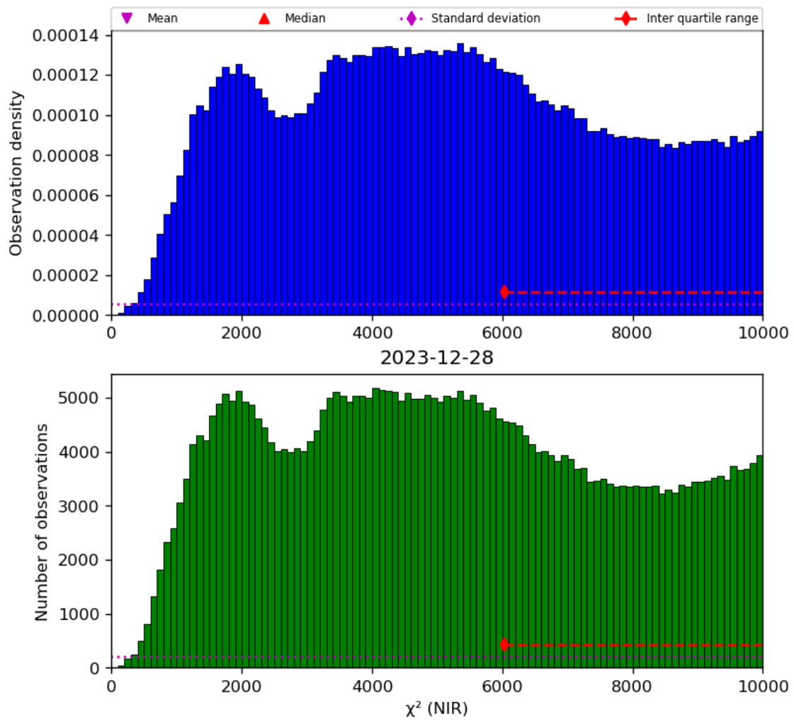
Figure 29: Histogram of “ \chi^2 (NIR)” for 2023-12-27 to 2023-12-29
