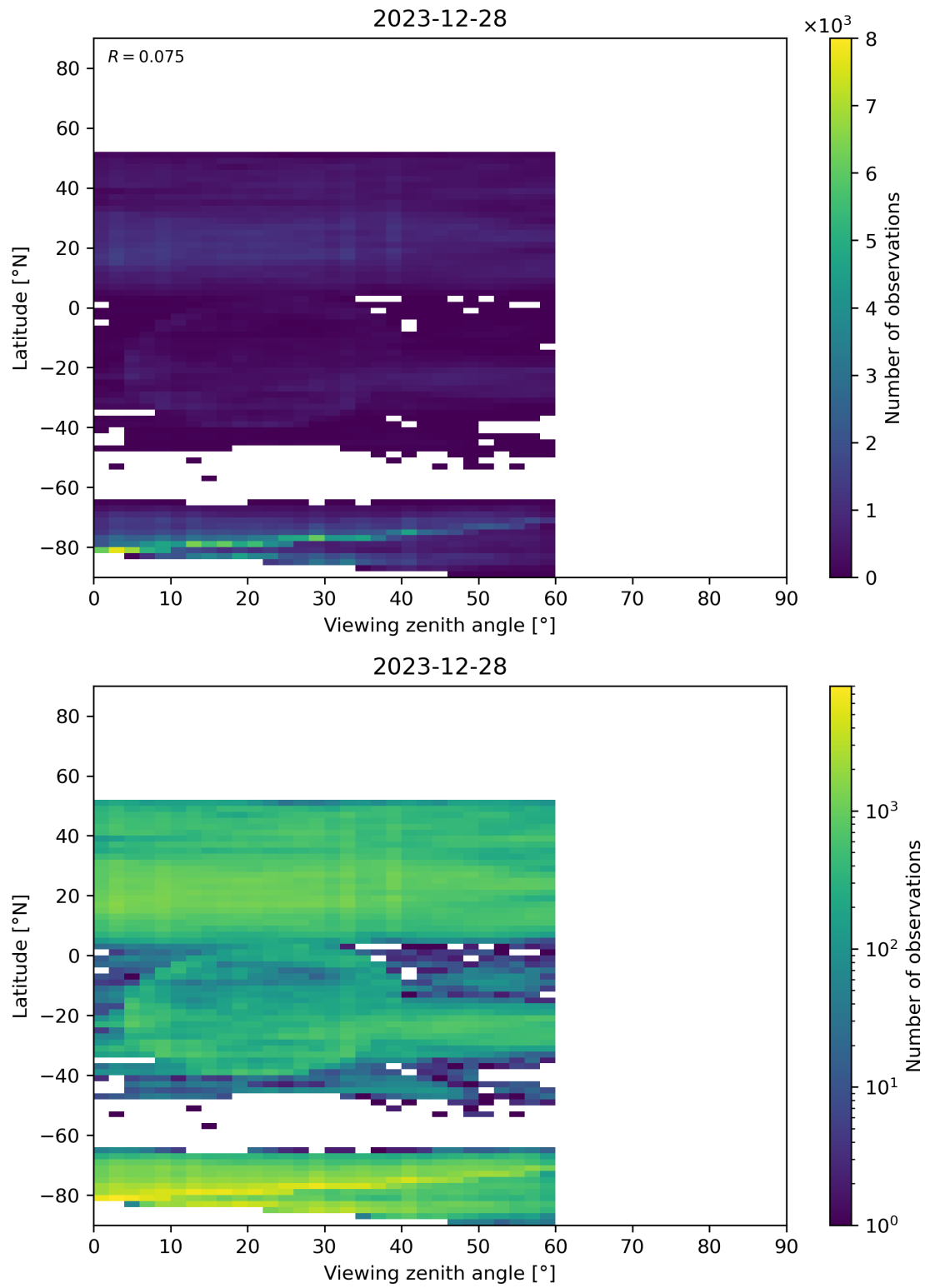
Figure 109: Scatter density plot of “Viewing zenith angle” against “Latitude” for 2023-12-27 to 2023-12-29.
