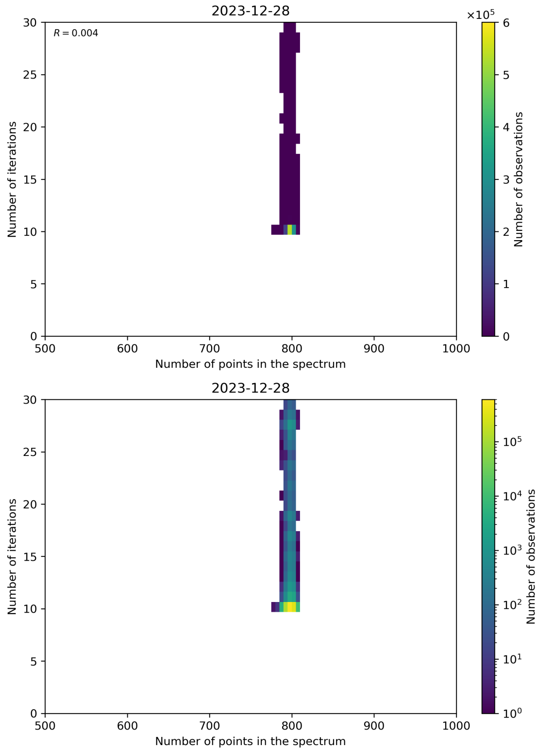
Figure 92: Scatter density plot of “Number of points in the spectrum” against “Number of iterations” for 2023-12-27 to 2023-12-29.
