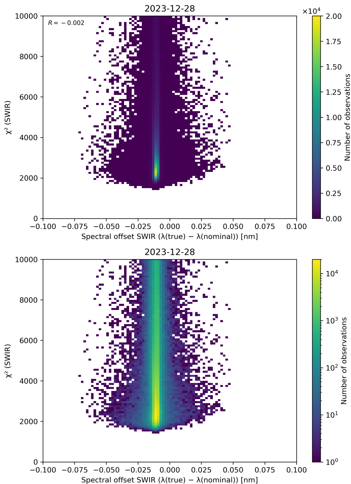
Figure 118: Scatter density plot of “Spectral offset SWIR ( \lambda(\text{true}) - \lambda(\text{nominal}) )” against “ \chi^2 (SWIR)” for 2023-12-27 to 2023-12-29.
