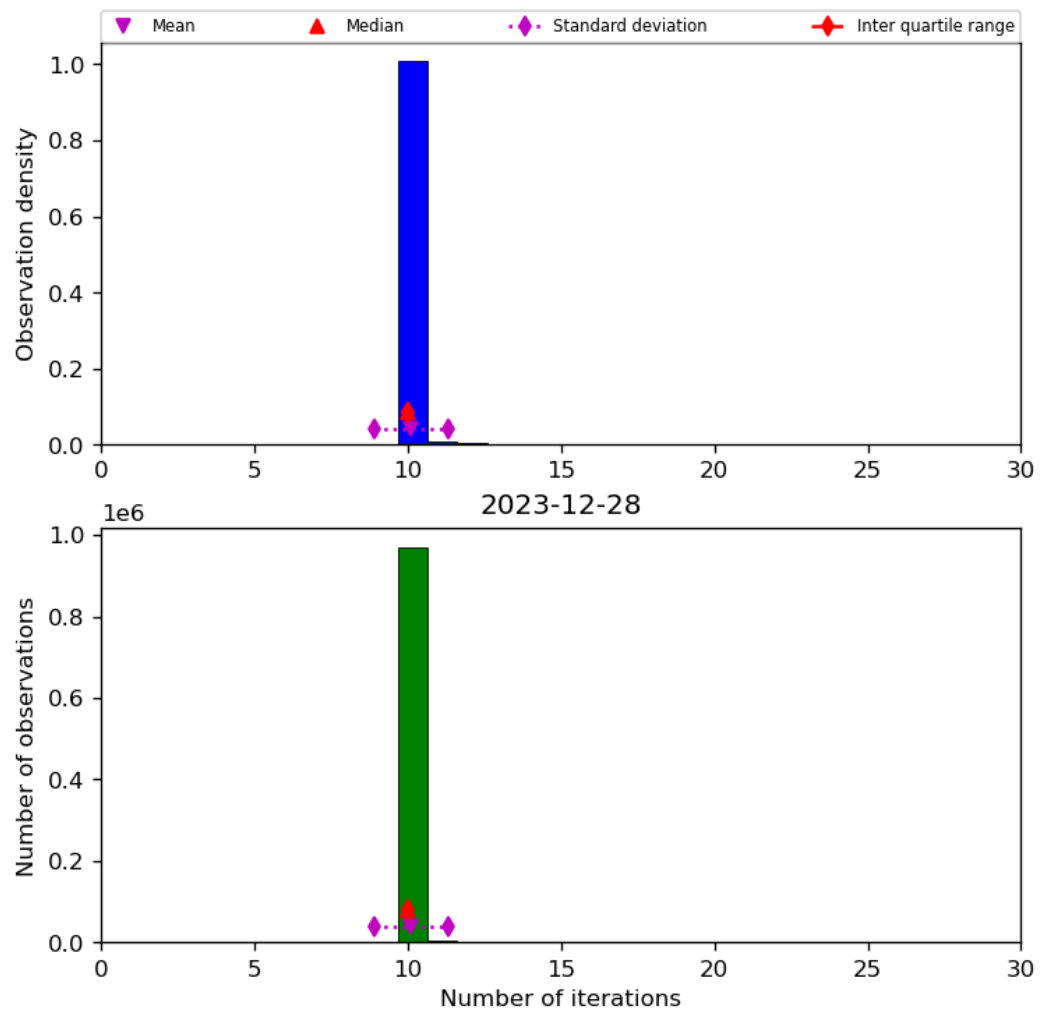
Figure 31: Histogram of “Number of iterations” for 2023-12-27 to 2023-12-29
