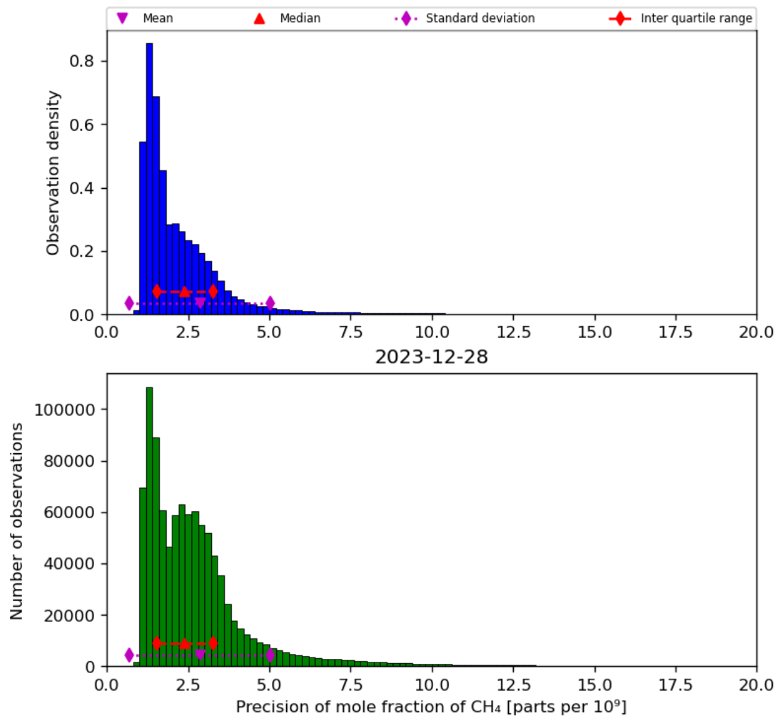
Figure 24: Histogram of “Precision of mole fraction of CH 4 ” for 2023-12-27 to 2023-12-29
