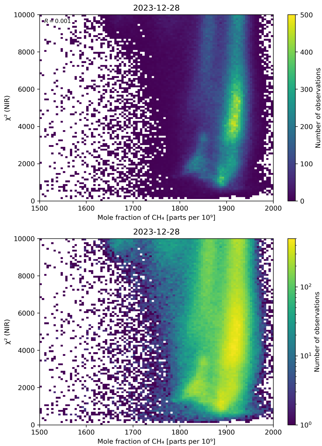
Figure 70: Scatter density plot of “Mole fraction of CH 4 ” against “ \chi^2 (NIR)” for 2023-12-27 to 2023-12-29.
