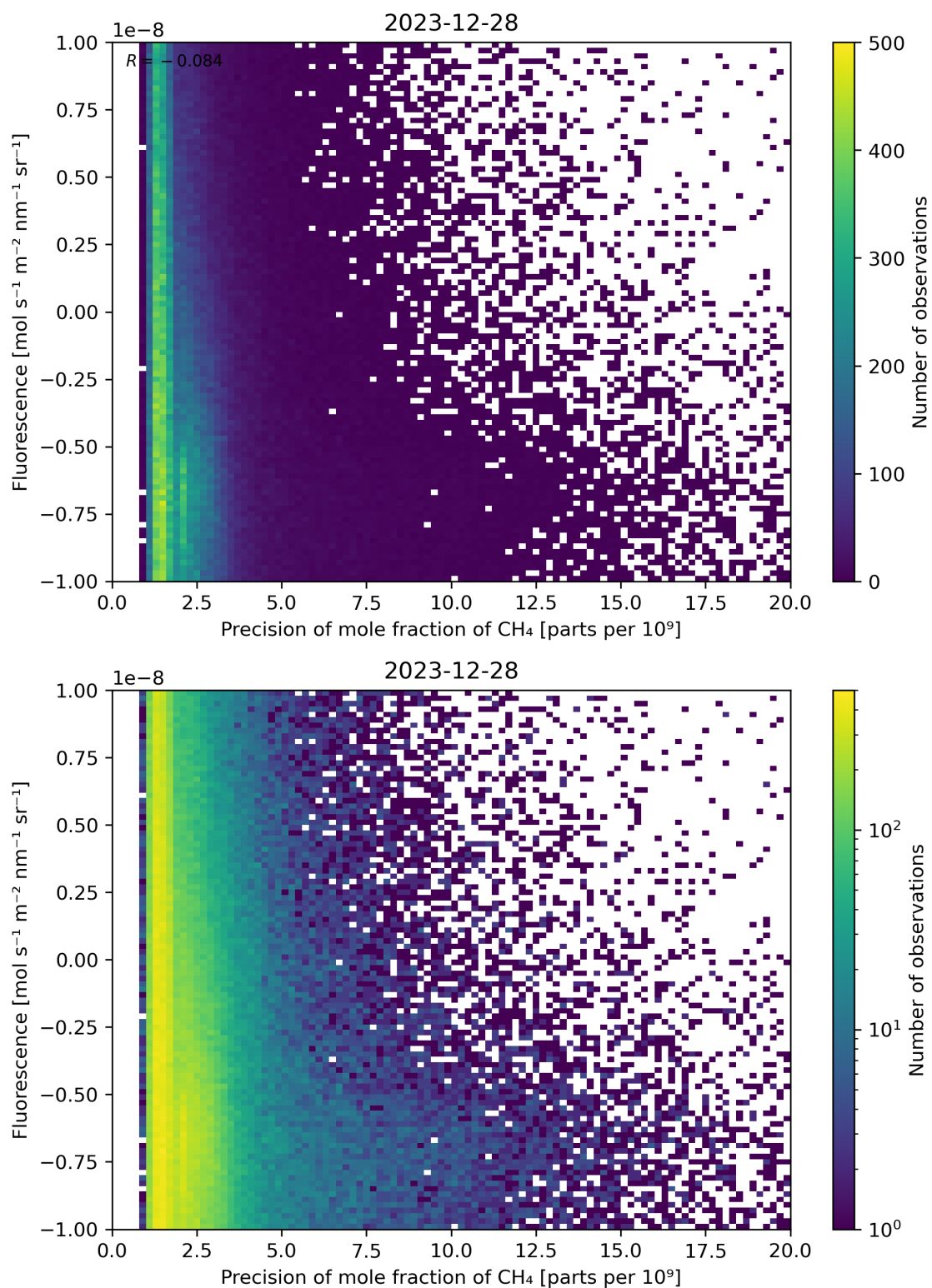
Figure 81: Scatter density plot of “Precision of mole fraction of \text{CH}_4 ” against “Fluorescence” for 2023-12-27 to 2023-12-29.
