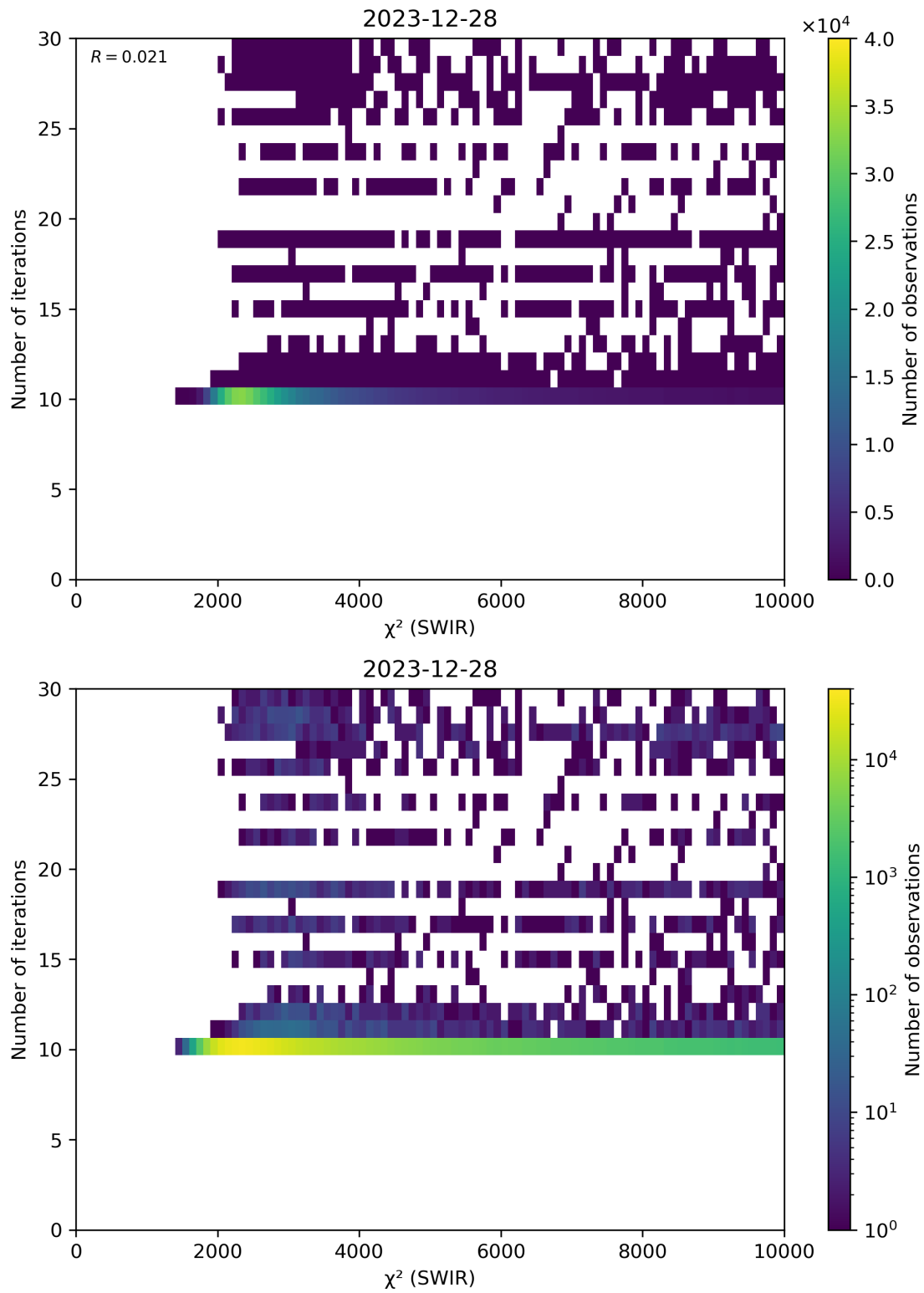
Figure 50: Scatter density plot of “ \chi^2 (SWIR)” against “Number of iterations” for 2023-12-27 to 2023-12-29.
