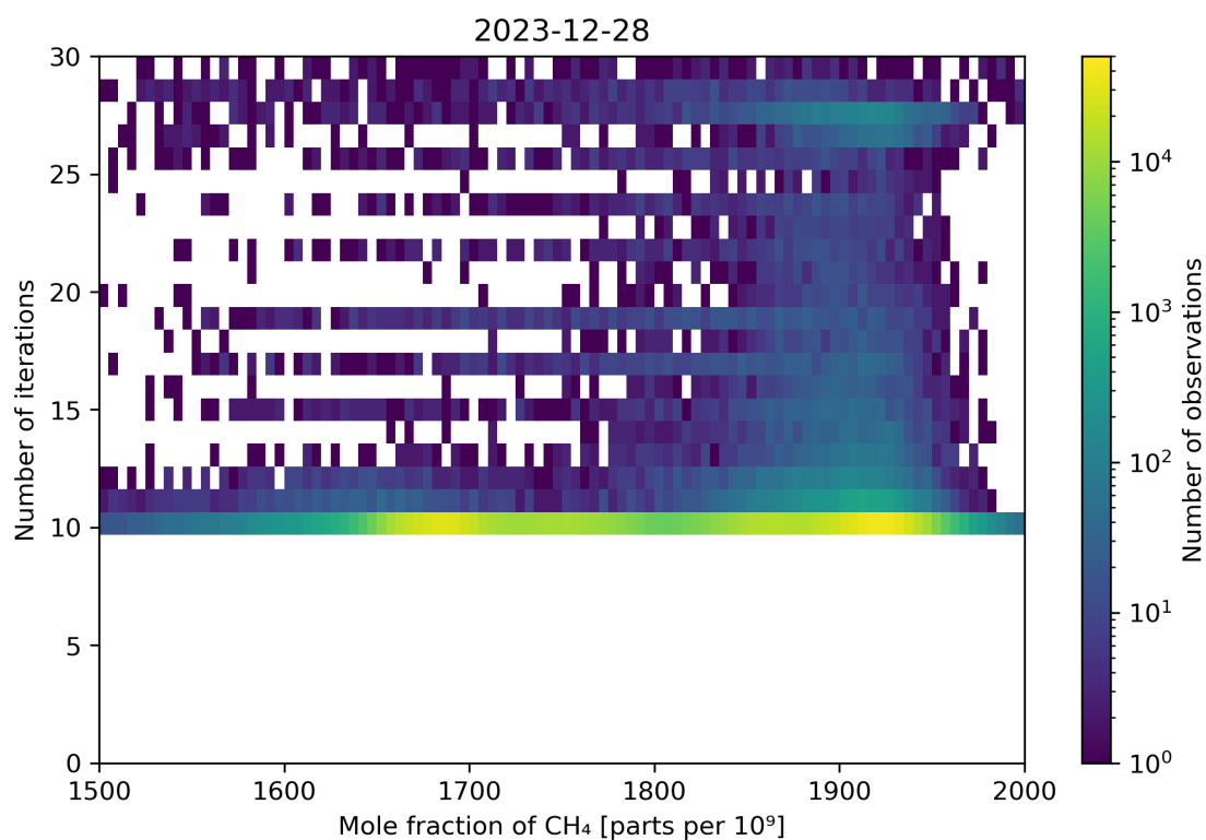
Figure 76: Scatter density plot of “Mole fraction of CH 4 ” against “Number of iterations” for 2023-12-27 to 2023-12-29.
