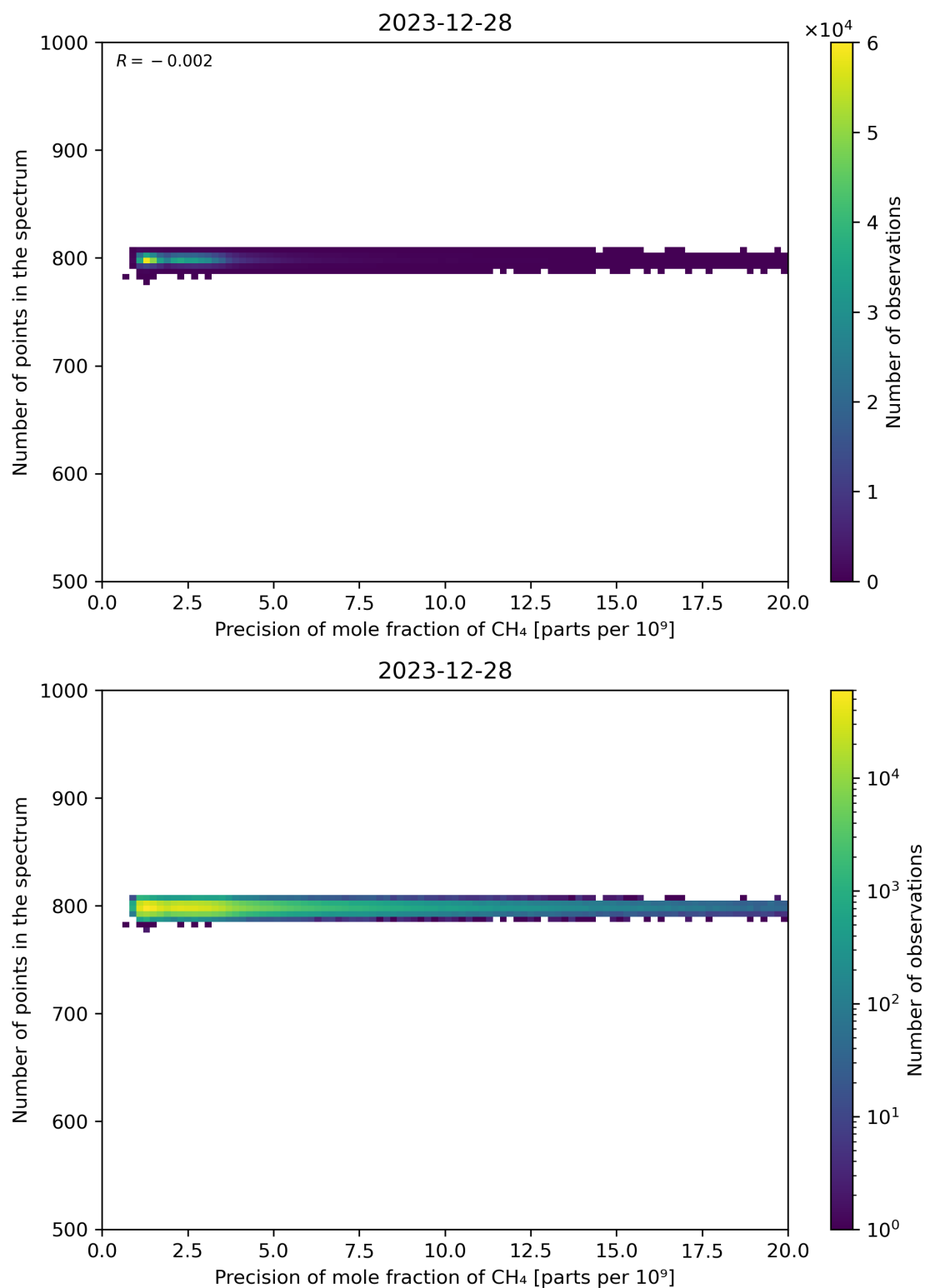
Figure 84: Scatter density plot of “Precision of mole fraction of CH 4 ” against “Number of points in the spectrum” for 2023-12-27 to 2023-12-29.
