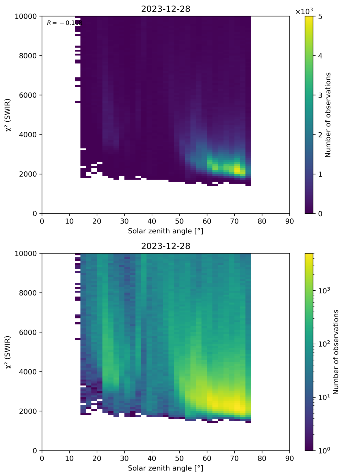
Figure 95: Scatter density plot of “Solar zenith angle” against “ \chi^2 (SWIR)” for 2023-12-27 to 2023-12-29.
