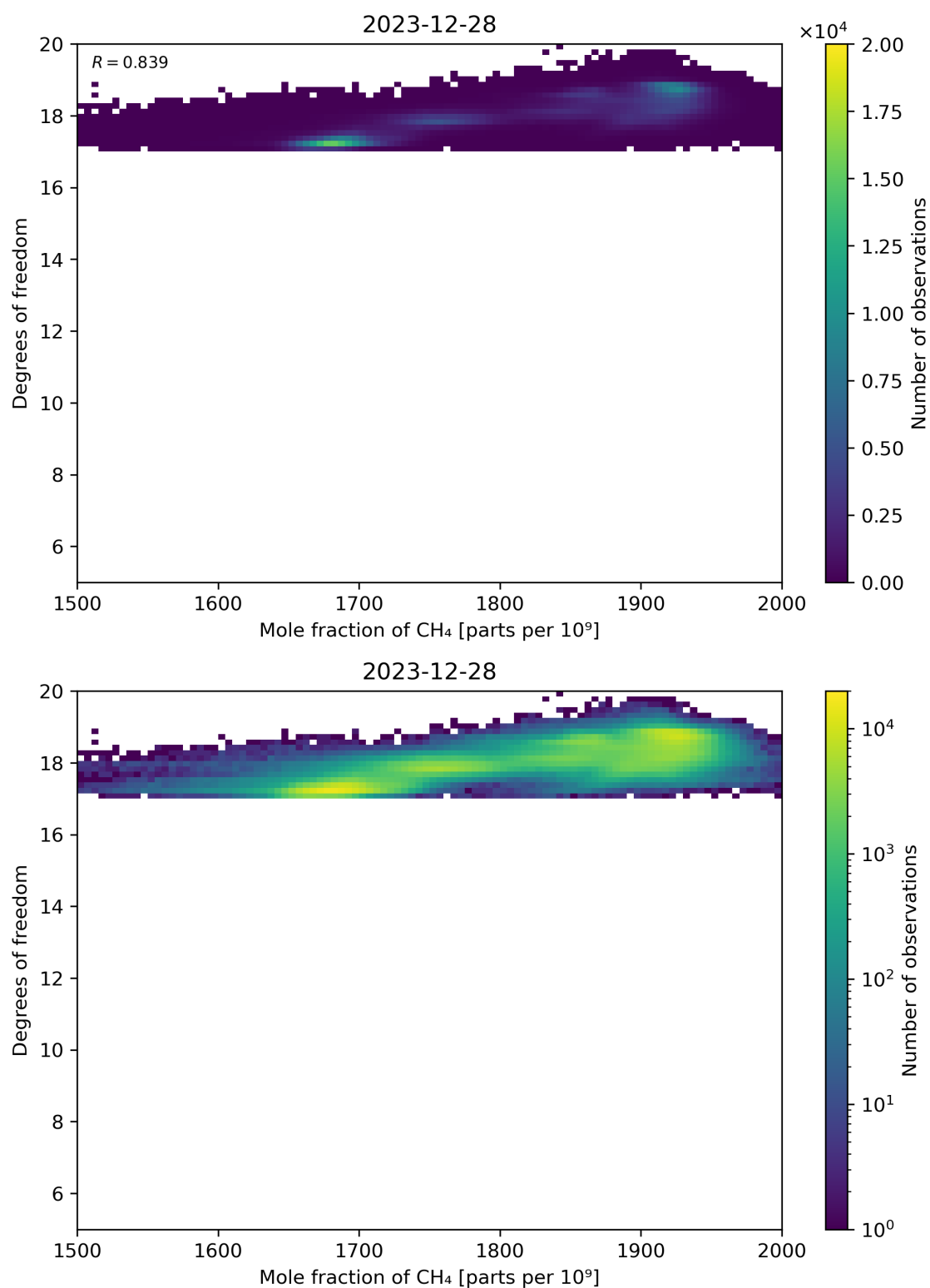
Figure 72: Scatter density plot of “Mole fraction of CH 4 ” against “Degrees of freedom” for 2023-12-27 to 2023-12-29.
