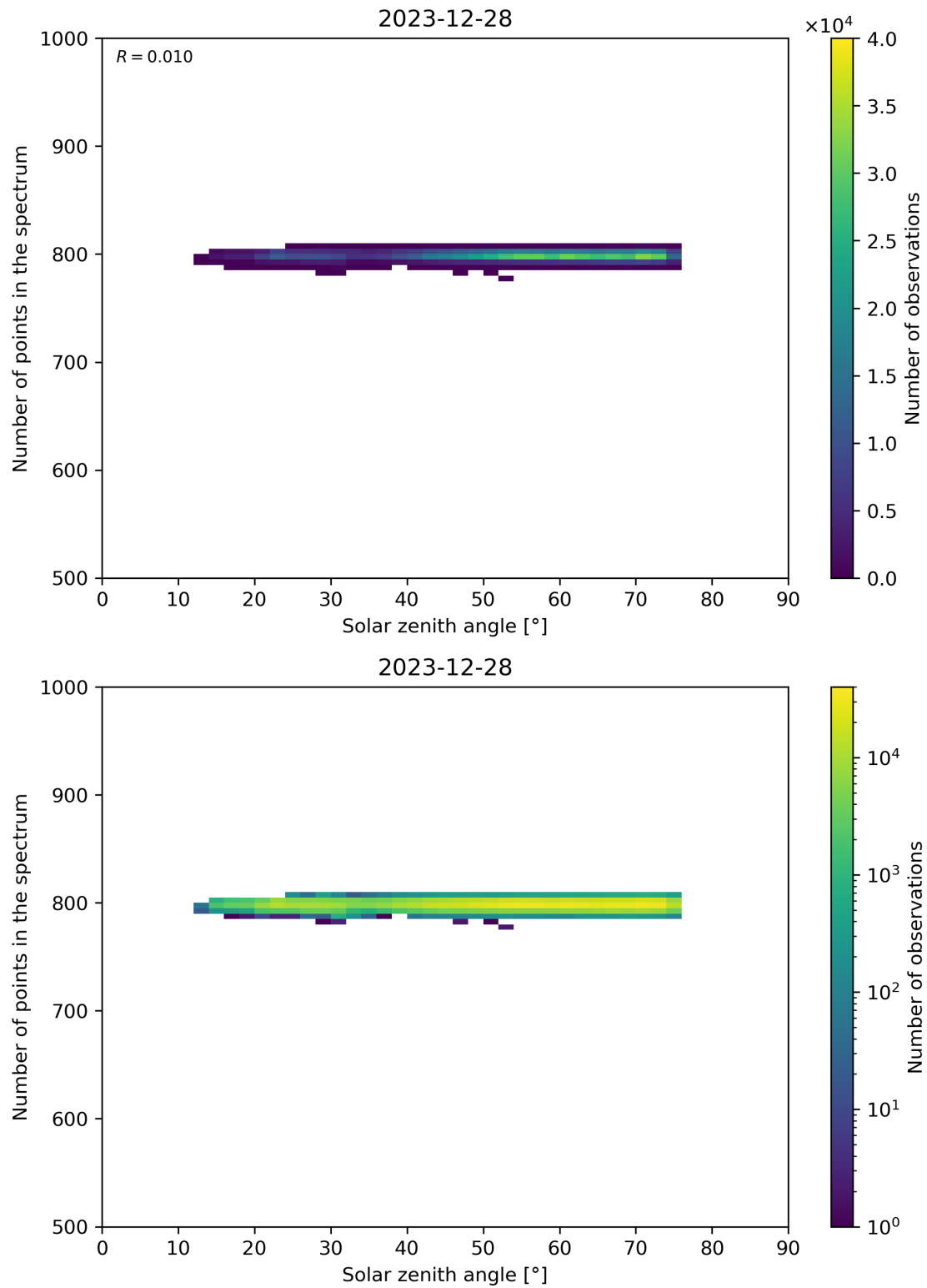
Figure 103: Scatter density plot of “Solar zenith angle” against “Number of points in the spectrum” for 2023-12-27 to 2023-12-29.
