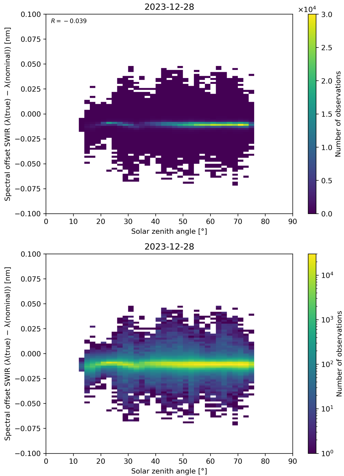
Figure 104: Scatter density plot of “Solar zenith angle” against “Spectral offset SWIR ( \lambda(\text{true}) - \lambda(\text{nominal}) )” for 2023-12-27 to 2023-12-29.
