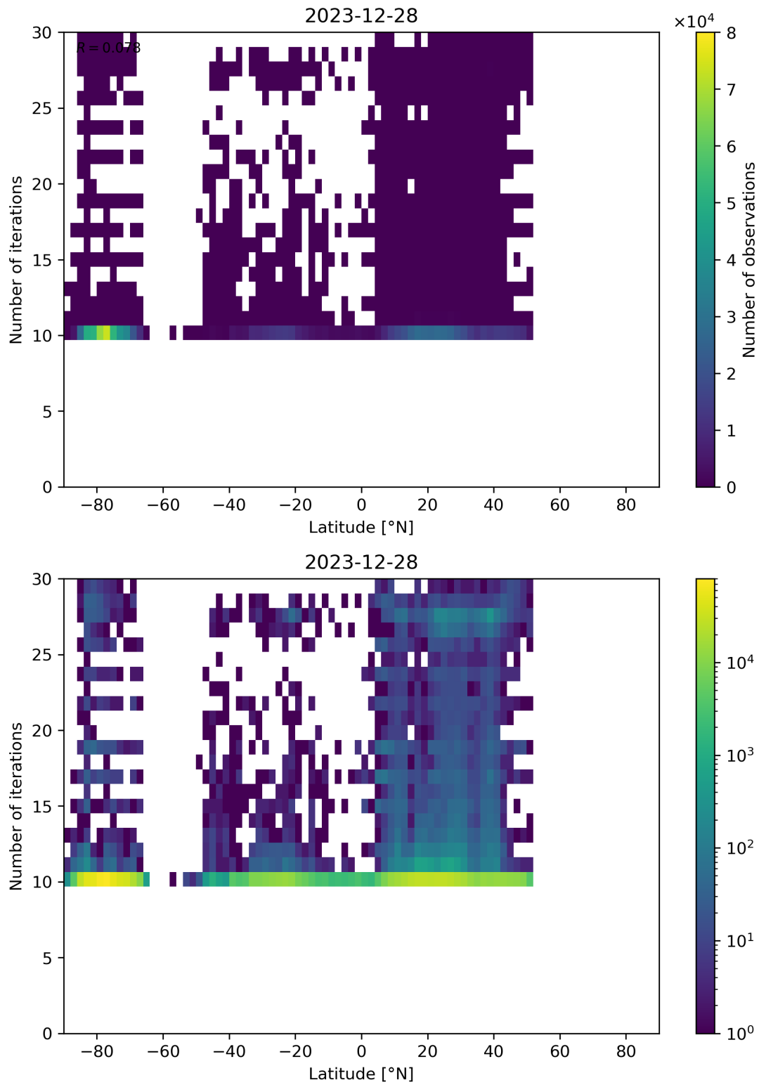
Figure 60: Scatter density plot of “Latitude” against “Number of iterations” for 2023-12-27 to 2023-12-29.
