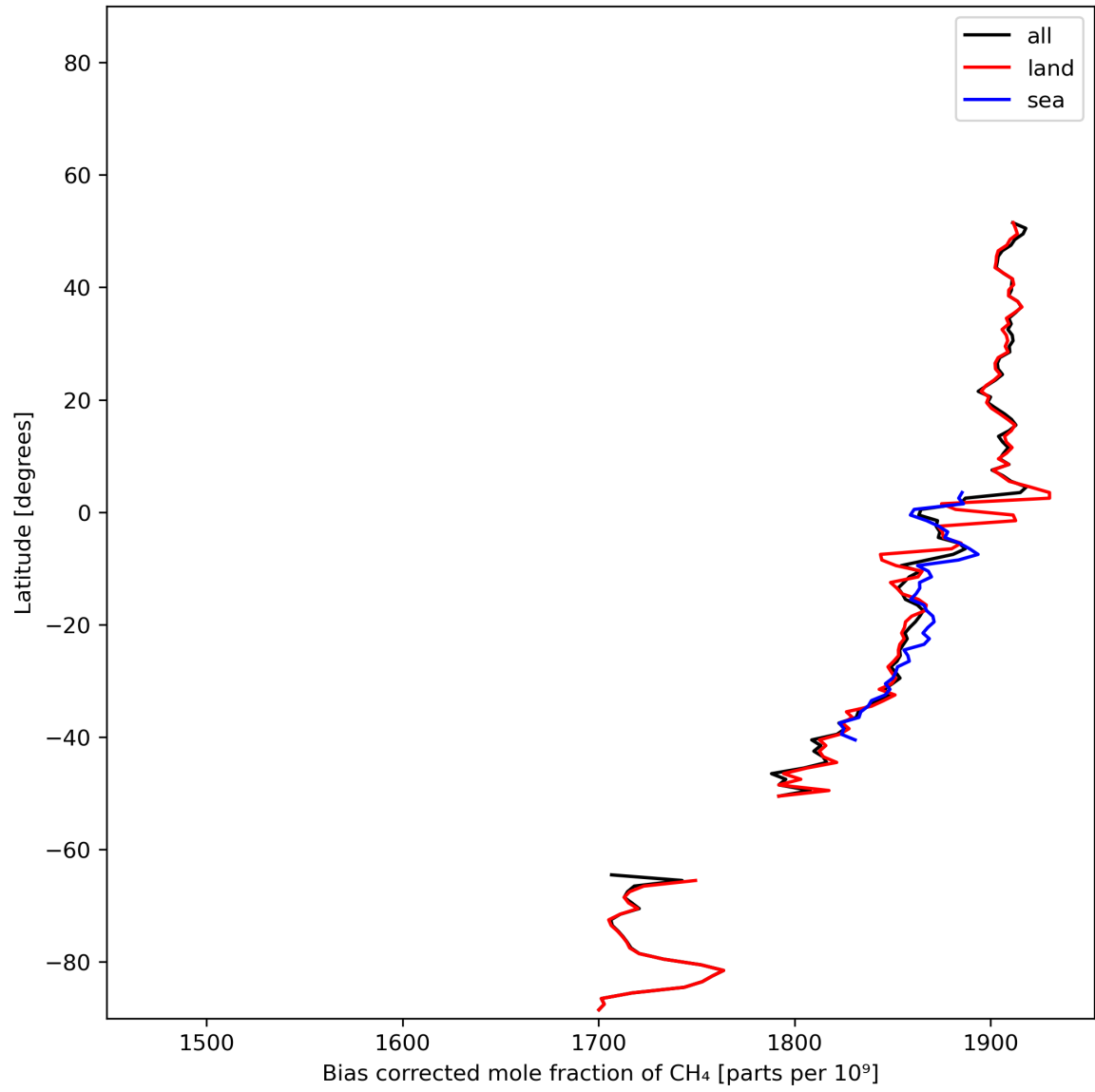
Figure 14: Zonal average of “Bias corrected mole fraction of CH 4 ” for 2023-12-27 to 2023-12-29.
