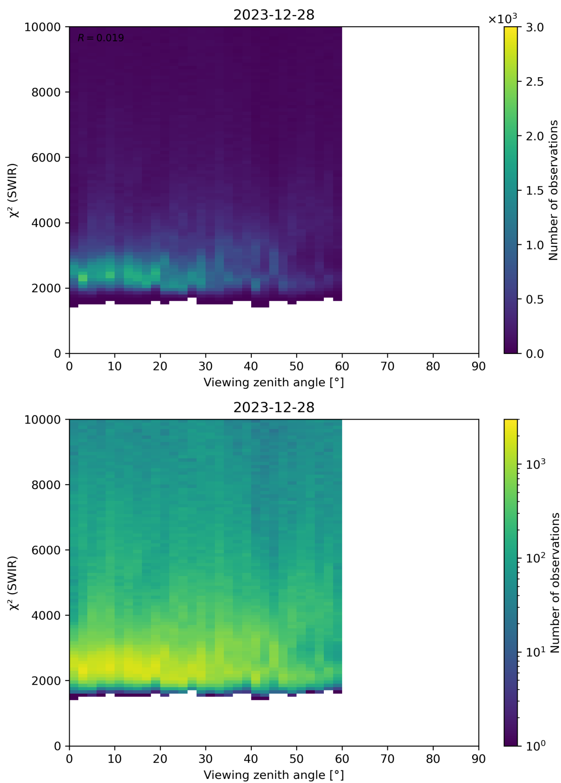
Figure 106: Scatter density plot of “Viewing zenith angle” against “ \chi^2 (SWIR)” for 2023-12-27 to 2023-12-29.
