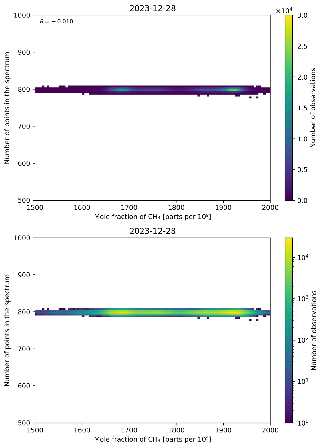
Figure 77: Scatter density plot of “Mole fraction of CH 4 ” against “Number of points in the spectrum” for 2023-12-27 to 2023-12-29.
