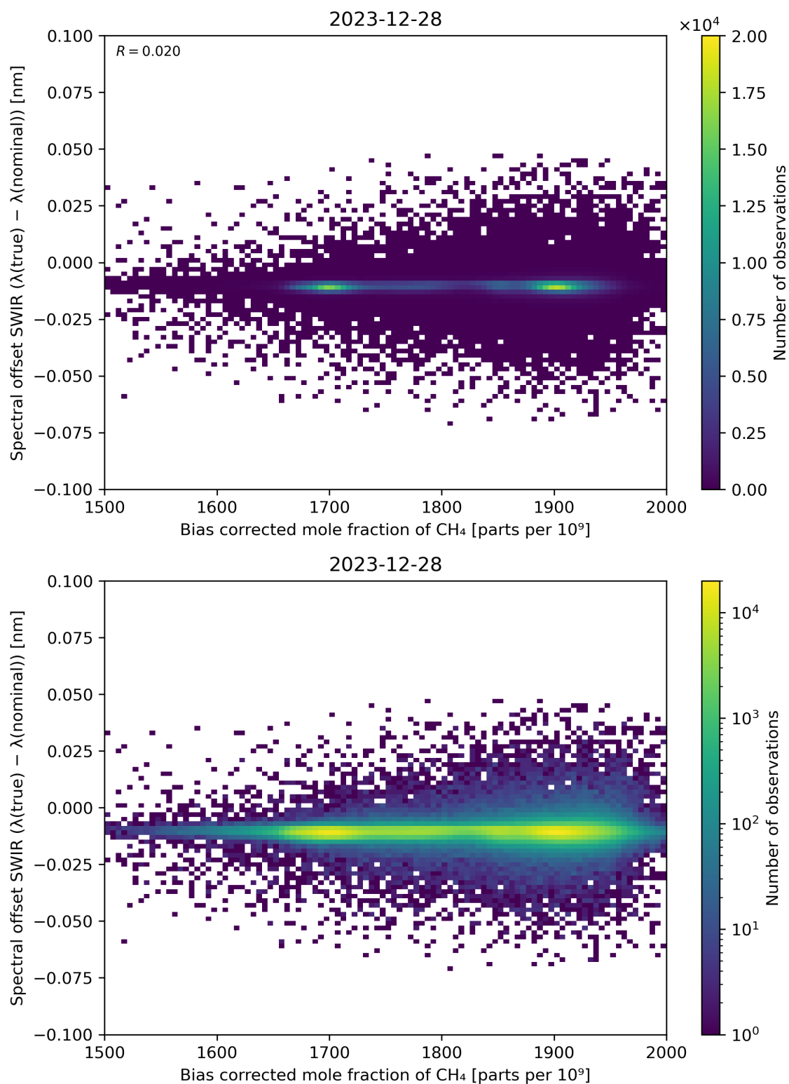
Figure 69: Scatter density plot of “Bias corrected mole fraction of \text{CH}_4 ” against “Spectral offset SWIR ( \lambda(\text{true}) - \lambda(\text{nominal}) )” for 2023-12-27 to 2023-12-29.
