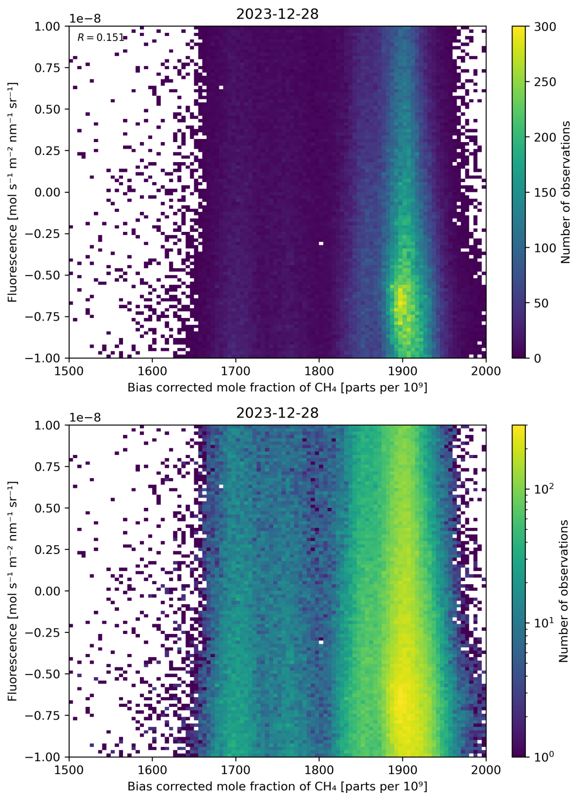
Figure 66: Scatter density plot of “Bias corrected mole fraction of \text{CH}_4 ” against “Fluorescence” for 2023-12-27 to 2023-12-29.
