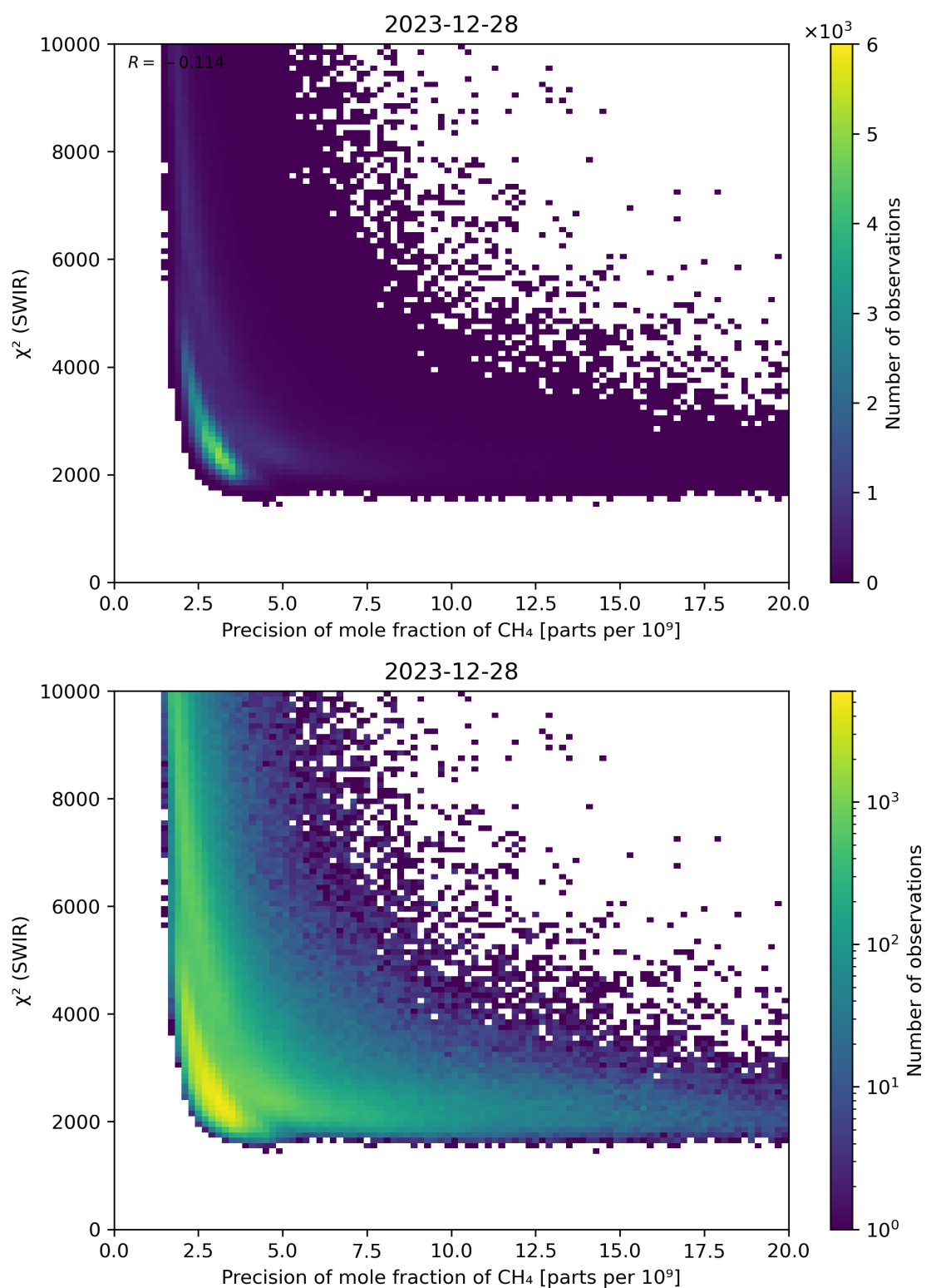
Figure 79: Scatter density plot of “Precision of mole fraction of CH 4 ” against “ \chi^2 (SWIR)” for 2023-12-27 to 2023-12-29.
