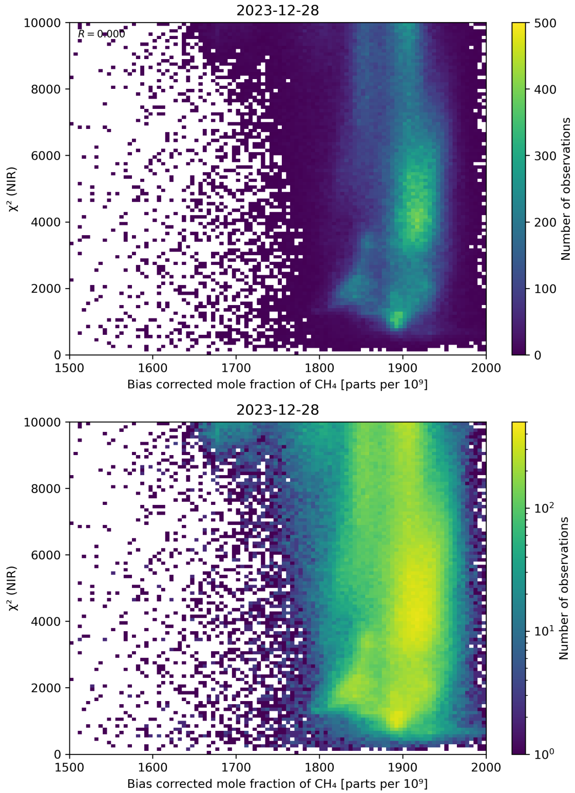
Figure 63: Scatter density plot of “Bias corrected mole fraction of CH 4 ” against “ \chi^2 (NIR)” for 2023-12-27 to 2023-12-29.
