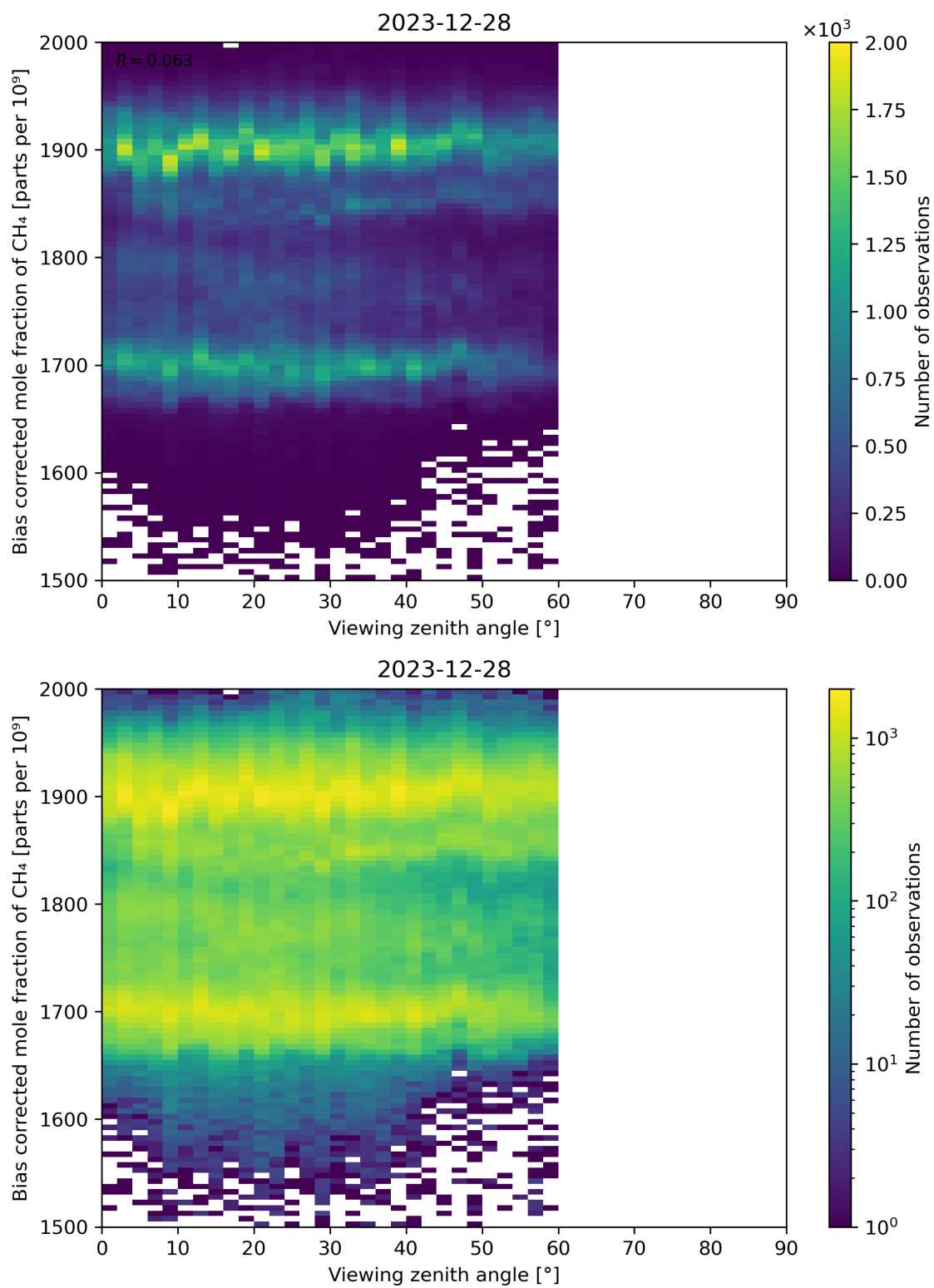
Figure 111: Scatter density plot of “Viewing zenith angle” against “Bias corrected mole fraction of CH 4 ” for 2023-12-27 to 2023-12-29.
