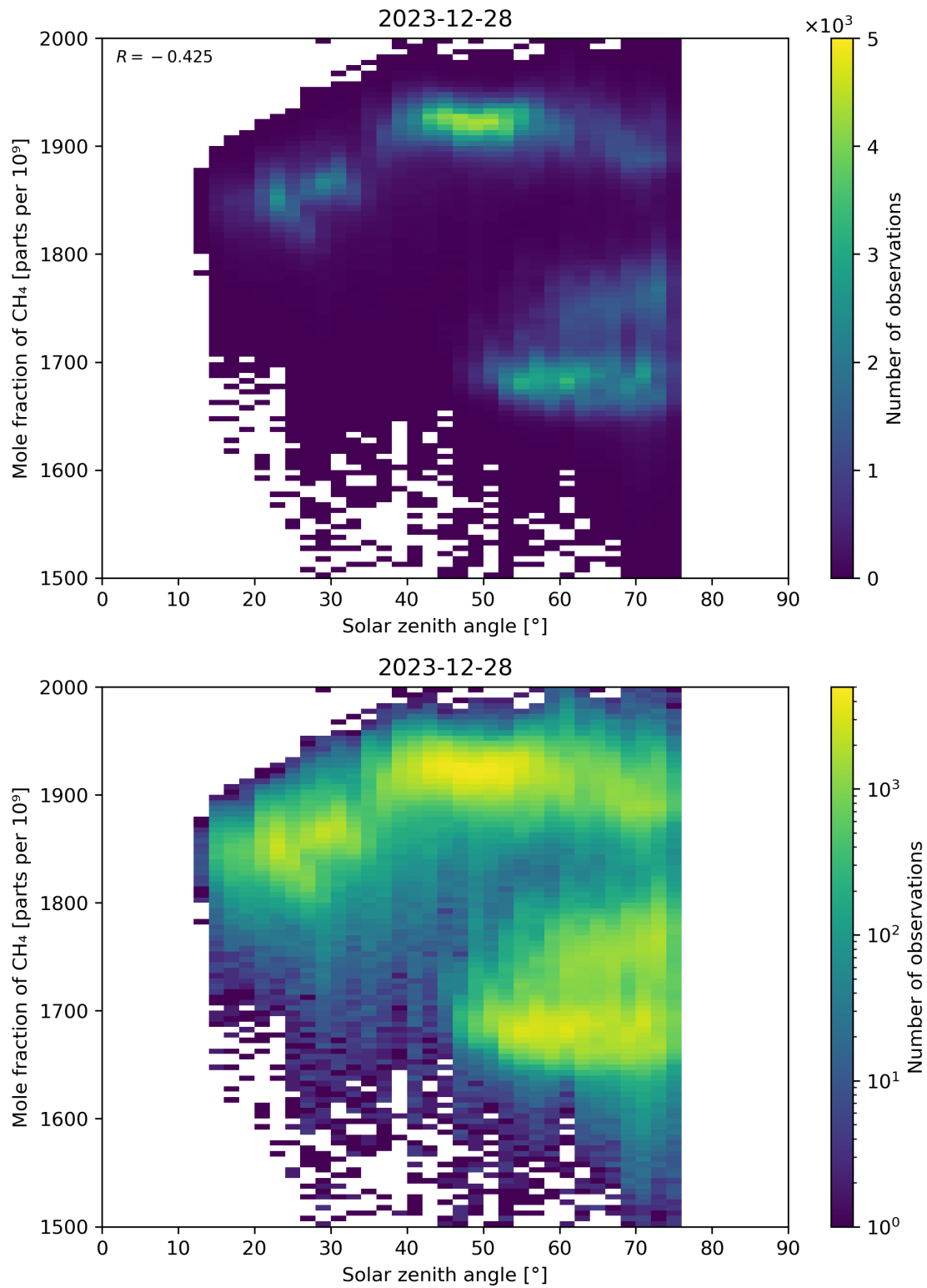
Figure 99: Scatter density plot of “Solar zenith angle” against “Mole fraction of CH 4 ” for 2023-12-27 to 2023-12-29.
