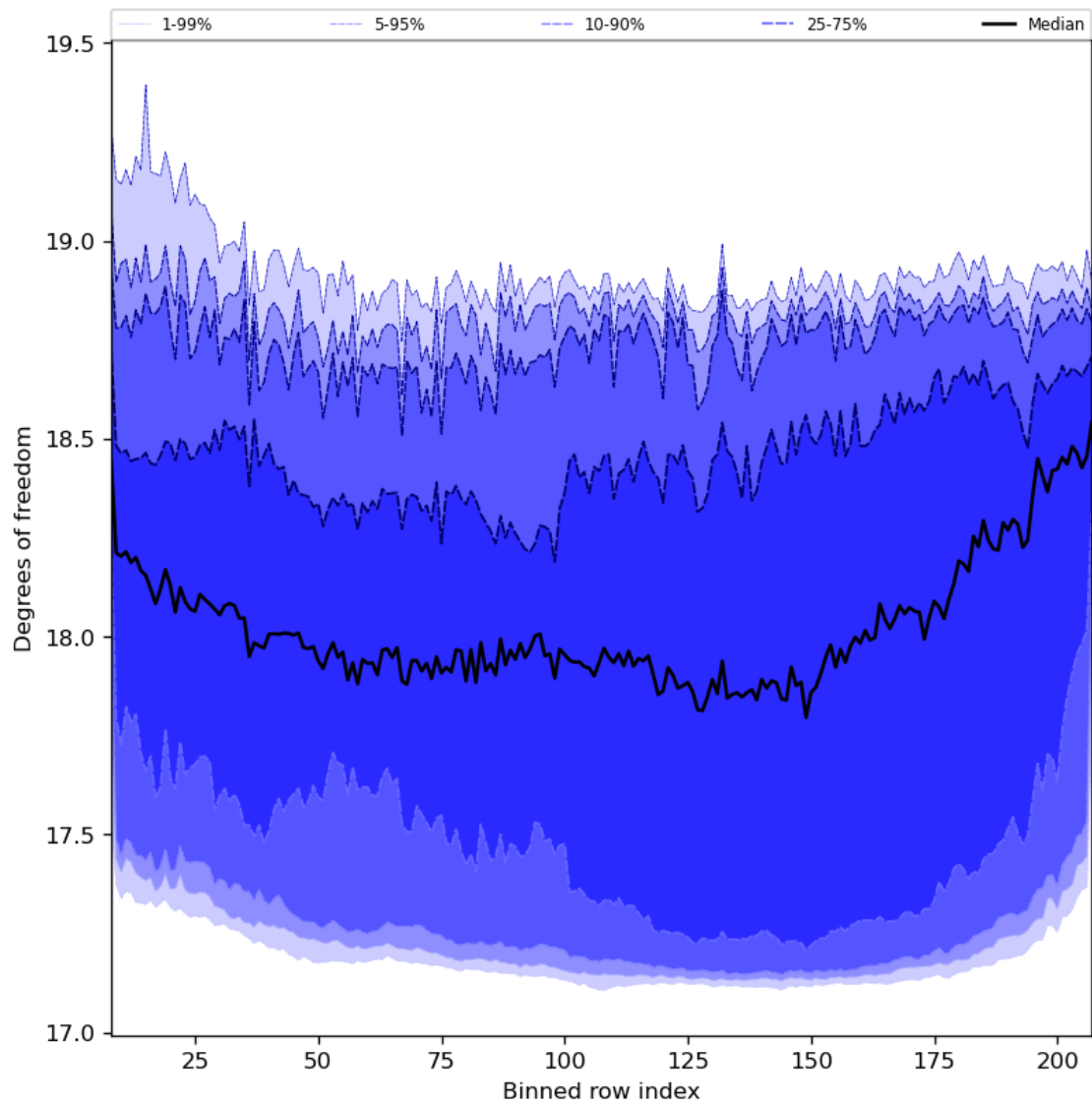
Figure 41: Along track statistics of “Degrees of freedom” for 2023-12-27 to 2023-12-29
