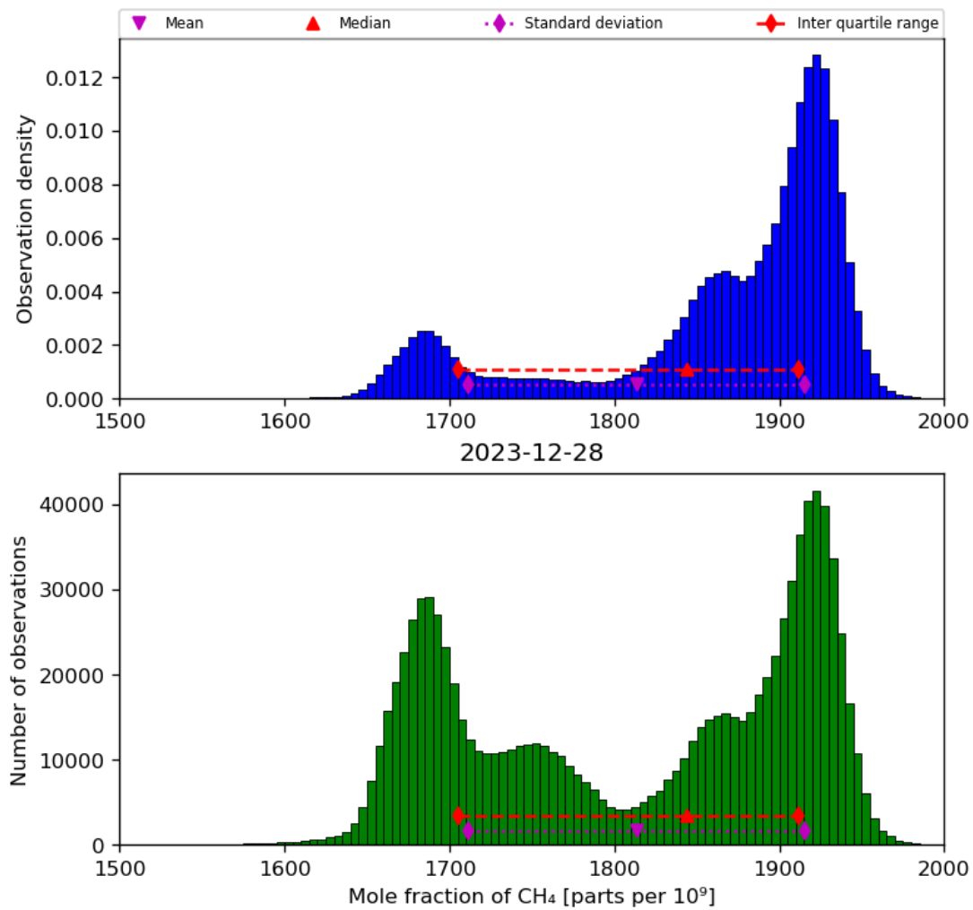
Figure 23: Histogram of “Mole fraction of CH 4 ” for 2023-12-27 to 2023-12-29
