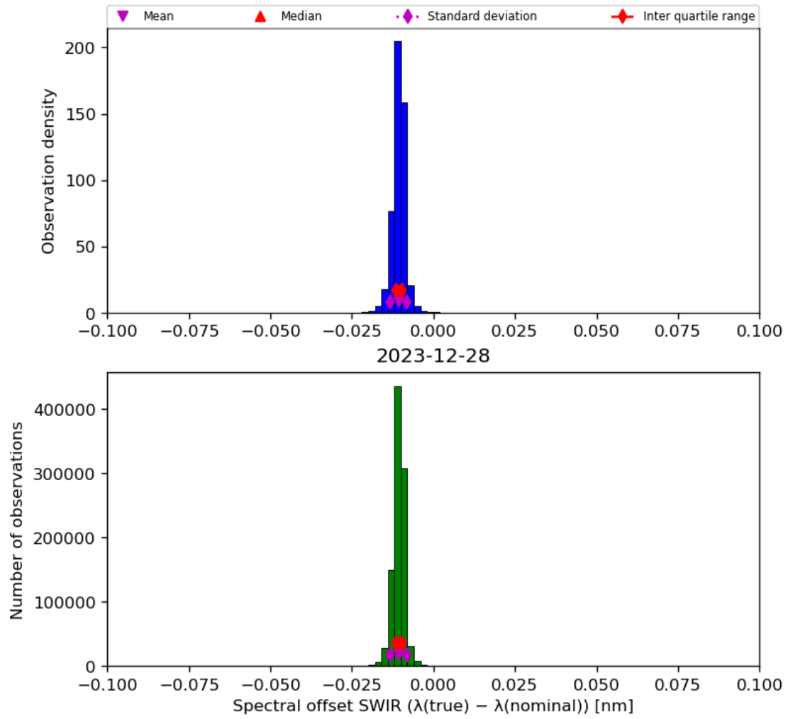
Figure 27: Histogram of “Spectral offset SWIR ( \lambda(\text{true}) - \lambda(\text{nominal}) )” for 2023-12-27 to 2023-12-29
