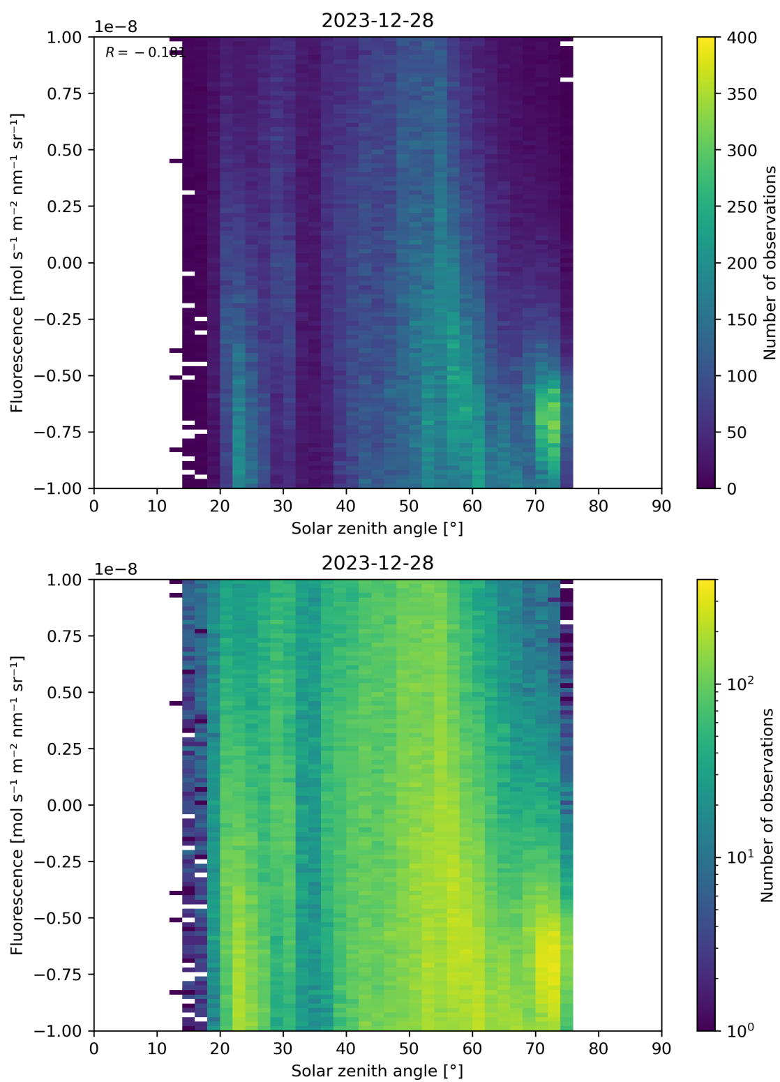
Figure 97: Scatter density plot of “Solar zenith angle” against “Fluorescence” for 2023-12-27 to 2023-12-29.
