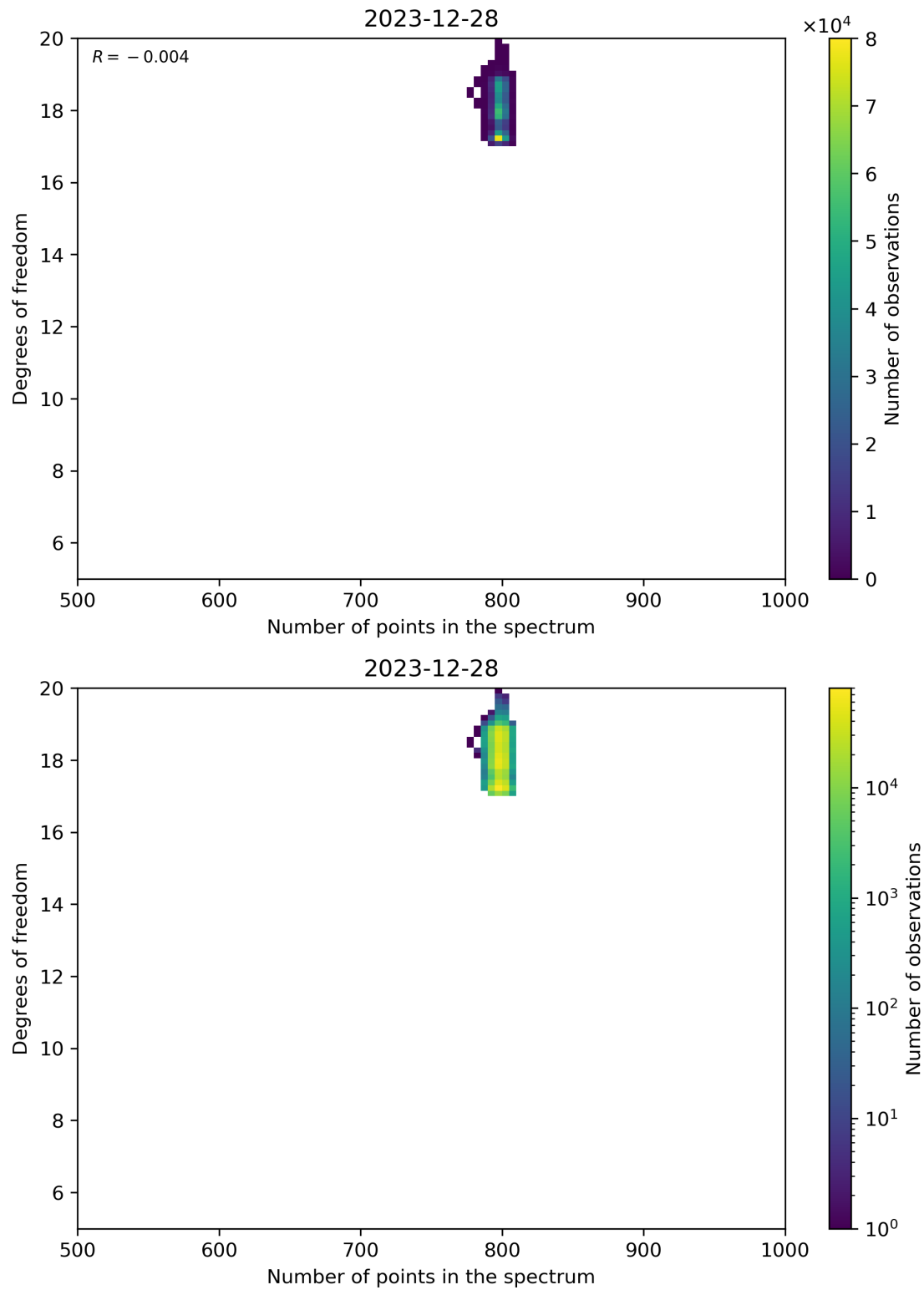
Figure 90: Scatter density plot of “Number of points in the spectrum” against “Degrees of freedom” for 2023-12-27 to 2023-12-29.
