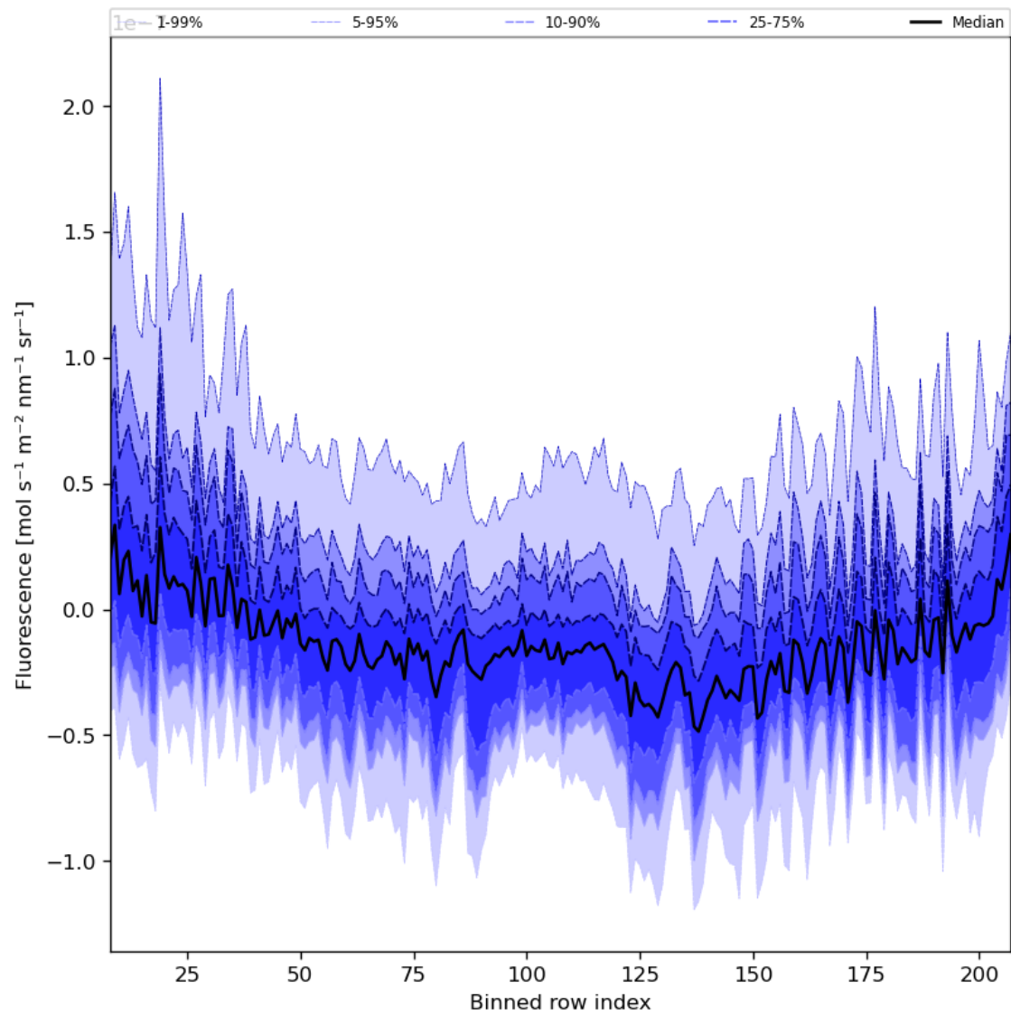
Figure 43: Along track statistics of “Fluorescence” for 2023-12-27 to 2023-12-29
