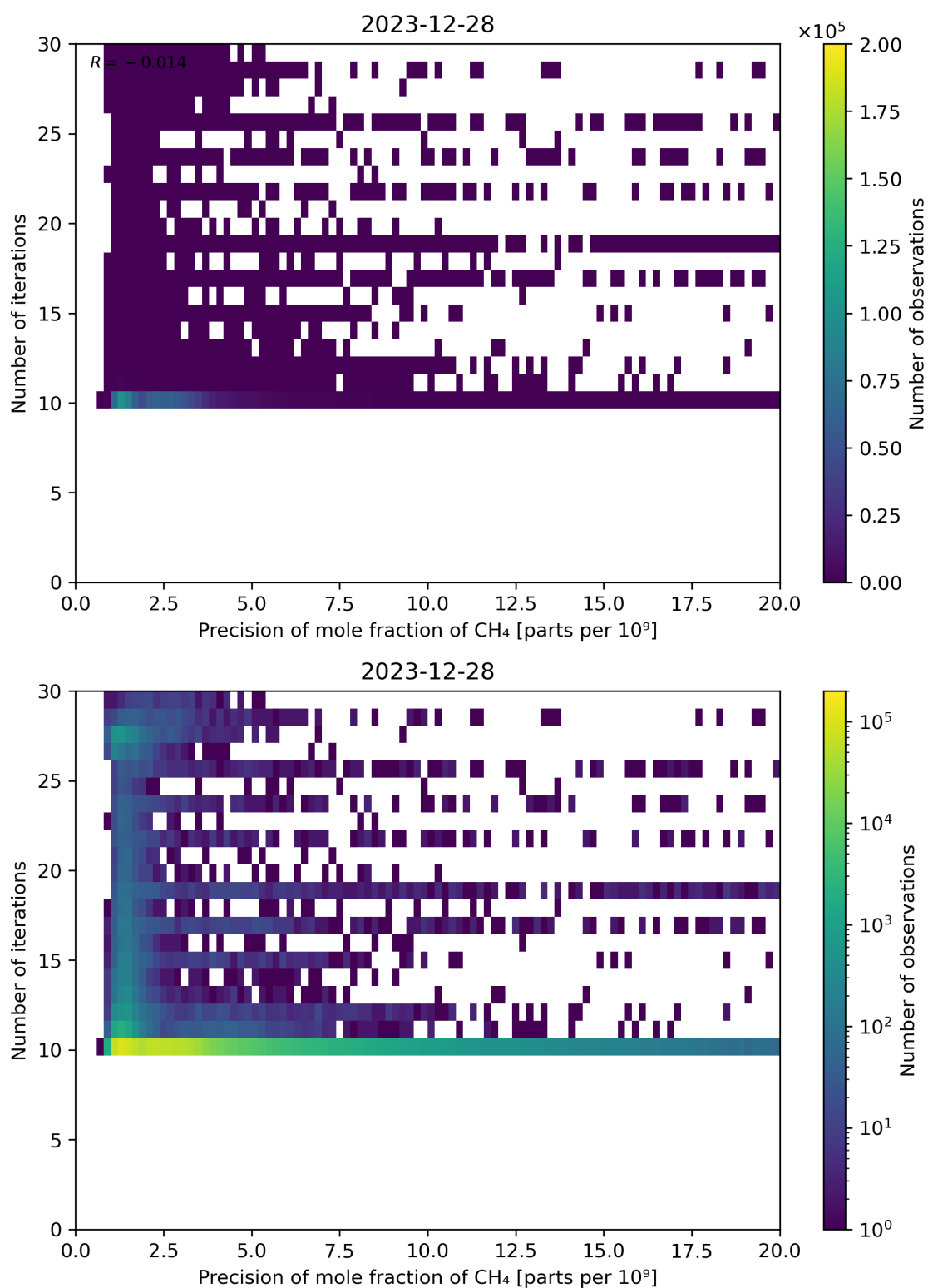
Figure 83: Scatter density plot of “Precision of mole fraction of CH 4 ” against “Number of iterations” for 2023-12-27 to 2023-12-29.
