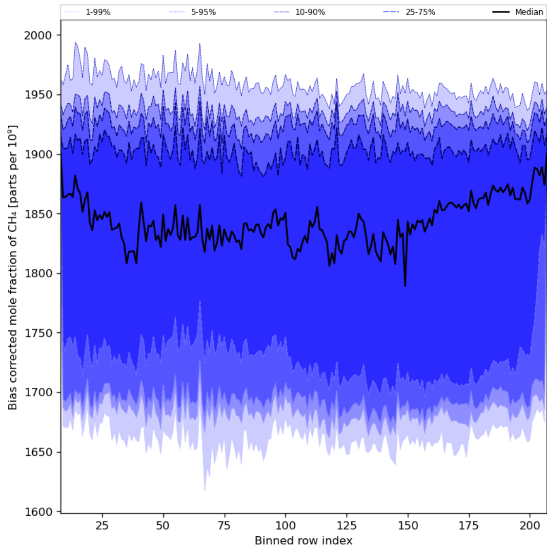
Figure 36: Along track statistics of “Bias corrected mole fraction of CH 4 ” for 2023-12-27 to 2023-12-29
