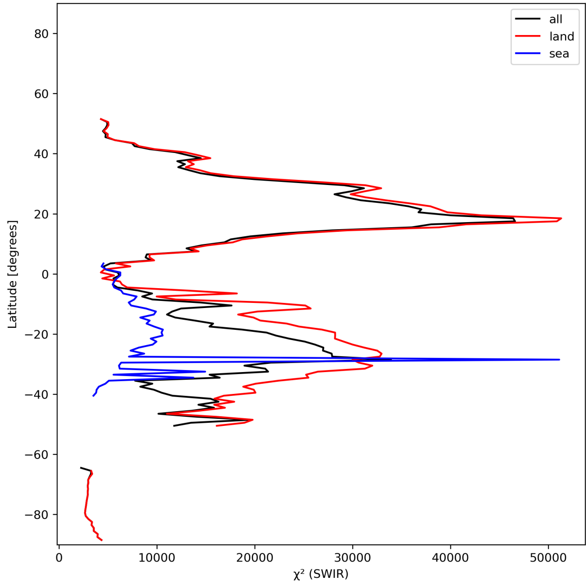
Figure 17: Zonal average of “ \chi^2 (SWIR)” for 2023-12-27 to 2023-12-29.
