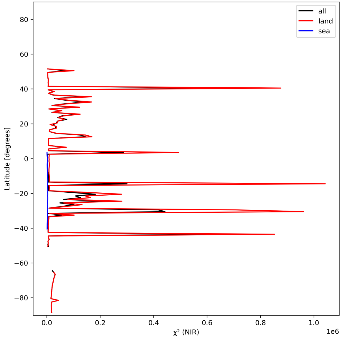
Figure 18: Zonal average of “ \chi^2 (NIR)” for 2023-12-27 to 2023-12-29.
