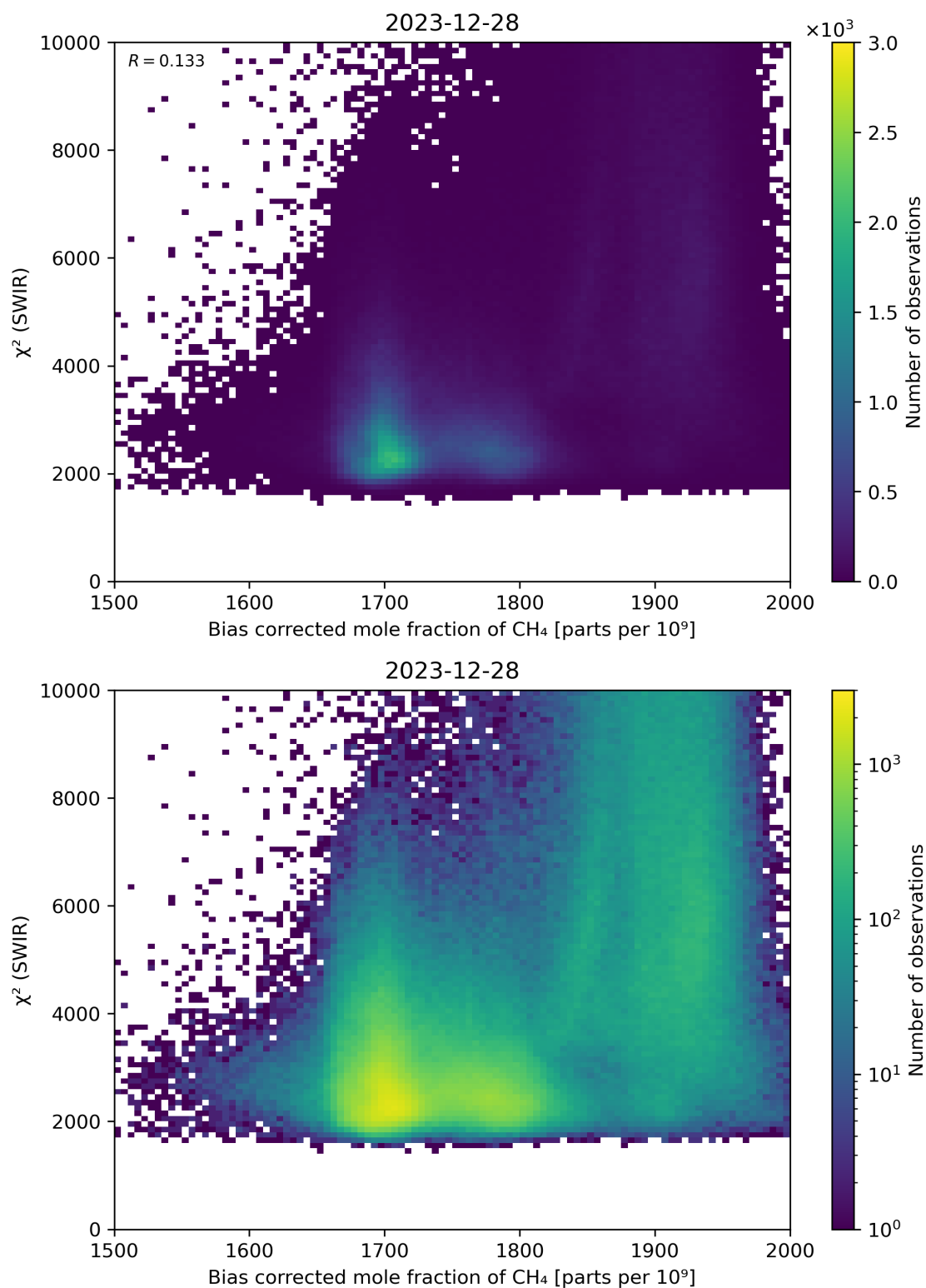
Figure 64: Scatter density plot of “Bias corrected mole fraction of \text{CH}_4 ” against “ \chi^2 (SWIR)” for 2023-12-27 to 2023-12-29.
