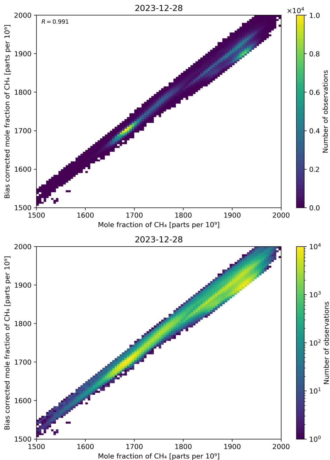
Figure 74: Scatter density plot of “Mole fraction of CH 4 ” against “Bias corrected mole fraction of CH 4 ” for 2023-12-27 to 2023-12-29.
