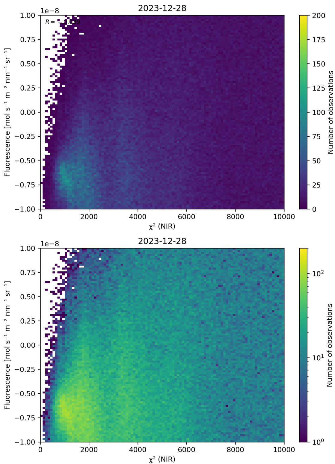
Figure 45: Scatter density plot of “ \chi^2 (NIR)” against “Fluorescence” for 2023-12-27 to 2023-12-29.
