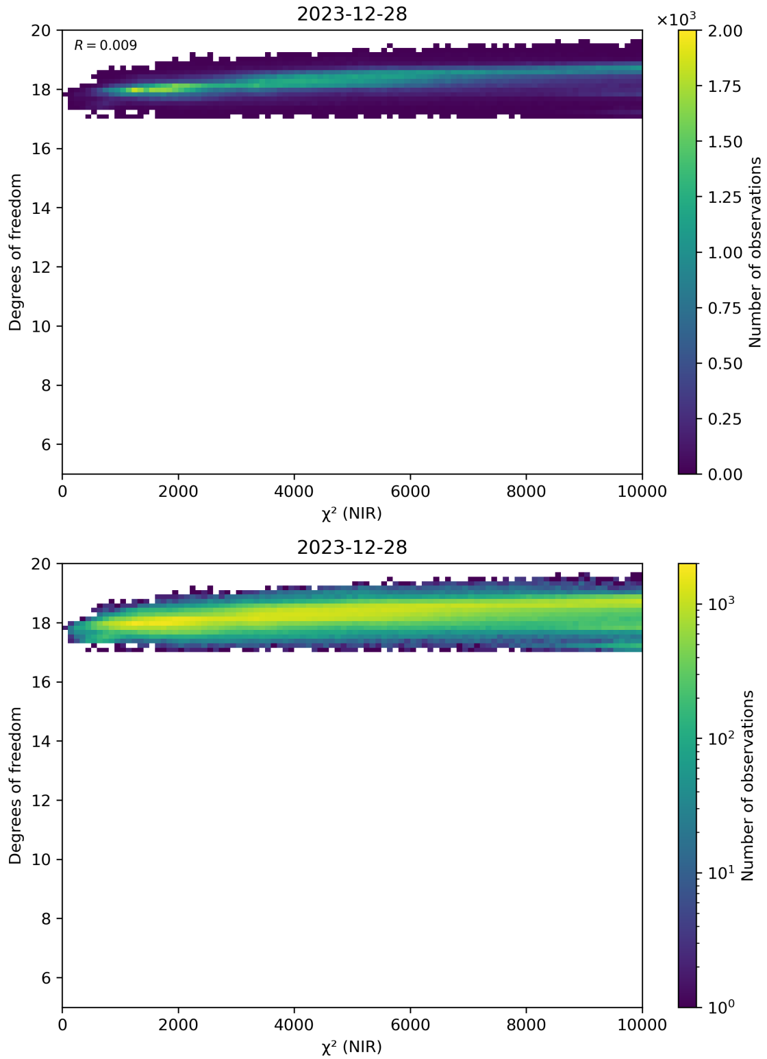
Figure 44: Scatter density plot of “ \chi^2 (NIR)” against “Degrees of freedom” for 2023-12-27 to 2023-12-29.
