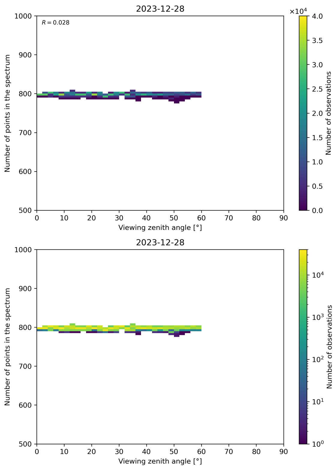
Figure 114: Scatter density plot of “Viewing zenith angle” against “Number of points in the spectrum” for 2023-12-27 to 2023-12-29.
