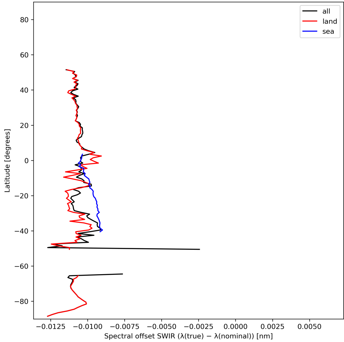
Figure 16: Zonal average of “Spectral offset SWIR ( \lambda(\text{true}) - \lambda(\text{nominal}) )” for 2023-12-27 to 2023-12-29.
