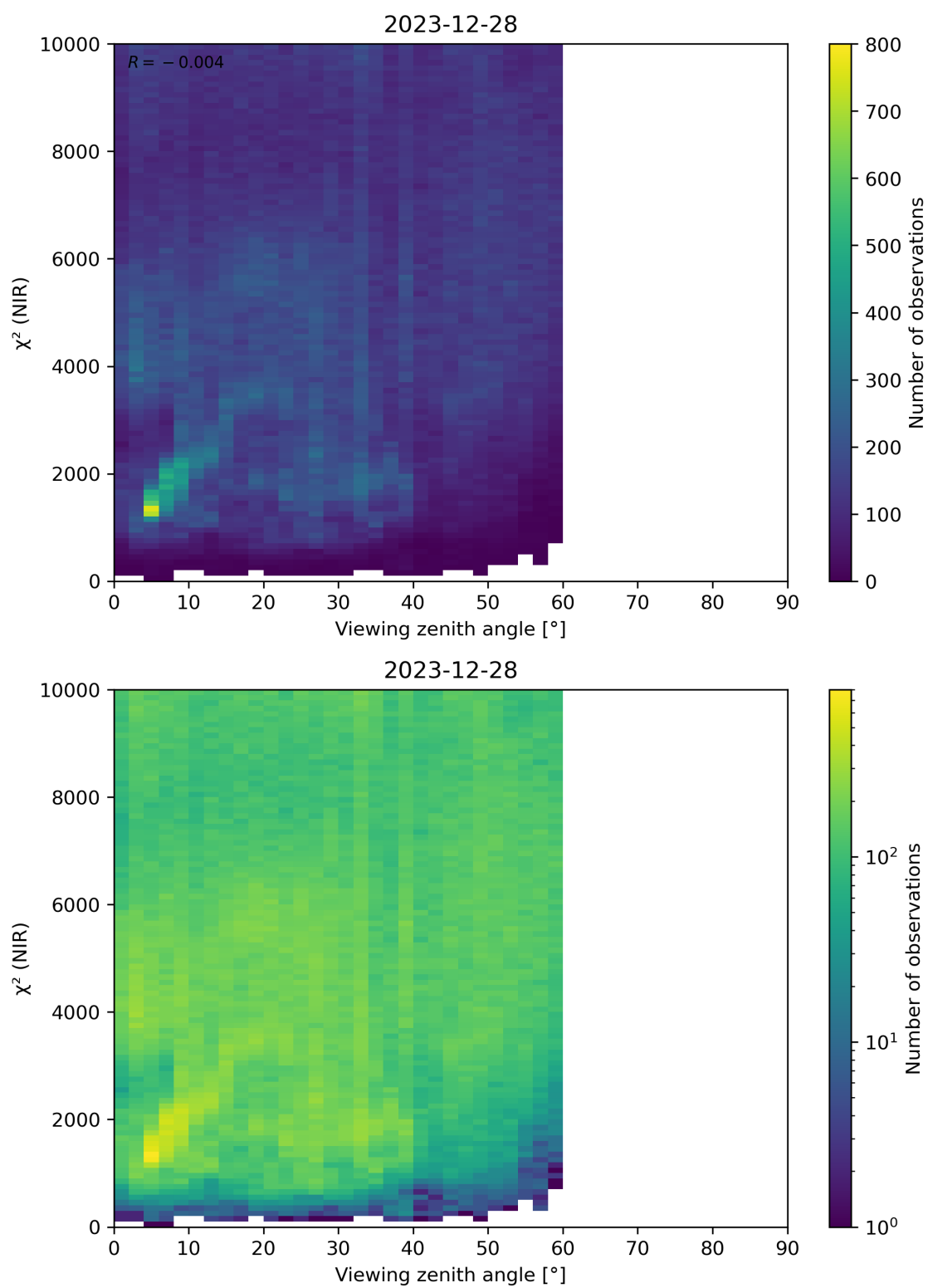
Figure 105: Scatter density plot of “Viewing zenith angle” against “ \chi^2 (NIR)” for 2023-12-27 to 2023-12-29.
