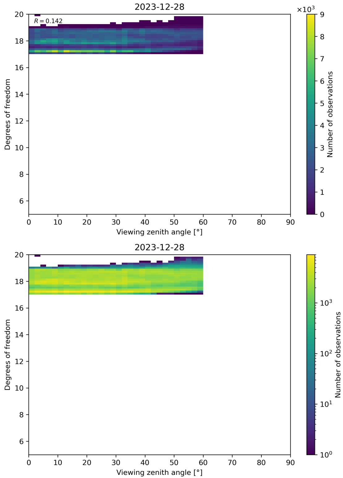
Figure 107: Scatter density plot of “Viewing zenith angle” against “Degrees of freedom” for 2023-12-27 to 2023-12-29.
