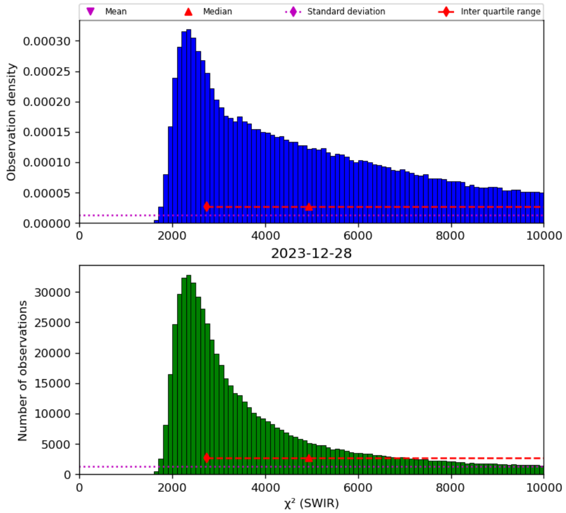
Figure 28: Histogram of “ \chi^2 (SWIR)” for 2023-12-27 to 2023-12-29
