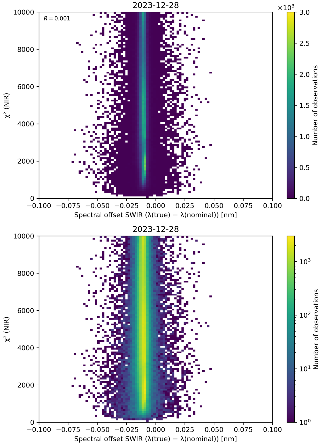
Figure 117: Scatter density plot of “Spectral offset SWIR ( \lambda(\text{true}) - \lambda(\text{nominal}) )” against “ \chi^2 (NIR)” for 2023-12-27 to 2023-12-29.
