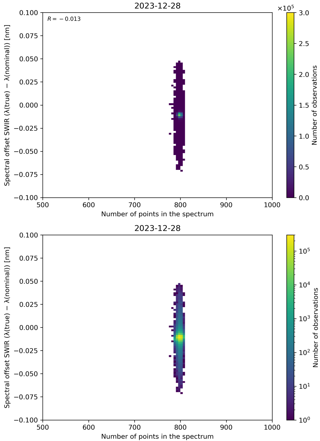
Figure 93: Scatter density plot of “Number of points in the spectrum” against “Spectral offset SWIR ( \lambda(\text{true}) - \lambda(\text{nominal}) )” for 2023-12-27 to 2023-12-29.
