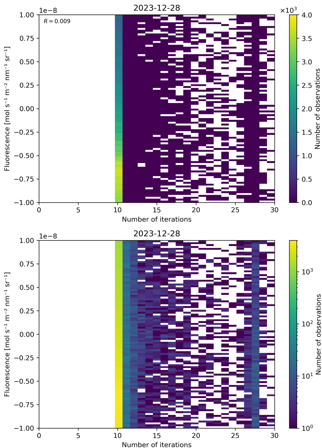
Figure 87: Scatter density plot of “Number of iterations” against “Fluorescence” for 2023-12-27 to 2023-12-29.
