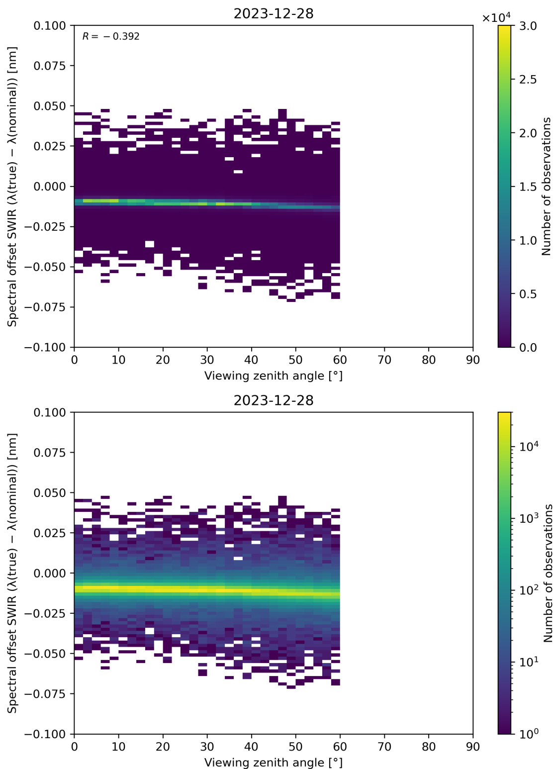
Figure 116: Scatter density plot of “Viewing zenith angle” against “Spectral offset SWIR ( \lambda(\text{true}) - \lambda(\text{nominal}) )” for 2023-12-27 to 2023-12-29.
