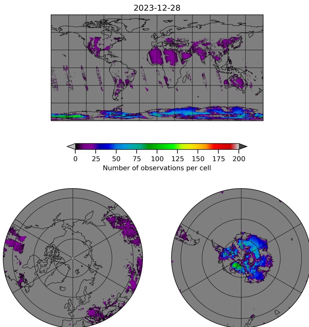
Figure 10: Map of the number of observations for 2023-12-27 to 2023-12-29
