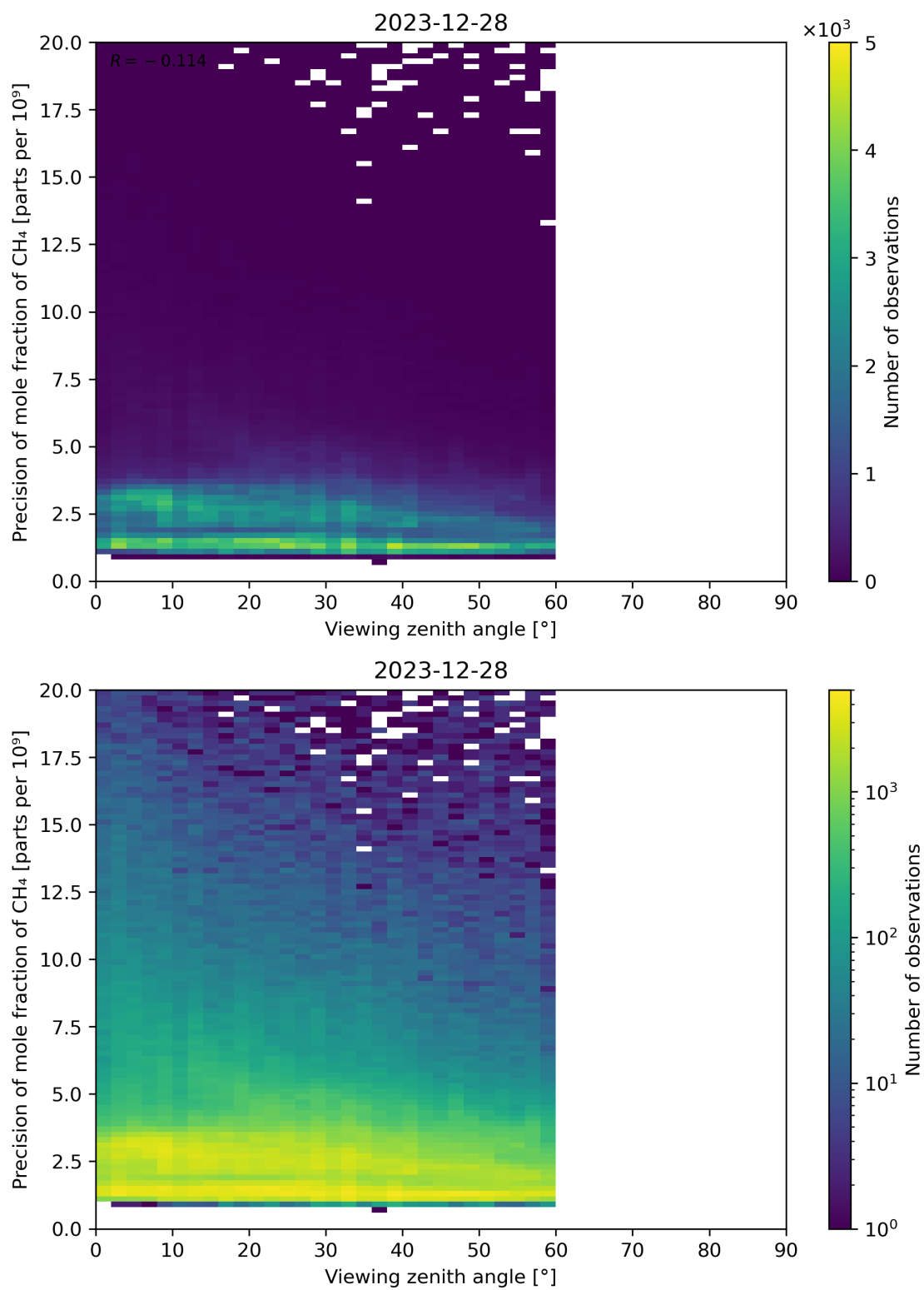
Figure 112: Scatter density plot of “Viewing zenith angle” against “Precision of mole fraction of \text{CH}_4 ” for 2023-12-27 to 2023-12-29.
