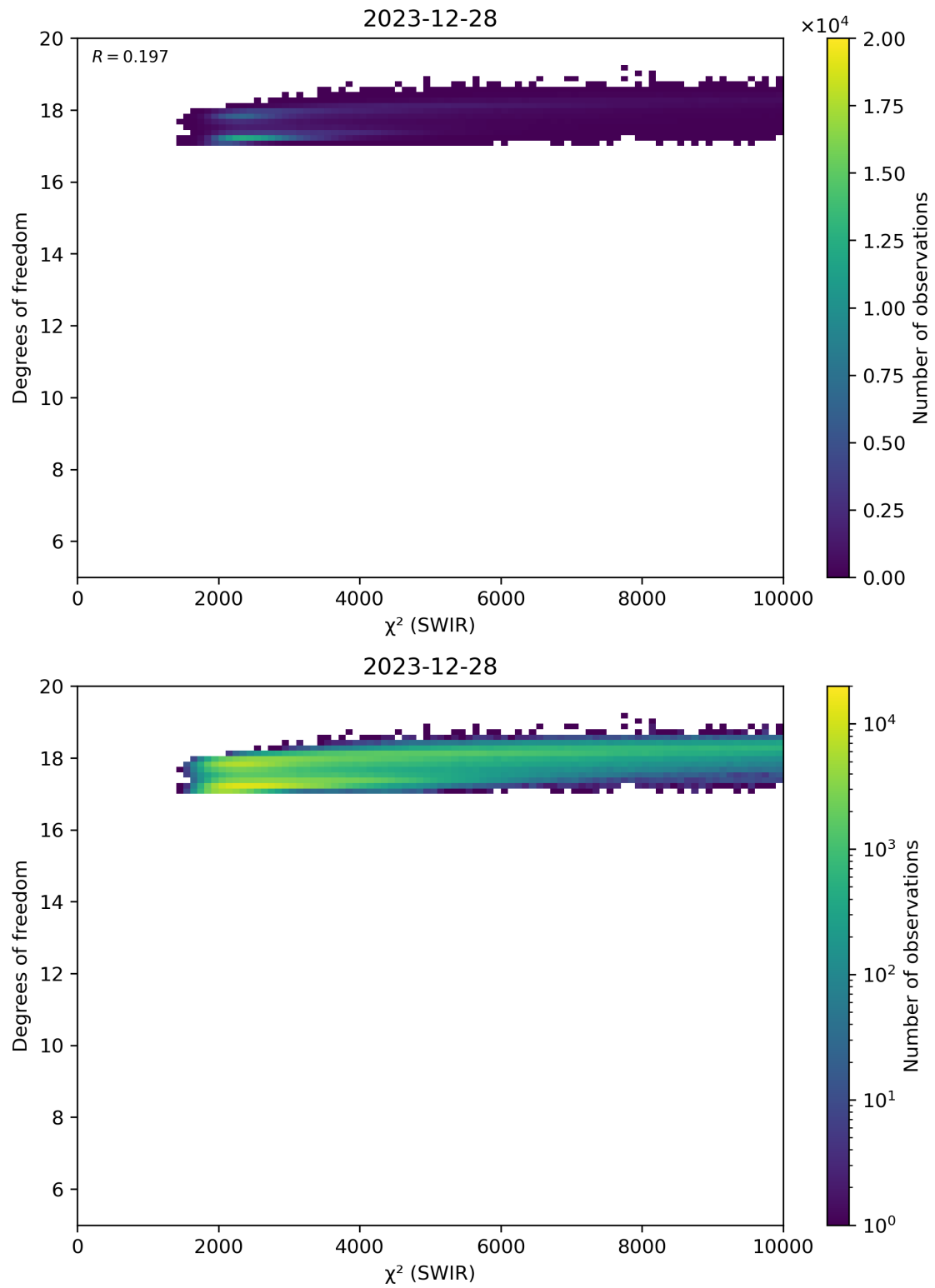
Figure 48: Scatter density plot of “ \chi^2 (SWIR)” against “Degrees of freedom” for 2023-12-27 to 2023-12-29.
