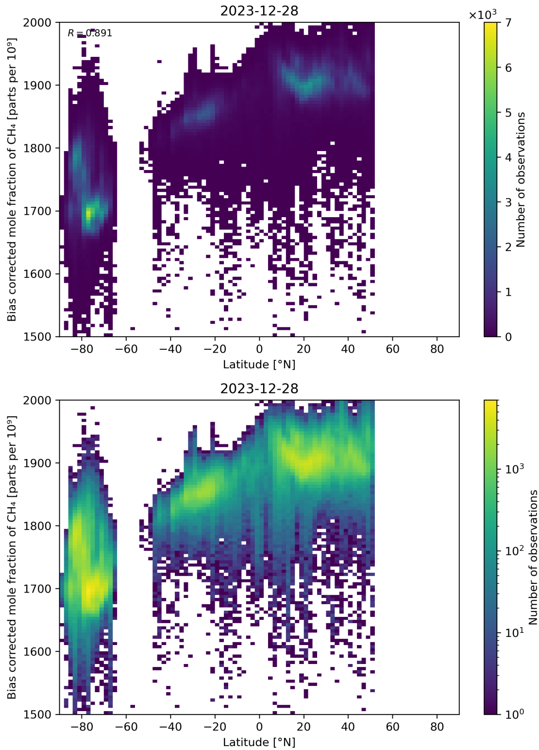
Figure 58: Scatter density plot of “Latitude” against “Bias corrected mole fraction of CH 4 ” for 2023-12-27 to 2023-12-29.
