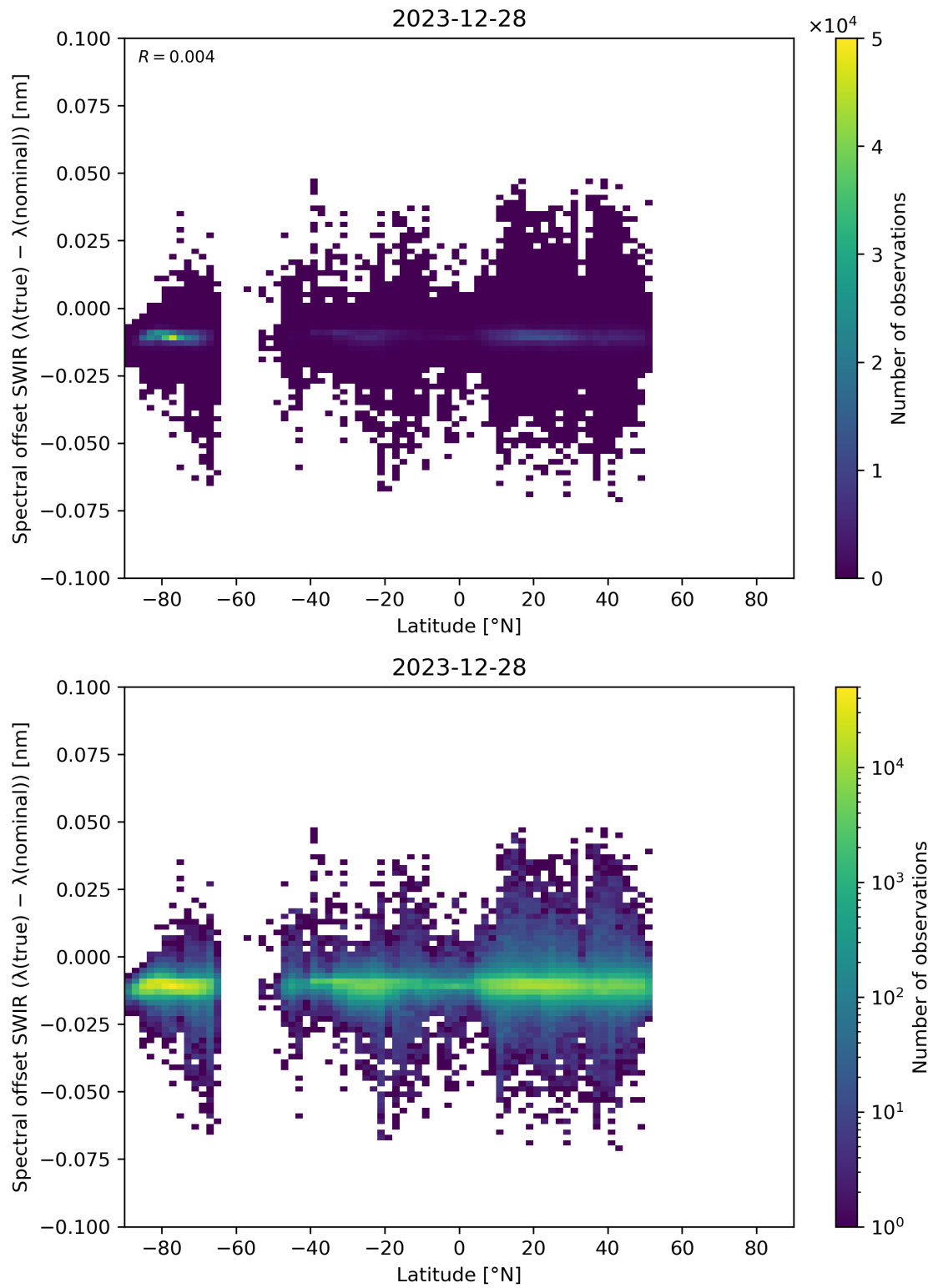
Figure 62: Scatter density plot of “Latitude” against “Spectral offset SWIR ( \lambda(\text{true}) - \lambda(\text{nominal}) )” for 2023-12-27 to 2023-12-29.
