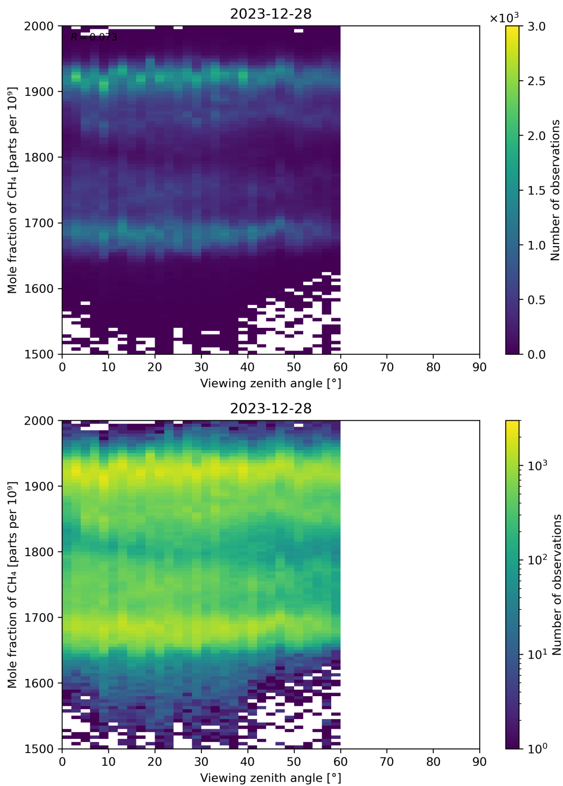
Figure 110: Scatter density plot of “Viewing zenith angle” against “Mole fraction of CH 4 ” for 2023-12-27 to 2023-12-29.
