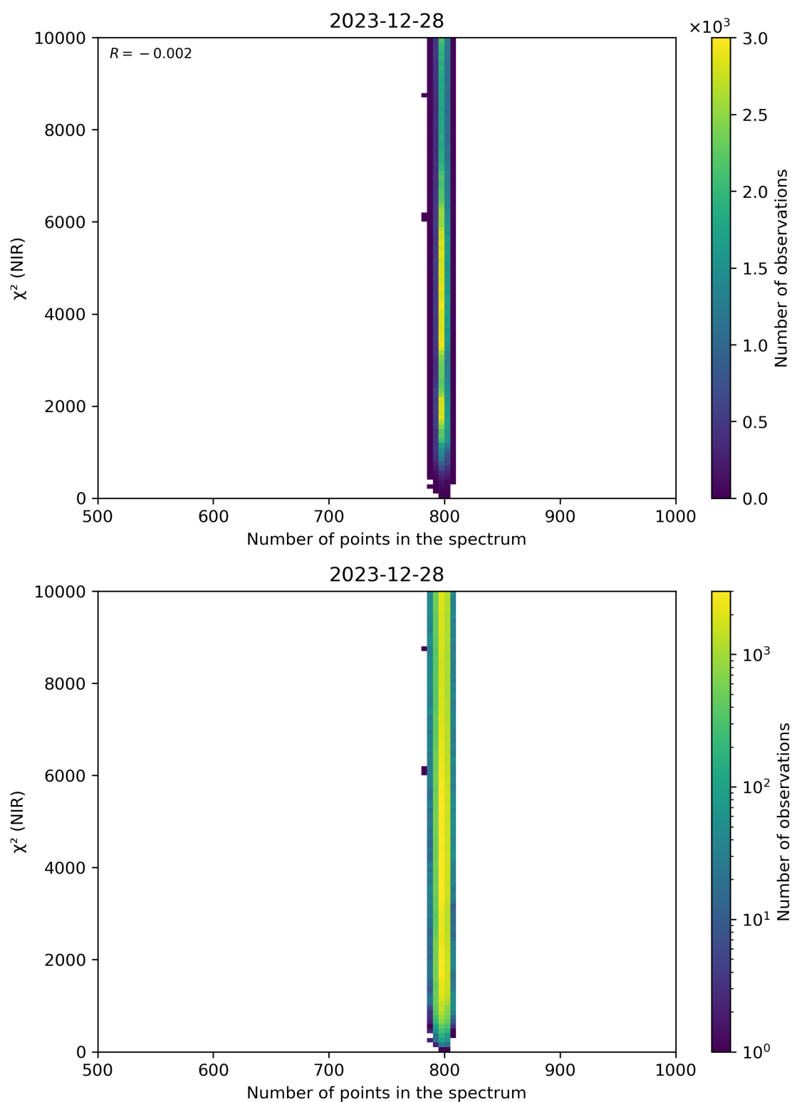
Figure 88: Scatter density plot of “Number of points in the spectrum” against “ \chi^2 (NIR)” for 2023-12-27 to 2023-12-29.
