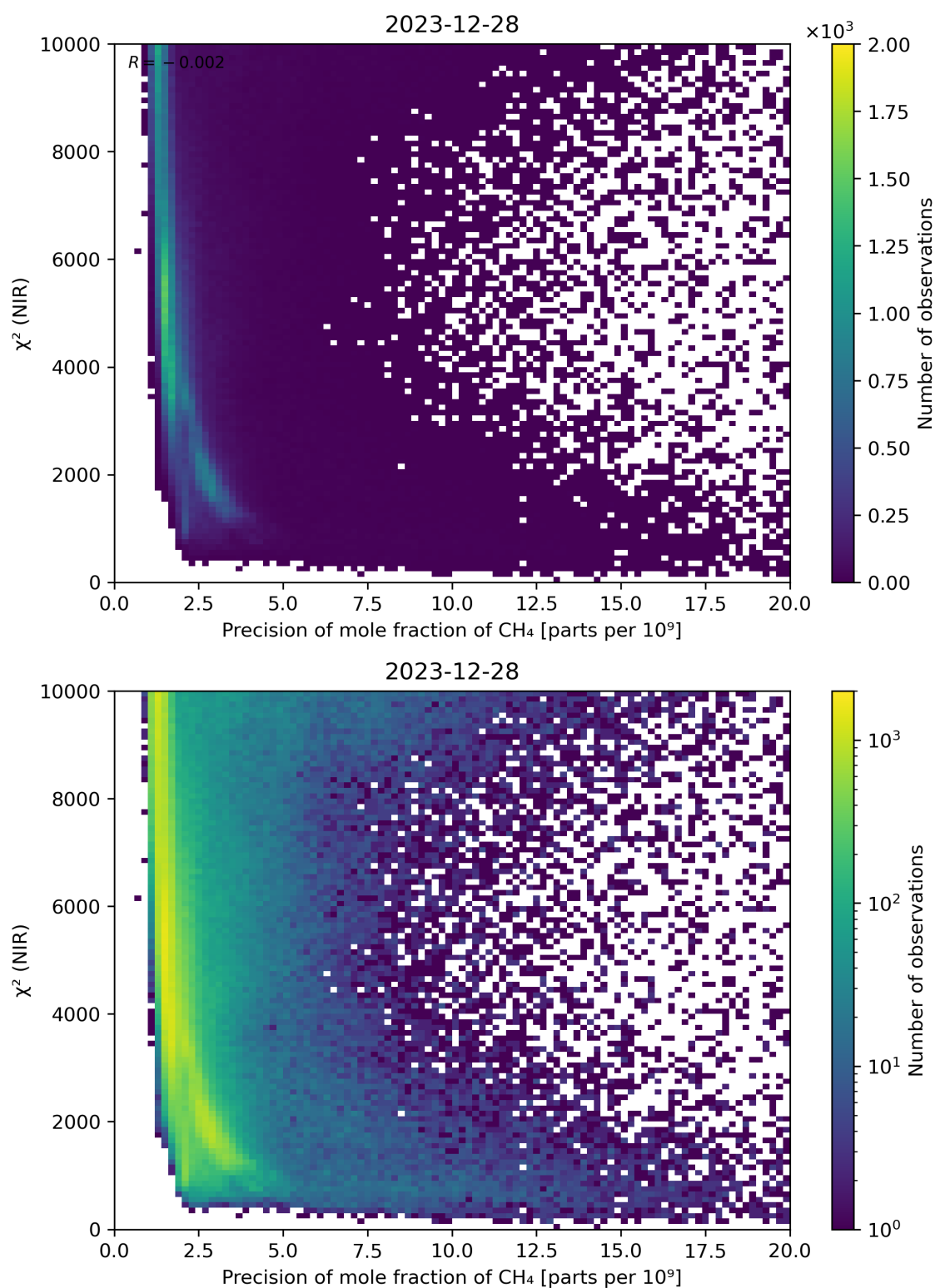
Figure 78: Scatter density plot of “Precision of mole fraction of CH 4 ” against “ \chi^2 (NIR)” for 2023-12-27 to 2023-12-29.
