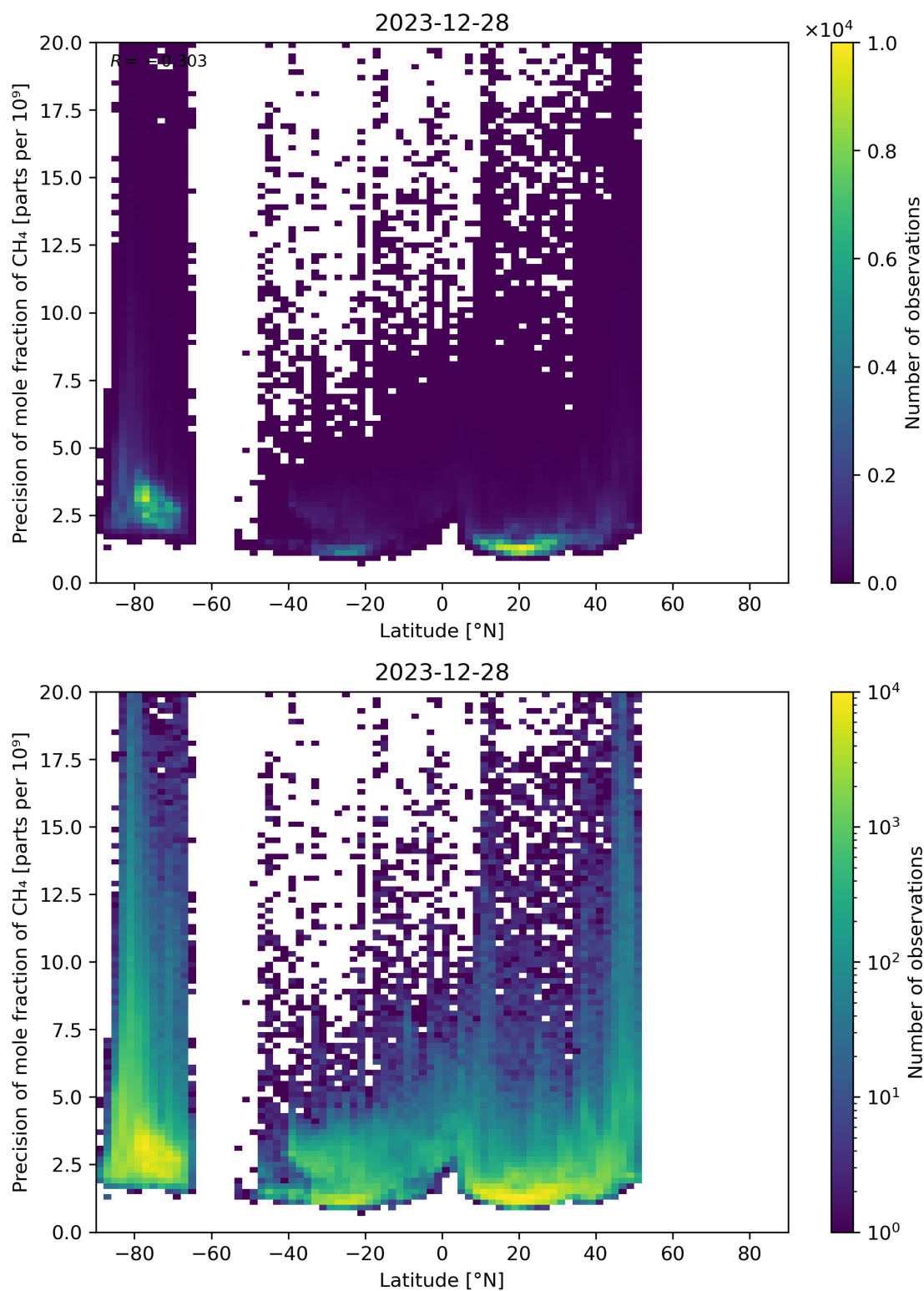
Figure 59: Scatter density plot of “Latitude” against “Precision of mole fraction of CH 4 ” for 2023-12-27 to 2023-12-29.
