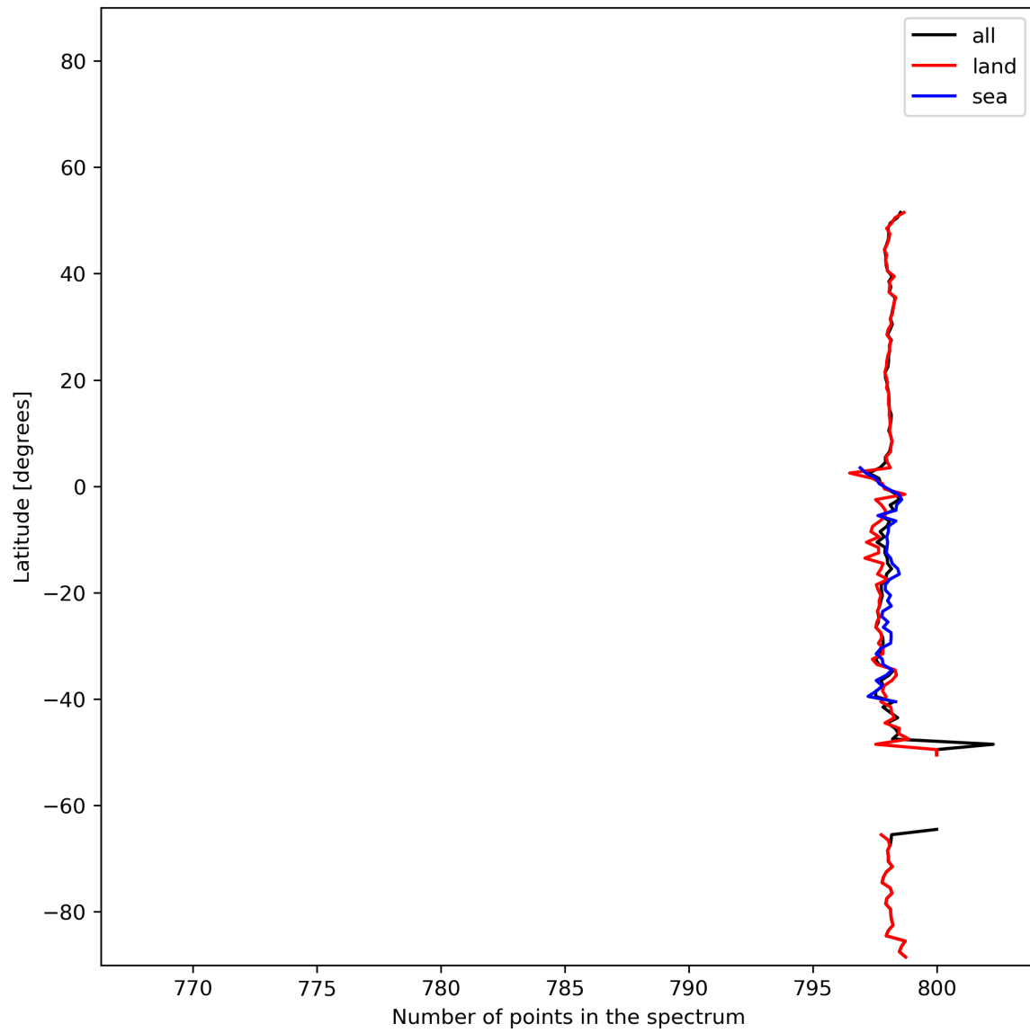
Figure 15: Zonal average of “Number of points in the spectrum” for 2023-12-27 to 2023-12-29.
