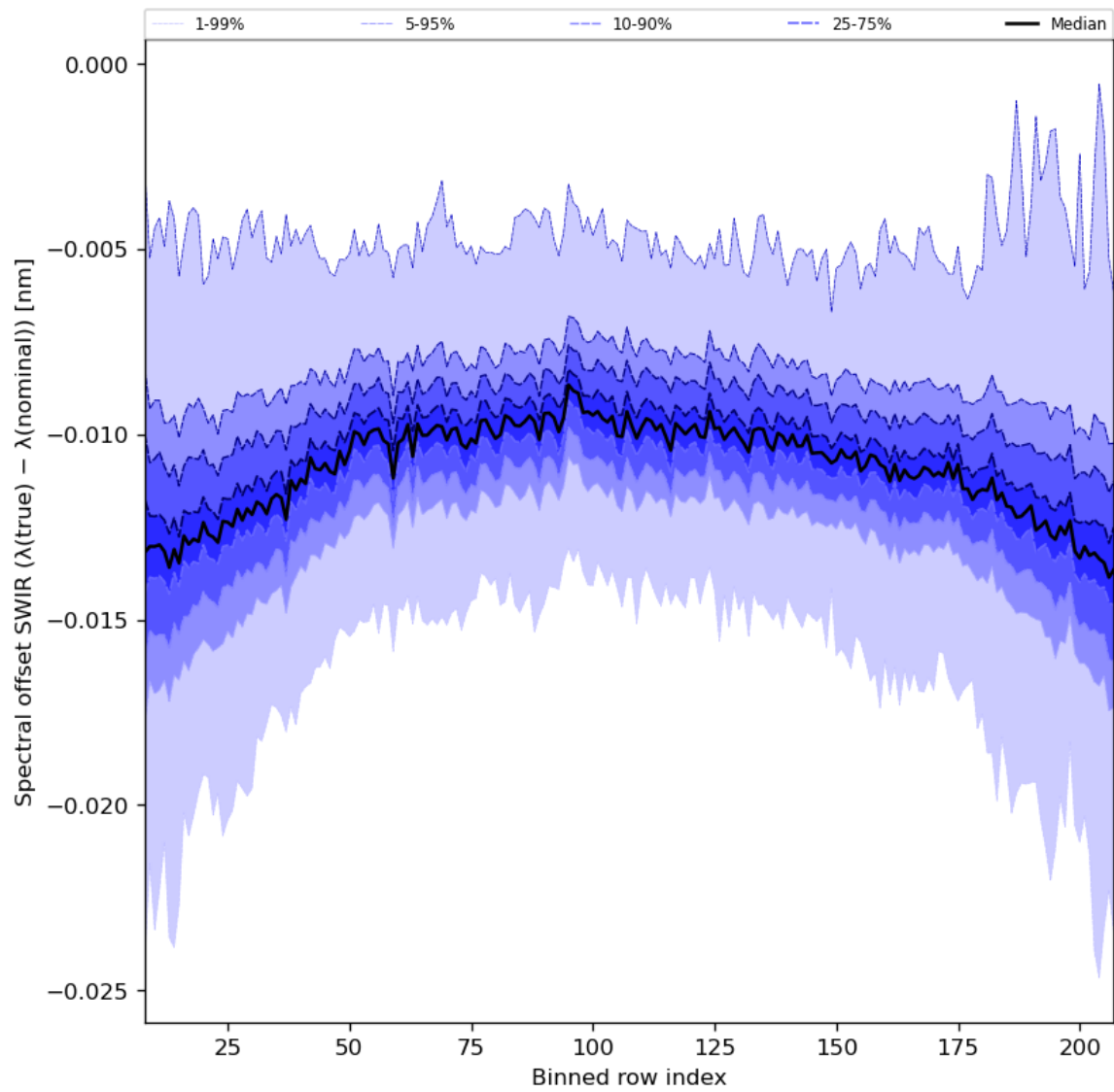
Figure 38: Along track statistics of “Spectral offset SWIR ( \lambda(\text{true}) - \lambda(\text{nominal}) )” for 2023-12-27 to 2023-12-29
