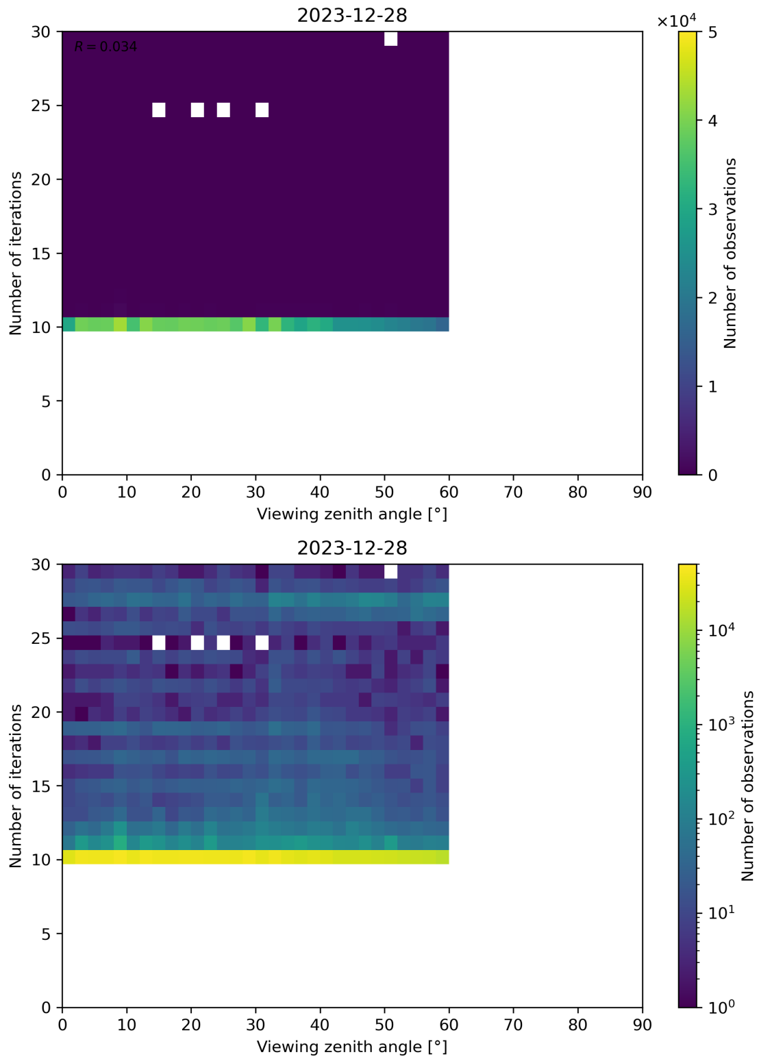
Figure 113: Scatter density plot of “Viewing zenith angle” against “Number of iterations” for 2023-12-27 to 2023-12-29.
