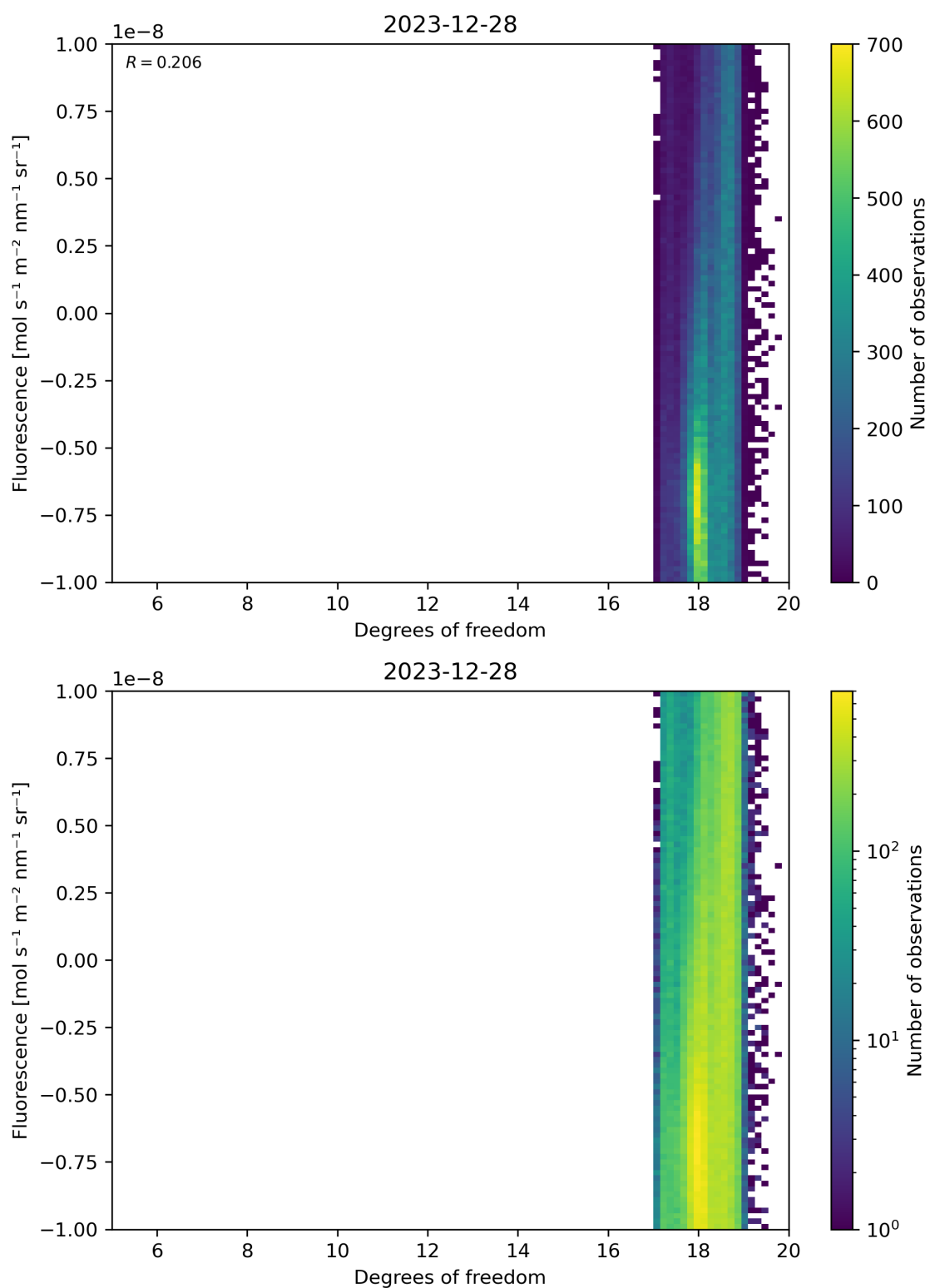
Figure 51: Scatter density plot of “Degrees of freedom” against “Fluorescence” for 2023-12-27 to 2023-12-29.
