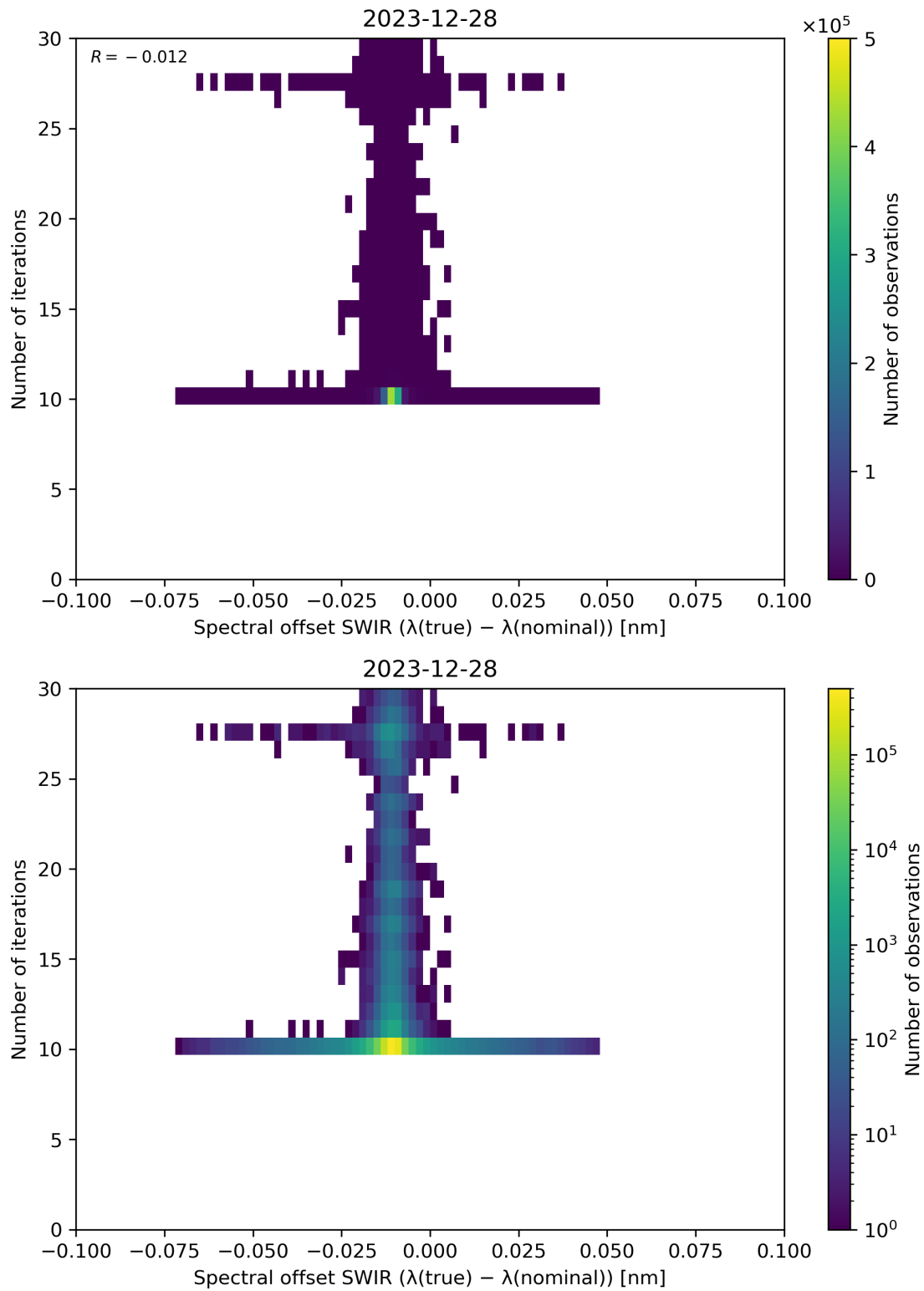
Figure 121: Scatter density plot of “Spectral offset SWIR ( \lambda(\text{true}) - \lambda(\text{nominal}) )” against “Number of iterations” for 2023-12-27 to 2023-12-29.
