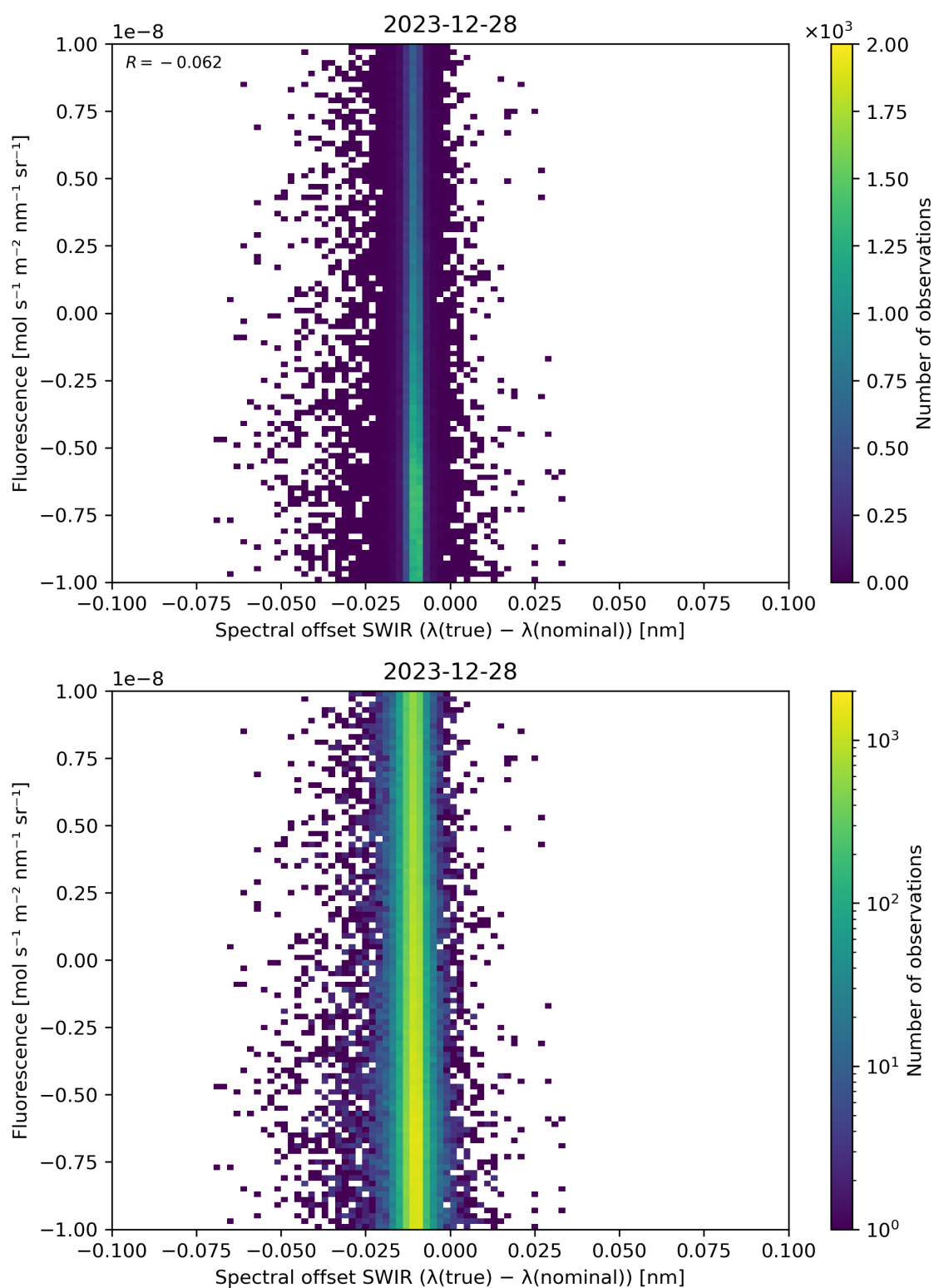
Figure 120: Scatter density plot of “Spectral offset SWIR ( \lambda(\text{true}) - \lambda(\text{nominal}) )” against “Fluorescence” for 2023-12-27 to 2023-12-29.
