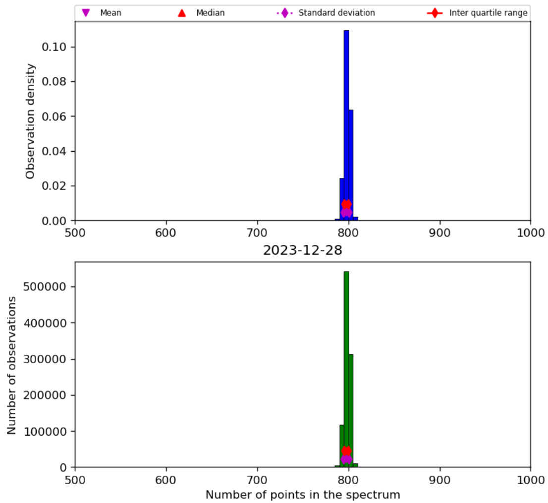
Figure 26: Histogram of “Number of points in the spectrum” for 2023-12-27 to 2023-12-29
