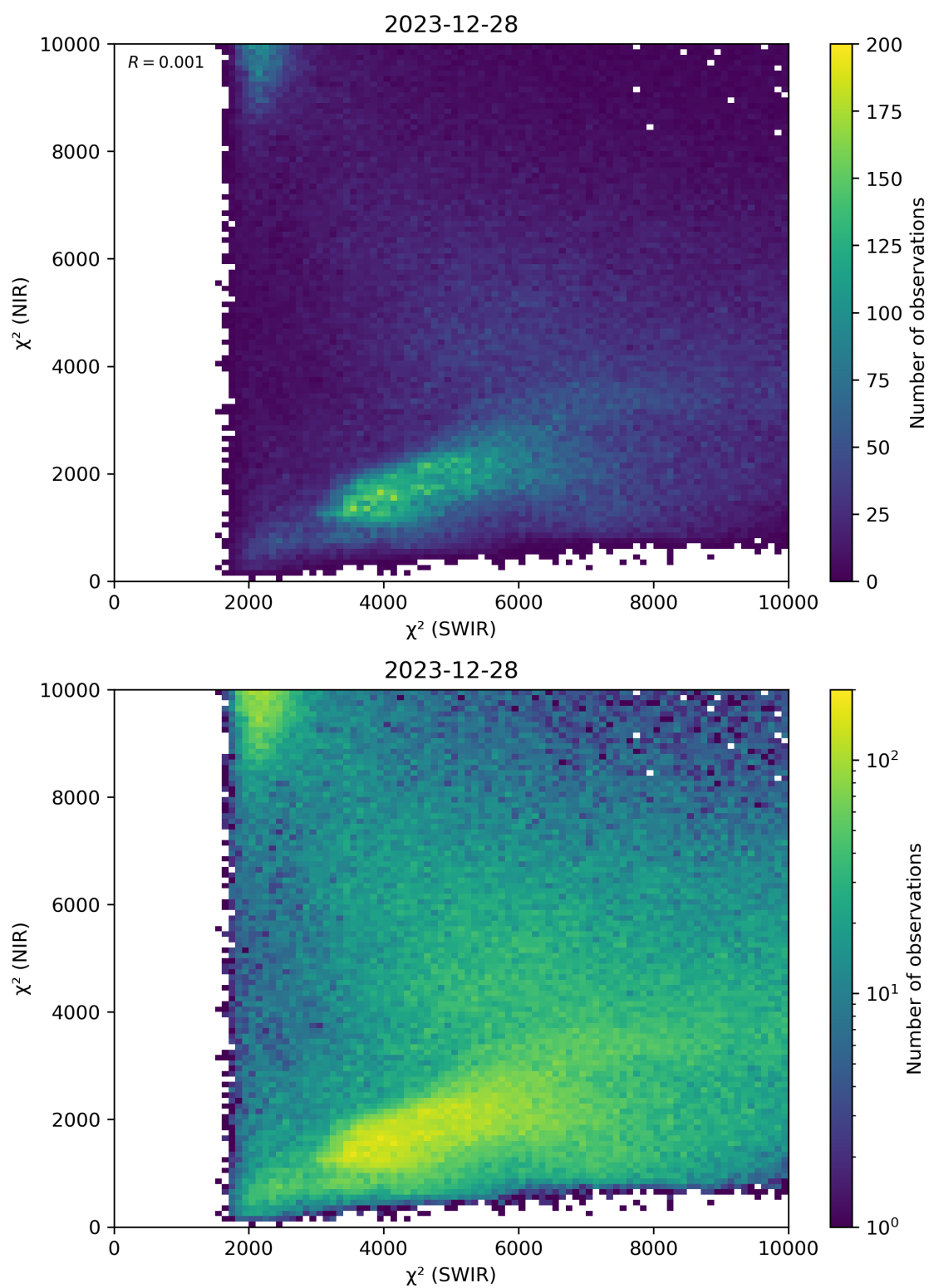
Figure 47: Scatter density plot of “ \chi^2 (SWIR)” against “ \chi^2 (NIR)” for 2023-12-27 to 2023-12-29.
