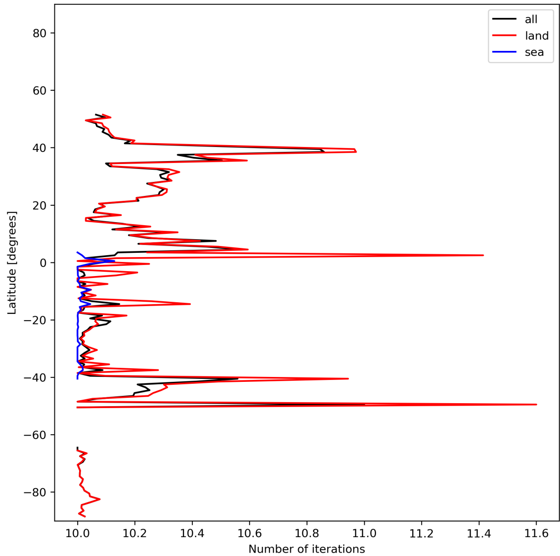
Figure 20: Zonal average of “Number of iterations” for 2023-12-27 to 2023-12-29.
