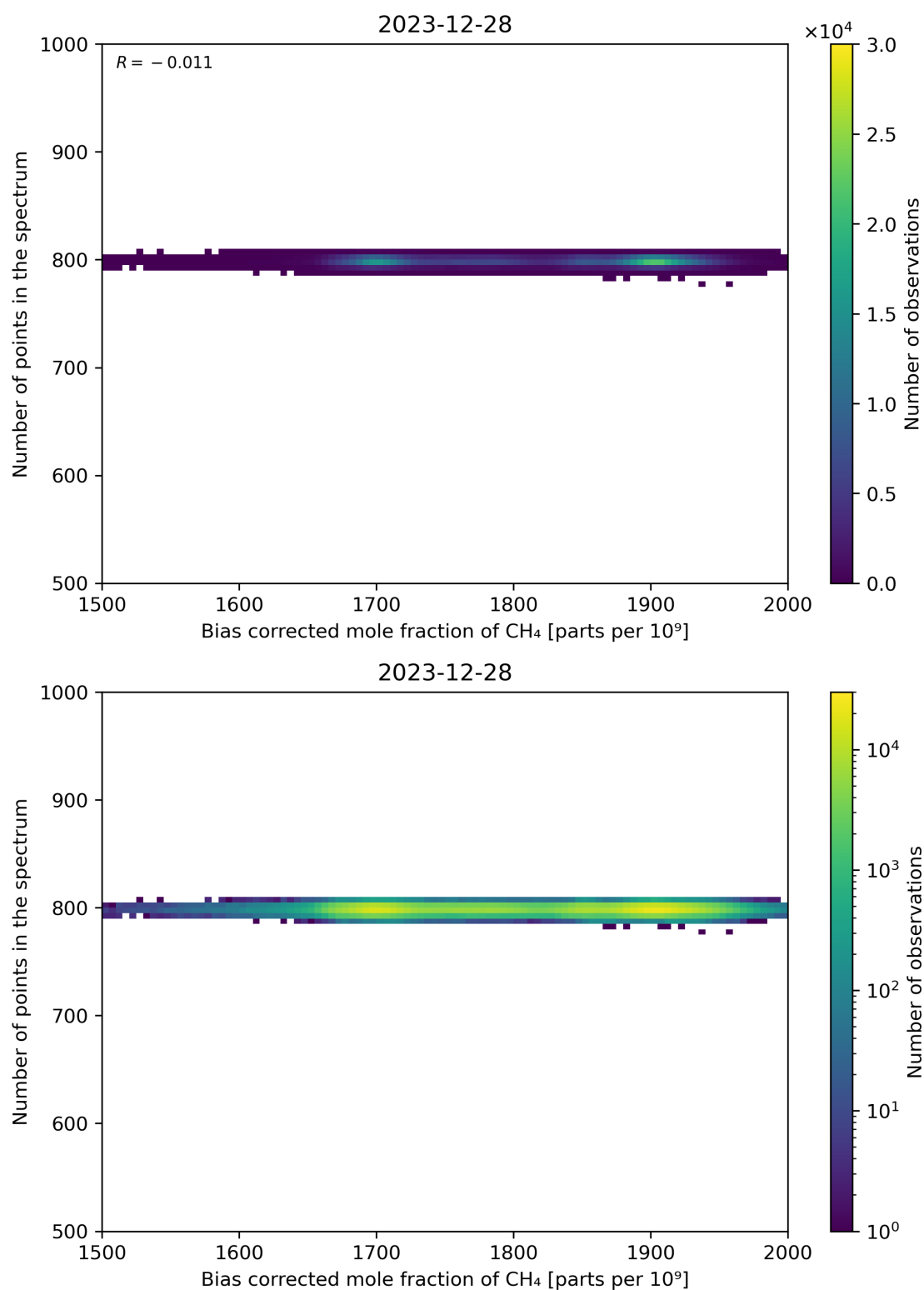
Figure 68: Scatter density plot of “Bias corrected mole fraction of CH 4 ” against “Number of points in the spectrum” for 2023-12-27 to 2023-12-29.
