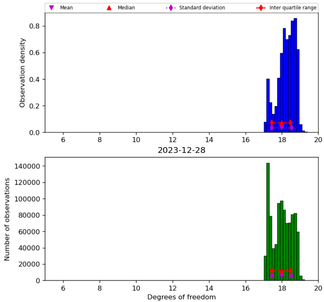
Figure 30: Histogram of “Degrees of freedom” for 2023-12-27 to 2023-12-29
