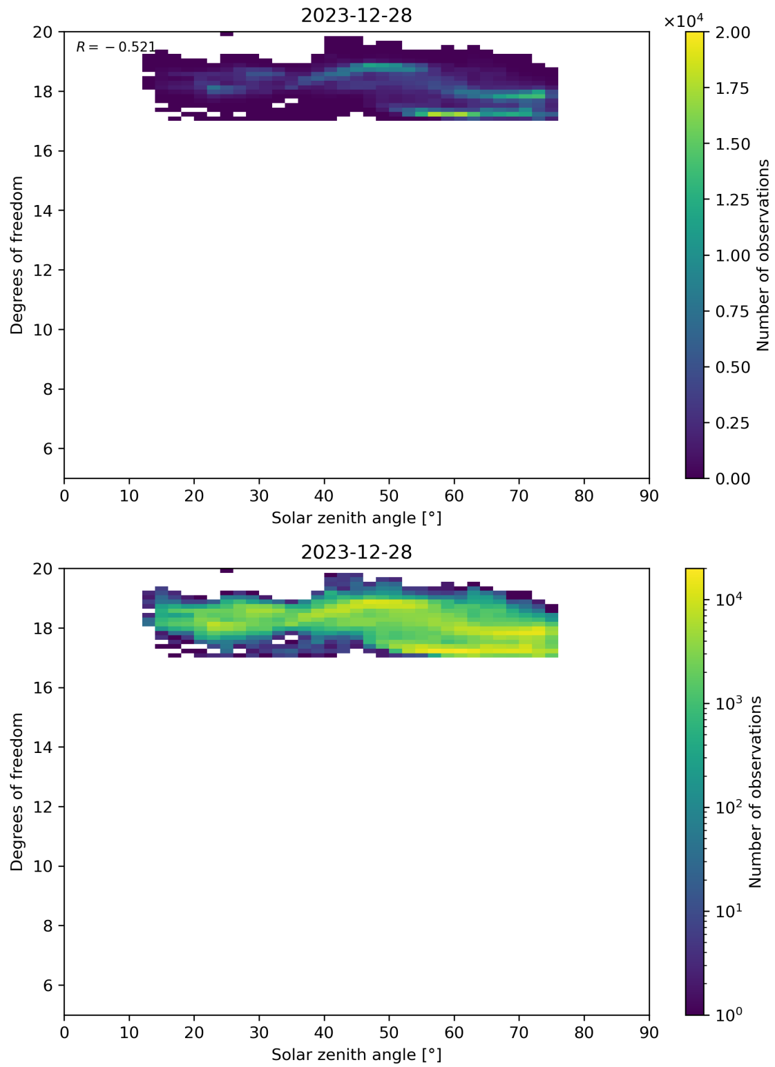
Figure 96: Scatter density plot of “Solar zenith angle” against “Degrees of freedom” for 2023-12-27 to 2023-12-29.
