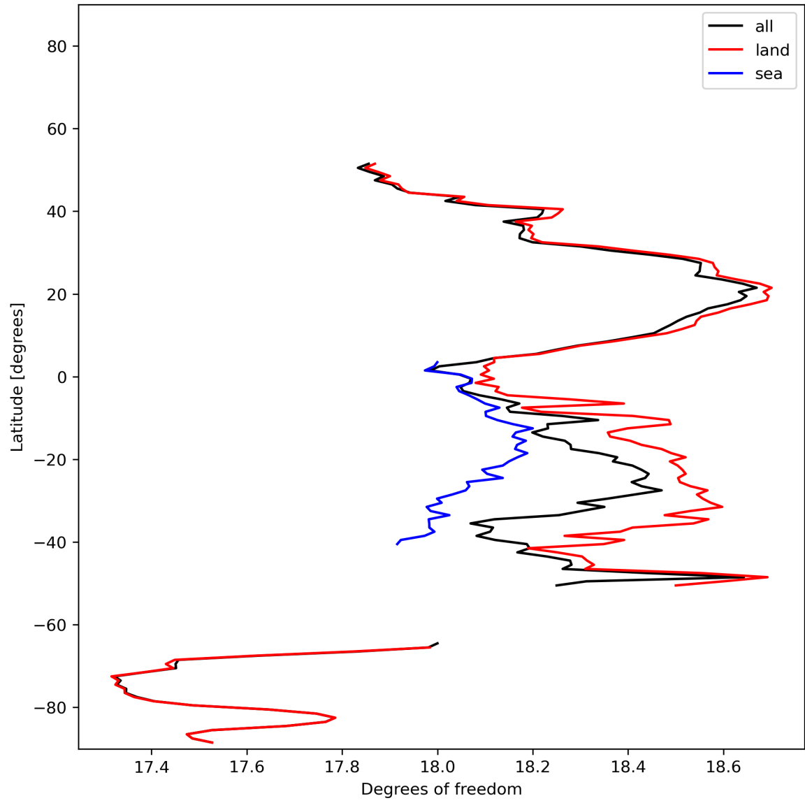
Figure 19: Zonal average of “Degrees of freedom” for 2023-12-27 to 2023-12-29.
