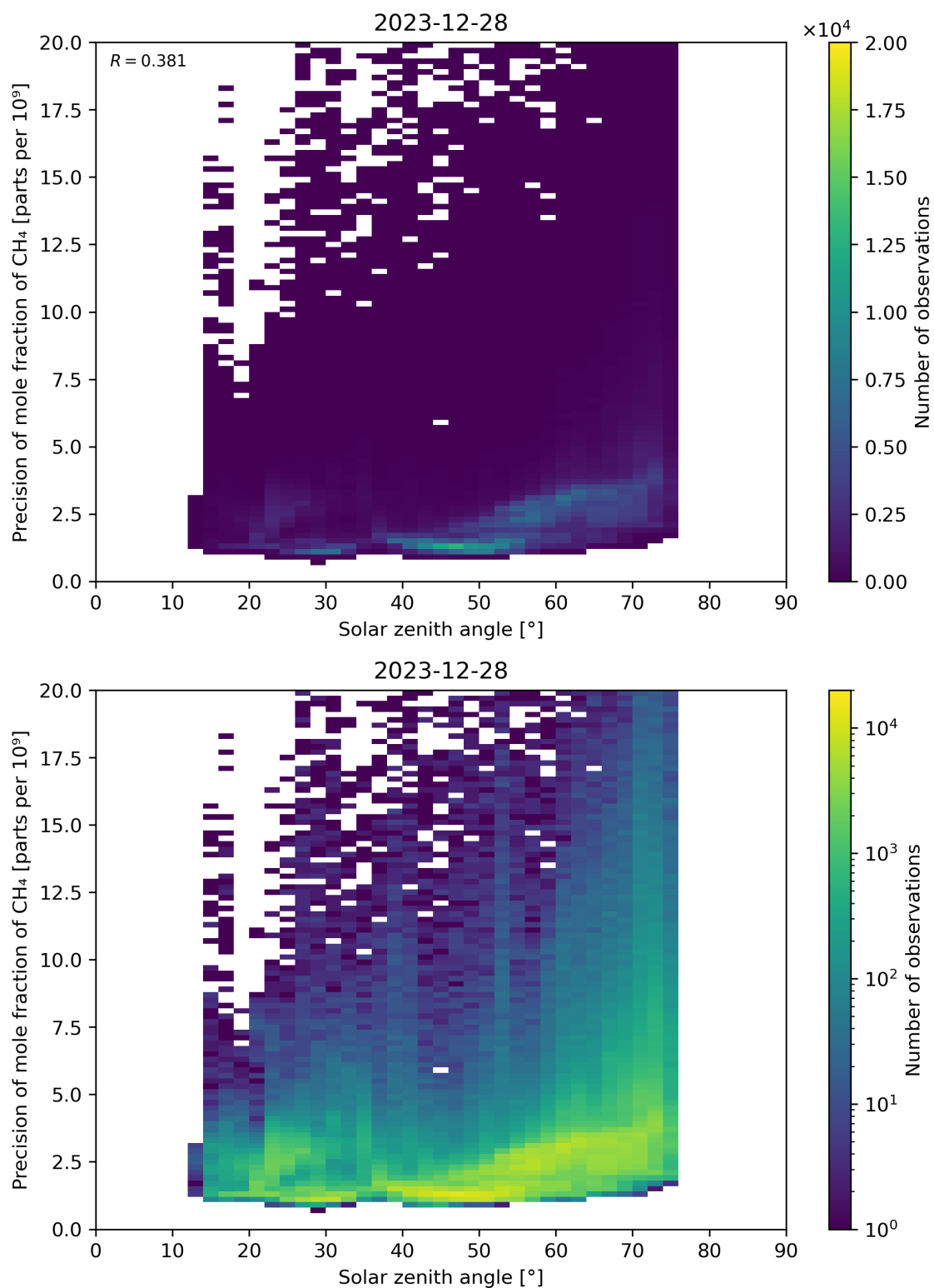
Figure 101: Scatter density plot of “Solar zenith angle” against “Precision of mole fraction of CH 4 ” for 2023-12-27 to 2023-12-29.
