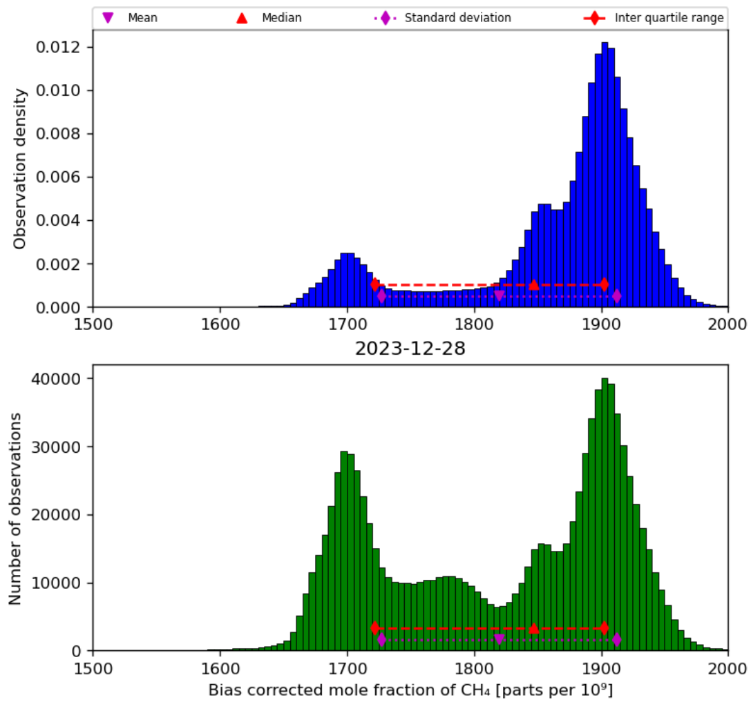
Figure 25: Histogram of “Bias corrected mole fraction of CH 4 ” for 2023-12-27 to 2023-12-29
