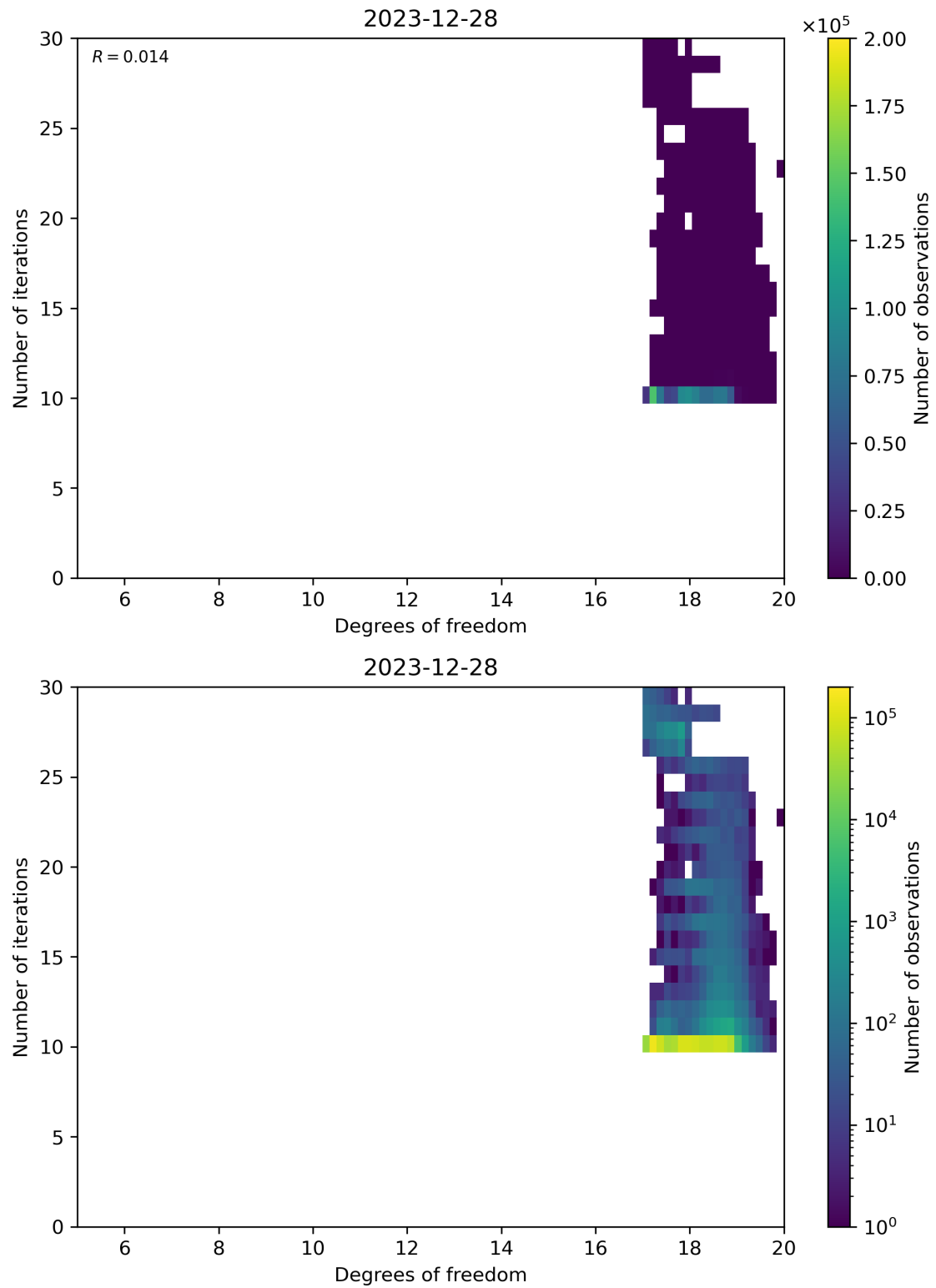
Figure 52: Scatter density plot of “Degrees of freedom” against “Number of iterations” for 2023-12-27 to 2023-12-29.
