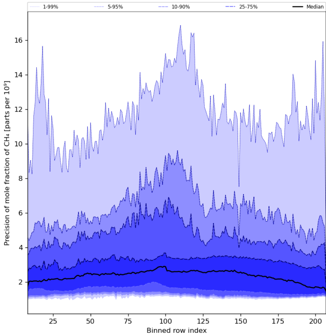
Figure 35: Along track statistics of “Precision of mole fraction of CH 4 ” for 2023-12-27 to 2023-12-29
