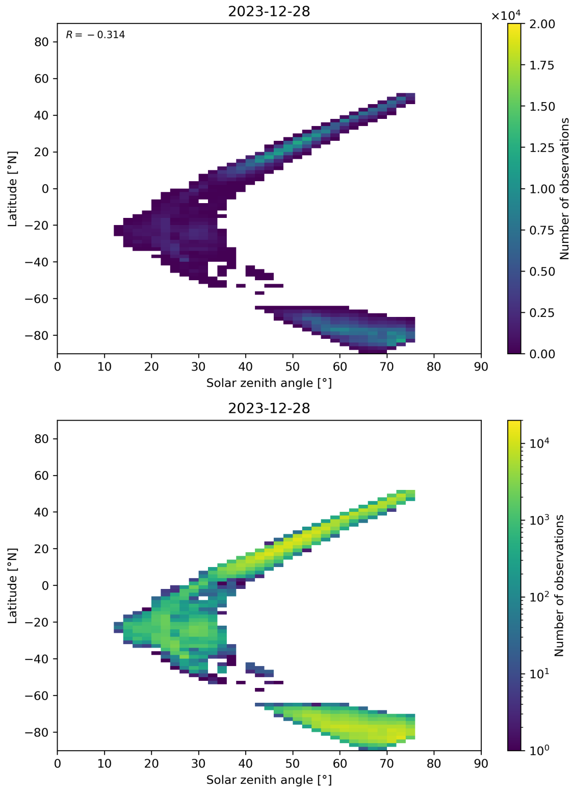
Figure 98: Scatter density plot of “Solar zenith angle” against “Latitude” for 2023-12-27 to 2023-12-29.
