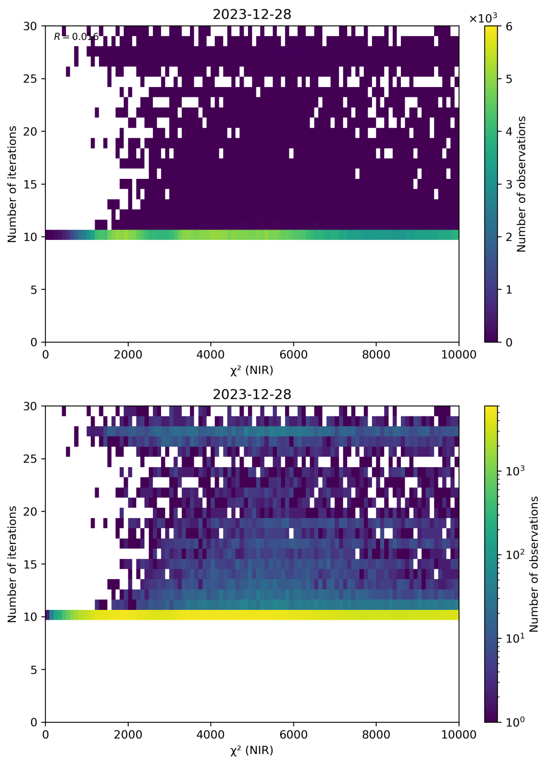
Figure 46: Scatter density plot of “ \chi^2 (NIR)” against “Number of iterations” for 2023-12-27 to 2023-12-29.
