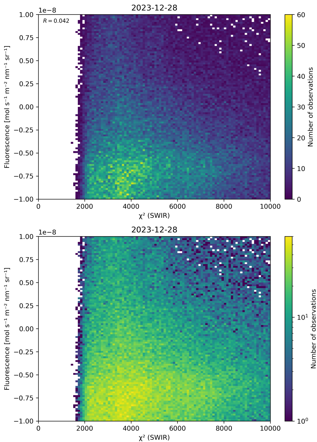
Figure 49: Scatter density plot of “ \chi^2 (SWIR)” against “Fluorescence” for 2023-12-27 to 2023-12-29.
