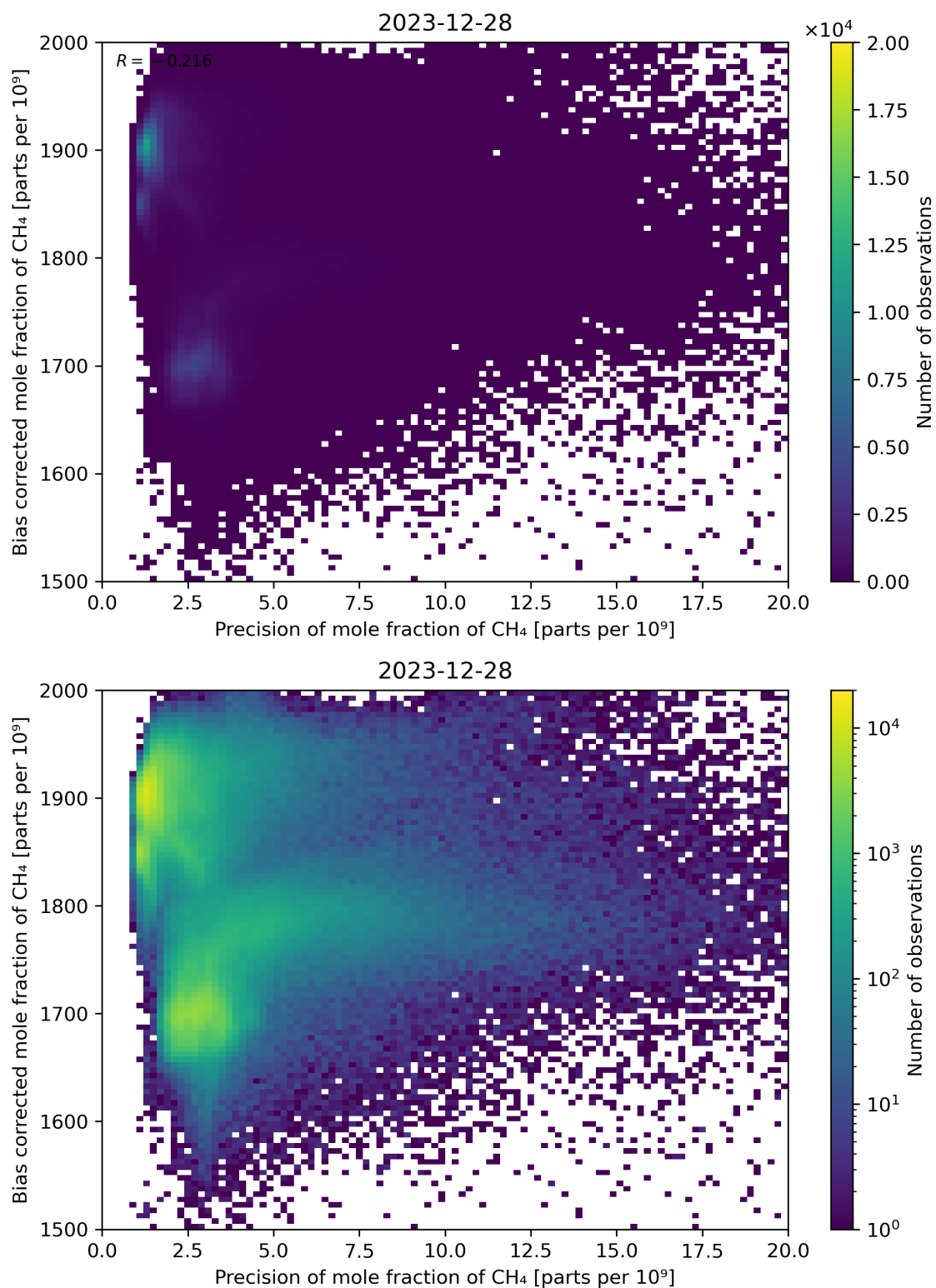
Figure 82: Scatter density plot of “Precision of mole fraction of CH 4 ” against “Bias corrected mole fraction of CH 4 ” for 2023-12-27 to 2023-12-29.
