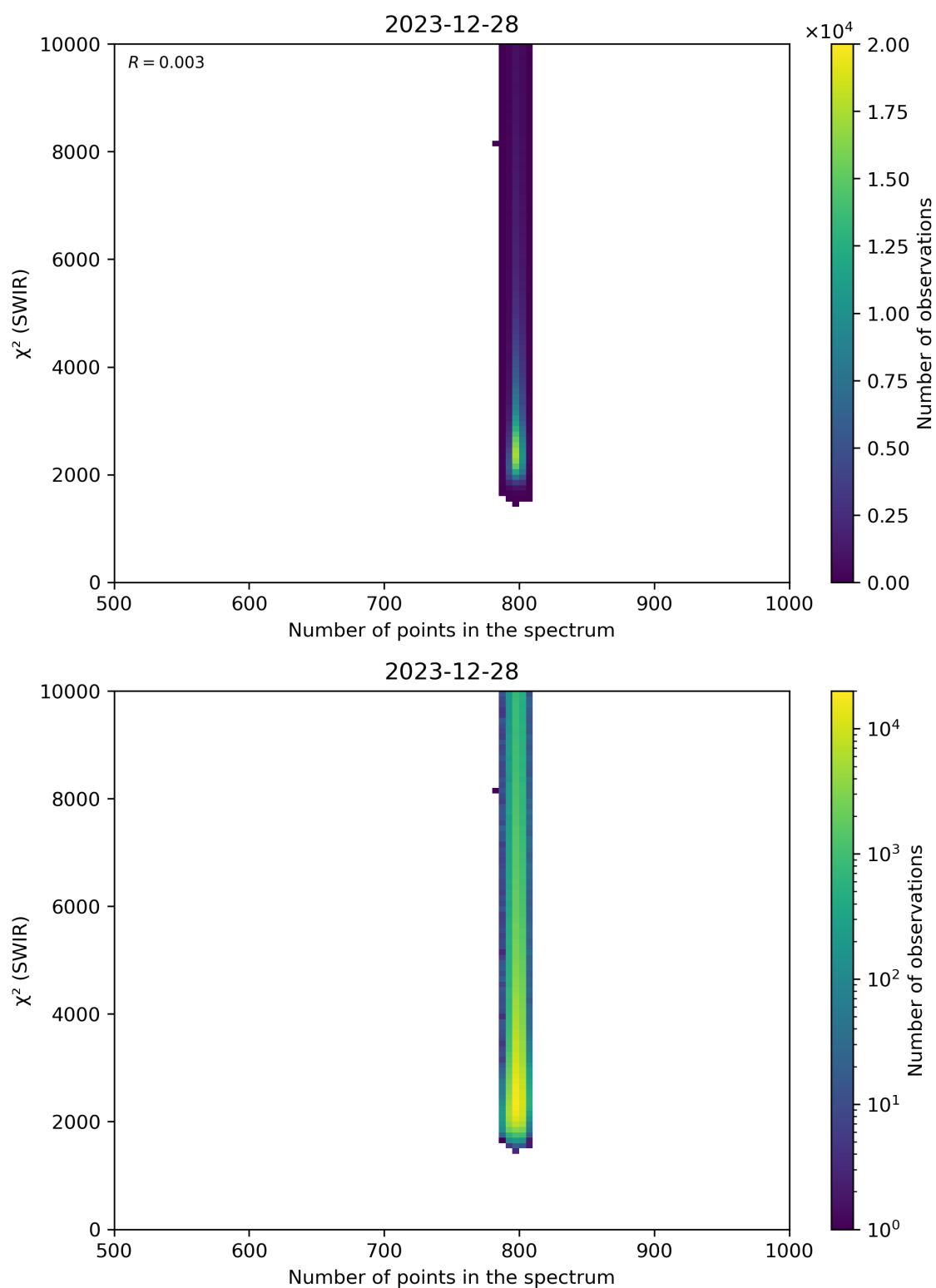
Figure 89: Scatter density plot of “Number of points in the spectrum” against “ \chi^2 (SWIR)” for 2023-12-27 to 2023-12-29.
