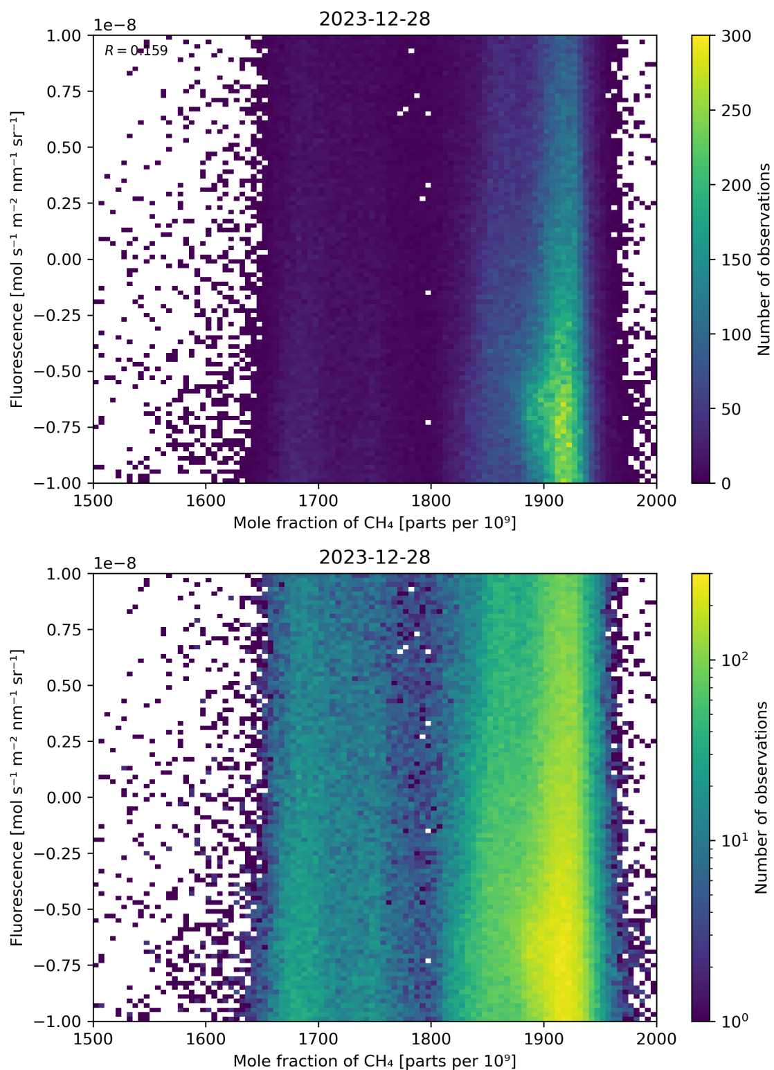
Figure 73: Scatter density plot of “Mole fraction of \text{CH}_4 ” against “Fluorescence” for 2023-12-27 to 2023-12-29.
