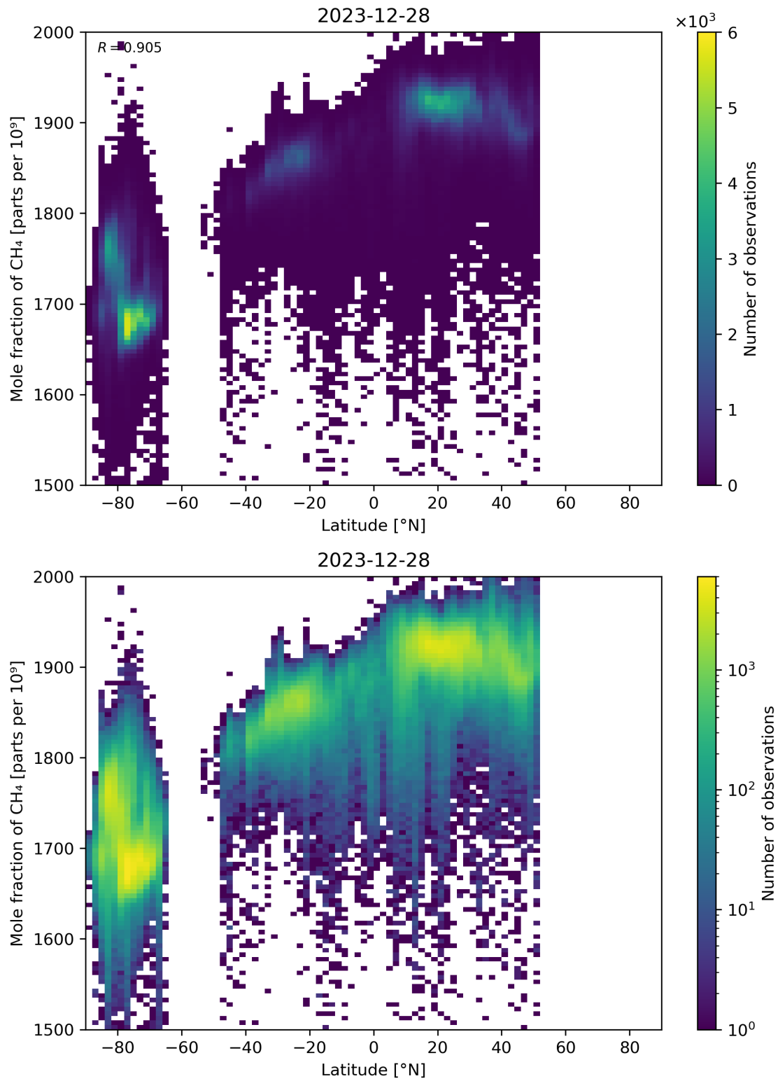
Figure 57: Scatter density plot of “Latitude” against “Mole fraction of CH 4 ” for 2023-12-27 to 2023-12-29.
