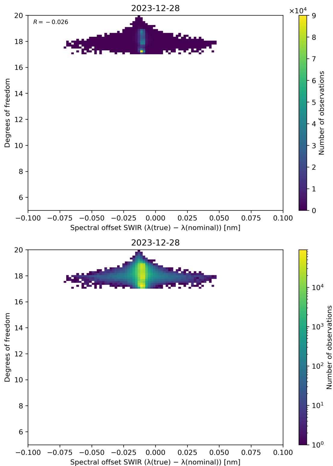
Figure 119: Scatter density plot of “Spectral offset SWIR ( \lambda(\text{true}) - \lambda(\text{nominal}) )” against “Degrees of freedom” for 2023-12-27 to 2023-12-29.
