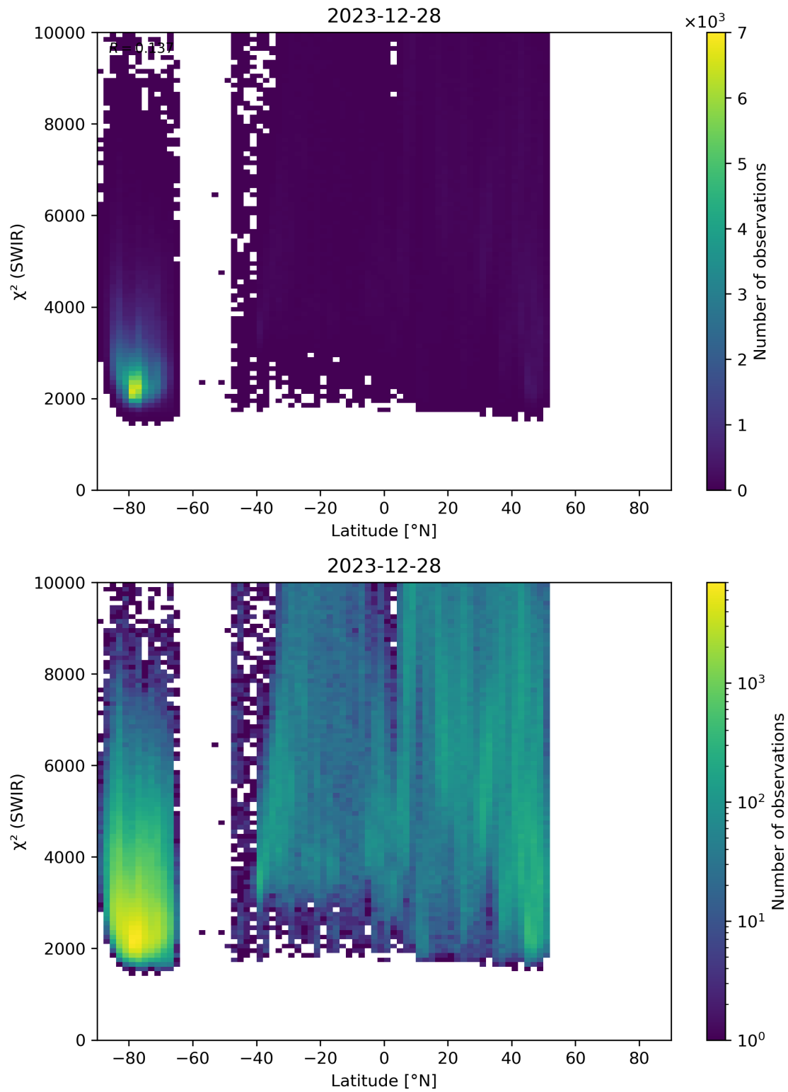
Figure 54: Scatter density plot of “Latitude” against “ \chi^2 (SWIR)” for 2023-12-27 to 2023-12-29.
