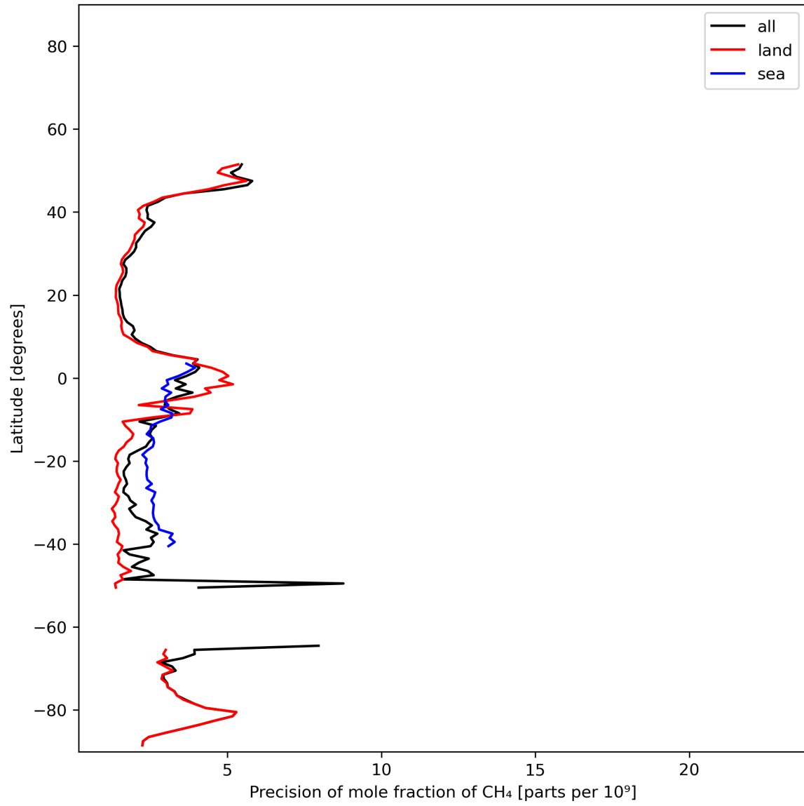
Figure 13: Zonal average of “Precision of mole fraction of CH 4 ” for 2023-12-27 to 2023-12-29.
