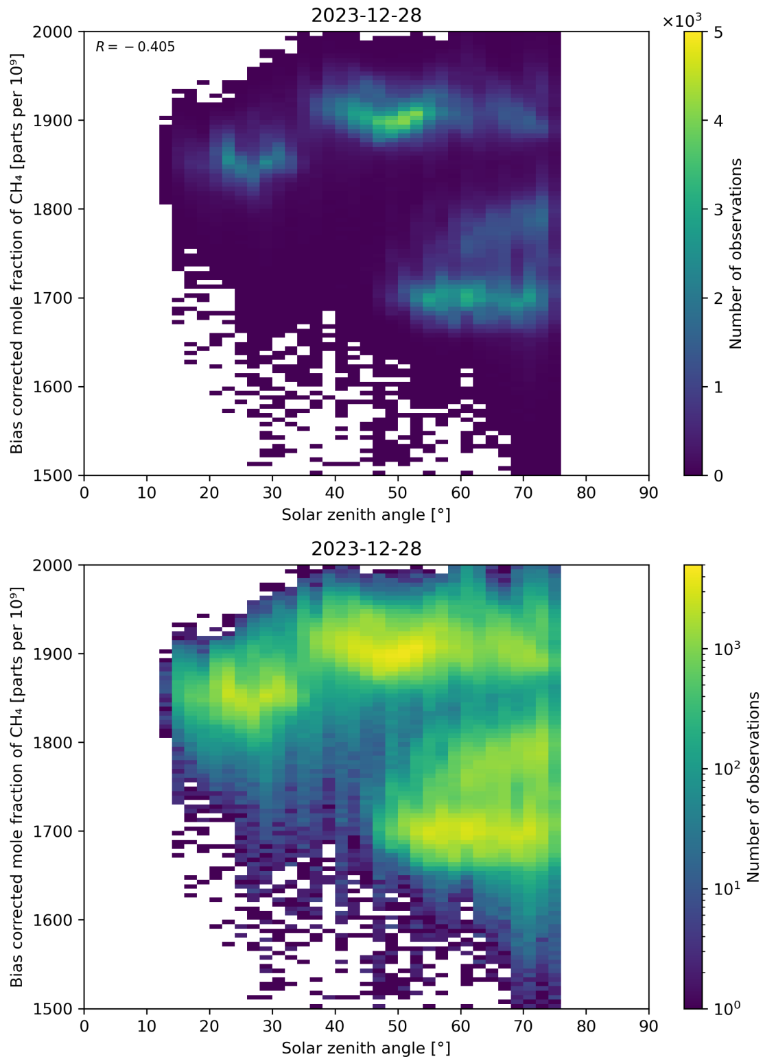
Figure 100: Scatter density plot of “Solar zenith angle” against “Bias corrected mole fraction of \text{CH}_4 ” for 2023-12-27 to 2023-12-29.
