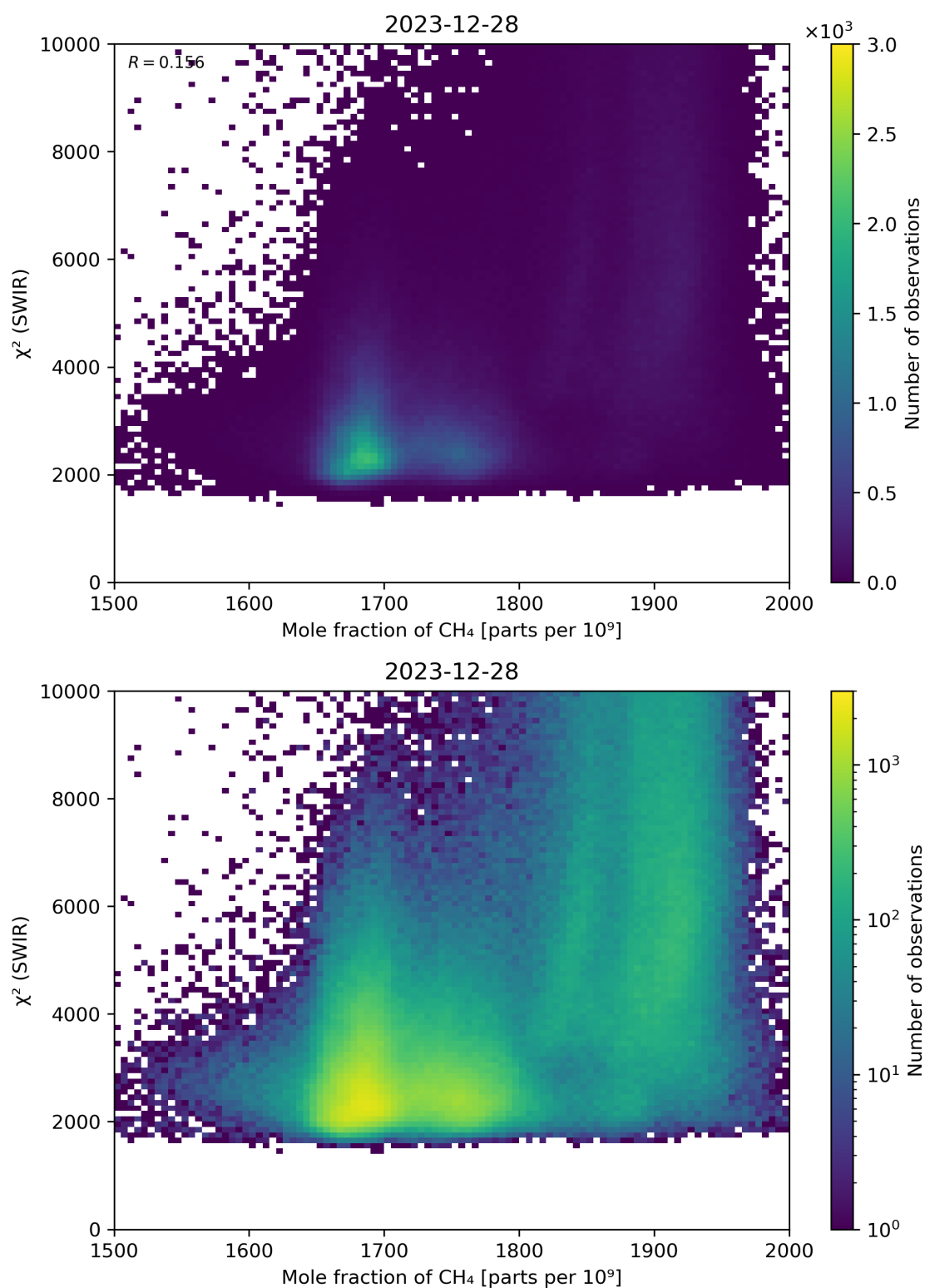
Figure 71: Scatter density plot of “Mole fraction of \text{CH}_4 ” against “ \chi^2 (SWIR)” for 2023-12-27 to 2023-12-29.
