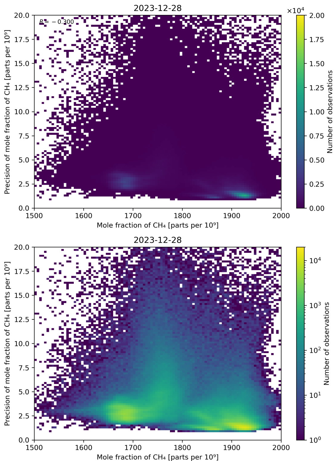
Figure 75: Scatter density plot of “Mole fraction of CH 4 ” against “Precision of mole fraction of CH 4 ” for 2023-12-27 to 2023-12-29.
