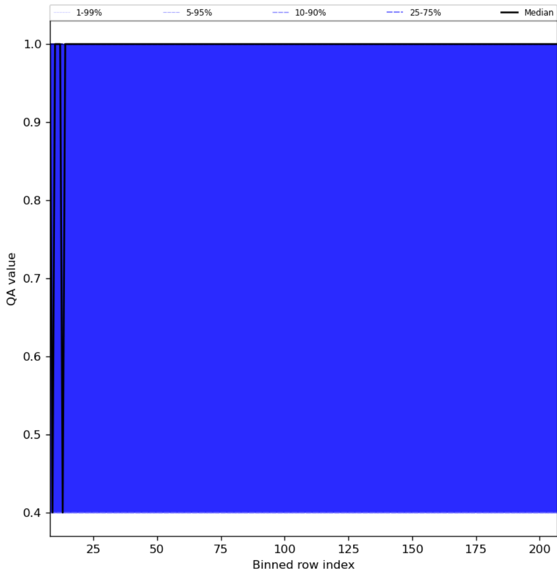
Figure 33: Along track statistics of “QA value” for 2023-12-27 to 2023-12-29
