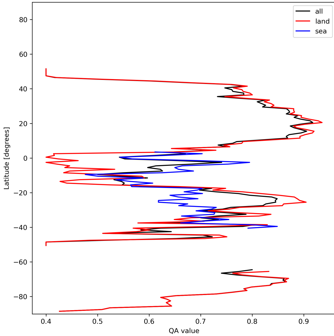
Figure 11: Zonal average of “QA value” for 2023-12-27 to 2023-12-29.
