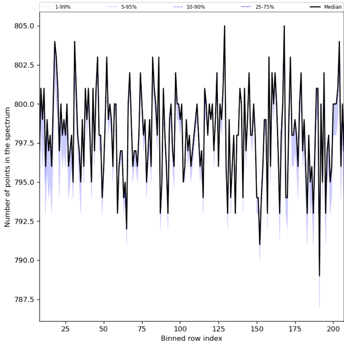
Figure 37: Along track statistics of “Number of points in the spectrum” for 2023-12-27 to 2023-12-29
