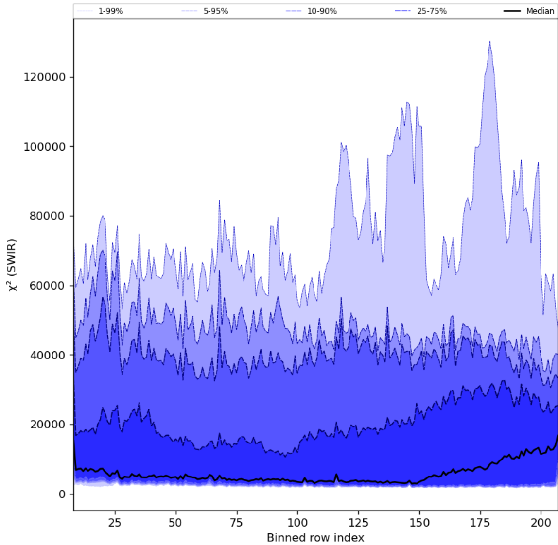
Figure 39: Along track statistics of “ \chi^2 (SWIR)” for 2023-12-27 to 2023-12-29
