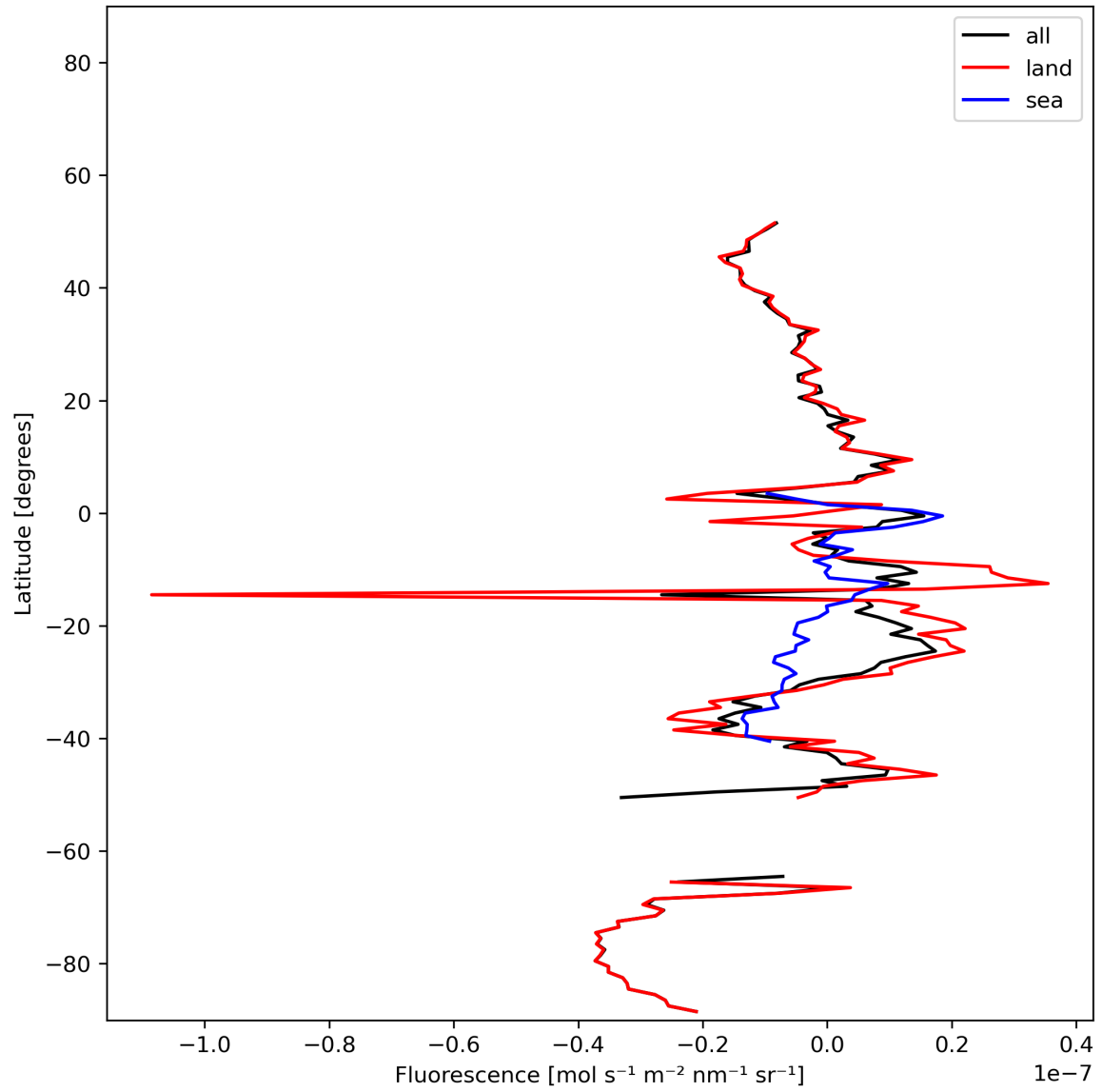
Figure 21: Zonal average of “Fluorescence” for 2023-12-27 to 2023-12-29.
