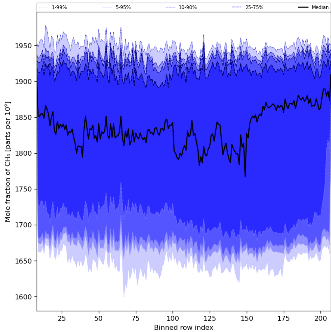
Figure 34: Along track statistics of “Mole fraction of CH 4 ” for 2023-12-27 to 2023-12-29
