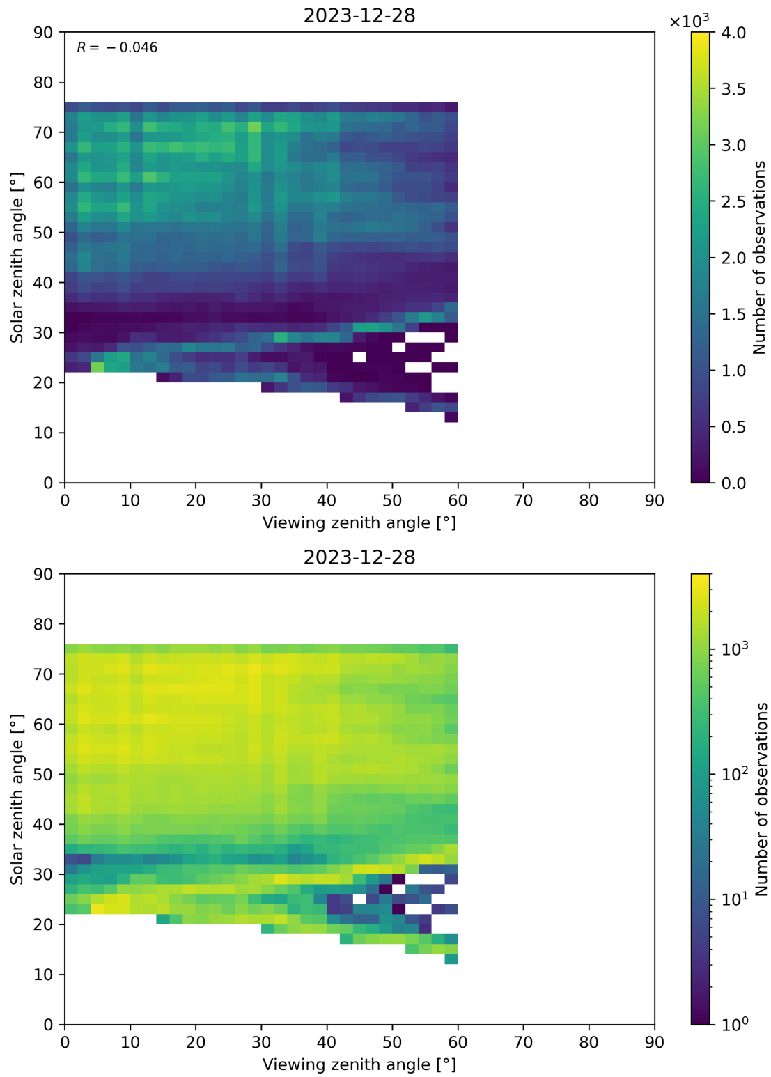
Figure 115: Scatter density plot of “Viewing zenith angle” against “Solar zenith angle” for 2023-12-27 to 2023-12-29.
