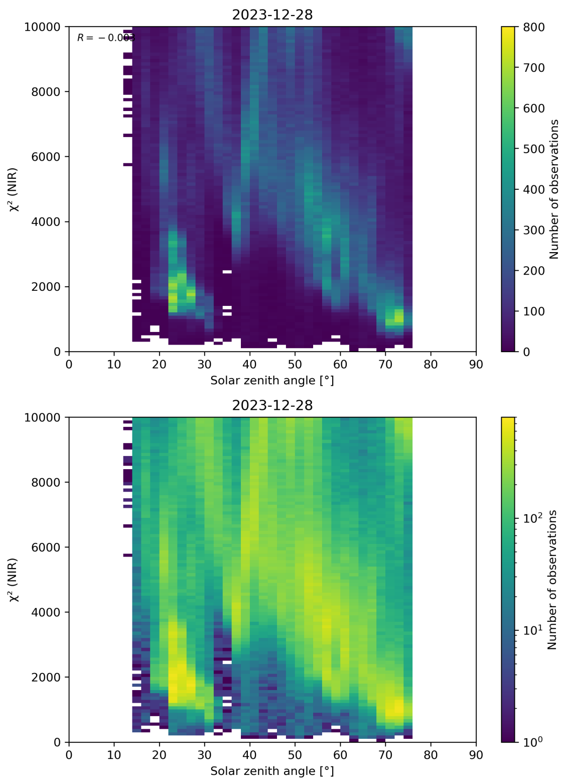
Figure 94: Scatter density plot of “Solar zenith angle” against “ \chi^2 (NIR)” for 2023-12-27 to 2023-12-29.
