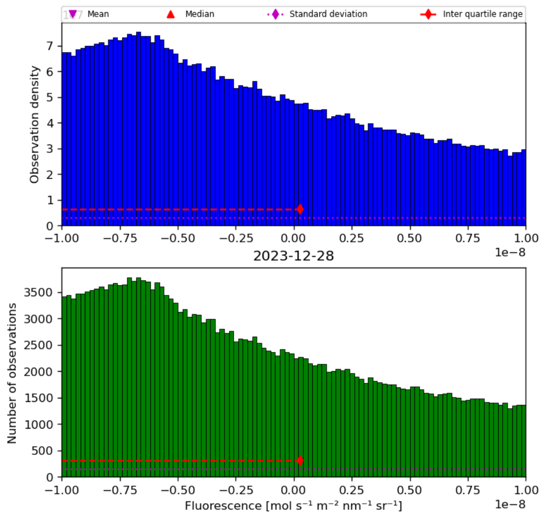
Figure 32: Histogram of “Fluorescence” for 2023-12-27 to 2023-12-29
