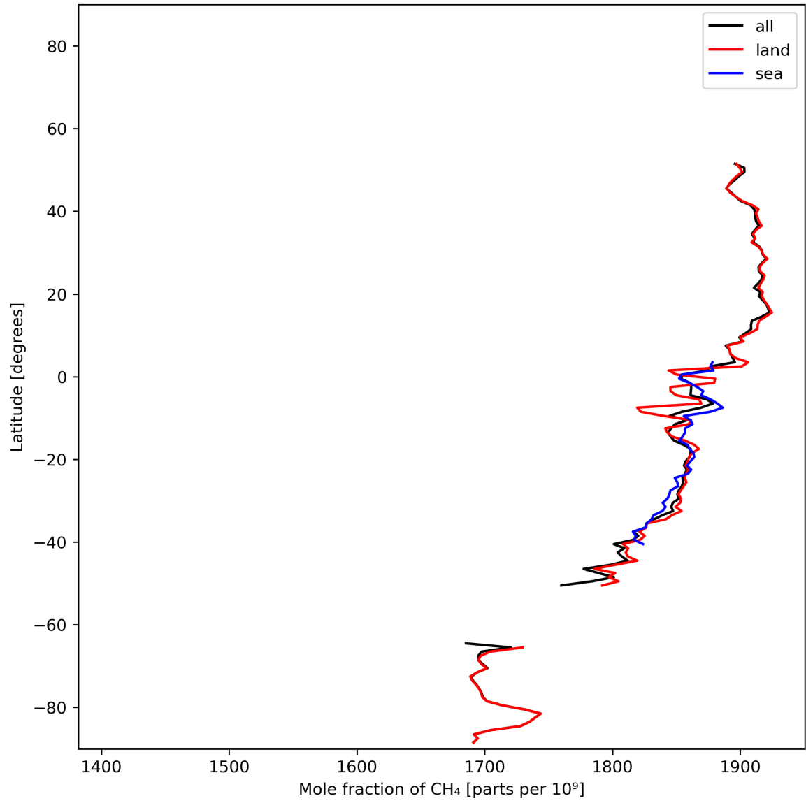
Figure 12: Zonal average of “Mole fraction of CH 4 ” for 2023-12-27 to 2023-12-29.
