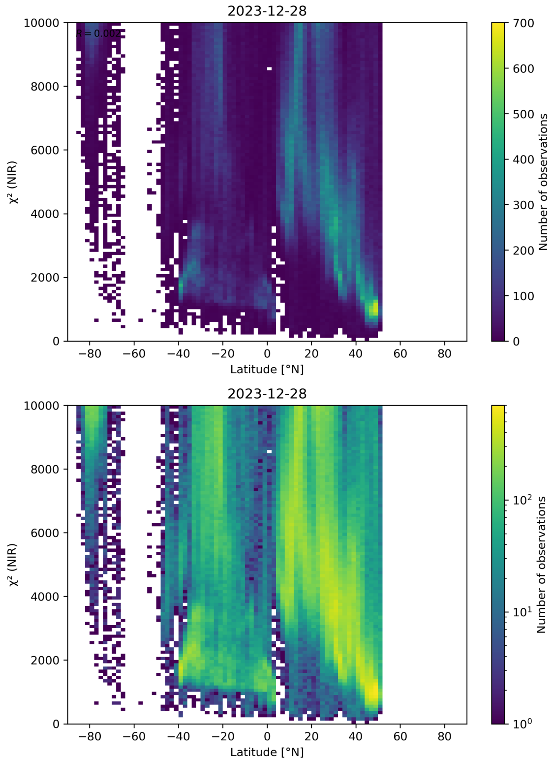
Figure 53: Scatter density plot of “Latitude” against “ \chi^2 (NIR)” for 2023-12-27 to 2023-12-29.
