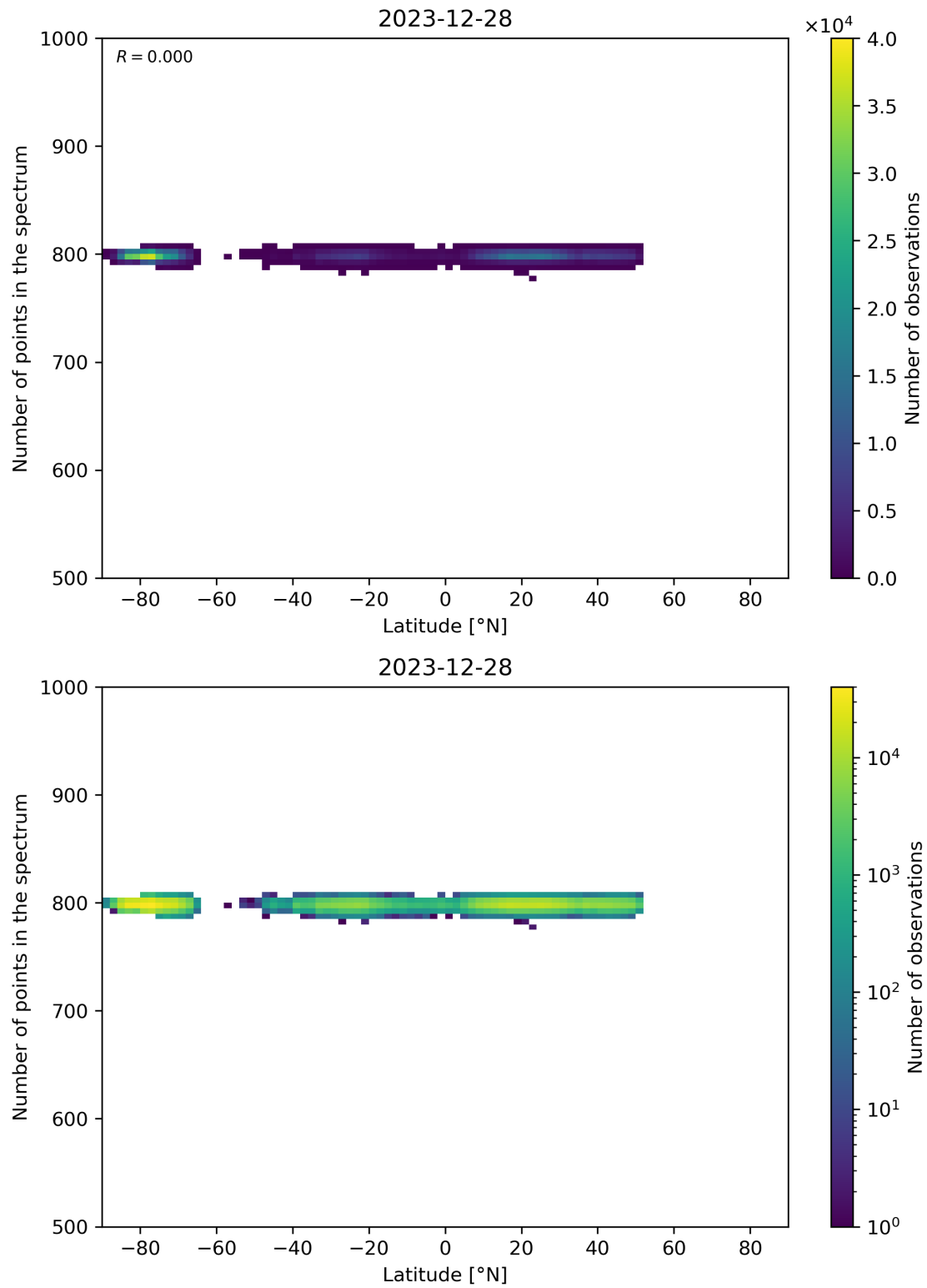
Figure 61: Scatter density plot of “Latitude” against “Number of points in the spectrum” for 2023-12-27 to 2023-12-29.
