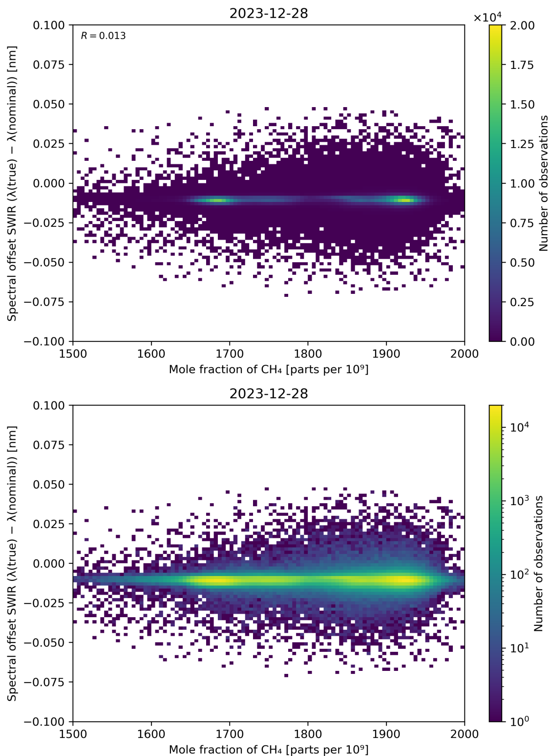
Figure 86: Scatter density plot of “Mole fraction of CH 4 ” against “Spectral offset SWIR ( \lambda(\text{true}) - \lambda(\text{nominal}) )” for 2023-12-27 to 2023-12-29.
