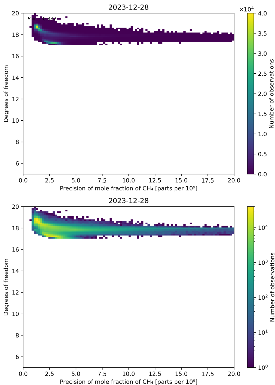
Figure 80: Scatter density plot of “Precision of mole fraction of CH 4 ” against “Degrees of freedom” for 2023-12-27 to 2023-12-29.
