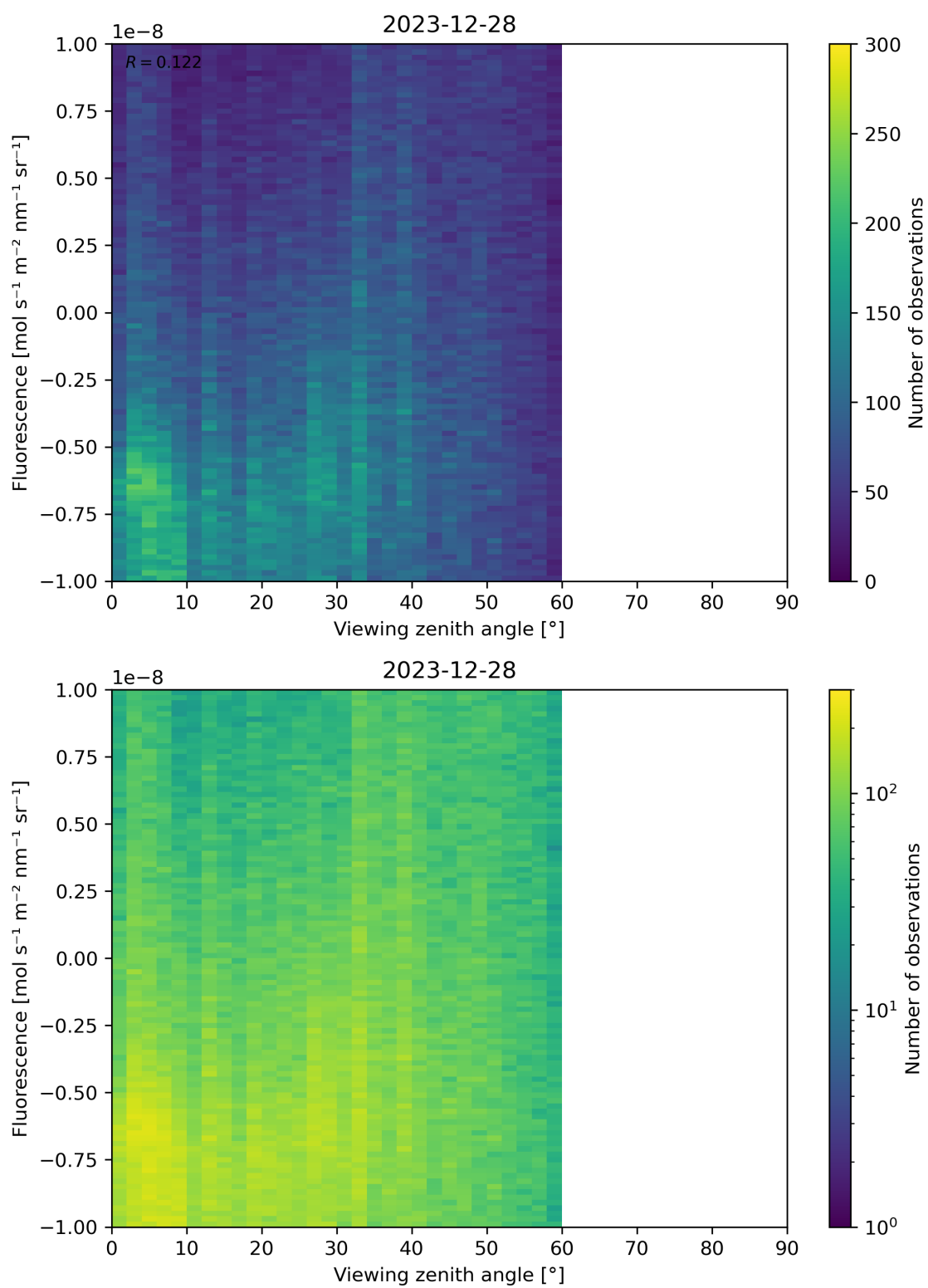
Figure 108: Scatter density plot of “Viewing zenith angle” against “Fluorescence” for 2023-12-27 to 2023-12-29.
