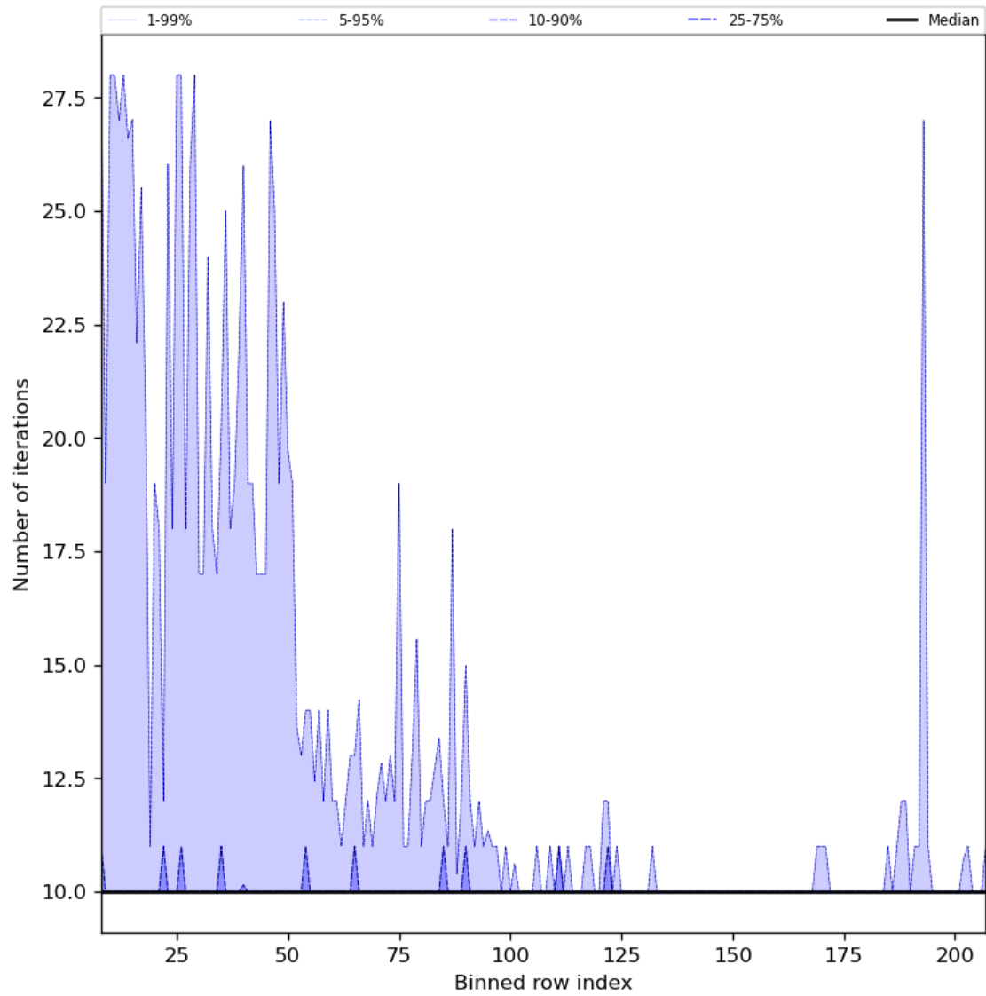
Figure 42: Along track statistics of “Number of iterations” for 2023-12-27 to 2023-12-29
