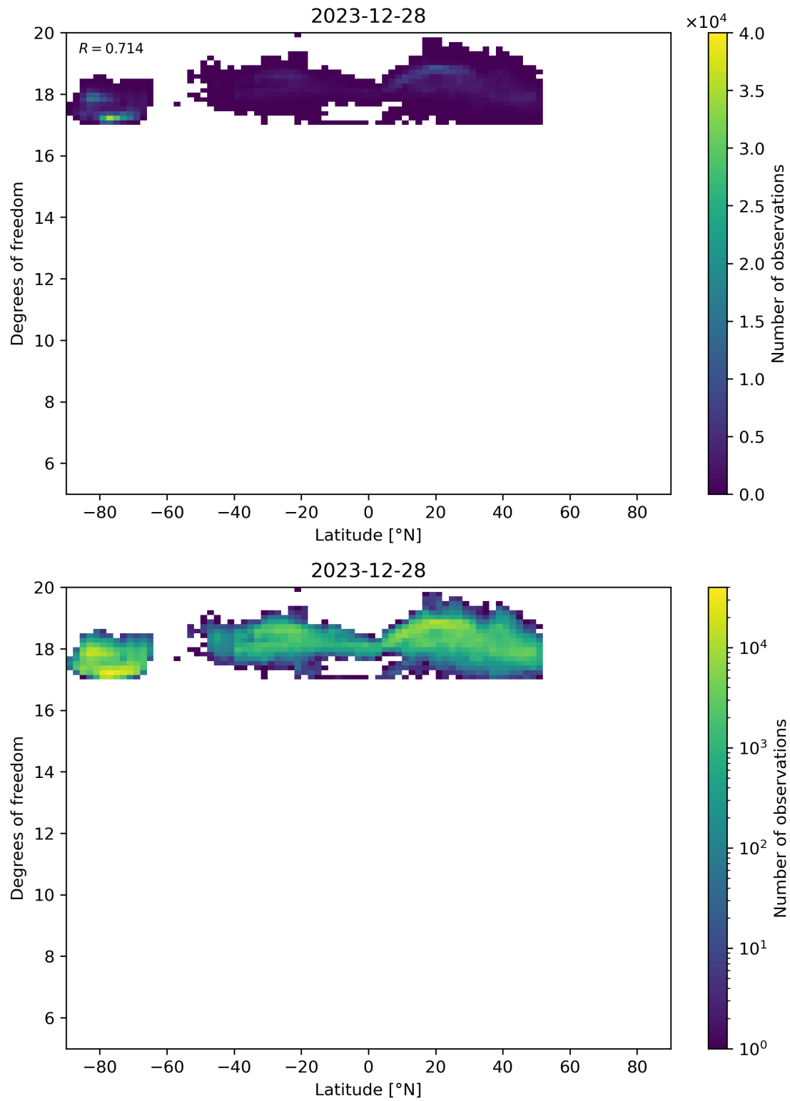
Figure 55: Scatter density plot of “Latitude” against “Degrees of freedom” for 2023-12-27 to 2023-12-29.
