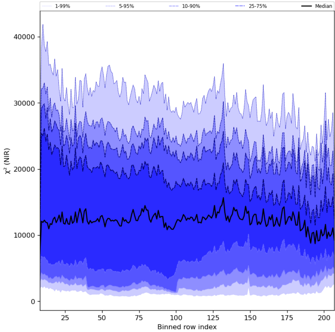
Figure 40: Along track statistics of “ \chi^2 (NIR)” for 2023-12-27 to 2023-12-29
