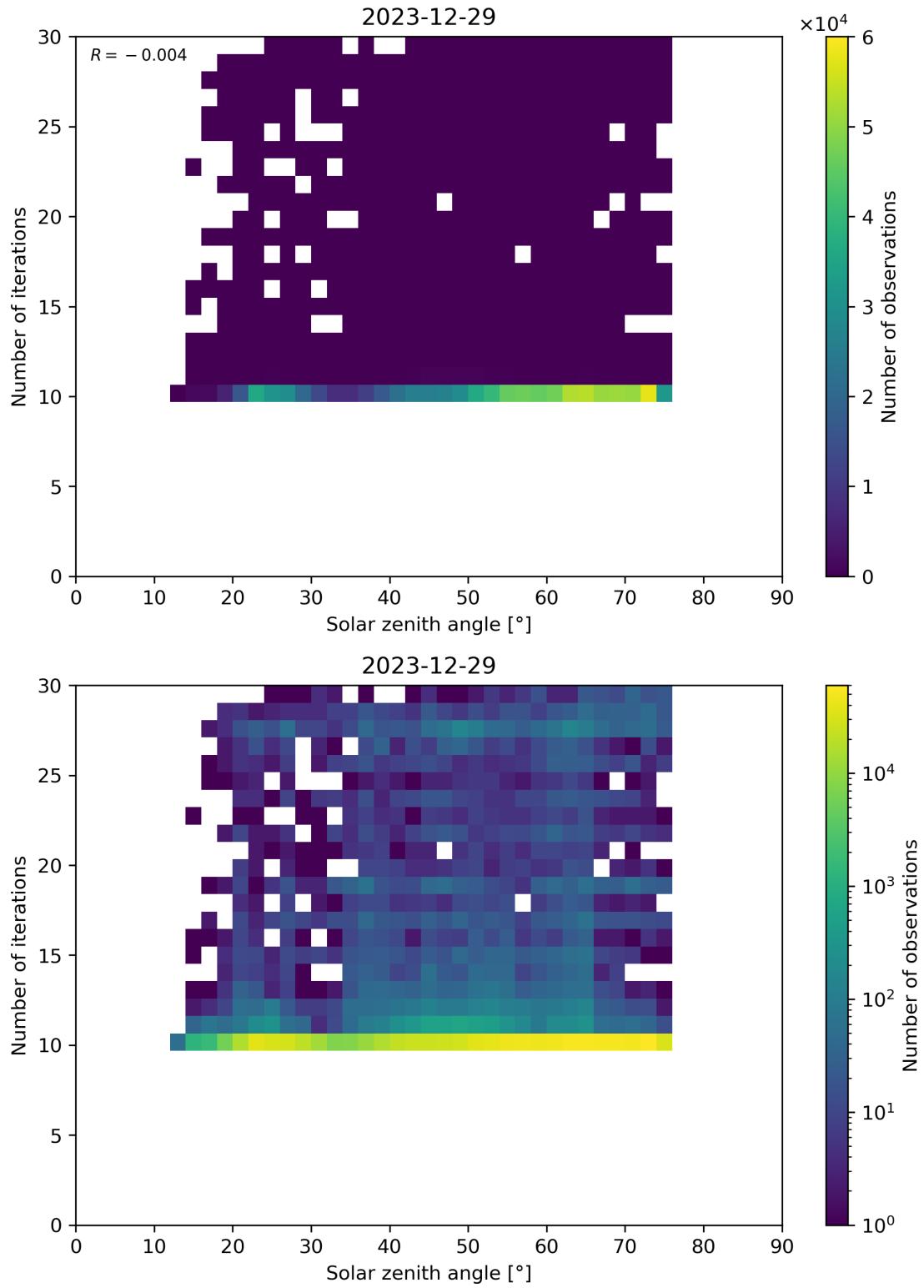
Figure 102: Scatter density plot of “Solar zenith angle” against “Number of iterations” for 2023-12-28 to 2023-12-30.
