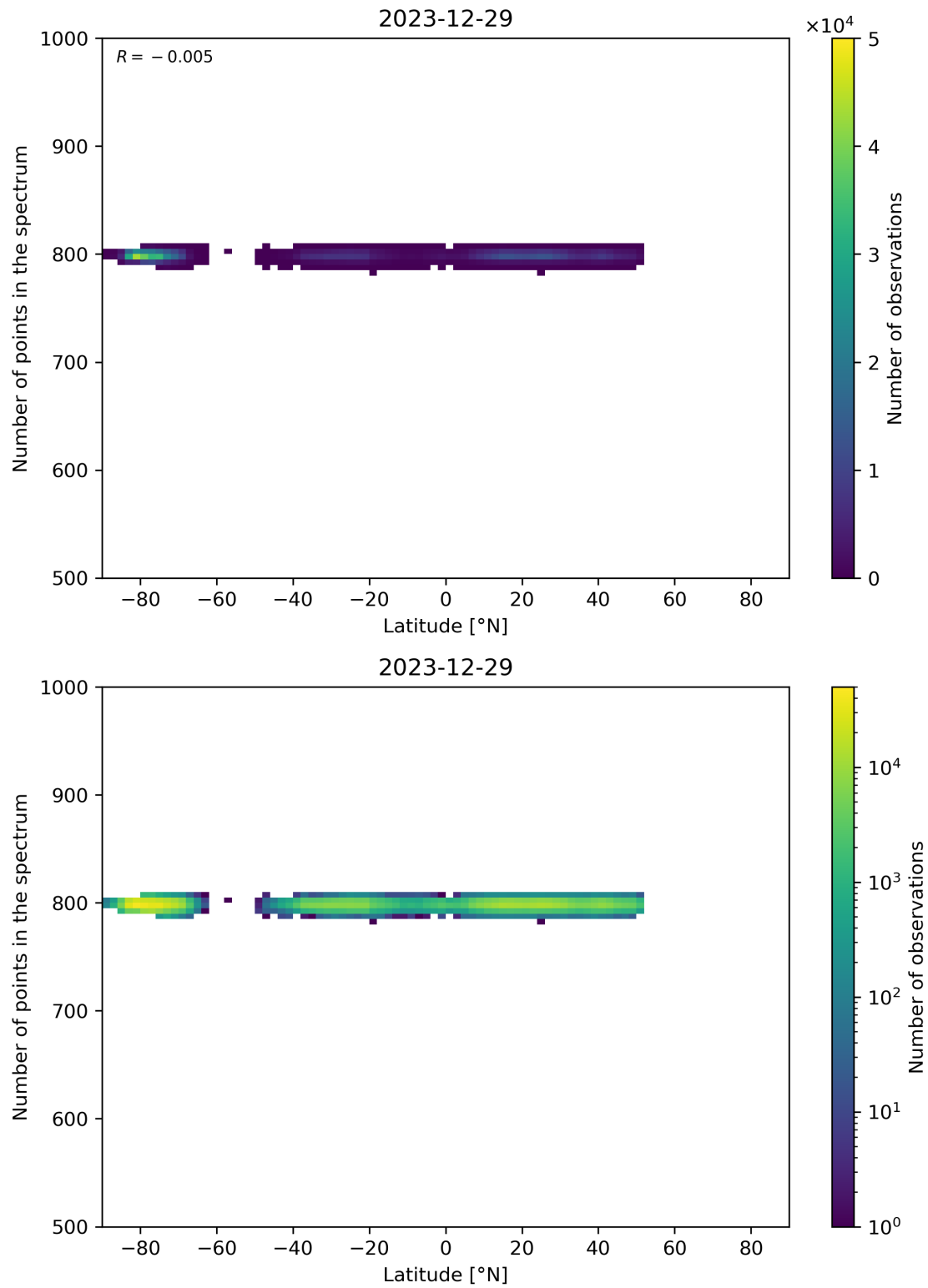
Figure 61: Scatter density plot of “Latitude” against “Number of points in the spectrum” for 2023-12-28 to 2023-12-30.
