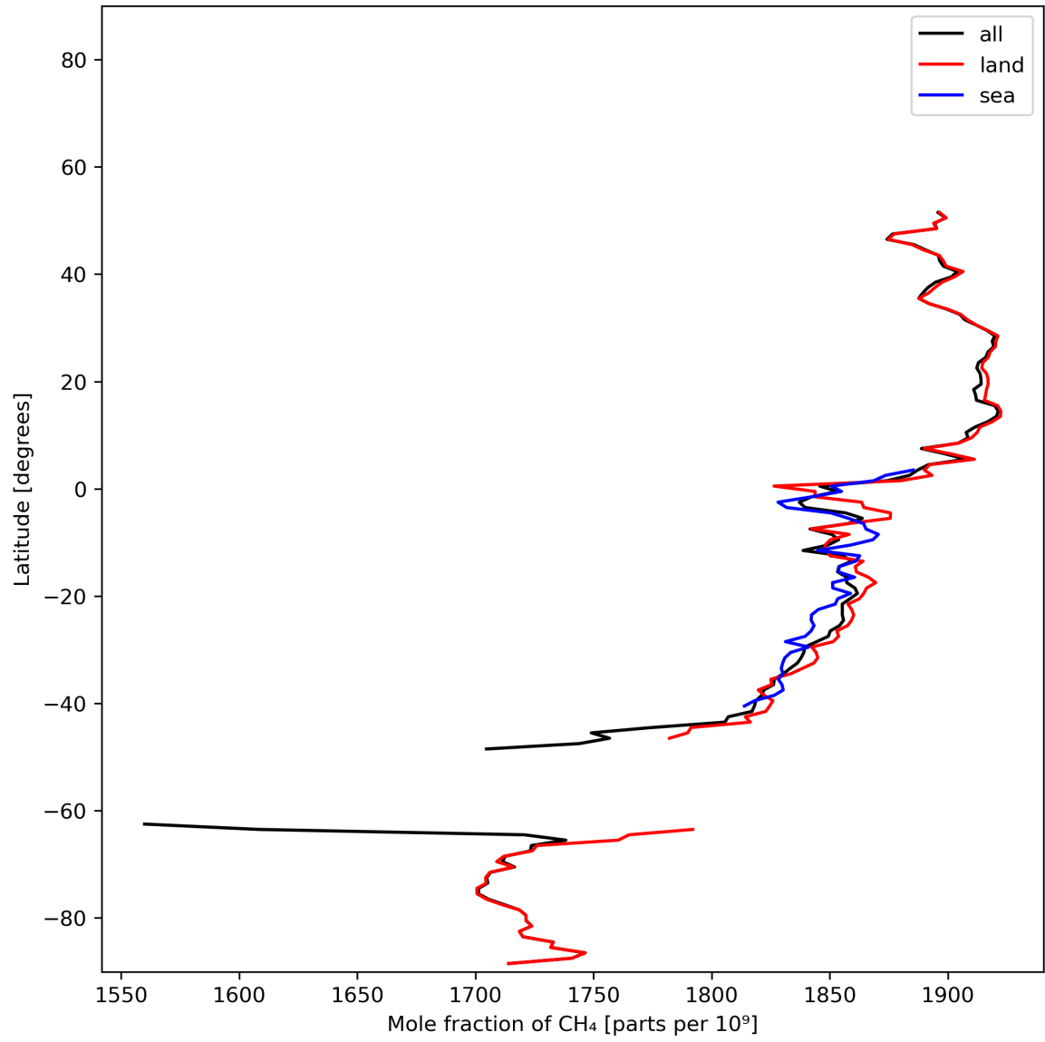
Figure 12: Zonal average of “Mole fraction of \text{CH}_4 ” for 2023-12-28 to 2023-12-30.
