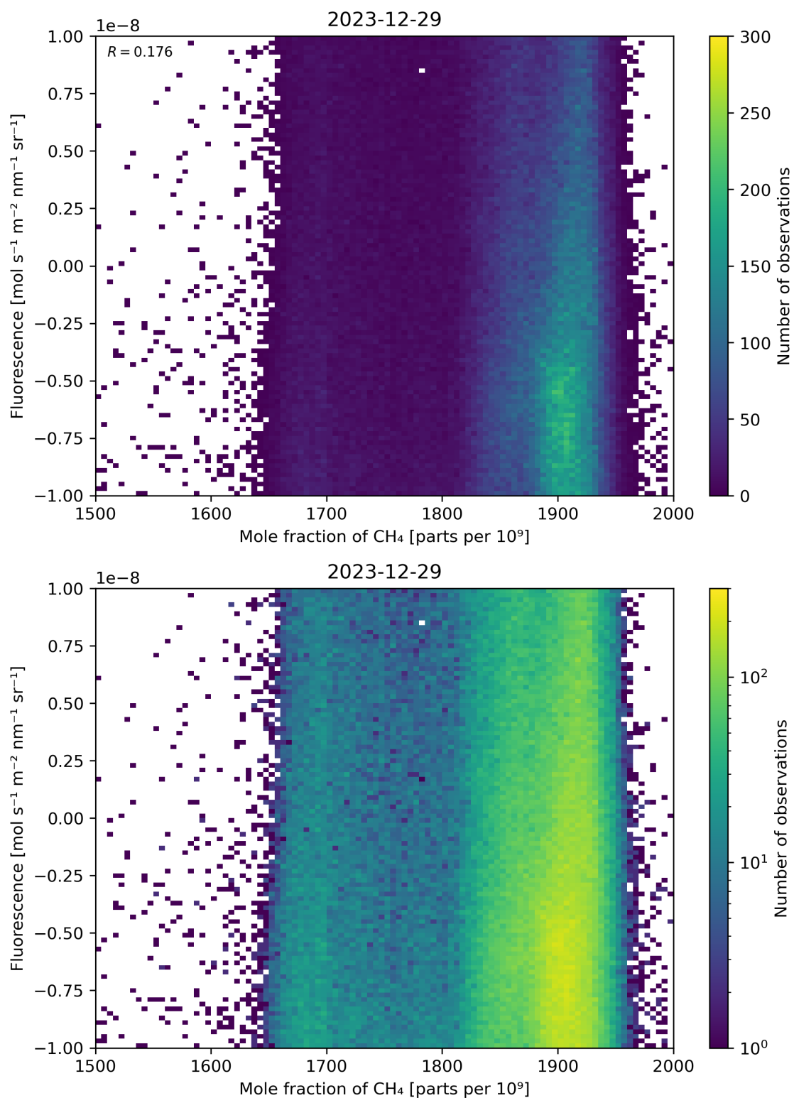
Figure 73: Scatter density plot of “Mole fraction of \text{CH}_4 ” against “Fluorescence” for 2023-12-28 to 2023-12-30.
