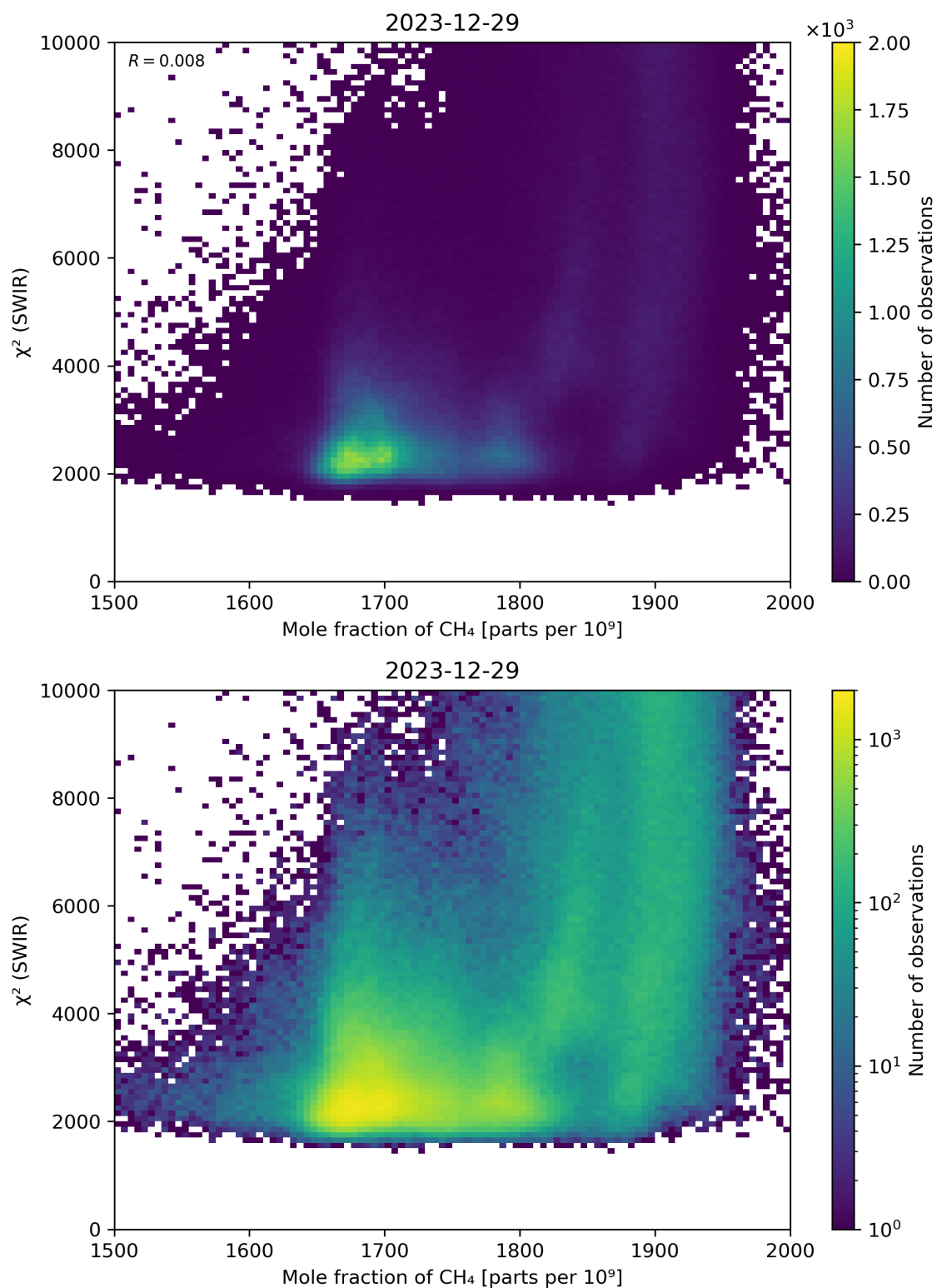
Figure 71: Scatter density plot of “Mole fraction of \text{CH}_4 ” against “ \chi^2 (SWIR)” for 2023-12-28 to 2023-12-30.
