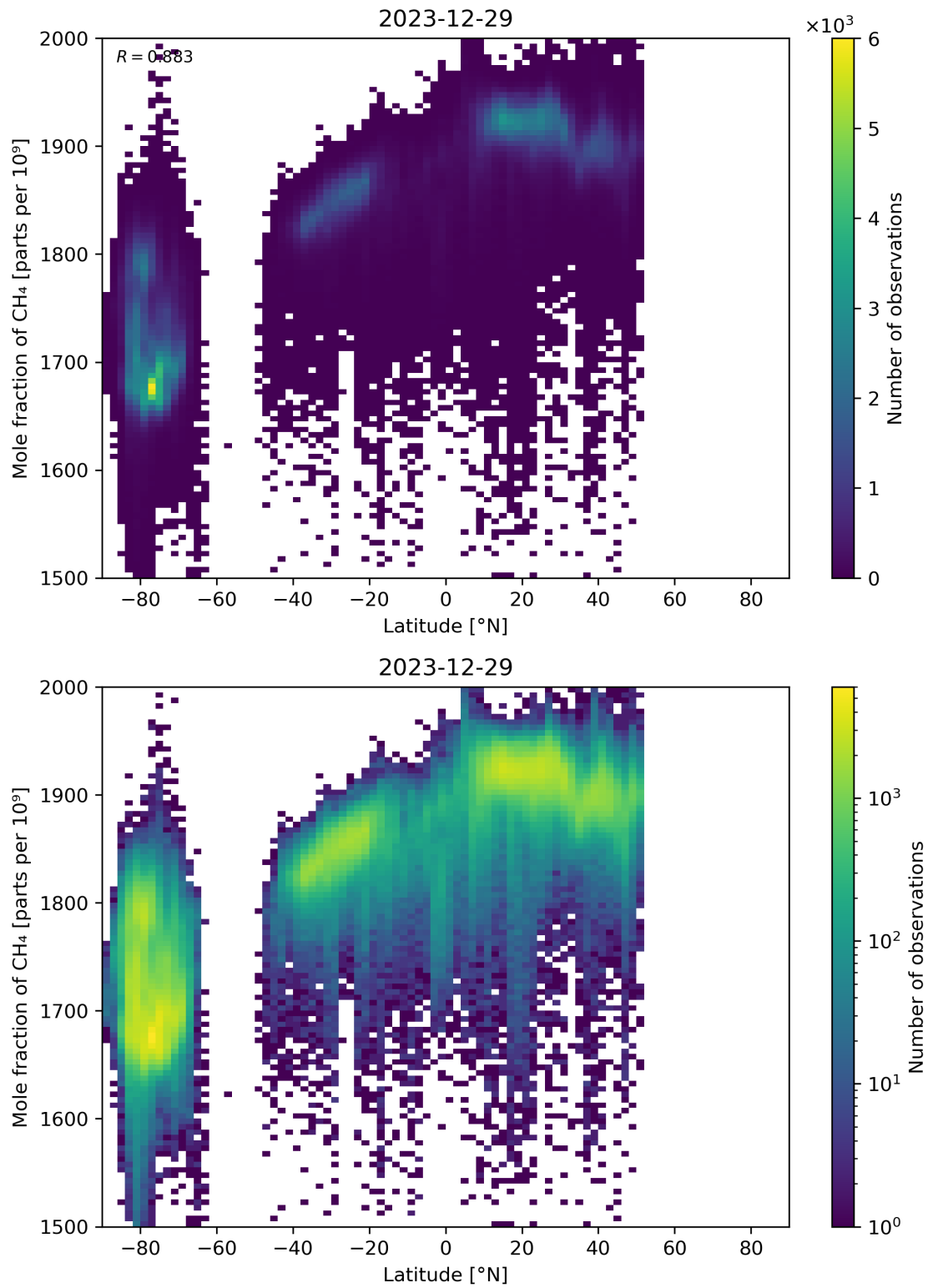
Figure 57: Scatter density plot of “Latitude” against “Mole fraction of CH 4 ” for 2023-12-28 to 2023-12-30.
