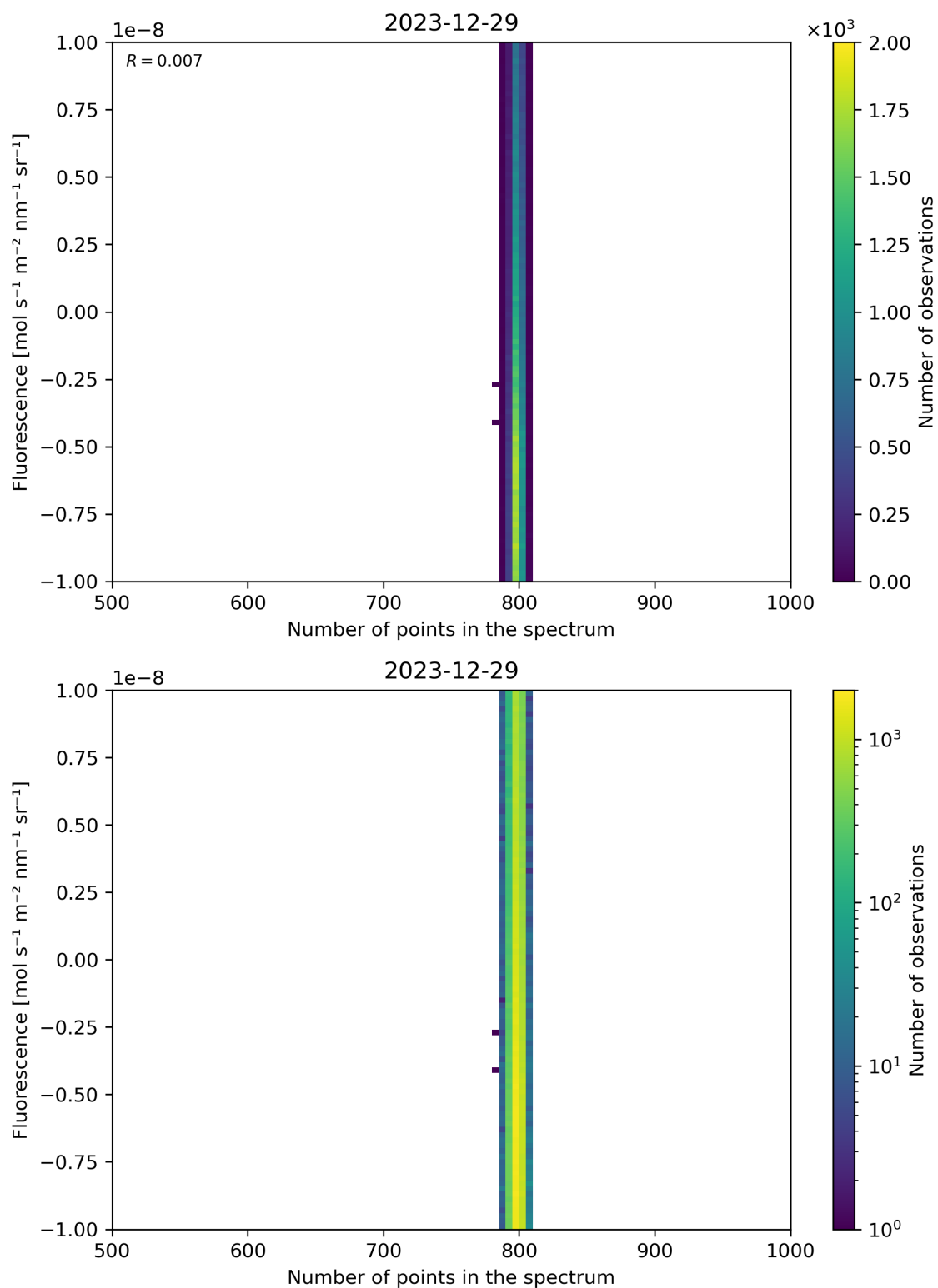
Figure 91: Scatter density plot of “Number of points in the spectrum” against “Fluorescence” for 2023-12-28 to 2023-12-30.
