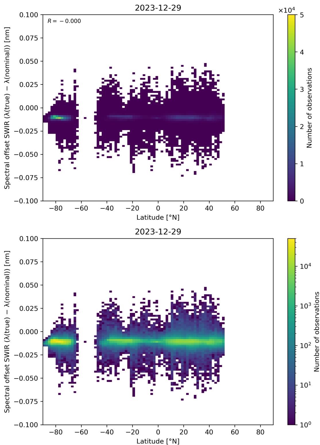
Figure 62: Scatter density plot of “Latitude” against “Spectral offset SWIR ( \lambda(\text{true}) - \lambda(\text{nominal}) )” for 2023-12-28 to 2023-12-30.
