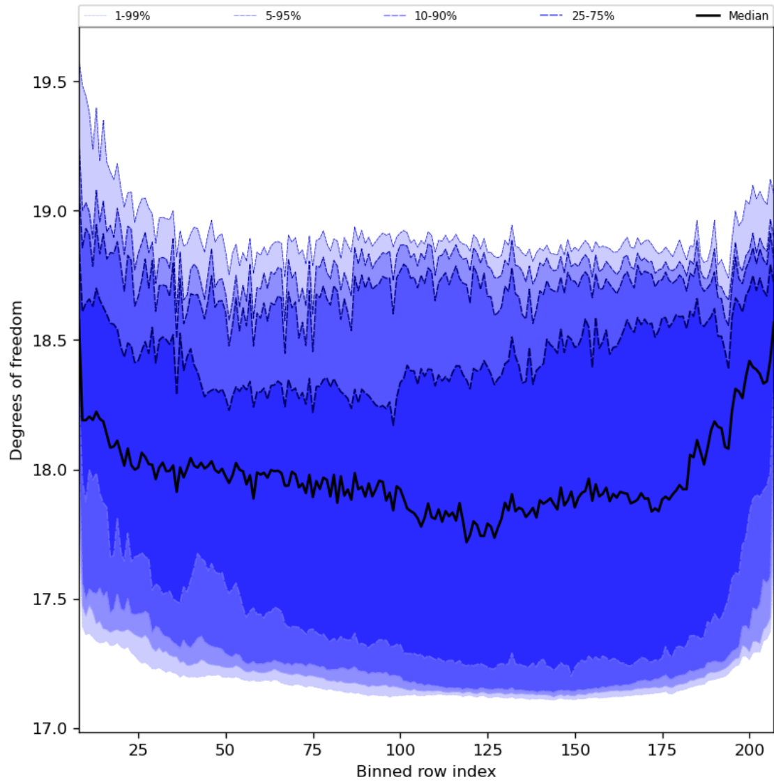
Figure 41: Along track statistics of “Degrees of freedom” for 2023-12-28 to 2023-12-30
