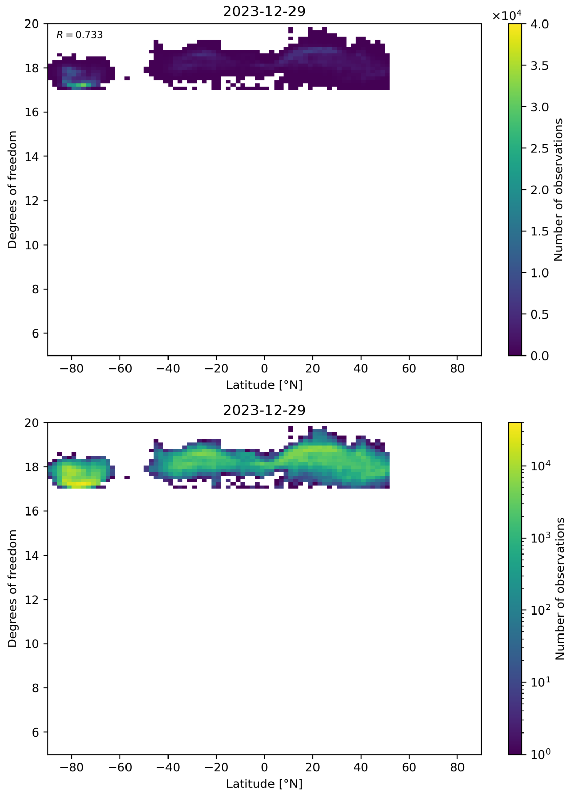
Figure 55: Scatter density plot of “Latitude” against “Degrees of freedom” for 2023-12-28 to 2023-12-30.
