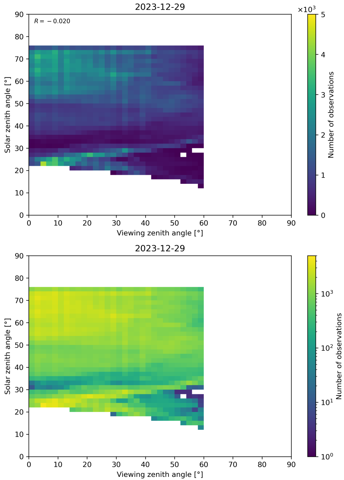
Figure 115: Scatter density plot of “Viewing zenith angle” against “Solar zenith angle” for 2023-12-28 to 2023-12-30.
