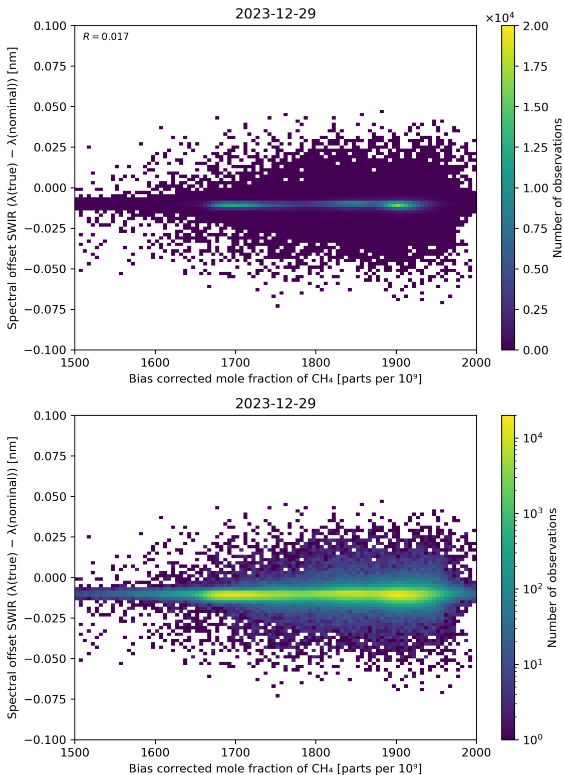
Figure 69: Scatter density plot of “Bias corrected mole fraction of \text{CH}_4 ” against “Spectral offset SWIR ( \lambda(\text{true}) - \lambda(\text{nominal}) )” for 2023-12-28 to 2023-12-30.
