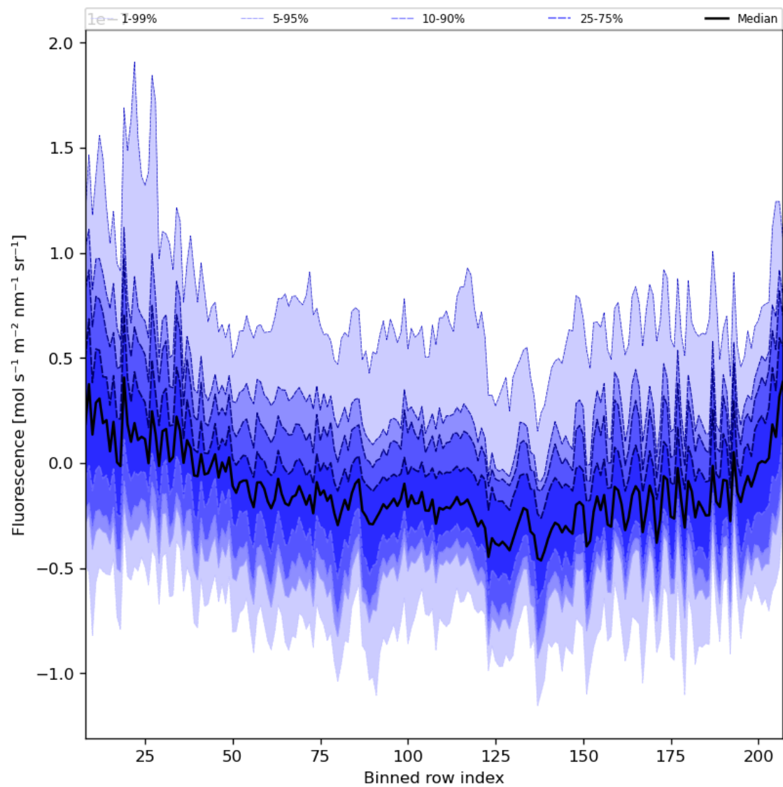
Figure 43: Along track statistics of “Fluorescence” for 2023-12-28 to 2023-12-30
