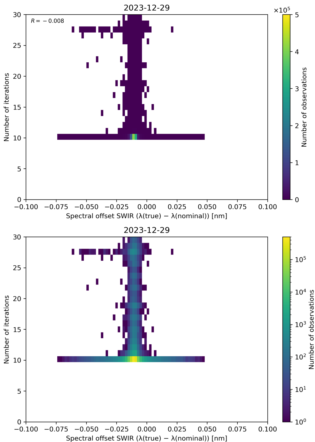
Figure 121: Scatter density plot of “Spectral offset SWIR ( \lambda(\text{true}) - \lambda(\text{nominal}) )” against “Number of iterations” for 2023-12-28 to 2023-12-30.
