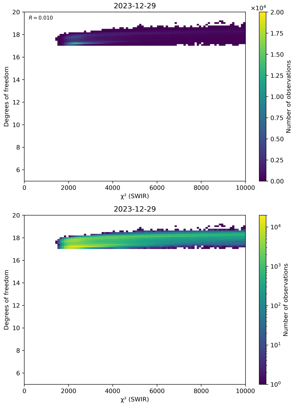
Figure 48: Scatter density plot of “ \chi^2 (SWIR)” against “Degrees of freedom” for 2023-12-28 to 2023-12-30.
