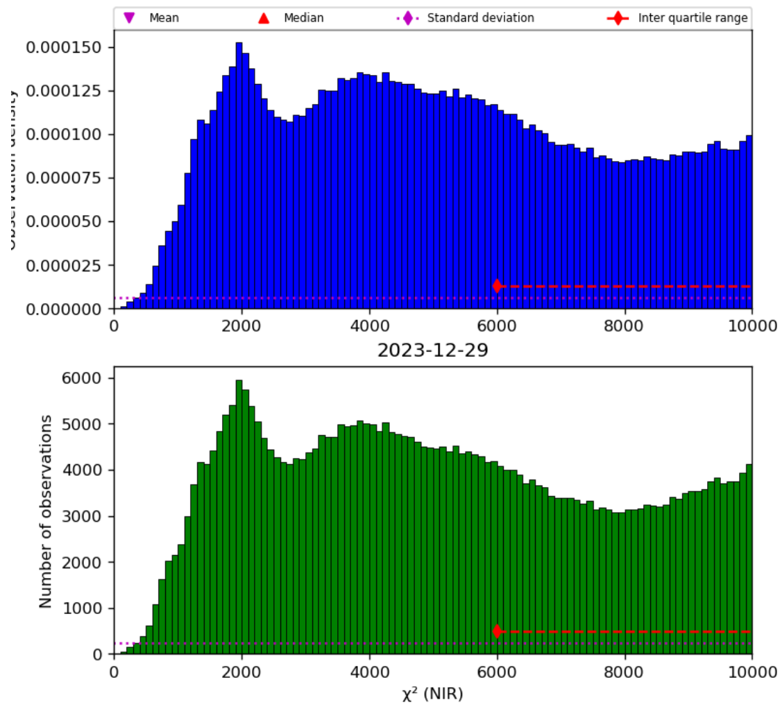
Figure 29: Histogram of “ \chi^2 (NIR)” for 2023-12-28 to 2023-12-30
