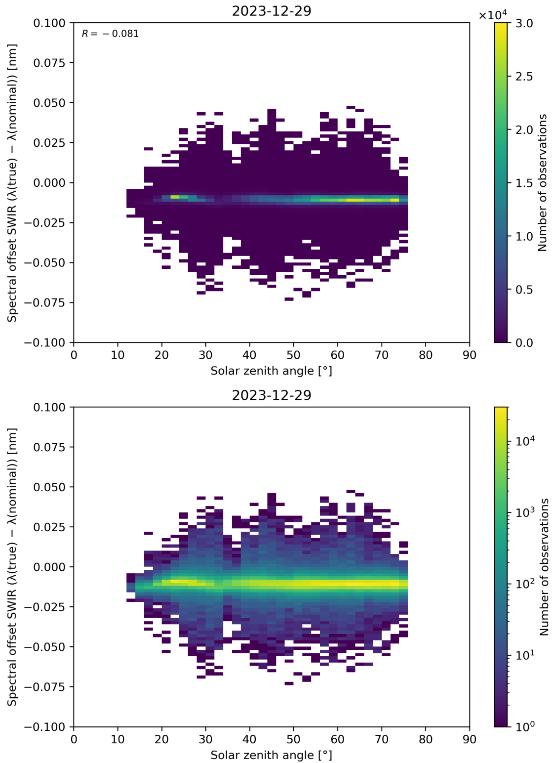
Figure 104: Scatter density plot of “Solar zenith angle” against “Spectral offset SWIR ( \lambda(\text{true}) - \lambda(\text{nominal}) )” for 2023-12-28 to 2023-12-30.
