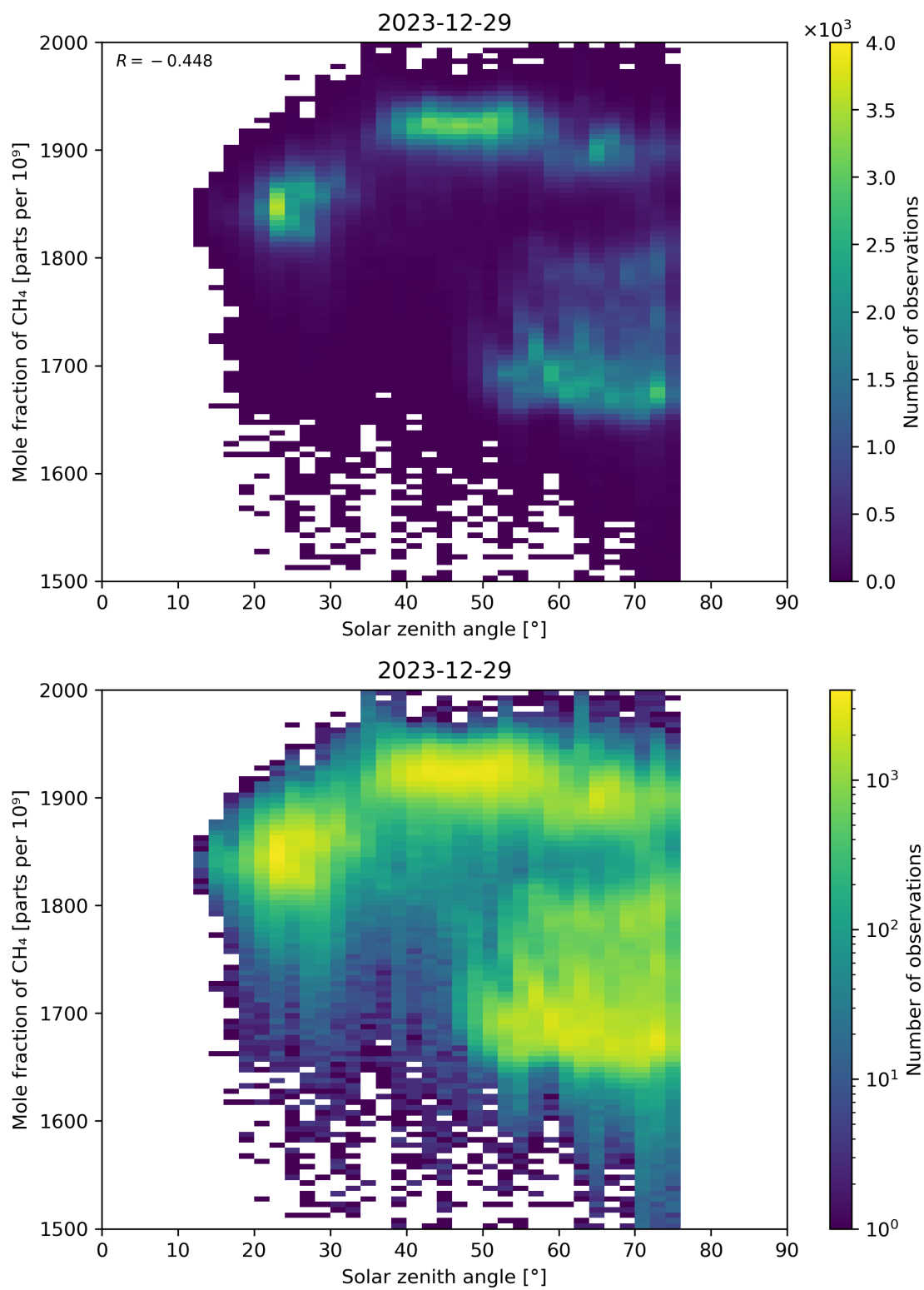
Figure 99: Scatter density plot of “Solar zenith angle” against “Mole fraction of CH 4 ” for 2023-12-28 to 2023-12-30.
