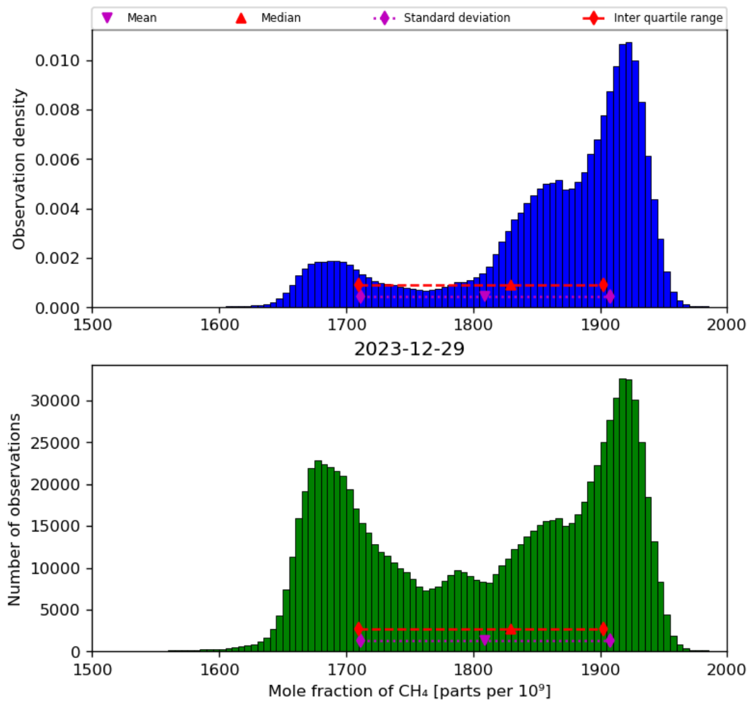
Figure 23: Histogram of “Mole fraction of CH 4 ” for 2023-12-28 to 2023-12-30
