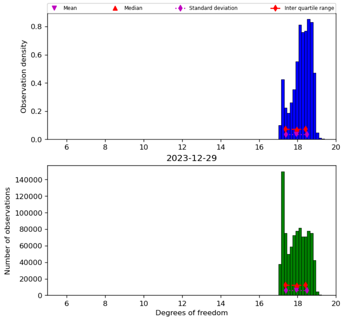
Figure 30: Histogram of “Degrees of freedom” for 2023-12-28 to 2023-12-30
