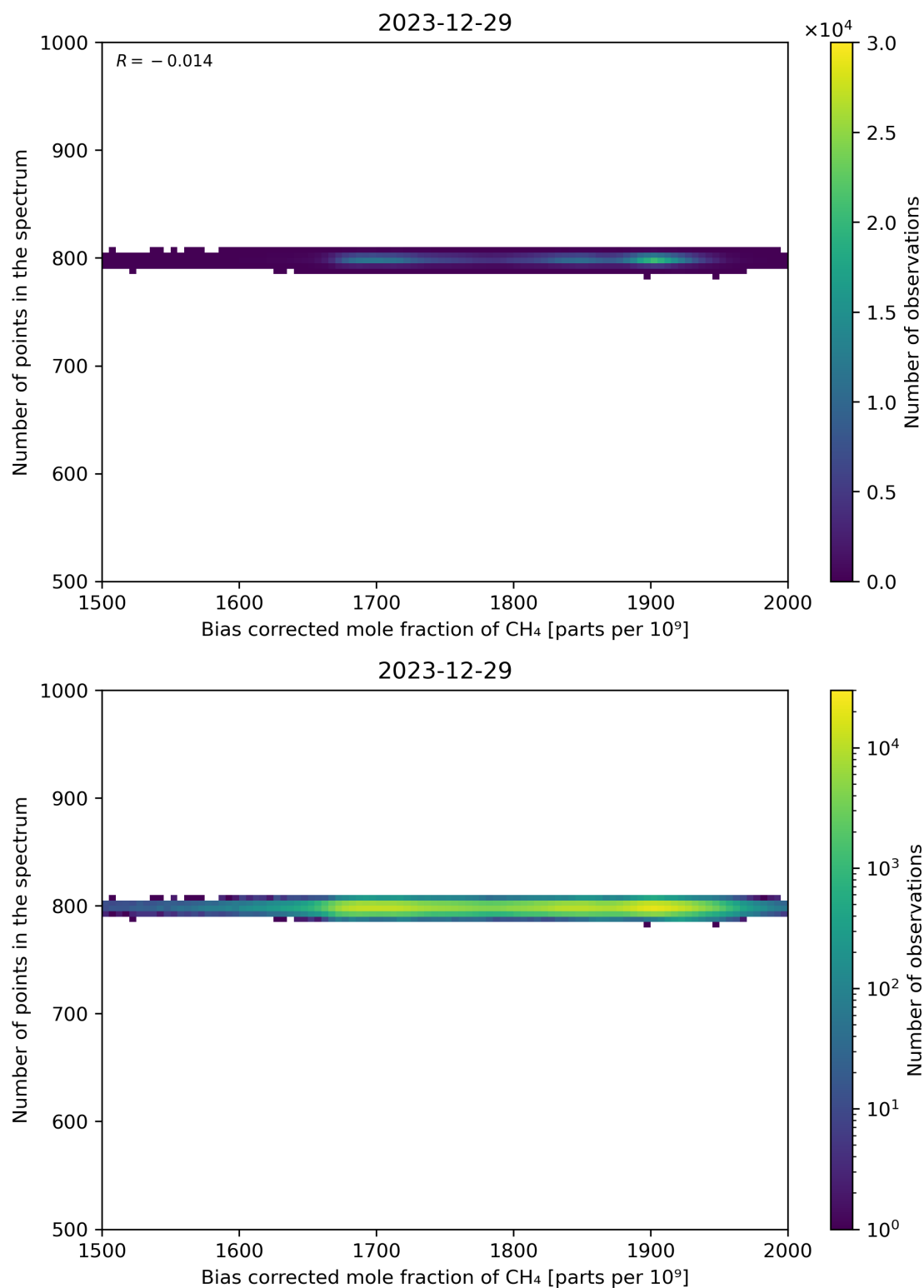
Figure 68: Scatter density plot of “Bias corrected mole fraction of CH 4 ” against “Number of points in the spectrum” for 2023-12-28 to 2023-12-30.
