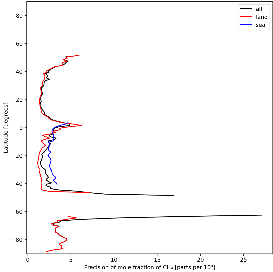
Figure 13: Zonal average of “Precision of mole fraction of CH 4 ” for 2023-12-28 to 2023-12-30.
