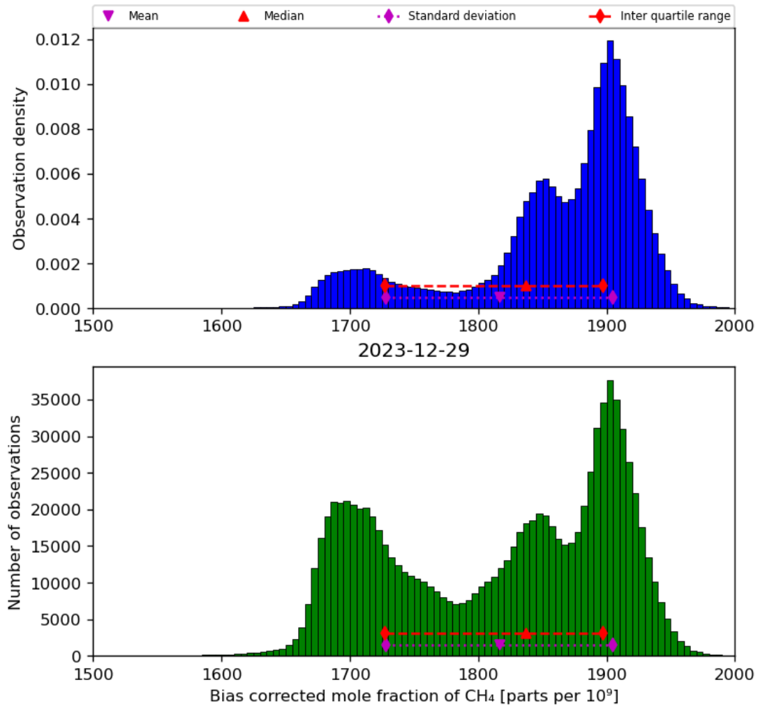
Figure 25: Histogram of “Bias corrected mole fraction of CH 4 ” for 2023-12-28 to 2023-12-30
