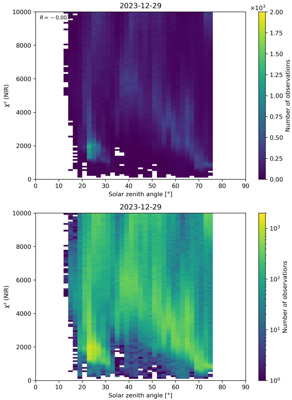
Figure 94: Scatter density plot of “Solar zenith angle” against “ \chi^2 (NIR)” for 2023-12-28 to 2023-12-30.
