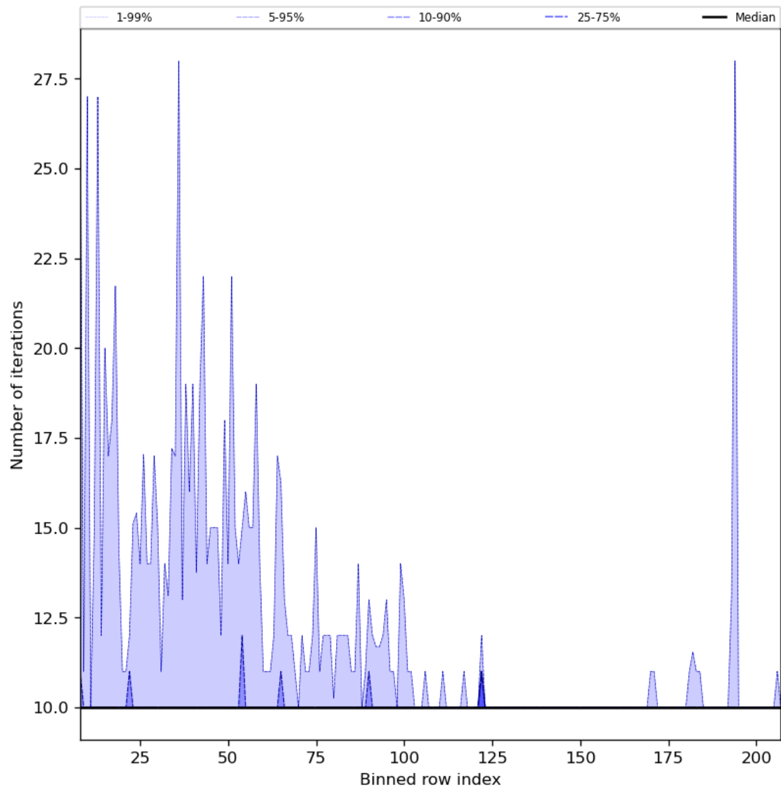
Figure 42: Along track statistics of “Number of iterations” for 2023-12-28 to 2023-12-30
