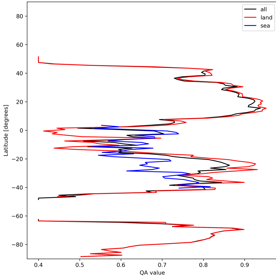
Figure 11: Zonal average of “QA value” for 2023-12-28 to 2023-12-30.
