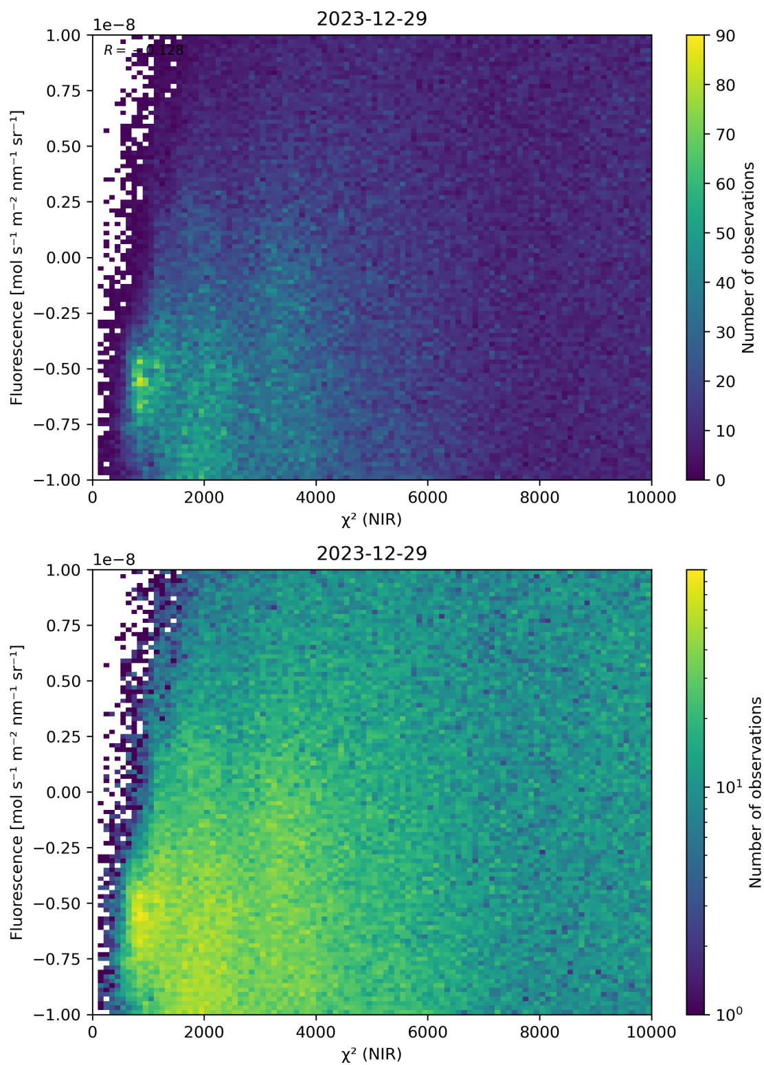
Figure 45: Scatter density plot of “ \chi^2 (NIR)” against “Fluorescence” for 2023-12-28 to 2023-12-30.
