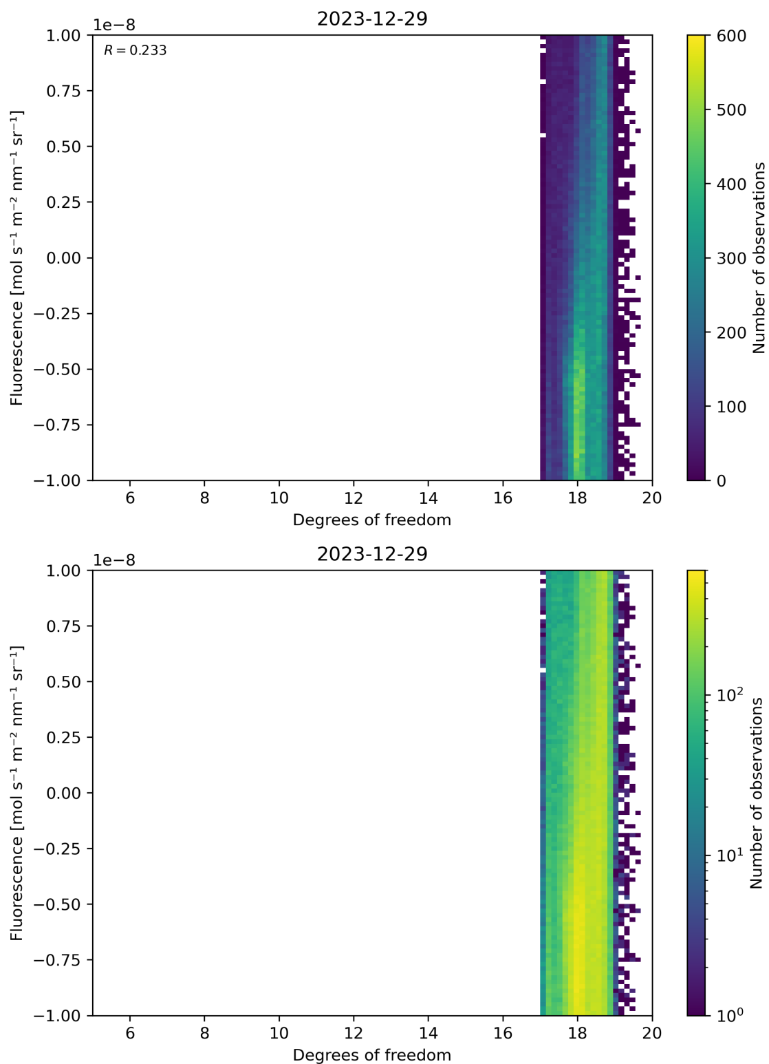
Figure 51: Scatter density plot of “Degrees of freedom” against “Fluorescence” for 2023-12-28 to 2023-12-30.
