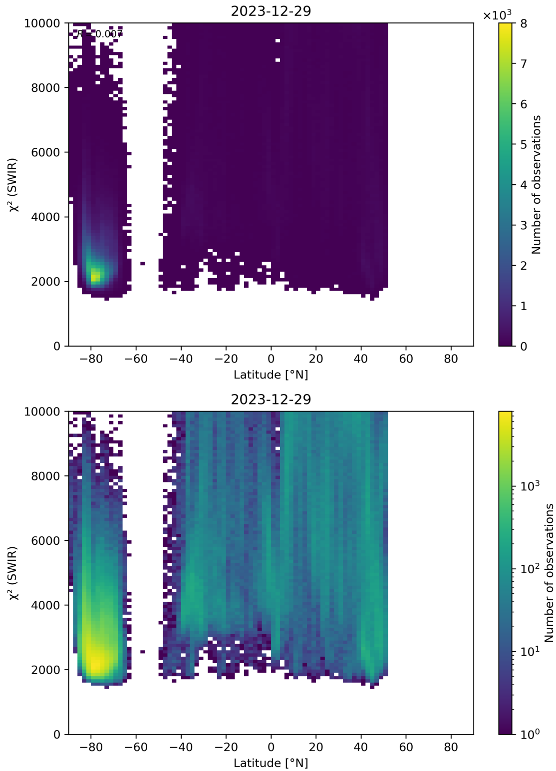
Figure 54: Scatter density plot of “Latitude” against “ \chi^2 (SWIR)” for 2023-12-28 to 2023-12-30.
