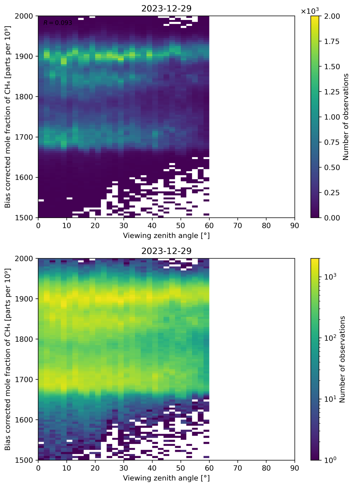
Figure 111: Scatter density plot of “Viewing zenith angle” against “Bias corrected mole fraction of CH 4 ” for 2023-12-28 to 2023-12-30.
