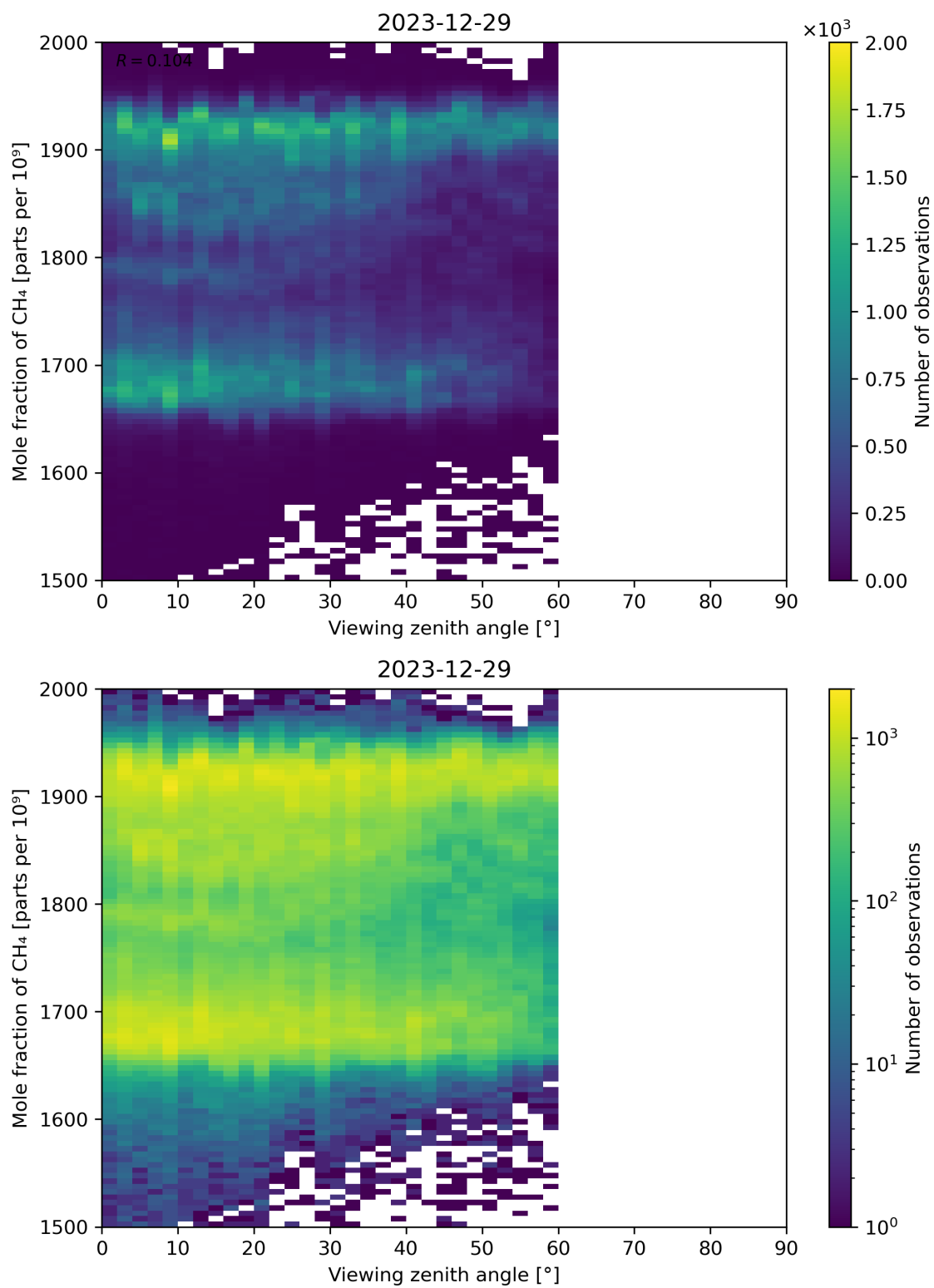
Figure 110: Scatter density plot of “Viewing zenith angle” against “Mole fraction of CH 4 ” for 2023-12-28 to 2023-12-30.
