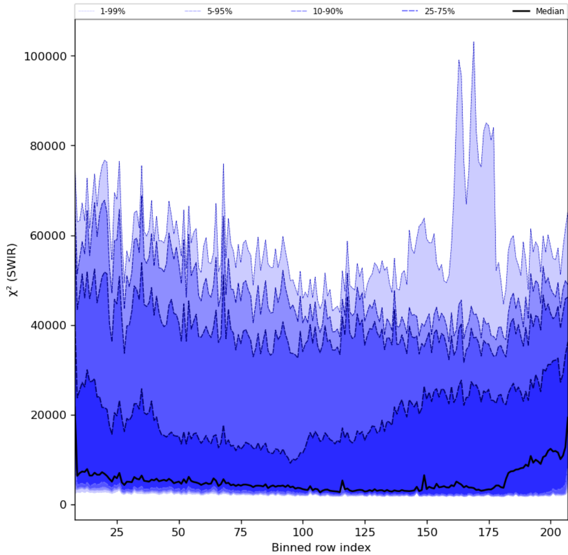
Figure 39: Along track statistics of “ \chi^2 (SWIR)” for 2023-12-28 to 2023-12-30
