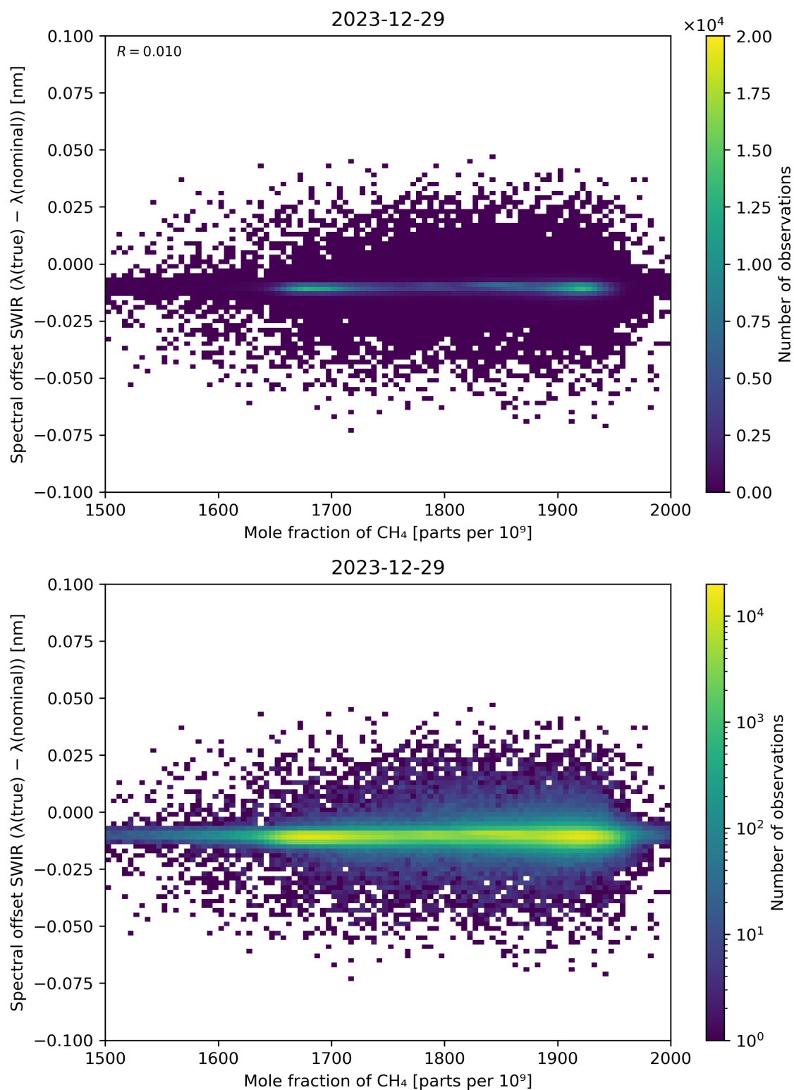
Figure 86: Scatter density plot of “Mole fraction of CH 4 ” against “Spectral offset SWIR ( \lambda(\text{true}) - \lambda(\text{nominal}) )” for 2023-12-28 to 2023-12-30.
