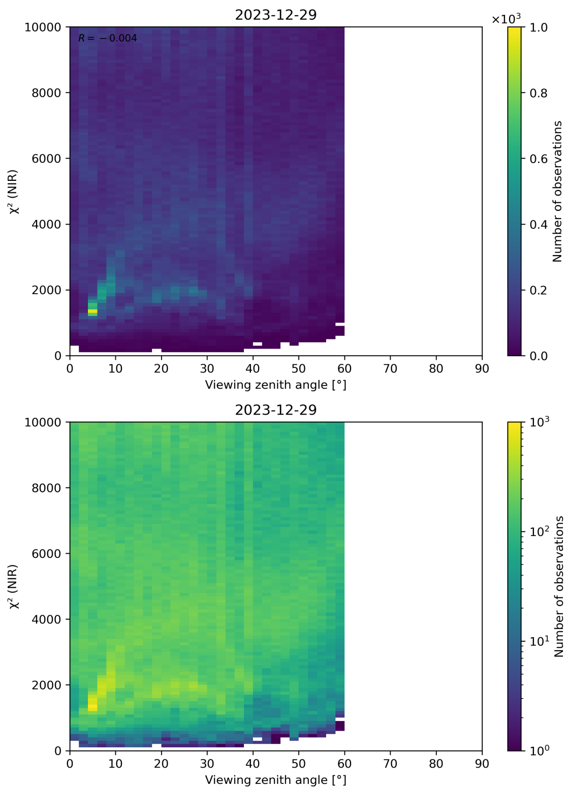
Figure 105: Scatter density plot of “Viewing zenith angle” against “ \chi^2 (NIR)” for 2023-12-28 to 2023-12-30.
