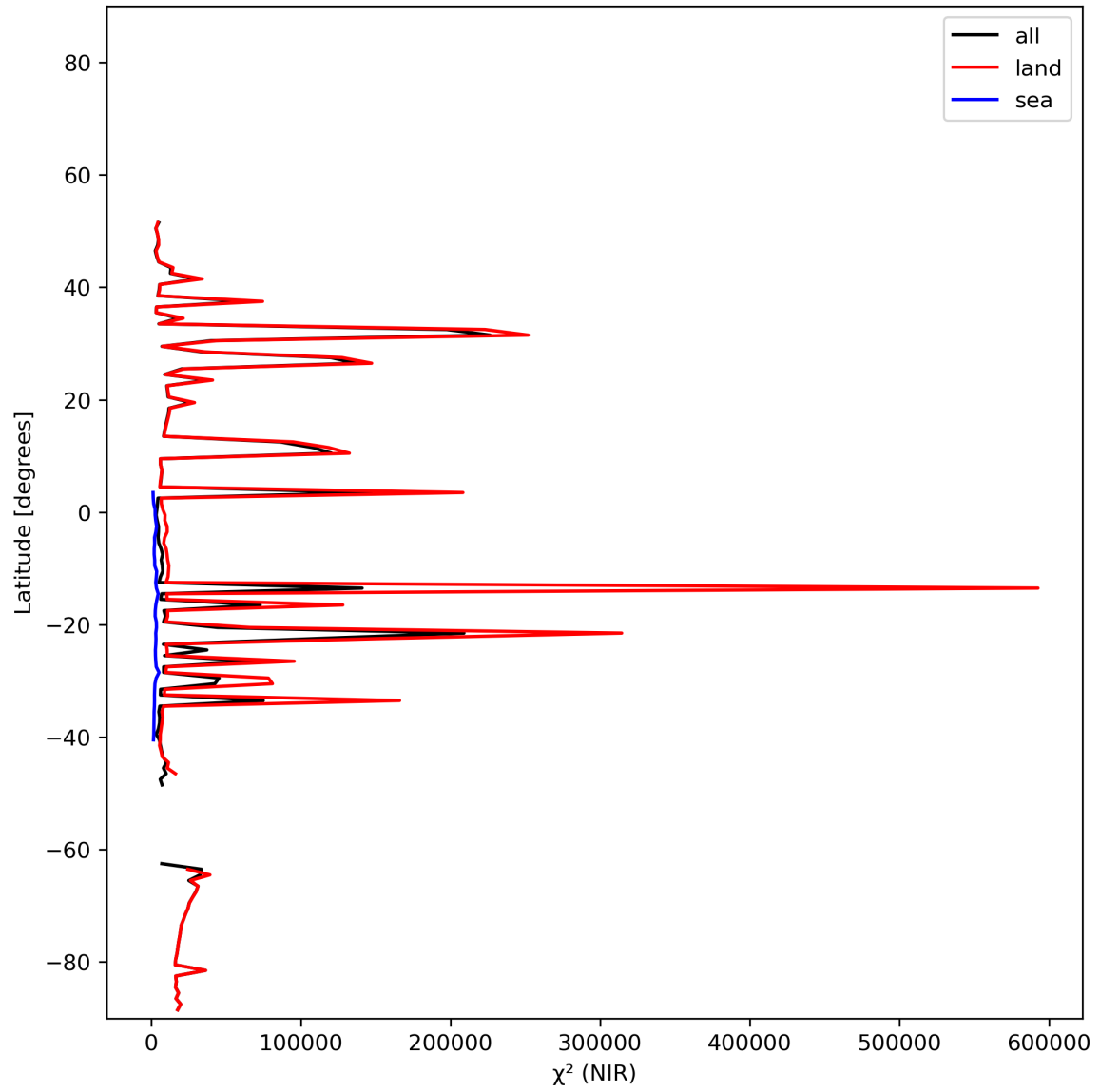
Figure 18: Zonal average of “ \chi^2 (NIR)” for 2023-12-28 to 2023-12-30.
