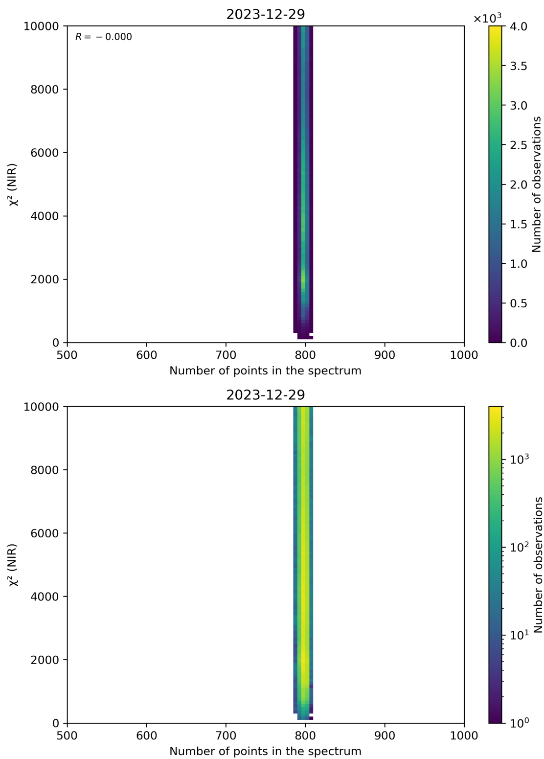
Figure 88: Scatter density plot of “Number of points in the spectrum” against “ \chi^2 (NIR)” for 2023-12-28 to 2023-12-30.
