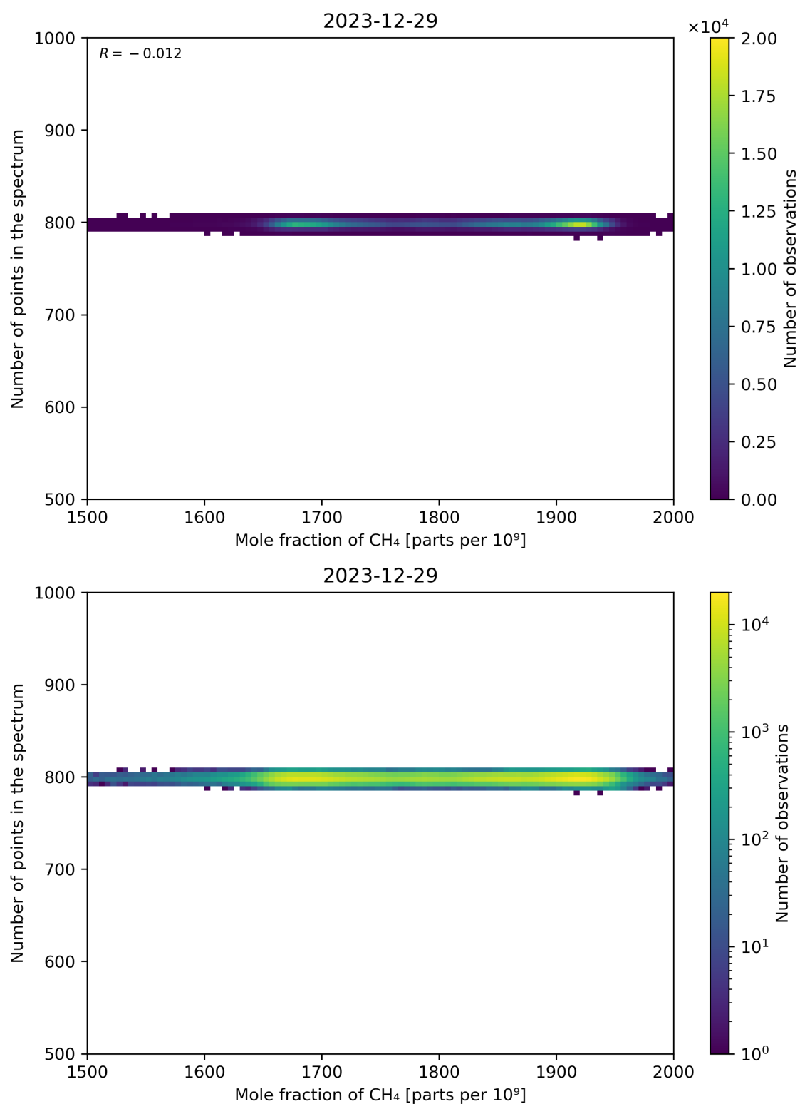
Figure 77: Scatter density plot of “Mole fraction of CH 4 ” against “Number of points in the spectrum” for 2023-12-28 to 2023-12-30.
