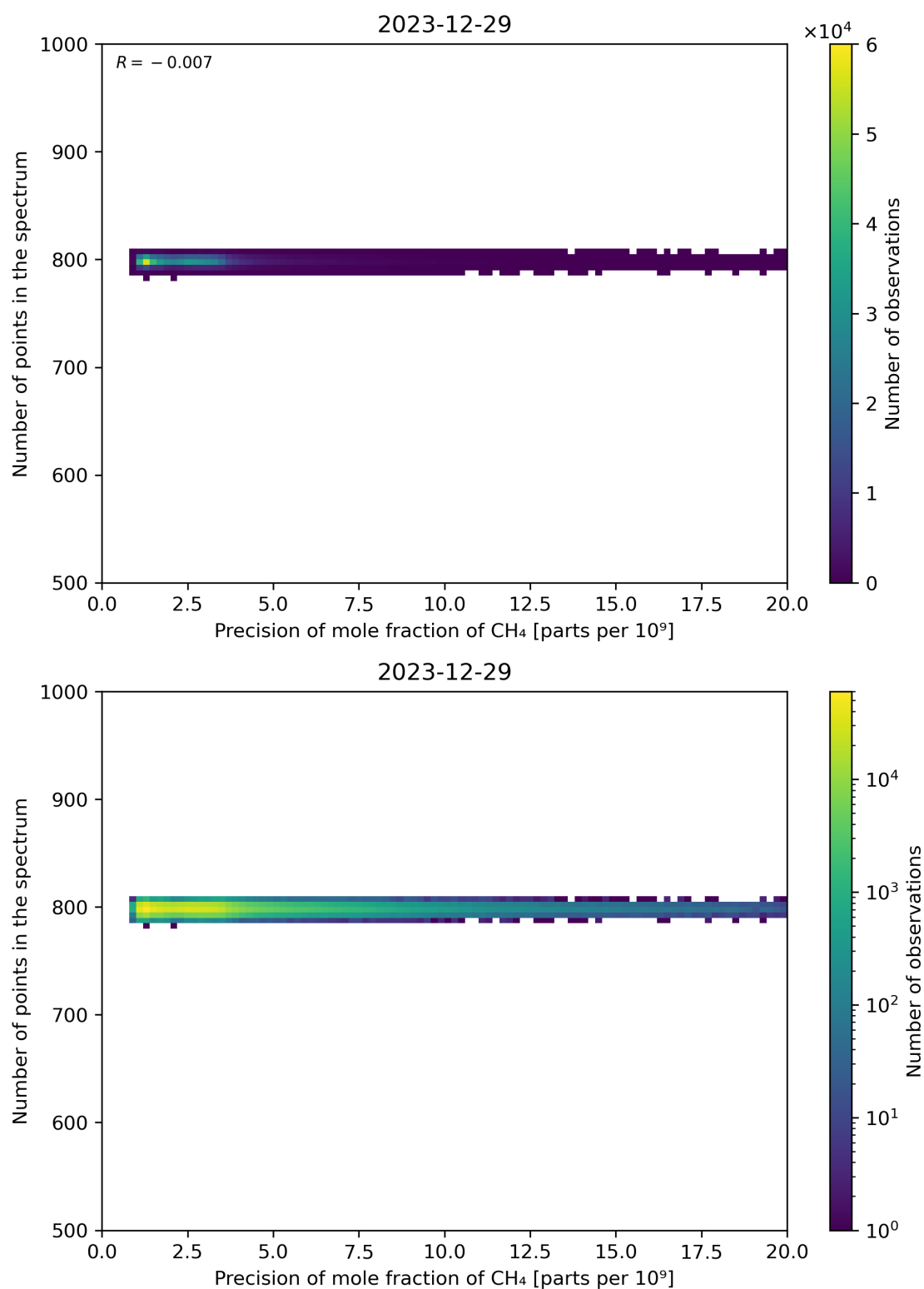
Figure 84: Scatter density plot of “Precision of mole fraction of CH 4 ” against “Number of points in the spectrum” for 2023-12-28 to 2023-12-30.
