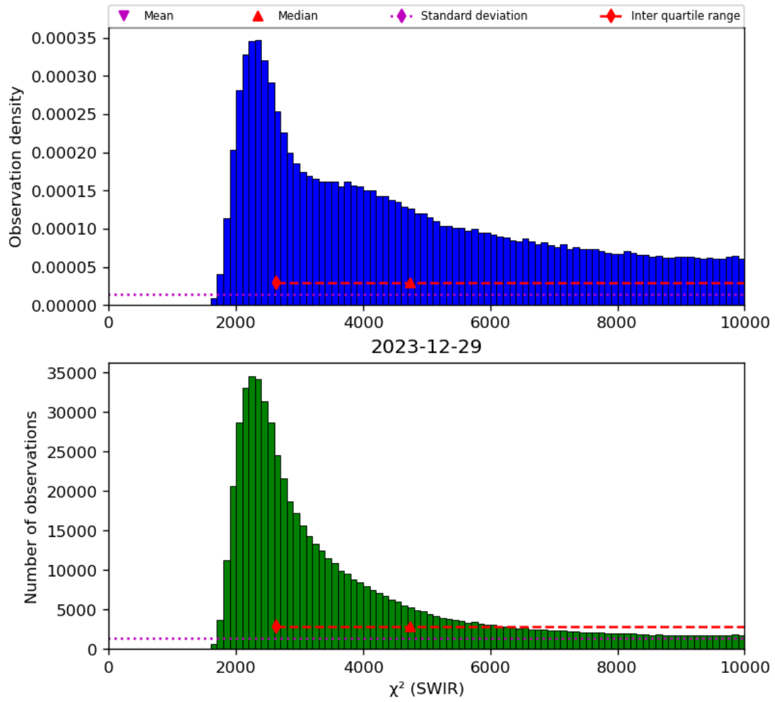
Figure 28: Histogram of “ \chi^2 (SWIR)” for 2023-12-28 to 2023-12-30
