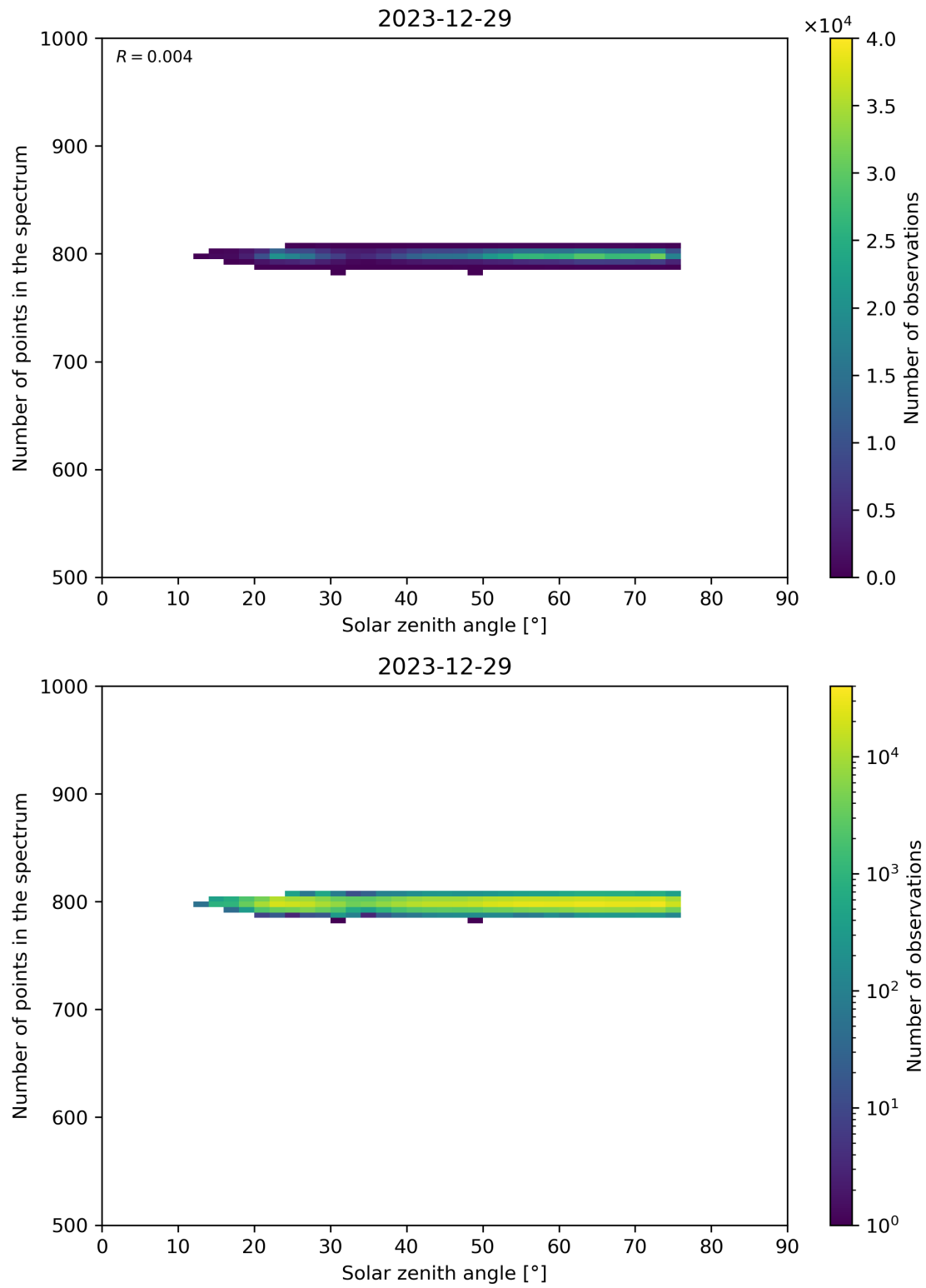
Figure 103: Scatter density plot of “Solar zenith angle” against “Number of points in the spectrum” for 2023-12-28 to 2023-12-30.
