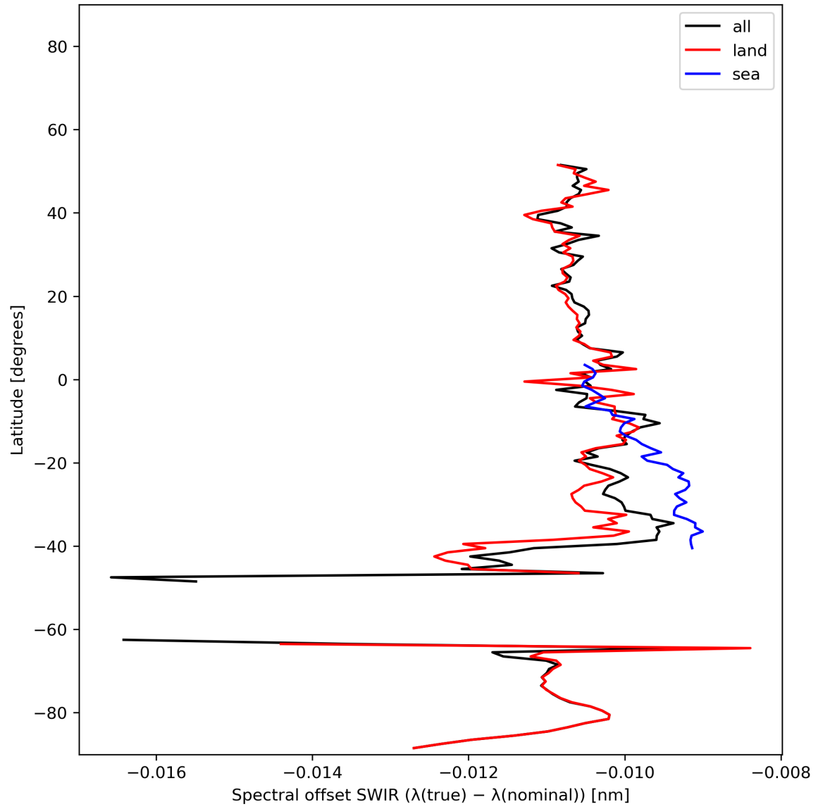
Figure 16: Zonal average of “Spectral offset SWIR ( \lambda(\text{true}) - \lambda(\text{nominal}) )” for 2023-12-28 to 2023-12-30.
