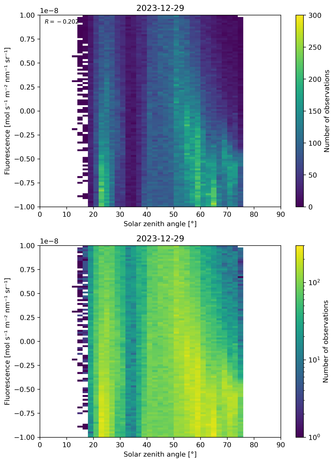
Figure 97: Scatter density plot of “Solar zenith angle” against “Fluorescence” for 2023-12-28 to 2023-12-30.
