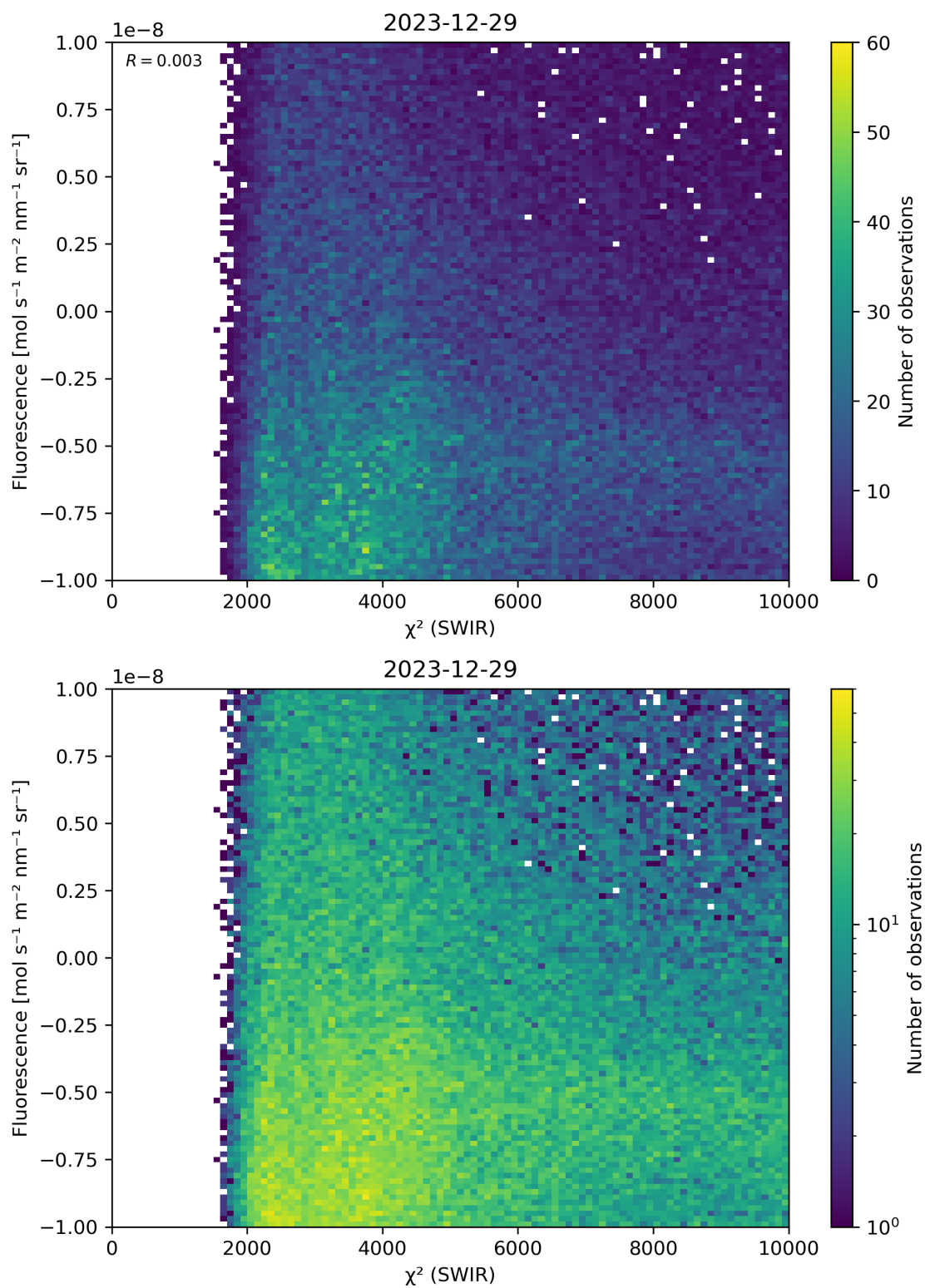
Figure 49: Scatter density plot of “ \chi^2 (SWIR)” against “Fluorescence” for 2023-12-28 to 2023-12-30.
