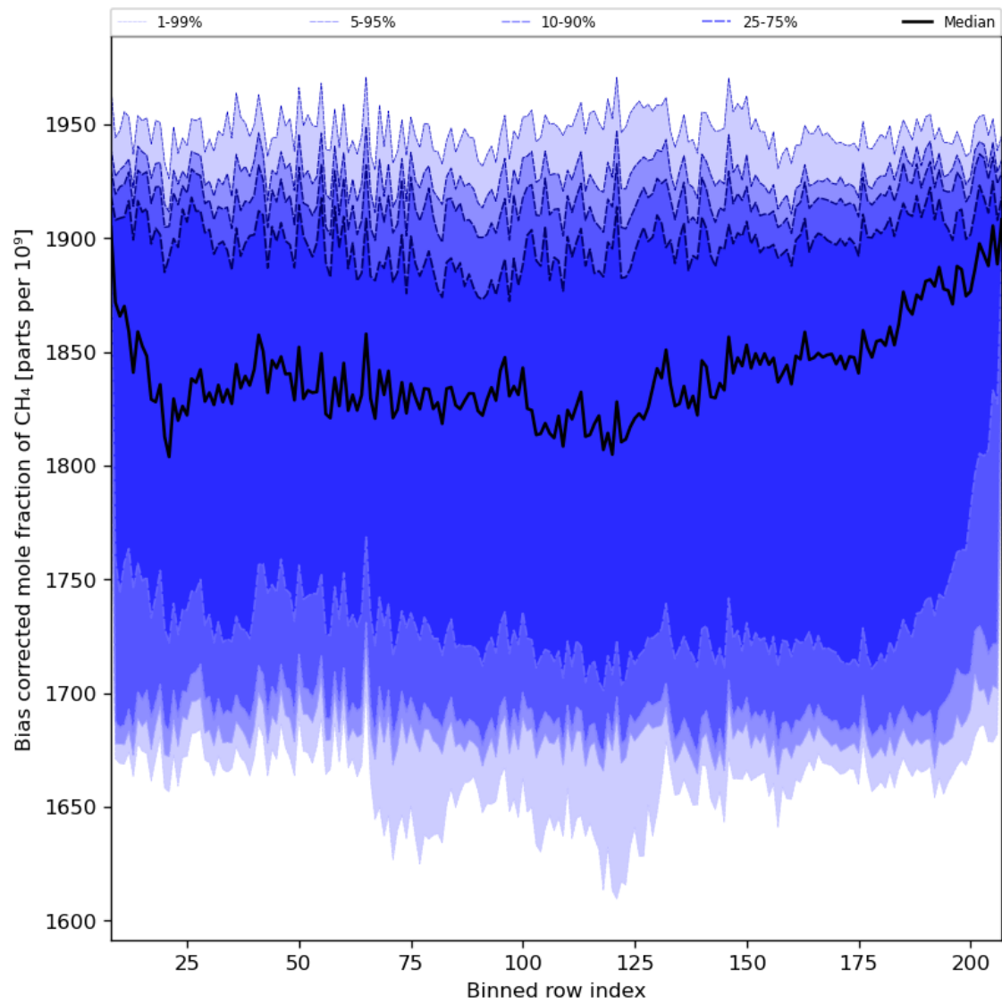
Figure 36: Along track statistics of “Bias corrected mole fraction of CH 4 ” for 2023-12-28 to 2023-12-30
