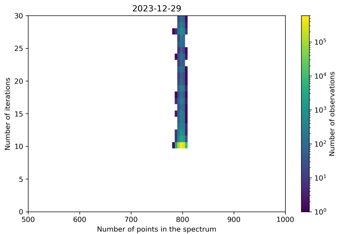
Figure 92: Scatter density plot of “Number of points in the spectrum” against “Number of iterations” for 2023-12-28 to 2023-12-30.
