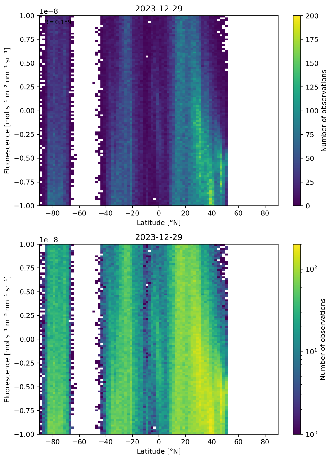
Figure 56: Scatter density plot of “Latitude” against “Fluorescence” for 2023-12-28 to 2023-12-30.
