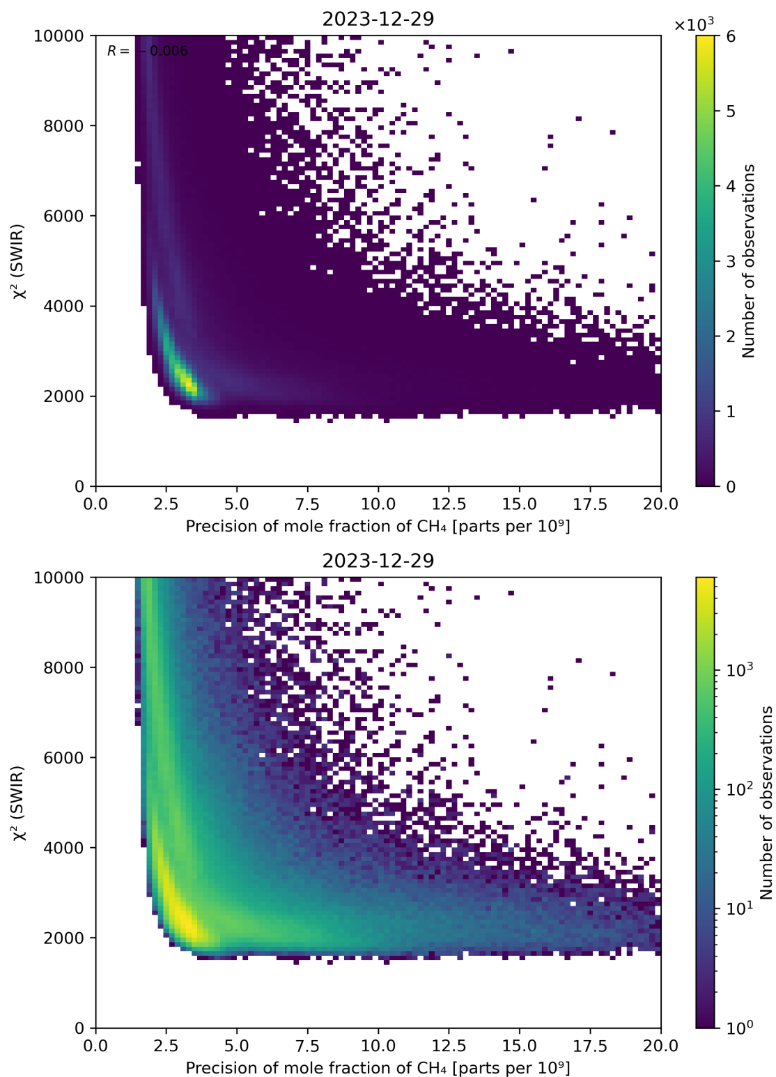
Figure 79: Scatter density plot of “Precision of mole fraction of \text{CH}_4 ” against “ \chi^2 (SWIR)” for 2023-12-28 to 2023-12-30.
