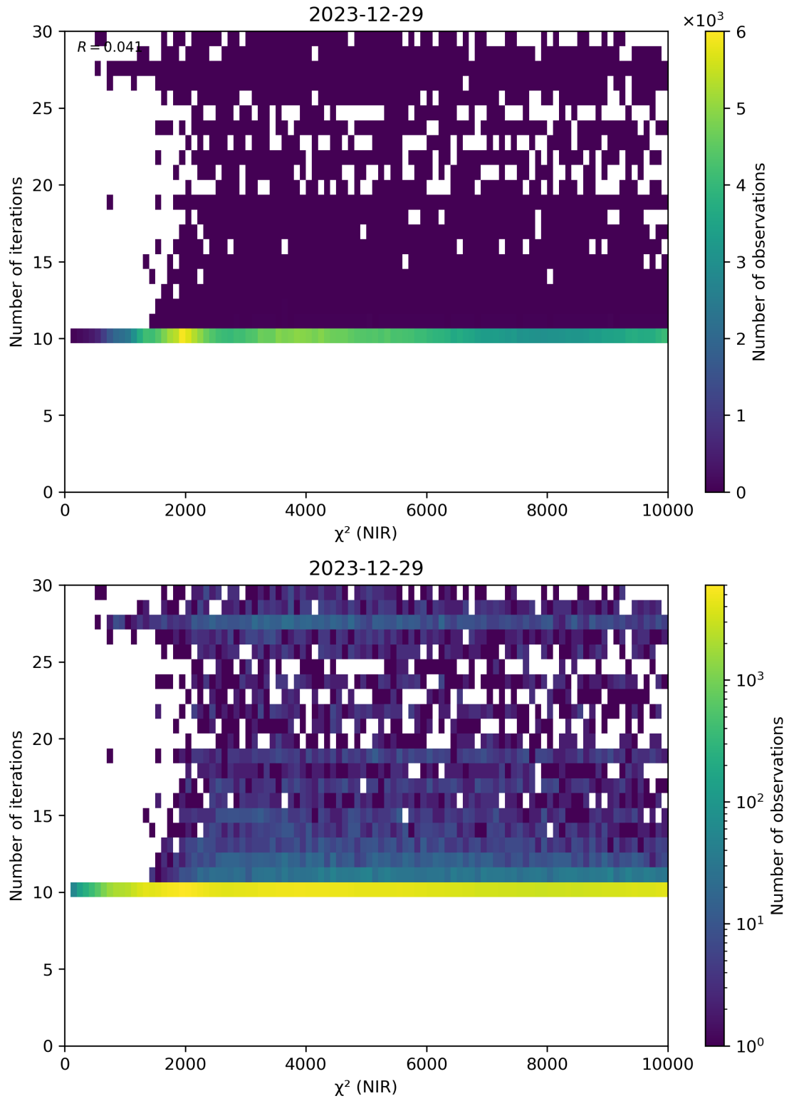
Figure 46: Scatter density plot of “ \chi^2 (NIR)” against “Number of iterations” for 2023-12-28 to 2023-12-30.
