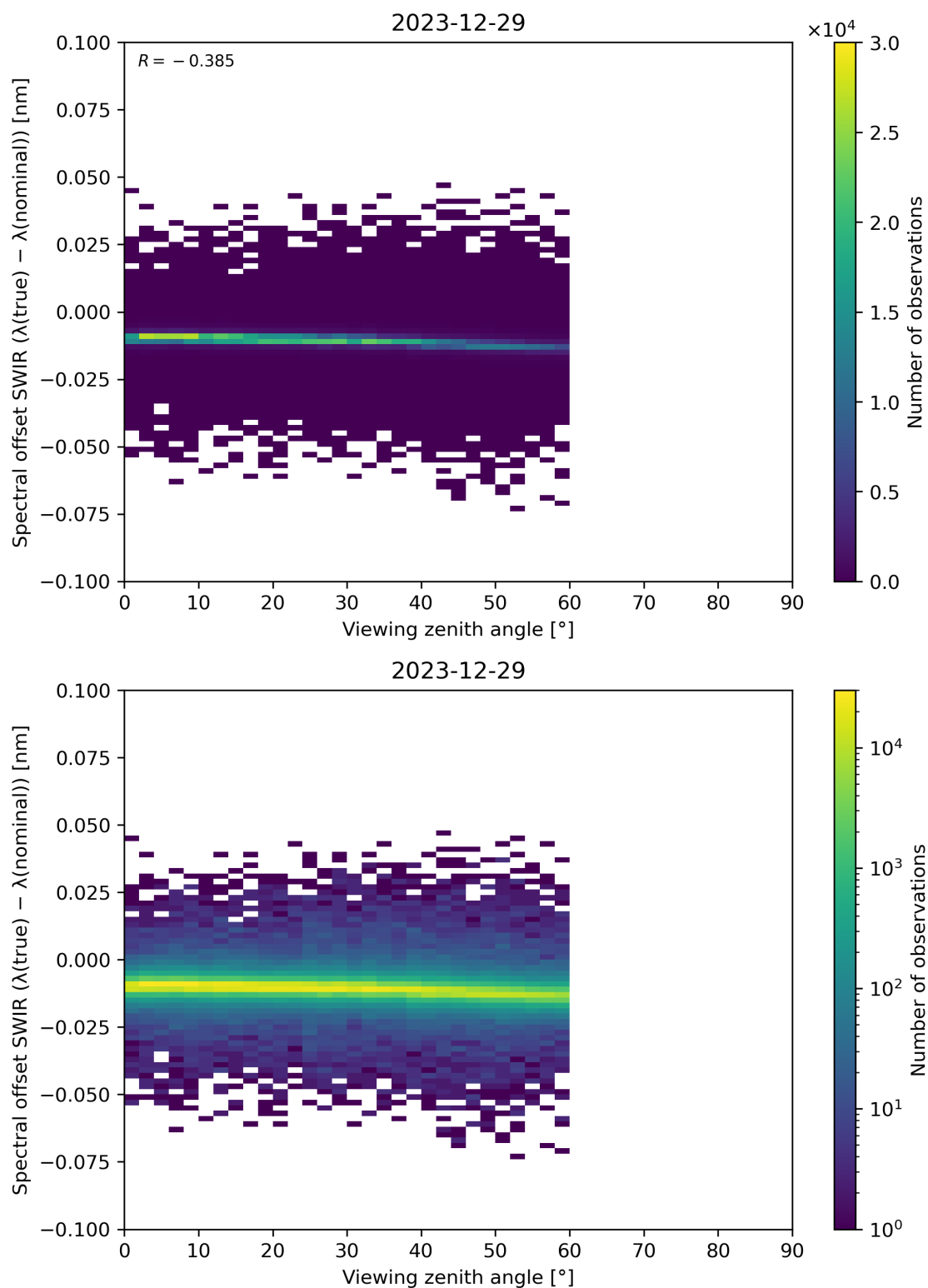
Figure 116: Scatter density plot of “Viewing zenith angle” against “Spectral offset SWIR ( \lambda(\text{true}) - \lambda(\text{nominal}) )” for 2023-12-28 to 2023-12-30.
