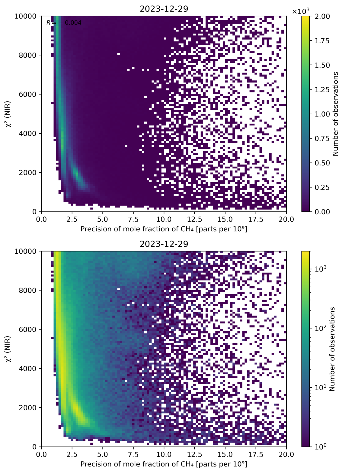
Figure 78: Scatter density plot of “Precision of mole fraction of CH 4 ” against “ \chi^2 (NIR)” for 2023-12-28 to 2023-12-30.
