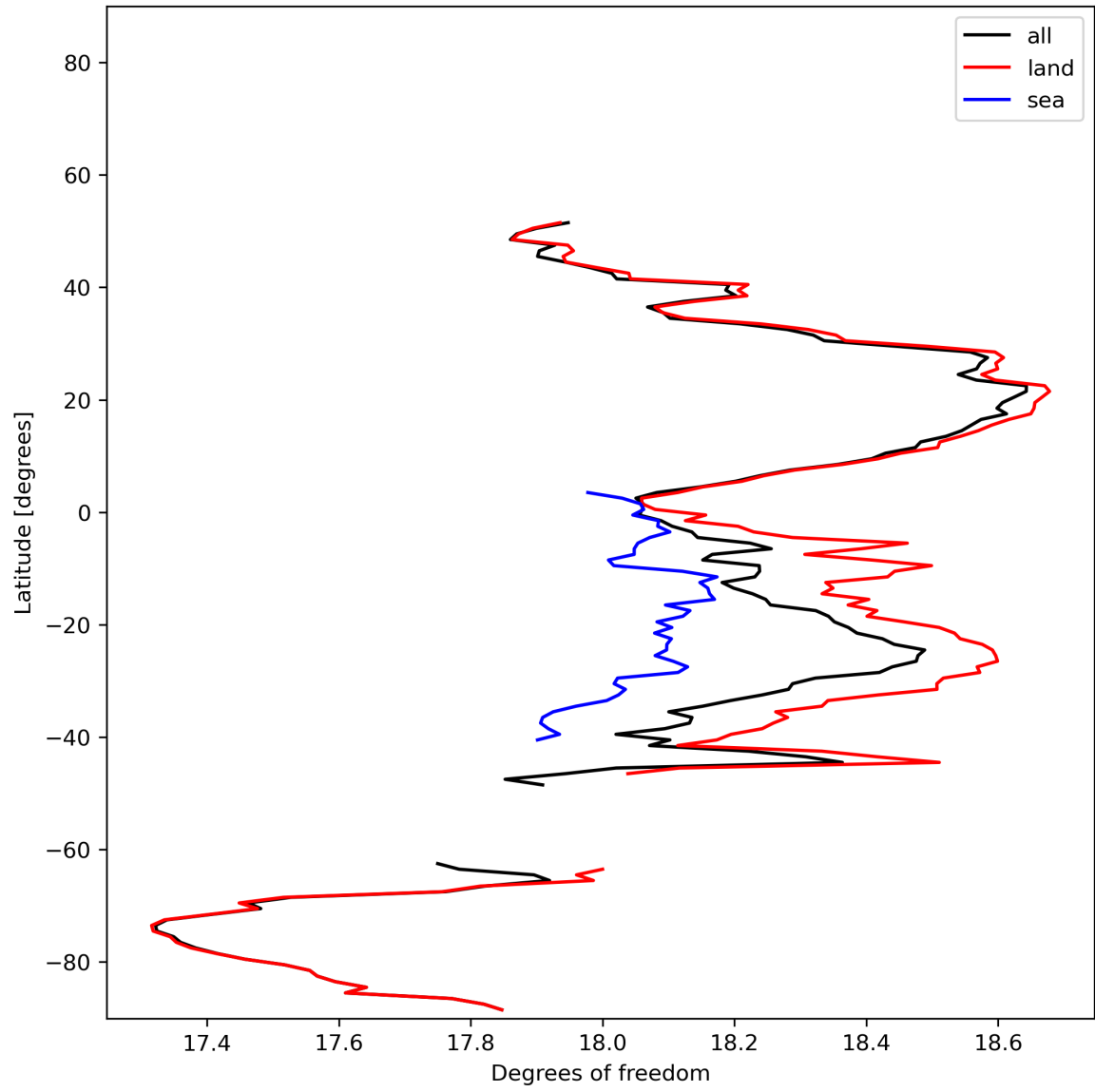
Figure 19: Zonal average of “Degrees of freedom” for 2023-12-28 to 2023-12-30.
