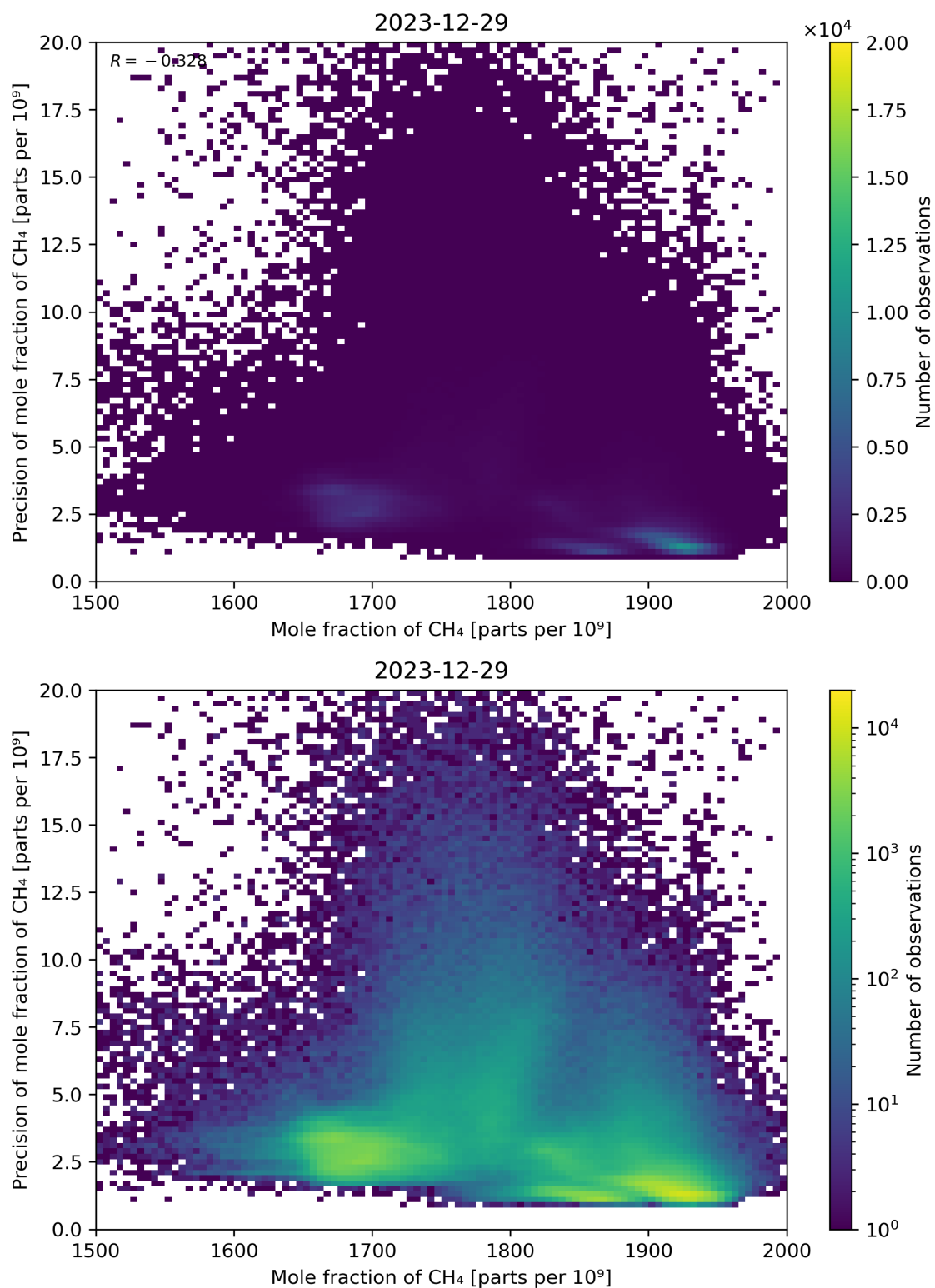
Figure 75: Scatter density plot of “Mole fraction of CH 4 ” against “Precision of mole fraction of CH 4 ” for 2023-12-28 to 2023-12-30.
