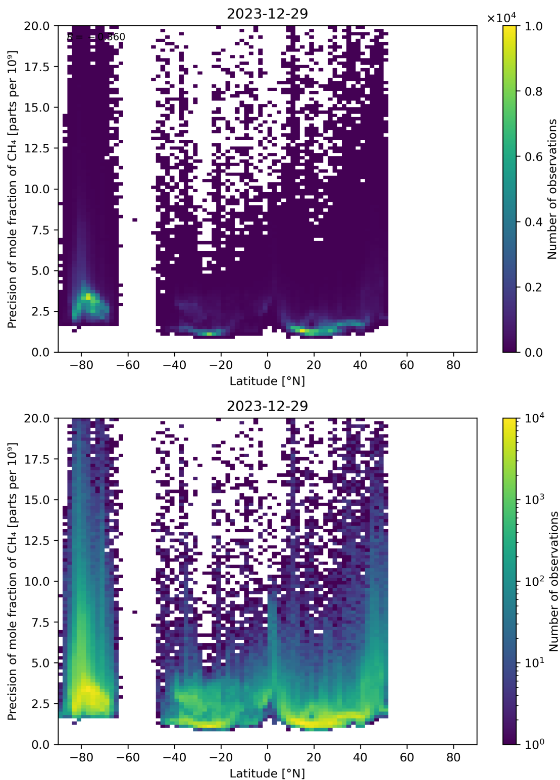
Figure 59: Scatter density plot of “Latitude” against “Precision of mole fraction of CH 4 ” for 2023-12-28 to 2023-12-30.
