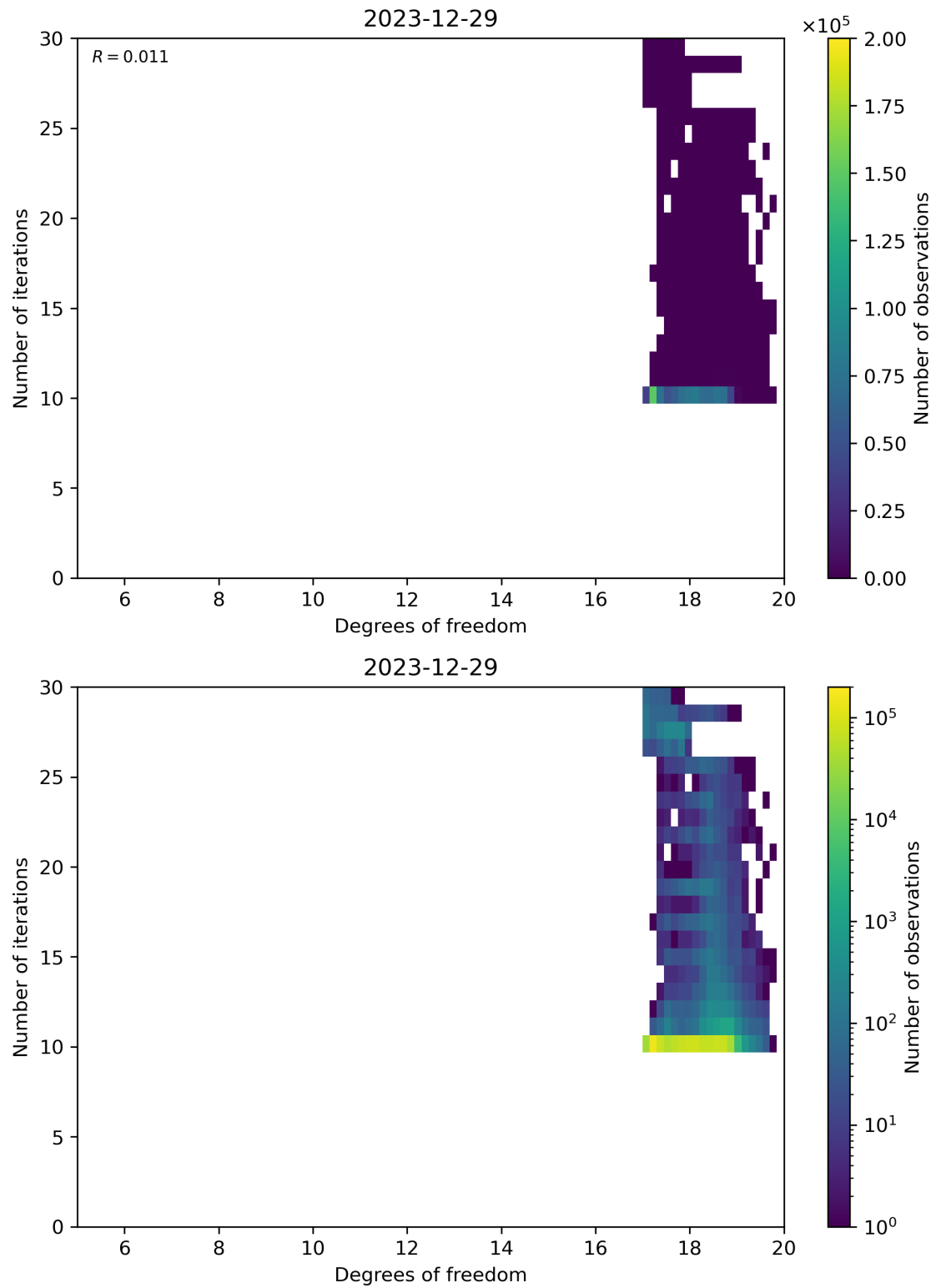
Figure 52: Scatter density plot of “Degrees of freedom” against “Number of iterations” for 2023-12-28 to 2023-12-30.
