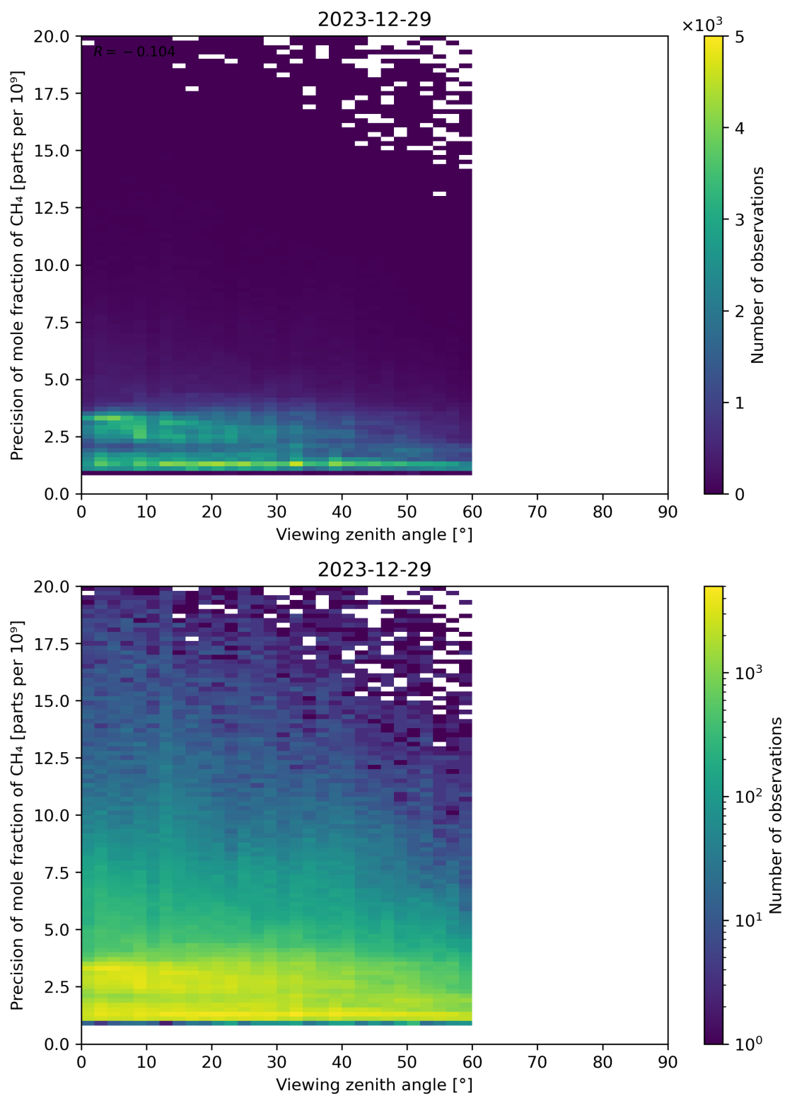
Figure 112: Scatter density plot of “Viewing zenith angle” against “Precision of mole fraction of CH 4 ” for 2023-12-28 to 2023-12-30.
