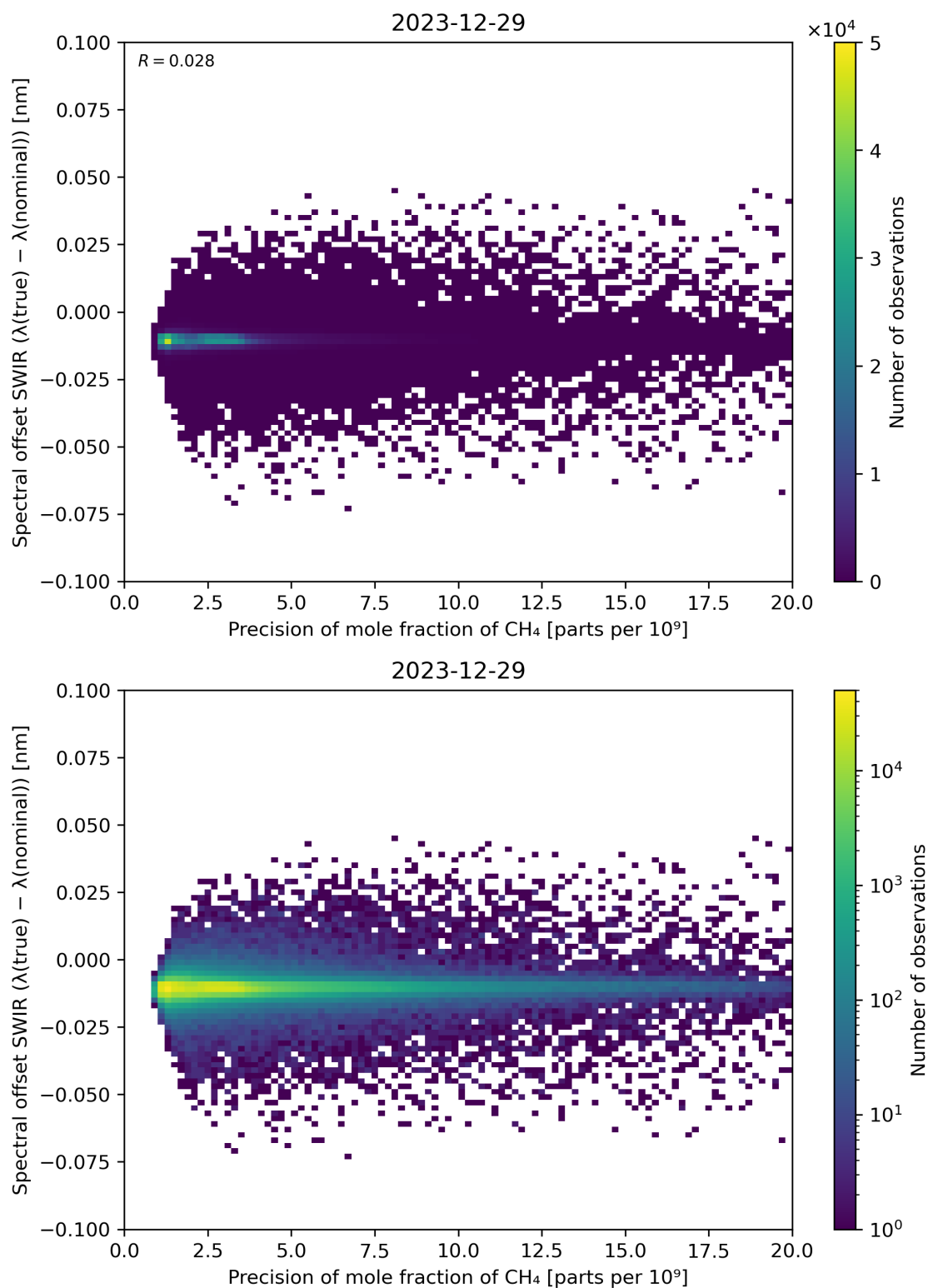
Figure 85: Scatter density plot of “Precision of mole fraction of CH 4 ” against “Spectral offset SWIR ( \lambda(\text{true}) - \lambda(\text{nominal}) )” for 2023-12-28 to 2023-12-30.
