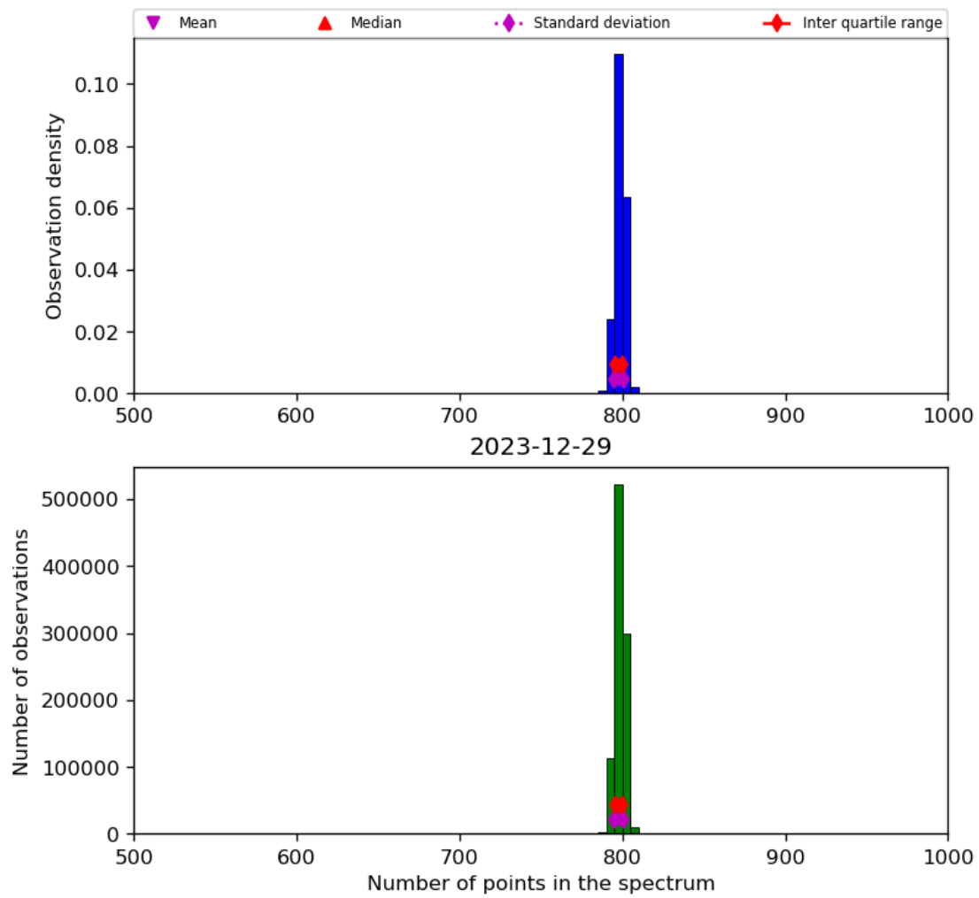
Figure 26: Histogram of “Number of points in the spectrum” for 2023-12-28 to 2023-12-30
