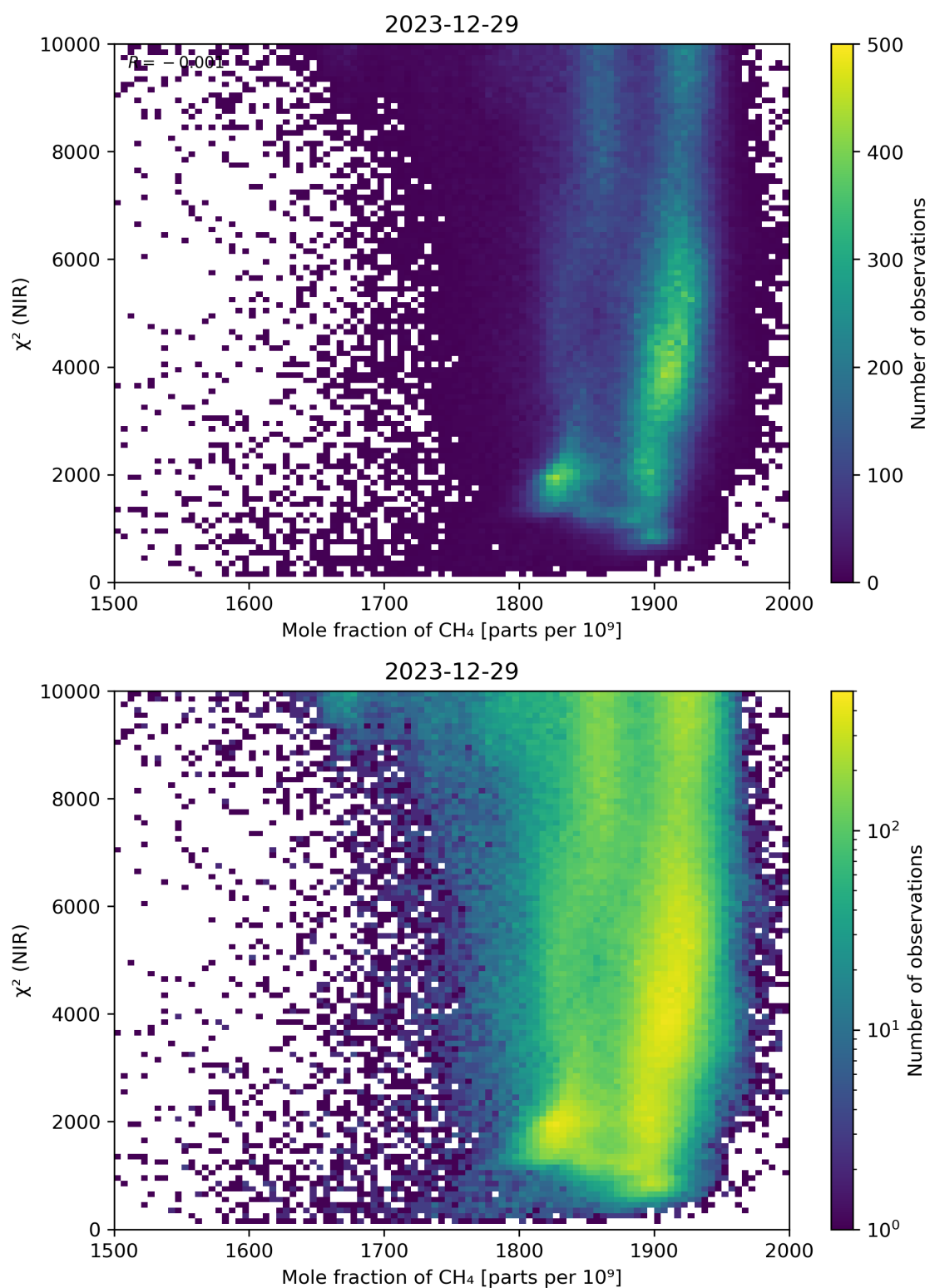
Figure 70: Scatter density plot of “Mole fraction of \text{CH}_4 ” against “ \chi^2 (NIR)” for 2023-12-28 to 2023-12-30.
