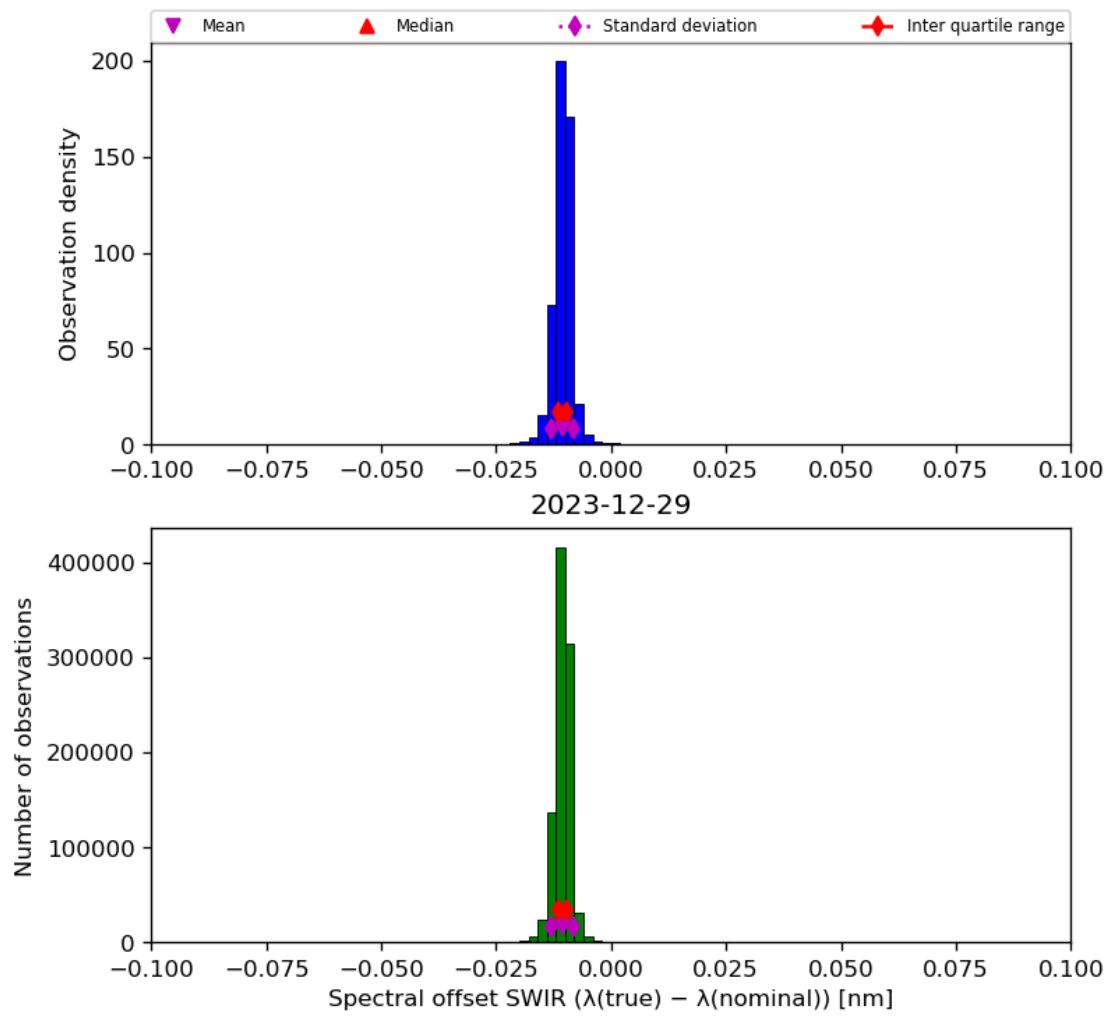
Figure 27: Histogram of “Spectral offset SWIR ( \lambda(\text{true}) - \lambda(\text{nominal}) )” for 2023-12-28 to 2023-12-30
