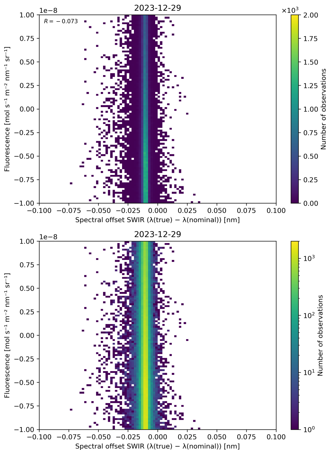
Figure 120: Scatter density plot of “Spectral offset SWIR ( \lambda(\text{true}) - \lambda(\text{nominal}) )” against “Fluorescence” for 2023-12-28 to 2023-12-30.
