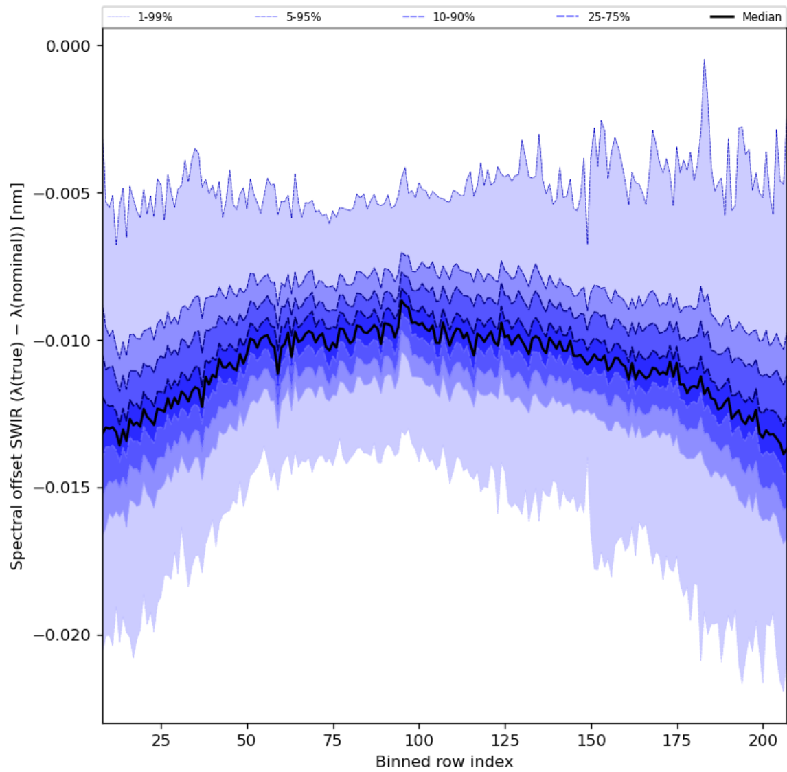
Figure 38: Along track statistics of “Spectral offset SWIR ( \lambda(\text{true}) - \lambda(\text{nominal}) )” for 2023-12-28 to 2023-12-30
