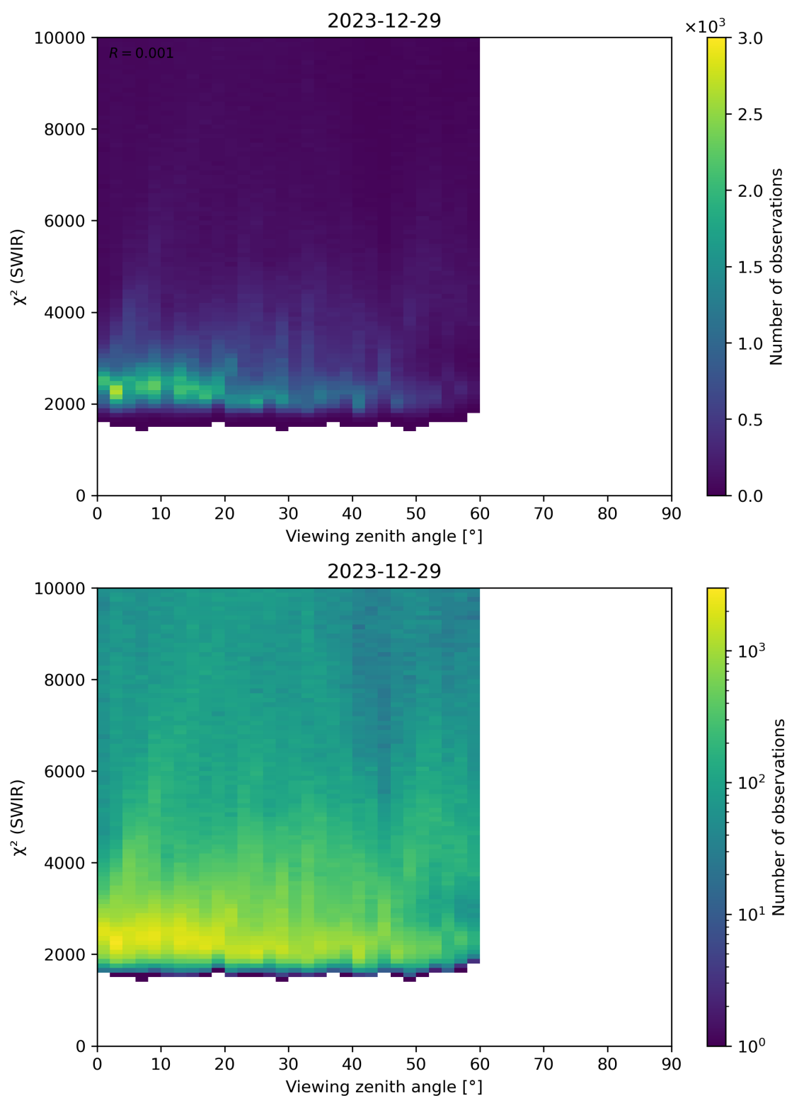
Figure 106: Scatter density plot of “Viewing zenith angle” against “ \chi^2 (SWIR)” for 2023-12-28 to 2023-12-30.
