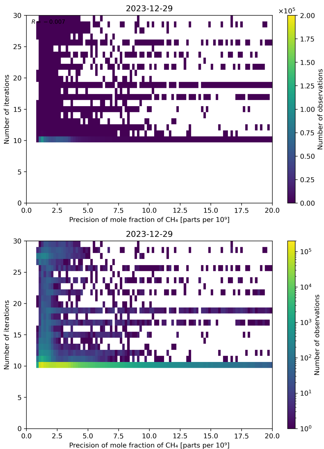
Figure 83: Scatter density plot of “Precision of mole fraction of CH 4 ” against “Number of iterations” for 2023-12-28 to 2023-12-30.
