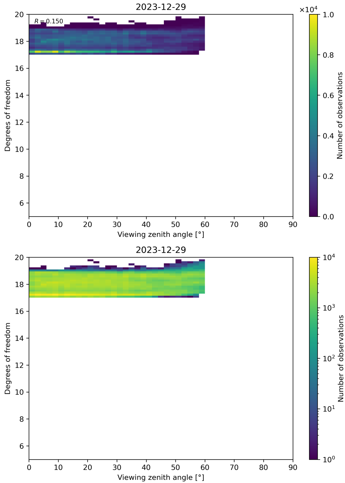
Figure 107: Scatter density plot of “Viewing zenith angle” against “Degrees of freedom” for 2023-12-28 to 2023-12-30.
