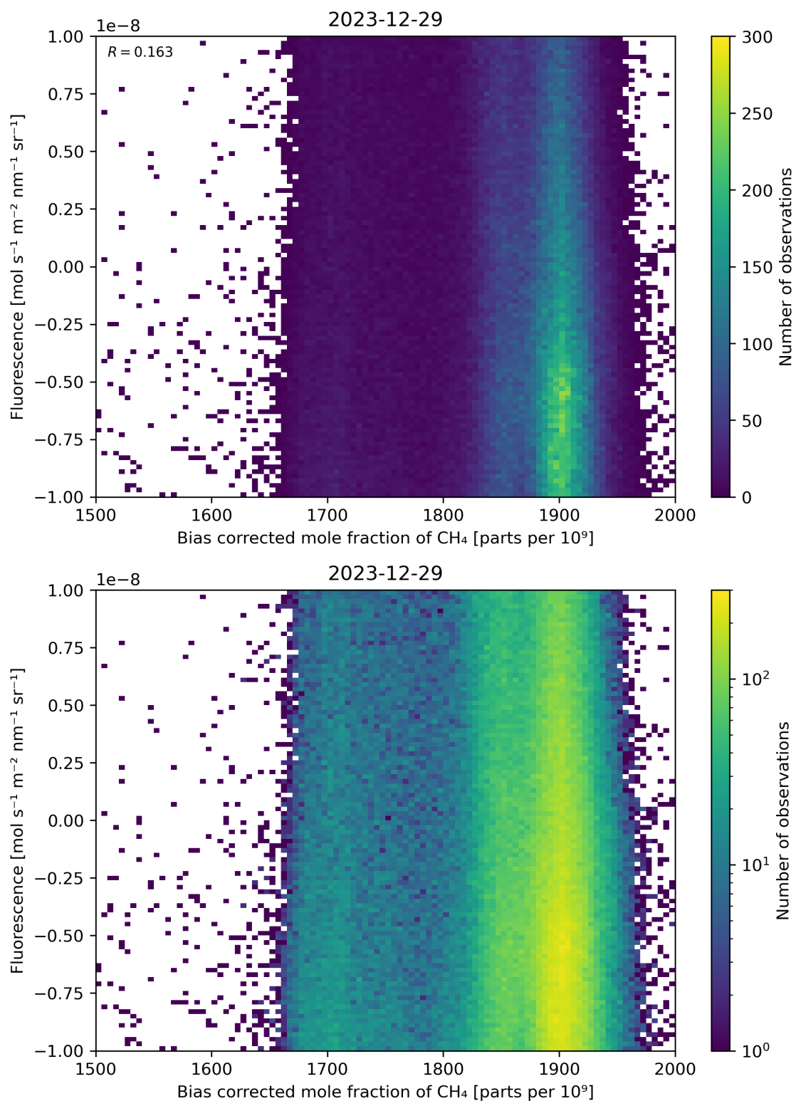
Figure 66: Scatter density plot of “Bias corrected mole fraction of \text{CH}_4 ” against “Fluorescence” for 2023-12-28 to 2023-12-30.
