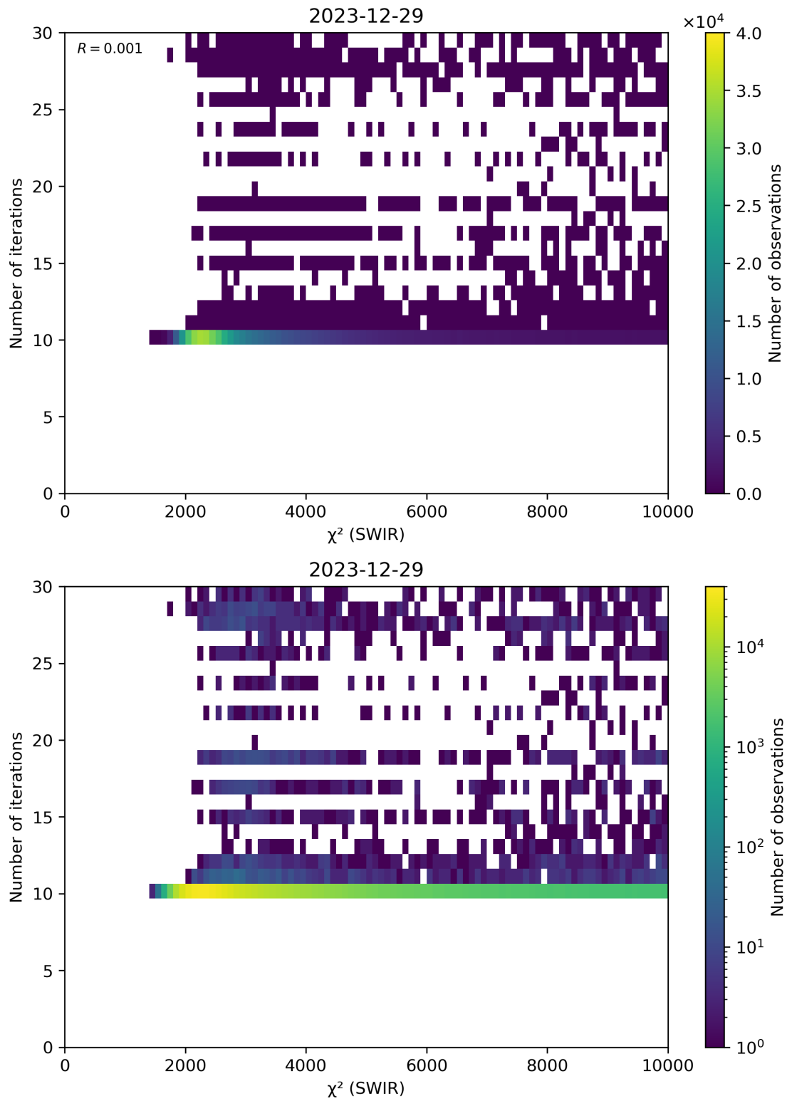
Figure 50: Scatter density plot of “ \chi^2 (SWIR)” against “Number of iterations” for 2023-12-28 to 2023-12-30.
