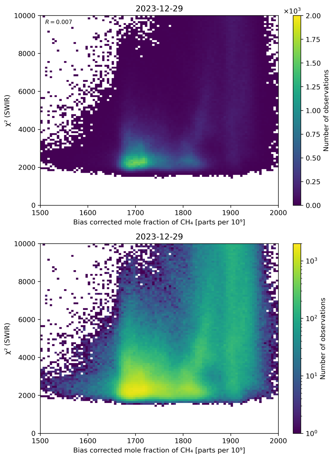
Figure 64: Scatter density plot of “Bias corrected mole fraction of \text{CH}_4 ” against “ \chi^2 (SWIR)” for 2023-12-28 to 2023-12-30.
