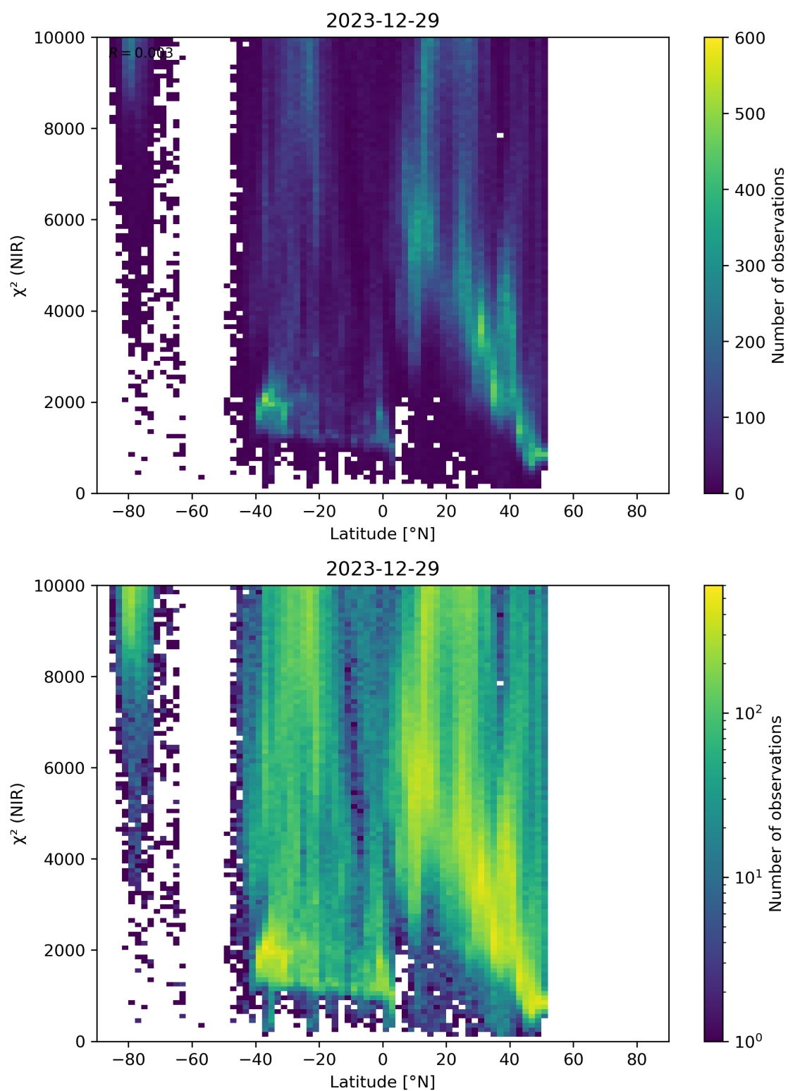
Figure 53: Scatter density plot of “Latitude” against “ \chi^2 (NIR)” for 2023-12-28 to 2023-12-30.
