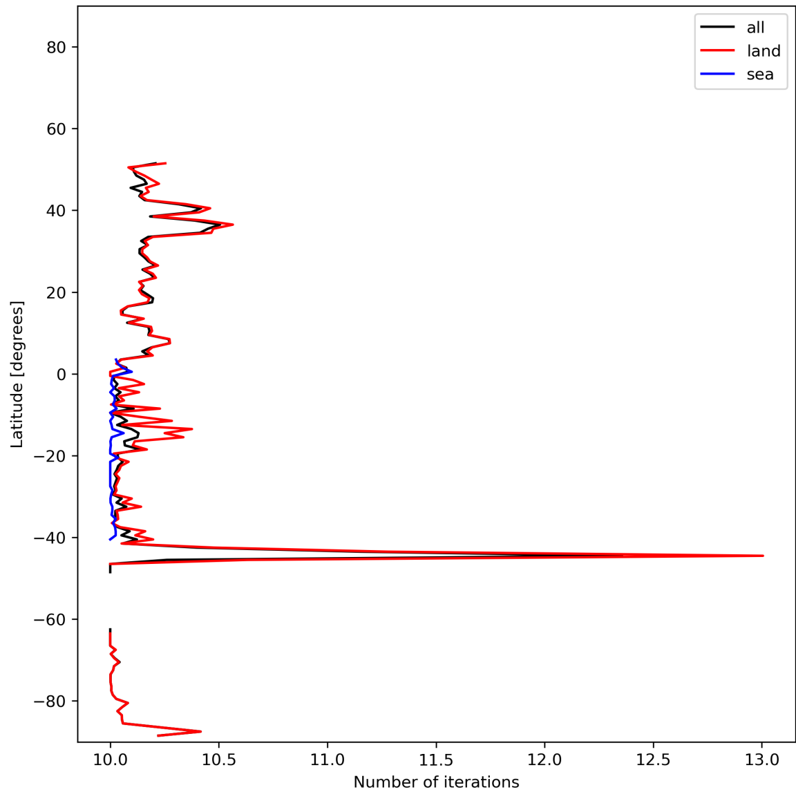
Figure 20: Zonal average of “Number of iterations” for 2023-12-28 to 2023-12-30.
