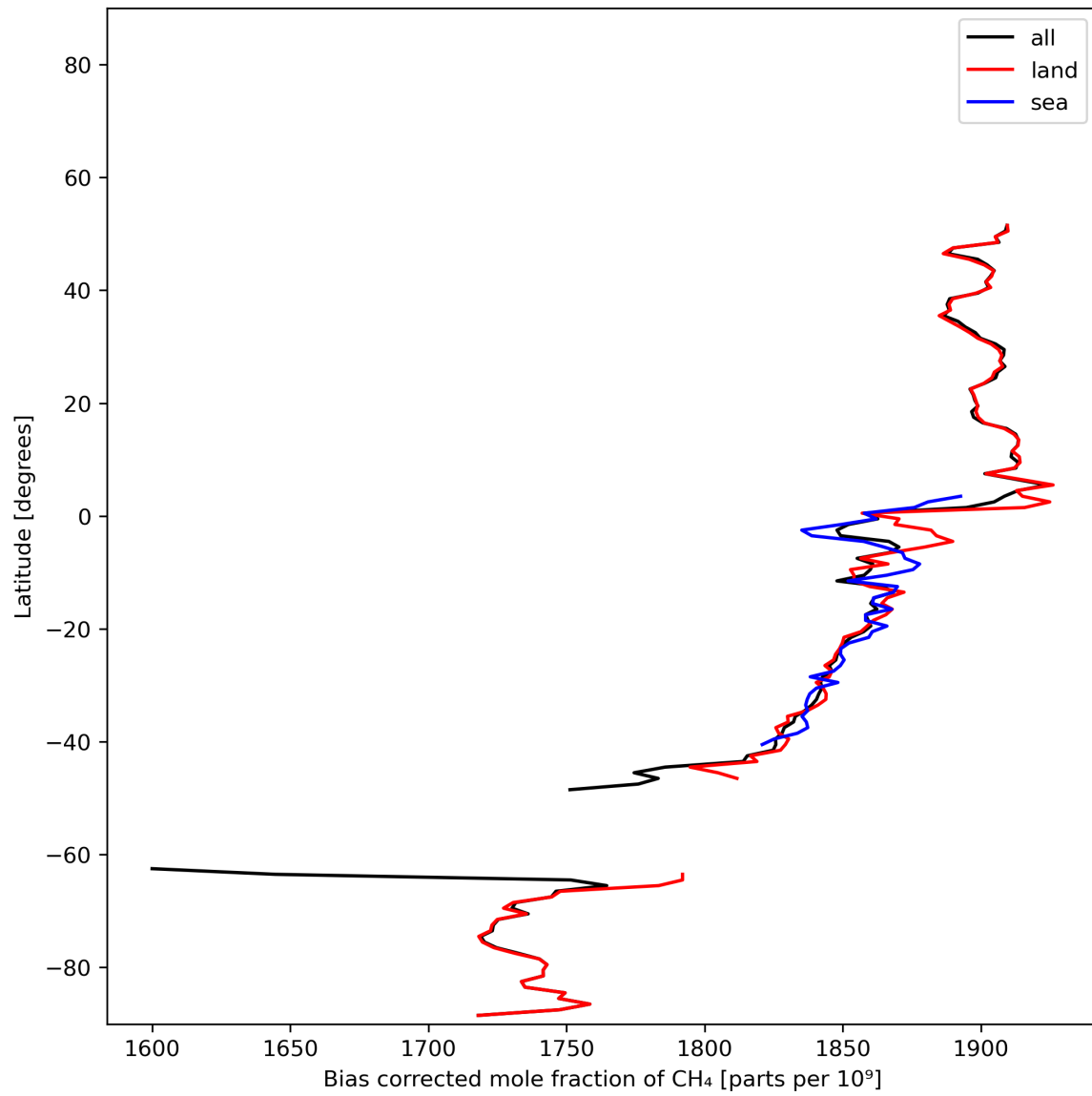
Figure 14: Zonal average of “Bias corrected mole fraction of CH 4 ” for 2023-12-28 to 2023-12-30.
