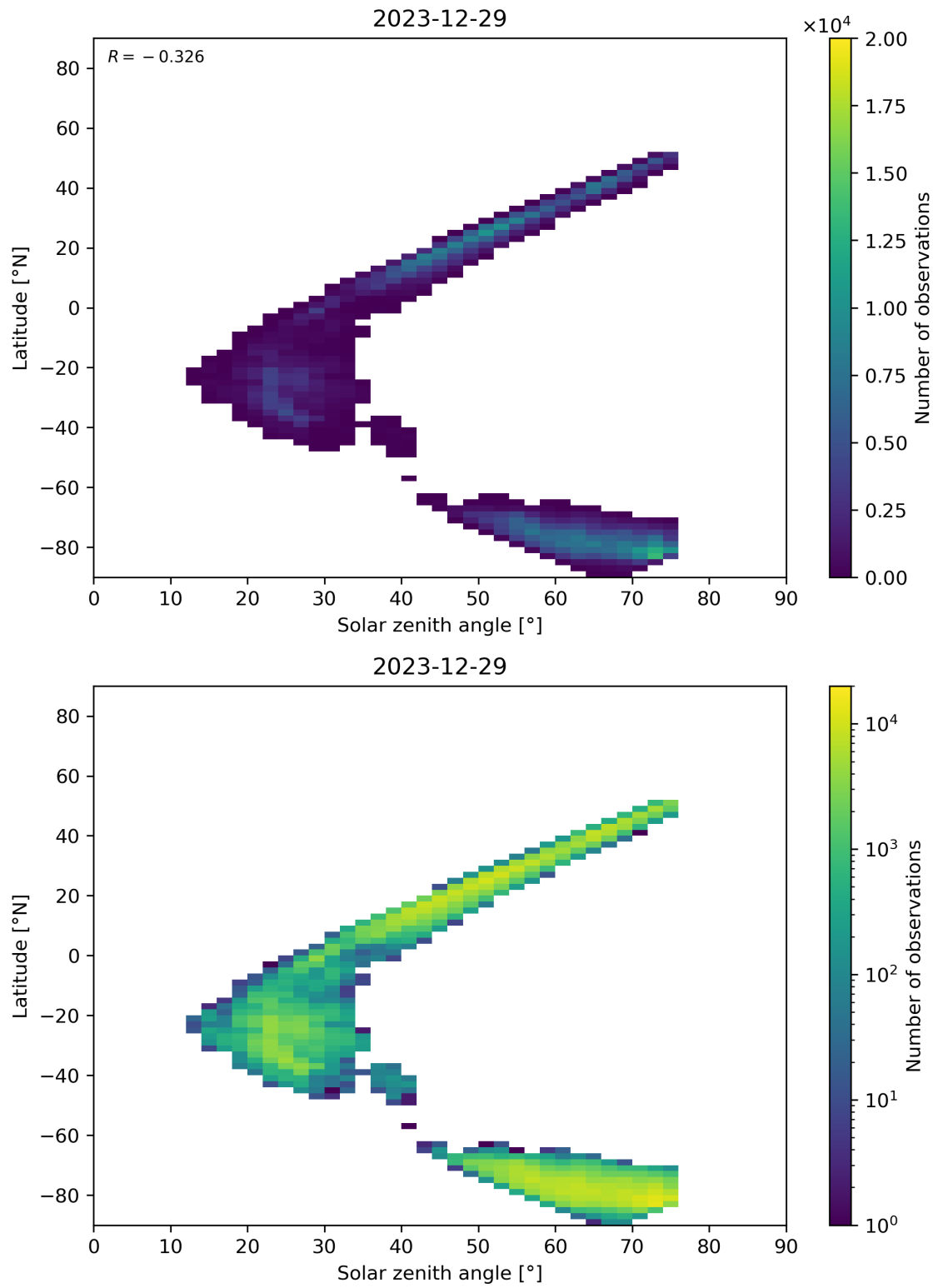
Figure 98: Scatter density plot of “Solar zenith angle” against “Latitude” for 2023-12-28 to 2023-12-30.
