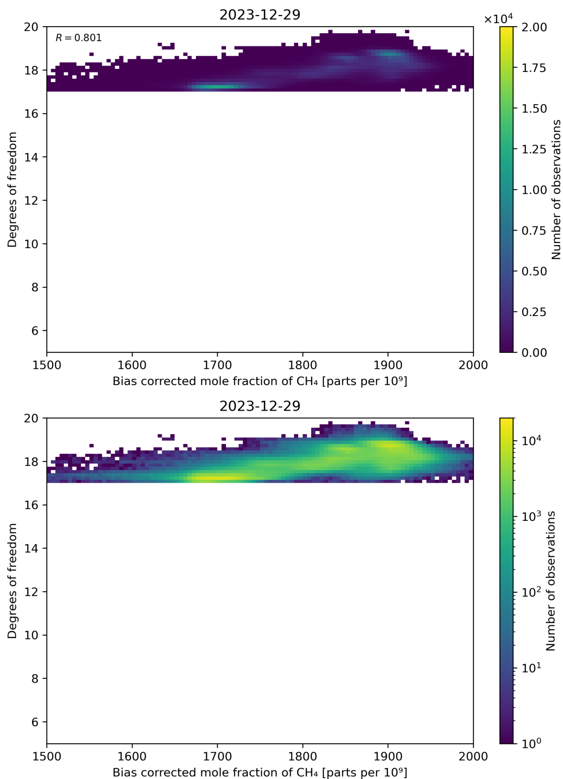
Figure 65: Scatter density plot of “Bias corrected mole fraction of CH 4 ” against “Degrees of freedom” for 2023-12-28 to 2023-12-30.
