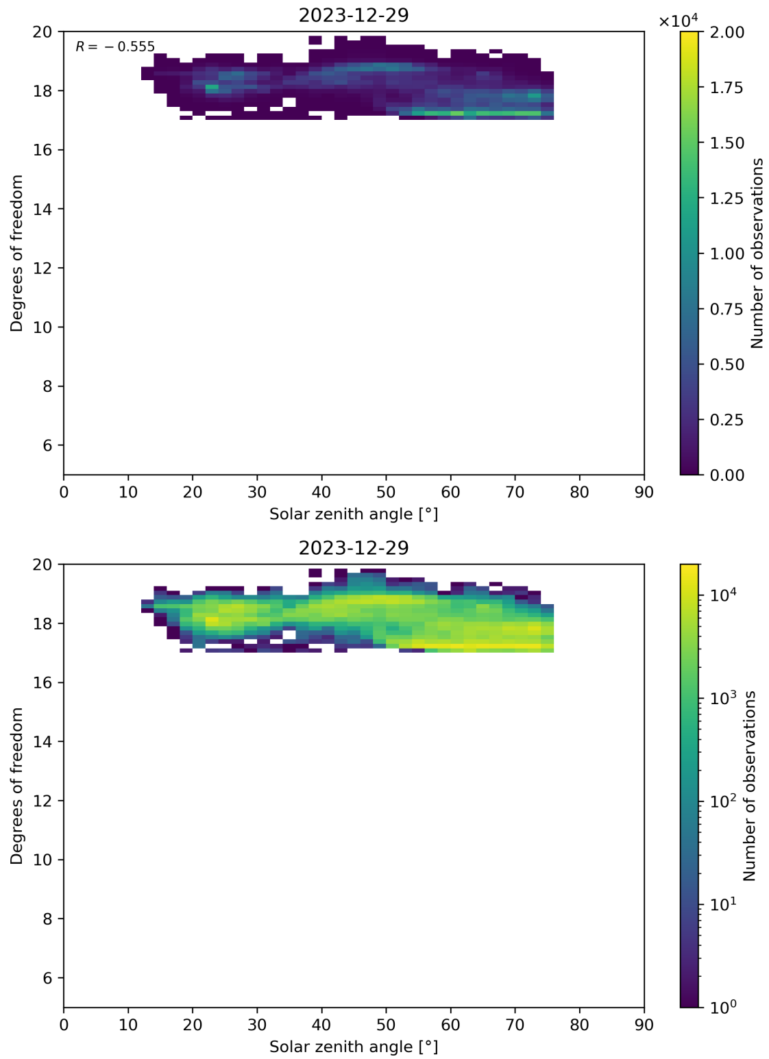
Figure 96: Scatter density plot of “Solar zenith angle” against “Degrees of freedom” for 2023-12-28 to 2023-12-30.
