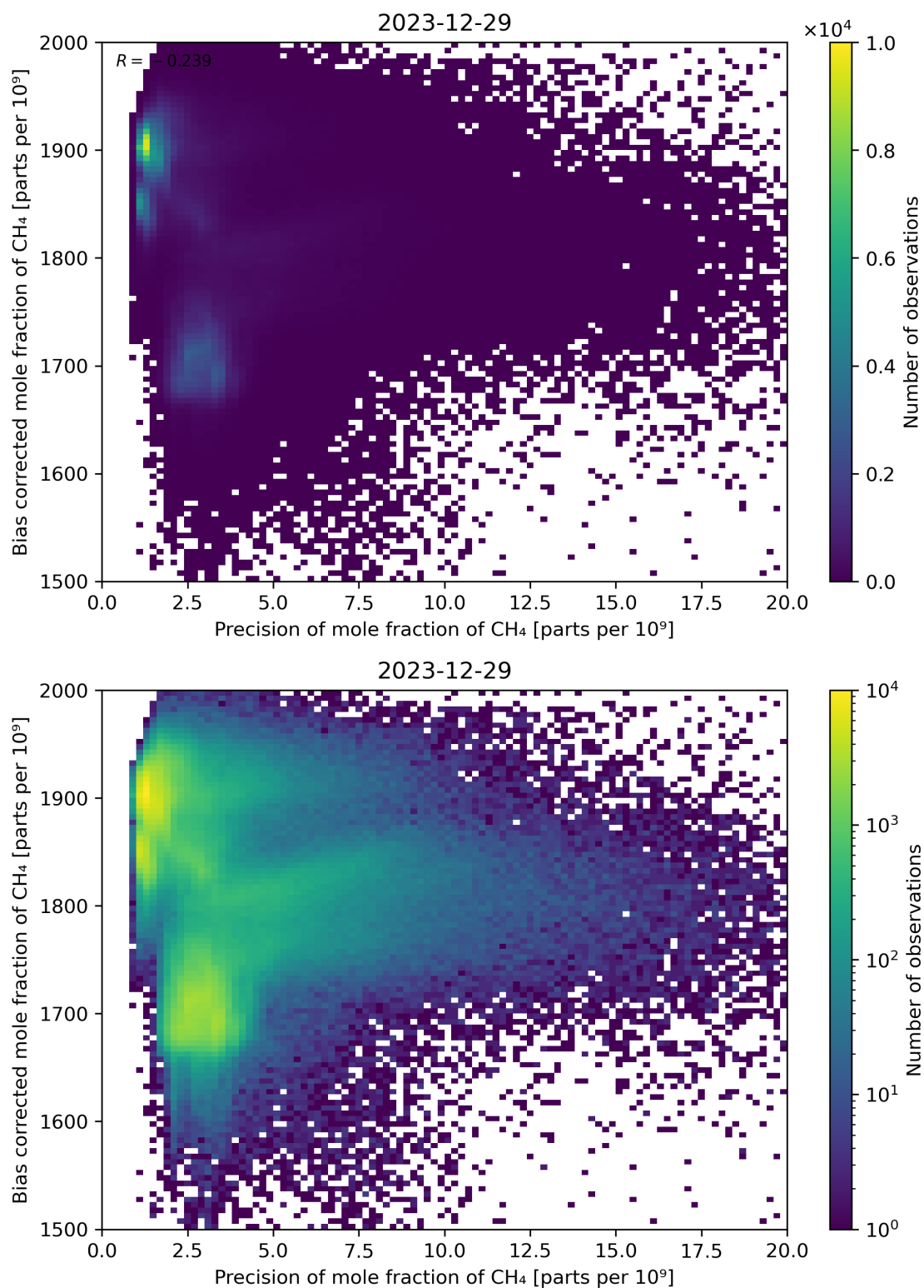
Figure 82: Scatter density plot of “Precision of mole fraction of \text{CH}_4 ” against “Bias corrected mole fraction of \text{CH}_4 ” for 2023-12-28 to 2023-12-30.
