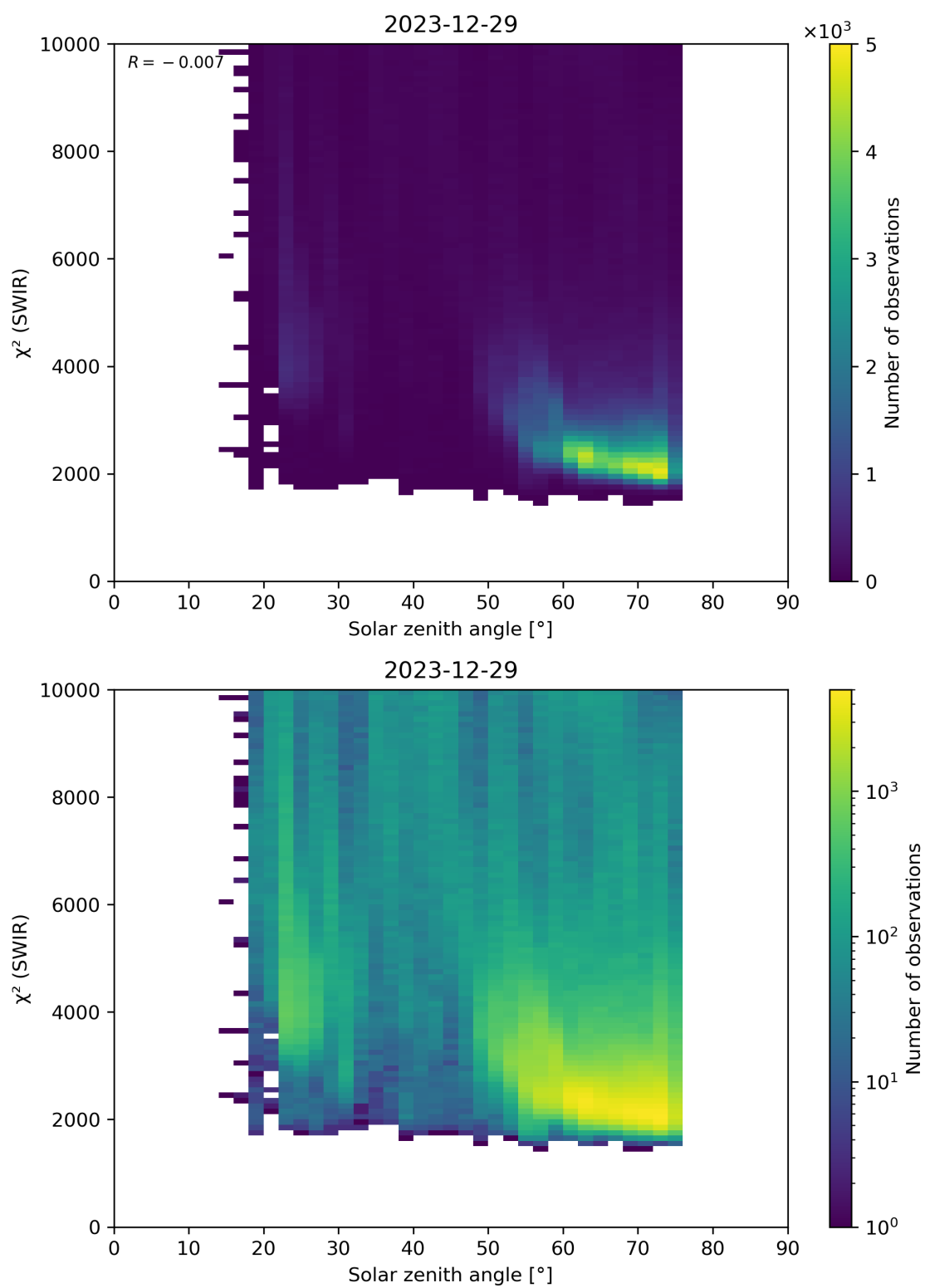
Figure 95: Scatter density plot of “Solar zenith angle” against “ \chi^2 (SWIR)” for 2023-12-28 to 2023-12-30.
