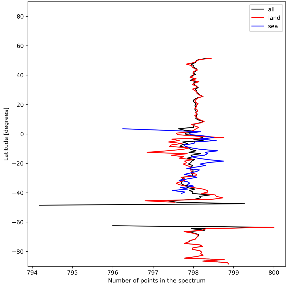
Figure 15: Zonal average of “Number of points in the spectrum” for 2023-12-28 to 2023-12-30.
