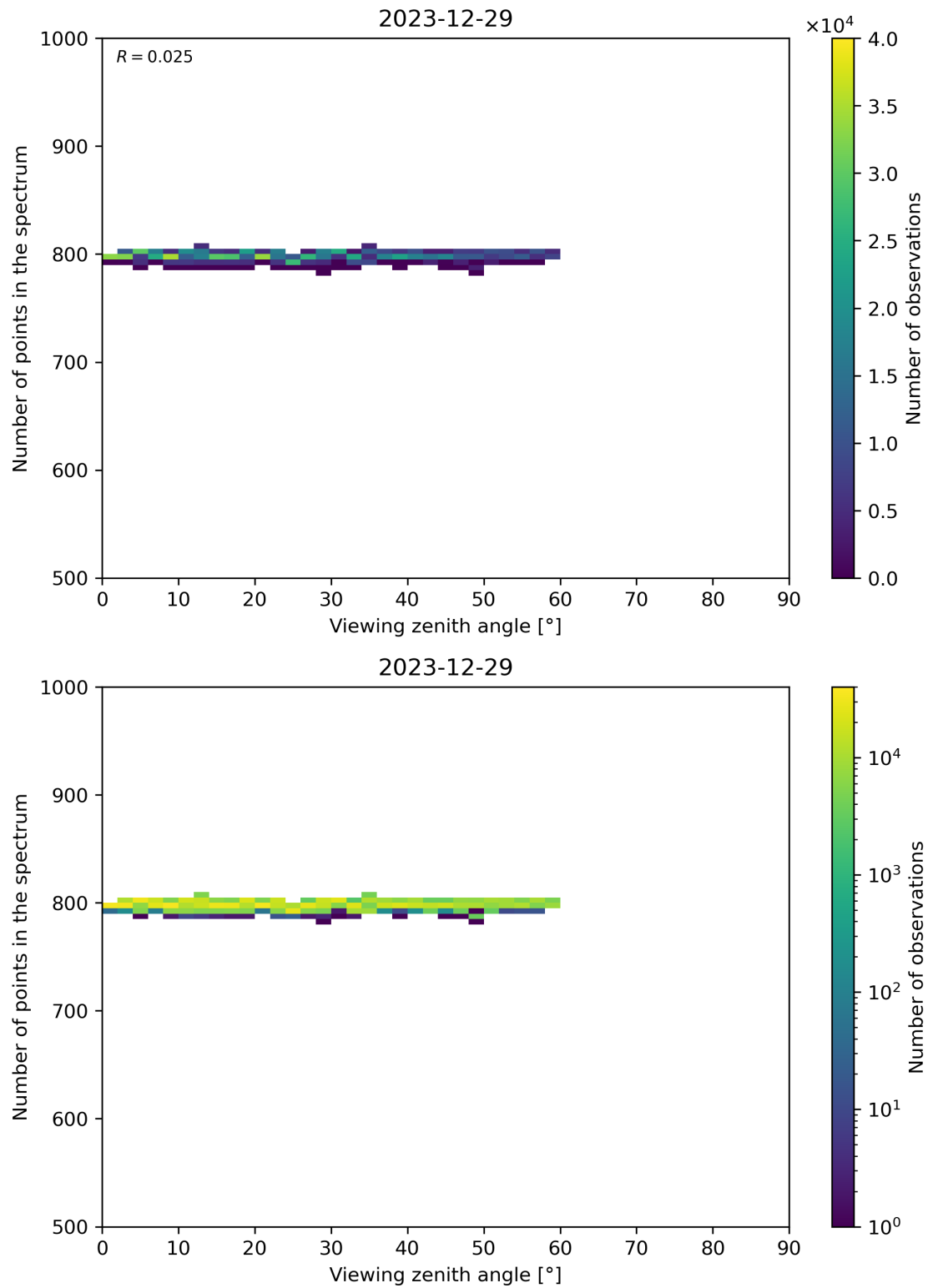
Figure 114: Scatter density plot of “Viewing zenith angle” against “Number of points in the spectrum” for 2023-12-28 to 2023-12-30.
