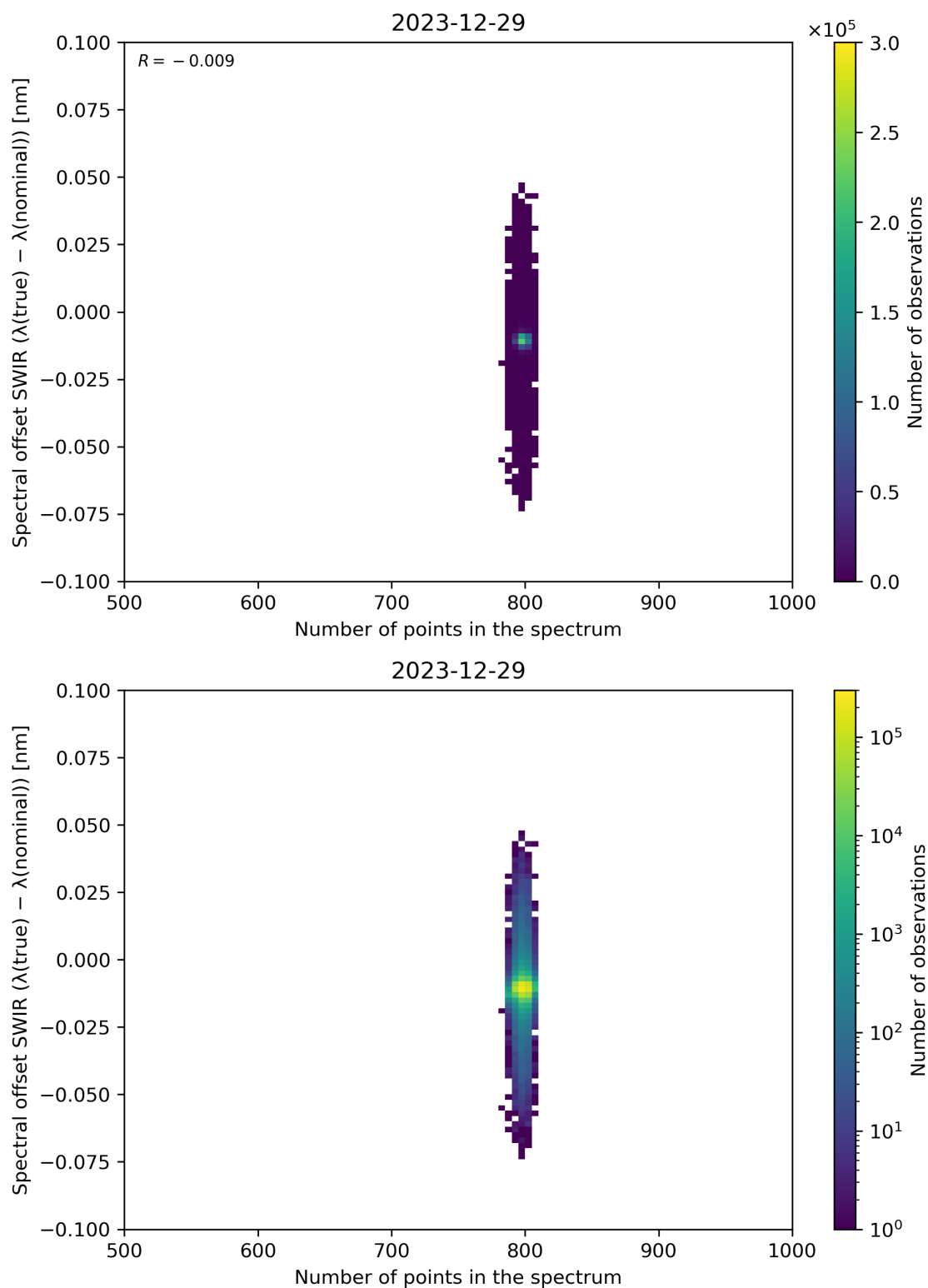
Figure 93: Scatter density plot of “Number of points in the spectrum” against “Spectral offset SWIR ( \lambda(\text{true}) - \lambda(\text{nominal}) )” for 2023-12-28 to 2023-12-30.
