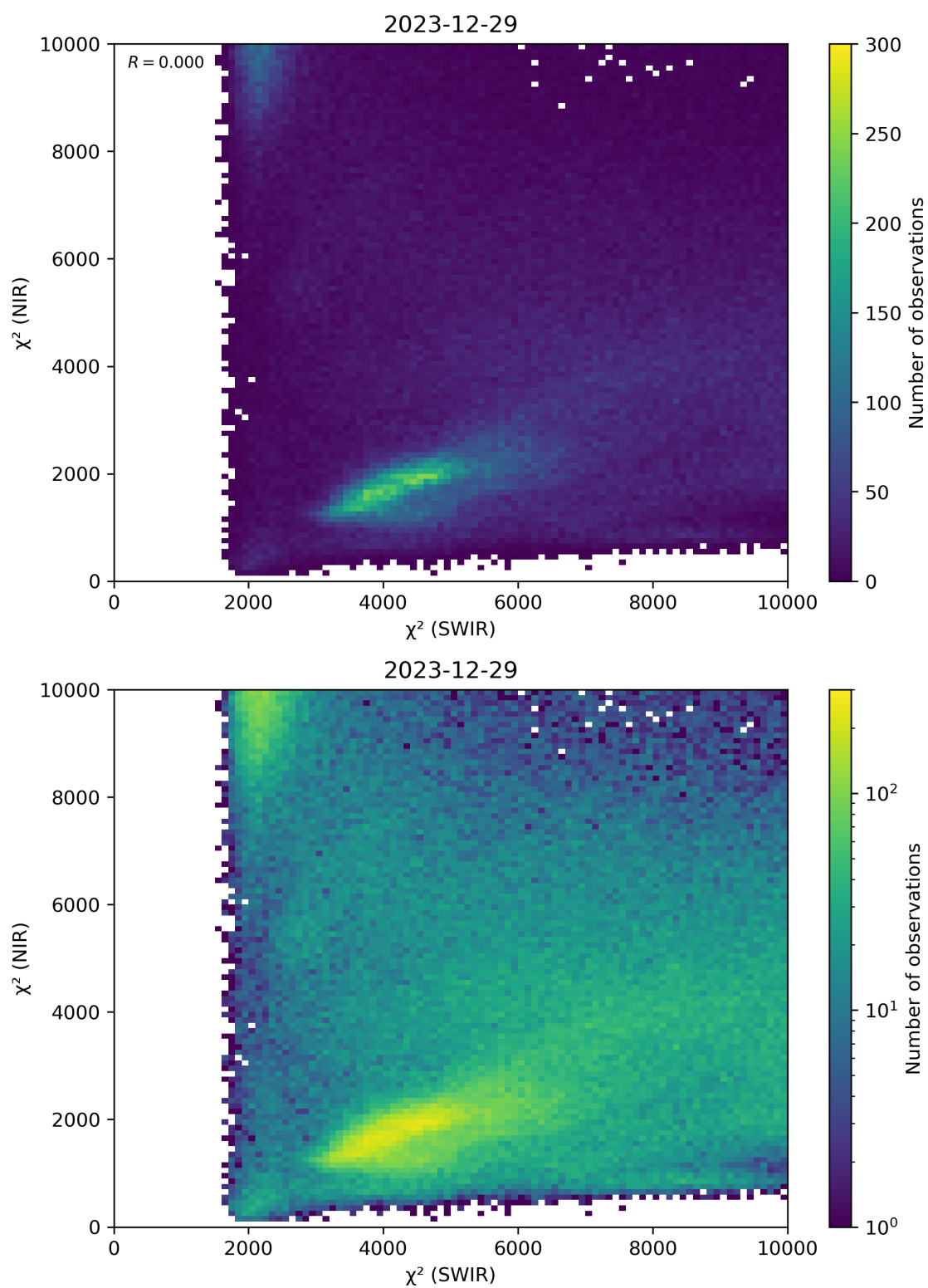
Figure 47: Scatter density plot of “ \chi^2 (SWIR)” against “ \chi^2 (NIR)” for 2023-12-28 to 2023-12-30.
