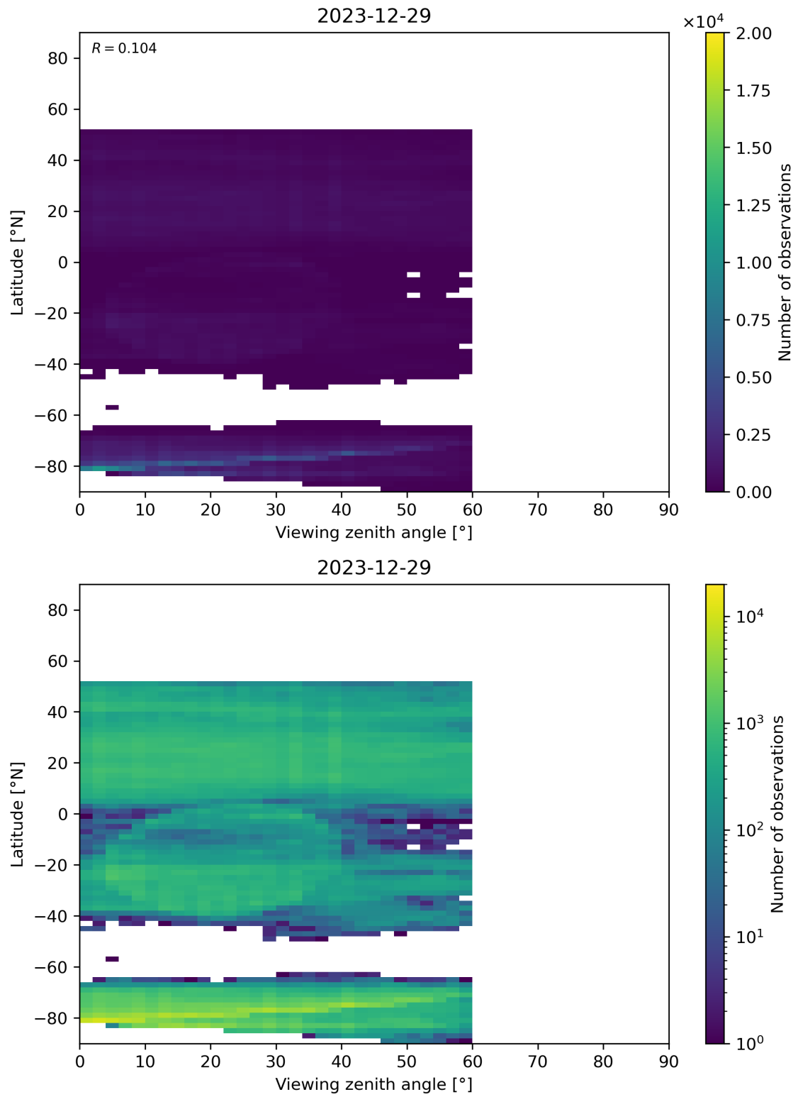
Figure 109: Scatter density plot of “Viewing zenith angle” against “Latitude” for 2023-12-28 to 2023-12-30.
