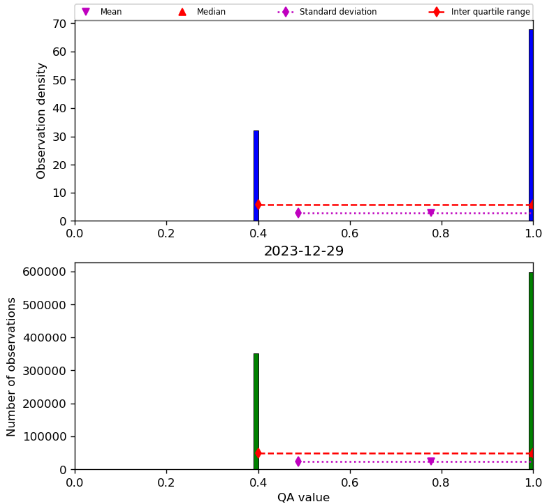
Figure 22: Histogram of “QA value” for 2023-12-28 to 2023-12-30
