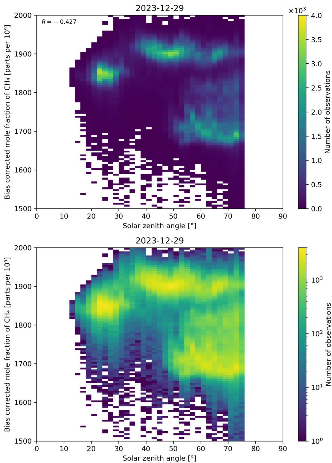
Figure 100: Scatter density plot of “Solar zenith angle” against “Bias corrected mole fraction of CH 4 ” for 2023-12-28 to 2023-12-30.
