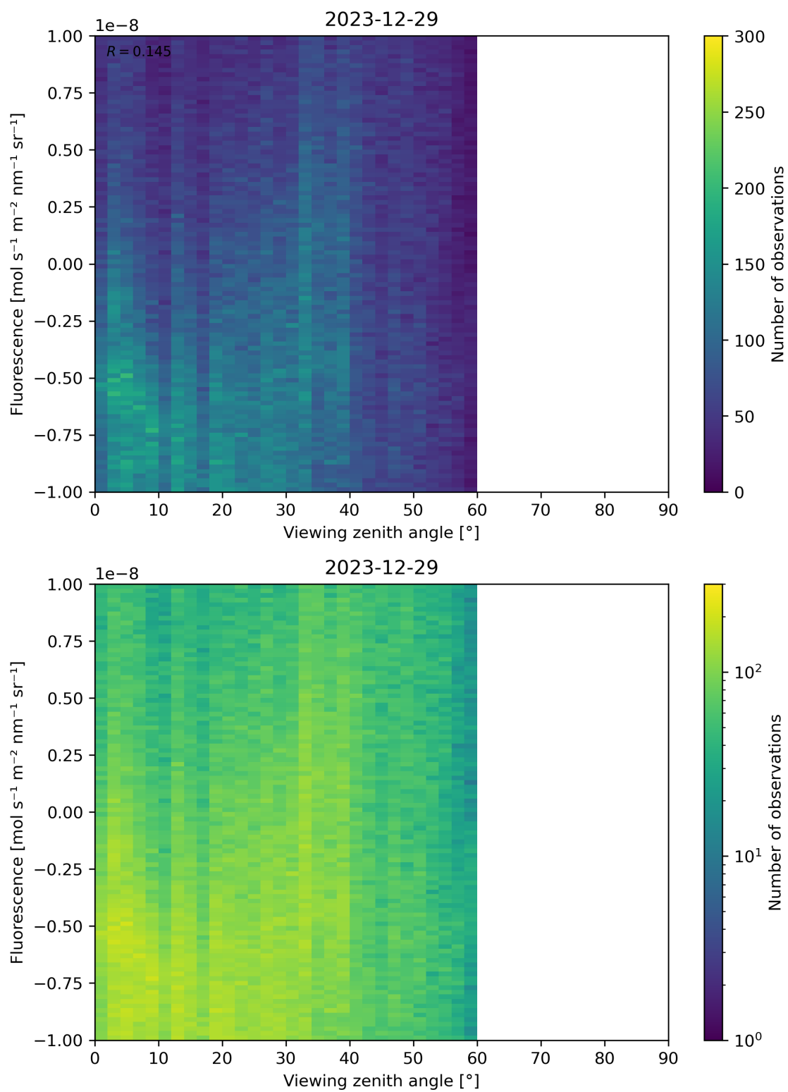
Figure 108: Scatter density plot of “Viewing zenith angle” against “Fluorescence” for 2023-12-28 to 2023-12-30.
