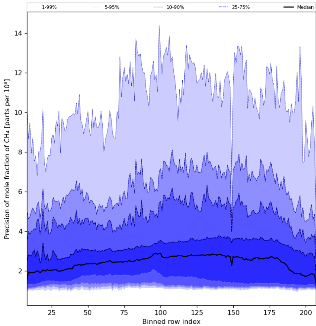
Figure 35: Along track statistics of “Precision of mole fraction of CH 4 ” for 2023-12-28 to 2023-12-30
