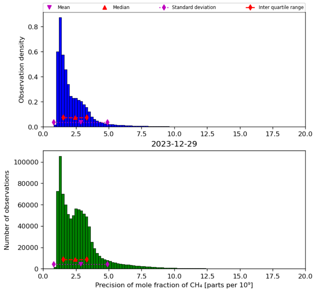
Figure 24: Histogram of “Precision of mole fraction of CH 4 ” for 2023-12-28 to 2023-12-30
