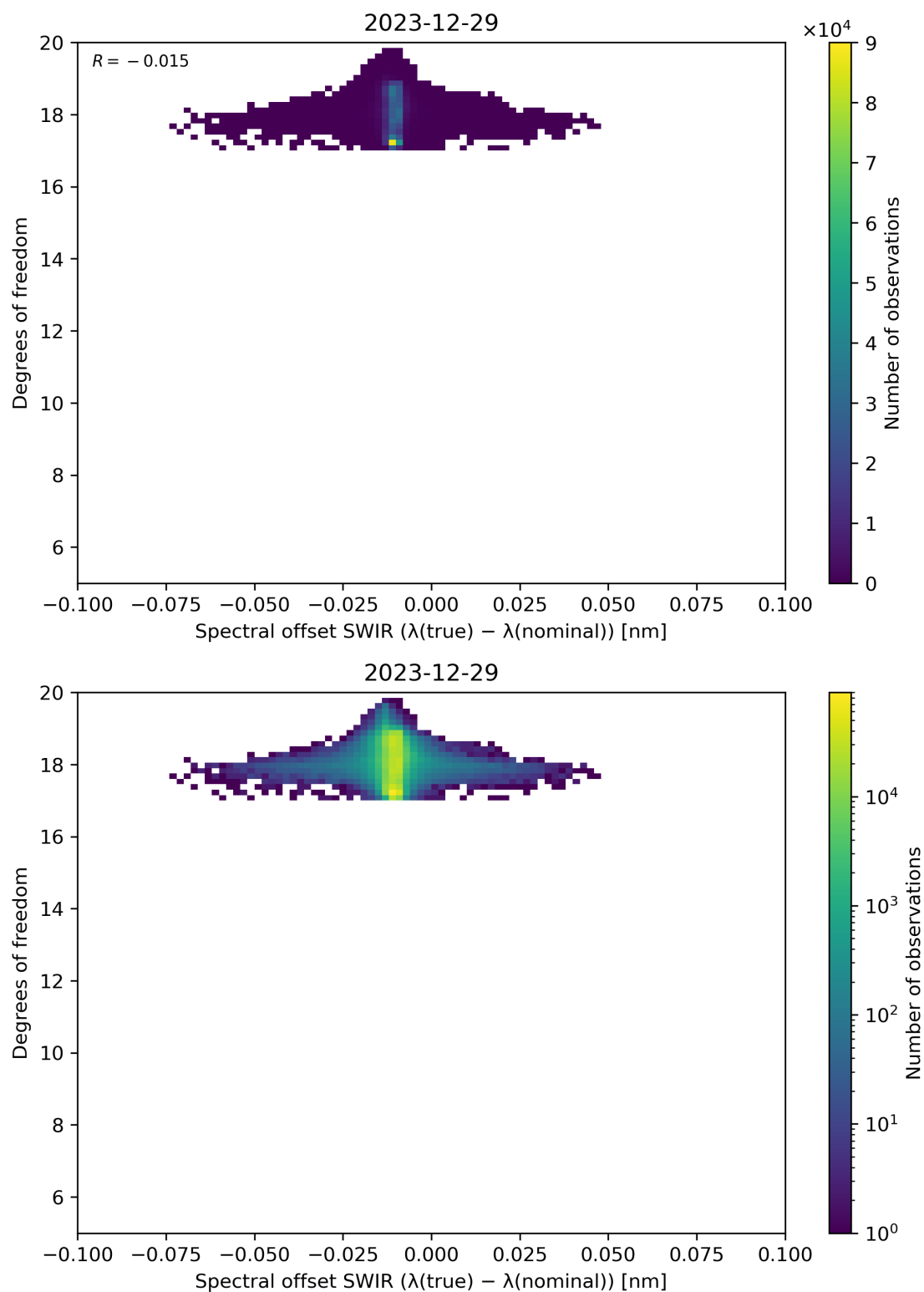
Figure 119: Scatter density plot of “Spectral offset SWIR ( \lambda(\text{true}) - \lambda(\text{nominal}) )” against “Degrees of freedom” for 2023-12-28 to 2023-12-30.
