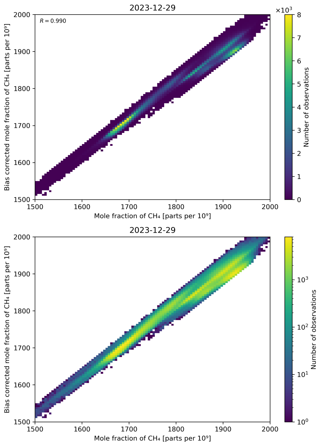
Figure 74: Scatter density plot of “Mole fraction of CH 4 ” against “Bias corrected mole fraction of CH 4 ” for 2023-12-28 to 2023-12-30.
