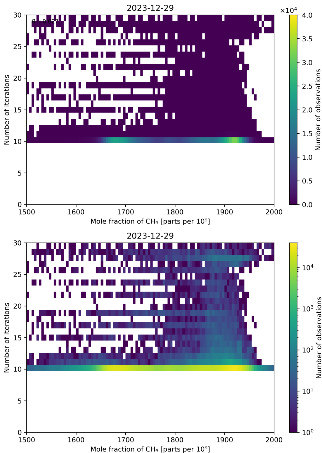
Figure 76: Scatter density plot of “Mole fraction of CH 4 ” against “Number of iterations” for 2023-12-28 to 2023-12-30.
