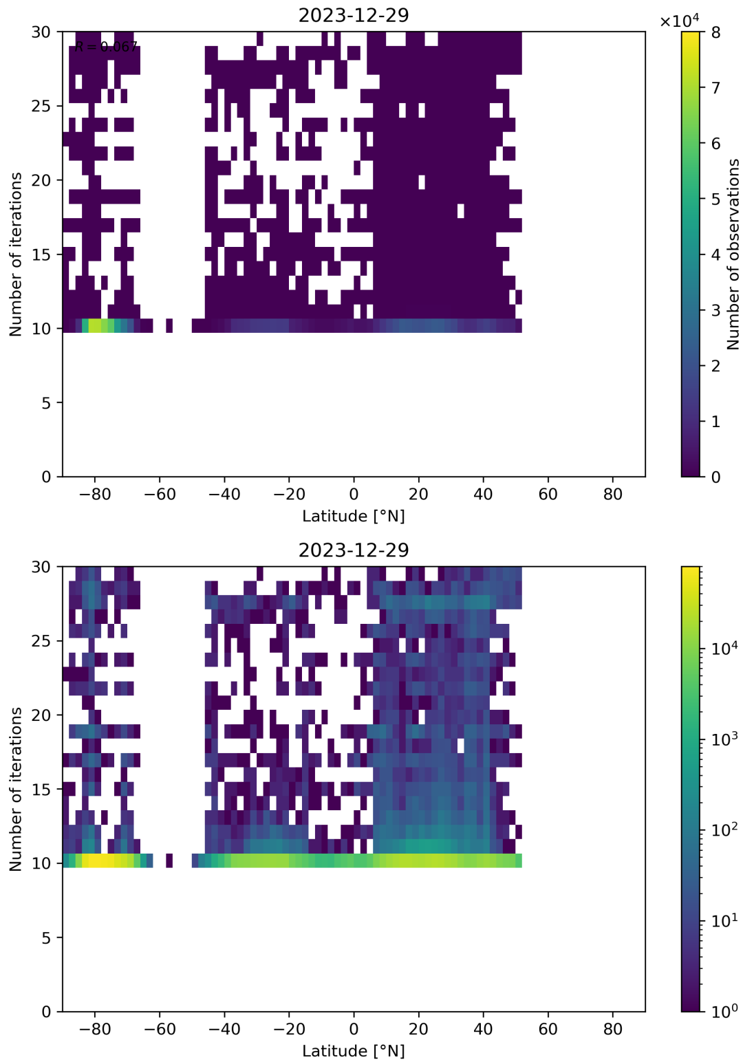
Figure 60: Scatter density plot of “Latitude” against “Number of iterations” for 2023-12-28 to 2023-12-30.
