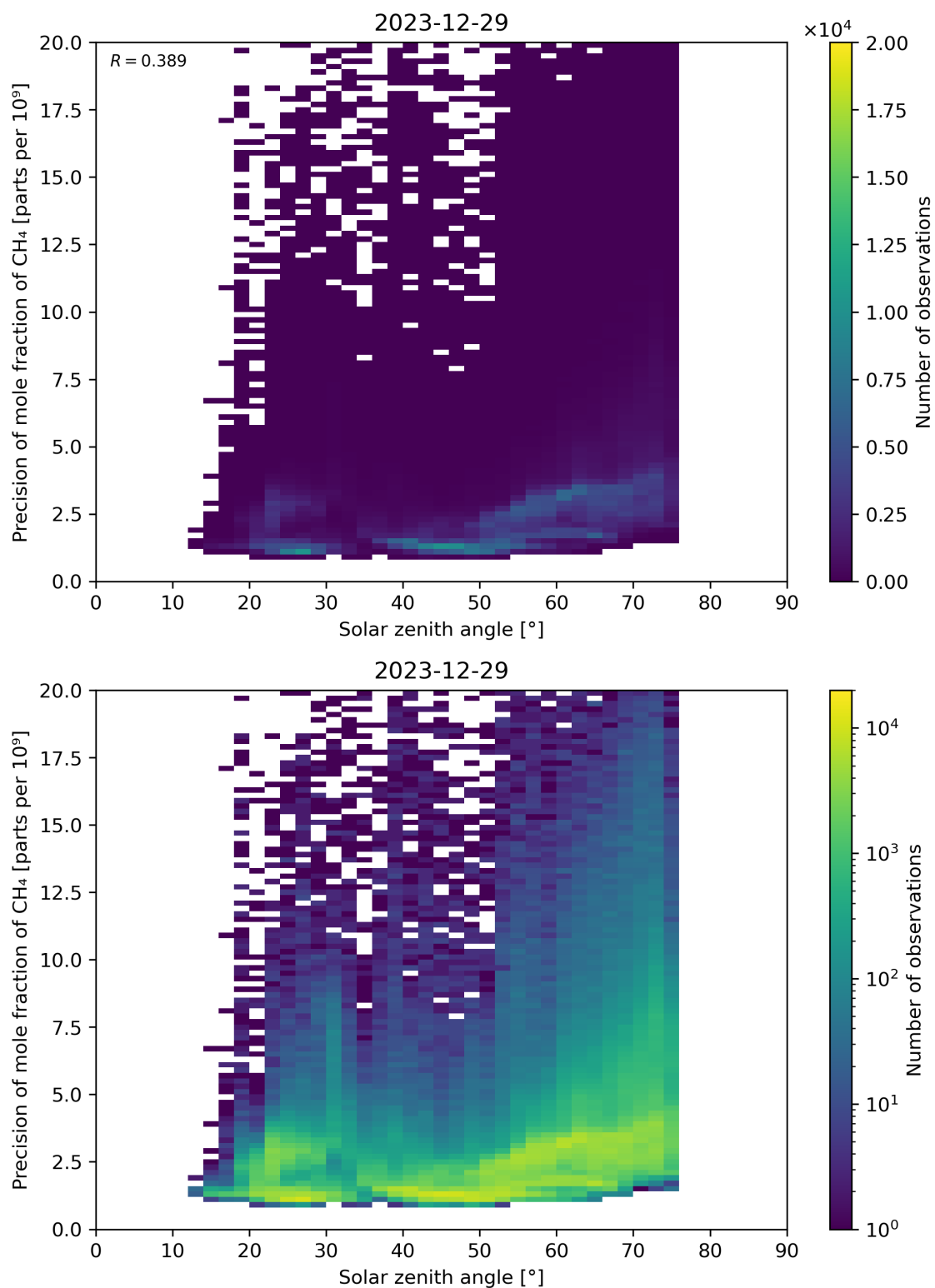
Figure 101: Scatter density plot of “Solar zenith angle” against “Precision of mole fraction of \text{CH}_4 ” for 2023-12-28 to 2023-12-30.
