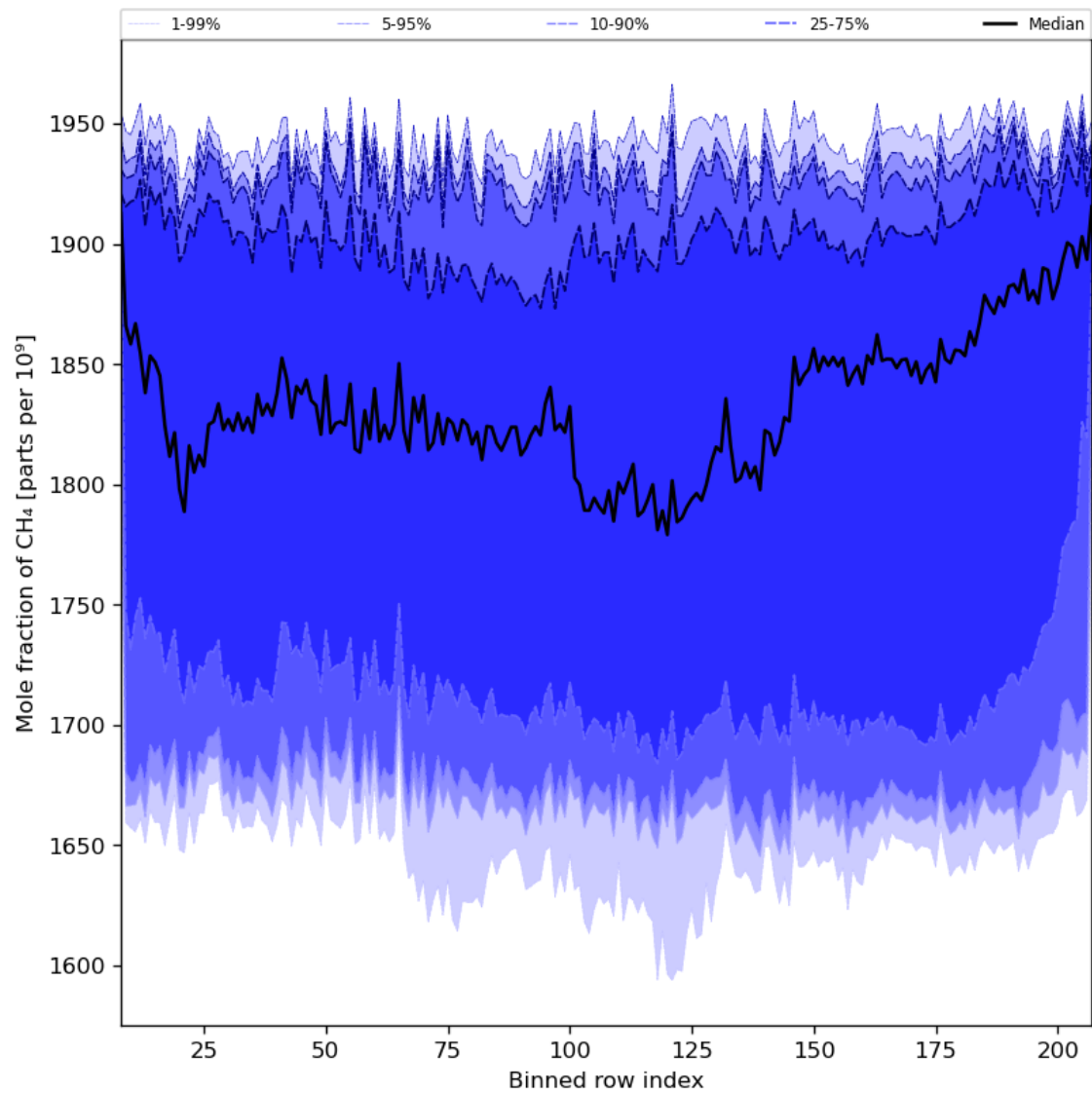
Figure 34: Along track statistics of “Mole fraction of CH 4 ” for 2023-12-28 to 2023-12-30
