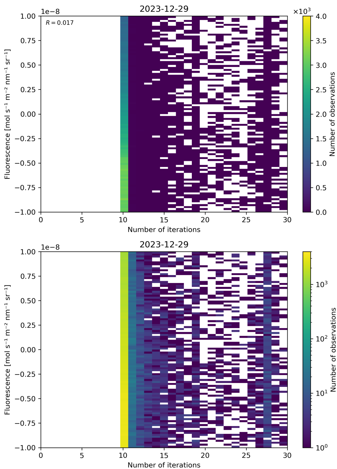
Figure 87: Scatter density plot of “Number of iterations” against “Fluorescence” for 2023-12-28 to 2023-12-30.
