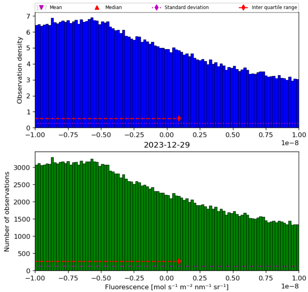
Figure 32: Histogram of “Fluorescence” for 2023-12-28 to 2023-12-30
