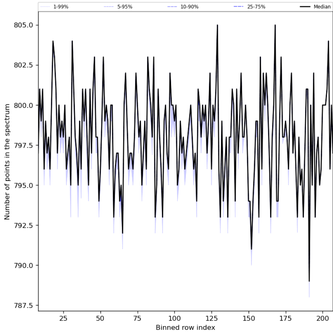
Figure 37: Along track statistics of “Number of points in the spectrum” for 2023-12-28 to 2023-12-30
