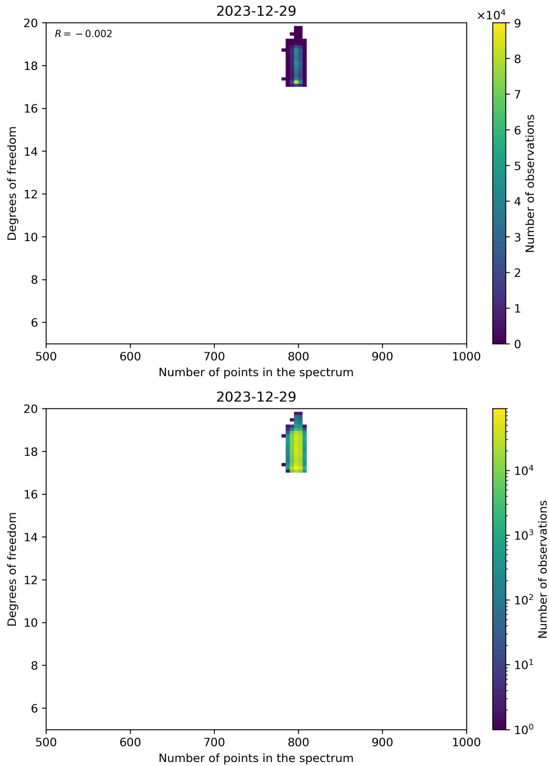
Figure 90: Scatter density plot of “Number of points in the spectrum” against “Degrees of freedom” for 2023-12-28 to 2023-12-30.
