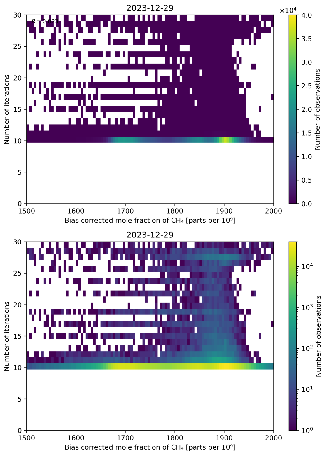
Figure 67: Scatter density plot of “Bias corrected mole fraction of CH 4 ” against “Number of iterations” for 2023-12-28 to 2023-12-30.
