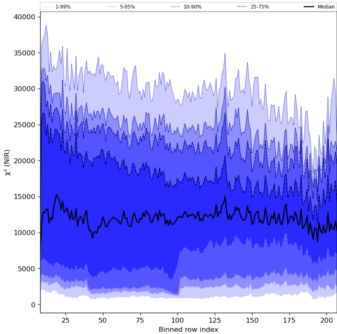
Figure 40: Along track statistics of “ \chi^2 (NIR)” for 2023-12-28 to 2023-12-30
