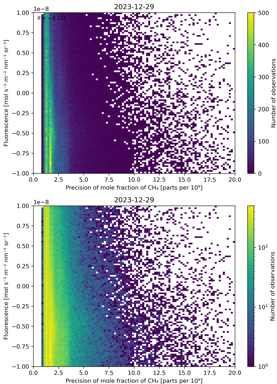
Figure 81: Scatter density plot of “Precision of mole fraction of \text{CH}_4 ” against “Fluorescence” for 2023-12-28 to 2023-12-30.
