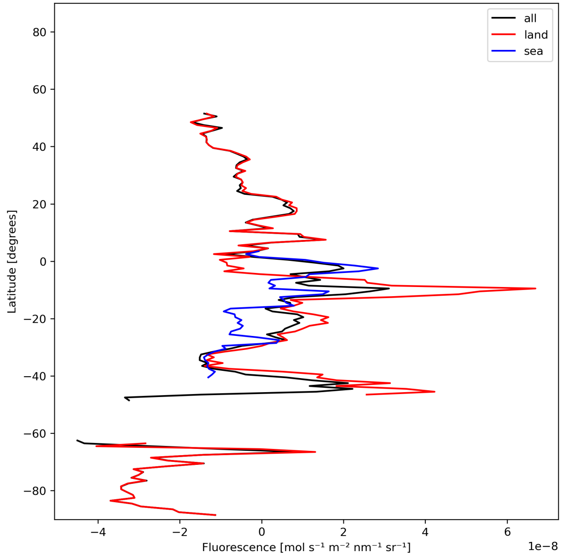
Figure 21: Zonal average of “Fluorescence” for 2023-12-28 to 2023-12-30.
