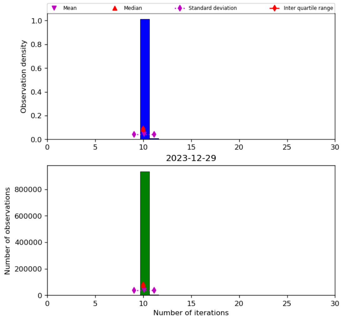
Figure 31: Histogram of “Number of iterations” for 2023-12-28 to 2023-12-30
