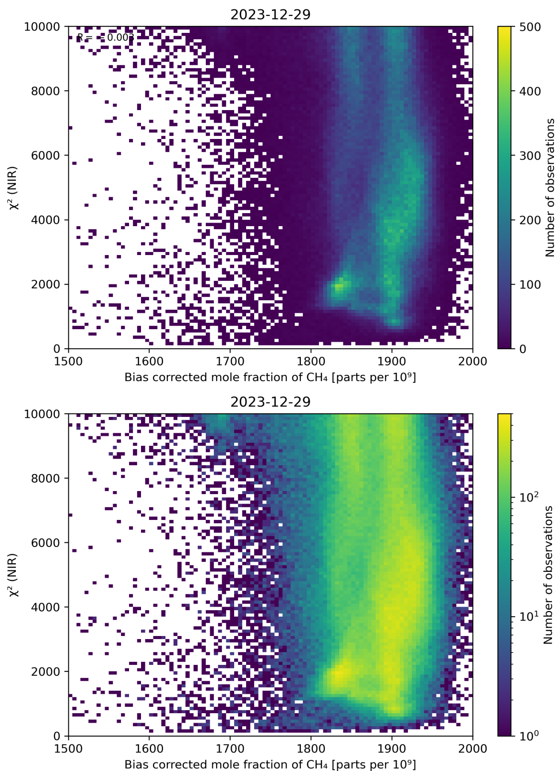
Figure 63: Scatter density plot of “Bias corrected mole fraction of CH 4 ” against “ \chi^2 (NIR)” for 2023-12-28 to 2023-12-30.
