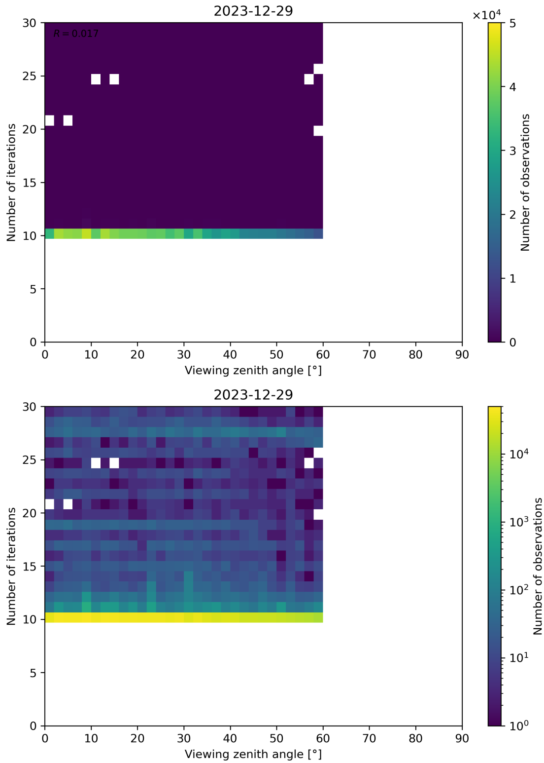
Figure 113: Scatter density plot of “Viewing zenith angle” against “Number of iterations” for 2023-12-28 to 2023-12-30.
