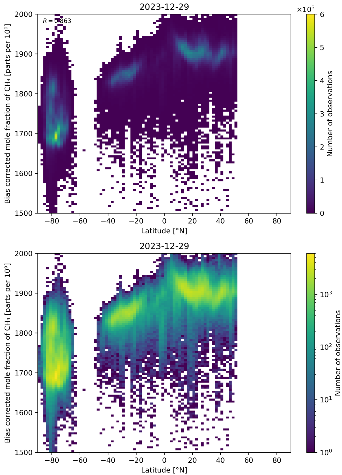
Figure 58: Scatter density plot of “Latitude” against “Bias corrected mole fraction of CH 4 ” for 2023-12-28 to 2023-12-30.
