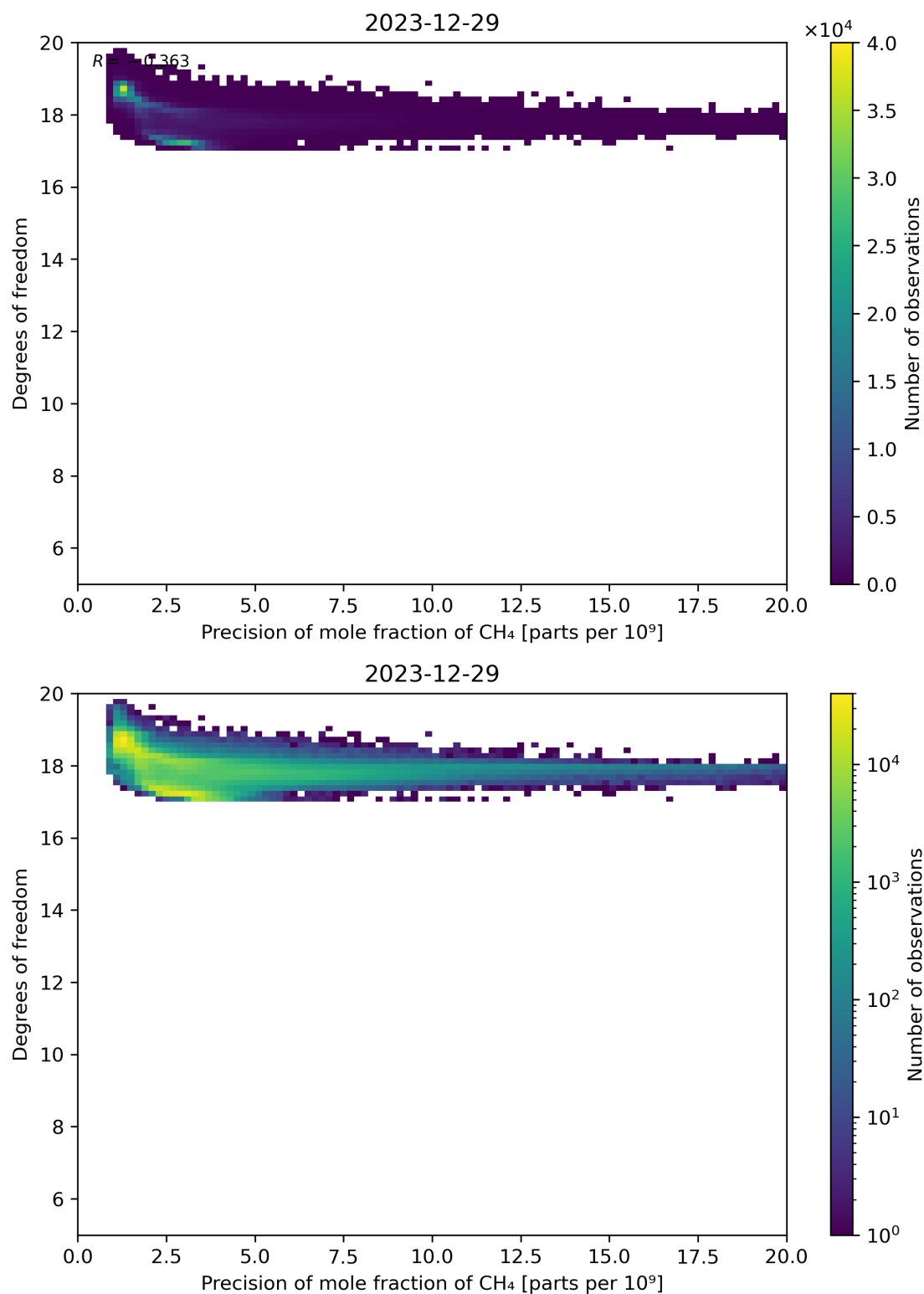
Figure 80: Scatter density plot of “Precision of mole fraction of CH 4 ” against “Degrees of freedom” for 2023-12-28 to 2023-12-30.
