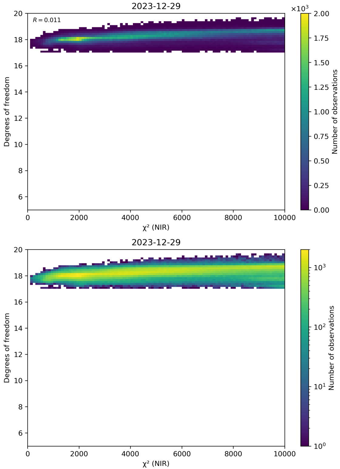
Figure 44: Scatter density plot of “ \chi^2 (NIR)” against “Degrees of freedom” for 2023-12-28 to 2023-12-30.
