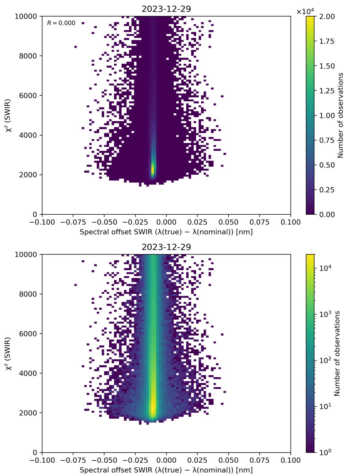
Figure 118: Scatter density plot of “Spectral offset SWIR ( \lambda(\text{true}) - \lambda(\text{nominal}) )” against “ \chi^2 (SWIR)” for 2023-12-28 to 2023-12-30.
