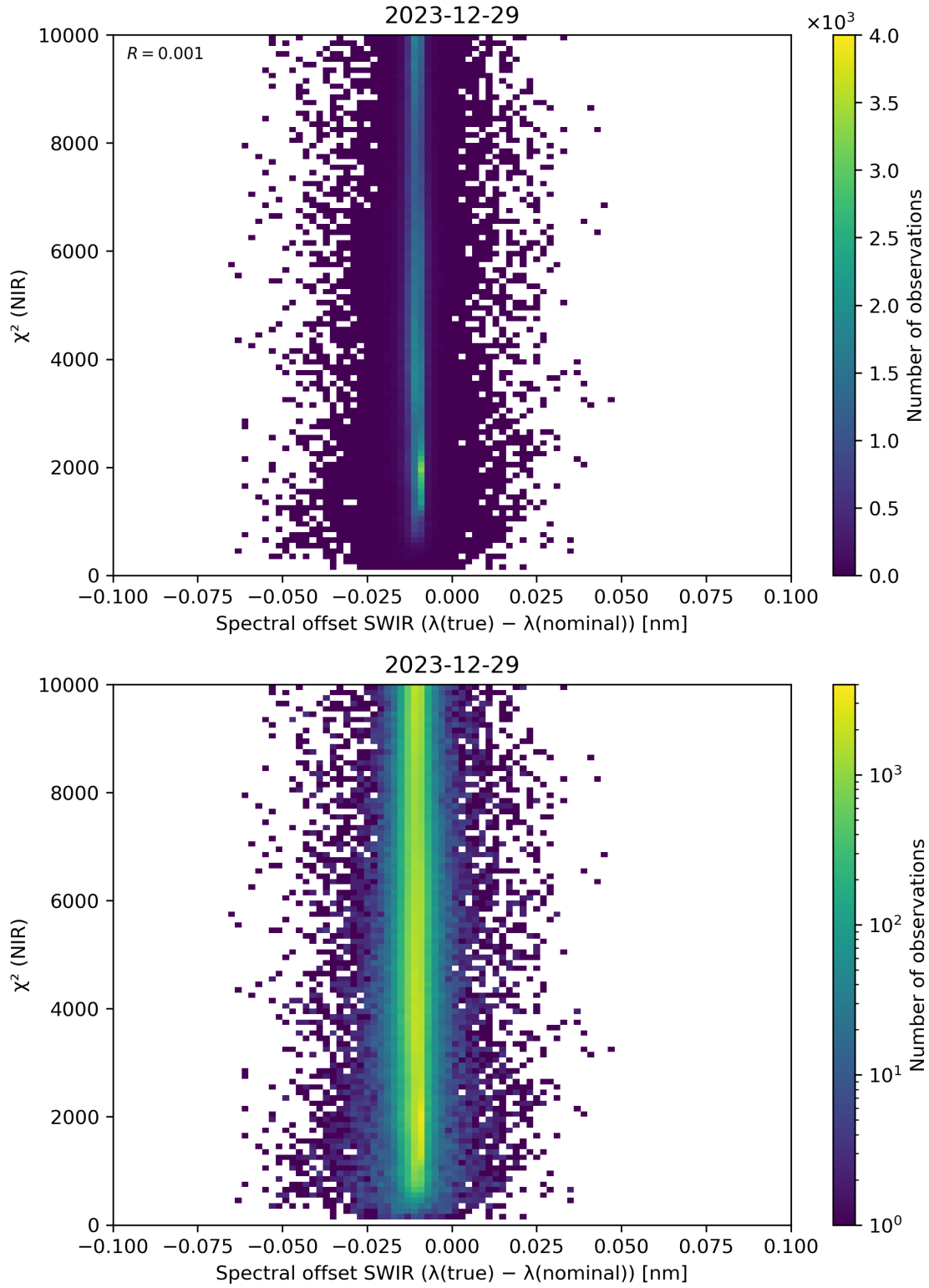
Figure 117: Scatter density plot of “Spectral offset SWIR ( \lambda(\text{true}) - \lambda(\text{nominal}) )” against “ \chi^2 (NIR)” for 2023-12-28 to 2023-12-30.
