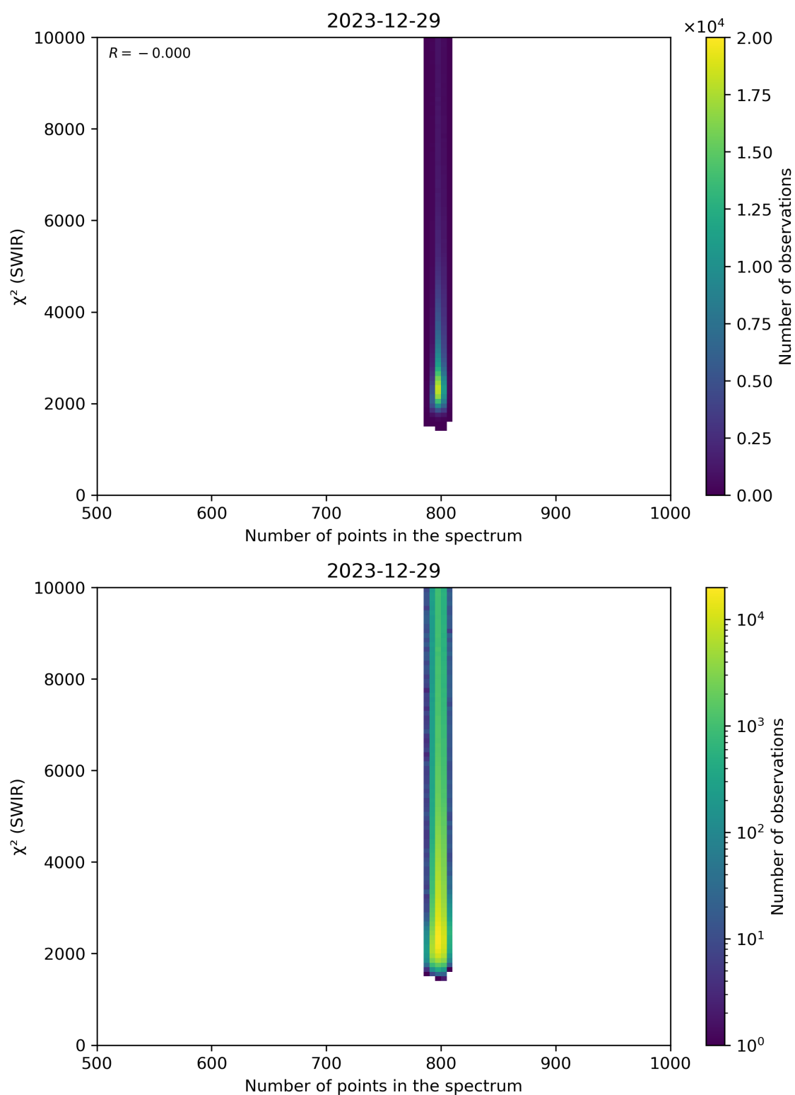
Figure 89: Scatter density plot of “Number of points in the spectrum” against “ \chi^2 (SWIR)” for 2023-12-28 to 2023-12-30.
