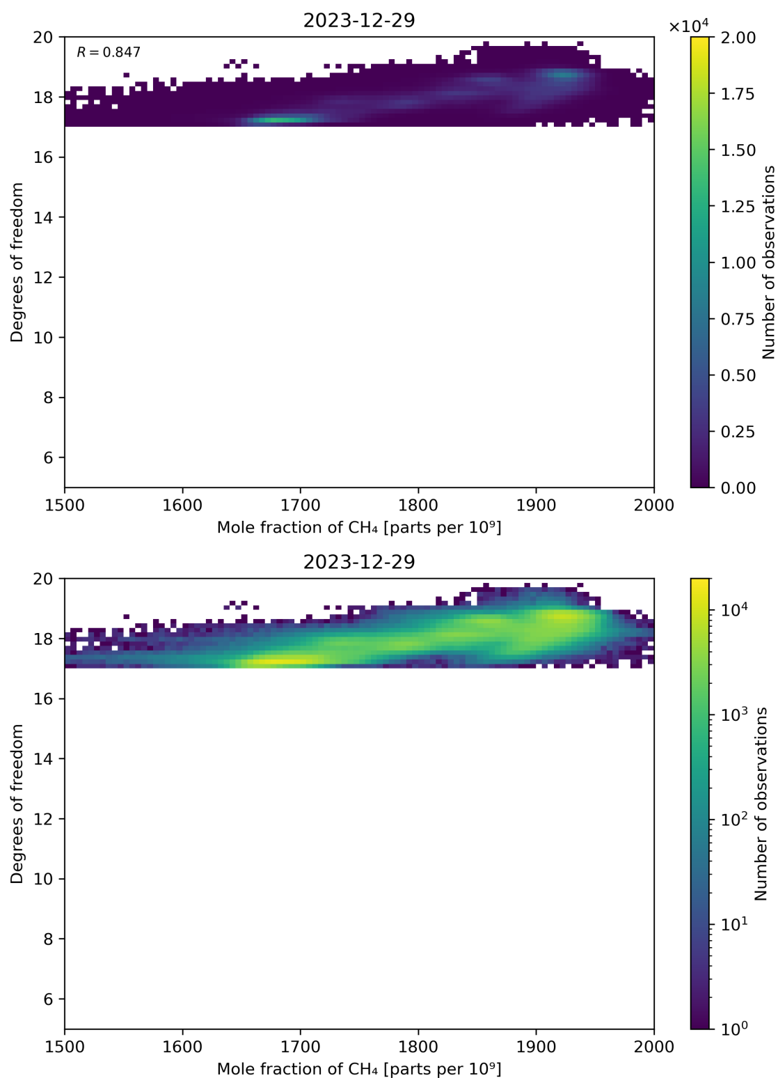
Figure 72: Scatter density plot of “Mole fraction of CH 4 ” against “Degrees of freedom” for 2023-12-28 to 2023-12-30.
