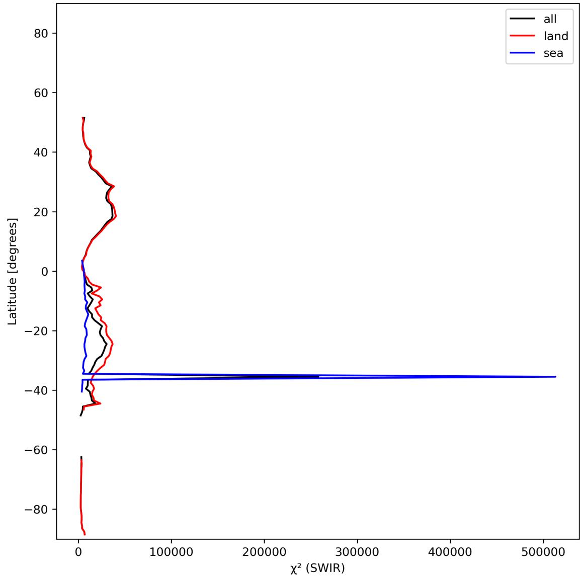
Figure 17: Zonal average of “ \chi^2 (SWIR)” for 2023-12-28 to 2023-12-30.
