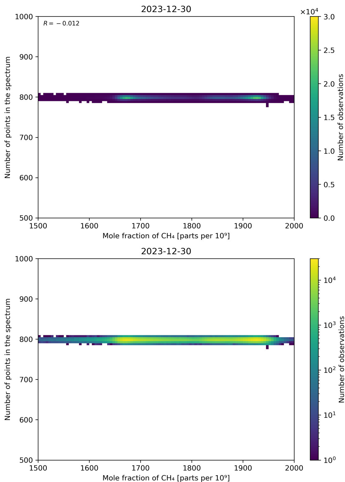
Figure 77: Scatter density plot of “Mole fraction of CH 4 ” against “Number of points in the spectrum” for 2023-12-30 to 2023-12-31.
