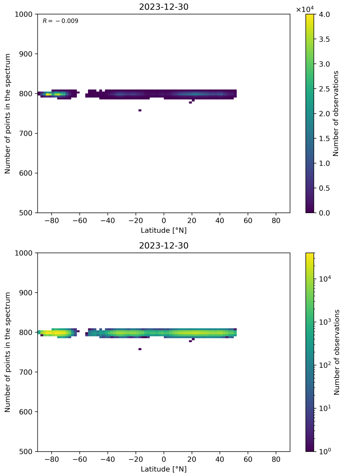
Figure 61: Scatter density plot of “Latitude” against “Number of points in the spectrum” for 2023-12-30 to 2023-12-31.
