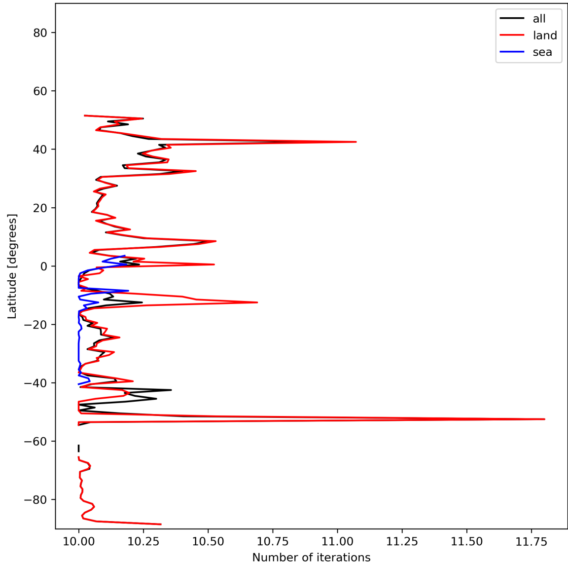
Figure 20: Zonal average of “Number of iterations” for 2023-12-30 to 2023-12-31.
