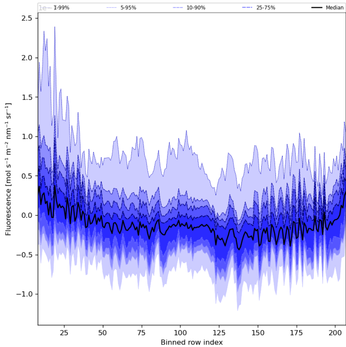
Figure 43: Along track statistics of “Fluorescence” for 2023-12-30 to 2023-12-31
