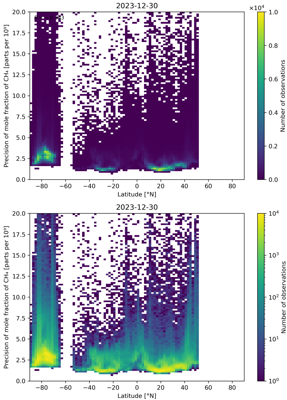
Figure 59: Scatter density plot of “Latitude” against “Precision of mole fraction of CH 4 ” for 2023-12-30 to 2023-12-31.
