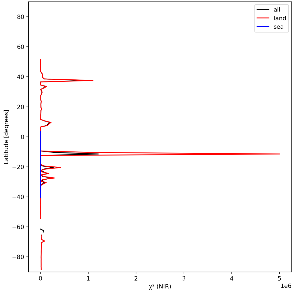
Figure 18: Zonal average of “ \chi^2 (NIR)” for 2023-12-30 to 2023-12-31.
