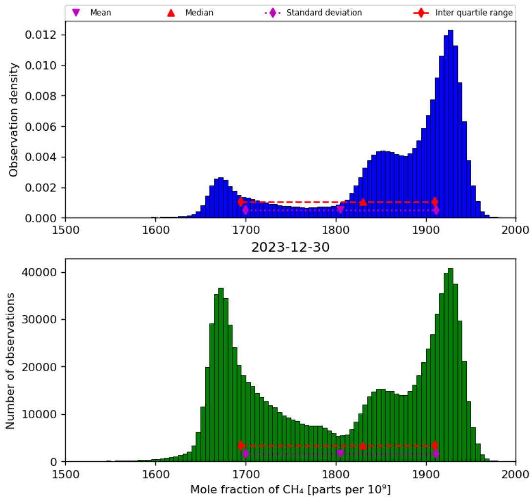
Figure 23: Histogram of “Mole fraction of CH 4 ” for 2023-12-30 to 2023-12-31
