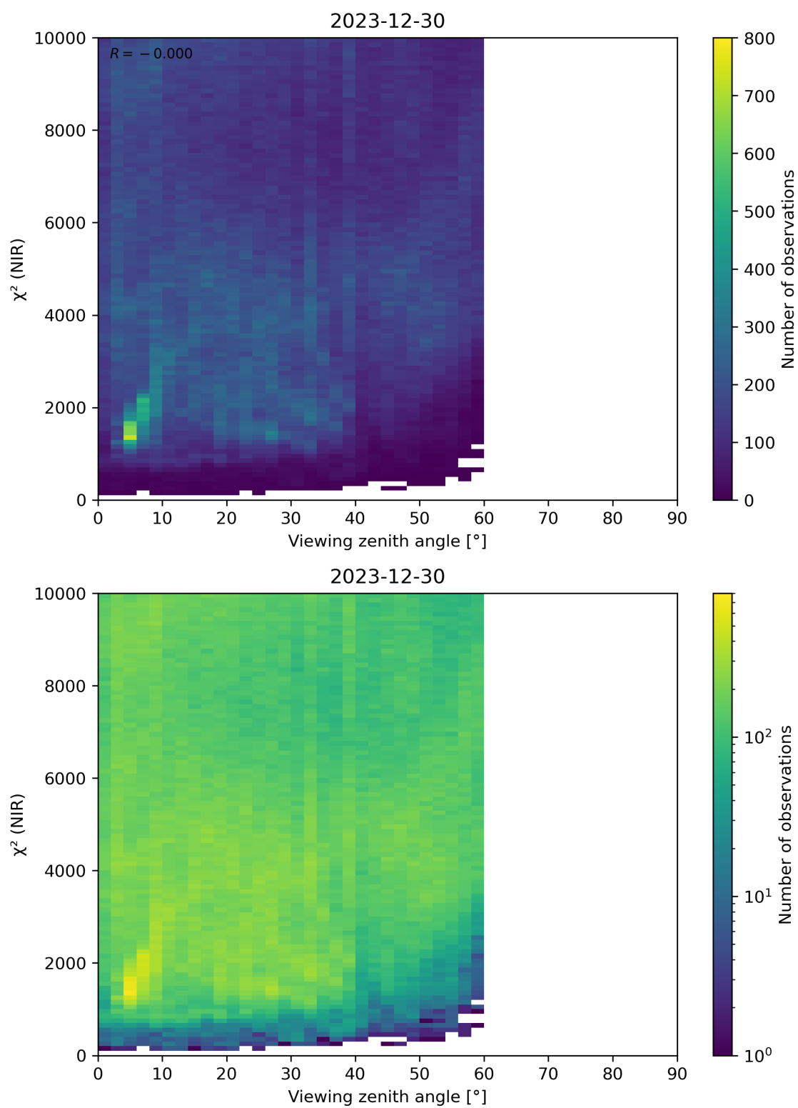
Figure 105: Scatter density plot of “Viewing zenith angle” against “ \chi^2 (NIR)” for 2023-12-30 to 2023-12-31.
