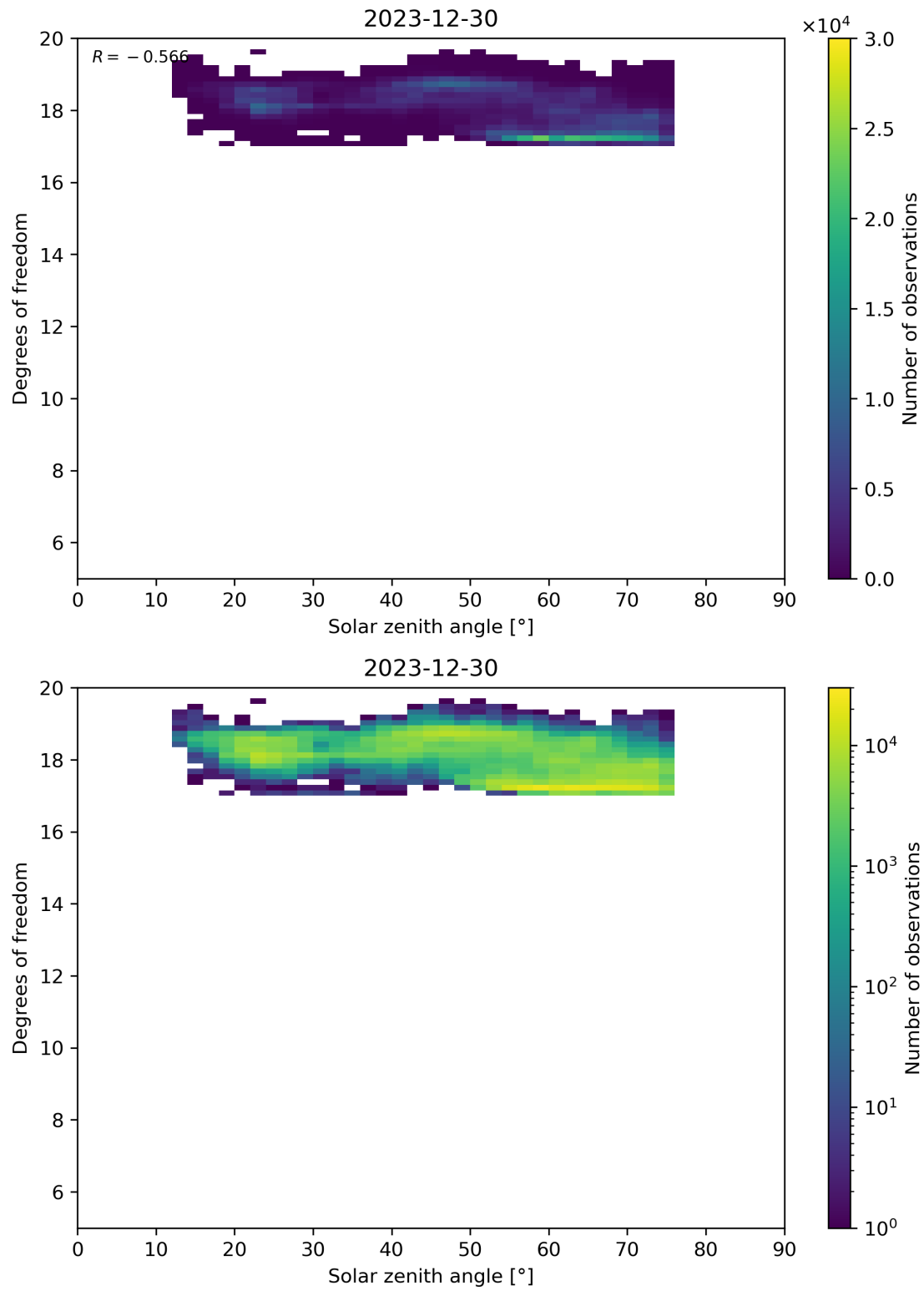
Figure 96: Scatter density plot of “Solar zenith angle” against “Degrees of freedom” for 2023-12-30 to 2023-12-31.
