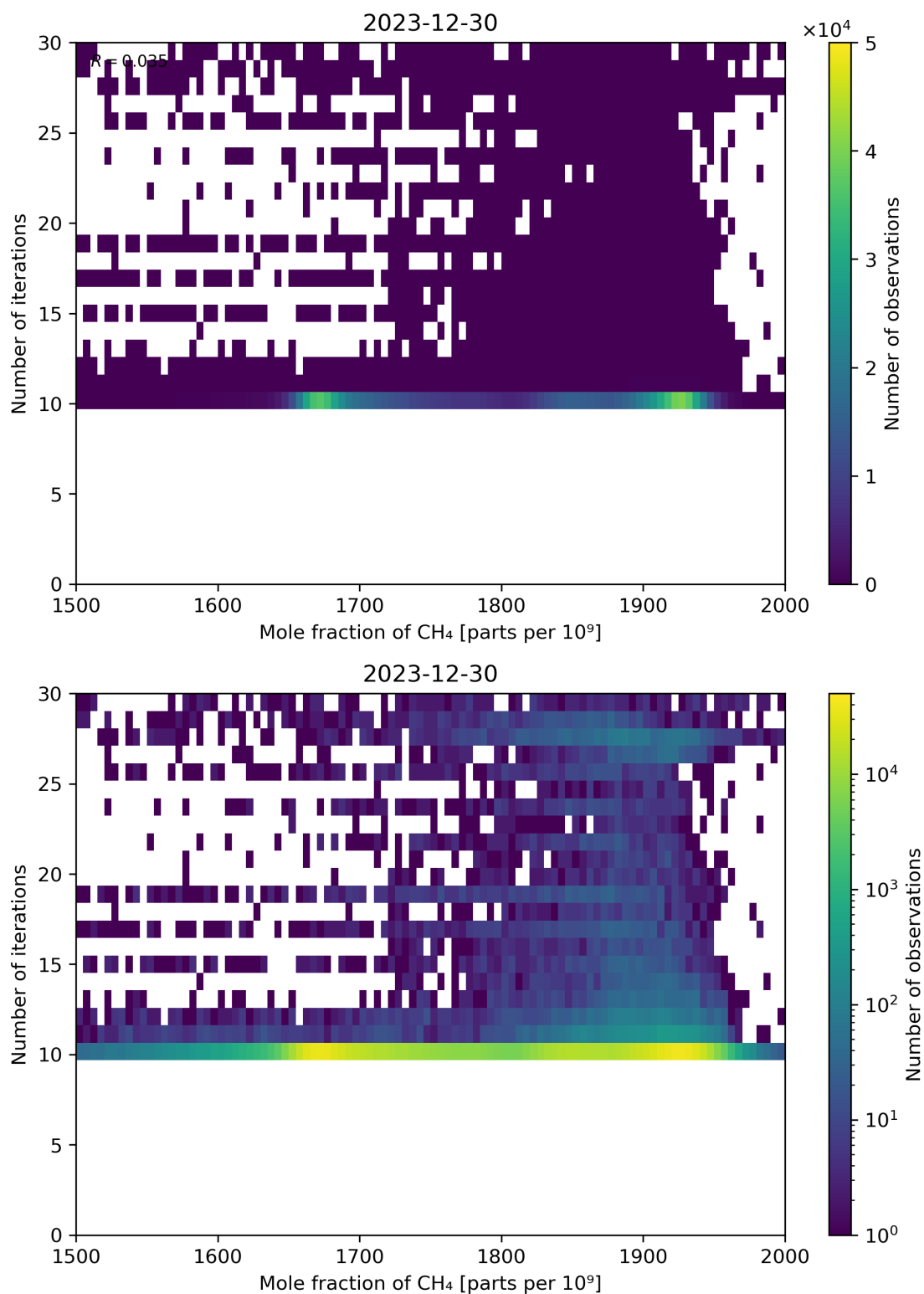
Figure 76: Scatter density plot of “Mole fraction of CH 4 ” against “Number of iterations” for 2023-12-30 to 2023-12-31.
