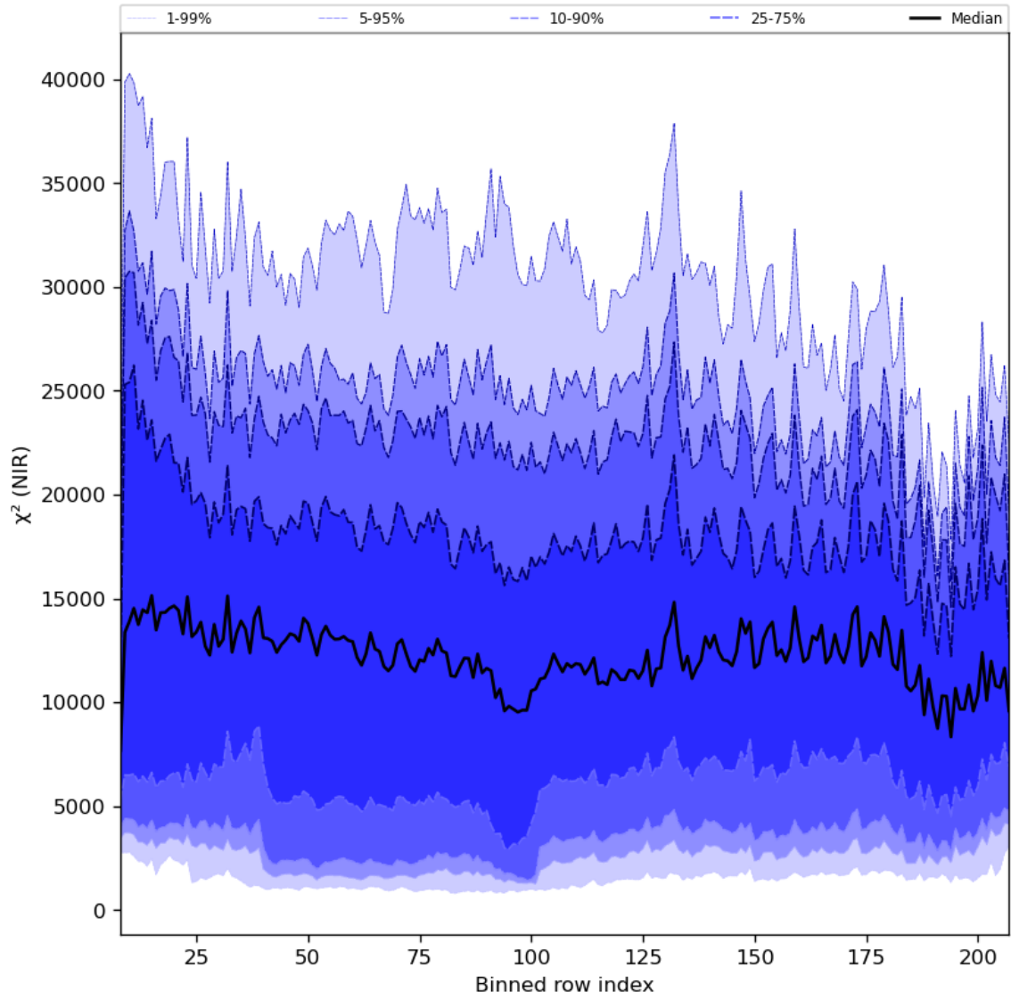
Figure 40: Along track statistics of “ \chi^2 (NIR)” for 2023-12-30 to 2023-12-31
