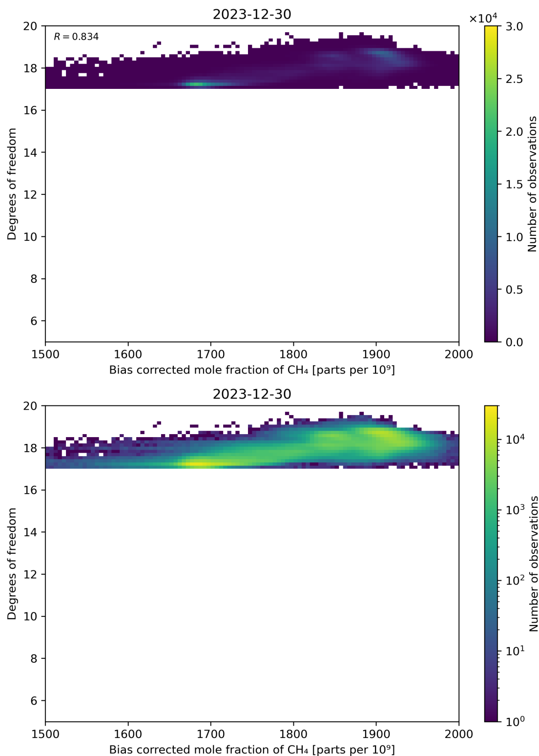
Figure 65: Scatter density plot of “Bias corrected mole fraction of \text{CH}_4 ” against “Degrees of freedom” for 2023-12-30 to 2023-12-31.
