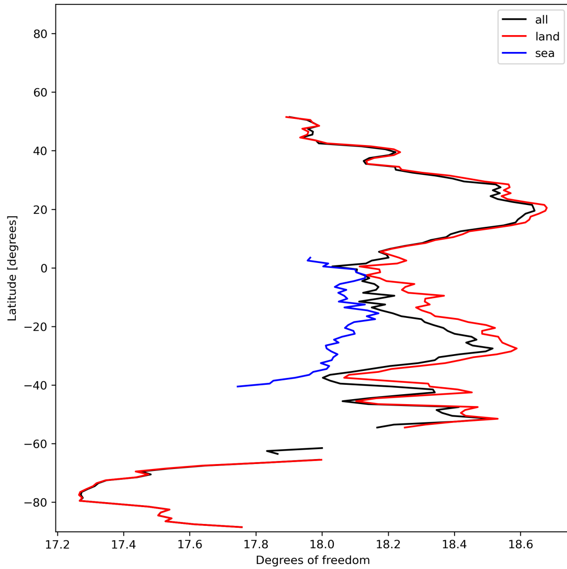
Figure 19: Zonal average of “Degrees of freedom” for 2023-12-30 to 2023-12-31.
