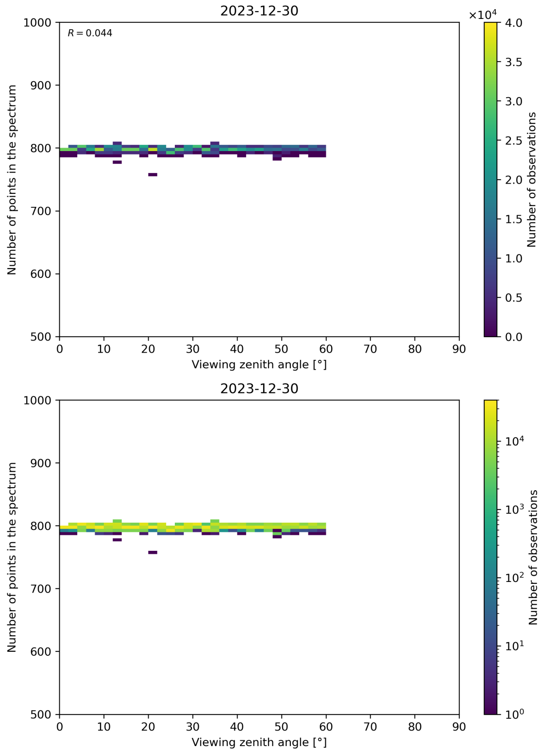
Figure 114: Scatter density plot of “Viewing zenith angle” against “Number of points in the spectrum” for 2023-12-30 to 2023-12-31.
