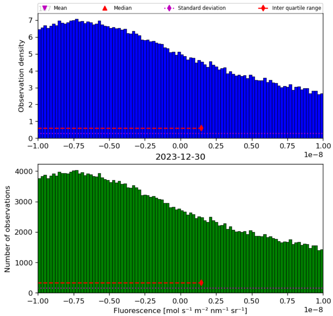
Figure 32: Histogram of “Fluorescence” for 2023-12-30 to 2023-12-31
