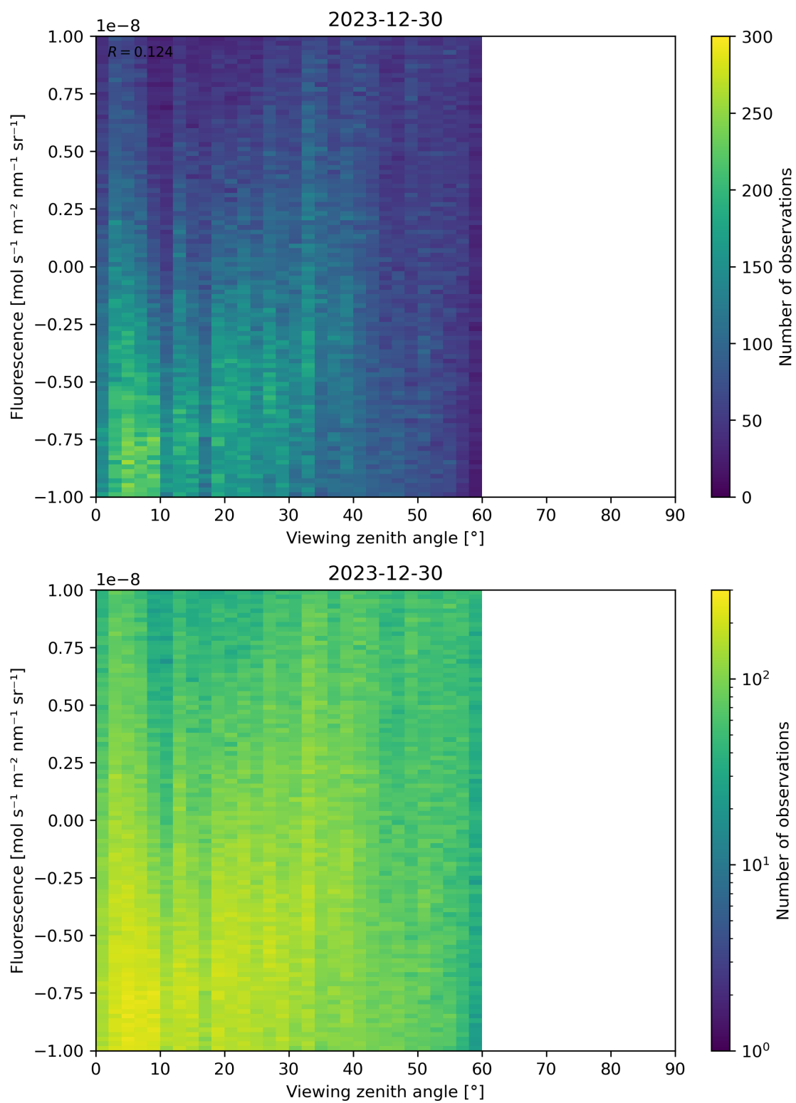
Figure 108: Scatter density plot of “Viewing zenith angle” against “Fluorescence” for 2023-12-30 to 2023-12-31.
