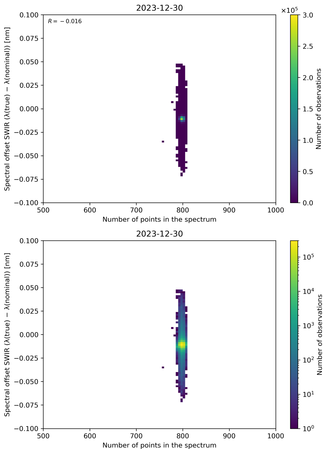
Figure 93: Scatter density plot of “Number of points in the spectrum” against “Spectral offset SWIR ( \lambda(\text{true}) - \lambda(\text{nominal}) )” for 2023-12-30 to 2023-12-31.
