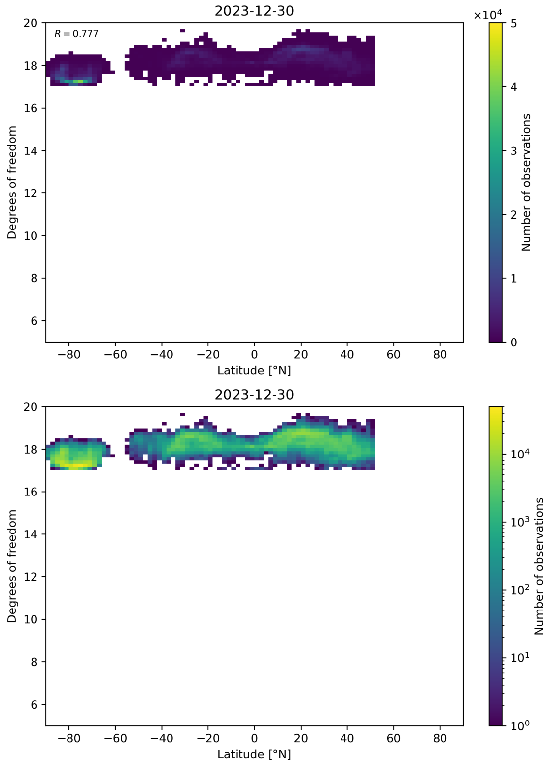
Figure 55: Scatter density plot of “Latitude” against “Degrees of freedom” for 2023-12-30 to 2023-12-31.
