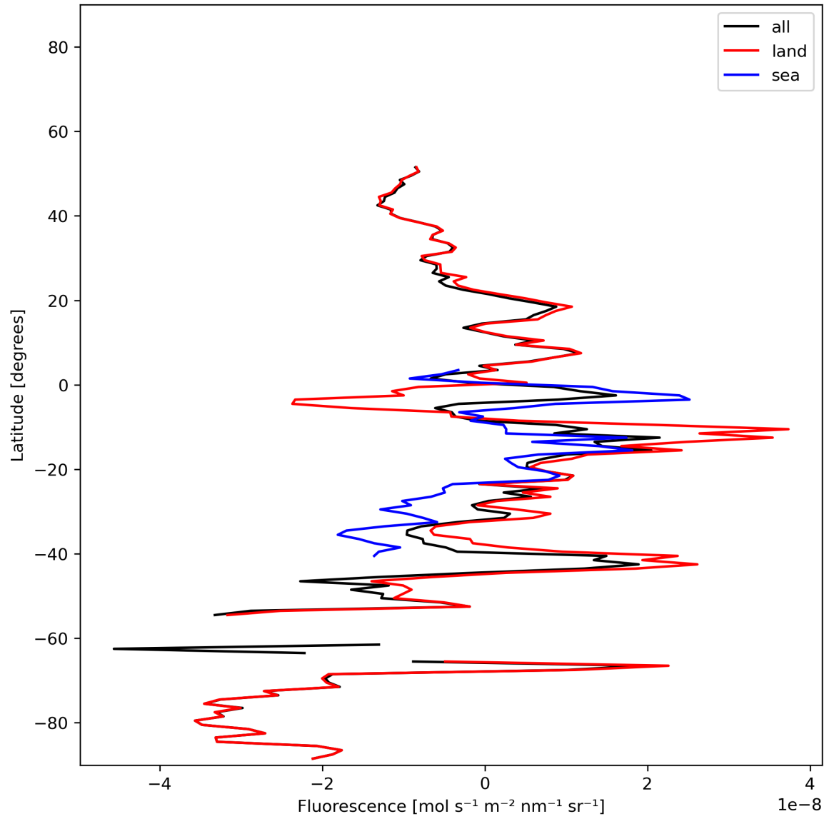
Figure 21: Zonal average of “Fluorescence” for 2023-12-30 to 2023-12-31.
