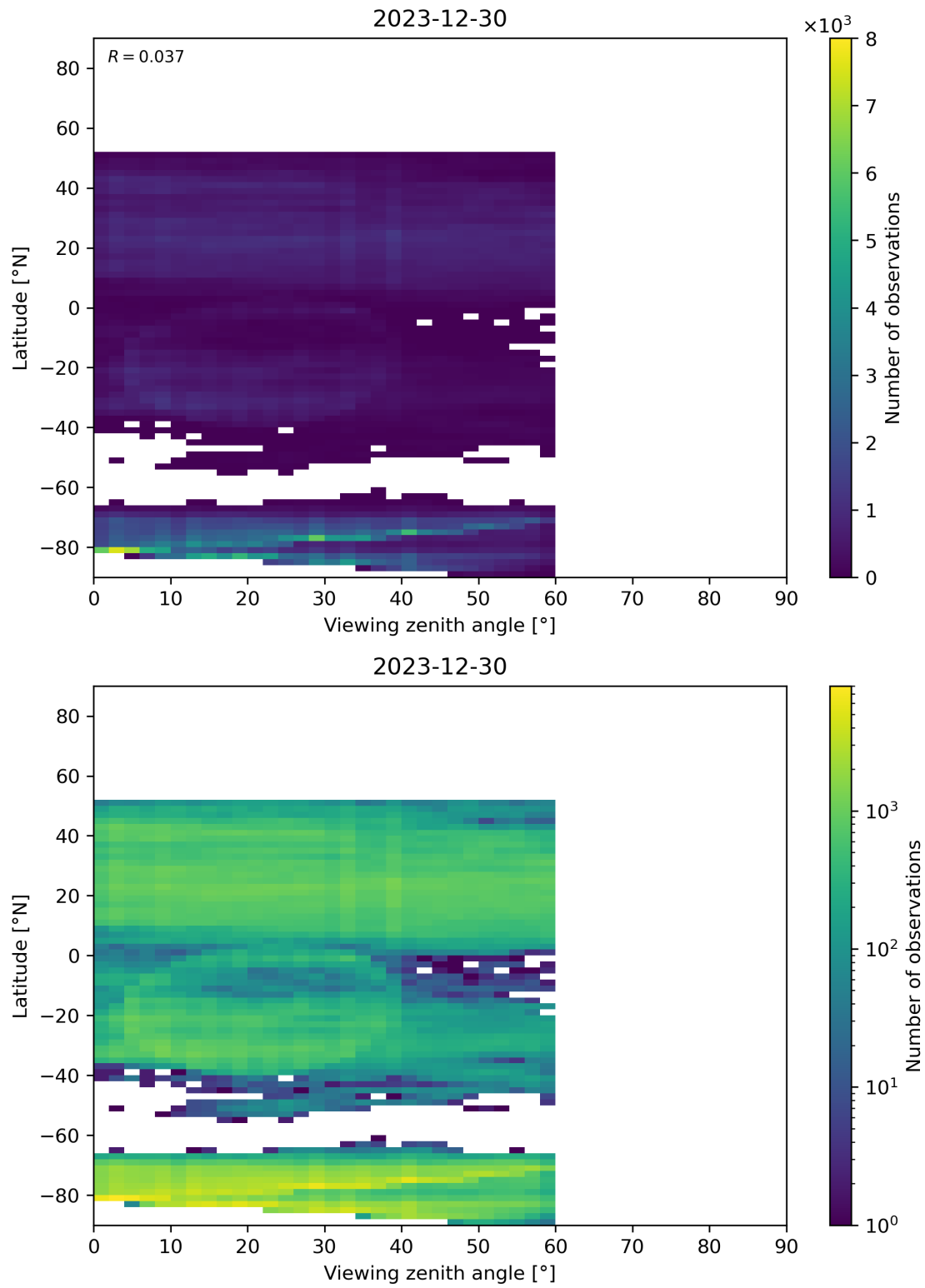
Figure 109: Scatter density plot of “Viewing zenith angle” against “Latitude” for 2023-12-30 to 2023-12-31.
