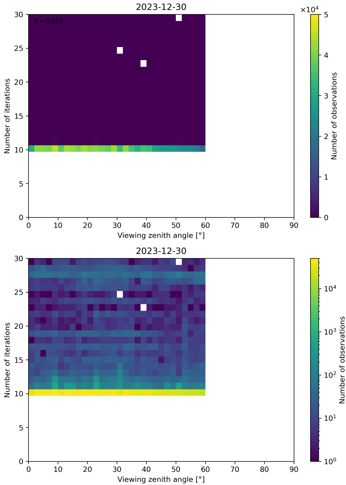
Figure 113: Scatter density plot of “Viewing zenith angle” against “Number of iterations” for 2023-12-30 to 2023-12-31.
