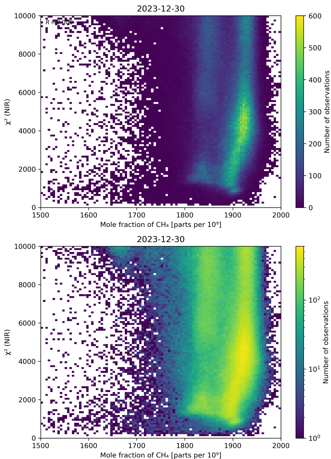
Figure 70: Scatter density plot of “Mole fraction of \text{CH}_4 ” against “ \chi^2 (NIR)” for 2023-12-30 to 2023-12-31.
