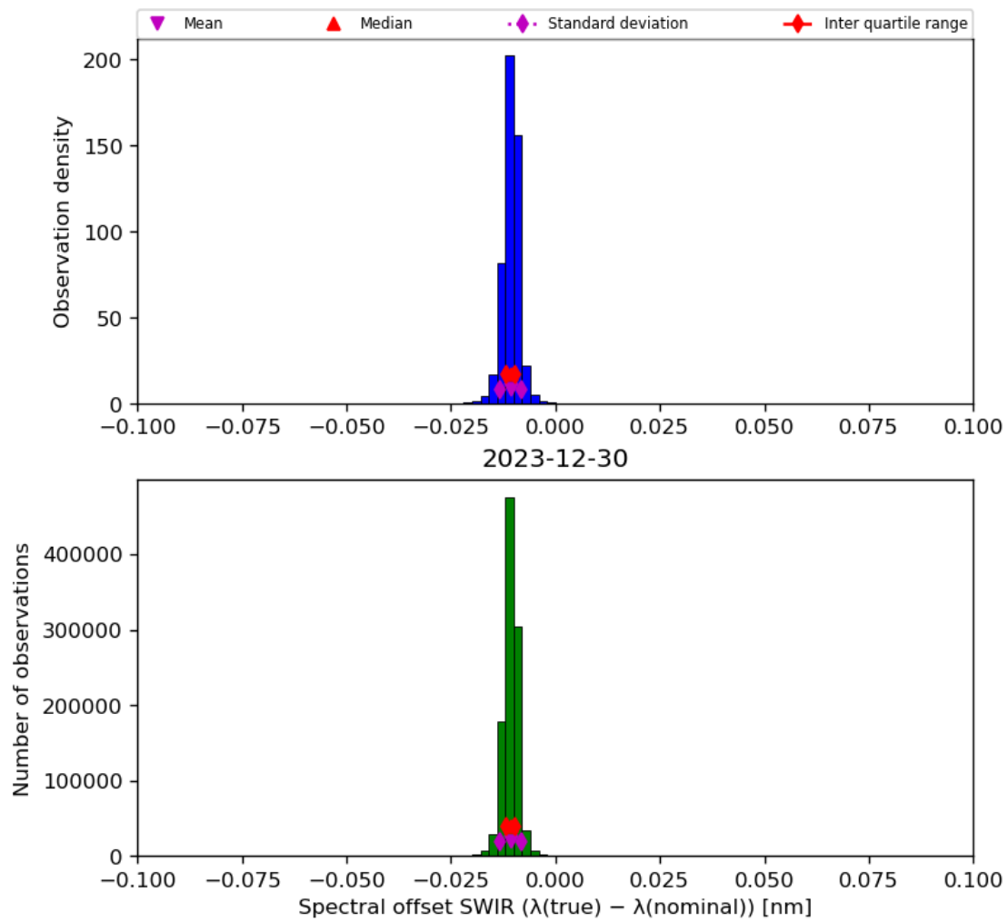
Figure 27: Histogram of “Spectral offset SWIR ( \lambda(\text{true}) - \lambda(\text{nominal}) )” for 2023-12-30 to 2023-12-31
