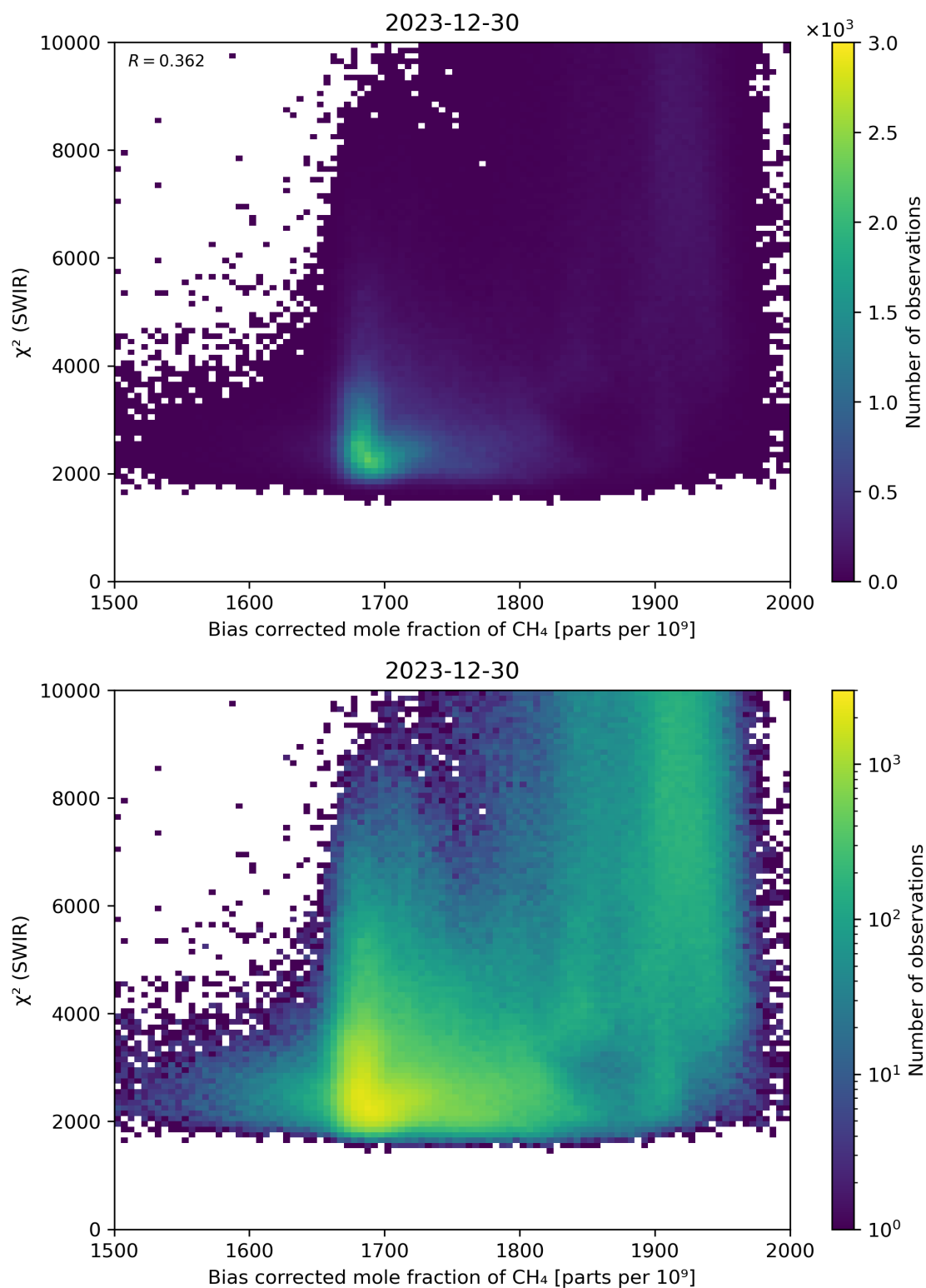
Figure 64: Scatter density plot of “Bias corrected mole fraction of CH 4 ” against “ \chi^2 (SWIR)” for 2023-12-30 to 2023-12-31.
