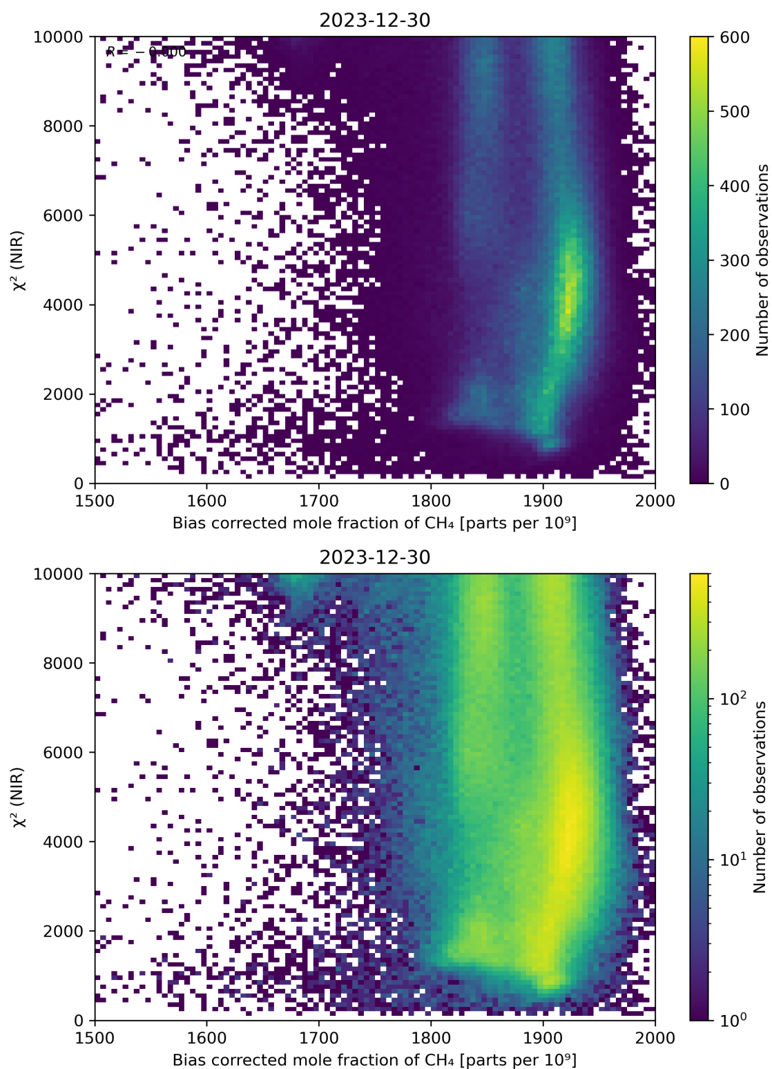
Figure 63: Scatter density plot of “Bias corrected mole fraction of CH 4 ” against “ \chi^2 (NIR)” for 2023-12-30 to 2023-12-31.
