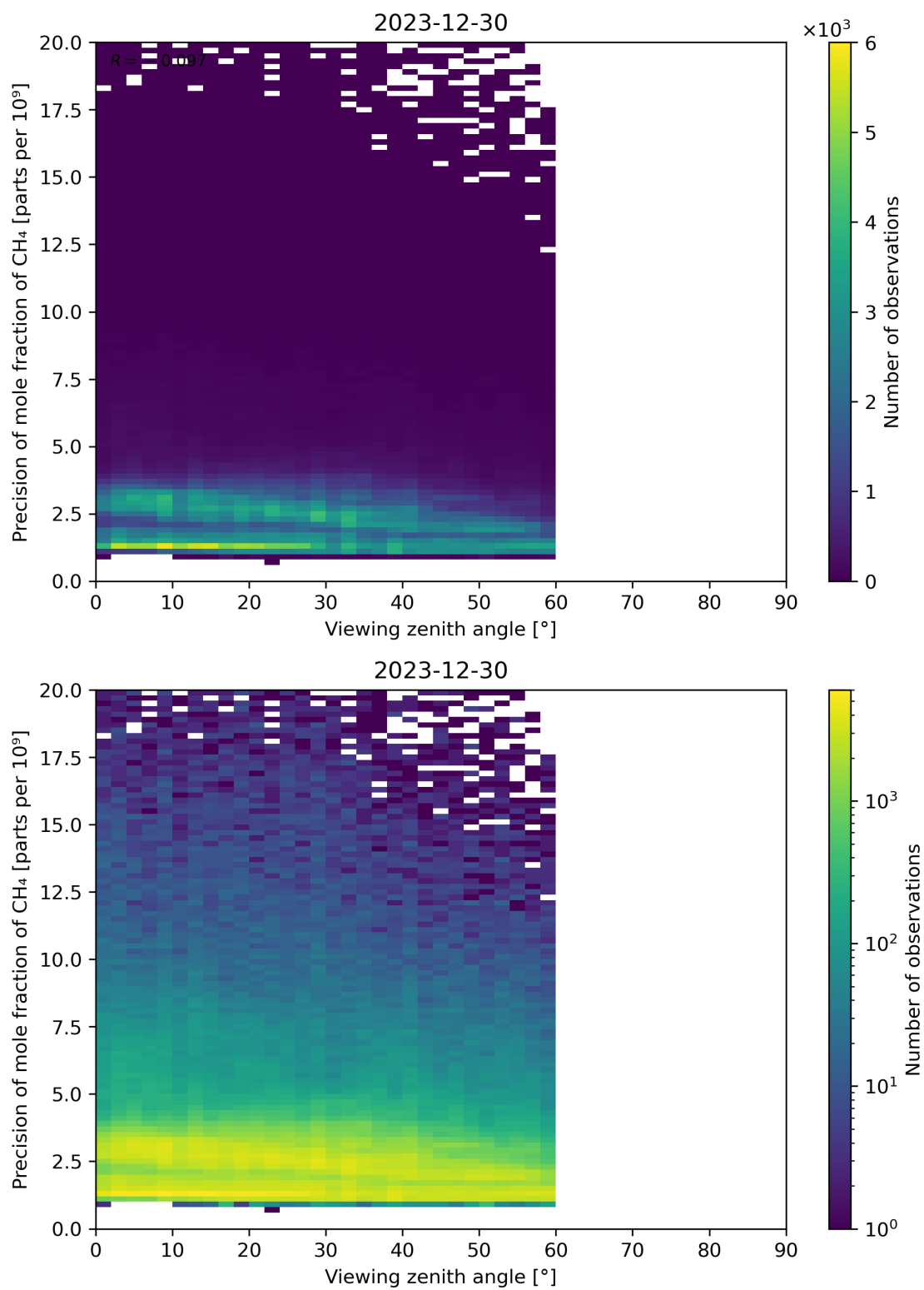
Figure 112: Scatter density plot of “Viewing zenith angle” against “Precision of mole fraction of CH 4 ” for 2023-12-30 to 2023-12-31.
