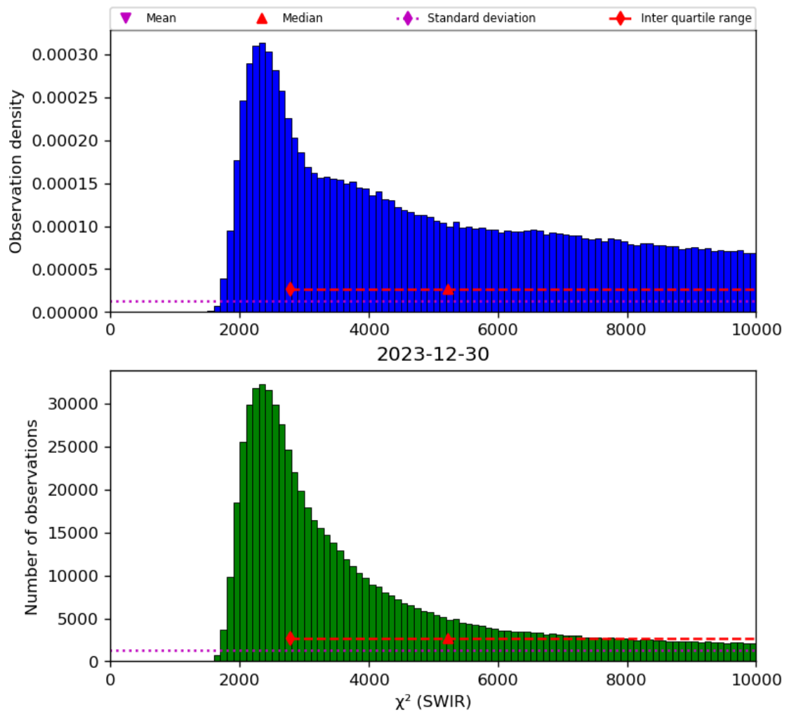
Figure 28: Histogram of “ \chi^2 (SWIR)” for 2023-12-30 to 2023-12-31
