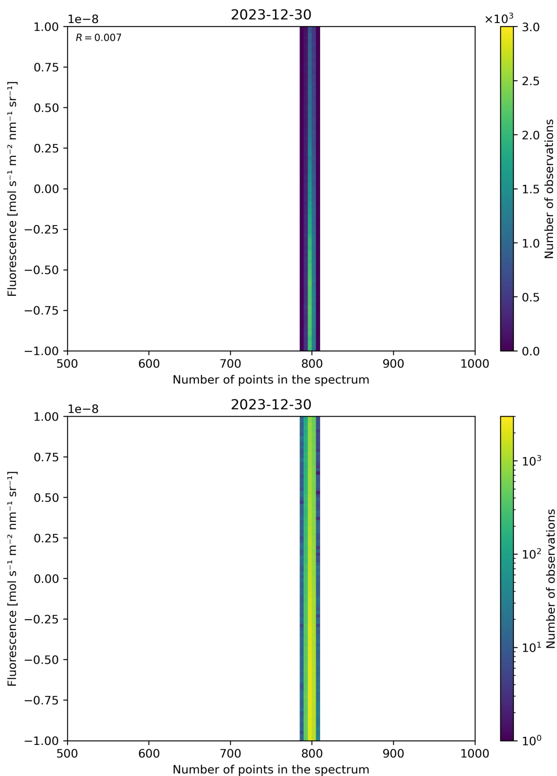
Figure 91: Scatter density plot of “Number of points in the spectrum” against “Fluorescence” for 2023-12-30 to 2023-12-31.
