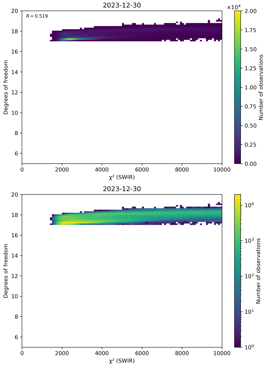
Figure 48: Scatter density plot of “ \chi^2 (SWIR)” against “Degrees of freedom” for 2023-12-30 to 2023-12-31.
