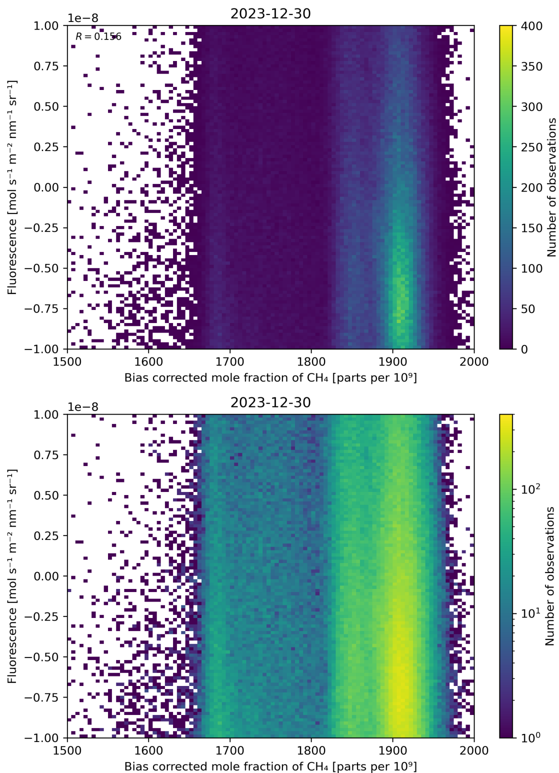
Figure 66: Scatter density plot of “Bias corrected mole fraction of \text{CH}_4 ” against “Fluorescence” for 2023-12-30 to 2023-12-31.
