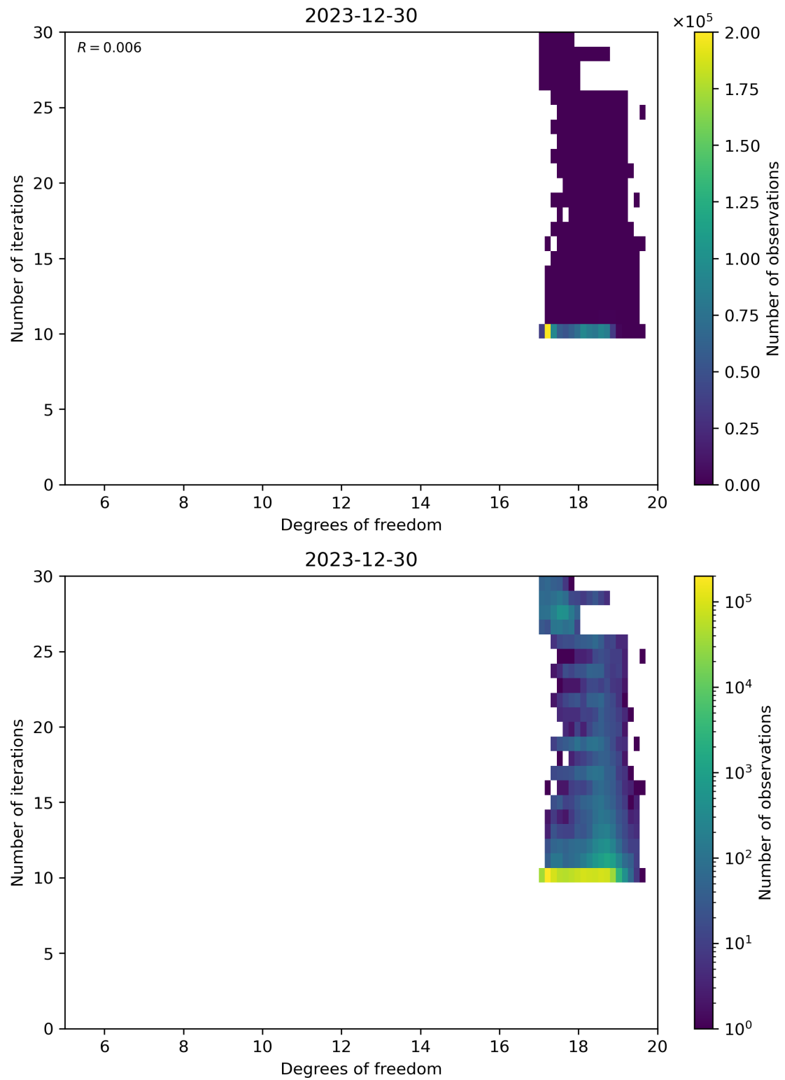
Figure 52: Scatter density plot of “Degrees of freedom” against “Number of iterations” for 2023-12-30 to 2023-12-31.
