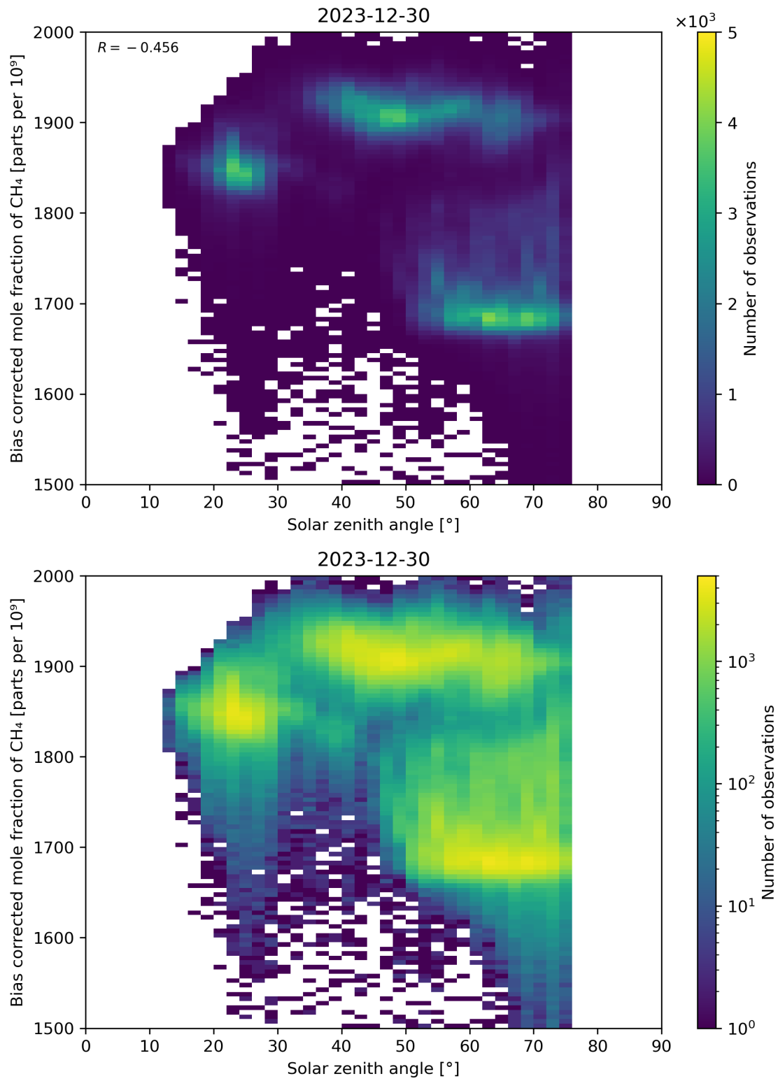
Figure 100: Scatter density plot of “Solar zenith angle” against “Bias corrected mole fraction of CH 4 ” for 2023-12-30 to 2023-12-31.
