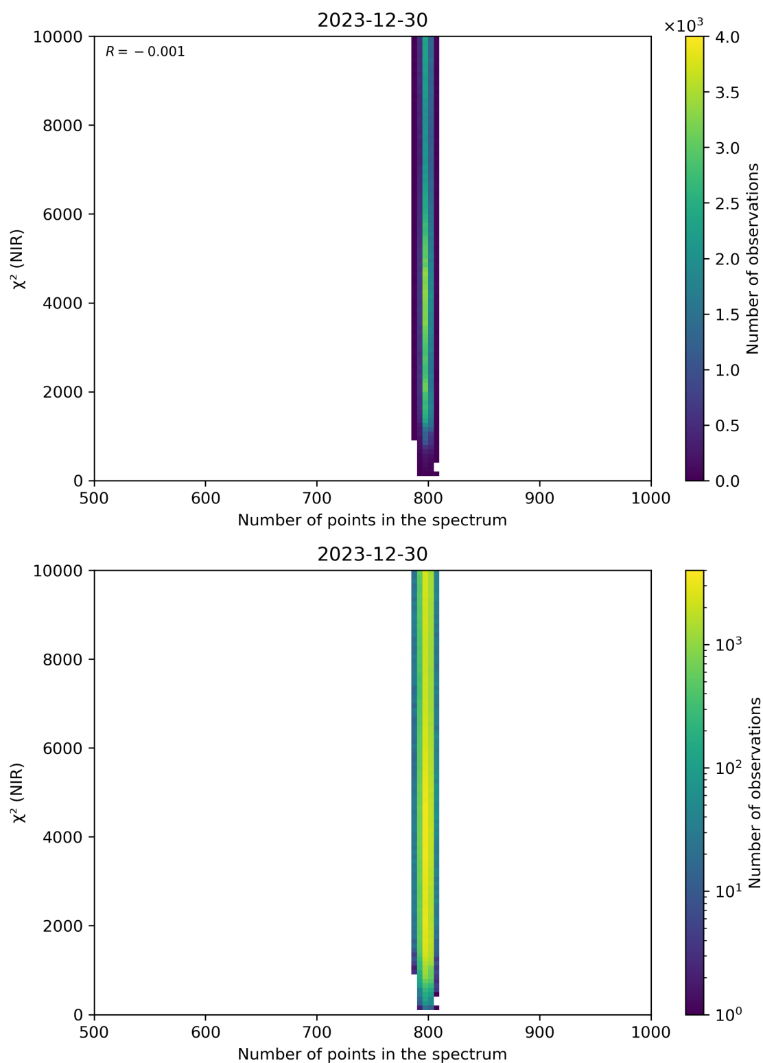
Figure 88: Scatter density plot of “Number of points in the spectrum” against “ \chi^2 (NIR)” for 2023-12-30 to 2023-12-31.
