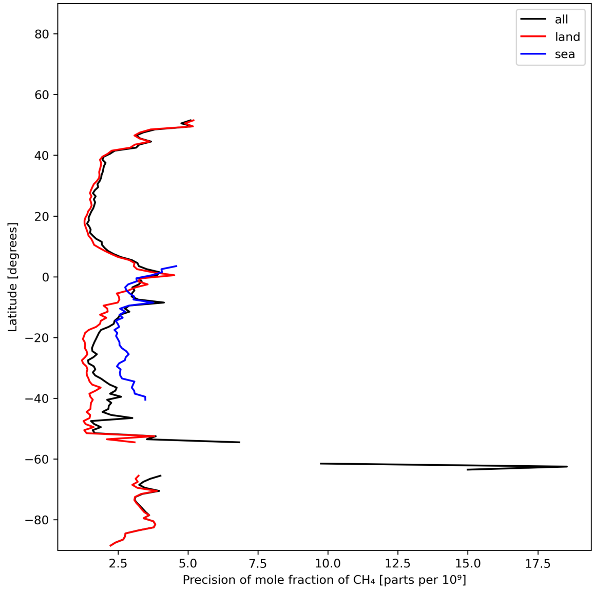
Figure 13: Zonal average of “Precision of mole fraction of \text{CH}_4 ” for 2023-12-30 to 2023-12-31.
