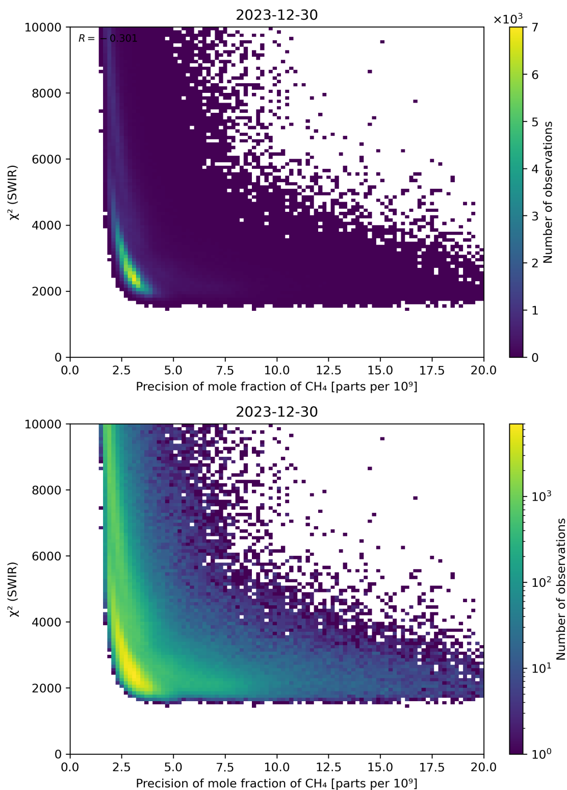
Figure 79: Scatter density plot of “Precision of mole fraction of \text{CH}_4 ” against “ \chi^2 (SWIR)” for 2023-12-30 to 2023-12-31.
