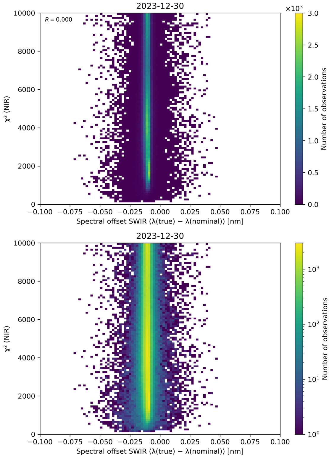
Figure 117: Scatter density plot of “Spectral offset SWIR ( \lambda(\text{true}) - \lambda(\text{nominal}) )” against “ \chi^2 (NIR)” for 2023-12-30 to 2023-12-31.
