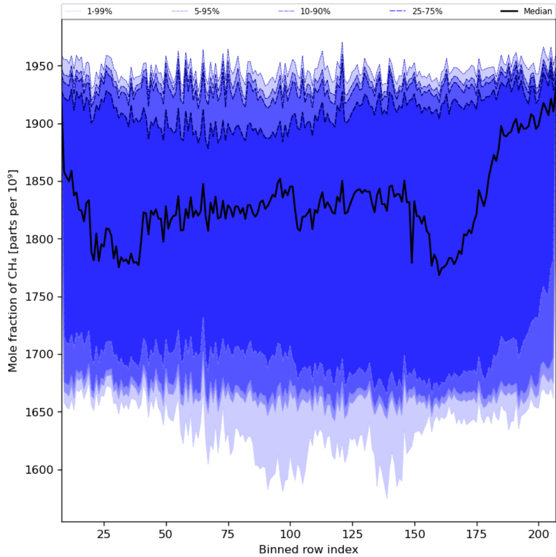
Figure 34: Along track statistics of “Mole fraction of CH 4 ” for 2023-12-30 to 2023-12-31
