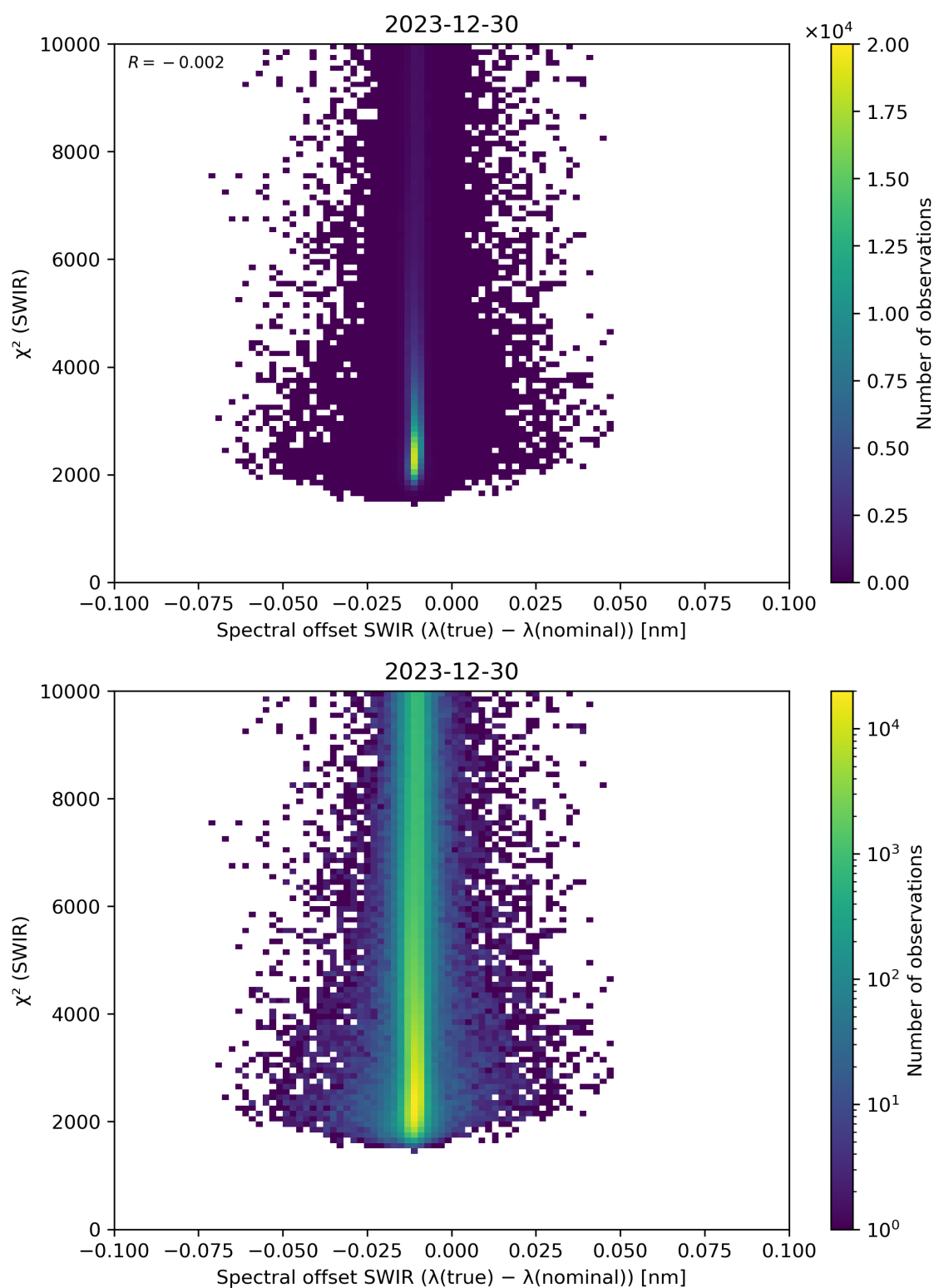
Figure 118: Scatter density plot of “Spectral offset SWIR ( \lambda(\text{true}) - \lambda(\text{nominal}) )” against “ \chi^2 (SWIR)” for 2023-12-30 to 2023-12-31.
