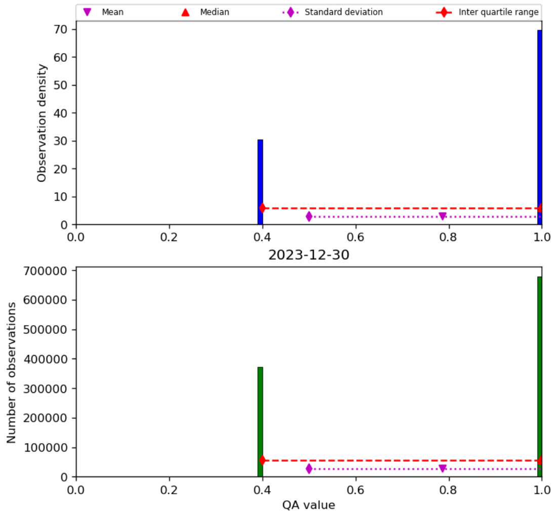
Figure 22: Histogram of “QA value” for 2023-12-30 to 2023-12-31
