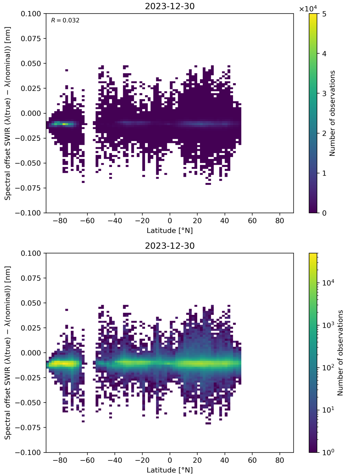
Figure 62: Scatter density plot of “Latitude” against “Spectral offset SWIR ( \lambda(\text{true}) - \lambda(\text{nominal}) )” for 2023-12-30 to 2023-12-31.
