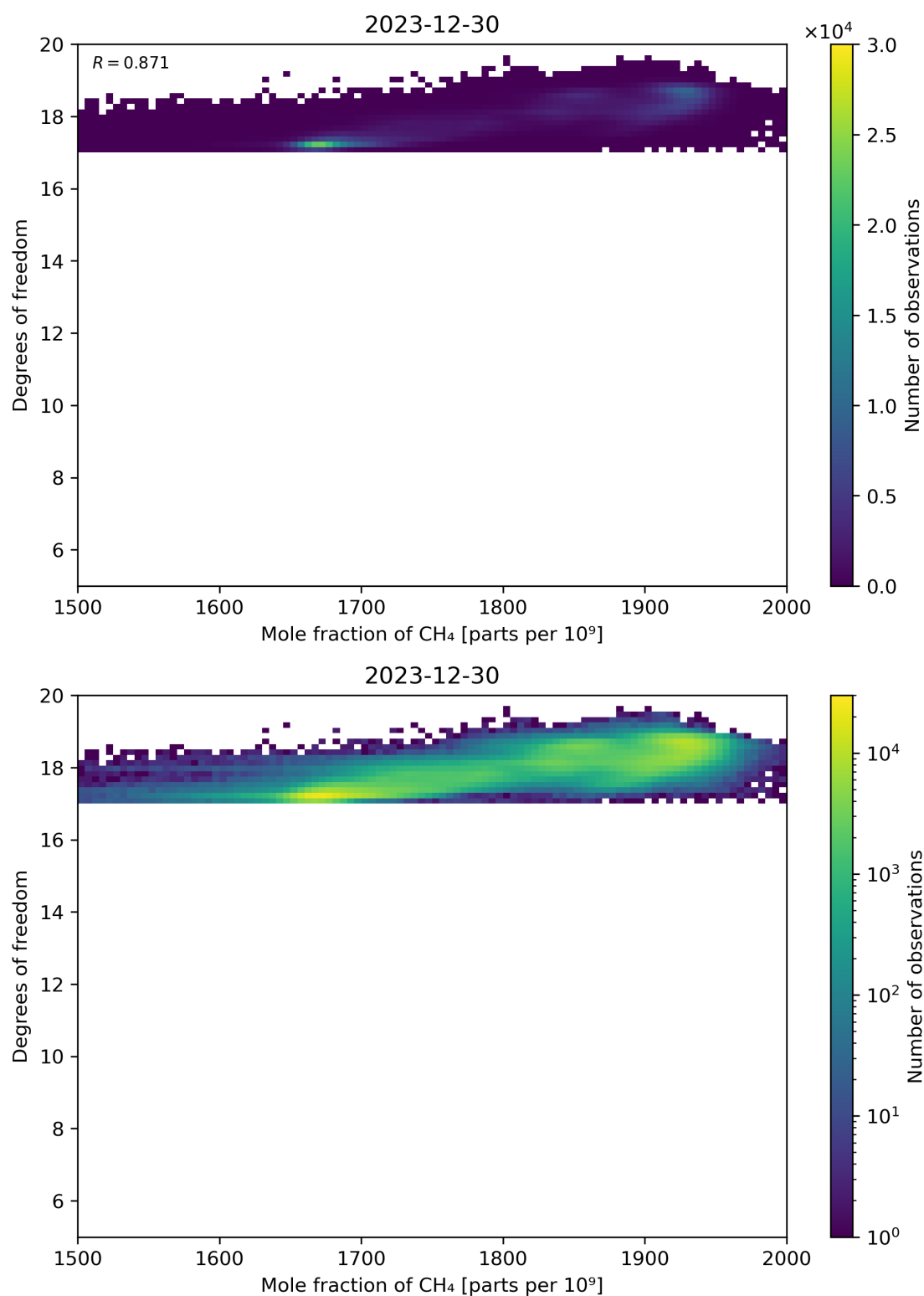
Figure 72: Scatter density plot of “Mole fraction of CH 4 ” against “Degrees of freedom” for 2023-12-30 to 2023-12-31.
