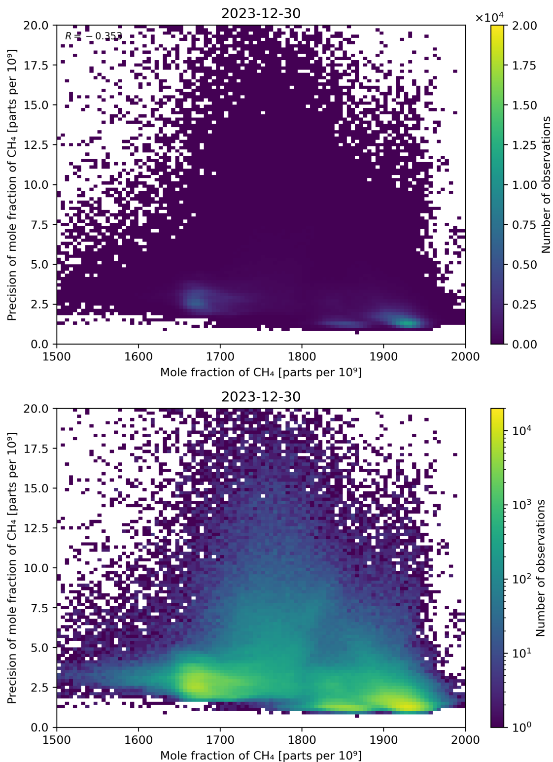
Figure 75: Scatter density plot of “Mole fraction of CH 4 ” against “Precision of mole fraction of CH 4 ” for 2023-12-30 to 2023-12-31.
