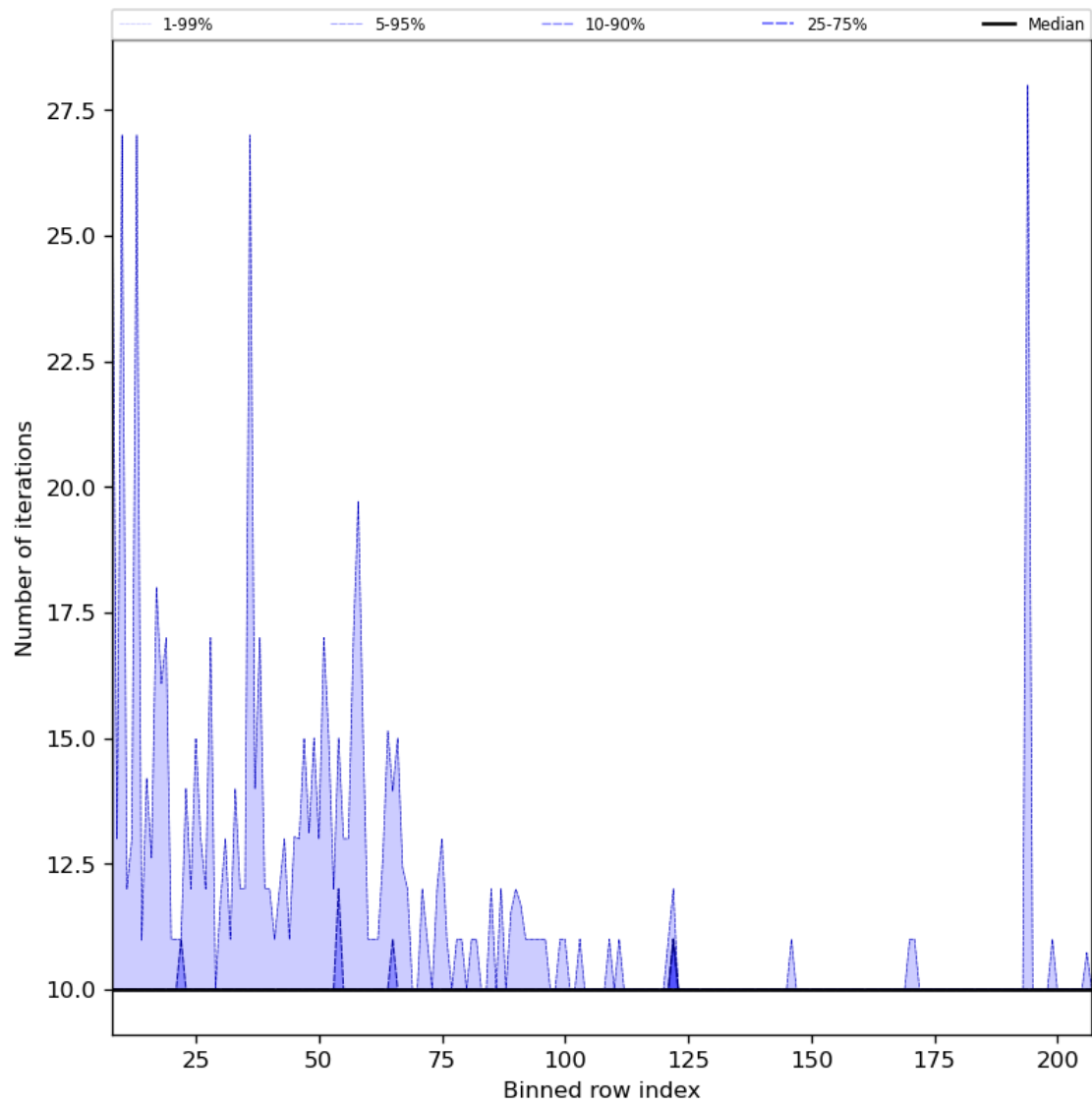
Figure 42: Along track statistics of “Number of iterations” for 2023-12-30 to 2023-12-31
