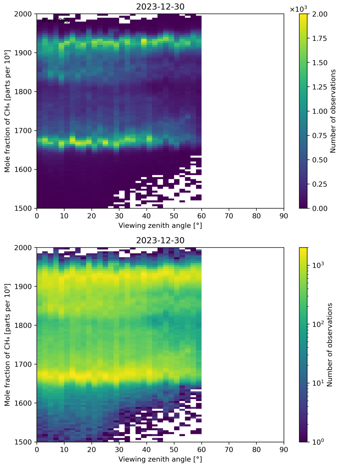
Figure 110: Scatter density plot of “Viewing zenith angle” against “Mole fraction of CH 4 ” for 2023-12-30 to 2023-12-31.
