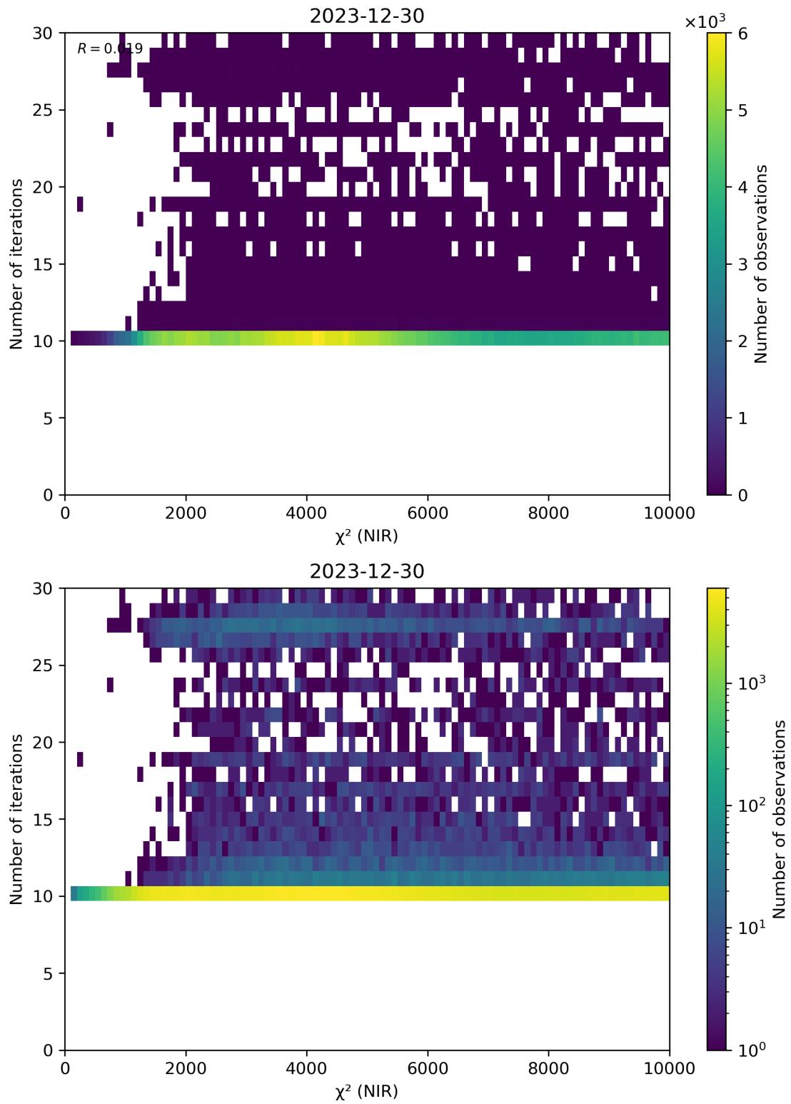
Figure 46: Scatter density plot of “ \chi^2 (NIR)” against “Number of iterations” for 2023-12-30 to 2023-12-31.
