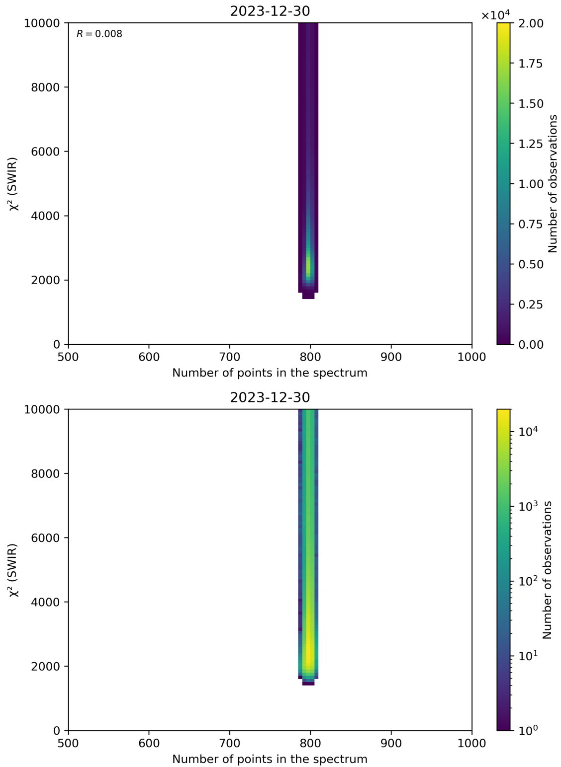
Figure 89: Scatter density plot of “Number of points in the spectrum” against “ \chi^2 (SWIR)” for 2023-12-30 to 2023-12-31.
