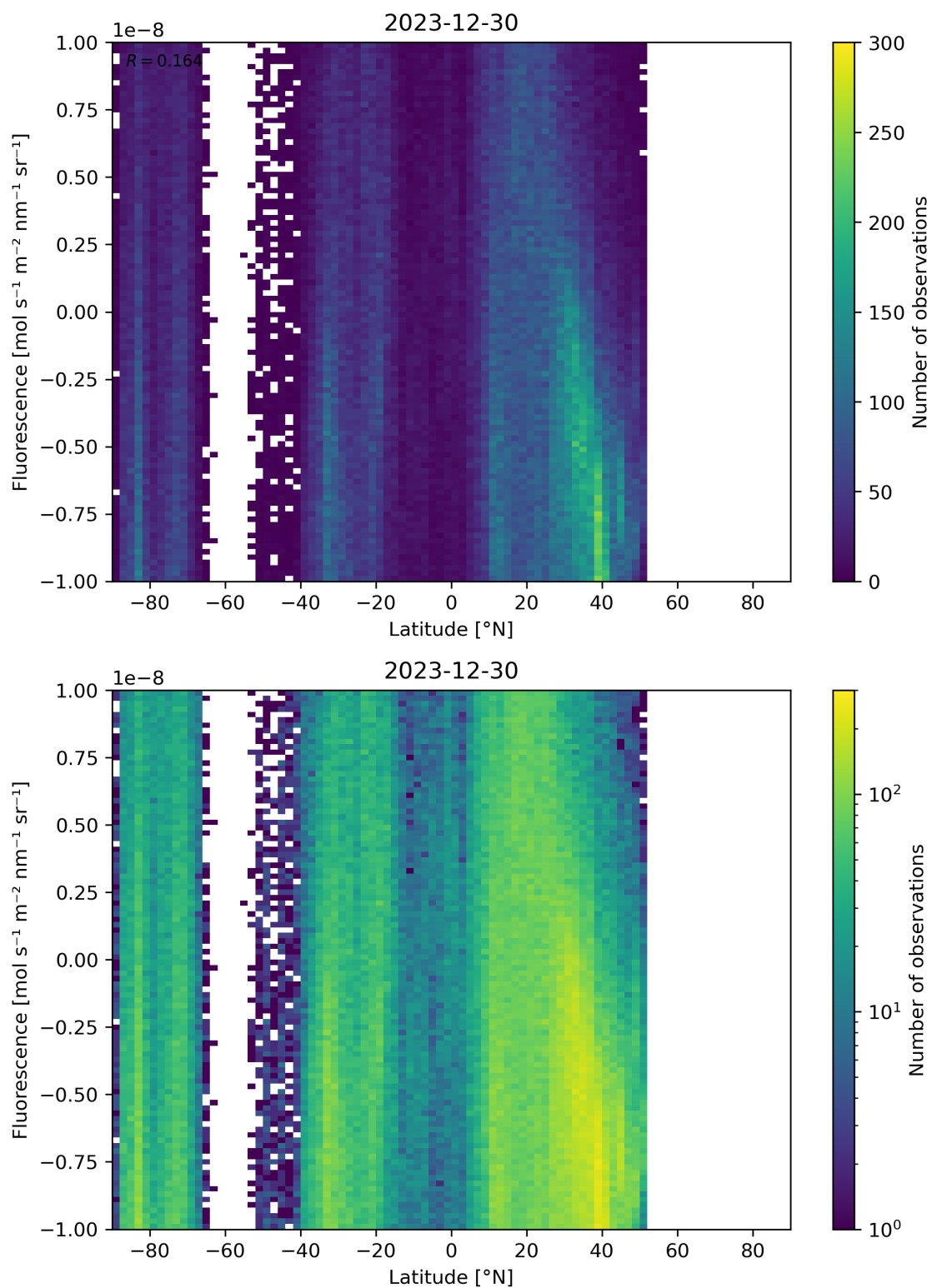
Figure 56: Scatter density plot of “Latitude” against “Fluorescence” for 2023-12-30 to 2023-12-31.
