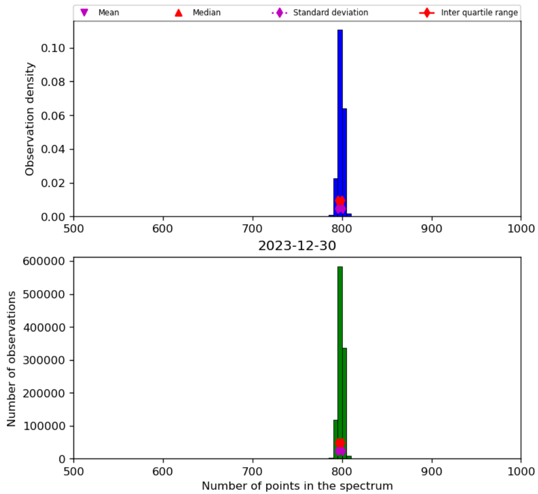
Figure 26: Histogram of “Number of points in the spectrum” for 2023-12-30 to 2023-12-31
