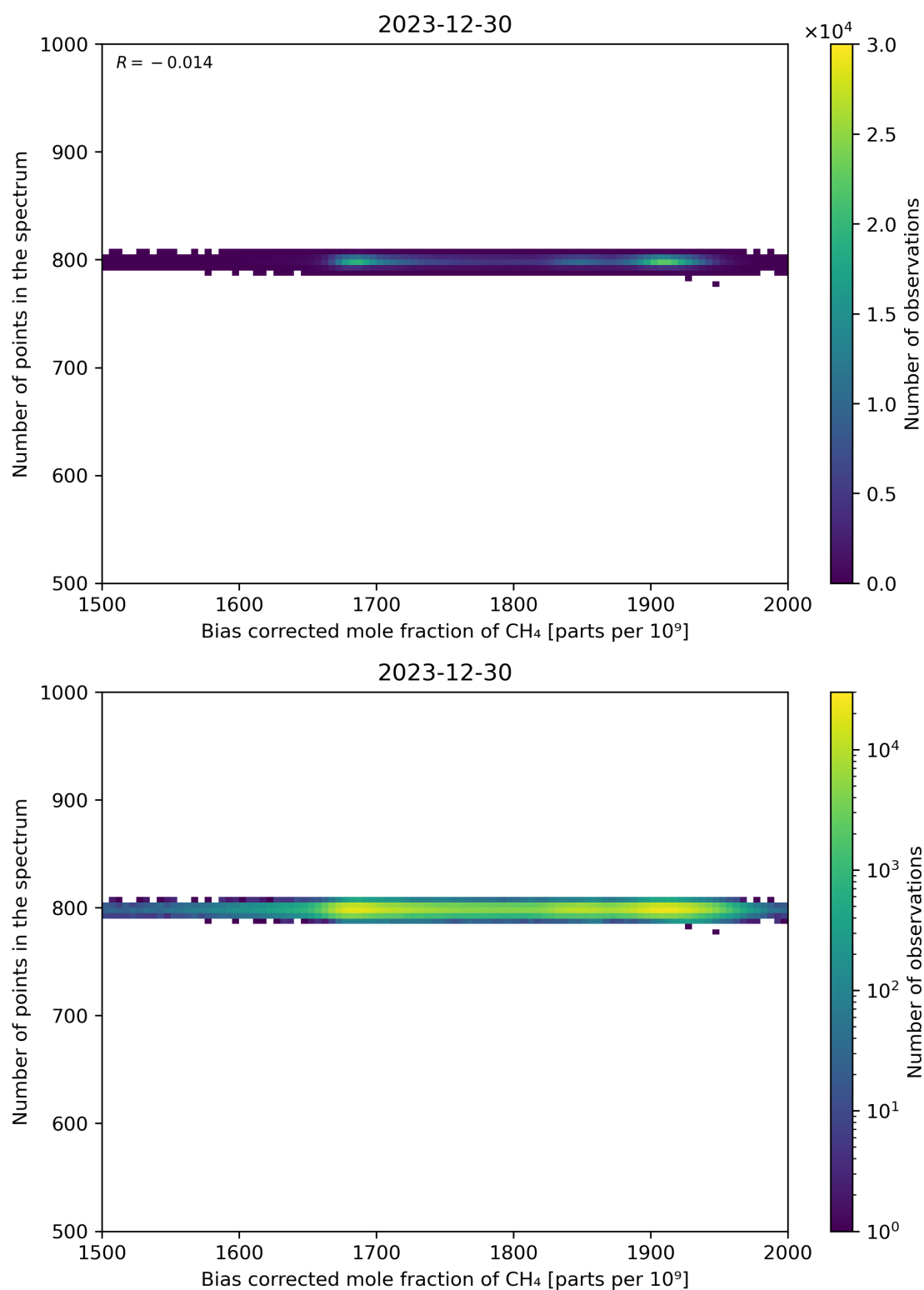
Figure 68: Scatter density plot of “Bias corrected mole fraction of CH 4 ” against “Number of points in the spectrum” for 2023-12-30 to 2023-12-31.
