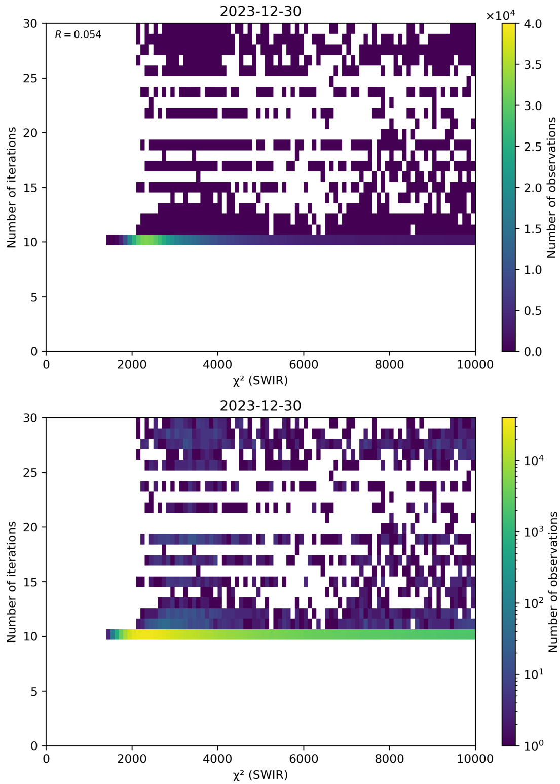
Figure 50: Scatter density plot of “ \chi^2 (SWIR)” against “Number of iterations” for 2023-12-30 to 2023-12-31.
