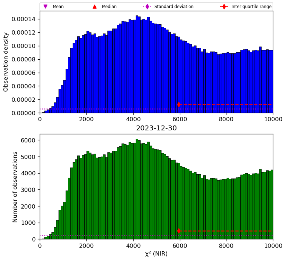
Figure 29: Histogram of “ \chi^2 (NIR)” for 2023-12-30 to 2023-12-31
