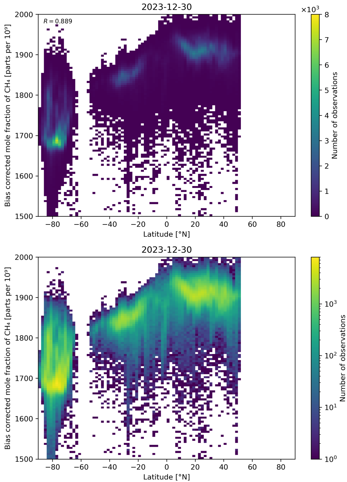
Figure 58: Scatter density plot of “Latitude” against “Bias corrected mole fraction of \text{CH}_4 ” for 2023-12-30 to 2023-12-31.
