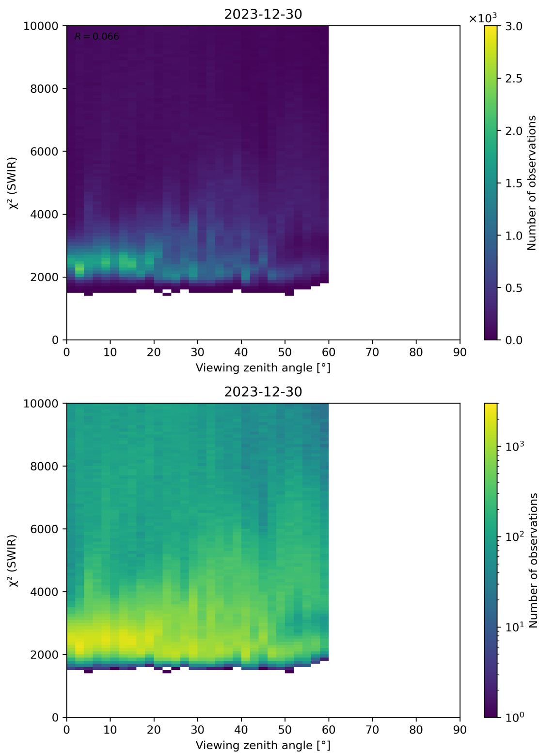
Figure 106: Scatter density plot of “Viewing zenith angle” against “ \chi^2 (SWIR)” for 2023-12-30 to 2023-12-31.
