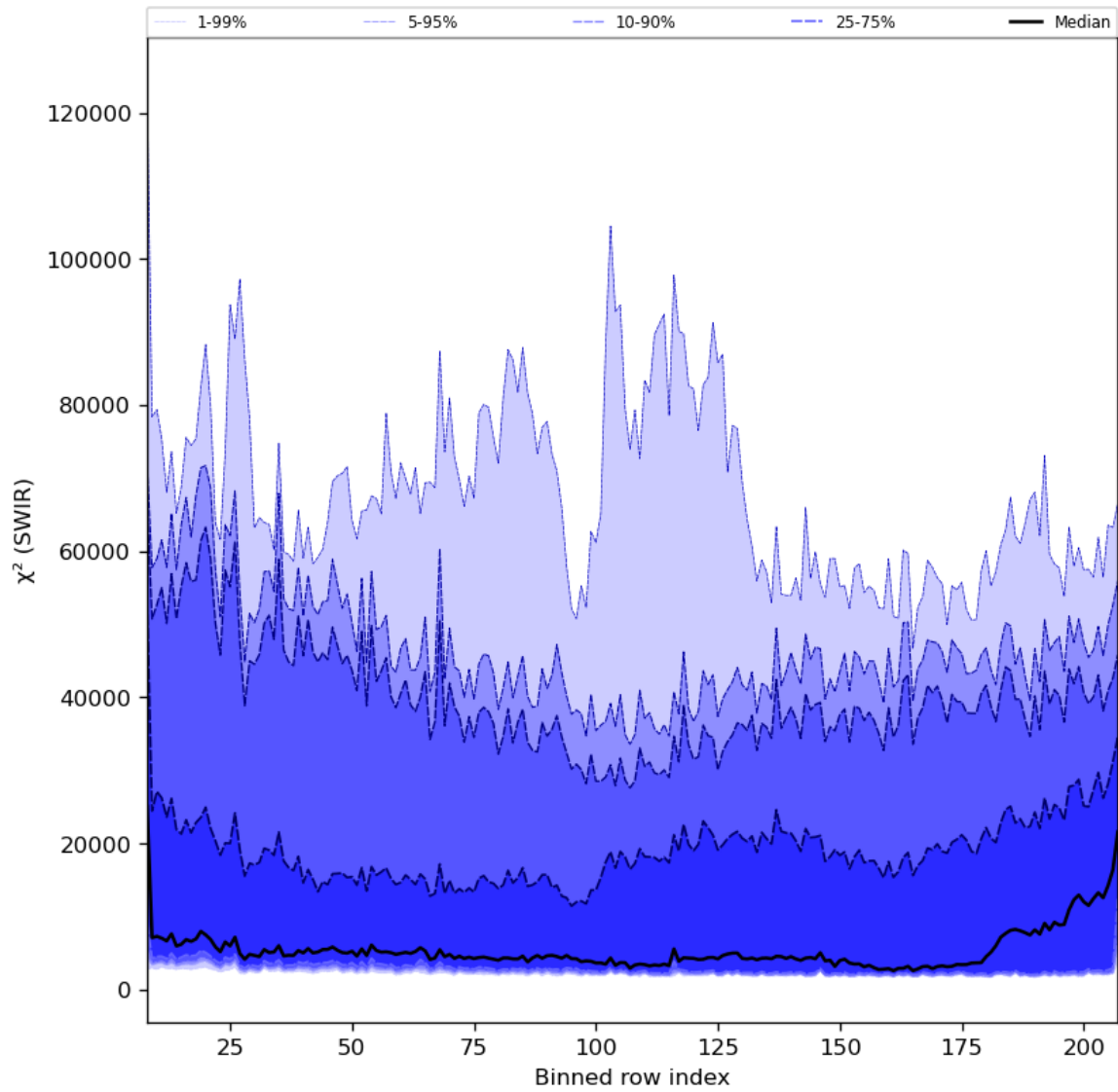
Figure 39: Along track statistics of “ \chi^2 (SWIR)” for 2023-12-30 to 2023-12-31
