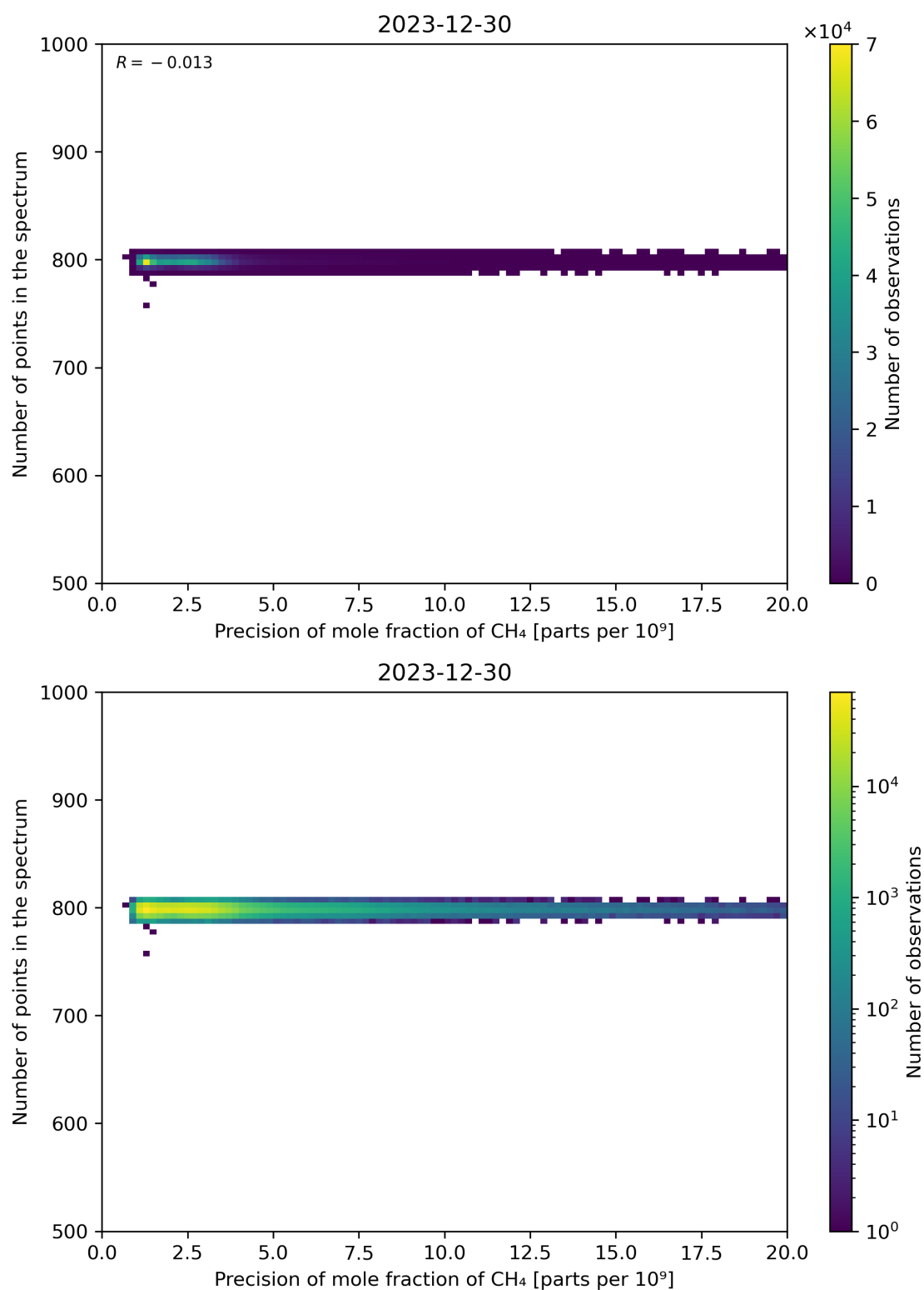
Figure 84: Scatter density plot of “Precision of mole fraction of CH 4 ” against “Number of points in the spectrum” for 2023-12-30 to 2023-12-31.
