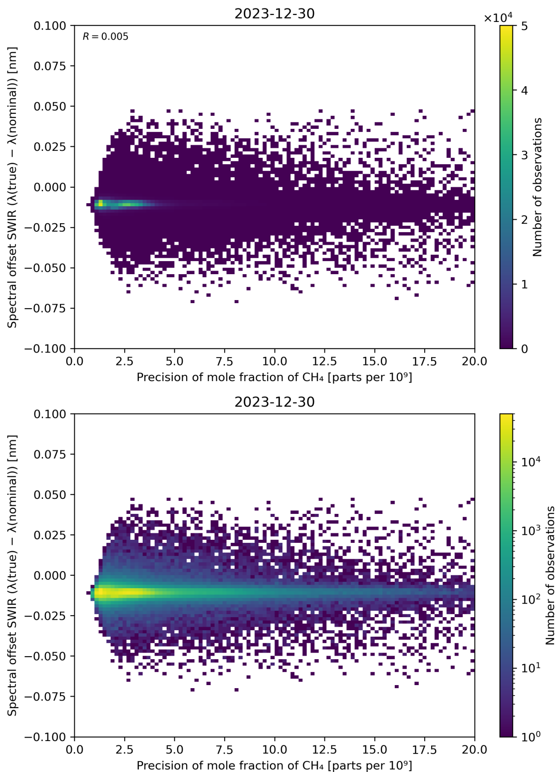
Figure 85: Scatter density plot of “Precision of mole fraction of \text{CH}_4 ” against “Spectral offset SWIR ( \lambda(\text{true}) - \lambda(\text{nominal}) )” for 2023-12-30 to 2023-12-31.
