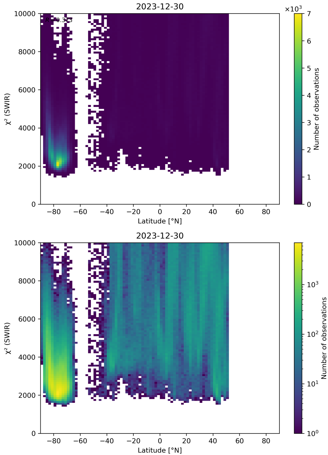
Figure 54: Scatter density plot of “Latitude” against “ \chi^2 (SWIR)” for 2023-12-30 to 2023-12-31.
