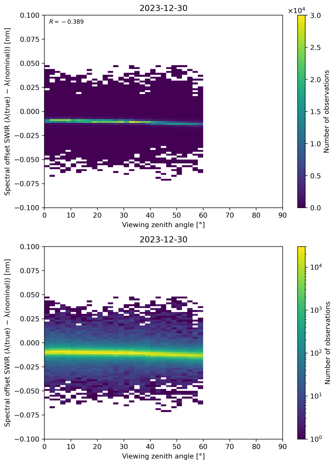
Figure 116: Scatter density plot of “Viewing zenith angle” against “Spectral offset SWIR ( \lambda(\text{true}) - \lambda(\text{nominal}) )” for 2023-12-30 to 2023-12-31.
