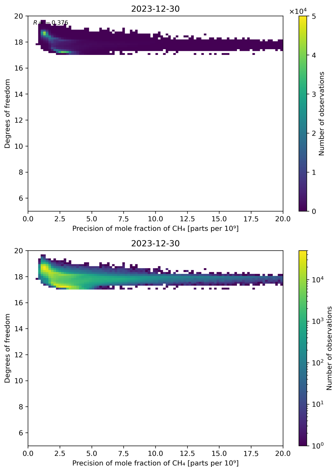
Figure 80: Scatter density plot of “Precision of mole fraction of CH 4 ” against “Degrees of freedom” for 2023-12-30 to 2023-12-31.
