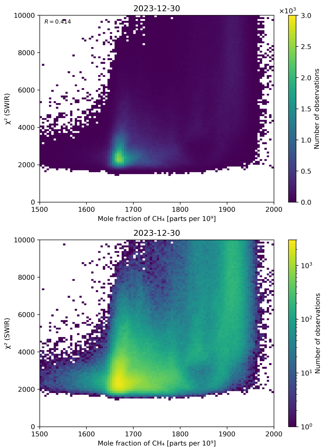
Figure 71: Scatter density plot of “Mole fraction of \text{CH}_4 ” against “ \chi^2 (SWIR)” for 2023-12-30 to 2023-12-31.
