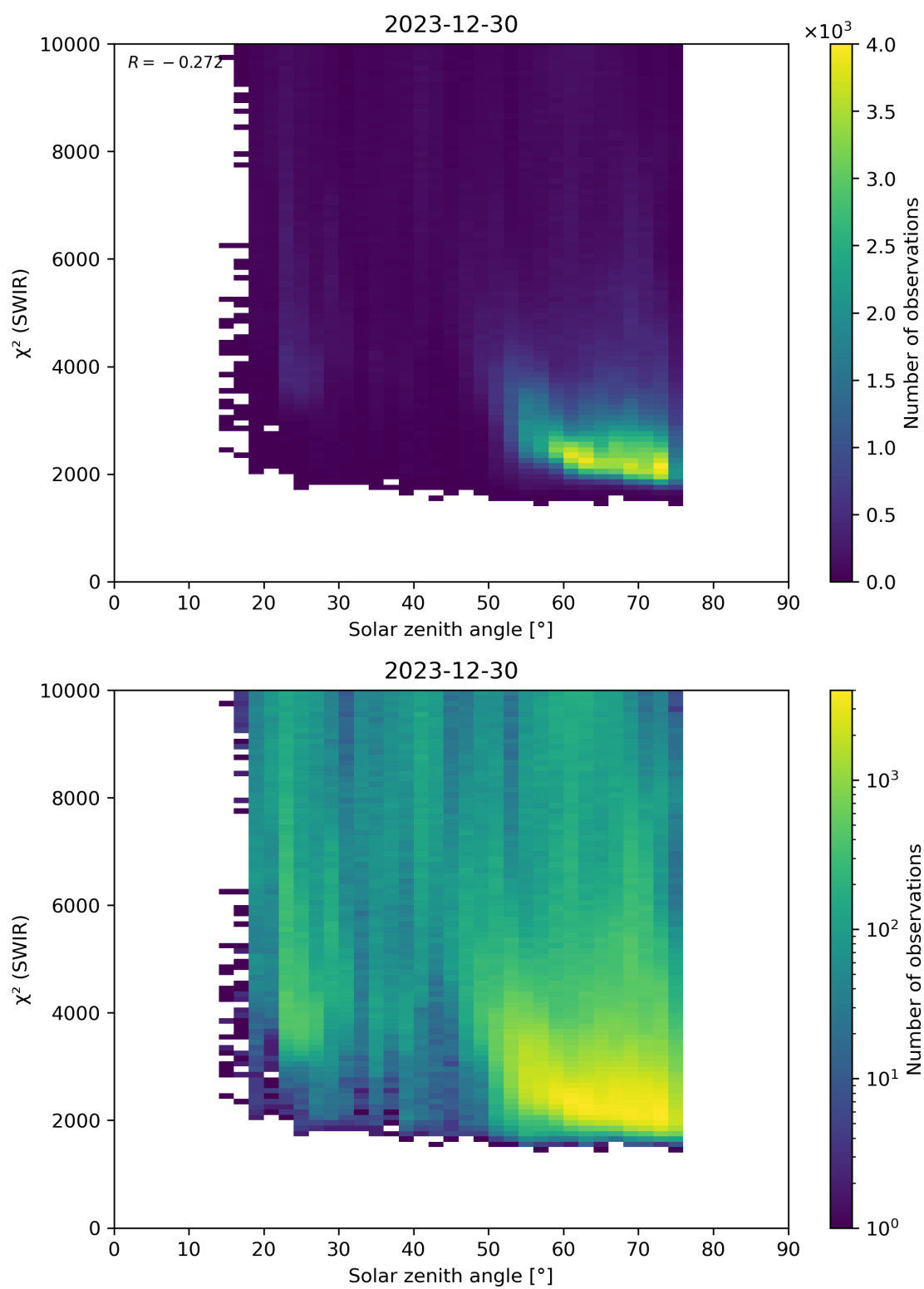
Figure 95: Scatter density plot of “Solar zenith angle” against “ \chi^2 (SWIR)” for 2023-12-30 to 2023-12-31.
