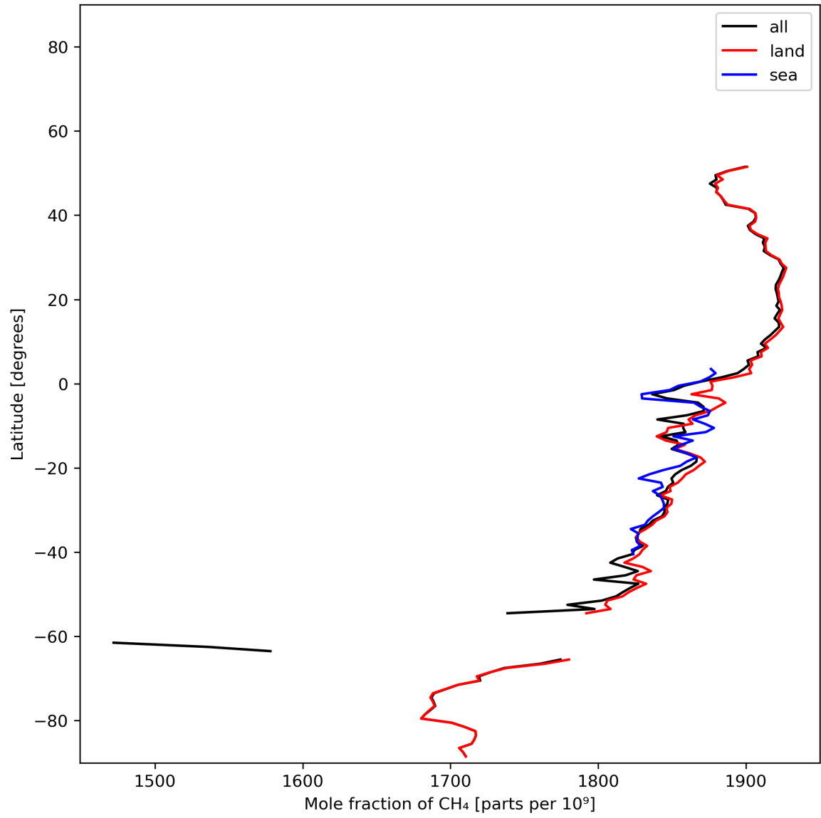
Figure 12: Zonal average of “Mole fraction of \text{CH}_4 ” for 2023-12-30 to 2023-12-31.
