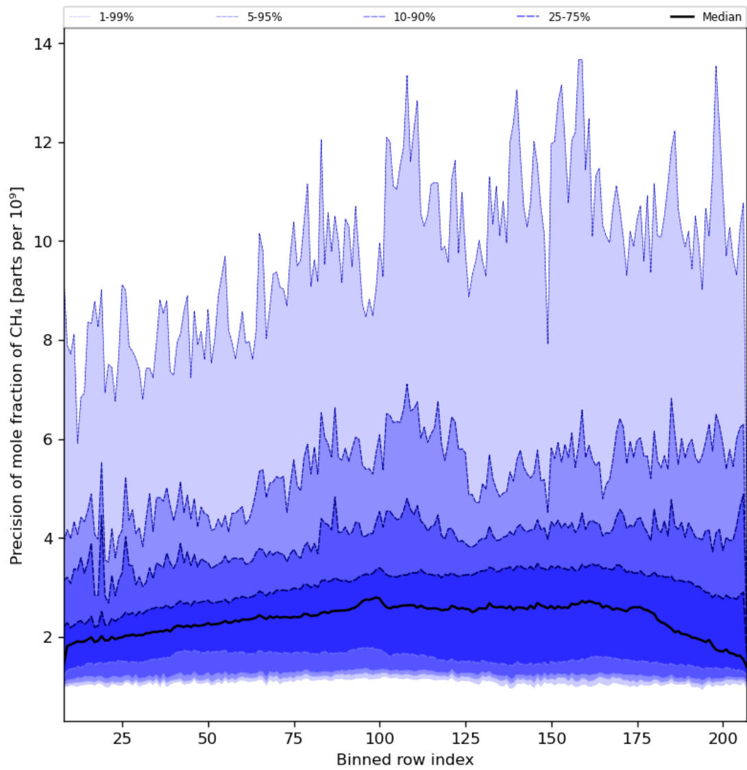
Figure 35: Along track statistics of “Precision of mole fraction of CH 4 ” for 2023-12-30 to 2023-12-31
