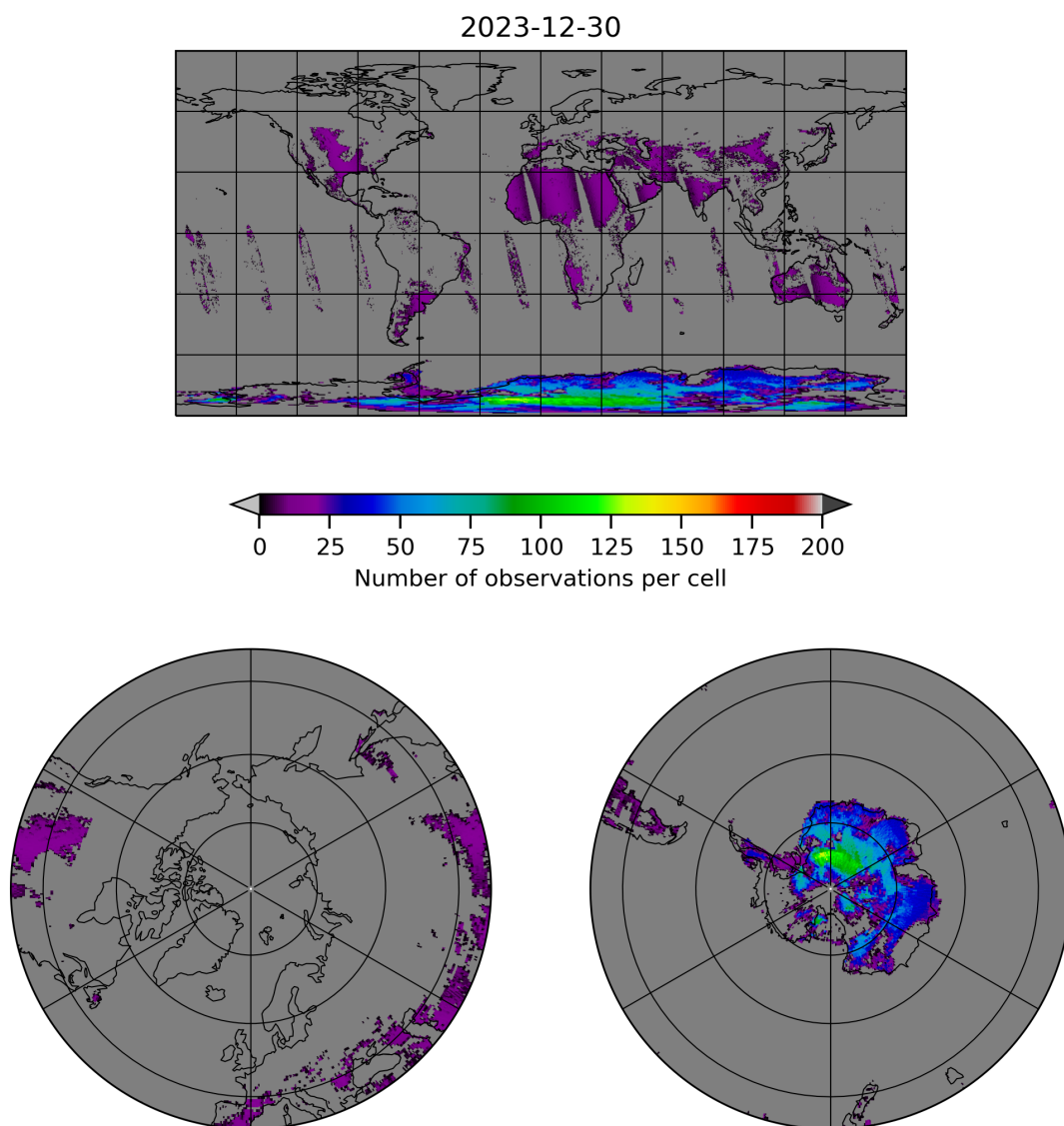
Figure 10: Map of the number of observations for 2023-12-30 to 2023-12-31
