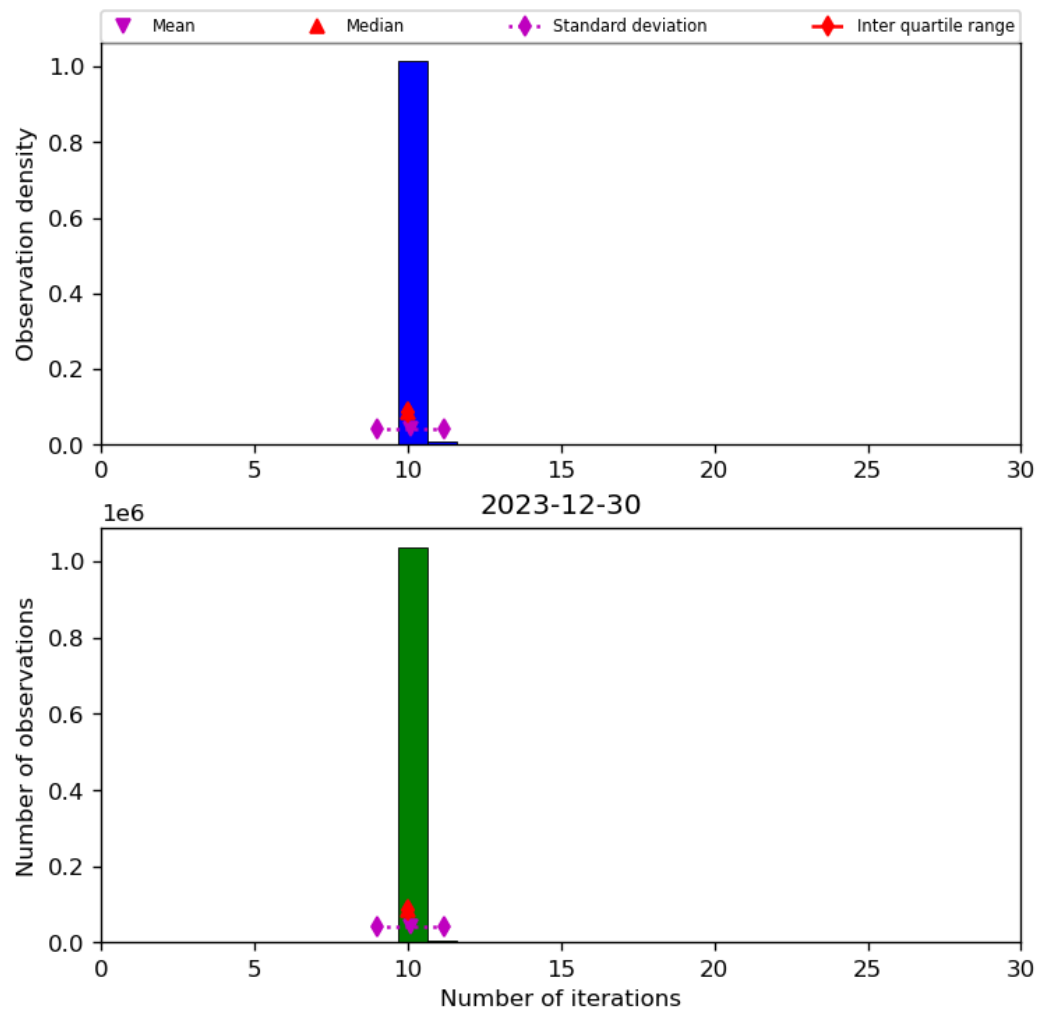
Figure 31: Histogram of “Number of iterations” for 2023-12-30 to 2023-12-31
