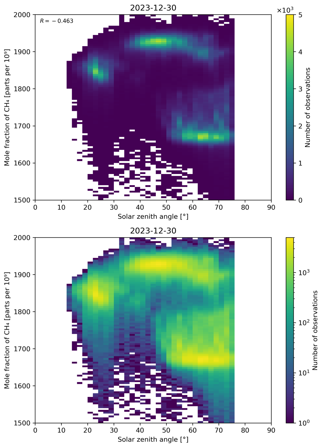
Figure 99: Scatter density plot of “Solar zenith angle” against “Mole fraction of CH 4 ” for 2023-12-30 to 2023-12-31.
