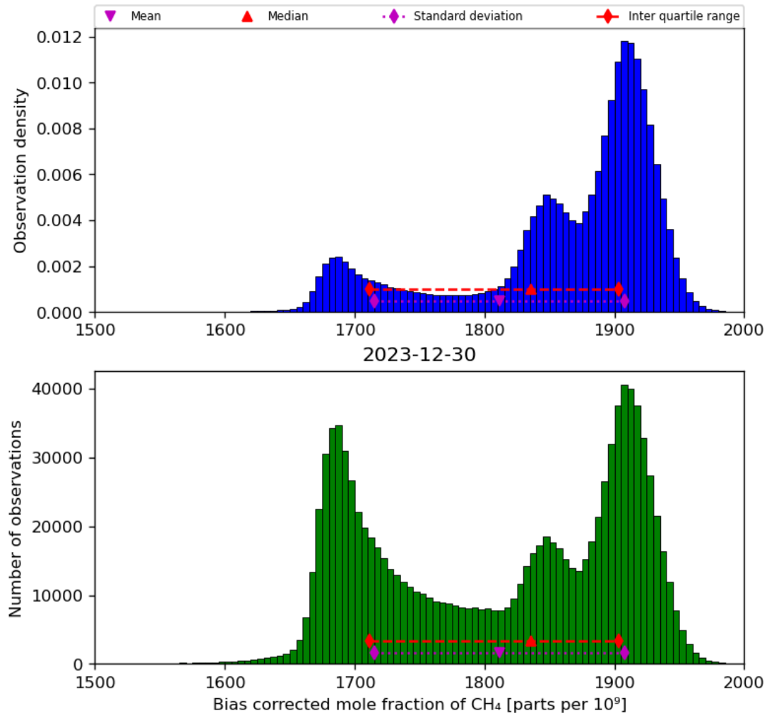
Figure 25: Histogram of “Bias corrected mole fraction of CH 4 ” for 2023-12-30 to 2023-12-31
