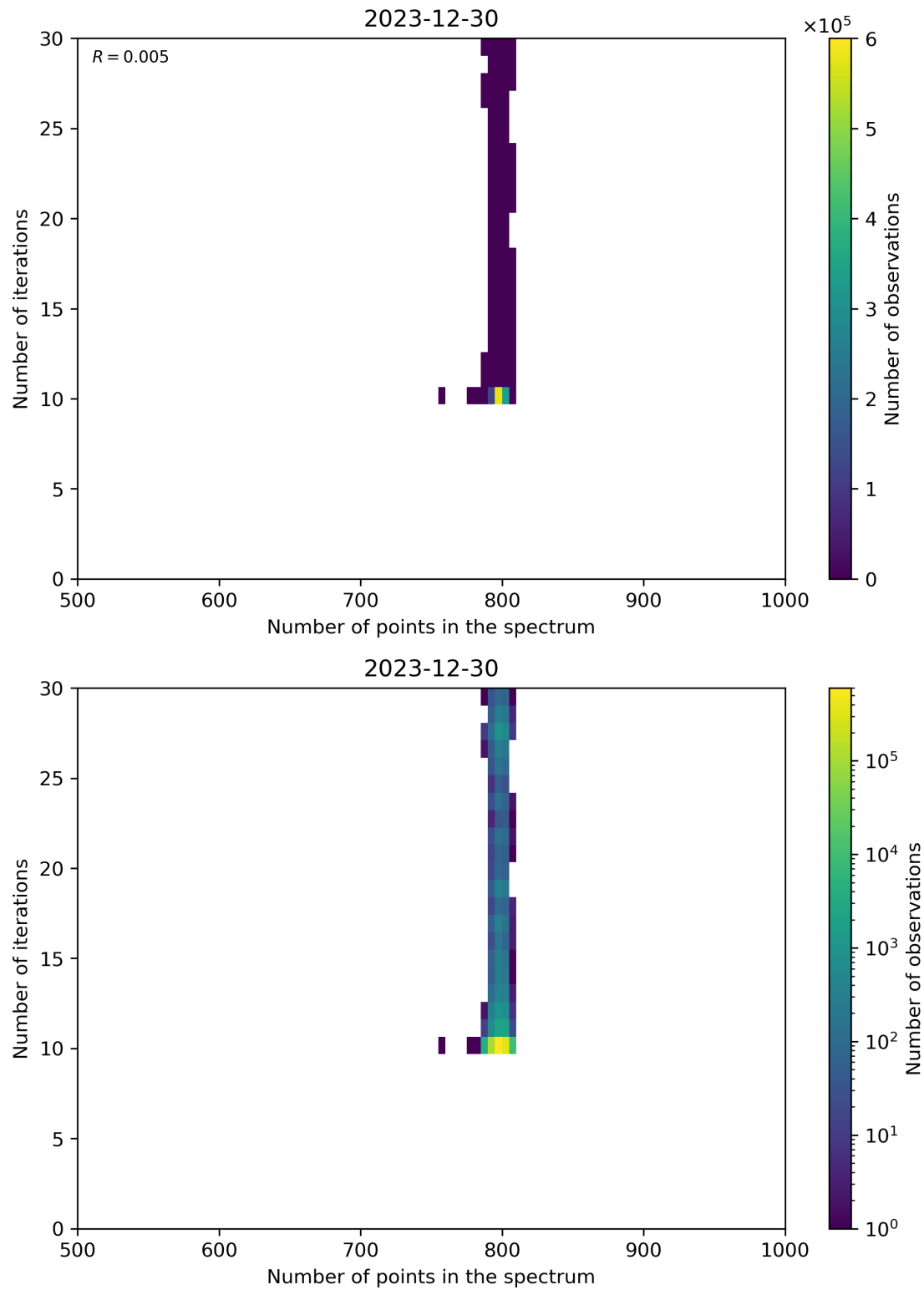
Figure 92: Scatter density plot of “Number of points in the spectrum” against “Number of iterations” for 2023-12-30 to 2023-12-31.
