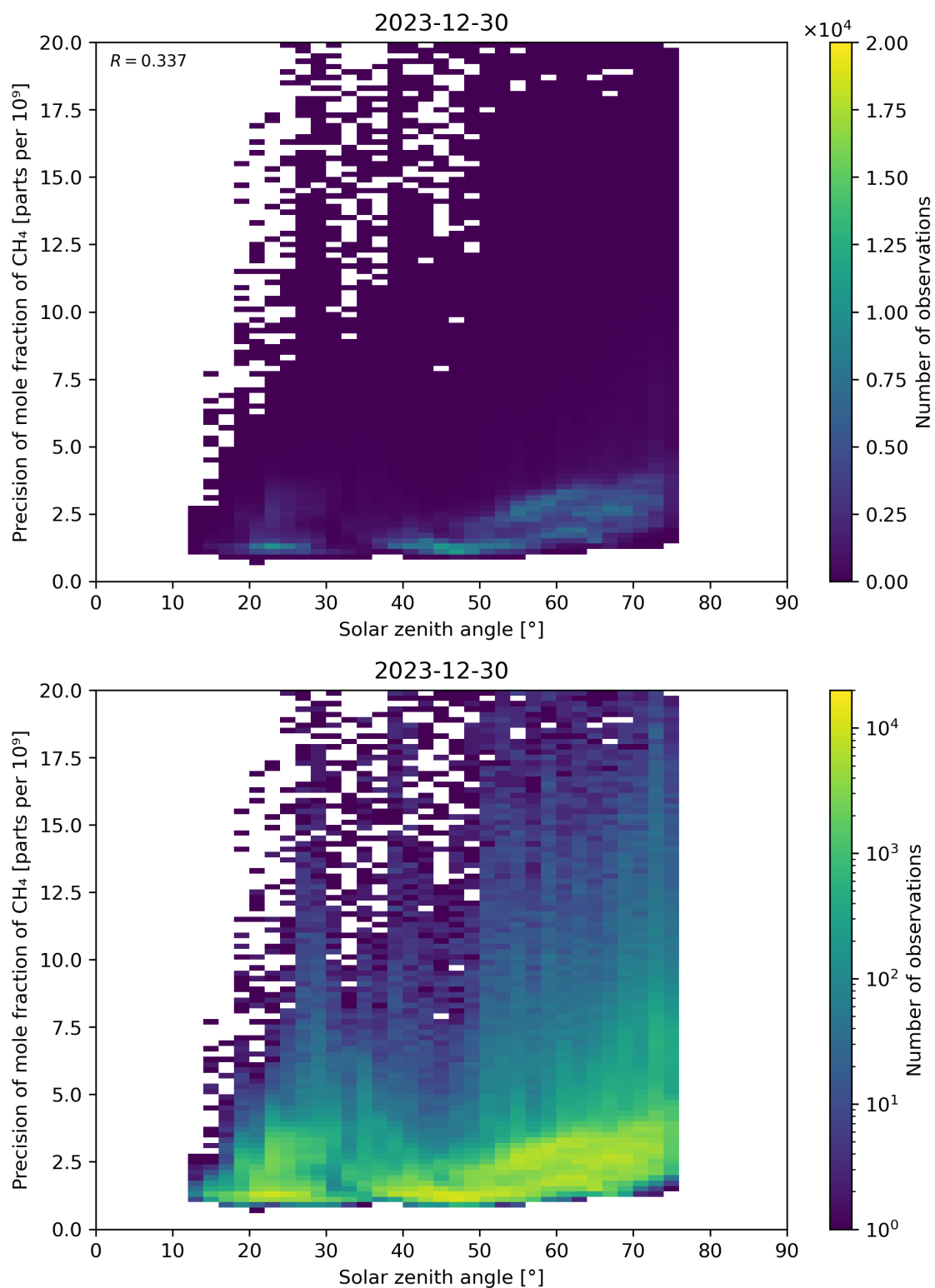
Figure 101: Scatter density plot of “Solar zenith angle” against “Precision of mole fraction of CH 4 ” for 2023-12-30 to 2023-12-31.
