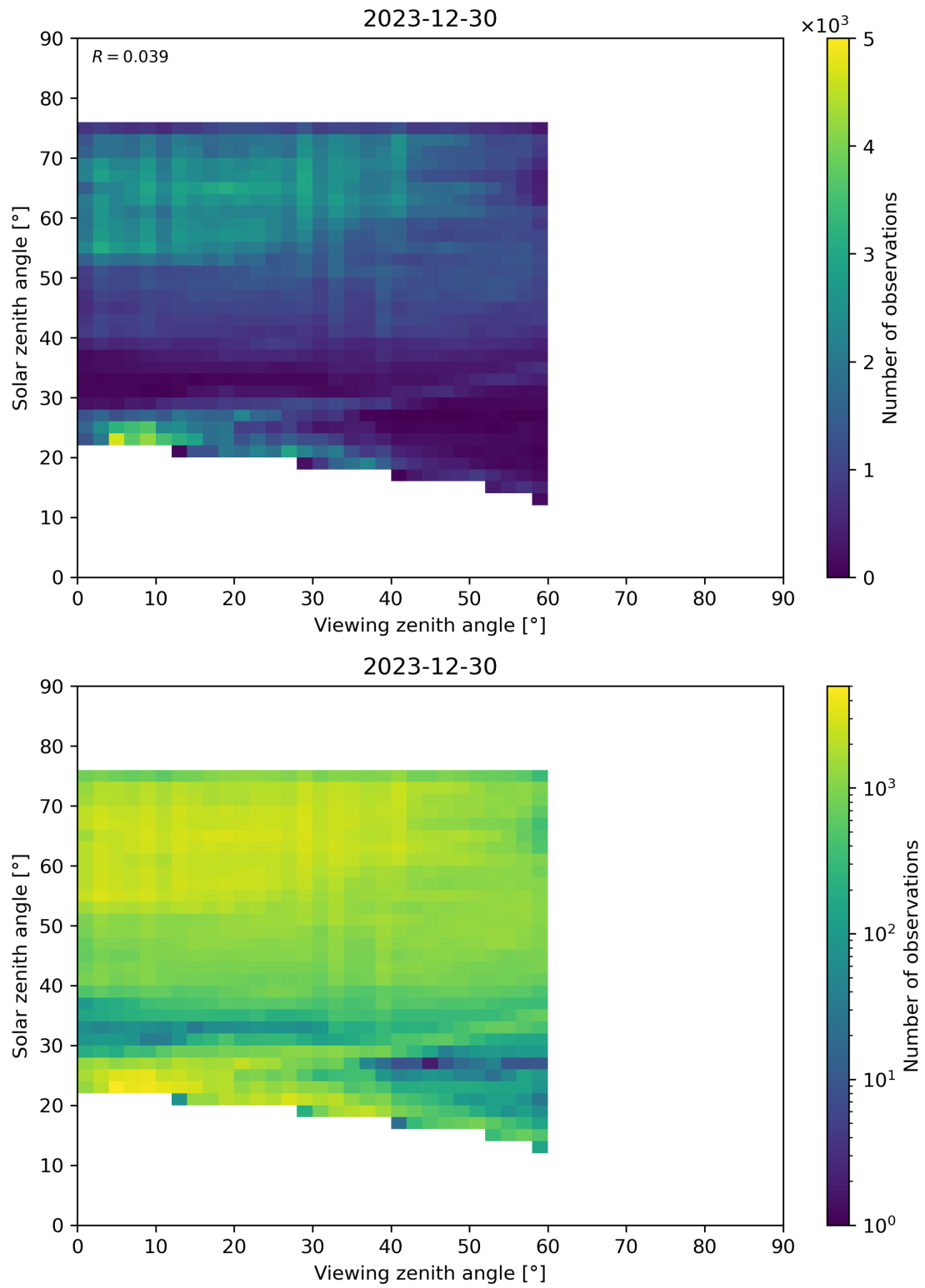
Figure 115: Scatter density plot of “Viewing zenith angle” against “Solar zenith angle” for 2023-12-30 to 2023-12-31.
