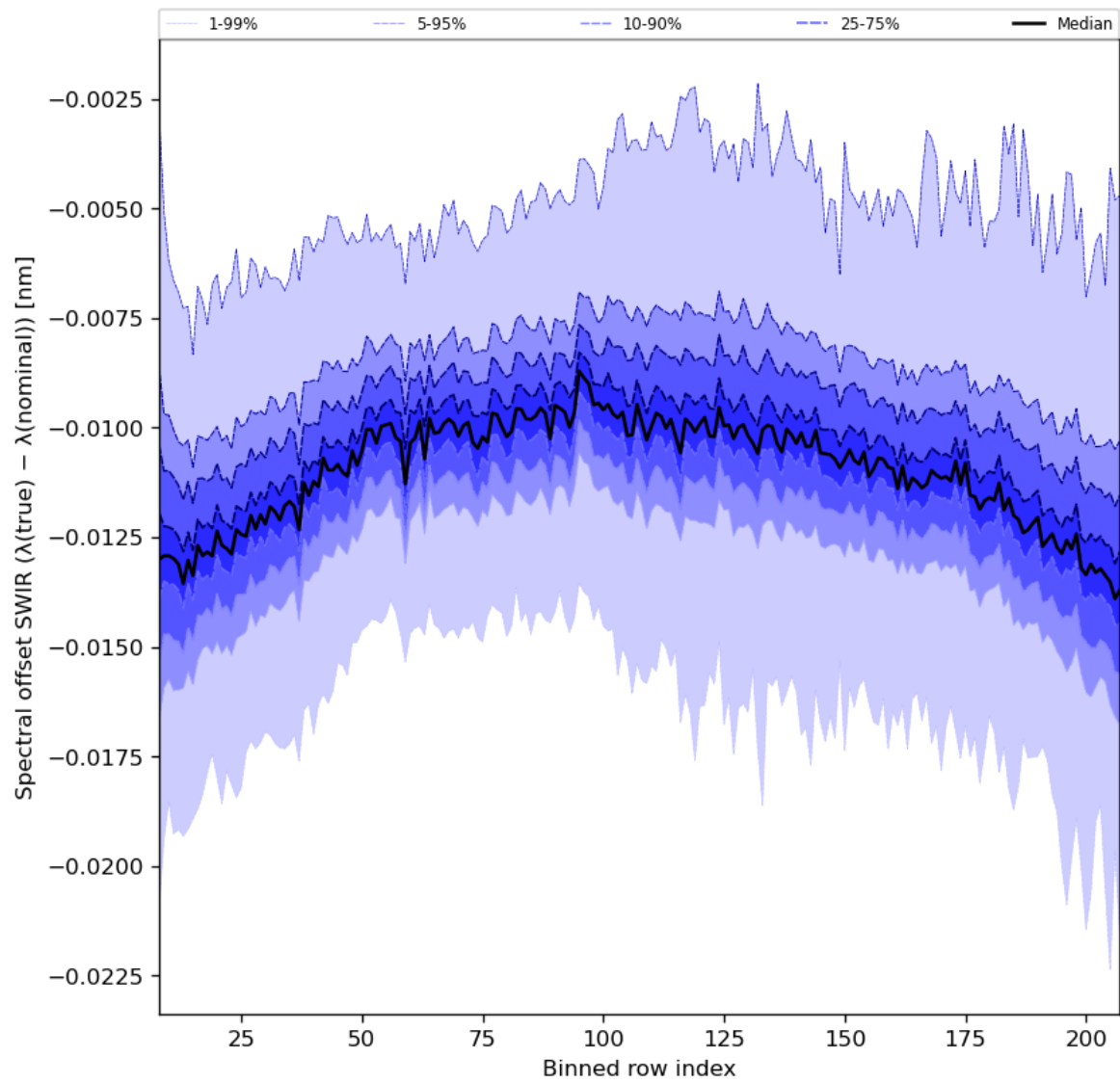
Figure 38: Along track statistics of “Spectral offset SWIR ( \lambda(\text{true}) - \lambda(\text{nominal}) )” for 2023-12-30 to 2023-12-31
