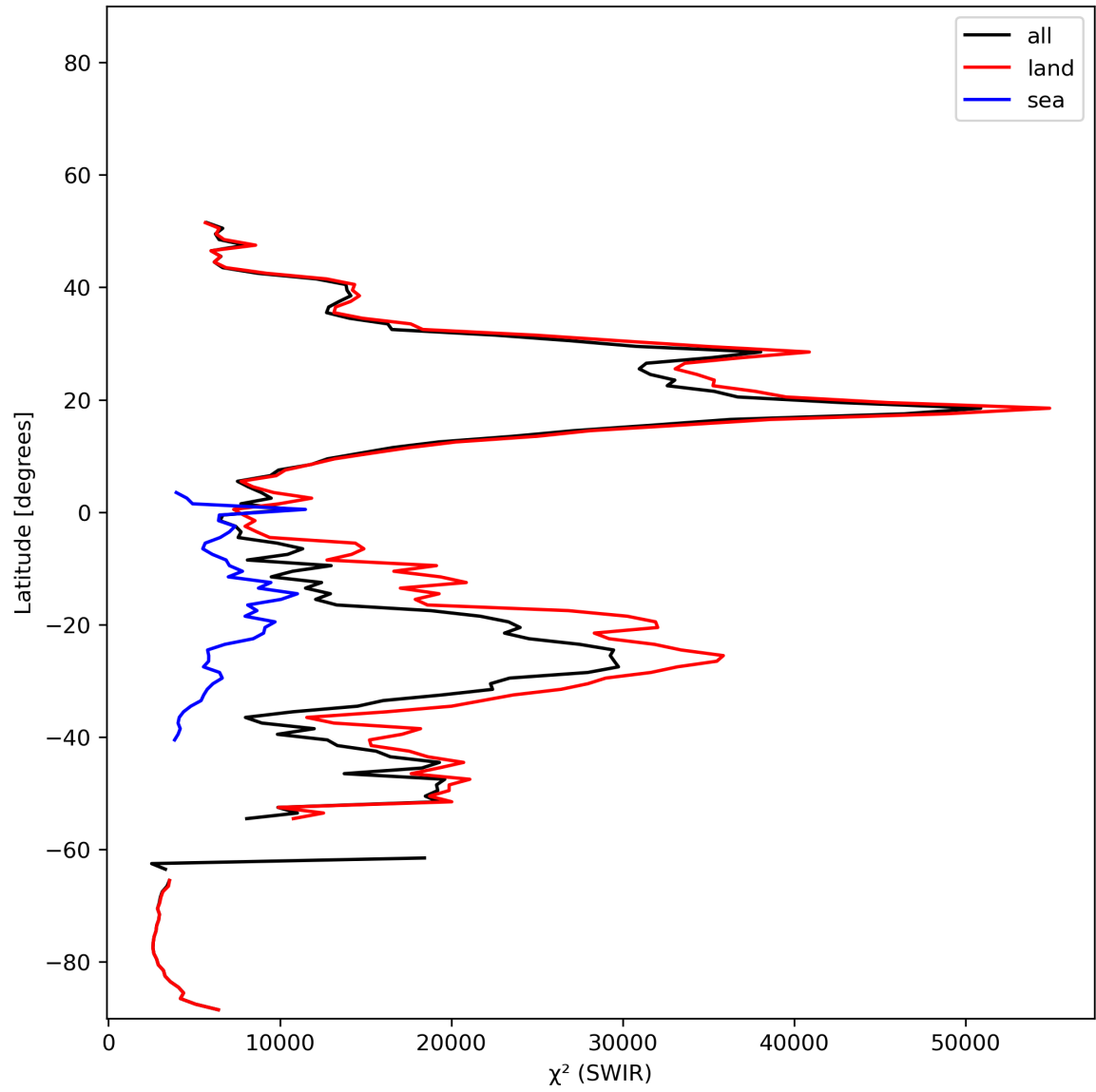
Figure 17: Zonal average of “ \chi^2 (SWIR)” for 2023-12-30 to 2023-12-31.
