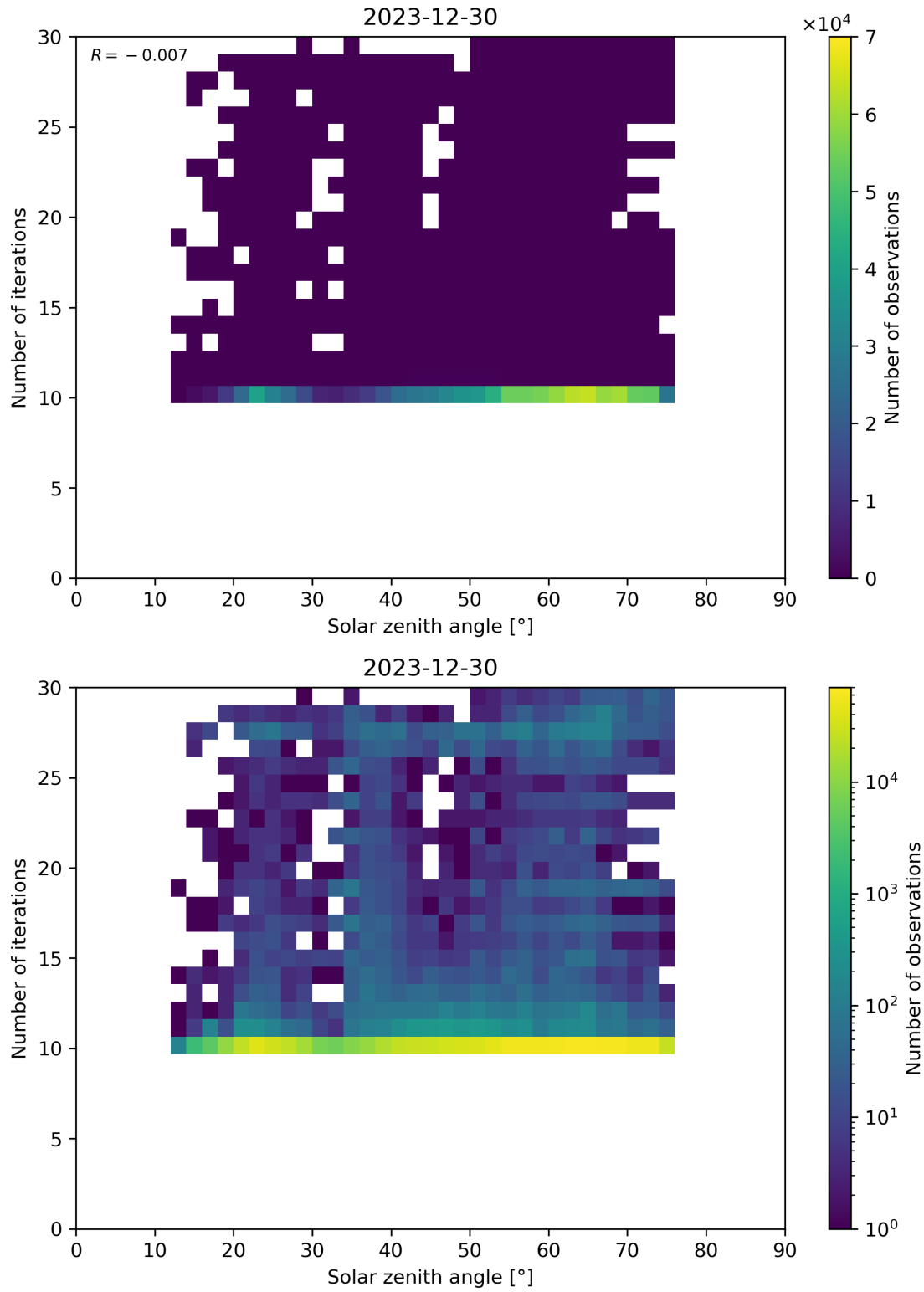
Figure 102: Scatter density plot of “Solar zenith angle” against “Number of iterations” for 2023-12-30 to 2023-12-31.
