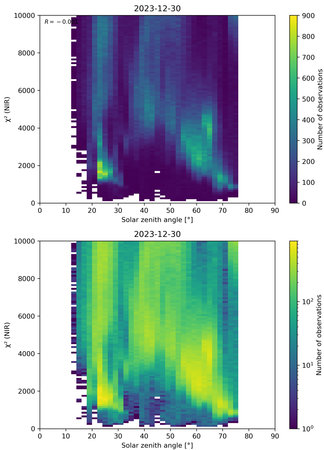
Figure 94: Scatter density plot of “Solar zenith angle” against “ \chi^2 (NIR)” for 2023-12-30 to 2023-12-31.
