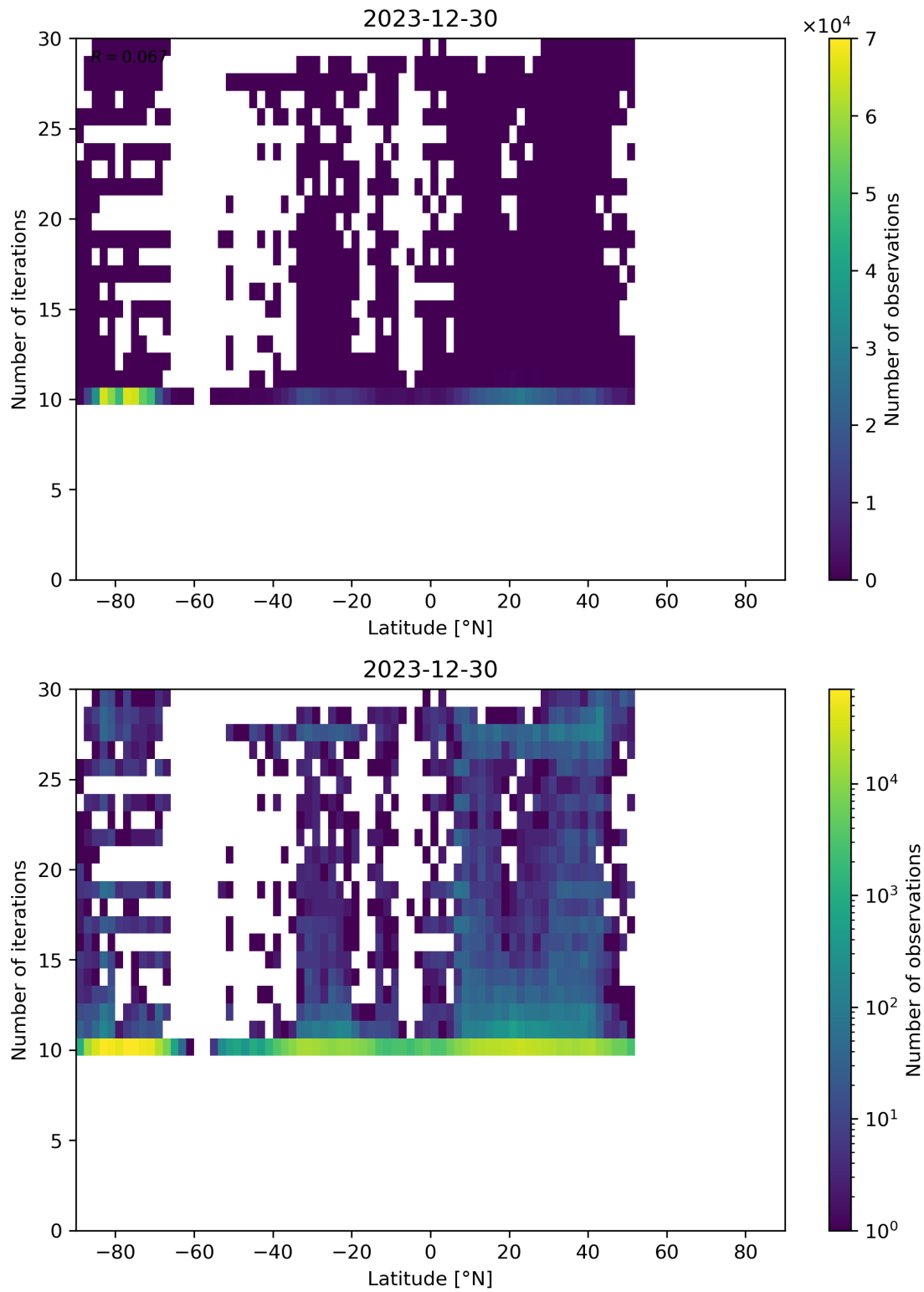
Figure 60: Scatter density plot of “Latitude” against “Number of iterations” for 2023-12-30 to 2023-12-31.
