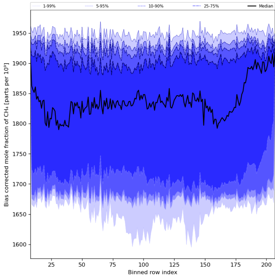
Figure 36: Along track statistics of “Bias corrected mole fraction of CH 4 ” for 2023-12-30 to 2023-12-31
