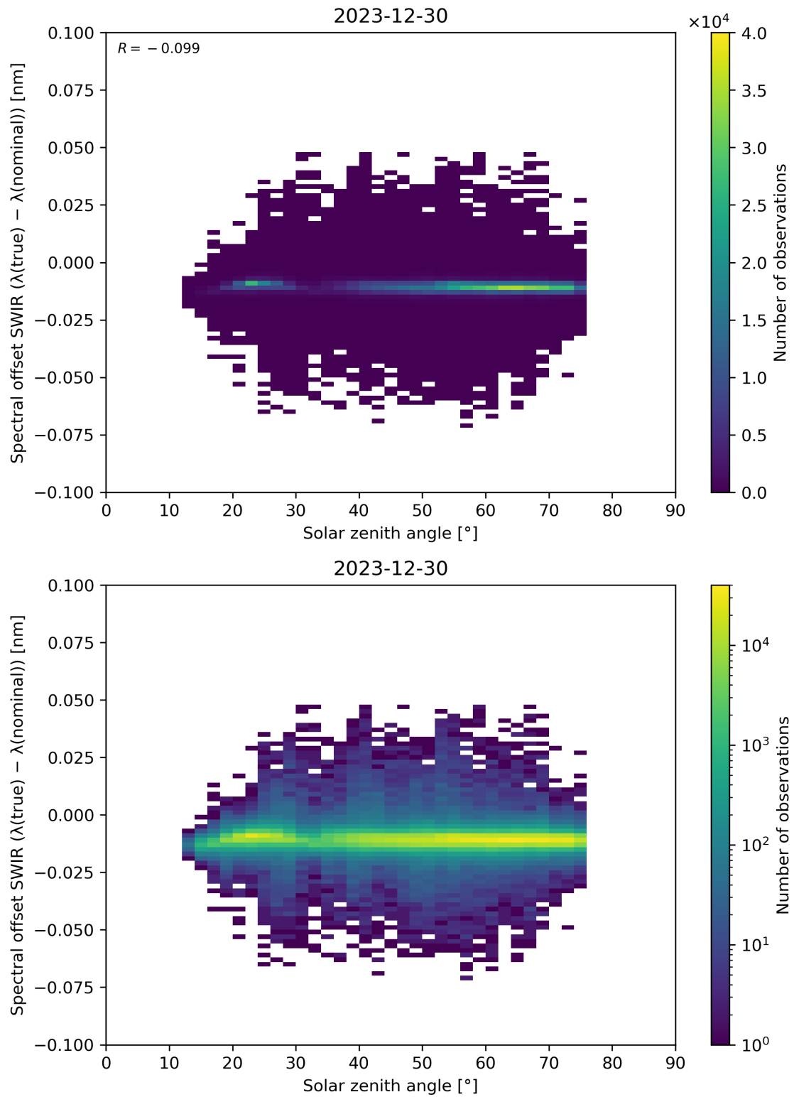
Figure 104: Scatter density plot of “Solar zenith angle” against “Spectral offset SWIR ( \lambda(\text{true}) - \lambda(\text{nominal}) )” for 2023-12-30 to 2023-12-31.
