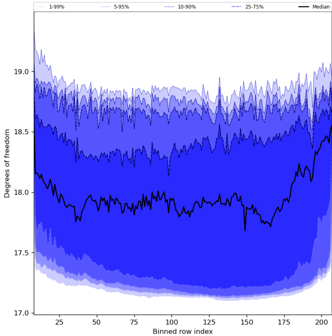
Figure 41: Along track statistics of “Degrees of freedom” for 2023-12-30 to 2023-12-31
