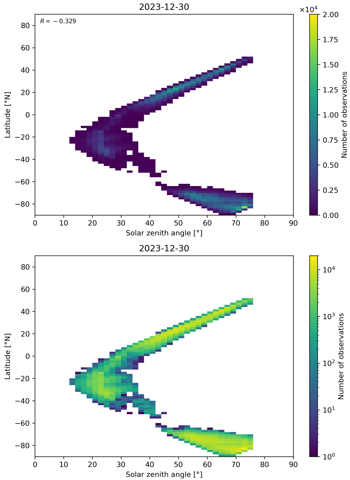
Figure 98: Scatter density plot of “Solar zenith angle” against “Latitude” for 2023-12-30 to 2023-12-31.
