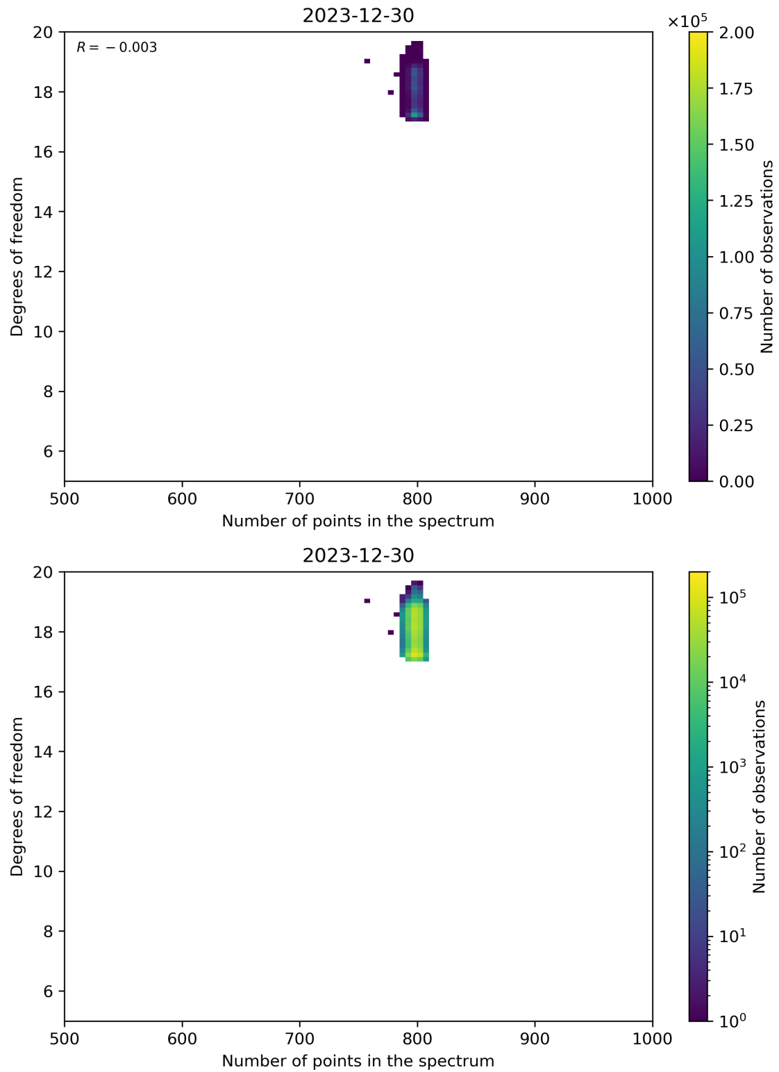
Figure 90: Scatter density plot of “Number of points in the spectrum” against “Degrees of freedom” for 2023-12-30 to 2023-12-31.
