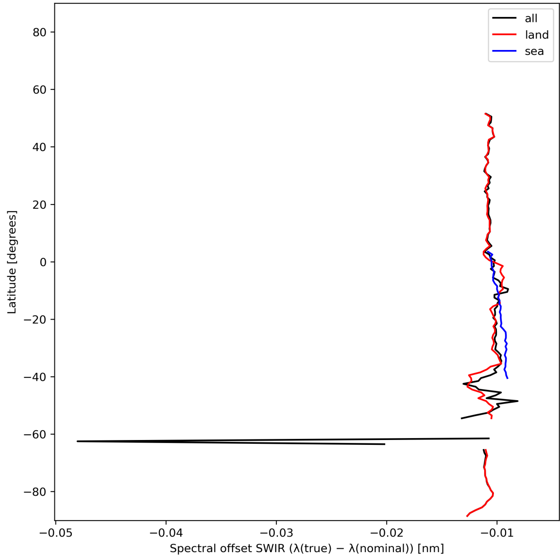
Figure 16: Zonal average of “Spectral offset SWIR ( \lambda(\text{true}) - \lambda(\text{nominal}) )” for 2023-12-30 to 2023-12-31.
