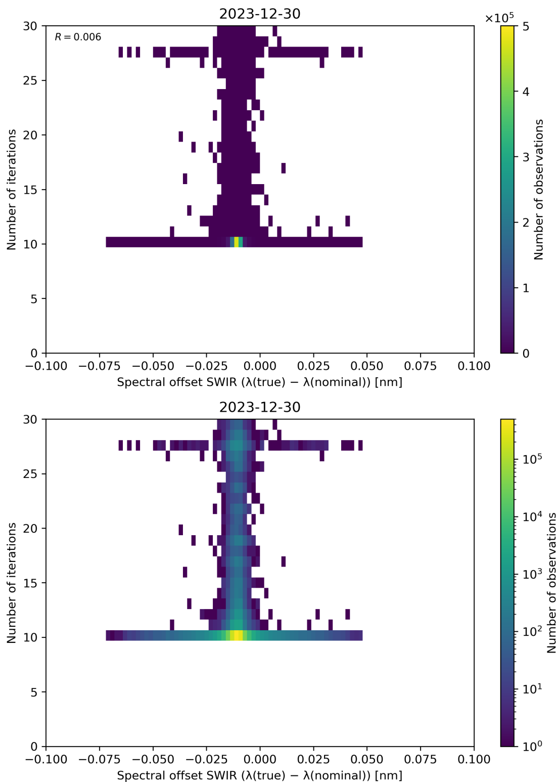
Figure 121: Scatter density plot of “Spectral offset SWIR ( \lambda(\text{true}) - \lambda(\text{nominal}) )” against “Number of iterations” for 2023-12-30 to 2023-12-31.
