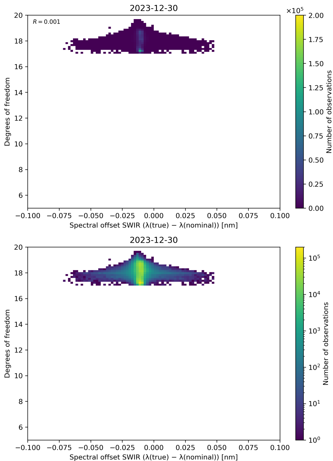
Figure 119: Scatter density plot of “Spectral offset SWIR ( \lambda(\text{true}) - \lambda(\text{nominal}) )” against “Degrees of freedom” for 2023-12-30 to 2023-12-31.
