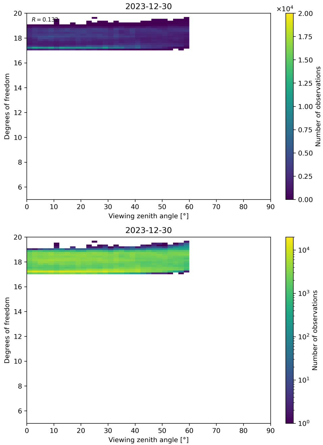
Figure 107: Scatter density plot of “Viewing zenith angle” against “Degrees of freedom” for 2023-12-30 to 2023-12-31.
