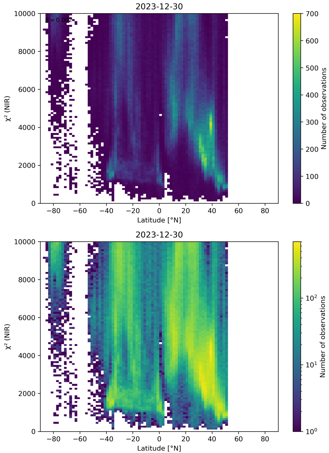
Figure 53: Scatter density plot of “Latitude” against “ \chi^2 (NIR)” for 2023-12-30 to 2023-12-31.
