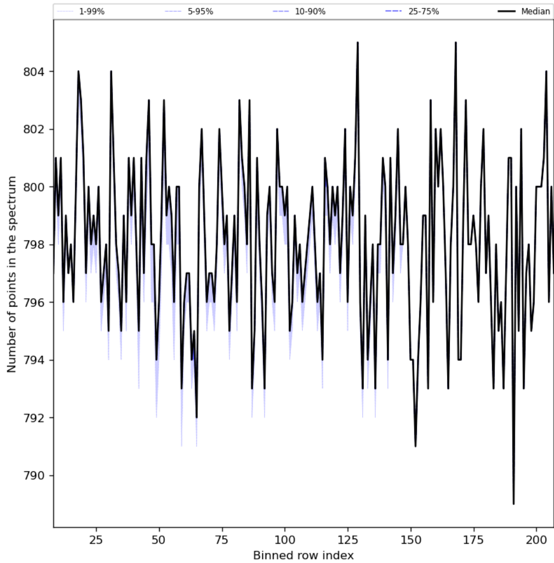
Figure 37: Along track statistics of “Number of points in the spectrum” for 2023-12-30 to 2023-12-31
