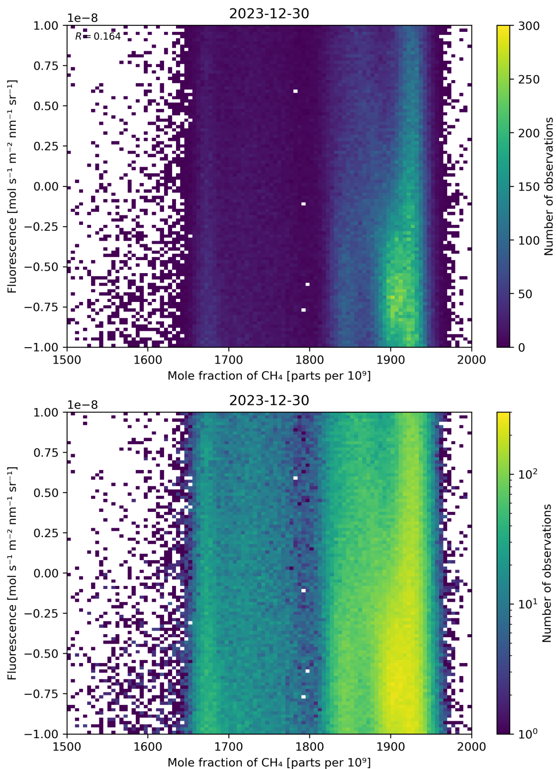
Figure 73: Scatter density plot of “Mole fraction of \text{CH}_4 ” against “Fluorescence” for 2023-12-30 to 2023-12-31.
