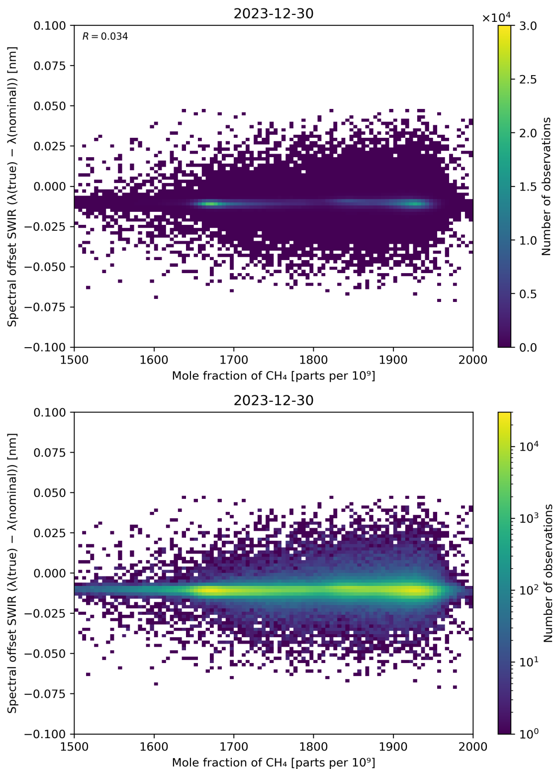
Figure 86: Scatter density plot of “Mole fraction of CH 4 ” against “Spectral offset SWIR ( \lambda(\text{true}) - \lambda(\text{nominal}) )” for 2023-12-30 to 2023-12-31.
