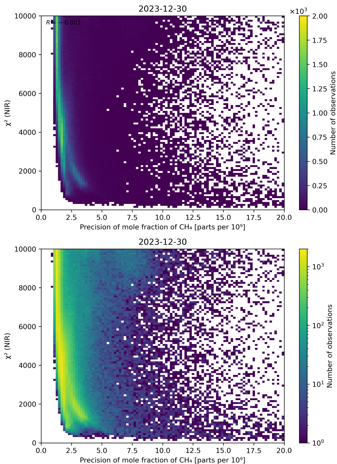
Figure 78: Scatter density plot of “Precision of mole fraction of CH 4 ” against “ \chi^2 (NIR)” for 2023-12-30 to 2023-12-31.
