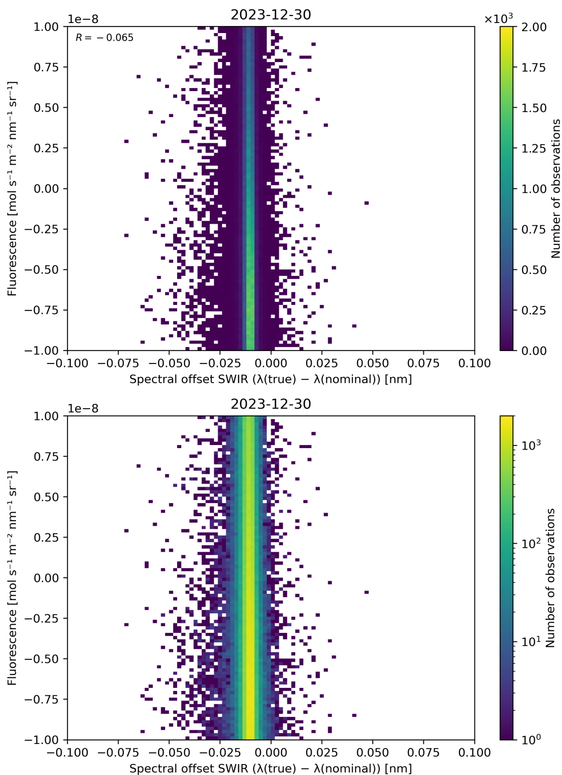
Figure 120: Scatter density plot of “Spectral offset SWIR ( \lambda(\text{true}) - \lambda(\text{nominal}) )” against “Fluorescence” for 2023-12-30 to 2023-12-31.
