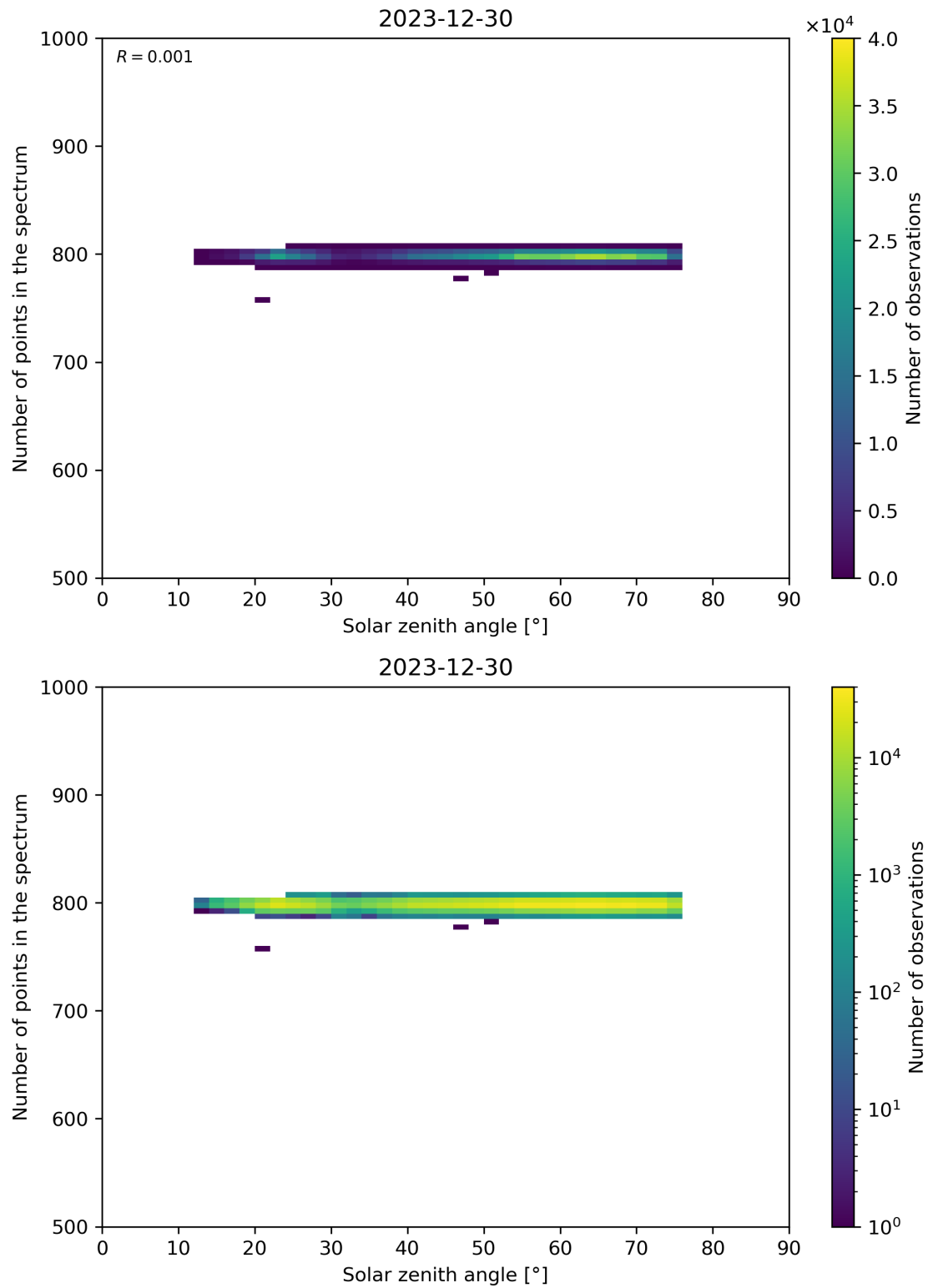
Figure 103: Scatter density plot of “Solar zenith angle” against “Number of points in the spectrum” for 2023-12-30 to 2023-12-31.
