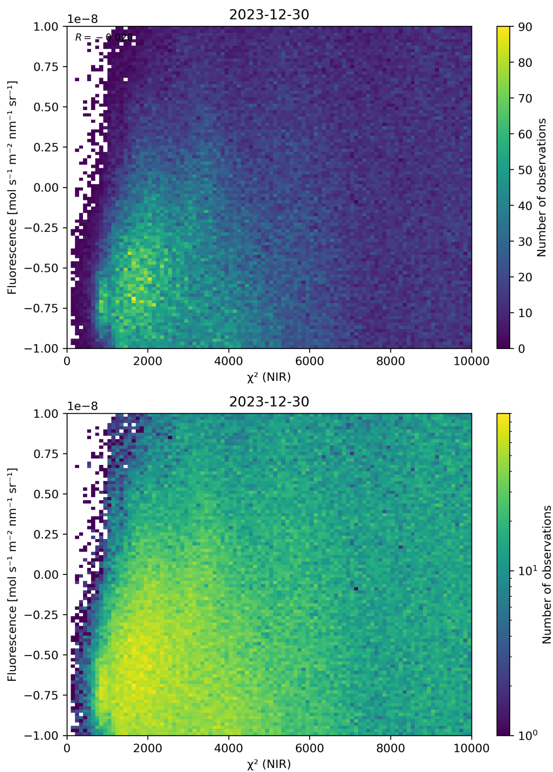
Figure 45: Scatter density plot of “ \chi^2 (NIR)” against “Fluorescence” for 2023-12-30 to 2023-12-31.
