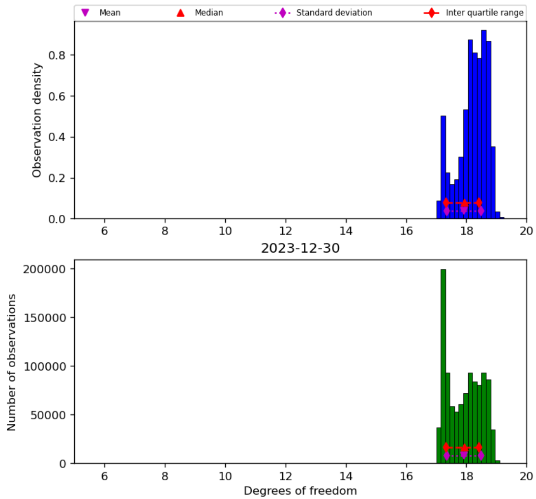
Figure 30: Histogram of “Degrees of freedom” for 2023-12-30 to 2023-12-31
