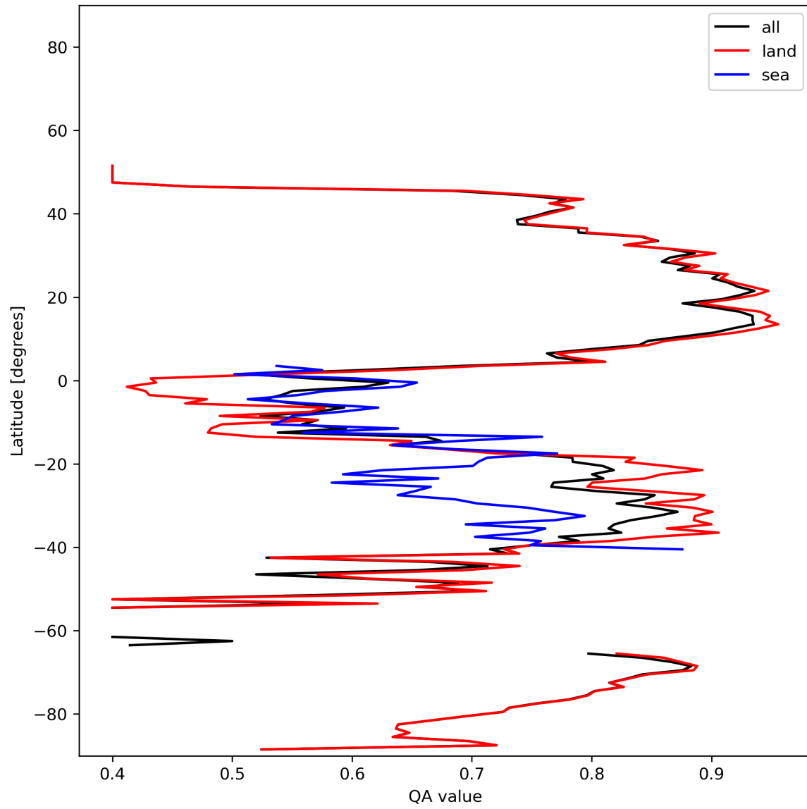
Figure 11: Zonal average of “QA value” for 2023-12-30 to 2023-12-31.
