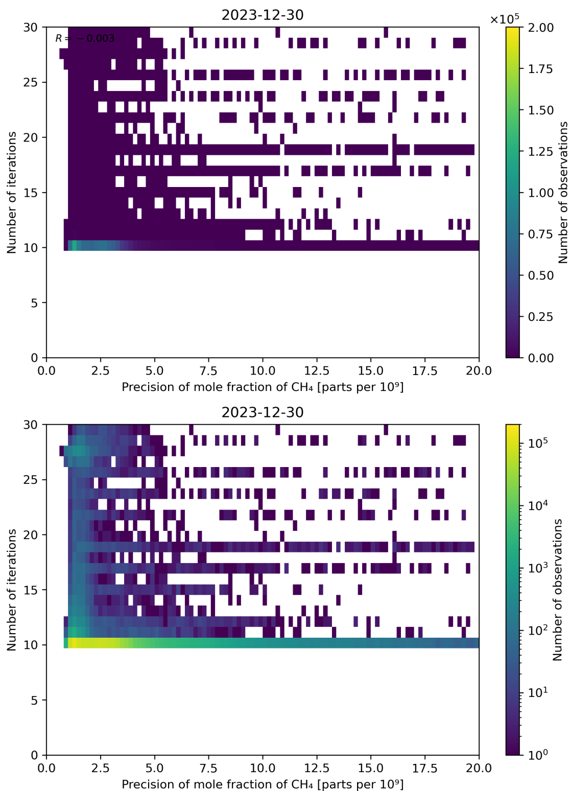
Figure 83: Scatter density plot of “Precision of mole fraction of CH 4 ” against “Number of iterations” for 2023-12-30 to 2023-12-31.
