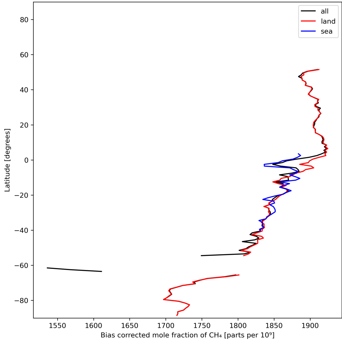
Figure 14: Zonal average of “Bias corrected mole fraction of CH 4 ” for 2023-12-30 to 2023-12-31.
