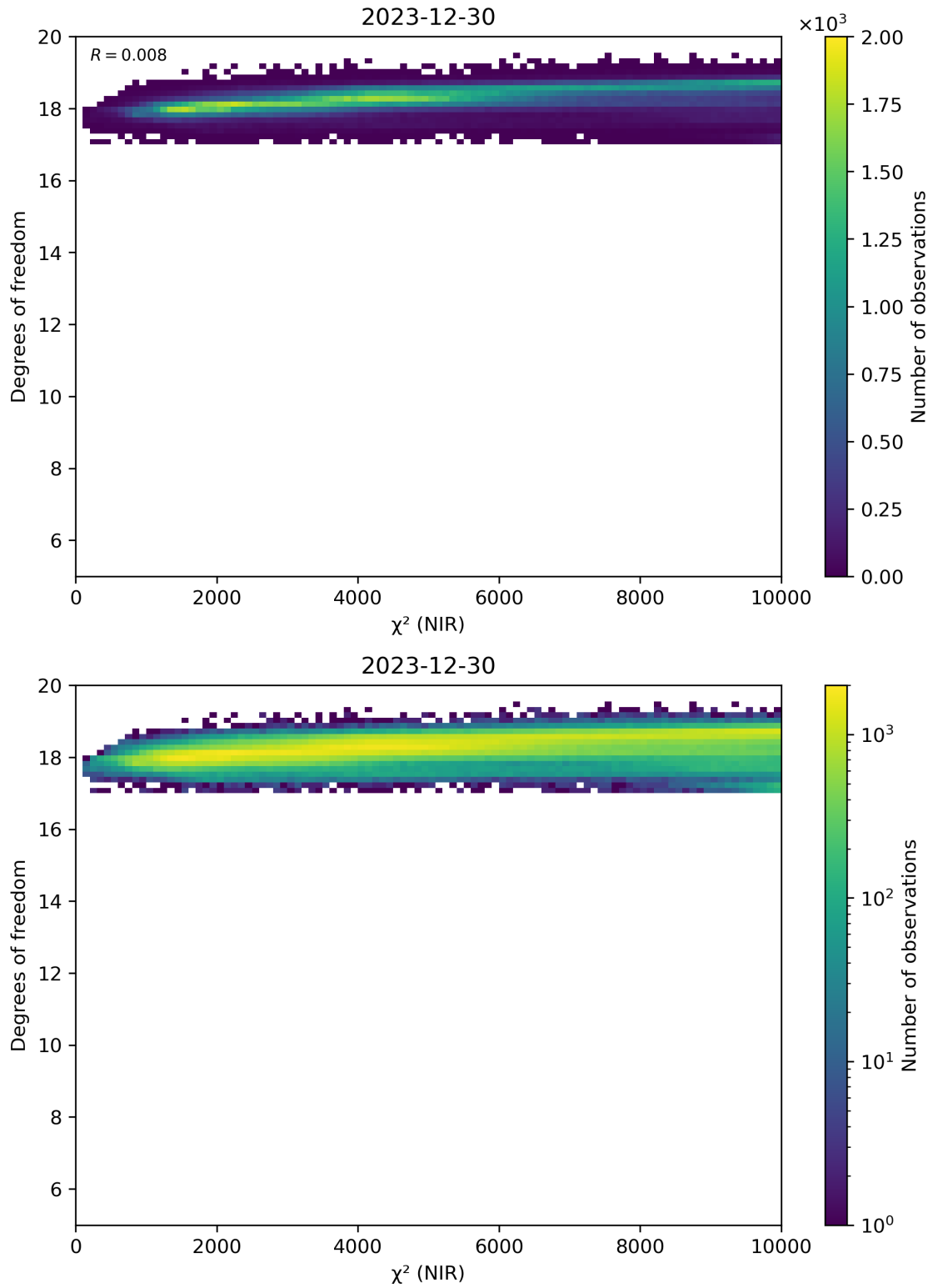
Figure 44: Scatter density plot of “ \chi^2 (NIR)” against “Degrees of freedom” for 2023-12-30 to 2023-12-31.
