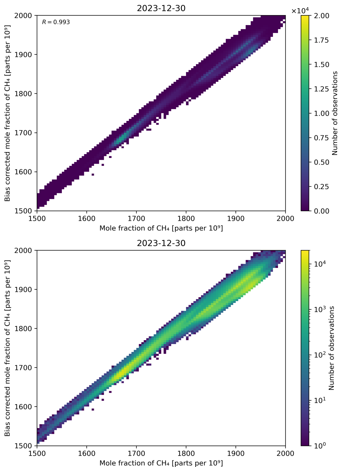
Figure 74: Scatter density plot of “Mole fraction of CH 4 ” against “Bias corrected mole fraction of CH 4 ” for 2023-12-30 to 2023-12-31.
