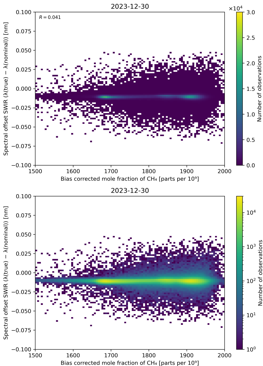
Figure 69: Scatter density plot of “Bias corrected mole fraction of \text{CH}_4 ” against “Spectral offset SWIR ( \lambda(\text{true}) - \lambda(\text{nominal}) )” for 2023-12-30 to 2023-12-31.
