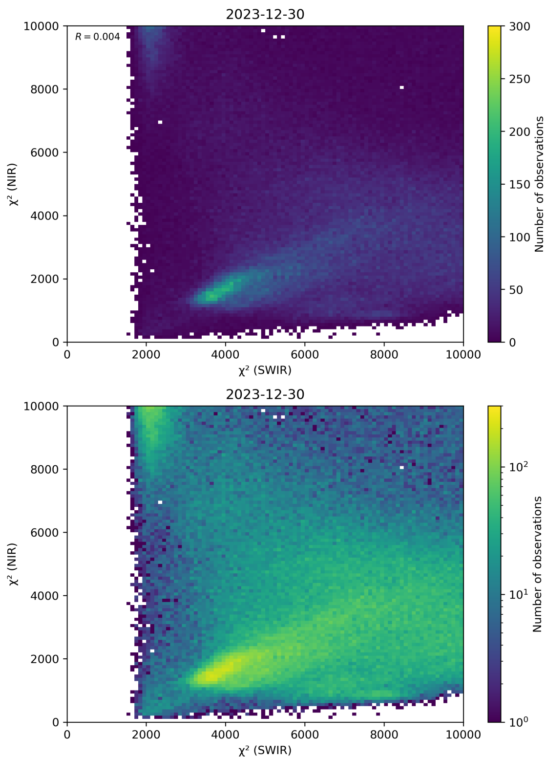
Figure 47: Scatter density plot of “ \chi^2 (SWIR)” against “ \chi^2 (NIR)” for 2023-12-30 to 2023-12-31.
