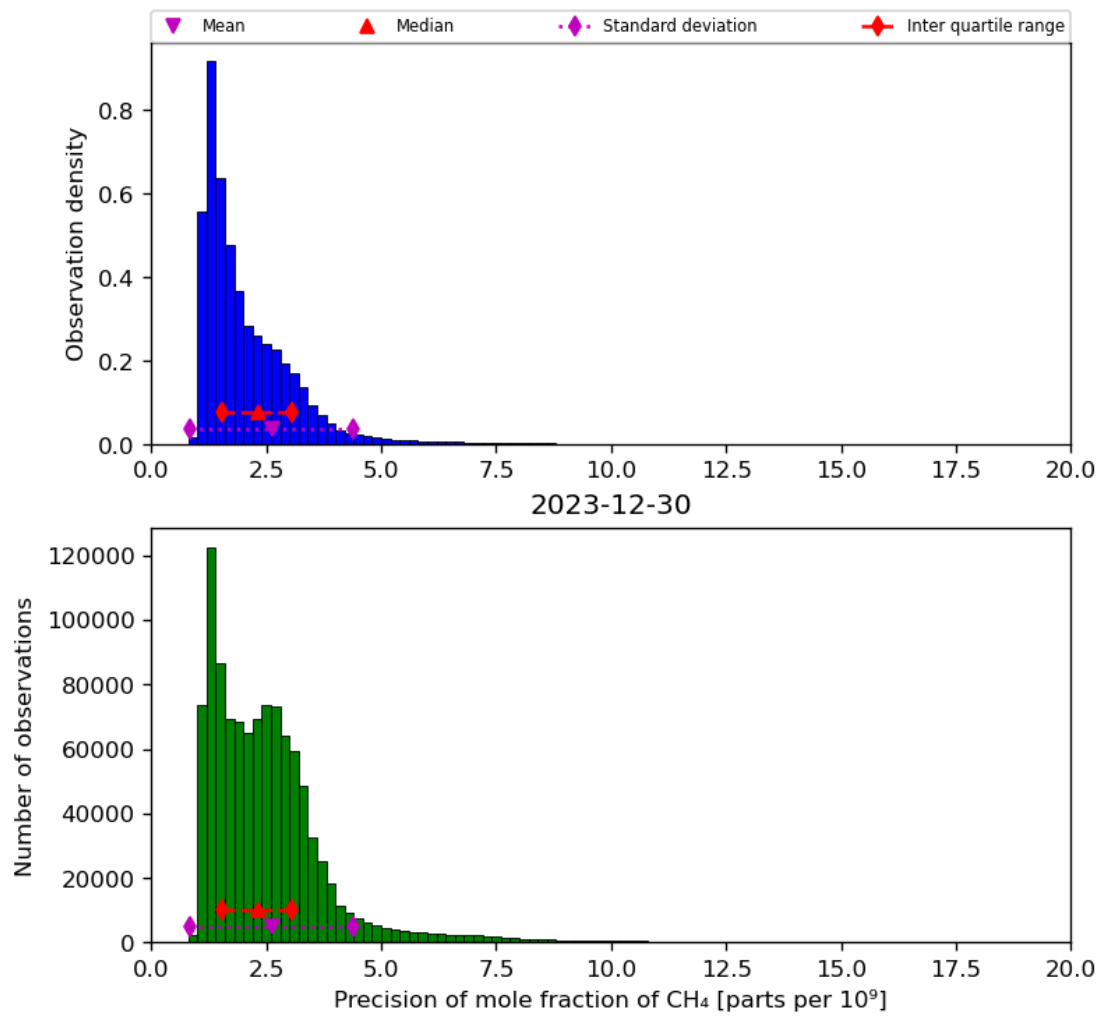
Figure 24: Histogram of “Precision of mole fraction of CH 4 ” for 2023-12-30 to 2023-12-31
