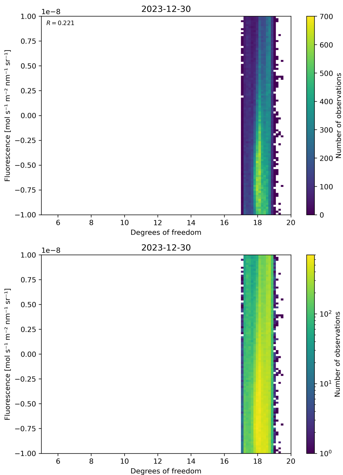
Figure 51: Scatter density plot of “Degrees of freedom” against “Fluorescence” for 2023-12-30 to 2023-12-31.
