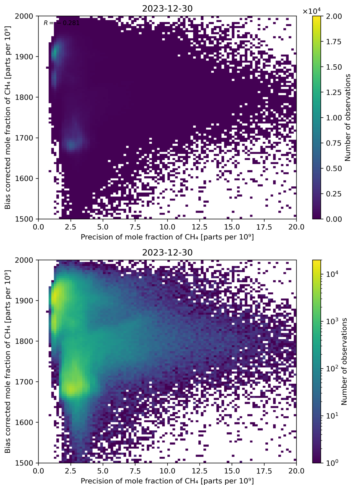
Figure 82: Scatter density plot of “Precision of mole fraction of CH 4 ” against “Bias corrected mole fraction of CH 4 ” for 2023-12-30 to 2023-12-31.
