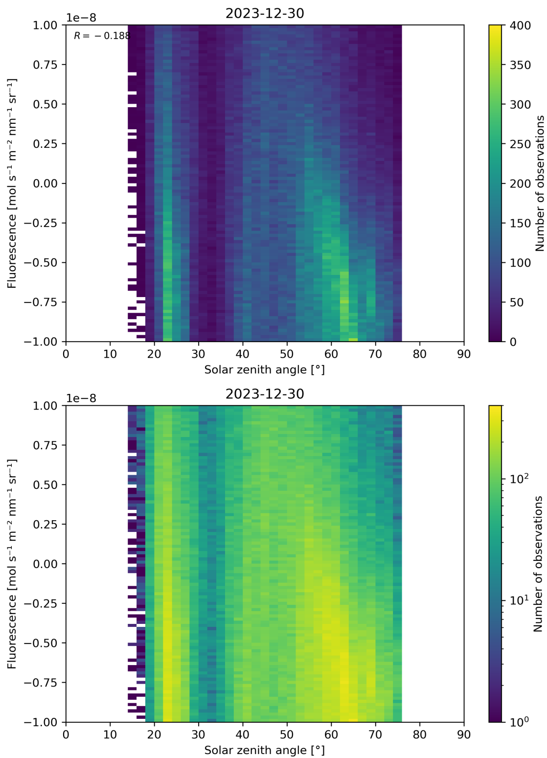
Figure 97: Scatter density plot of “Solar zenith angle” against “Fluorescence” for 2023-12-30 to 2023-12-31.
