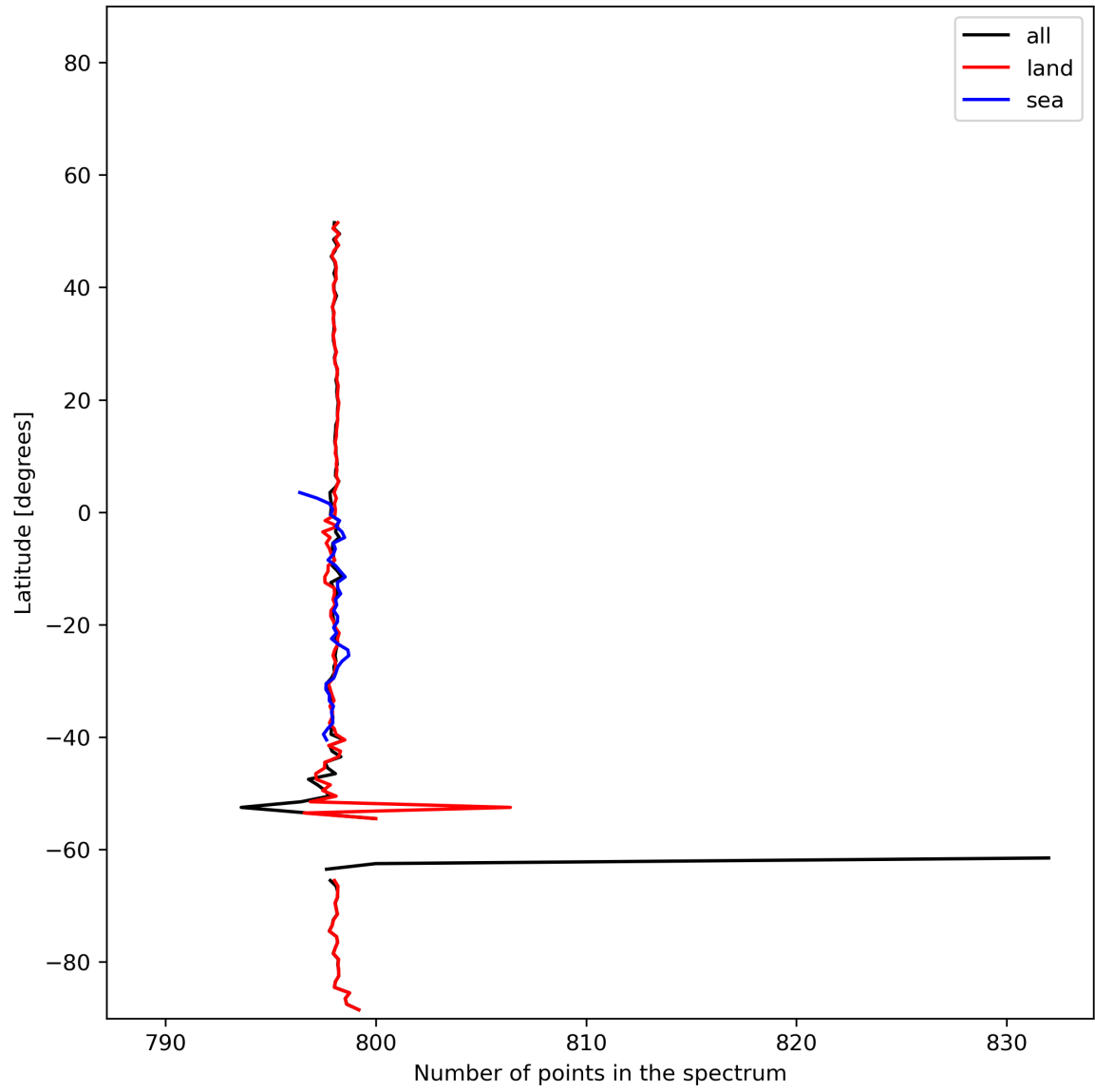
Figure 15: Zonal average of “Number of points in the spectrum” for 2023-12-30 to 2023-12-31.
