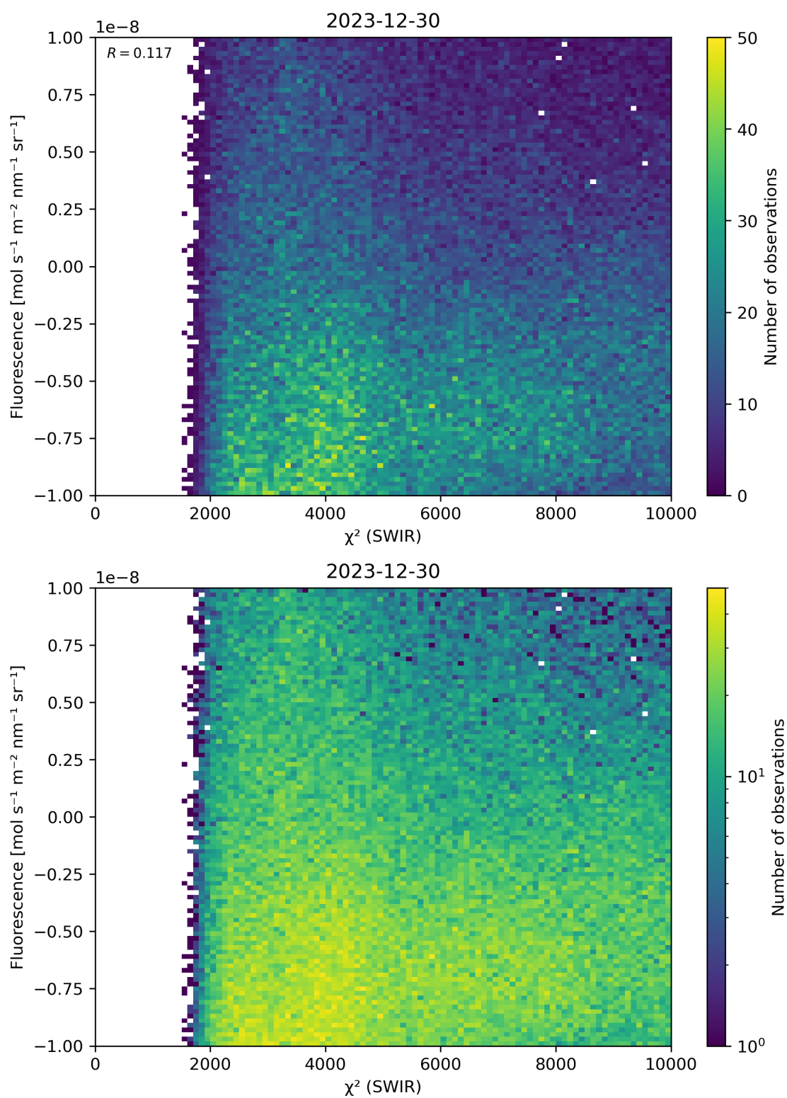
Figure 49: Scatter density plot of “ \chi^2 (SWIR)” against “Fluorescence” for 2023-12-30 to 2023-12-31.
