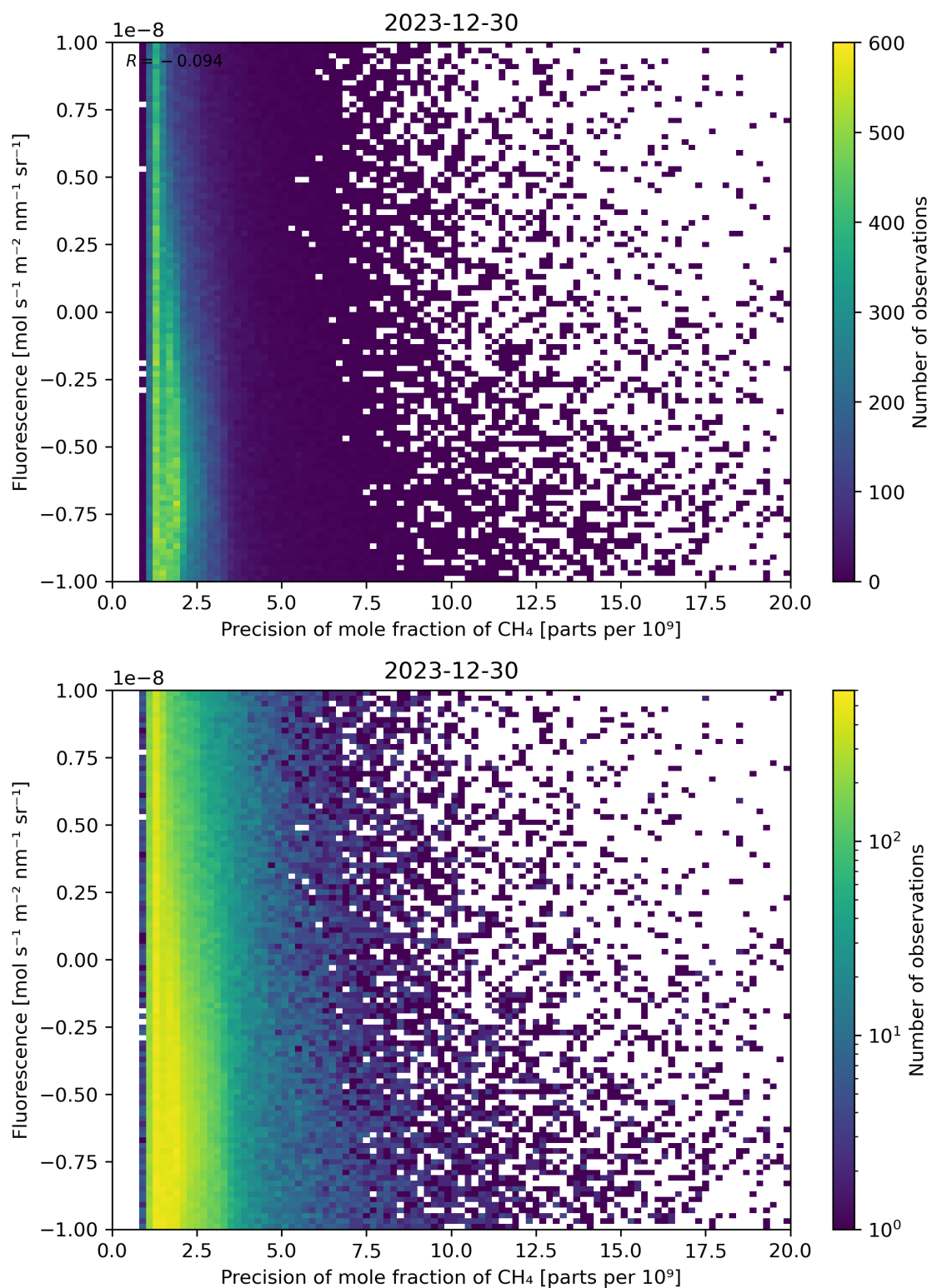
Figure 81: Scatter density plot of “Precision of mole fraction of \text{CH}_4 ” against “Fluorescence” for 2023-12-30 to 2023-12-31.
