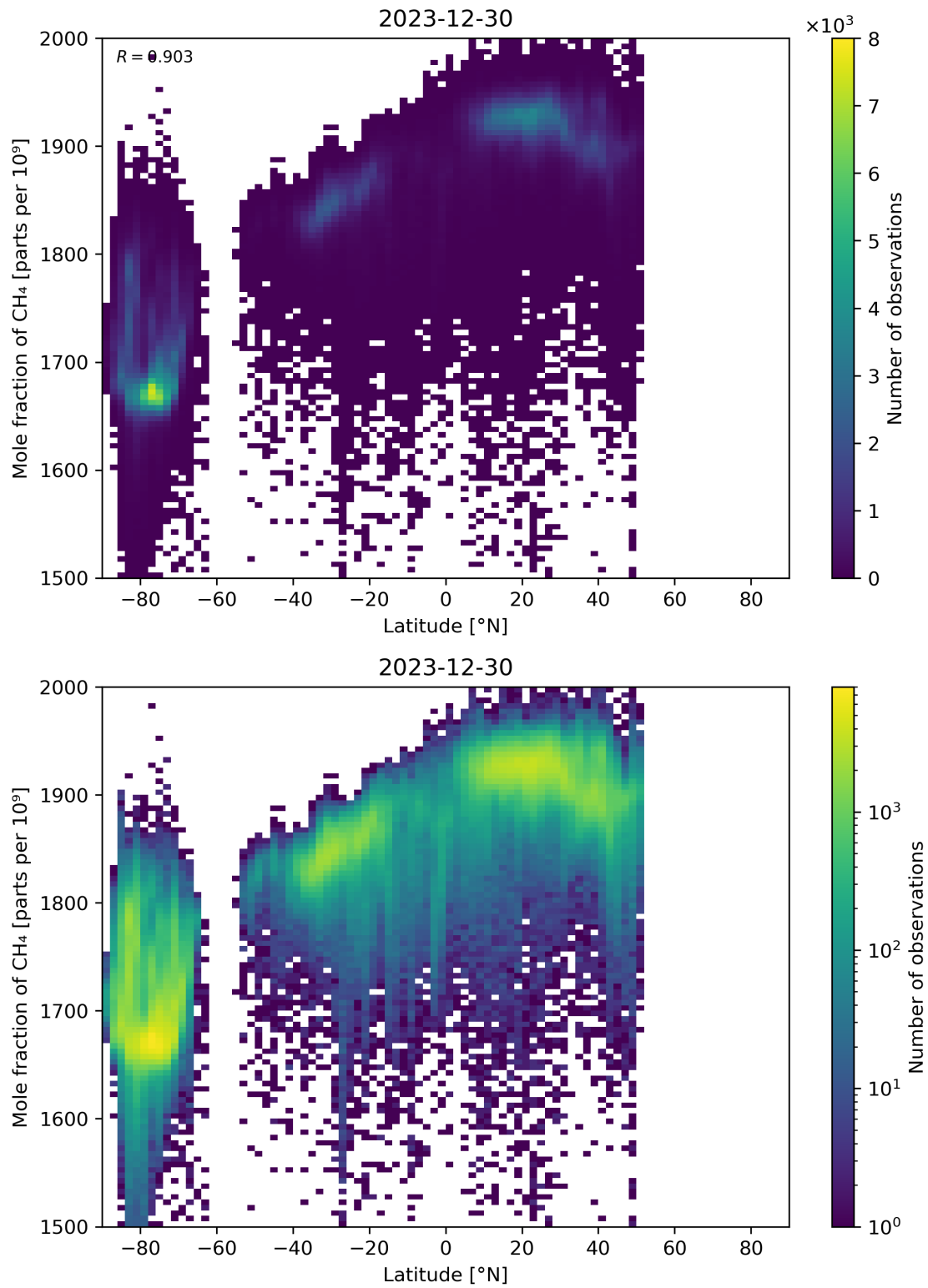
Figure 57: Scatter density plot of “Latitude” against “Mole fraction of CH 4 ” for 2023-12-30 to 2023-12-31.
