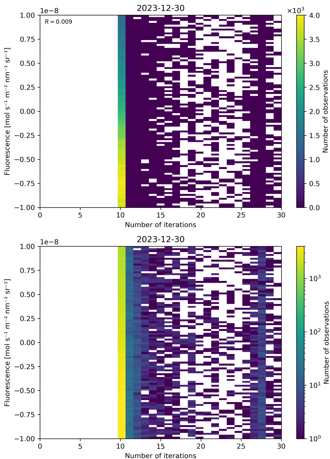
Figure 87: Scatter density plot of “Number of iterations” against “Fluorescence” for 2023-12-30 to 2023-12-31.
