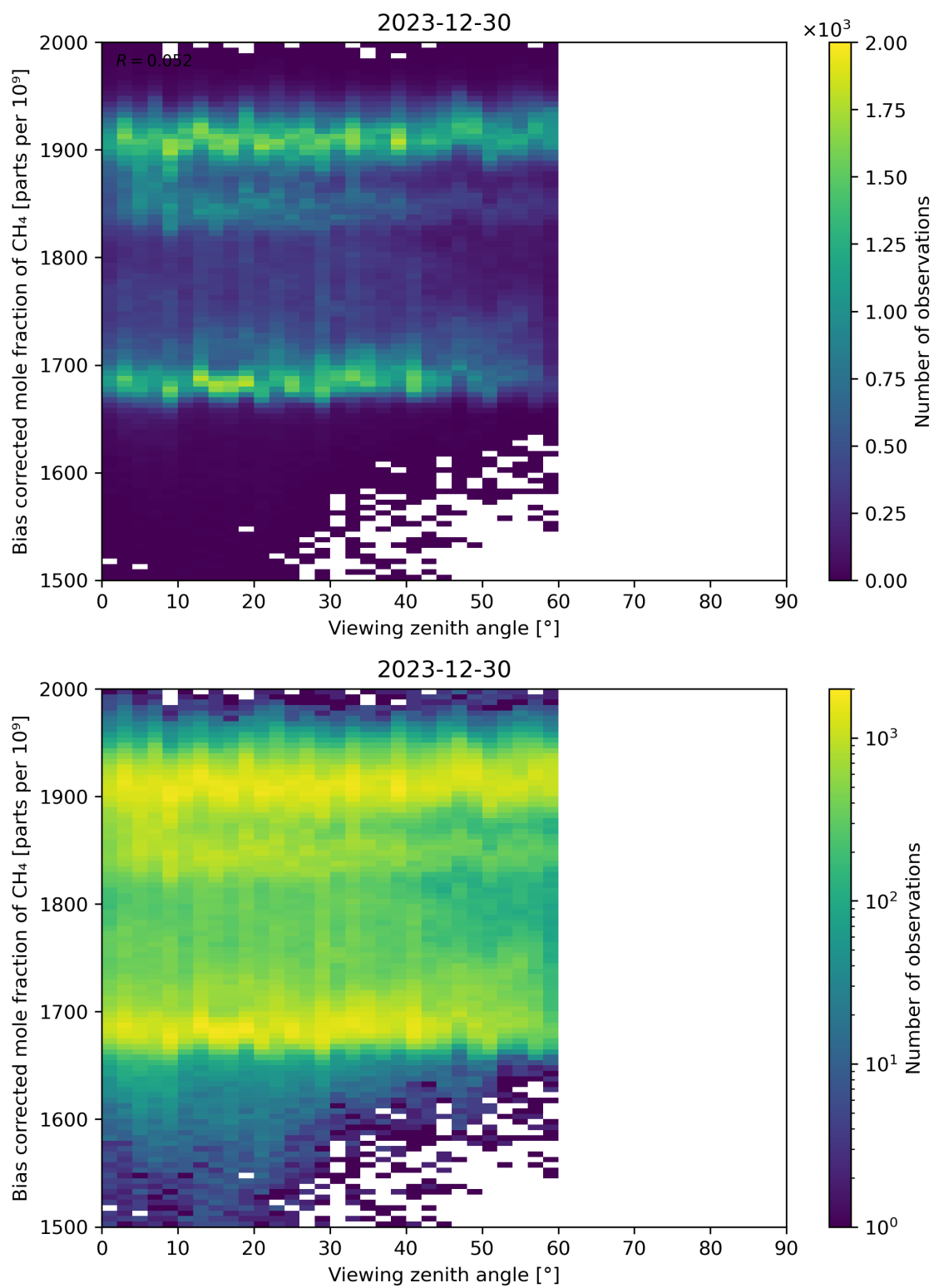
Figure 111: Scatter density plot of “Viewing zenith angle” against “Bias corrected mole fraction of CH 4 ” for 2023-12-30 to 2023-12-31.
