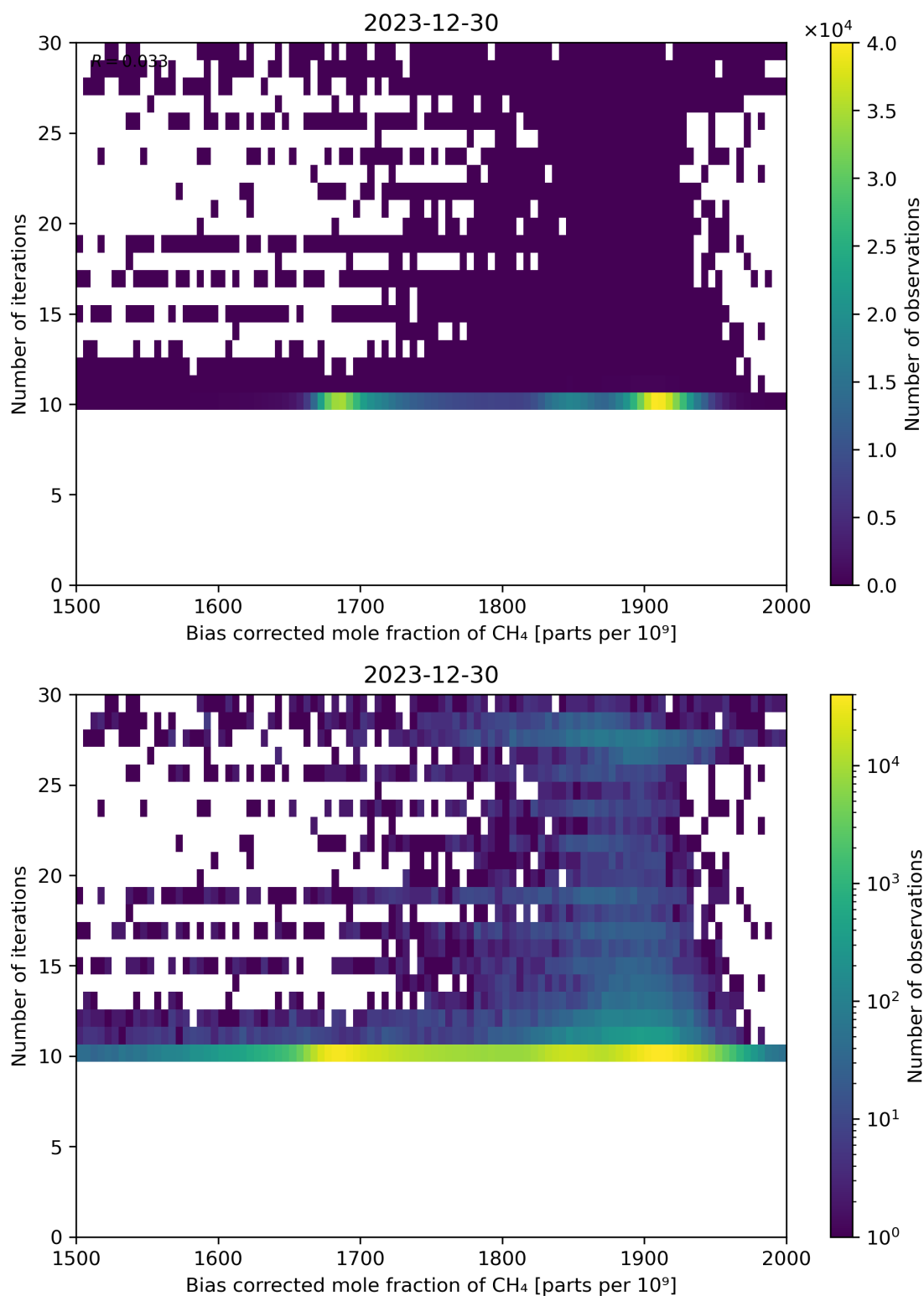
Figure 67: Scatter density plot of “Bias corrected mole fraction of CH 4 ” against “Number of iterations” for 2023-12-30 to 2023-12-31.
