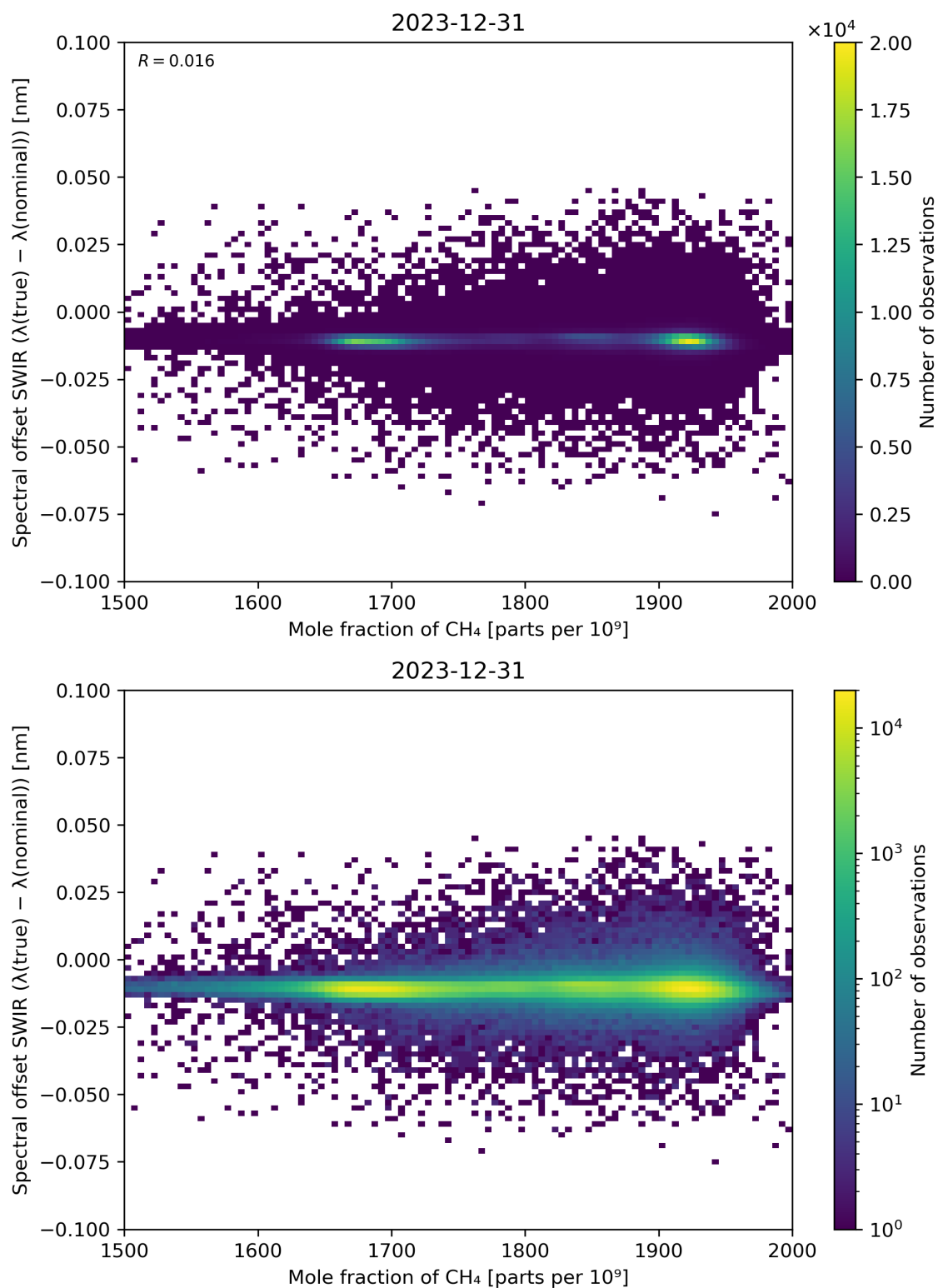
Figure 86: Scatter density plot of “Mole fraction of CH 4 ” against “Spectral offset SWIR ( \lambda(\text{true}) - \lambda(\text{nominal}) )” for 2023-12-30 to 2023-12-31.
