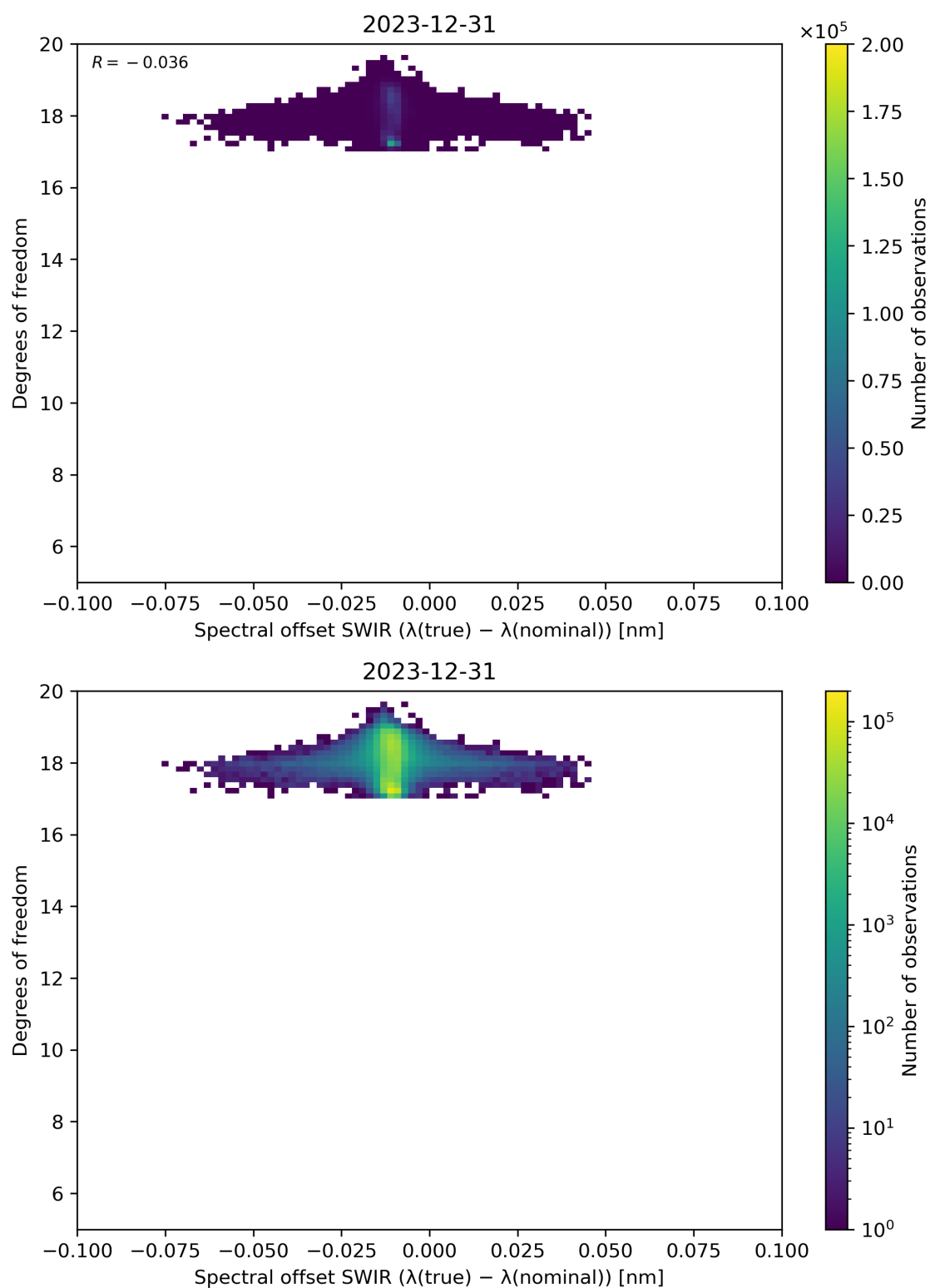
Figure 119: Scatter density plot of “Spectral offset SWIR ( \lambda(\text{true}) - \lambda(\text{nominal}) )” against “Degrees of freedom” for 2023-12-30 to 2023-12-31.
