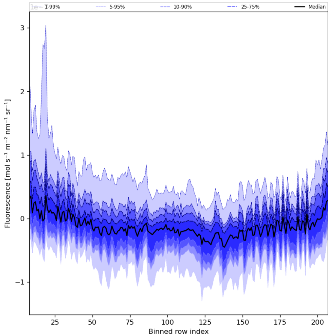
Figure 43: Along track statistics of “Fluorescence” for 2023-12-30 to 2023-12-31
