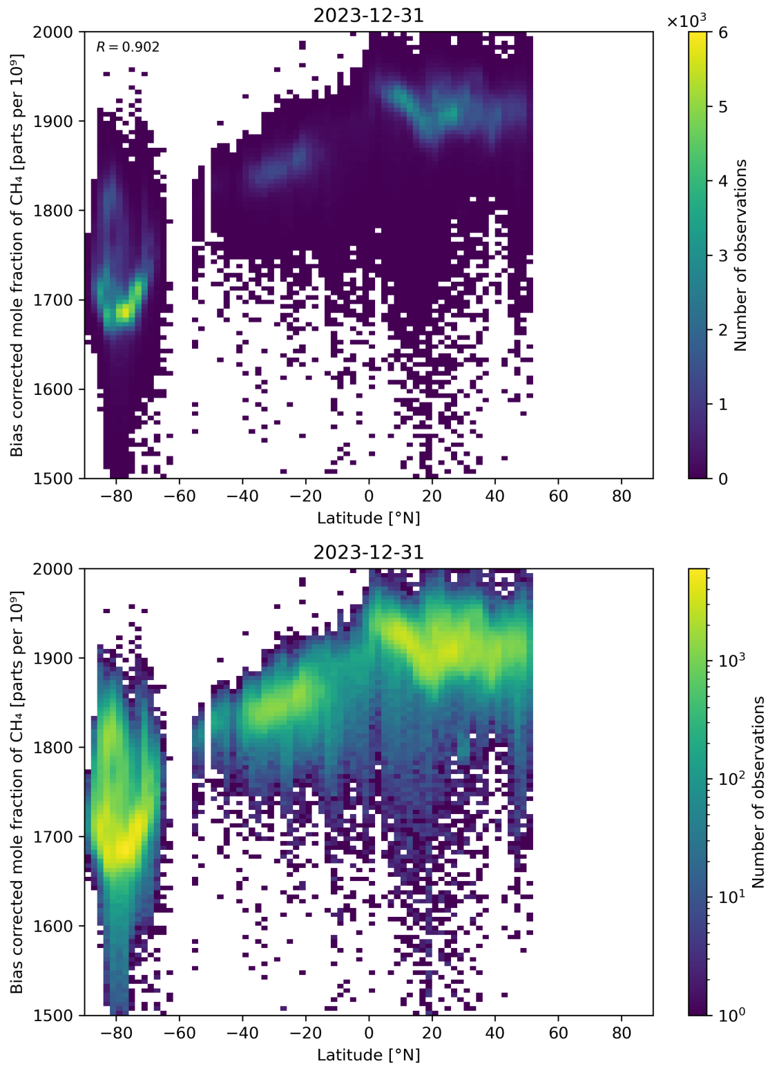
Figure 58: Scatter density plot of “Latitude” against “Bias corrected mole fraction of CH 4 ” for 2023-12-30 to 2023-12-31.
