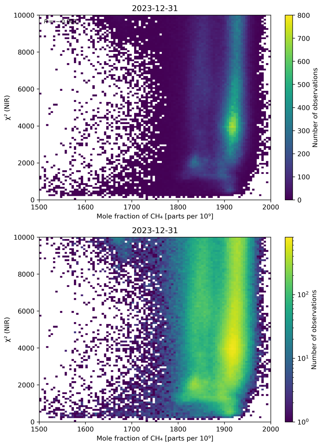
Figure 70: Scatter density plot of “Mole fraction of CH 4 ” against “ \chi^2 (NIR)” for 2023-12-30 to 2023-12-31.
