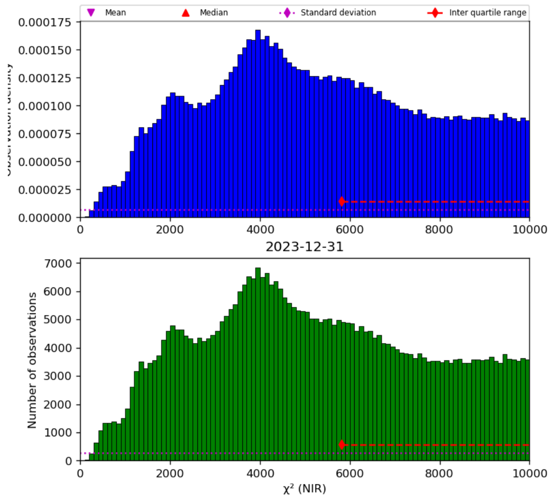
Figure 29: Histogram of “ \chi^2 (NIR)” for 2023-12-30 to 2023-12-31
