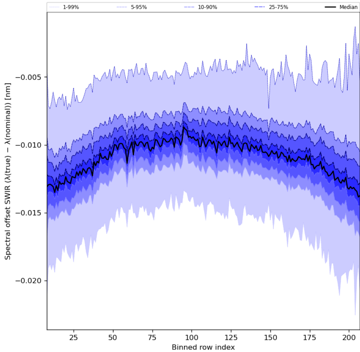
Figure 38: Along track statistics of “Spectral offset SWIR ( \lambda(\text{true}) - \lambda(\text{nominal}) )” for 2023-12-30 to 2023-12-31
