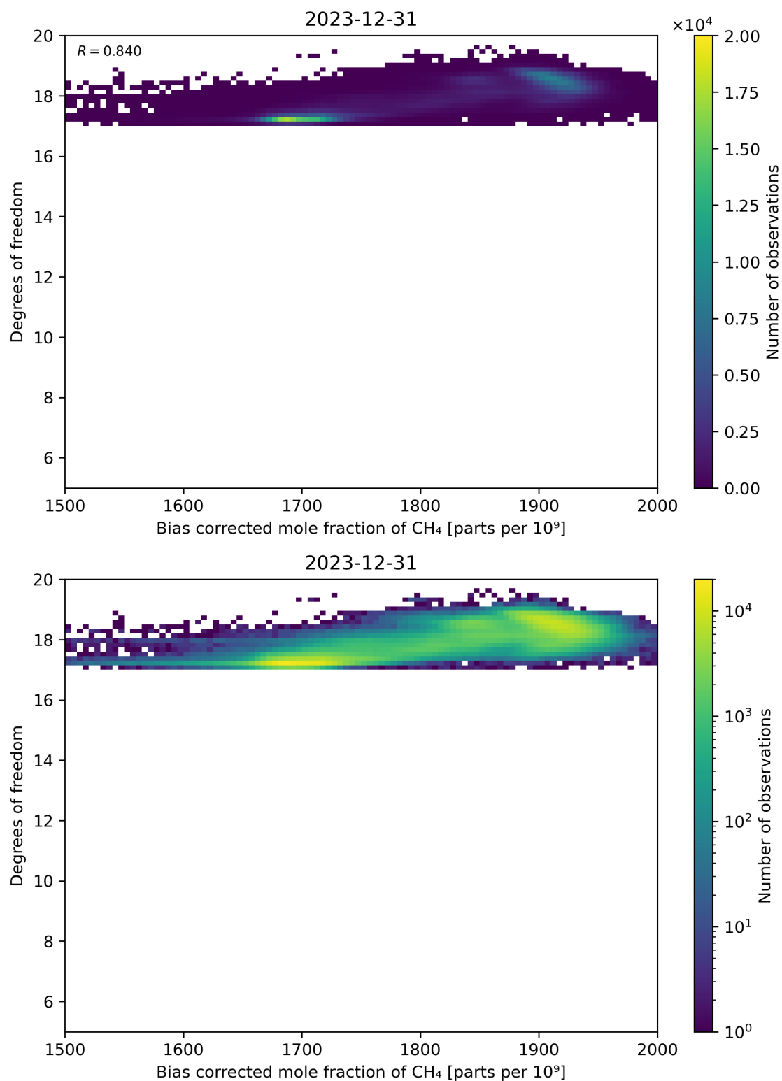
Figure 65: Scatter density plot of “Bias corrected mole fraction of CH 4 ” against “Degrees of freedom” for 2023-12-30 to 2023-12-31.
