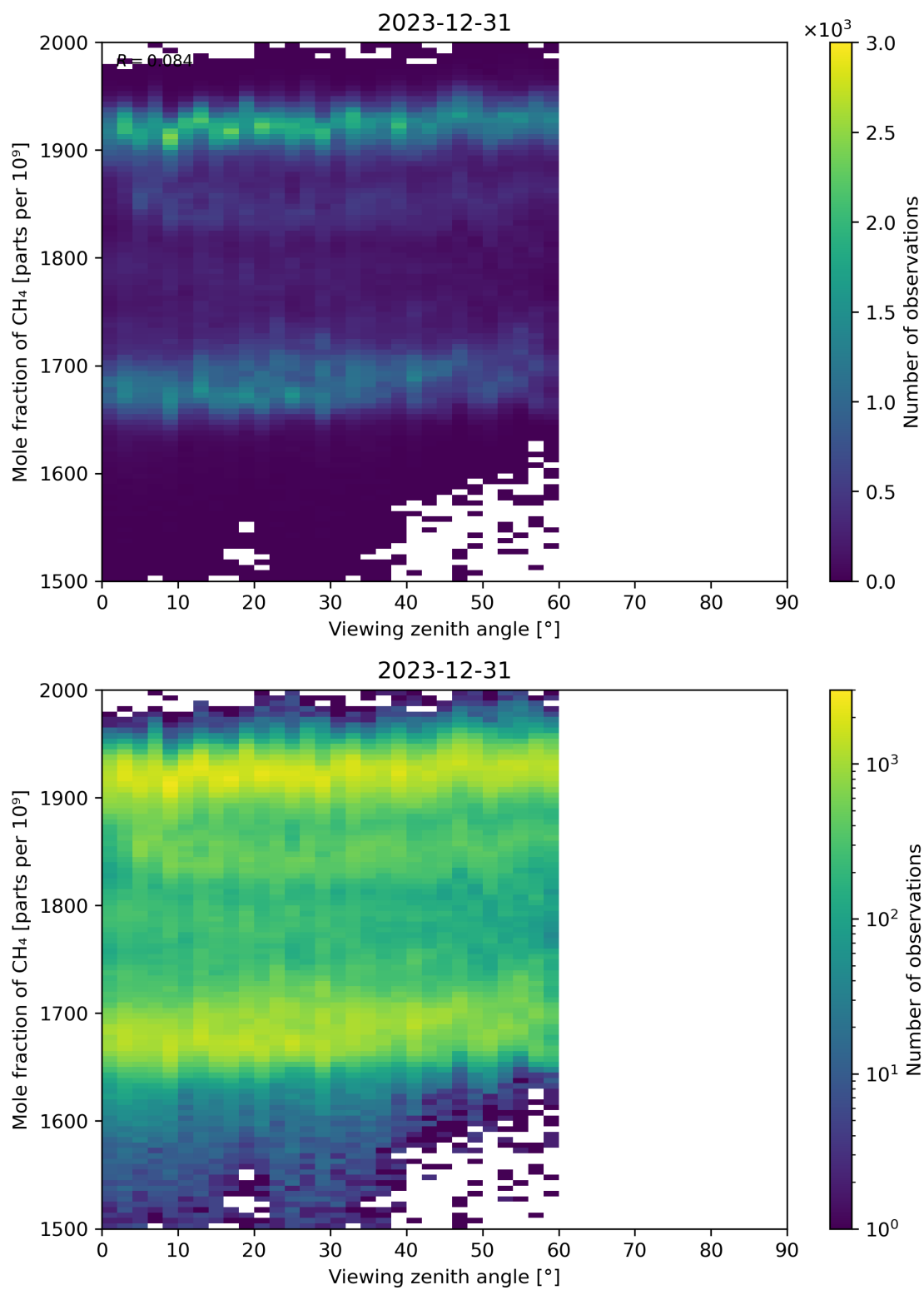
Figure 110: Scatter density plot of “Viewing zenith angle” against “Mole fraction of CH 4 ” for 2023-12-30 to 2023-12-31.
