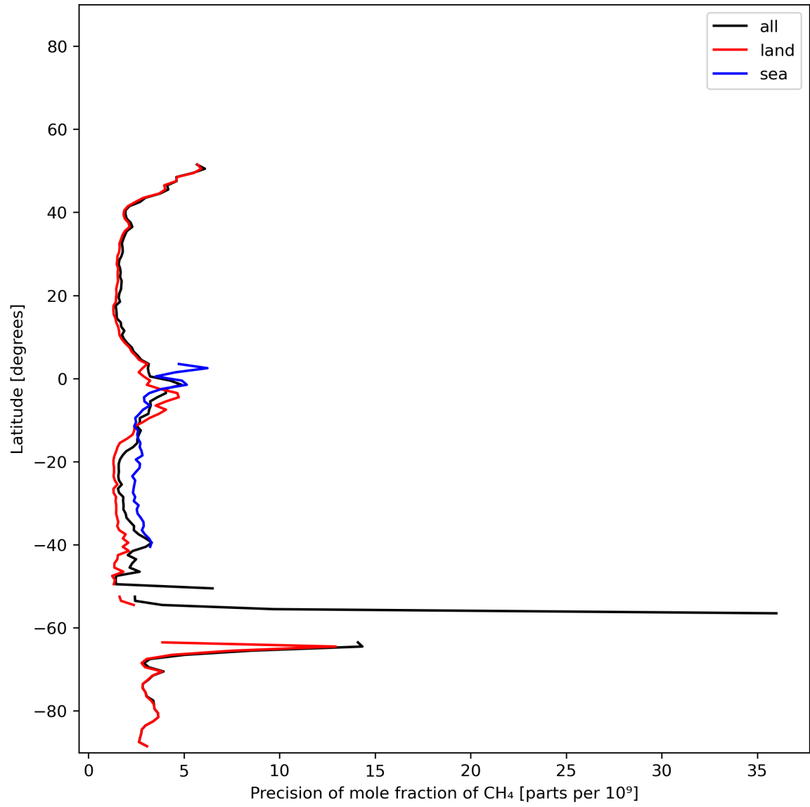
Figure 13: Zonal average of “Precision of mole fraction of CH 4 ” for 2023-12-30 to 2023-12-31.
