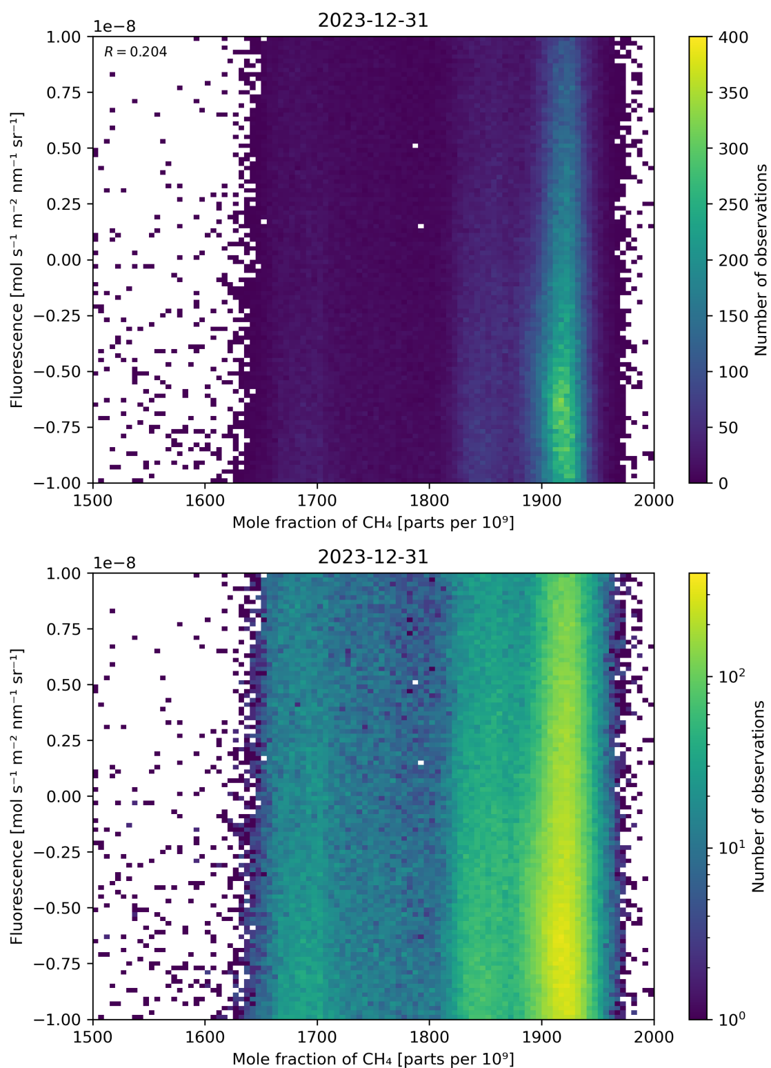
Figure 73: Scatter density plot of “Mole fraction of \text{CH}_4 ” against “Fluorescence” for 2023-12-30 to 2023-12-31.
