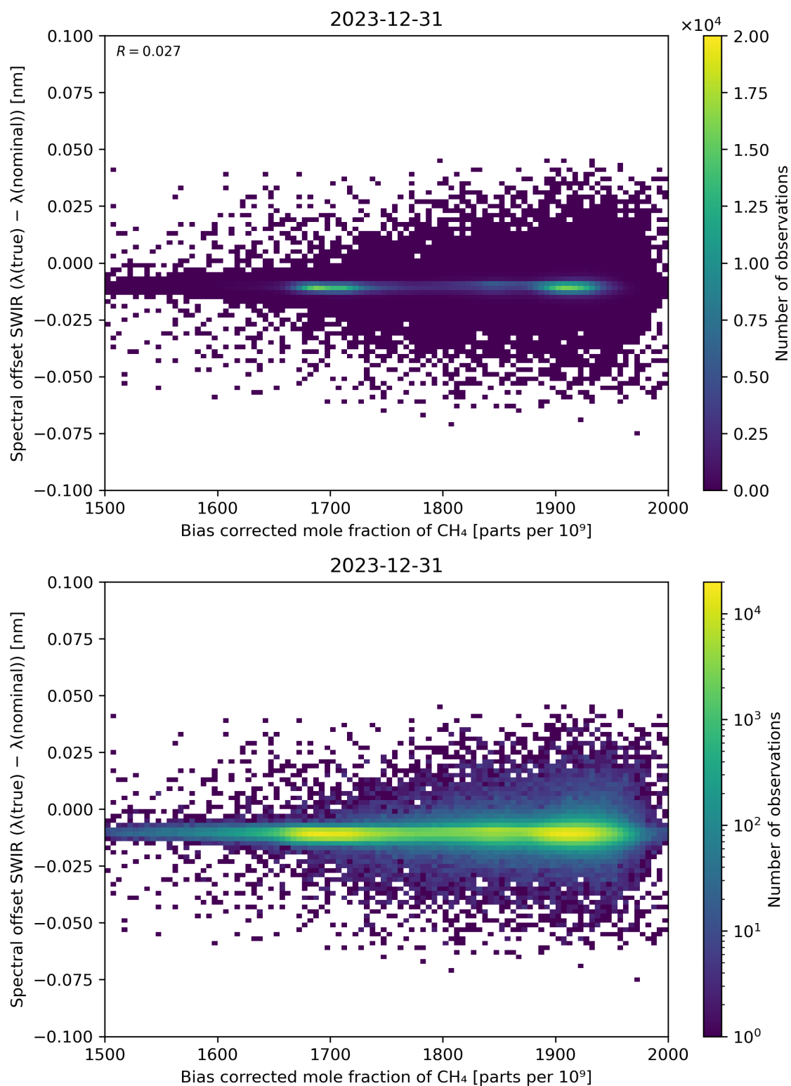
Figure 69: Scatter density plot of “Bias corrected mole fraction of \text{CH}_4 ” against “Spectral offset SWIR ( \lambda(\text{true}) - \lambda(\text{nominal}) )” for 2023-12-30 to 2023-12-31.
