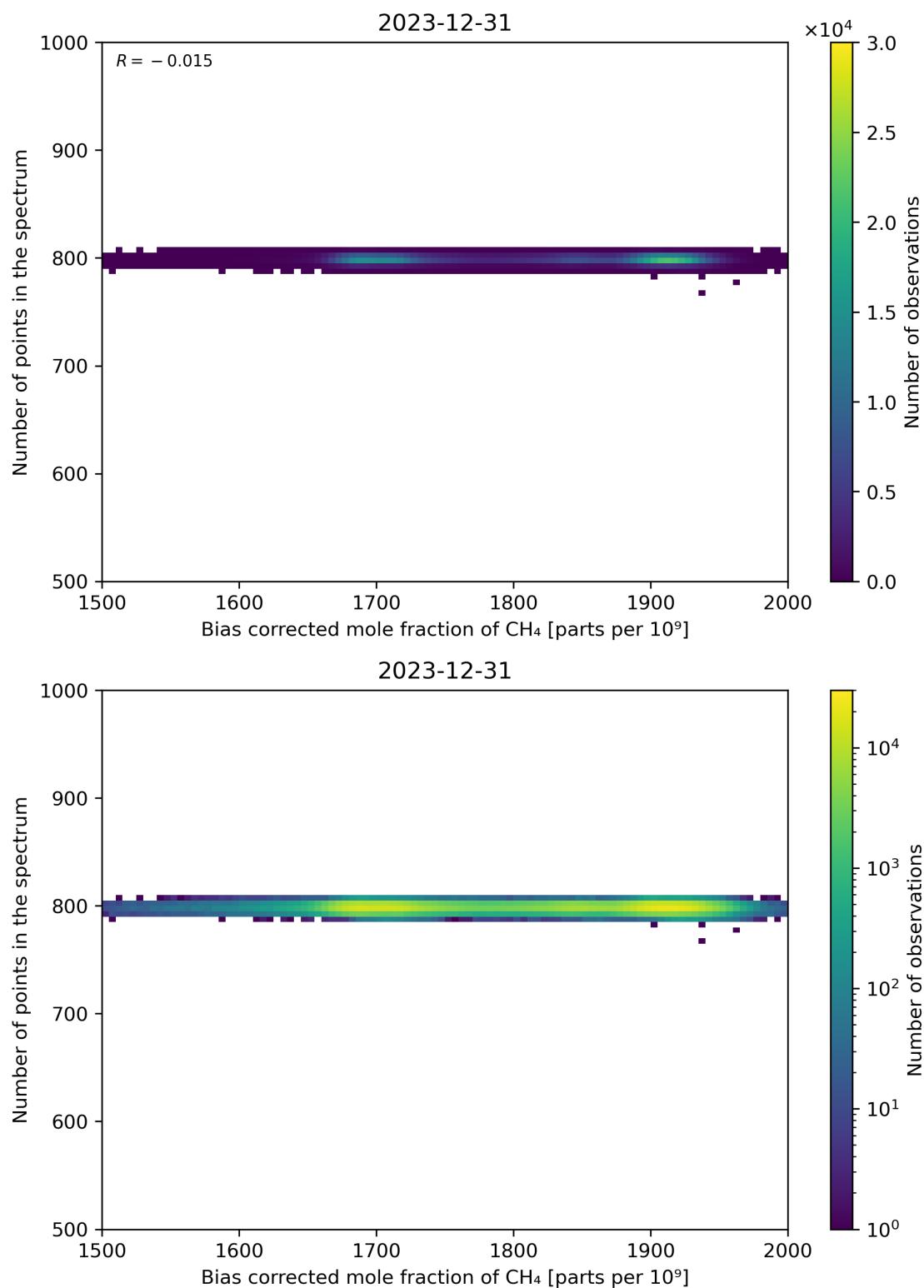
Figure 68: Scatter density plot of “Bias corrected mole fraction of \text{CH}_4 ” against “Number of points in the spectrum” for 2023-12-30 to 2023-12-31.
