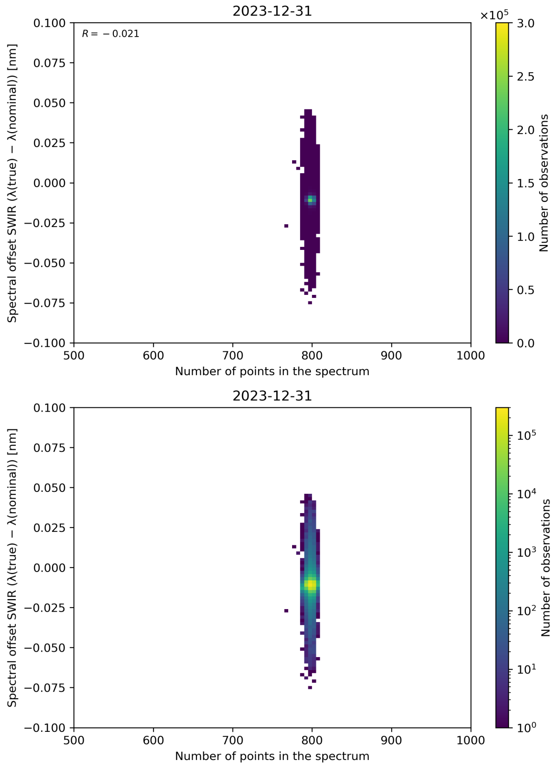
Figure 93: Scatter density plot of “Number of points in the spectrum” against “Spectral offset SWIR ( \lambda(\text{true}) - \lambda(\text{nominal}) )” for 2023-12-30 to 2023-12-31.
