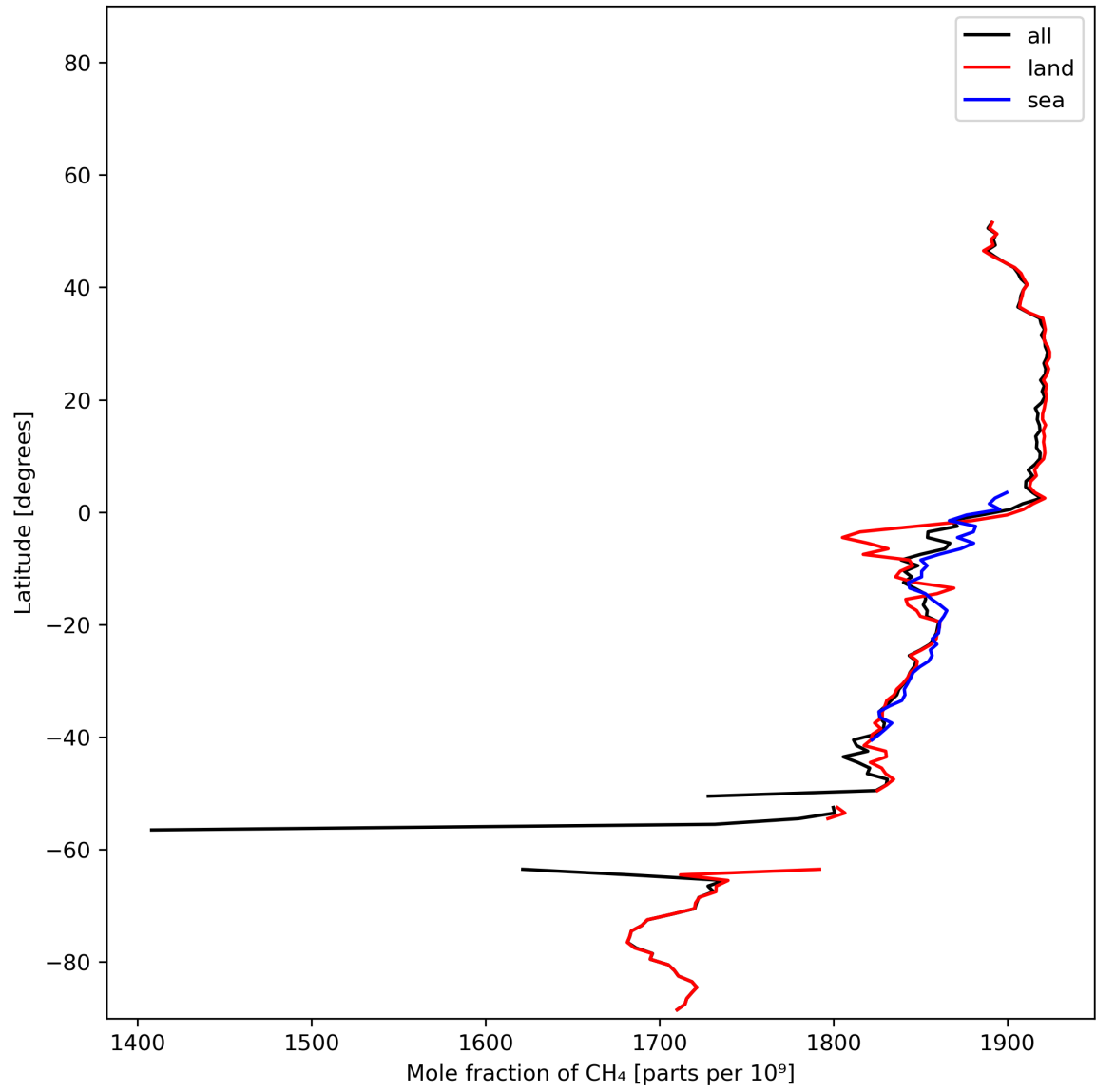
Figure 12: Zonal average of “Mole fraction of CH 4 ” for 2023-12-30 to 2023-12-31.
