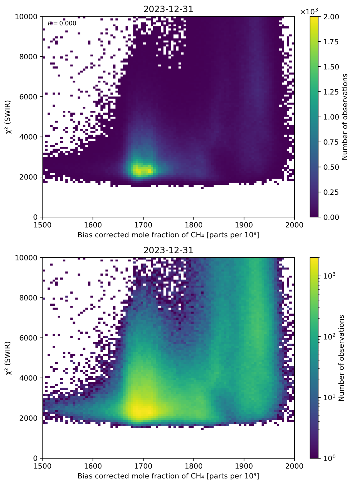
Figure 64: Scatter density plot of “Bias corrected mole fraction of \text{CH}_4 ” against “ \chi^2 (SWIR)” for 2023-12-30 to 2023-12-31.
