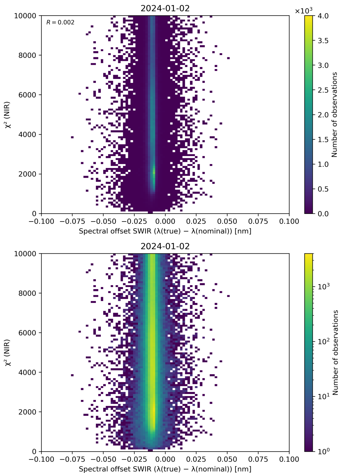
Figure 117: Scatter density plot of “Spectral offset SWIR ( \lambda(\text{true}) - \lambda(\text{nominal}) )” against “ \chi^2 (NIR)” for 2024-01-01 to 2024-01-03.
