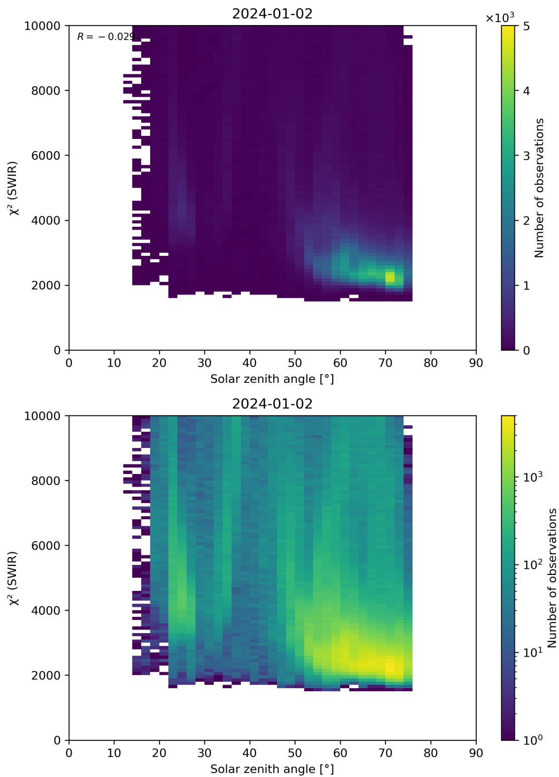
Figure 95: Scatter density plot of “Solar zenith angle” against “ \chi^2 (SWIR)” for 2024-01-01 to 2024-01-03.
