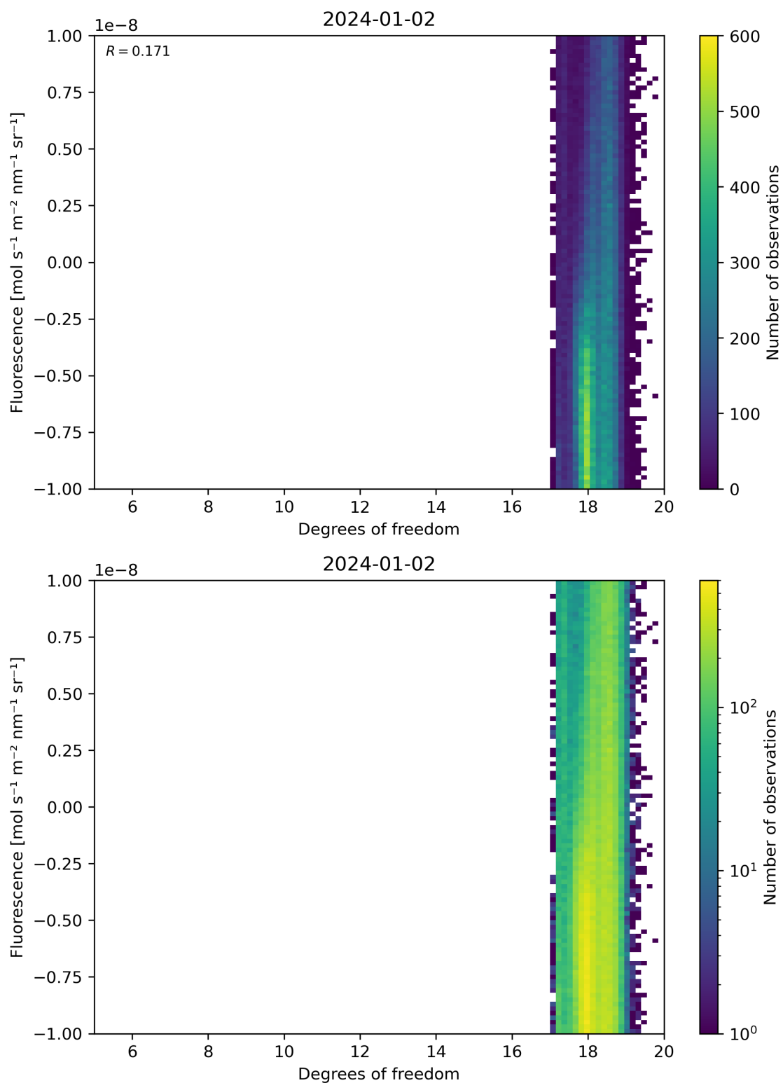
Figure 51: Scatter density plot of “Degrees of freedom” against “Fluorescence” for 2024-01-01 to 2024-01-03.
