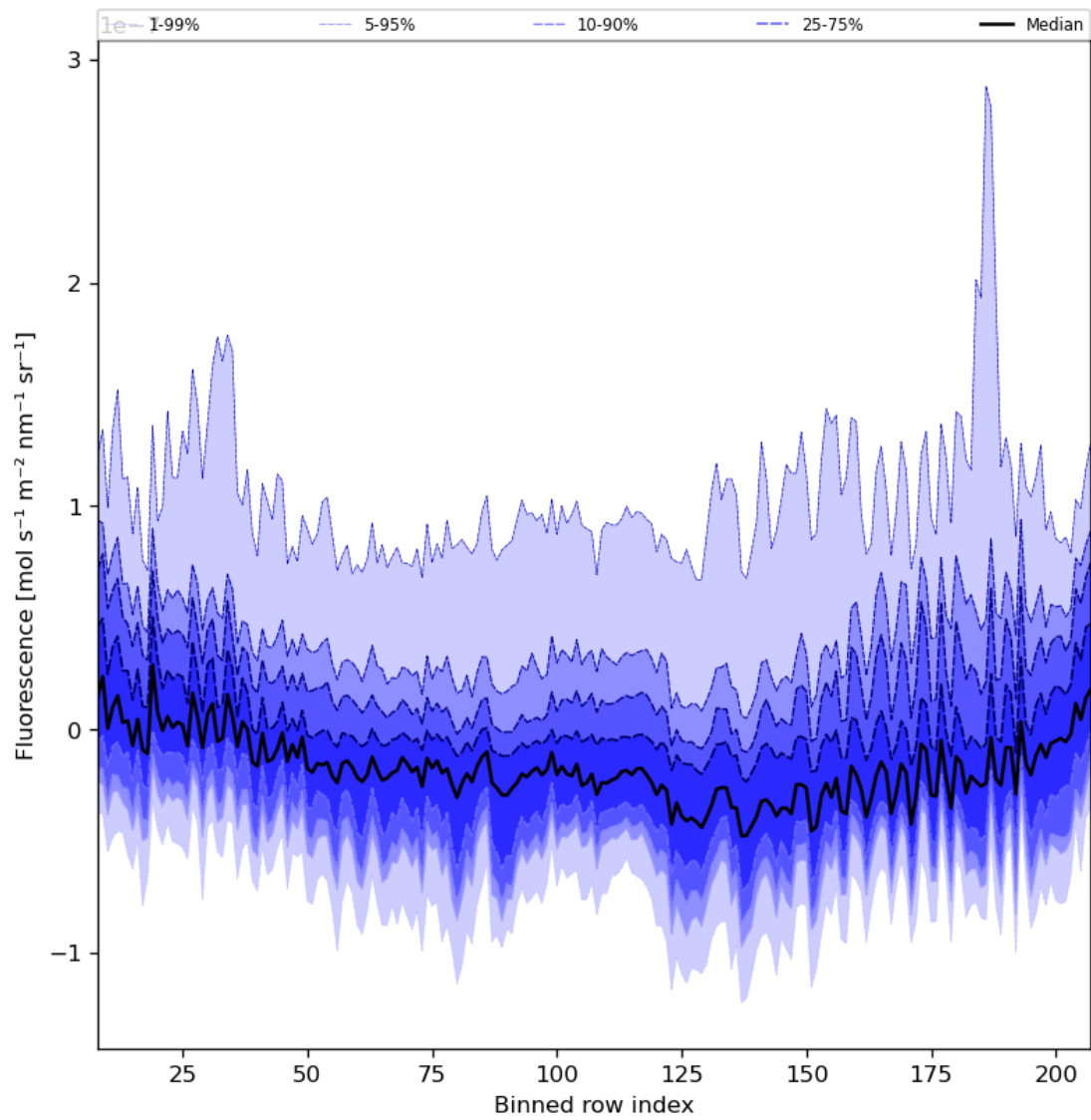
Figure 43: Along track statistics of “Fluorescence” for 2024-01-01 to 2024-01-03
