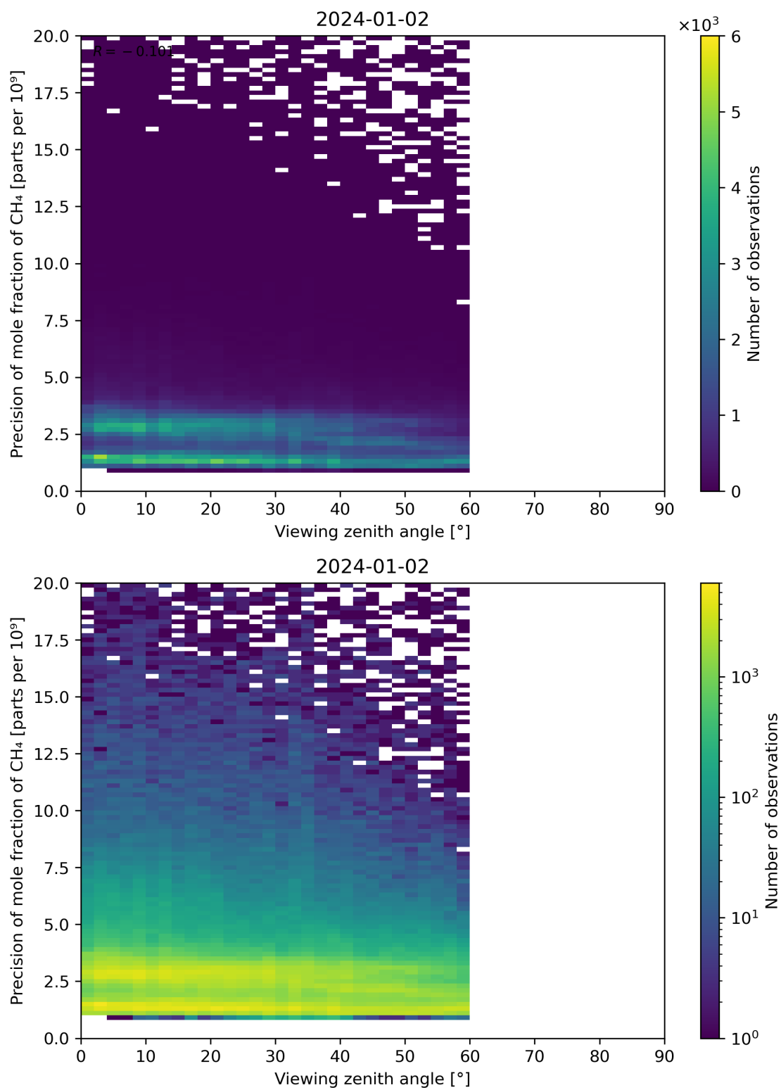
Figure 112: Scatter density plot of “Viewing zenith angle” against “Precision of mole fraction of CH 4 ” for 2024-01-01 to 2024-01-03.
