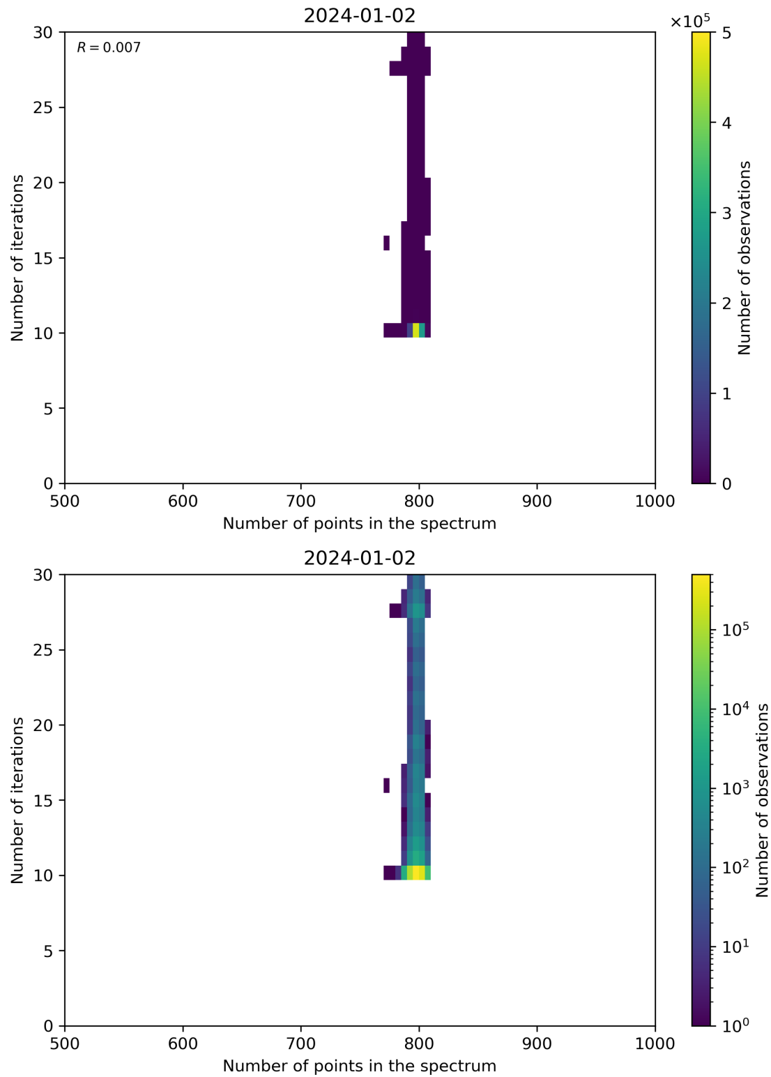
Figure 92: Scatter density plot of “Number of points in the spectrum” against “Number of iterations” for 2024-01-01 to 2024-01-03.
