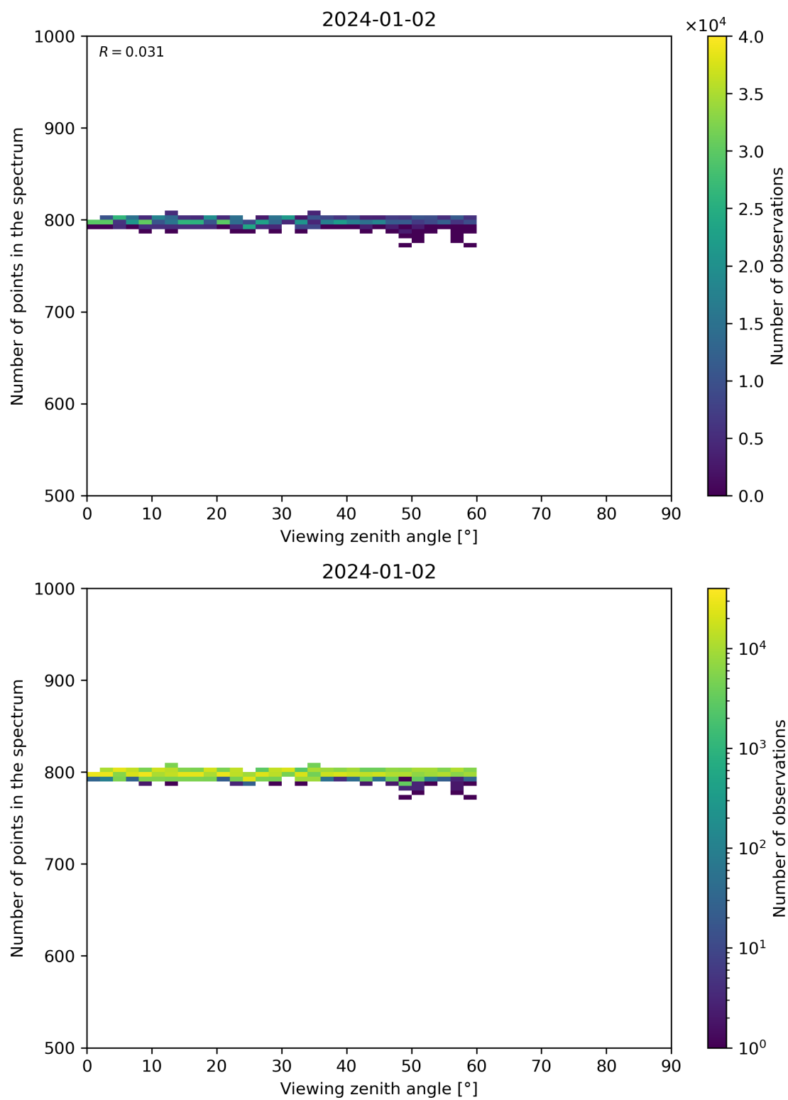
Figure 114: Scatter density plot of “Viewing zenith angle” against “Number of points in the spectrum” for 2024-01-01 to 2024-01-03.
