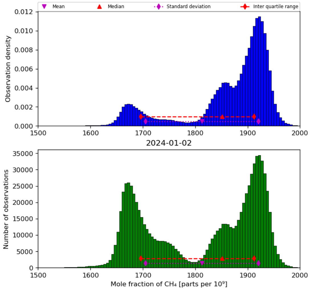
Figure 23: Histogram of “Mole fraction of CH 4 ” for 2024-01-01 to 2024-01-03
