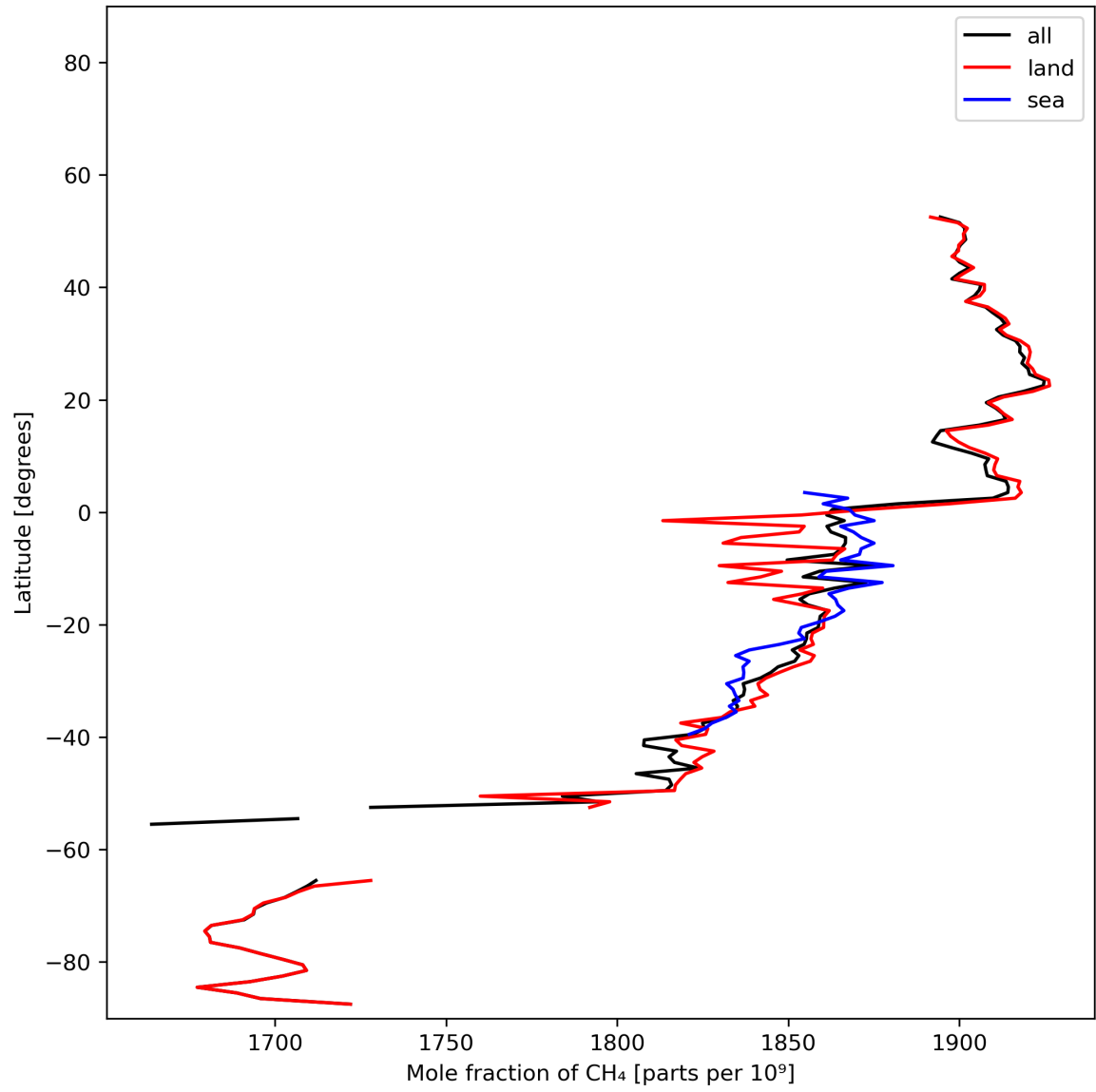
Figure 12: Zonal average of “Mole fraction of \text{CH}_4 ” for 2024-01-01 to 2024-01-03.
