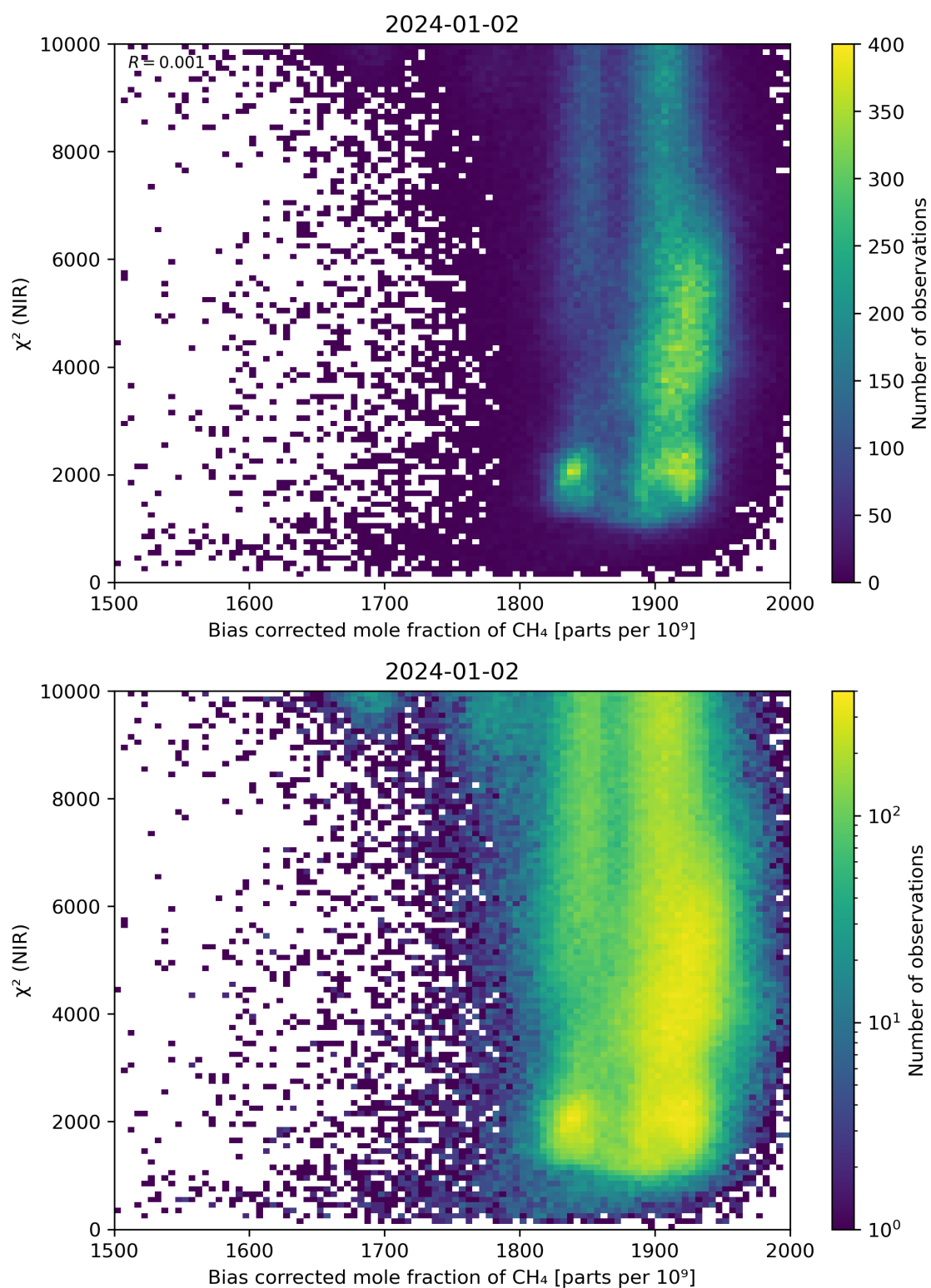
Figure 63: Scatter density plot of “Bias corrected mole fraction of CH 4 ” against “ \chi^2 (NIR)” for 2024-01-01 to 2024-01-03.
