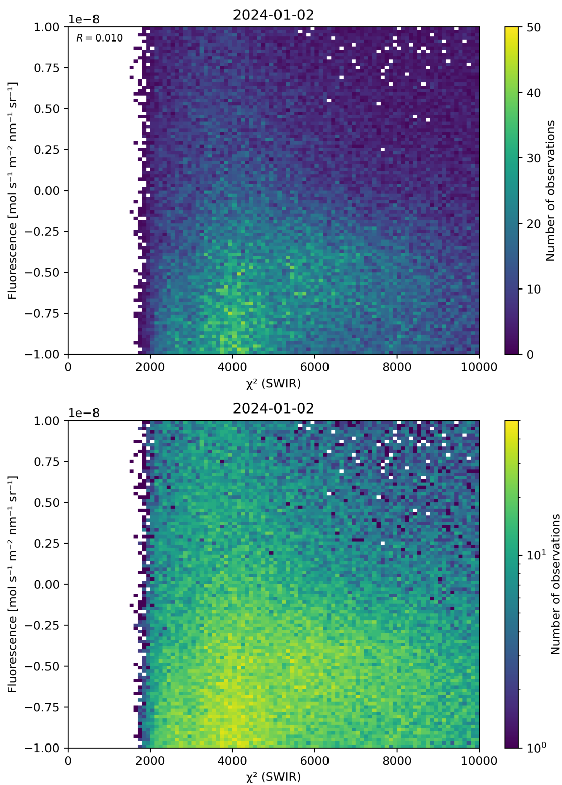
Figure 49: Scatter density plot of “ \chi^2 (SWIR)” against “Fluorescence” for 2024-01-01 to 2024-01-03.
