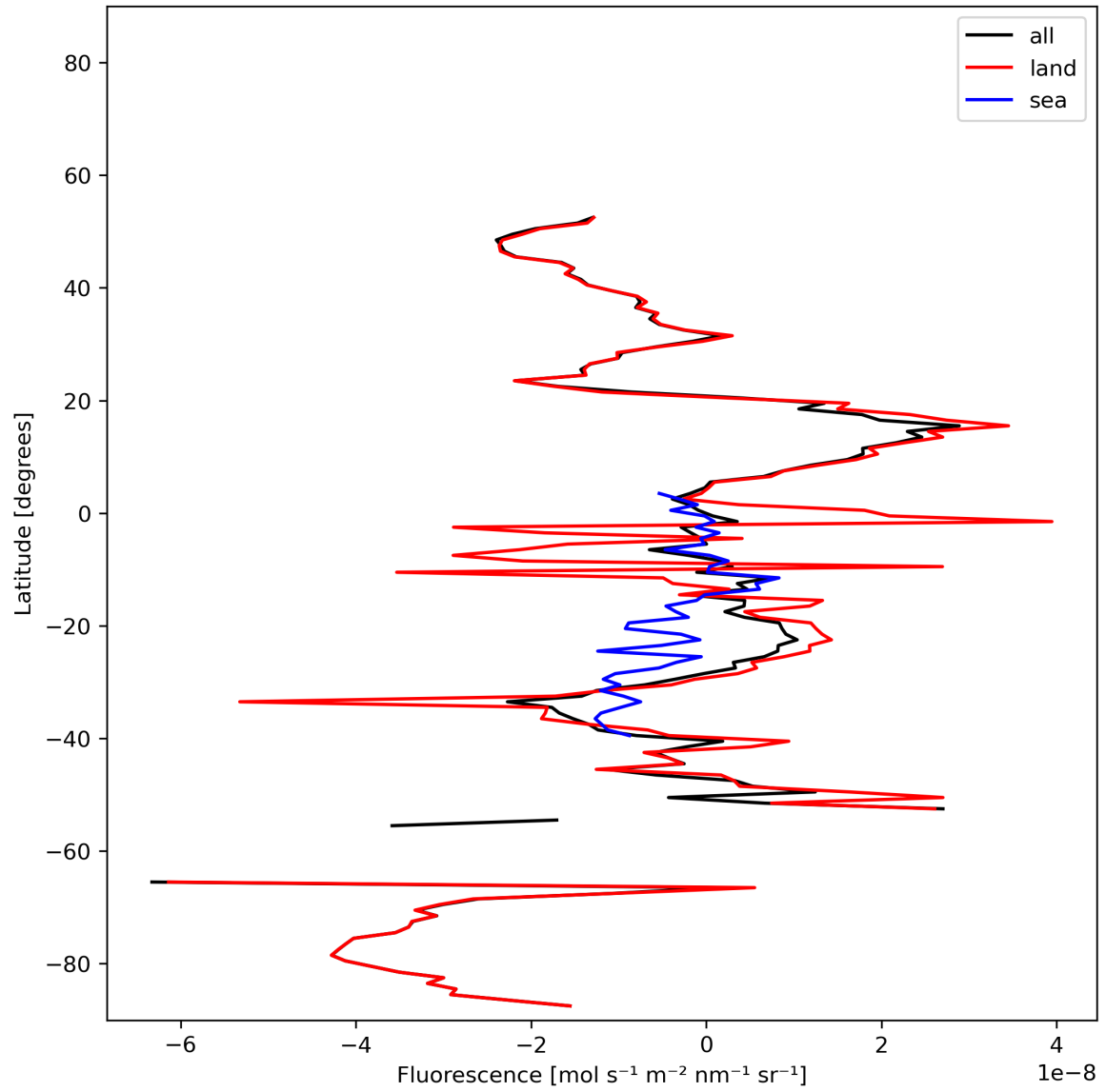
Figure 21: Zonal average of “Fluorescence” for 2024-01-01 to 2024-01-03.
