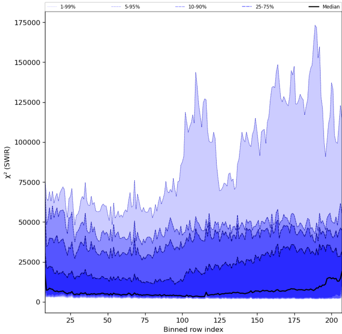
Figure 39: Along track statistics of “ \chi^2 (SWIR)” for 2024-01-01 to 2024-01-03
