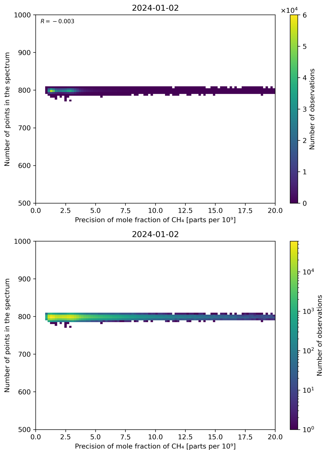
Figure 84: Scatter density plot of “Precision of mole fraction of CH 4 ” against “Number of points in the spectrum” for 2024-01-01 to 2024-01-03.
