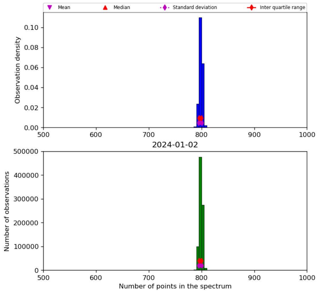
Figure 26: Histogram of “Number of points in the spectrum” for 2024-01-01 to 2024-01-03
