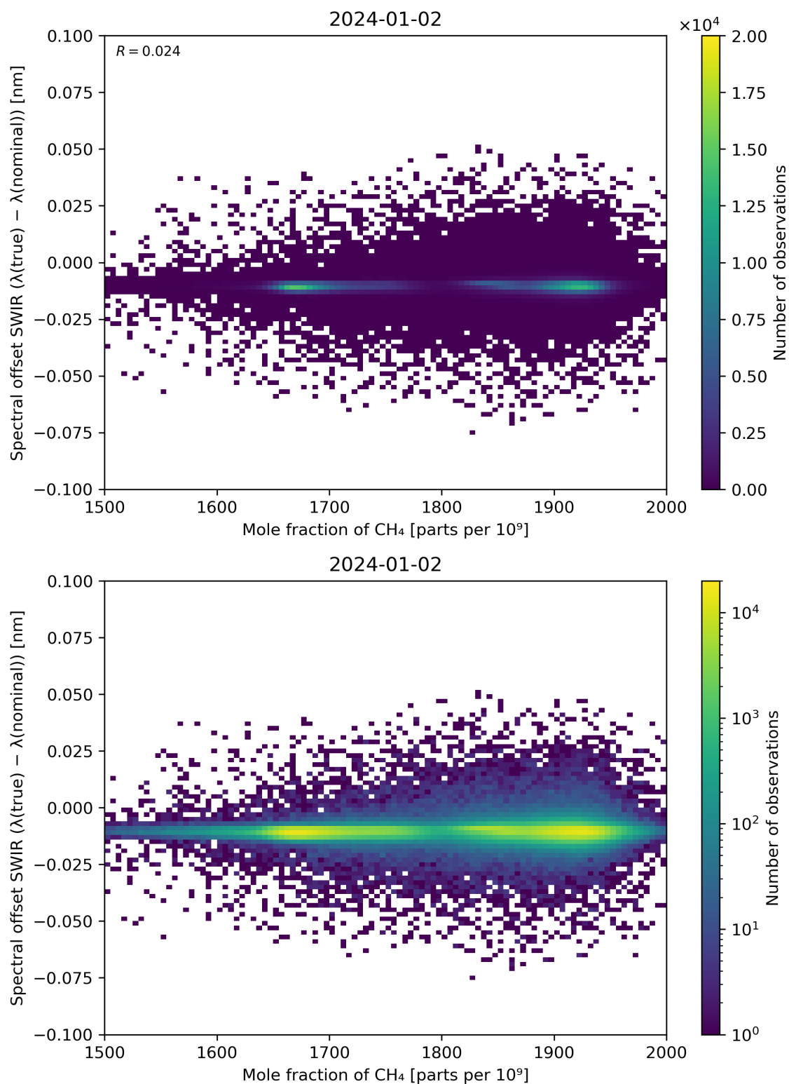
Figure 86: Scatter density plot of “Mole fraction of \text{CH}_4 ” against “Spectral offset SWIR ( \lambda(\text{true}) - \lambda(\text{nominal}) )” for 2024-01-01 to 2024-01-03.
