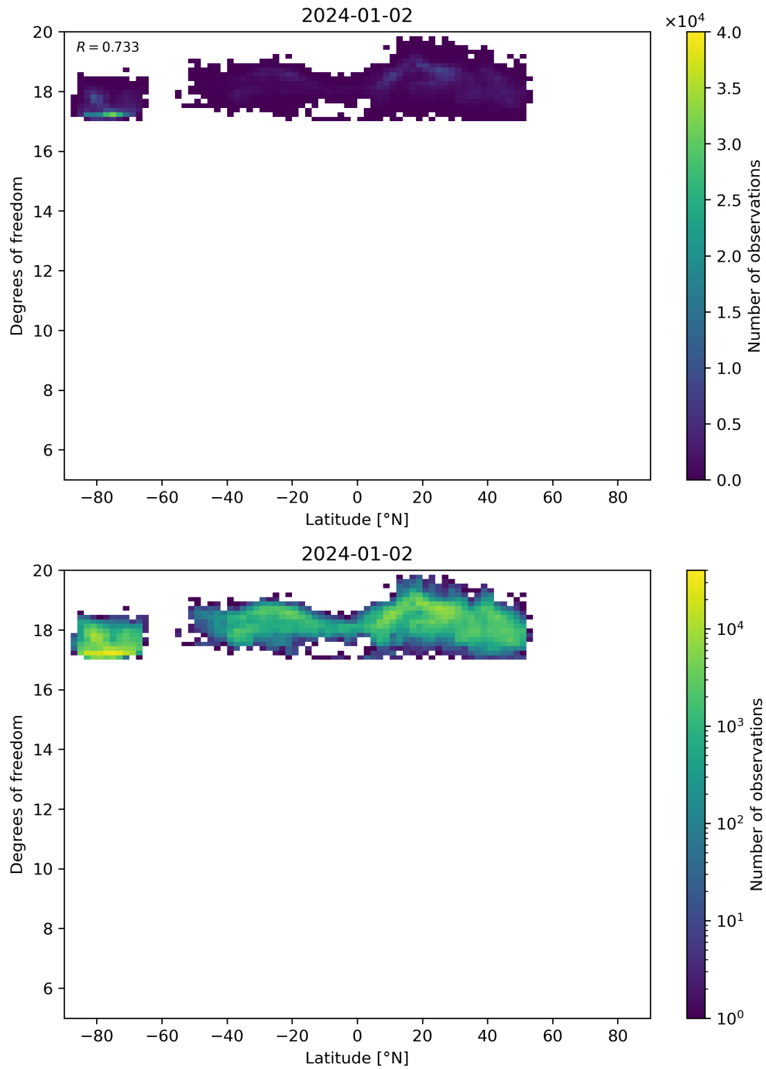
Figure 55: Scatter density plot of “Latitude” against “Degrees of freedom” for 2024-01-01 to 2024-01-03.
