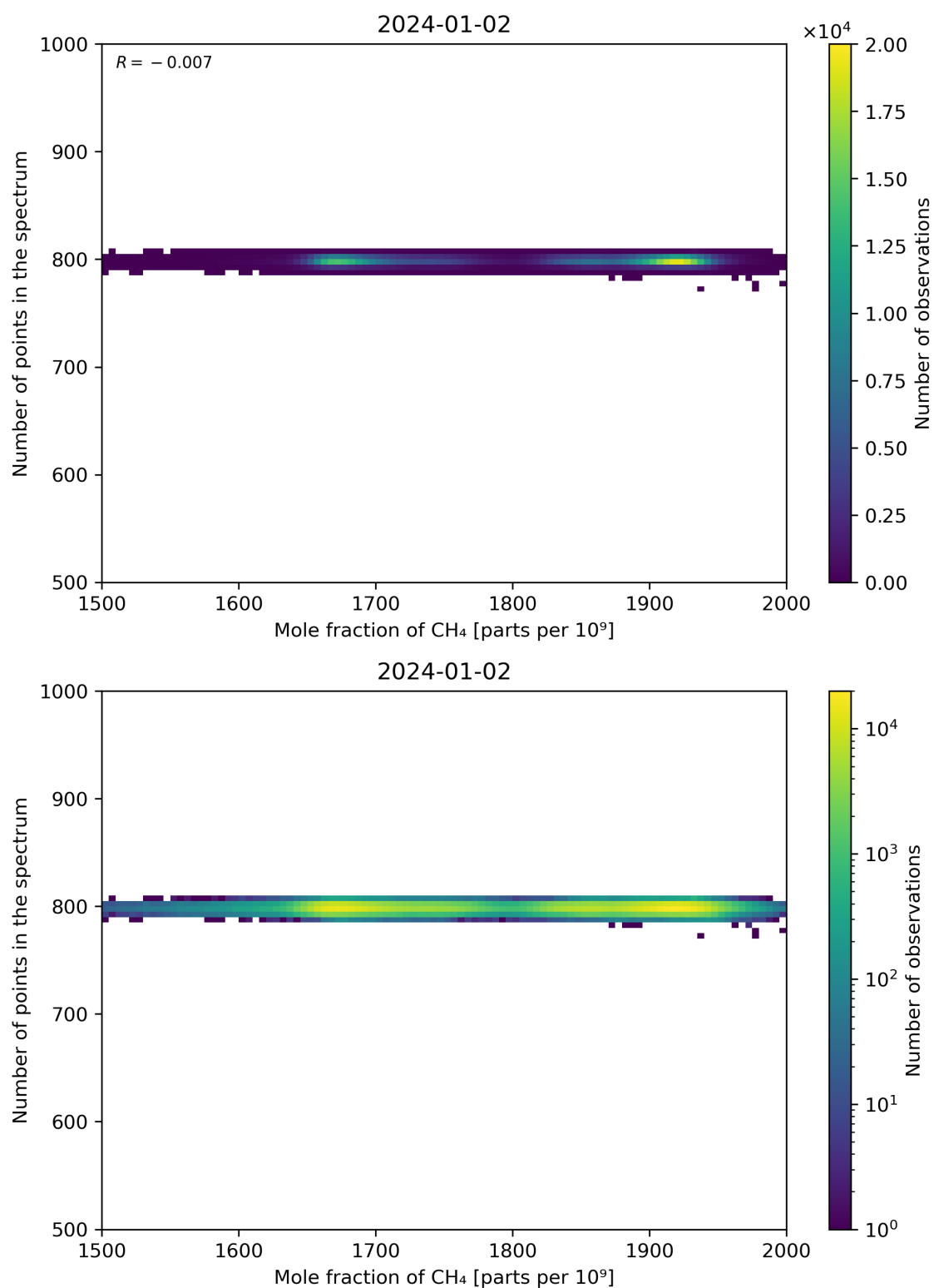
Figure 77: Scatter density plot of “Mole fraction of CH 4 ” against “Number of points in the spectrum” for 2024-01-01 to 2024-01-03.
