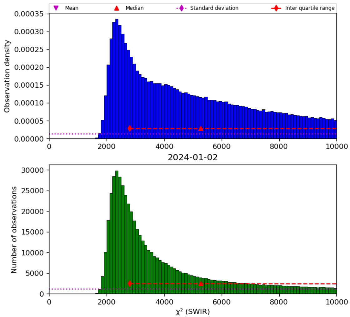
Figure 28: Histogram of “ \chi^2 (SWIR)” for 2024-01-01 to 2024-01-03
