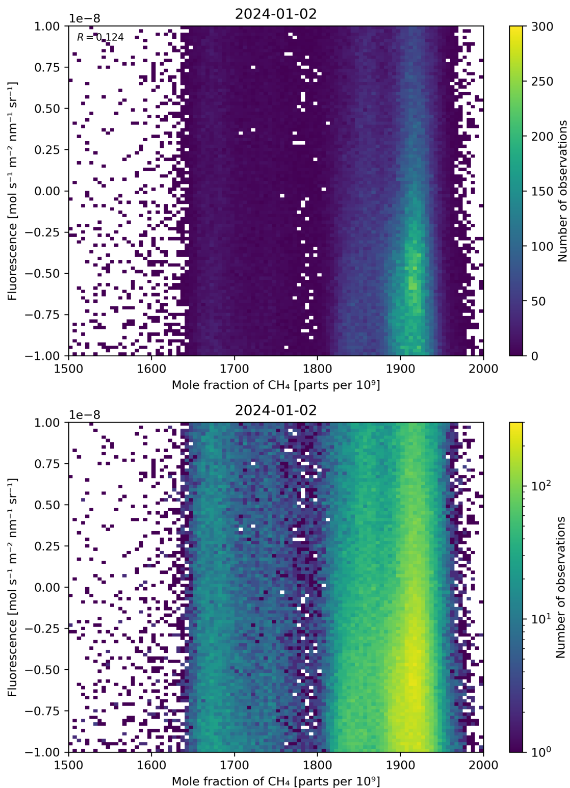
Figure 73: Scatter density plot of “Mole fraction of \text{CH}_4 ” against “Fluorescence” for 2024-01-01 to 2024-01-03.
