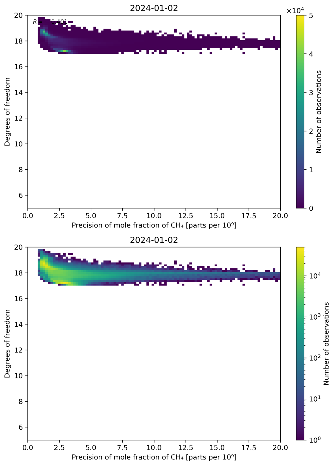
Figure 80: Scatter density plot of “Precision of mole fraction of CH 4 ” against “Degrees of freedom” for 2024-01-01 to 2024-01-03.
