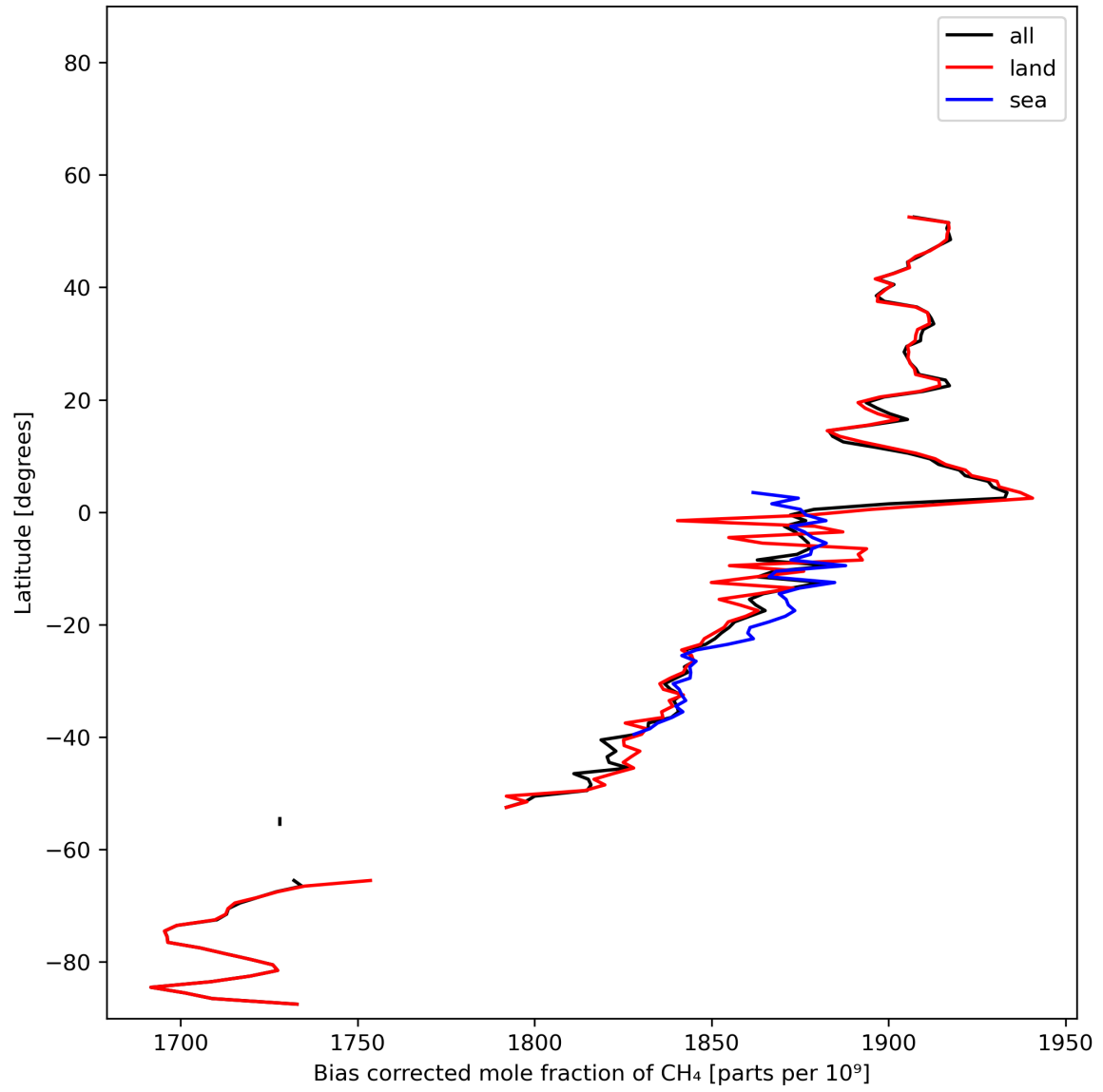
Figure 14: Zonal average of “Bias corrected mole fraction of CH 4 ” for 2024-01-01 to 2024-01-03.
