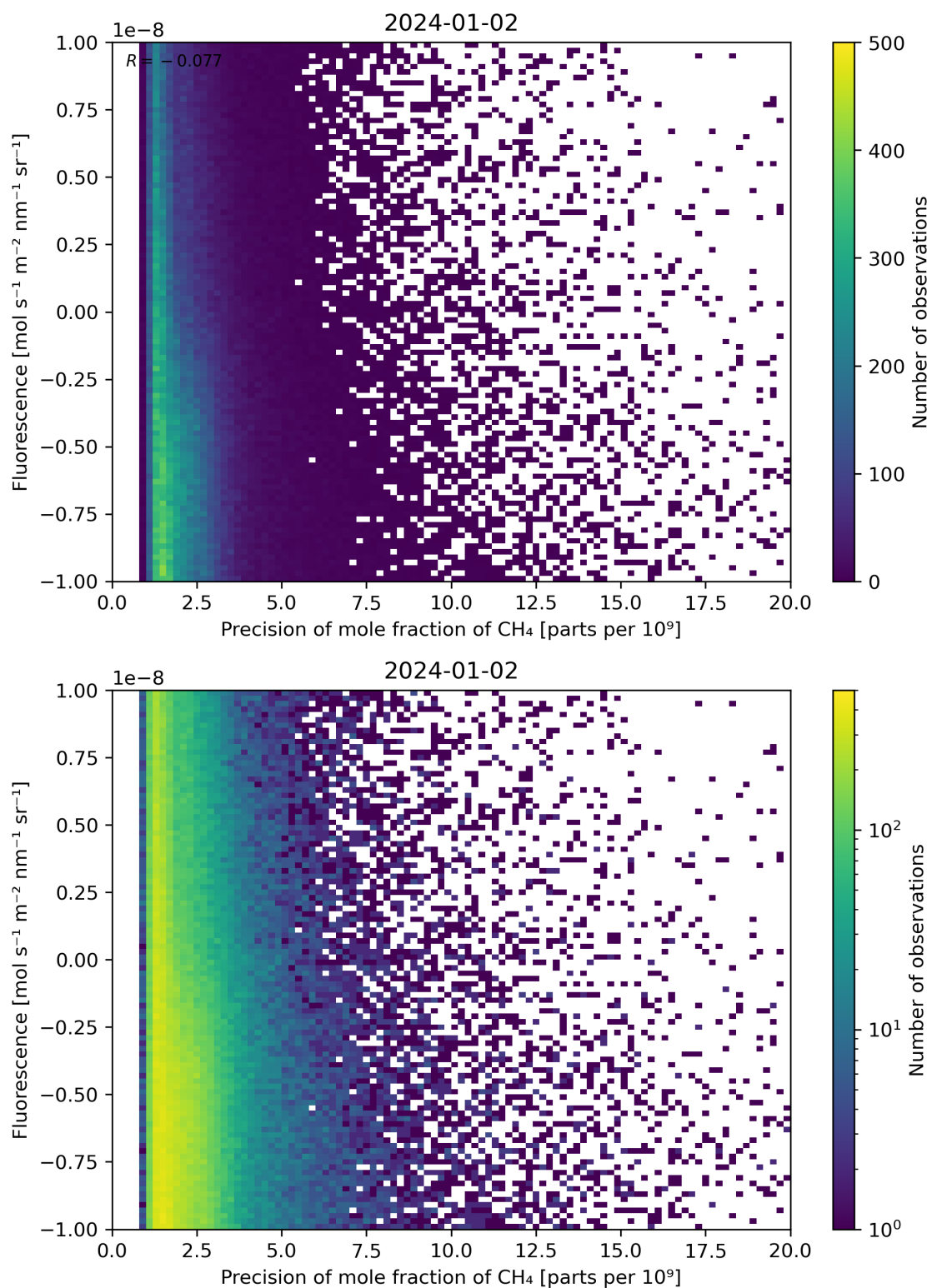
Figure 81: Scatter density plot of “Precision of mole fraction of \text{CH}_4 ” against “Fluorescence” for 2024-01-01 to 2024-01-03.
