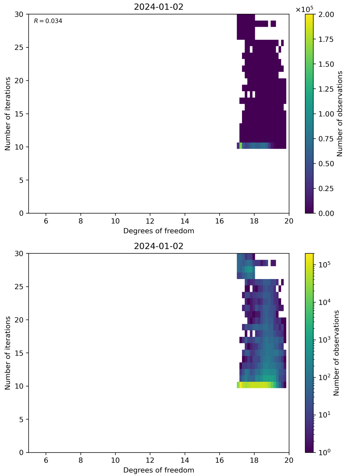
Figure 52: Scatter density plot of “Degrees of freedom” against “Number of iterations” for 2024-01-01 to 2024-01-03.
