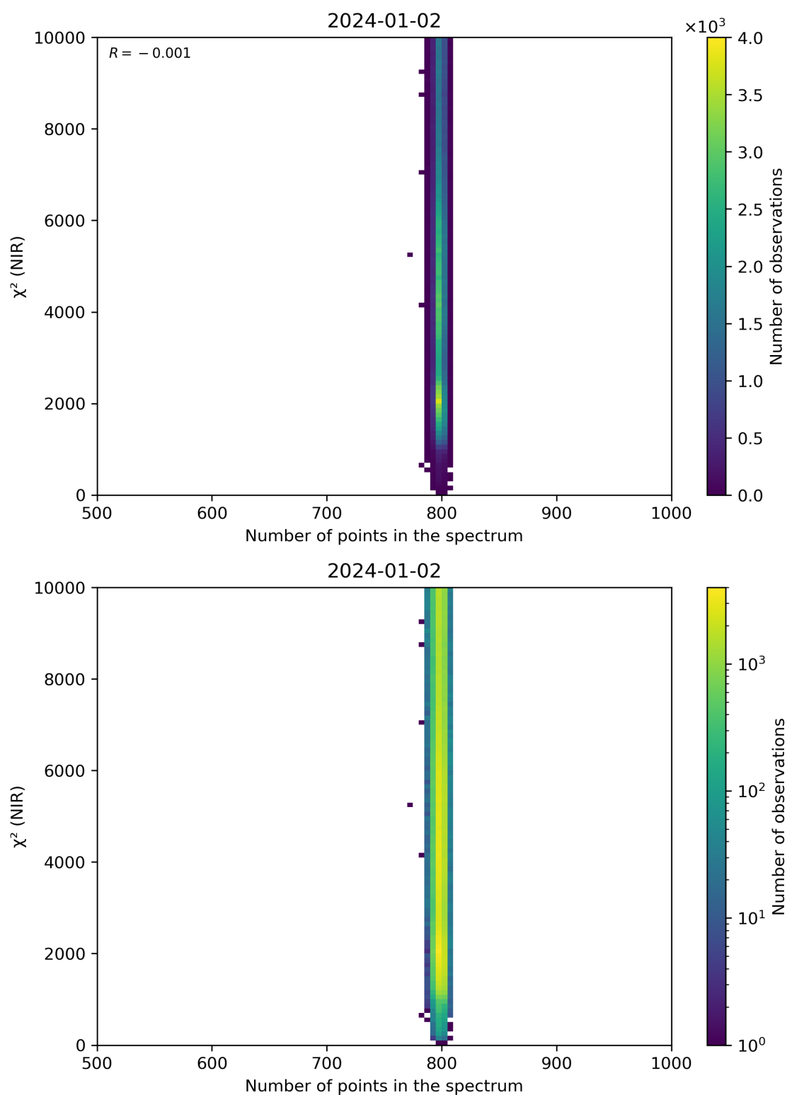
Figure 88: Scatter density plot of “Number of points in the spectrum” against “ \chi^2 (NIR)” for 2024-01-01 to 2024-01-03.
