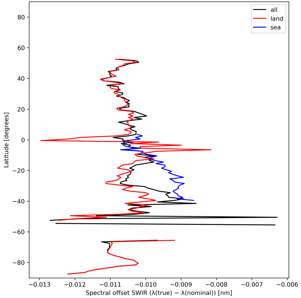
Figure 16: Zonal average of “Spectral offset SWIR ( \lambda(\text{true}) - \lambda(\text{nominal}) )” for 2024-01-01 to 2024-01-03.
