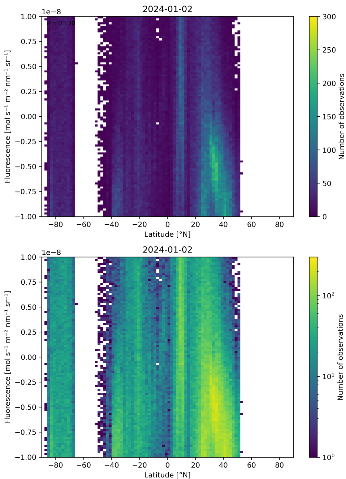
Figure 56: Scatter density plot of “Latitude” against “Fluorescence” for 2024-01-01 to 2024-01-03.
