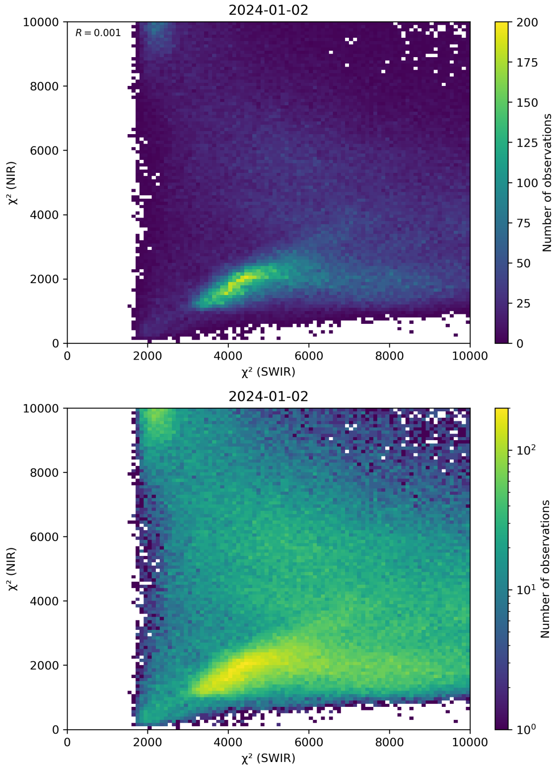
Figure 47: Scatter density plot of “ \chi^2 (SWIR)” against “ \chi^2 (NIR)” for 2024-01-01 to 2024-01-03.
