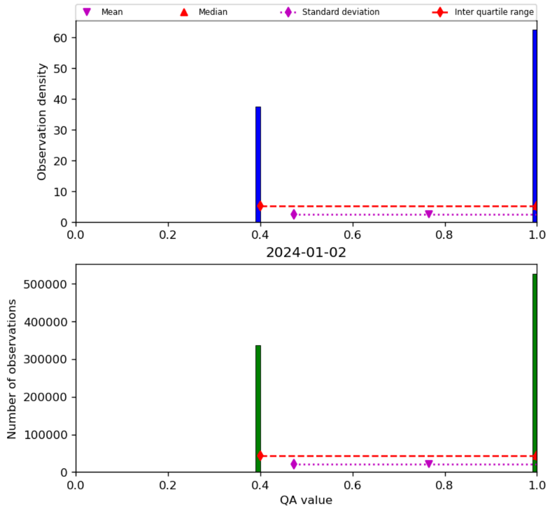
Figure 22: Histogram of “QA value” for 2024-01-01 to 2024-01-03
