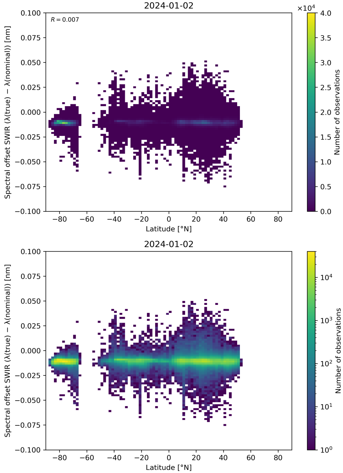
Figure 62: Scatter density plot of “Latitude” against “Spectral offset SWIR ( \lambda(\text{true}) - \lambda(\text{nominal}) )” for 2024-01-01 to 2024-01-03.
