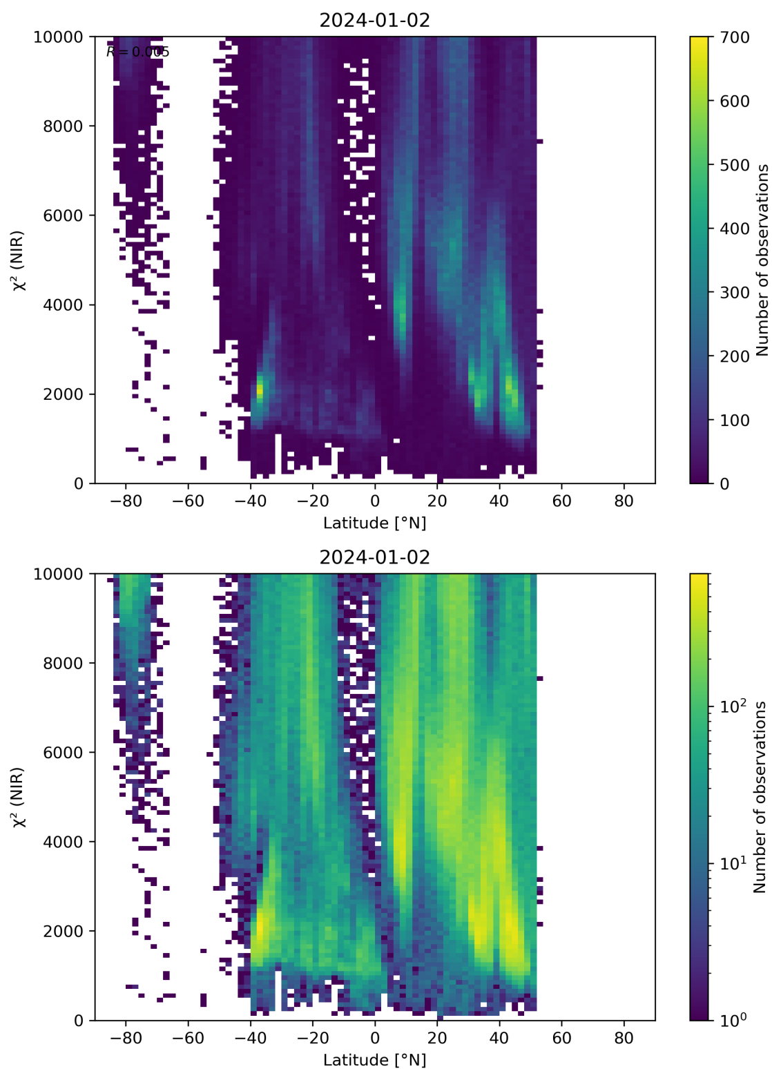
Figure 53: Scatter density plot of “Latitude” against “ \chi^2 (NIR)” for 2024-01-01 to 2024-01-03.
