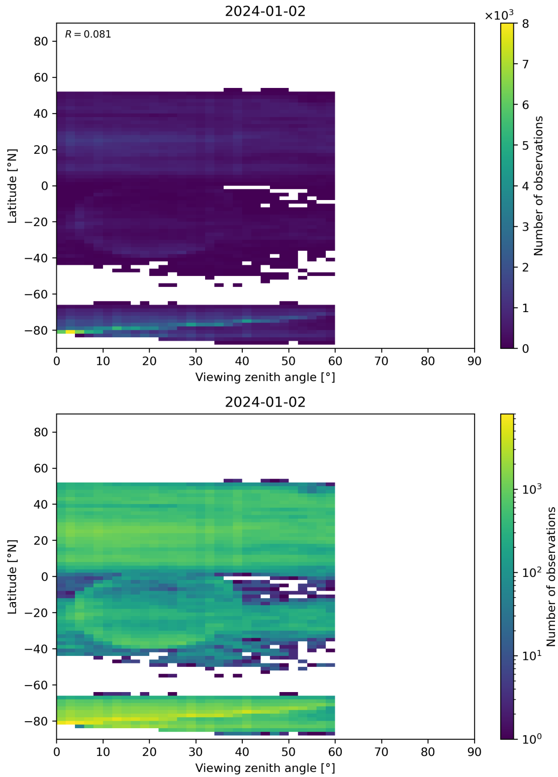
Figure 109: Scatter density plot of “Viewing zenith angle” against “Latitude” for 2024-01-01 to 2024-01-03.
