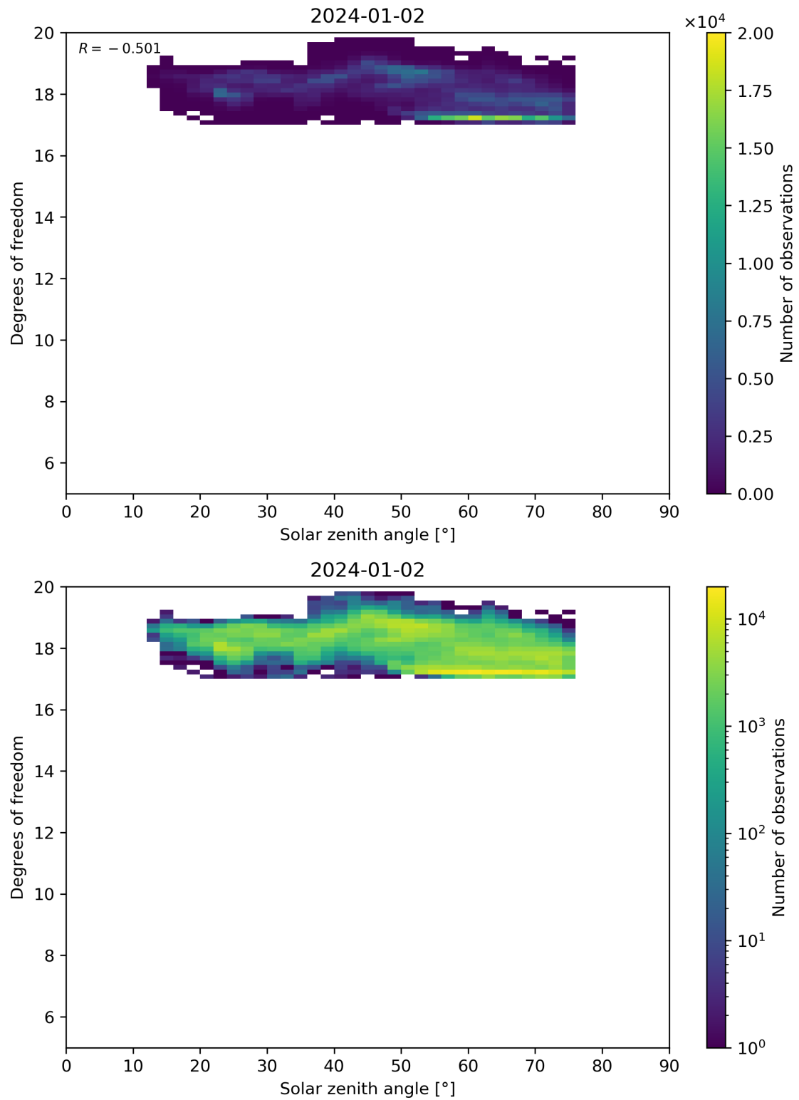
Figure 96: Scatter density plot of “Solar zenith angle” against “Degrees of freedom” for 2024-01-01 to 2024-01-03.
