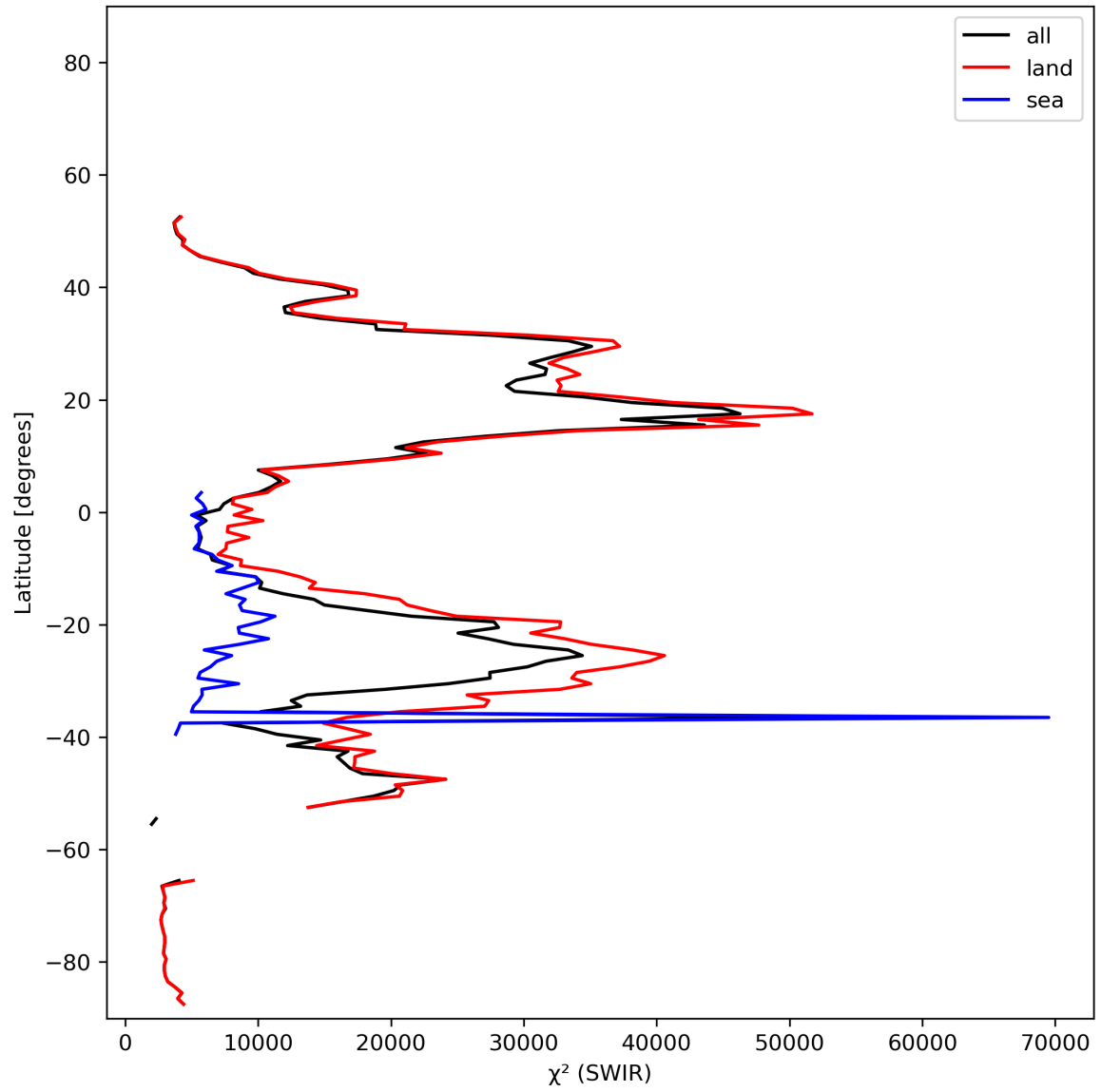
Figure 17: Zonal average of “ \chi^2 (SWIR)” for 2024-01-01 to 2024-01-03.
