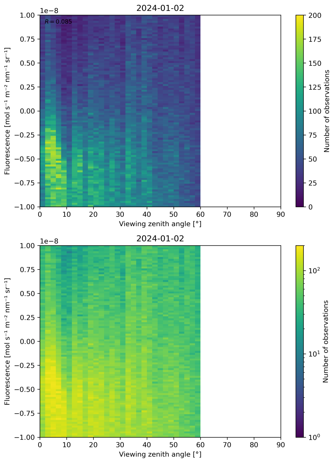
Figure 108: Scatter density plot of “Viewing zenith angle” against “Fluorescence” for 2024-01-01 to 2024-01-03.
