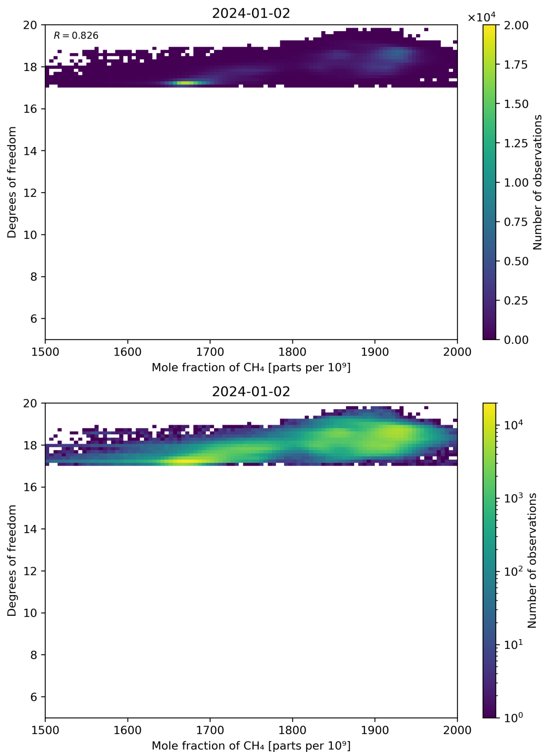
Figure 72: Scatter density plot of “Mole fraction of CH 4 ” against “Degrees of freedom” for 2024-01-01 to 2024-01-03.
