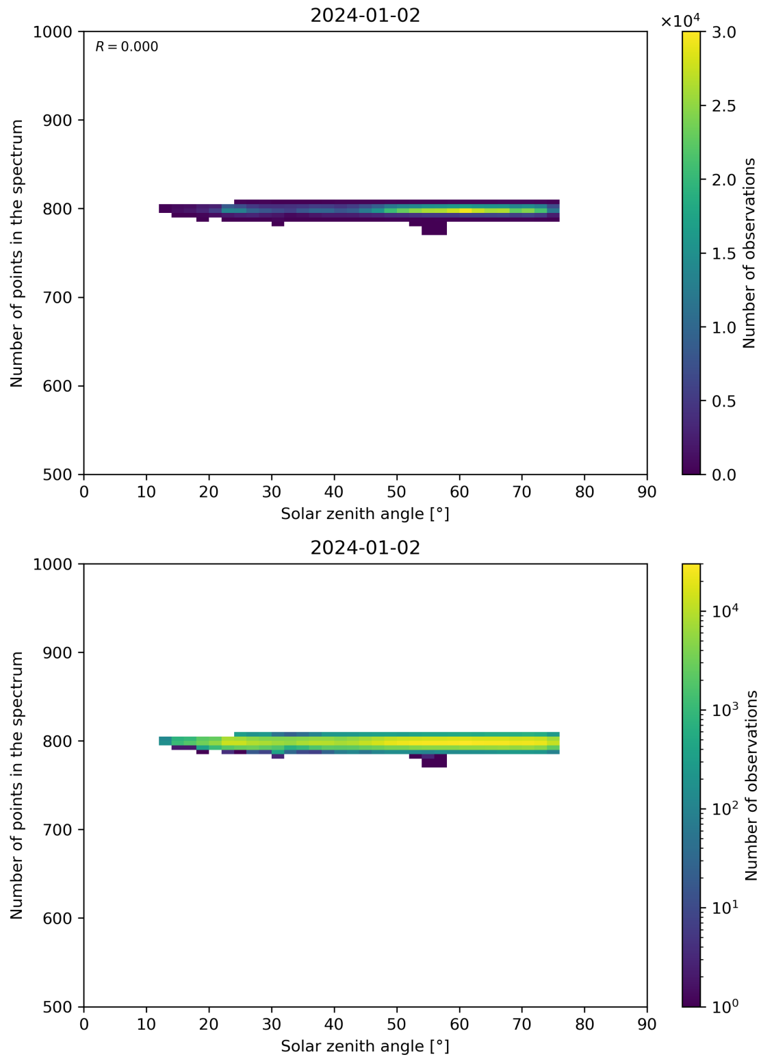
Figure 103: Scatter density plot of “Solar zenith angle” against “Number of points in the spectrum” for 2024-01-01 to 2024-01-03.
