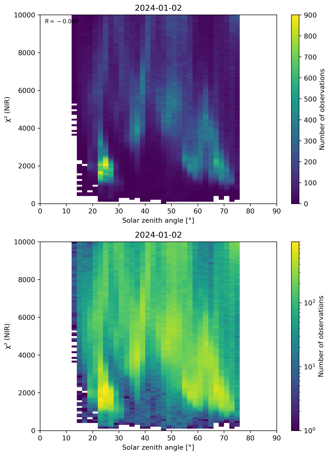
Figure 94: Scatter density plot of “Solar zenith angle” against “ \chi^2 (NIR)” for 2024-01-01 to 2024-01-03.
