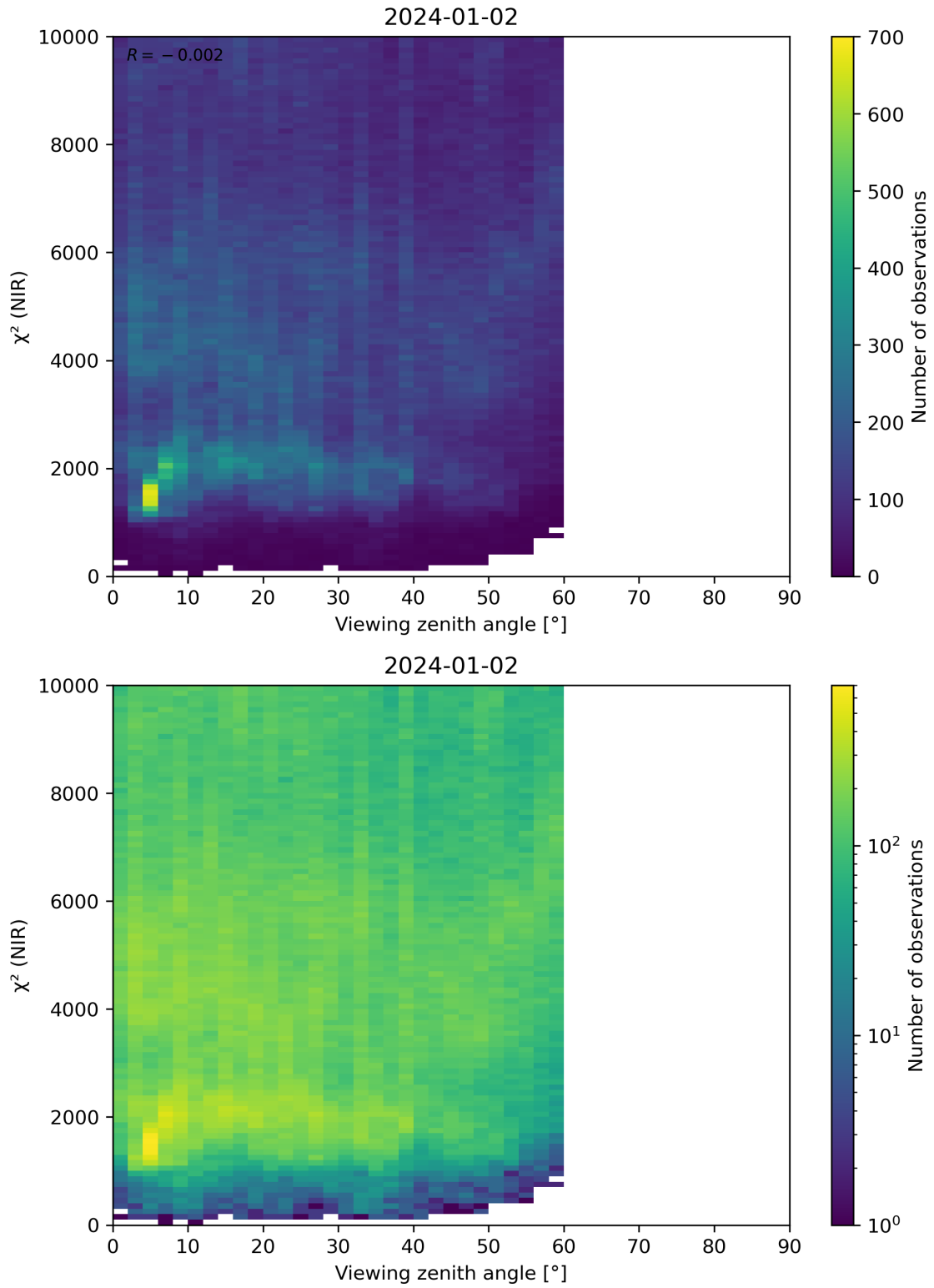
Figure 105: Scatter density plot of “Viewing zenith angle” against “ \chi^2 (NIR)” for 2024-01-01 to 2024-01-03.
