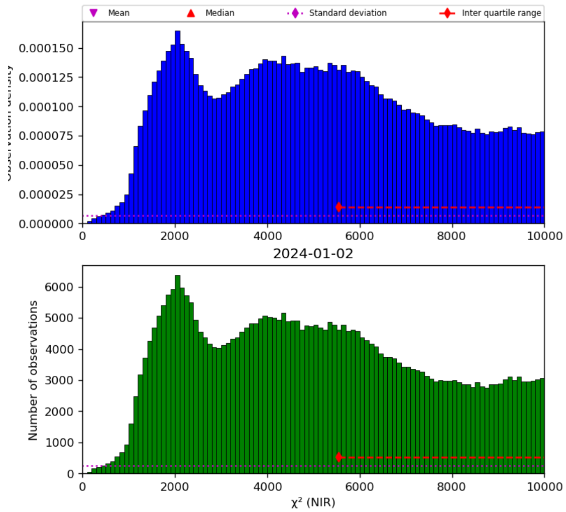
Figure 29: Histogram of “ \chi^2 (NIR)” for 2024-01-01 to 2024-01-03
