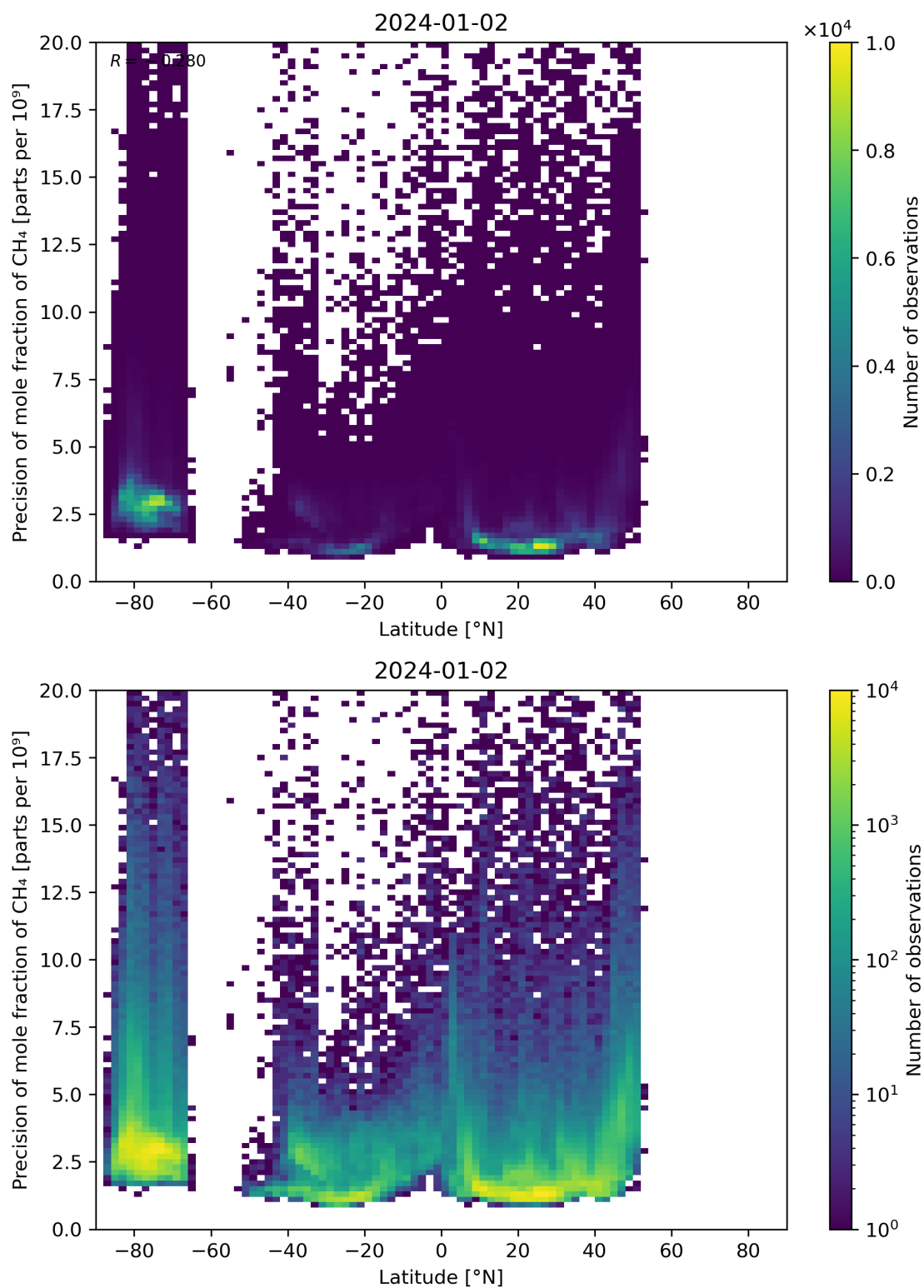
Figure 59: Scatter density plot of “Latitude” against “Precision of mole fraction of CH 4 ” for 2024-01-01 to 2024-01-03.
