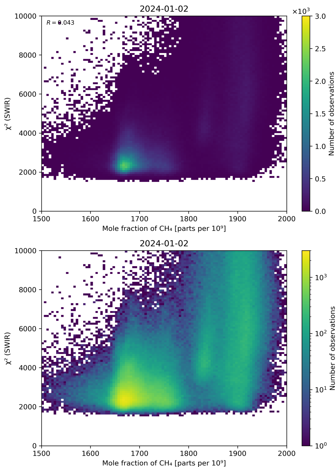
Figure 71: Scatter density plot of “Mole fraction of \text{CH}_4 ” against “ \chi^2 (SWIR)” for 2024-01-01 to 2024-01-03.
