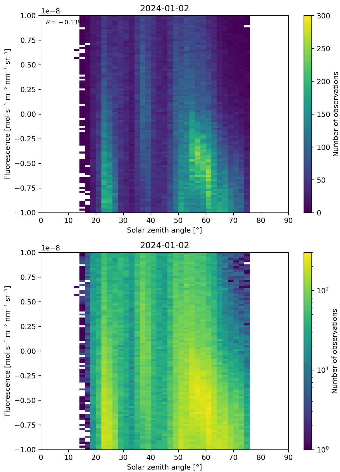
Figure 97: Scatter density plot of “Solar zenith angle” against “Fluorescence” for 2024-01-01 to 2024-01-03.
