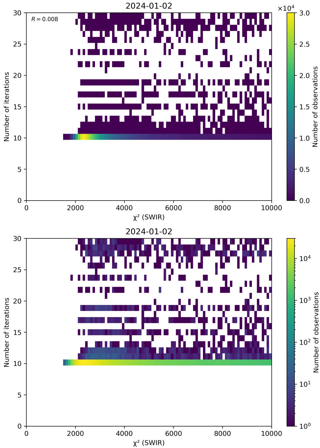
Figure 50: Scatter density plot of “ \chi^2 (SWIR)” against “Number of iterations” for 2024-01-01 to 2024-01-03.
