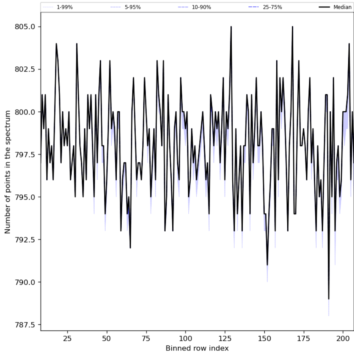
Figure 37: Along track statistics of “Number of points in the spectrum” for 2024-01-01 to 2024-01-03
