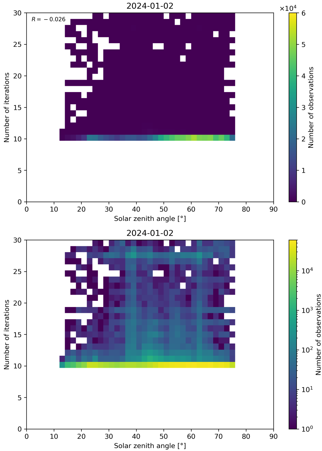
Figure 102: Scatter density plot of “Solar zenith angle” against “Number of iterations” for 2024-01-01 to 2024-01-03.
