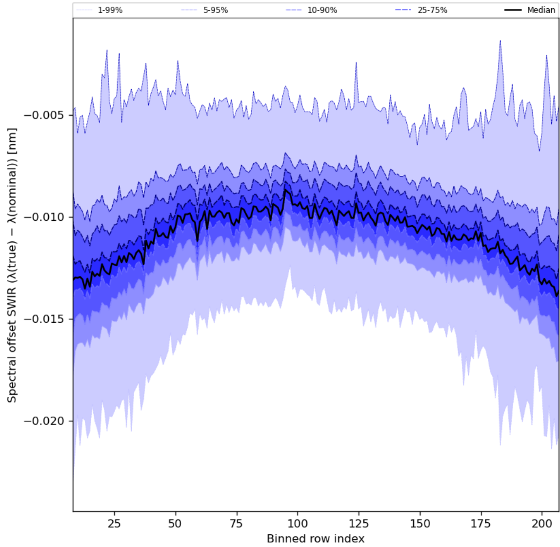
Figure 38: Along track statistics of “Spectral offset SWIR ( \lambda(\text{true}) - \lambda(\text{nominal}) )” for 2024-01-01 to 2024-01-03
