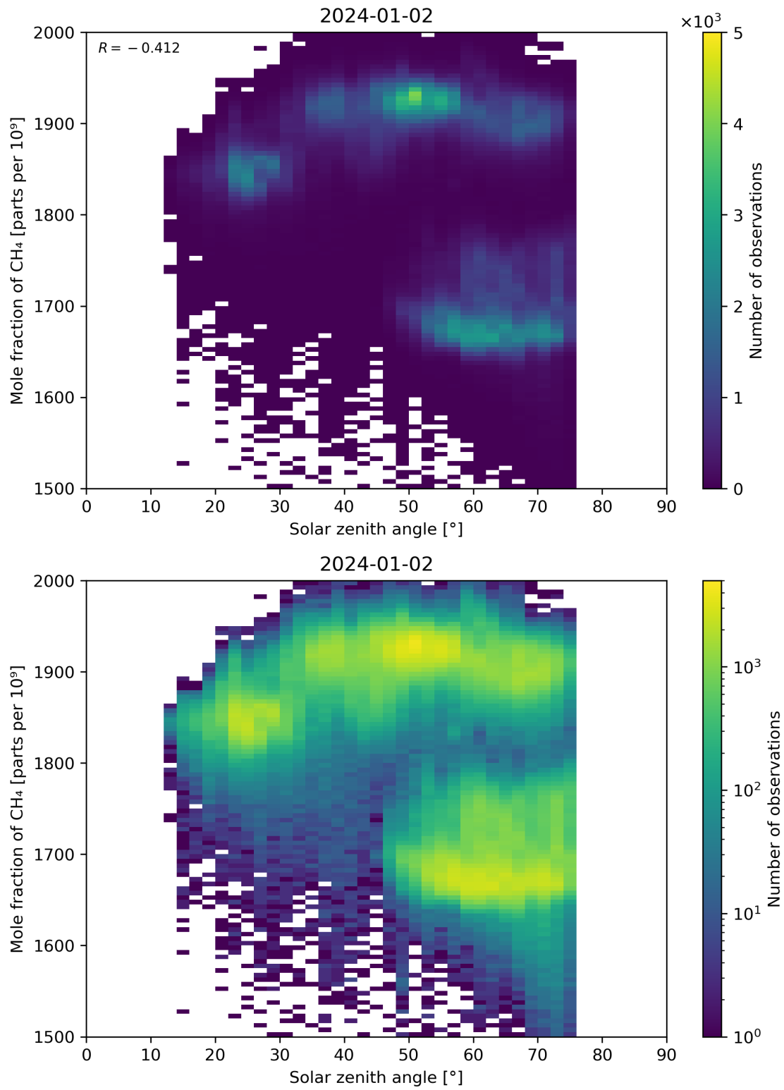
Figure 99: Scatter density plot of “Solar zenith angle” against “Mole fraction of CH 4 ” for 2024-01-01 to 2024-01-03.
