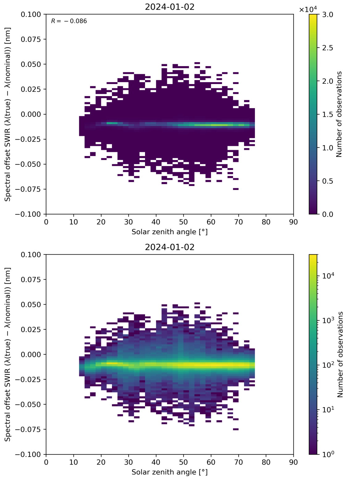
Figure 104: Scatter density plot of “Solar zenith angle” against “Spectral offset SWIR ( \lambda(\text{true}) - \lambda(\text{nominal}) )” for 2024-01-01 to 2024-01-03.
