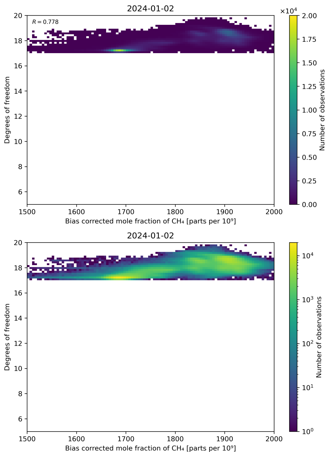
Figure 65: Scatter density plot of “Bias corrected mole fraction of CH 4 ” against “Degrees of freedom” for 2024-01-01 to 2024-01-03.
