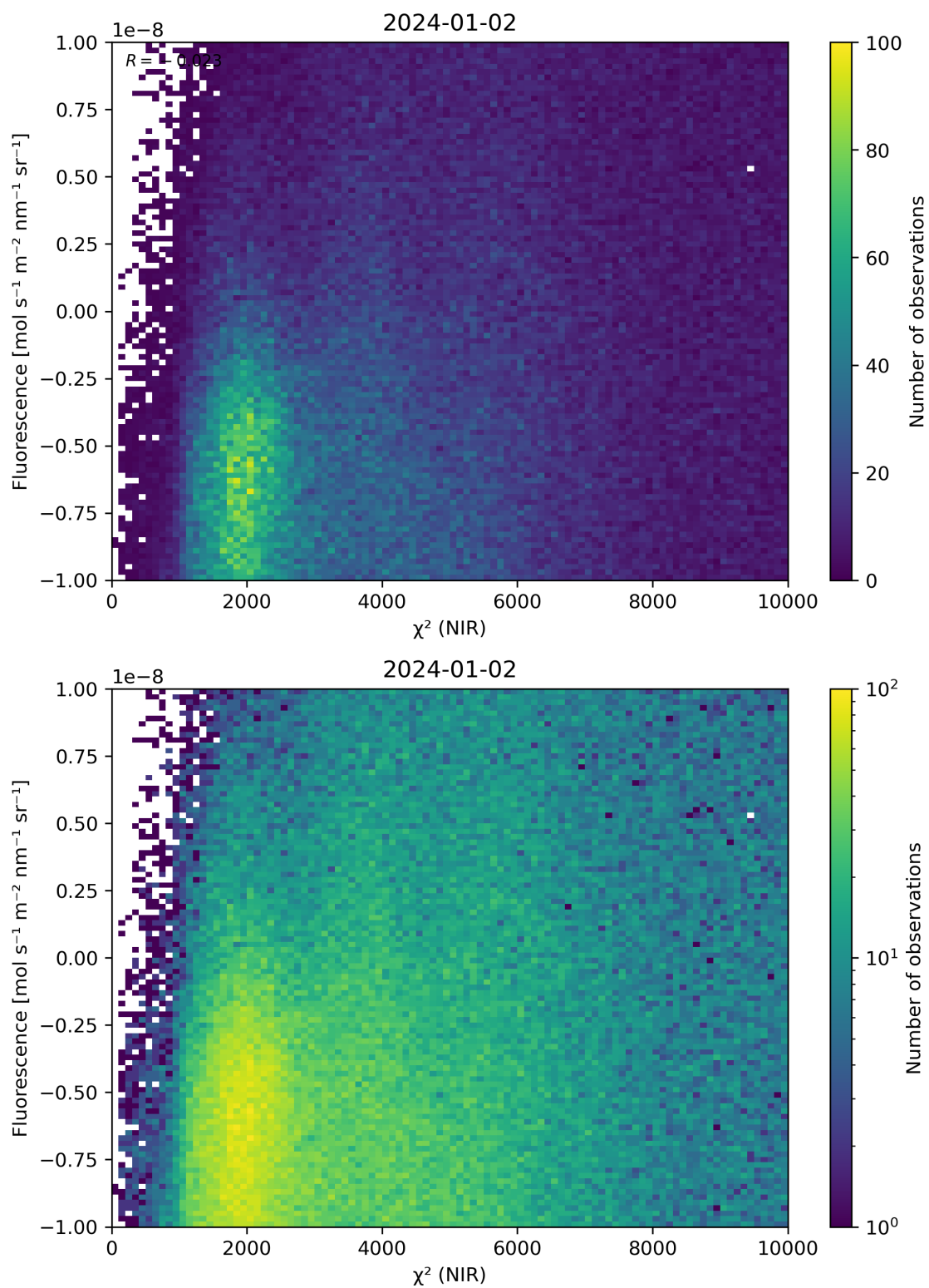
Figure 45: Scatter density plot of “ \chi^2 (NIR)” against “Fluorescence” for 2024-01-01 to 2024-01-03.
