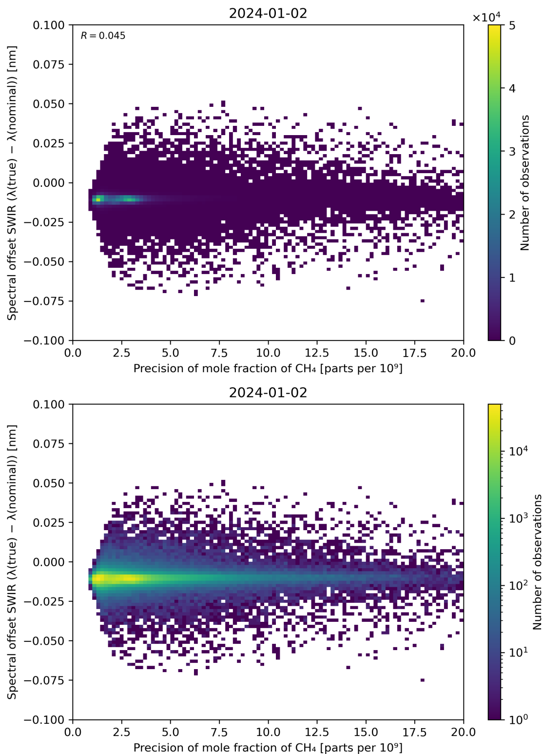
Figure 85: Scatter density plot of “Precision of mole fraction of CH 4 ” against “Spectral offset SWIR ( \lambda(\text{true}) - \lambda(\text{nominal}) )” for 2024-01-01 to 2024-01-03.
