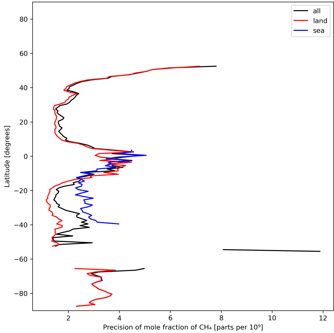
Figure 13: Zonal average of “Precision of mole fraction of CH 4 ” for 2024-01-01 to 2024-01-03.
