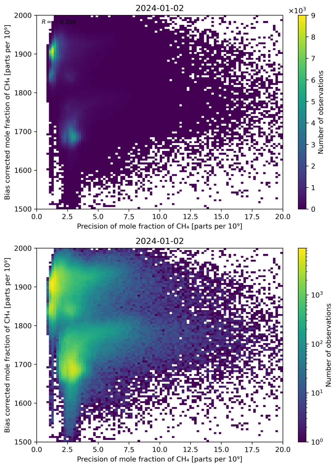
Figure 82: Scatter density plot of “Precision of mole fraction of CH 4 ” against “Bias corrected mole fraction of CH 4 ” for 2024-01-01 to 2024-01-03.
