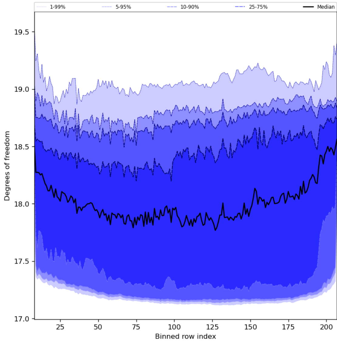
Figure 41: Along track statistics of “Degrees of freedom” for 2024-01-01 to 2024-01-03
