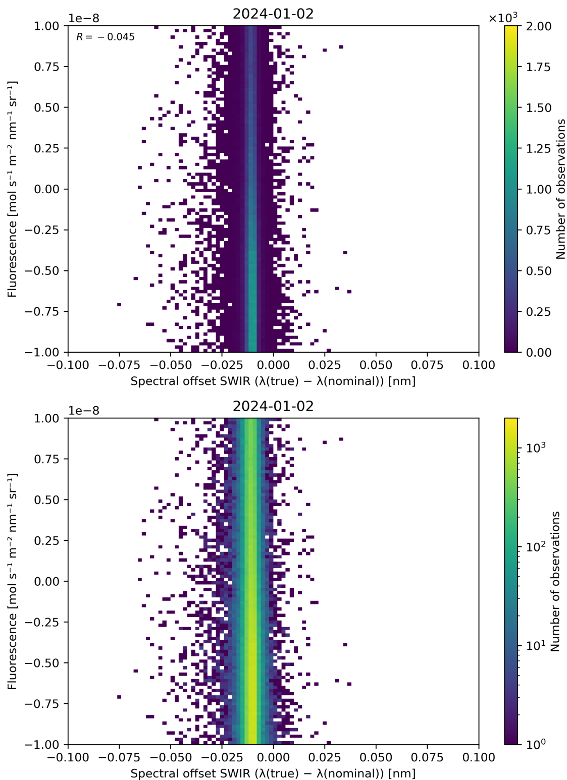
Figure 120: Scatter density plot of “Spectral offset SWIR ( \lambda(\text{true}) - \lambda(\text{nominal}) )” against “Fluorescence” for 2024-01-01 to 2024-01-03.
