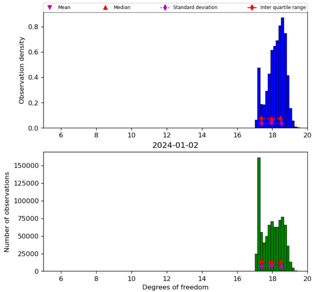
Figure 30: Histogram of “Degrees of freedom” for 2024-01-01 to 2024-01-03
