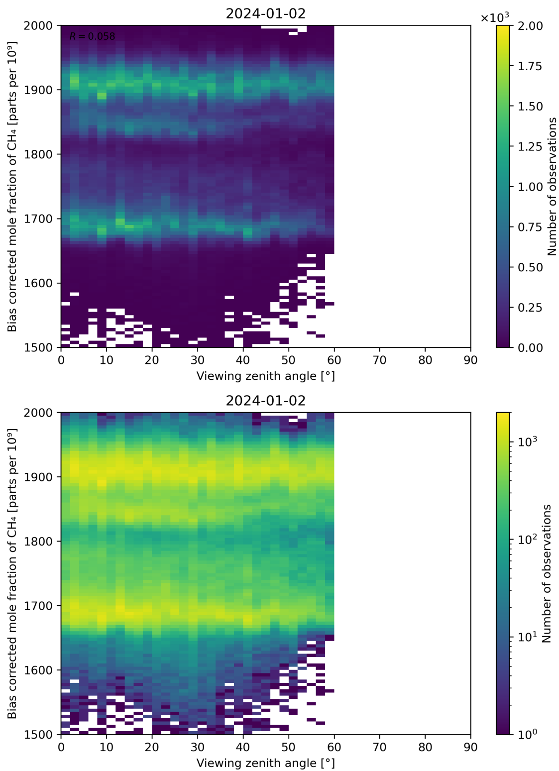
Figure 111: Scatter density plot of “Viewing zenith angle” against “Bias corrected mole fraction of CH 4 ” for 2024-01-01 to 2024-01-03.
