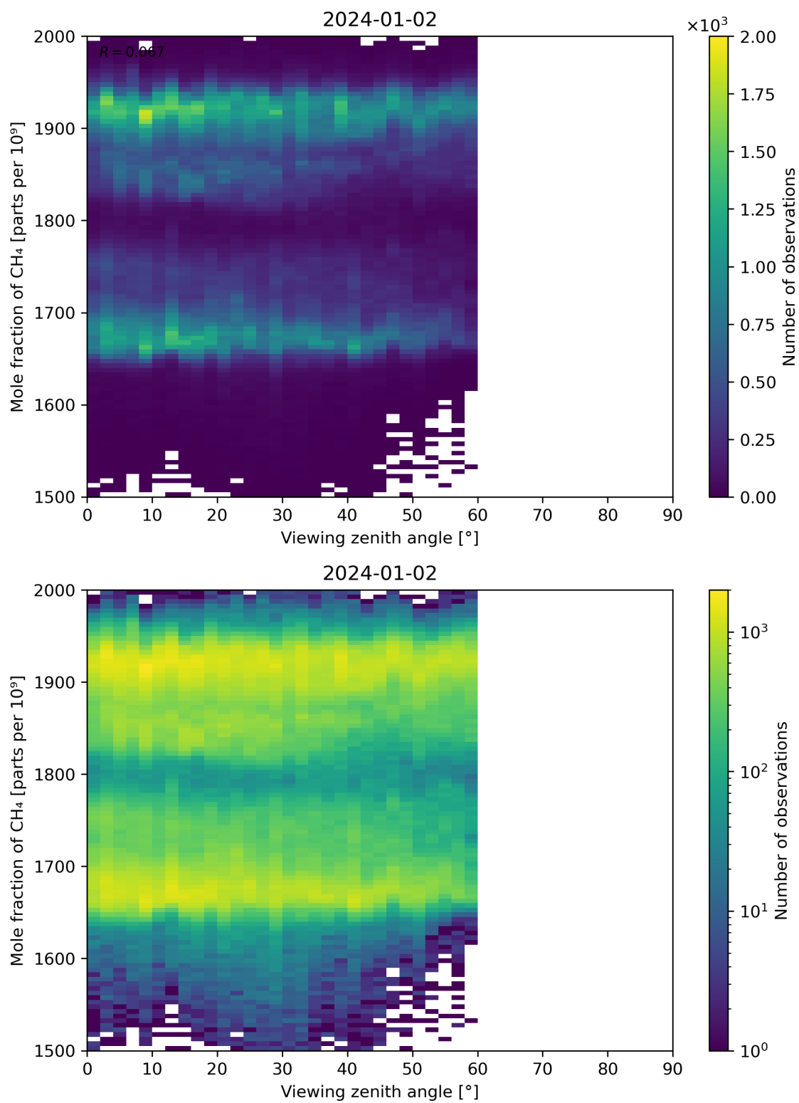
Figure 110: Scatter density plot of “Viewing zenith angle” against “Mole fraction of CH 4 ” for 2024-01-01 to 2024-01-03.
