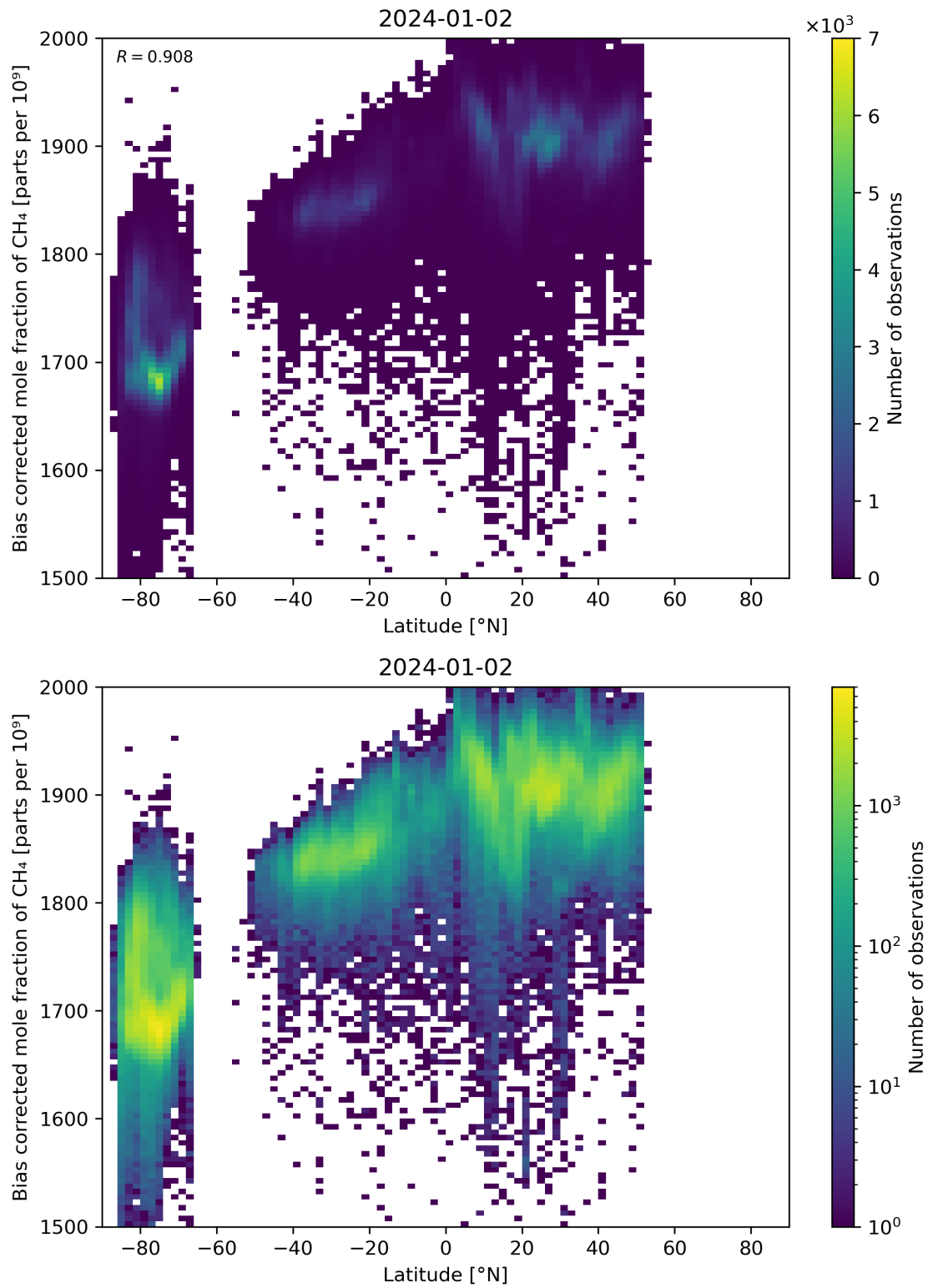
Figure 58: Scatter density plot of “Latitude” against “Bias corrected mole fraction of CH 4 ” for 2024-01-01 to 2024-01-03.
