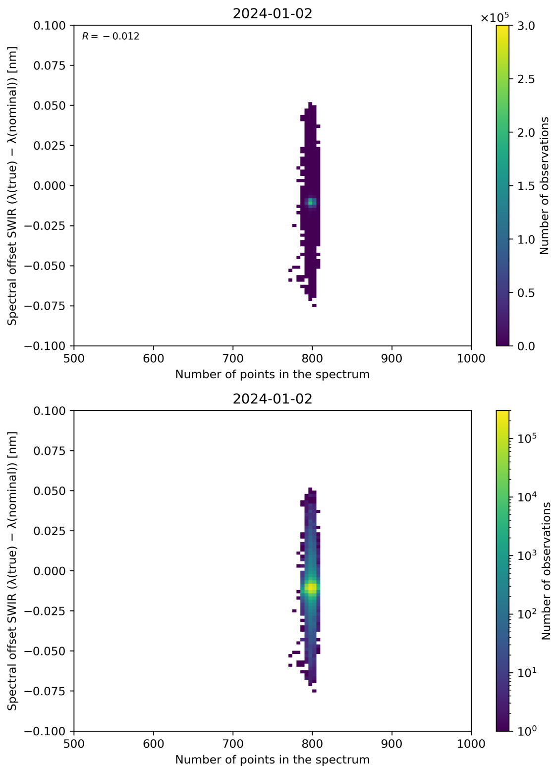
Figure 93: Scatter density plot of “Number of points in the spectrum” against “Spectral offset SWIR ( \lambda(\text{true}) - \lambda(\text{nominal}) )” for 2024-01-01 to 2024-01-03.
