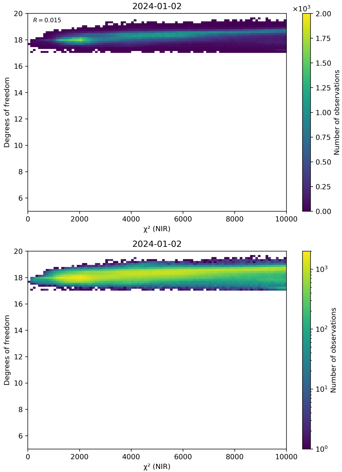
Figure 44: Scatter density plot of “ \chi^2 (NIR)” against “Degrees of freedom” for 2024-01-01 to 2024-01-03.
