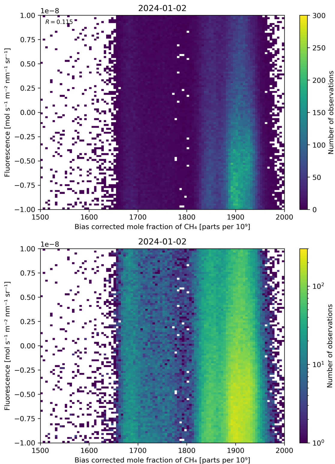
Figure 66: Scatter density plot of “Bias corrected mole fraction of \text{CH}_4 ” against “Fluorescence” for 2024-01-01 to 2024-01-03.
