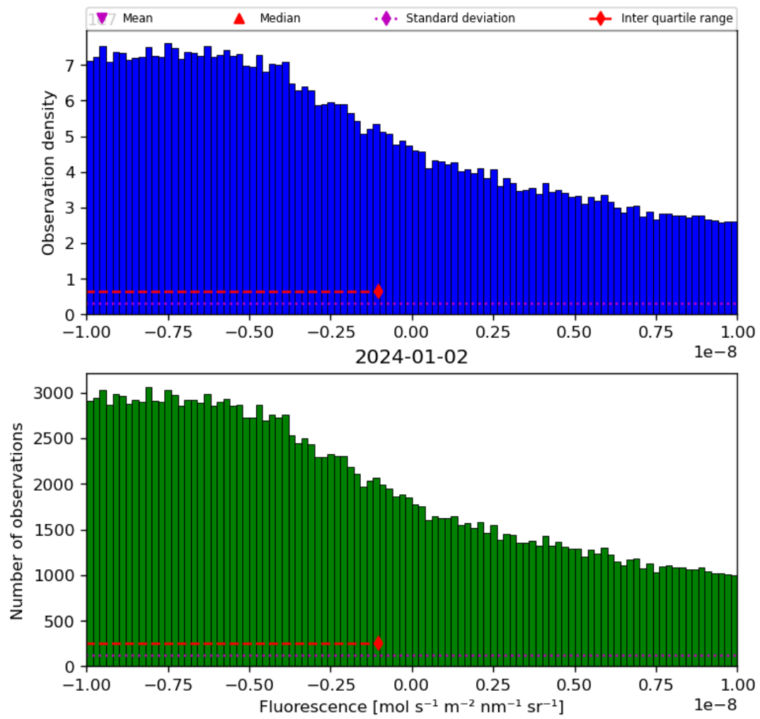
Figure 32: Histogram of “Fluorescence” for 2024-01-01 to 2024-01-03
