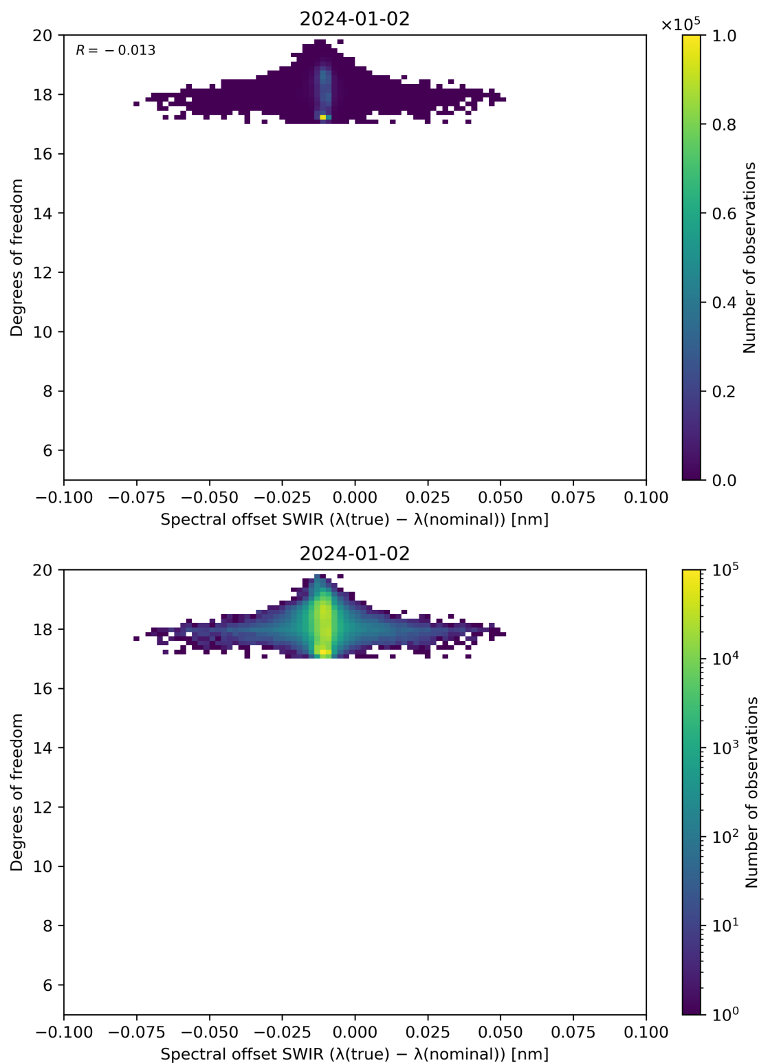
Figure 119: Scatter density plot of “Spectral offset SWIR ( \lambda(\text{true}) - \lambda(\text{nominal}) )” against “Degrees of freedom” for 2024-01-01 to 2024-01-03.
