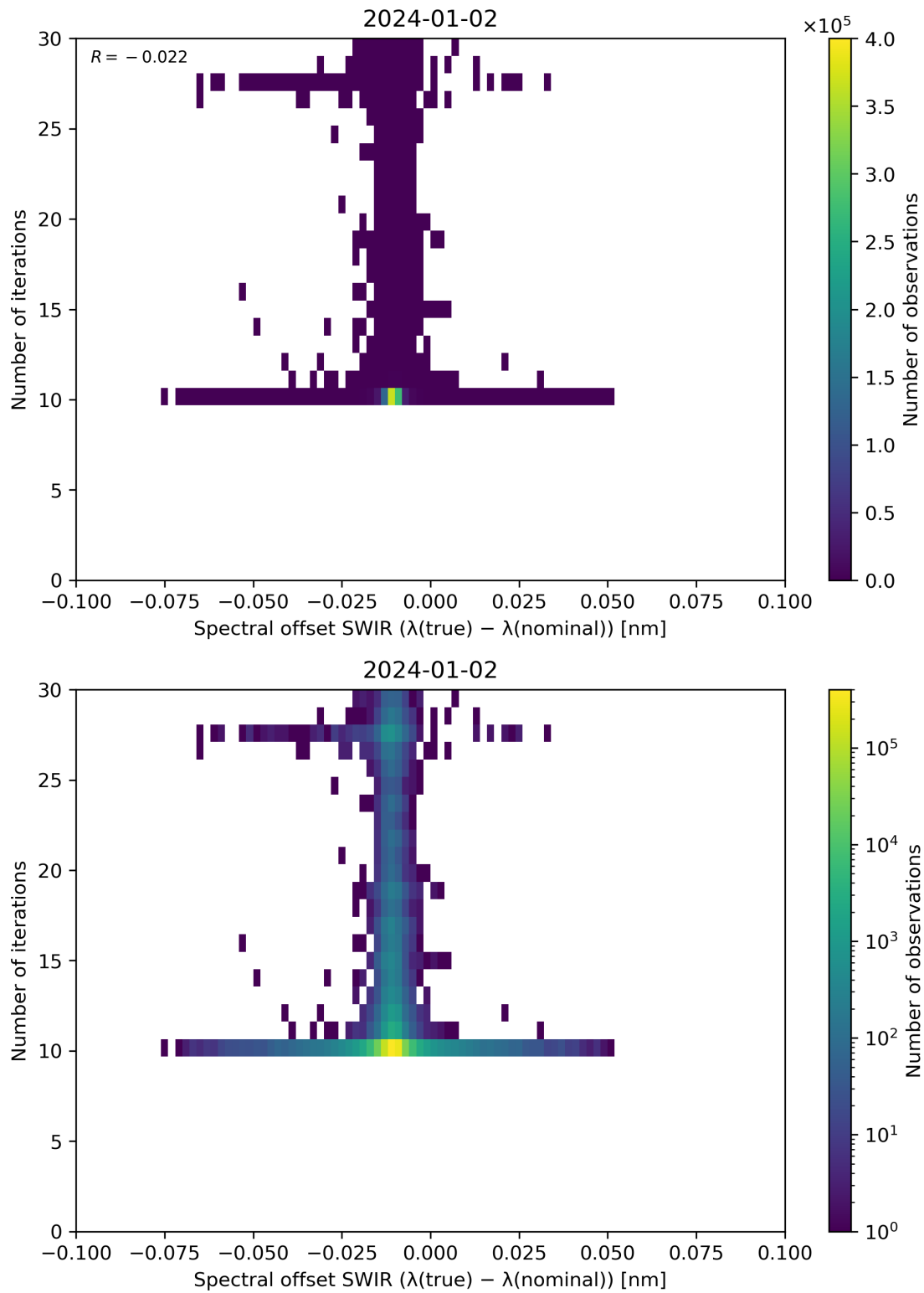
Figure 121: Scatter density plot of “Spectral offset SWIR ( \lambda(\text{true}) - \lambda(\text{nominal}) )” against “Number of iterations” for 2024-01-01 to 2024-01-03.
