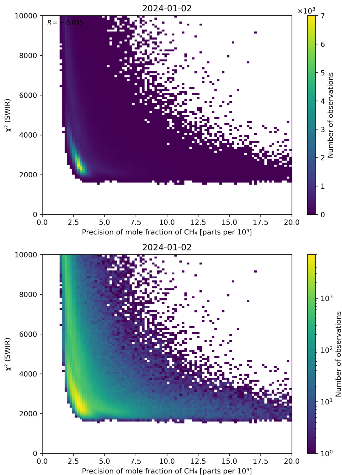
Figure 79: Scatter density plot of “Precision of mole fraction of CH 4 ” against “ \chi^2 (SWIR)” for 2024-01-01 to 2024-01-03.
