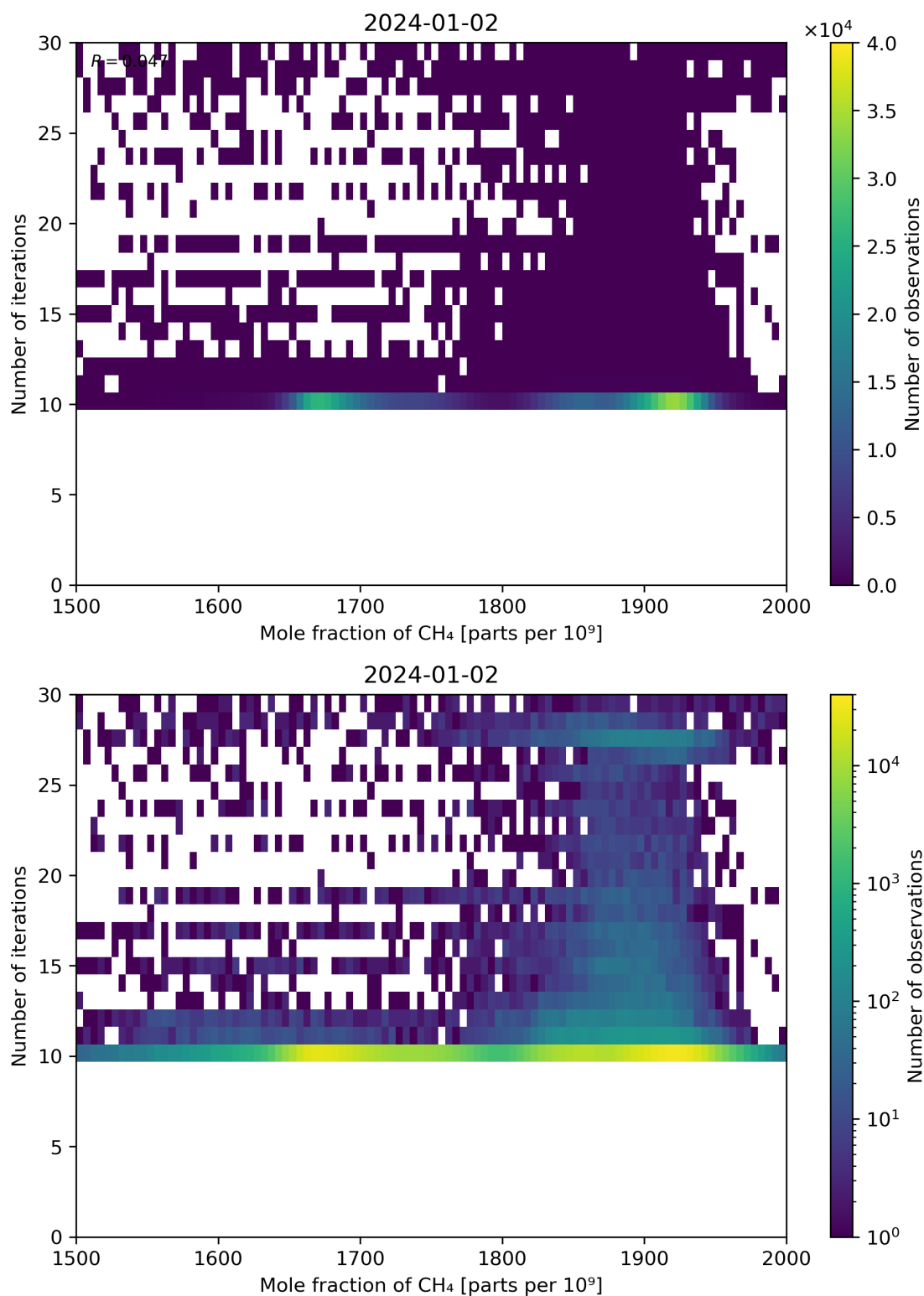
Figure 76: Scatter density plot of “Mole fraction of CH 4 ” against “Number of iterations” for 2024-01-01 to 2024-01-03.
