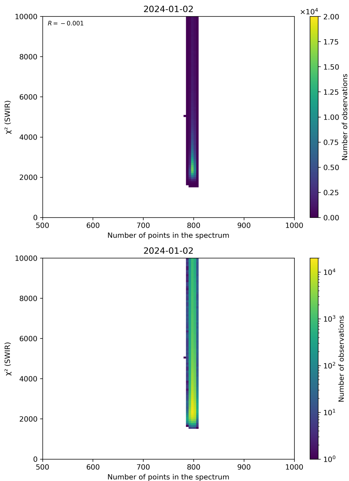
Figure 89: Scatter density plot of “Number of points in the spectrum” against “ \chi^2 (SWIR)” for 2024-01-01 to 2024-01-03.
