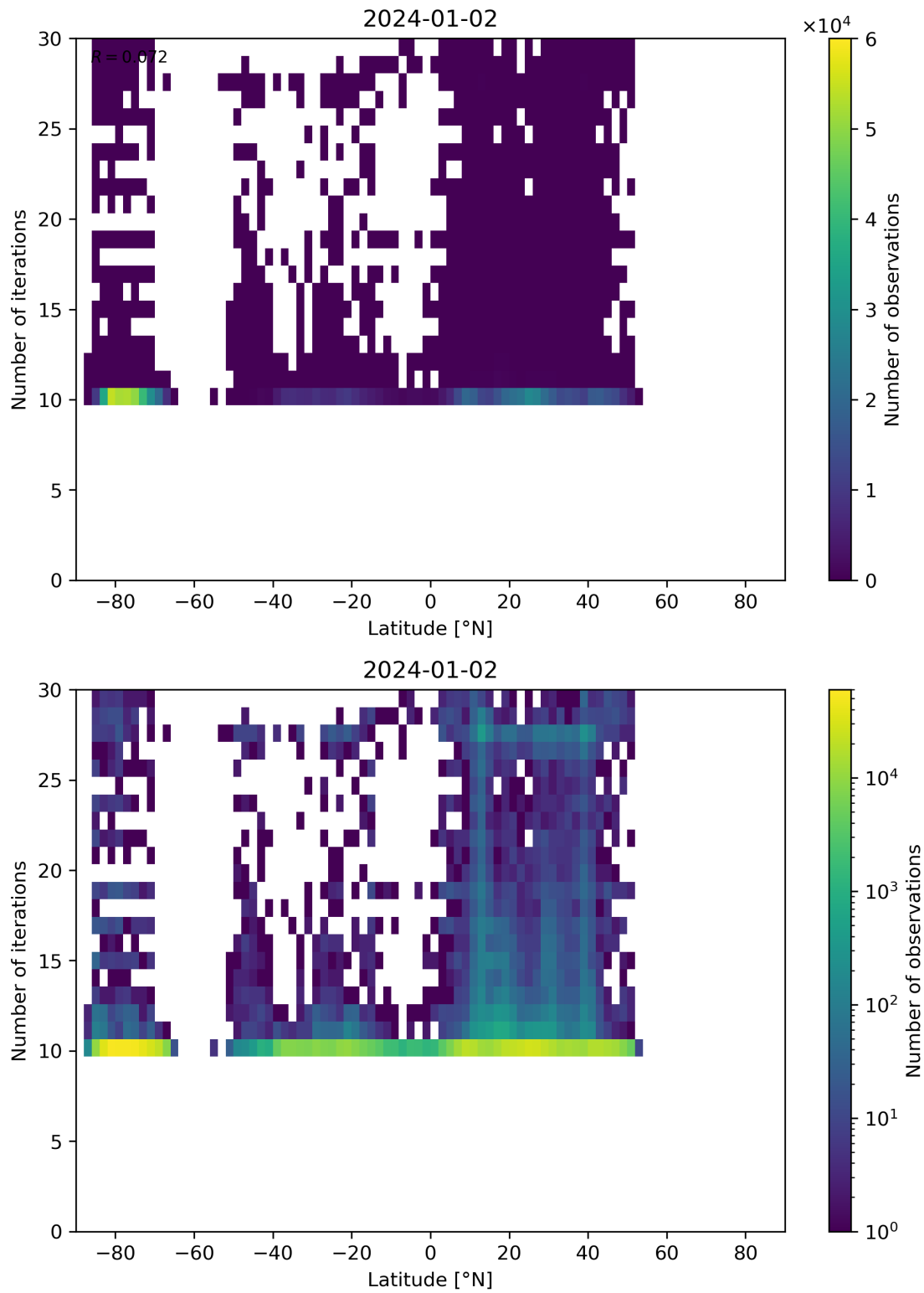
Figure 60: Scatter density plot of “Latitude” against “Number of iterations” for 2024-01-01 to 2024-01-03.
