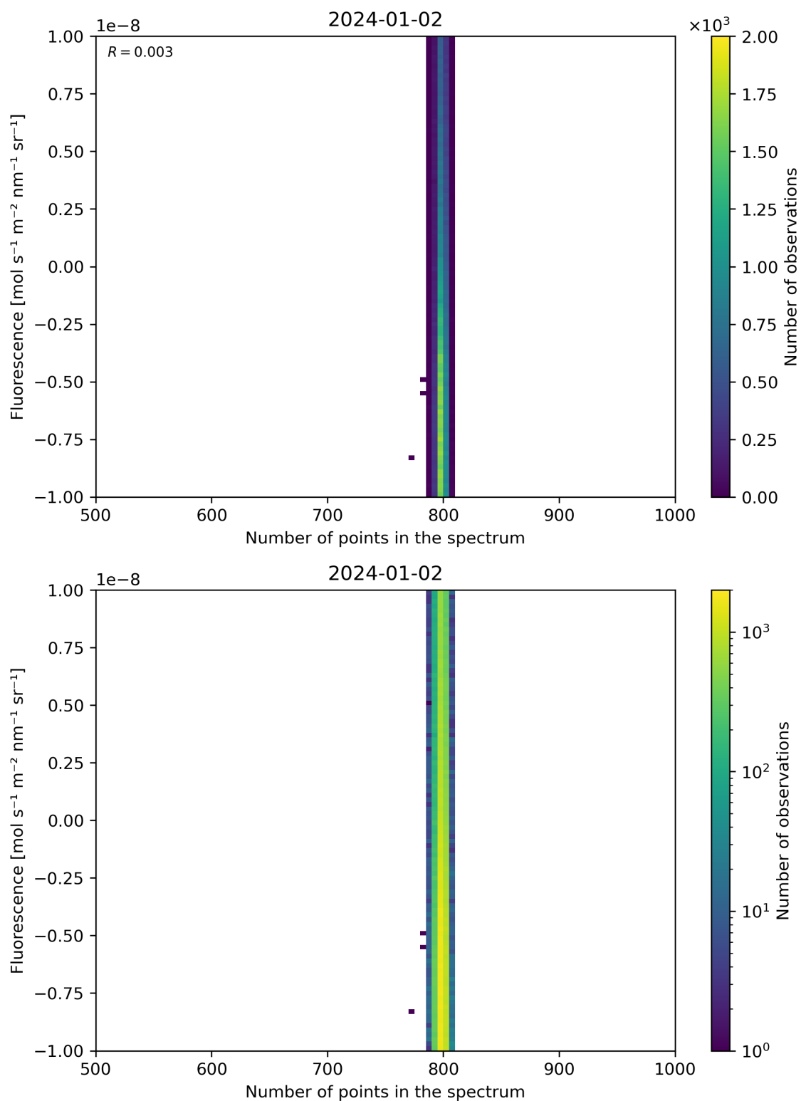
Figure 91: Scatter density plot of “Number of points in the spectrum” against “Fluorescence” for 2024-01-01 to 2024-01-03.
