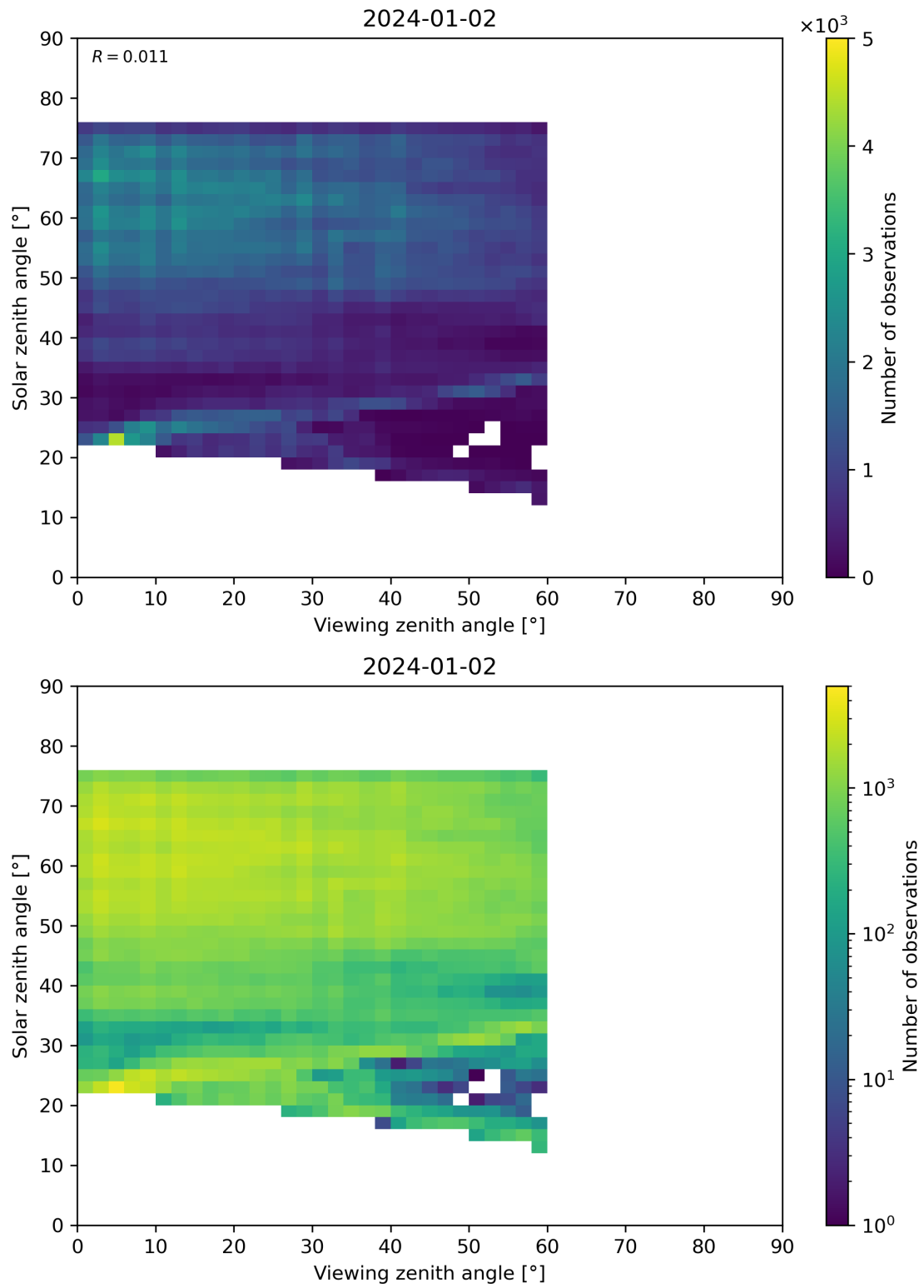
Figure 115: Scatter density plot of “Viewing zenith angle” against “Solar zenith angle” for 2024-01-01 to 2024-01-03.
