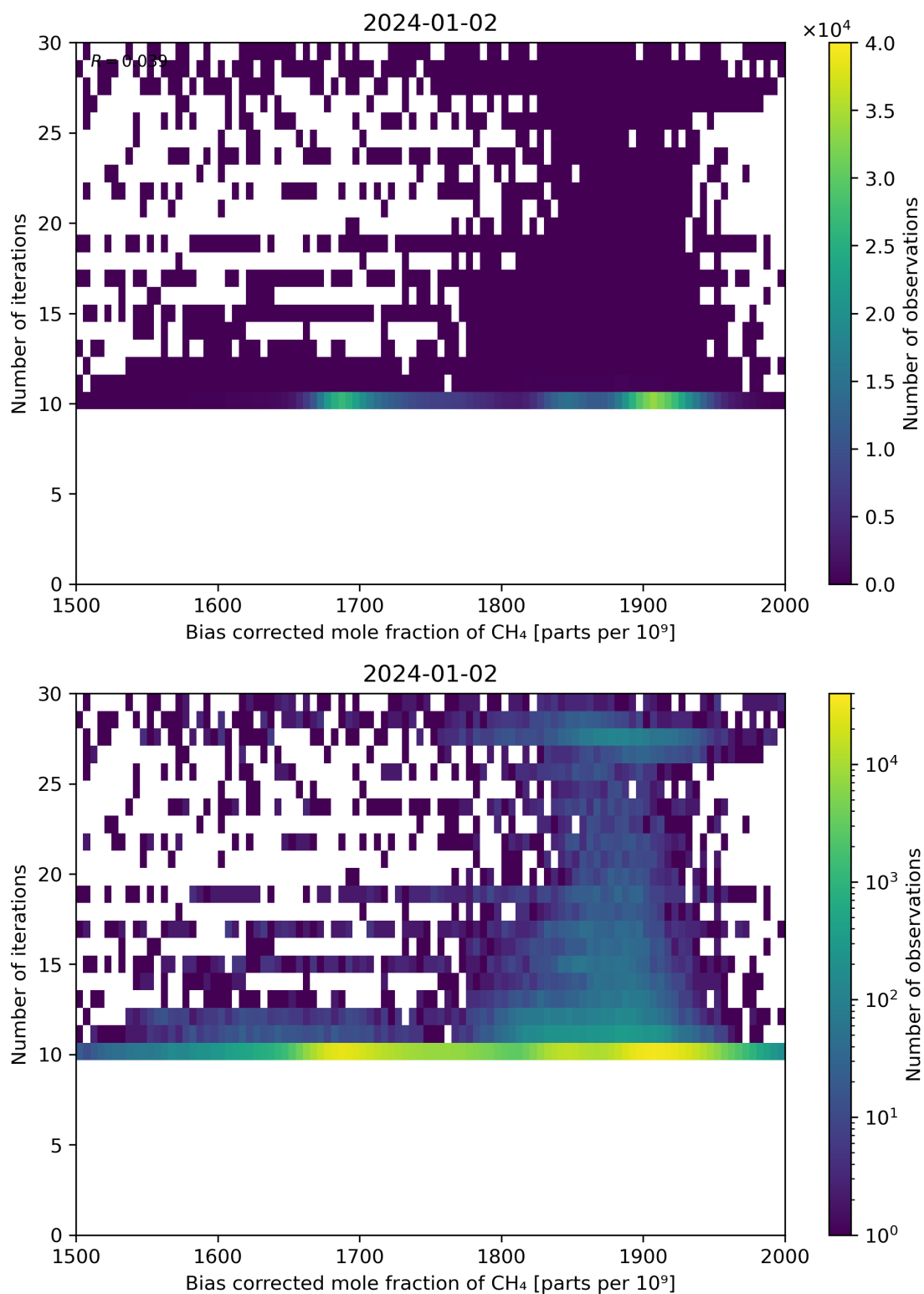
Figure 67: Scatter density plot of “Bias corrected mole fraction of CH 4 ” against “Number of iterations” for 2024-01-01 to 2024-01-03.
