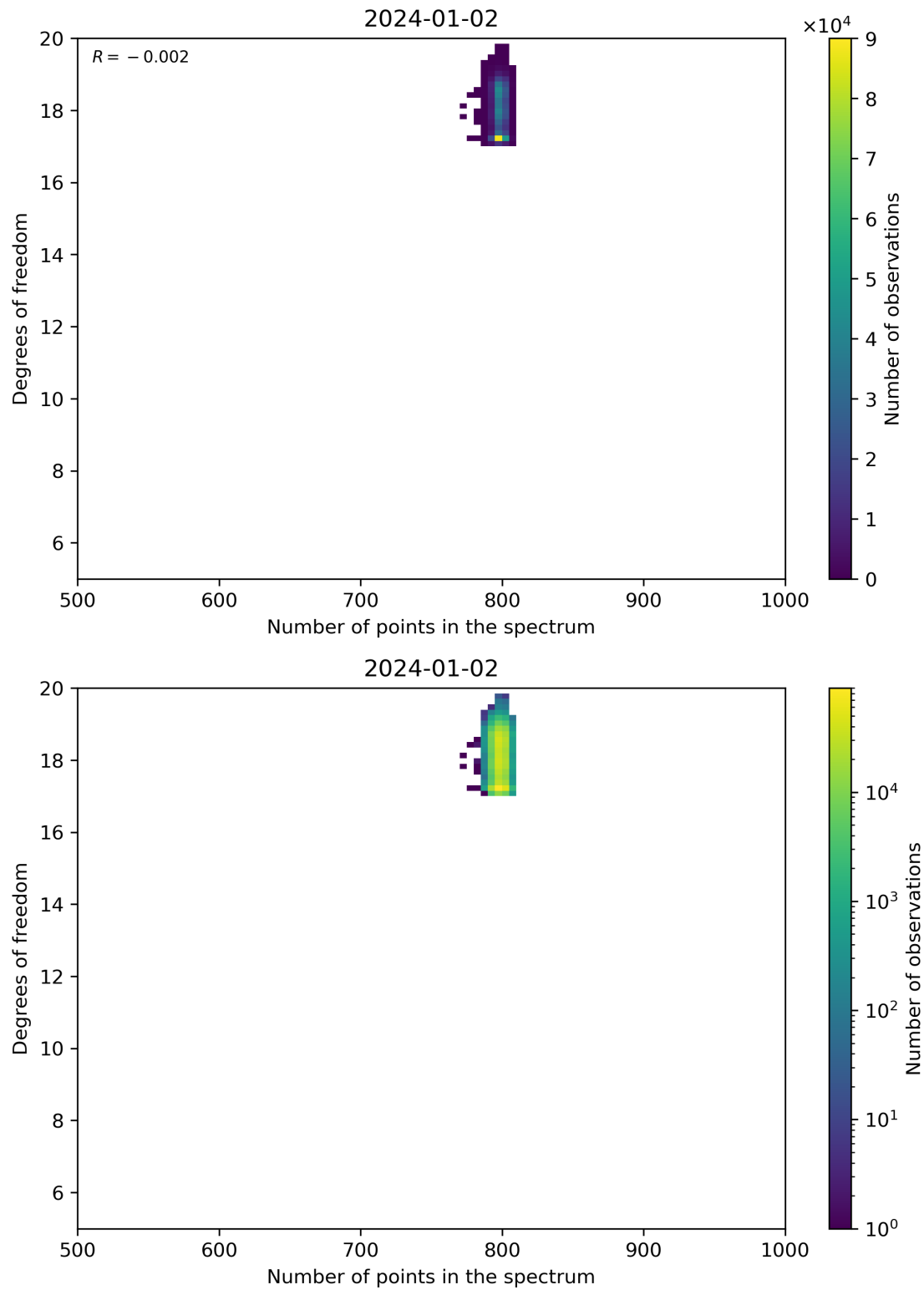
Figure 90: Scatter density plot of “Number of points in the spectrum” against “Degrees of freedom” for 2024-01-01 to 2024-01-03.
