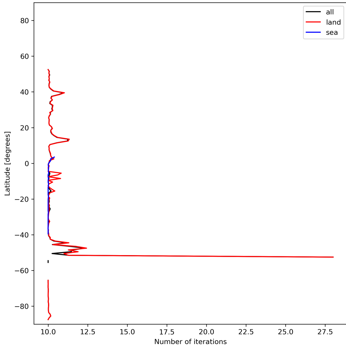
Figure 20: Zonal average of “Number of iterations” for 2024-01-01 to 2024-01-03.
