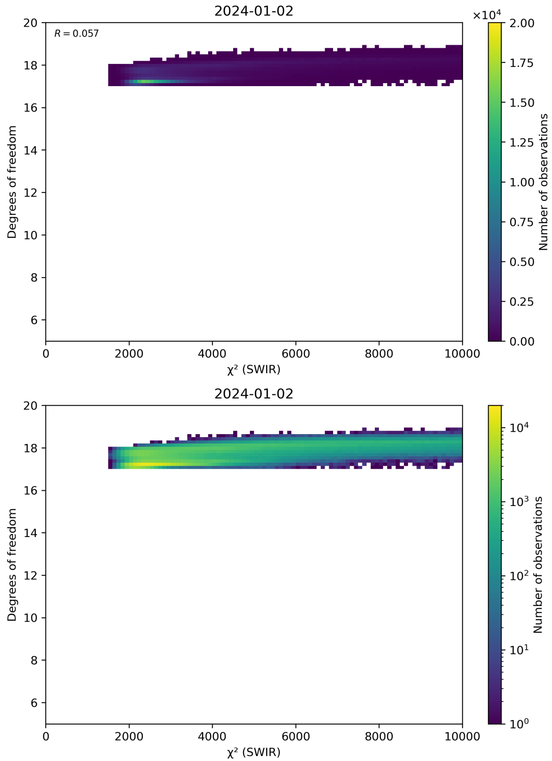
Figure 48: Scatter density plot of “ \chi^2 (SWIR)” against “Degrees of freedom” for 2024-01-01 to 2024-01-03.
