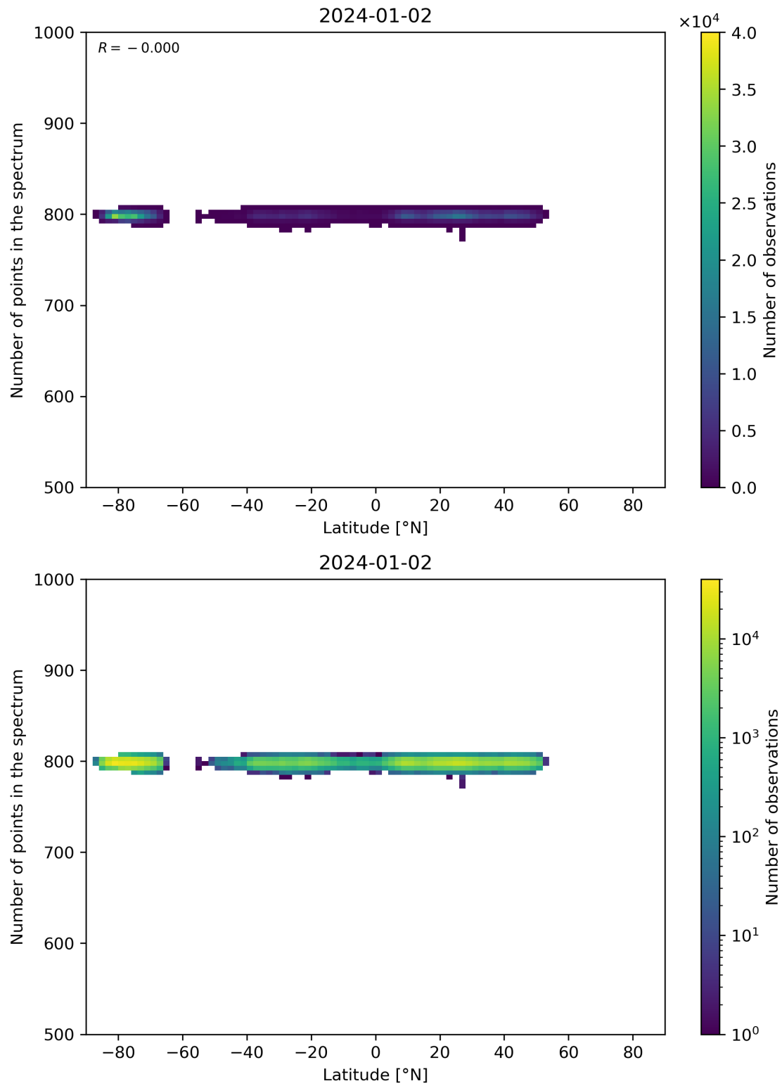
Figure 61: Scatter density plot of “Latitude” against “Number of points in the spectrum” for 2024-01-01 to 2024-01-03.
