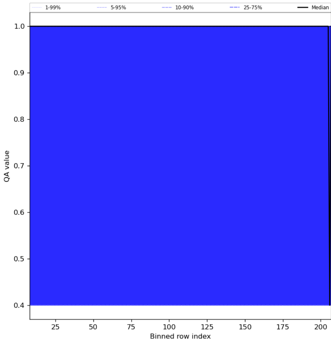
Figure 33: Along track statistics of “QA value” for 2024-01-01 to 2024-01-03
