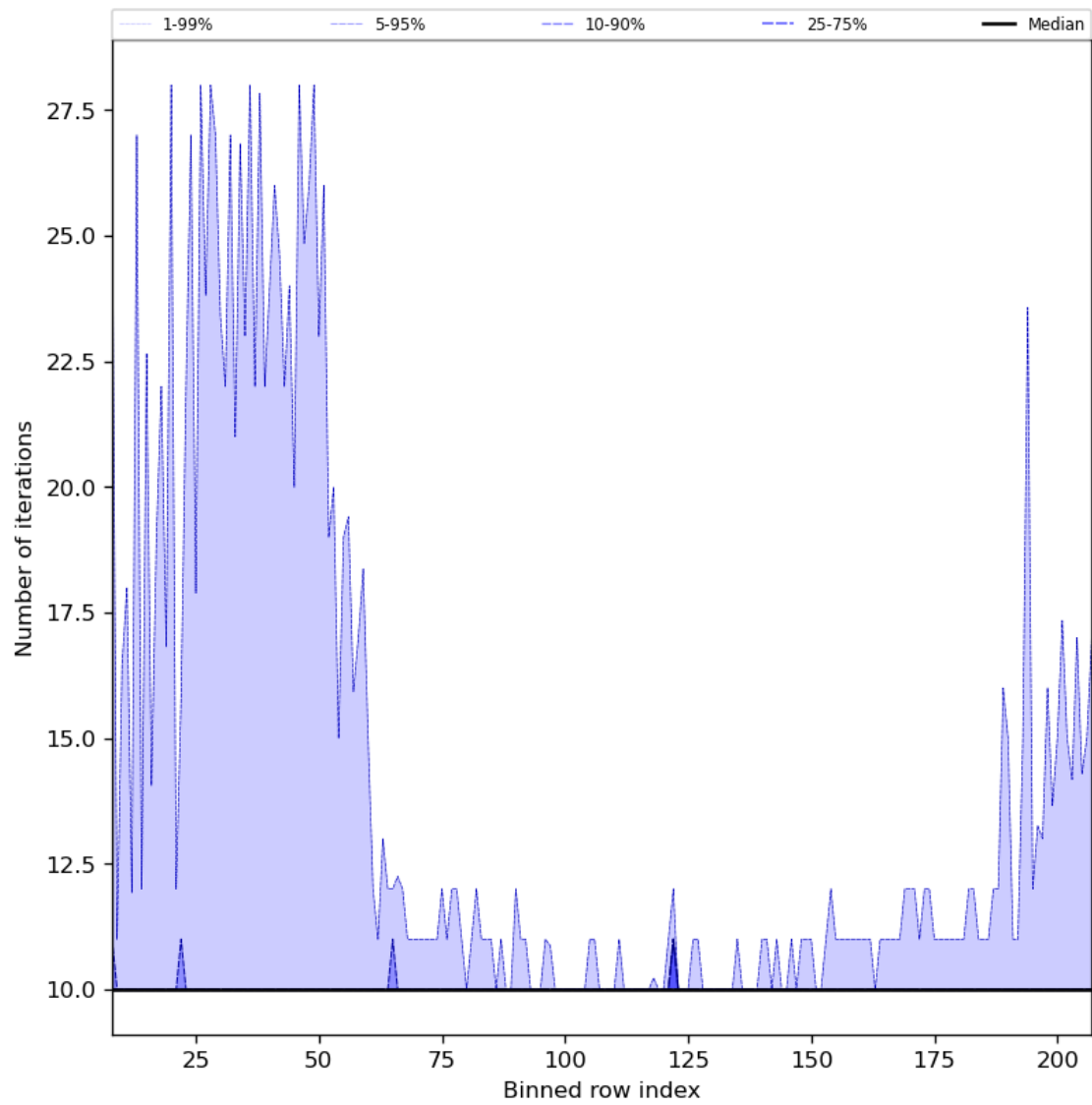
Figure 42: Along track statistics of “Number of iterations” for 2024-01-01 to 2024-01-03
