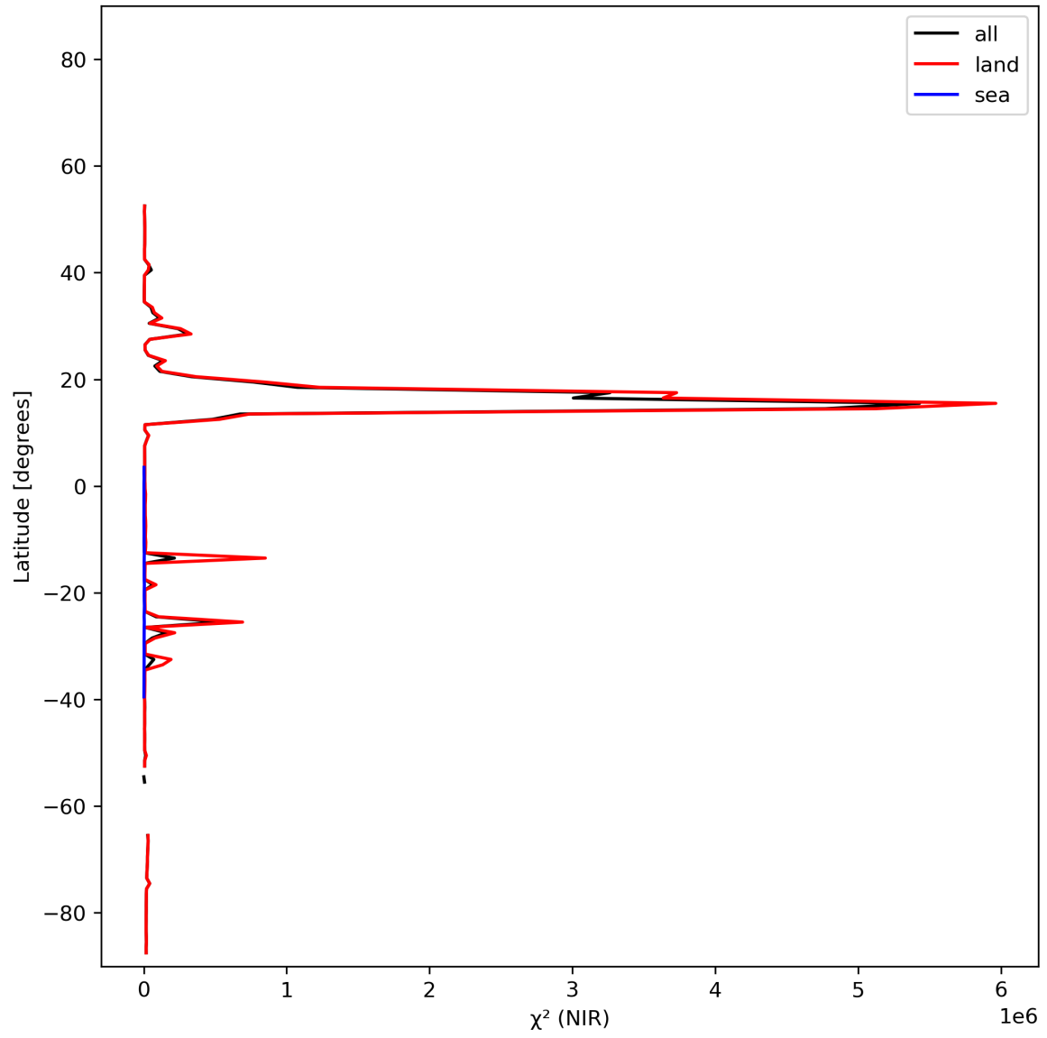
Figure 18: Zonal average of “ \chi^2 (NIR)” for 2024-01-01 to 2024-01-03.
