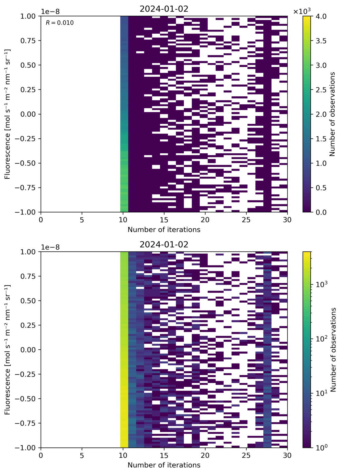
Figure 87: Scatter density plot of “Number of iterations” against “Fluorescence” for 2024-01-01 to 2024-01-03.
