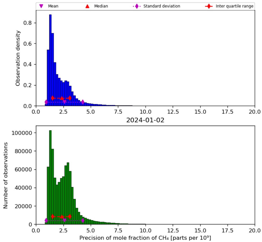
Figure 24: Histogram of “Precision of mole fraction of CH 4 ” for 2024-01-01 to 2024-01-03
