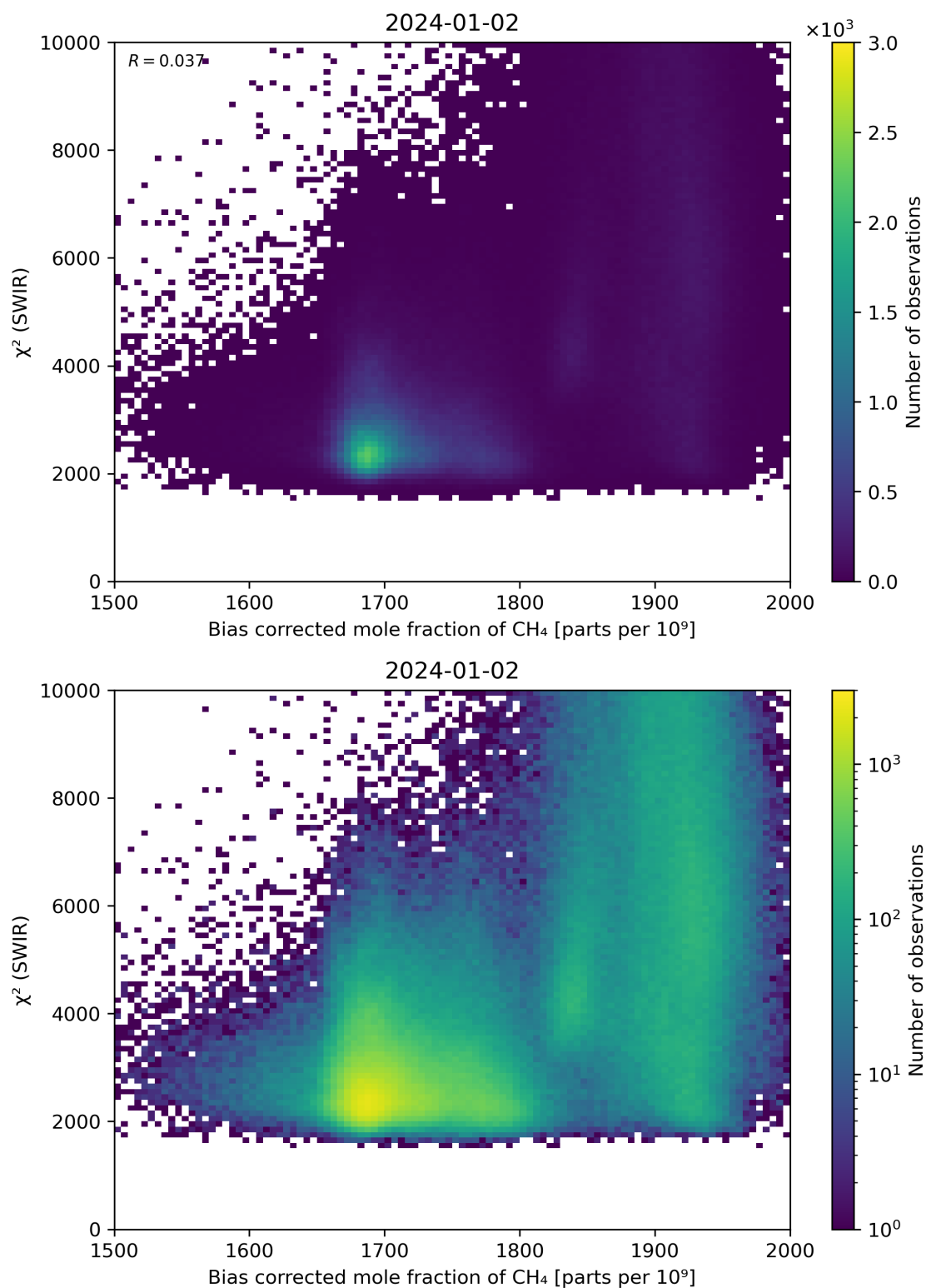
Figure 64: Scatter density plot of “Bias corrected mole fraction of \text{CH}_4 ” against “ \chi^2 (SWIR)” for 2024-01-01 to 2024-01-03.
