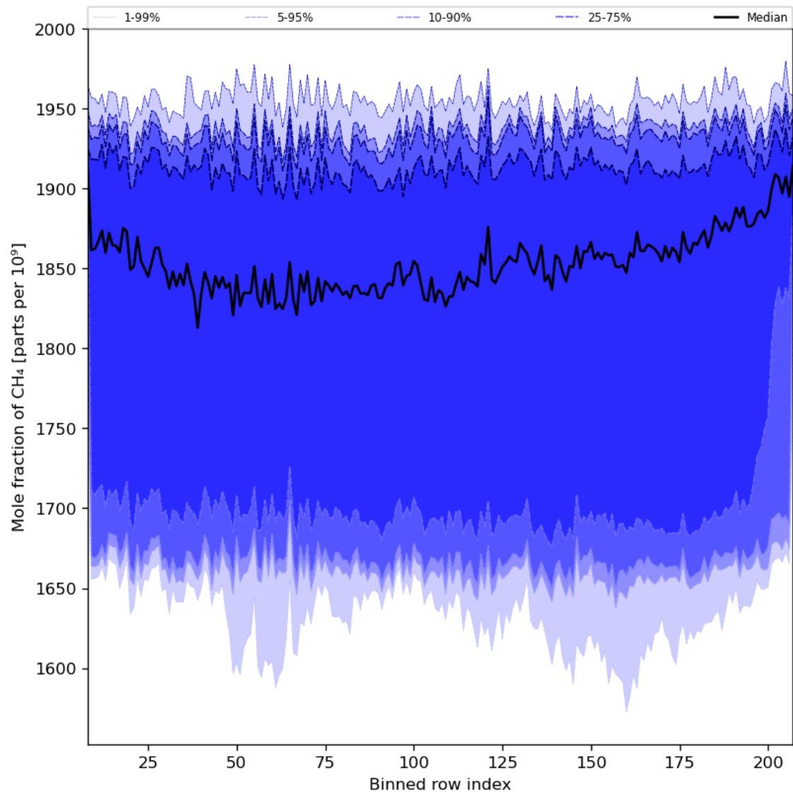
Figure 34: Along track statistics of “Mole fraction of CH 4 ” for 2024-01-01 to 2024-01-03
