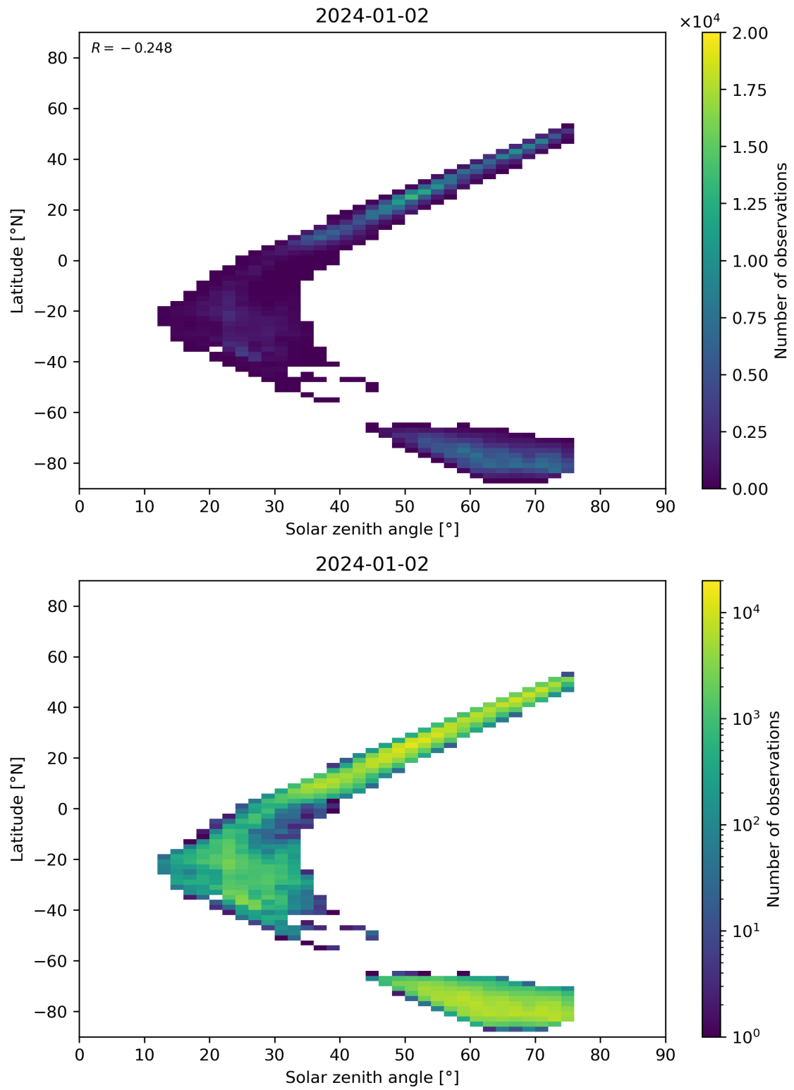
Figure 98: Scatter density plot of “Solar zenith angle” against “Latitude” for 2024-01-01 to 2024-01-03.
