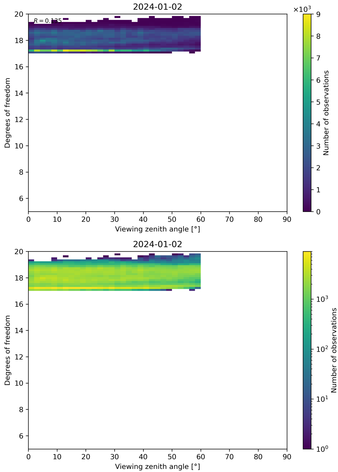
Figure 107: Scatter density plot of “Viewing zenith angle” against “Degrees of freedom” for 2024-01-01 to 2024-01-03.
