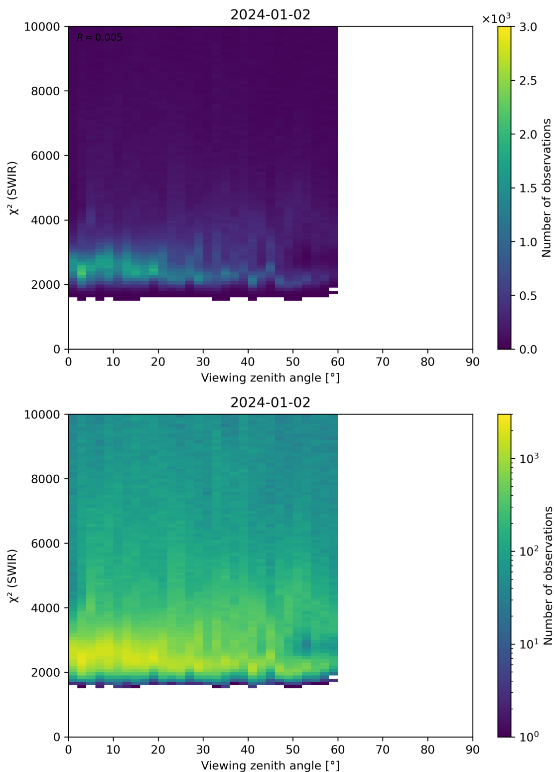
Figure 106: Scatter density plot of “Viewing zenith angle” against “ \chi^2 (SWIR)” for 2024-01-01 to 2024-01-03.
