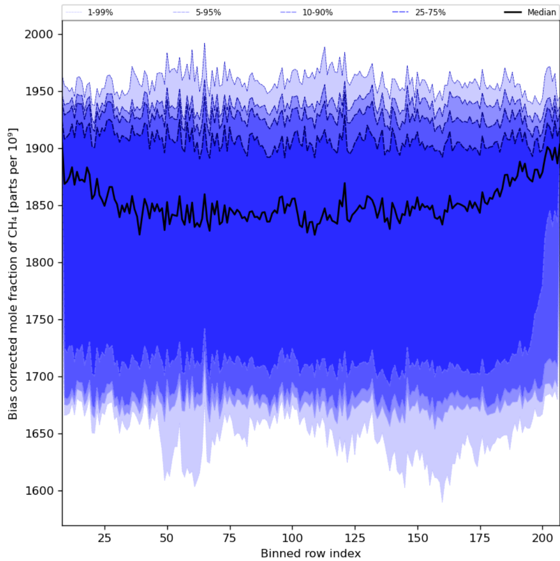
Figure 36: Along track statistics of “Bias corrected mole fraction of CH 4 ” for 2024-01-01 to 2024-01-03
