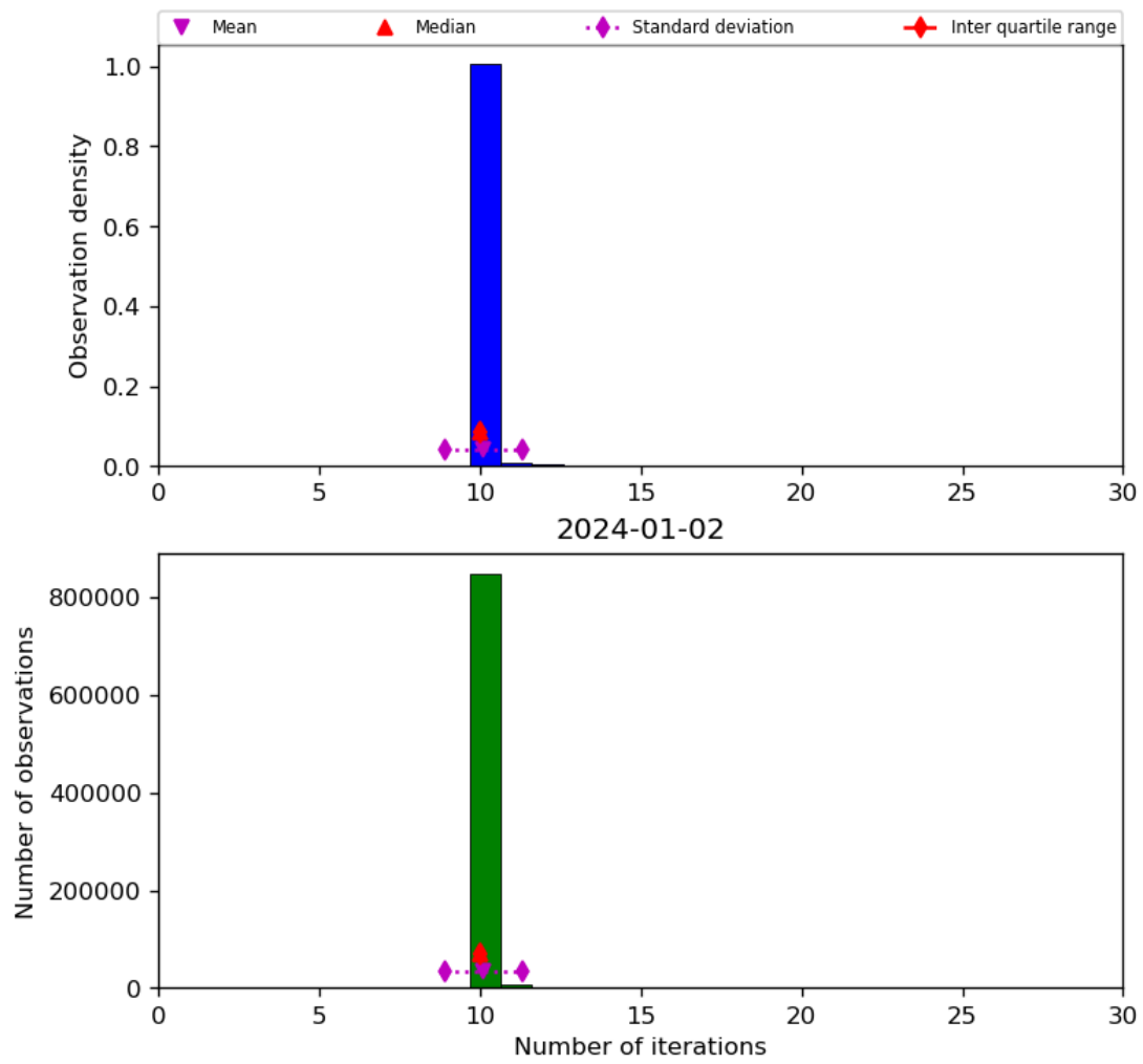
Figure 31: Histogram of “Number of iterations” for 2024-01-01 to 2024-01-03
