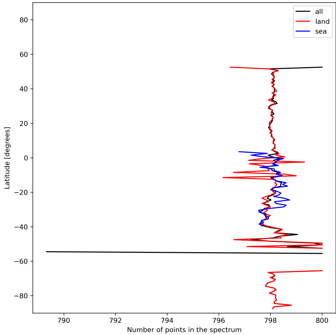
Figure 15: Zonal average of “Number of points in the spectrum” for 2024-01-01 to 2024-01-03.
