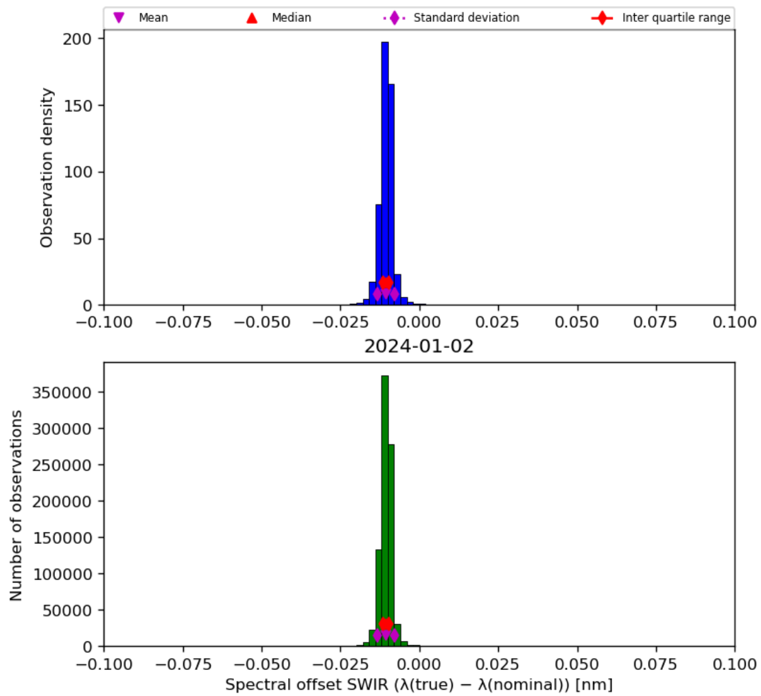
Figure 27: Histogram of “Spectral offset SWIR ( \lambda(\text{true}) - \lambda(\text{nominal}) )” for 2024-01-01 to 2024-01-03
