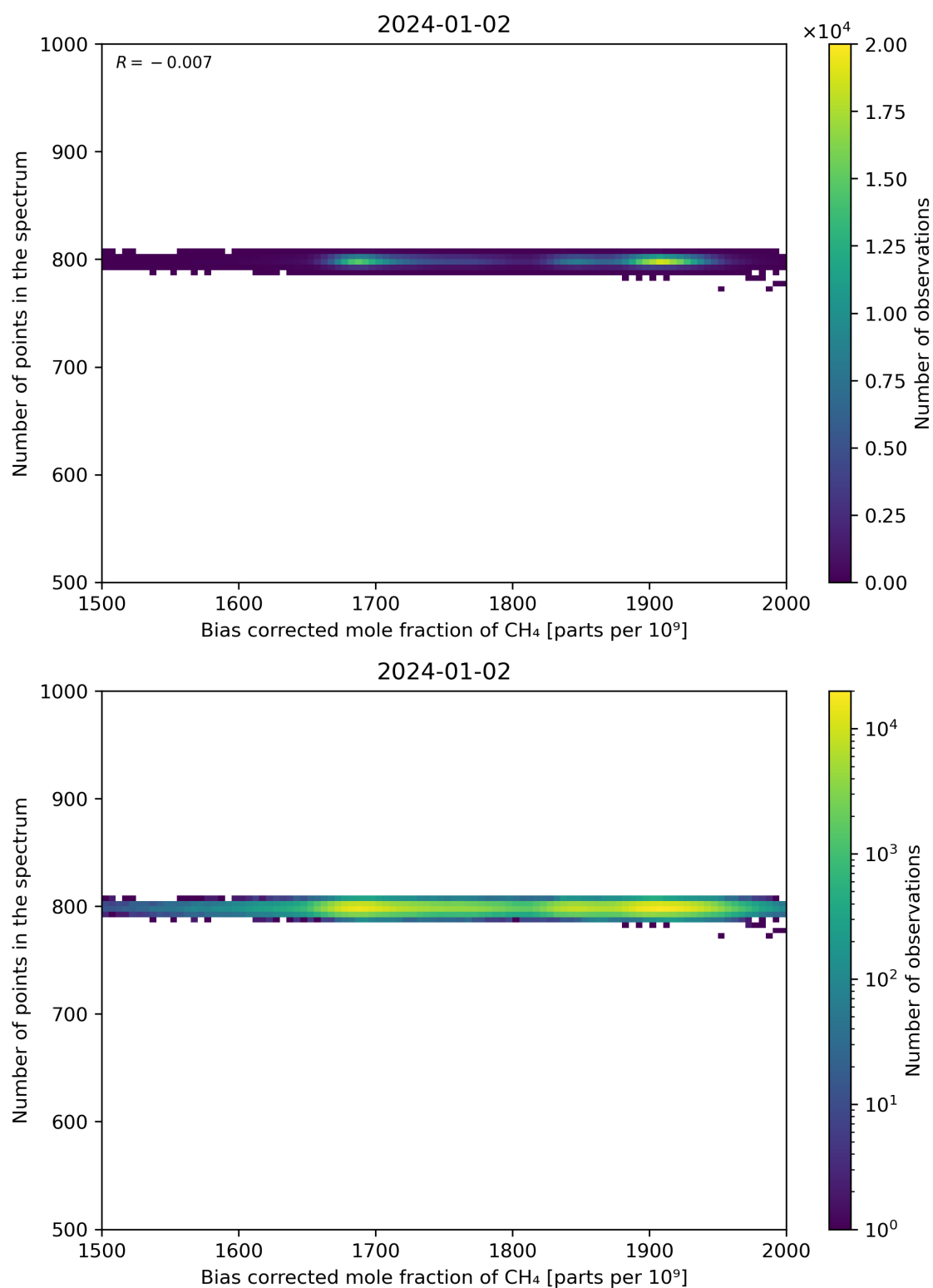
Figure 68: Scatter density plot of “Bias corrected mole fraction of CH 4 ” against “Number of points in the spectrum” for 2024-01-01 to 2024-01-03.
