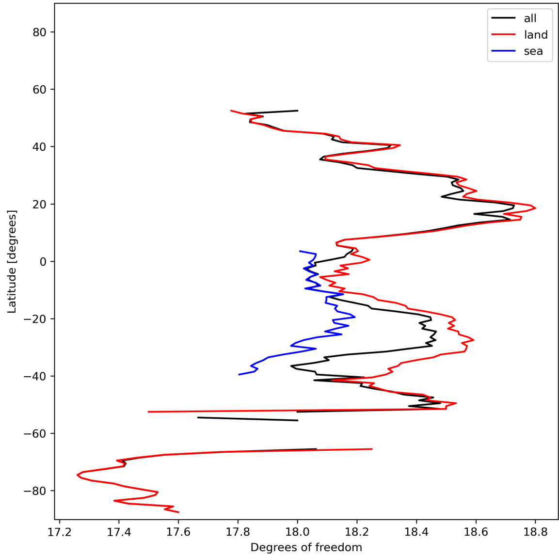
Figure 19: Zonal average of “Degrees of freedom” for 2024-01-01 to 2024-01-03.
