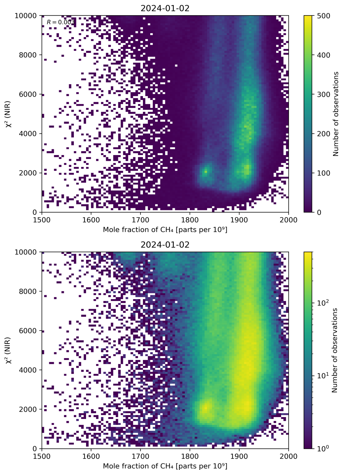
Figure 70: Scatter density plot of “Mole fraction of \text{CH}_4 ” against “ \chi^2 (NIR)” for 2024-01-01 to 2024-01-03.
