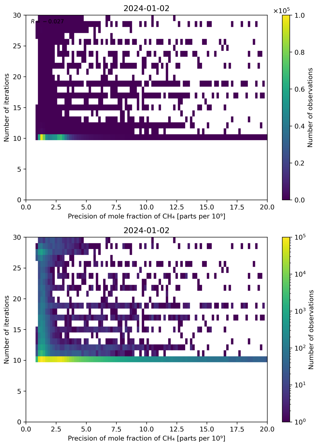
Figure 83: Scatter density plot of “Precision of mole fraction of CH 4 ” against “Number of iterations” for 2024-01-01 to 2024-01-03.
