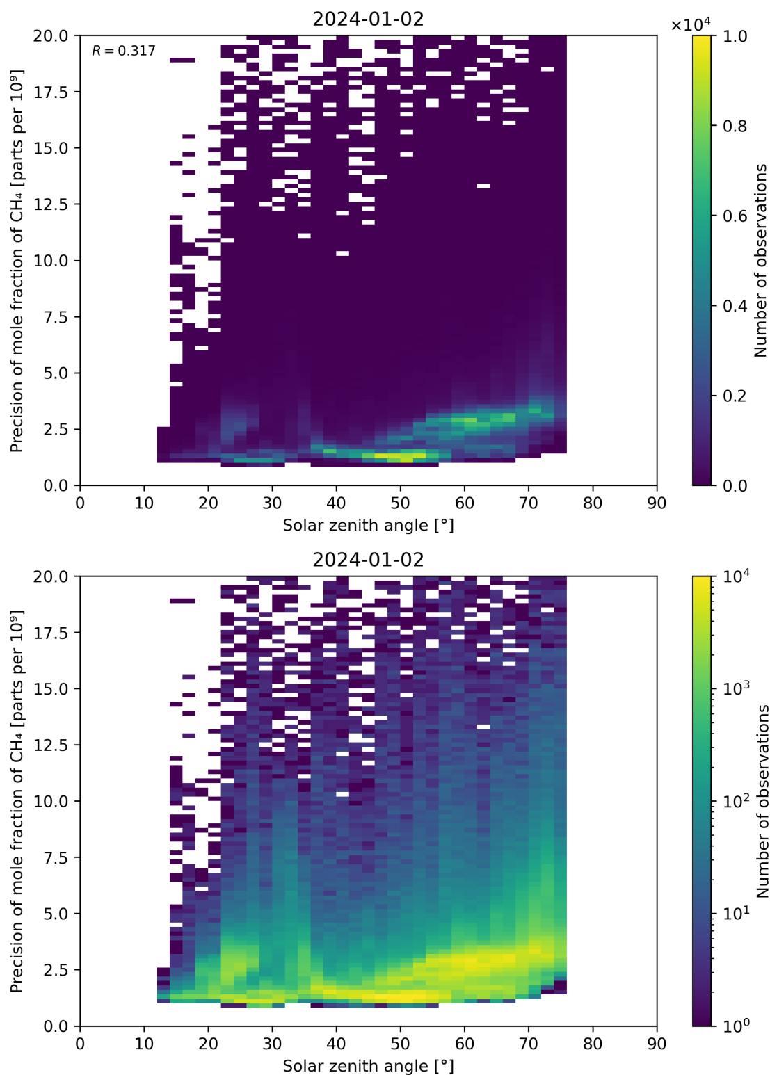
Figure 101: Scatter density plot of “Solar zenith angle” against “Precision of mole fraction of CH 4 ” for 2024-01-01 to 2024-01-03.
