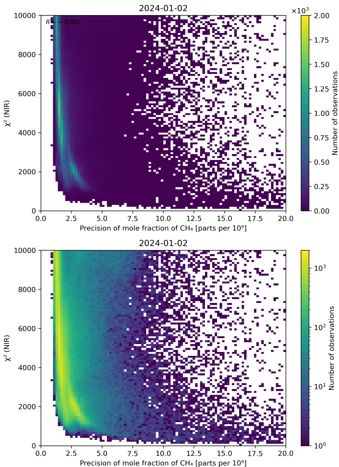
Figure 78: Scatter density plot of “Precision of mole fraction of \text{CH}_4 ” against “ \chi^2 (NIR)” for 2024-01-01 to 2024-01-03.
