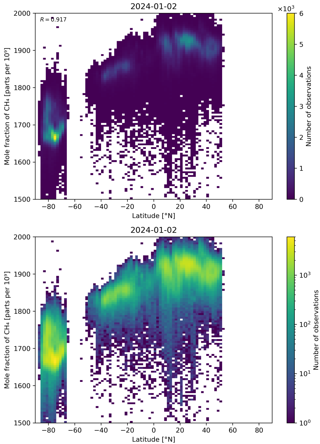
Figure 57: Scatter density plot of “Latitude” against “Mole fraction of CH 4 ” for 2024-01-01 to 2024-01-03.
