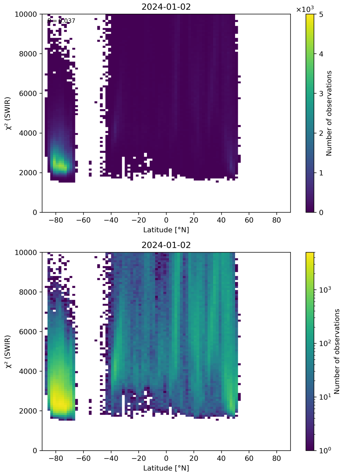
Figure 54: Scatter density plot of “Latitude” against “ \chi^2 (SWIR)” for 2024-01-01 to 2024-01-03.
