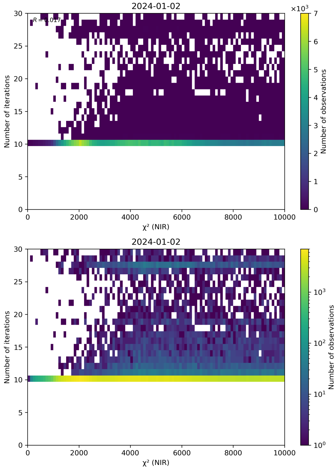
Figure 46: Scatter density plot of “ \chi^2 (NIR)” against “Number of iterations” for 2024-01-01 to 2024-01-03.
