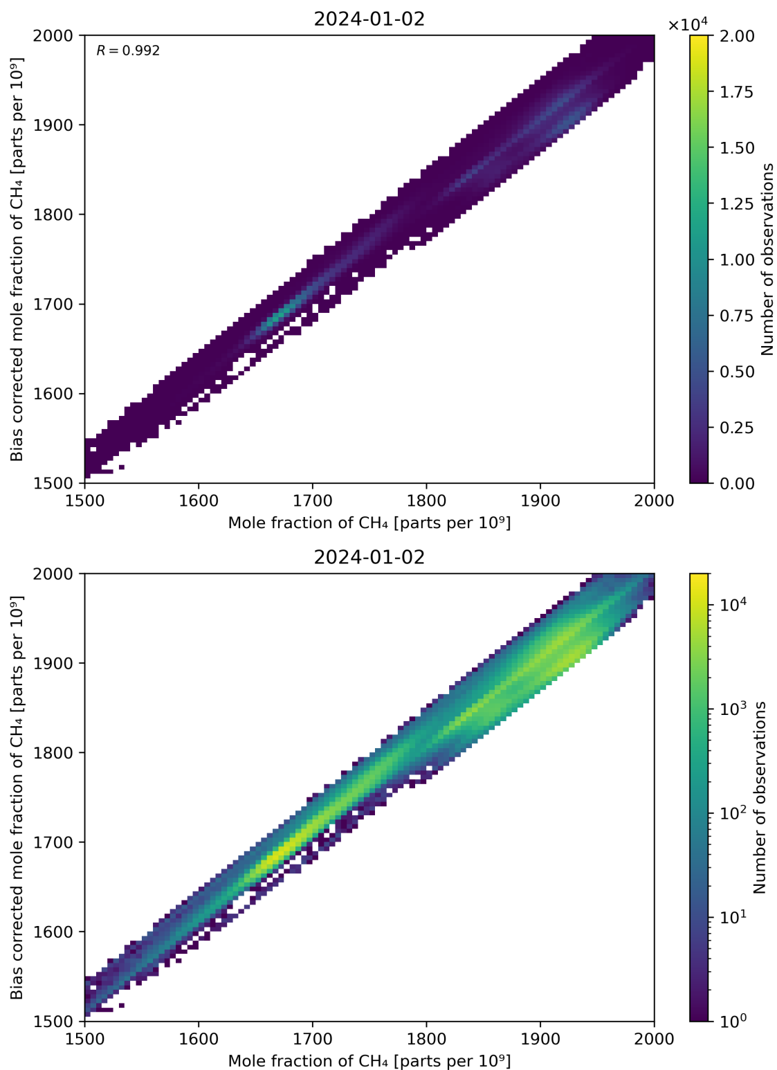
Figure 74: Scatter density plot of “Mole fraction of CH 4 ” against “Bias corrected mole fraction of CH 4 ” for 2024-01-01 to 2024-01-03.
