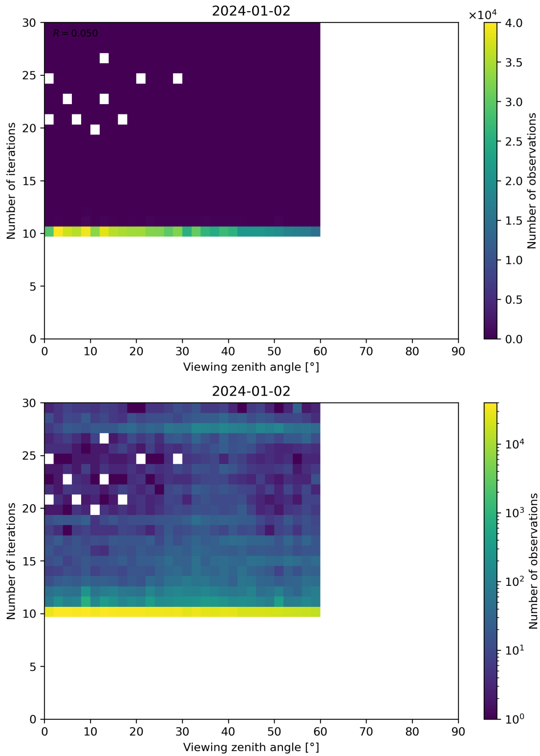
Figure 113: Scatter density plot of “Viewing zenith angle” against “Number of iterations” for 2024-01-01 to 2024-01-03.
