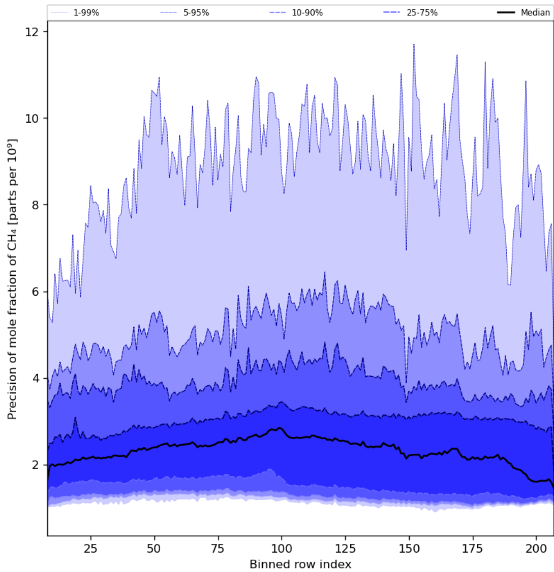
Figure 35: Along track statistics of “Precision of mole fraction of CH 4 ” for 2024-01-01 to 2024-01-03
