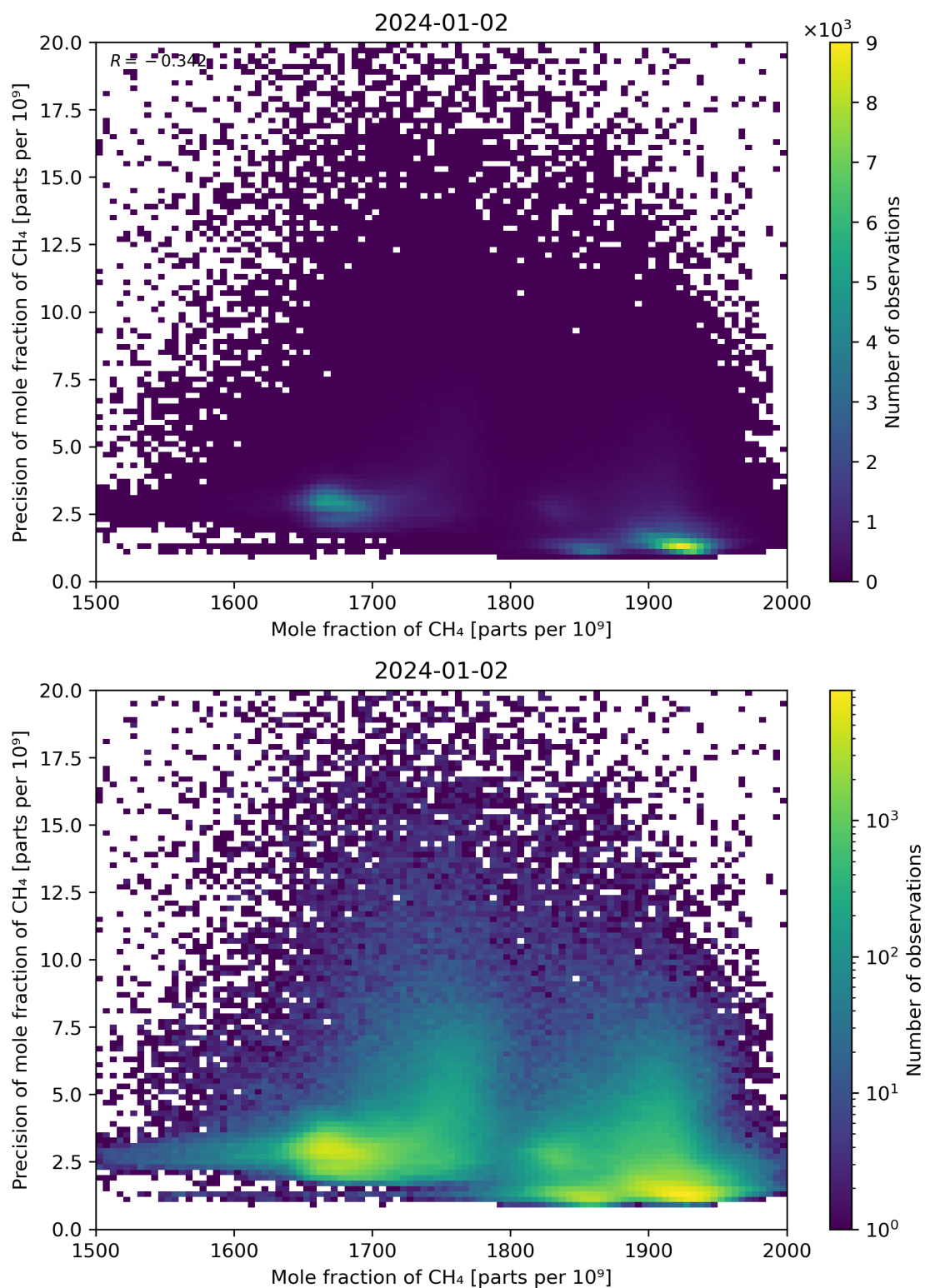
Figure 75: Scatter density plot of “Mole fraction of CH 4 ” against “Precision of mole fraction of CH 4 ” for 2024-01-01 to 2024-01-03.
