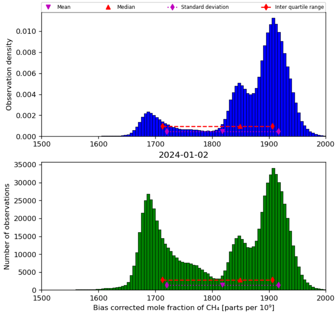
Figure 25: Histogram of “Bias corrected mole fraction of CH 4 ” for 2024-01-01 to 2024-01-03
