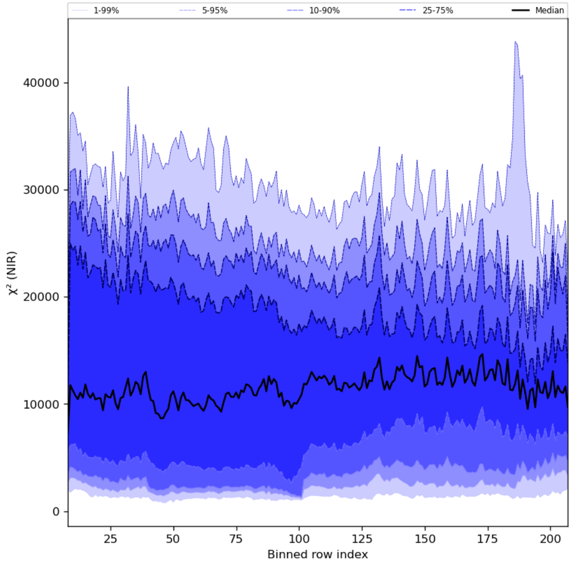
Figure 40: Along track statistics of “ \chi^2 (NIR)” for 2024-01-01 to 2024-01-03
