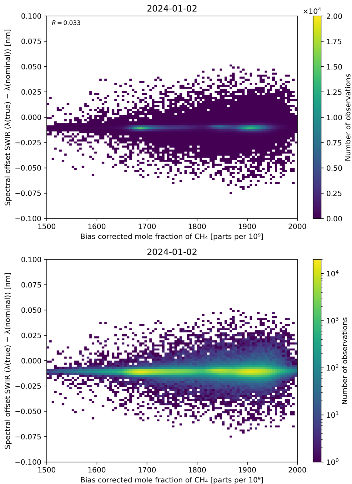
Figure 69: Scatter density plot of “Bias corrected mole fraction of \text{CH}_4 ” against “Spectral offset SWIR ( \lambda(\text{true}) - \lambda(\text{nominal}) )” for 2024-01-01 to 2024-01-03.
