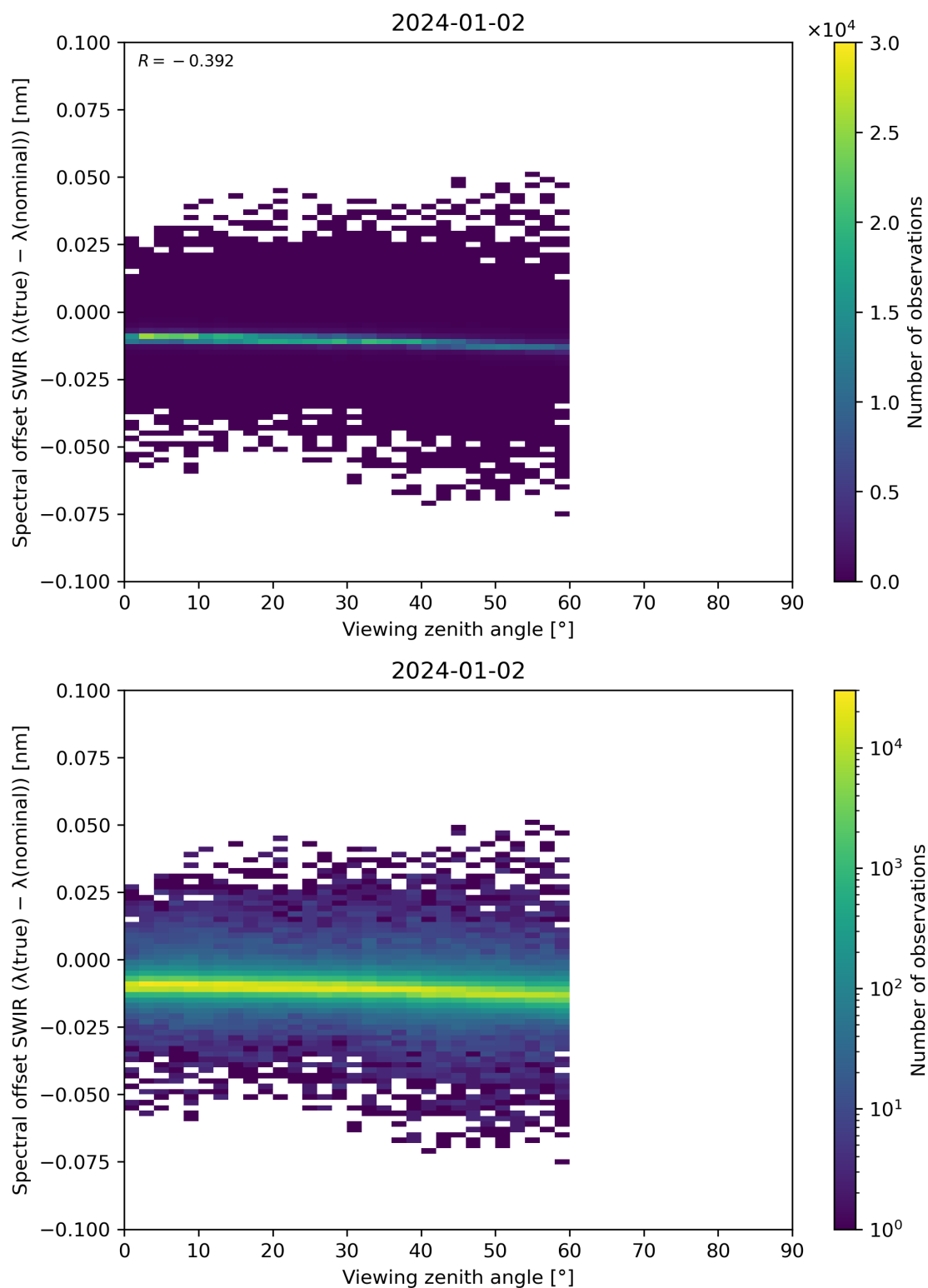
Figure 116: Scatter density plot of “Viewing zenith angle” against “Spectral offset SWIR ( \lambda(\text{true}) - \lambda(\text{nominal}) )” for 2024-01-01 to 2024-01-03.
