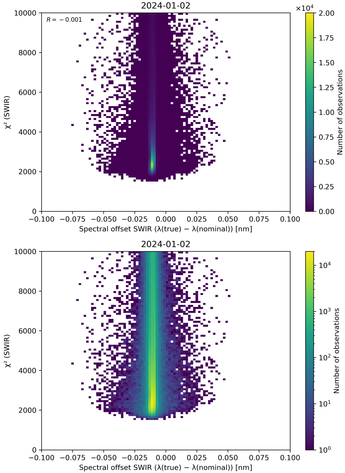
Figure 118: Scatter density plot of “Spectral offset SWIR ( \lambda(\text{true}) - \lambda(\text{nominal}) )” against “ \chi^2 (SWIR)” for 2024-01-01 to 2024-01-03.
