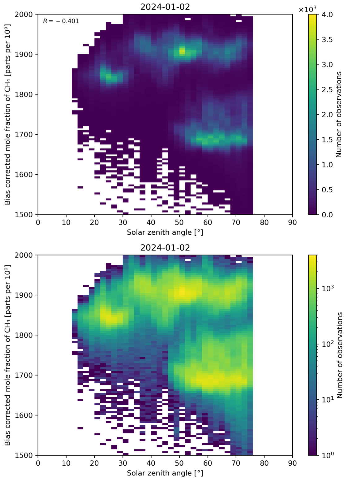
Figure 100: Scatter density plot of “Solar zenith angle” against “Bias corrected mole fraction of \text{CH}_4 ” for 2024-01-01 to 2024-01-03.
