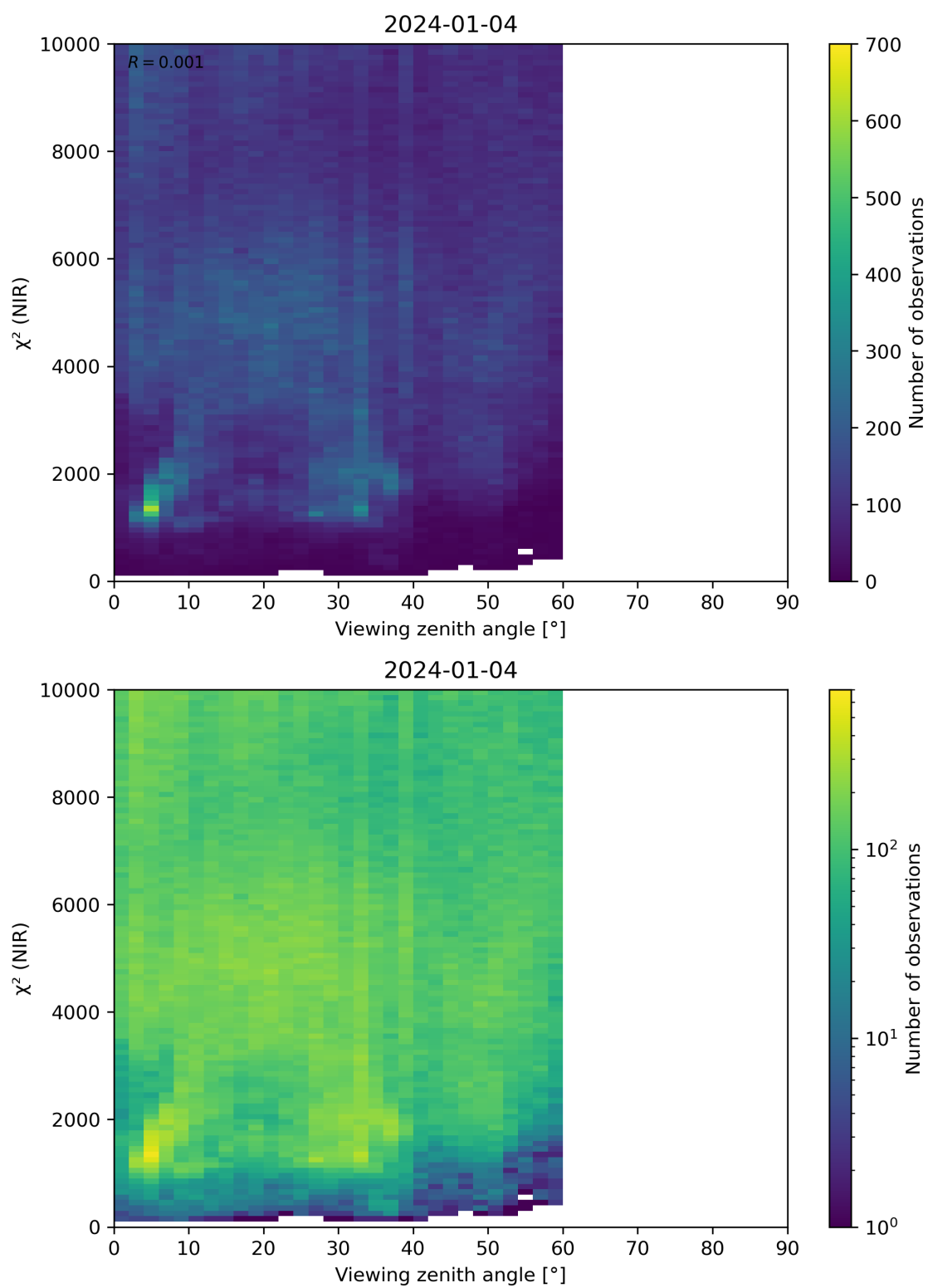
Figure 105: Scatter density plot of “Viewing zenith angle” against “ \chi^2 (NIR)” for 2024-01-03 to 2024-01-05.
