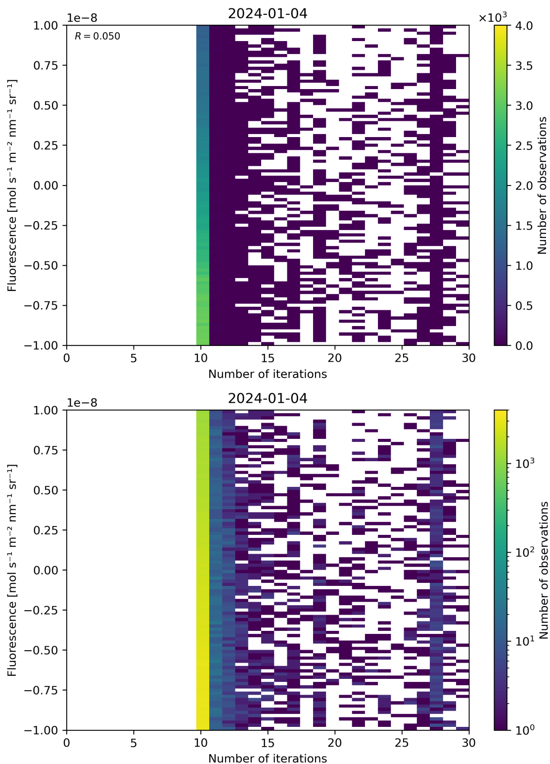
Figure 87: Scatter density plot of “Number of iterations” against “Fluorescence” for 2024-01-03 to 2024-01-05.
