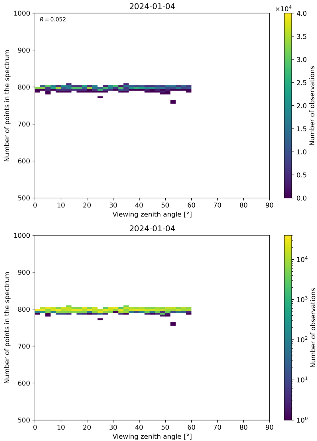
Figure 114: Scatter density plot of “Viewing zenith angle” against “Number of points in the spectrum” for 2024-01-03 to 2024-01-05.
