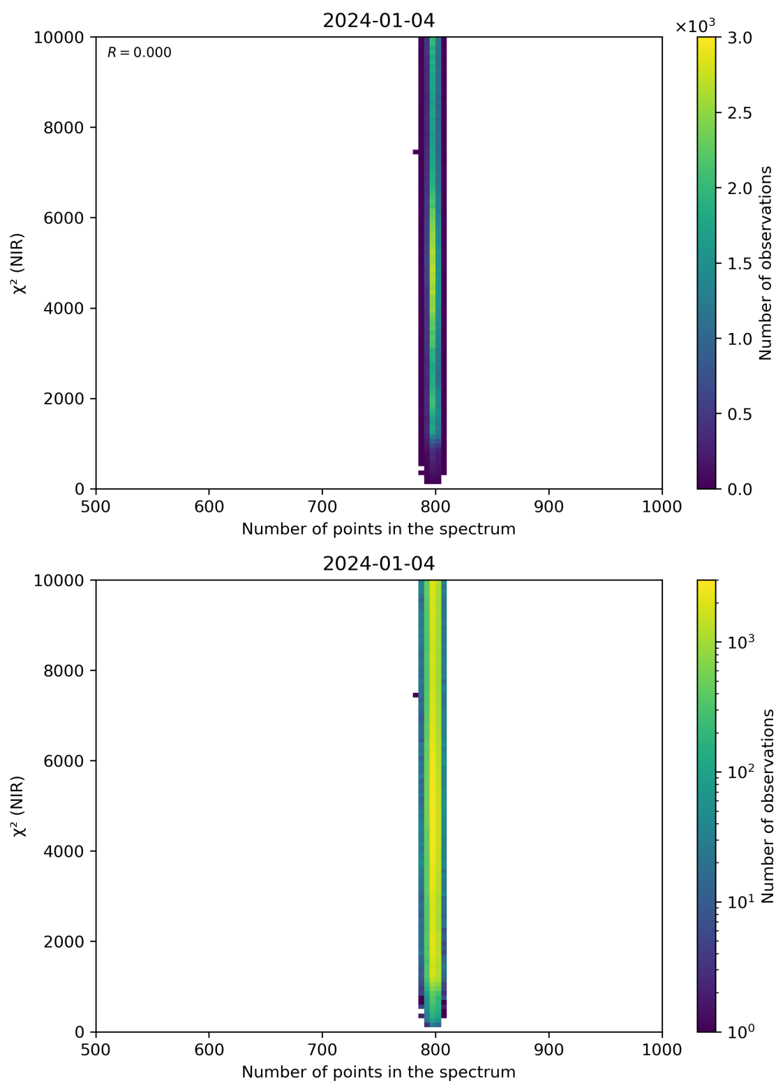
Figure 88: Scatter density plot of “Number of points in the spectrum” against “ \chi^2 (NIR)” for 2024-01-03 to 2024-01-05.
