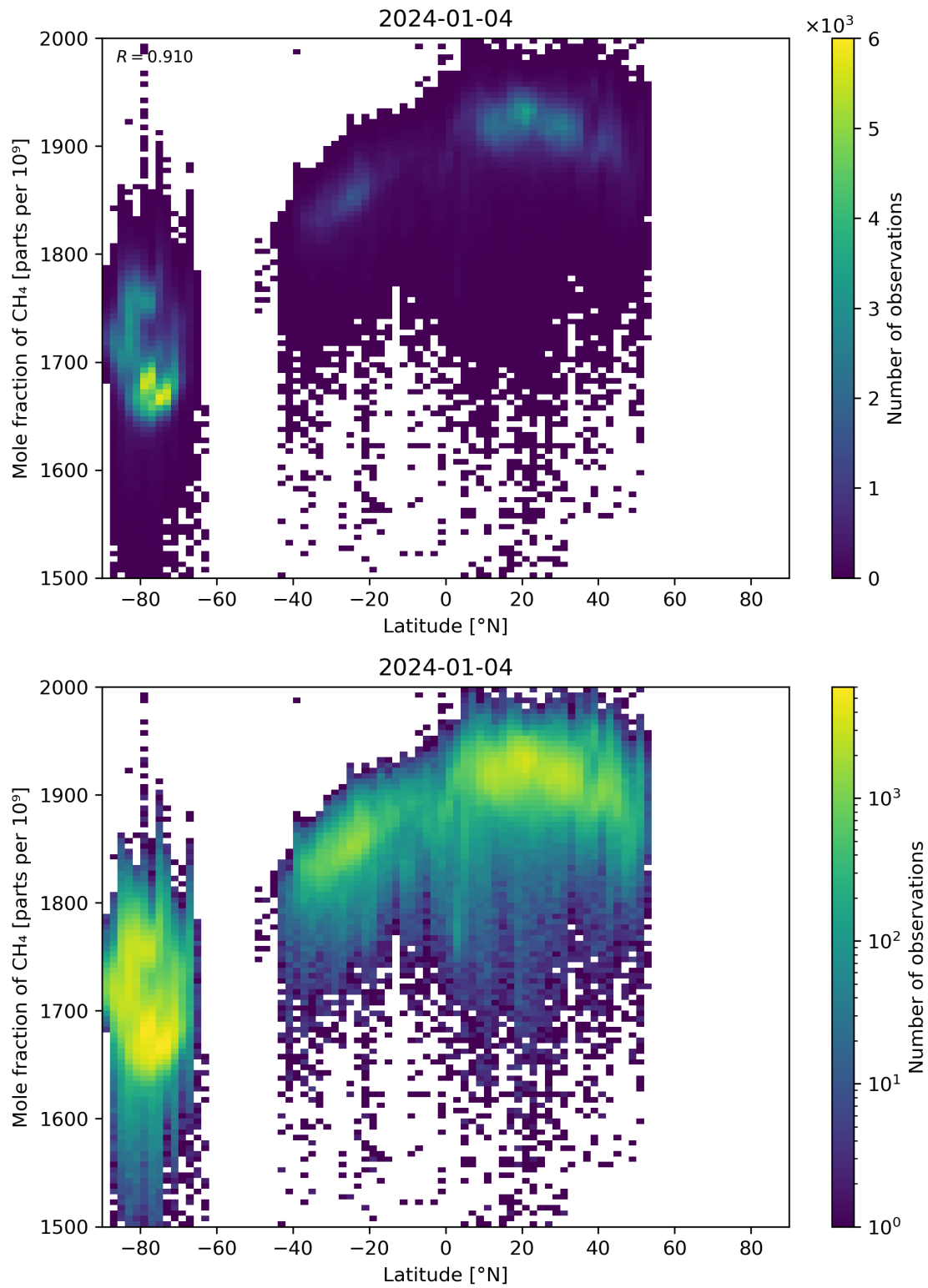
Figure 57: Scatter density plot of “Latitude” against “Mole fraction of CH 4 ” for 2024-01-03 to 2024-01-05.
