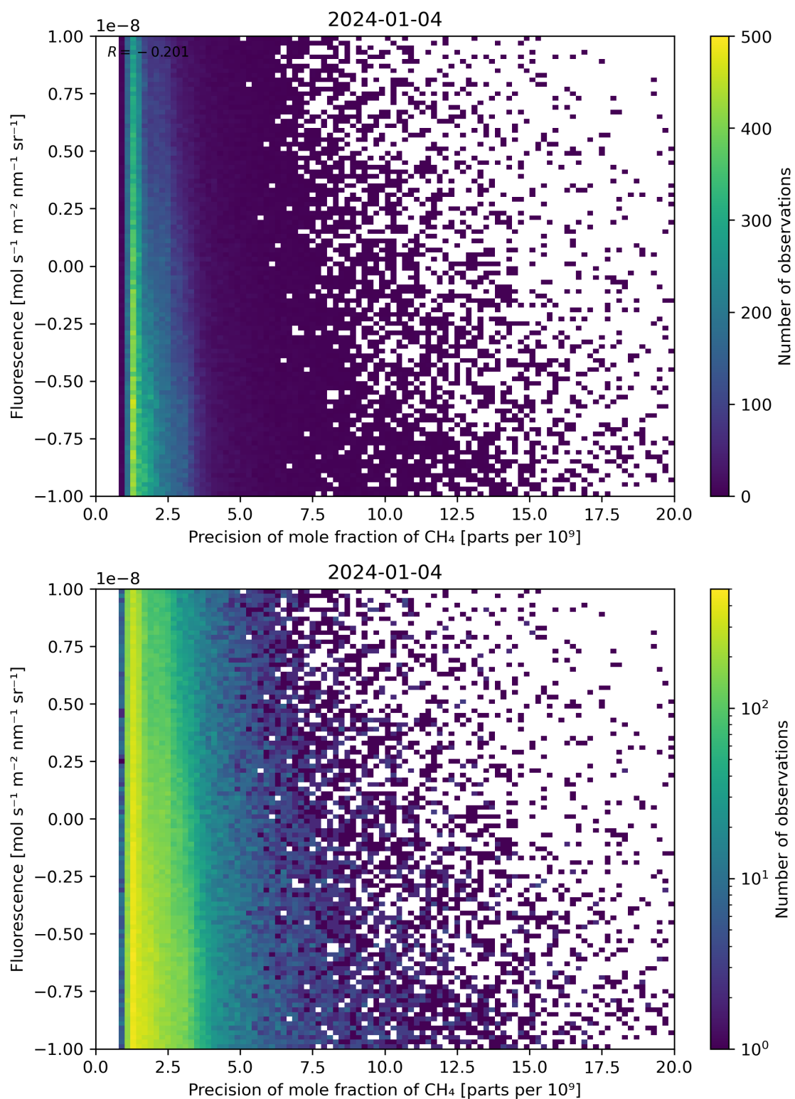
Figure 81: Scatter density plot of “Precision of mole fraction of \text{CH}_4 ” against “Fluorescence” for 2024-01-03 to 2024-01-05.
