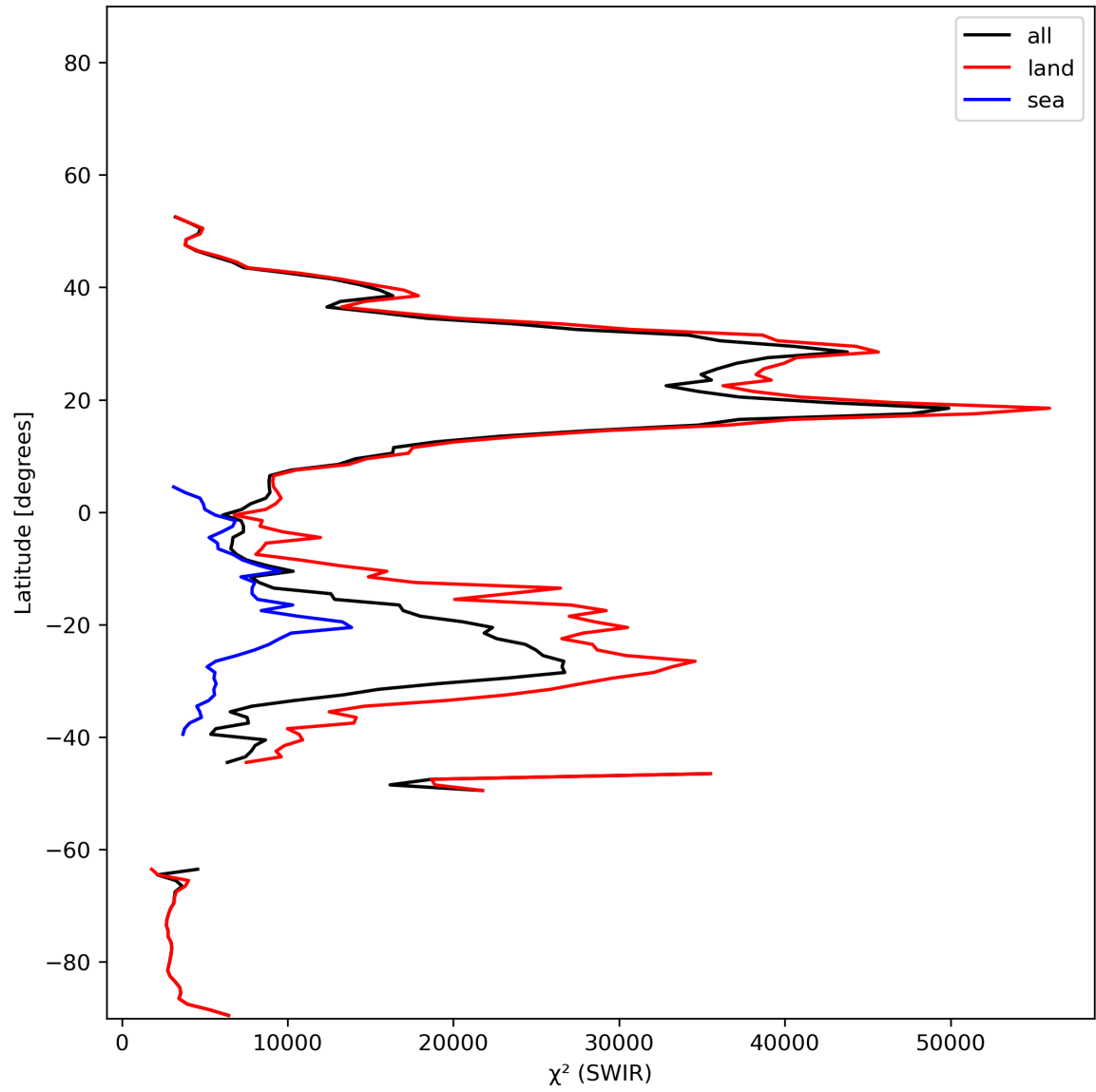
Figure 17: Zonal average of “ \chi^2 (SWIR)” for 2024-01-03 to 2024-01-05.
