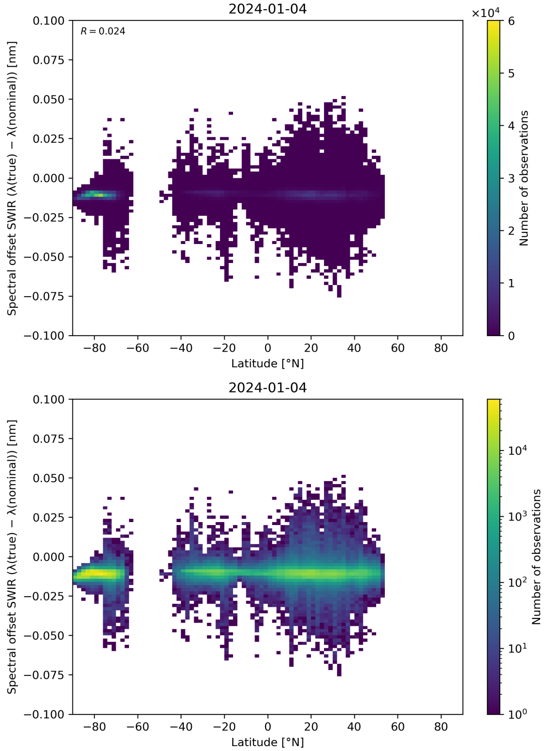
Figure 62: Scatter density plot of “Latitude” against “Spectral offset SWIR ( \lambda(\text{true}) - \lambda(\text{nominal}) )” for 2024-01-03 to 2024-01-05.
