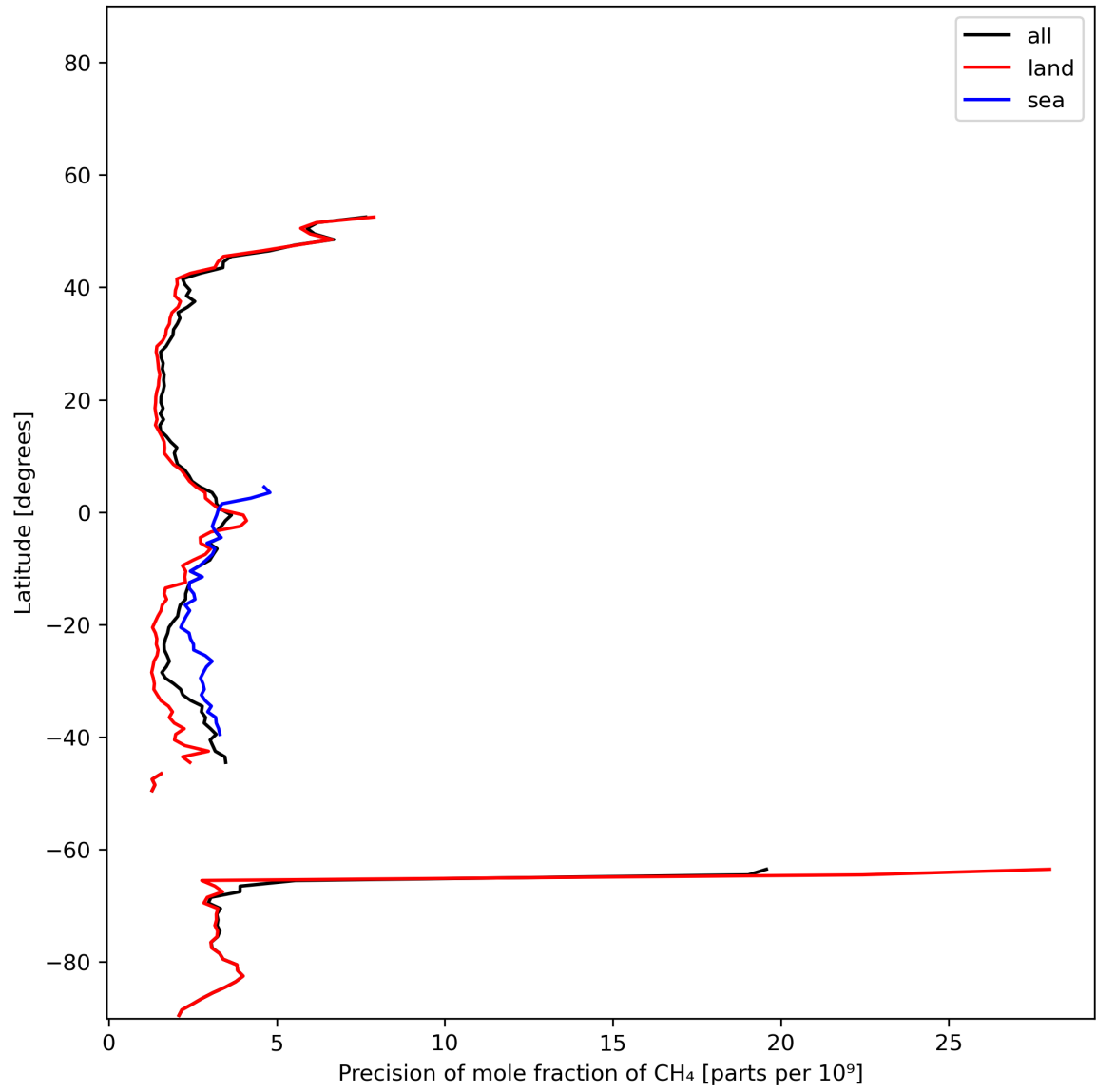
Figure 13: Zonal average of “Precision of mole fraction of CH 4 ” for 2024-01-03 to 2024-01-05.
