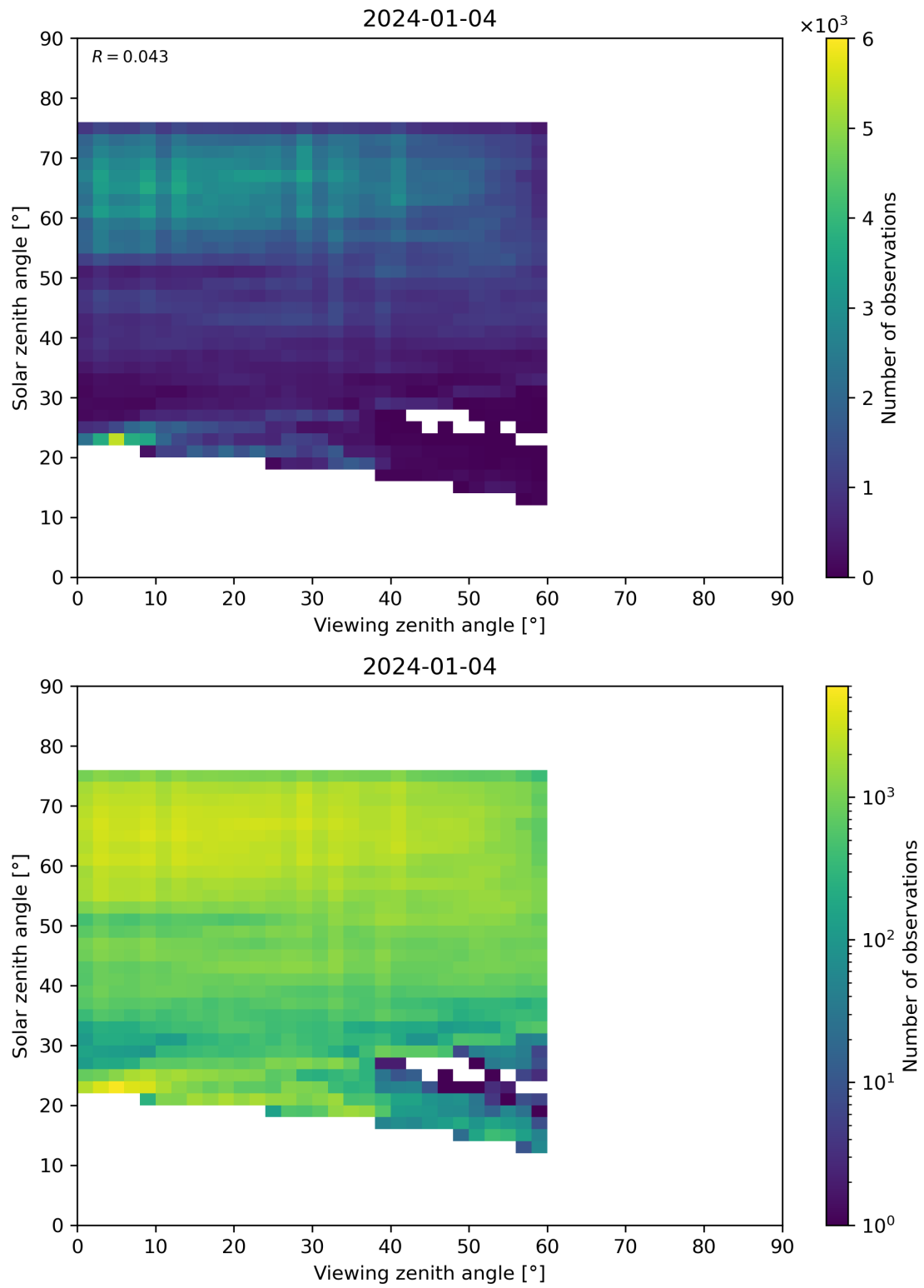
Figure 115: Scatter density plot of “Viewing zenith angle” against “Solar zenith angle” for 2024-01-03 to 2024-01-05.
