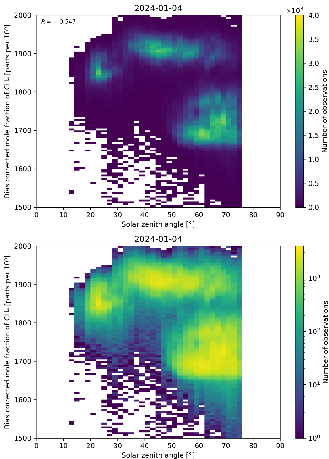
Figure 100: Scatter density plot of “Solar zenith angle” against “Bias corrected mole fraction of CH 4 ” for 2024-01-03 to 2024-01-05.
