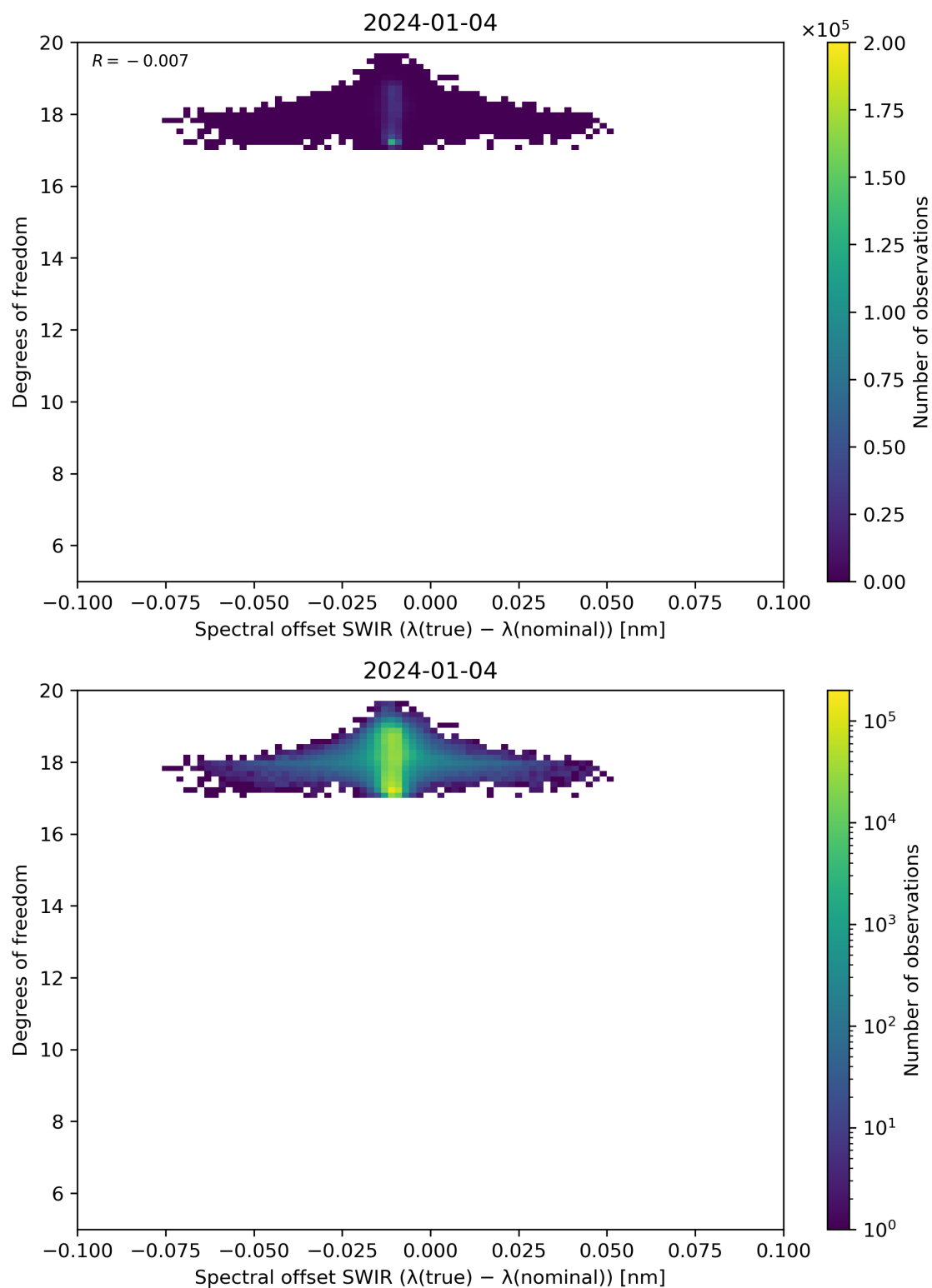
Figure 119: Scatter density plot of “Spectral offset SWIR ( \lambda(\text{true}) - \lambda(\text{nominal}) )” against “Degrees of freedom” for 2024-01-03 to 2024-01-05.
