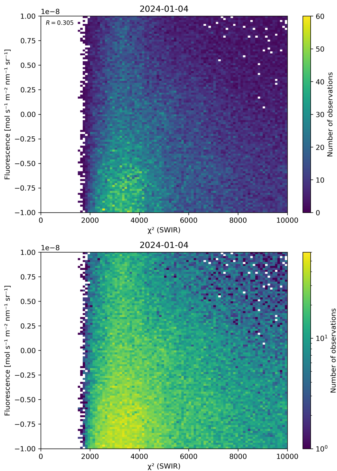
Figure 49: Scatter density plot of “ \chi^2 (SWIR)” against “Fluorescence” for 2024-01-03 to 2024-01-05.
