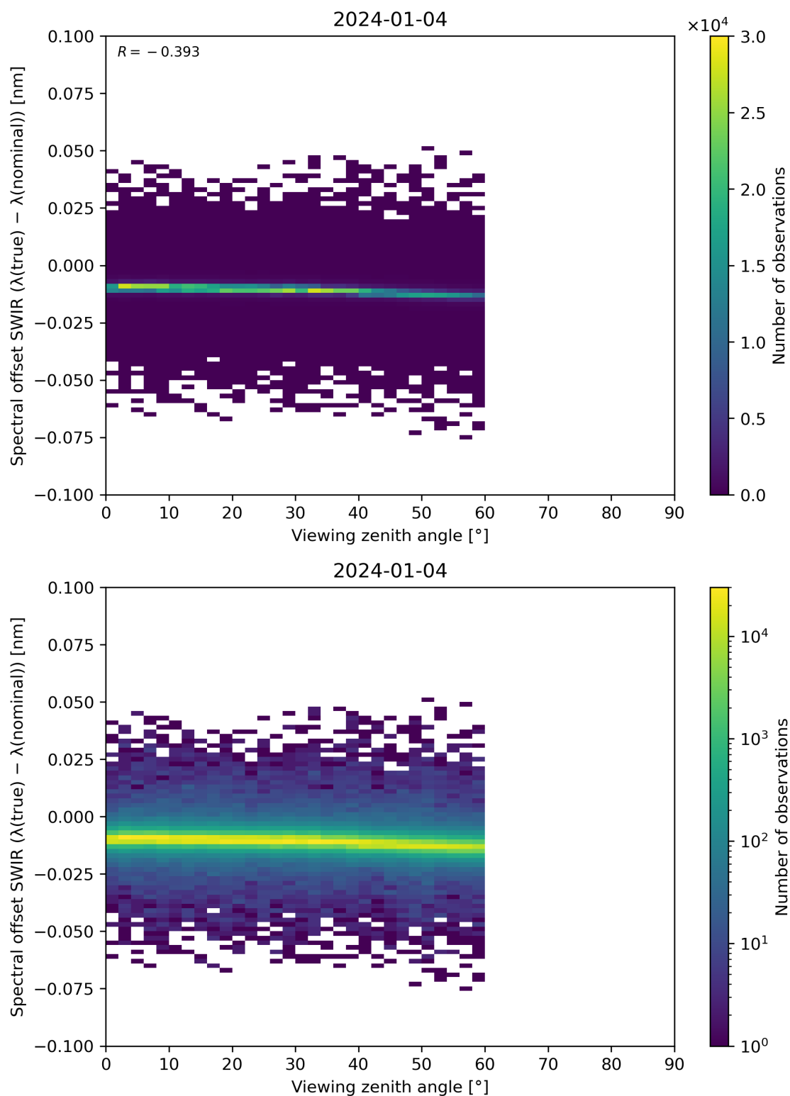
Figure 116: Scatter density plot of “Viewing zenith angle” against “Spectral offset SWIR ( \lambda(\text{true}) - \lambda(\text{nominal}) )” for 2024-01-03 to 2024-01-05.
