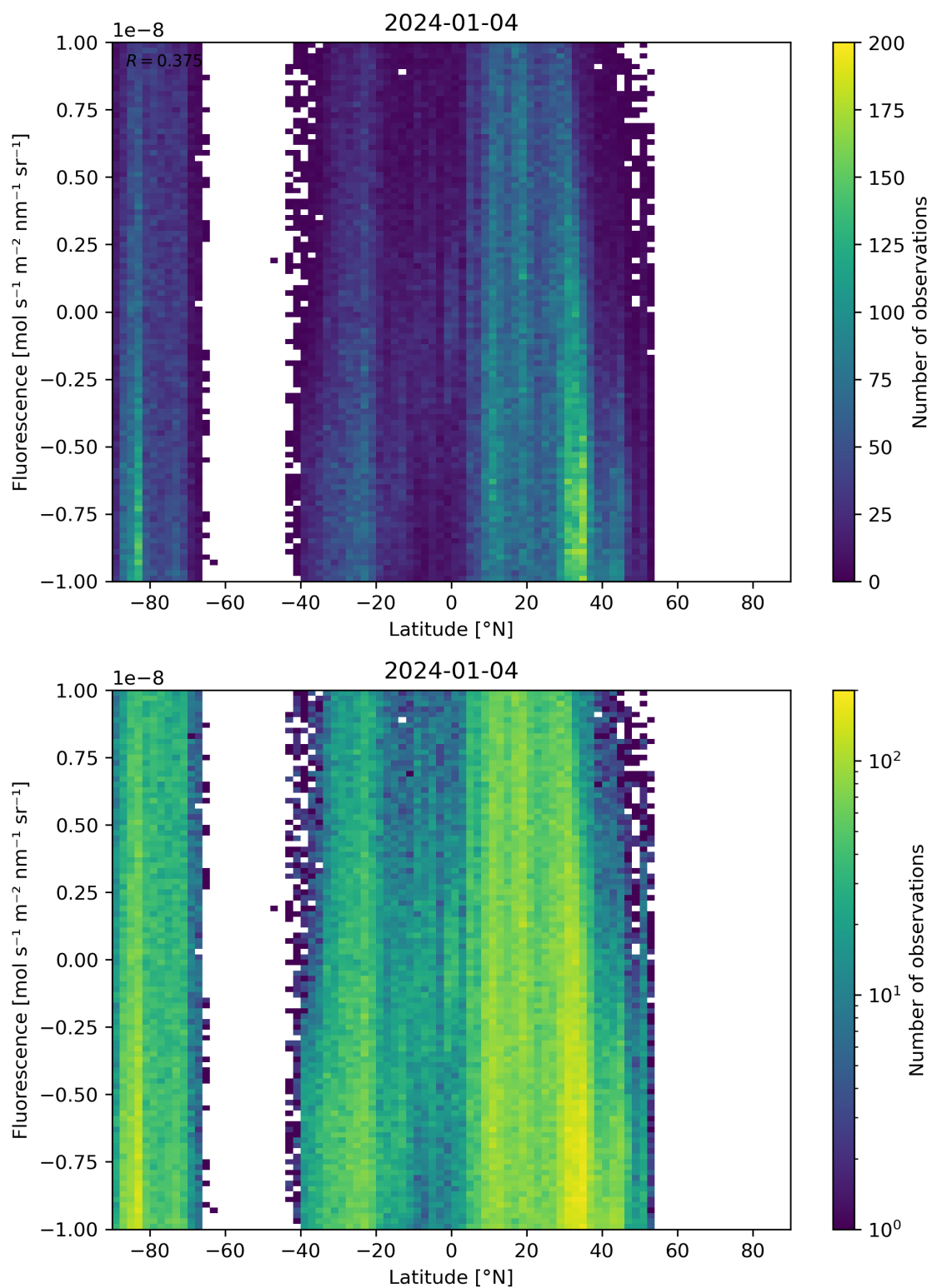
Figure 56: Scatter density plot of “Latitude” against “Fluorescence” for 2024-01-03 to 2024-01-05.
