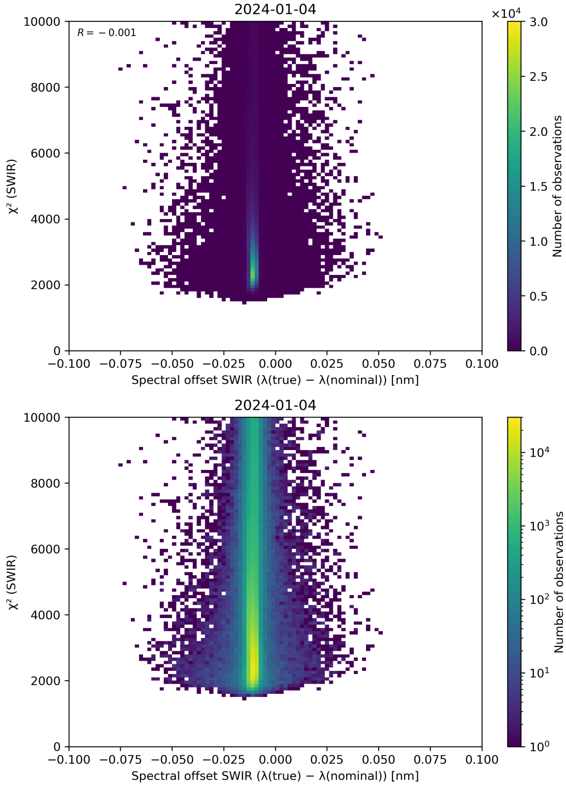
Figure 118: Scatter density plot of “Spectral offset SWIR ( \lambda(\text{true}) - \lambda(\text{nominal}) )” against “ \chi^2 (SWIR)” for 2024-01-03 to 2024-01-05.
