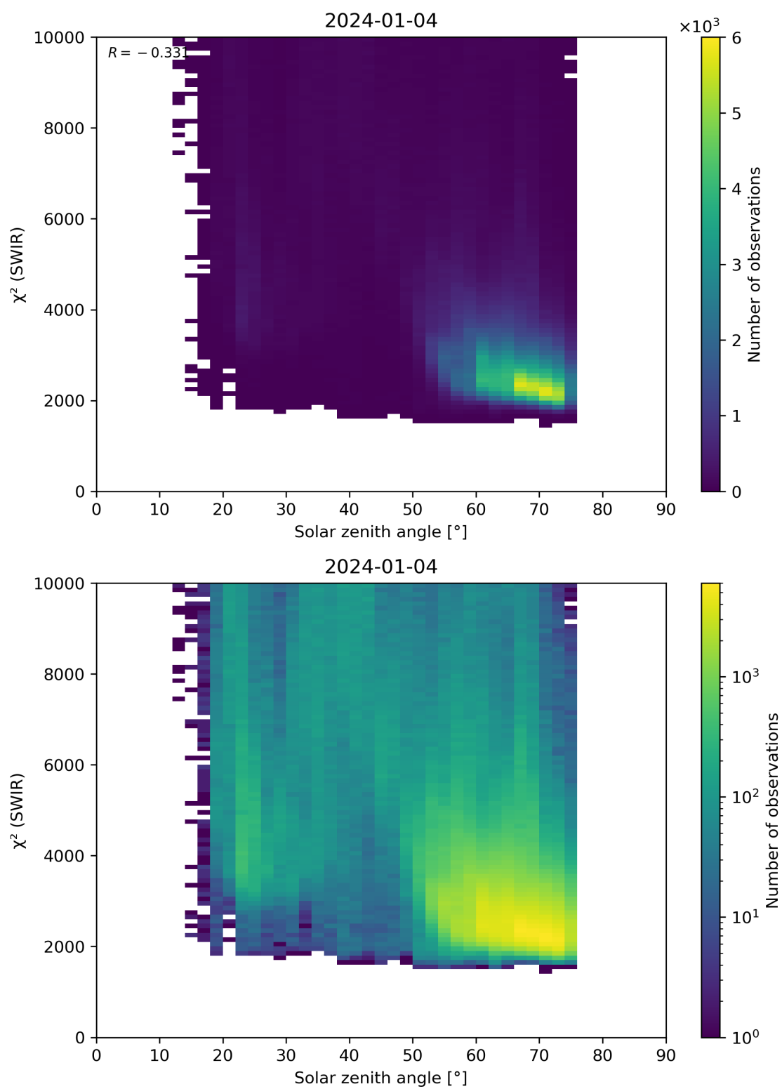
Figure 95: Scatter density plot of “Solar zenith angle” against “ \chi^2 (SWIR)” for 2024-01-03 to 2024-01-05.
