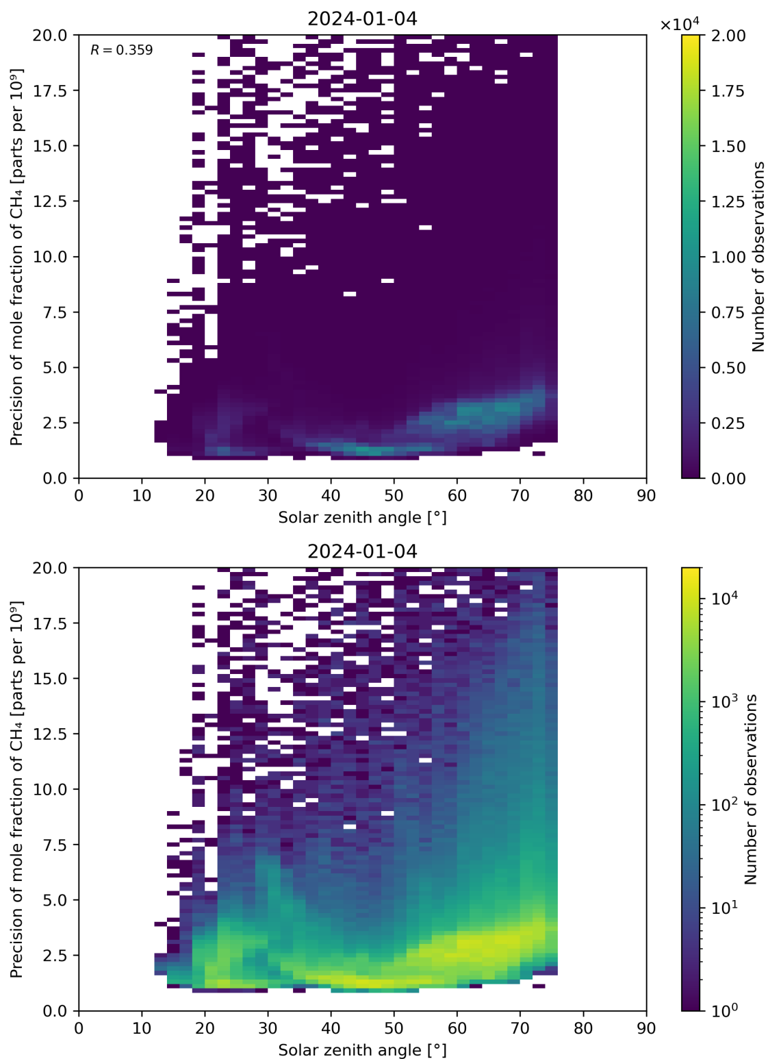
Figure 101: Scatter density plot of “Solar zenith angle” against “Precision of mole fraction of CH 4 ” for 2024-01-03 to 2024-01-05.
