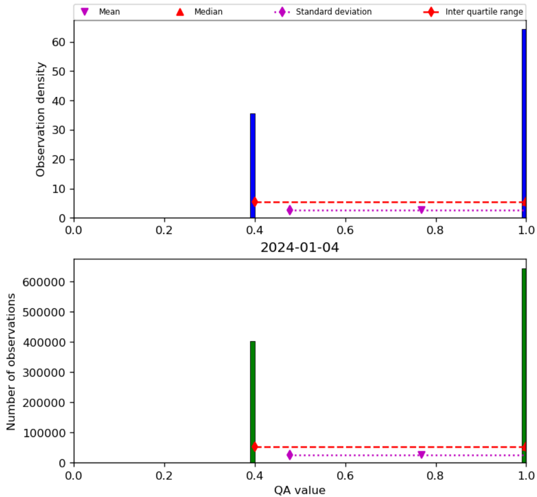
Figure 22: Histogram of “QA value” for 2024-01-03 to 2024-01-05
