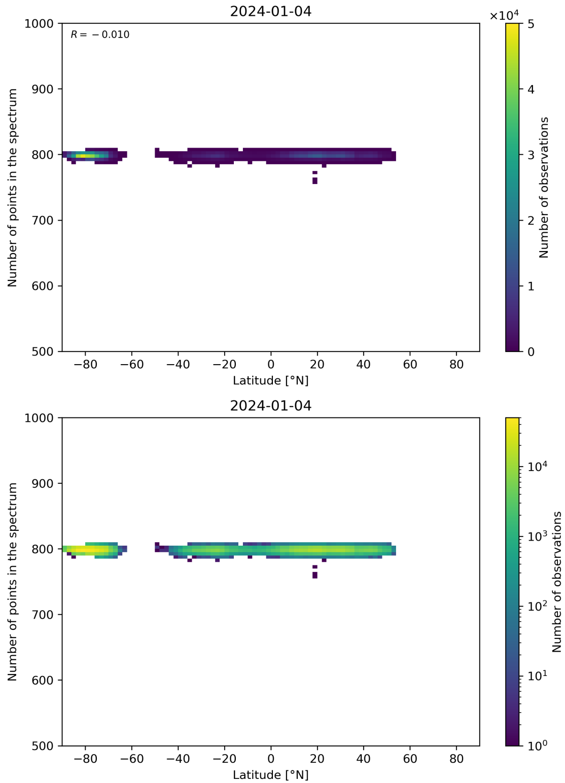
Figure 61: Scatter density plot of “Latitude” against “Number of points in the spectrum” for 2024-01-03 to 2024-01-05.
