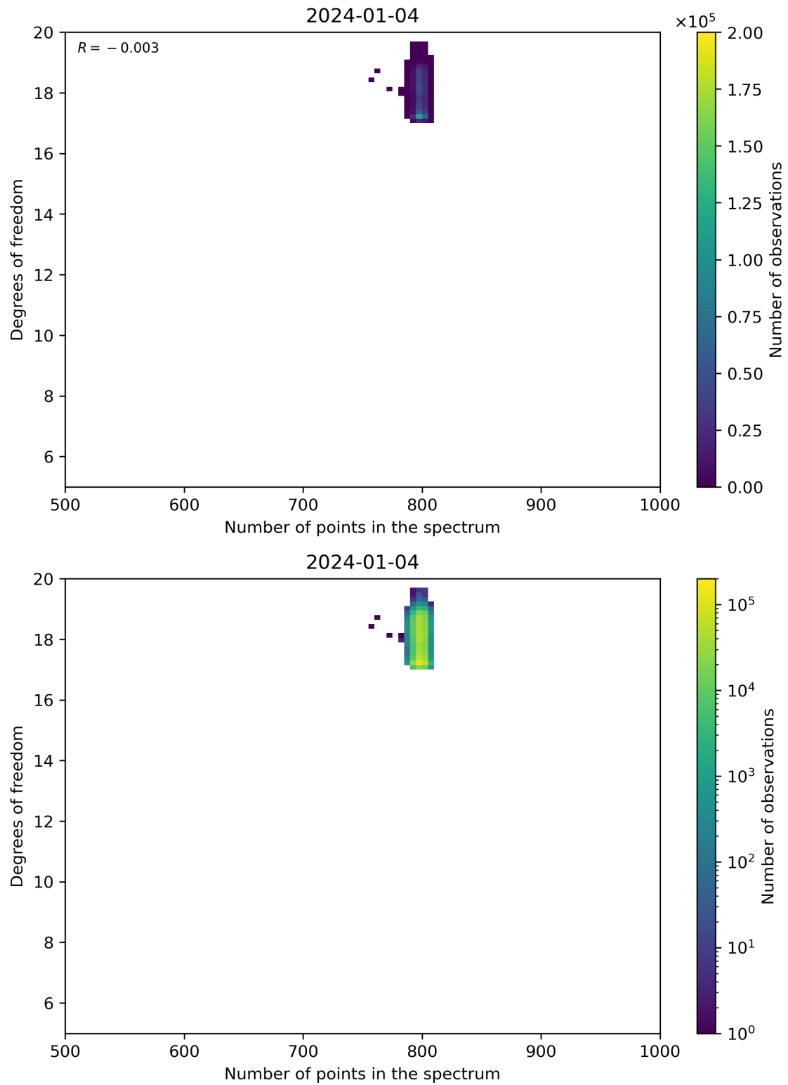
Figure 90: Scatter density plot of “Number of points in the spectrum” against “Degrees of freedom” for 2024-01-03 to 2024-01-05.
