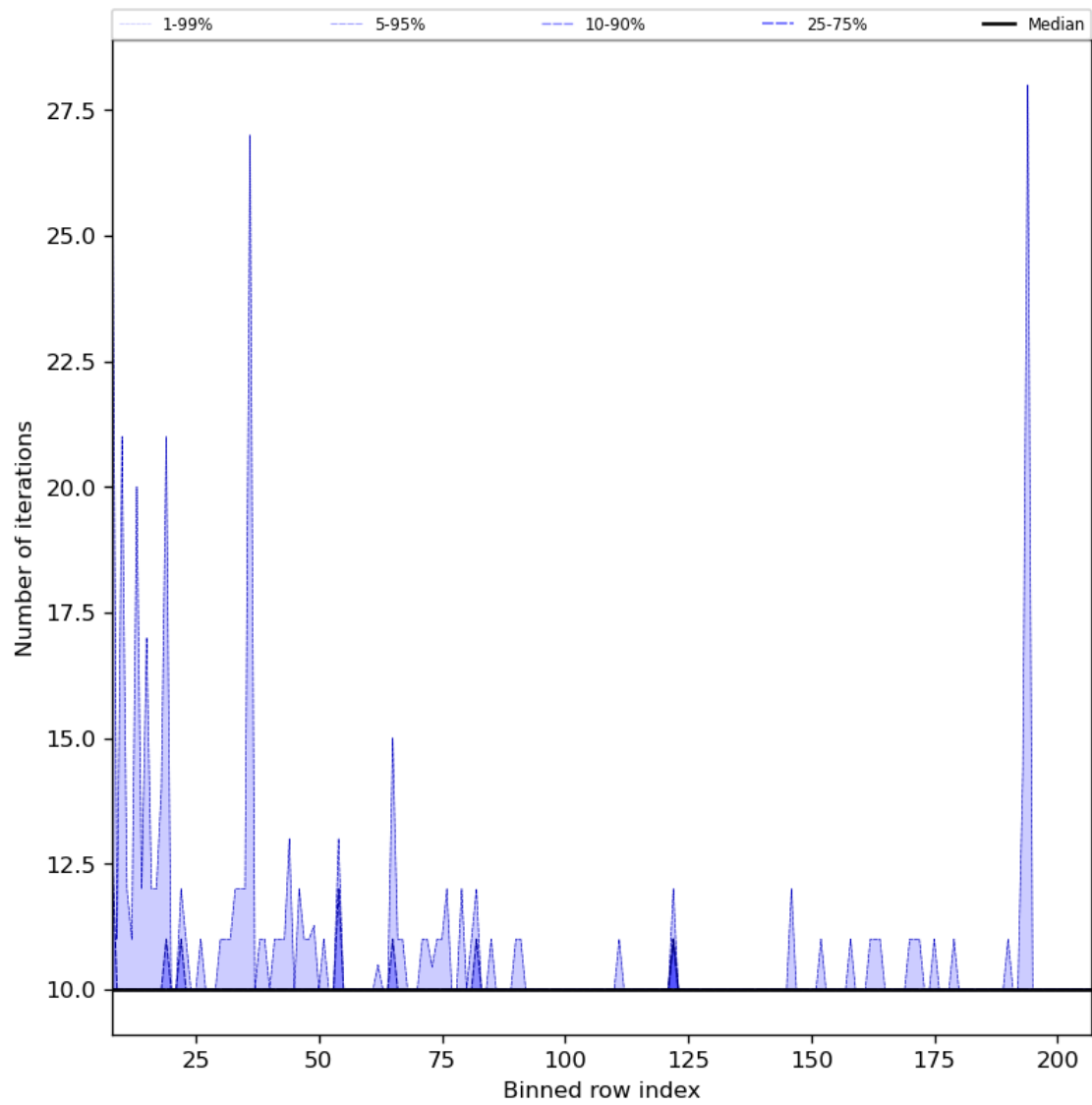
Figure 42: Along track statistics of “Number of iterations” for 2024-01-03 to 2024-01-05
