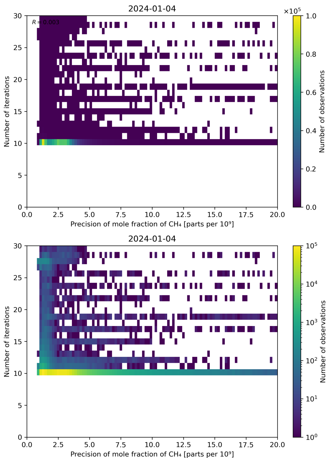
Figure 83: Scatter density plot of “Precision of mole fraction of \text{CH}_4 ” against “Number of iterations” for 2024-01-03 to 2024-01-05.
