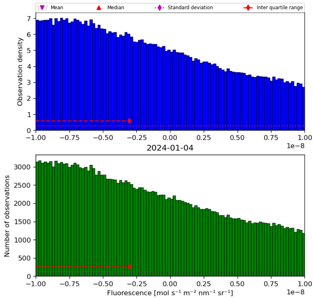
Figure 32: Histogram of “Fluorescence” for 2024-01-03 to 2024-01-05
