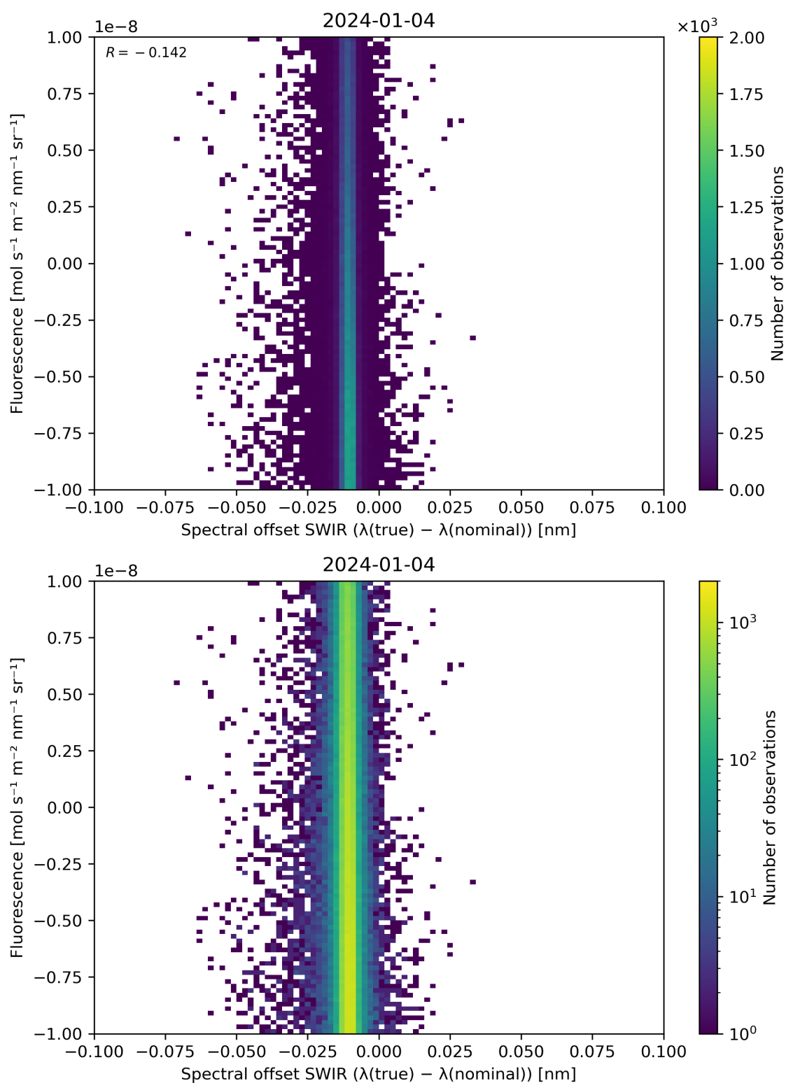
Figure 120: Scatter density plot of “Spectral offset SWIR ( \lambda(\text{true}) - \lambda(\text{nominal}) )” against “Fluorescence” for 2024-01-03 to 2024-01-05.
