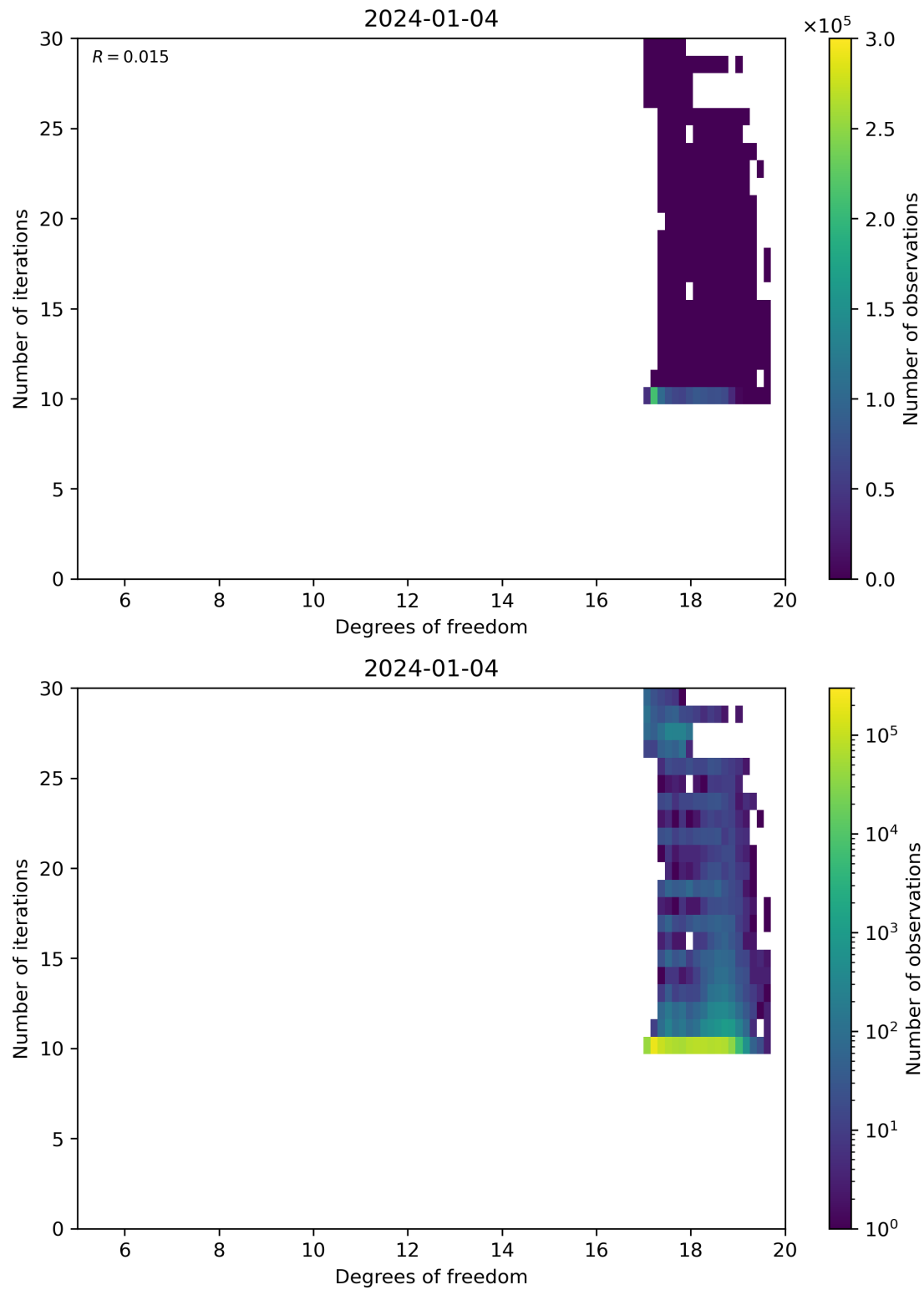
Figure 52: Scatter density plot of “Degrees of freedom” against “Number of iterations” for 2024-01-03 to 2024-01-05.
