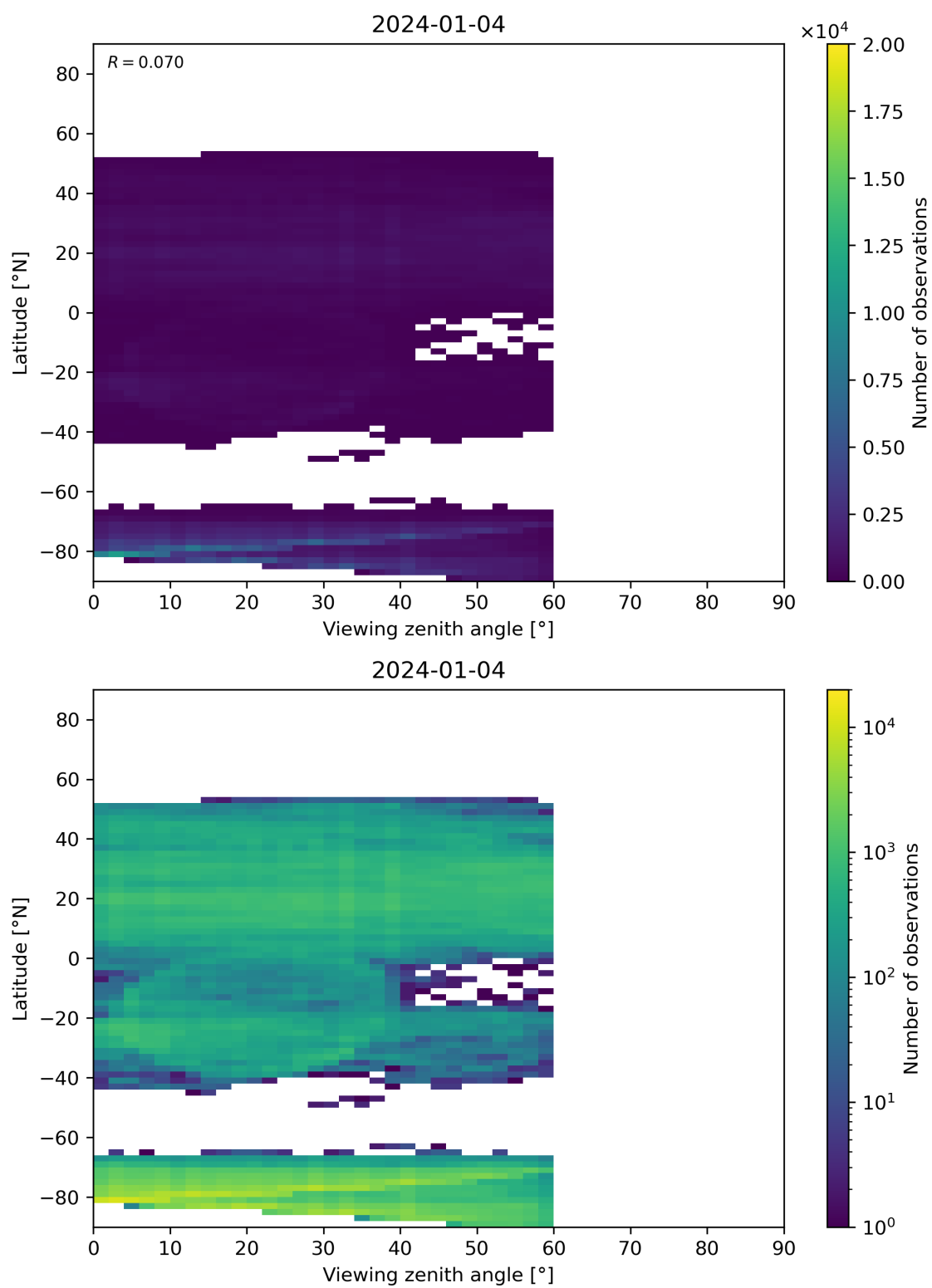
Figure 109: Scatter density plot of “Viewing zenith angle” against “Latitude” for 2024-01-03 to 2024-01-05.
