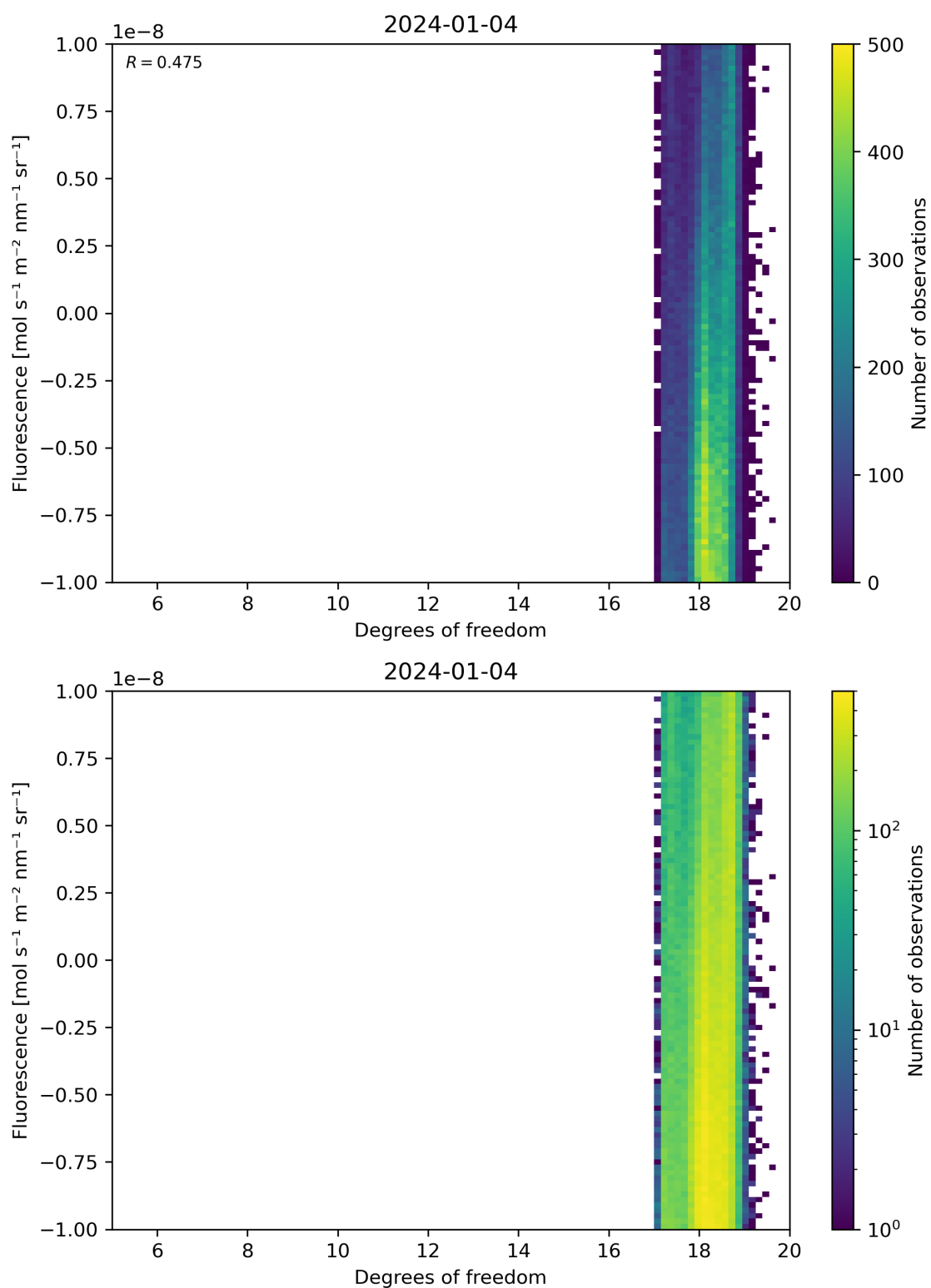
Figure 51: Scatter density plot of “Degrees of freedom” against “Fluorescence” for 2024-01-03 to 2024-01-05.
