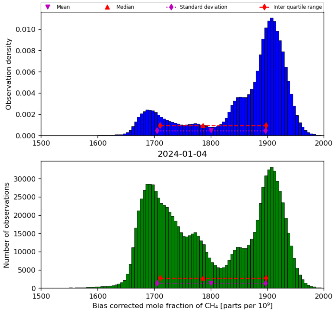
Figure 25: Histogram of “Bias corrected mole fraction of CH 4 ” for 2024-01-03 to 2024-01-05
