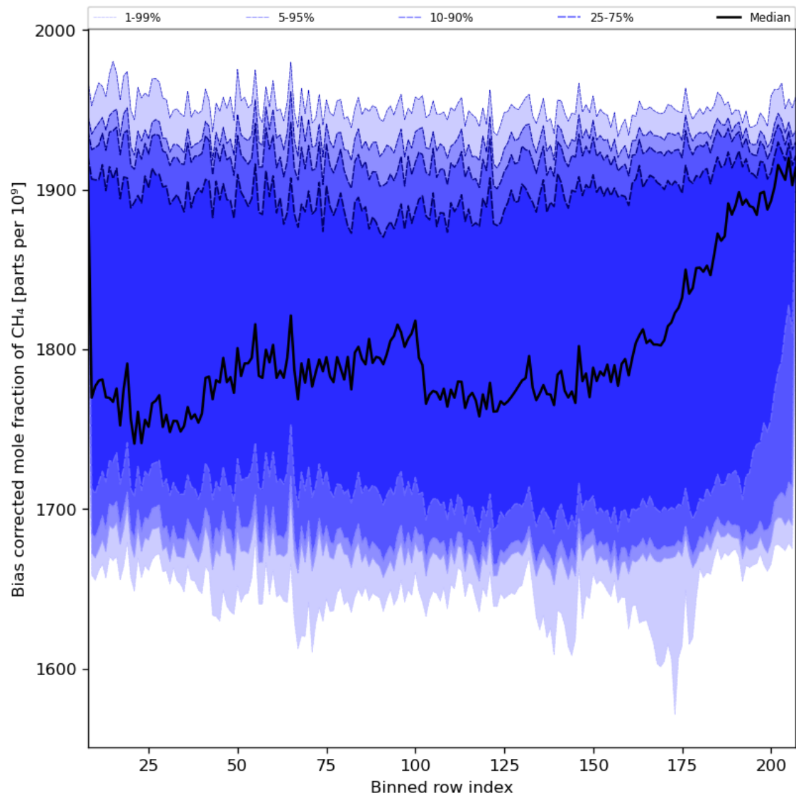
Figure 36: Along track statistics of “Bias corrected mole fraction of CH 4 ” for 2024-01-03 to 2024-01-05
