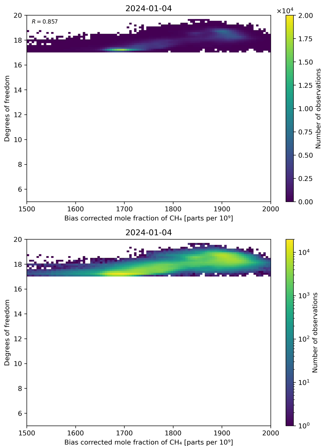
Figure 65: Scatter density plot of “Bias corrected mole fraction of CH 4 ” against “Degrees of freedom” for 2024-01-03 to 2024-01-05.
