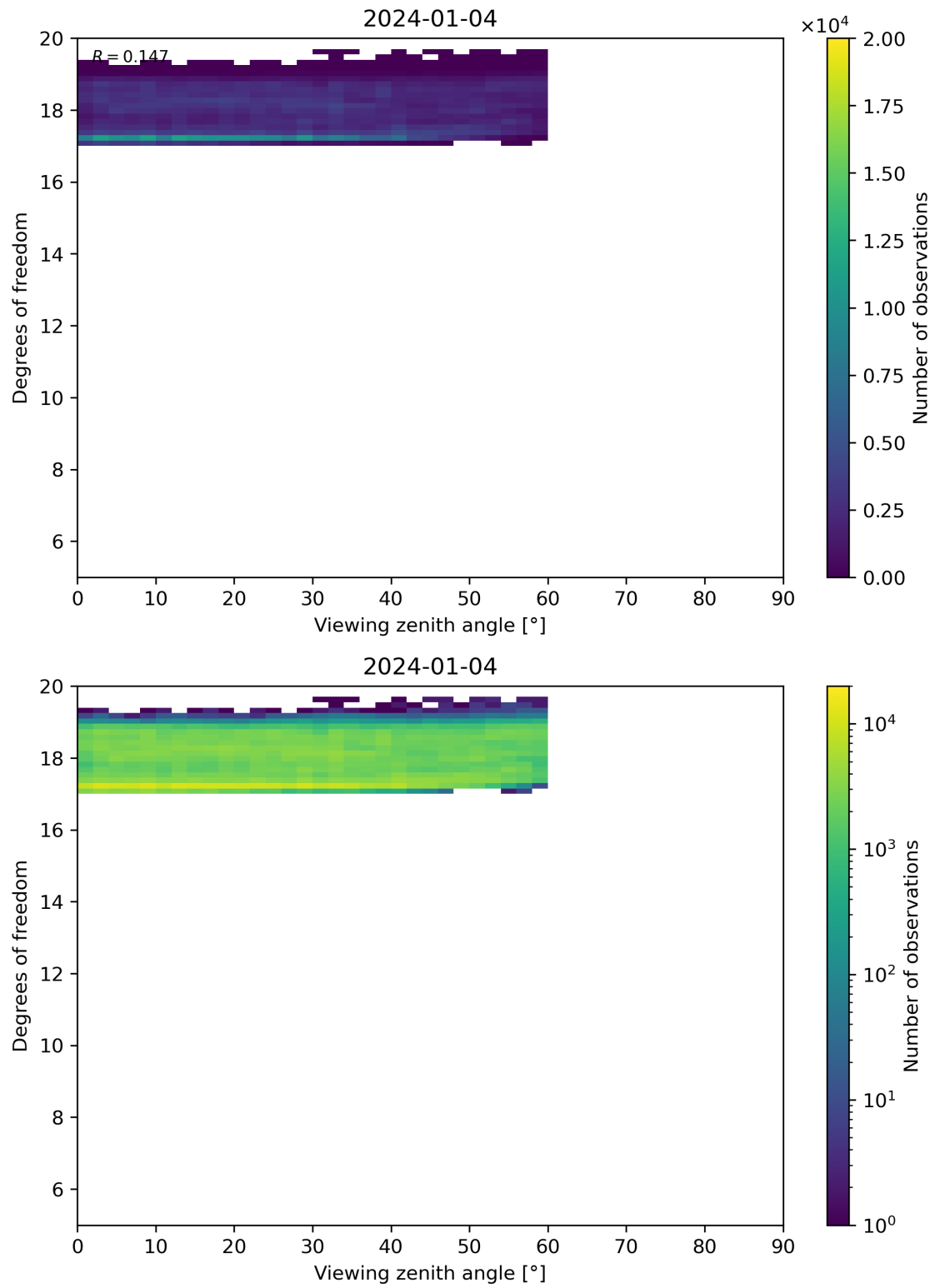
Figure 107: Scatter density plot of “Viewing zenith angle” against “Degrees of freedom” for 2024-01-03 to 2024-01-05.
