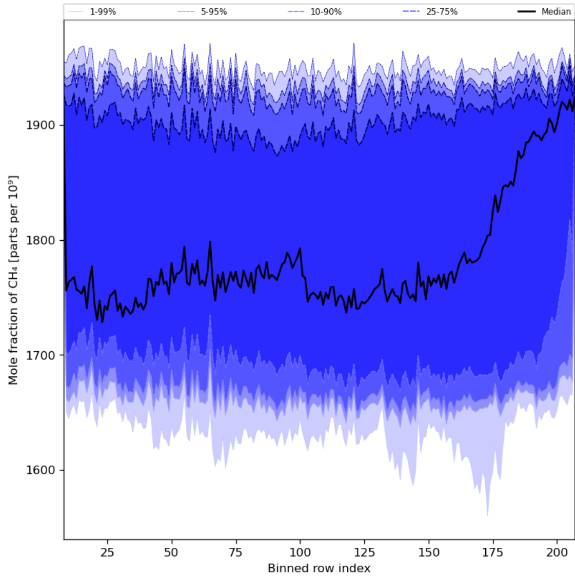
Figure 34: Along track statistics of “Mole fraction of CH 4 ” for 2024-01-03 to 2024-01-05
