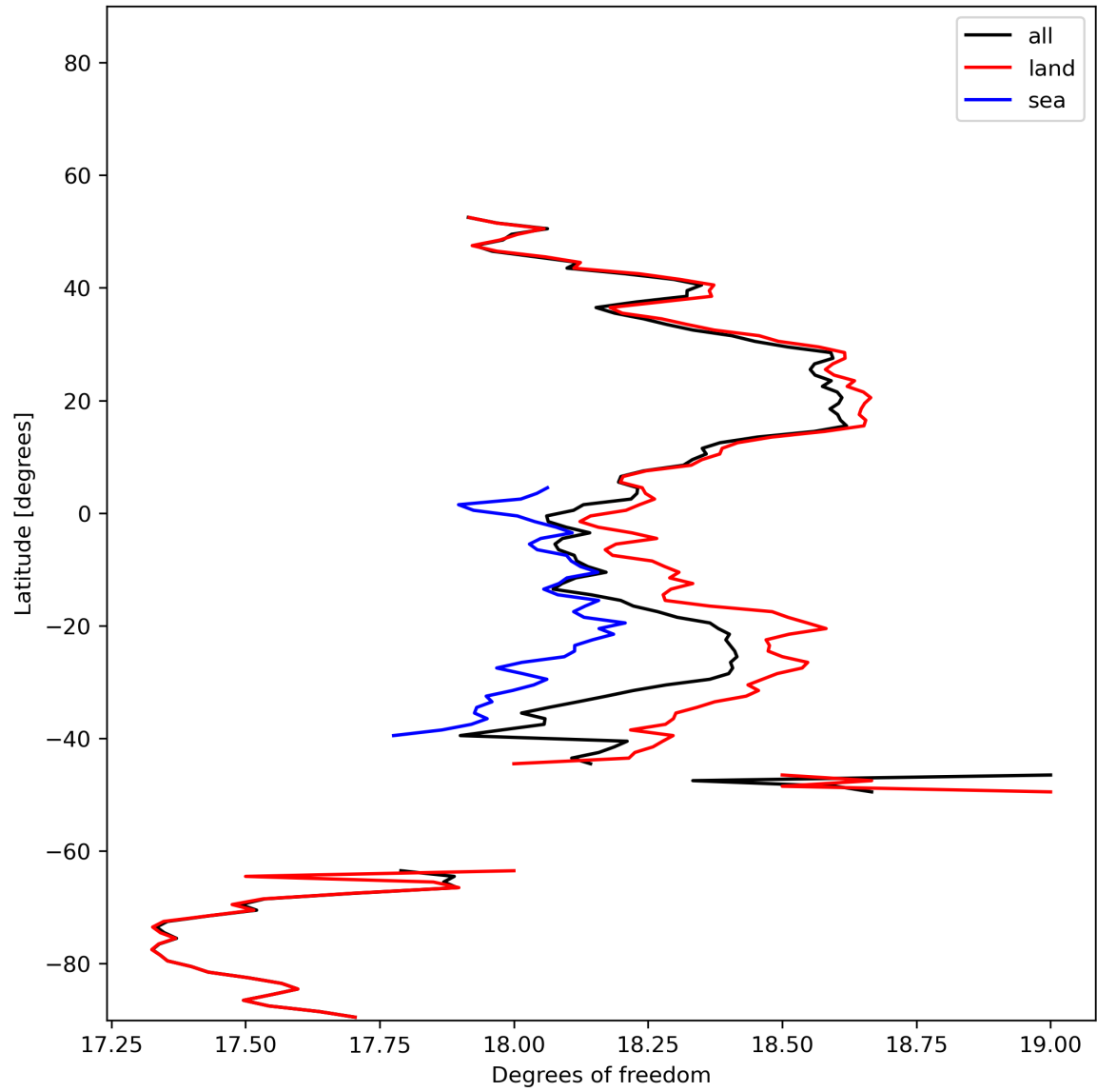
Figure 19: Zonal average of “Degrees of freedom” for 2024-01-03 to 2024-01-05.
