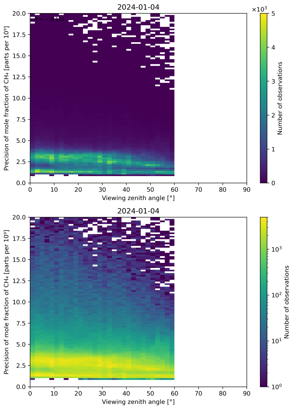
Figure 112: Scatter density plot of “Viewing zenith angle” against “Precision of mole fraction of CH 4 ” for 2024-01-03 to 2024-01-05.
