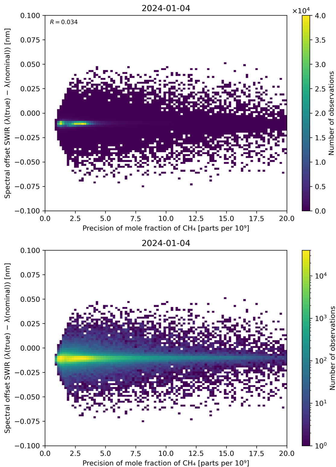
Figure 85: Scatter density plot of “Precision of mole fraction of \text{CH}_4 ” against “Spectral offset SWIR ( \lambda(\text{true}) - \lambda(\text{nominal}) )” for 2024-01-03 to 2024-01-05.
