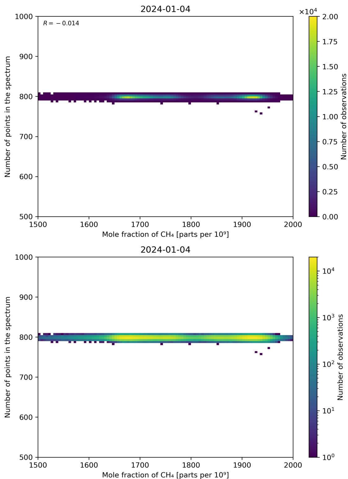
Figure 77: Scatter density plot of “Mole fraction of CH 4 ” against “Number of points in the spectrum” for 2024-01-03 to 2024-01-05.
