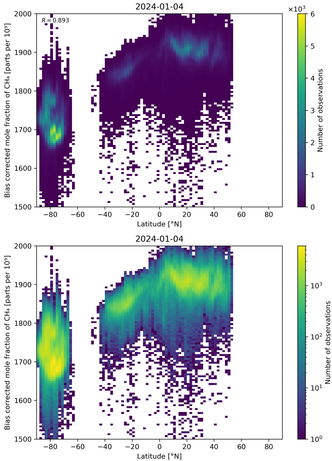
Figure 58: Scatter density plot of “Latitude” against “Bias corrected mole fraction of CH 4 ” for 2024-01-03 to 2024-01-05.
