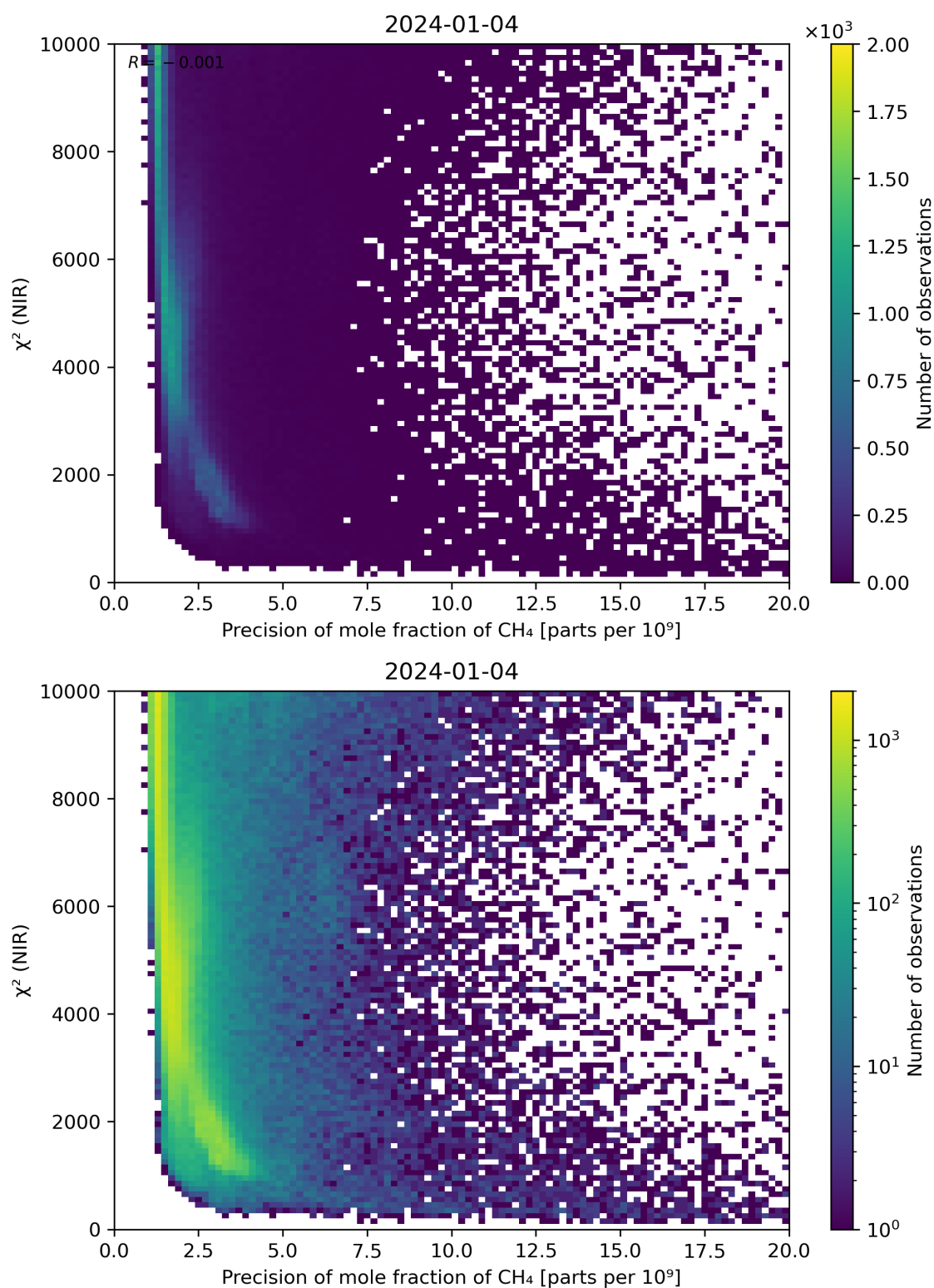
Figure 78: Scatter density plot of “Precision of mole fraction of CH 4 ” against “ \chi^2 (NIR)” for 2024-01-03 to 2024-01-05.
