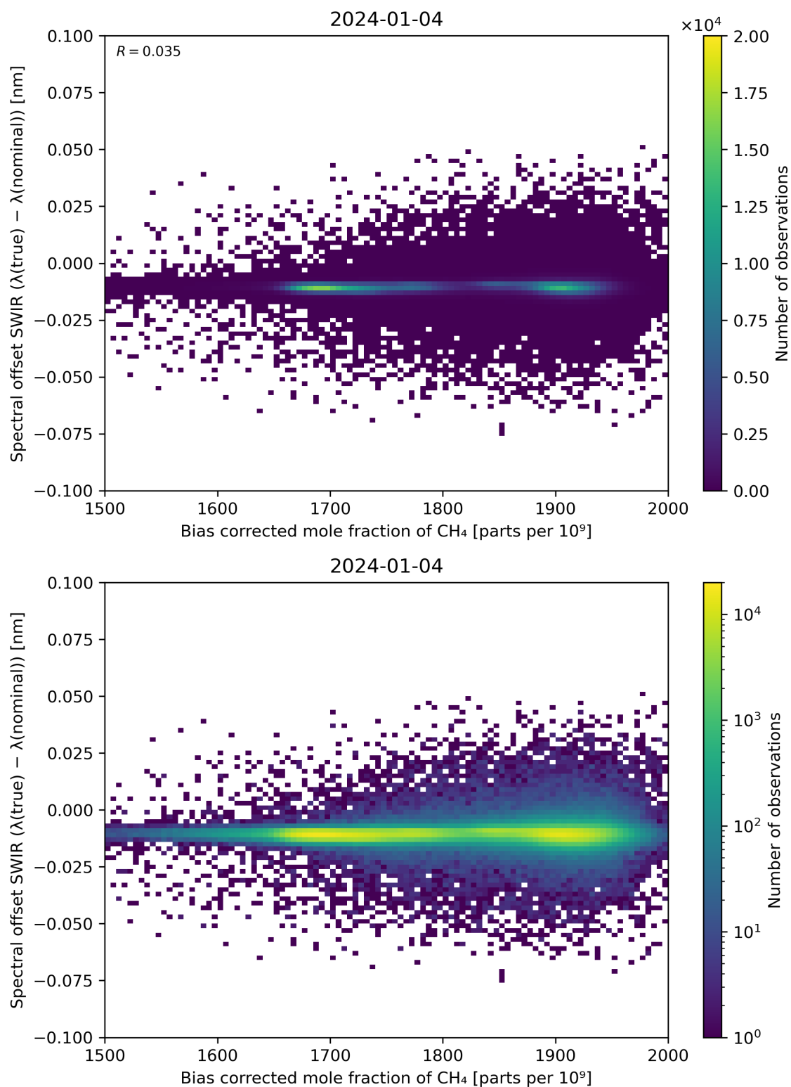
Figure 69: Scatter density plot of “Bias corrected mole fraction of \text{CH}_4 ” against “Spectral offset SWIR ( \lambda(\text{true}) - \lambda(\text{nominal}) )” for 2024-01-03 to 2024-01-05.
