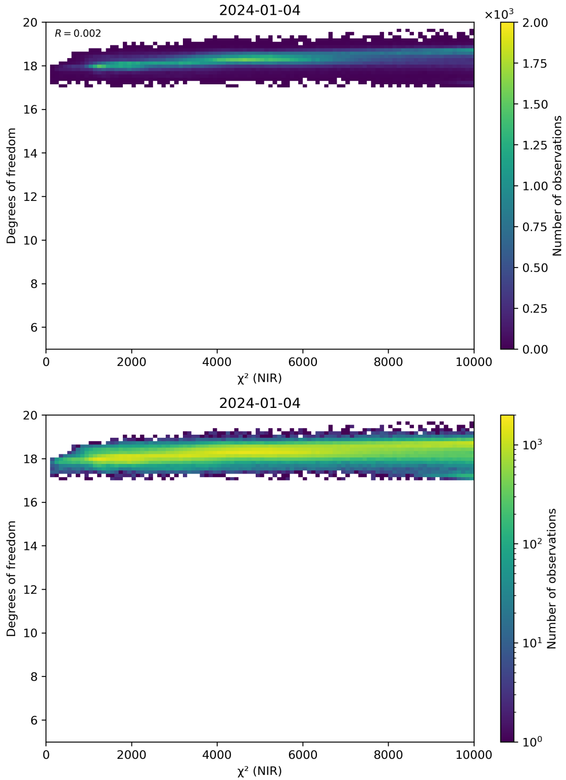
Figure 44: Scatter density plot of “ \chi^2 (NIR)” against “Degrees of freedom” for 2024-01-03 to 2024-01-05.
