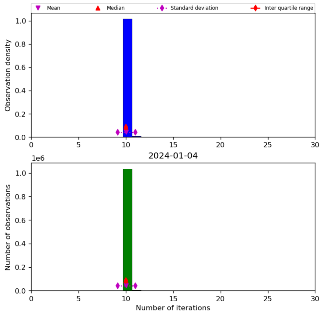
Figure 31: Histogram of “Number of iterations” for 2024-01-03 to 2024-01-05
