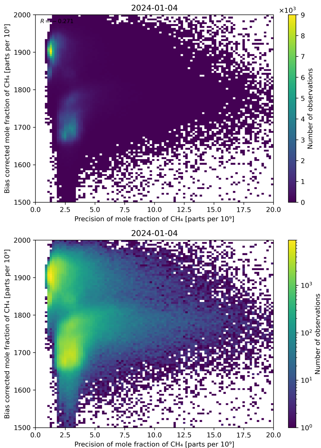
Figure 82: Scatter density plot of “Precision of mole fraction of CH 4 ” against “Bias corrected mole fraction of CH 4 ” for 2024-01-03 to 2024-01-05.
