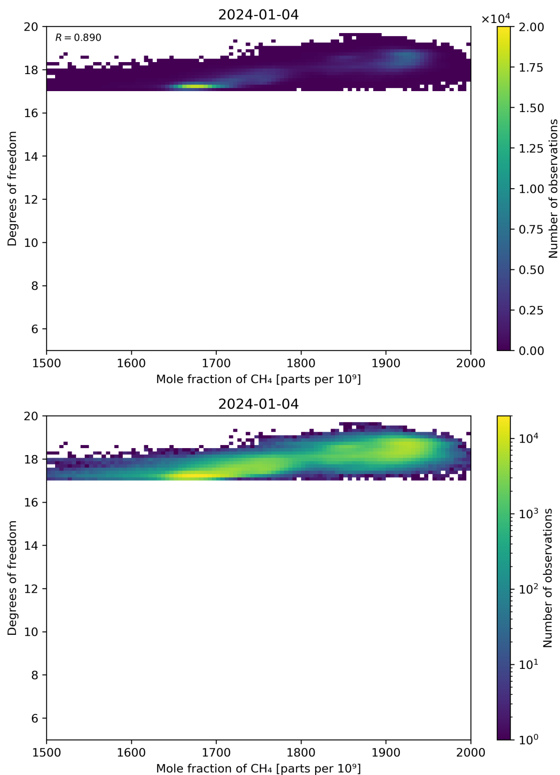
Figure 72: Scatter density plot of “Mole fraction of CH 4 ” against “Degrees of freedom” for 2024-01-03 to 2024-01-05.
