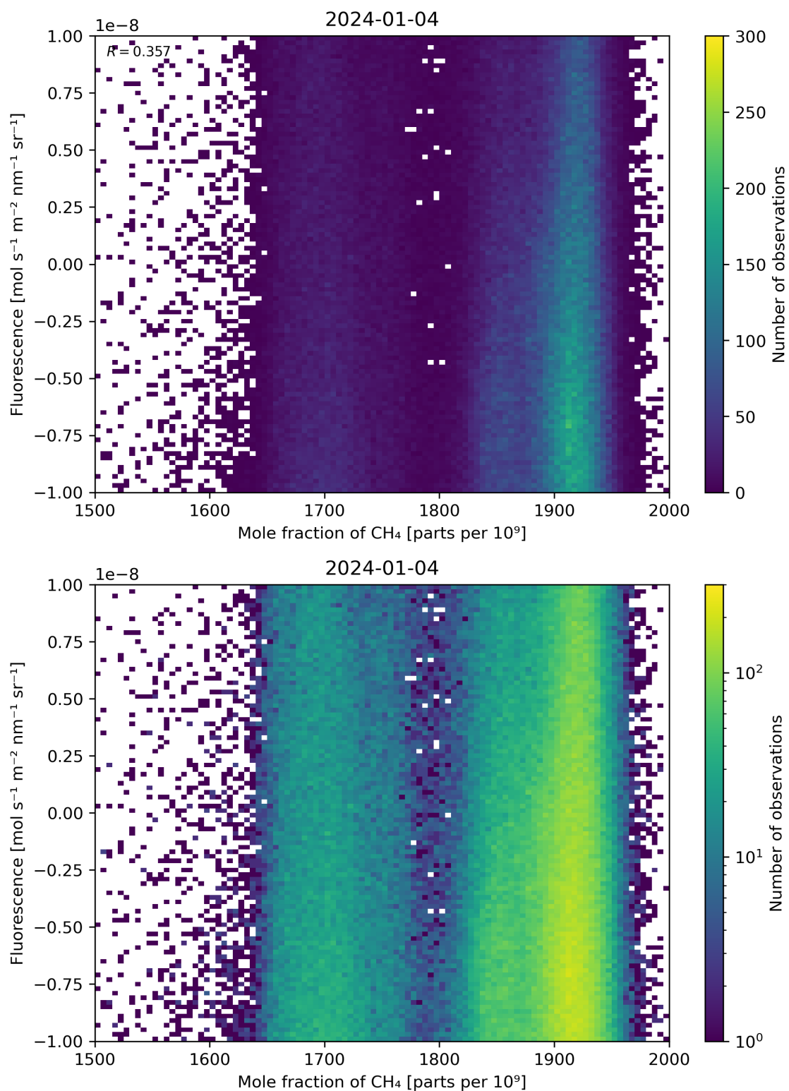
Figure 73: Scatter density plot of “Mole fraction of \text{CH}_4 ” against “Fluorescence” for 2024-01-03 to 2024-01-05.
