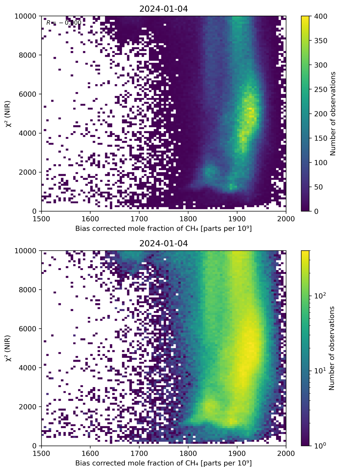
Figure 63: Scatter density plot of “Bias corrected mole fraction of CH 4 ” against “ \chi^2 (NIR)” for 2024-01-03 to 2024-01-05.
