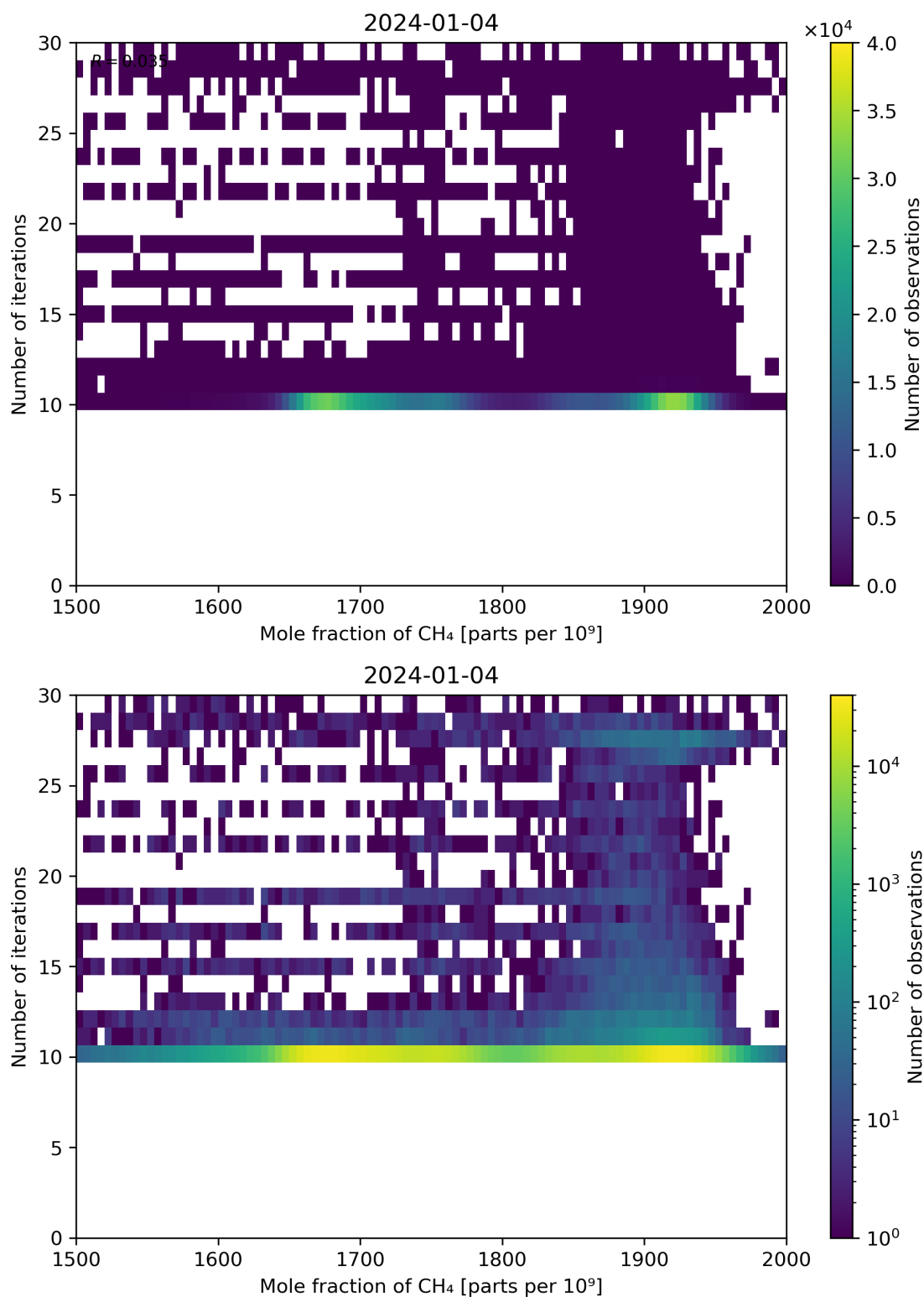
Figure 76: Scatter density plot of “Mole fraction of CH 4 ” against “Number of iterations” for 2024-01-03 to 2024-01-05.
