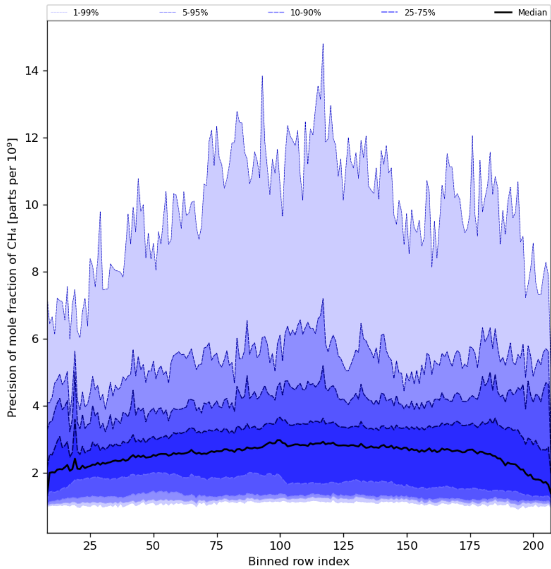
Figure 35: Along track statistics of “Precision of mole fraction of CH 4 ” for 2024-01-03 to 2024-01-05
