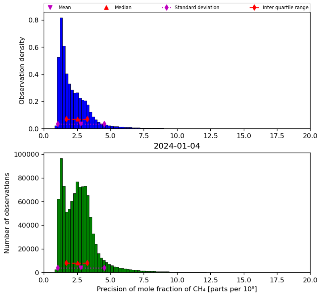
Figure 24: Histogram of “Precision of mole fraction of CH 4 ” for 2024-01-03 to 2024-01-05
