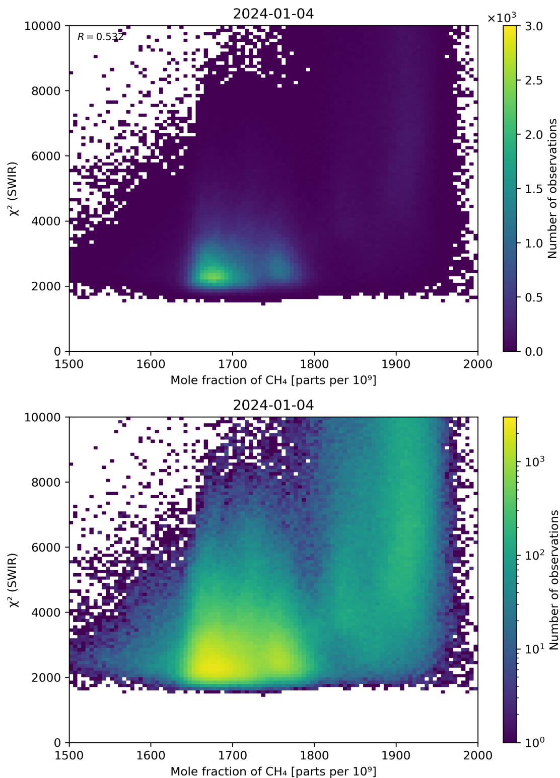
Figure 71: Scatter density plot of “Mole fraction of \text{CH}_4 ” against “ \chi^2 (SWIR)” for 2024-01-03 to 2024-01-05.
