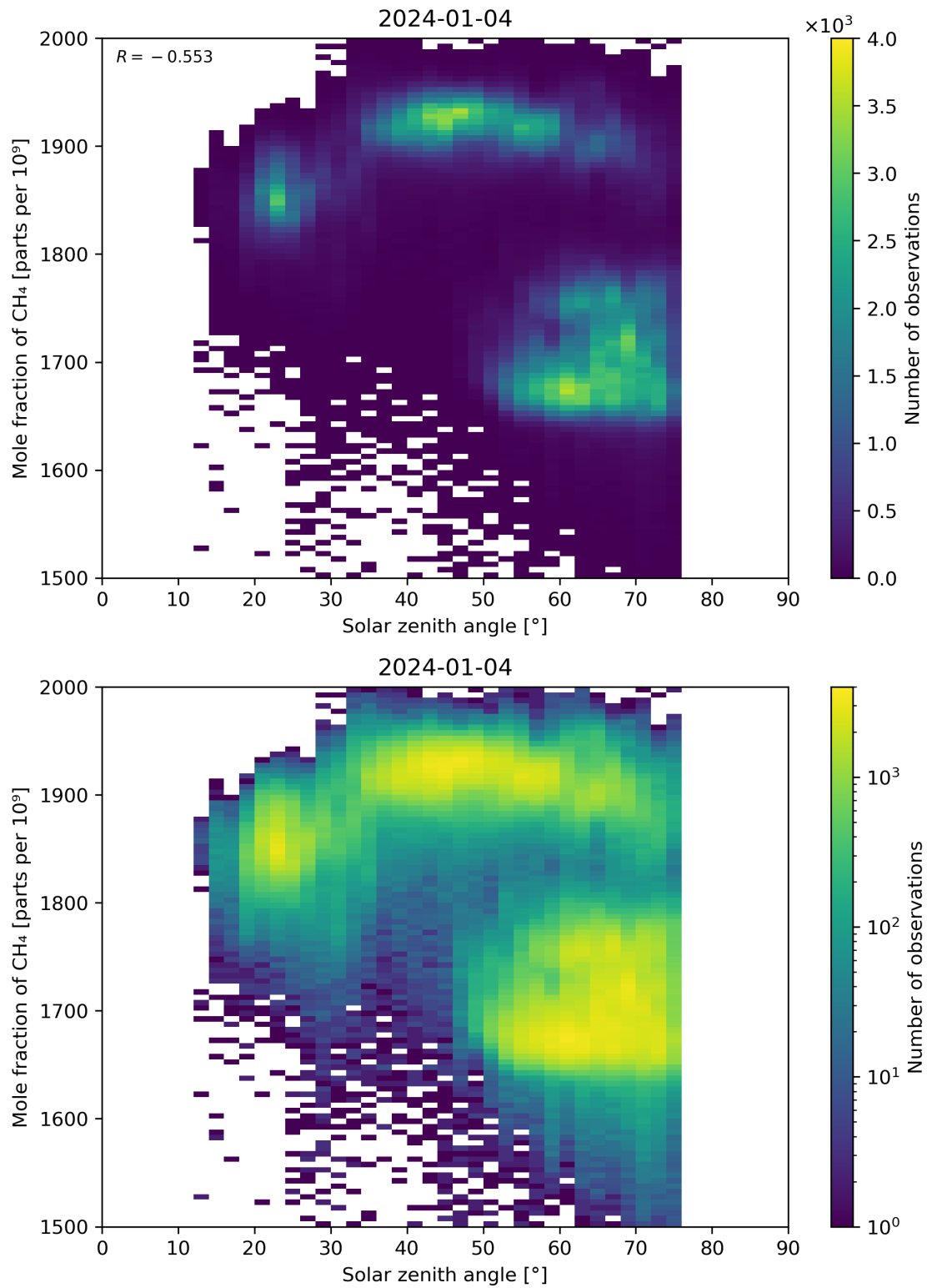
Figure 99: Scatter density plot of “Solar zenith angle” against “Mole fraction of \text{CH}_4 ” for 2024-01-03 to 2024-01-05.
