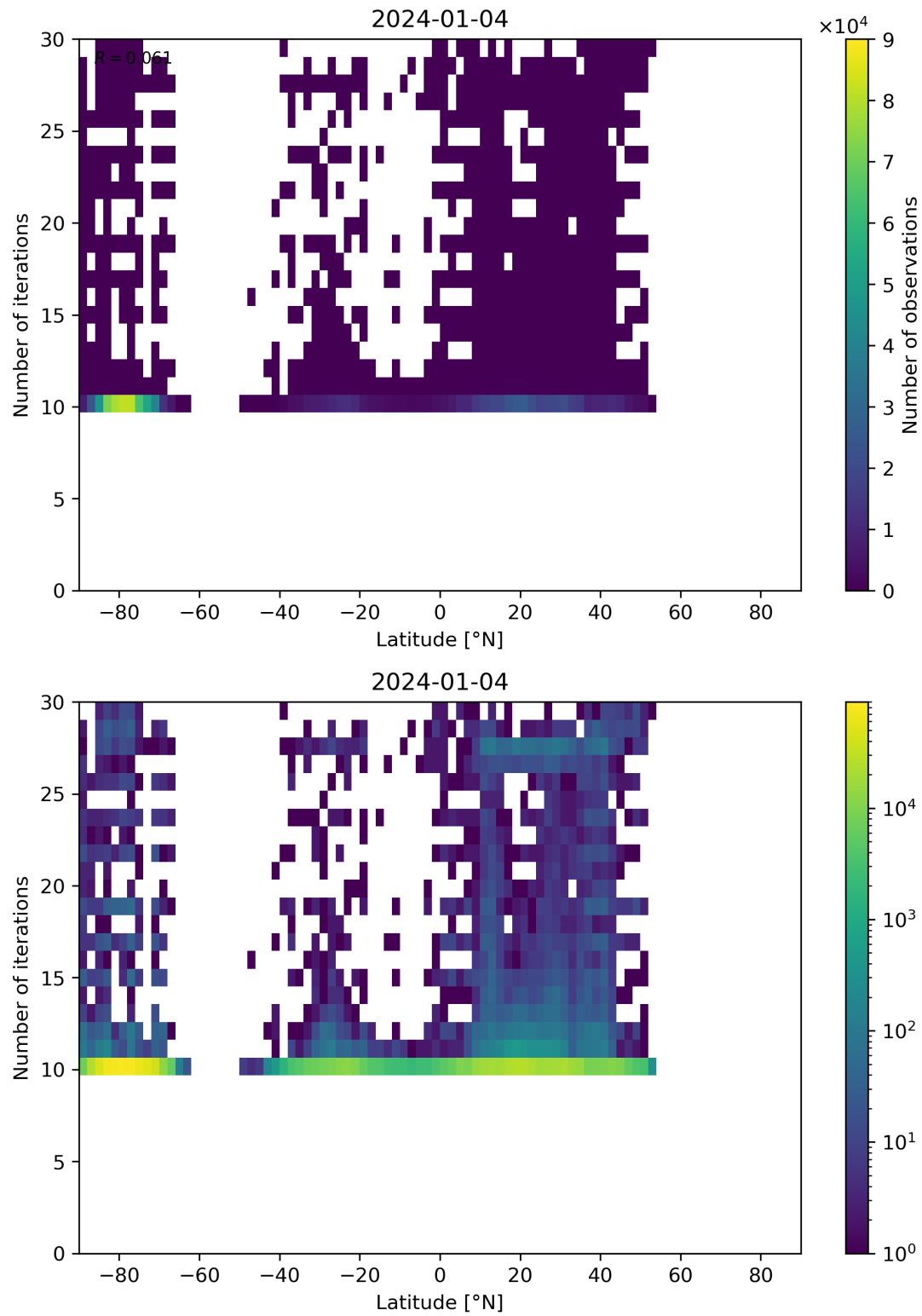
Figure 60: Scatter density plot of “Latitude” against “Number of iterations” for 2024-01-03 to 2024-01-05.
