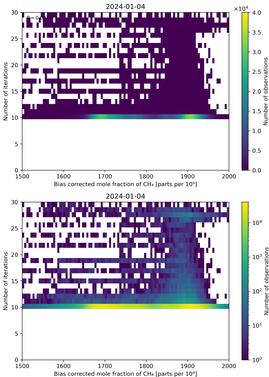
Figure 67: Scatter density plot of “Bias corrected mole fraction of \text{CH}_4 ” against “Number of iterations” for 2024-01-03 to 2024-01-05.
