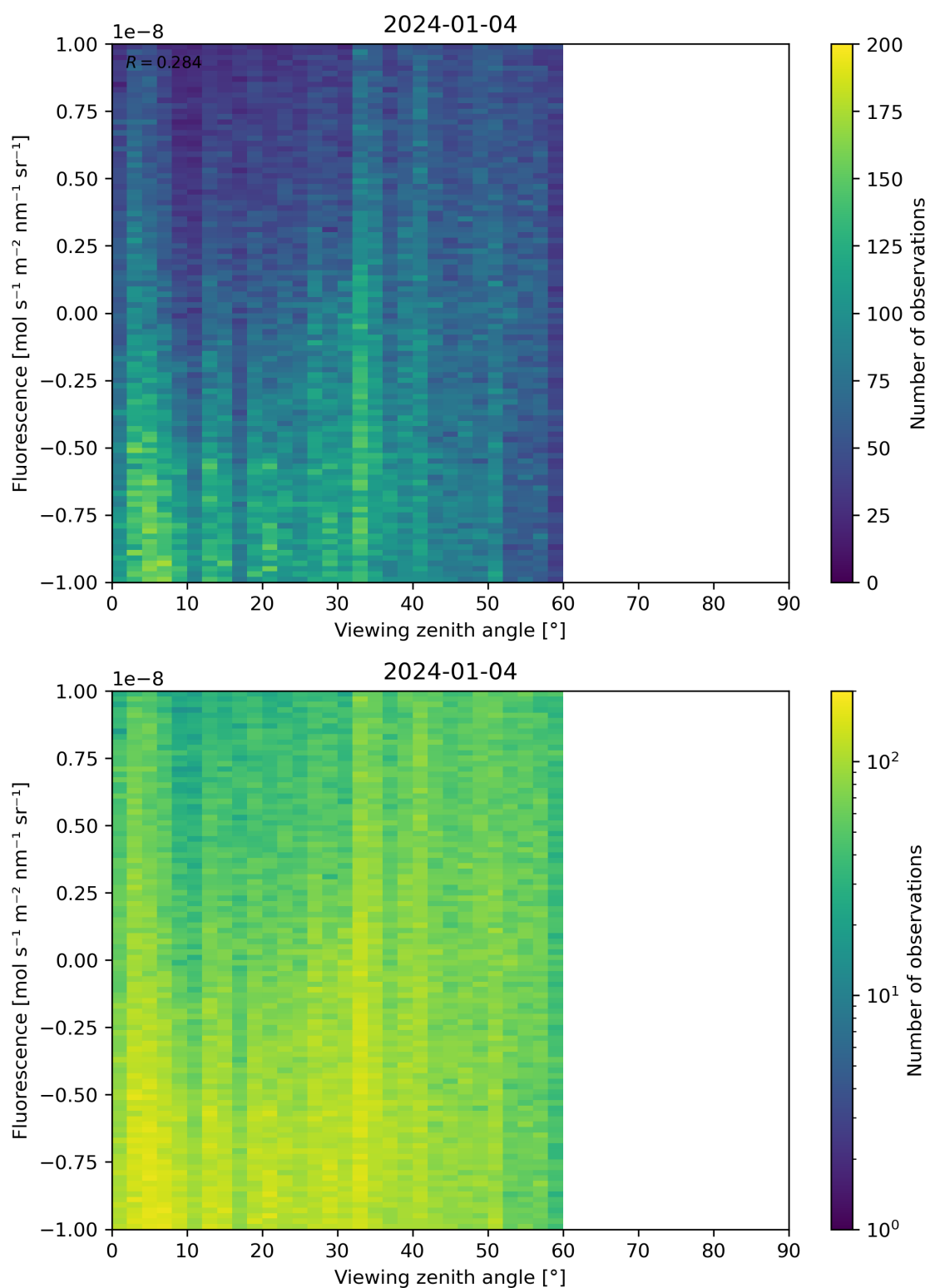
Figure 108: Scatter density plot of “Viewing zenith angle” against “Fluorescence” for 2024-01-03 to 2024-01-05.
