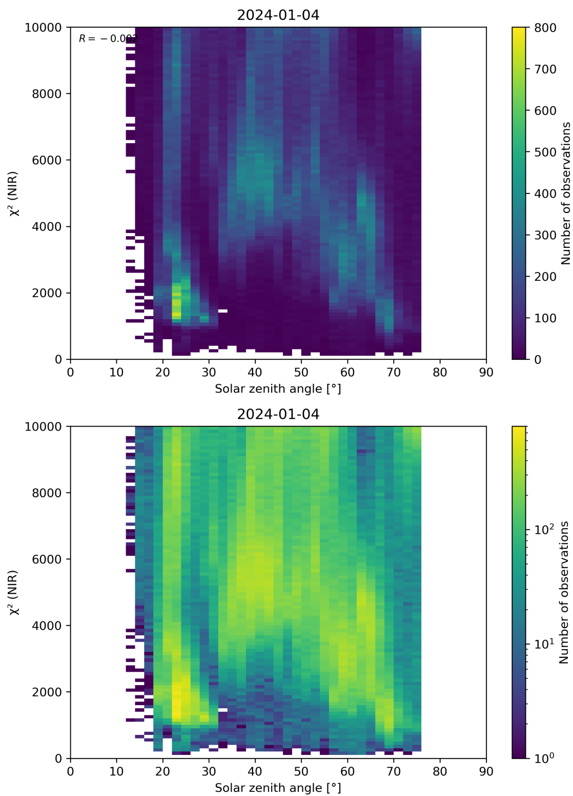
Figure 94: Scatter density plot of “Solar zenith angle” against “ \chi^2 (NIR)” for 2024-01-03 to 2024-01-05.
