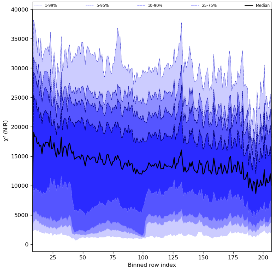
Figure 40: Along track statistics of “ \chi^2 (NIR)” for 2024-01-03 to 2024-01-05
