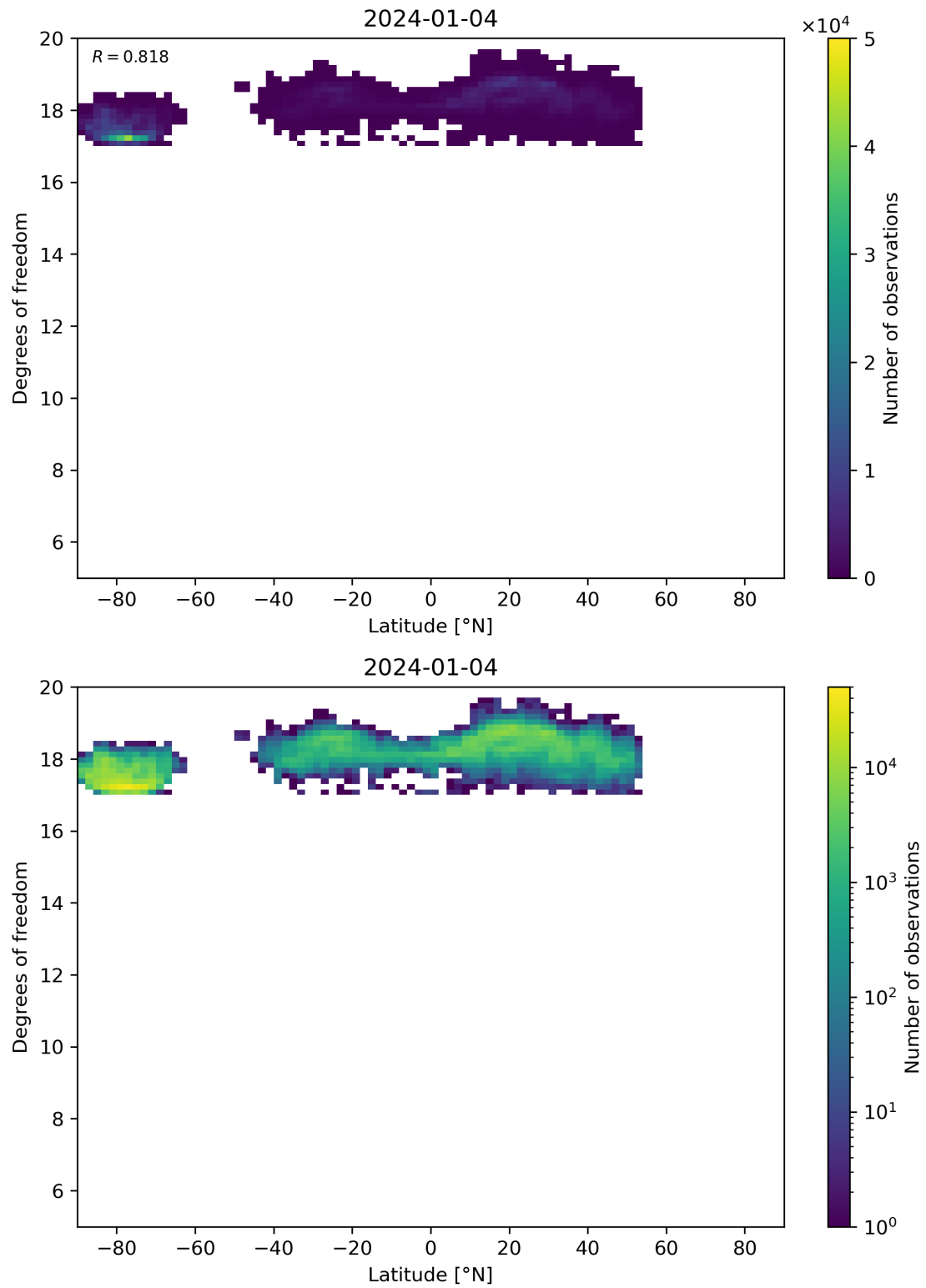
Figure 55: Scatter density plot of “Latitude” against “Degrees of freedom” for 2024-01-03 to 2024-01-05.
