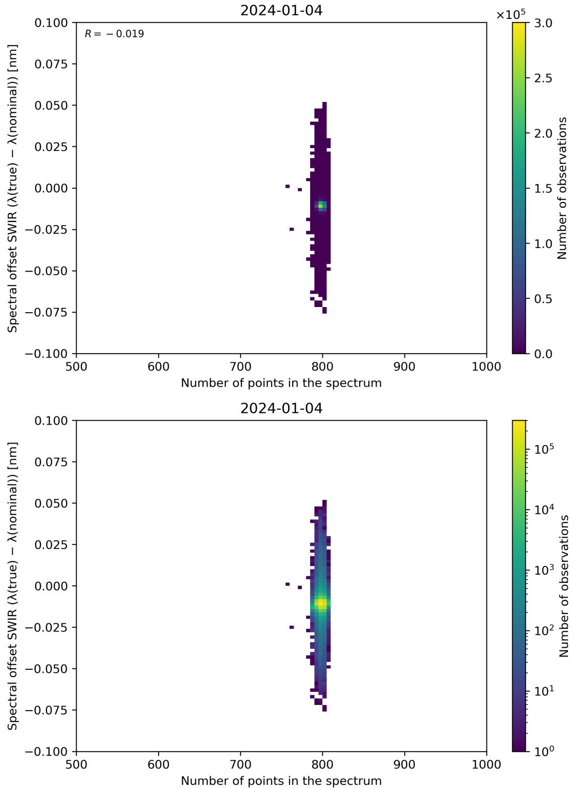
Figure 93: Scatter density plot of “Number of points in the spectrum” against “Spectral offset SWIR ( \lambda(\text{true}) - \lambda(\text{nominal}) )” for 2024-01-03 to 2024-01-05.
