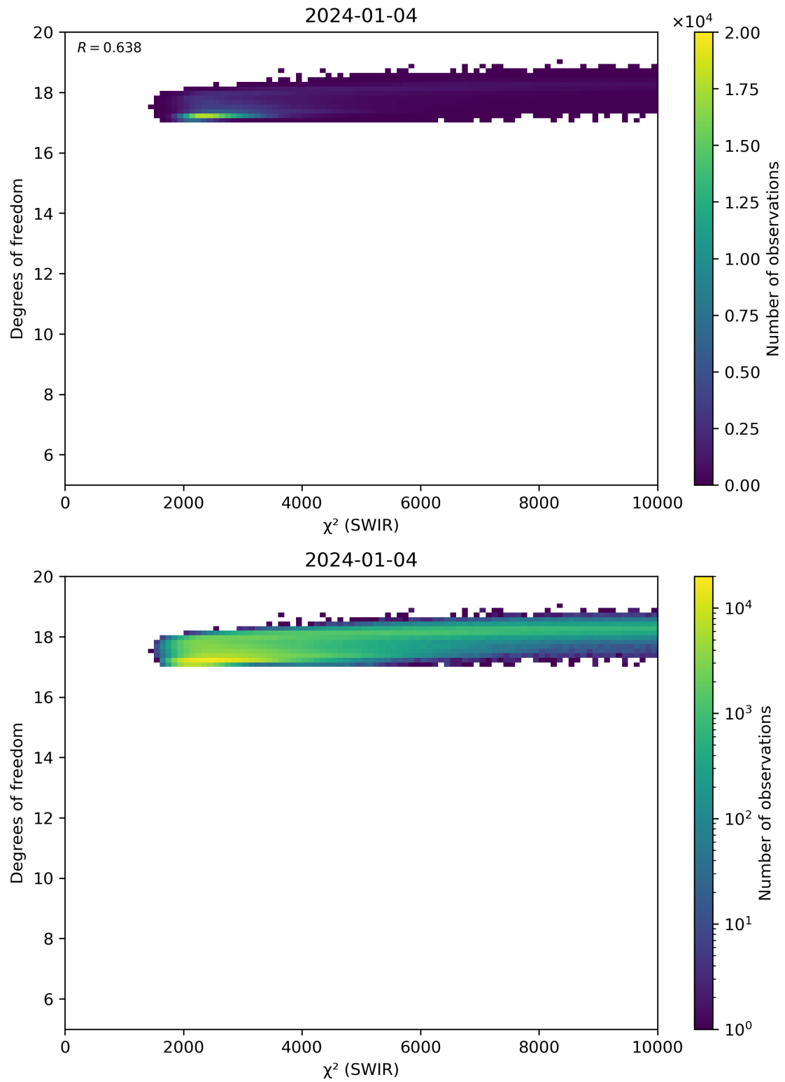
Figure 48: Scatter density plot of “ \chi^2 (SWIR)” against “Degrees of freedom” for 2024-01-03 to 2024-01-05.
