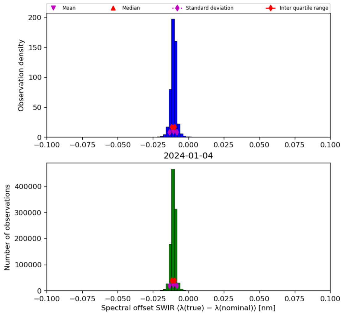
Figure 27: Histogram of “Spectral offset SWIR ( \lambda(\text{true}) - \lambda(\text{nominal}) )” for 2024-01-03 to 2024-01-05
