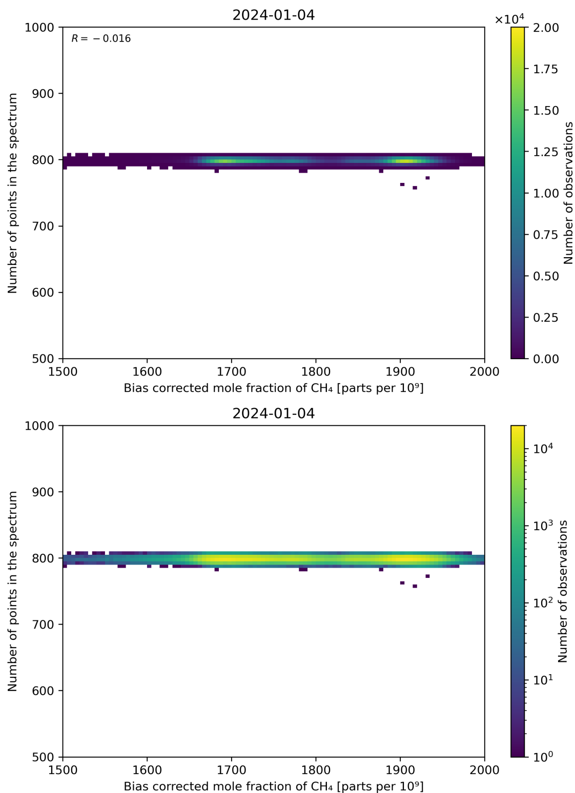
Figure 68: Scatter density plot of “Bias corrected mole fraction of CH 4 ” against “Number of points in the spectrum” for 2024-01-03 to 2024-01-05.
