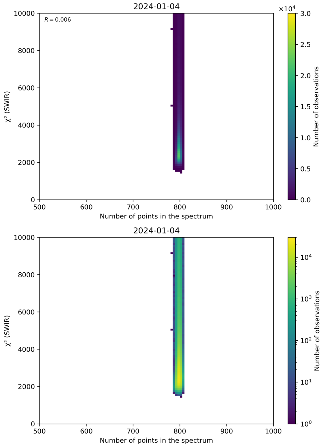
Figure 89: Scatter density plot of “Number of points in the spectrum” against “ \chi^2 (SWIR)” for 2024-01-03 to 2024-01-05.
