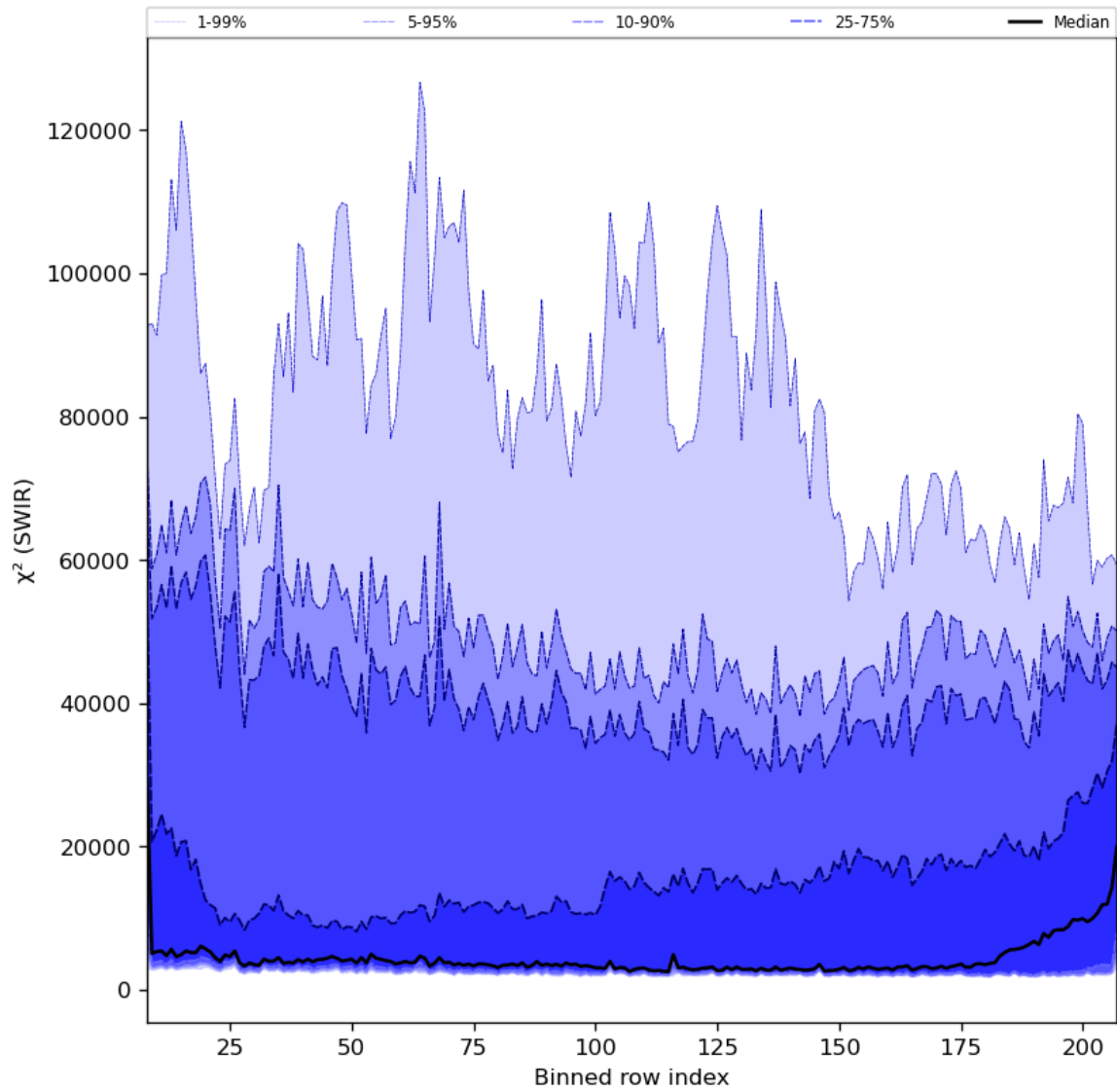
Figure 39: Along track statistics of " \chi^2 (SWIR)" for 2024-01-03 to 2024-01-05
