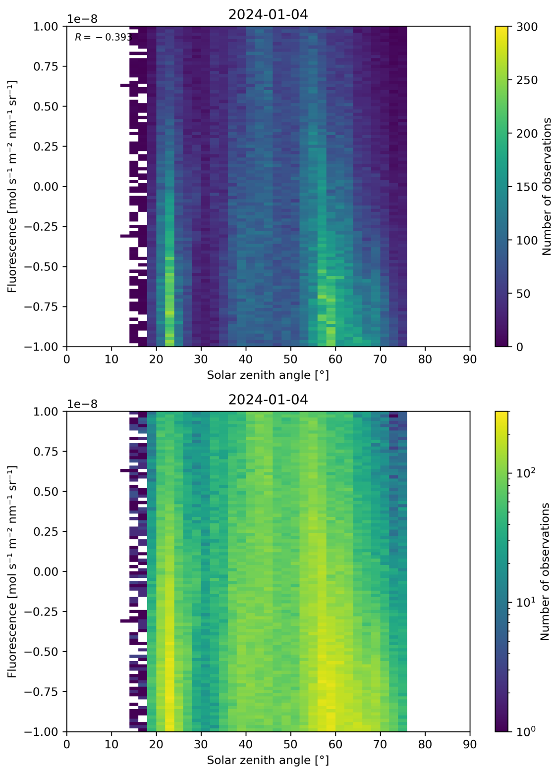
Figure 97: Scatter density plot of “Solar zenith angle” against “Fluorescence” for 2024-01-03 to 2024-01-05.
