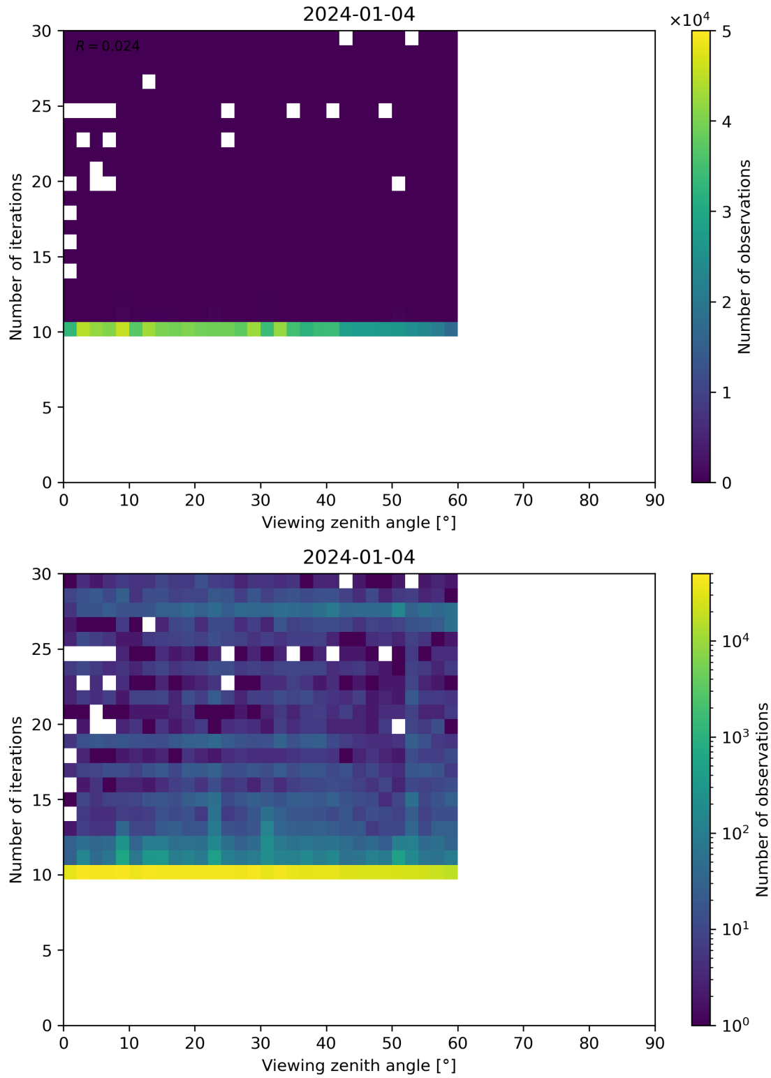
Figure 113: Scatter density plot of “Viewing zenith angle” against “Number of iterations” for 2024-01-03 to 2024-01-05.
