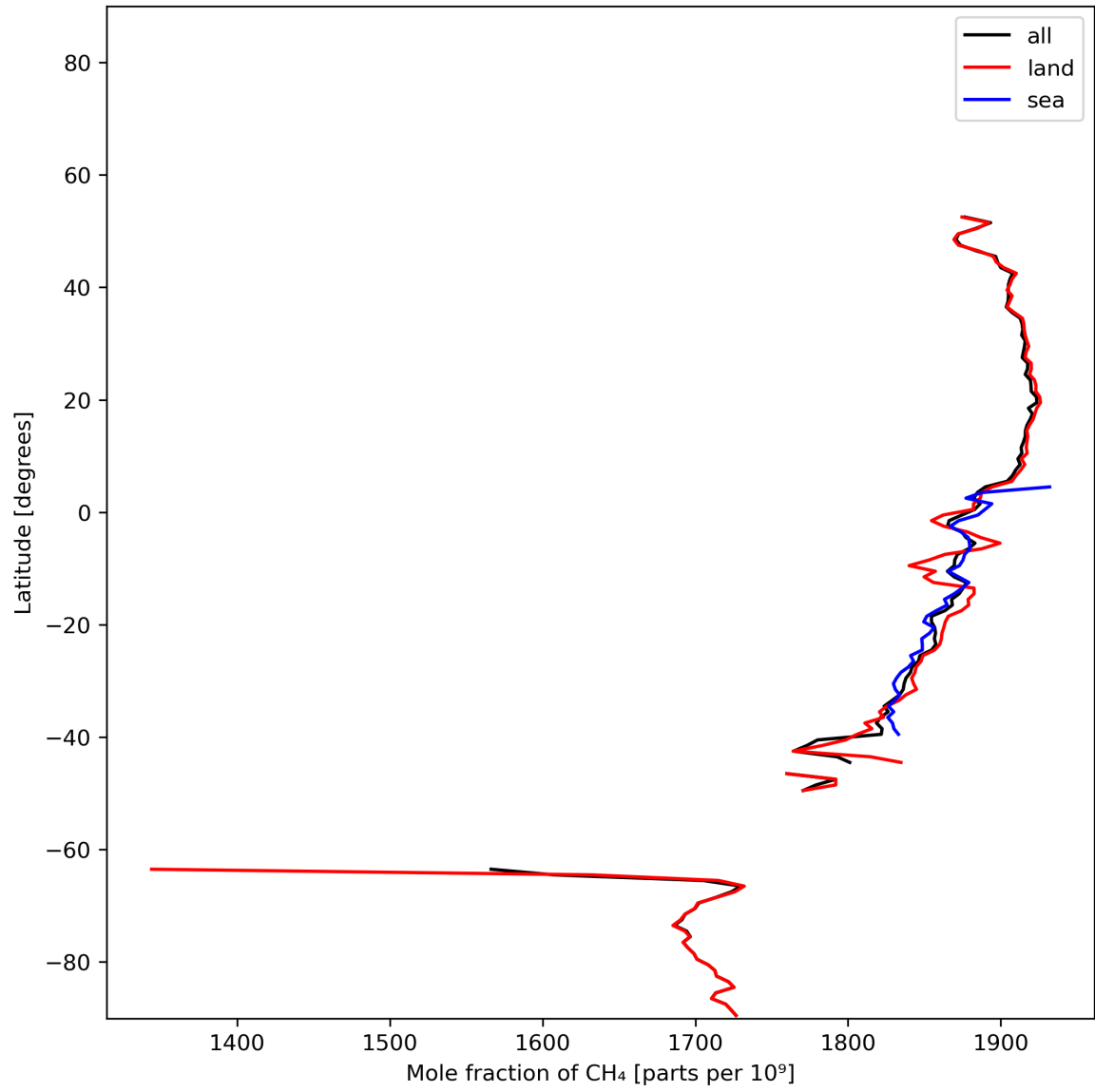
Figure 12: Zonal average of “Mole fraction of \text{CH}_4 ” for 2024-01-03 to 2024-01-05.
