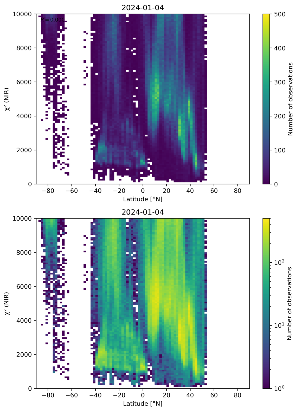
Figure 53: Scatter density plot of “Latitude” against “ \chi^2 (NIR)” for 2024-01-03 to 2024-01-05.
