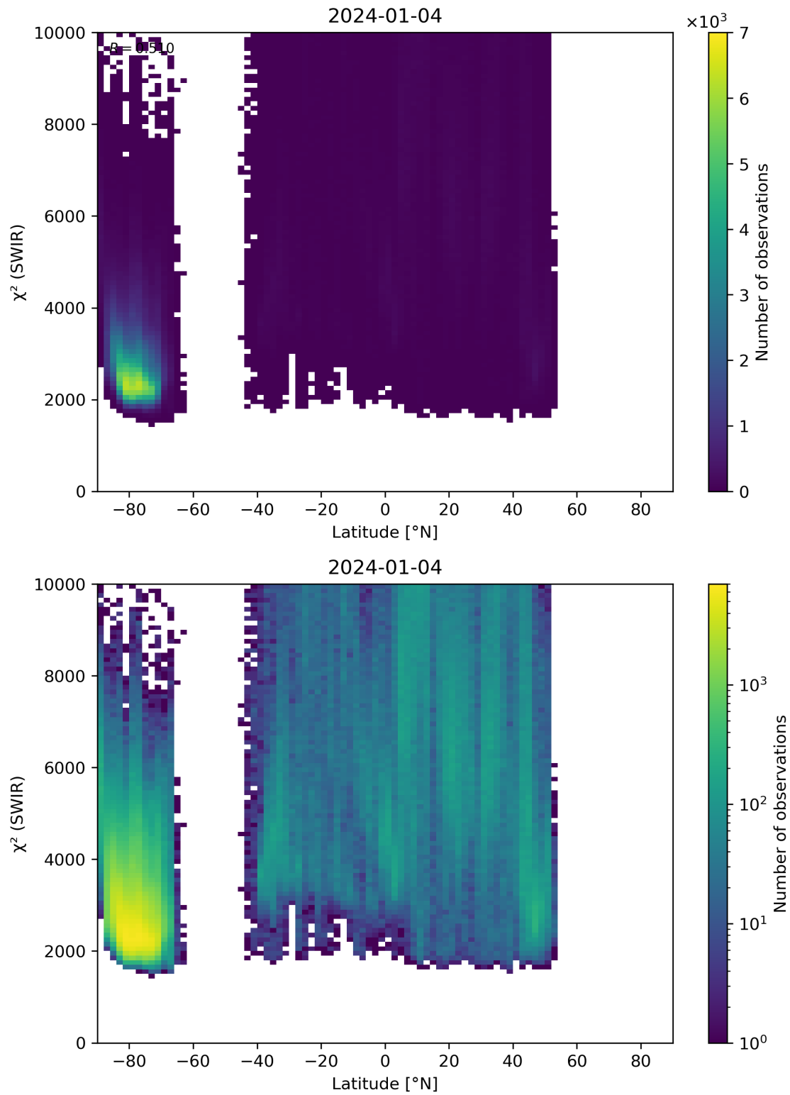
Figure 54: Scatter density plot of “Latitude” against “ \chi^2 (SWIR)” for 2024-01-03 to 2024-01-05.
