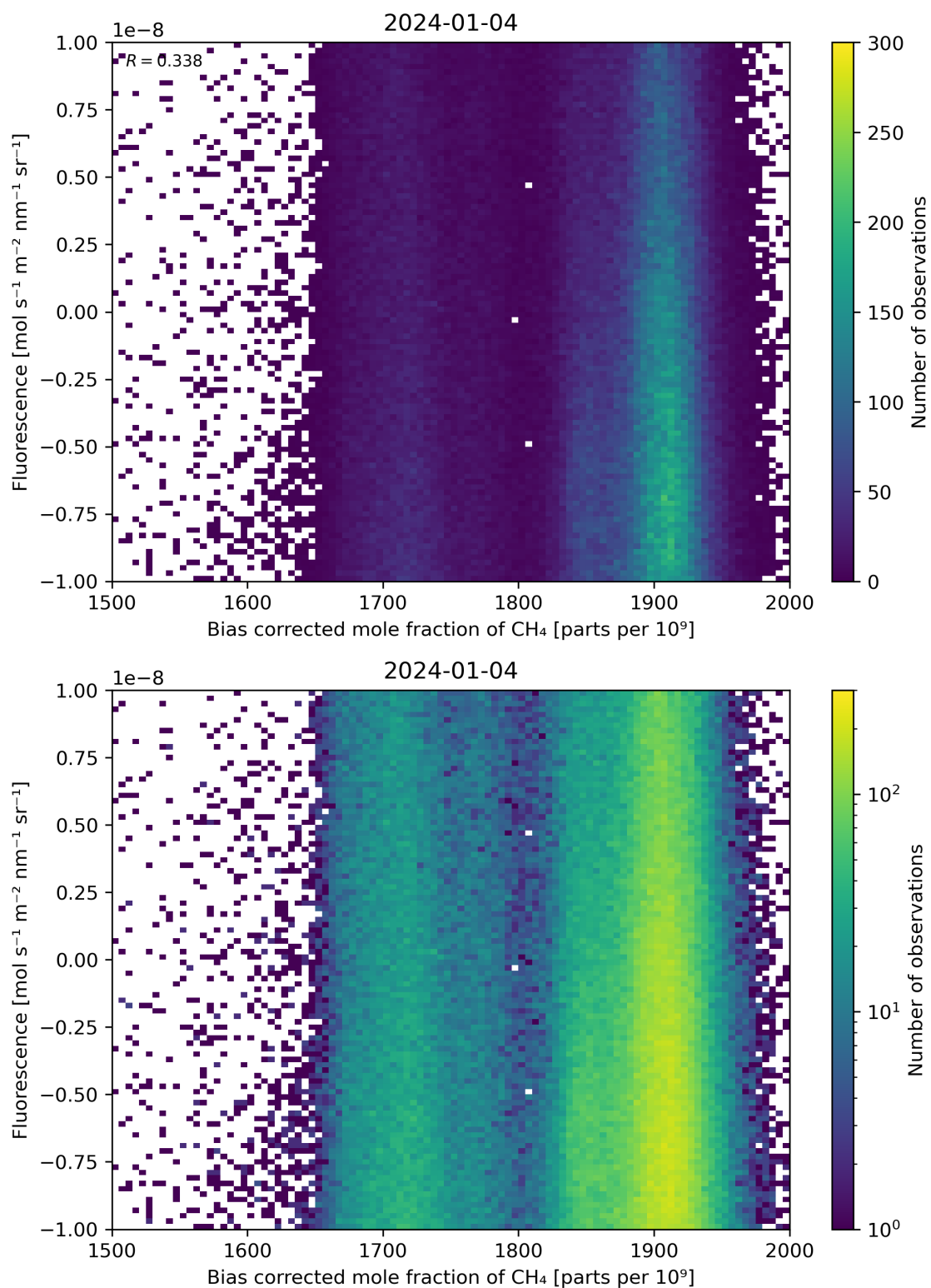
Figure 66: Scatter density plot of “Bias corrected mole fraction of \text{CH}_4 ” against “Fluorescence” for 2024-01-03 to 2024-01-05.
