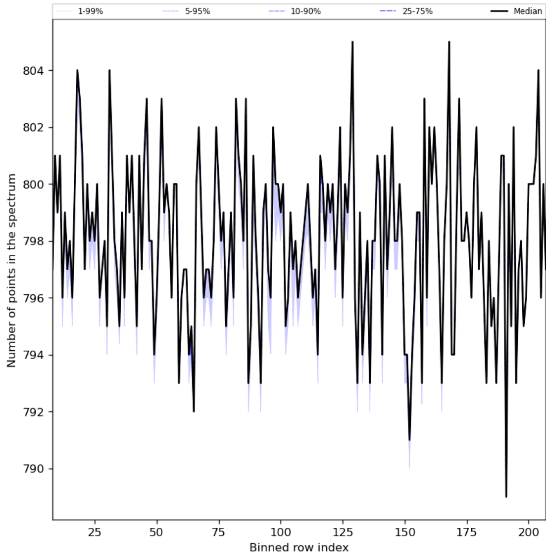
Figure 37: Along track statistics of “Number of points in the spectrum” for 2024-01-03 to 2024-01-05
