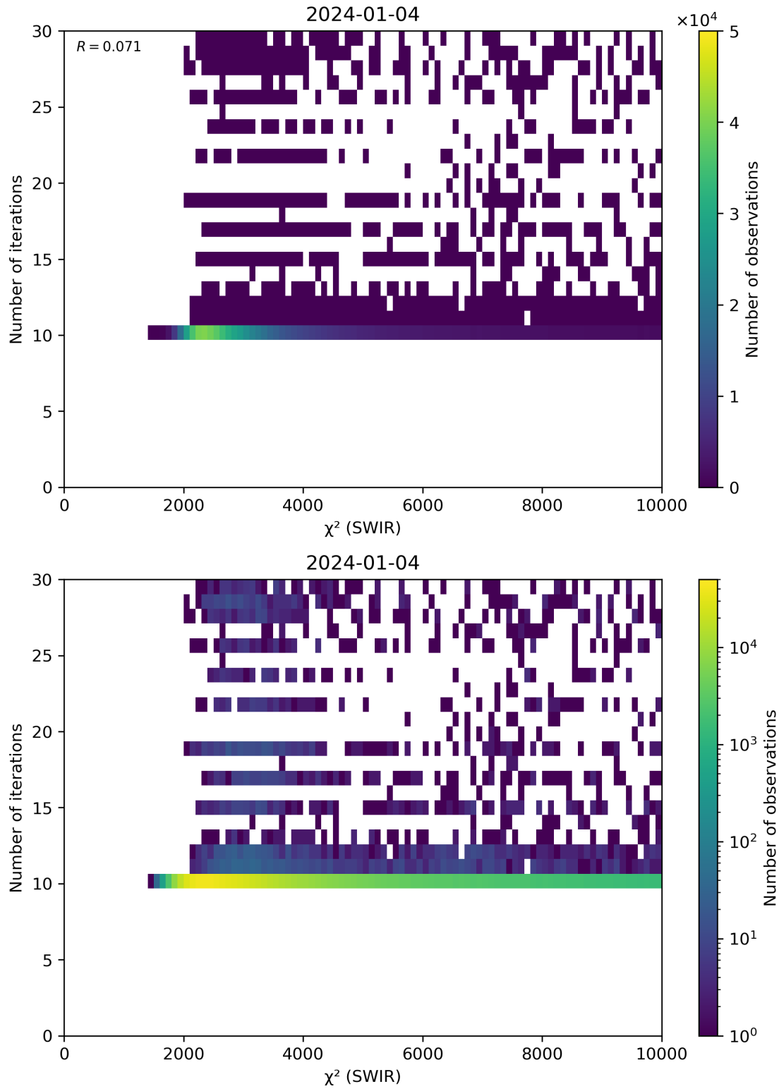
Figure 50: Scatter density plot of “ \chi^2 (SWIR)” against “Number of iterations” for 2024-01-03 to 2024-01-05.
