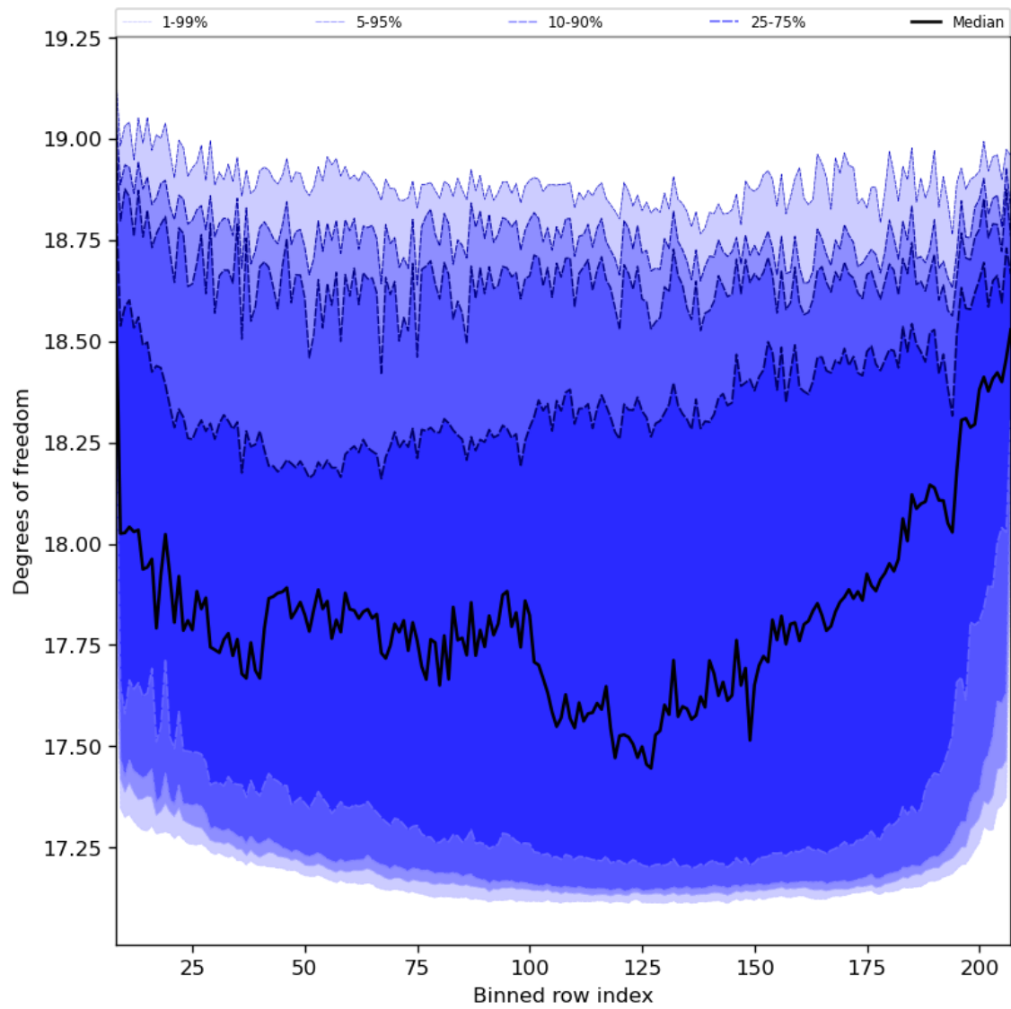
Figure 41: Along track statistics of “Degrees of freedom” for 2024-01-03 to 2024-01-05
