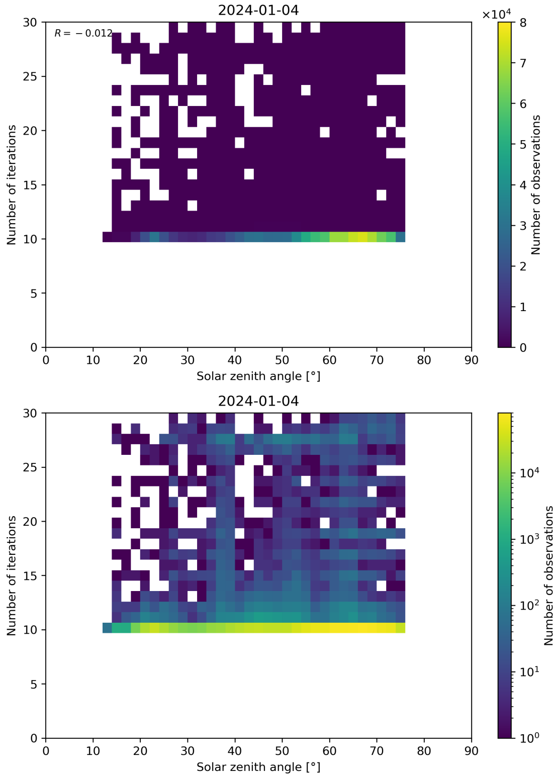
Figure 102: Scatter density plot of “Solar zenith angle” against “Number of iterations” for 2024-01-03 to 2024-01-05.
