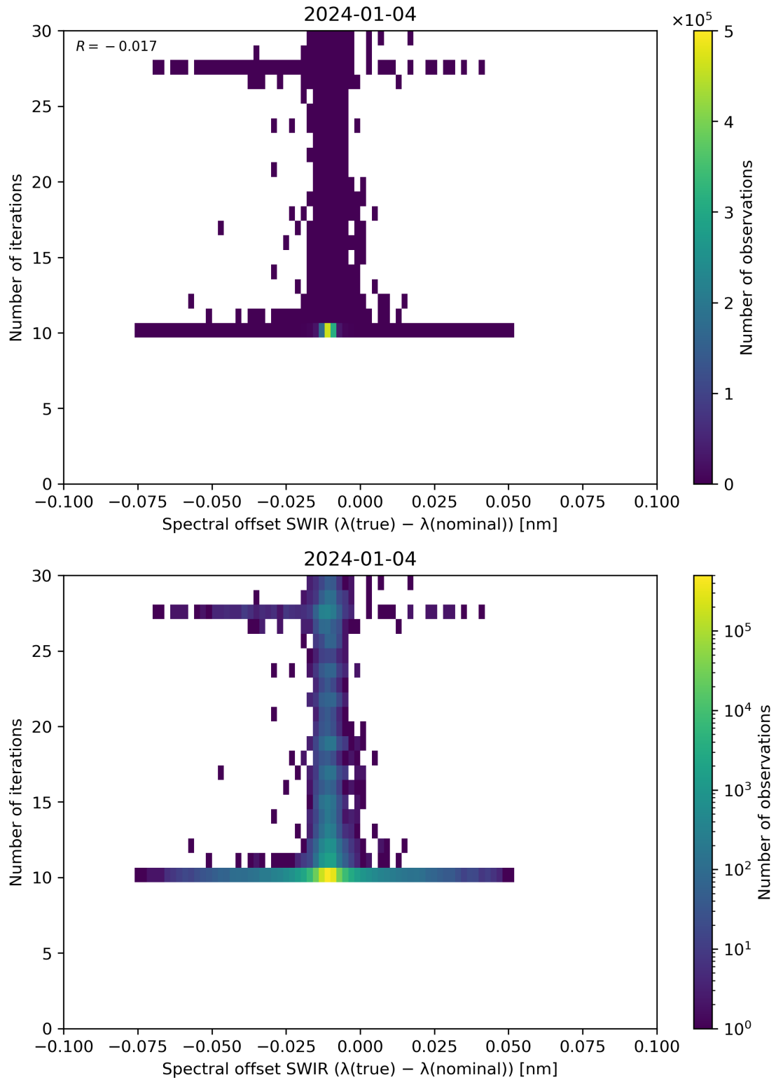
Figure 121: Scatter density plot of “Spectral offset SWIR ( \lambda(\text{true}) - \lambda(\text{nominal}) )” against “Number of iterations” for 2024-01-03 to 2024-01-05.
