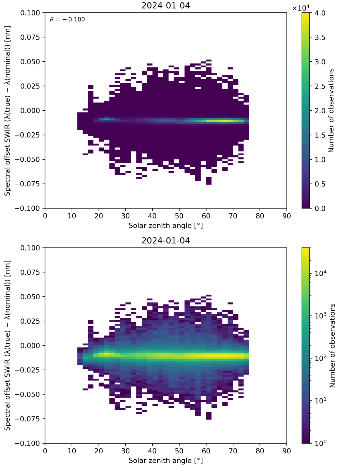
Figure 104: Scatter density plot of “Solar zenith angle” against “Spectral offset SWIR ( \lambda(\text{true}) - \lambda(\text{nominal}) )” for 2024-01-03 to 2024-01-05.
