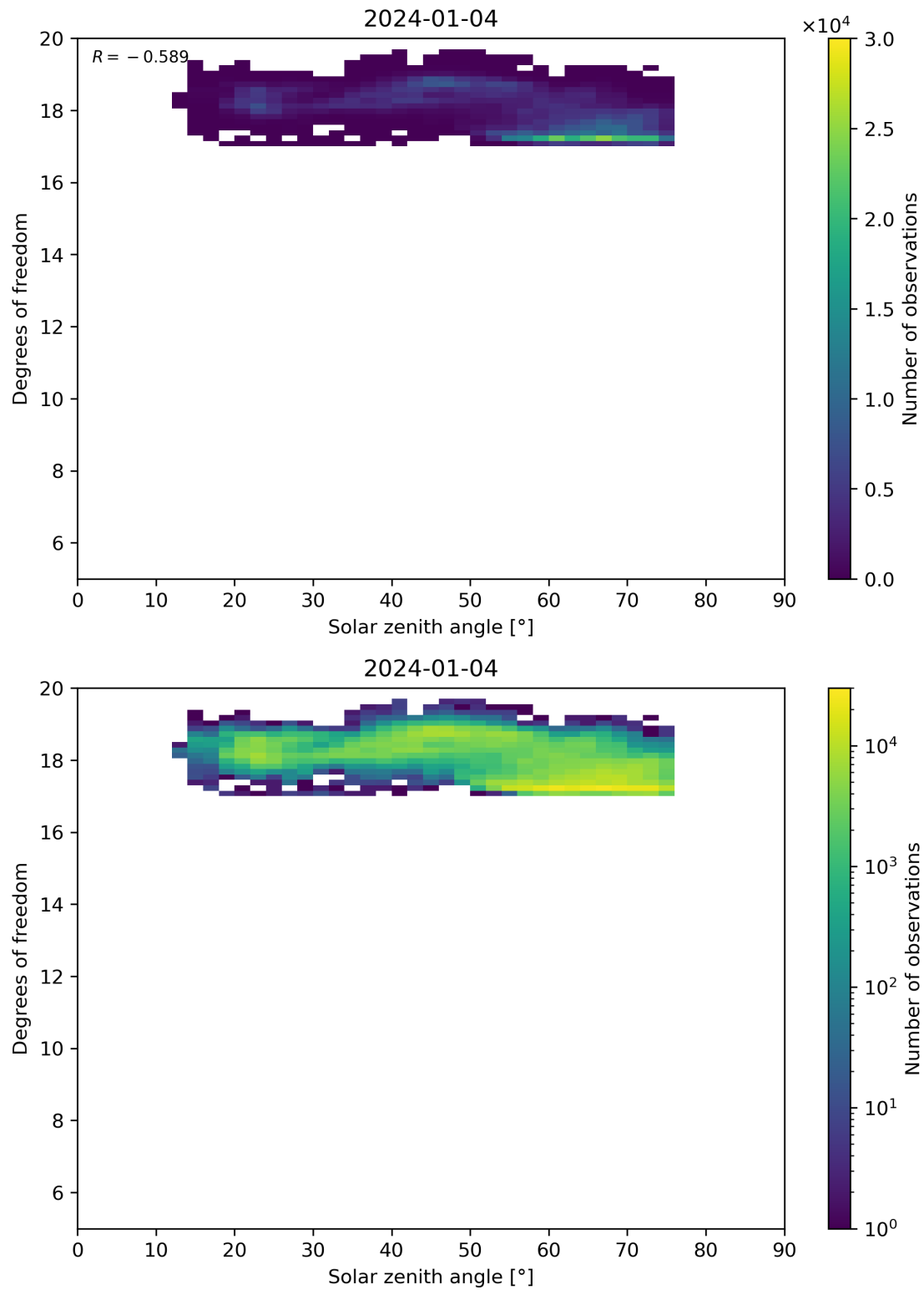
Figure 96: Scatter density plot of “Solar zenith angle” against “Degrees of freedom” for 2024-01-03 to 2024-01-05.
