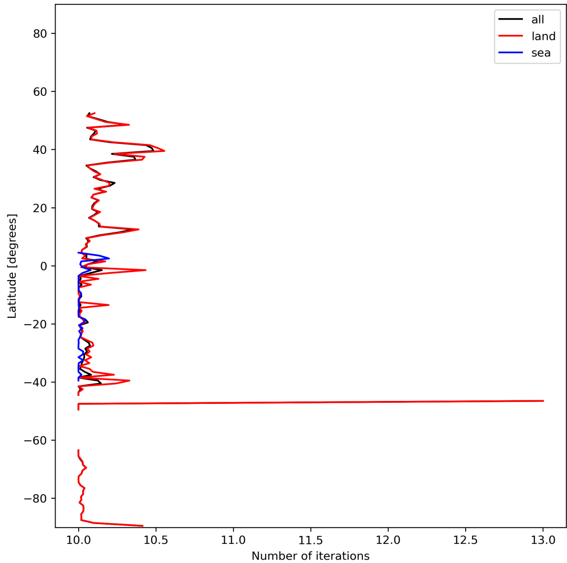
Figure 20: Zonal average of “Number of iterations” for 2024-01-03 to 2024-01-05.
