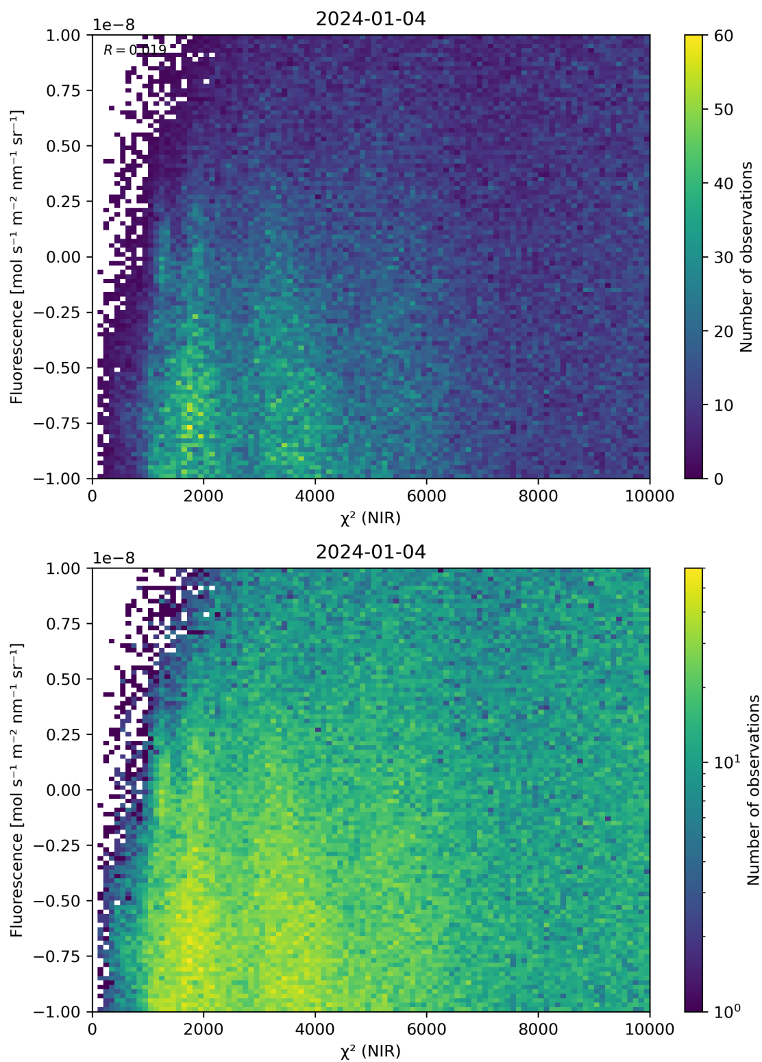
Figure 45: Scatter density plot of “ \chi^2 (NIR)” against “Fluorescence” for 2024-01-03 to 2024-01-05.
