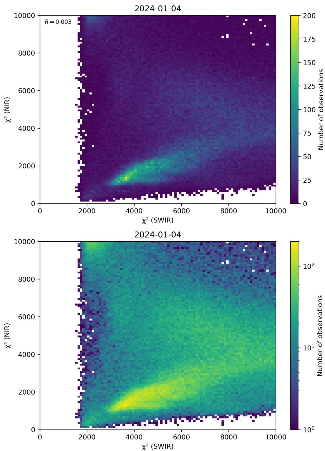
Figure 47: Scatter density plot of “ \chi^2 (SWIR)” against “ \chi^2 (NIR)” for 2024-01-03 to 2024-01-05.
