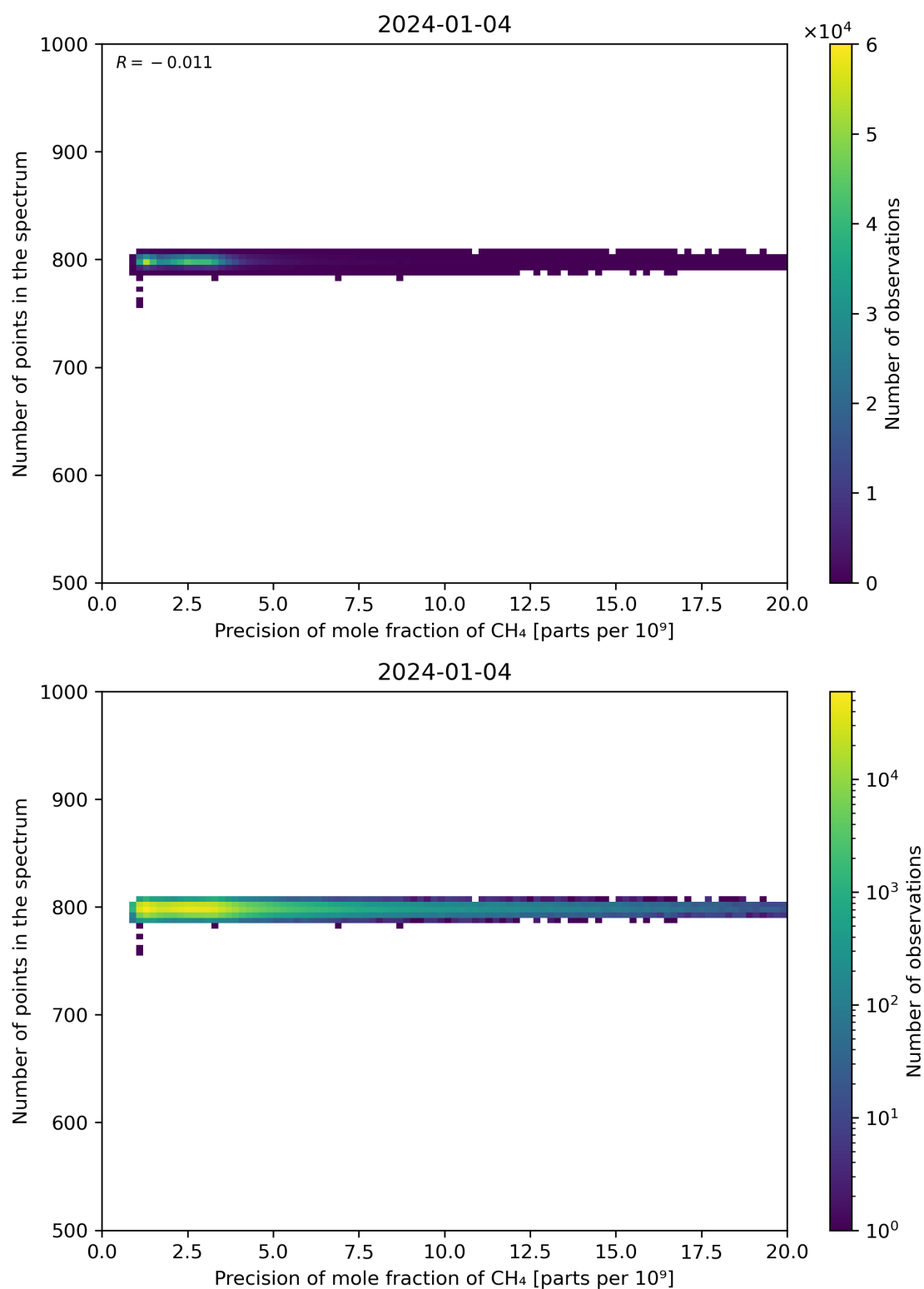
Figure 84: Scatter density plot of “Precision of mole fraction of CH 4 ” against “Number of points in the spectrum” for 2024-01-03 to 2024-01-05.
