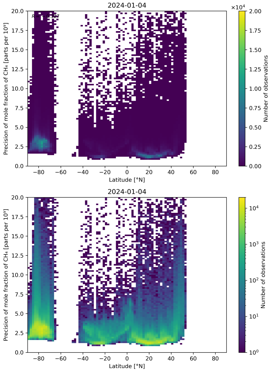
Figure 59: Scatter density plot of “Latitude” against “Precision of mole fraction of CH 4 ” for 2024-01-03 to 2024-01-05.
