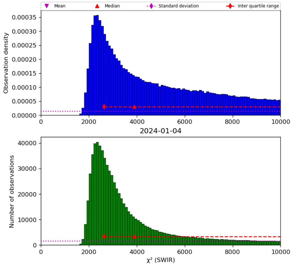
Figure 28: Histogram of “ \chi^2 (SWIR)” for 2024-01-03 to 2024-01-05
