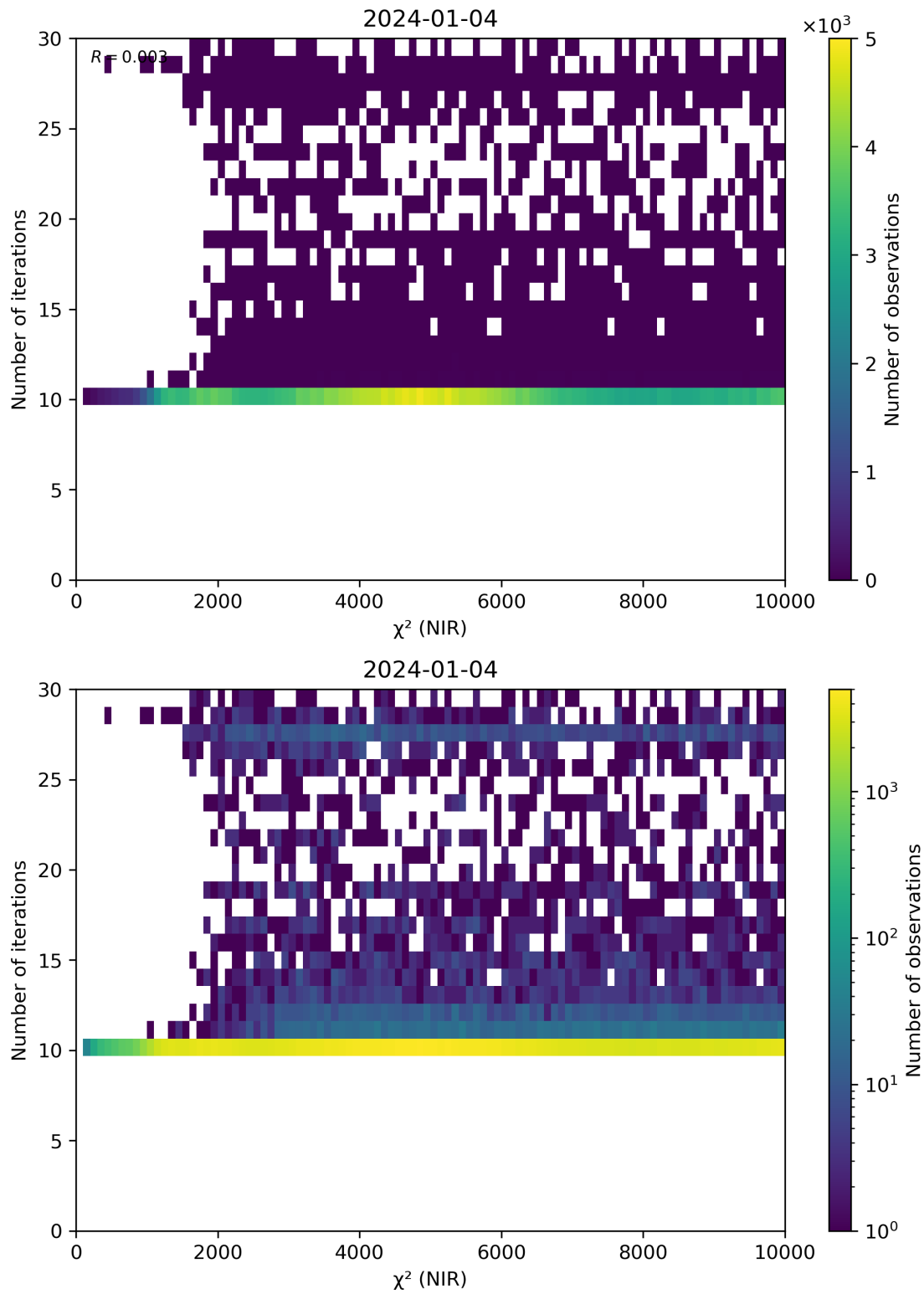
Figure 46: Scatter density plot of “ \chi^2 (NIR)” against “Number of iterations” for 2024-01-03 to 2024-01-05.
