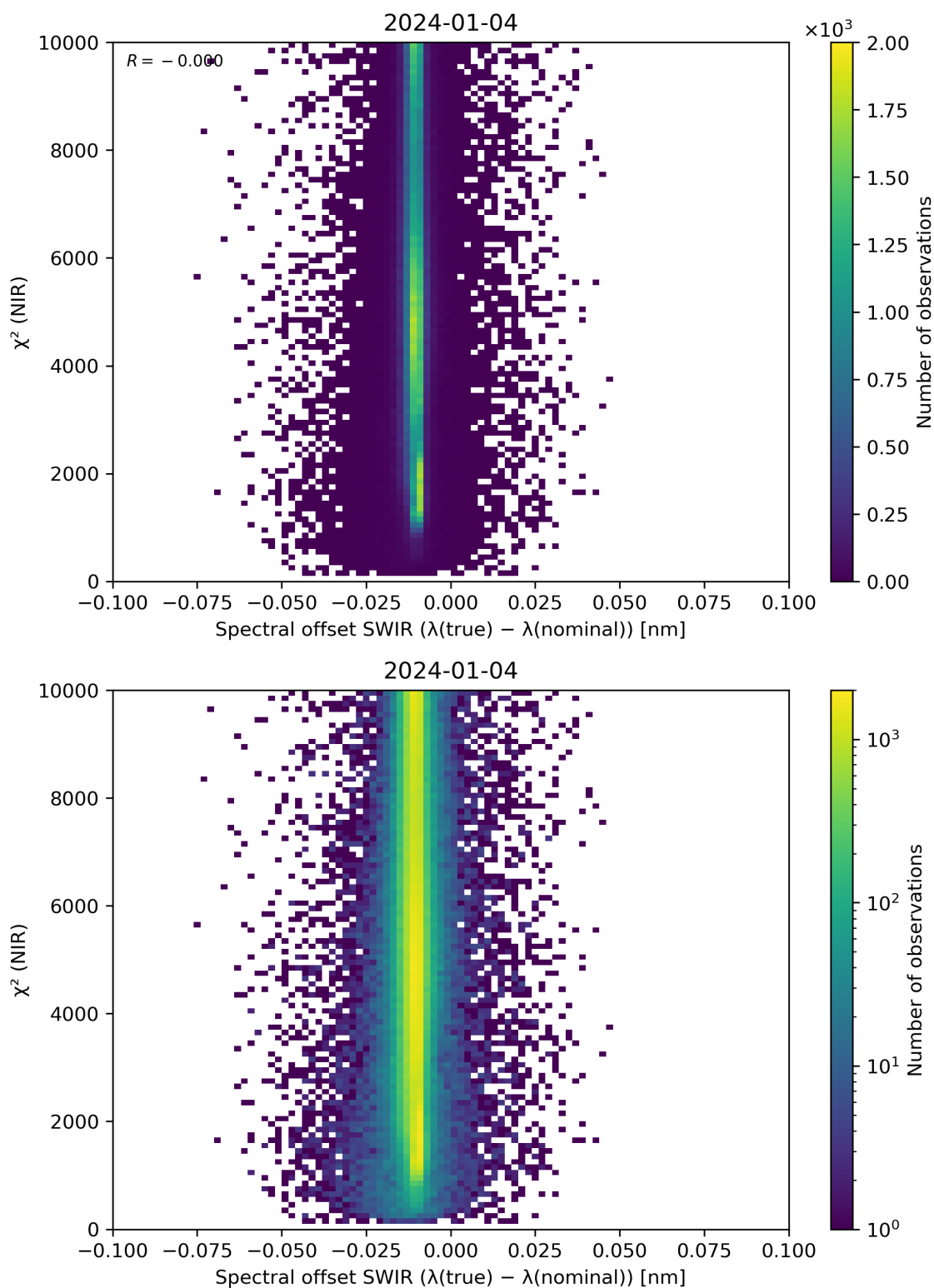
Figure 117: Scatter density plot of “Spectral offset SWIR ( \lambda(\text{true}) - \lambda(\text{nominal}) )” against “ \chi^2 (NIR)” for 2024-01-03 to 2024-01-05.
