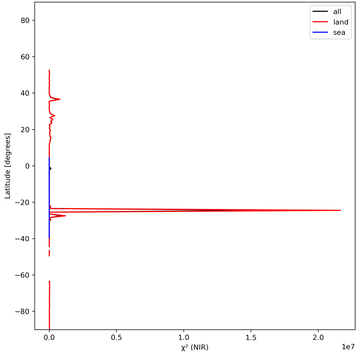
Figure 18: Zonal average of “ \chi^2 (NIR)” for 2024-01-03 to 2024-01-05.
