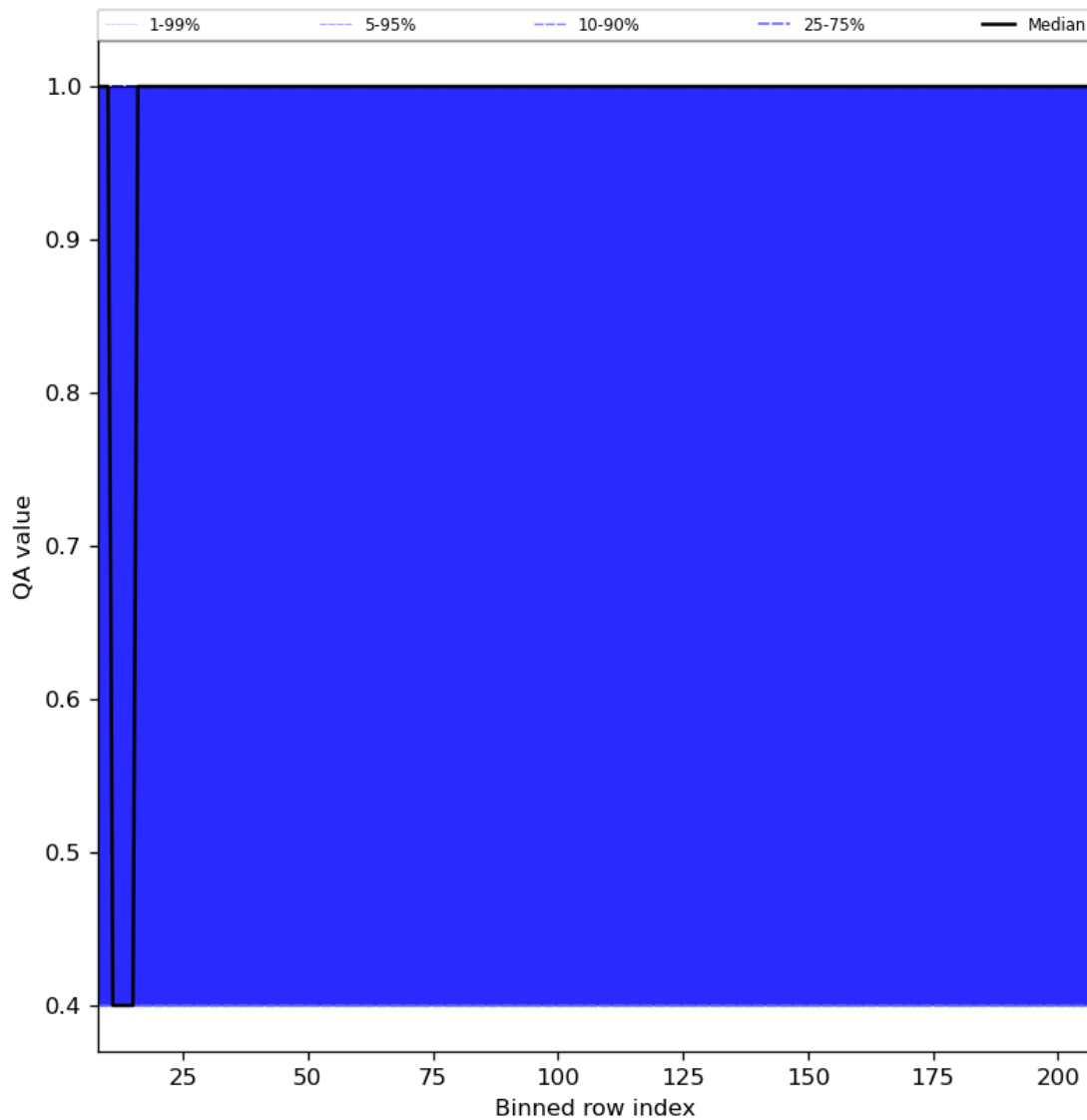
Figure 33: Along track statistics of “QA value” for 2024-01-03 to 2024-01-05
