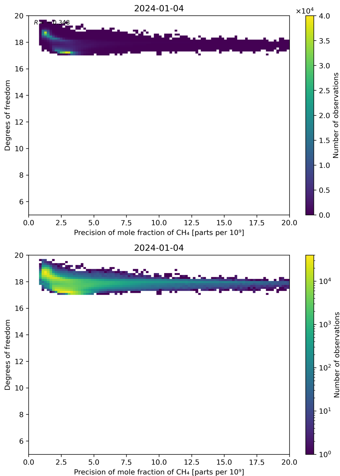
Figure 80: Scatter density plot of “Precision of mole fraction of CH 4 ” against “Degrees of freedom” for 2024-01-03 to 2024-01-05.
