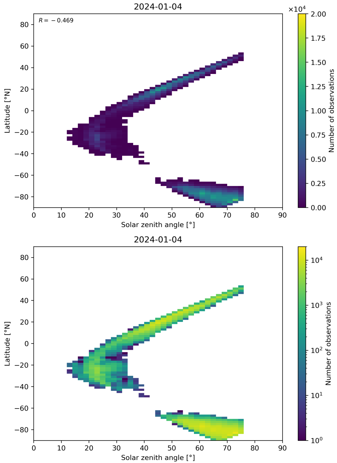
Figure 98: Scatter density plot of “Solar zenith angle” against “Latitude” for 2024-01-03 to 2024-01-05.
