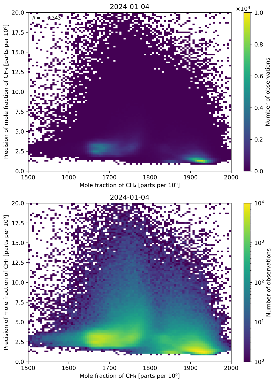
Figure 75: Scatter density plot of “Mole fraction of CH 4 ” against “Precision of mole fraction of CH 4 ” for 2024-01-03 to 2024-01-05.
