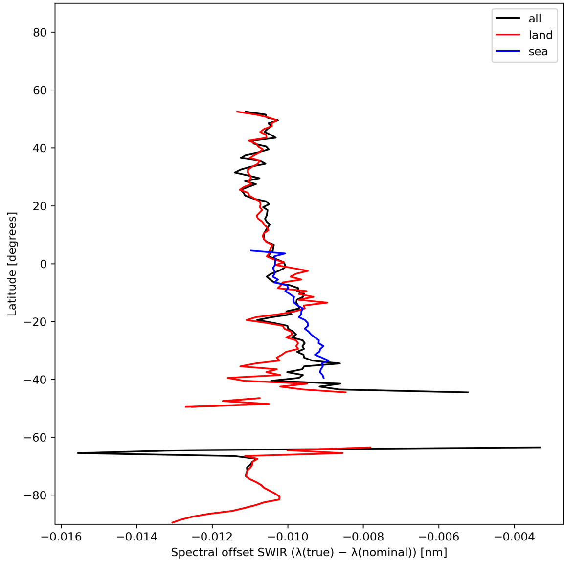
Figure 16: Zonal average of “Spectral offset SWIR ( \lambda(\text{true}) - \lambda(\text{nominal}) )” for 2024-01-03 to 2024-01-05.
