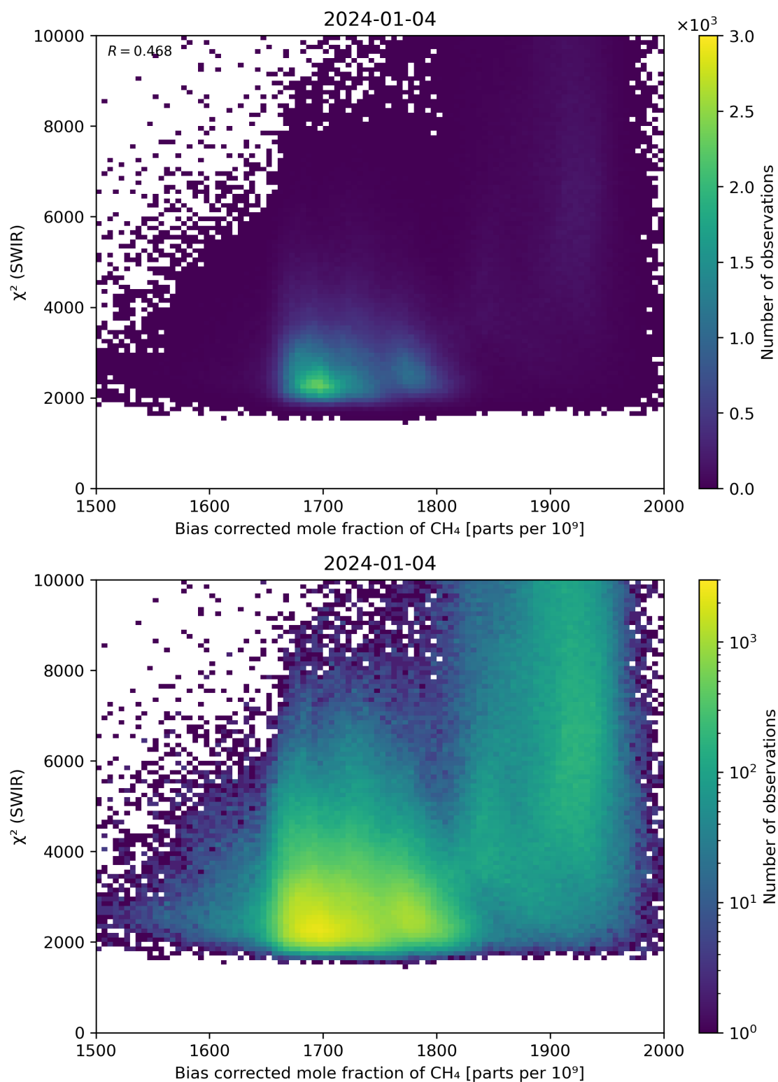
Figure 64: Scatter density plot of “Bias corrected mole fraction of \text{CH}_4 ” against “ \chi^2 (SWIR)” for 2024-01-03 to 2024-01-05.
