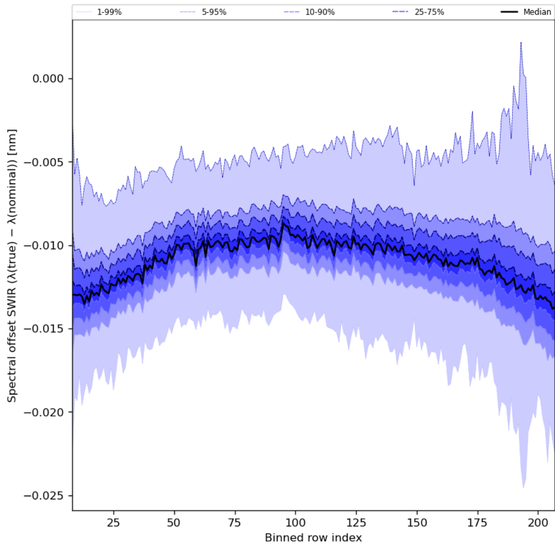
Figure 38: Along track statistics of “Spectral offset SWIR ( \lambda(\text{true}) - \lambda(\text{nominal}) )” for 2024-01-03 to 2024-01-05
