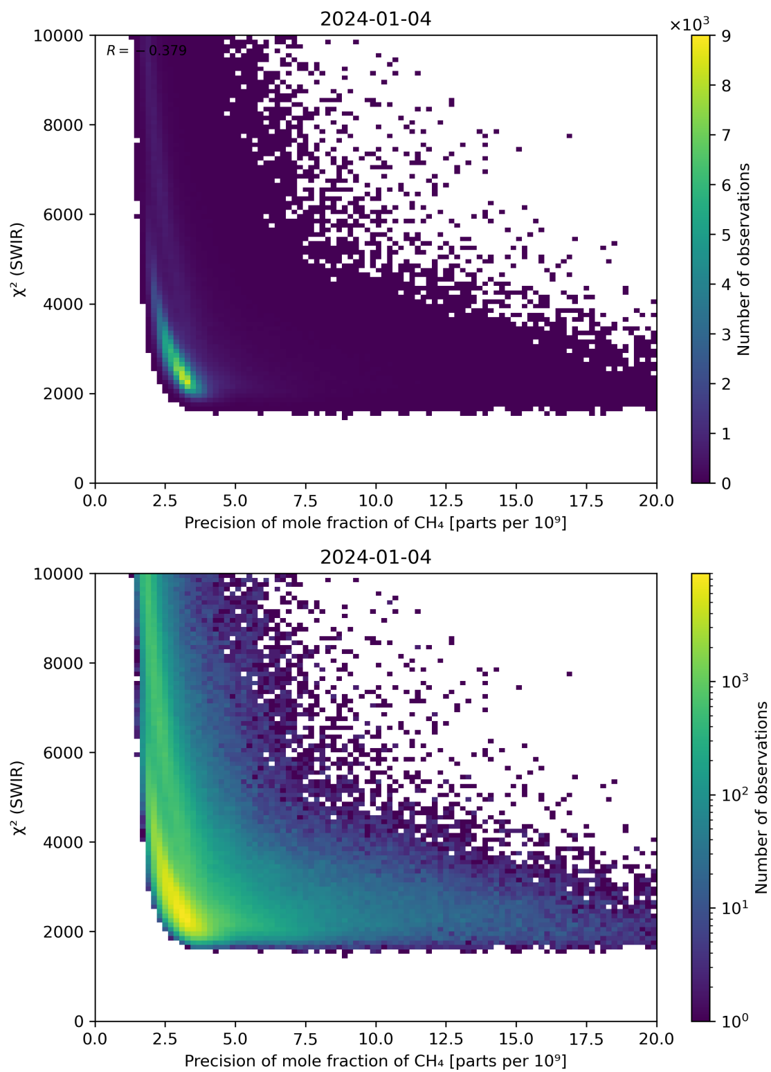
Figure 79: Scatter density plot of “Precision of mole fraction of \text{CH}_4 ” against “ \chi^2 (SWIR)” for 2024-01-03 to 2024-01-05.
