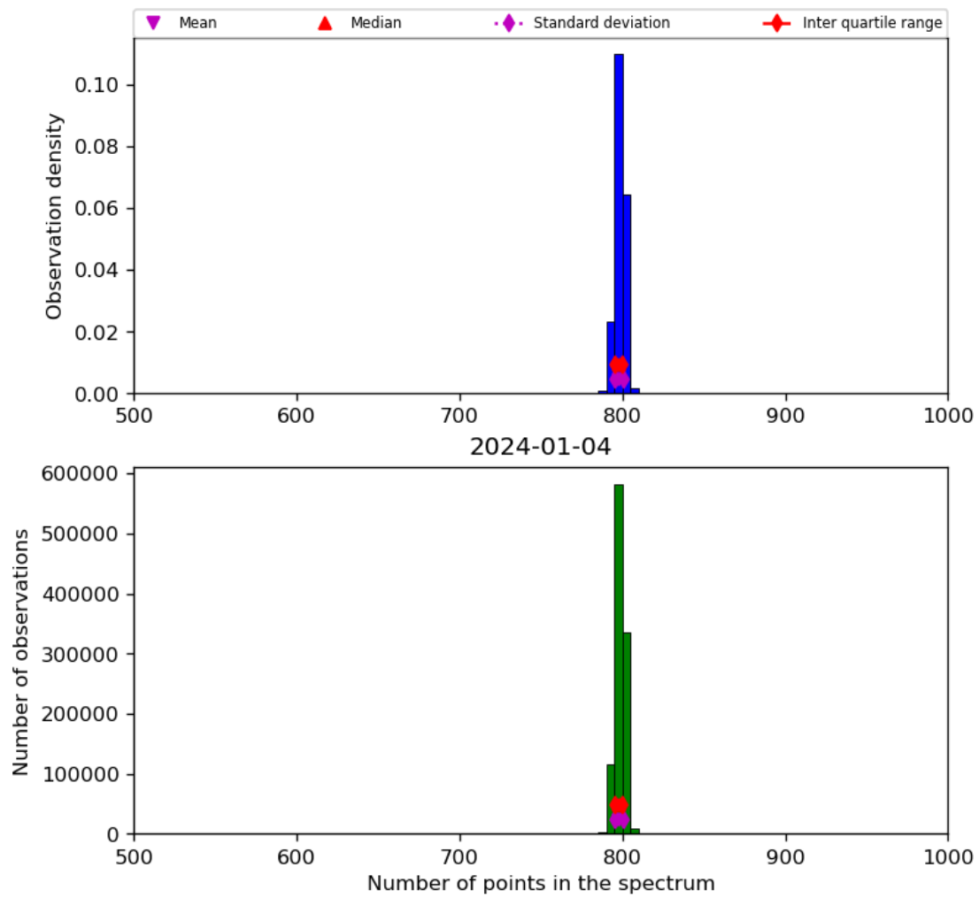
Figure 26: Histogram of “Number of points in the spectrum” for 2024-01-03 to 2024-01-05
