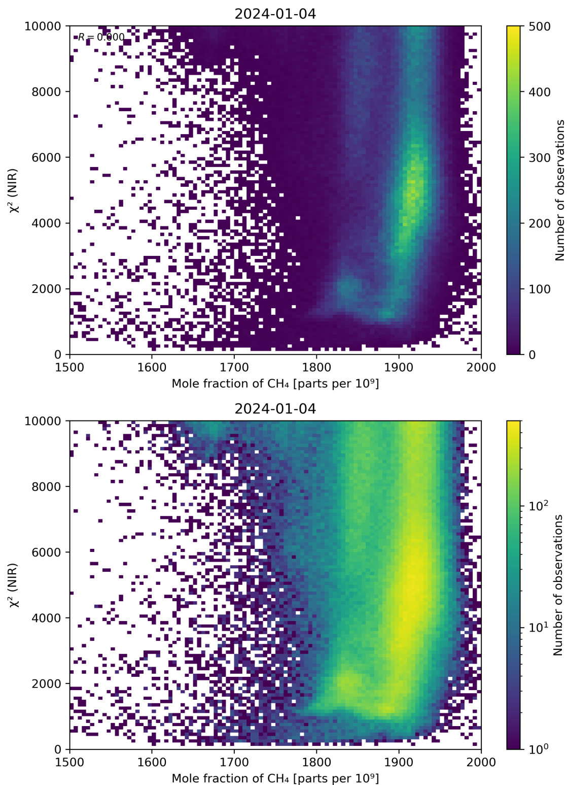
Figure 70: Scatter density plot of “Mole fraction of \text{CH}_4 ” against “ \chi^2 (NIR)” for 2024-01-03 to 2024-01-05.
