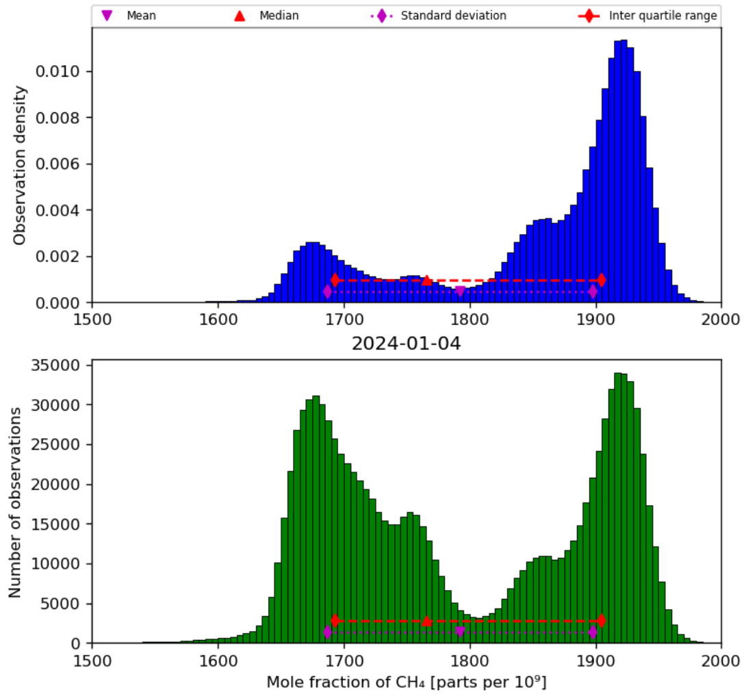
Figure 23: Histogram of “Mole fraction of CH 4 ” for 2024-01-03 to 2024-01-05
