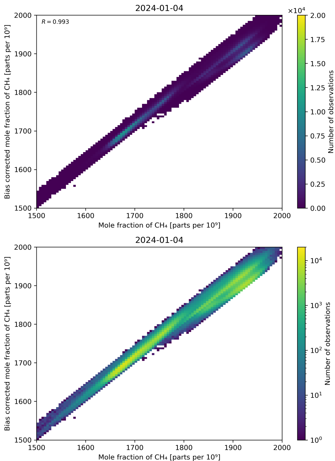
Figure 74: Scatter density plot of “Mole fraction of CH 4 ” against “Bias corrected mole fraction of CH 4 ” for 2024-01-03 to 2024-01-05.
