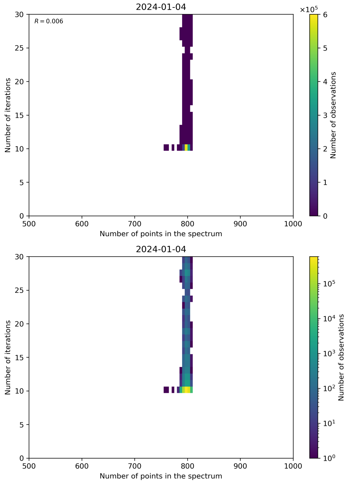
Figure 92: Scatter density plot of “Number of points in the spectrum” against “Number of iterations” for 2024-01-03 to 2024-01-05.
