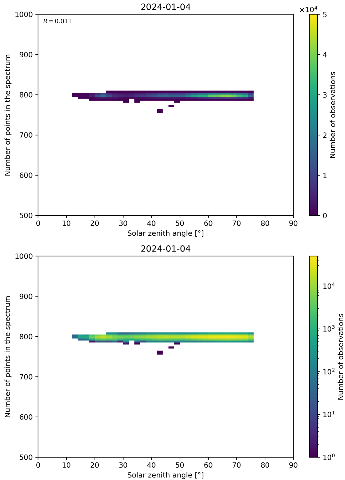
Figure 103: Scatter density plot of “Solar zenith angle” against “Number of points in the spectrum” for 2024-01-03 to 2024-01-05.
