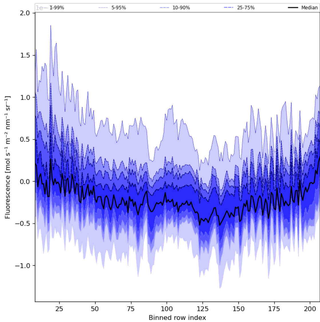
Figure 43: Along track statistics of "Fluorescence" for 2024-01-03 to 2024-01-05
