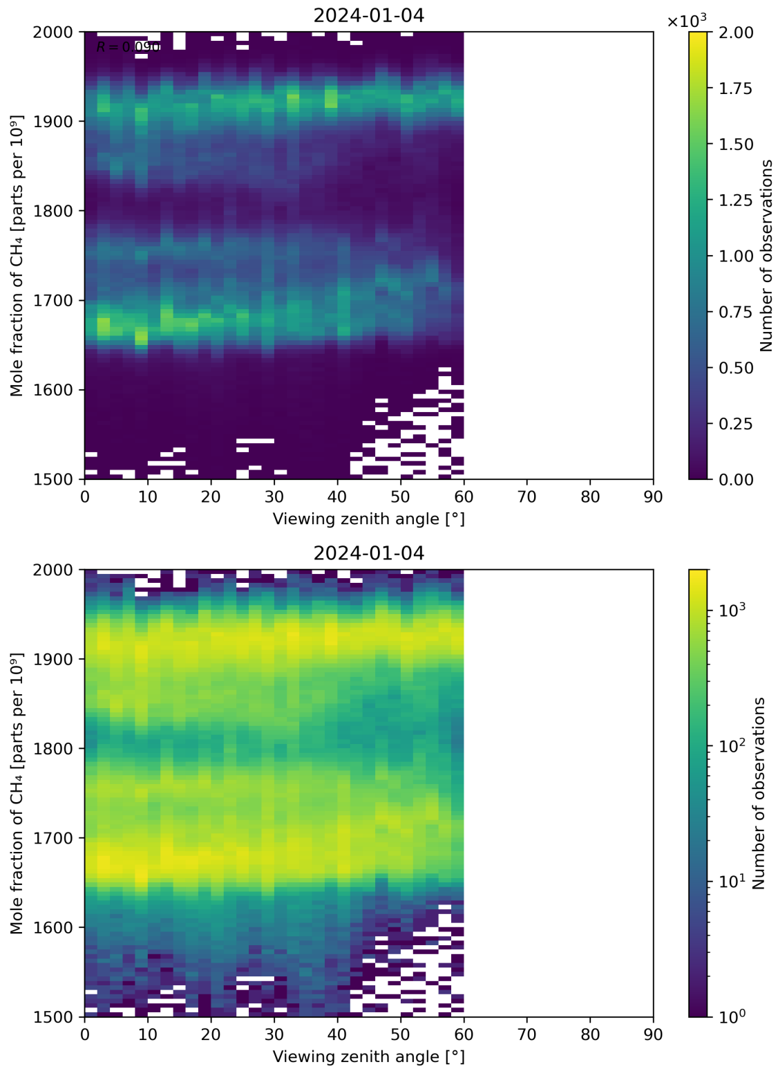
Figure 110: Scatter density plot of “Viewing zenith angle” against “Mole fraction of CH 4 ” for 2024-01-03 to 2024-01-05.
