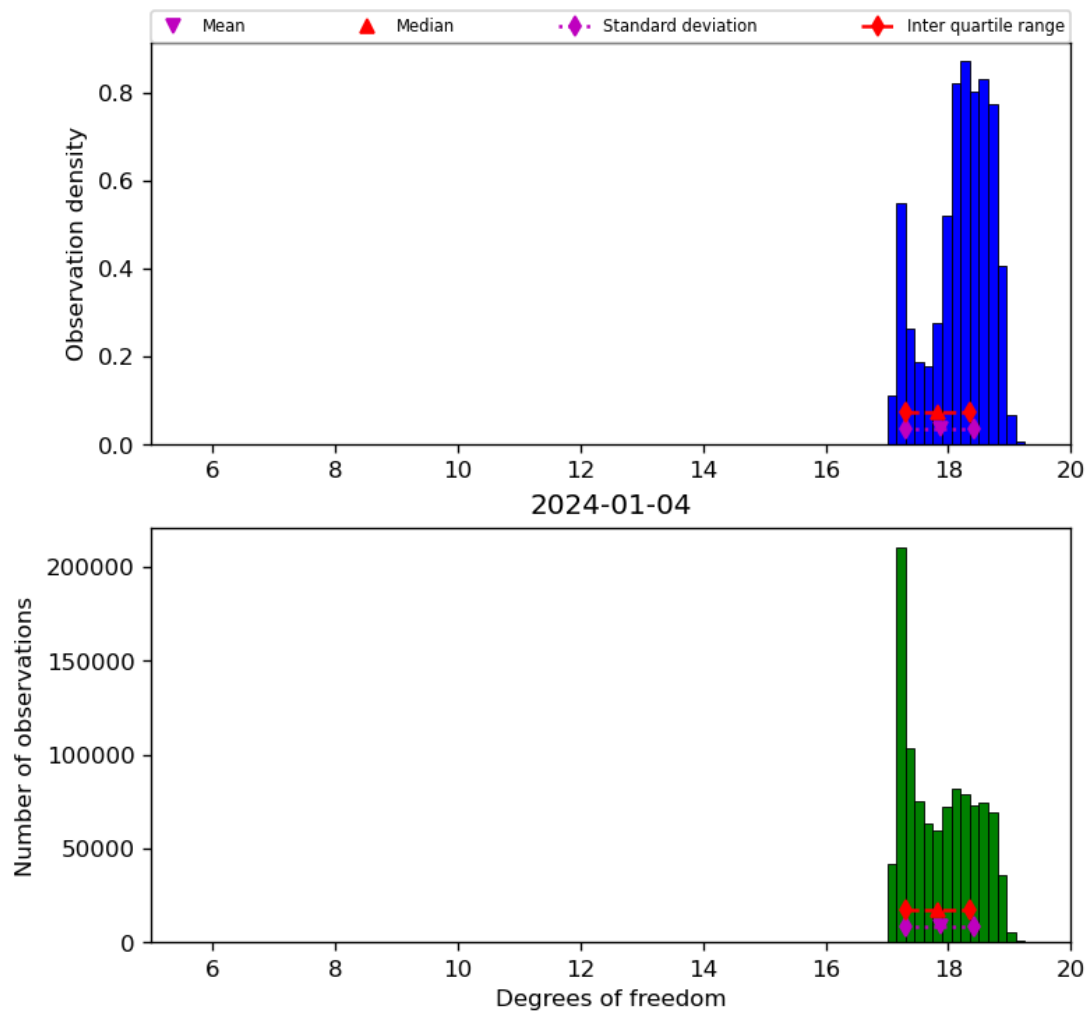
Figure 30: Histogram of “Degrees of freedom” for 2024-01-03 to 2024-01-05
