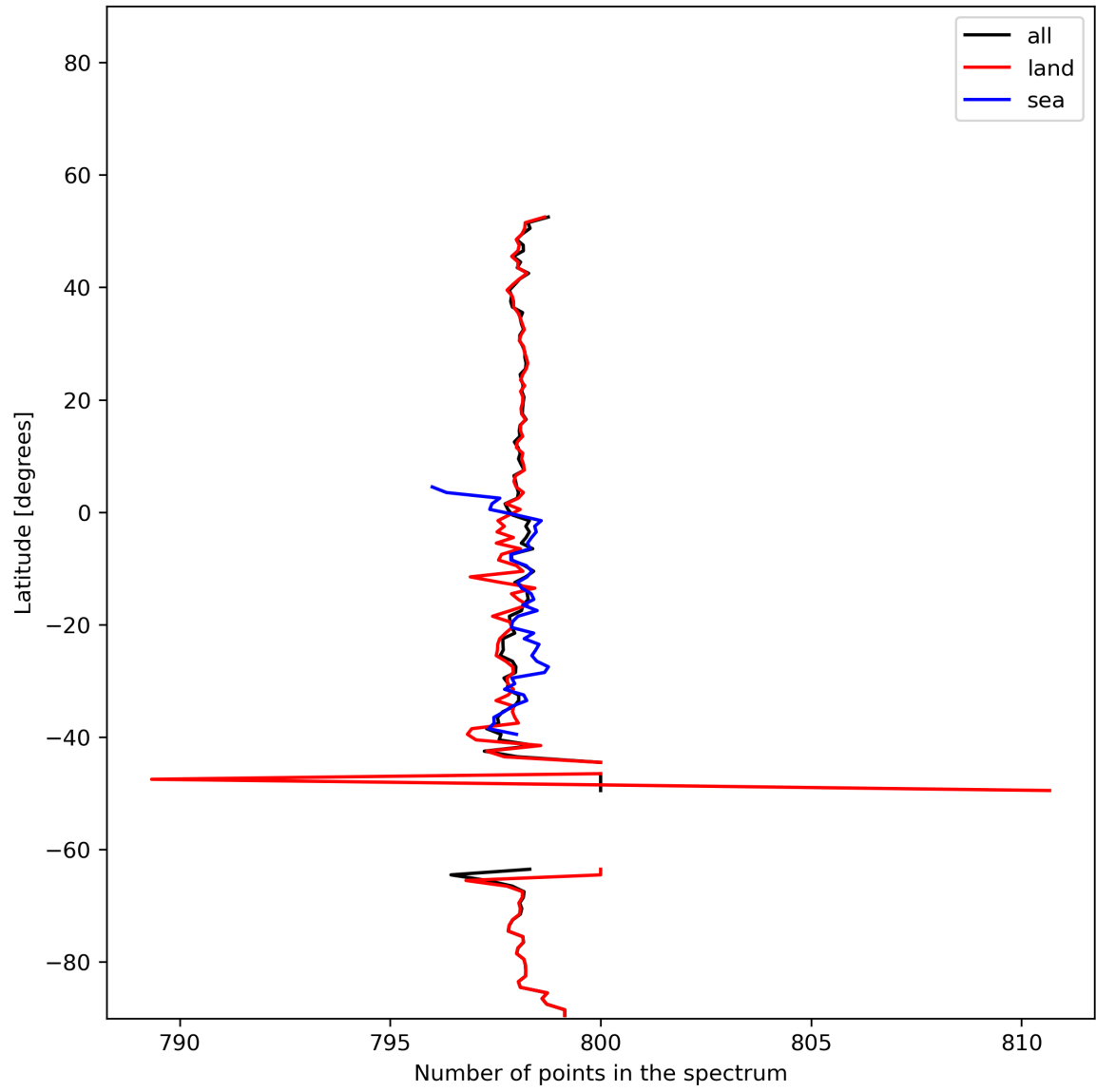
Figure 15: Zonal average of “Number of points in the spectrum” for 2024-01-03 to 2024-01-05.
