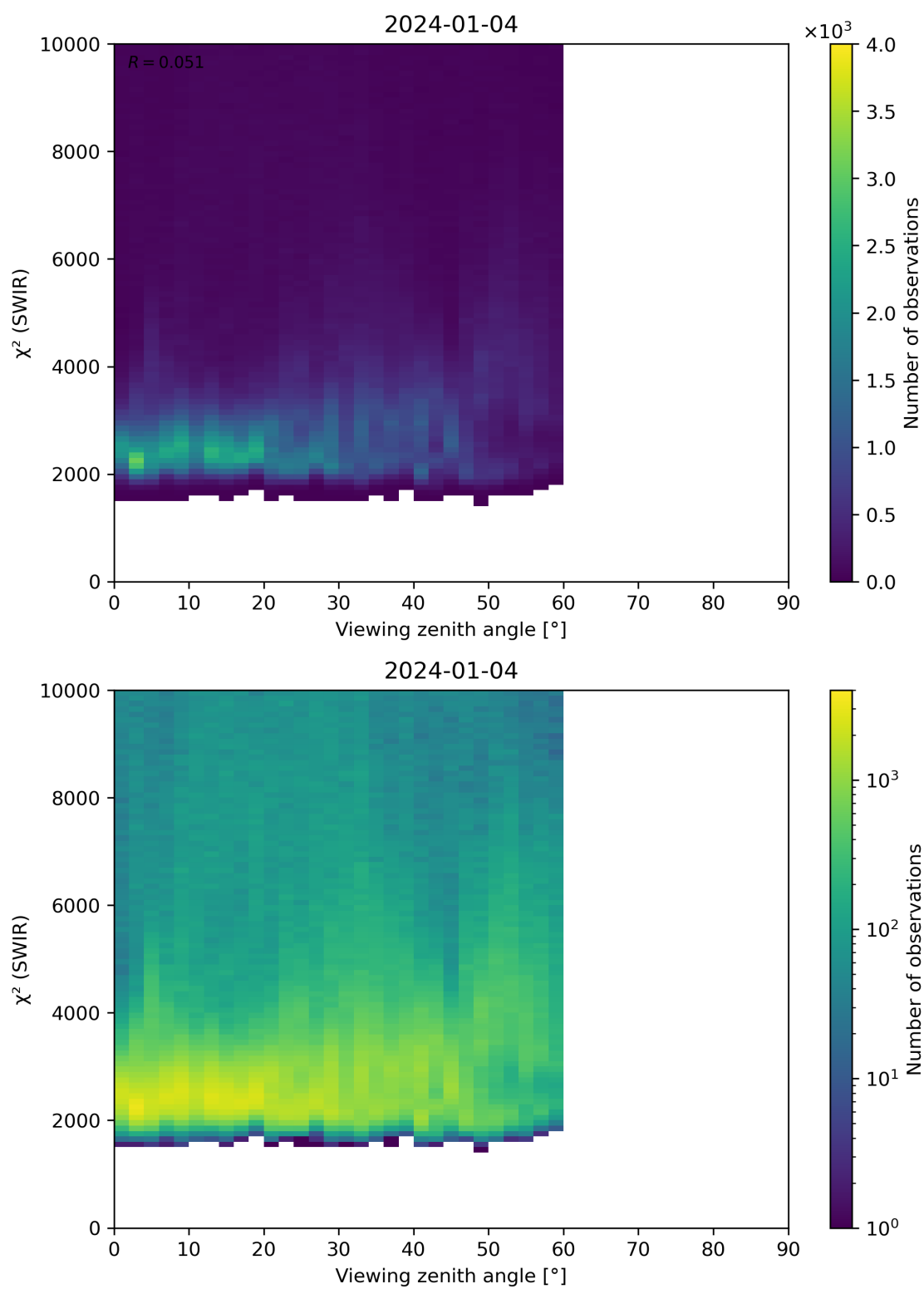
Figure 106: Scatter density plot of “Viewing zenith angle” against “ \chi^2 (SWIR)” for 2024-01-03 to 2024-01-05.
