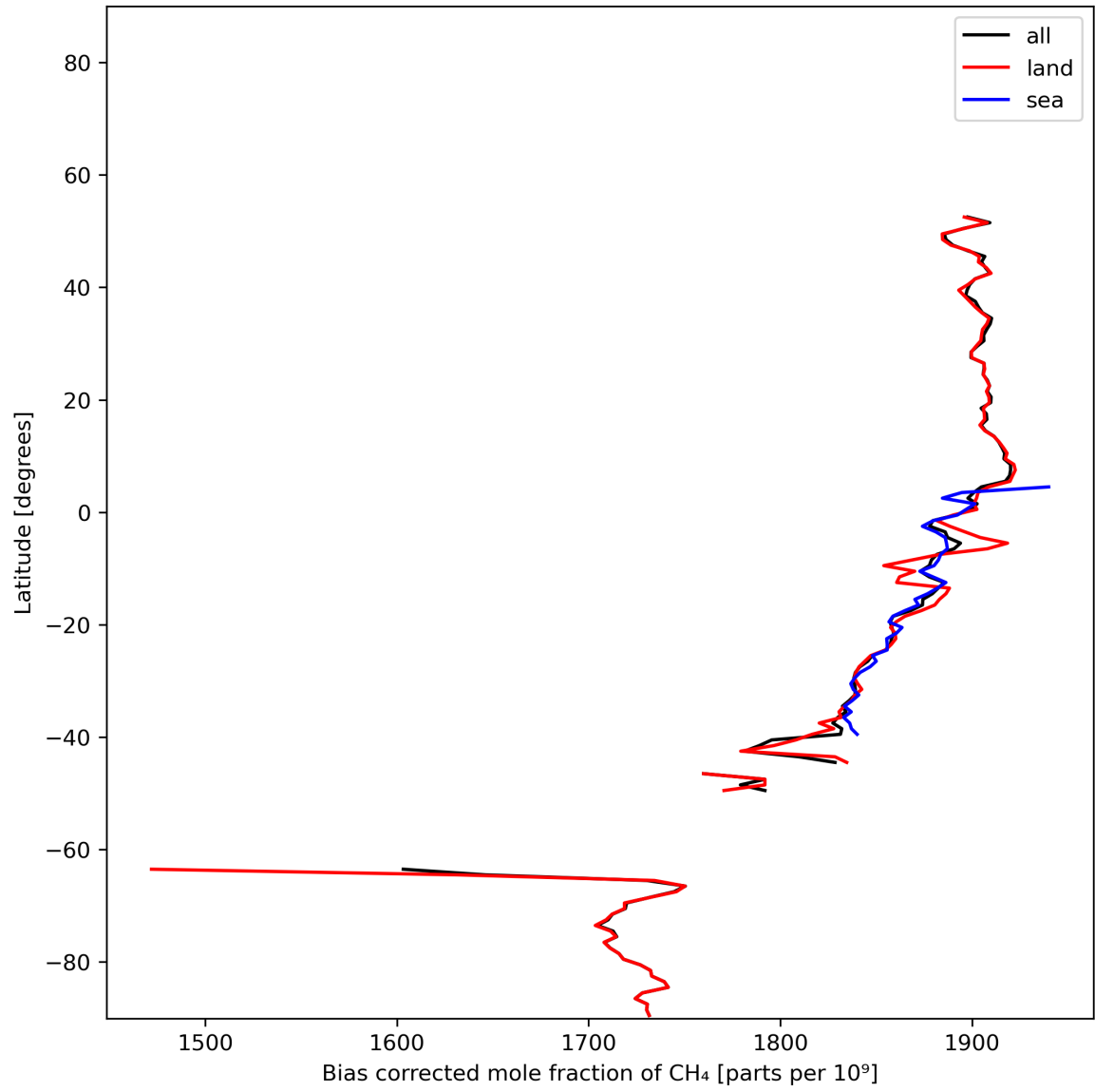
Figure 14: Zonal average of “Bias corrected mole fraction of CH 4 ” for 2024-01-03 to 2024-01-05.
