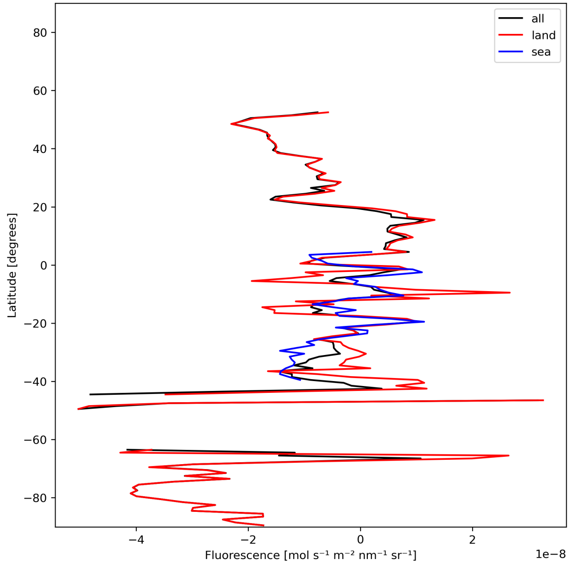
Figure 21: Zonal average of “Fluorescence” for 2024-01-03 to 2024-01-05.
