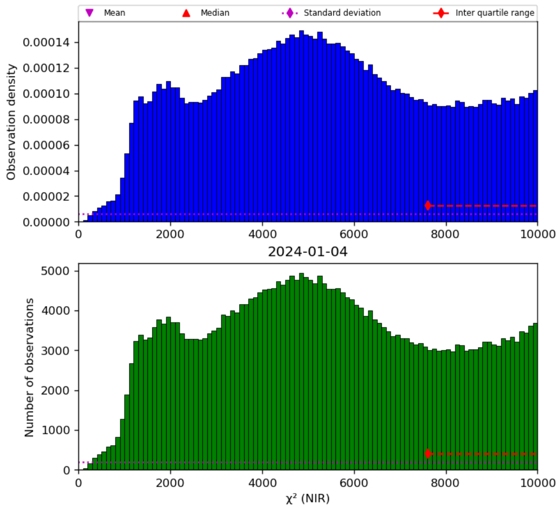
Figure 29: Histogram of “ \chi^2 (NIR)” for 2024-01-03 to 2024-01-05
