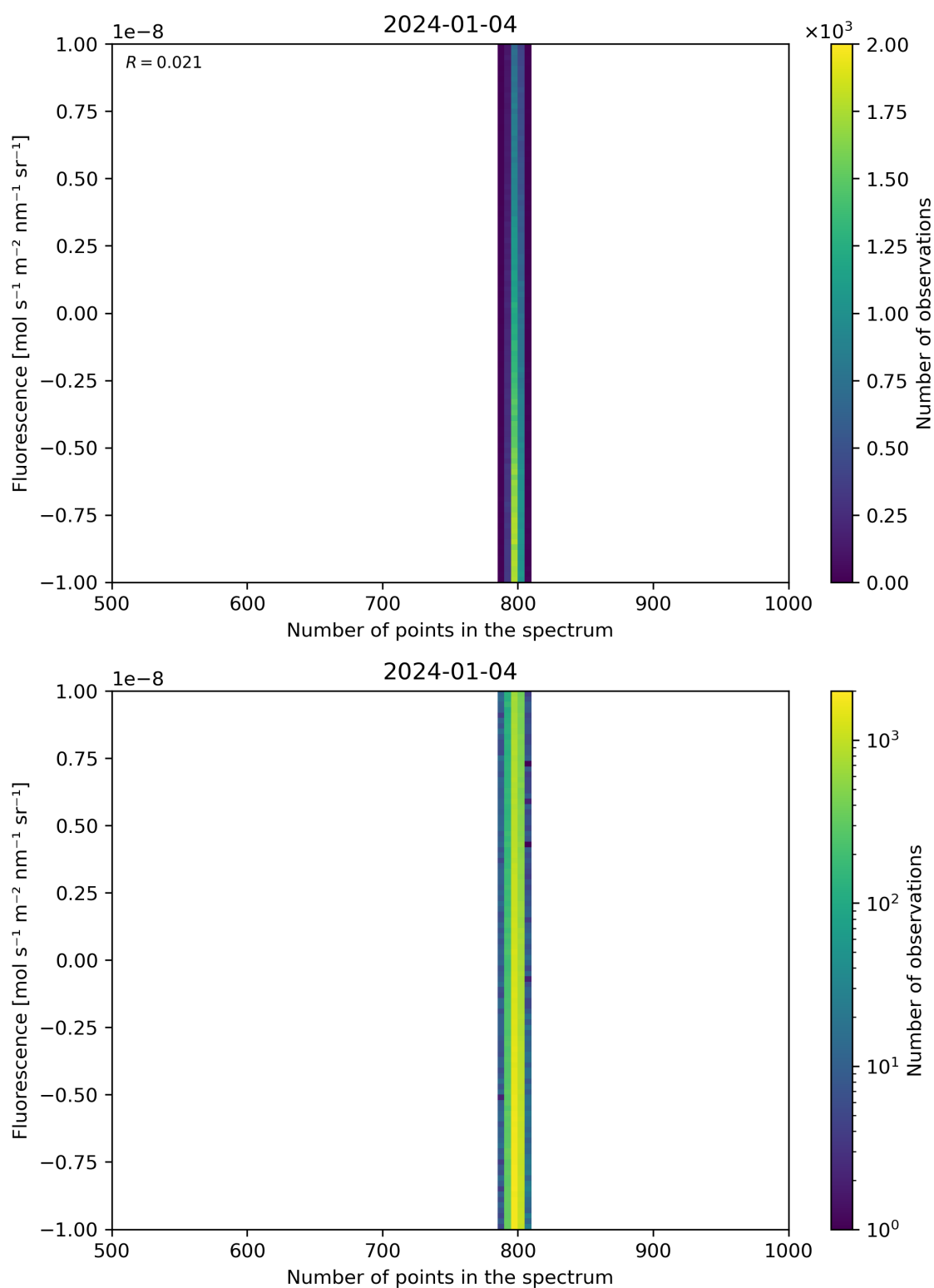
Figure 91: Scatter density plot of “Number of points in the spectrum” against “Fluorescence” for 2024-01-03 to 2024-01-05.
