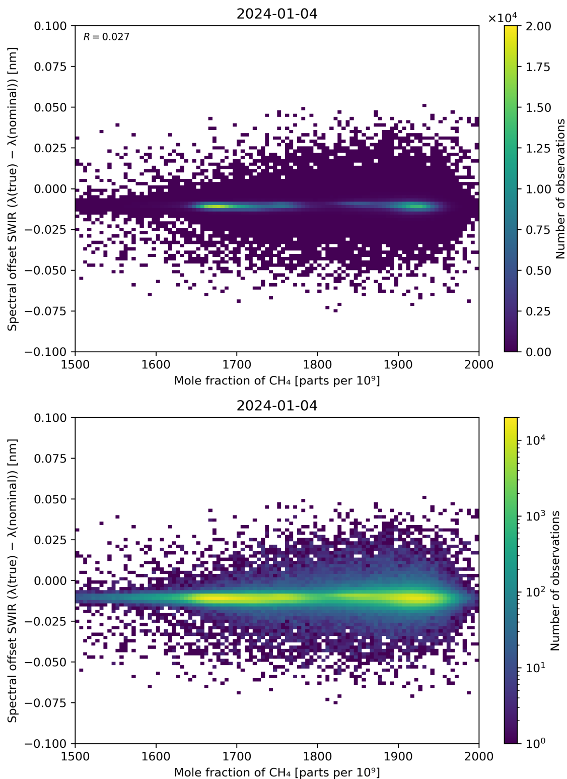
Figure 86: Scatter density plot of “Mole fraction of CH 4 ” against “Spectral offset SWIR ( \lambda(\text{true}) - \lambda(\text{nominal}) )” for 2024-01-03 to 2024-01-05.
