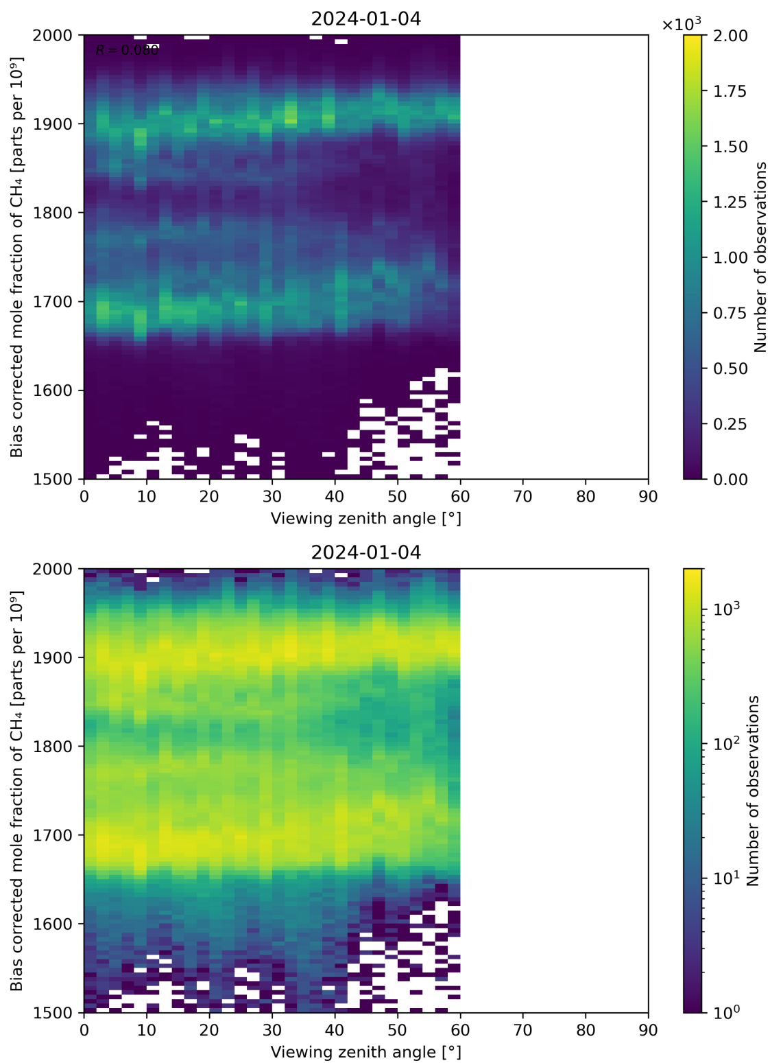
Figure 111: Scatter density plot of “Viewing zenith angle” against “Bias corrected mole fraction of CH 4 ” for 2024-01-03 to 2024-01-05.
