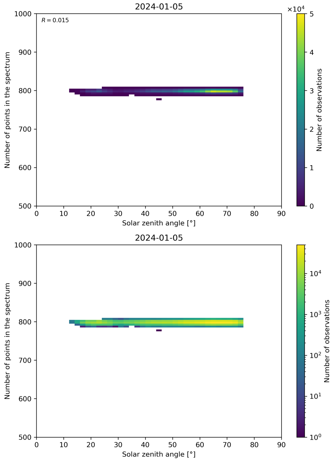
Figure 103: Scatter density plot of “Solar zenith angle” against “Number of points in the spectrum” for 2024-01-05 to 2024-01-06.
