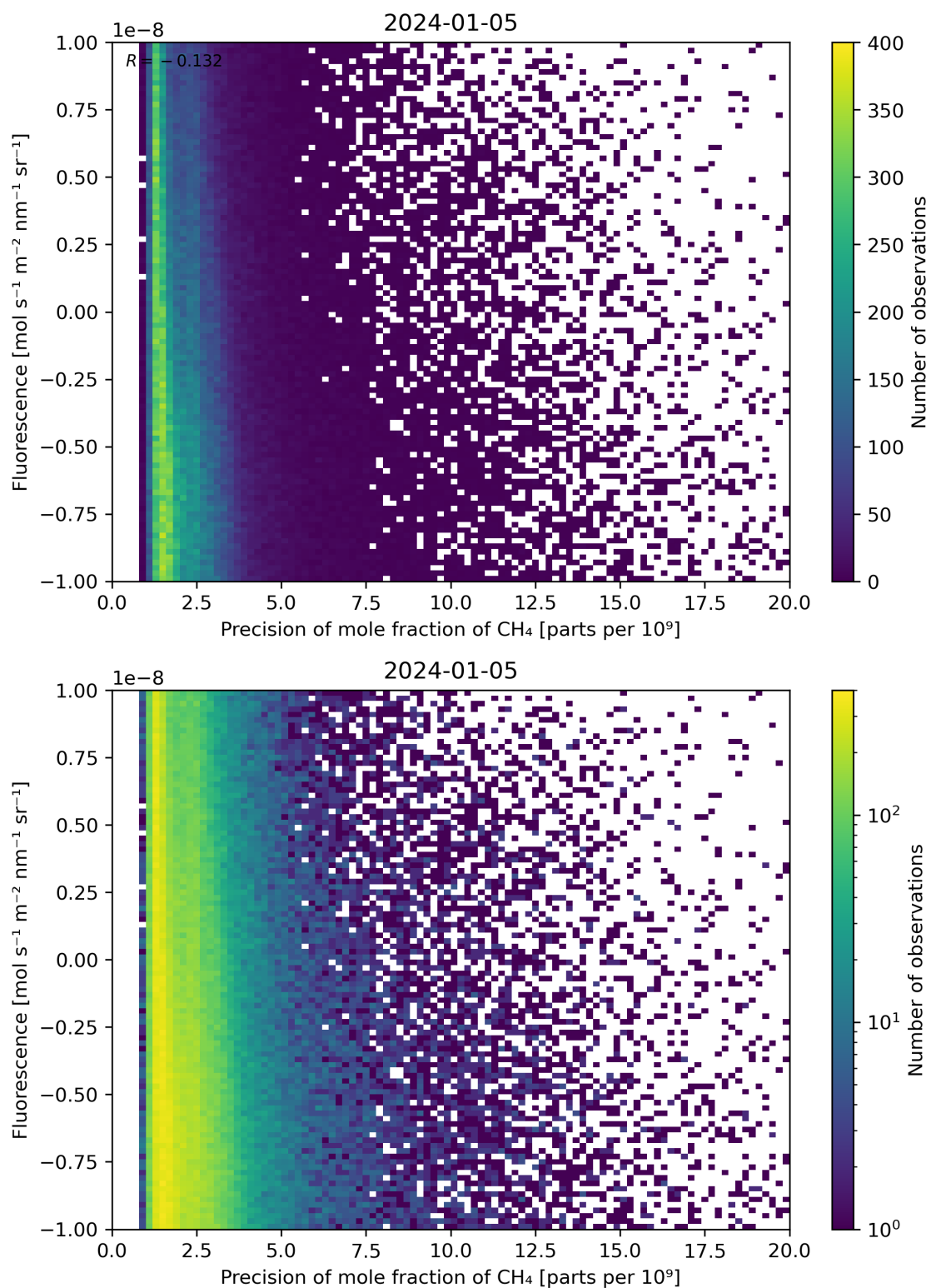
Figure 81: Scatter density plot of “Precision of mole fraction of \text{CH}_4 ” against “Fluorescence” for 2024-01-05 to 2024-01-06.
