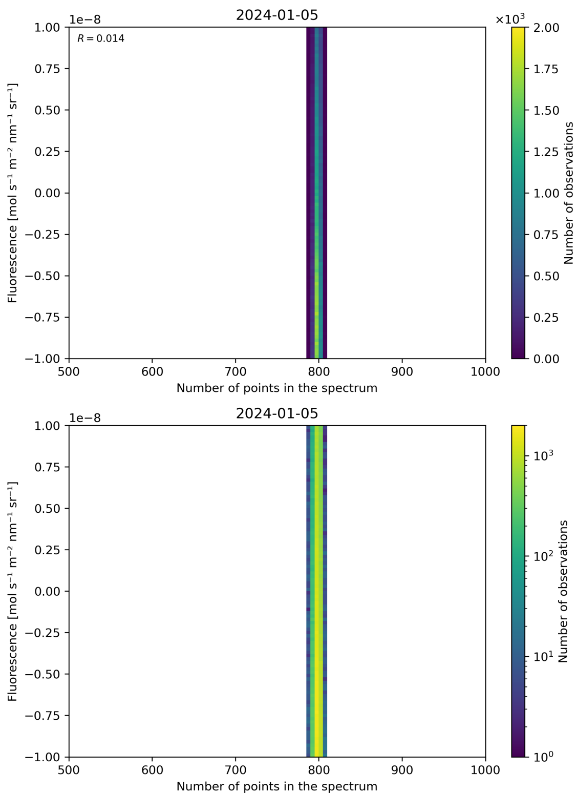
Figure 91: Scatter density plot of “Number of points in the spectrum” against “Fluorescence” for 2024-01-05 to 2024-01-06.
