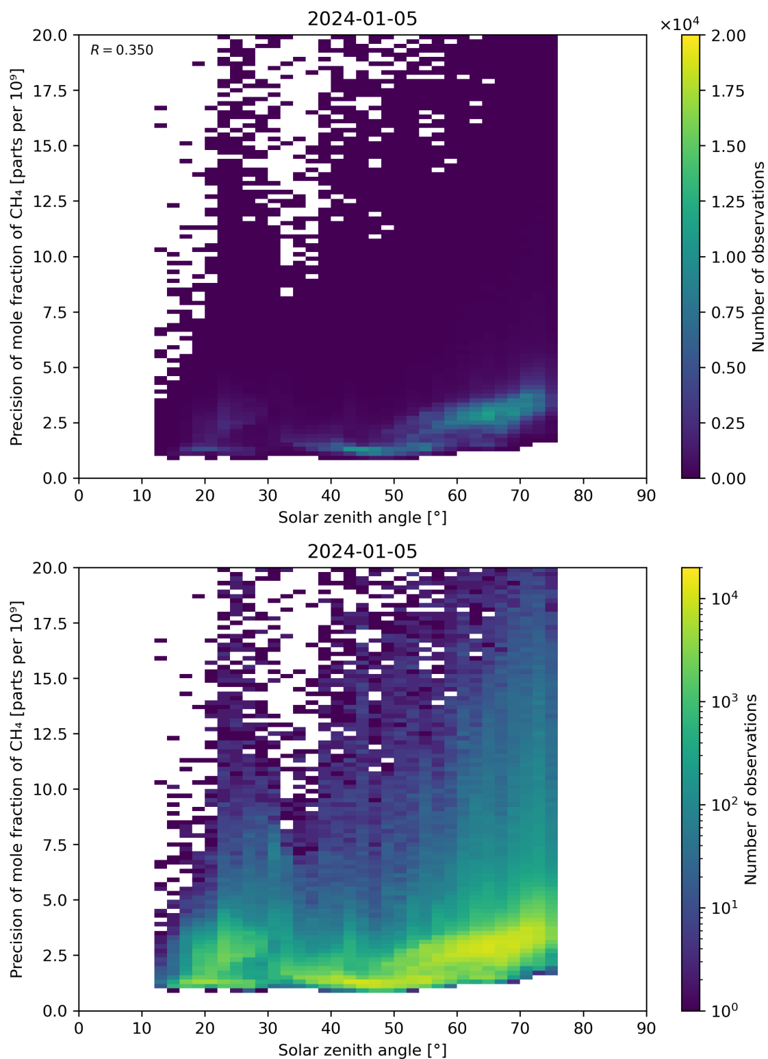
Figure 101: Scatter density plot of “Solar zenith angle” against “Precision of mole fraction of CH 4 ” for 2024-01-05 to 2024-01-06.
