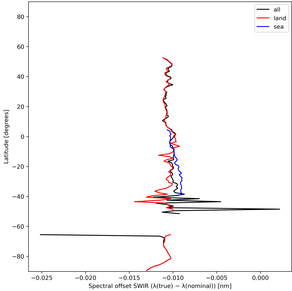
Figure 16: Zonal average of “Spectral offset SWIR ( \lambda(\text{true}) - \lambda(\text{nominal}) )” for 2024-01-05 to 2024-01-06.
