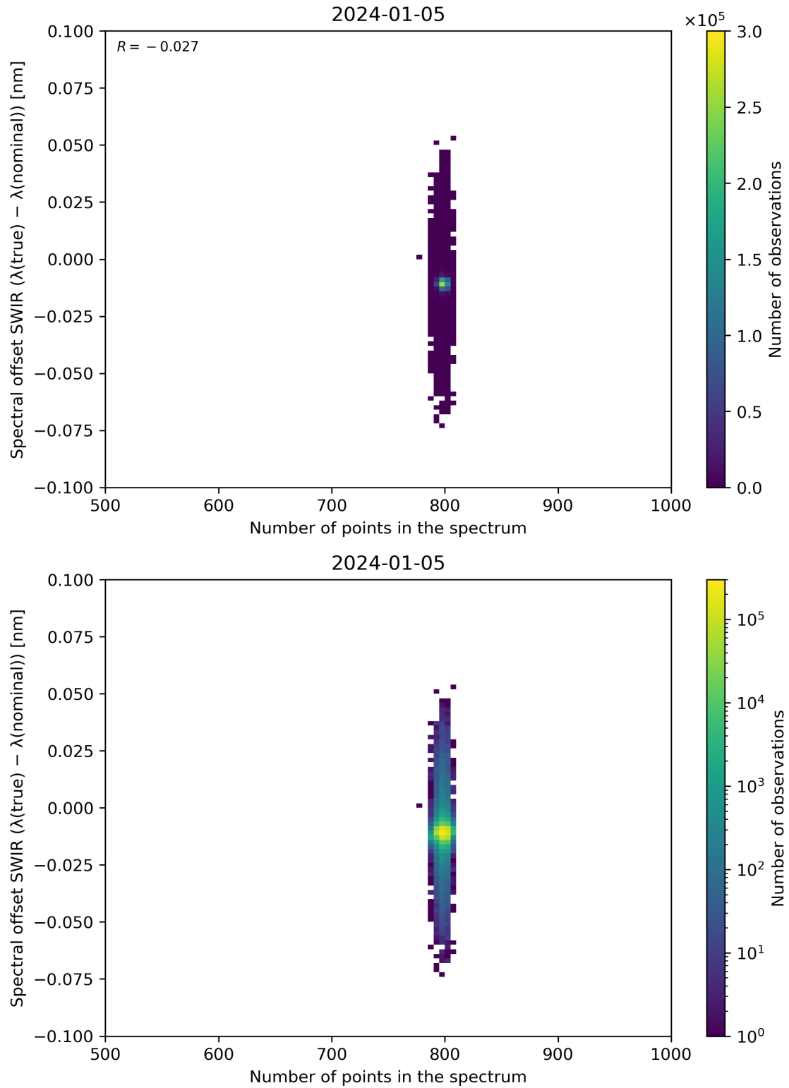
Figure 93: Scatter density plot of “Number of points in the spectrum” against “Spectral offset SWIR ( \lambda(\text{true}) - \lambda(\text{nominal}) )” for 2024-01-05 to 2024-01-06.
