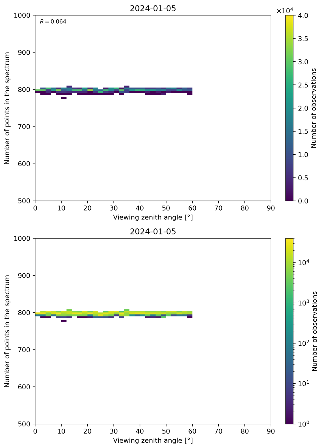
Figure 114: Scatter density plot of “Viewing zenith angle” against “Number of points in the spectrum” for 2024-01-05 to 2024-01-06.
