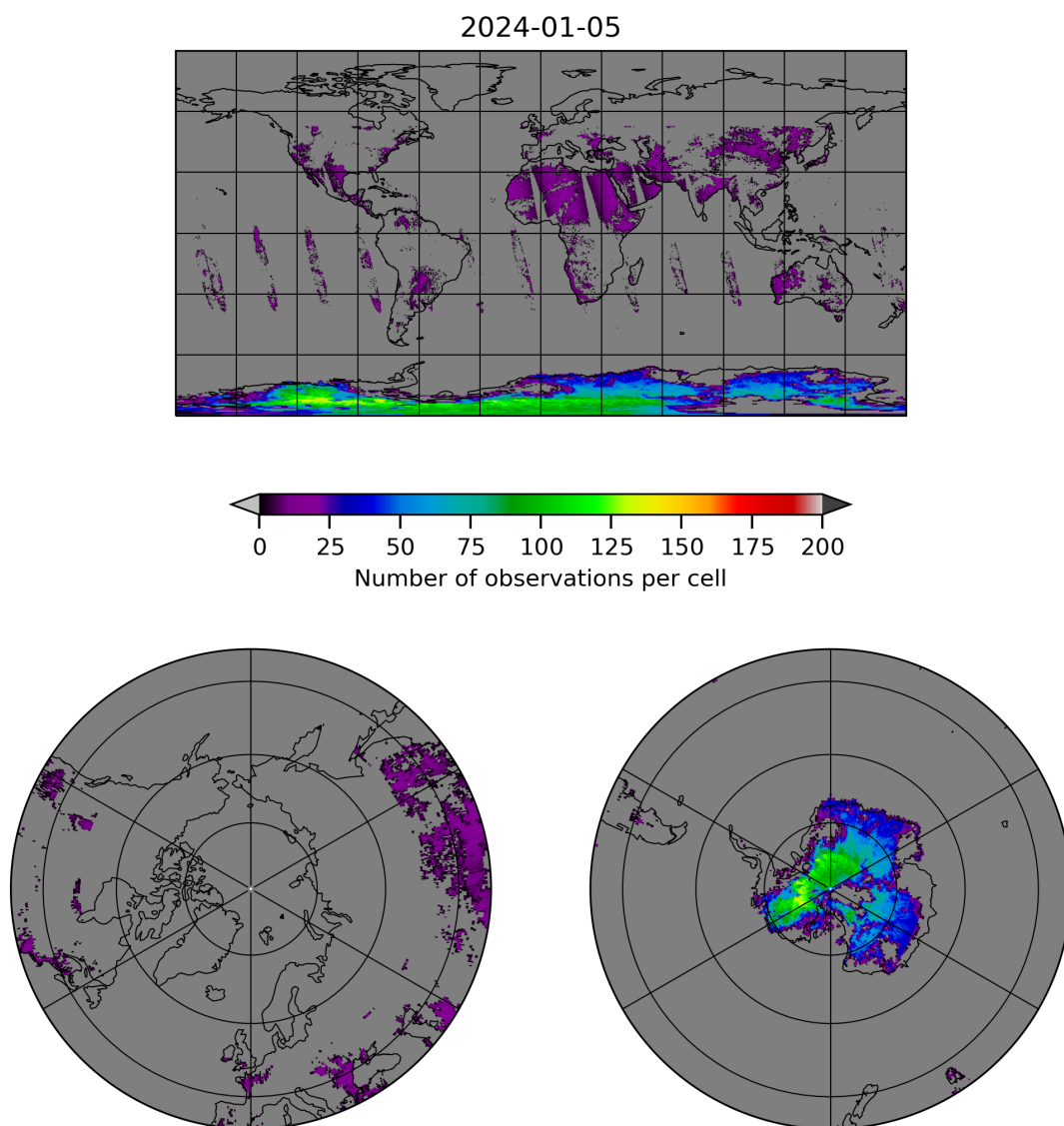
Figure 10: Map of the number of observations for 2024-01-05 to 2024-01-06
