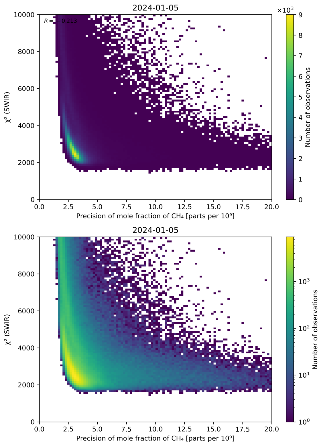
Figure 79: Scatter density plot of “Precision of mole fraction of \text{CH}_4 ” against “ \chi^2 (SWIR)” for 2024-01-05 to 2024-01-06.
