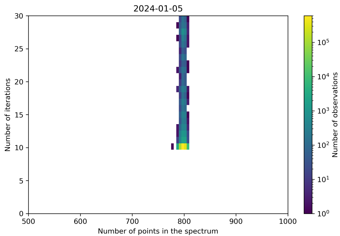
Figure 92: Scatter density plot of “Number of points in the spectrum” against “Number of iterations” for 2024-01-05 to 2024-01-06.
