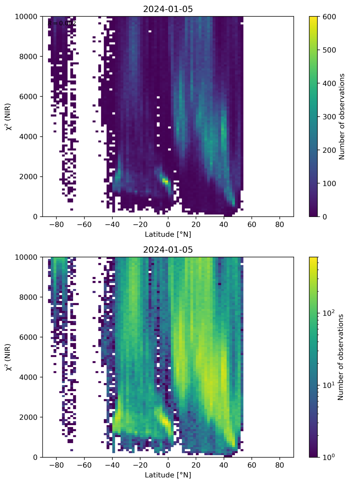
Figure 53: Scatter density plot of “Latitude” against “ \chi^2 (NIR)” for 2024-01-05 to 2024-01-06.
