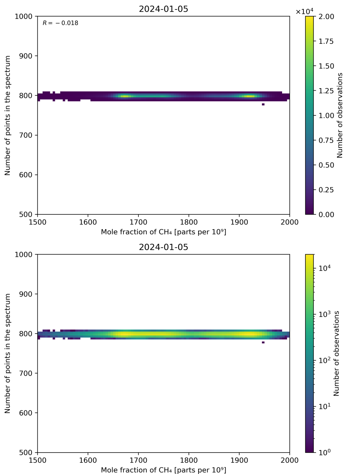
Figure 77: Scatter density plot of “Mole fraction of CH 4 ” against “Number of points in the spectrum” for 2024-01-05 to 2024-01-06.
