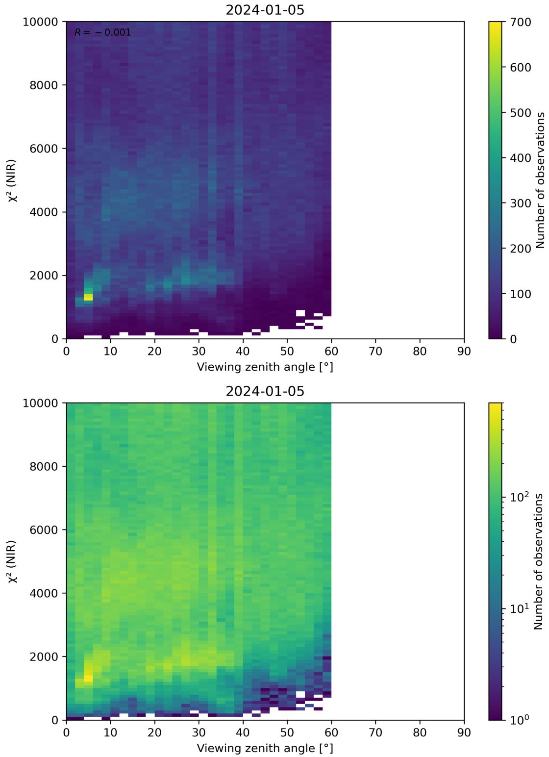
Figure 105: Scatter density plot of “Viewing zenith angle” against “ \chi^2 (NIR)” for 2024-01-05 to 2024-01-06.
