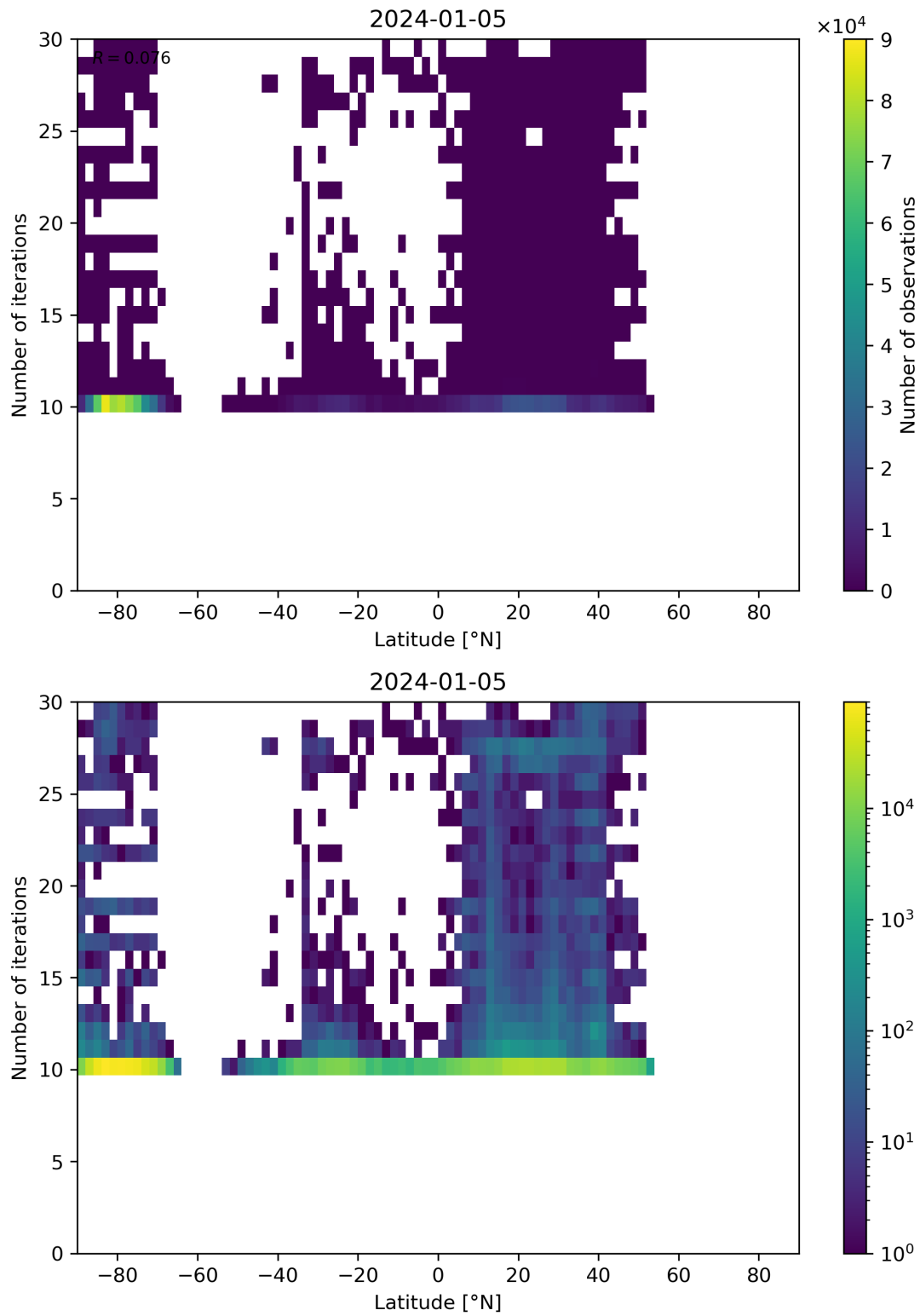
Figure 60: Scatter density plot of “Latitude” against “Number of iterations” for 2024-01-05 to 2024-01-06.
