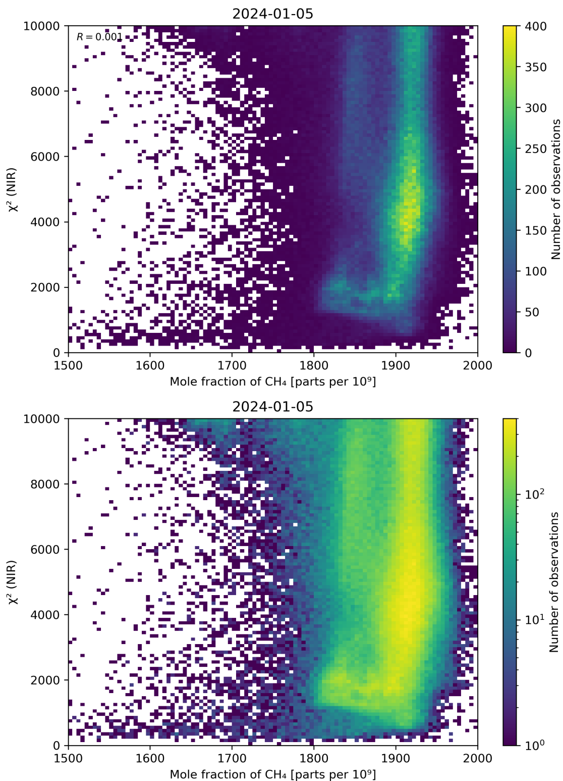
Figure 70: Scatter density plot of “Mole fraction of CH 4 ” against “ \chi^2 (NIR)” for 2024-01-05 to 2024-01-06.
