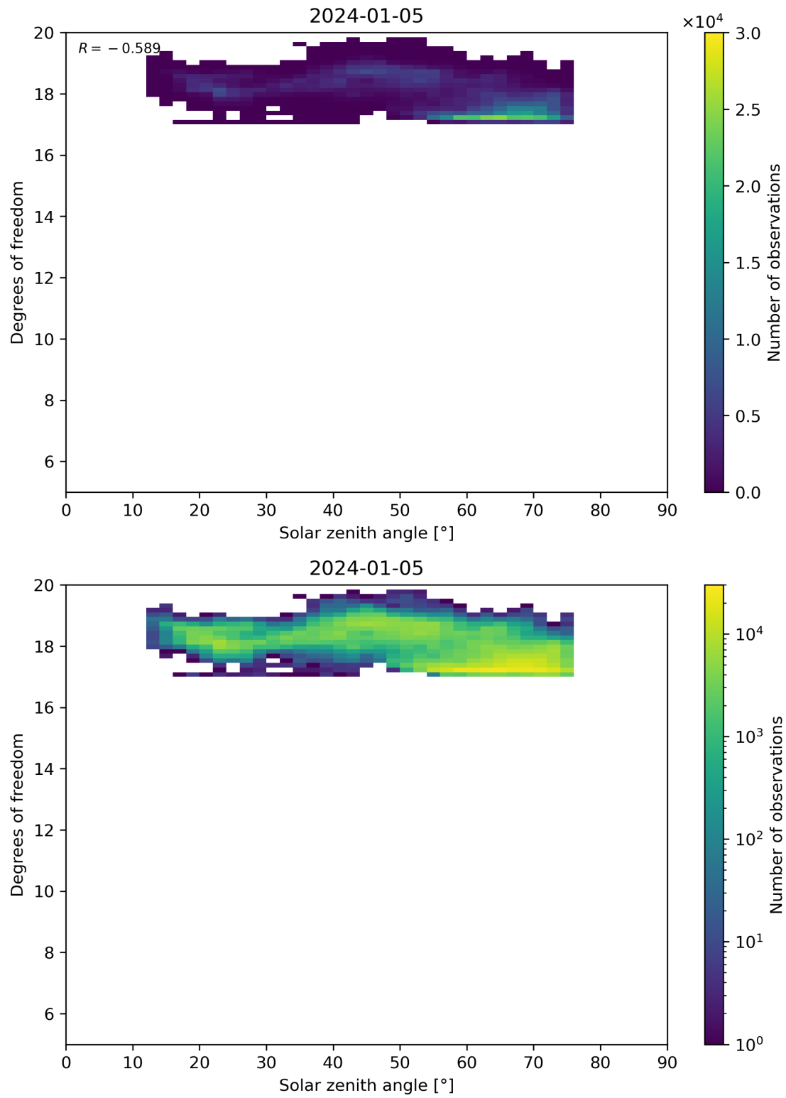
Figure 96: Scatter density plot of “Solar zenith angle” against “Degrees of freedom” for 2024-01-05 to 2024-01-06.
