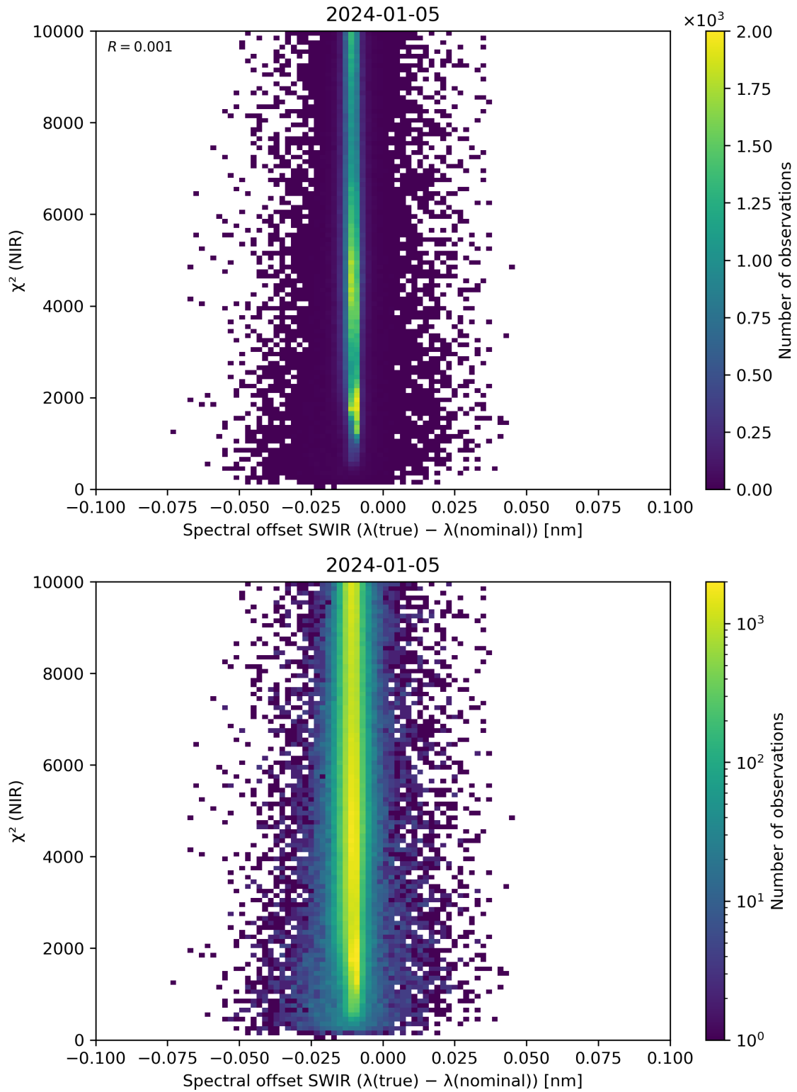
Figure 117: Scatter density plot of “Spectral offset SWIR ( \lambda(\text{true}) - \lambda(\text{nominal}) )” against “ \chi^2 (NIR)” for 2024-01-05 to 2024-01-06.
