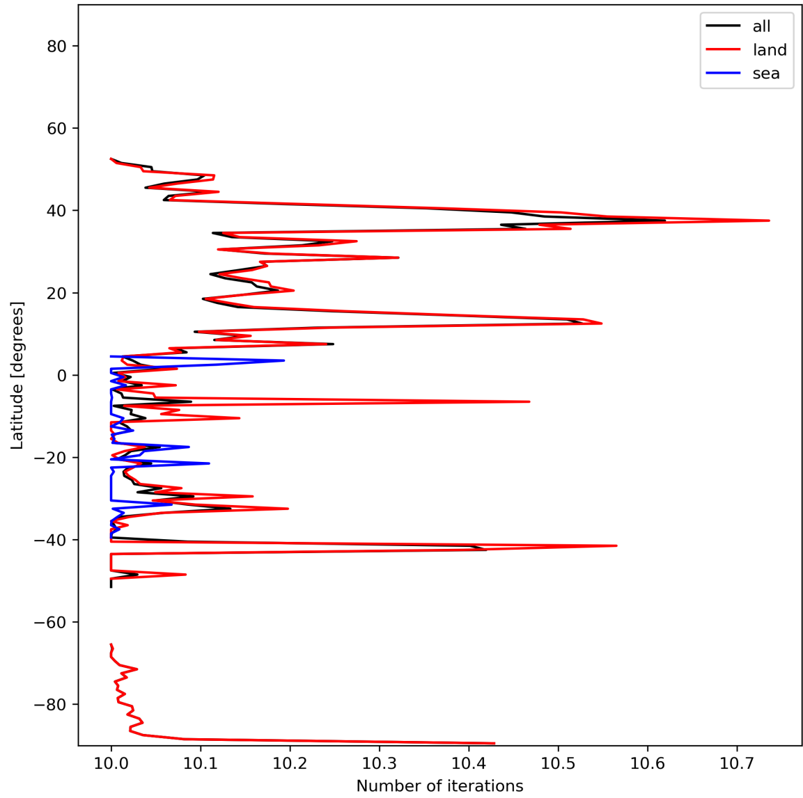
Figure 20: Zonal average of “Number of iterations” for 2024-01-05 to 2024-01-06.
