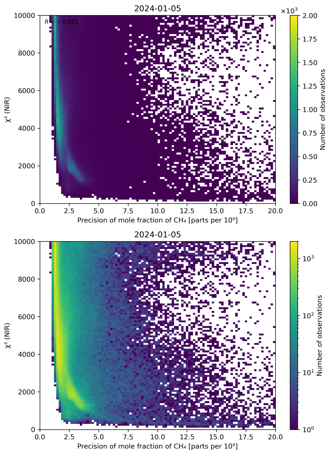
Figure 78: Scatter density plot of “Precision of mole fraction of CH 4 ” against “ \chi^2 (NIR)” for 2024-01-05 to 2024-01-06.
