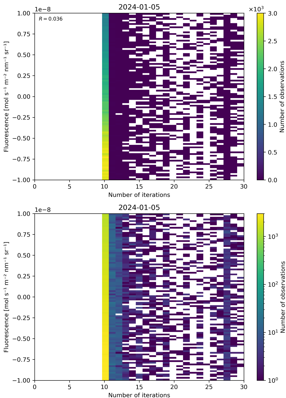
Figure 87: Scatter density plot of “Number of iterations” against “Fluorescence” for 2024-01-05 to 2024-01-06.
