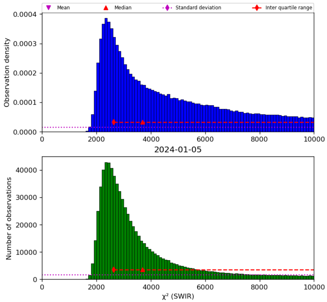
Figure 28: Histogram of “ \chi^2 (SWIR)” for 2024-01-05 to 2024-01-06
