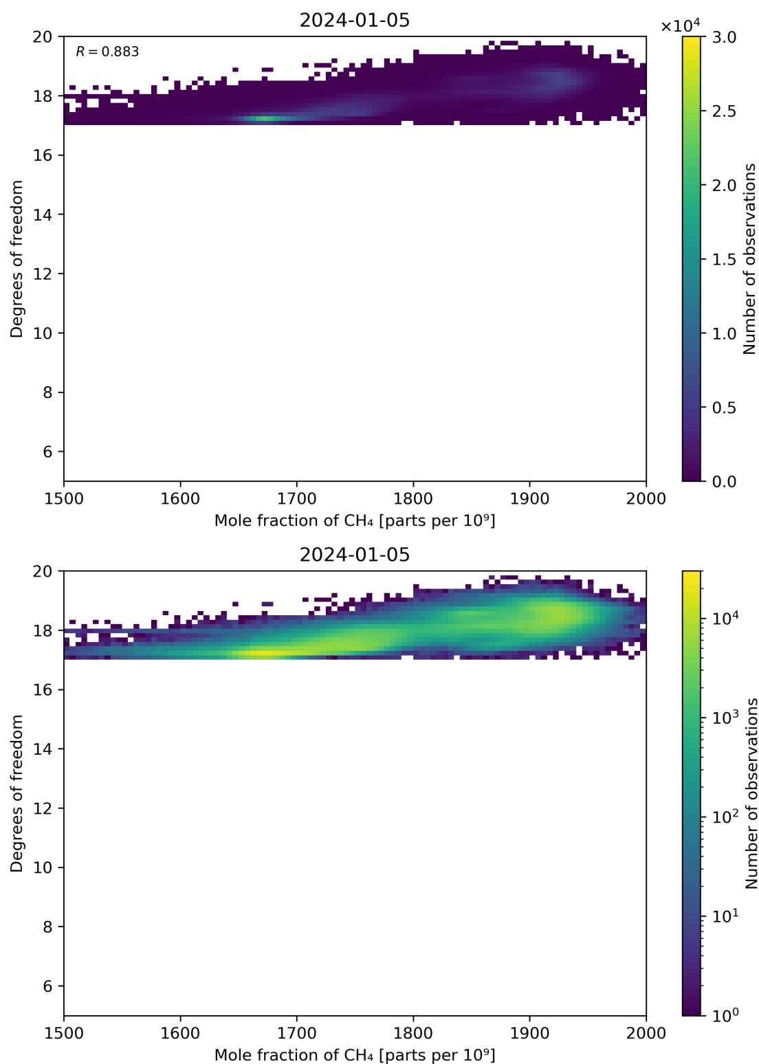
Figure 72: Scatter density plot of “Mole fraction of CH 4 ” against “Degrees of freedom” for 2024-01-05 to 2024-01-06.
