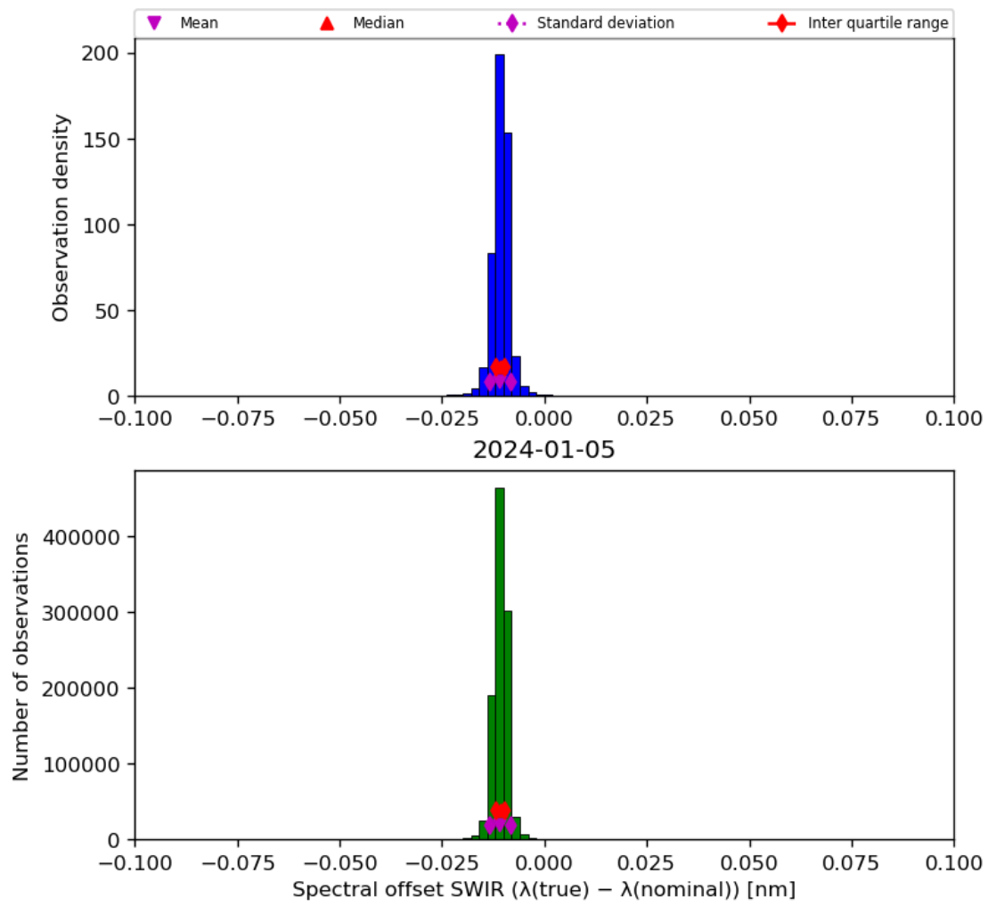
Figure 27: Histogram of “Spectral offset SWIR ( \lambda(\text{true}) - \lambda(\text{nominal}) )” for 2024-01-05 to 2024-01-06
