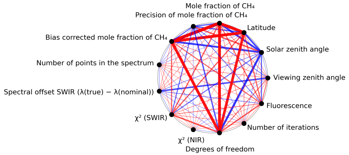
Figure 1: Map of correlation graph for 2024-01-05 to 2024-01-06.
