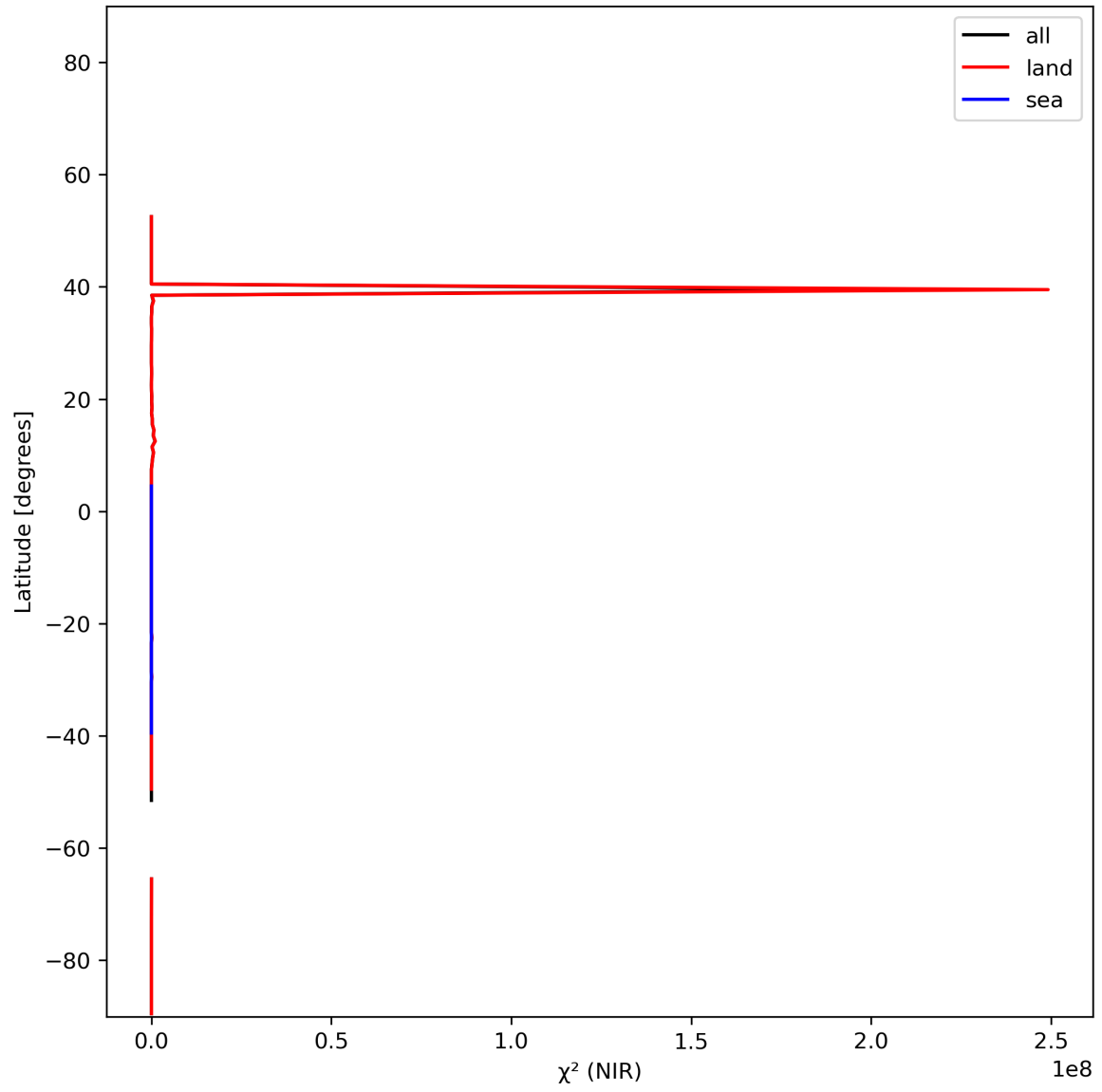
Figure 18: Zonal average of “ \chi^2 (NIR)” for 2024-01-05 to 2024-01-06.
