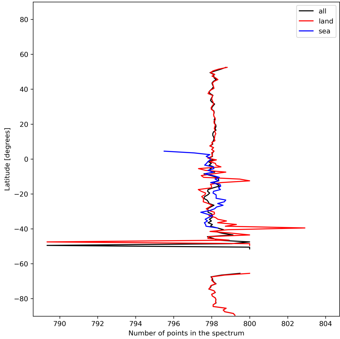
Figure 15: Zonal average of “Number of points in the spectrum” for 2024-01-05 to 2024-01-06.
