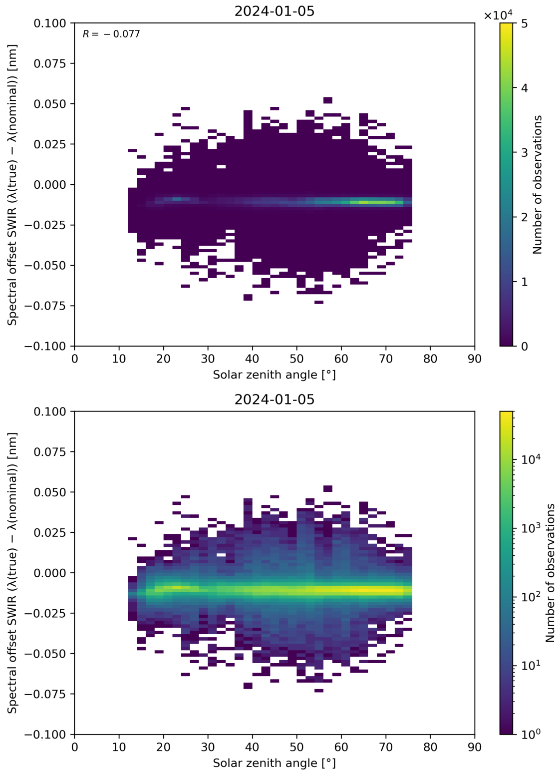
Figure 104: Scatter density plot of “Solar zenith angle” against “Spectral offset SWIR ( \lambda(\text{true}) - \lambda(\text{nominal}) )” for 2024-01-05 to 2024-01-06.
