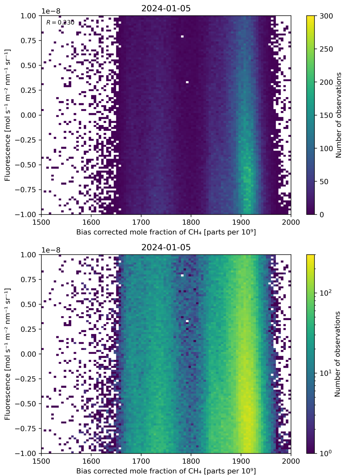
Figure 66: Scatter density plot of “Bias corrected mole fraction of \text{CH}_4 ” against “Fluorescence” for 2024-01-05 to 2024-01-06.
