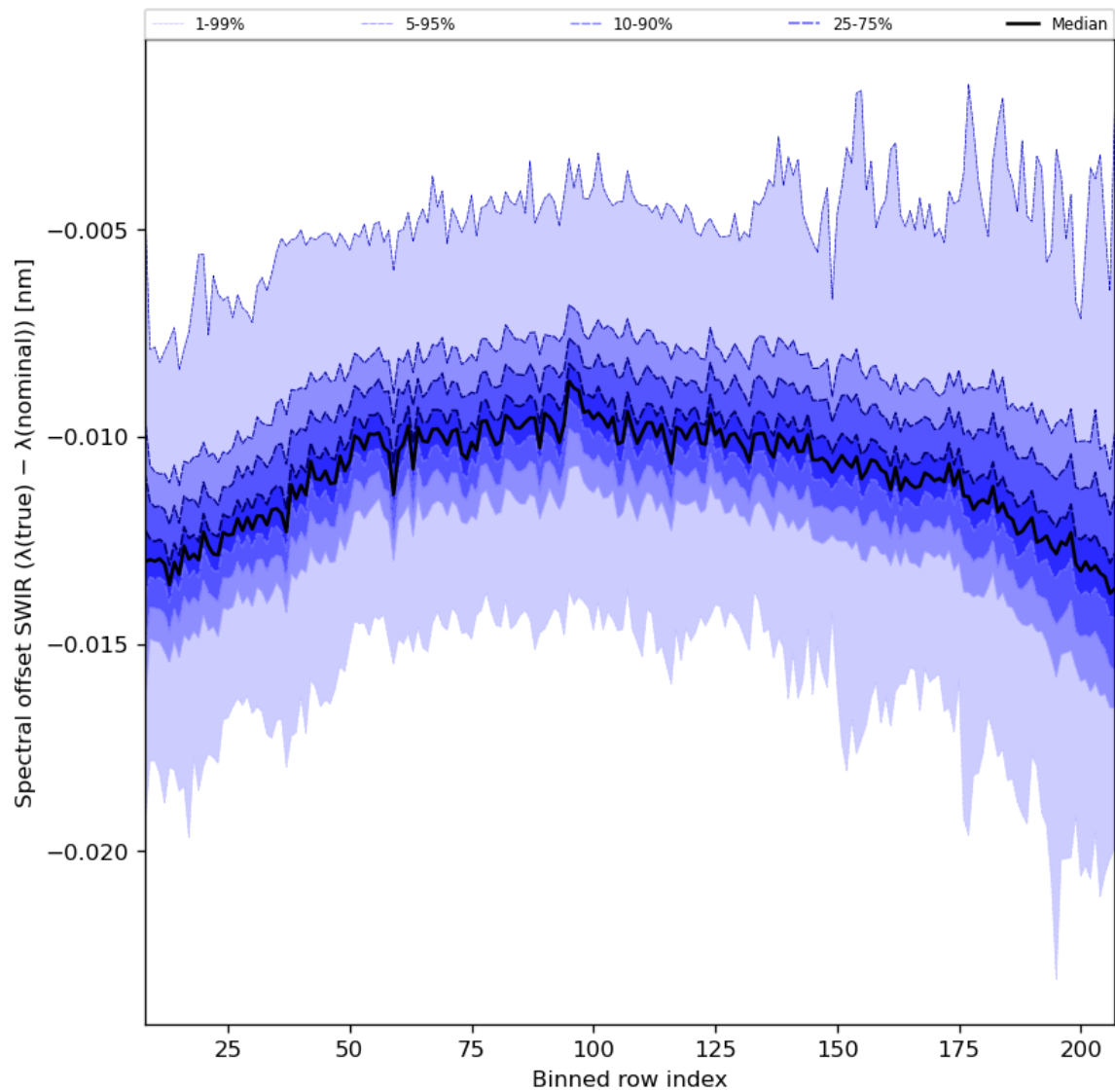
Figure 38: Along track statistics of “Spectral offset SWIR ( \lambda(\text{true}) - \lambda(\text{nominal}) )” for 2024-01-05 to 2024-01-06
