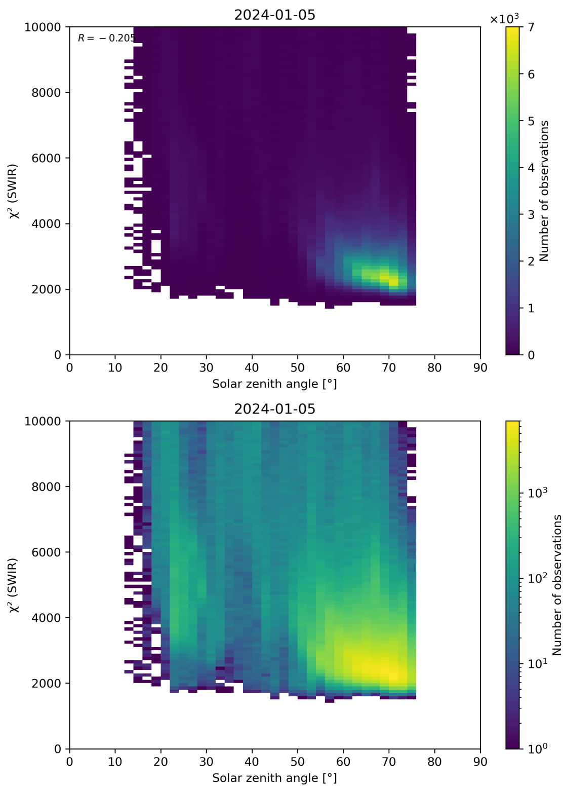
Figure 95: Scatter density plot of “Solar zenith angle” against “ \chi^2 (SWIR)” for 2024-01-05 to 2024-01-06.
