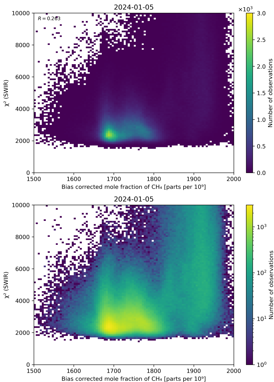
Figure 64: Scatter density plot of “Bias corrected mole fraction of \text{CH}_4 ” against “ \chi^2 (SWIR)” for 2024-01-05 to 2024-01-06.
