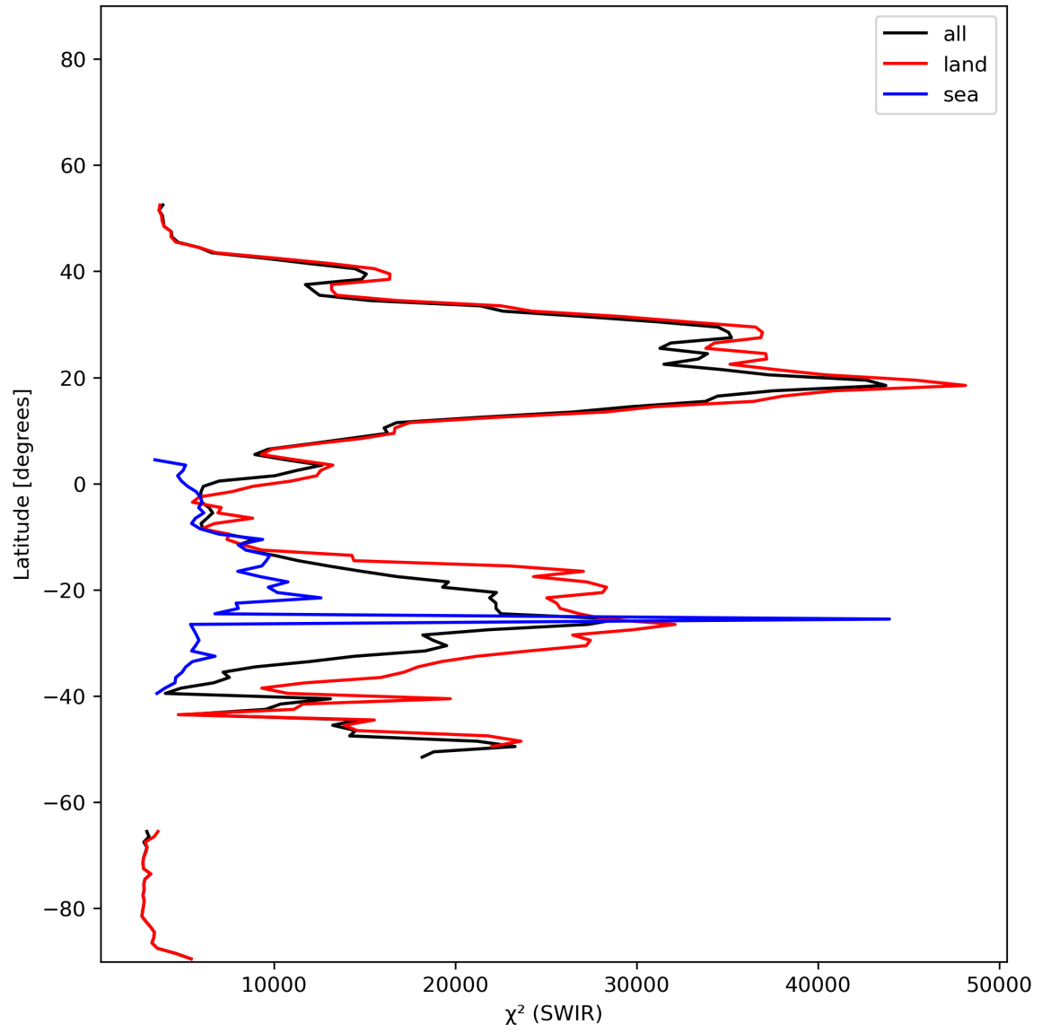
Figure 17: Zonal average of “ \chi^2 (SWIR)” for 2024-01-05 to 2024-01-06.
