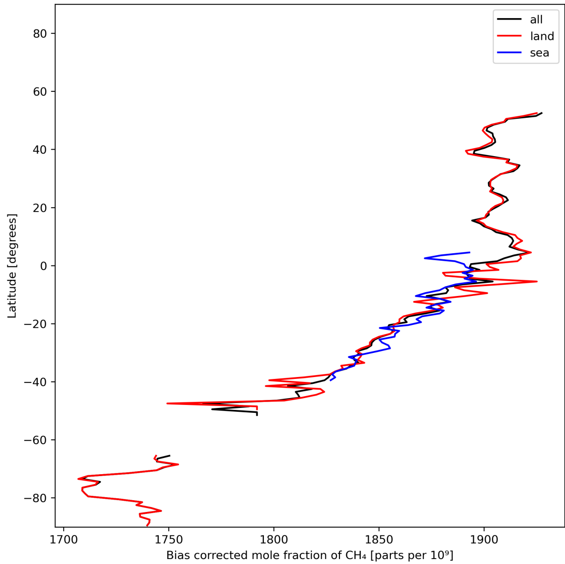
Figure 14: Zonal average of “Bias corrected mole fraction of CH 4 ” for 2024-01-05 to 2024-01-06.
