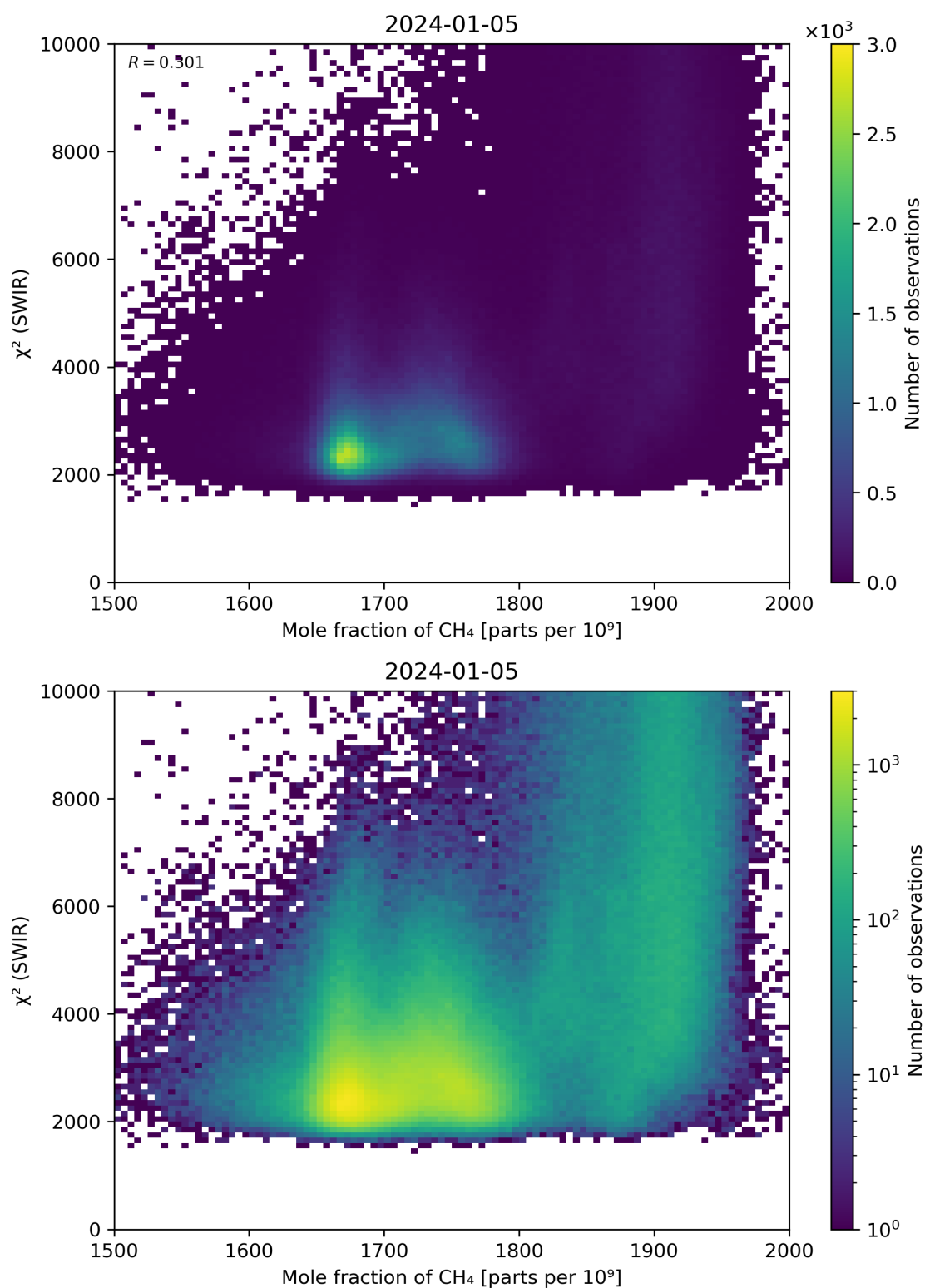
Figure 71: Scatter density plot of “Mole fraction of \text{CH}_4 ” against “ \chi^2 (SWIR)” for 2024-01-05 to 2024-01-06.
