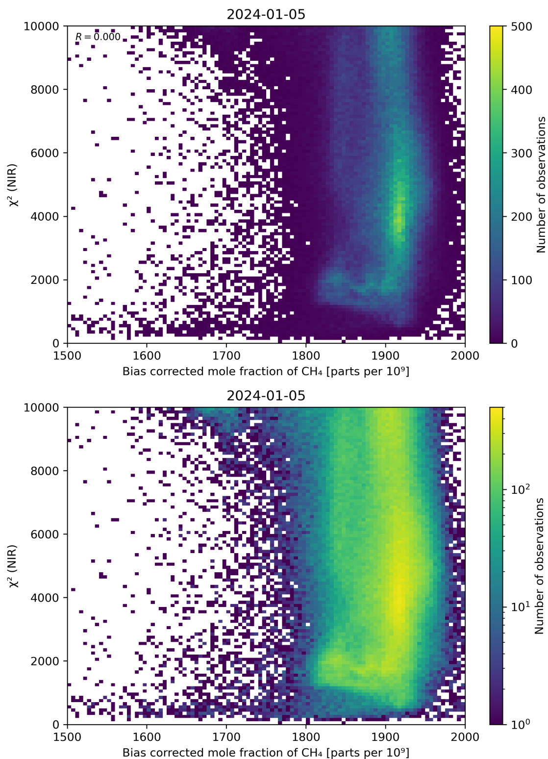
Figure 63: Scatter density plot of “Bias corrected mole fraction of CH 4 ” against “ \chi^2 (NIR)” for 2024-01-05 to 2024-01-06.
