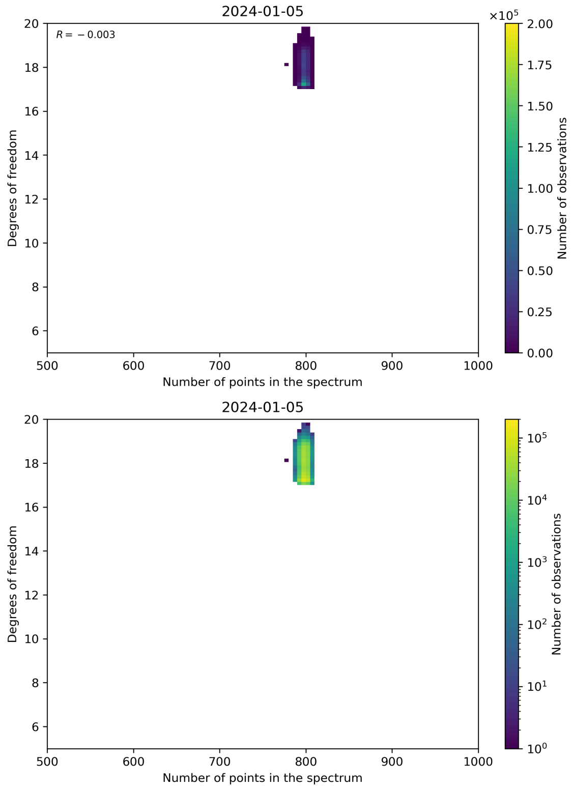
Figure 90: Scatter density plot of “Number of points in the spectrum” against “Degrees of freedom” for 2024-01-05 to 2024-01-06.
