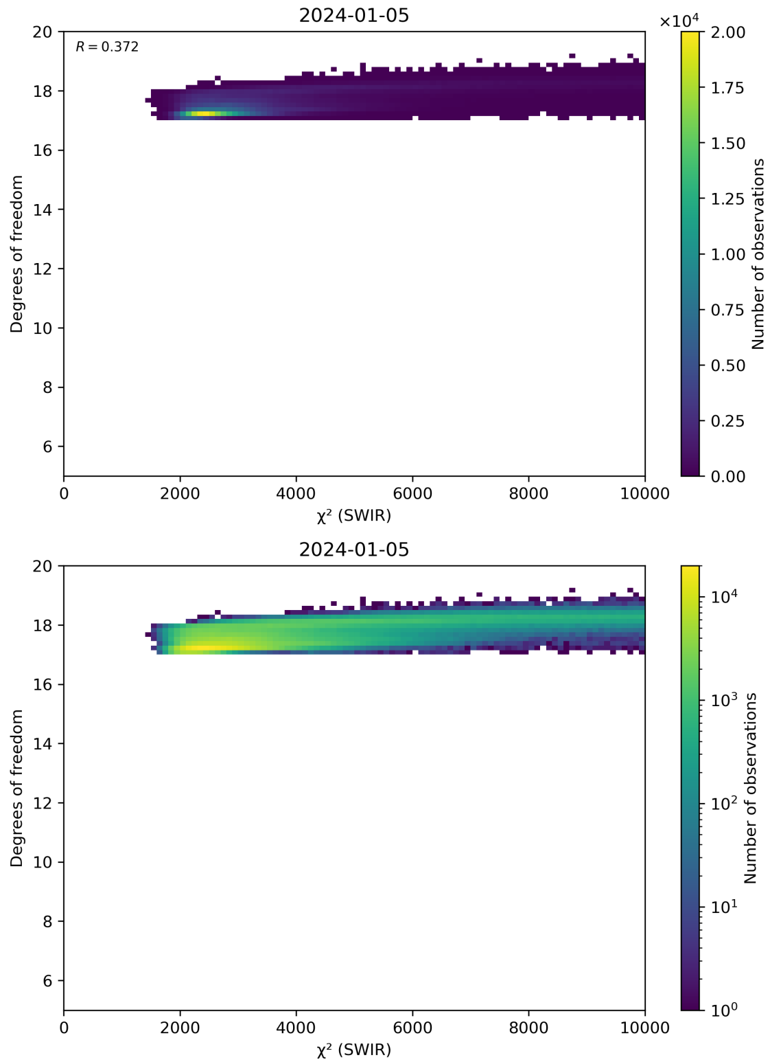
Figure 48: Scatter density plot of “ \chi^2 (SWIR)” against “Degrees of freedom” for 2024-01-05 to 2024-01-06.
