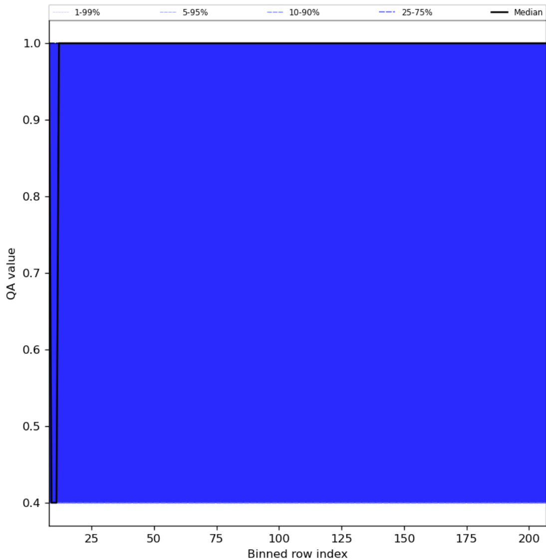
Figure 33: Along track statistics of “QA value” for 2024-01-05 to 2024-01-06
