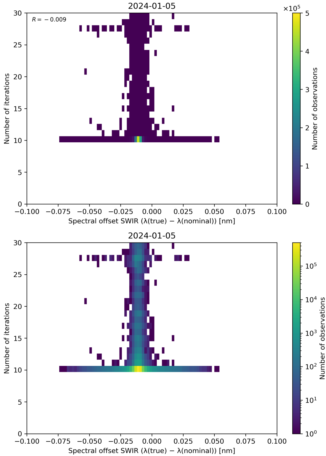
Figure 121: Scatter density plot of “Spectral offset SWIR ( \lambda(\text{true}) - \lambda(\text{nominal}) )” against “Number of iterations” for 2024-01-05 to 2024-01-06.
