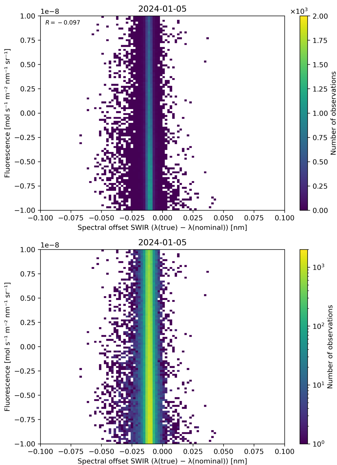
Figure 120: Scatter density plot of “Spectral offset SWIR ( \lambda(\text{true}) - \lambda(\text{nominal}) )” against “Fluorescence” for 2024-01-05 to 2024-01-06.
