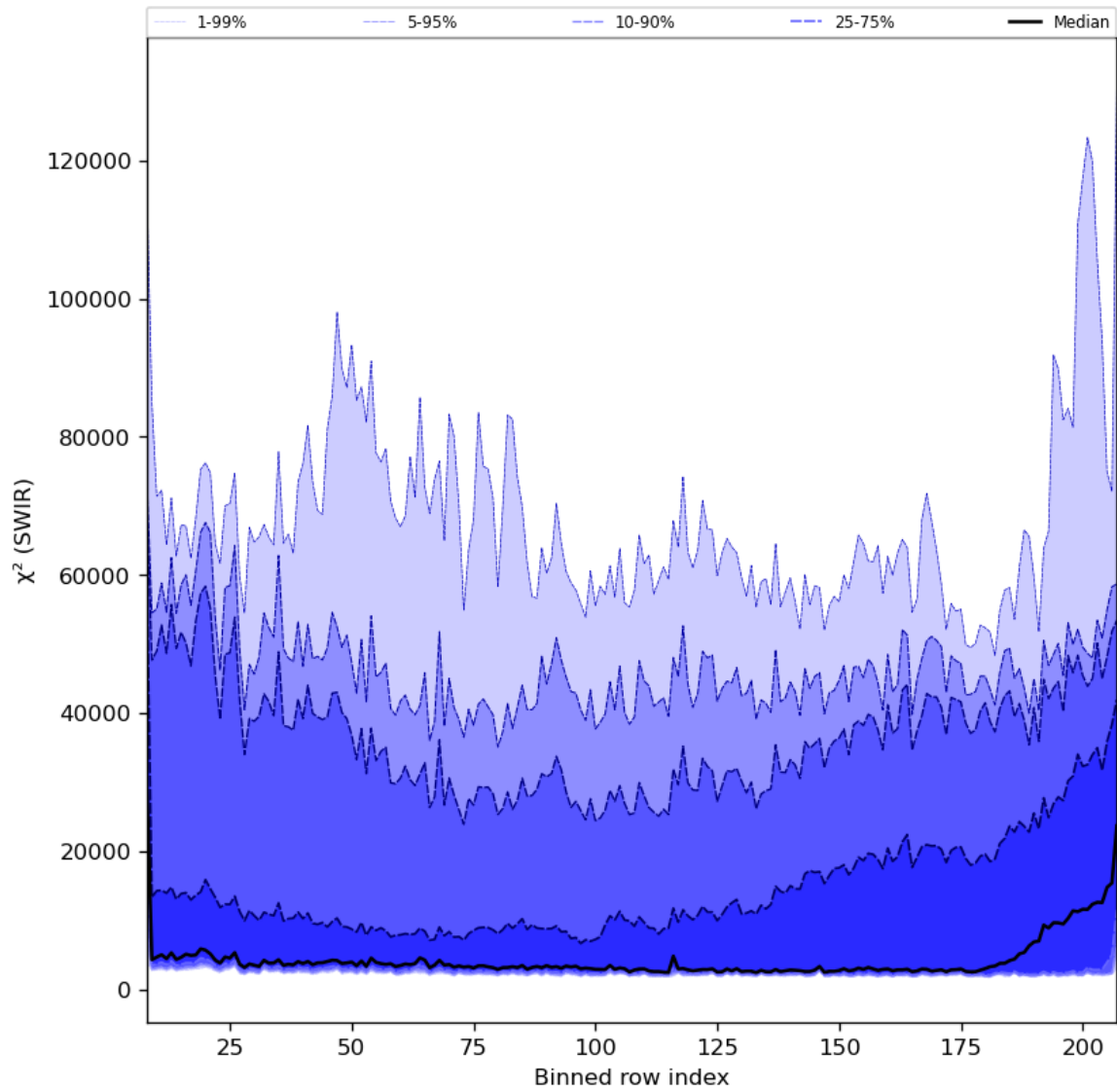
Figure 39: Along track statistics of " \chi^2 (SWIR)" for 2024-01-05 to 2024-01-06
