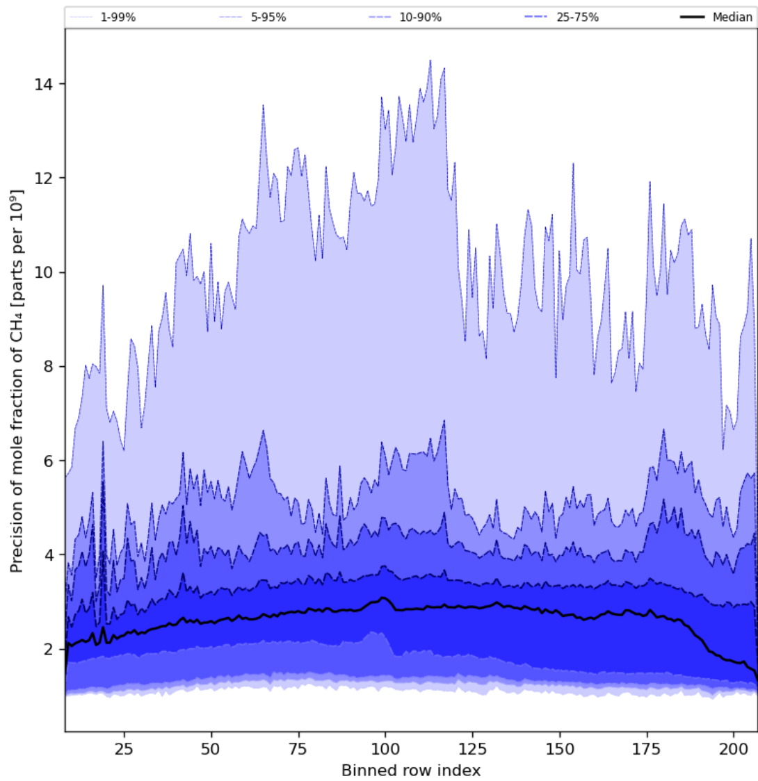
Figure 35: Along track statistics of “Precision of mole fraction of CH 4 ” for 2024-01-05 to 2024-01-06
