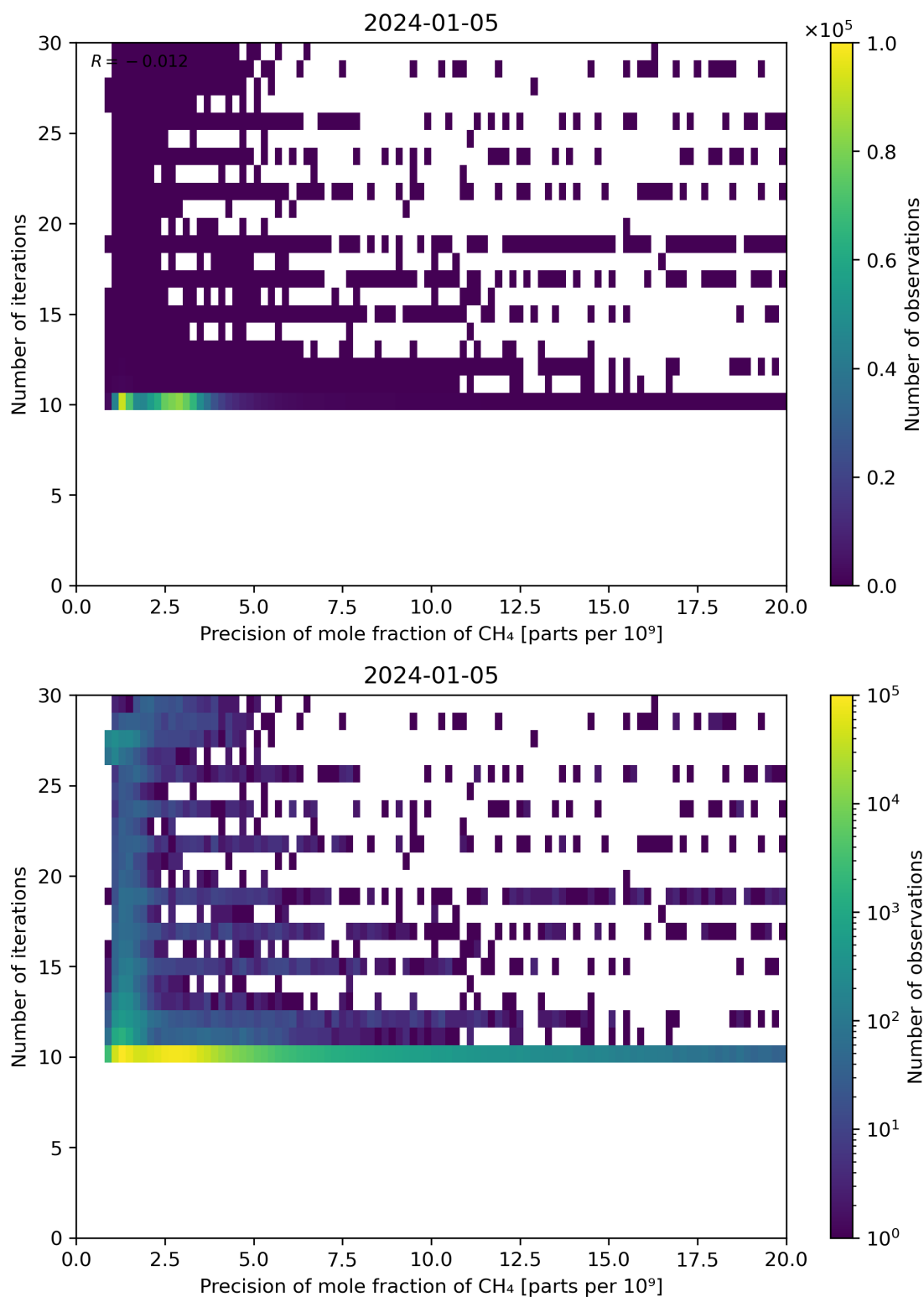
Figure 83: Scatter density plot of “Precision of mole fraction of CH 4 ” against “Number of iterations” for 2024-01-05 to 2024-01-06.
