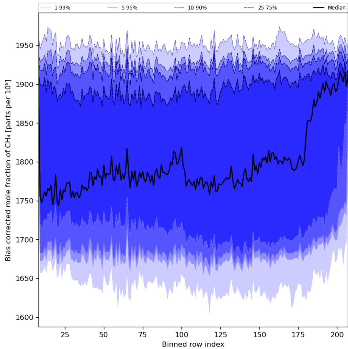
Figure 36: Along track statistics of “Bias corrected mole fraction of CH 4 ” for 2024-01-05 to 2024-01-06
