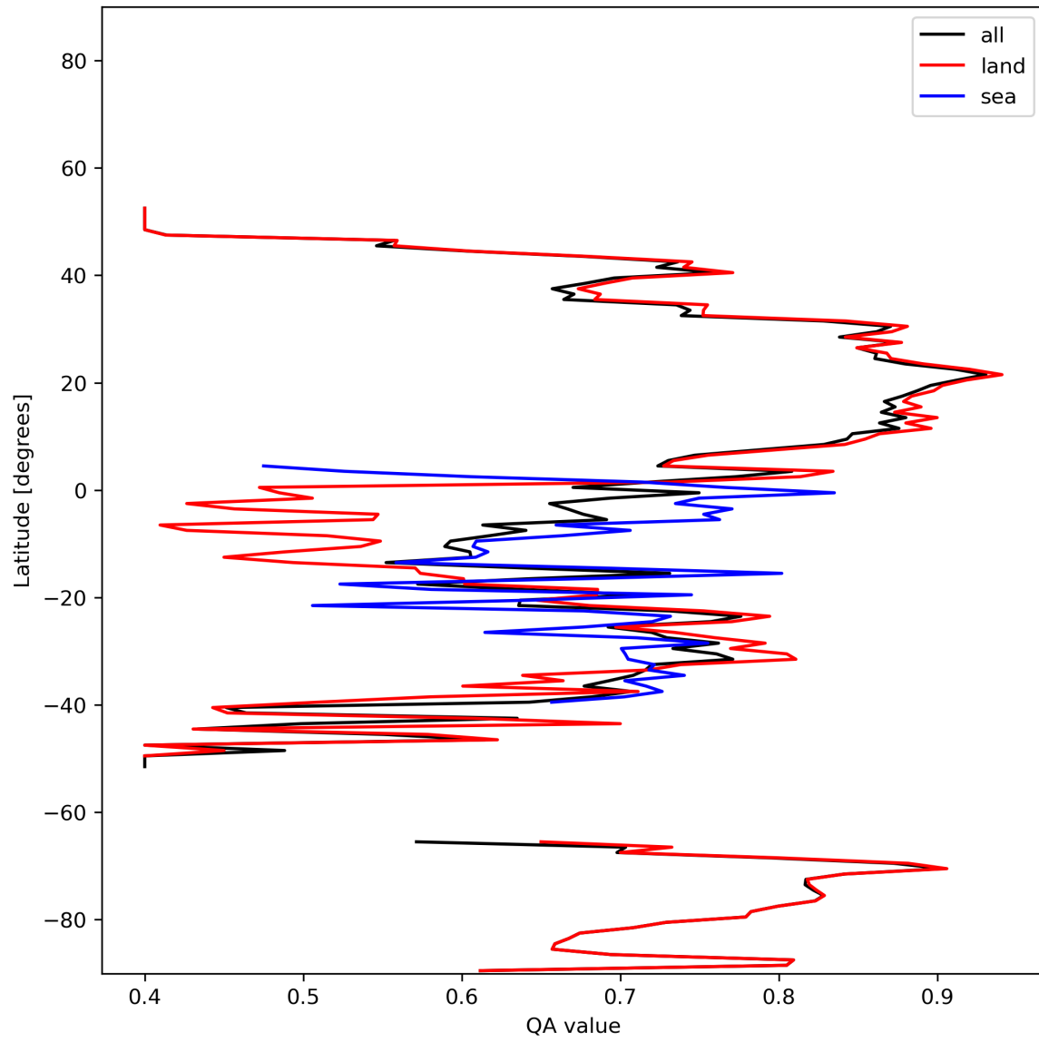
Figure 11: Zonal average of “QA value” for 2024-01-05 to 2024-01-06.
