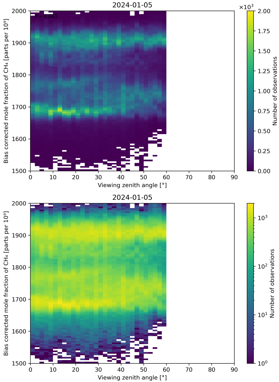
Figure 111: Scatter density plot of “Viewing zenith angle” against “Bias corrected mole fraction of CH 4 ” for 2024-01-05 to 2024-01-06.
