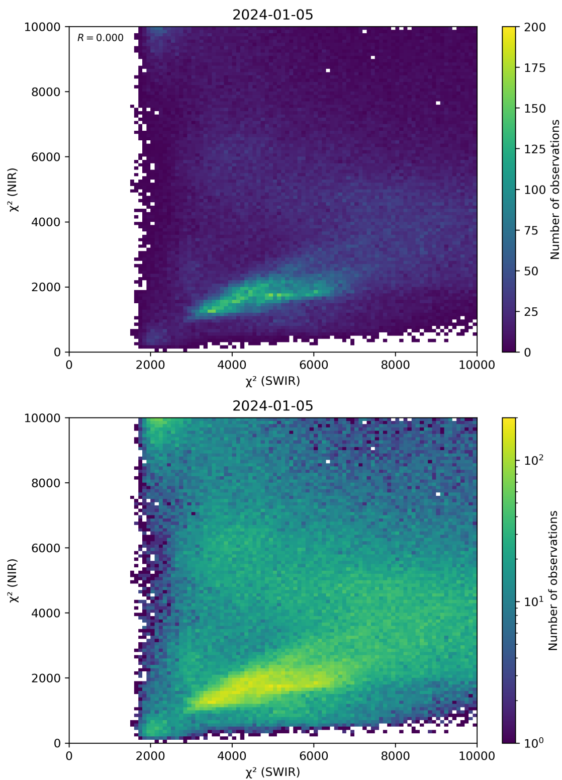
Figure 47: Scatter density plot of “ \chi^2 (SWIR)” against “ \chi^2 (NIR)” for 2024-01-05 to 2024-01-06.
