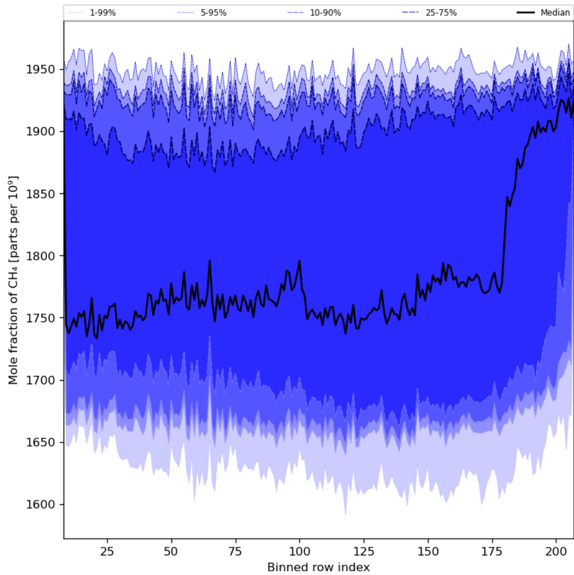
Figure 34: Along track statistics of “Mole fraction of CH 4 ” for 2024-01-05 to 2024-01-06
