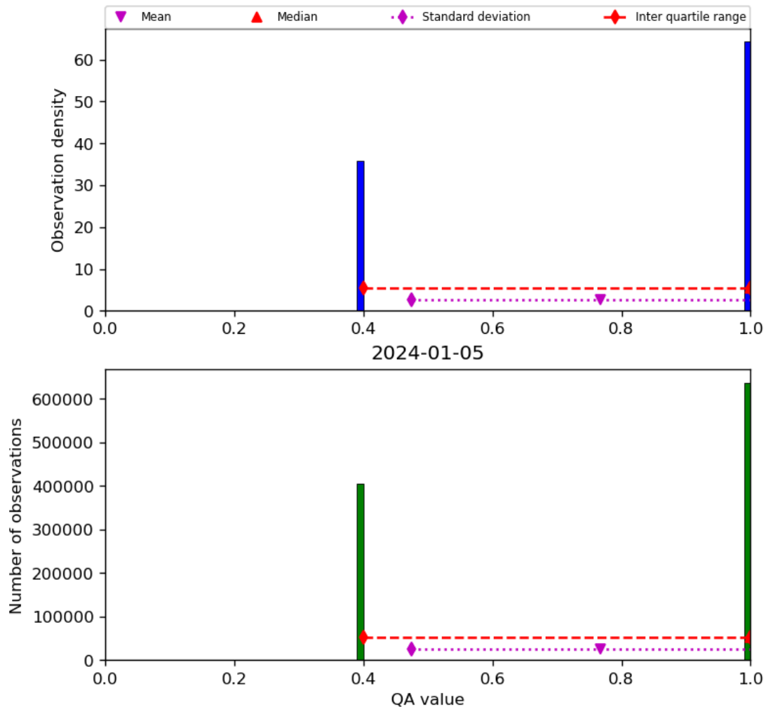
Figure 22: Histogram of “QA value” for 2024-01-05 to 2024-01-06
