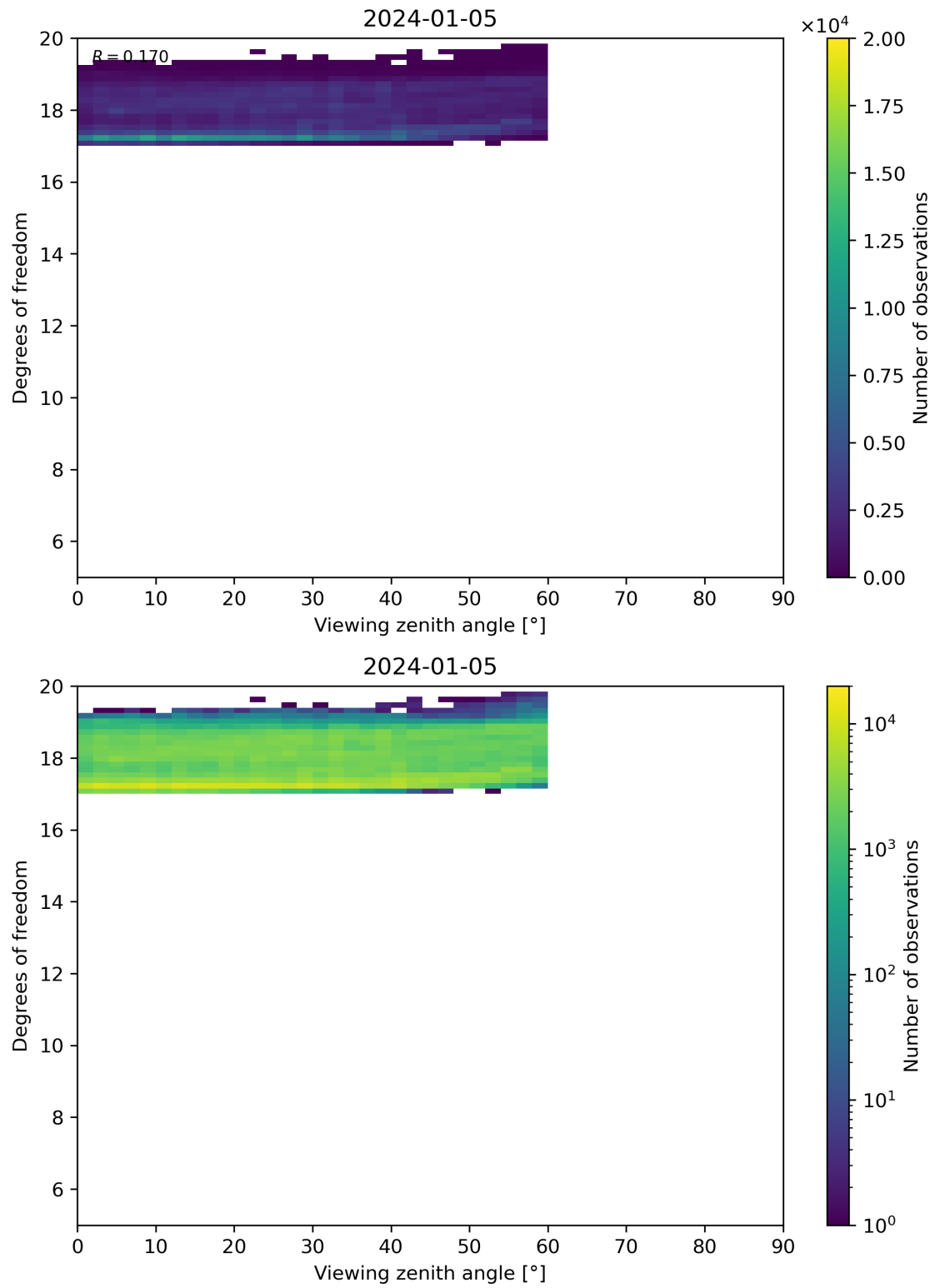
Figure 107: Scatter density plot of “Viewing zenith angle” against “Degrees of freedom” for 2024-01-05 to 2024-01-06.
