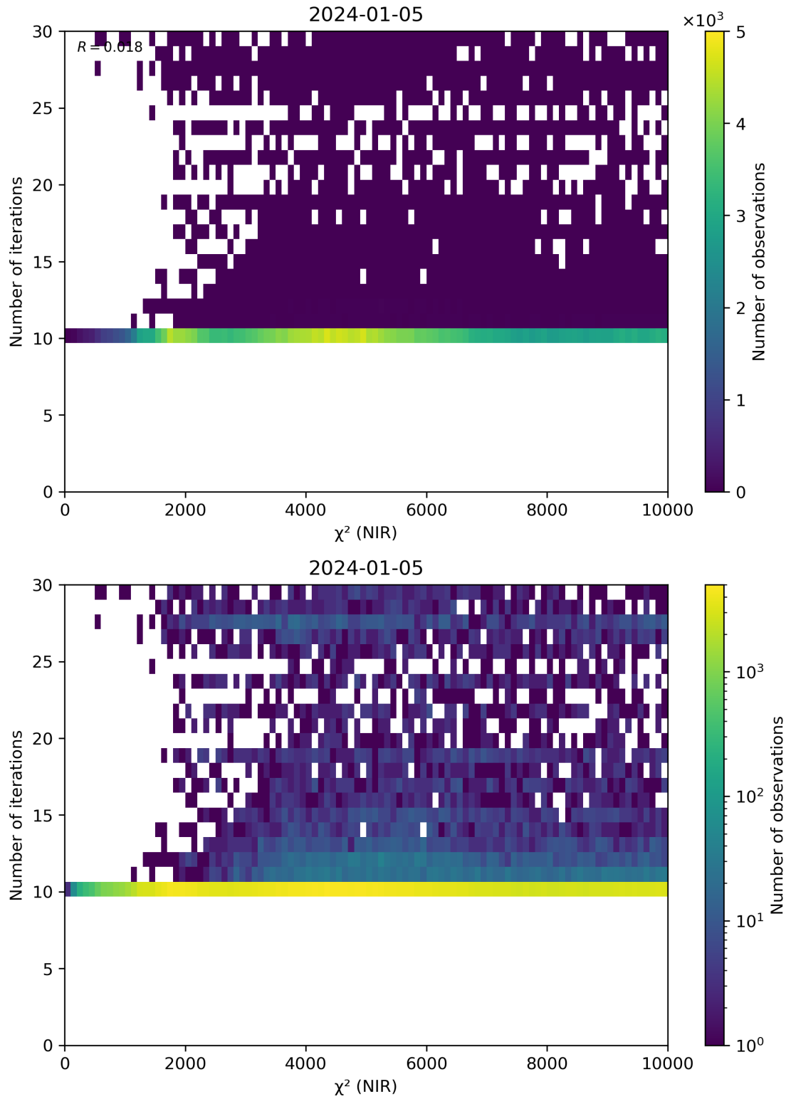
Figure 46: Scatter density plot of “ \chi^2 (NIR)” against “Number of iterations” for 2024-01-05 to 2024-01-06.
