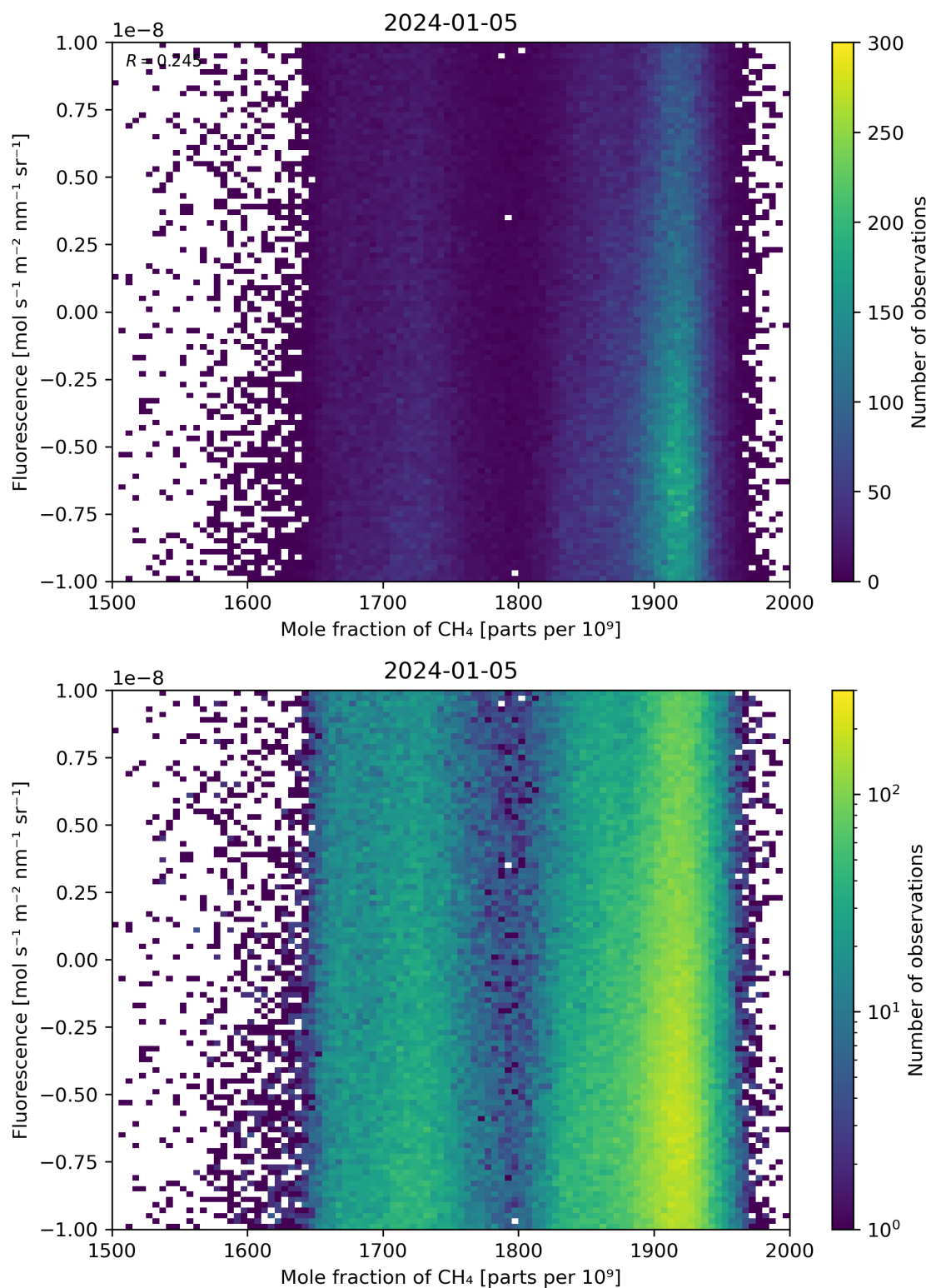
Figure 73: Scatter density plot of “Mole fraction of \text{CH}_4 ” against “Fluorescence” for 2024-01-05 to 2024-01-06.
