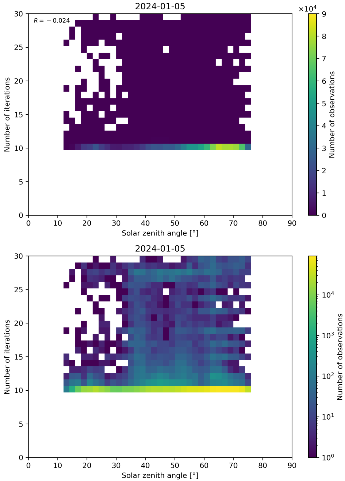
Figure 102: Scatter density plot of “Solar zenith angle” against “Number of iterations” for 2024-01-05 to 2024-01-06.
