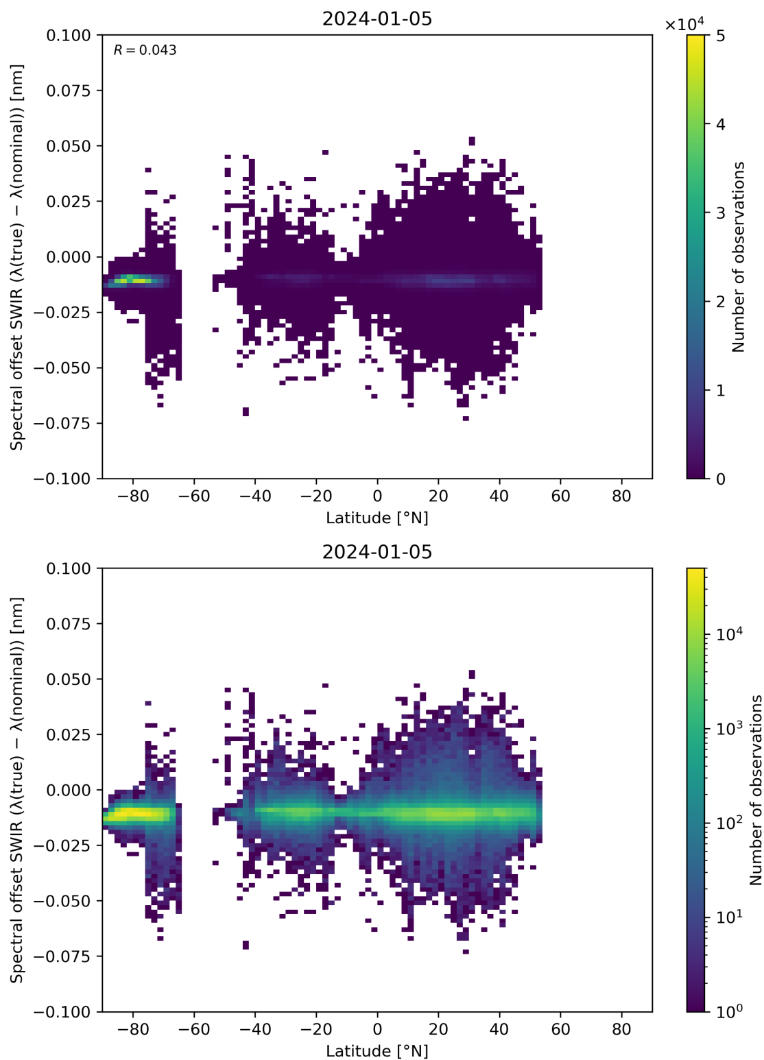
Figure 62: Scatter density plot of “Latitude” against “Spectral offset SWIR ( \lambda(\text{true}) - \lambda(\text{nominal}) )” for 2024-01-05 to 2024-01-06.
