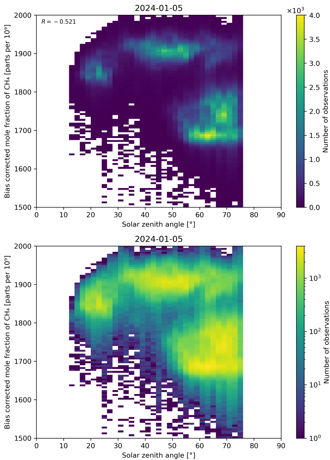
Figure 100: Scatter density plot of “Solar zenith angle” against “Bias corrected mole fraction of CH 4 ” for 2024-01-05 to 2024-01-06.
