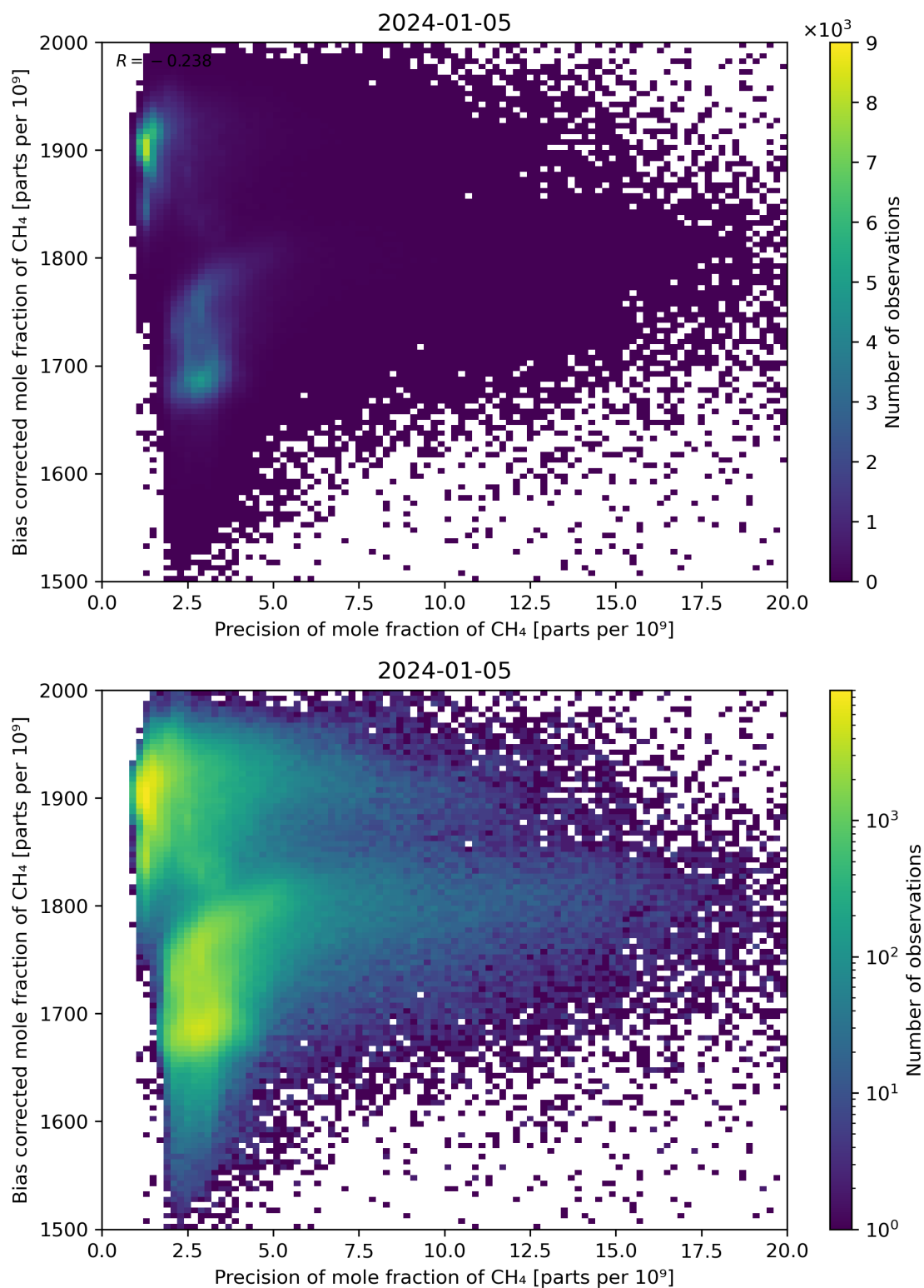
Figure 82: Scatter density plot of “Precision of mole fraction of CH 4 ” against “Bias corrected mole fraction of CH 4 ” for 2024-01-05 to 2024-01-06.
