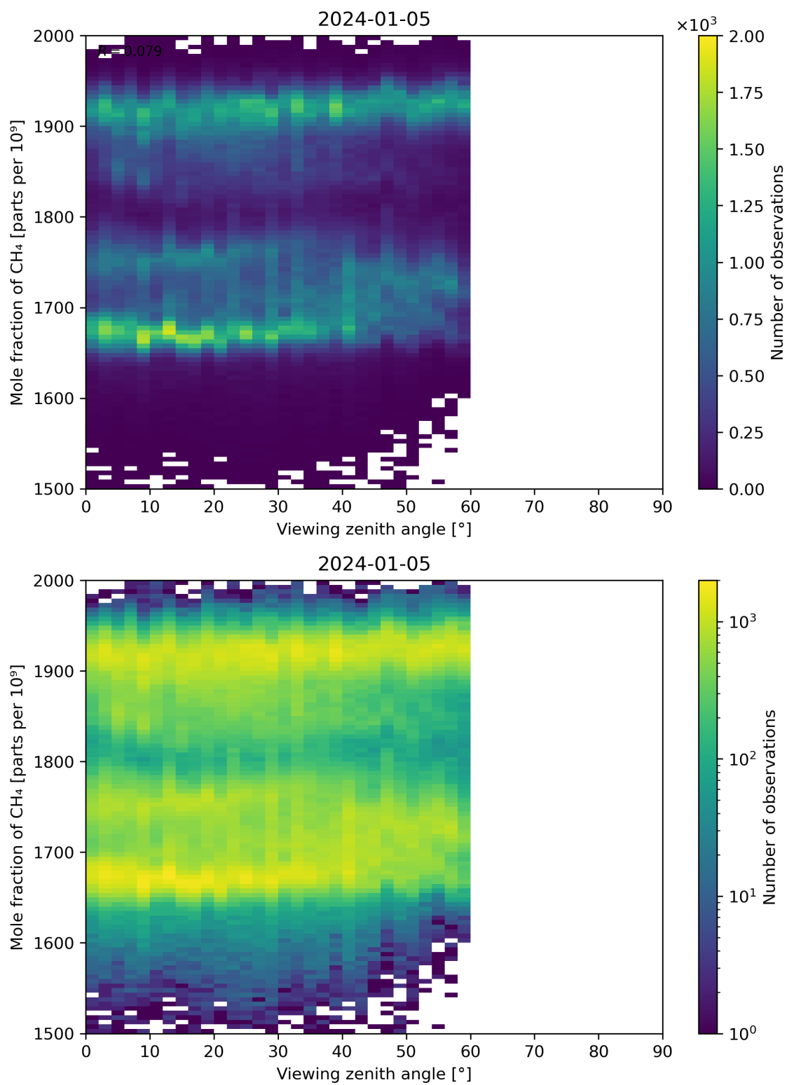
Figure 110: Scatter density plot of “Viewing zenith angle” against “Mole fraction of CH 4 ” for 2024-01-05 to 2024-01-06.
