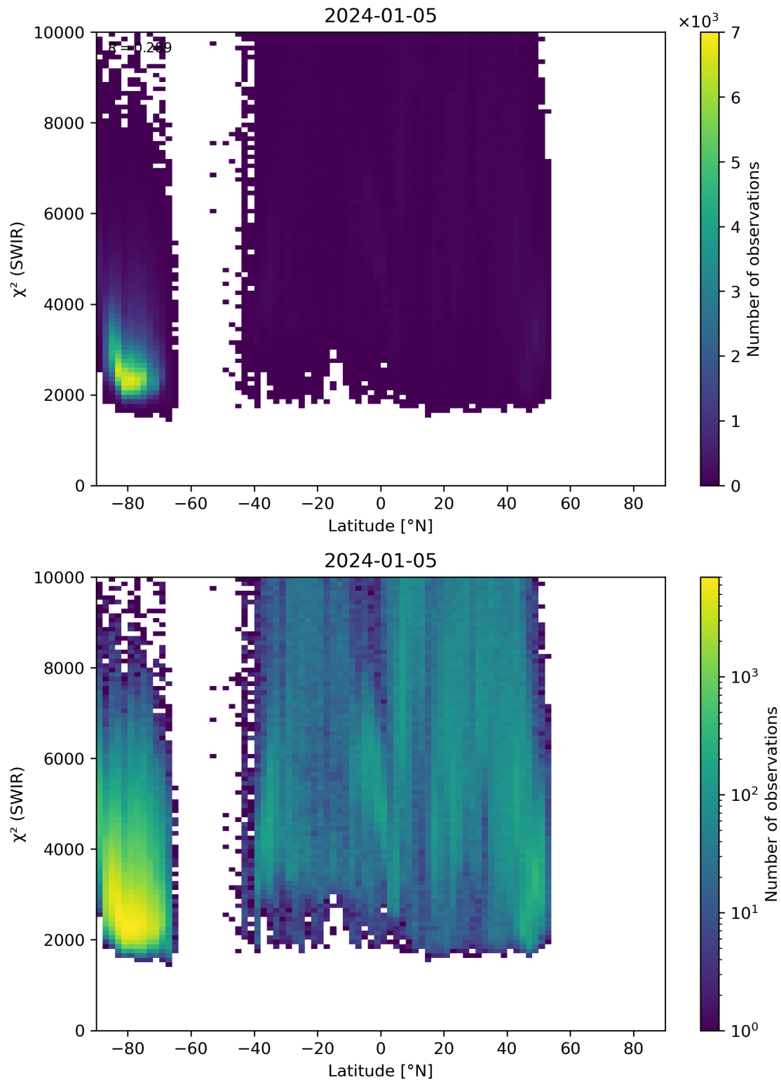
Figure 54: Scatter density plot of “Latitude” against “ \chi^2 (SWIR)” for 2024-01-05 to 2024-01-06.
