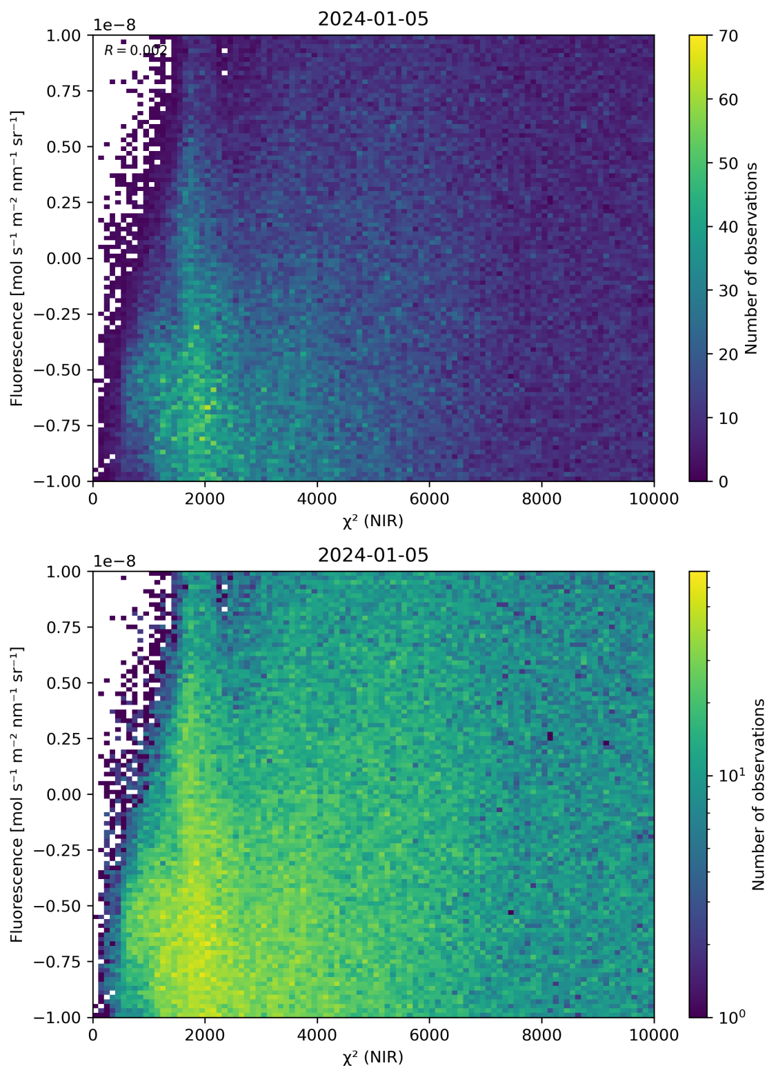
Figure 45: Scatter density plot of “ \chi^2 (NIR)” against “Fluorescence” for 2024-01-05 to 2024-01-06.
