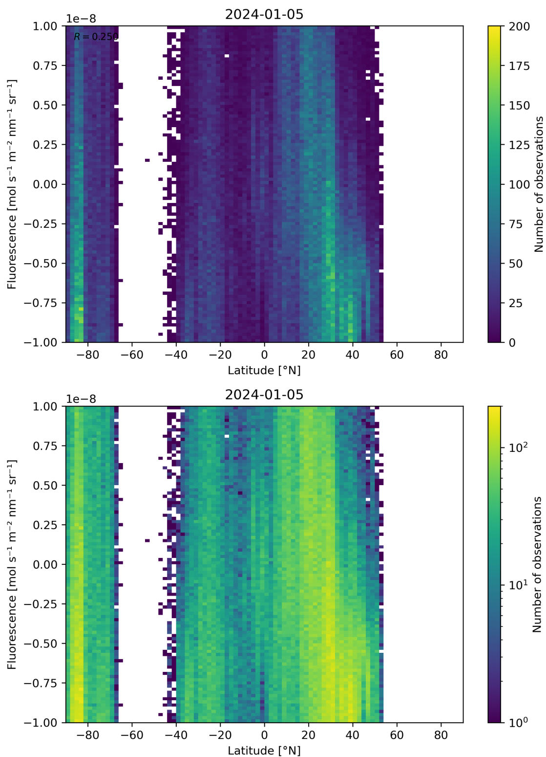
Figure 56: Scatter density plot of “Latitude” against “Fluorescence” for 2024-01-05 to 2024-01-06.
