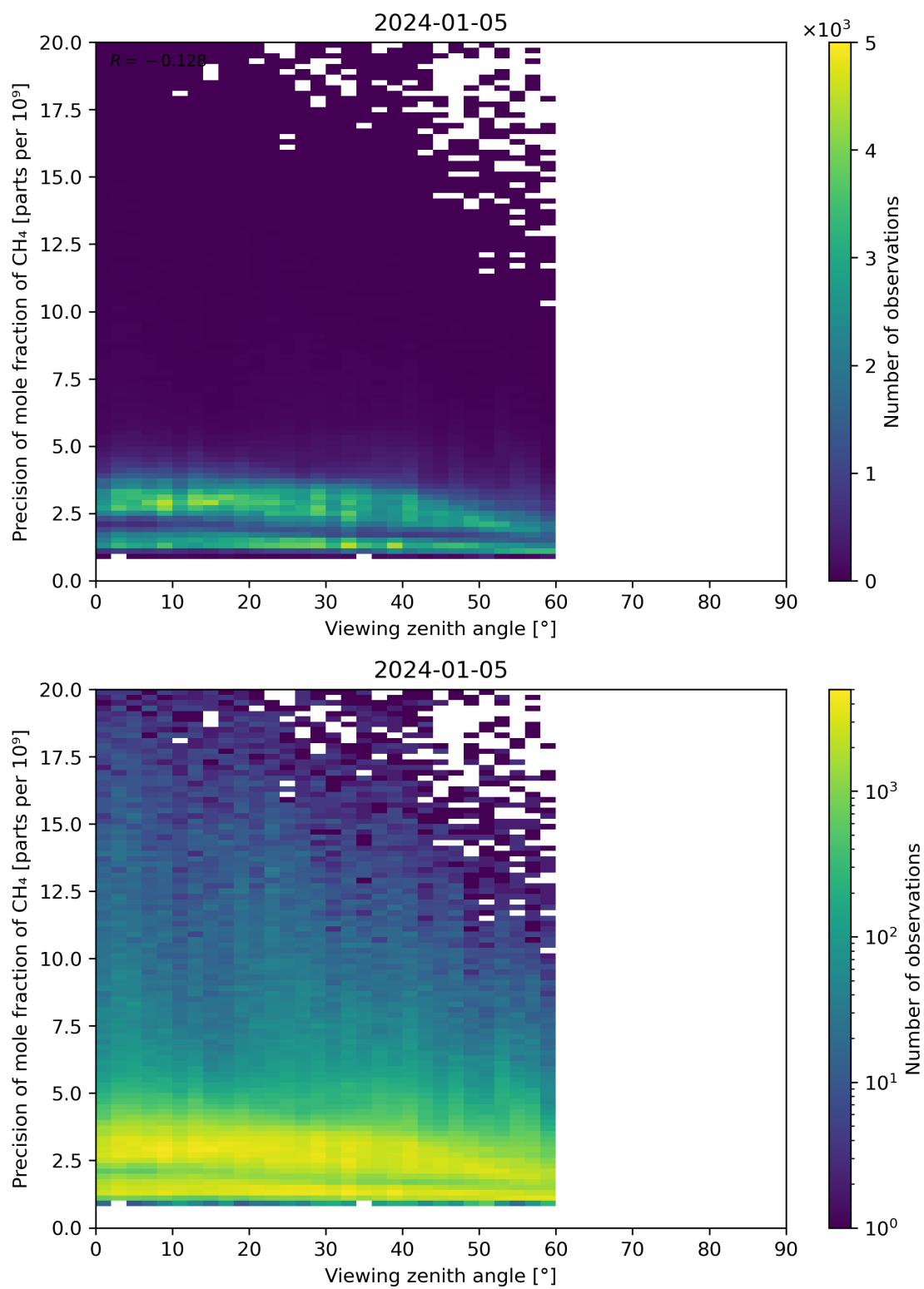
Figure 112: Scatter density plot of “Viewing zenith angle” against “Precision of mole fraction of CH 4 ” for 2024-01-05 to 2024-01-06.
