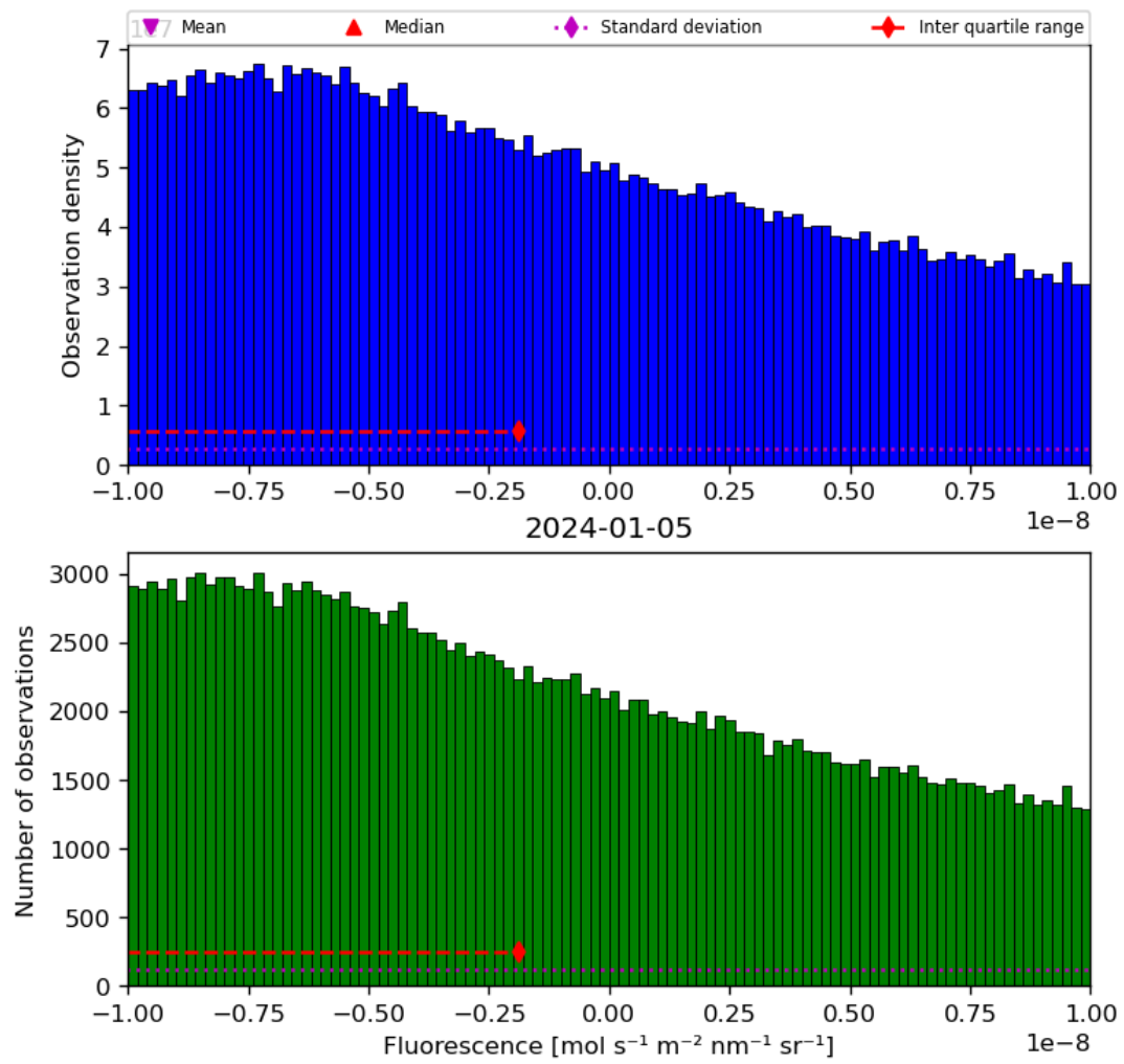
Figure 32: Histogram of “Fluorescence” for 2024-01-05 to 2024-01-06
