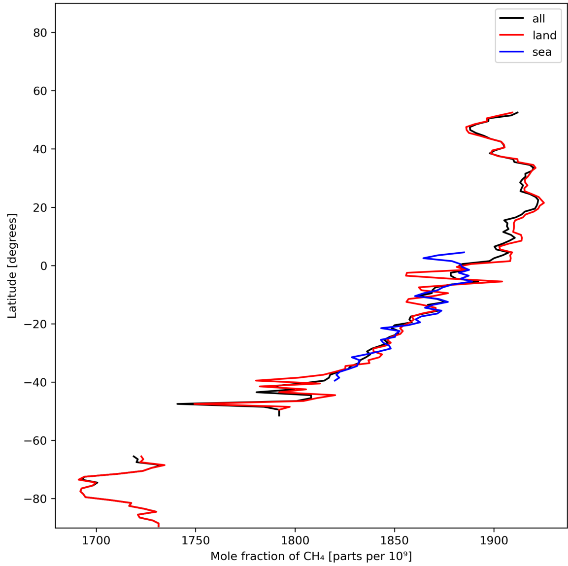
Figure 12: Zonal average of “Mole fraction of CH 4 ” for 2024-01-05 to 2024-01-06.
