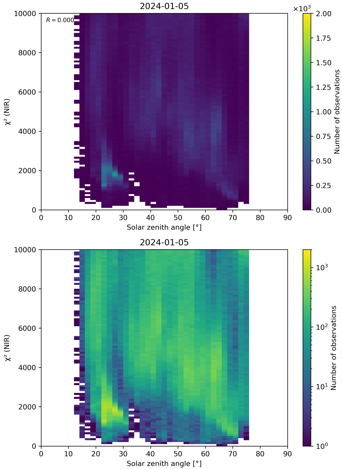
Figure 94: Scatter density plot of “Solar zenith angle” against “ \chi^2 (NIR)” for 2024-01-05 to 2024-01-06.
