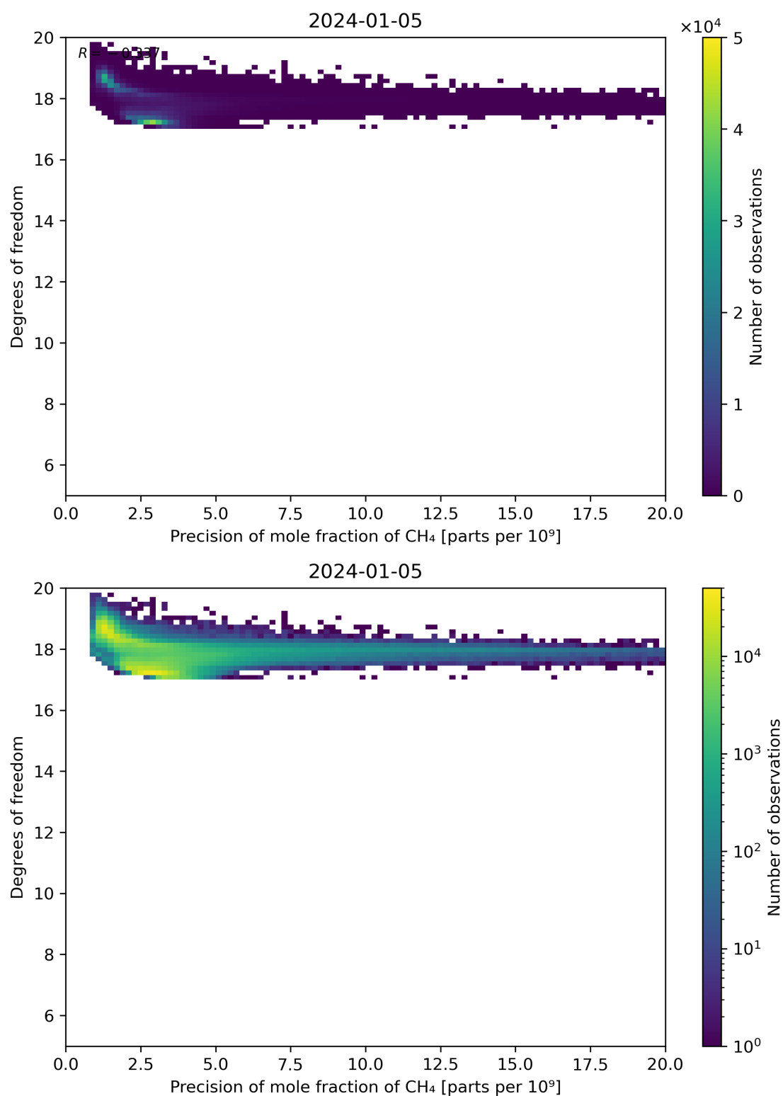
Figure 80: Scatter density plot of “Precision of mole fraction of CH 4 ” against “Degrees of freedom” for 2024-01-05 to 2024-01-06.
