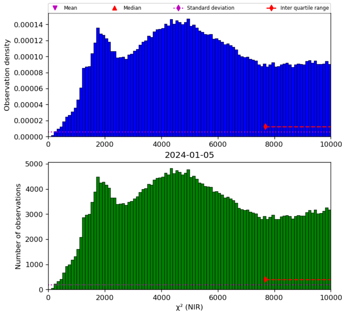
Figure 29: Histogram of “ \chi^2 (NIR)” for 2024-01-05 to 2024-01-06
