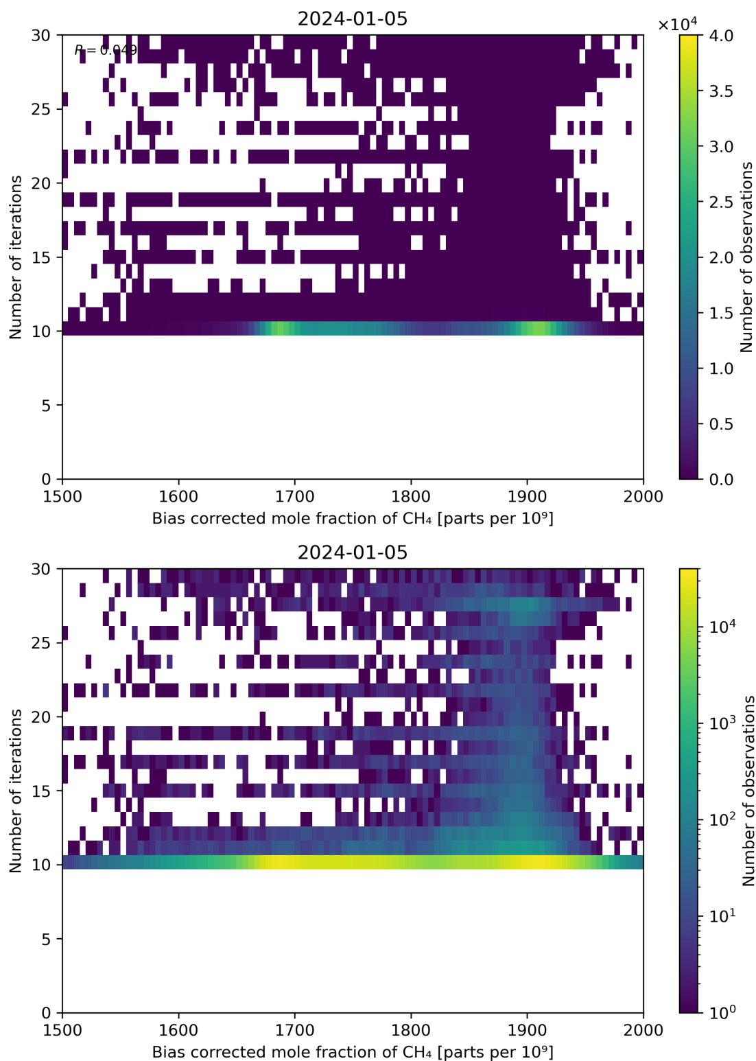
Figure 67: Scatter density plot of “Bias corrected mole fraction of CH 4 ” against “Number of iterations” for 2024-01-05 to 2024-01-06.
