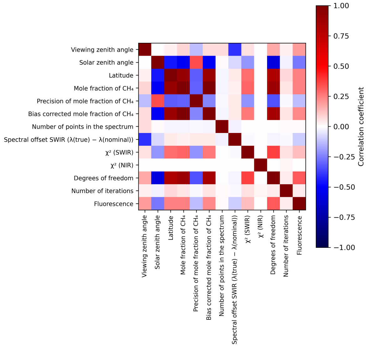
Figure 2: Map of correlation matrix for 2024-01-05 to 2024-01-06.
