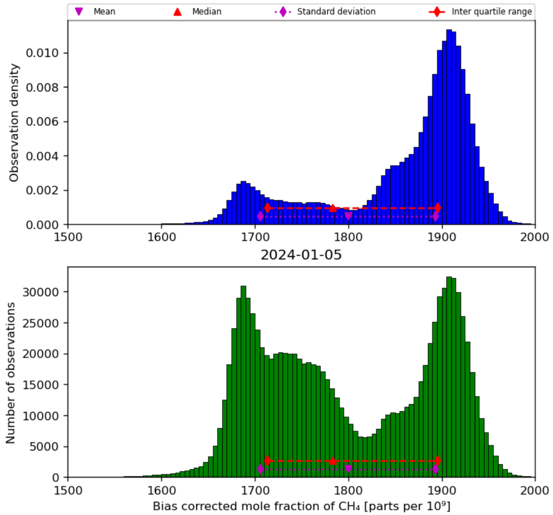
Figure 25: Histogram of “Bias corrected mole fraction of CH 4 ” for 2024-01-05 to 2024-01-06
