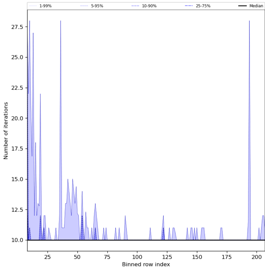
Figure 42: Along track statistics of “Number of iterations” for 2024-01-05 to 2024-01-06
