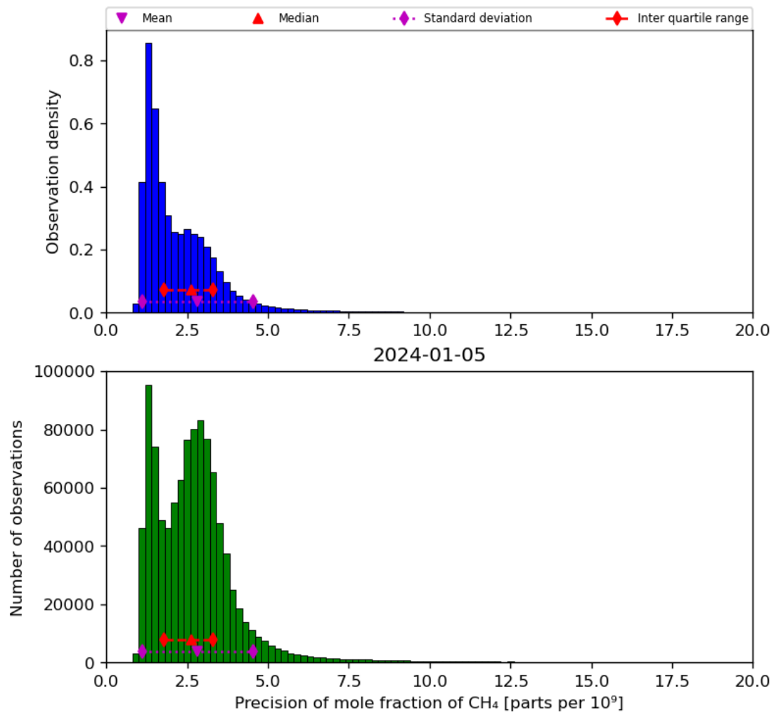
Figure 24: Histogram of “Precision of mole fraction of CH 4 ” for 2024-01-05 to 2024-01-06
