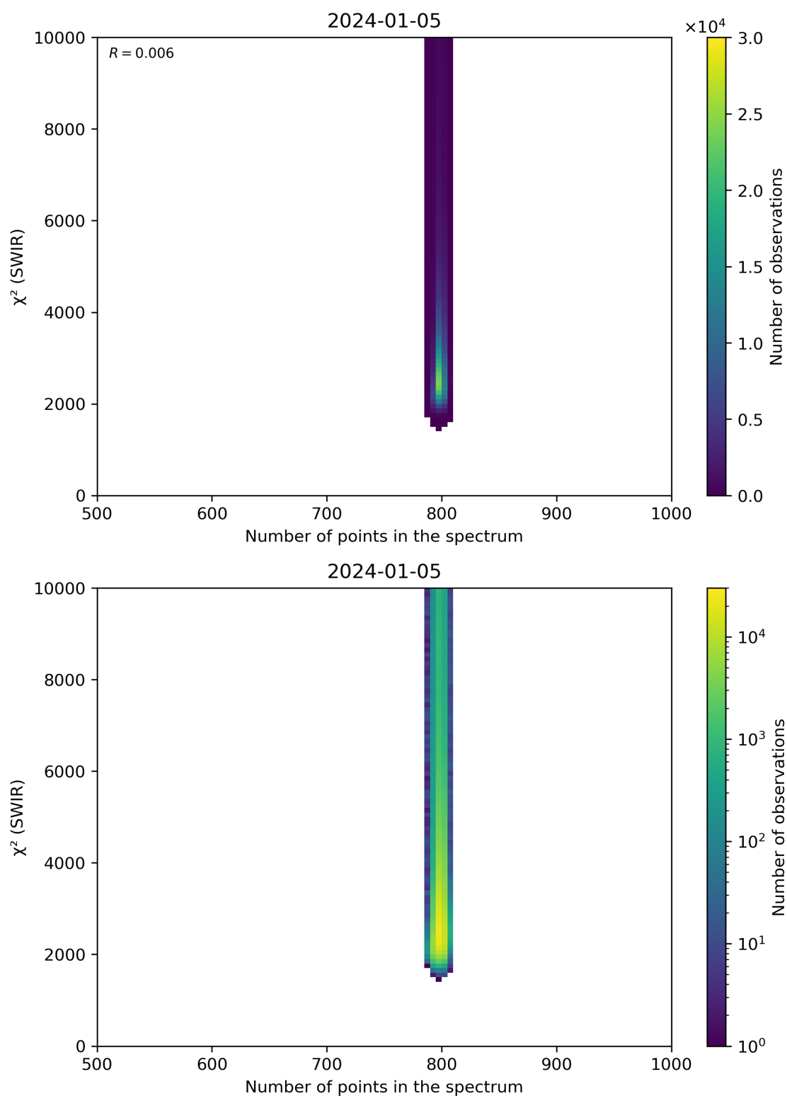
Figure 89: Scatter density plot of “Number of points in the spectrum” against “ \chi^2 (SWIR)” for 2024-01-05 to 2024-01-06.
