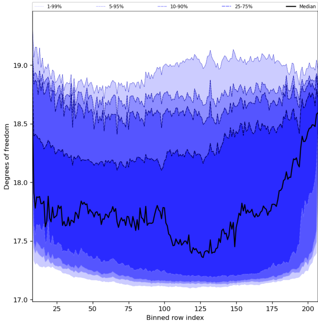
Figure 41: Along track statistics of “Degrees of freedom” for 2024-01-05 to 2024-01-06
