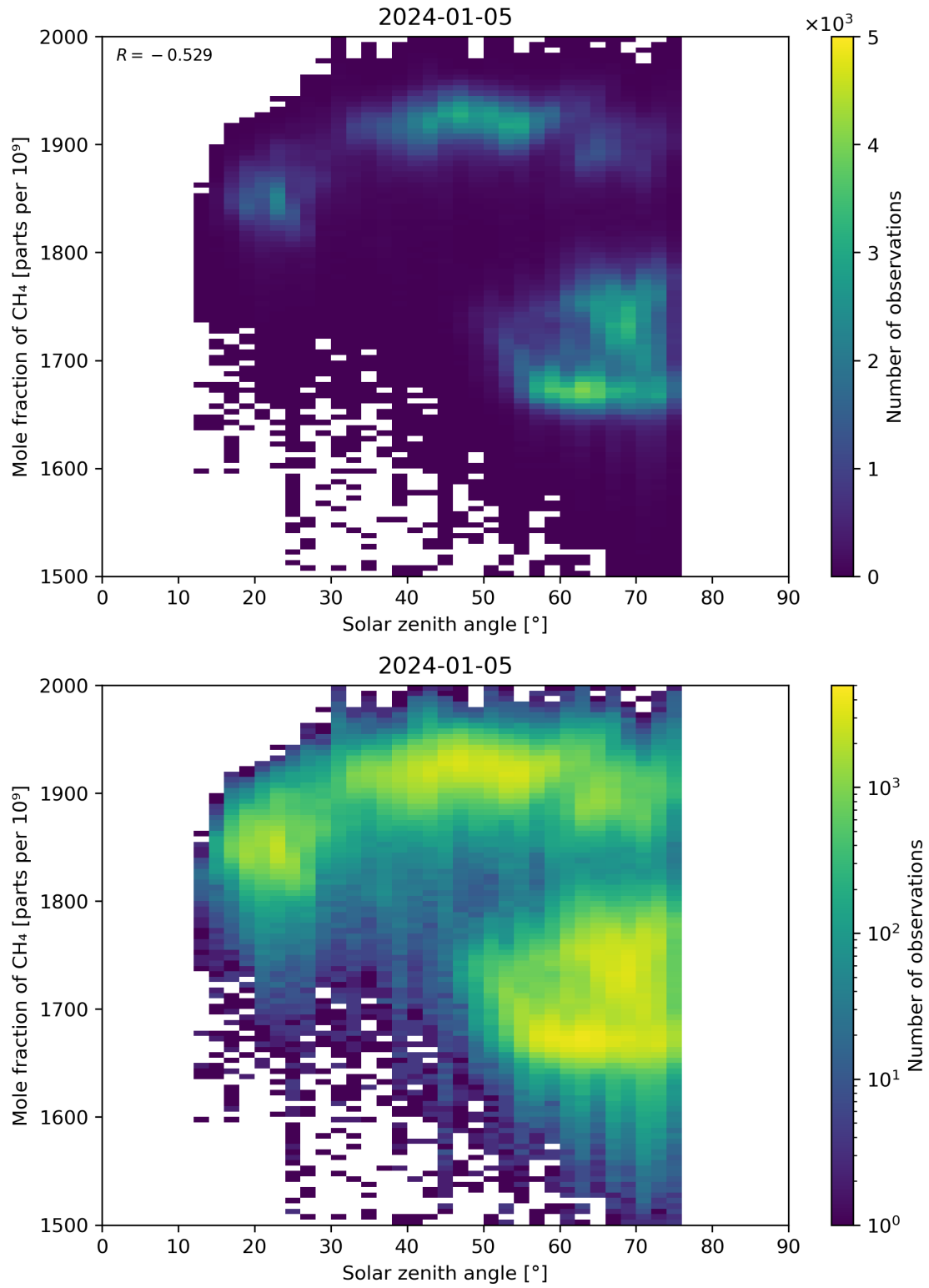
Figure 99: Scatter density plot of “Solar zenith angle” against “Mole fraction of CH 4 ” for 2024-01-05 to 2024-01-06.
