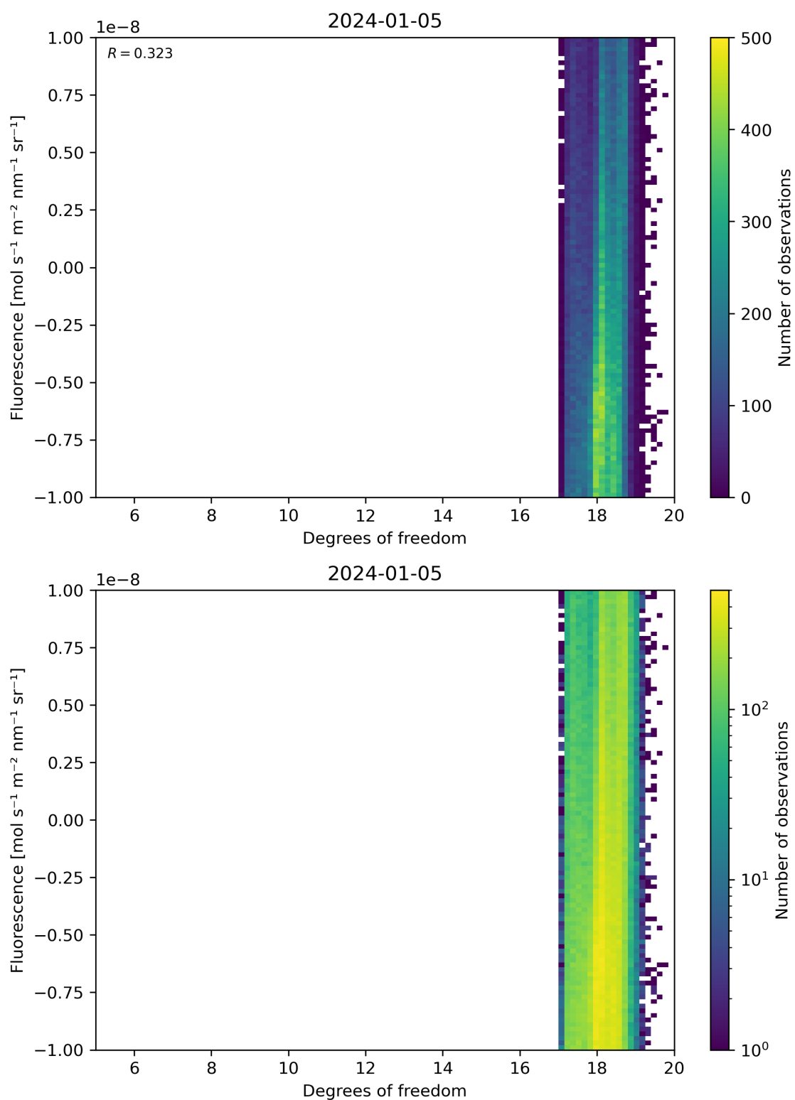
Figure 51: Scatter density plot of “Degrees of freedom” against “Fluorescence” for 2024-01-05 to 2024-01-06.
