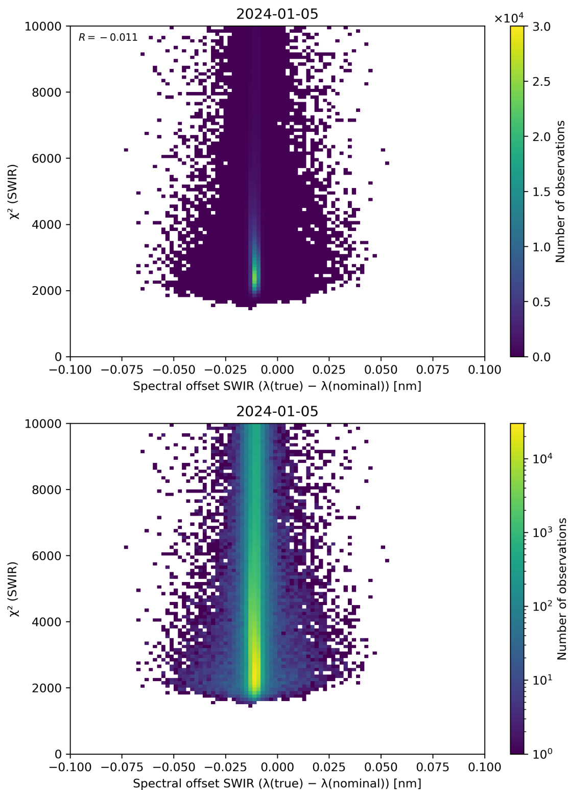
Figure 118: Scatter density plot of “Spectral offset SWIR ( \lambda(\text{true}) - \lambda(\text{nominal}) )” against “ \chi^2 (SWIR)” for 2024-01-05 to 2024-01-06.
