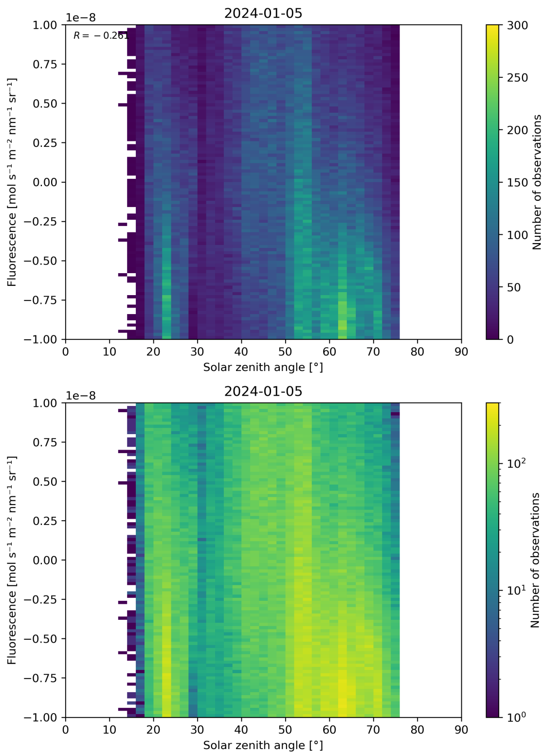
Figure 97: Scatter density plot of “Solar zenith angle” against “Fluorescence” for 2024-01-05 to 2024-01-06.
