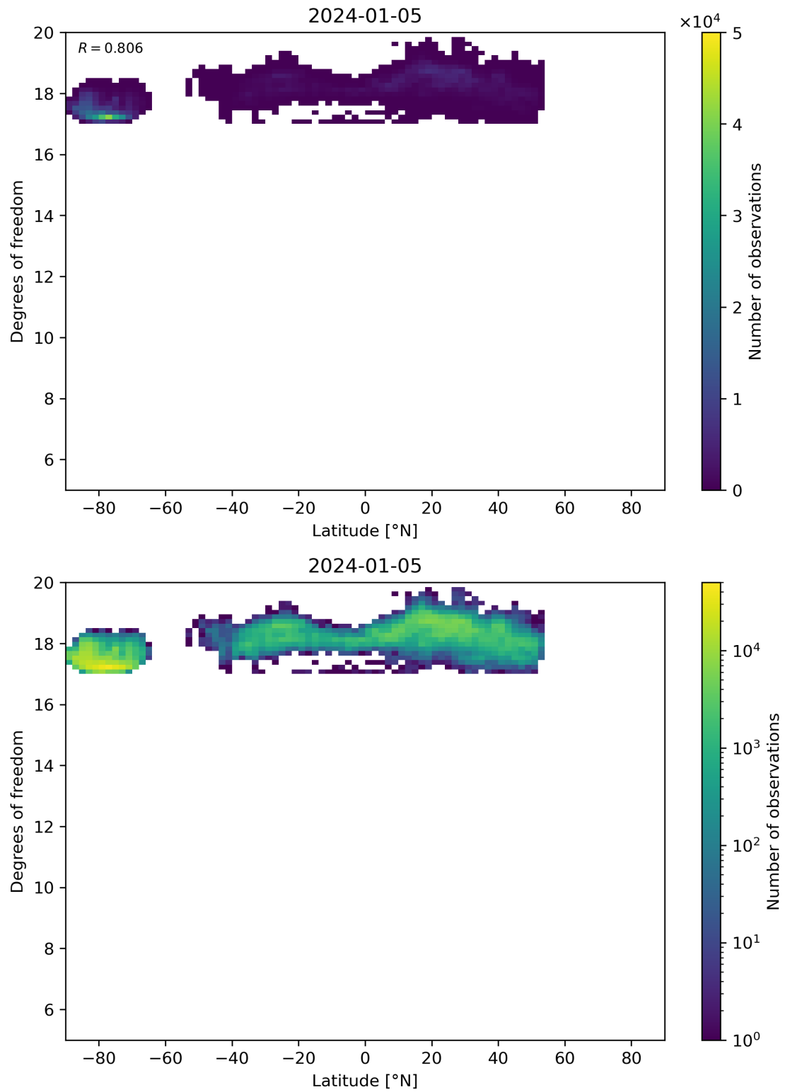
Figure 55: Scatter density plot of “Latitude” against “Degrees of freedom” for 2024-01-05 to 2024-01-06.
