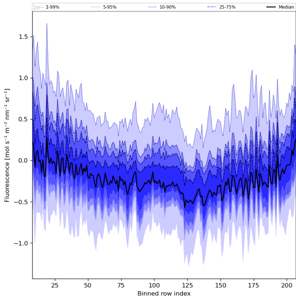
Figure 43: Along track statistics of “Fluorescence” for 2024-01-05 to 2024-01-06
