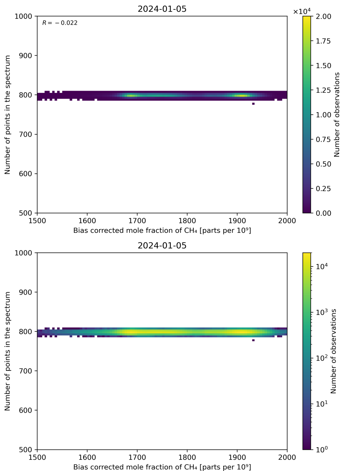
Figure 68: Scatter density plot of “Bias corrected mole fraction of CH 4 ” against “Number of points in the spectrum” for 2024-01-05 to 2024-01-06.
