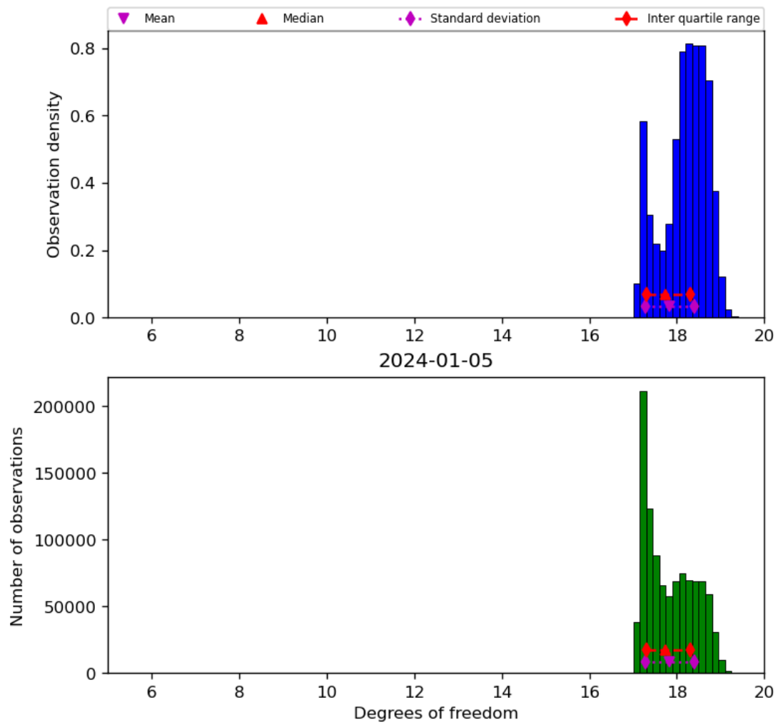
Figure 30: Histogram of “Degrees of freedom” for 2024-01-05 to 2024-01-06
