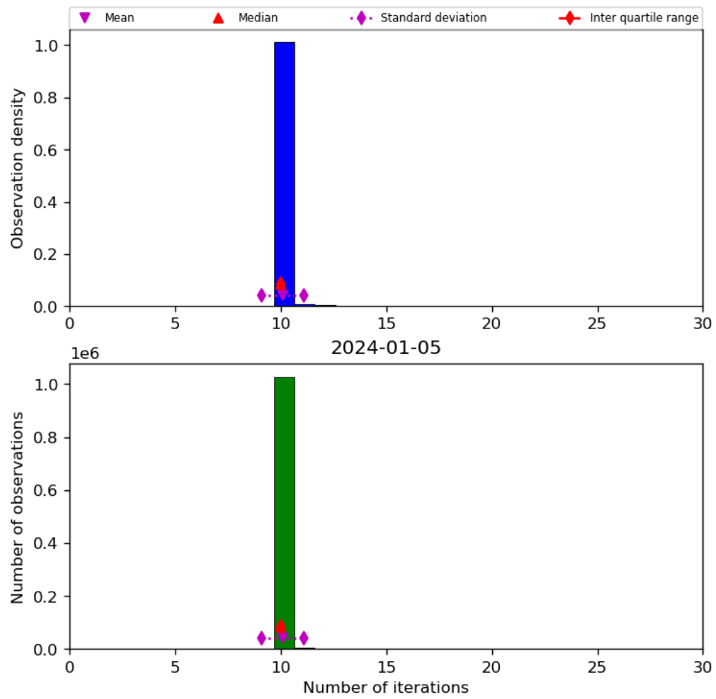
Figure 31: Histogram of “Number of iterations” for 2024-01-05 to 2024-01-06
