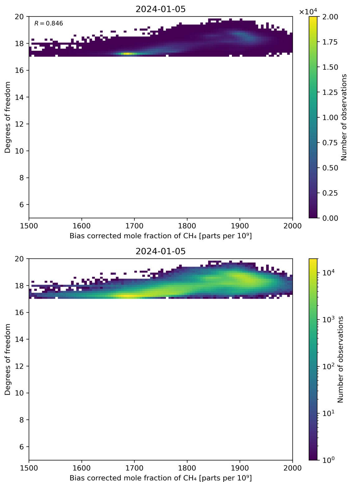
Figure 65: Scatter density plot of “Bias corrected mole fraction of CH 4 ” against “Degrees of freedom” for 2024-01-05 to 2024-01-06.
