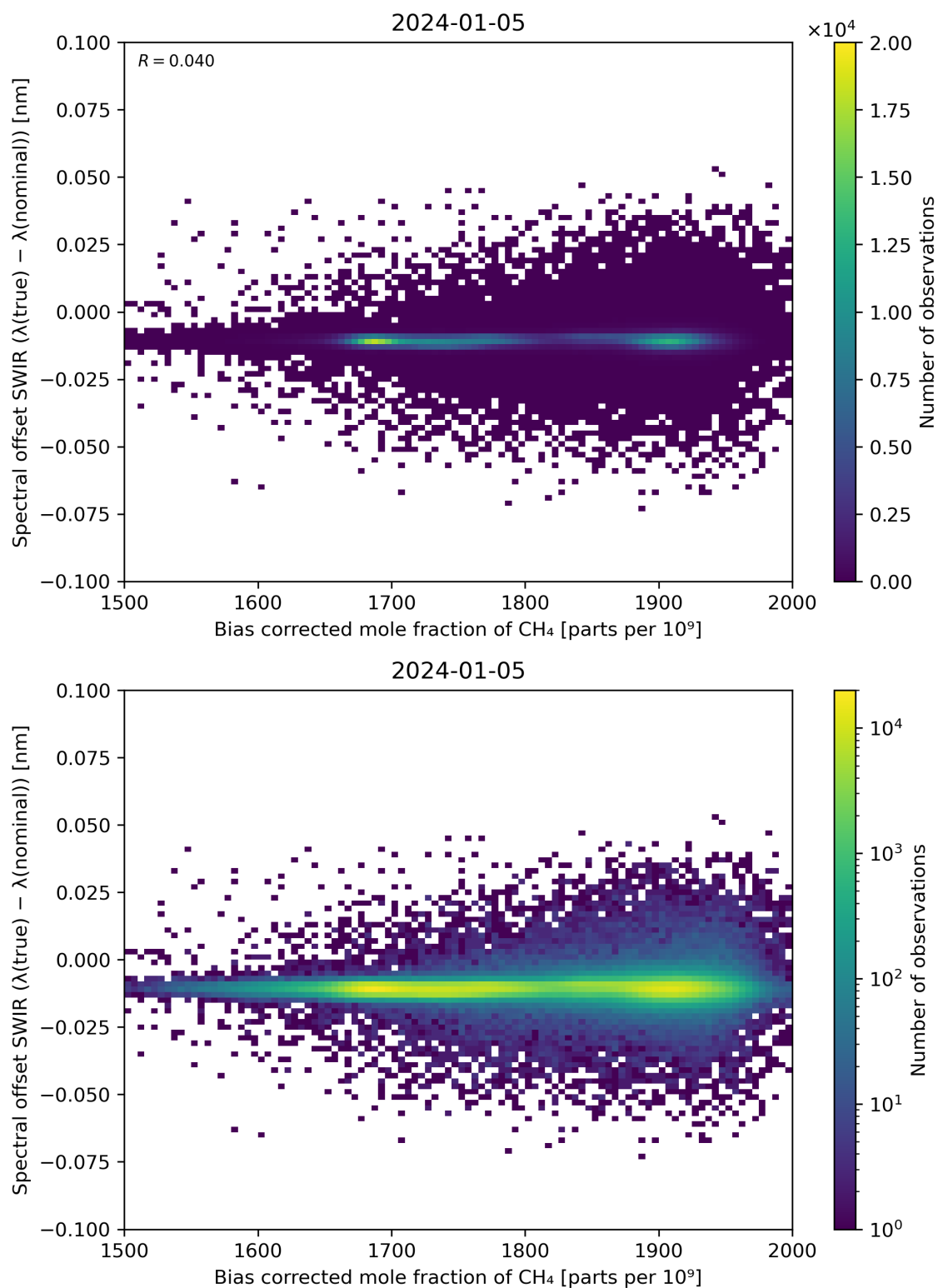
Figure 69: Scatter density plot of “Bias corrected mole fraction of \text{CH}_4 ” against “Spectral offset SWIR ( \lambda(\text{true}) - \lambda(\text{nominal}) )” for 2024-01-05 to 2024-01-06.
