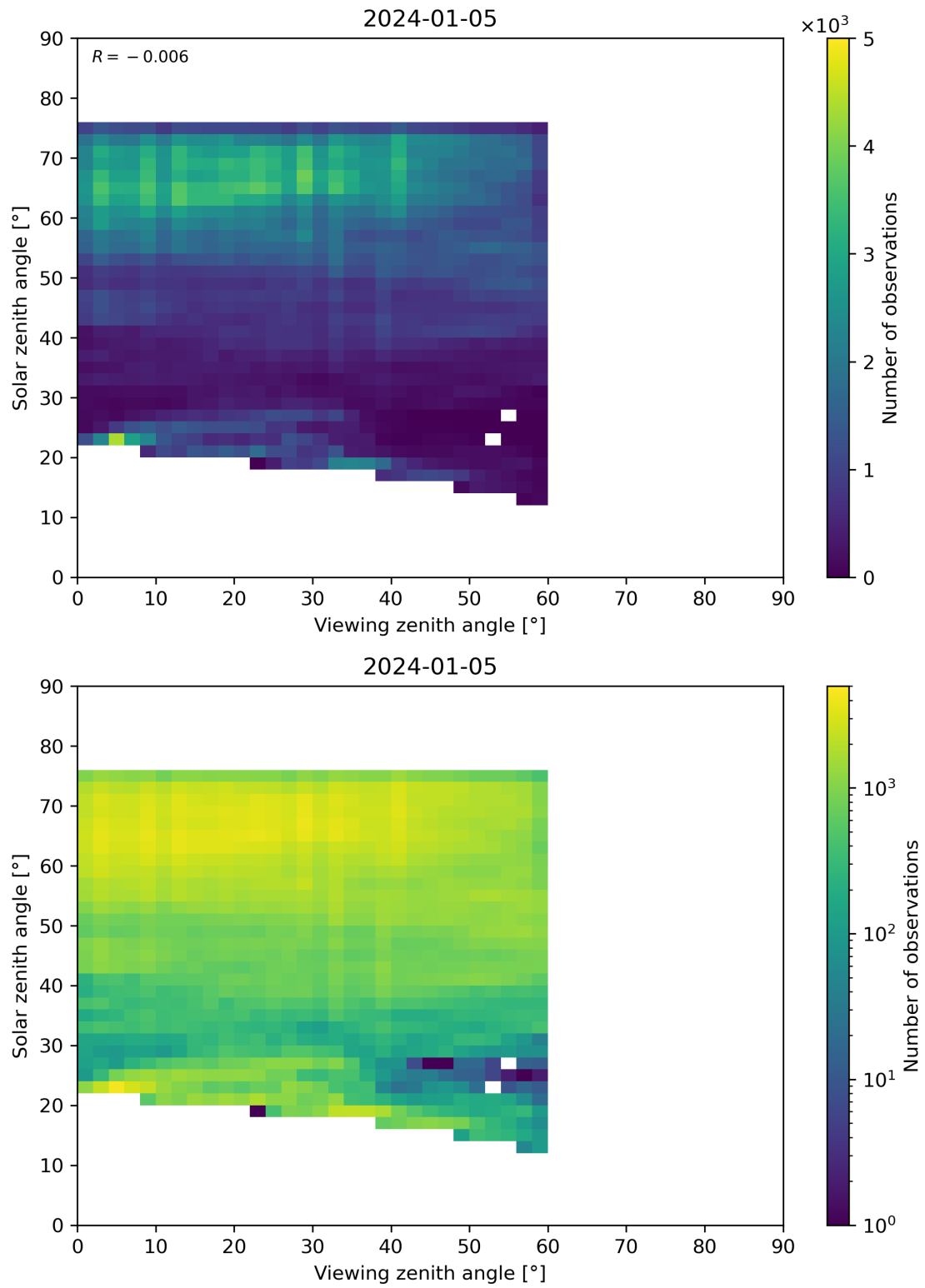
Figure 115: Scatter density plot of “Viewing zenith angle” against “Solar zenith angle” for 2024-01-05 to 2024-01-06.
