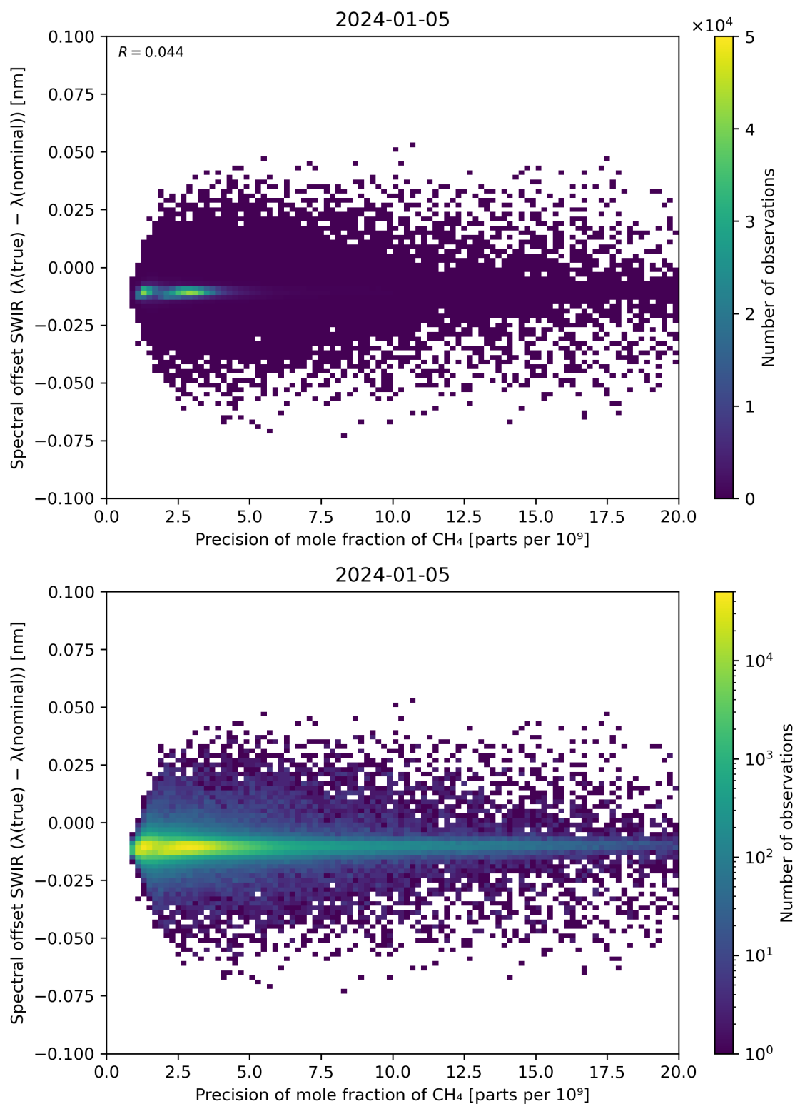
Figure 85: Scatter density plot of “Precision of mole fraction of \text{CH}_4 ” against “Spectral offset SWIR ( \lambda(\text{true}) - \lambda(\text{nominal}) )” for 2024-01-05 to 2024-01-06.
