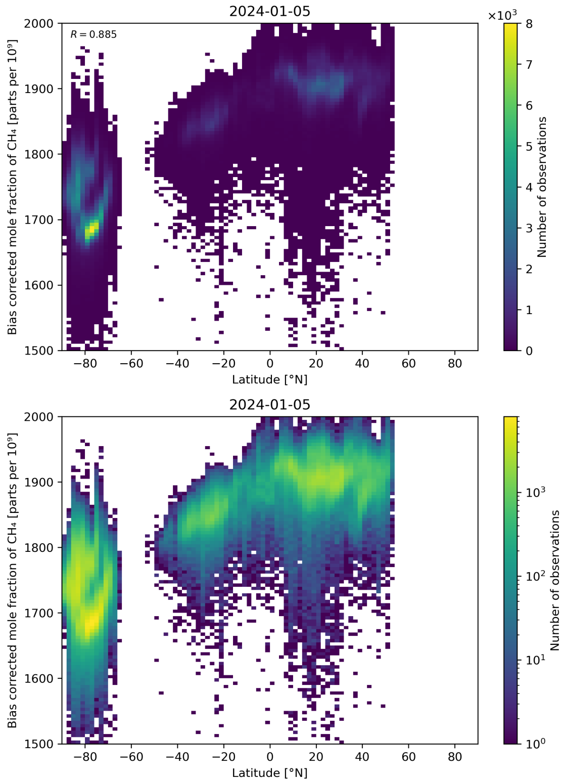
Figure 58: Scatter density plot of “Latitude” against “Bias corrected mole fraction of CH 4 ” for 2024-01-05 to 2024-01-06.
