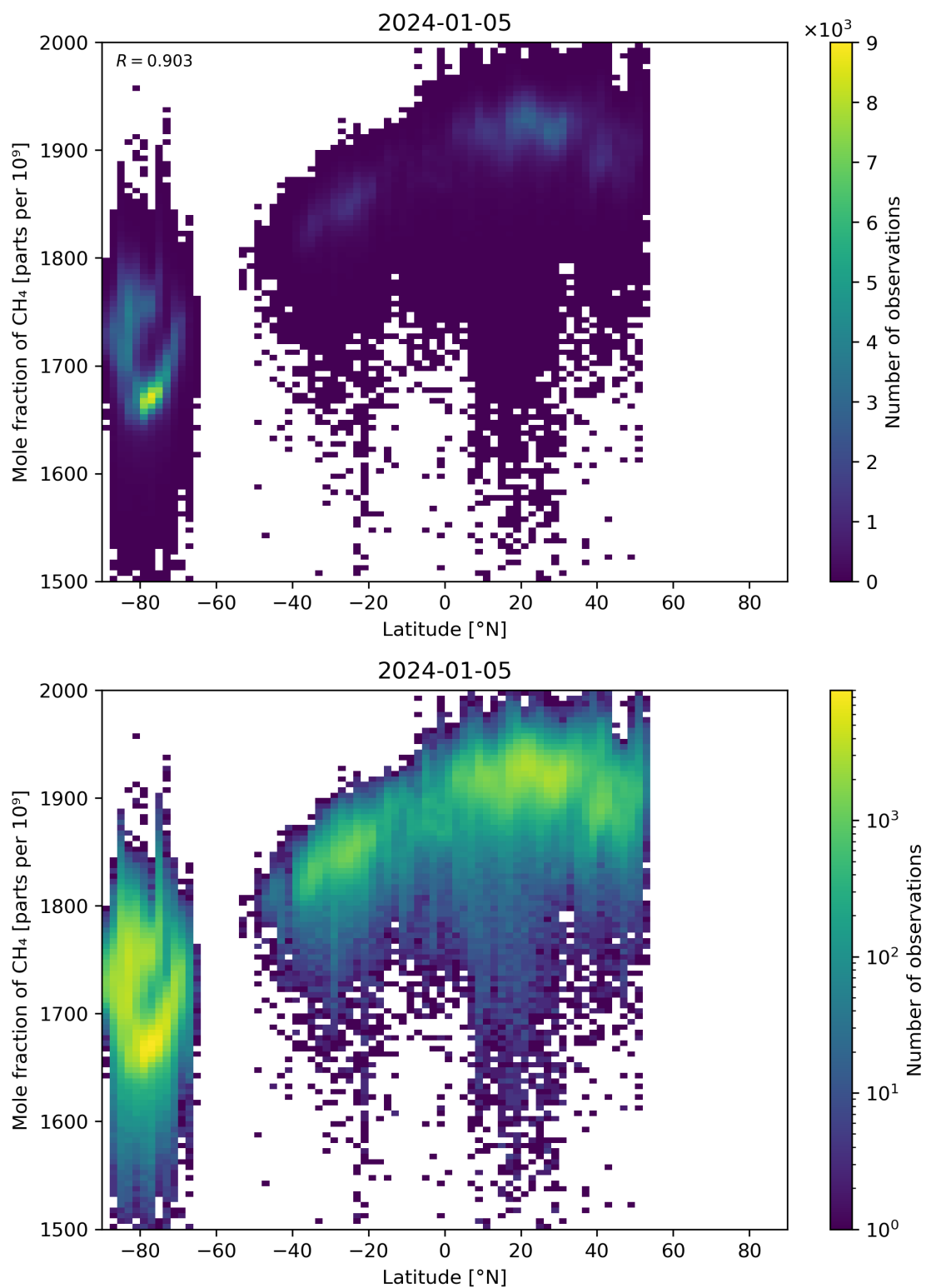
Figure 57: Scatter density plot of “Latitude” against “Mole fraction of CH 4 ” for 2024-01-05 to 2024-01-06.
