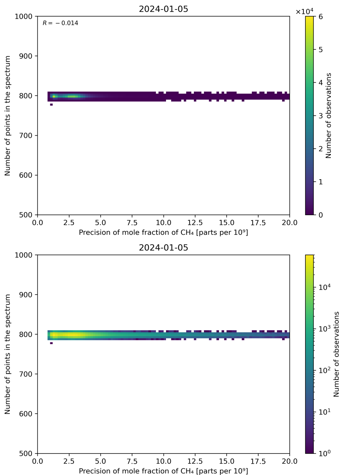
Figure 84: Scatter density plot of “Precision of mole fraction of CH 4 ” against “Number of points in the spectrum” for 2024-01-05 to 2024-01-06.
