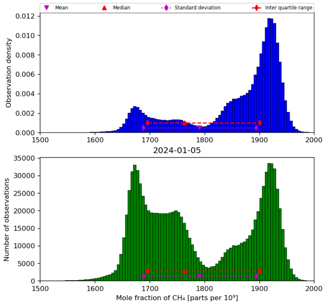
Figure 23: Histogram of “Mole fraction of CH 4 ” for 2024-01-05 to 2024-01-06
