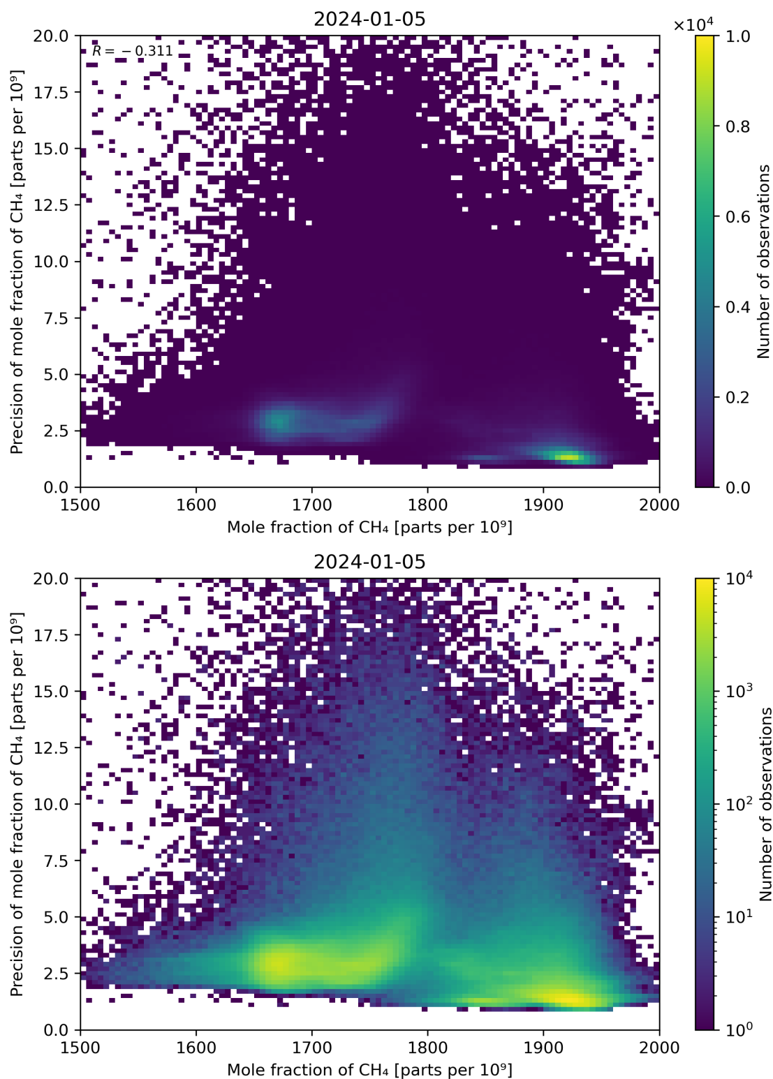
Figure 75: Scatter density plot of “Mole fraction of CH 4 ” against “Precision of mole fraction of CH 4 ” for 2024-01-05 to 2024-01-06.
