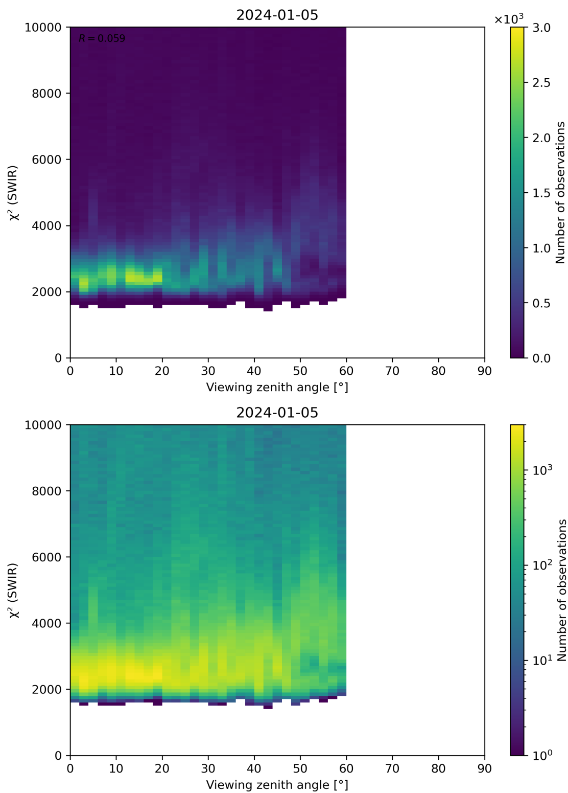
Figure 106: Scatter density plot of “Viewing zenith angle” against “ \chi^2 (SWIR)” for 2024-01-05 to 2024-01-06.
