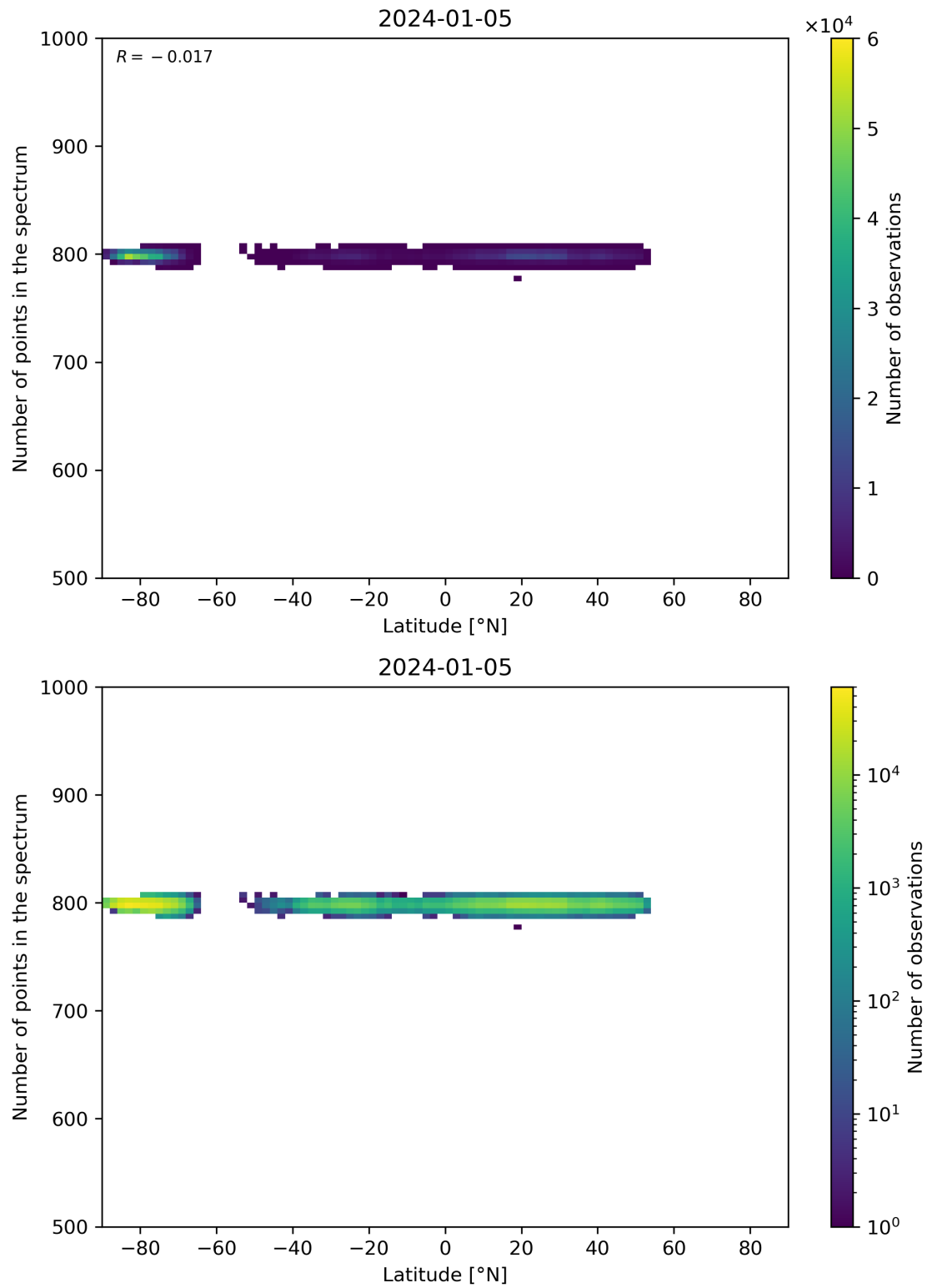
Figure 61: Scatter density plot of “Latitude” against “Number of points in the spectrum” for 2024-01-05 to 2024-01-06.
