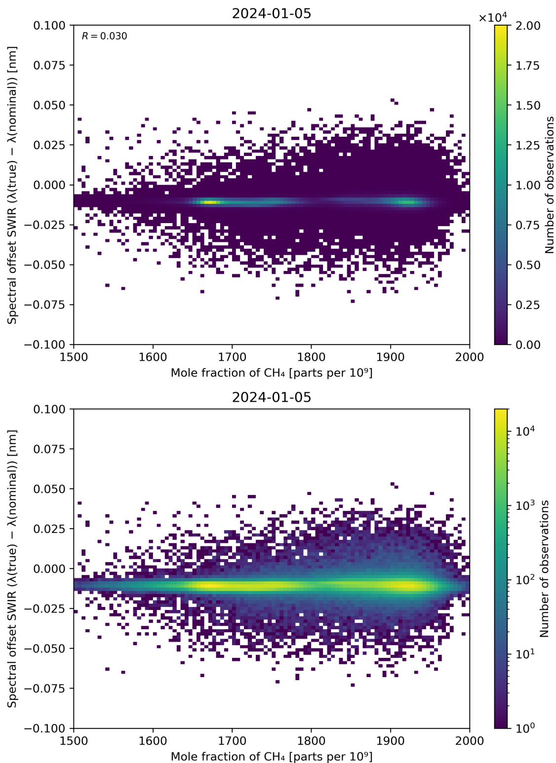
Figure 86: Scatter density plot of “Mole fraction of \text{CH}_4 ” against “Spectral offset SWIR ( \lambda(\text{true}) - \lambda(\text{nominal}) )” for 2024-01-05 to 2024-01-06.
