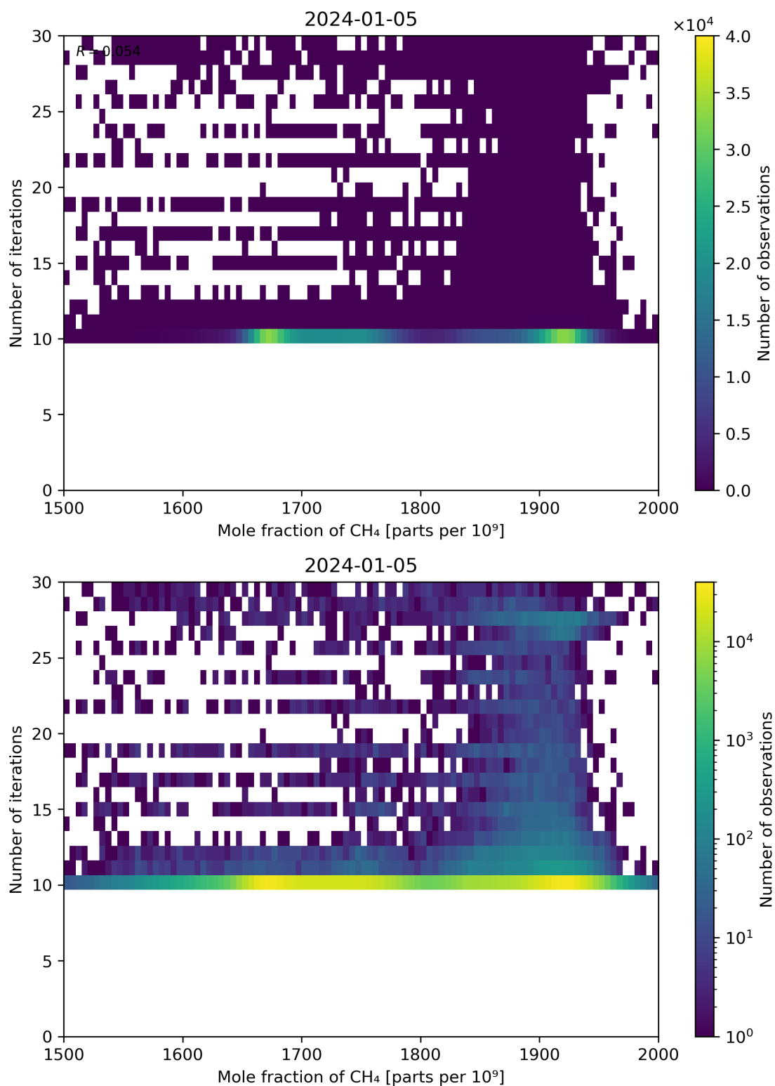
Figure 76: Scatter density plot of “Mole fraction of CH 4 ” against “Number of iterations” for 2024-01-05 to 2024-01-06.
