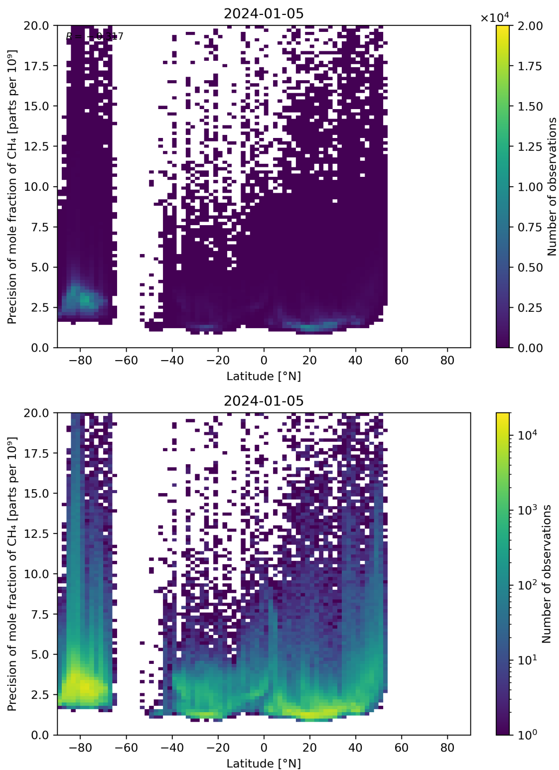
Figure 59: Scatter density plot of “Latitude” against “Precision of mole fraction of CH 4 ” for 2024-01-05 to 2024-01-06.
