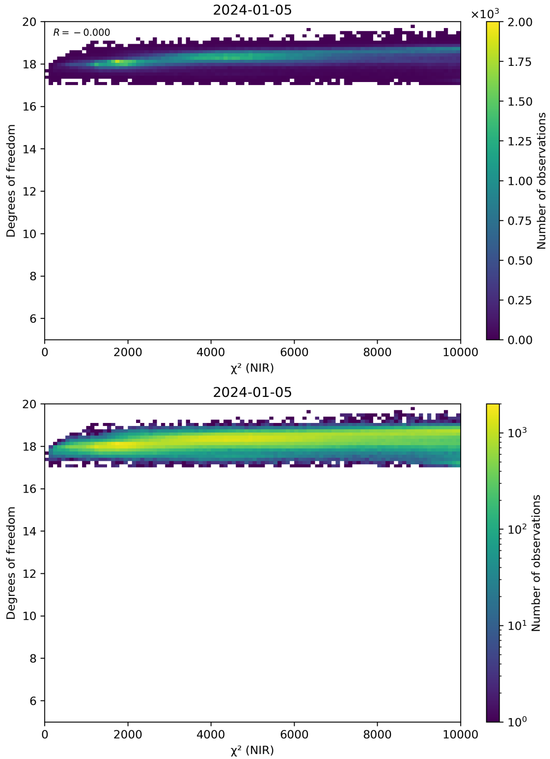
Figure 44: Scatter density plot of “ \chi^2 (NIR)” against “Degrees of freedom” for 2024-01-05 to 2024-01-06.
