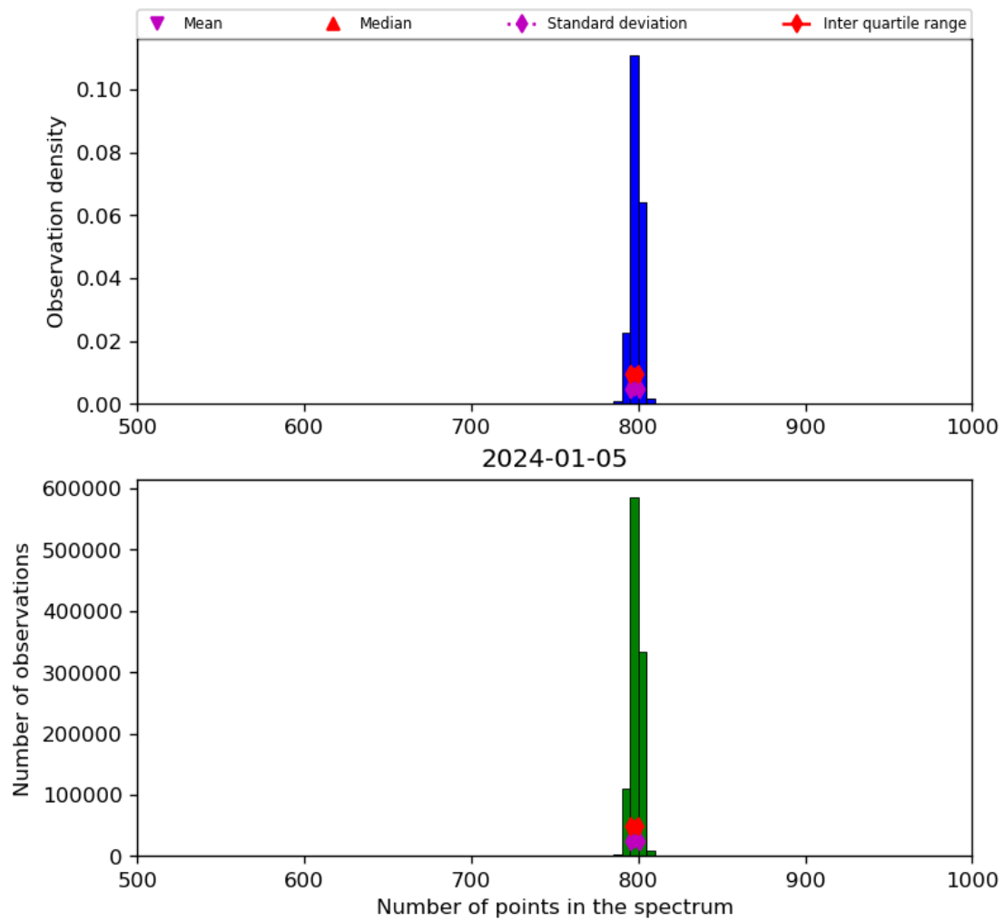
Figure 26: Histogram of “Number of points in the spectrum” for 2024-01-05 to 2024-01-06
