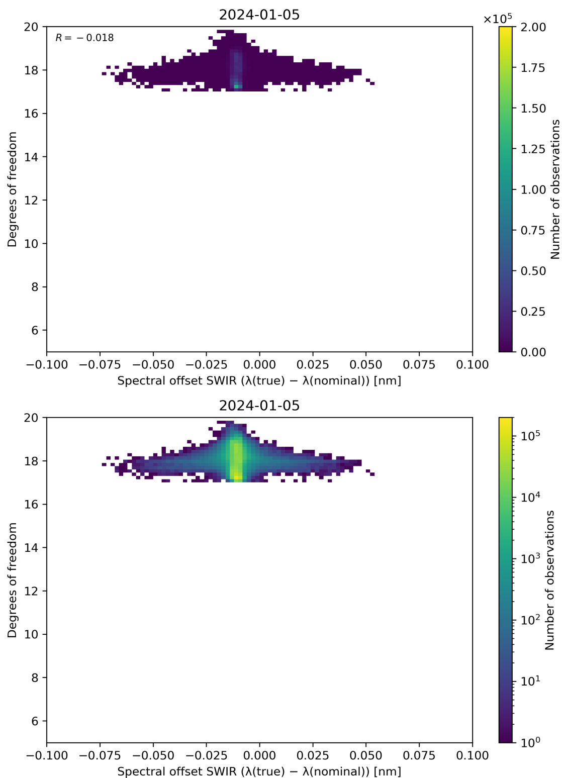
Figure 119: Scatter density plot of “Spectral offset SWIR ( \lambda(\text{true}) - \lambda(\text{nominal}) )” against “Degrees of freedom” for 2024-01-05 to 2024-01-06.
