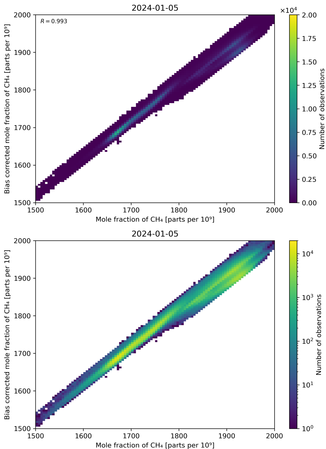
Figure 74: Scatter density plot of “Mole fraction of CH 4 ” against “Bias corrected mole fraction of CH 4 ” for 2024-01-05 to 2024-01-06.
