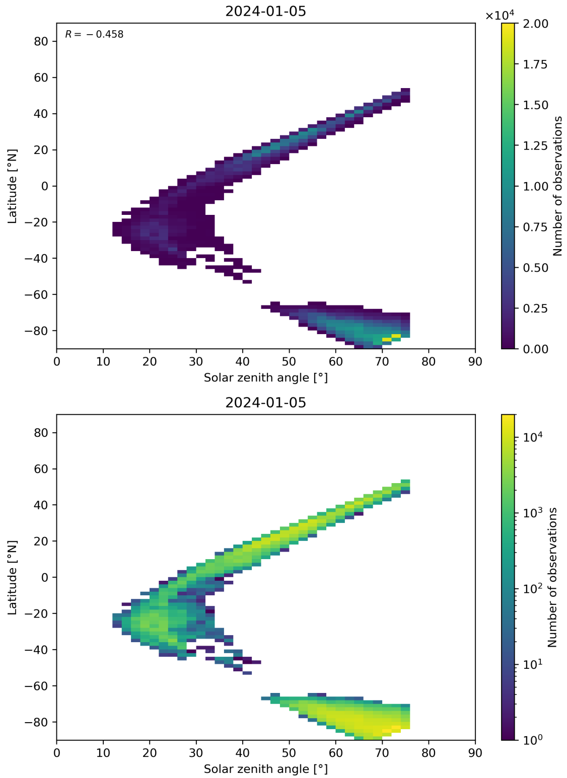
Figure 98: Scatter density plot of “Solar zenith angle” against “Latitude” for 2024-01-05 to 2024-01-06.
