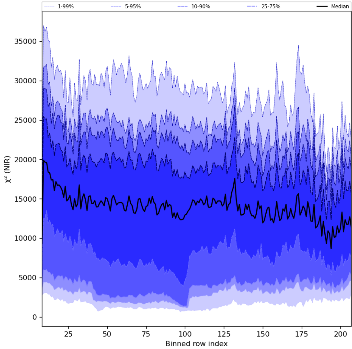
Figure 40: Along track statistics of " \chi^2 (NIR)" for 2024-01-05 to 2024-01-06
