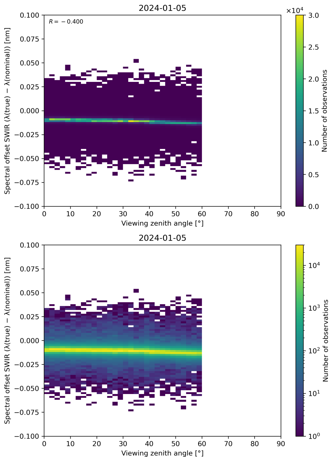
Figure 116: Scatter density plot of “Viewing zenith angle” against “Spectral offset SWIR ( \lambda(\text{true}) - \lambda(\text{nominal}) )” for 2024-01-05 to 2024-01-06.
