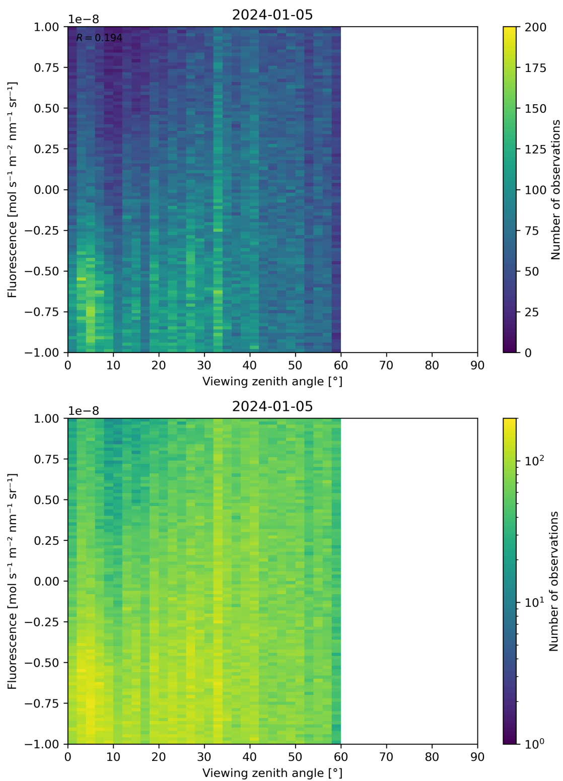
Figure 108: Scatter density plot of “Viewing zenith angle” against “Fluorescence” for 2024-01-05 to 2024-01-06.
