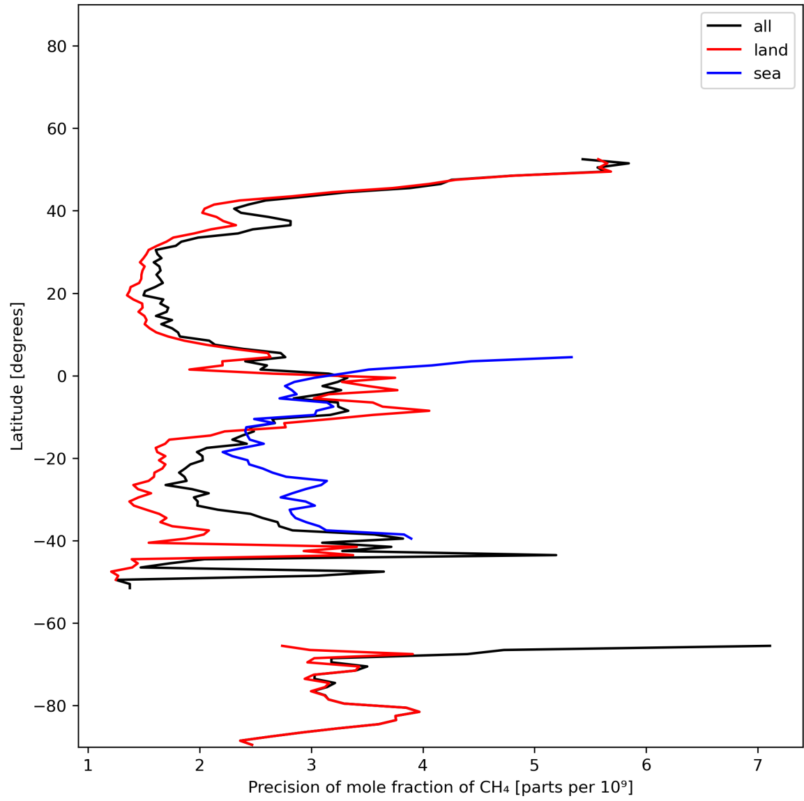
Figure 13: Zonal average of “Precision of mole fraction of CH 4 ” for 2024-01-05 to 2024-01-06.
