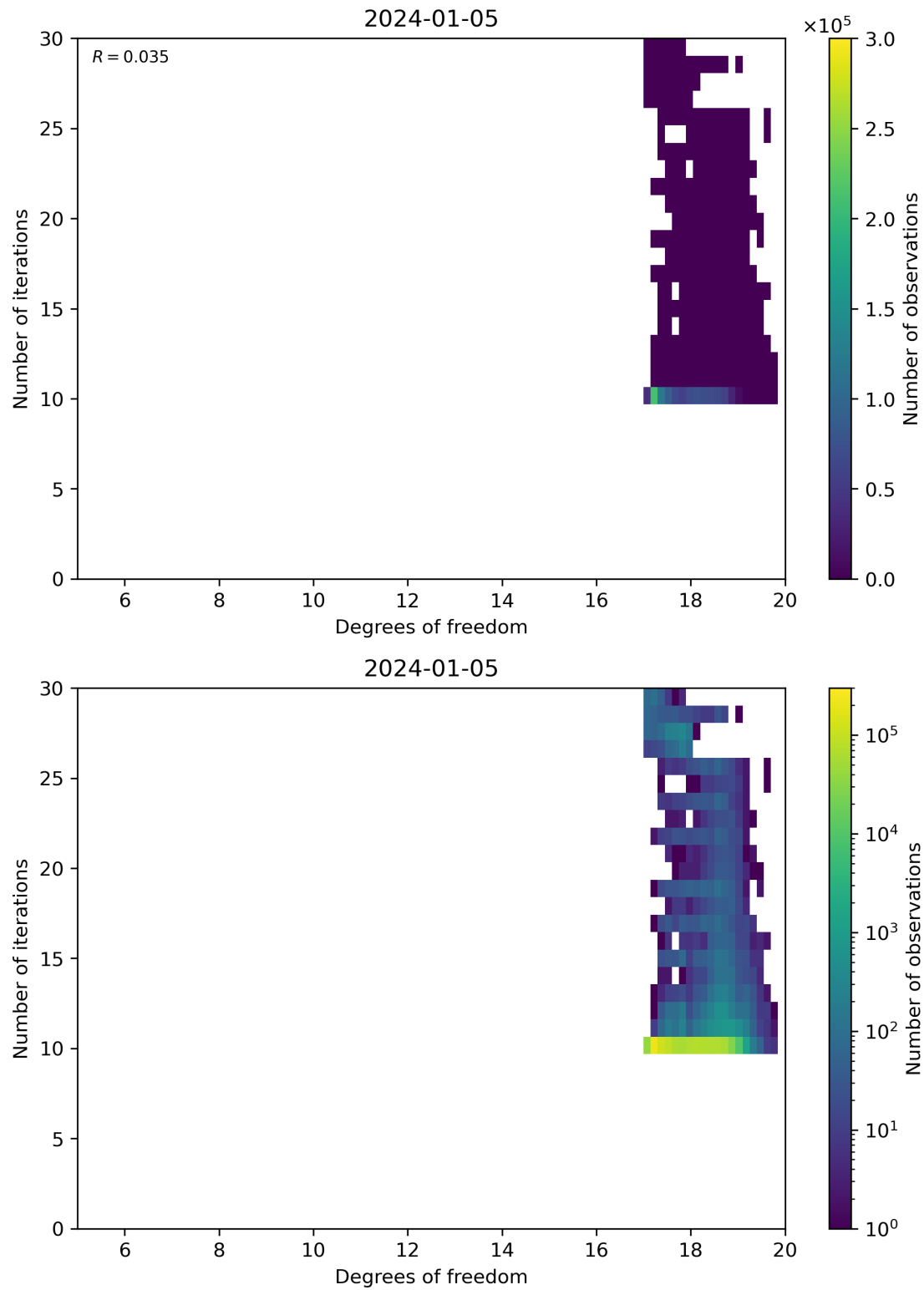
Figure 52: Scatter density plot of “Degrees of freedom” against “Number of iterations” for 2024-01-05 to 2024-01-06.
