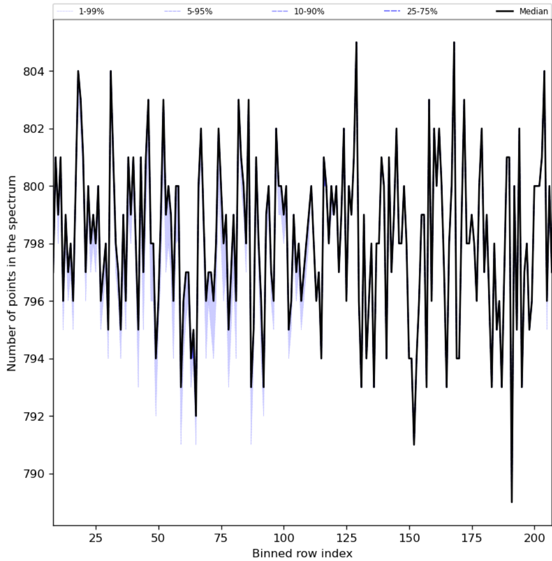
Figure 37: Along track statistics of “Number of points in the spectrum” for 2024-01-05 to 2024-01-06
