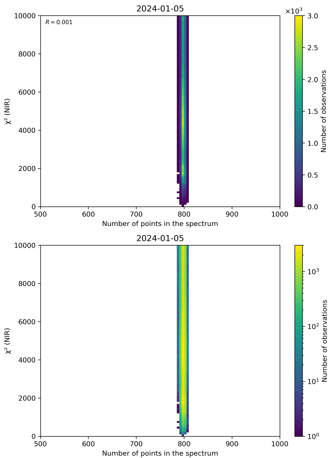
Figure 88: Scatter density plot of “Number of points in the spectrum” against “ \chi^2 (NIR)” for 2024-01-05 to 2024-01-06.
