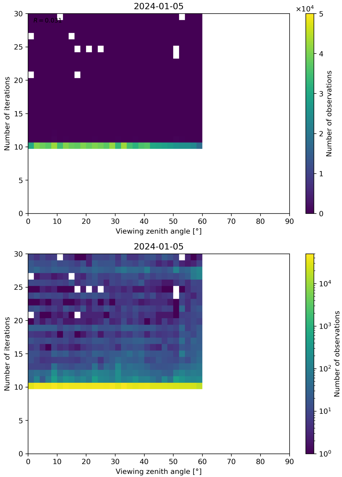
Figure 113: Scatter density plot of “Viewing zenith angle” against “Number of iterations” for 2024-01-05 to 2024-01-06.
