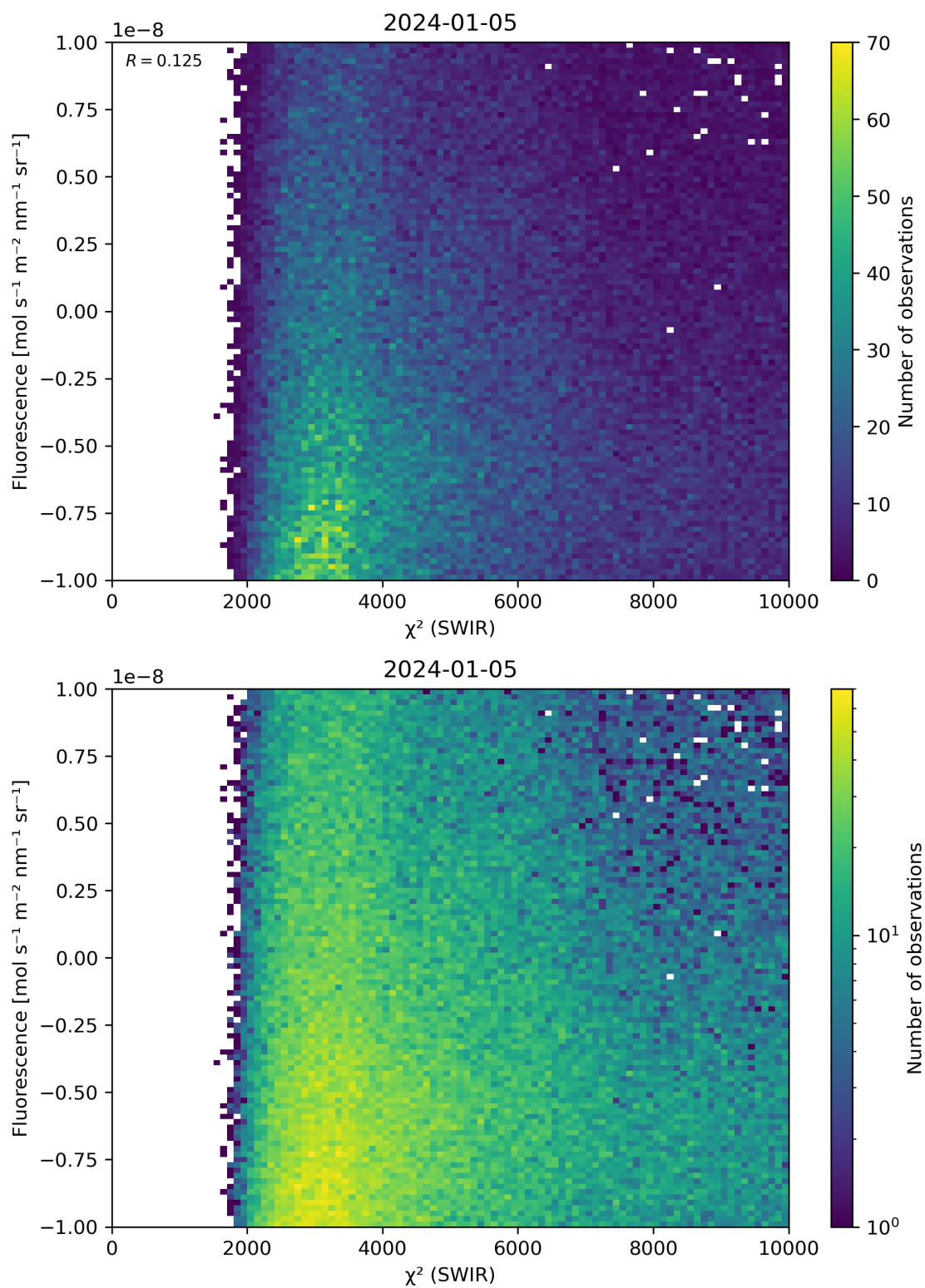
Figure 49: Scatter density plot of “ \chi^2 (SWIR)” against “Fluorescence” for 2024-01-05 to 2024-01-06.
