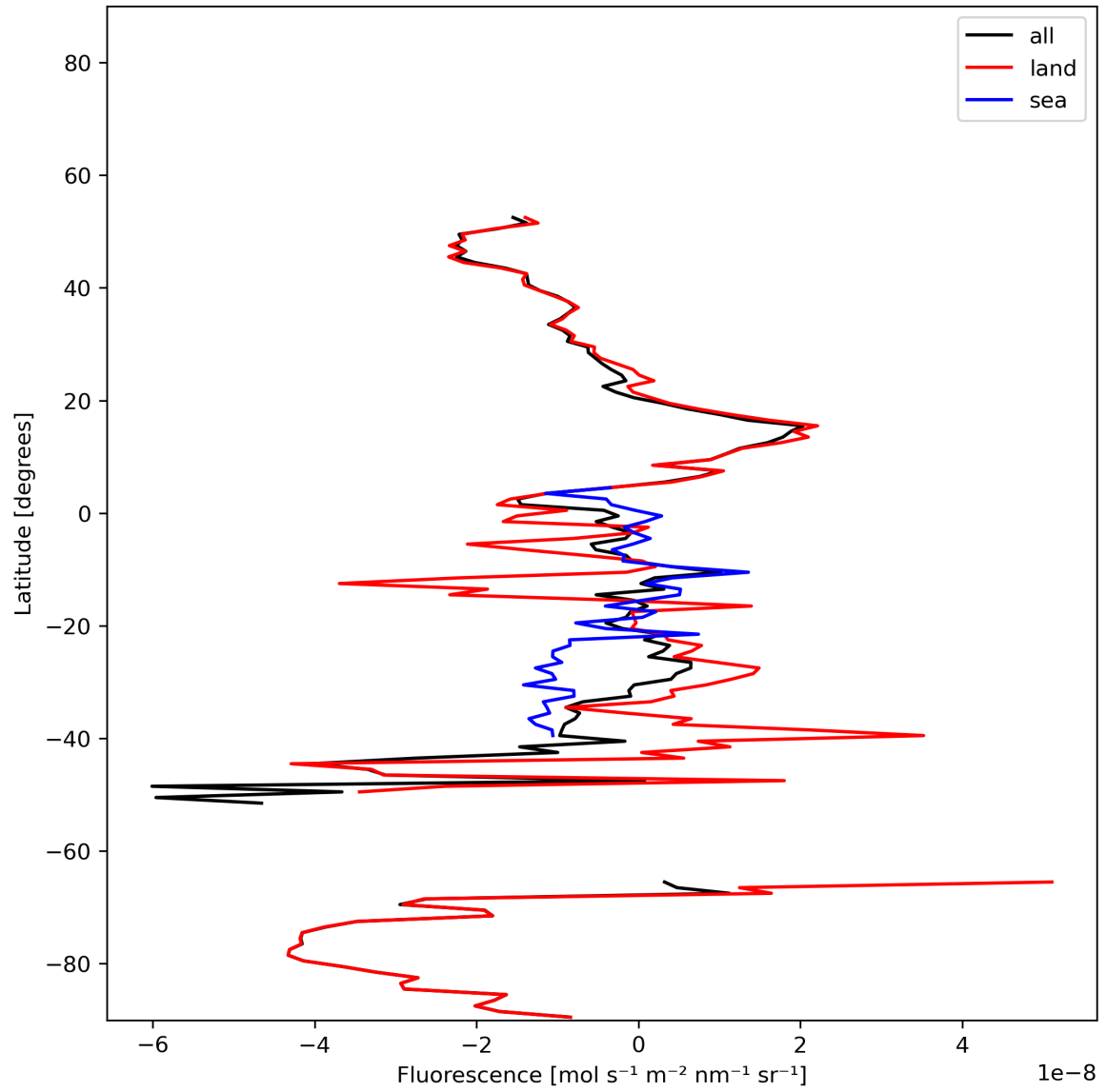
Figure 21: Zonal average of “Fluorescence” for 2024-01-05 to 2024-01-06.
