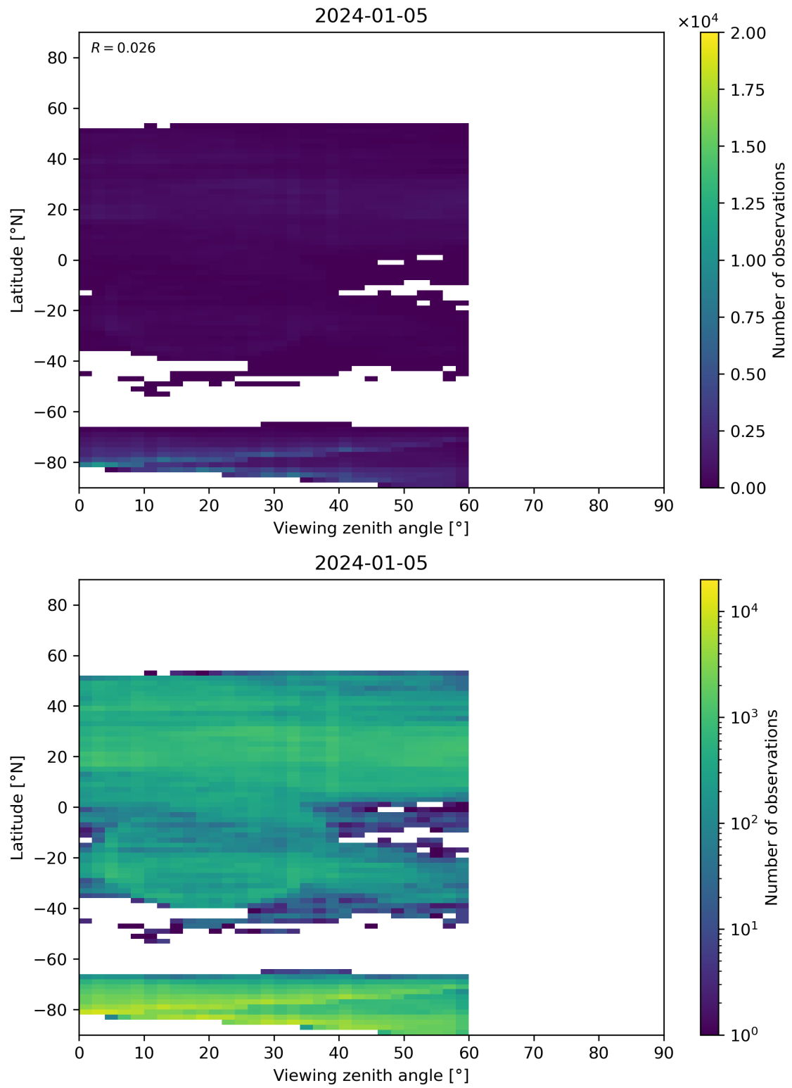
Figure 109: Scatter density plot of “Viewing zenith angle” against “Latitude” for 2024-01-05 to 2024-01-06.
