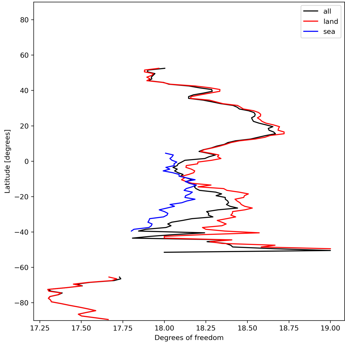
Figure 19: Zonal average of “Degrees of freedom” for 2024-01-05 to 2024-01-06.
