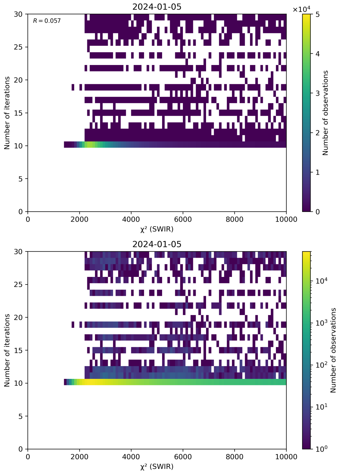
Figure 50: Scatter density plot of “ \chi^2 (SWIR)” against “Number of iterations” for 2024-01-05 to 2024-01-06.
