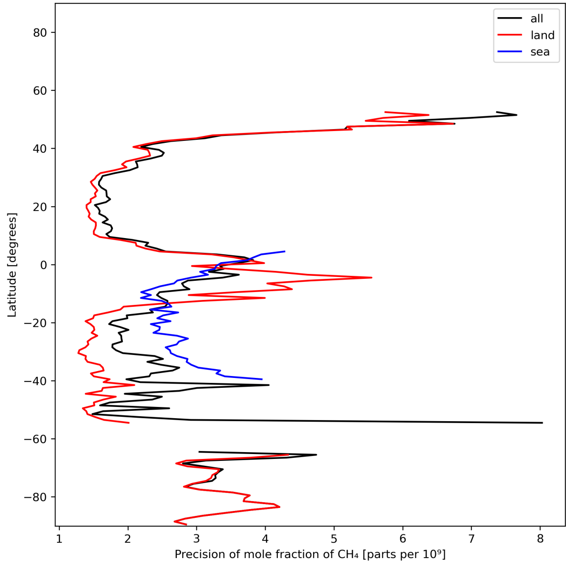
Figure 13: Zonal average of “Precision of mole fraction of CH 4 ” for 2024-01-06 to 2024-01-08.
