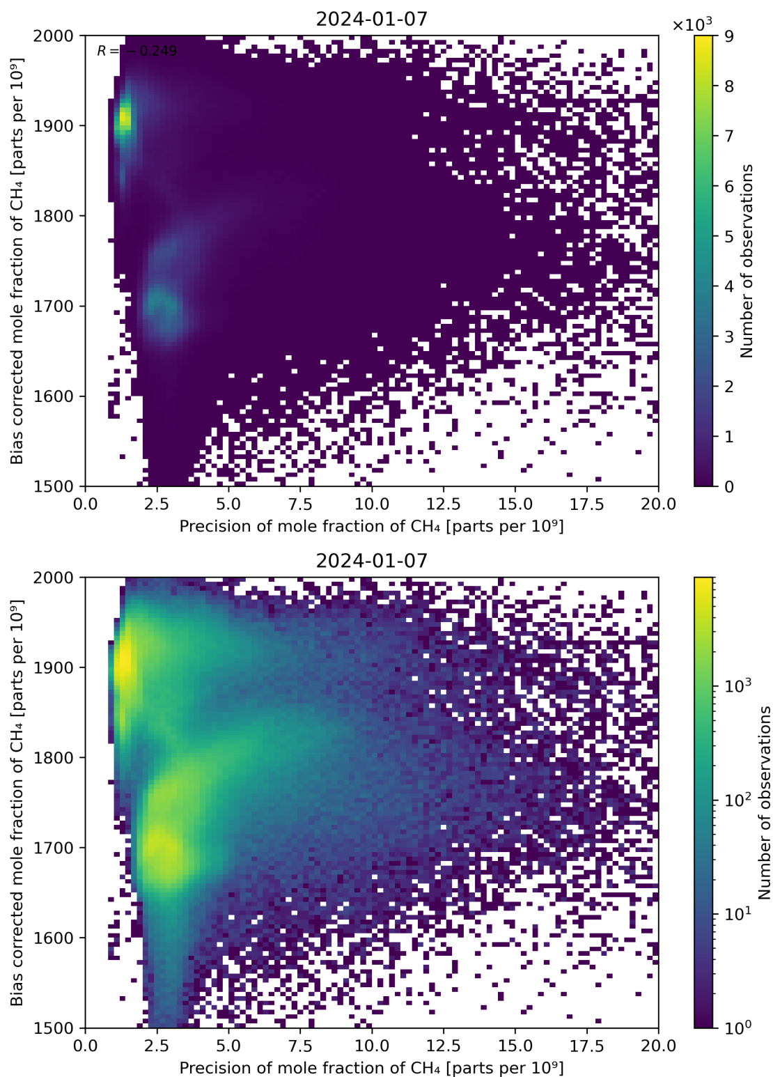
Figure 82: Scatter density plot of “Precision of mole fraction of CH 4 ” against “Bias corrected mole fraction of CH 4 ” for 2024-01-06 to 2024-01-08.
