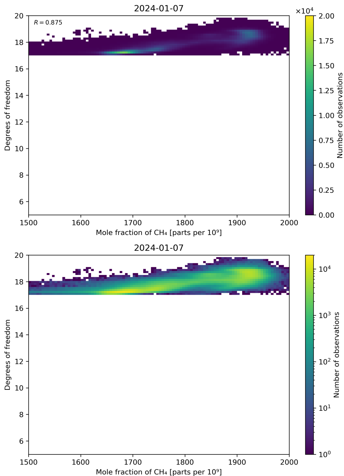
Figure 72: Scatter density plot of “Mole fraction of CH 4 ” against “Degrees of freedom” for 2024-01-06 to 2024-01-08.
