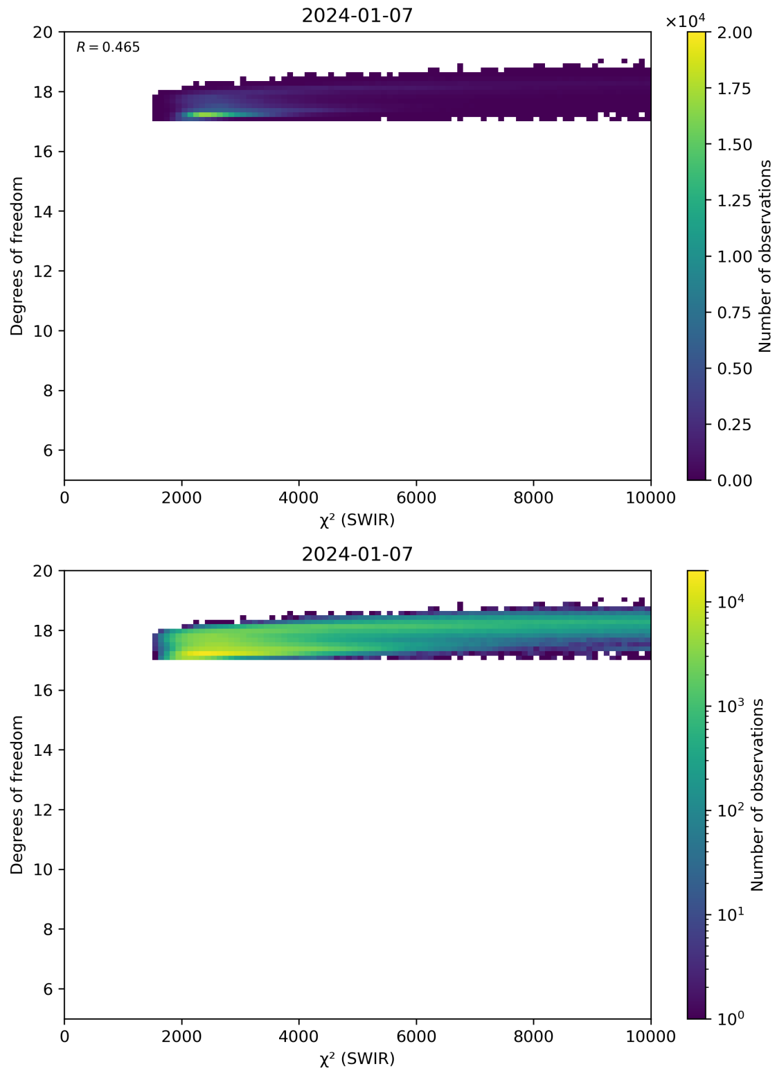
Figure 48: Scatter density plot of “ \chi^2 (SWIR)” against “Degrees of freedom” for 2024-01-06 to 2024-01-08.
