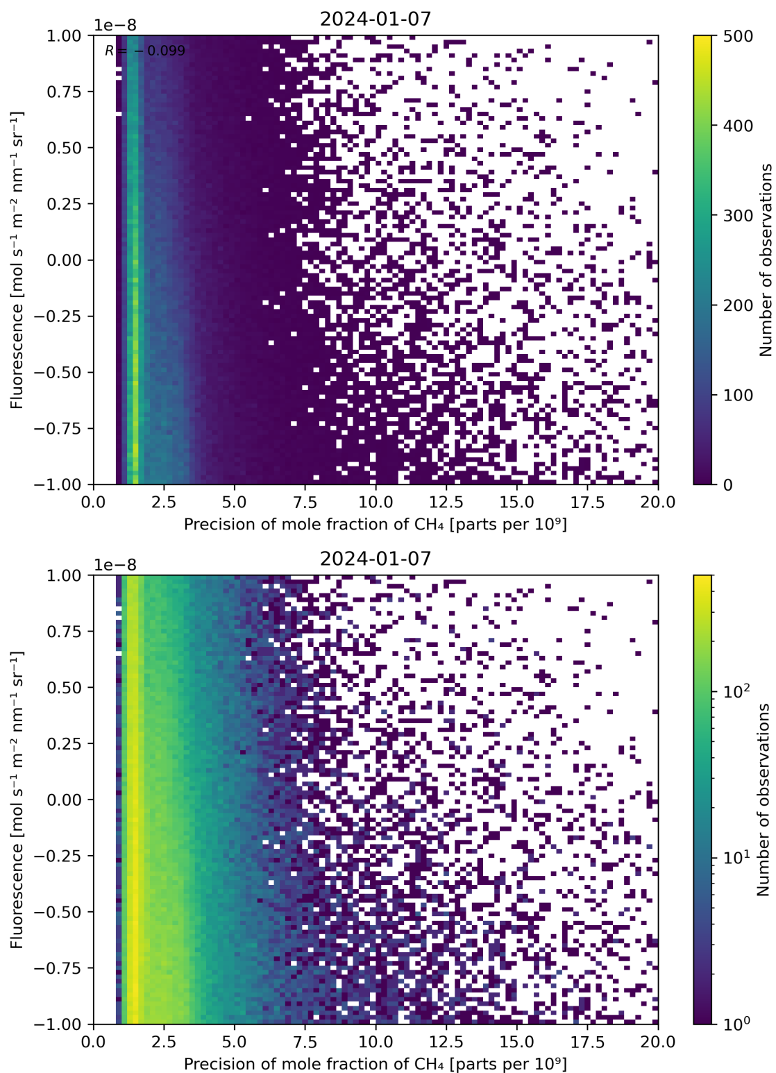
Figure 81: Scatter density plot of “Precision of mole fraction of \text{CH}_4 ” against “Fluorescence” for 2024-01-06 to 2024-01-08.
