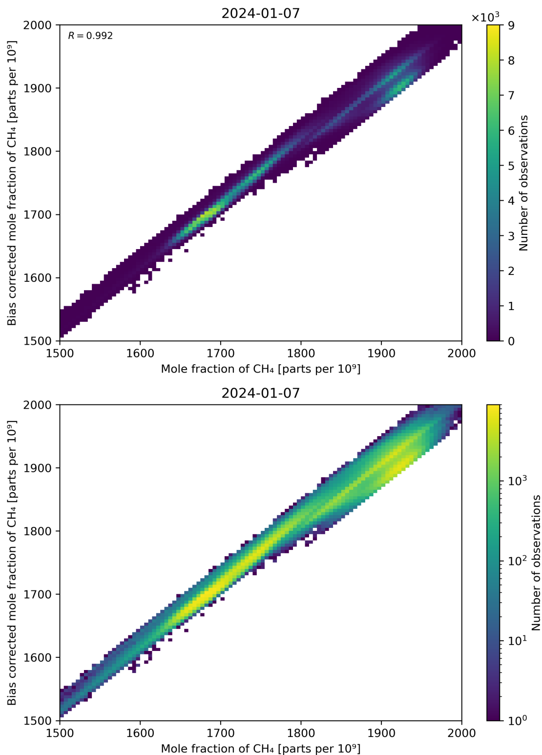
Figure 74: Scatter density plot of “Mole fraction of CH 4 ” against “Bias corrected mole fraction of CH 4 ” for 2024-01-06 to 2024-01-08.
