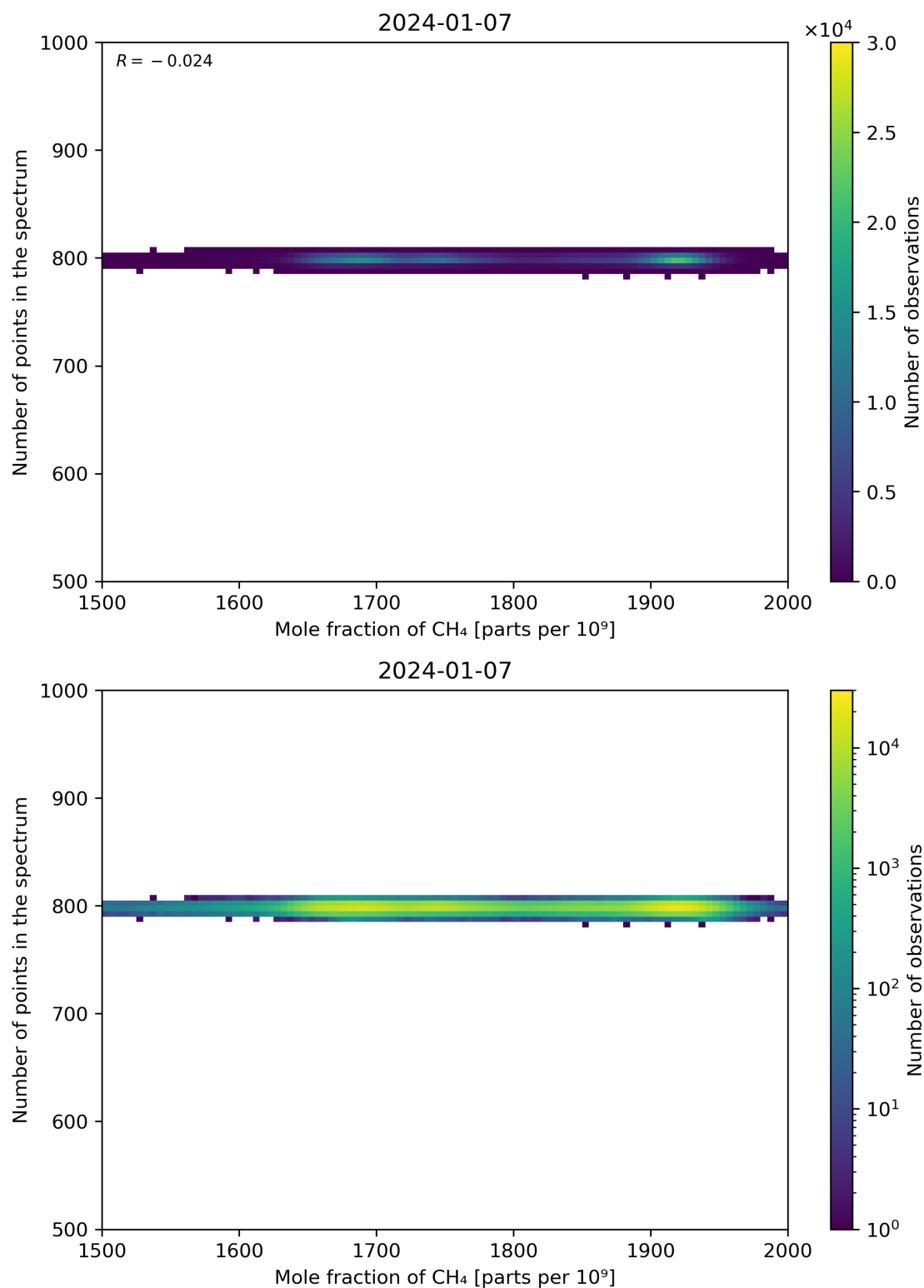
Figure 77: Scatter density plot of “Mole fraction of CH 4 ” against “Number of points in the spectrum” for 2024-01-06 to 2024-01-08.
