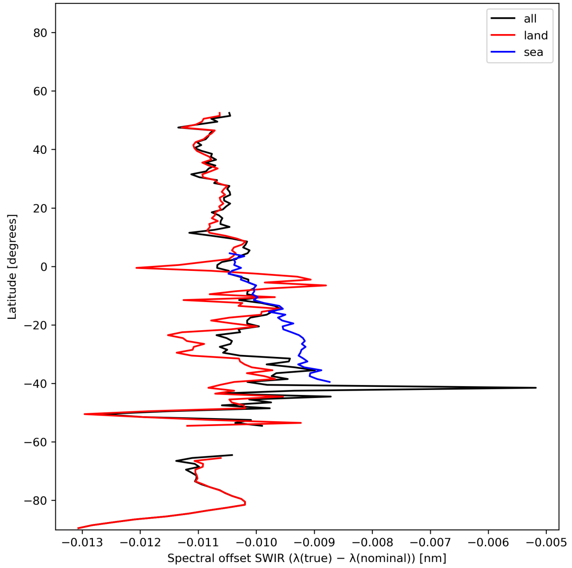
Figure 16: Zonal average of “Spectral offset SWIR ( \lambda(\text{true}) - \lambda(\text{nominal}) )” for 2024-01-06 to 2024-01-08.
