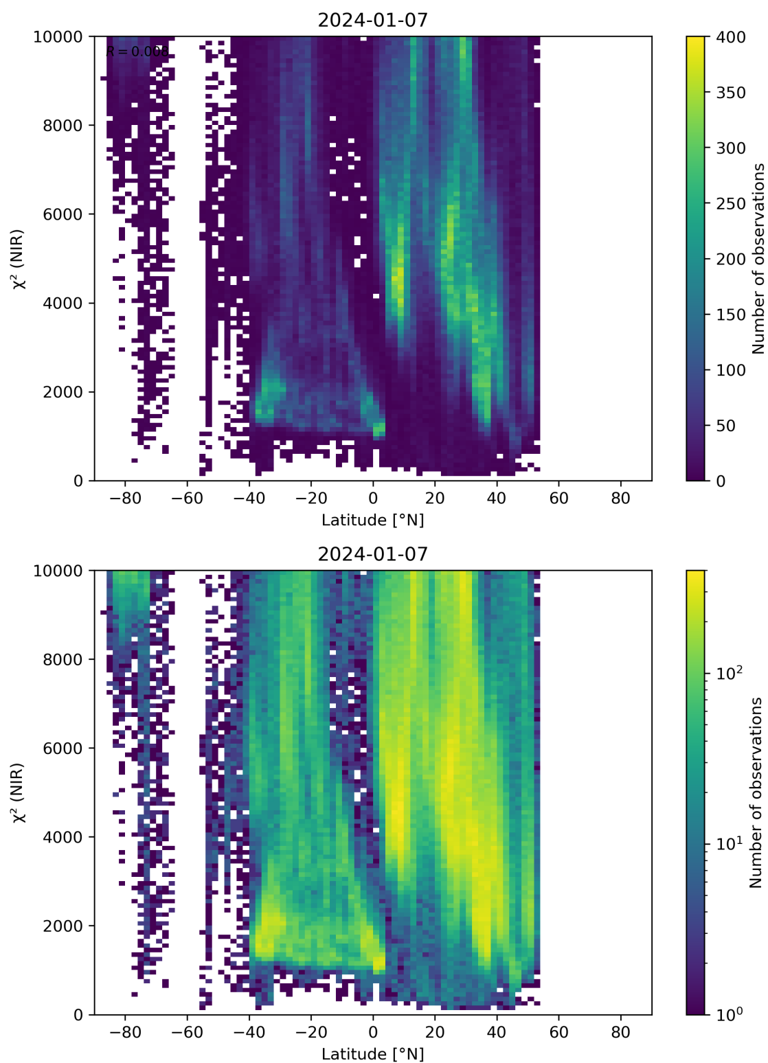
Figure 53: Scatter density plot of “Latitude” against “ \chi^2 (NIR)” for 2024-01-06 to 2024-01-08.
