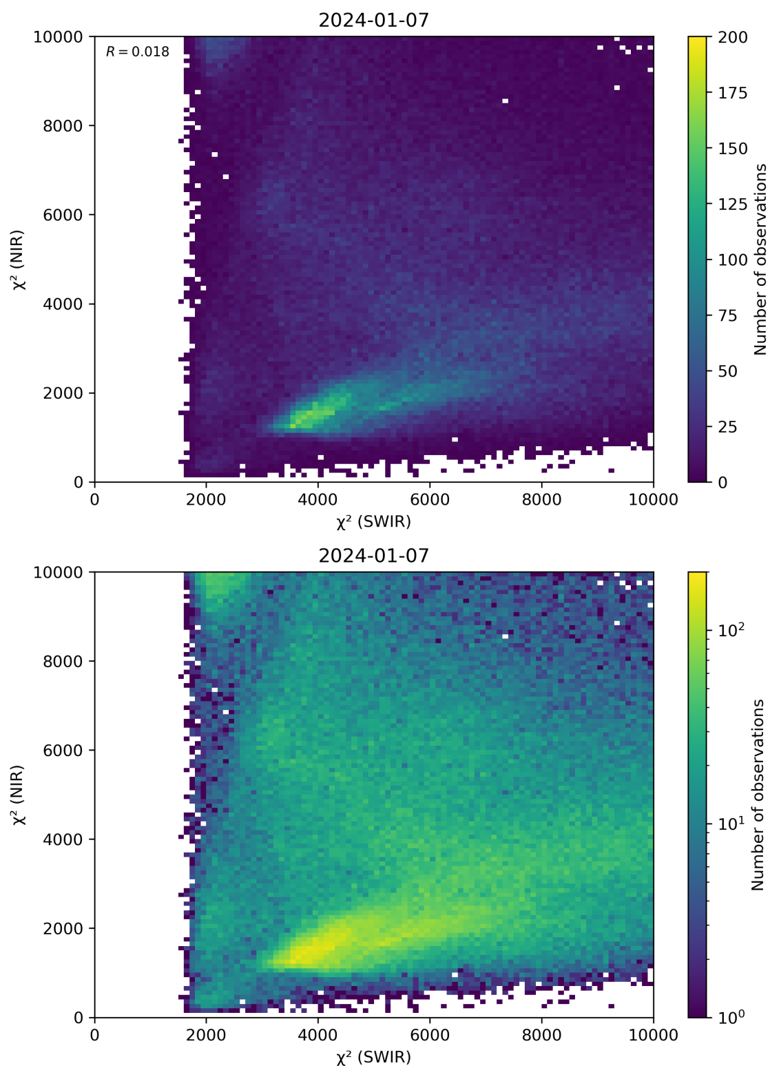
Figure 47: Scatter density plot of “ \chi^2 (SWIR)” against “ \chi^2 (NIR)” for 2024-01-06 to 2024-01-08.
