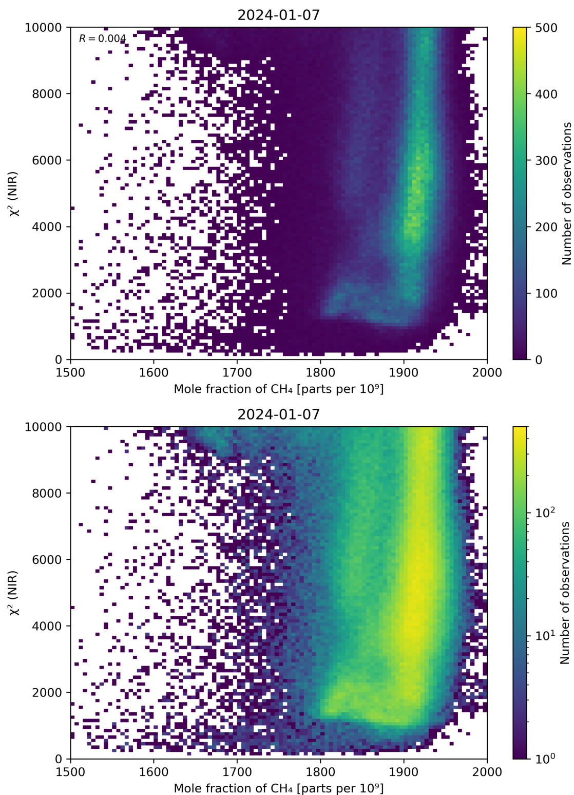
Figure 70: Scatter density plot of “Mole fraction of \text{CH}_4 ” against “ \chi^2 (NIR)” for 2024-01-06 to 2024-01-08.
