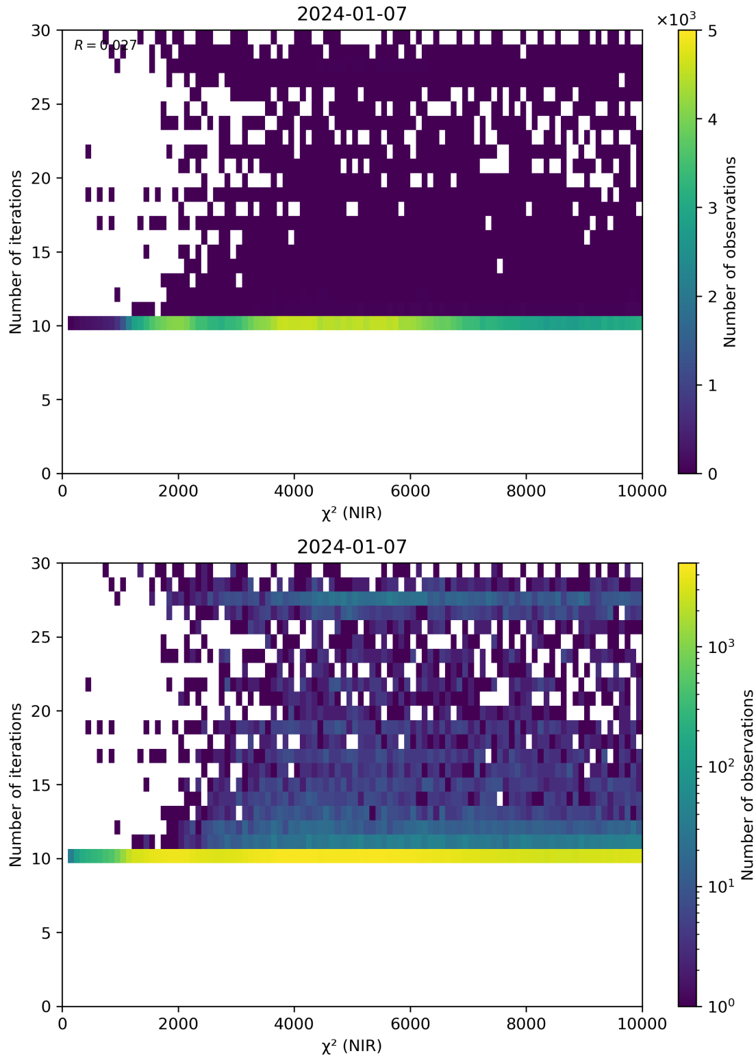
Figure 46: Scatter density plot of “ \chi^2 (NIR)” against “Number of iterations” for 2024-01-06 to 2024-01-08.
