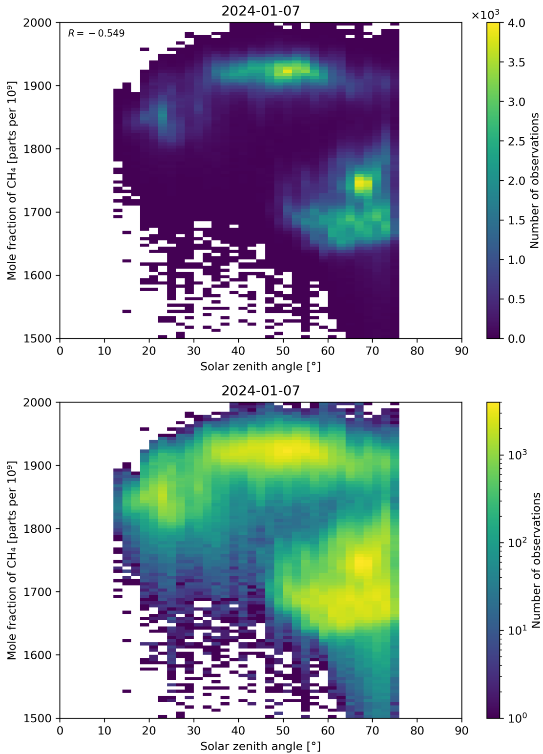
Figure 99: Scatter density plot of “Solar zenith angle” against “Mole fraction of \text{CH}_4 ” for 2024-01-06 to 2024-01-08.
