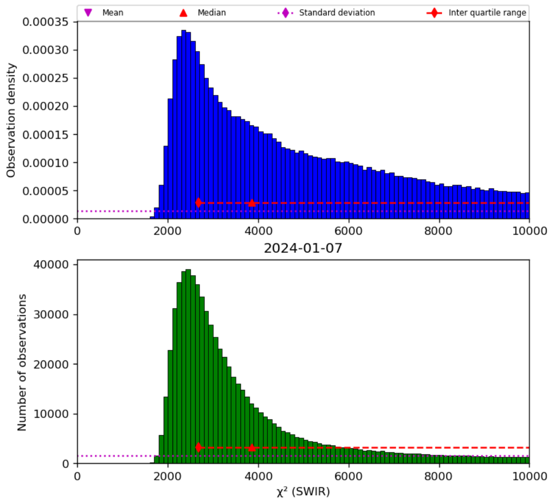
Figure 28: Histogram of “ \chi^2 (SWIR)” for 2024-01-06 to 2024-01-08
