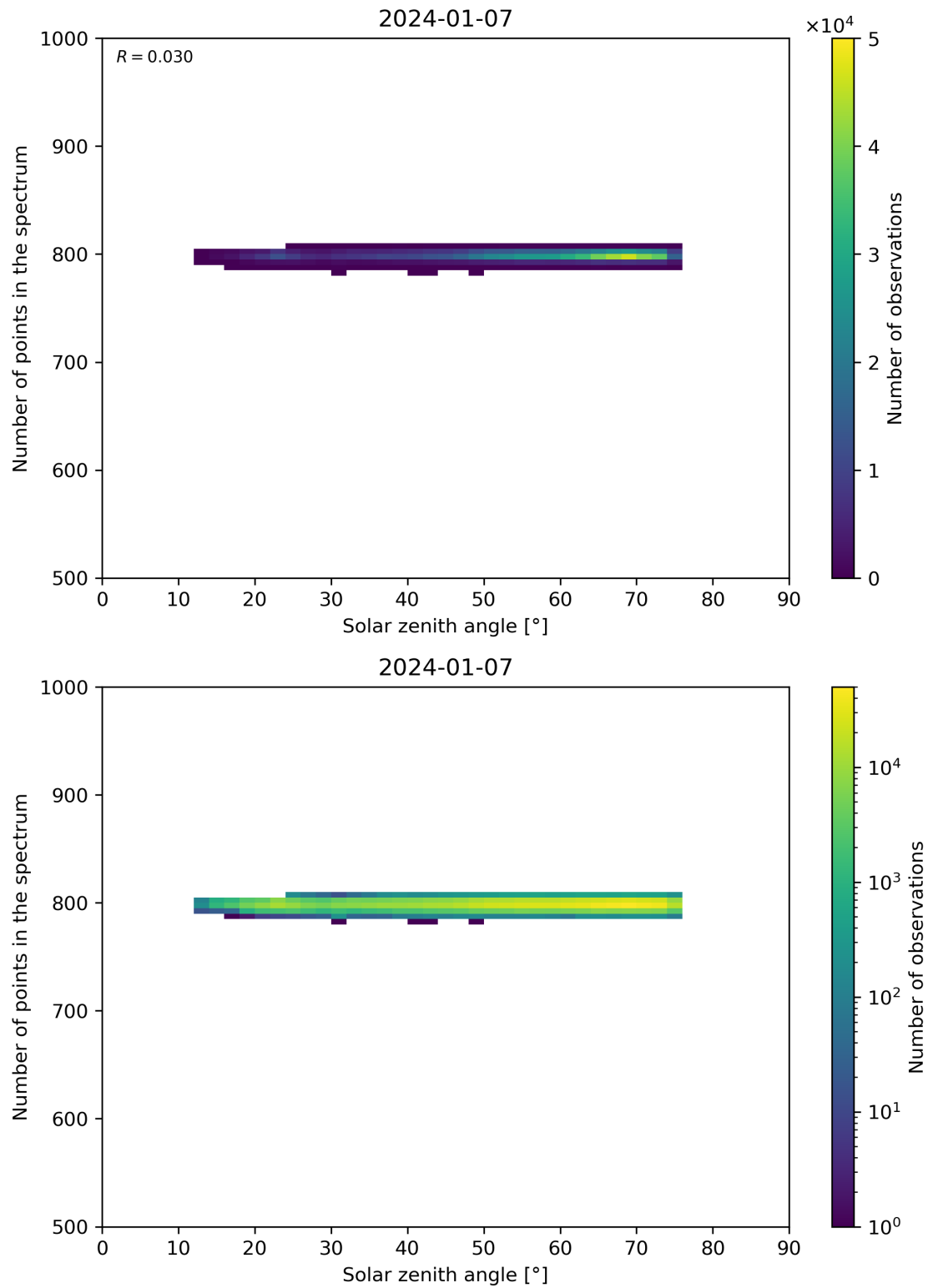
Figure 103: Scatter density plot of “Solar zenith angle” against “Number of points in the spectrum” for 2024-01-06 to 2024-01-08.
