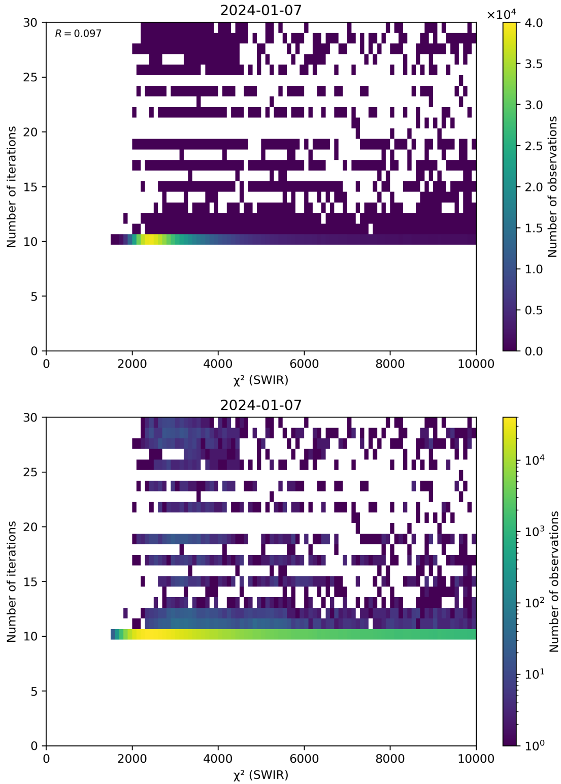
Figure 50: Scatter density plot of “ \chi^2 (SWIR)” against “Number of iterations” for 2024-01-06 to 2024-01-08.
