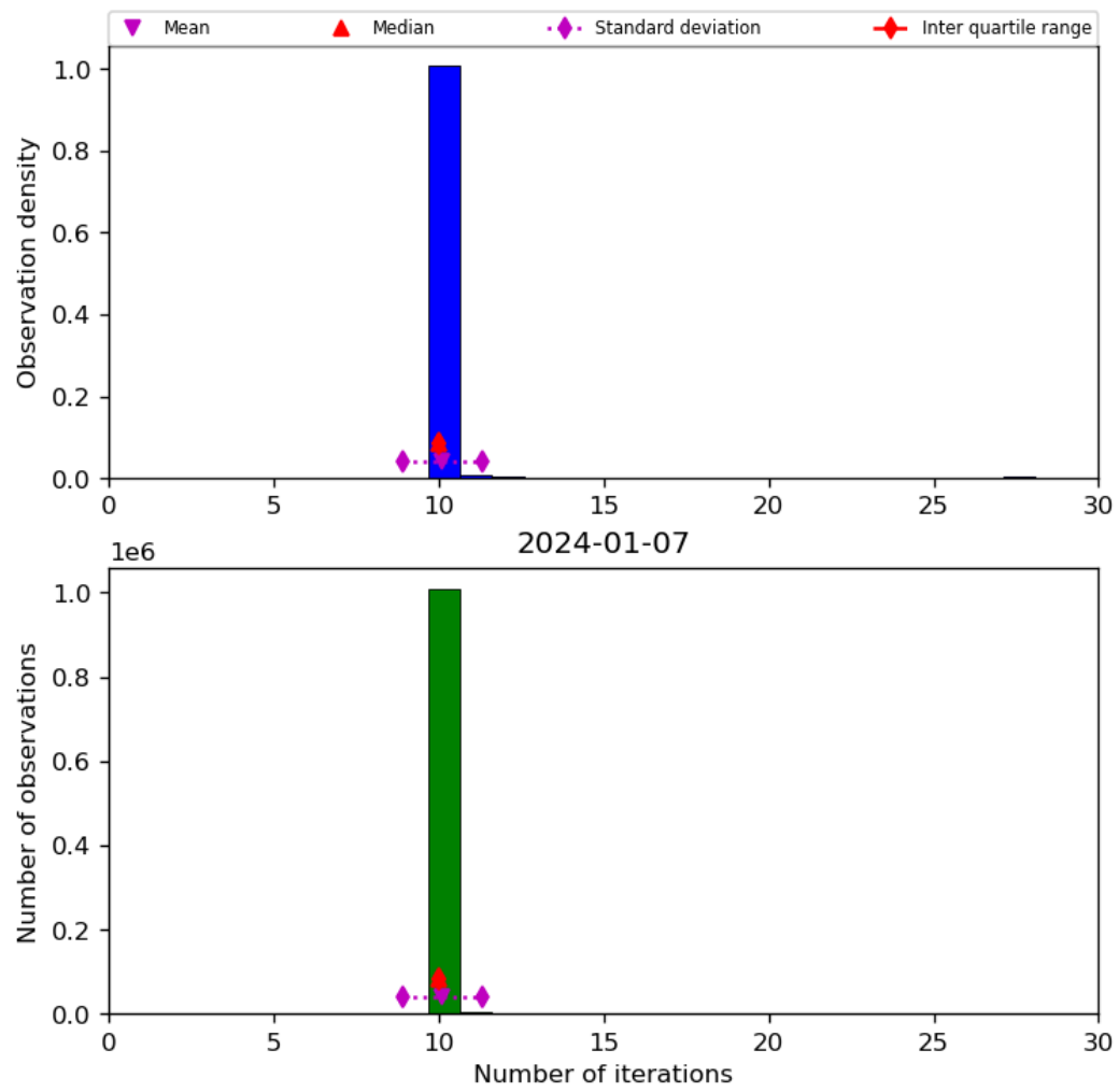
Figure 31: Histogram of “Number of iterations” for 2024-01-06 to 2024-01-08
