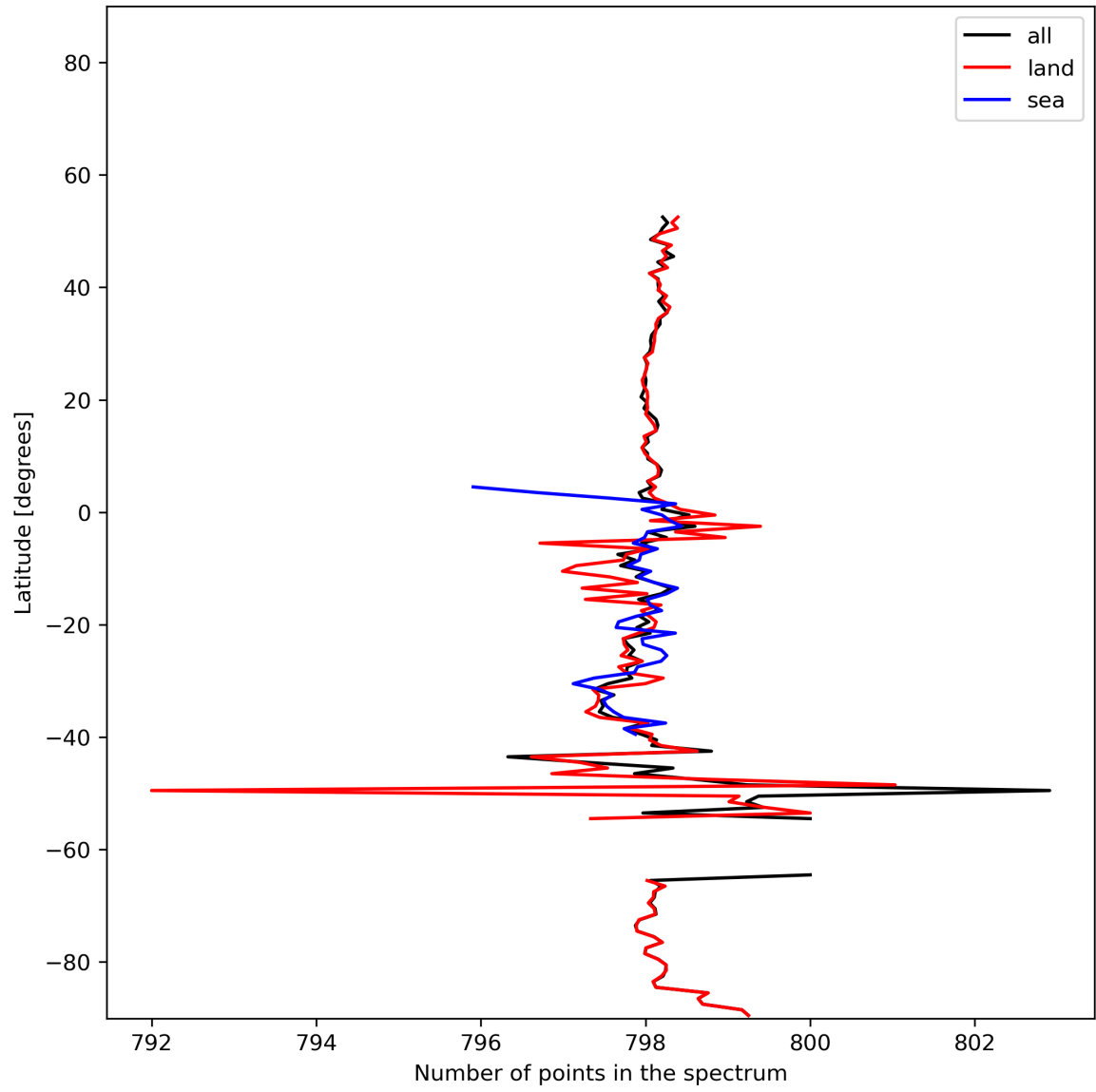
Figure 15: Zonal average of “Number of points in the spectrum” for 2024-01-06 to 2024-01-08.
