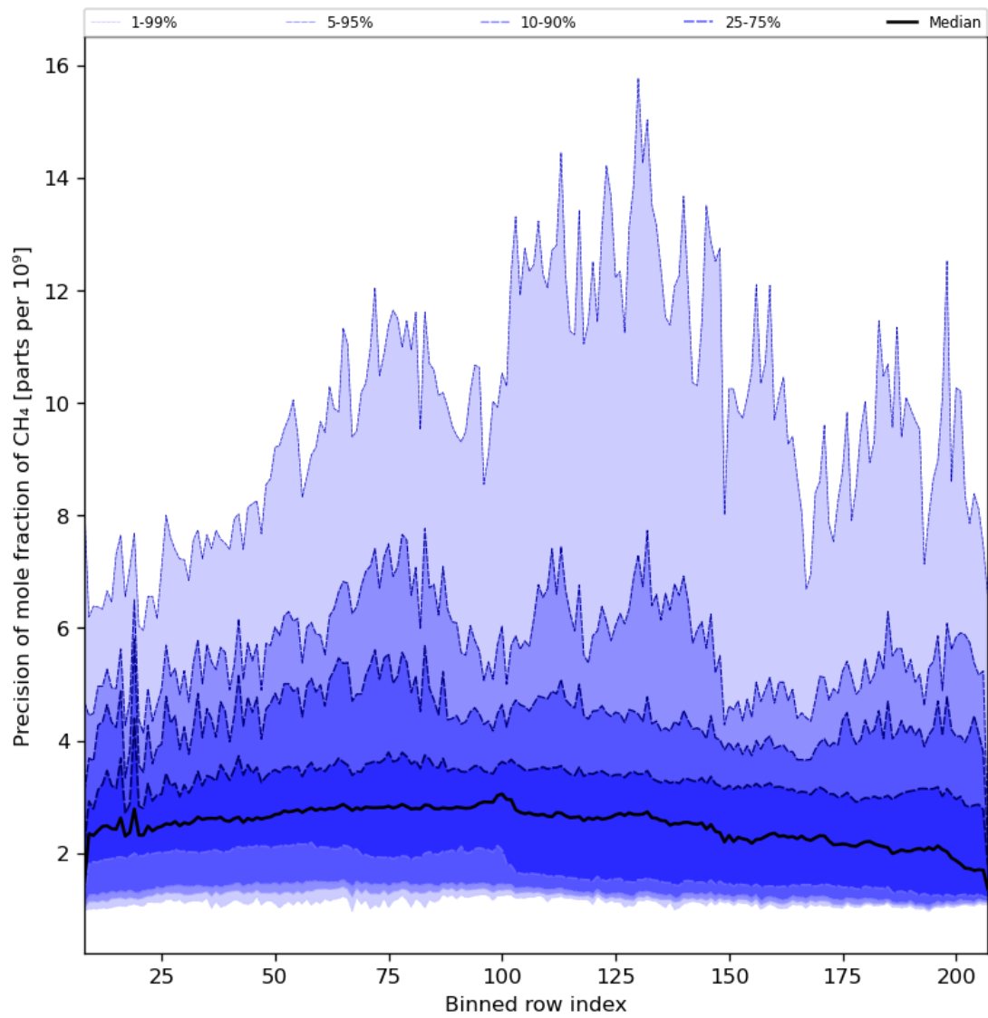
Figure 35: Along track statistics of “Precision of mole fraction of CH 4 ” for 2024-01-06 to 2024-01-08
