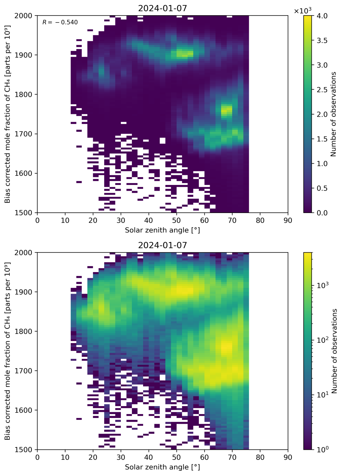
Figure 100: Scatter density plot of “Solar zenith angle” against “Bias corrected mole fraction of CH 4 ” for 2024-01-06 to 2024-01-08.
