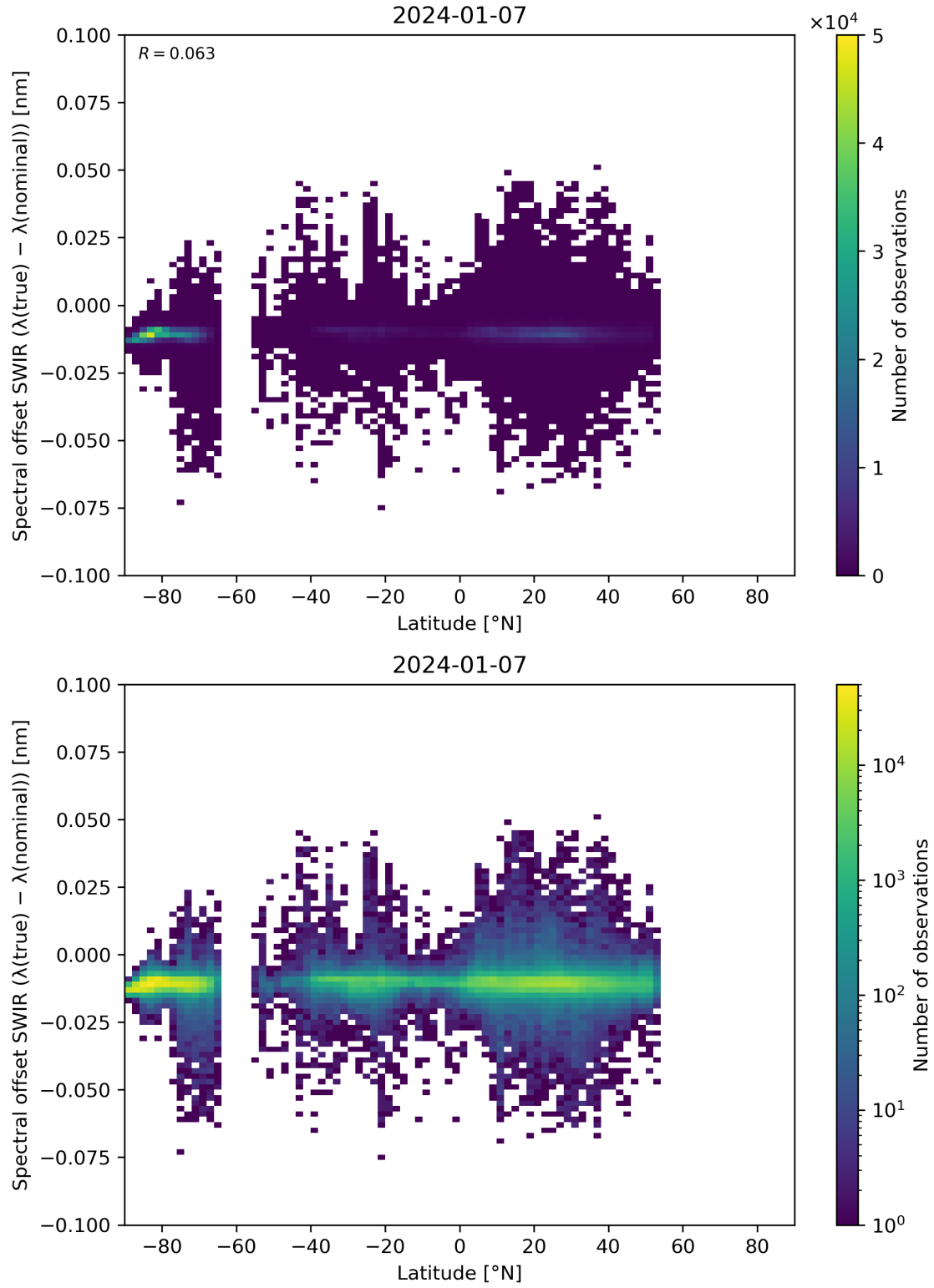
Figure 62: Scatter density plot of “Latitude” against “Spectral offset SWIR ( \lambda(\text{true}) - \lambda(\text{nominal}) )” for 2024-01-06 to 2024-01-08.
