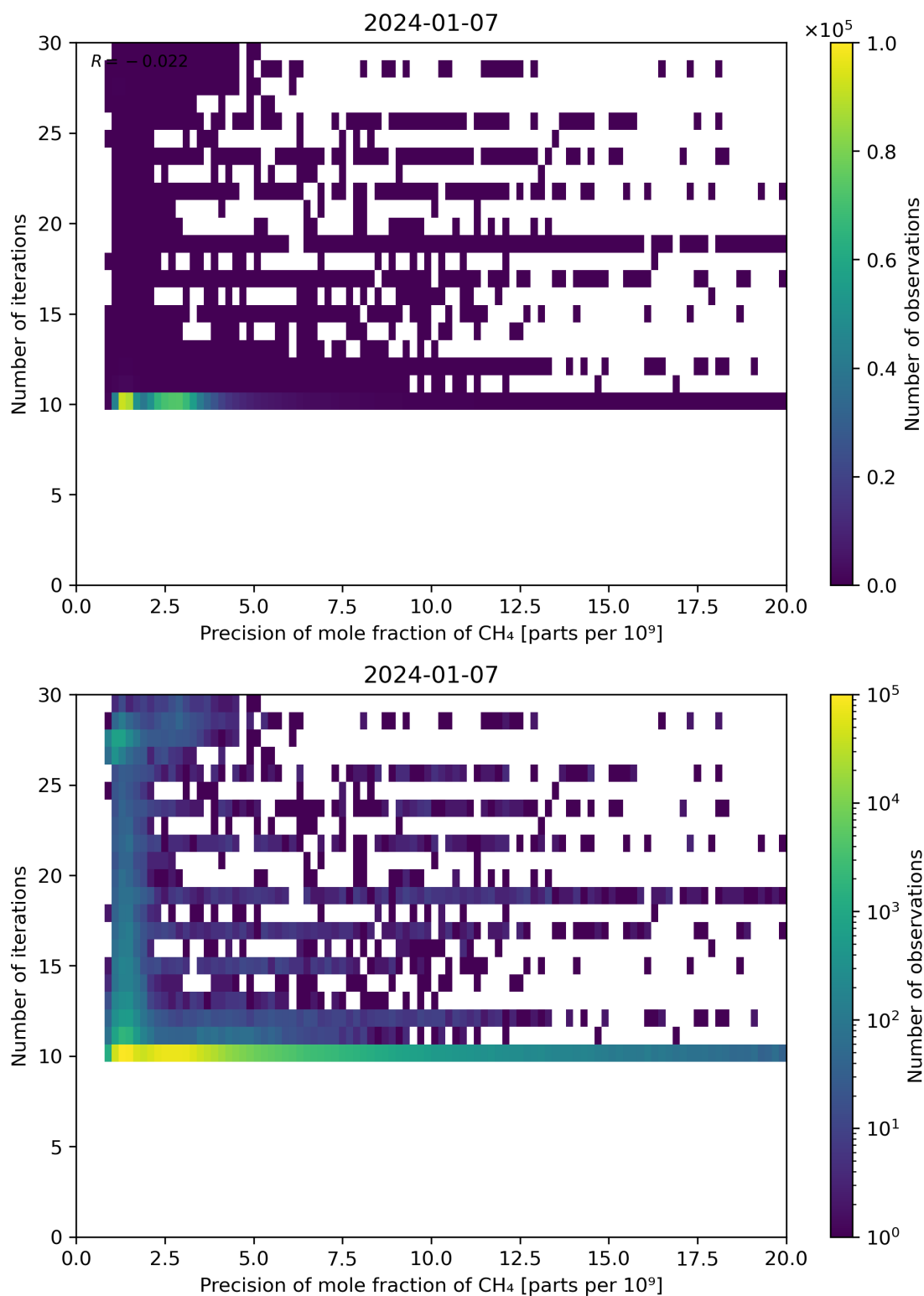
Figure 83: Scatter density plot of “Precision of mole fraction of CH 4 ” against “Number of iterations” for 2024-01-06 to 2024-01-08.
