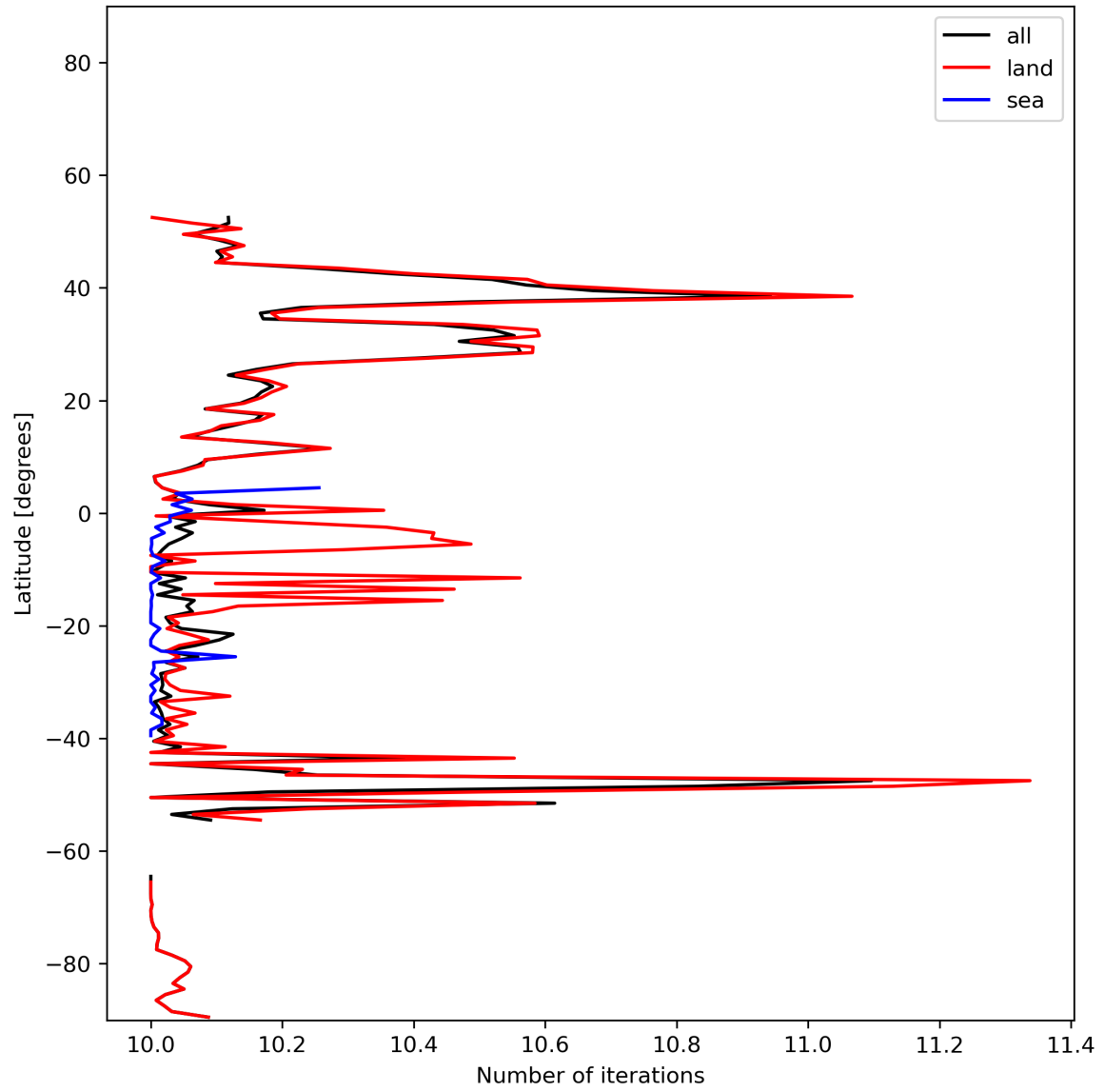
Figure 20: Zonal average of “Number of iterations” for 2024-01-06 to 2024-01-08.
