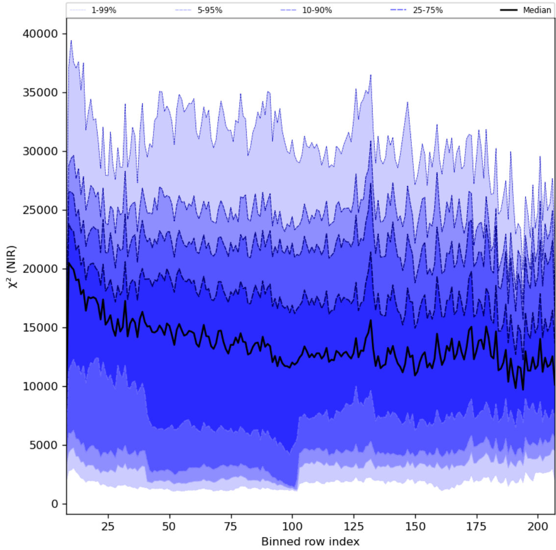
Figure 40: Along track statistics of “ \chi^2 (NIR)” for 2024-01-06 to 2024-01-08
