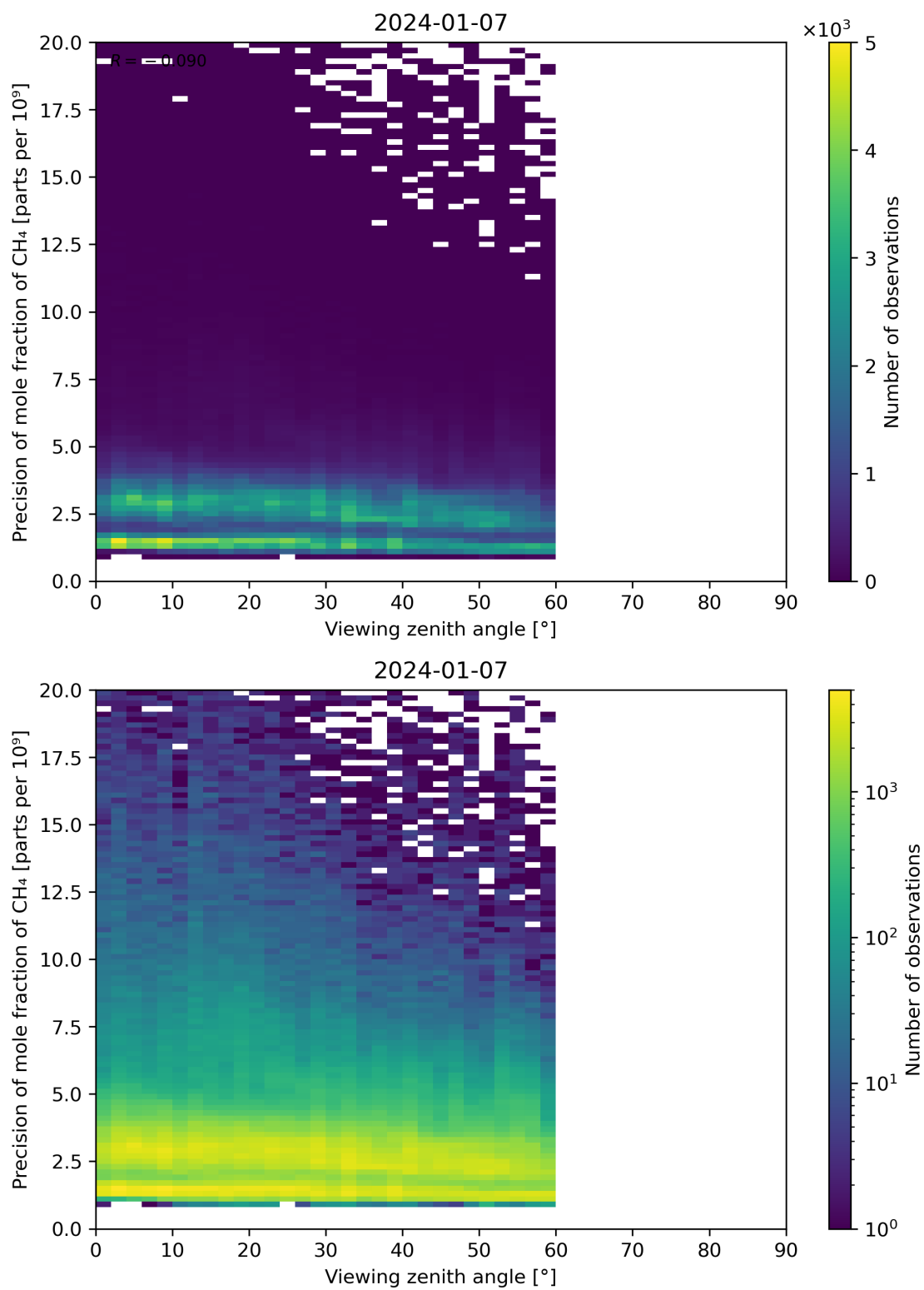
Figure 112: Scatter density plot of “Viewing zenith angle” against “Precision of mole fraction of CH 4 ” for 2024-01-06 to 2024-01-08.
