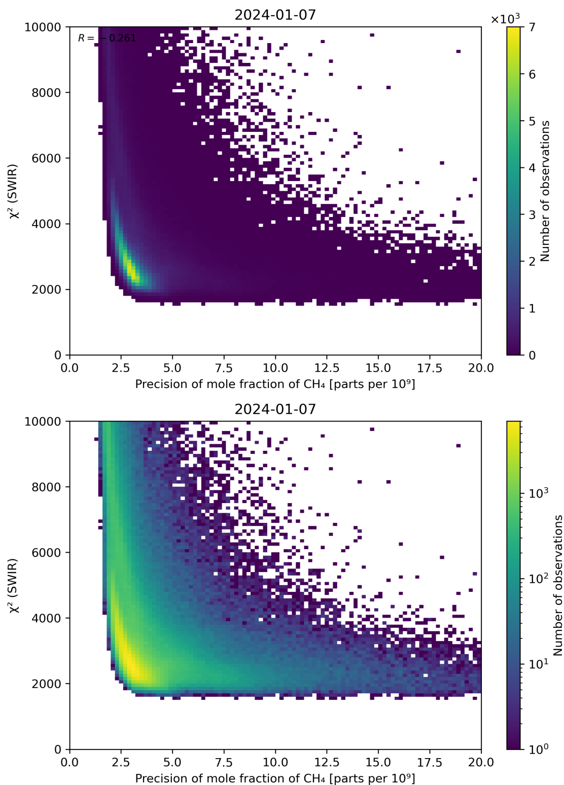
Figure 79: Scatter density plot of “Precision of mole fraction of CH 4 ” against “ \chi^2 (SWIR)” for 2024-01-06 to 2024-01-08.
