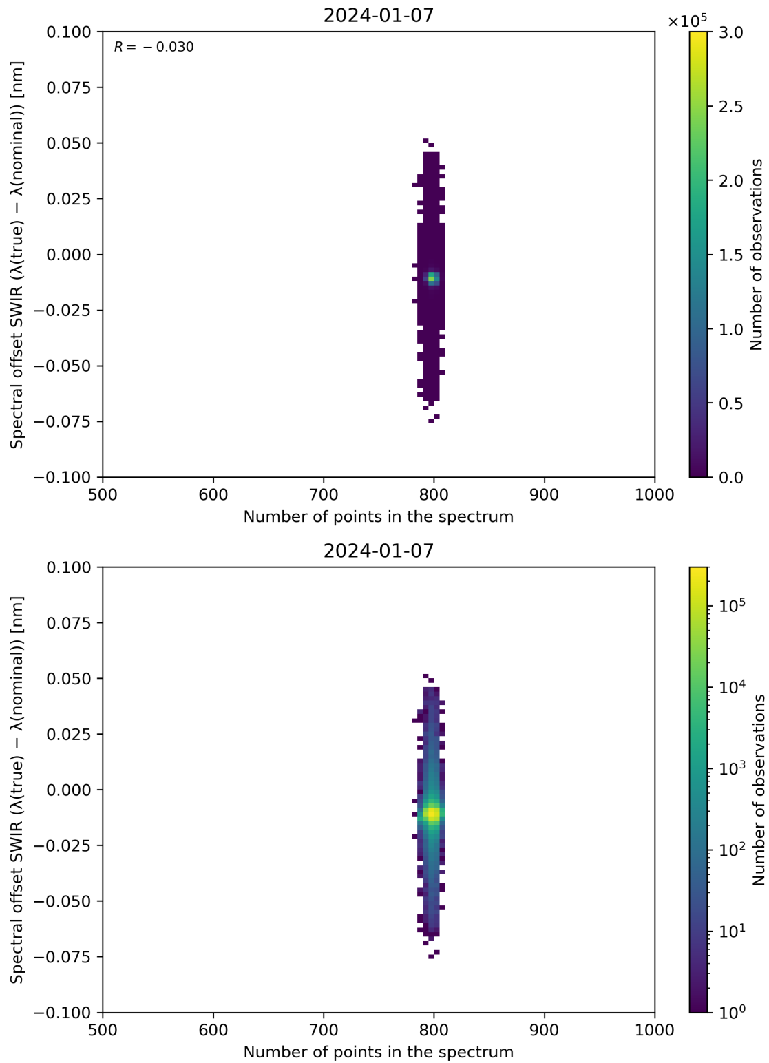
Figure 93: Scatter density plot of “Number of points in the spectrum” against “Spectral offset SWIR ( \lambda(\text{true}) - \lambda(\text{nominal}) )” for 2024-01-06 to 2024-01-08.
