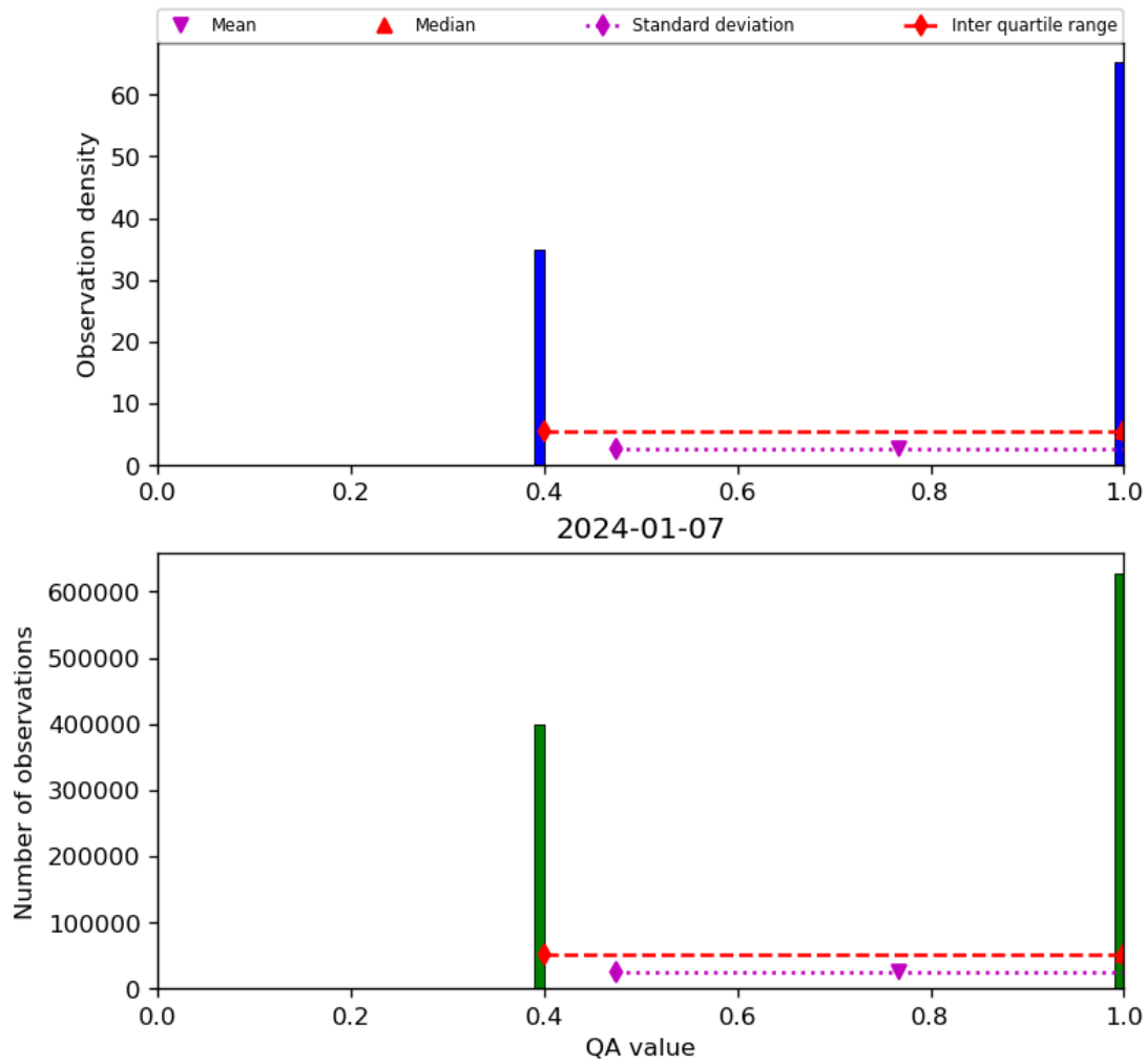
Figure 22: Histogram of “QA value” for 2024-01-06 to 2024-01-08
