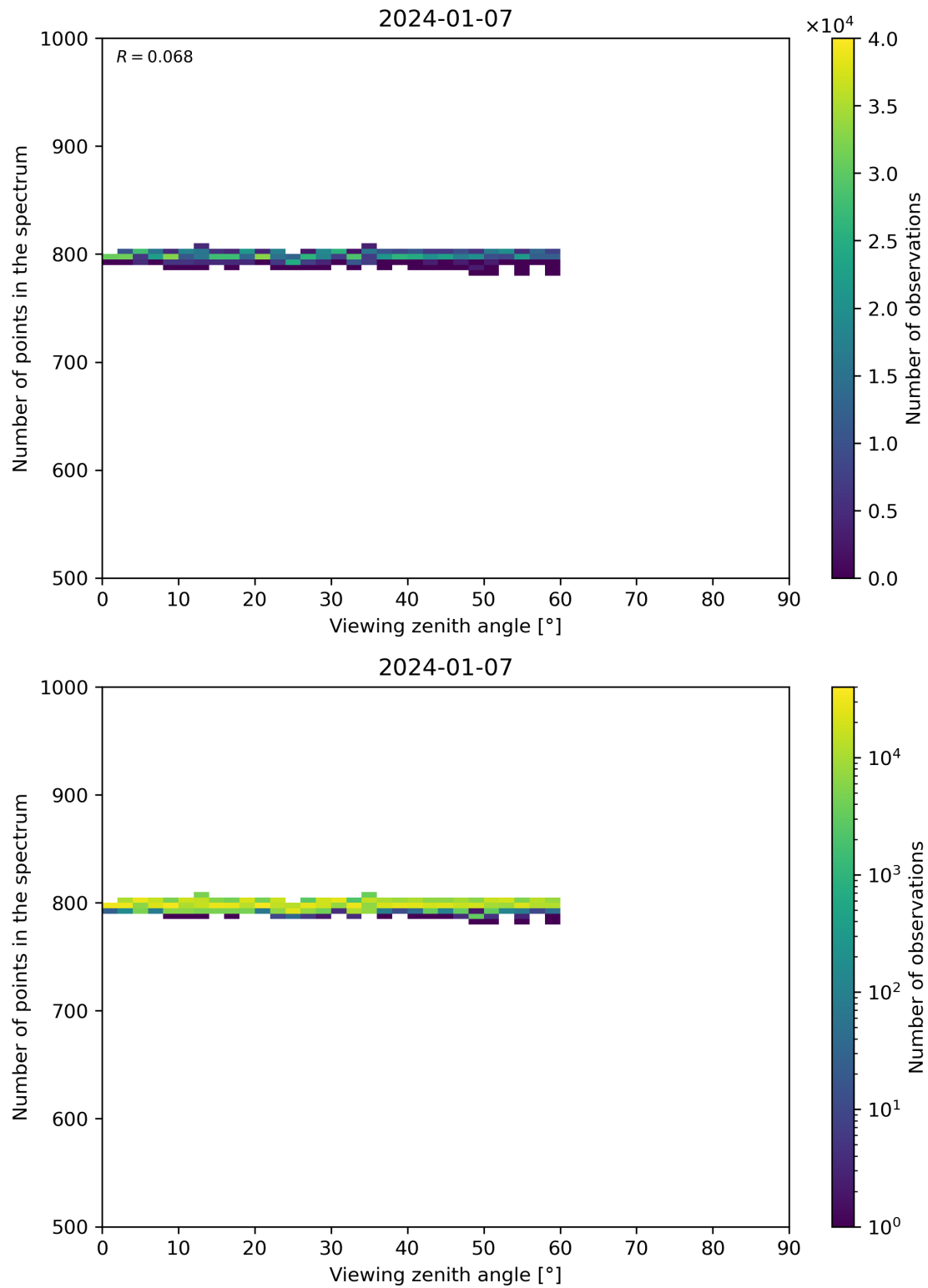
Figure 114: Scatter density plot of “Viewing zenith angle” against “Number of points in the spectrum” for 2024-01-06 to 2024-01-08.
