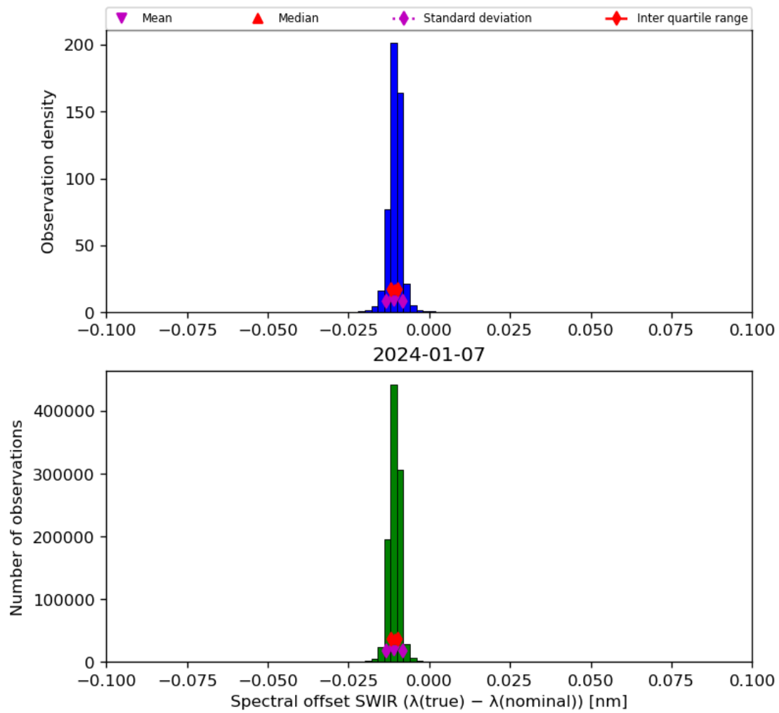
Figure 27: Histogram of “Spectral offset SWIR ( \lambda(\text{true}) - \lambda(\text{nominal}) )” for 2024-01-06 to 2024-01-08
