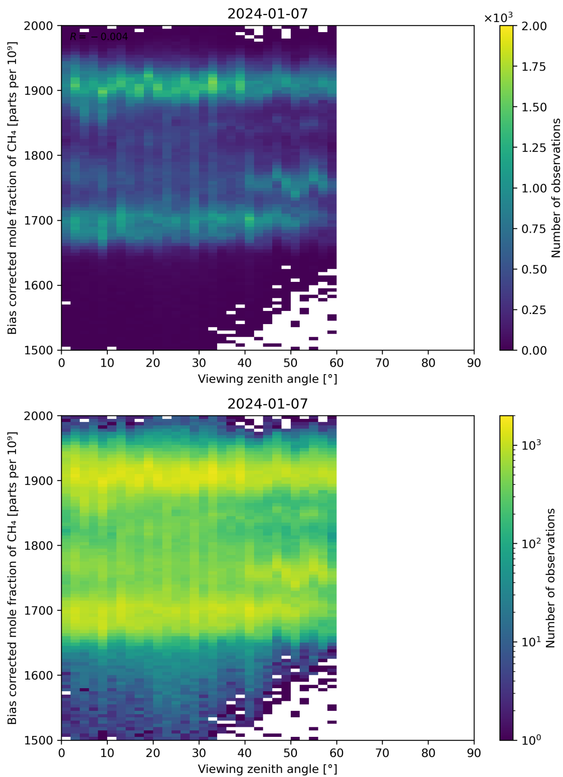
Figure 111: Scatter density plot of “Viewing zenith angle” against “Bias corrected mole fraction of CH 4 ” for 2024-01-06 to 2024-01-08.
