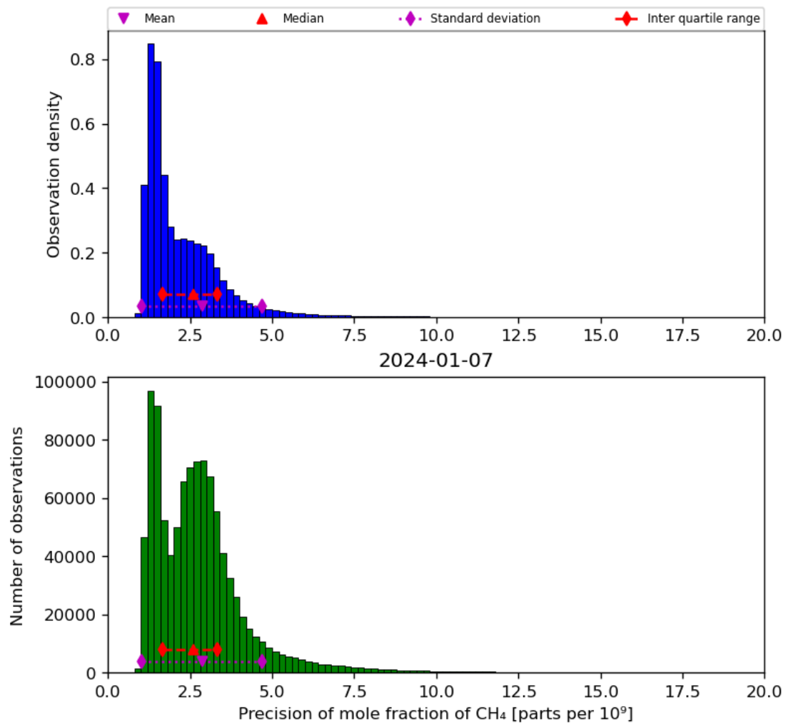
Figure 24: Histogram of “Precision of mole fraction of CH 4 ” for 2024-01-06 to 2024-01-08
