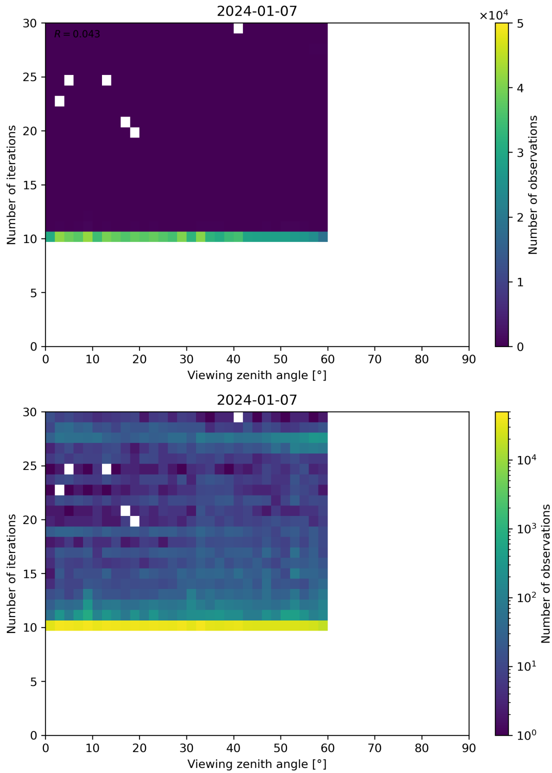
Figure 113: Scatter density plot of “Viewing zenith angle” against “Number of iterations” for 2024-01-06 to 2024-01-08.
