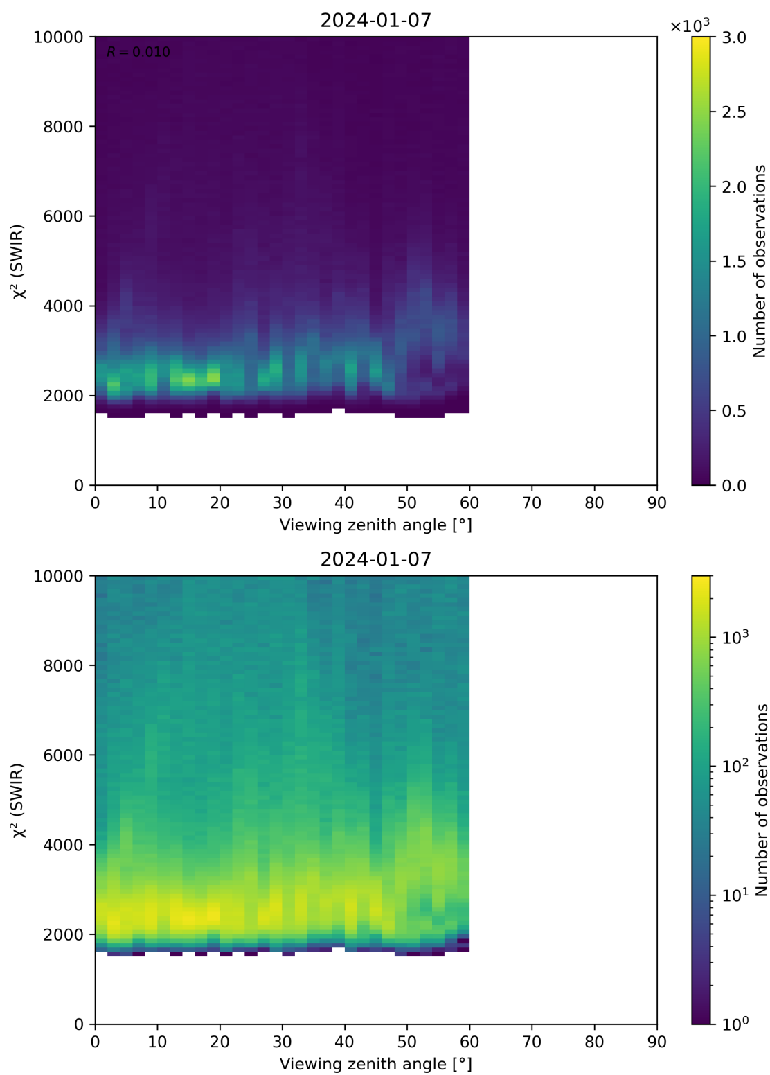
Figure 106: Scatter density plot of “Viewing zenith angle” against “ \chi^2 (SWIR)” for 2024-01-06 to 2024-01-08.
