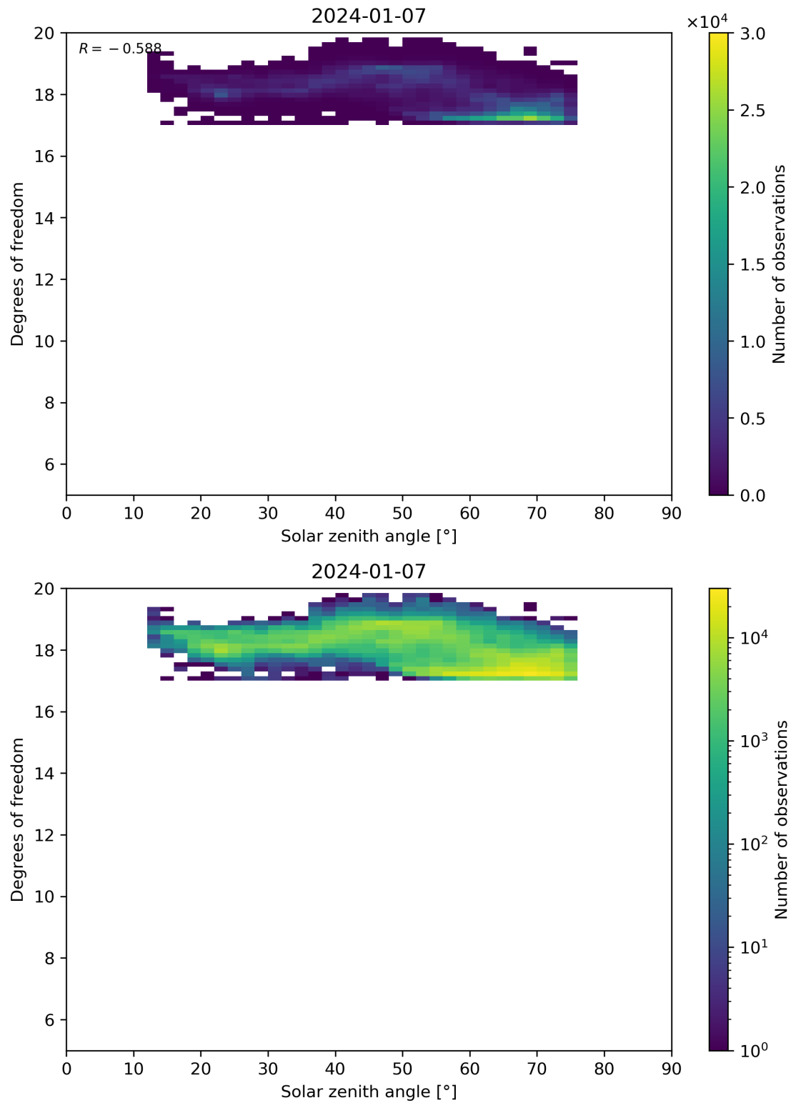
Figure 96: Scatter density plot of “Solar zenith angle” against “Degrees of freedom” for 2024-01-06 to 2024-01-08.
