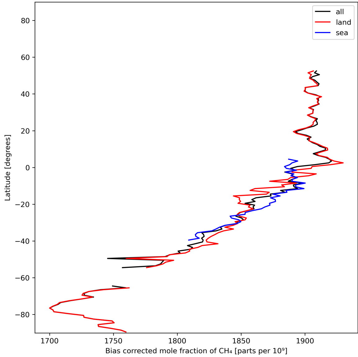
Figure 14: Zonal average of “Bias corrected mole fraction of \text{CH}_4 ” for 2024-01-06 to 2024-01-08.
