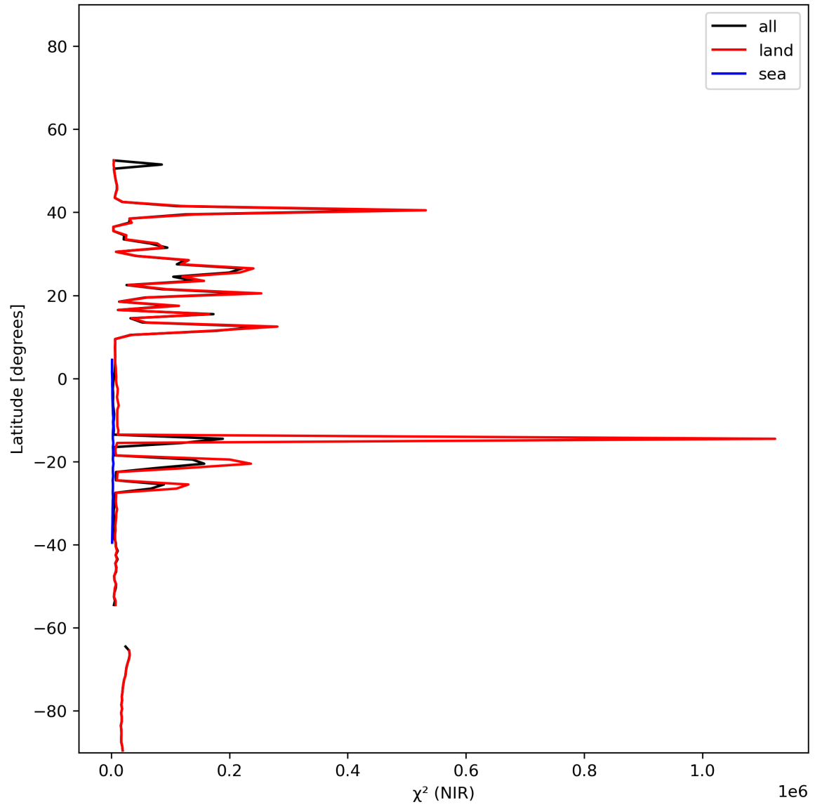
Figure 18: Zonal average of “ \chi^2 (NIR)” for 2024-01-06 to 2024-01-08.
