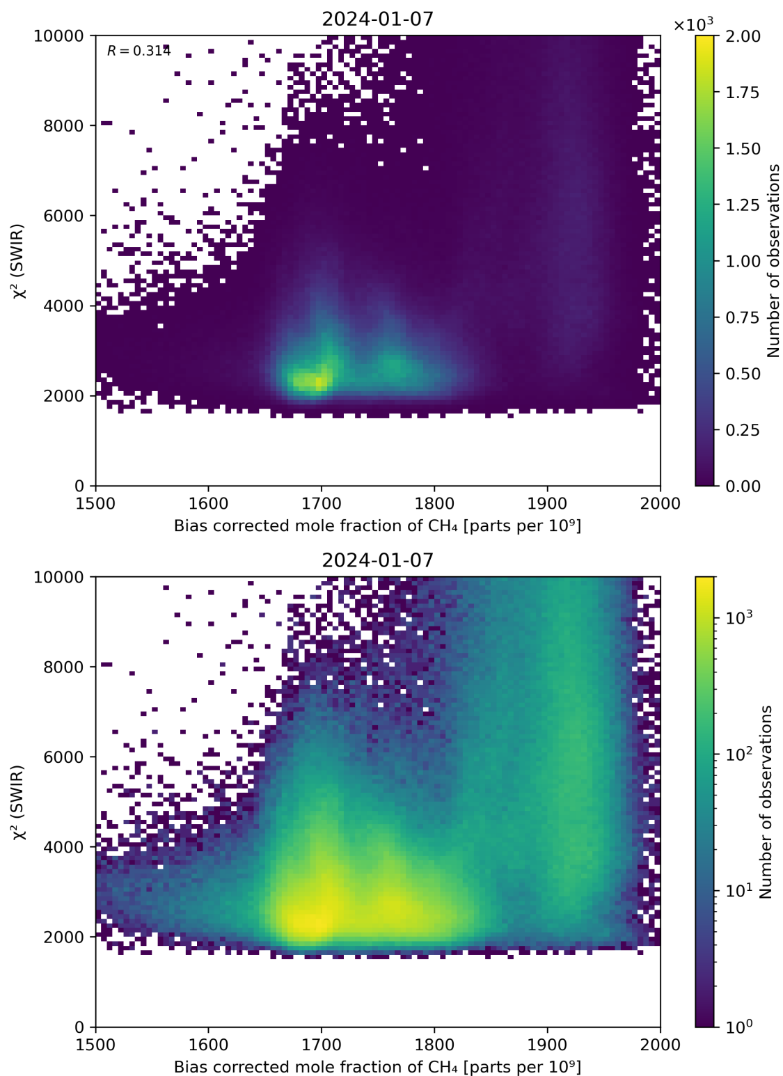
Figure 64: Scatter density plot of “Bias corrected mole fraction of \text{CH}_4 ” against “ \chi^2 (SWIR)” for 2024-01-06 to 2024-01-08.
