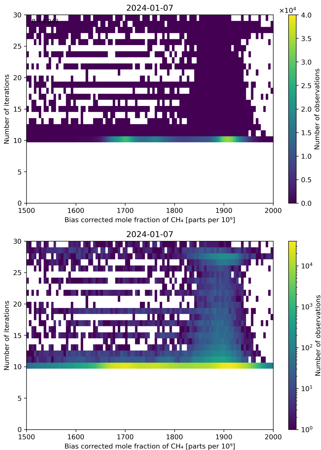
Figure 67: Scatter density plot of “Bias corrected mole fraction of \text{CH}_4 ” against “Number of iterations” for 2024-01-06 to 2024-01-08.
