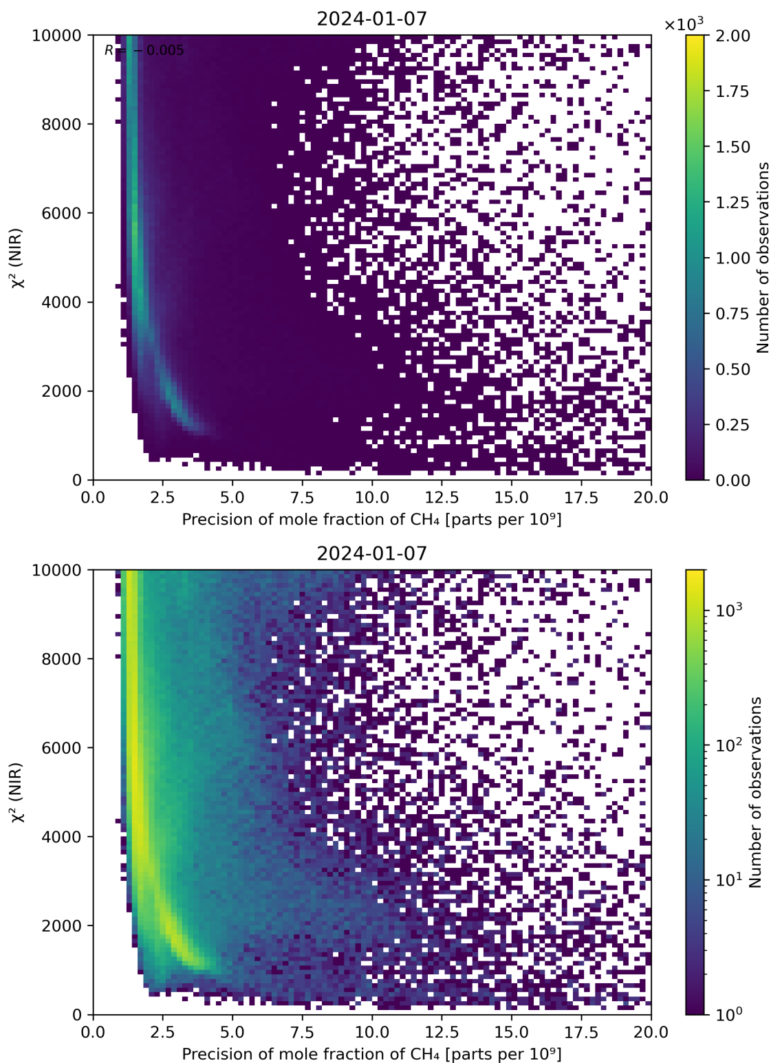
Figure 78: Scatter density plot of “Precision of mole fraction of CH 4 ” against “ \chi^2 (NIR)” for 2024-01-06 to 2024-01-08.
