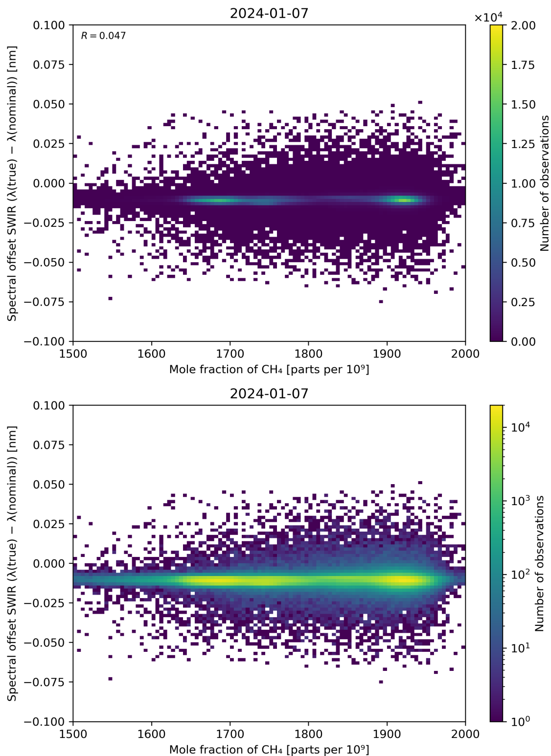
Figure 86: Scatter density plot of “Mole fraction of CH 4 ” against “Spectral offset SWIR ( \lambda(\text{true}) - \lambda(\text{nominal}) )” for 2024-01-06 to 2024-01-08.
