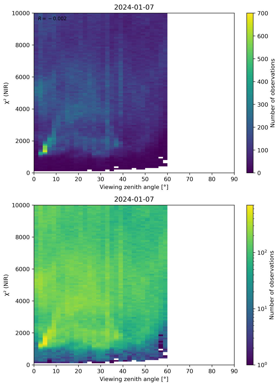
Figure 105: Scatter density plot of “Viewing zenith angle” against “ \chi^2 (NIR)” for 2024-01-06 to 2024-01-08.
