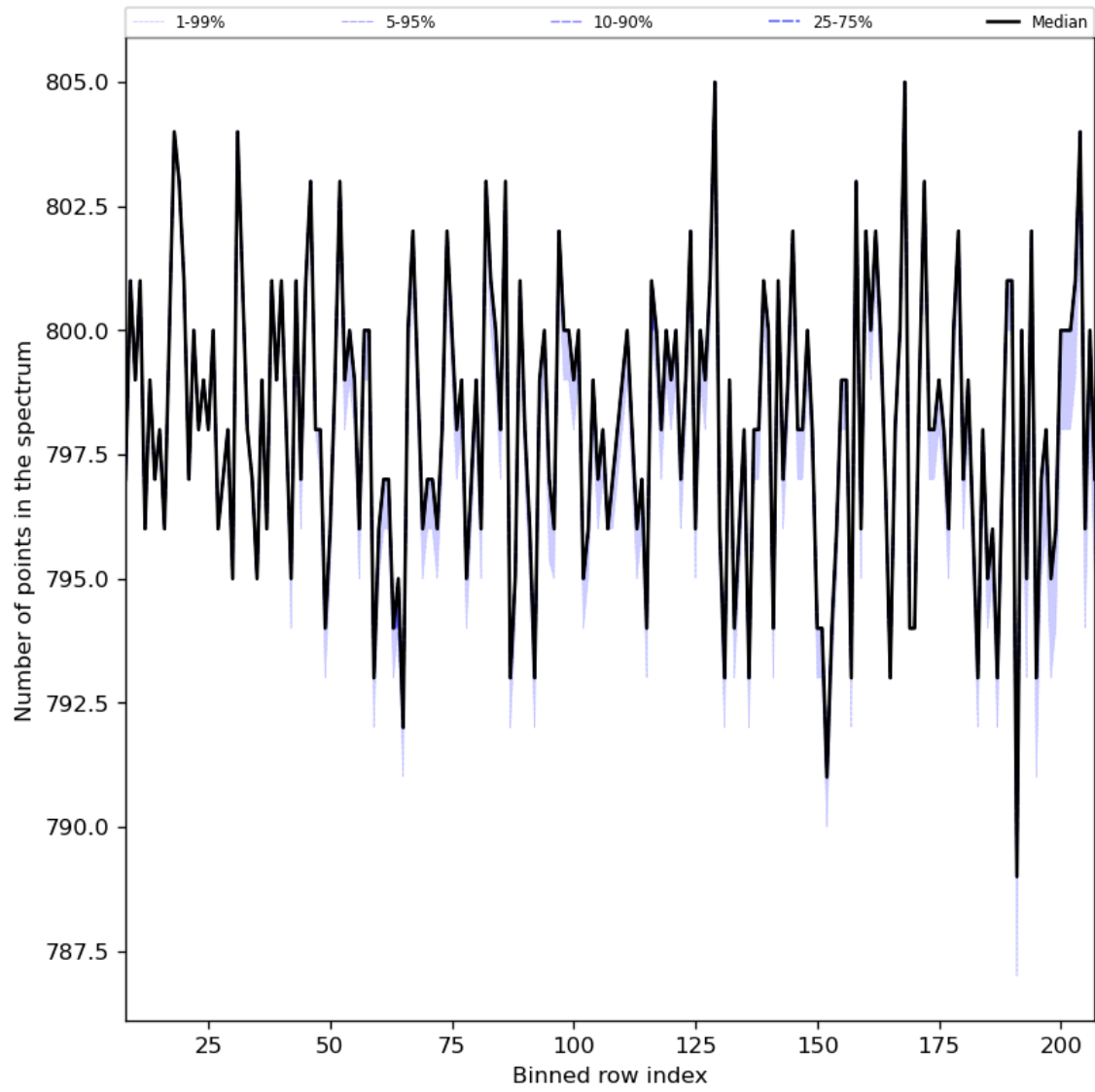
Figure 37: Along track statistics of “Number of points in the spectrum” for 2024-01-06 to 2024-01-08
