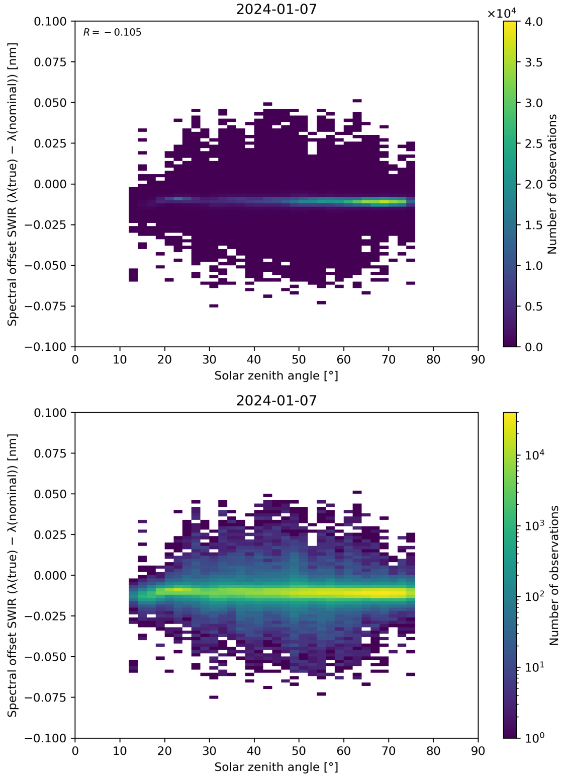
Figure 104: Scatter density plot of “Solar zenith angle” against “Spectral offset SWIR ( \lambda(\text{true}) - \lambda(\text{nominal}) )” for 2024-01-06 to 2024-01-08.
