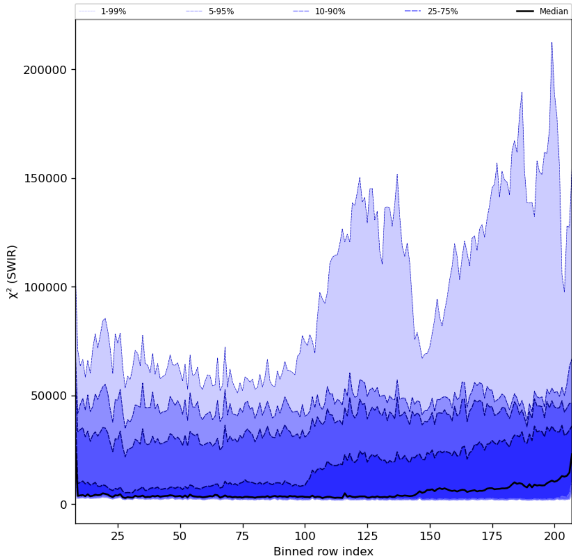
Figure 39: Along track statistics of “ \chi^2 (SWIR)” for 2024-01-06 to 2024-01-08
