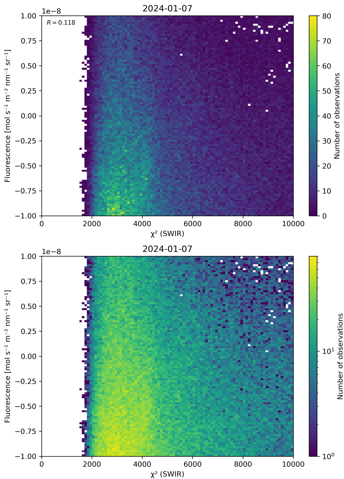
Figure 49: Scatter density plot of “ \chi^2 (SWIR)” against “Fluorescence” for 2024-01-06 to 2024-01-08.
