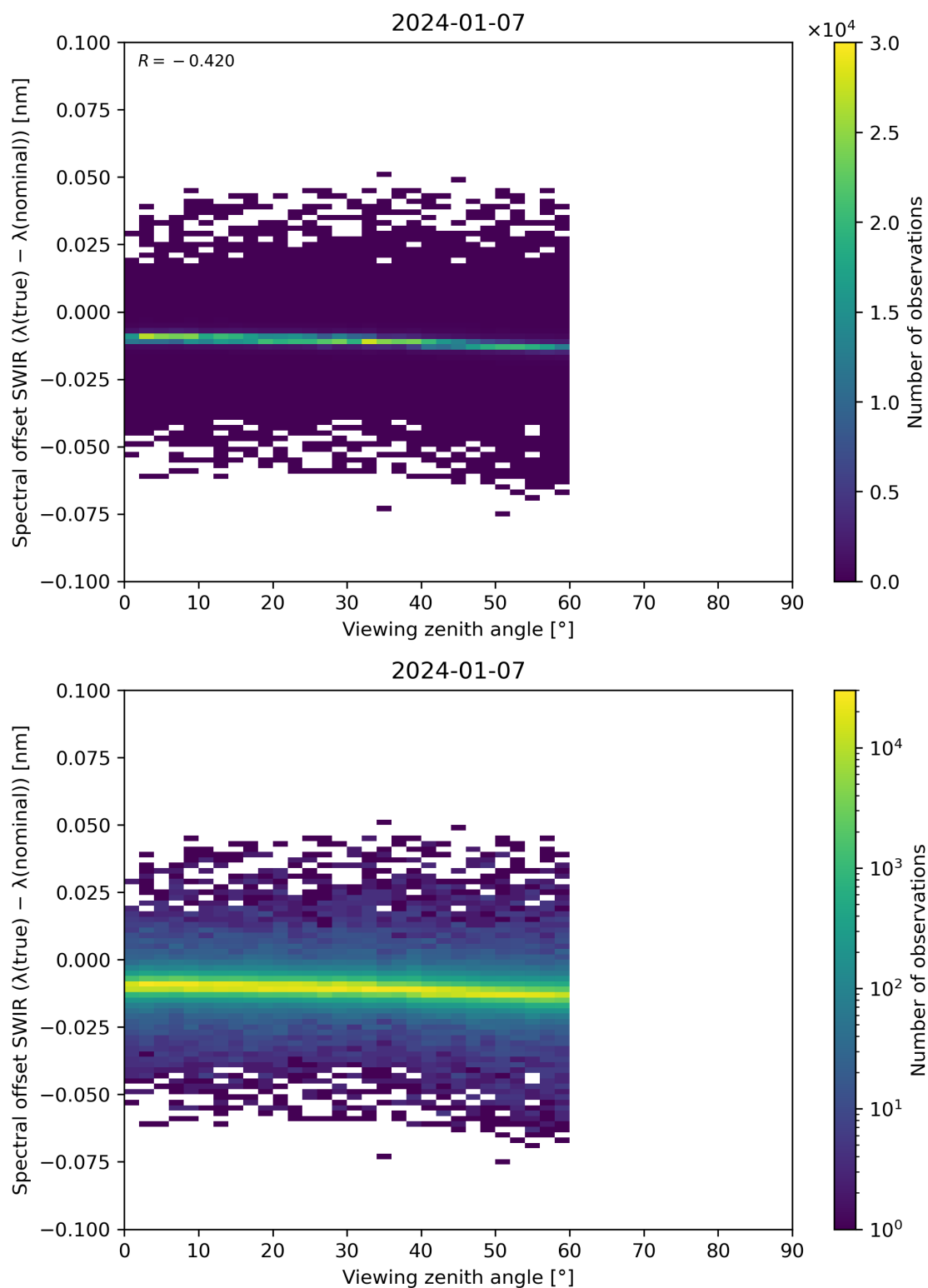
Figure 116: Scatter density plot of “Viewing zenith angle” against “Spectral offset SWIR ( \lambda(\text{true}) - \lambda(\text{nominal}) )” for 2024-01-06 to 2024-01-08.
