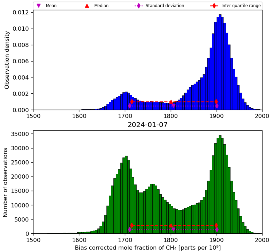
Figure 25: Histogram of “Bias corrected mole fraction of CH 4 ” for 2024-01-06 to 2024-01-08
