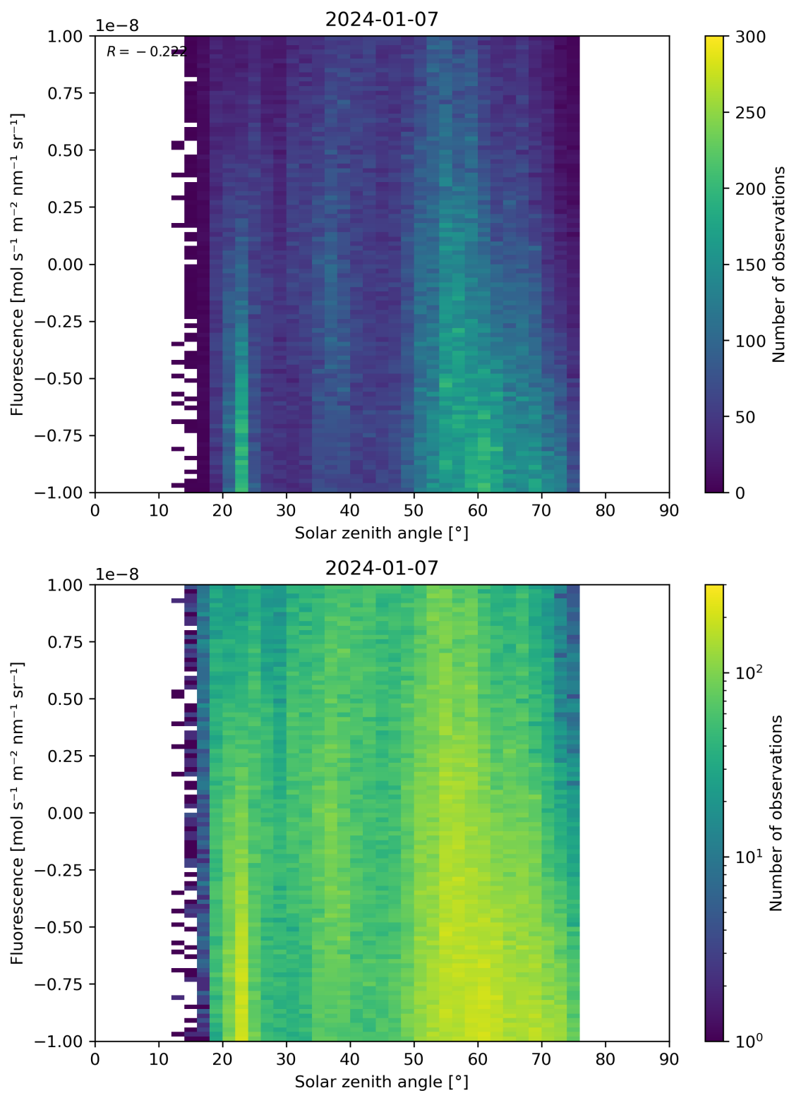
Figure 97: Scatter density plot of “Solar zenith angle” against “Fluorescence” for 2024-01-06 to 2024-01-08.
