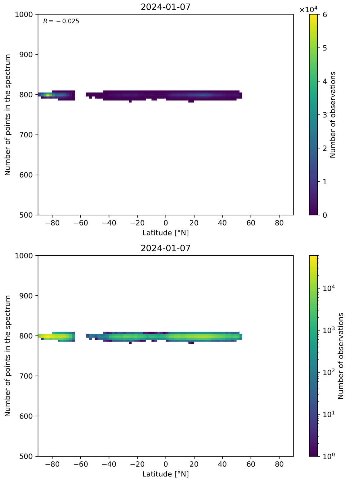
Figure 61: Scatter density plot of “Latitude” against “Number of points in the spectrum” for 2024-01-06 to 2024-01-08.
