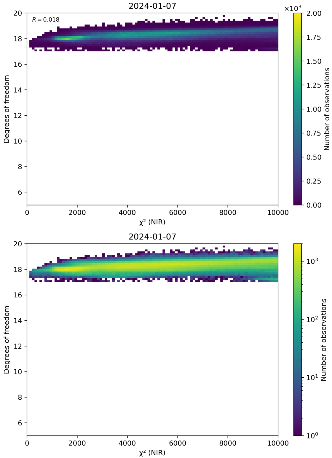
Figure 44: Scatter density plot of “ \chi^2 (NIR)” against “Degrees of freedom” for 2024-01-06 to 2024-01-08.
