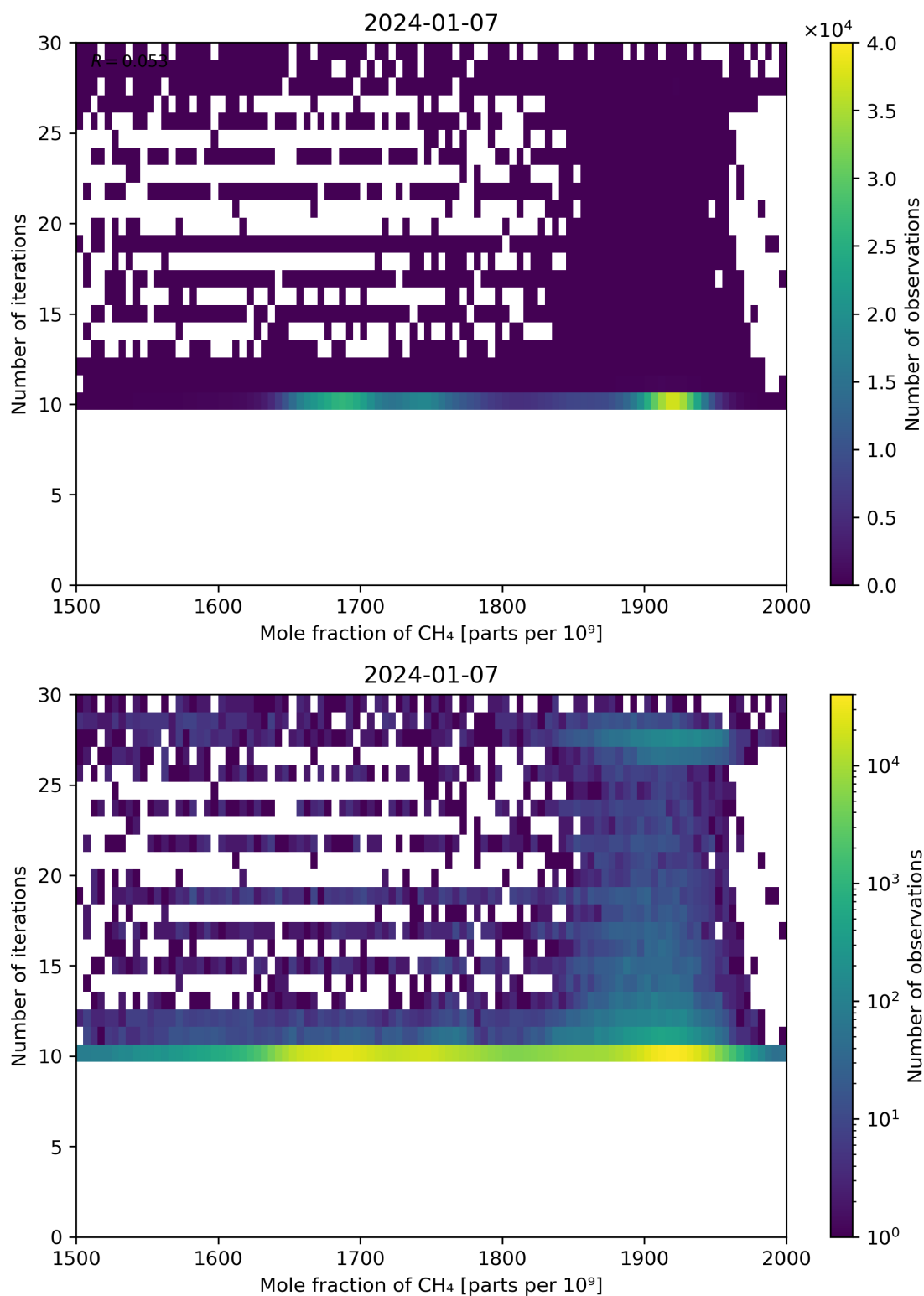
Figure 76: Scatter density plot of “Mole fraction of CH 4 ” against “Number of iterations” for 2024-01-06 to 2024-01-08.
