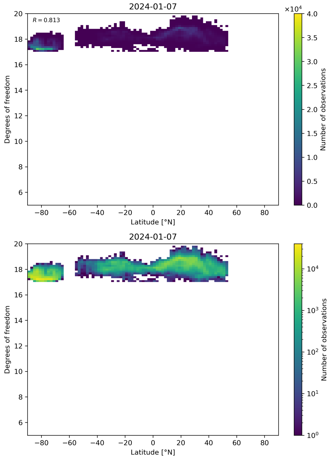
Figure 55: Scatter density plot of “Latitude” against “Degrees of freedom” for 2024-01-06 to 2024-01-08.
