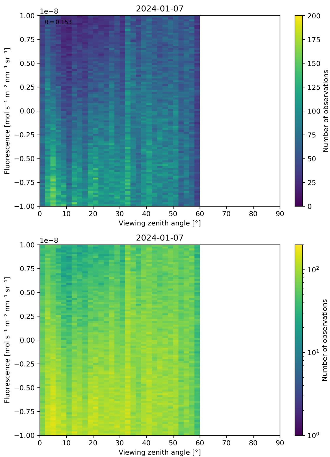
Figure 108: Scatter density plot of “Viewing zenith angle” against “Fluorescence” for 2024-01-06 to 2024-01-08.
