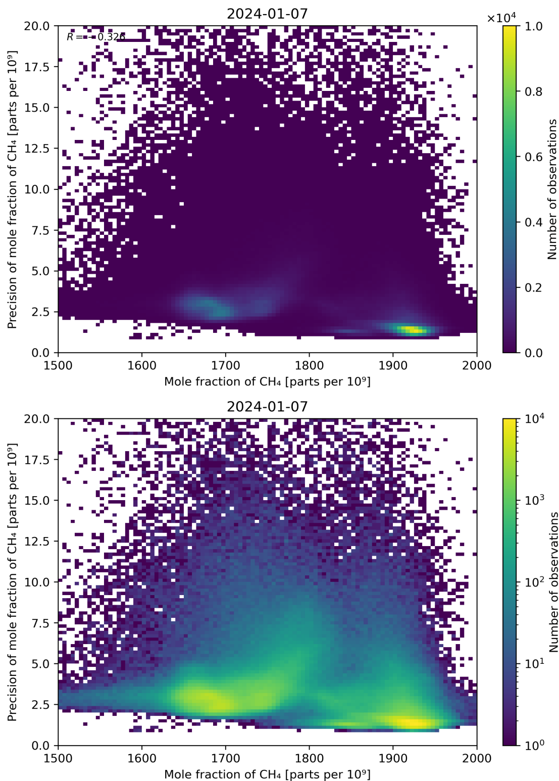
Figure 75: Scatter density plot of “Mole fraction of CH 4 ” against “Precision of mole fraction of CH 4 ” for 2024-01-06 to 2024-01-08.
