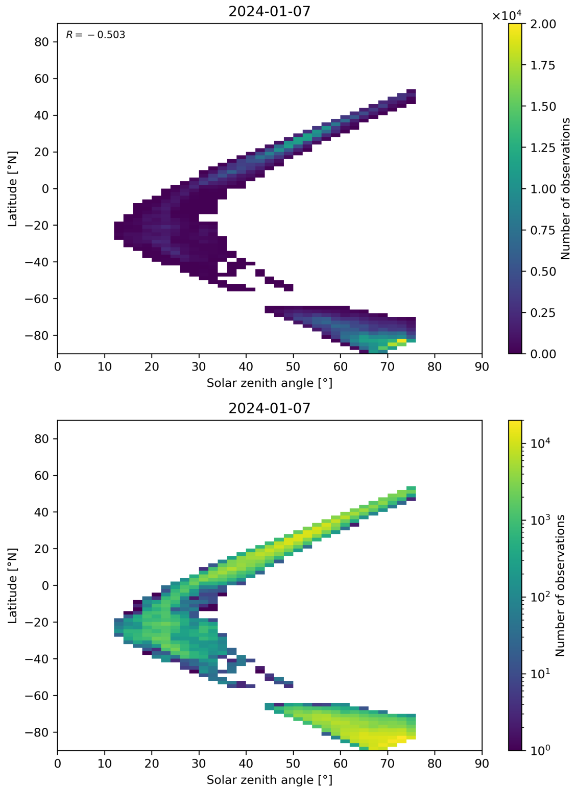
Figure 98: Scatter density plot of “Solar zenith angle” against “Latitude” for 2024-01-06 to 2024-01-08.
