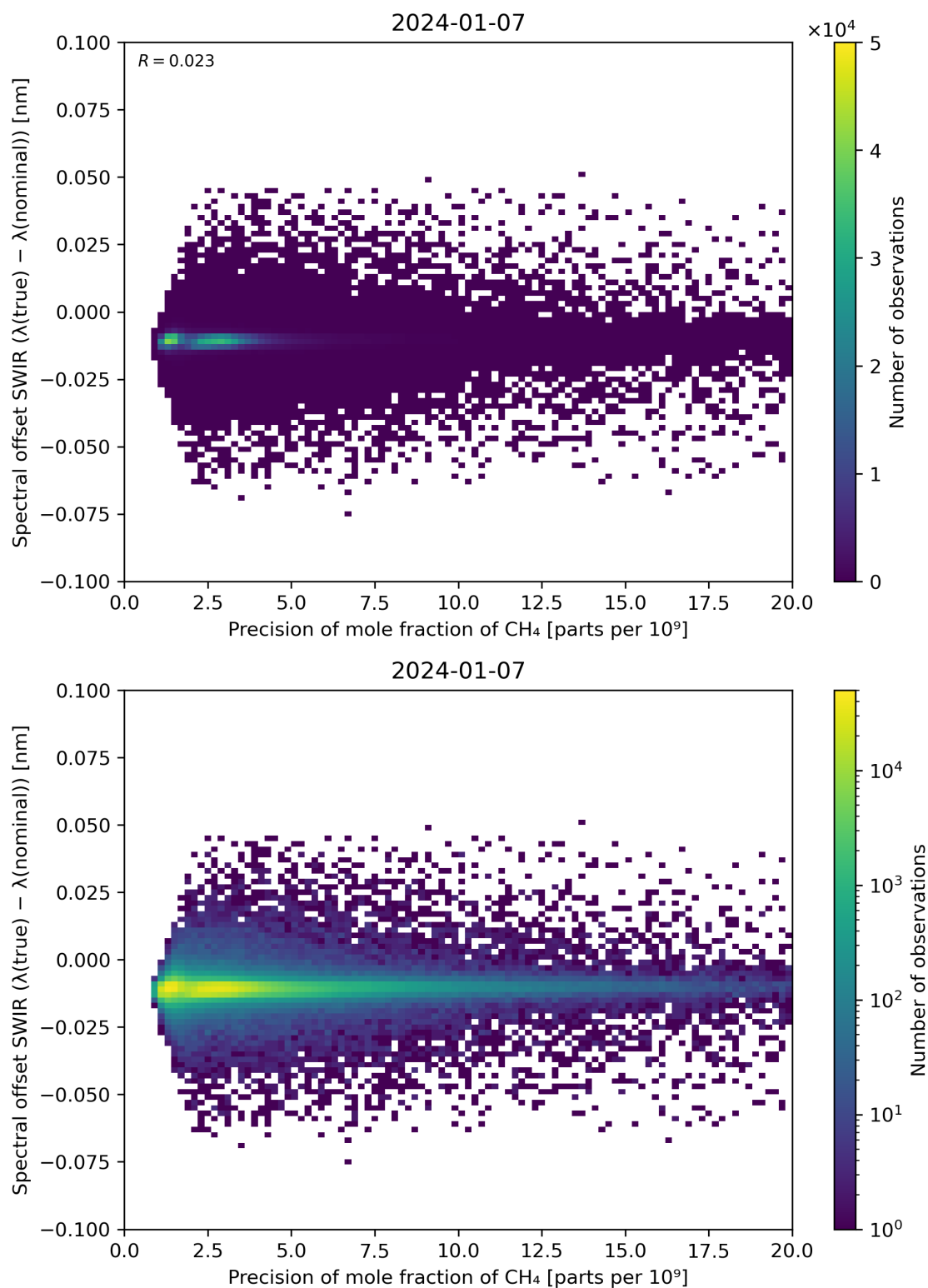
Figure 85: Scatter density plot of “Precision of mole fraction of CH 4 ” against “Spectral offset SWIR ( \lambda(\text{true}) - \lambda(\text{nominal}) )” for 2024-01-06 to 2024-01-08.
