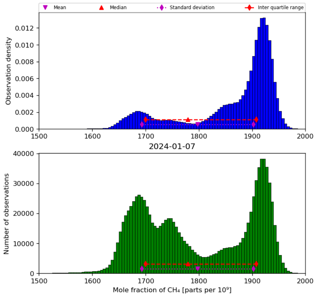
Figure 23: Histogram of “Mole fraction of CH 4 ” for 2024-01-06 to 2024-01-08
