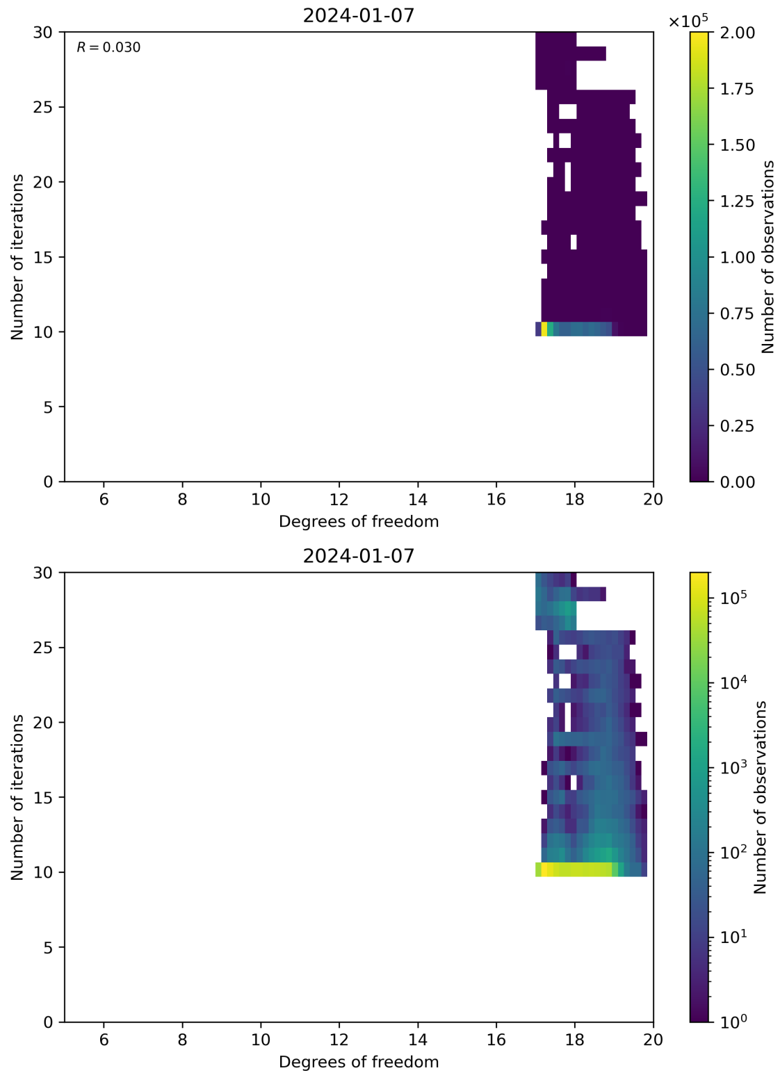
Figure 52: Scatter density plot of “Degrees of freedom” against “Number of iterations” for 2024-01-06 to 2024-01-08.
