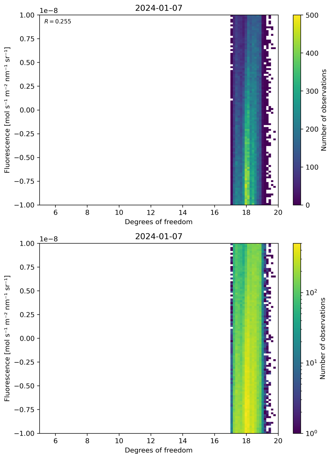
Figure 51: Scatter density plot of “Degrees of freedom” against “Fluorescence” for 2024-01-06 to 2024-01-08.
