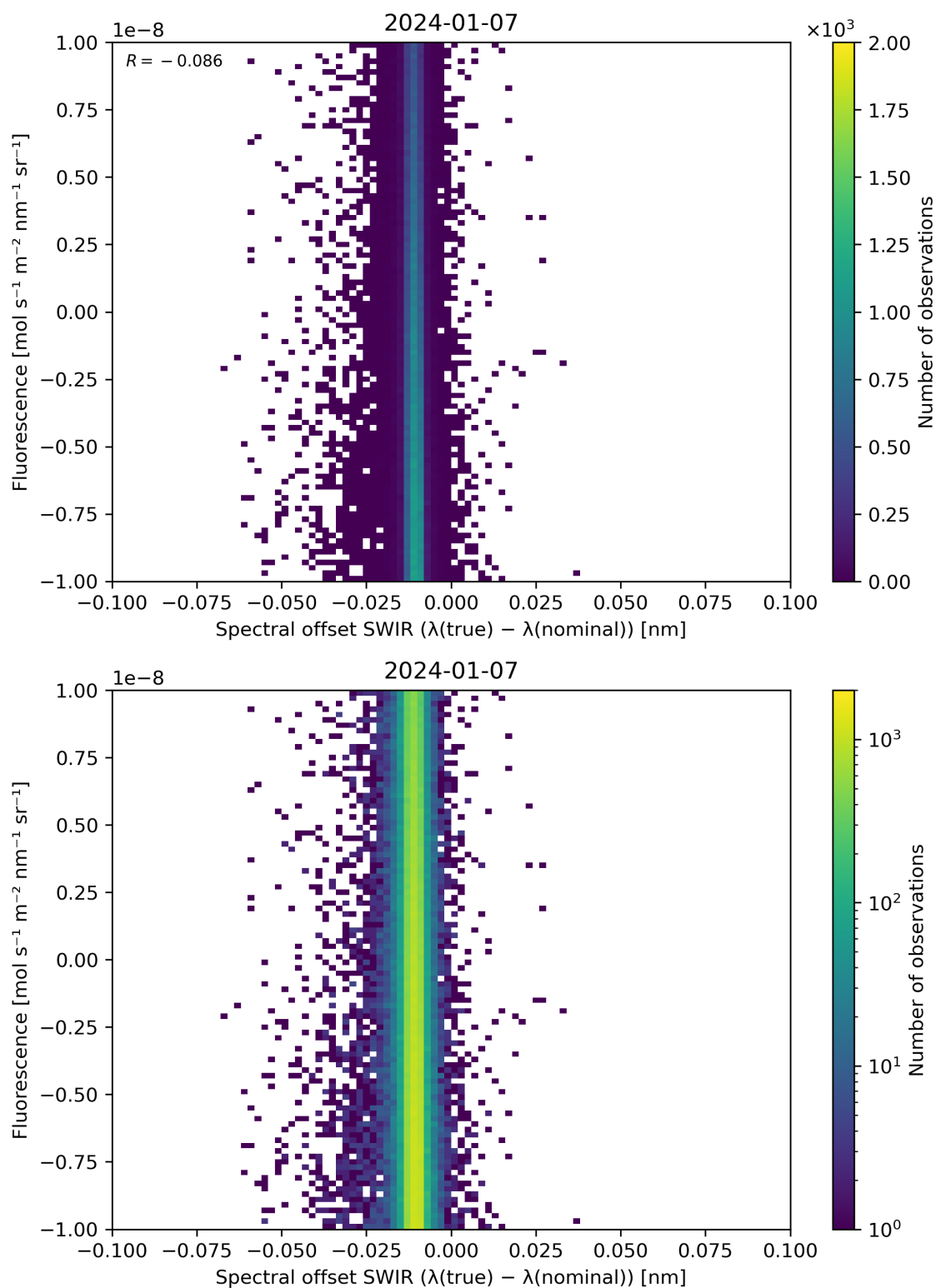
Figure 120: Scatter density plot of “Spectral offset SWIR ( \lambda(\text{true}) - \lambda(\text{nominal}) )” against “Fluorescence” for 2024-01-06 to 2024-01-08.
