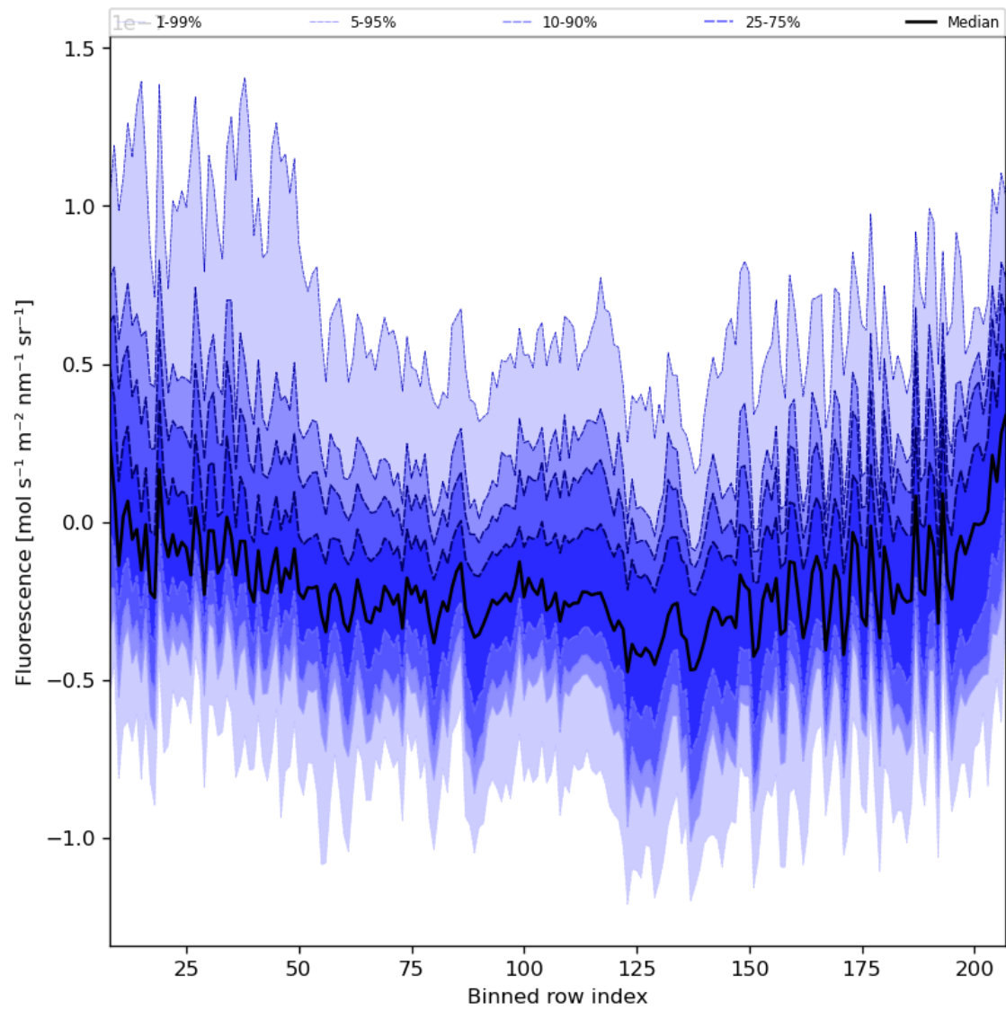
Figure 43: Along track statistics of “Fluorescence” for 2024-01-06 to 2024-01-08
