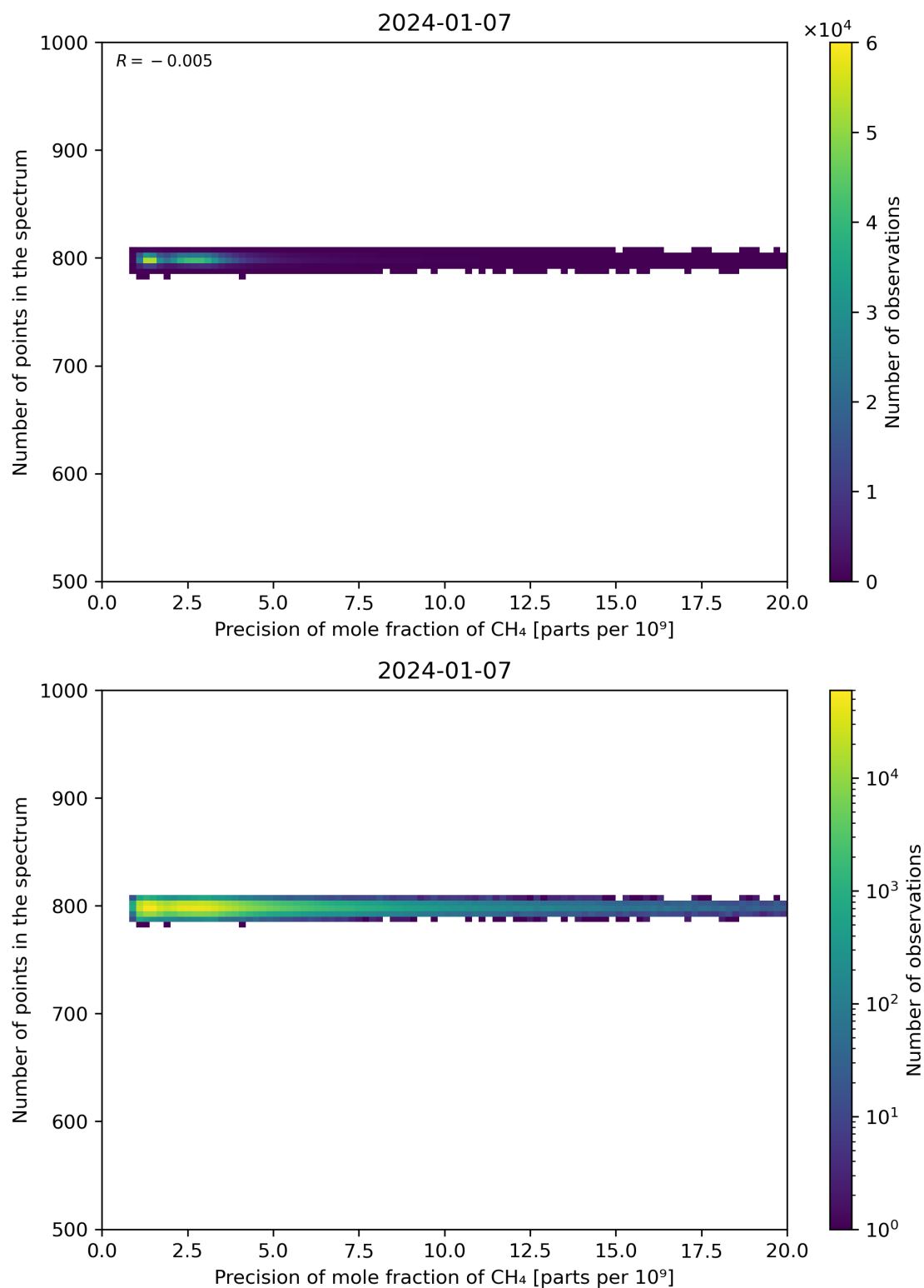
Figure 84: Scatter density plot of “Precision of mole fraction of CH 4 ” against “Number of points in the spectrum” for 2024-01-06 to 2024-01-08.
