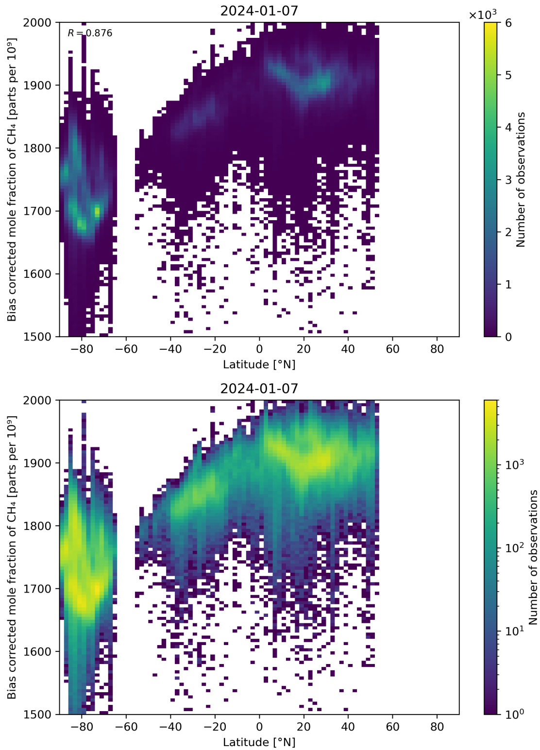
Figure 58: Scatter density plot of “Latitude” against “Bias corrected mole fraction of CH 4 ” for 2024-01-06 to 2024-01-08.
