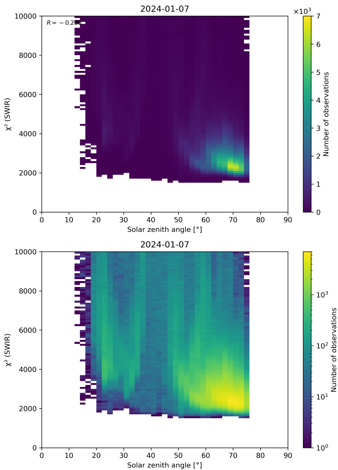
Figure 95: Scatter density plot of “Solar zenith angle” against “ \chi^2 (SWIR)” for 2024-01-06 to 2024-01-08.
