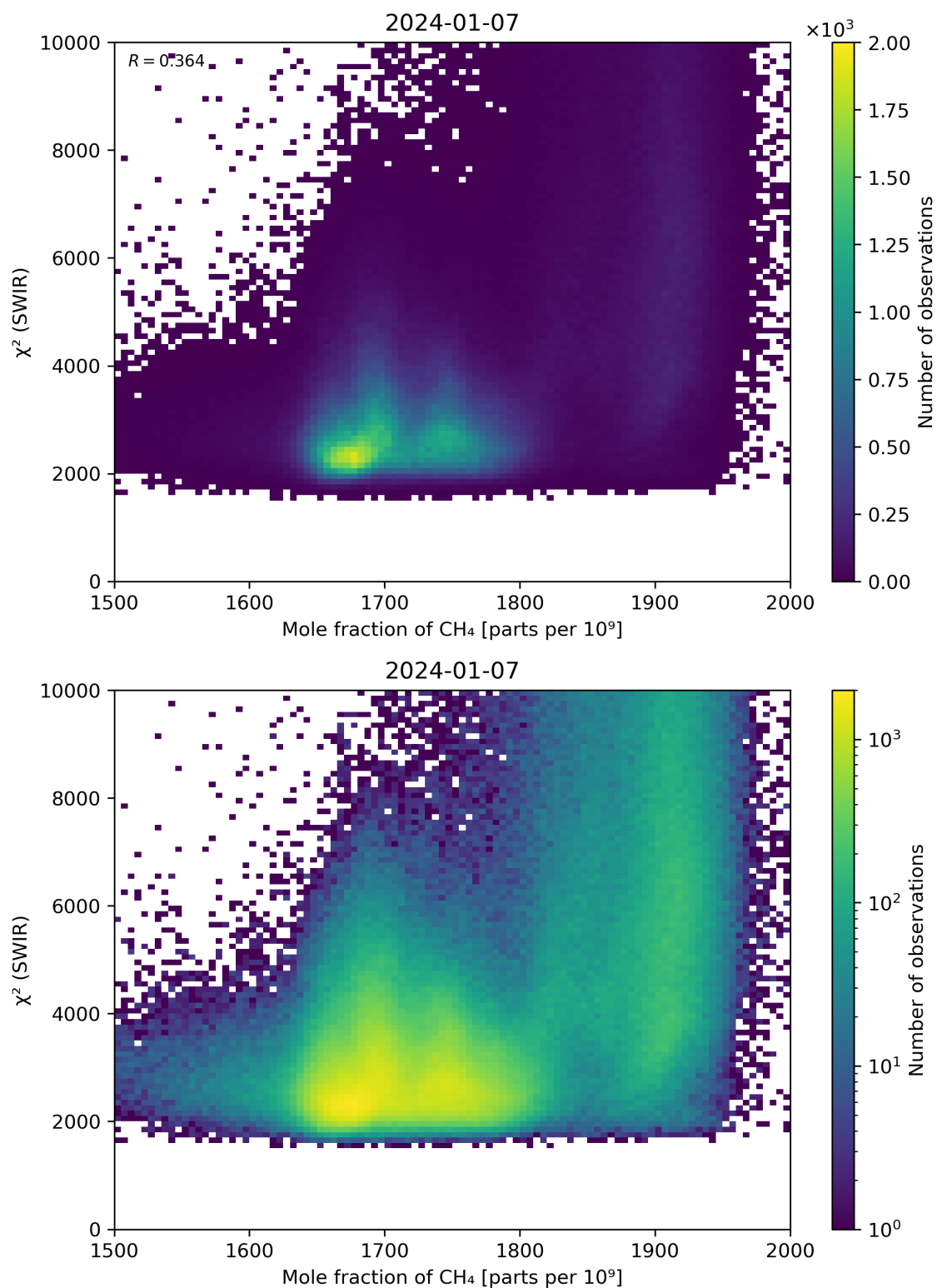
Figure 71: Scatter density plot of “Mole fraction of \text{CH}_4 ” against “ \chi^2 (SWIR)” for 2024-01-06 to 2024-01-08.
