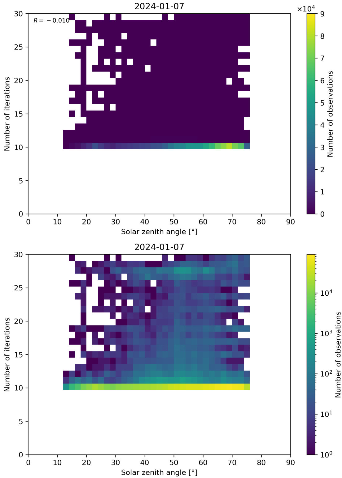
Figure 102: Scatter density plot of “Solar zenith angle” against “Number of iterations” for 2024-01-06 to 2024-01-08.
