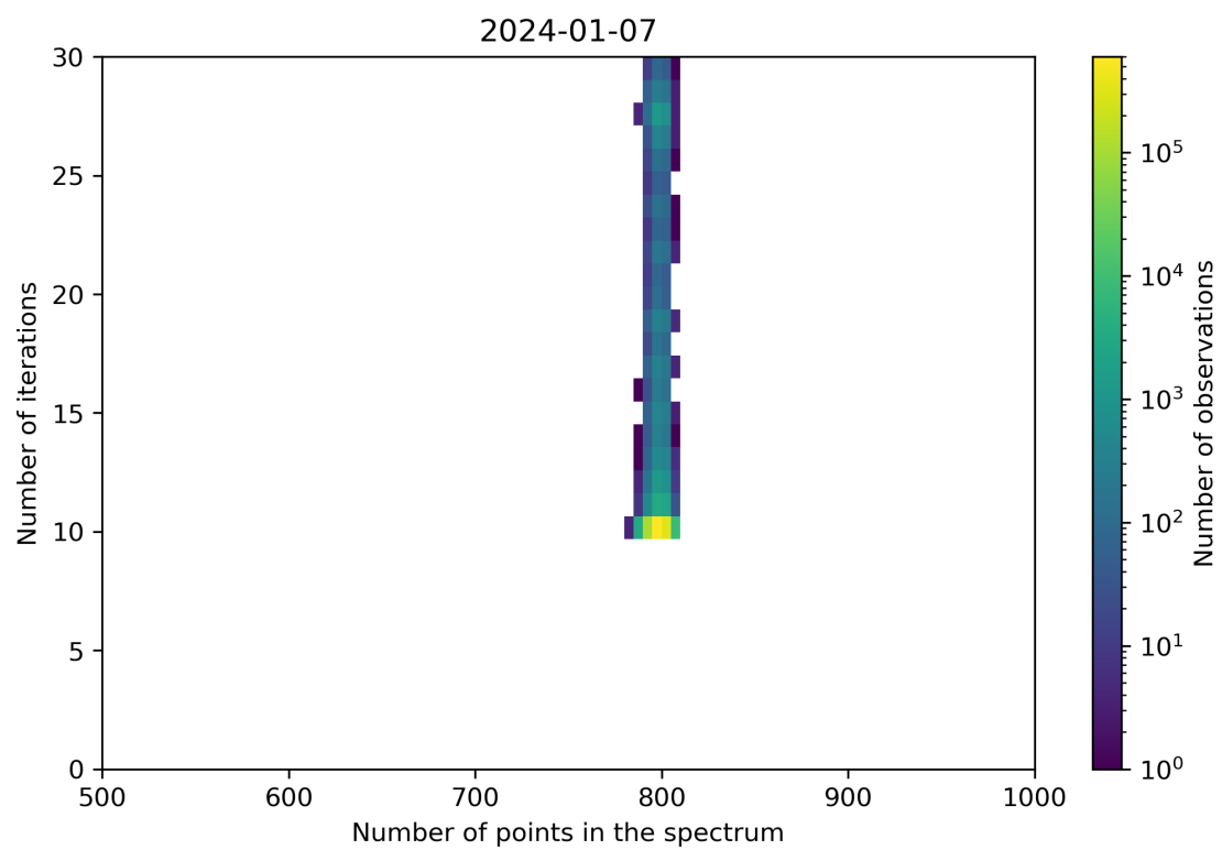
Figure 92: Scatter density plot of “Number of points in the spectrum” against “Number of iterations” for 2024-01-06 to 2024-01-08.
