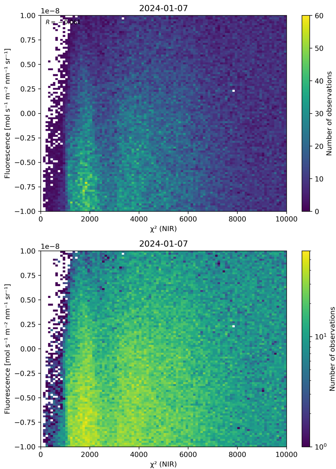
Figure 45: Scatter density plot of “ \chi^2 (NIR)” against “Fluorescence” for 2024-01-06 to 2024-01-08.
