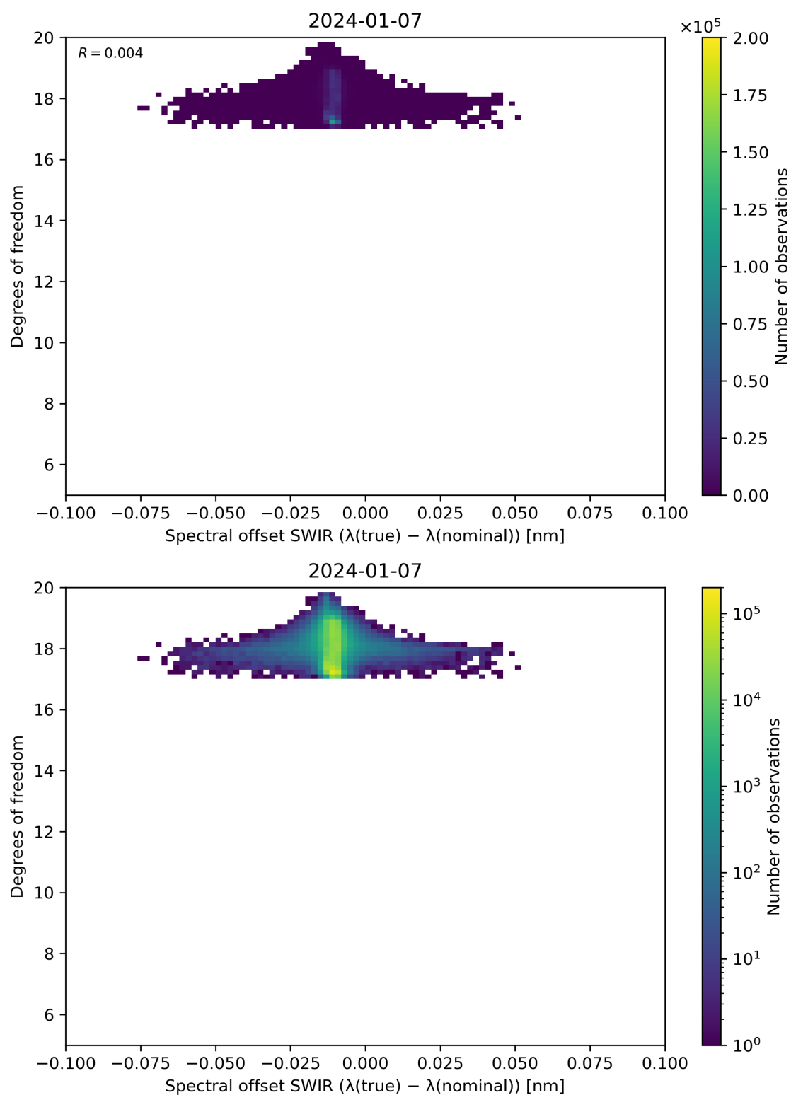
Figure 119: Scatter density plot of “Spectral offset SWIR ( \lambda(\text{true}) - \lambda(\text{nominal}) )” against “Degrees of freedom” for 2024-01-06 to 2024-01-08.
