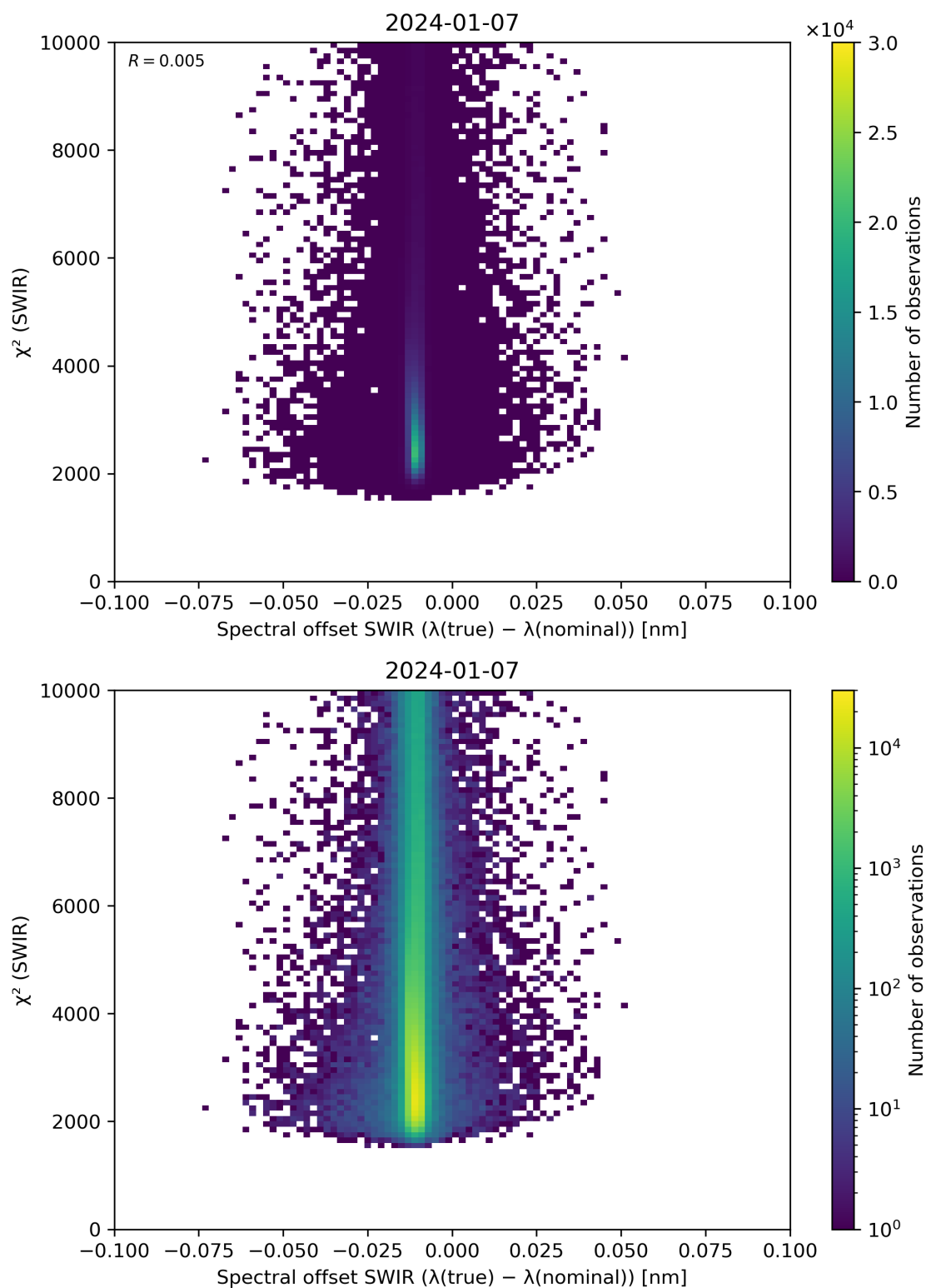
Figure 118: Scatter density plot of “Spectral offset SWIR ( \lambda(\text{true}) - \lambda(\text{nominal}) )” against “ \chi^2 (SWIR)” for 2024-01-06 to 2024-01-08.
