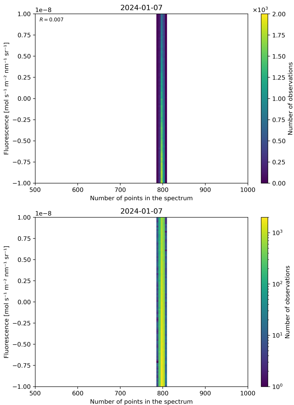
Figure 91: Scatter density plot of “Number of points in the spectrum” against “Fluorescence” for 2024-01-06 to 2024-01-08.
