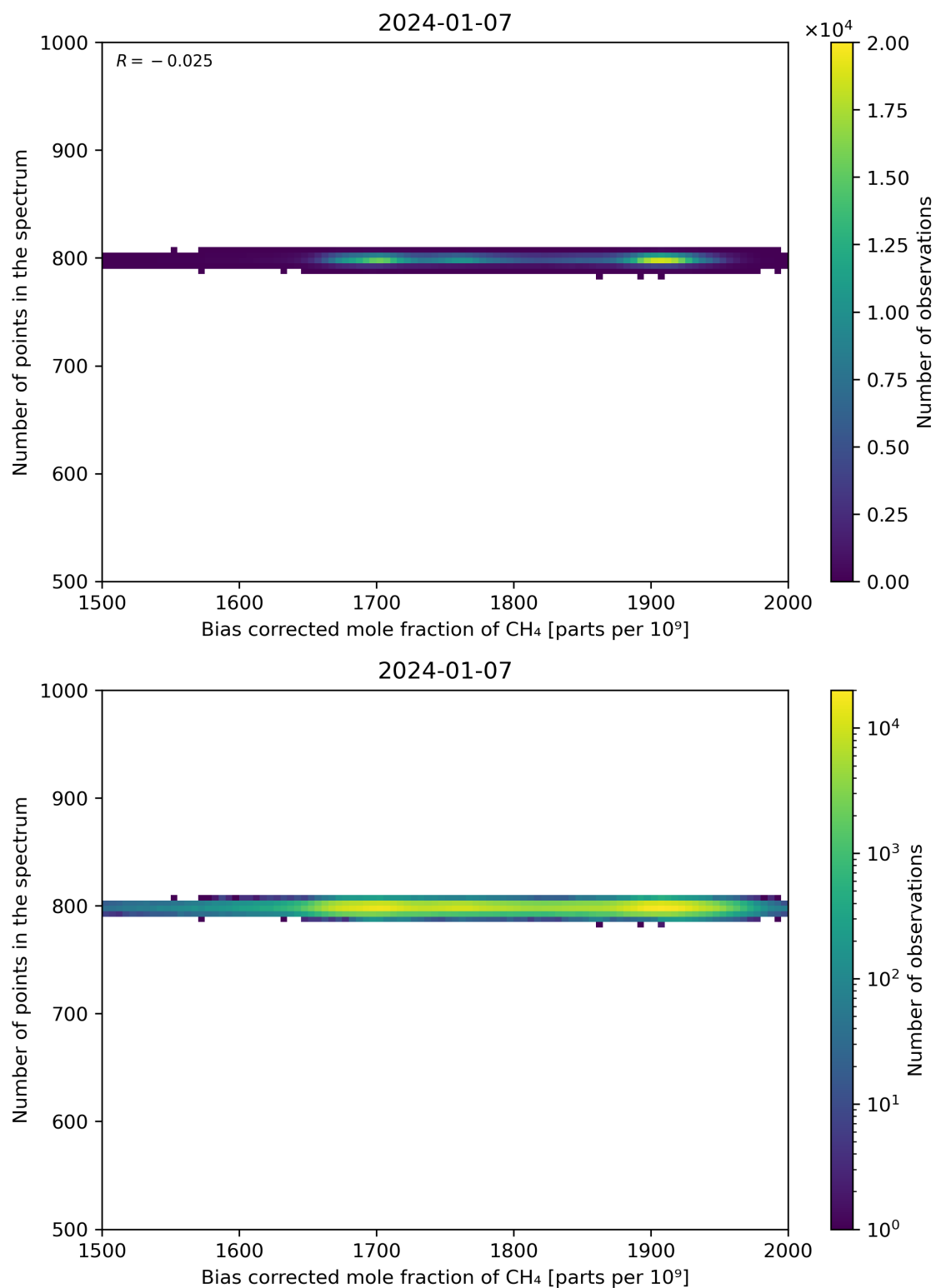
Figure 68: Scatter density plot of “Bias corrected mole fraction of CH 4 ” against “Number of points in the spectrum” for 2024-01-06 to 2024-01-08.
