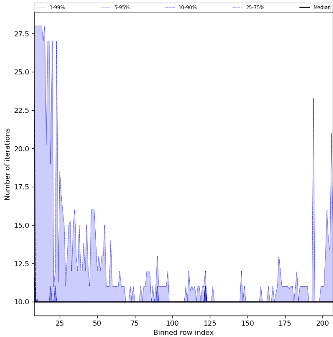
Figure 42: Along track statistics of “Number of iterations” for 2024-01-06 to 2024-01-08
