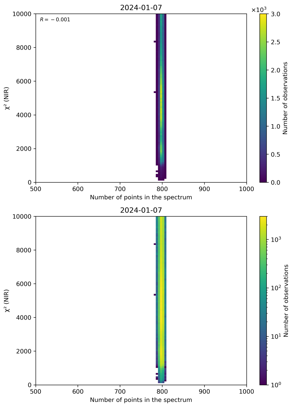
Figure 88: Scatter density plot of “Number of points in the spectrum” against “ \chi^2 (NIR)” for 2024-01-06 to 2024-01-08.
