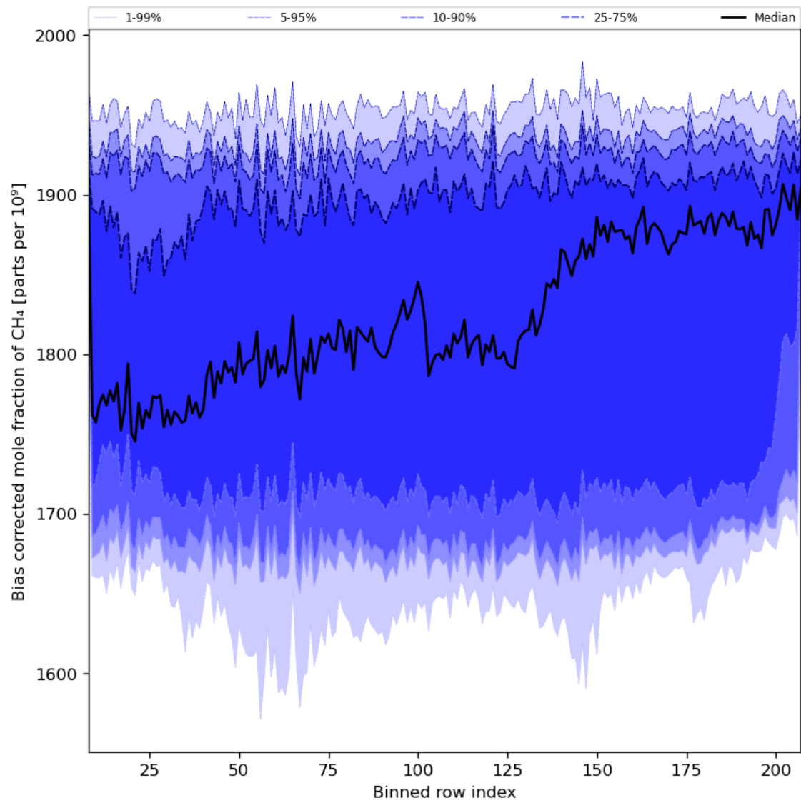
Figure 36: Along track statistics of “Bias corrected mole fraction of CH 4 ” for 2024-01-06 to 2024-01-08
