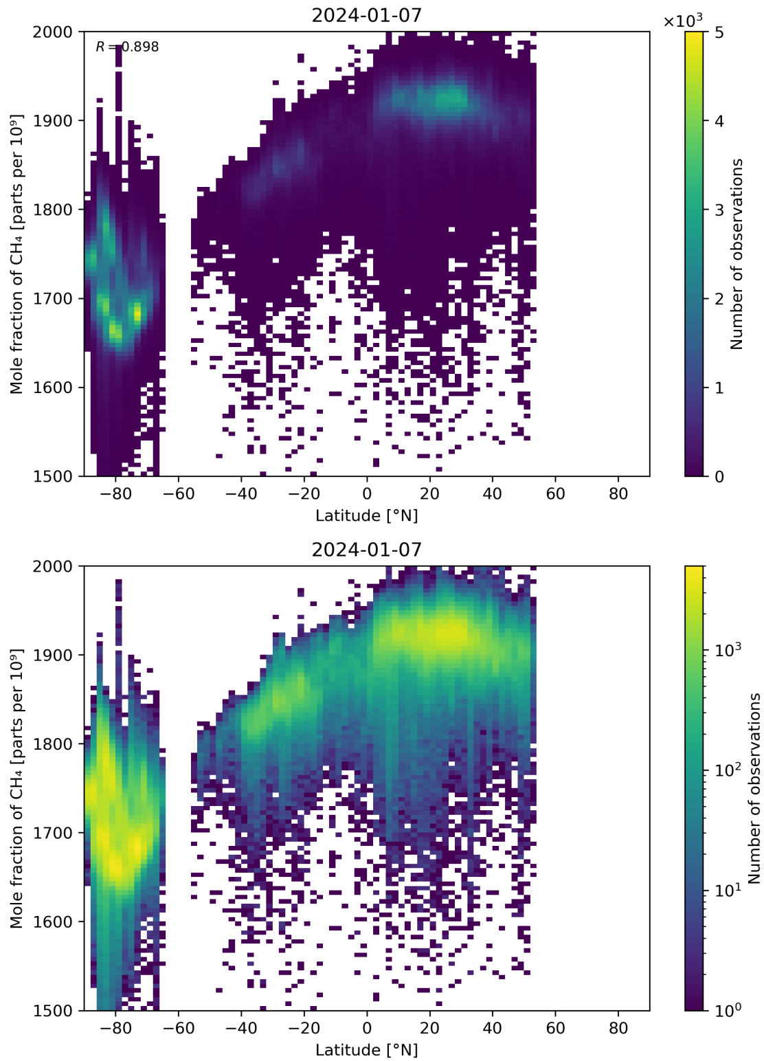
Figure 57: Scatter density plot of “Latitude” against “Mole fraction of CH 4 ” for 2024-01-06 to 2024-01-08.
