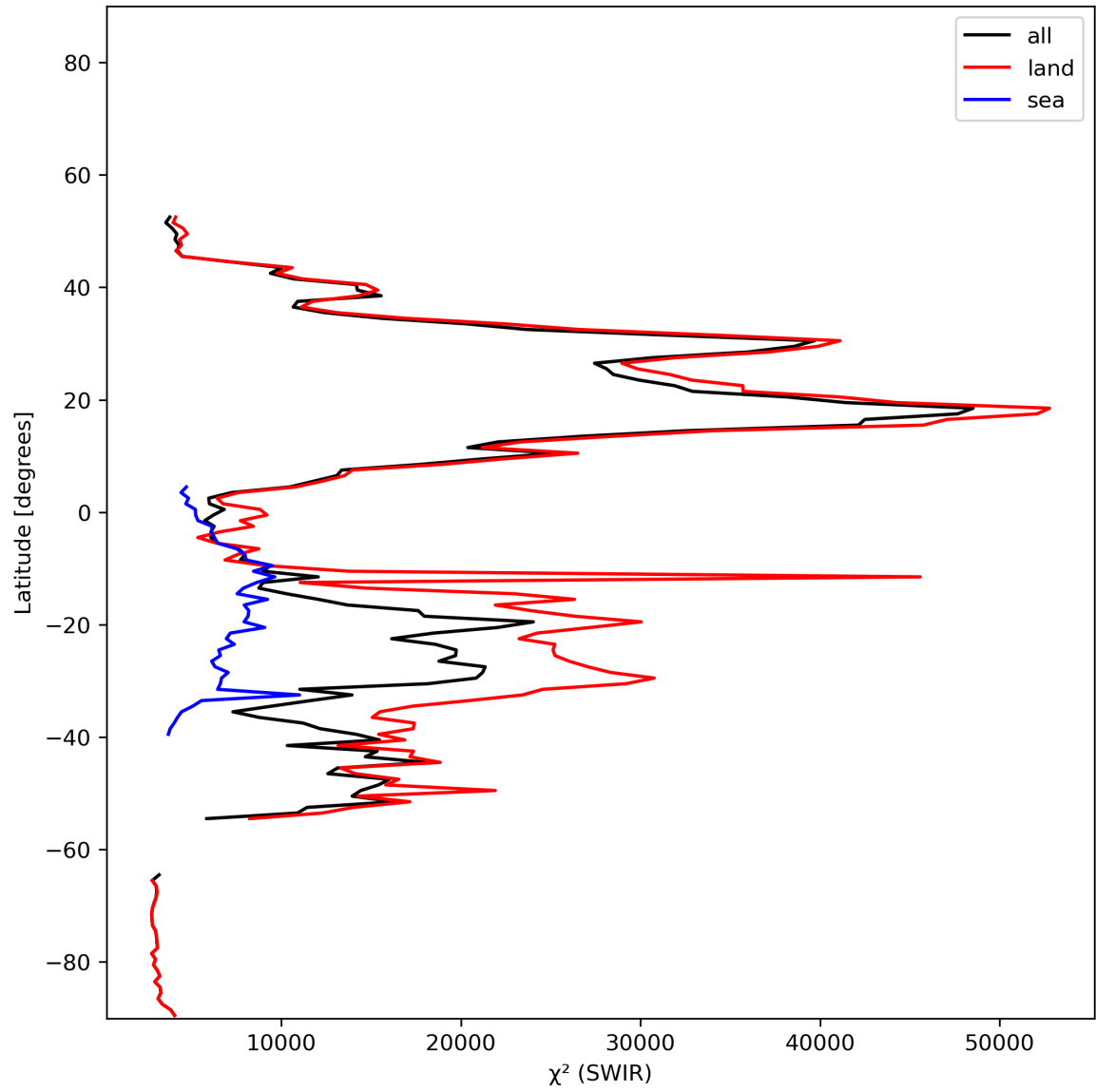
Figure 17: Zonal average of “ \chi^2 (SWIR)” for 2024-01-06 to 2024-01-08.
