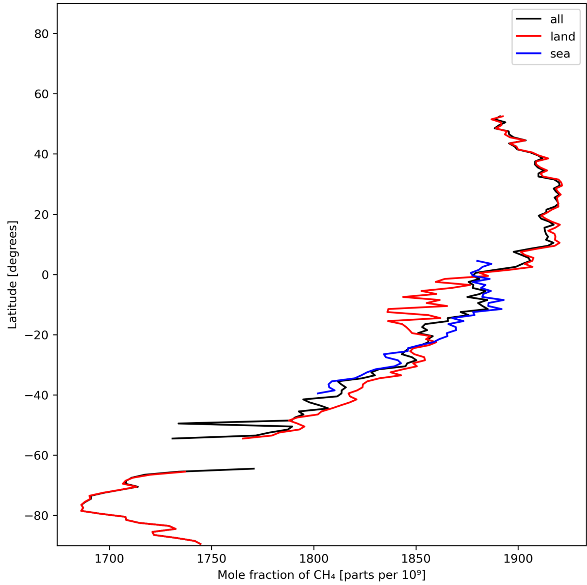
Figure 12: Zonal average of “Mole fraction of \text{CH}_4 ” for 2024-01-06 to 2024-01-08.
