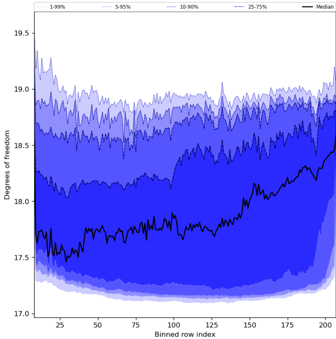
Figure 41: Along track statistics of “Degrees of freedom” for 2024-01-06 to 2024-01-08
