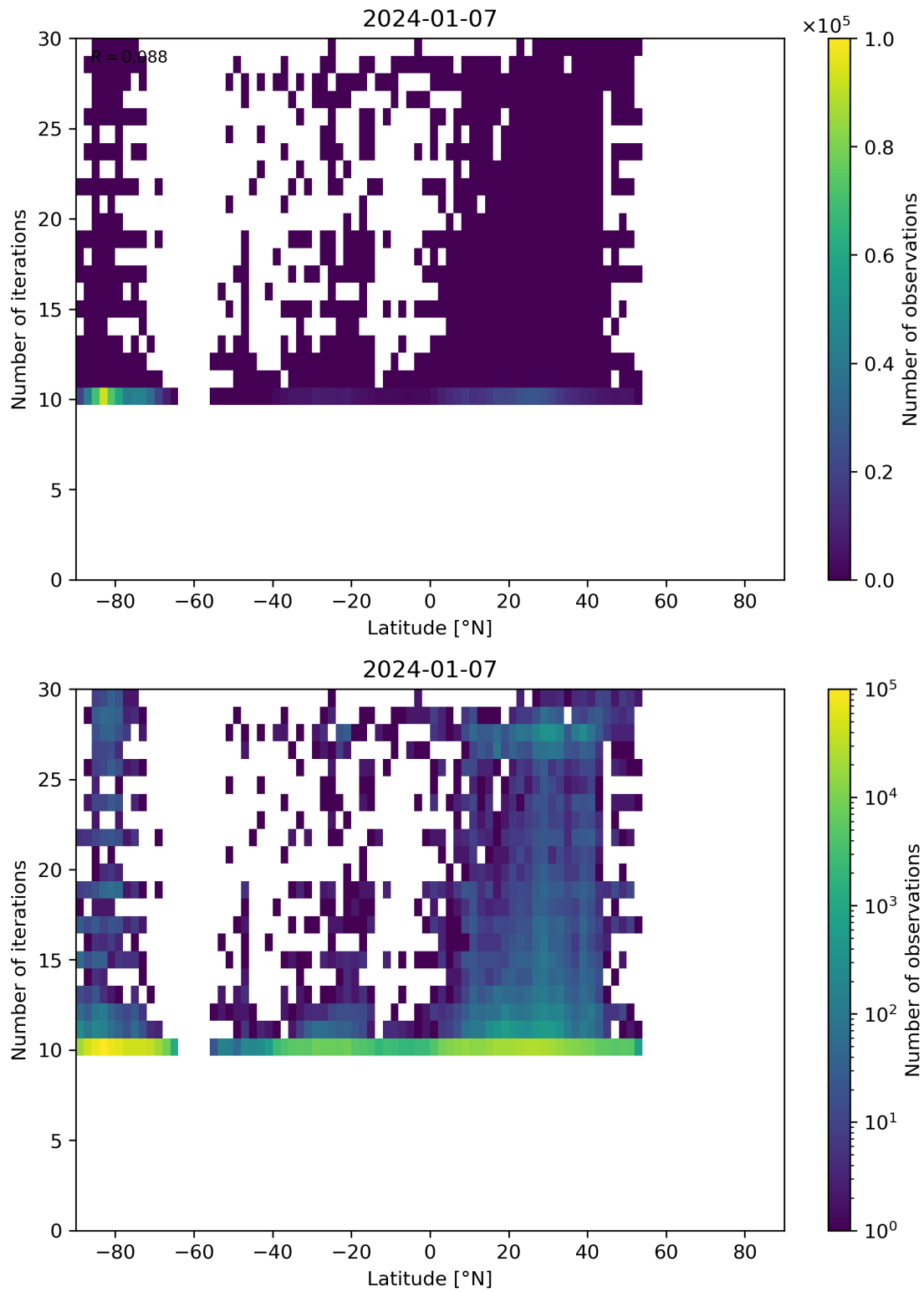
Figure 60: Scatter density plot of “Latitude” against “Number of iterations” for 2024-01-06 to 2024-01-08.
