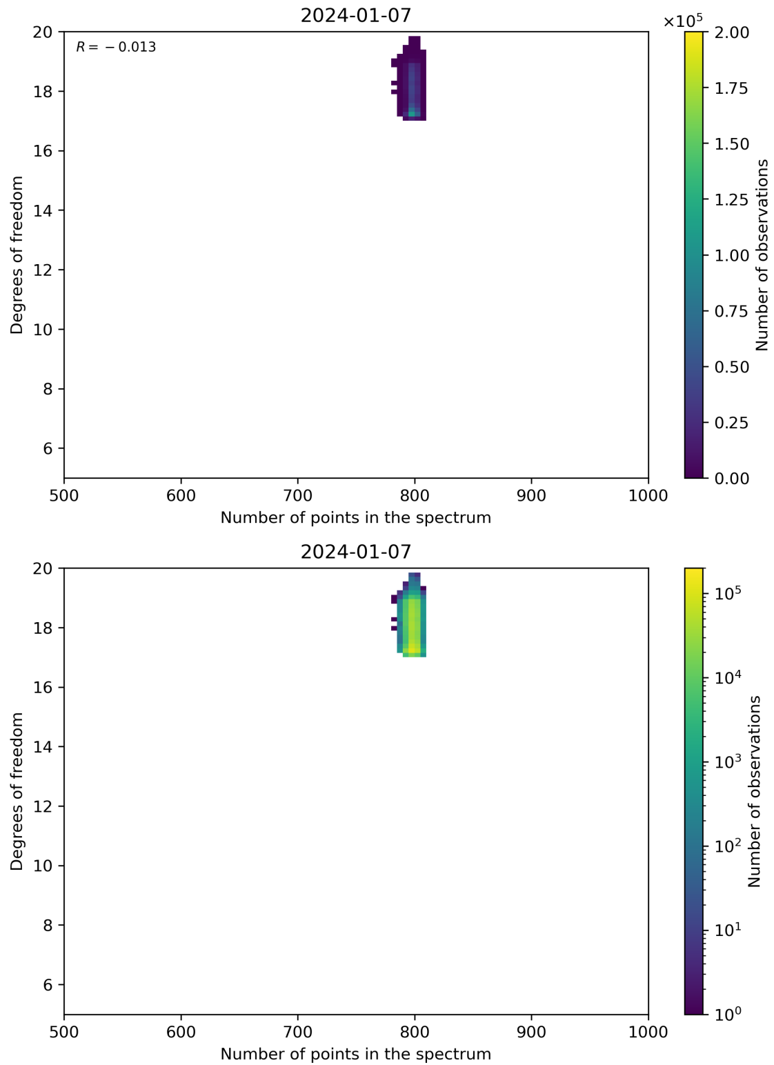
Figure 90: Scatter density plot of “Number of points in the spectrum” against “Degrees of freedom” for 2024-01-06 to 2024-01-08.
