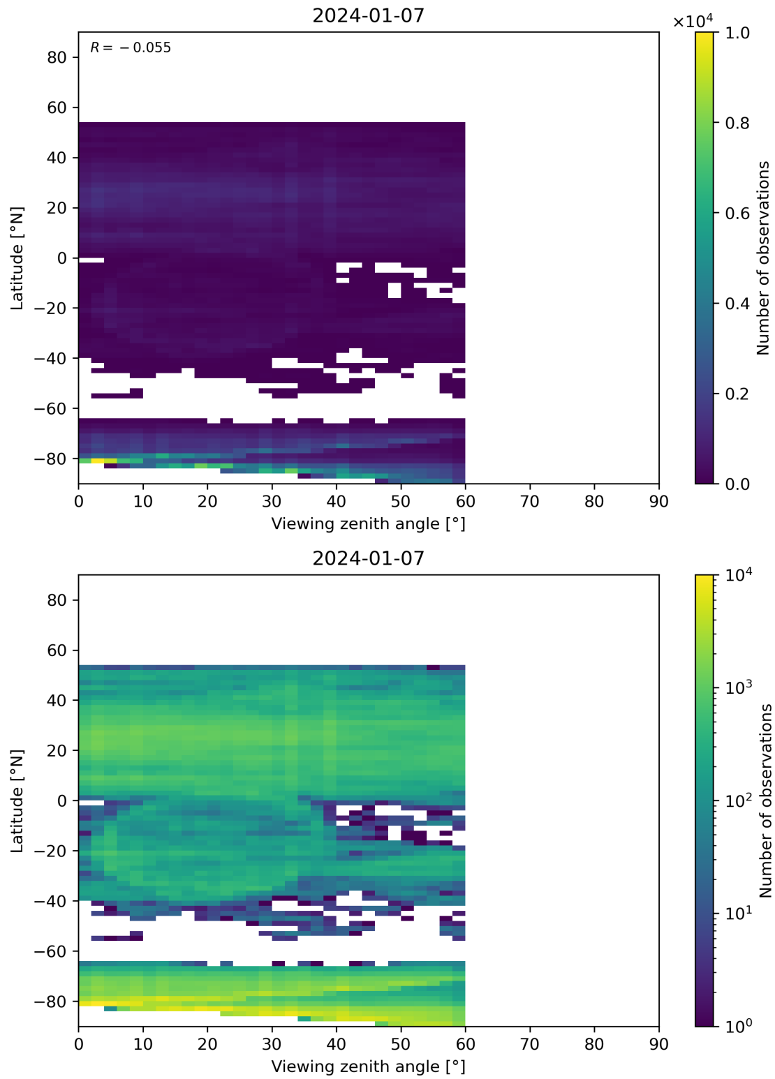
Figure 109: Scatter density plot of “Viewing zenith angle” against “Latitude” for 2024-01-06 to 2024-01-08.
