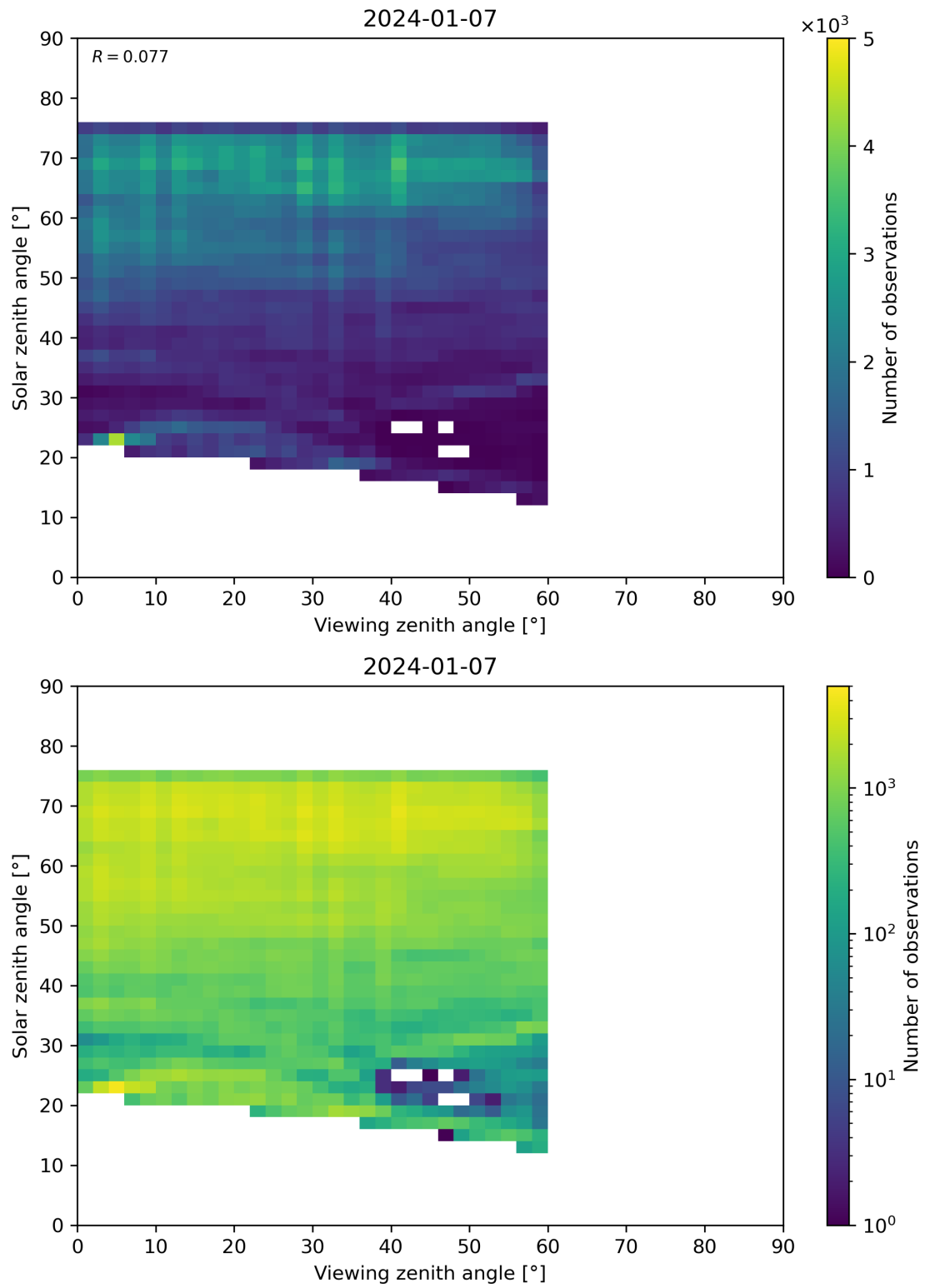
Figure 115: Scatter density plot of “Viewing zenith angle” against “Solar zenith angle” for 2024-01-06 to 2024-01-08.
