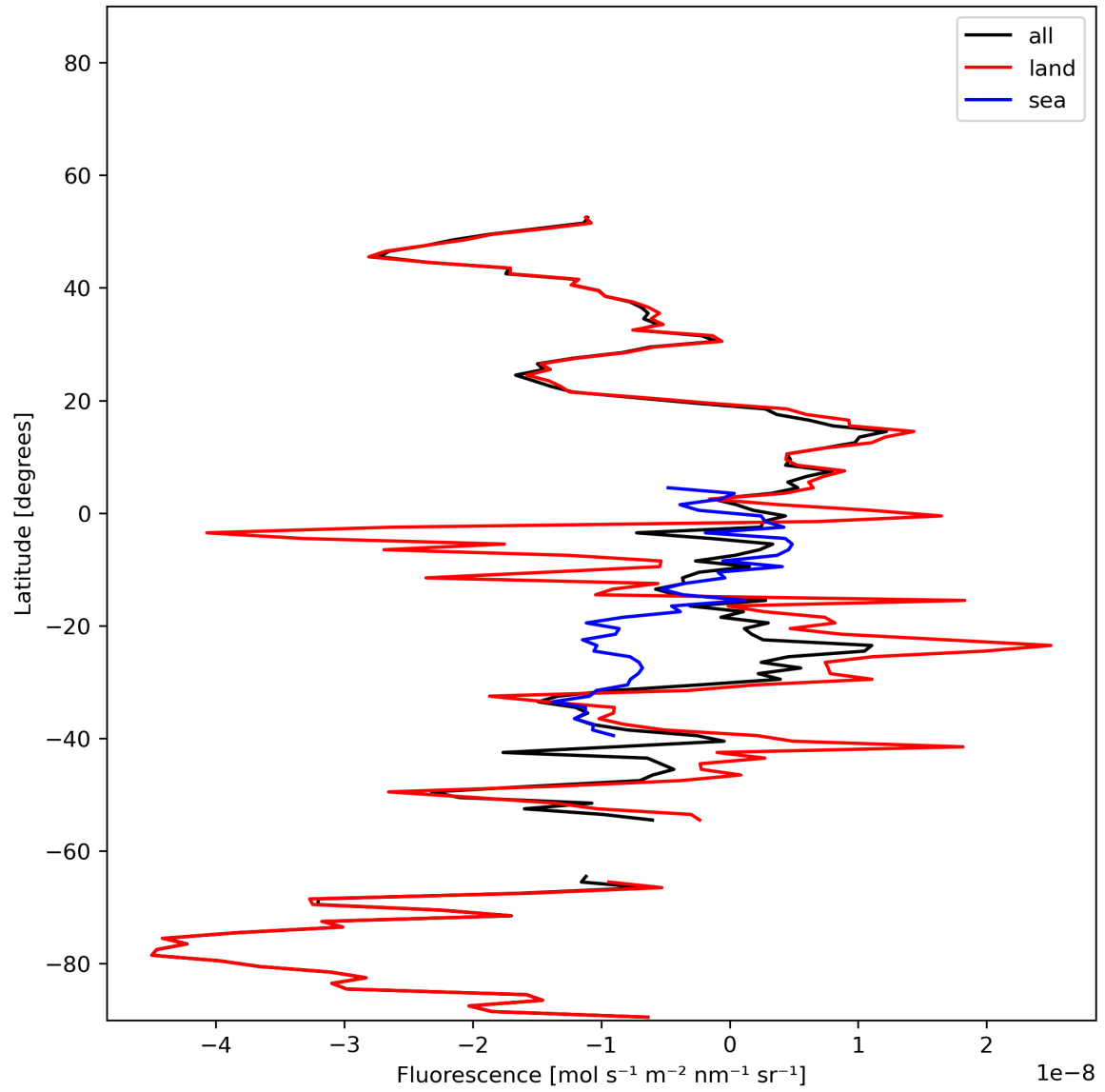
Figure 21: Zonal average of “Fluorescence” for 2024-01-06 to 2024-01-08.
