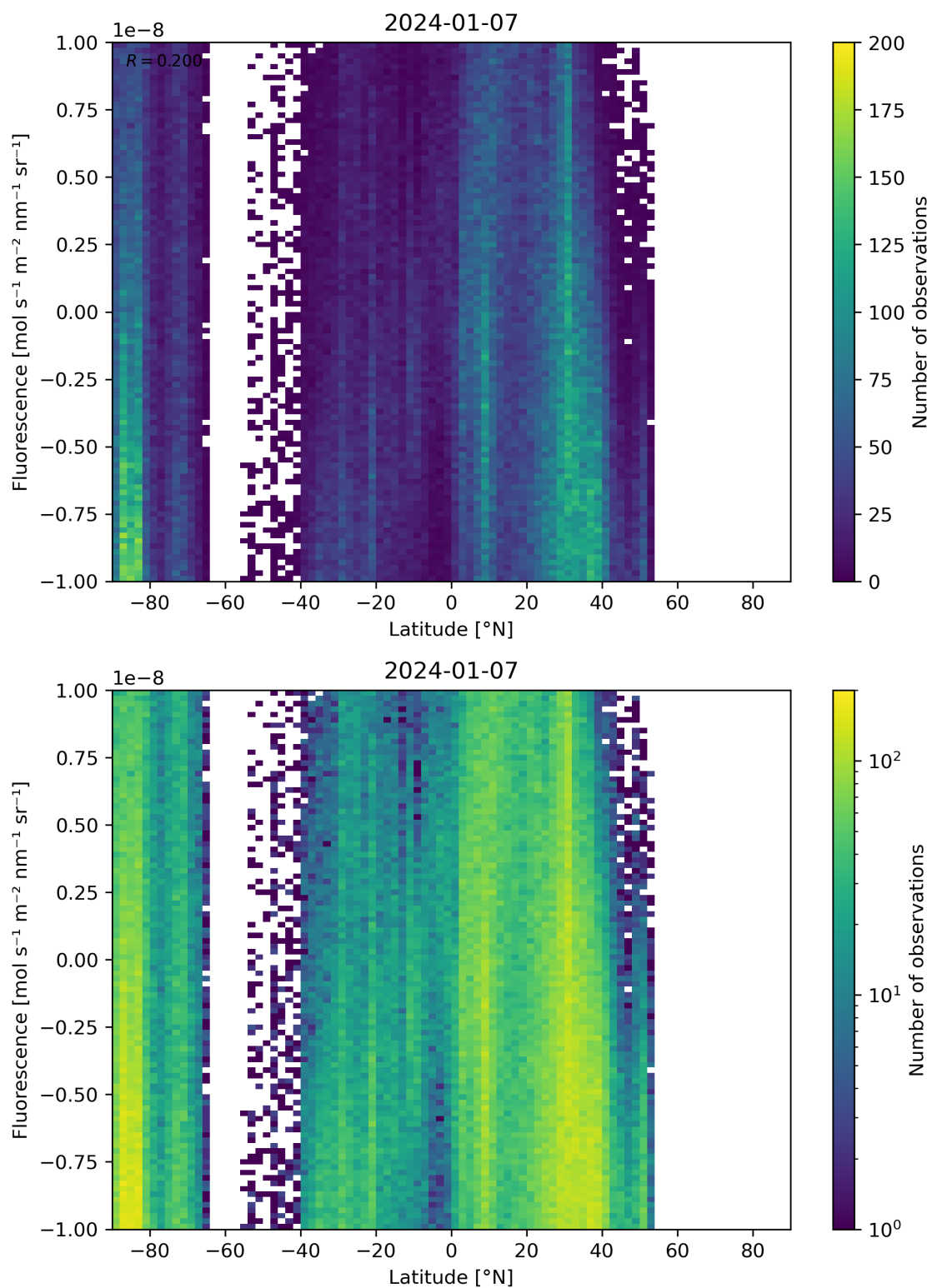
Figure 56: Scatter density plot of “Latitude” against “Fluorescence” for 2024-01-06 to 2024-01-08.
