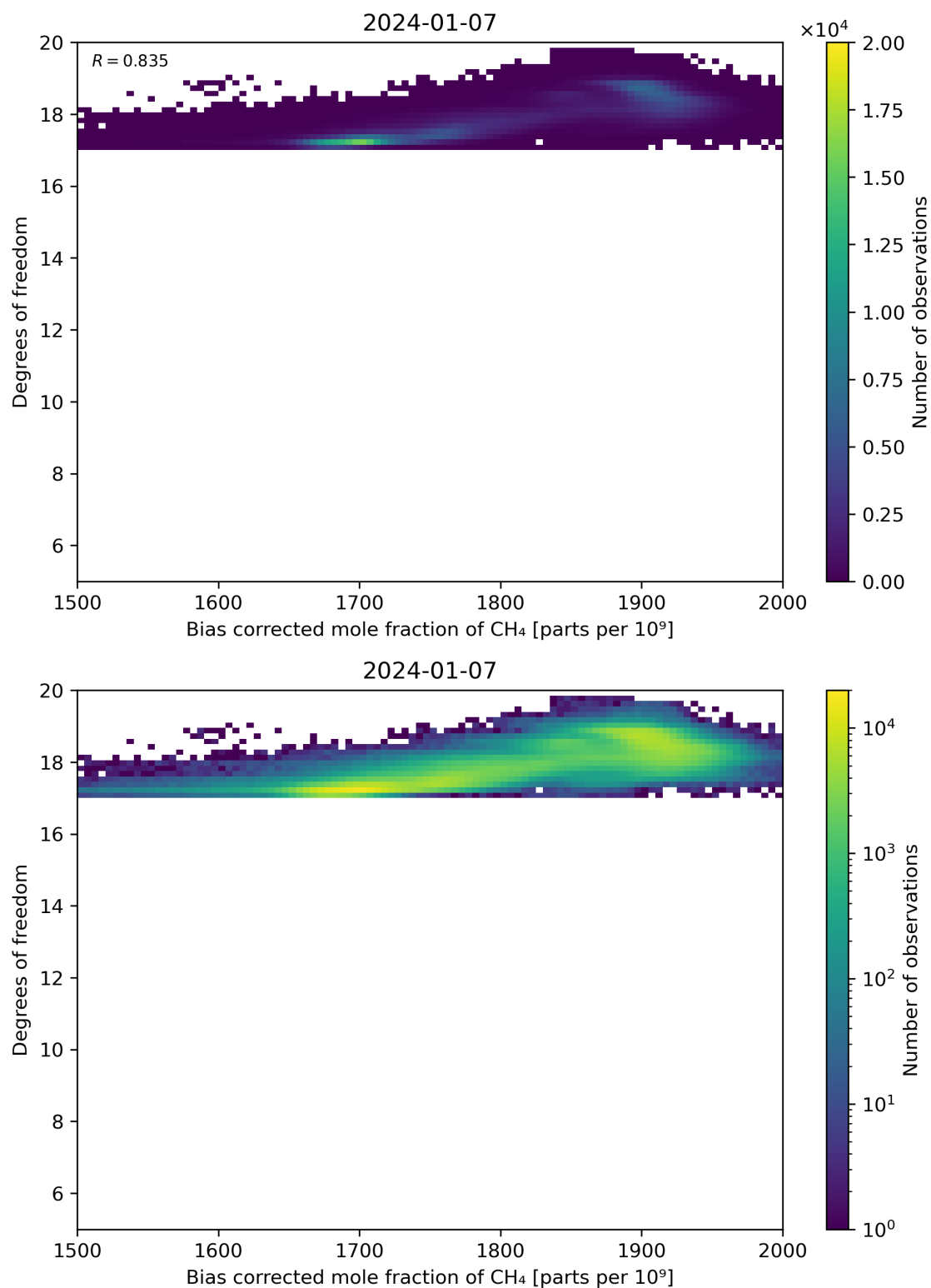
Figure 65: Scatter density plot of “Bias corrected mole fraction of CH 4 ” against “Degrees of freedom” for 2024-01-06 to 2024-01-08.
