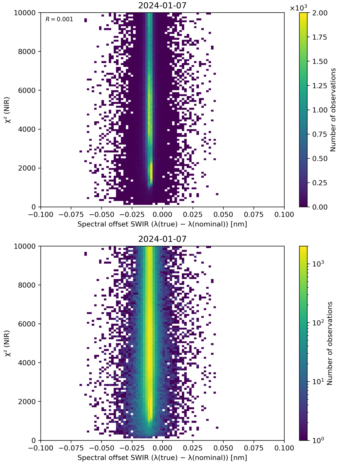
Figure 117: Scatter density plot of “Spectral offset SWIR ( \lambda(\text{true}) - \lambda(\text{nominal}) )” against “ \chi^2 (NIR)” for 2024-01-06 to 2024-01-08.
