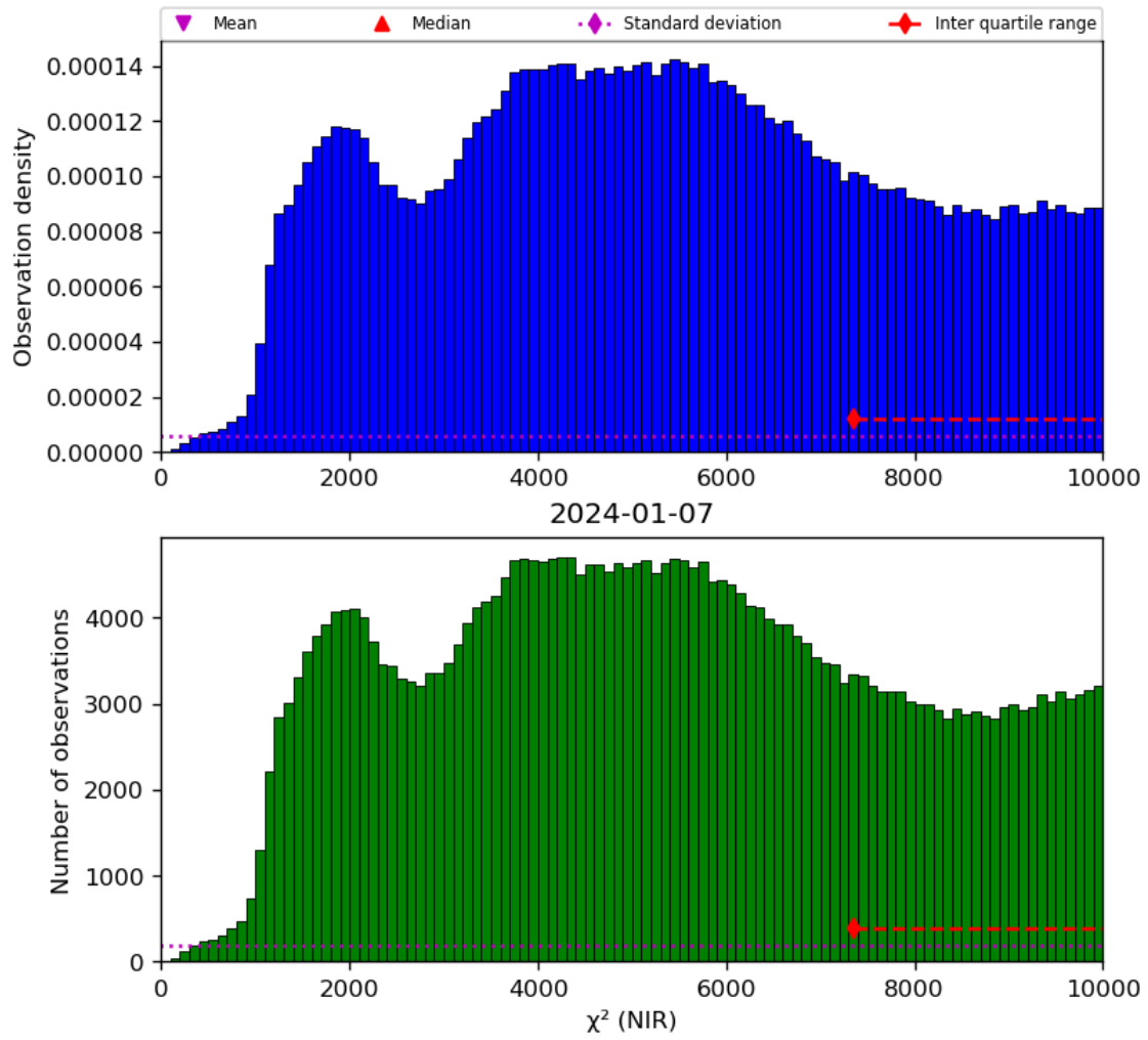
Figure 29: Histogram of “ \chi^2 (NIR)” for 2024-01-06 to 2024-01-08
