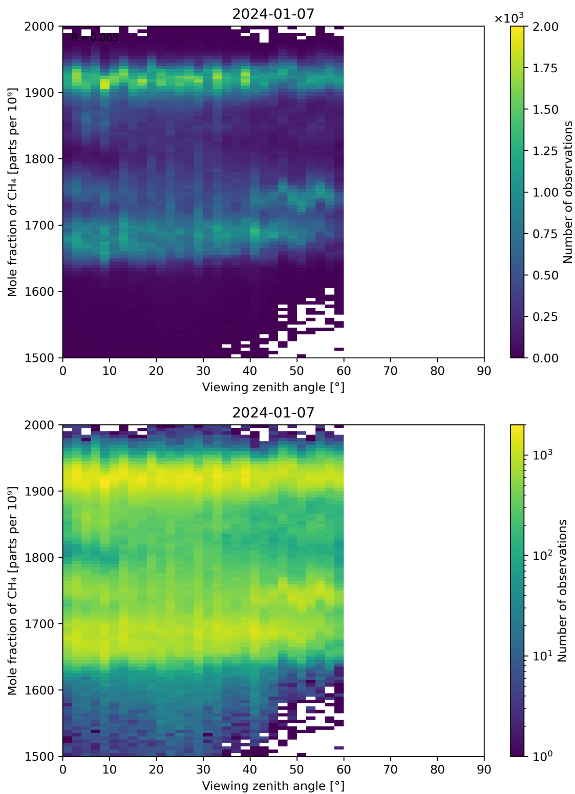
Figure 110: Scatter density plot of “Viewing zenith angle” against “Mole fraction of CH 4 ” for 2024-01-06 to 2024-01-08.
