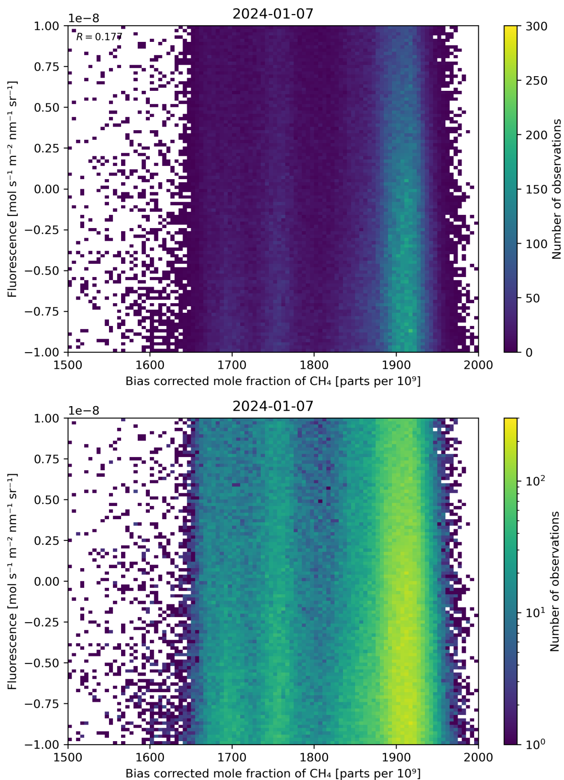
Figure 66: Scatter density plot of “Bias corrected mole fraction of \text{CH}_4 ” against “Fluorescence” for 2024-01-06 to 2024-01-08.
