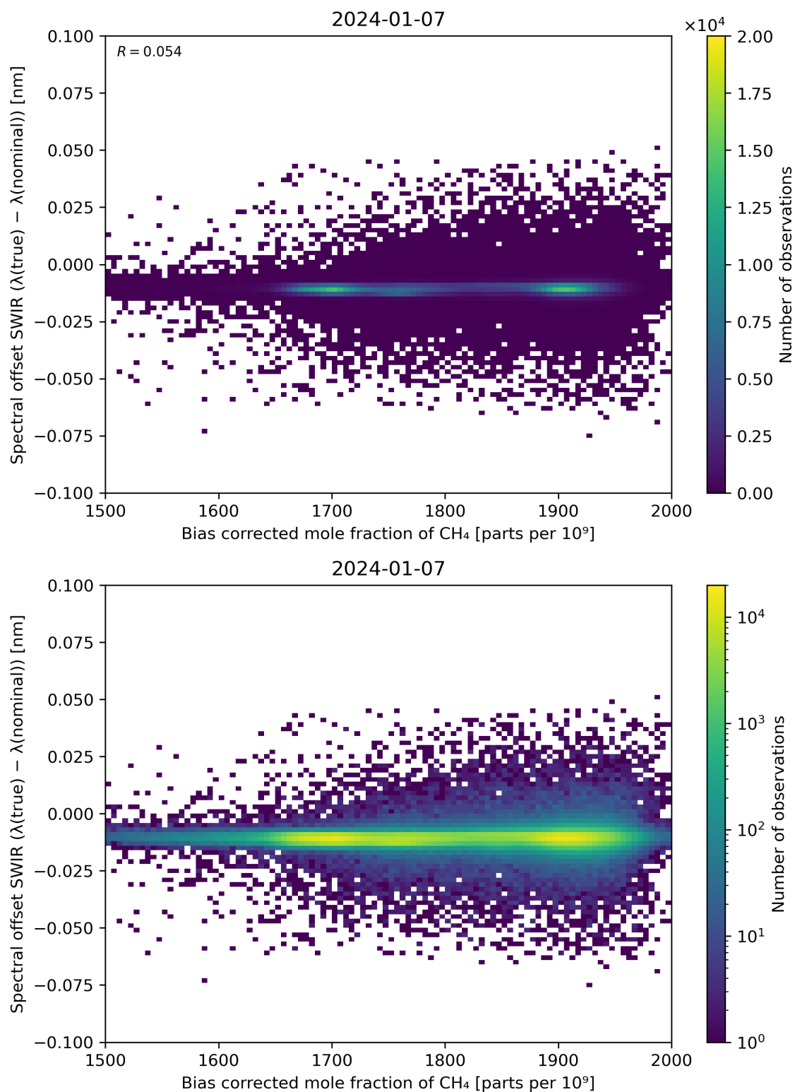
Figure 69: Scatter density plot of “Bias corrected mole fraction of \text{CH}_4 ” against “Spectral offset SWIR ( \lambda(\text{true}) - \lambda(\text{nominal}) )” for 2024-01-06 to 2024-01-08.
