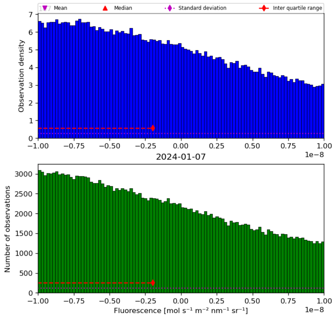
Figure 32: Histogram of “Fluorescence” for 2024-01-06 to 2024-01-08
