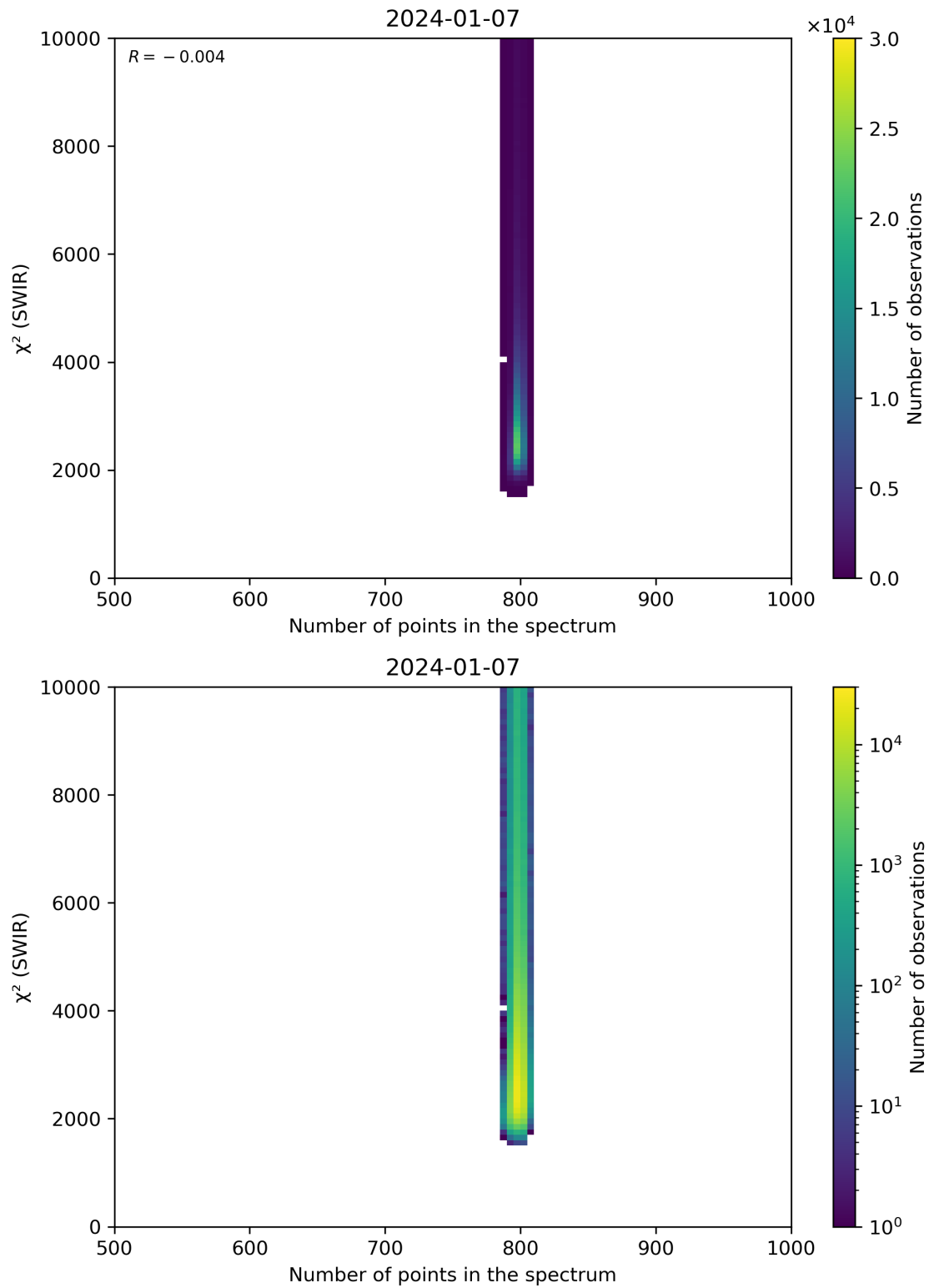
Figure 89: Scatter density plot of “Number of points in the spectrum” against “ \chi^2 (SWIR)” for 2024-01-06 to 2024-01-08.
