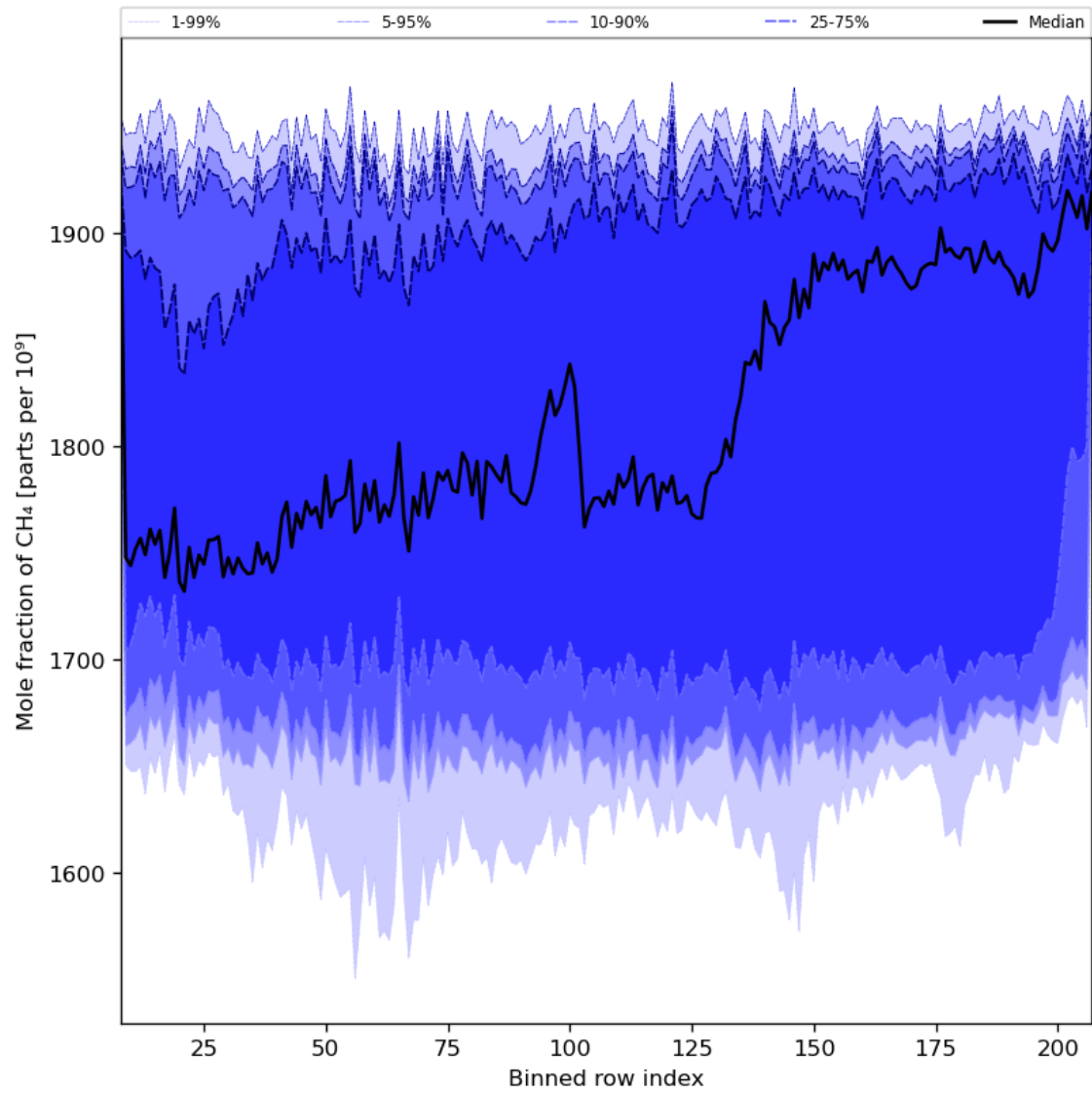
Figure 34: Along track statistics of “Mole fraction of CH 4 ” for 2024-01-06 to 2024-01-08
