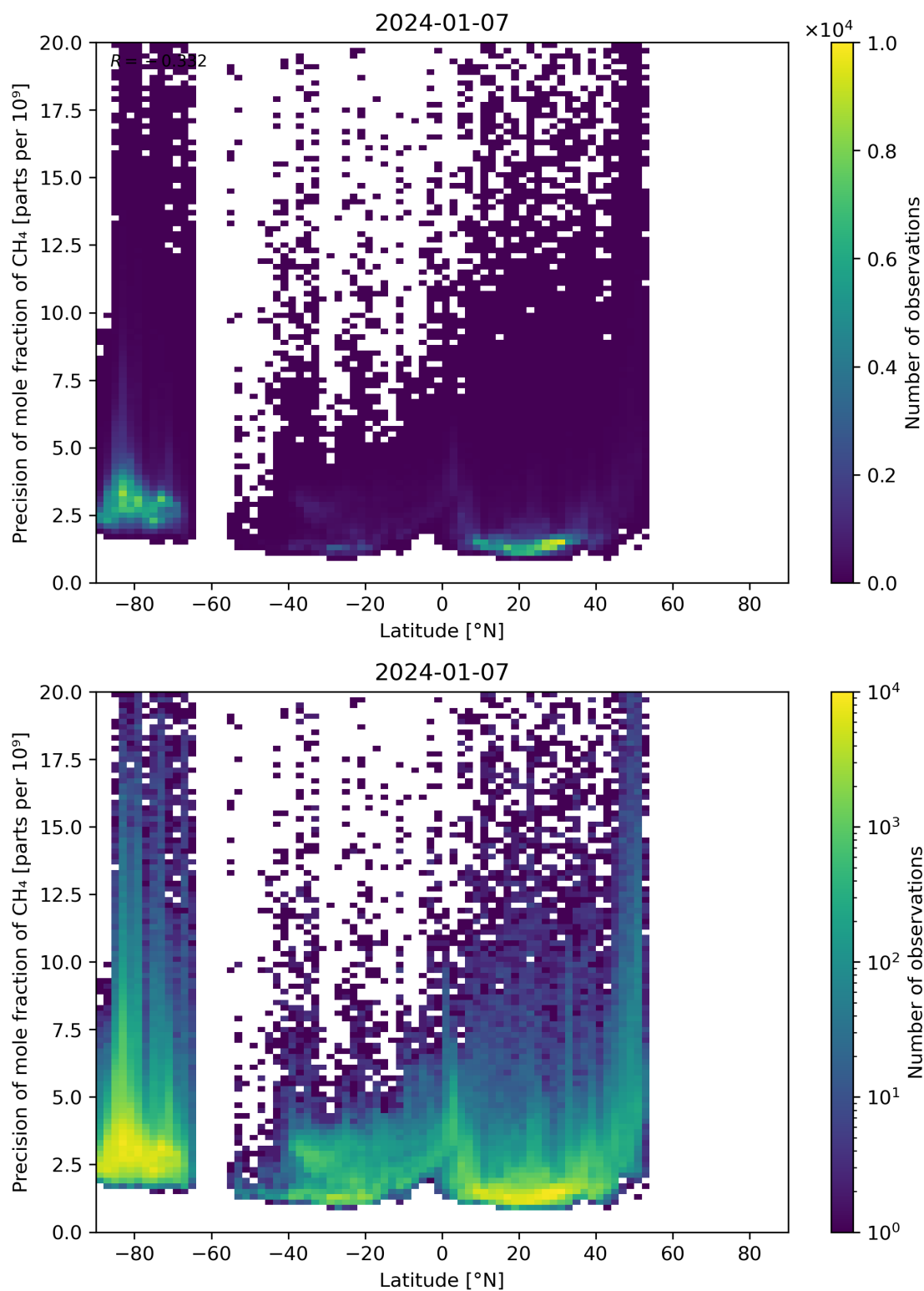
Figure 59: Scatter density plot of “Latitude” against “Precision of mole fraction of CH 4 ” for 2024-01-06 to 2024-01-08.
