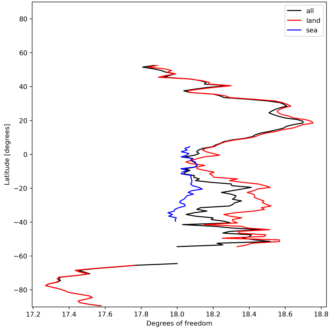
Figure 19: Zonal average of “Degrees of freedom” for 2024-01-06 to 2024-01-08.
