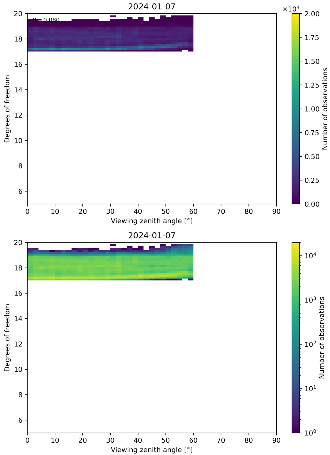
Figure 107: Scatter density plot of “Viewing zenith angle” against “Degrees of freedom” for 2024-01-06 to 2024-01-08.
