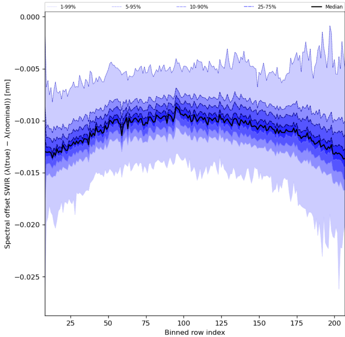
Figure 38: Along track statistics of “Spectral offset SWIR ( \lambda(\text{true}) - \lambda(\text{nominal}) )” for 2024-01-06 to 2024-01-08
