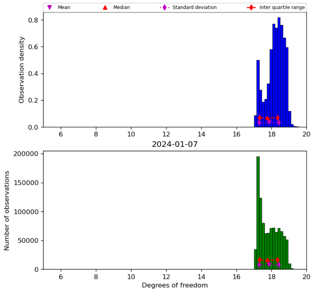
Figure 30: Histogram of “Degrees of freedom” for 2024-01-06 to 2024-01-08
