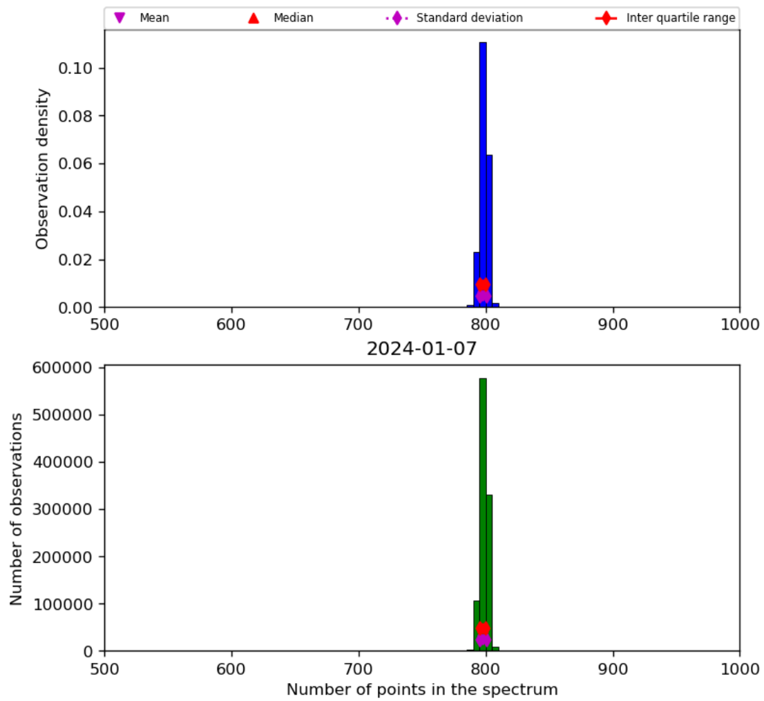
Figure 26: Histogram of “Number of points in the spectrum” for 2024-01-06 to 2024-01-08
