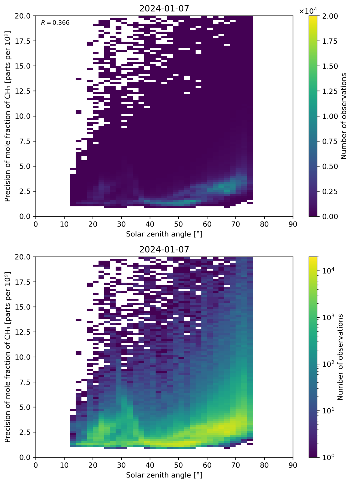
Figure 101: Scatter density plot of “Solar zenith angle” against “Precision of mole fraction of CH 4 ” for 2024-01-06 to 2024-01-08.
