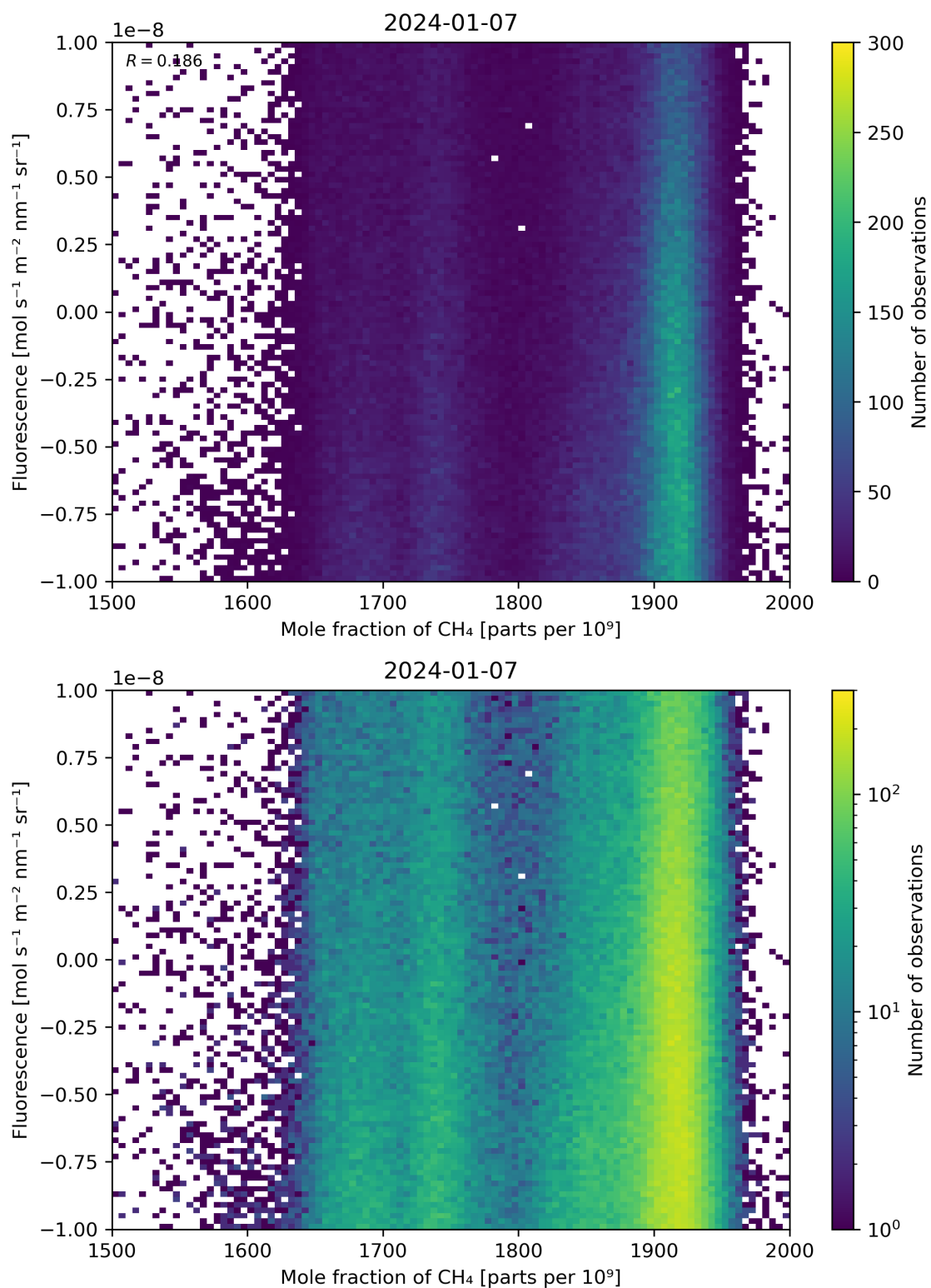
Figure 73: Scatter density plot of “Mole fraction of \text{CH}_4 ” against “Fluorescence” for 2024-01-06 to 2024-01-08.
