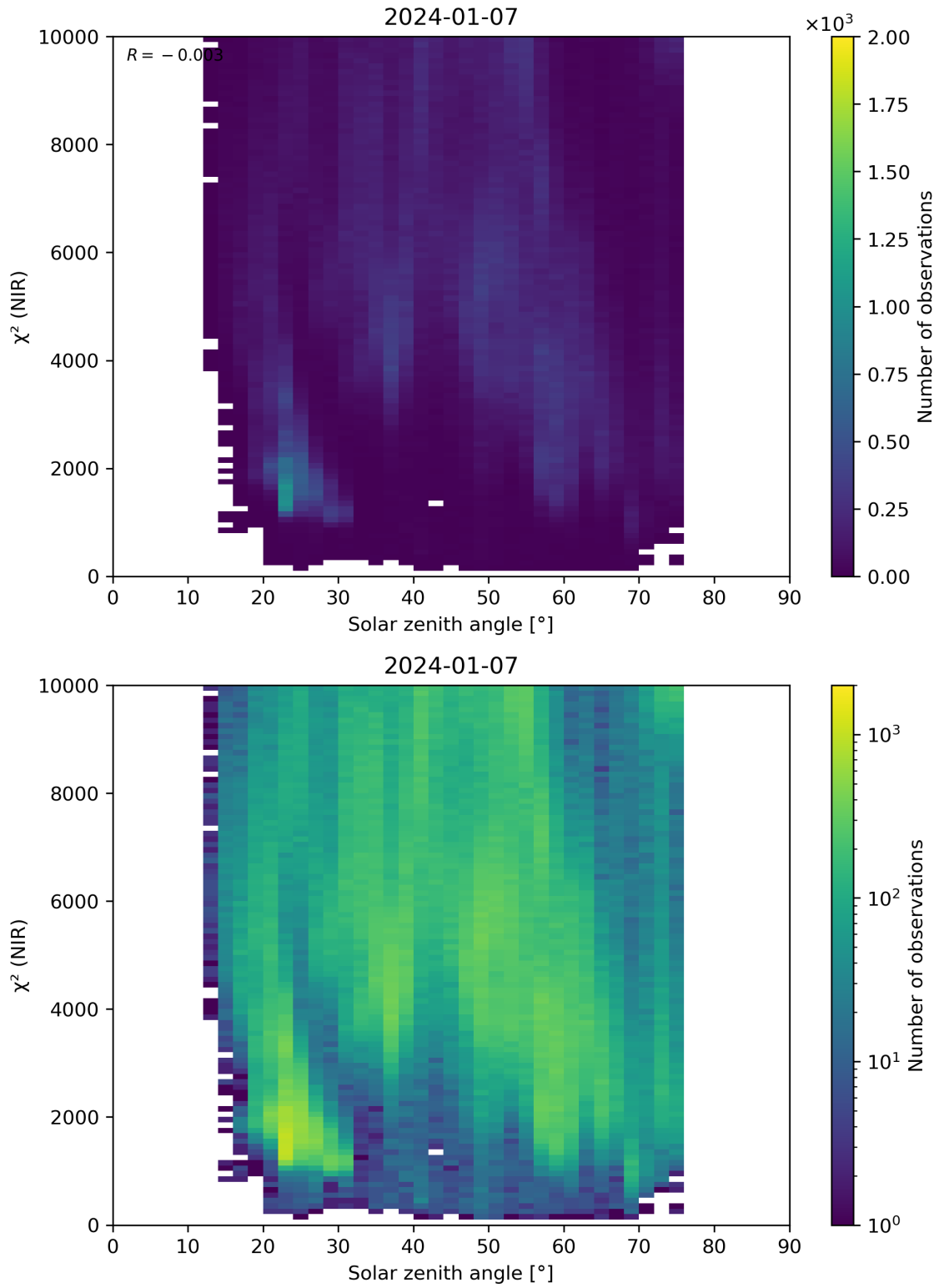
Figure 94: Scatter density plot of “Solar zenith angle” against “ \chi^2 (NIR)” for 2024-01-06 to 2024-01-08.
