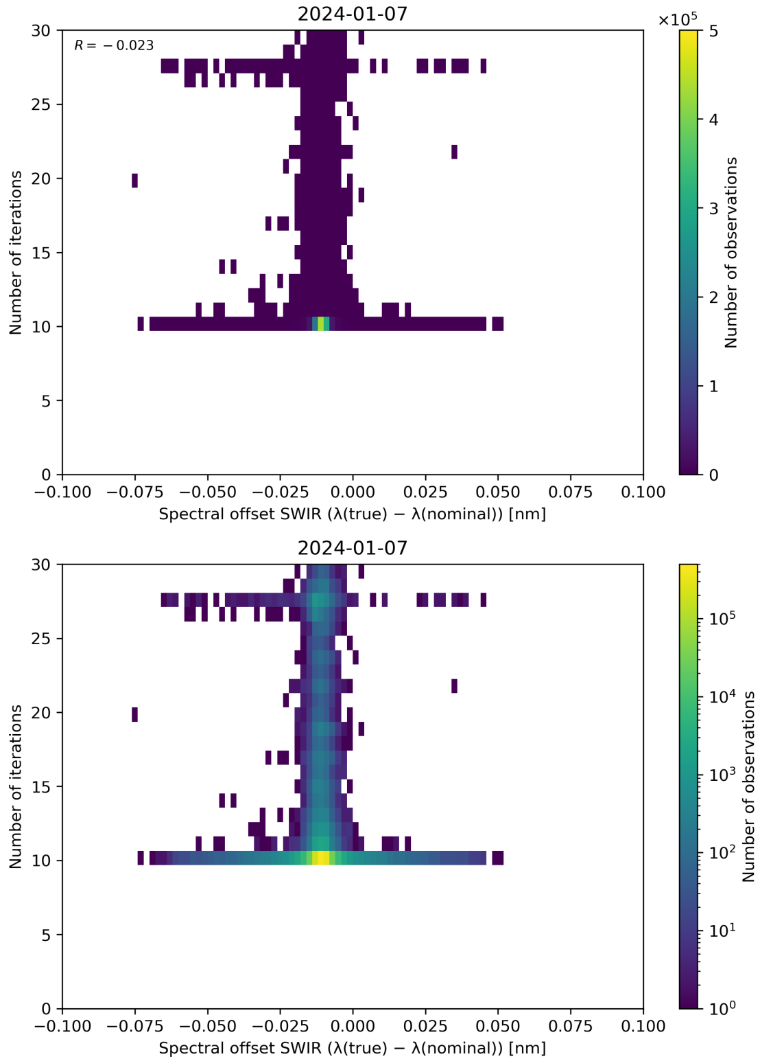
Figure 121: Scatter density plot of “Spectral offset SWIR ( \lambda(\text{true}) - \lambda(\text{nominal}) )” against “Number of iterations” for 2024-01-06 to 2024-01-08.
