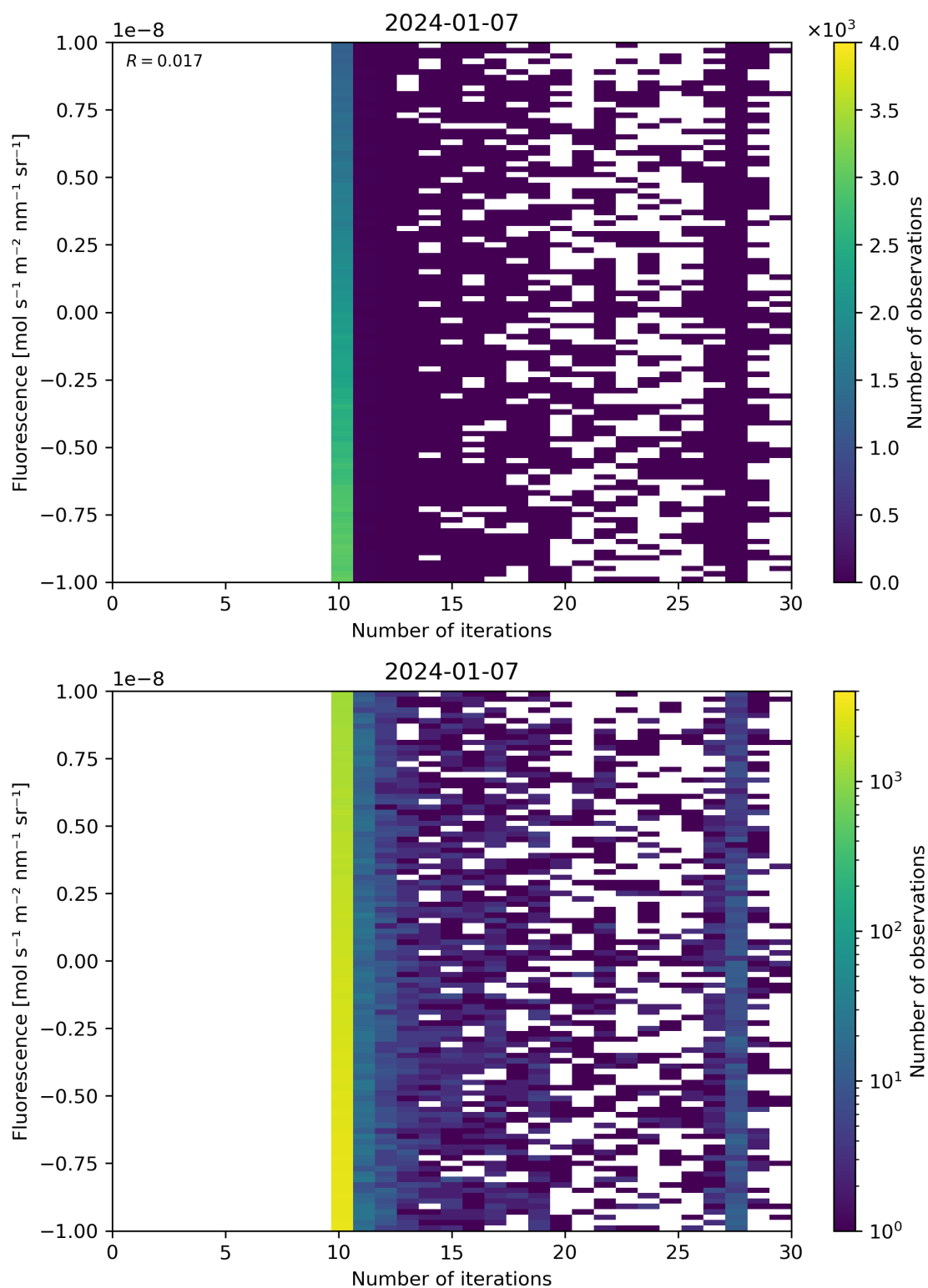
Figure 87: Scatter density plot of “Number of iterations” against “Fluorescence” for 2024-01-06 to 2024-01-08.
