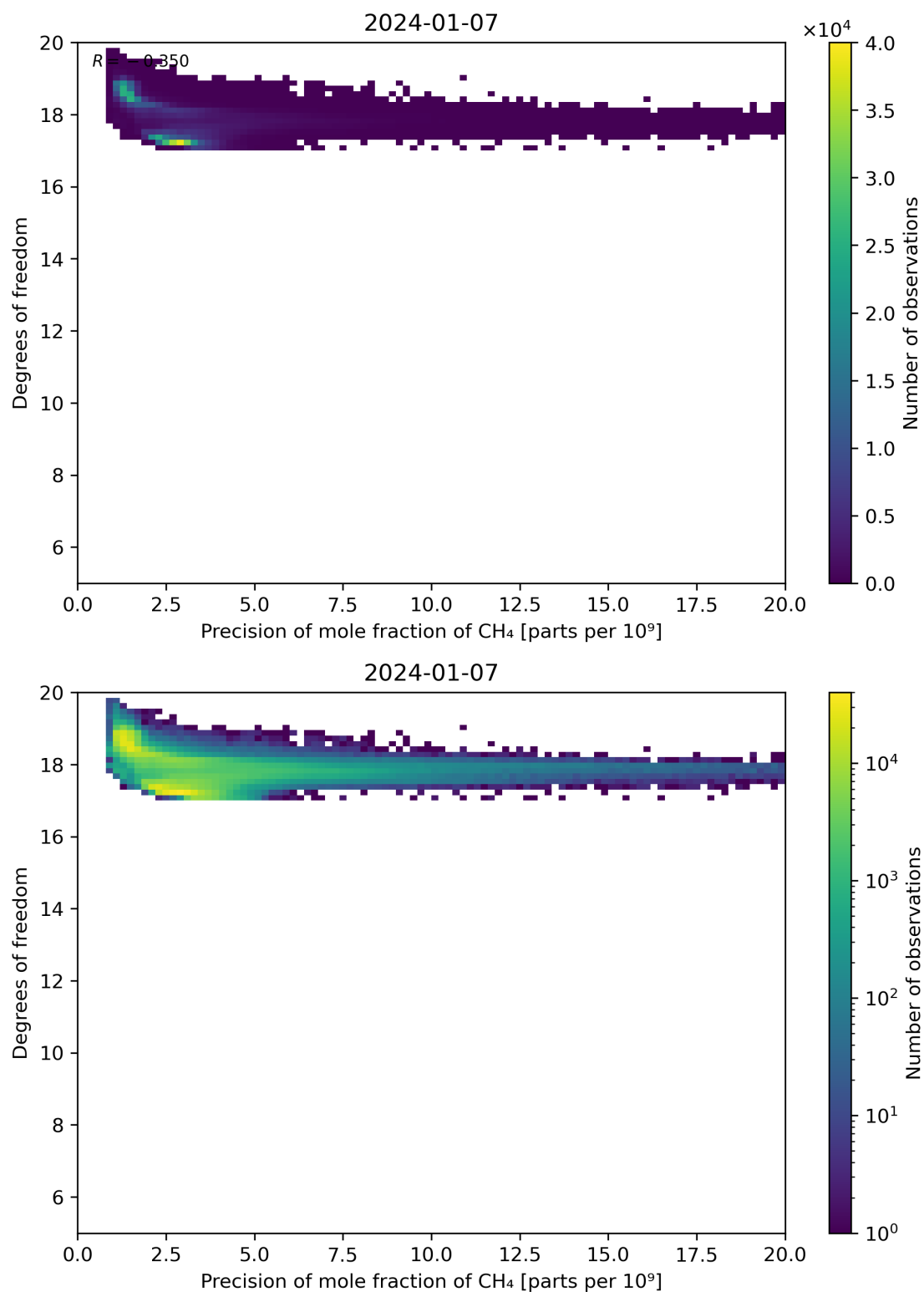
Figure 80: Scatter density plot of “Precision of mole fraction of CH 4 ” against “Degrees of freedom” for 2024-01-06 to 2024-01-08.
