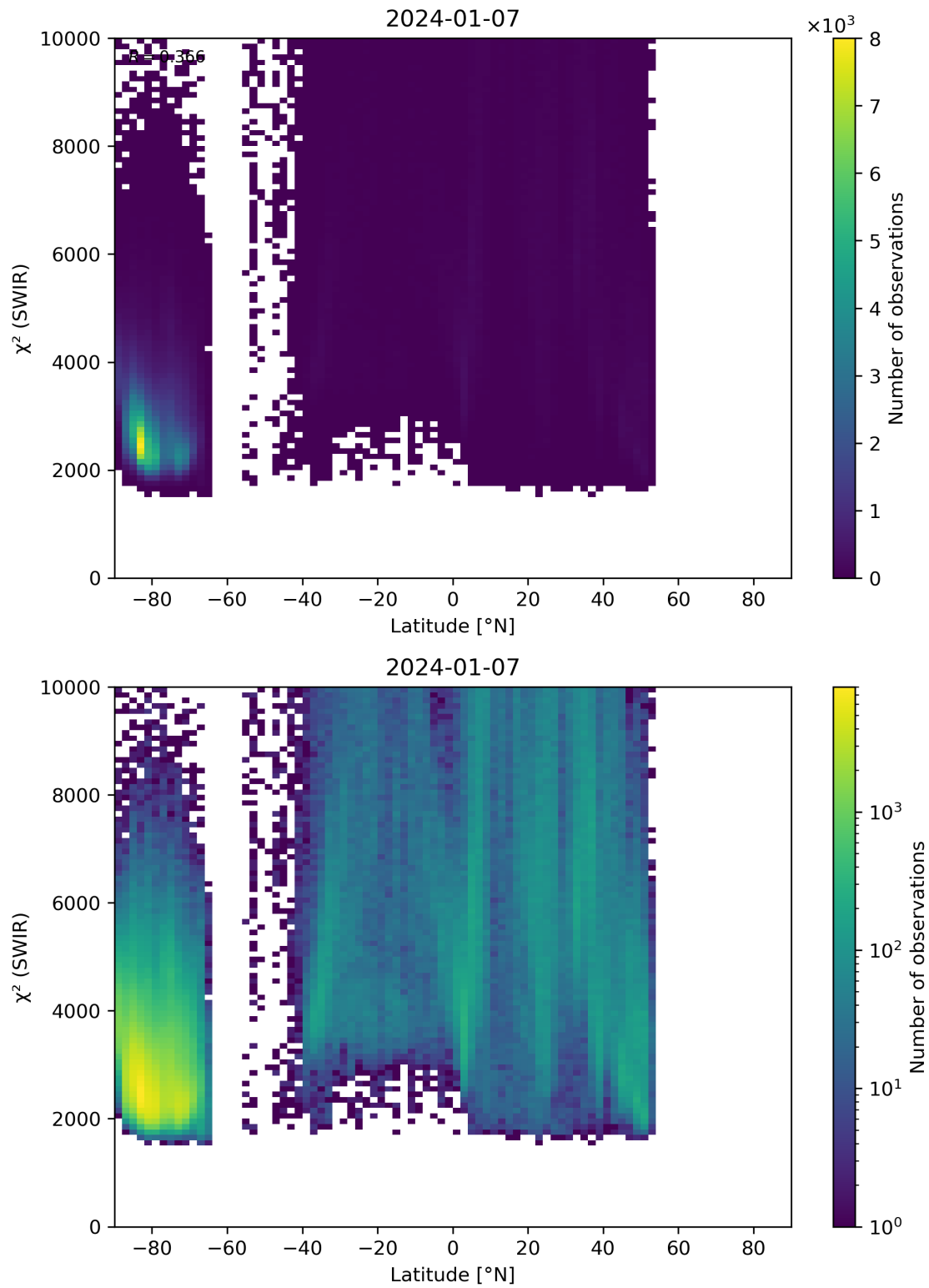
Figure 54: Scatter density plot of “Latitude” against “ \chi^2 (SWIR)” for 2024-01-06 to 2024-01-08.
