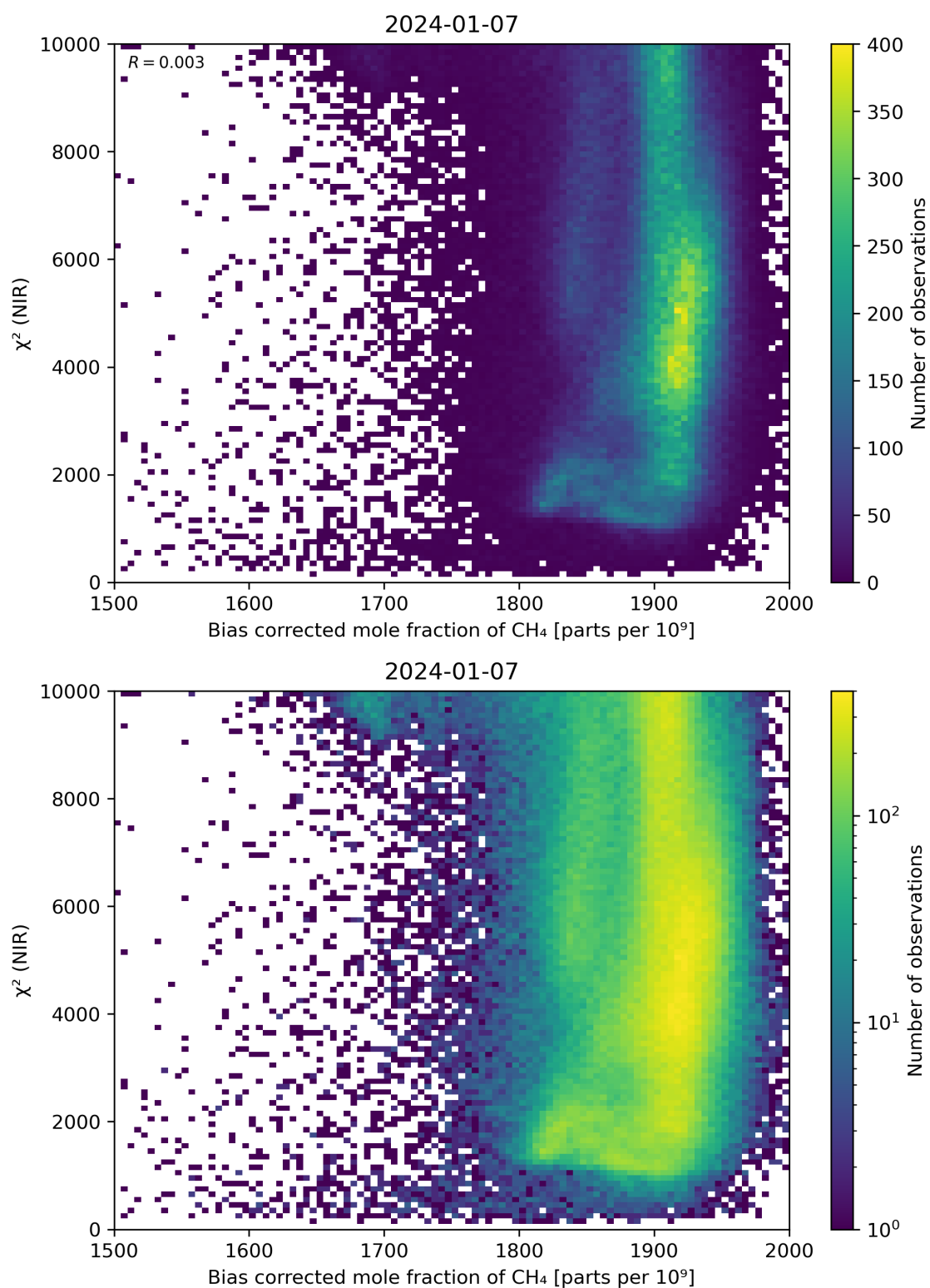
Figure 63: Scatter density plot of “Bias corrected mole fraction of CH 4 ” against “ \chi^2 (NIR)” for 2024-01-06 to 2024-01-08.
