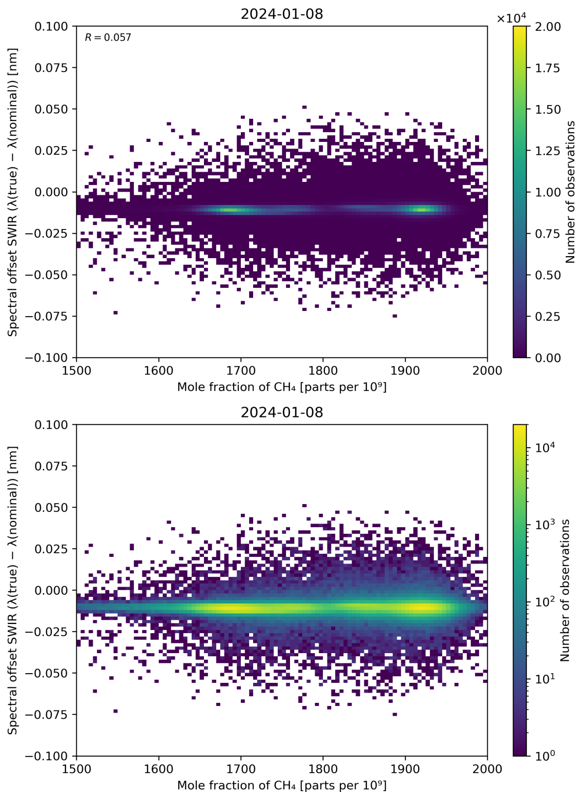
Figure 86: Scatter density plot of “Mole fraction of CH 4 ” against “Spectral offset SWIR ( \lambda(\text{true}) - \lambda(\text{nominal}) )” for 2024-01-07 to 2024-01-09.
