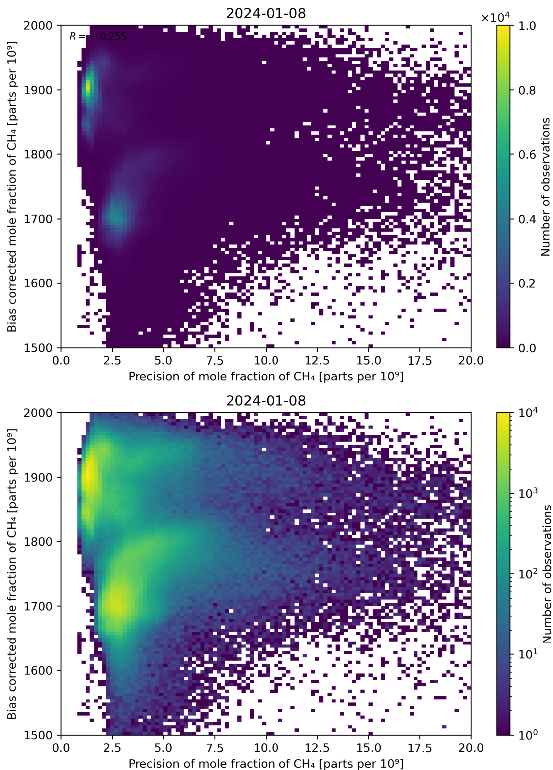
Figure 82: Scatter density plot of “Precision of mole fraction of CH 4 ” against “Bias corrected mole fraction of CH 4 ” for 2024-01-07 to 2024-01-09.
