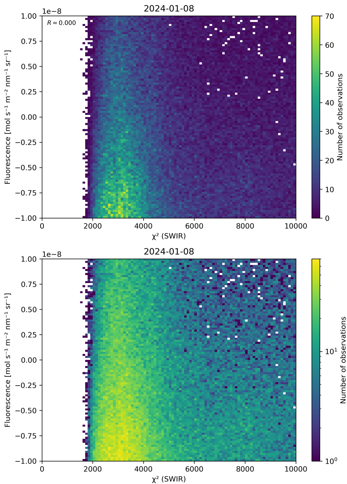
Figure 49: Scatter density plot of “ \chi^2 (SWIR)” against “Fluorescence” for 2024-01-07 to 2024-01-09.
