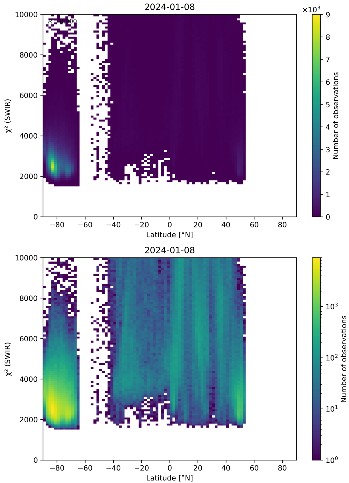
Figure 54: Scatter density plot of “Latitude” against “ \chi^2 (SWIR)” for 2024-01-07 to 2024-01-09.
