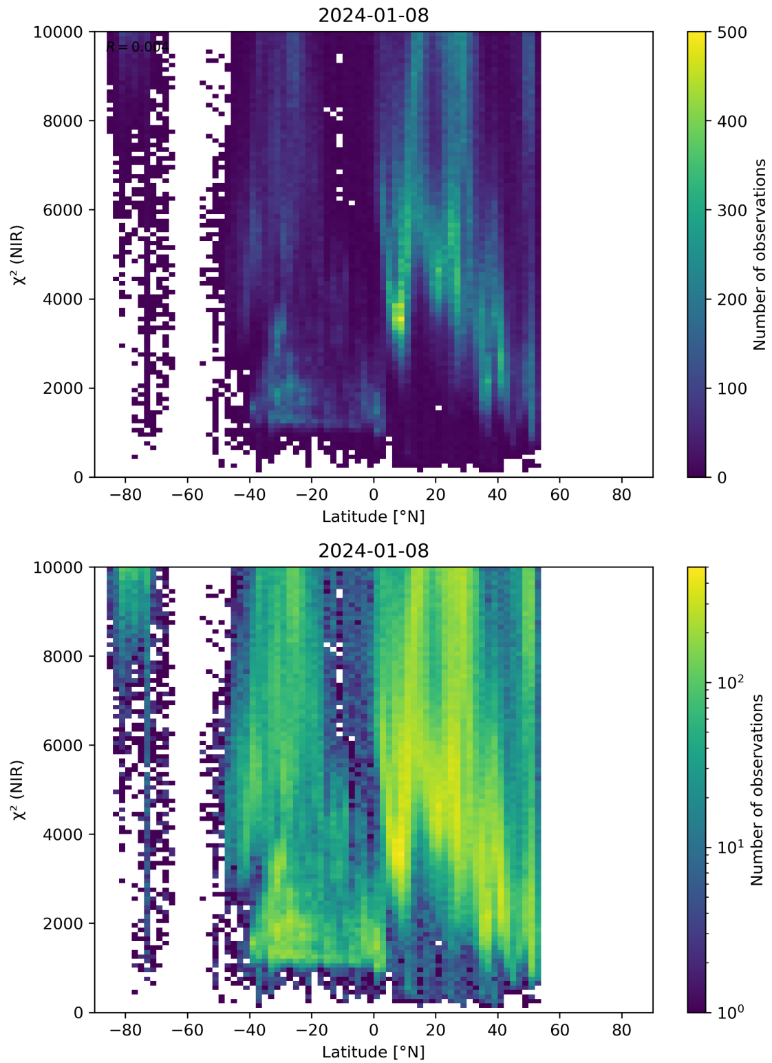
Figure 53: Scatter density plot of “Latitude” against “ \chi^2 (NIR)” for 2024-01-07 to 2024-01-09.
