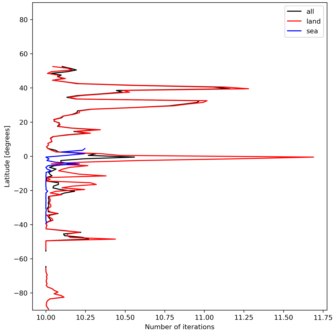
Figure 20: Zonal average of “Number of iterations” for 2024-01-07 to 2024-01-09.
