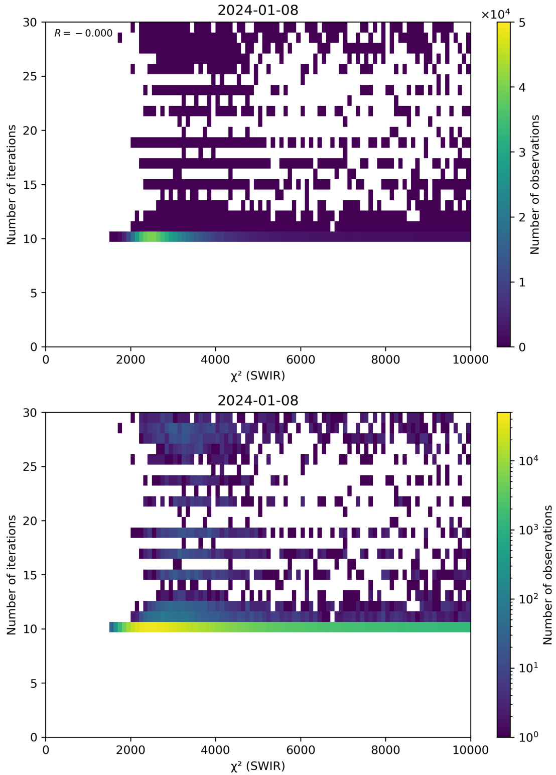
Figure 50: Scatter density plot of “ \chi^2 (SWIR)” against “Number of iterations” for 2024-01-07 to 2024-01-09.
