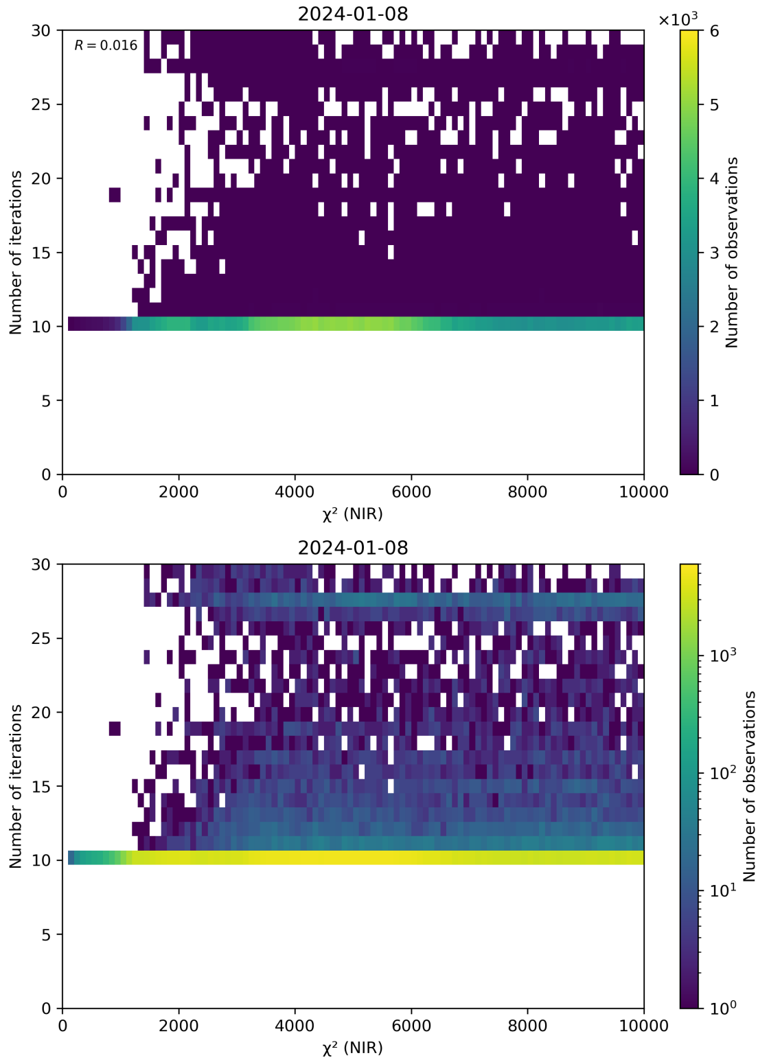
Figure 46: Scatter density plot of “ \chi^2 (NIR)” against “Number of iterations” for 2024-01-07 to 2024-01-09.
