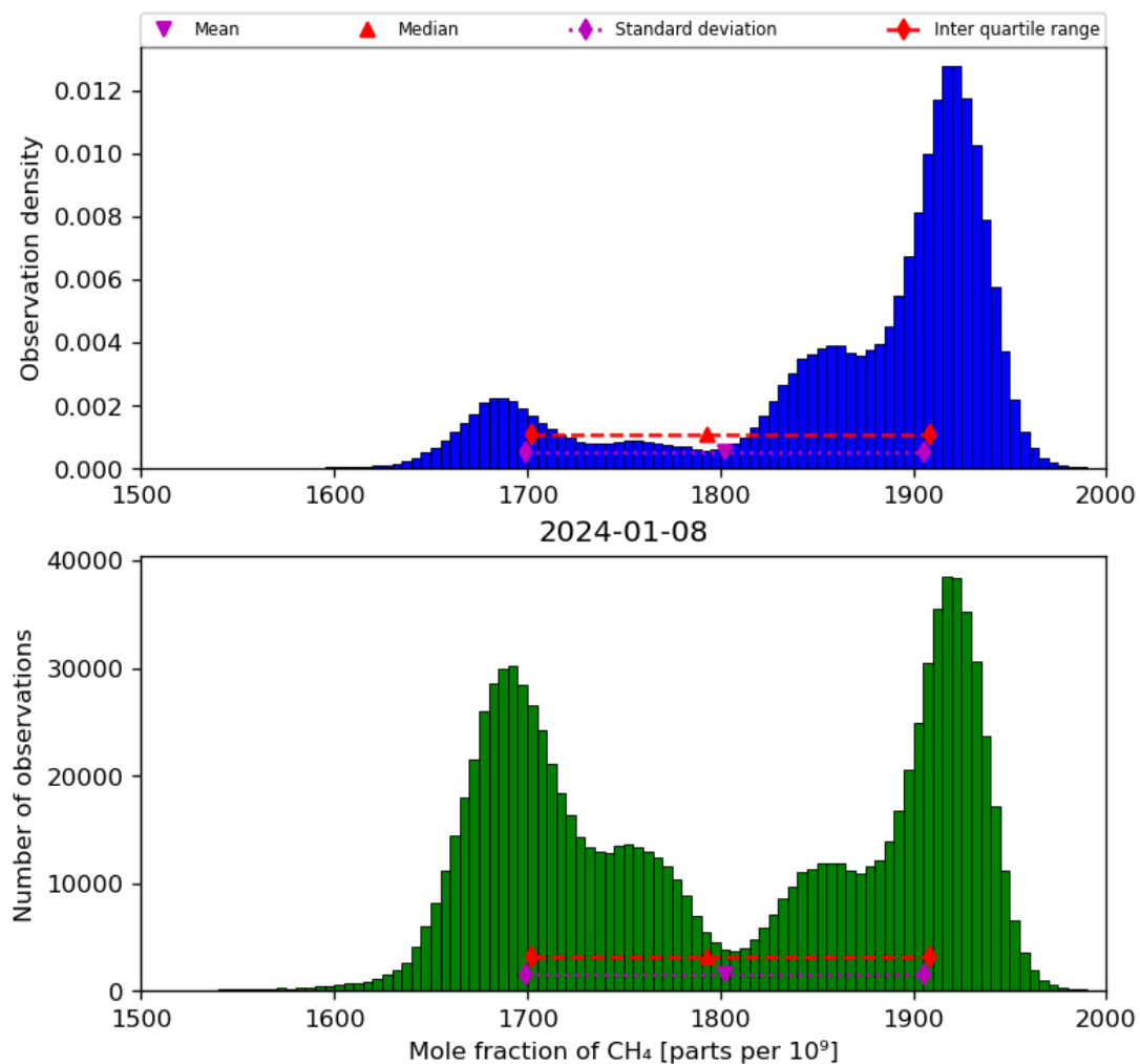
Figure 23: Histogram of “Mole fraction of CH 4 ” for 2024-01-07 to 2024-01-09
