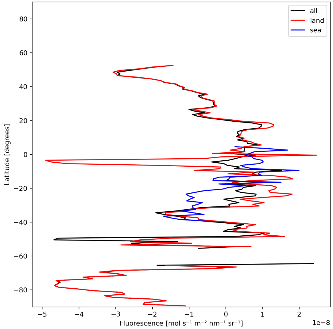
Figure 21: Zonal average of “Fluorescence” for 2024-01-07 to 2024-01-09.
