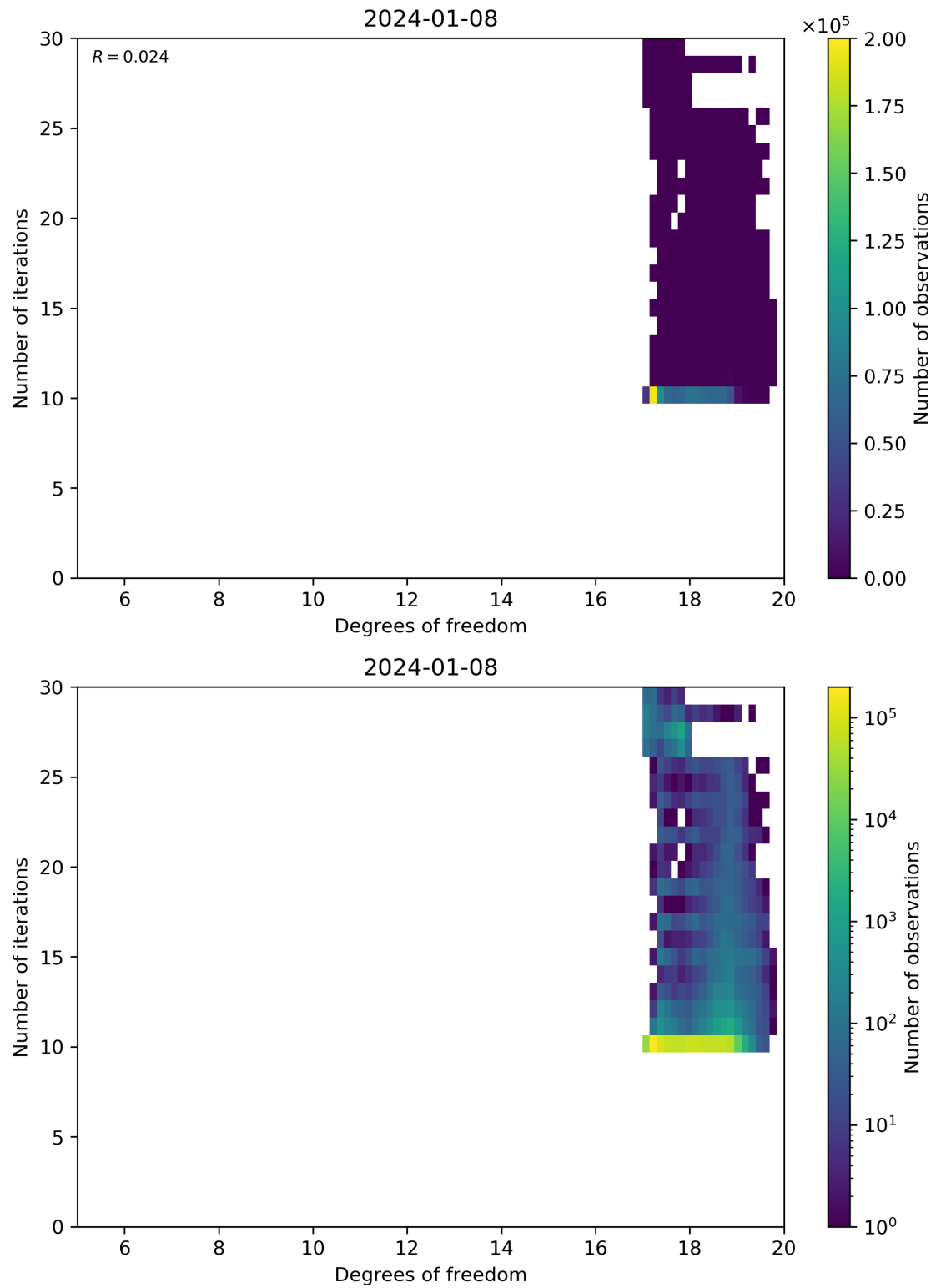
Figure 52: Scatter density plot of “Degrees of freedom” against “Number of iterations” for 2024-01-07 to 2024-01-09.
