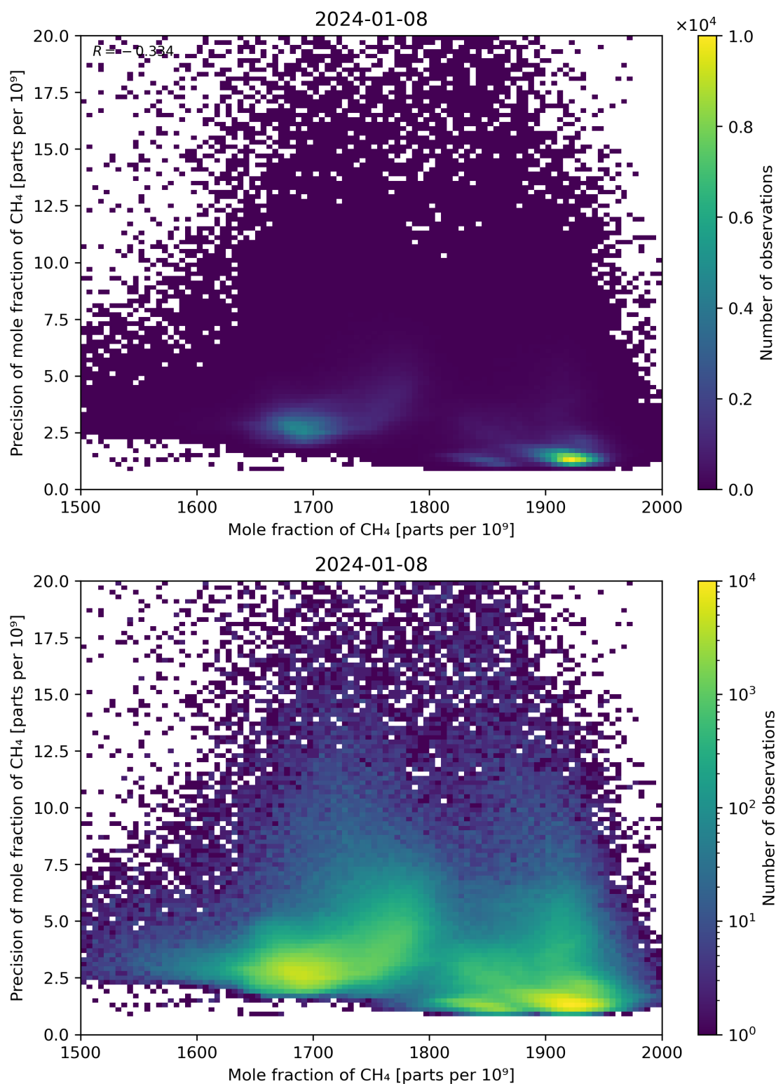
Figure 75: Scatter density plot of “Mole fraction of CH 4 ” against “Precision of mole fraction of CH 4 ” for 2024-01-07 to 2024-01-09.
