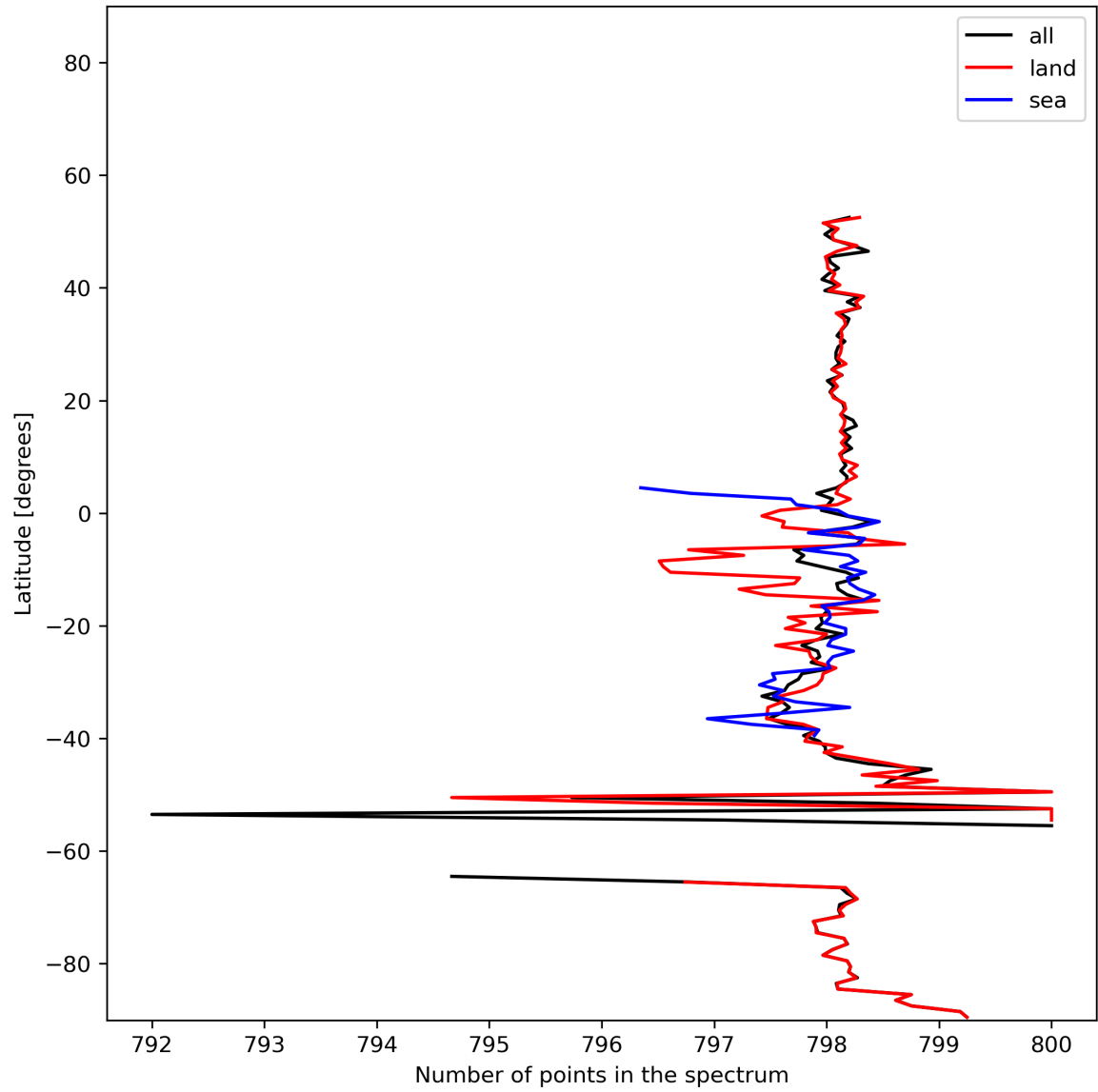
Figure 15: Zonal average of “Number of points in the spectrum” for 2024-01-07 to 2024-01-09.
