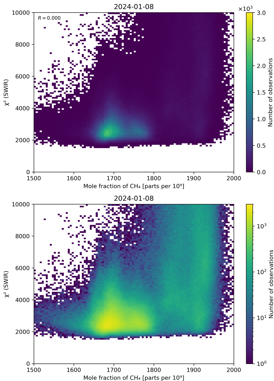
Figure 71: Scatter density plot of “Mole fraction of CH 4 ” against “ \chi^2 (SWIR)” for 2024-01-07 to 2024-01-09.
