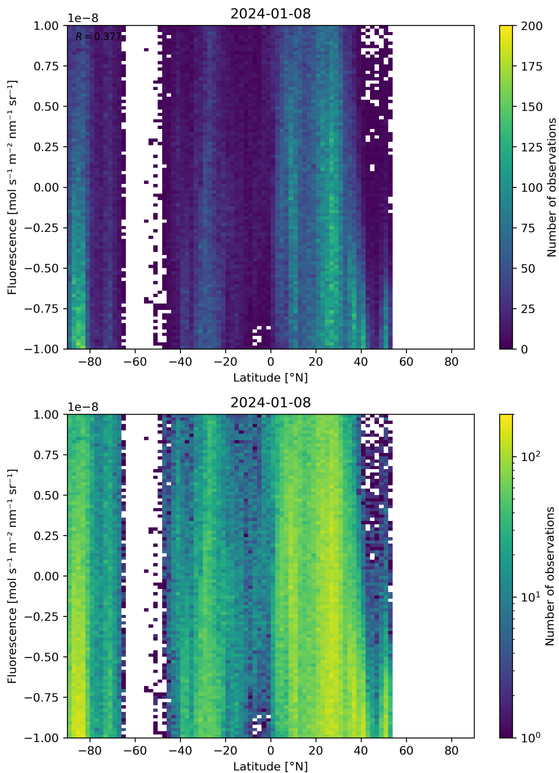
Figure 56: Scatter density plot of “Latitude” against “Fluorescence” for 2024-01-07 to 2024-01-09.
