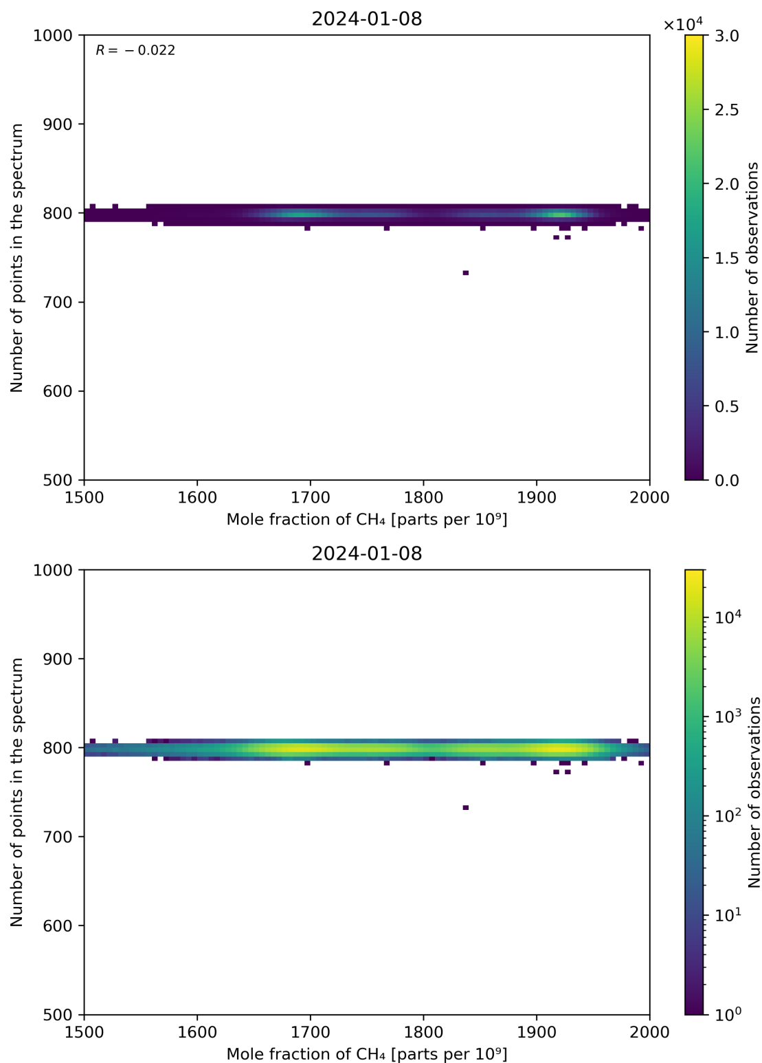
Figure 77: Scatter density plot of “Mole fraction of CH 4 ” against “Number of points in the spectrum” for 2024-01-07 to 2024-01-09.
