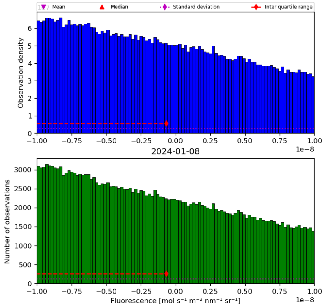
Figure 32: Histogram of “Fluorescence” for 2024-01-07 to 2024-01-09
