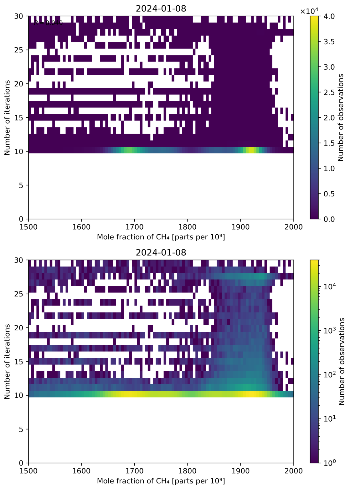
Figure 76: Scatter density plot of “Mole fraction of CH 4 ” against “Number of iterations” for 2024-01-07 to 2024-01-09.
