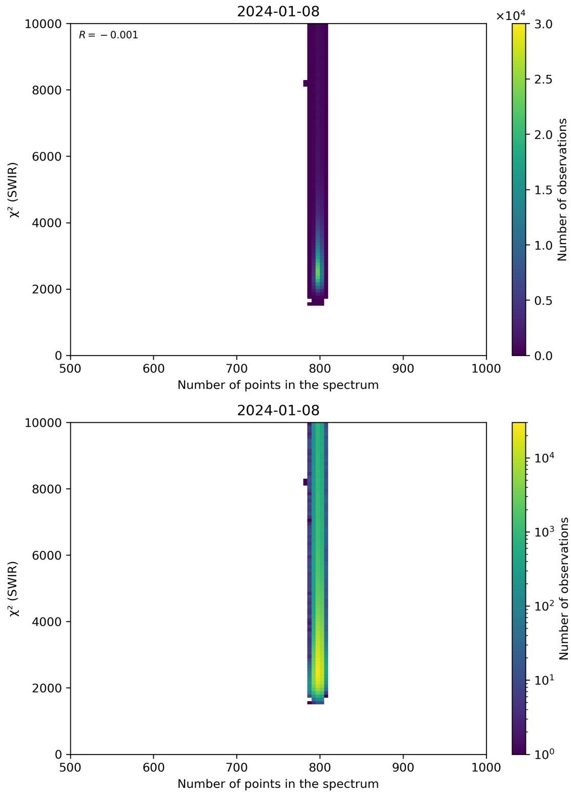
Figure 89: Scatter density plot of “Number of points in the spectrum” against “ \chi^2 (SWIR)” for 2024-01-07 to 2024-01-09.
