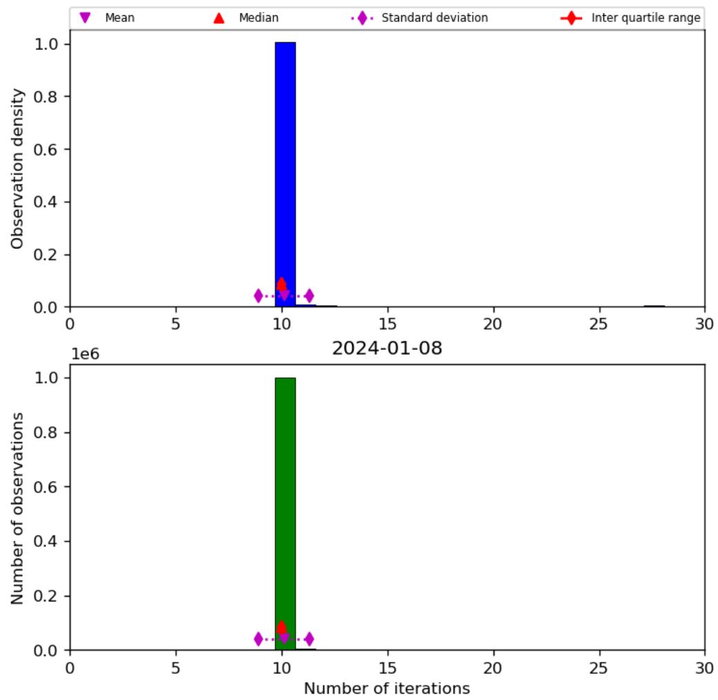
Figure 31: Histogram of “Number of iterations” for 2024-01-07 to 2024-01-09
