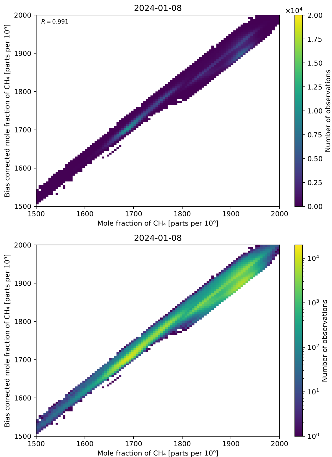
Figure 74: Scatter density plot of “Mole fraction of CH 4 ” against “Bias corrected mole fraction of CH 4 ” for 2024-01-07 to 2024-01-09.
