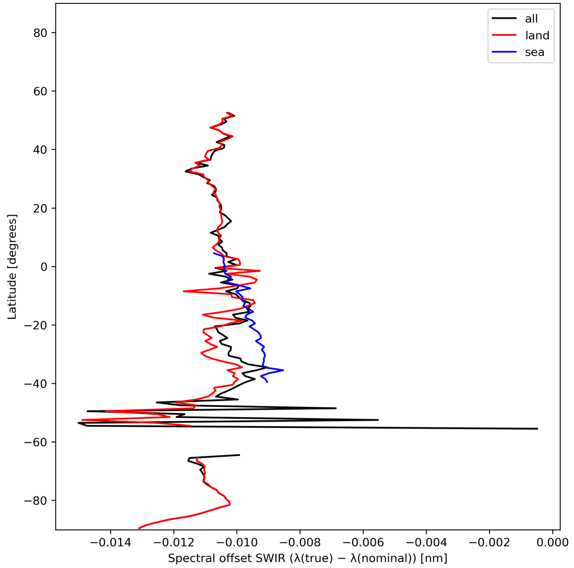
Figure 16: Zonal average of “Spectral offset SWIR ( \lambda(\text{true}) - \lambda(\text{nominal}) )” for 2024-01-07 to 2024-01-09.
