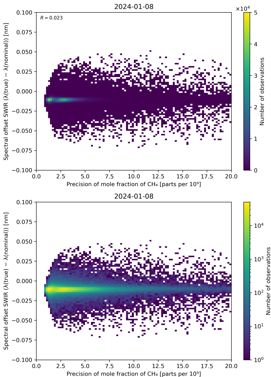
Figure 85: Scatter density plot of “Precision of mole fraction of CH 4 ” against “Spectral offset SWIR ( \lambda(\text{true}) - \lambda(\text{nominal}) )” for 2024-01-07 to 2024-01-09.
