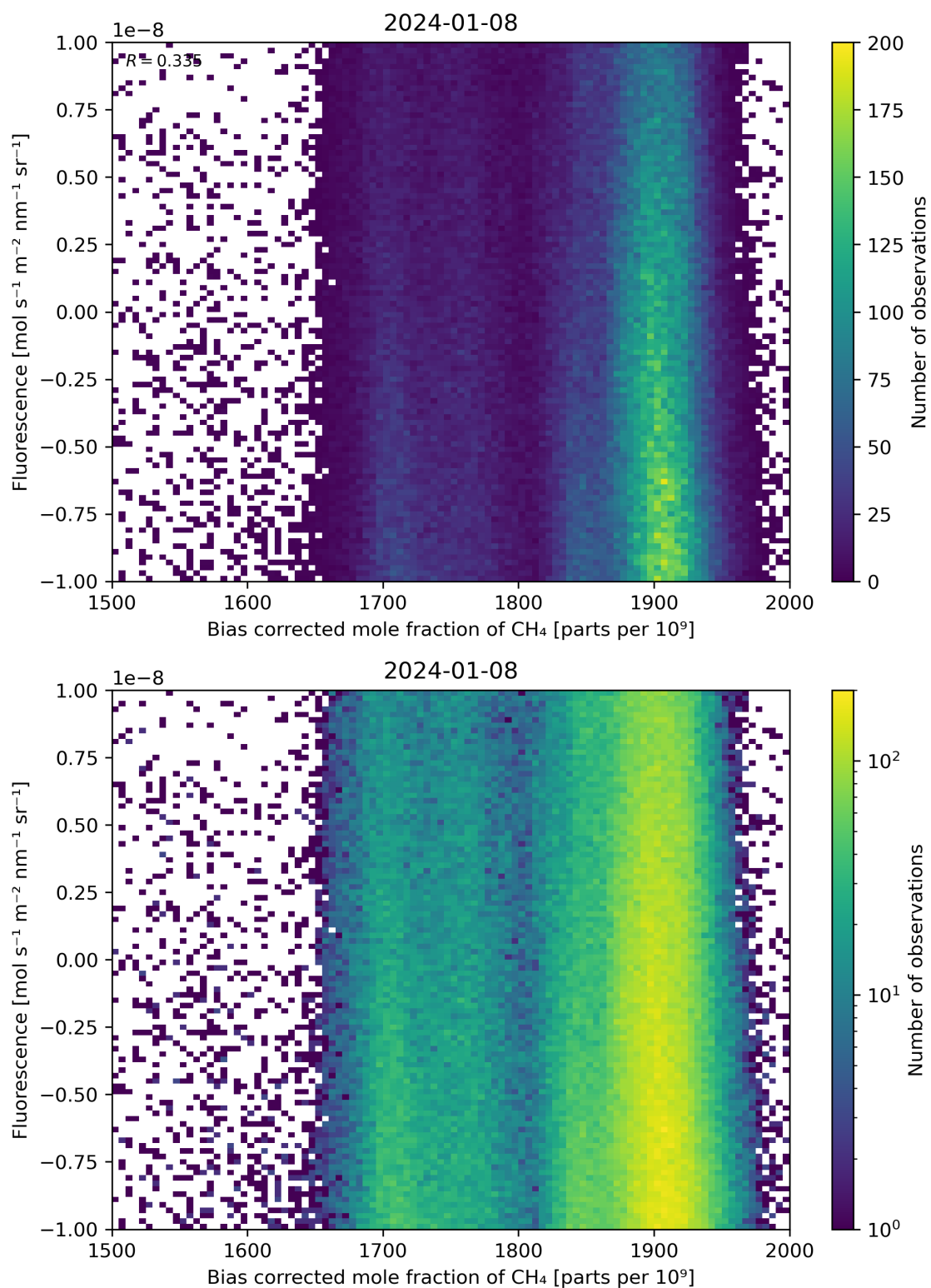
Figure 66: Scatter density plot of “Bias corrected mole fraction of \text{CH}_4 ” against “Fluorescence” for 2024-01-07 to 2024-01-09.
