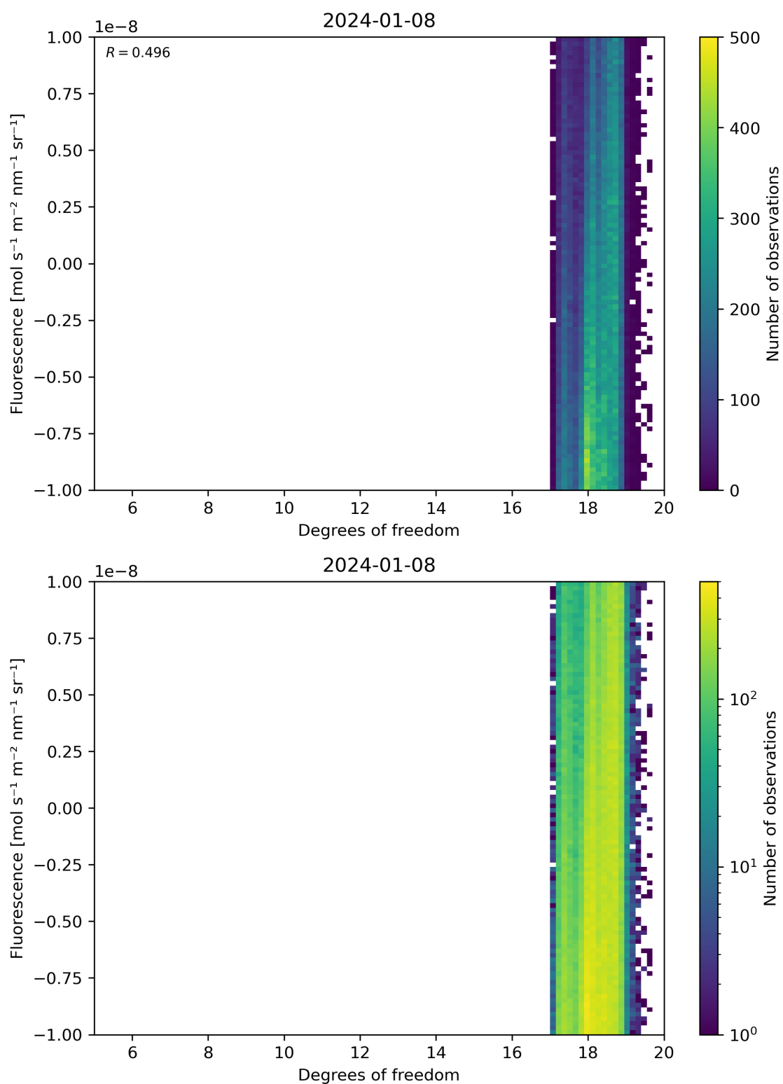
Figure 51: Scatter density plot of “Degrees of freedom” against “Fluorescence” for 2024-01-07 to 2024-01-09.
