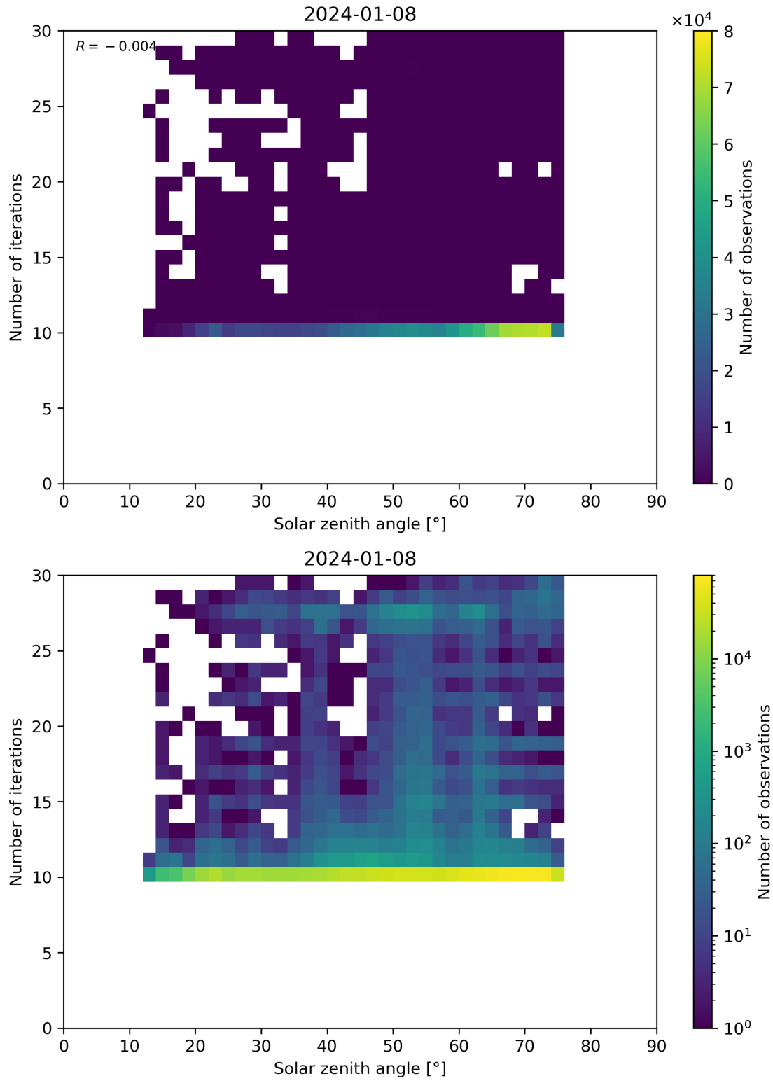
Figure 102: Scatter density plot of “Solar zenith angle” against “Number of iterations” for 2024-01-07 to 2024-01-09.
