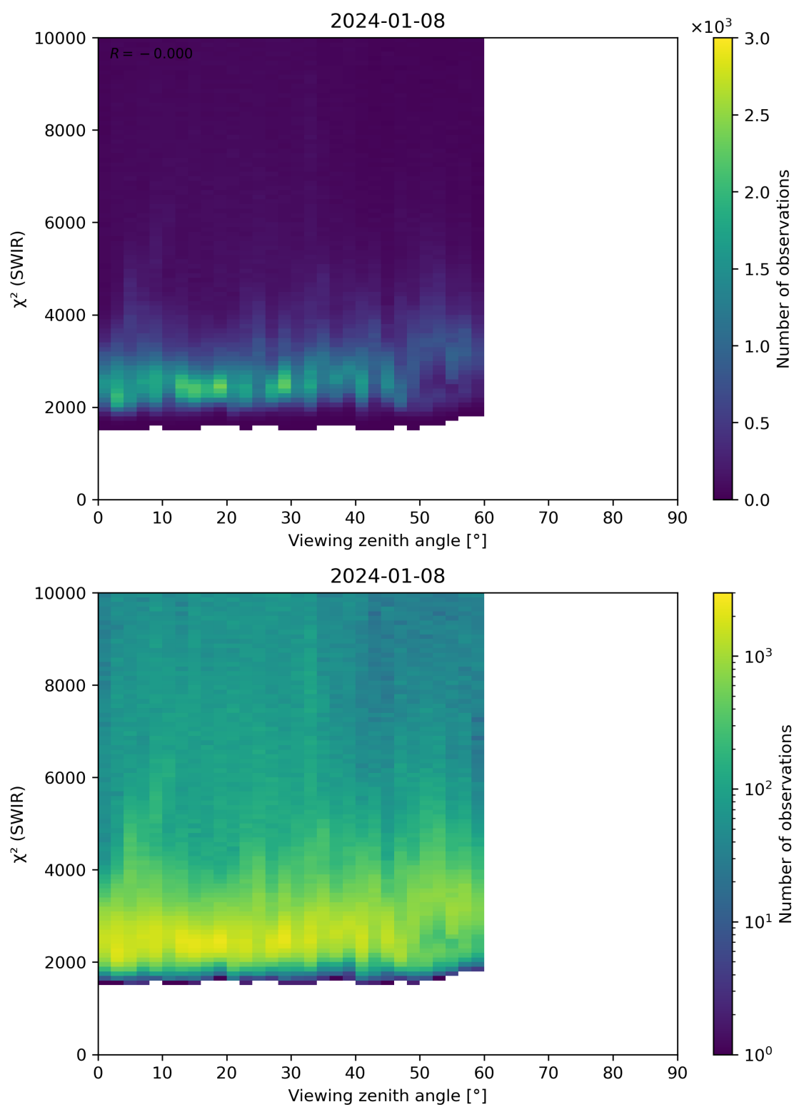
Figure 106: Scatter density plot of “Viewing zenith angle” against “ \chi^2 (SWIR)” for 2024-01-07 to 2024-01-09.
