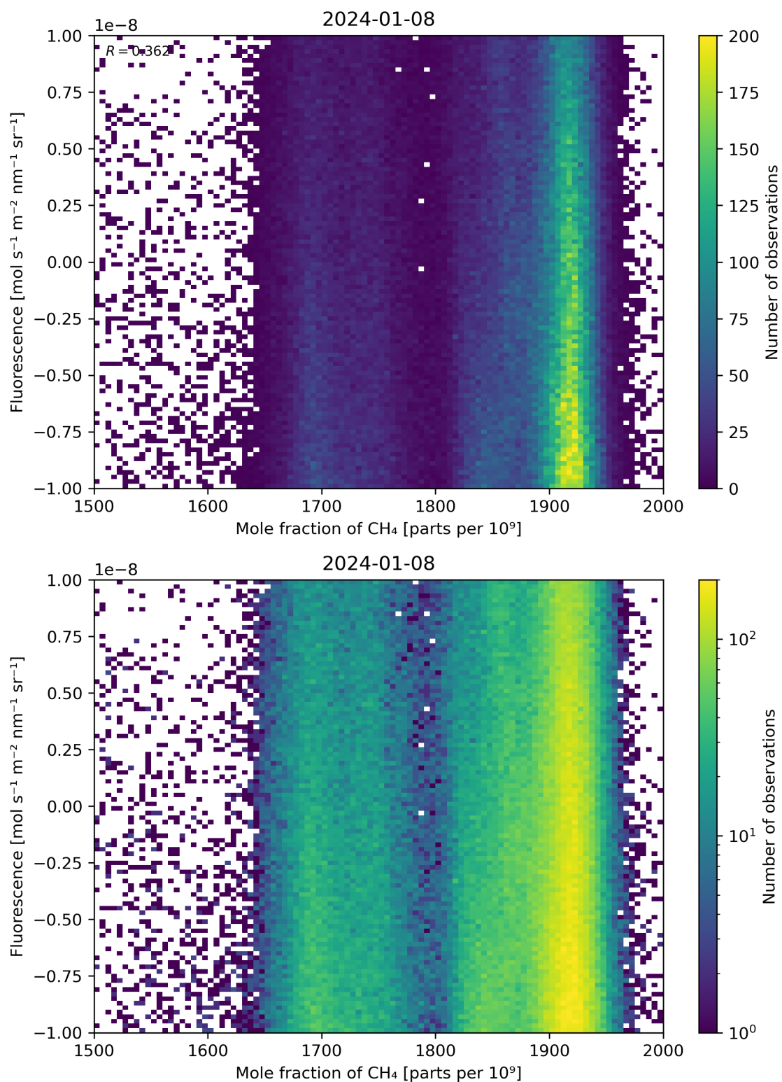
Figure 73: Scatter density plot of “Mole fraction of \text{CH}_4 ” against “Fluorescence” for 2024-01-07 to 2024-01-09.
