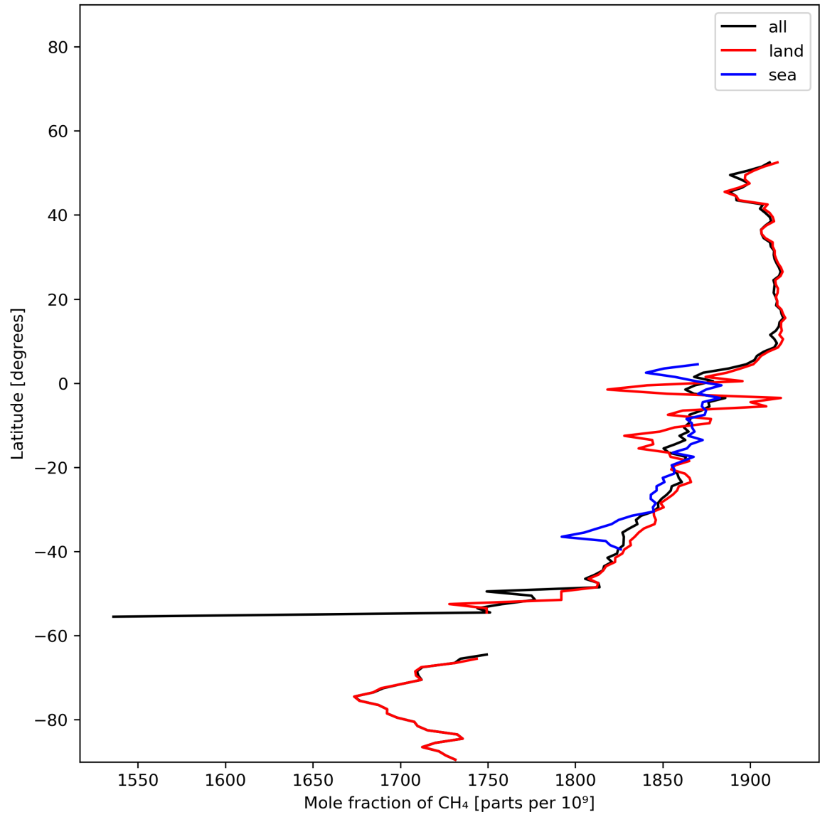
Figure 12: Zonal average of “Mole fraction of CH 4 ” for 2024-01-07 to 2024-01-09.
