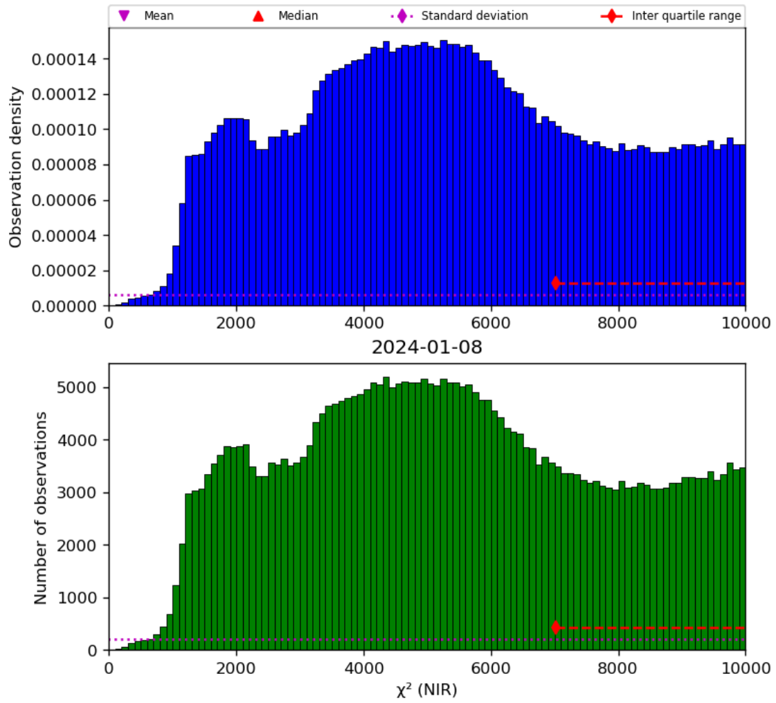
Figure 29: Histogram of “ \chi^2 (NIR)” for 2024-01-07 to 2024-01-09
