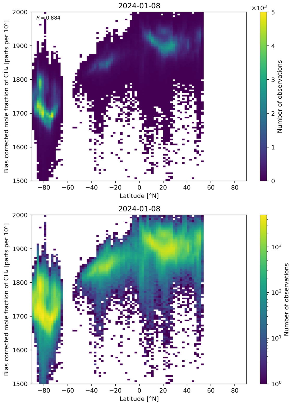
Figure 58: Scatter density plot of “Latitude” against “Bias corrected mole fraction of CH 4 ” for 2024-01-07 to 2024-01-09.
