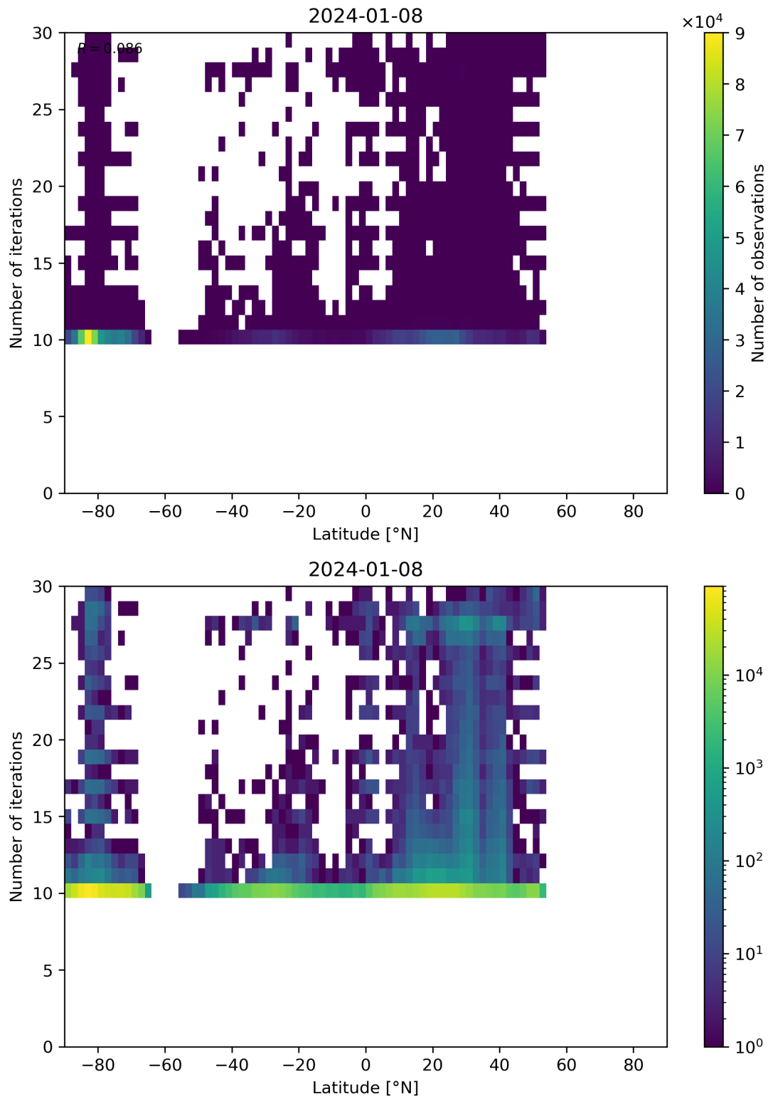
Figure 60: Scatter density plot of “Latitude” against “Number of iterations” for 2024-01-07 to 2024-01-09.
