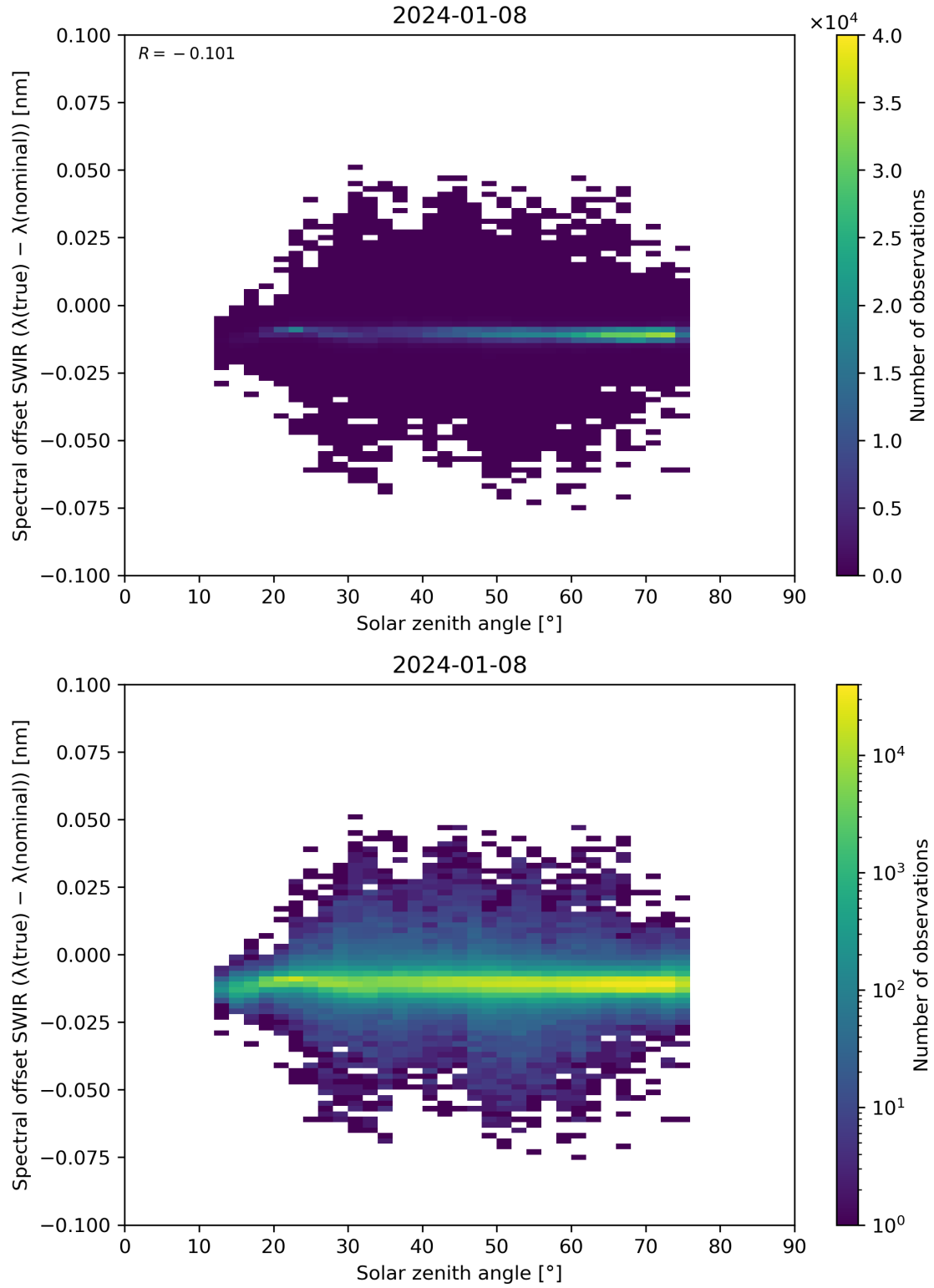
Figure 104: Scatter density plot of “Solar zenith angle” against “Spectral offset SWIR ( \lambda(\text{true}) - \lambda(\text{nominal}) )” for 2024-01-07 to 2024-01-09.
