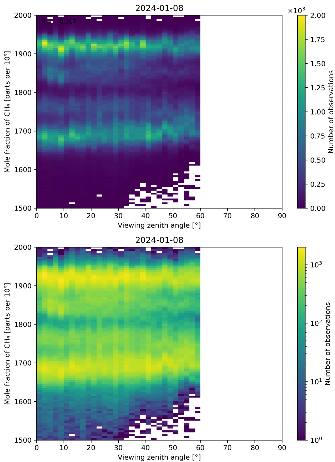
Figure 110: Scatter density plot of “Viewing zenith angle” against “Mole fraction of CH 4 ” for 2024-01-07 to 2024-01-09.
