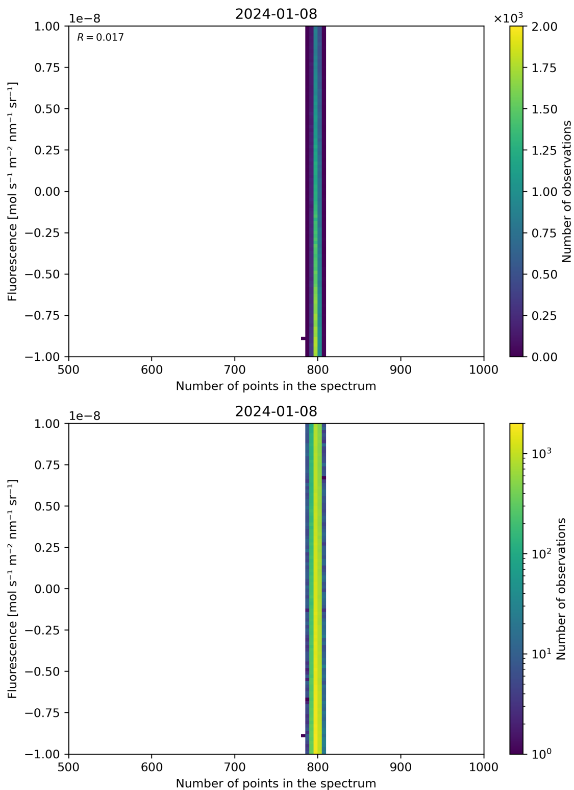
Figure 91: Scatter density plot of “Number of points in the spectrum” against “Fluorescence” for 2024-01-07 to 2024-01-09.
