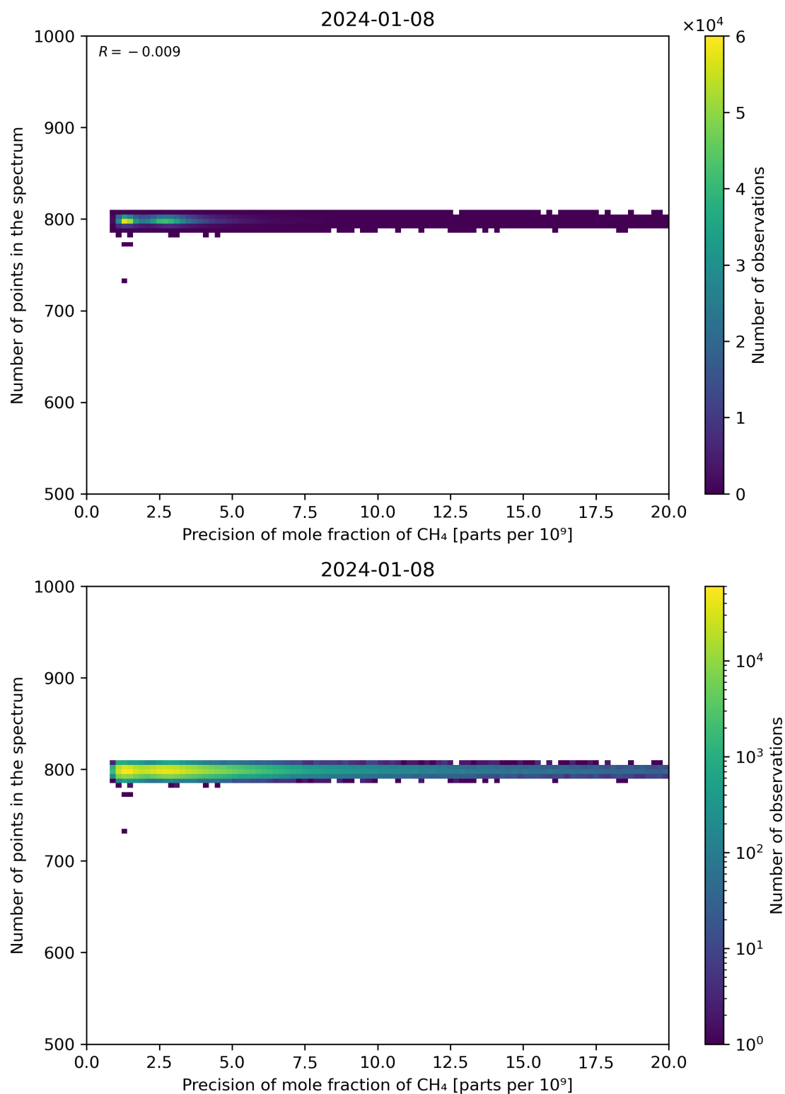
Figure 84: Scatter density plot of “Precision of mole fraction of CH 4 ” against “Number of points in the spectrum” for 2024-01-07 to 2024-01-09.
