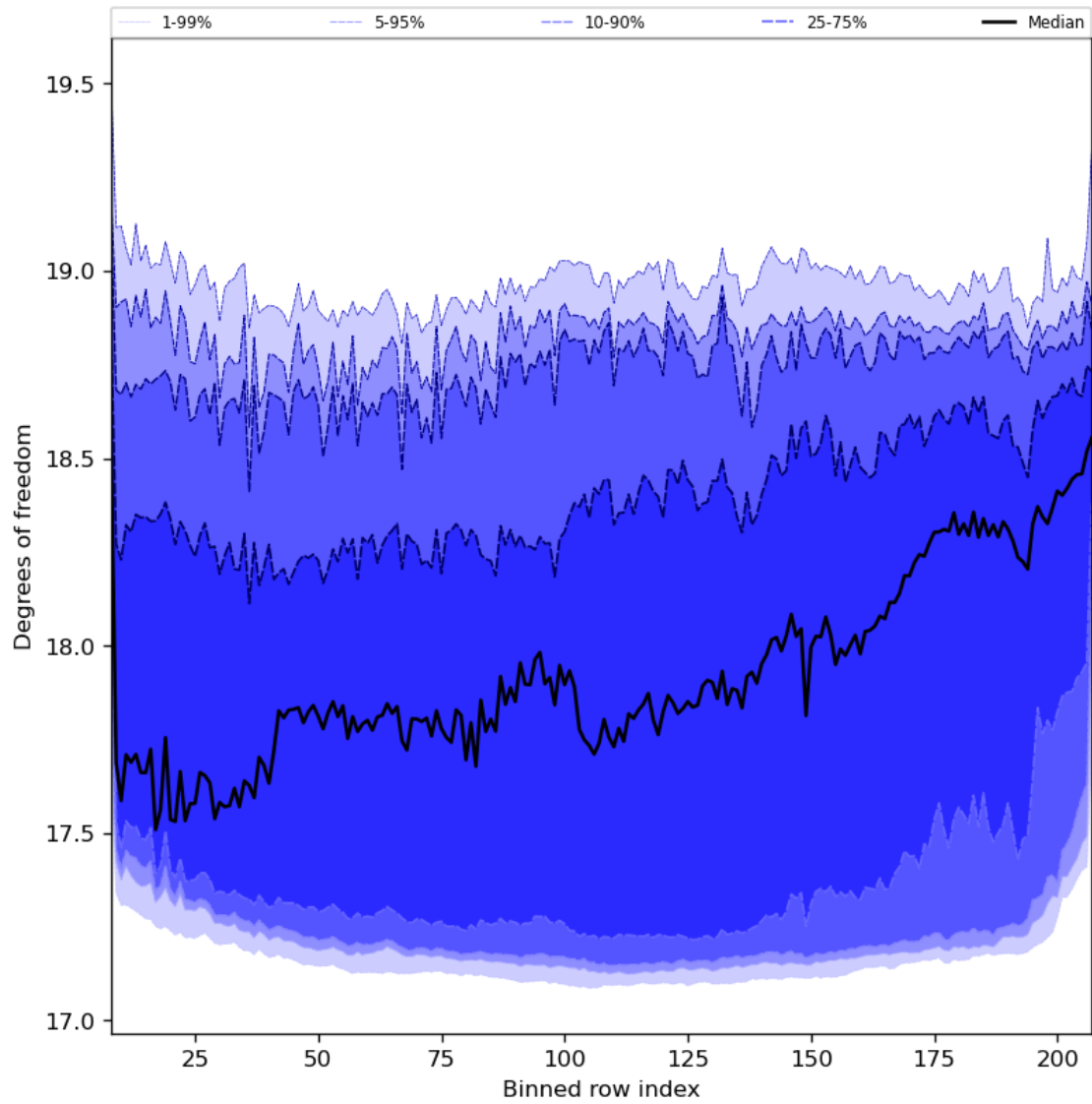
Figure 41: Along track statistics of “Degrees of freedom” for 2024-01-07 to 2024-01-09
