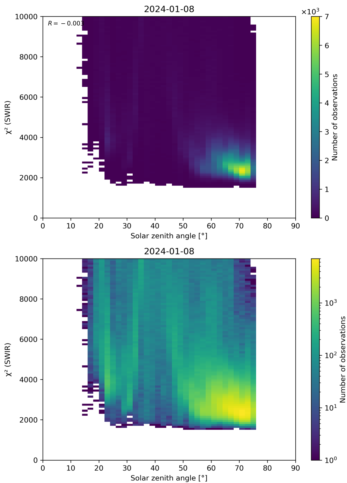
Figure 95: Scatter density plot of “Solar zenith angle” against “ \chi^2 (SWIR)” for 2024-01-07 to 2024-01-09.
