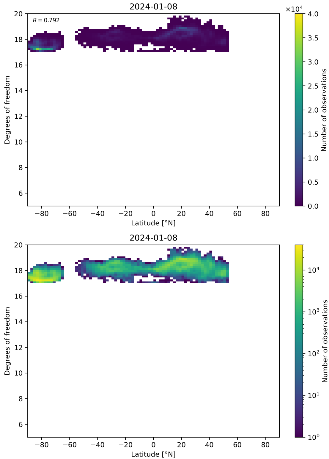
Figure 55: Scatter density plot of “Latitude” against “Degrees of freedom” for 2024-01-07 to 2024-01-09.
