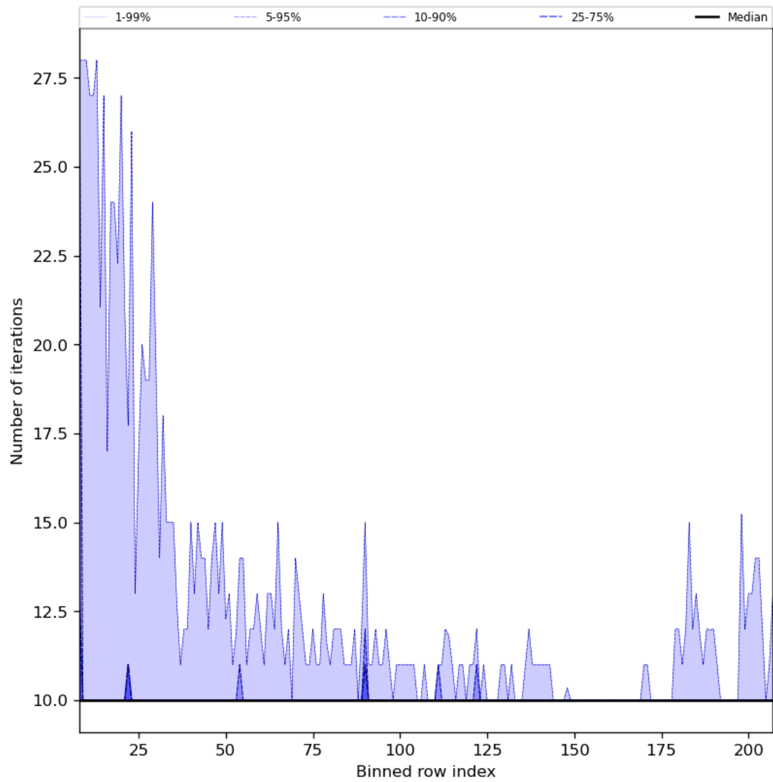
Figure 42: Along track statistics of “Number of iterations” for 2024-01-07 to 2024-01-09
