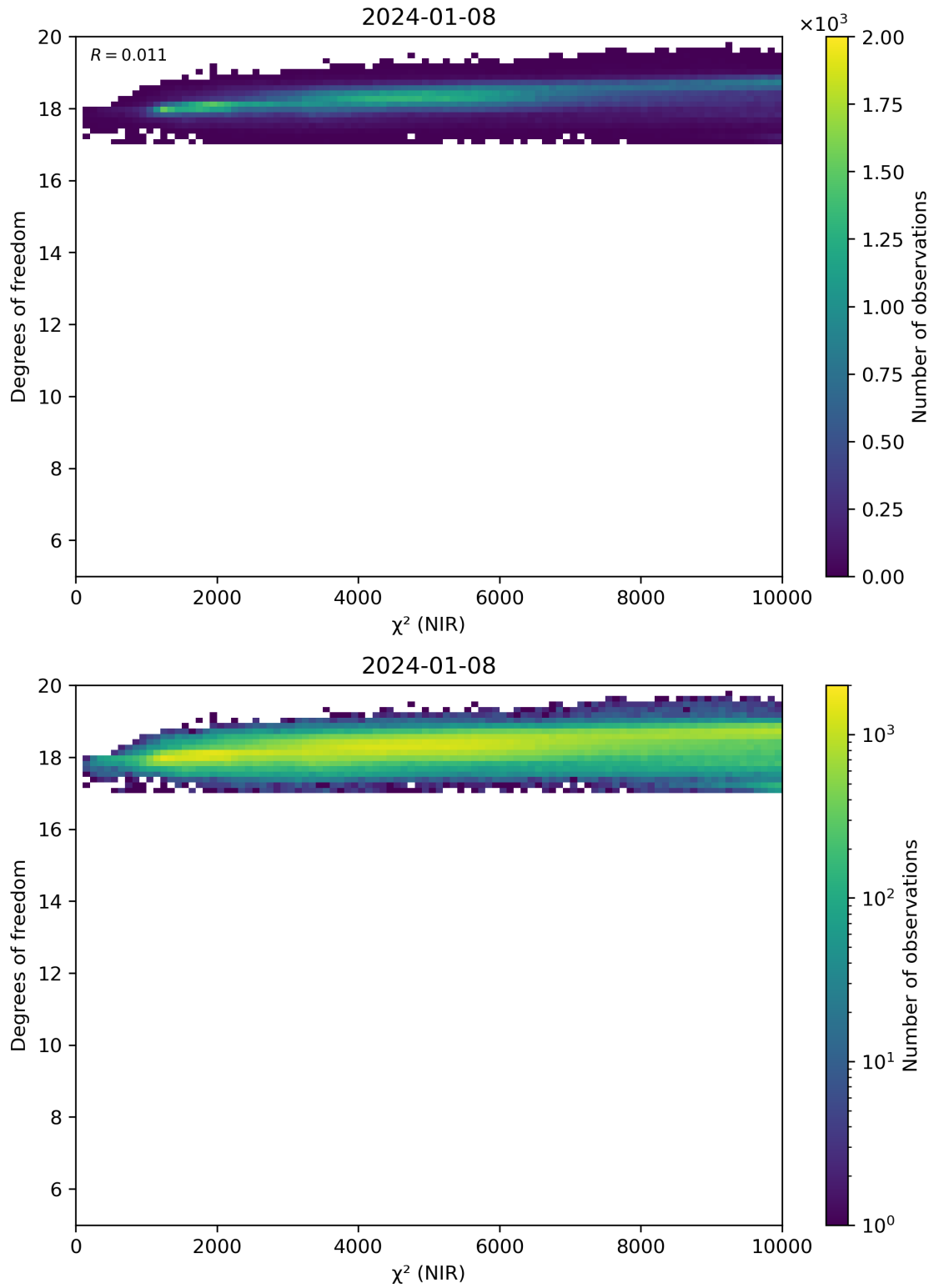
Figure 44: Scatter density plot of “ \chi^2 (NIR)” against “Degrees of freedom” for 2024-01-07 to 2024-01-09.
