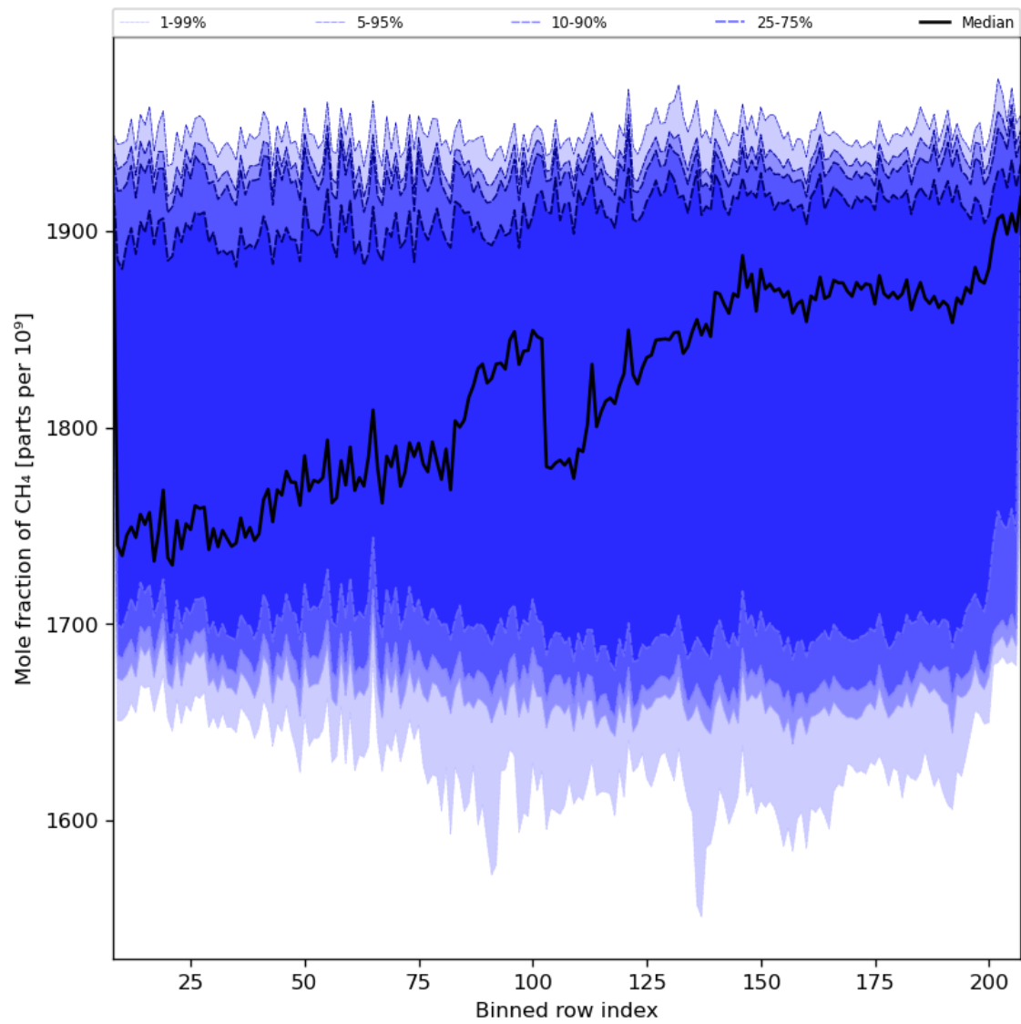
Figure 34: Along track statistics of “Mole fraction of CH 4 ” for 2024-01-07 to 2024-01-09
