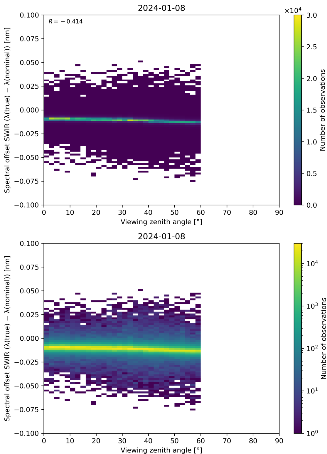
Figure 116: Scatter density plot of “Viewing zenith angle” against “Spectral offset SWIR ( \lambda(\text{true}) - \lambda(\text{nominal}) )” for 2024-01-07 to 2024-01-09.
