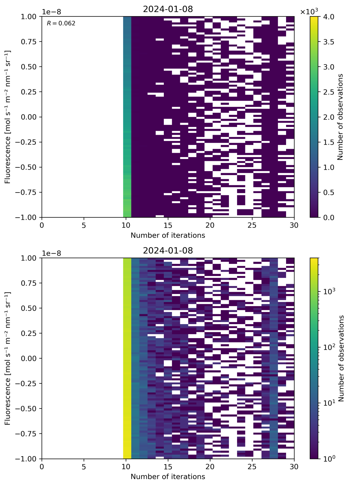
Figure 87: Scatter density plot of “Number of iterations” against “Fluorescence” for 2024-01-07 to 2024-01-09.
