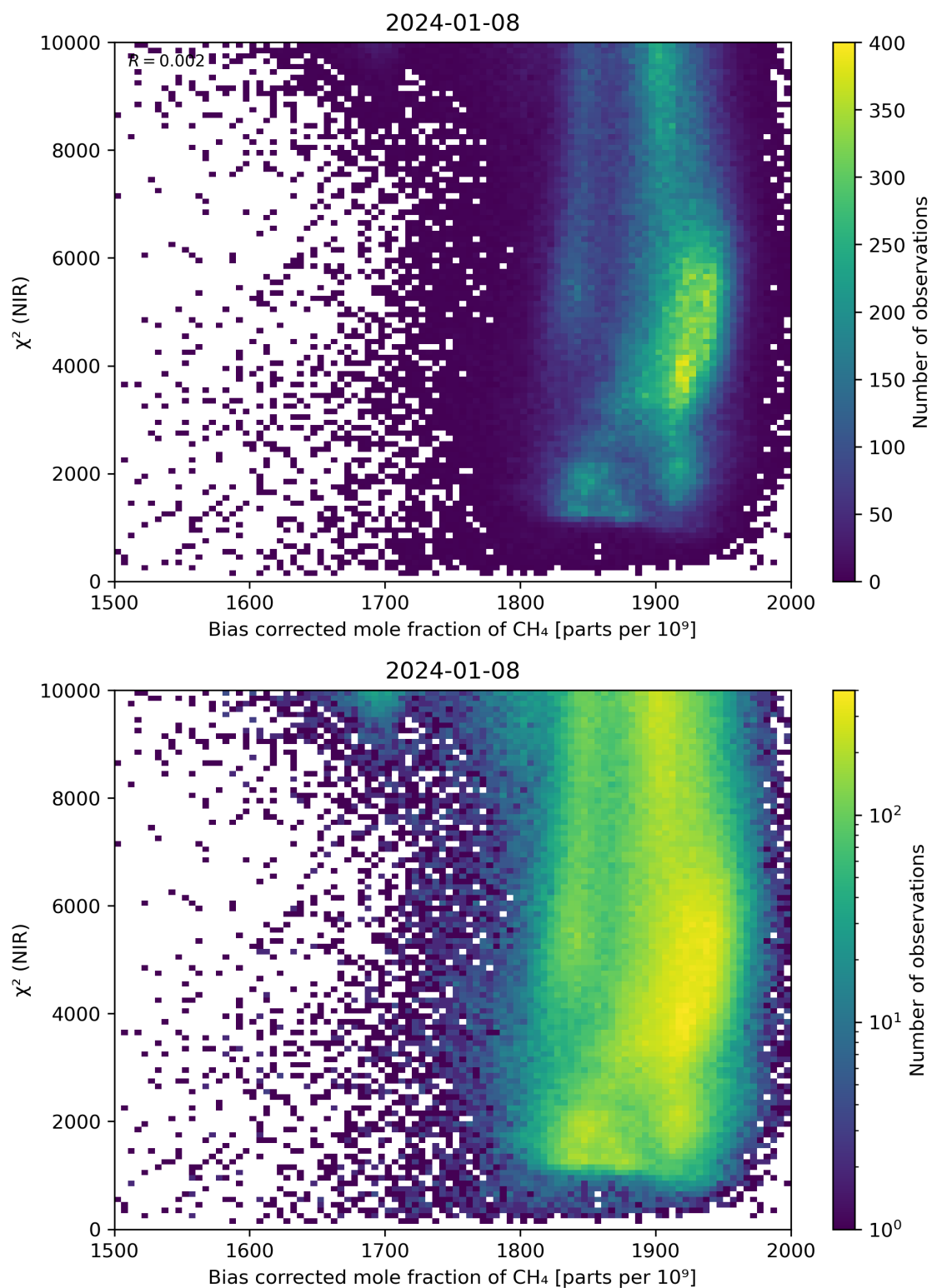
Figure 63: Scatter density plot of “Bias corrected mole fraction of CH 4 ” against “ \chi^2 (NIR)” for 2024-01-07 to 2024-01-09.
