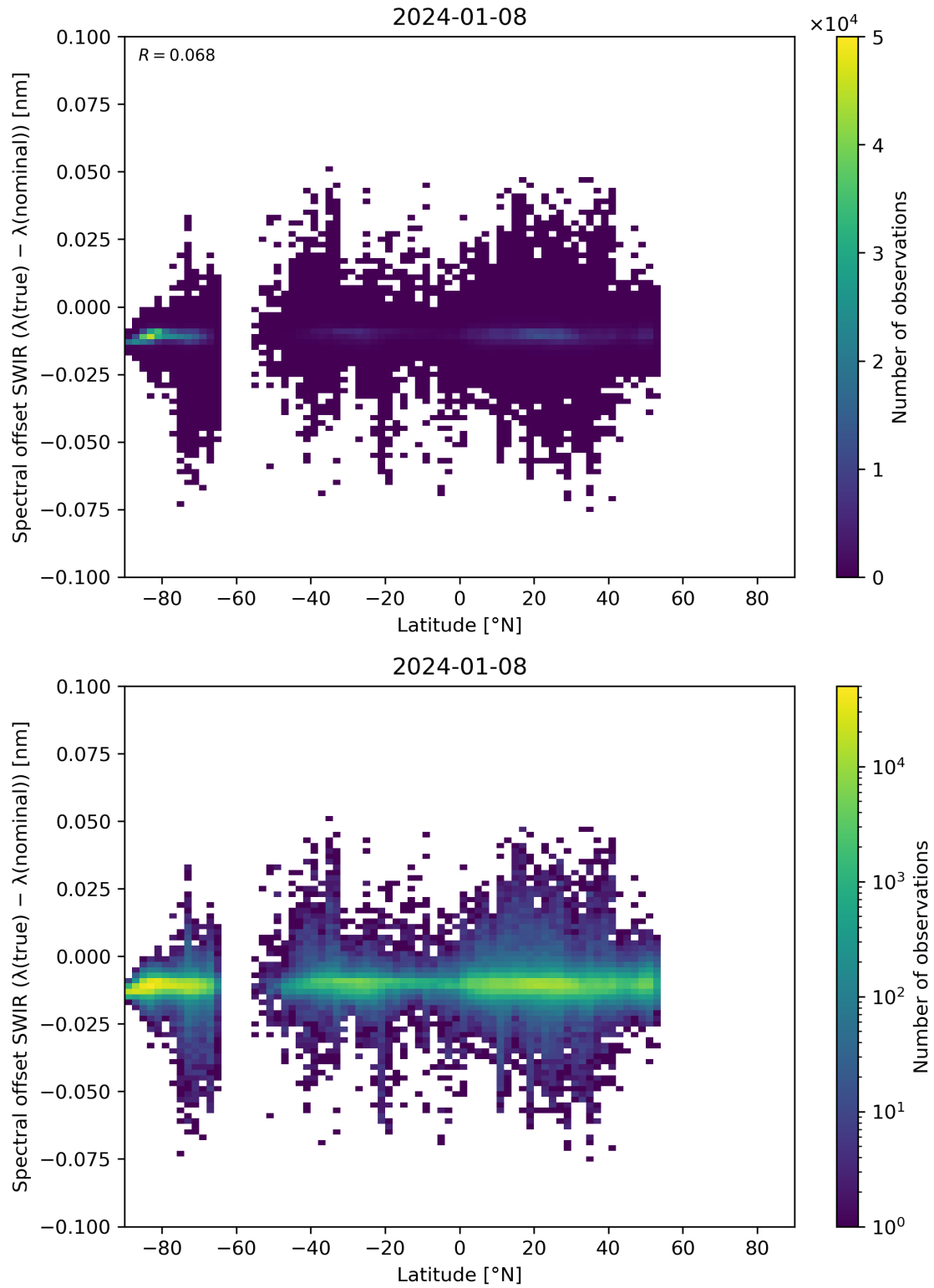
Figure 62: Scatter density plot of “Latitude” against “Spectral offset SWIR ( \lambda(\text{true}) - \lambda(\text{nominal}) )” for 2024-01-07 to 2024-01-09.
