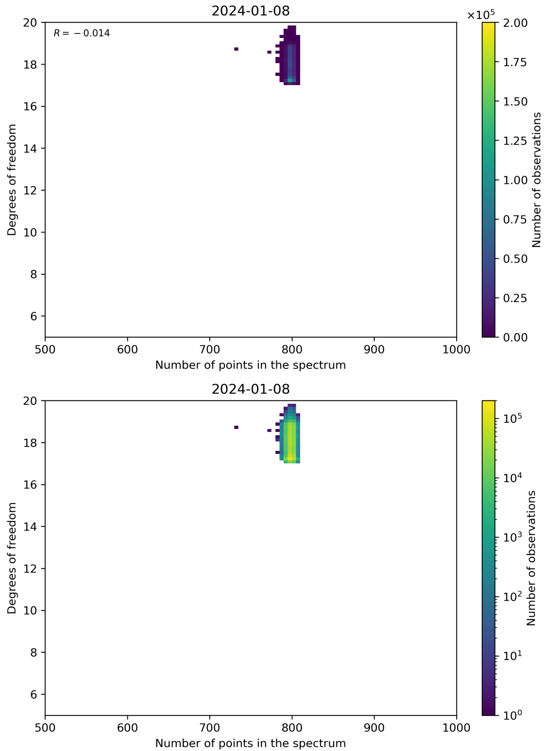
Figure 90: Scatter density plot of “Number of points in the spectrum” against “Degrees of freedom” for 2024-01-07 to 2024-01-09.
