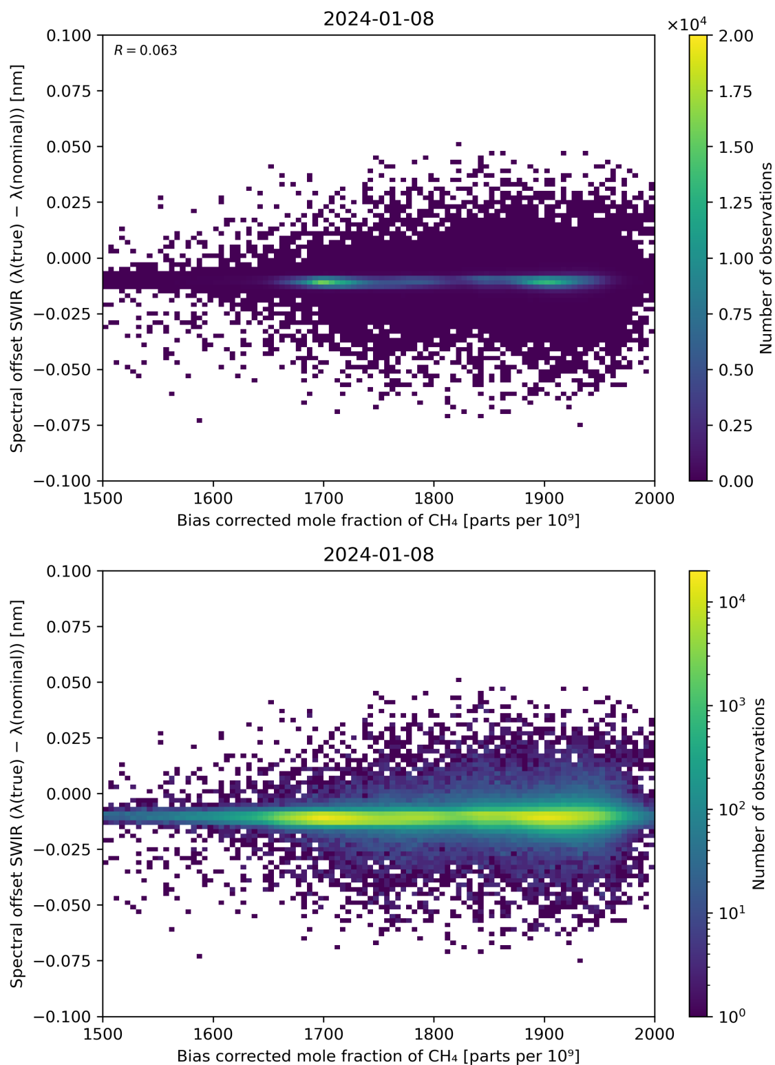
Figure 69: Scatter density plot of “Bias corrected mole fraction of \text{CH}_4 ” against “Spectral offset SWIR ( \lambda(\text{true}) - \lambda(\text{nominal}) )” for 2024-01-07 to 2024-01-09.
