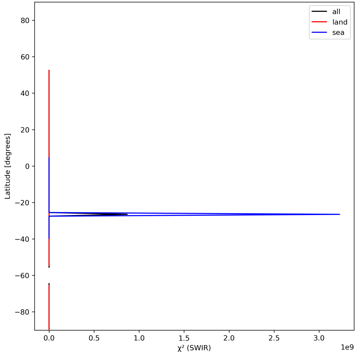
Figure 17: Zonal average of “ \chi^2 (SWIR)” for 2024-01-07 to 2024-01-09.
