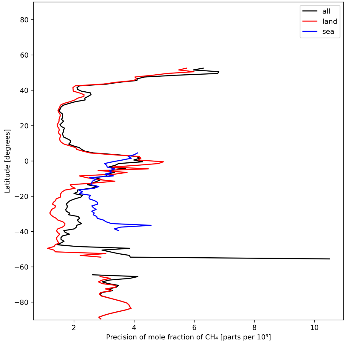
Figure 13: Zonal average of “Precision of mole fraction of CH 4 ” for 2024-01-07 to 2024-01-09.
