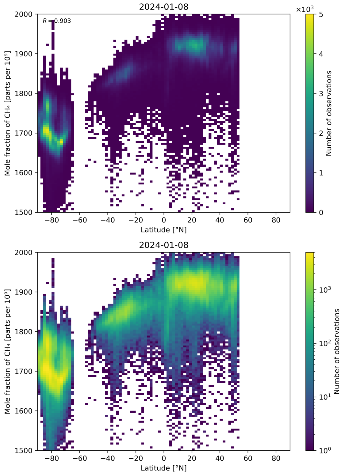
Figure 57: Scatter density plot of “Latitude” against “Mole fraction of CH 4 ” for 2024-01-07 to 2024-01-09.
