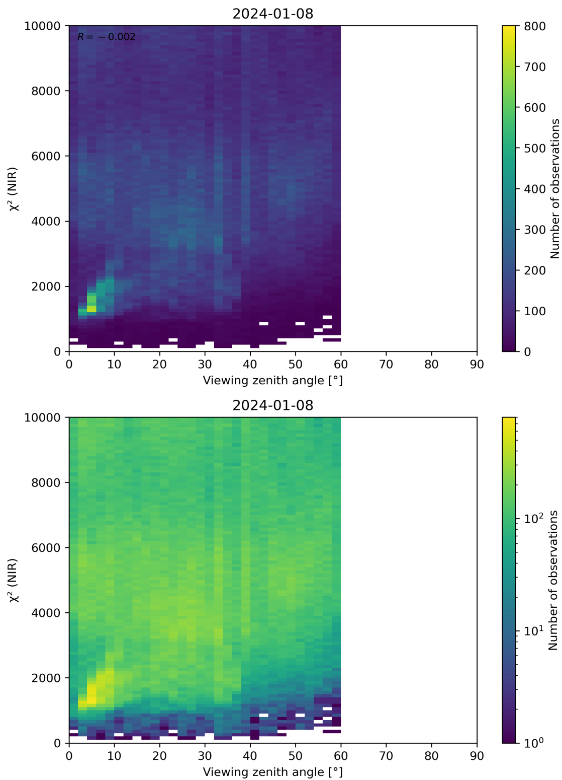
Figure 105: Scatter density plot of “Viewing zenith angle” against “ \chi^2 (NIR)” for 2024-01-07 to 2024-01-09.
