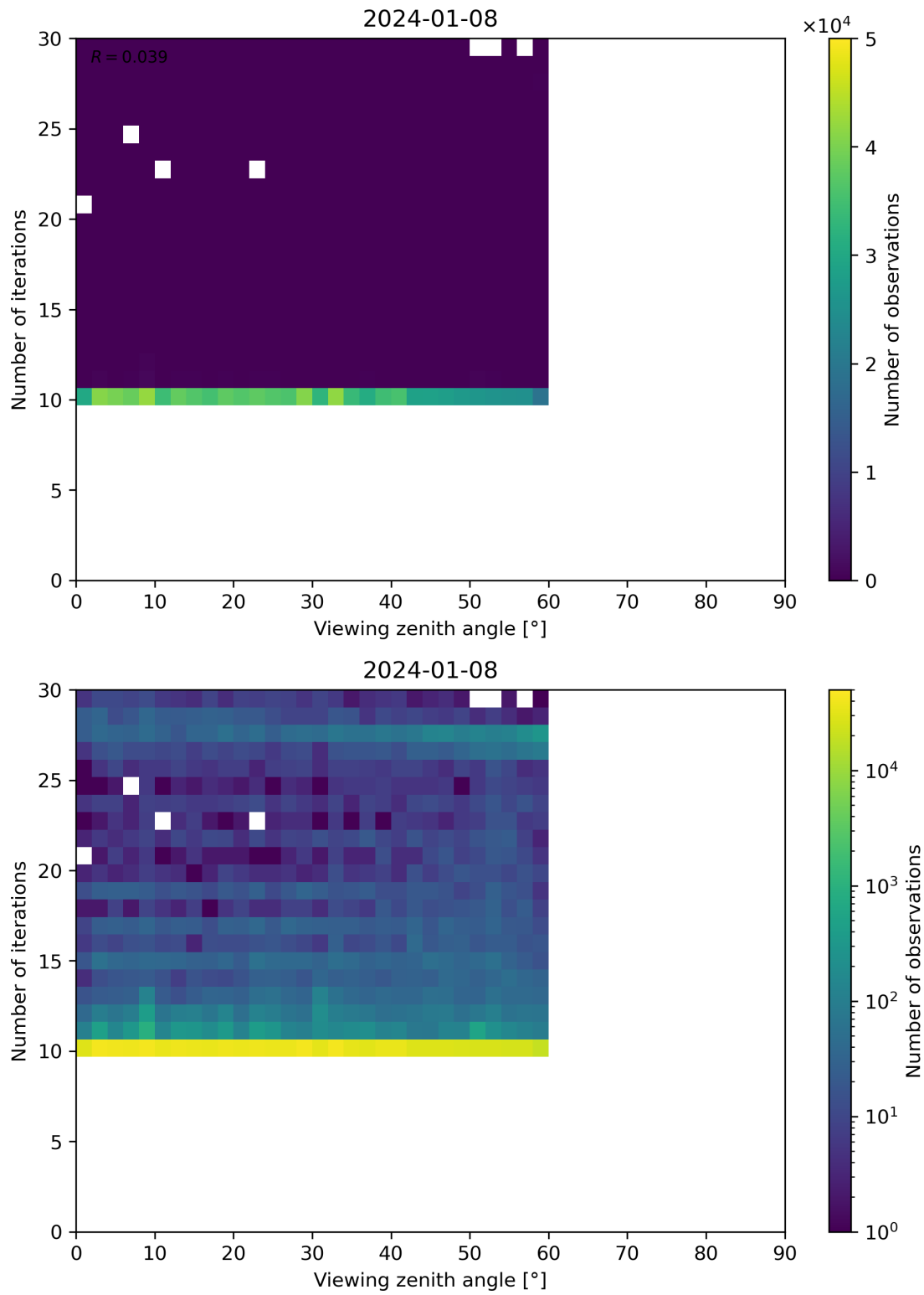
Figure 113: Scatter density plot of “Viewing zenith angle” against “Number of iterations” for 2024-01-07 to 2024-01-09.
