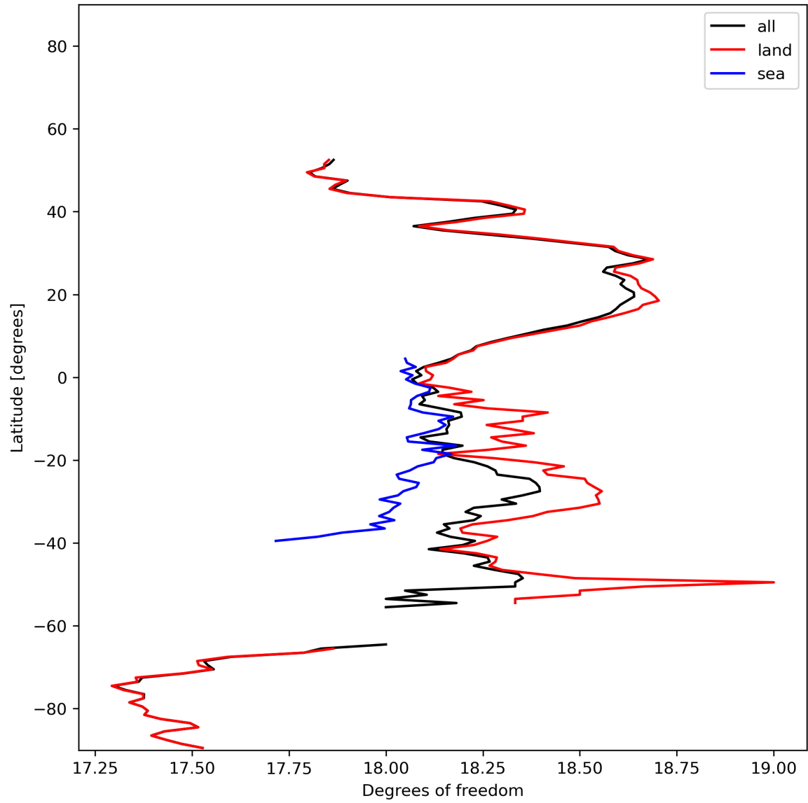
Figure 19: Zonal average of “Degrees of freedom” for 2024-01-07 to 2024-01-09.
