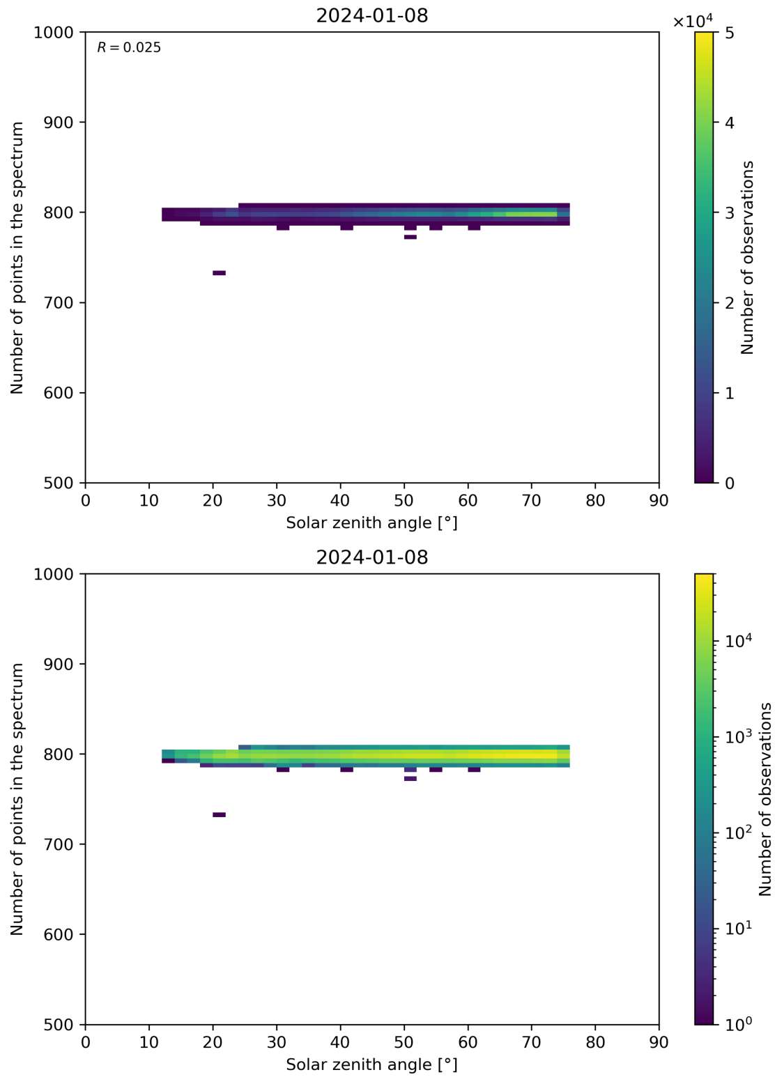
Figure 103: Scatter density plot of “Solar zenith angle” against “Number of points in the spectrum” for 2024-01-07 to 2024-01-09.
