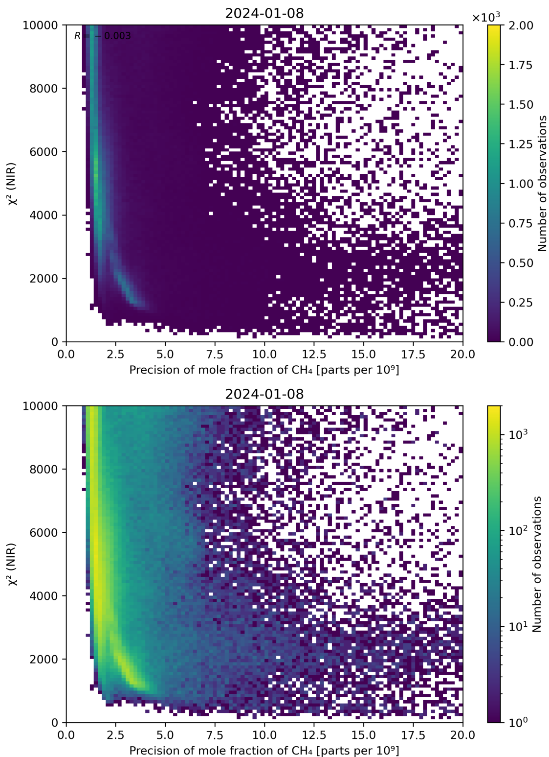
Figure 78: Scatter density plot of “Precision of mole fraction of CH 4 ” against “ \chi^2 (NIR)” for 2024-01-07 to 2024-01-09.
