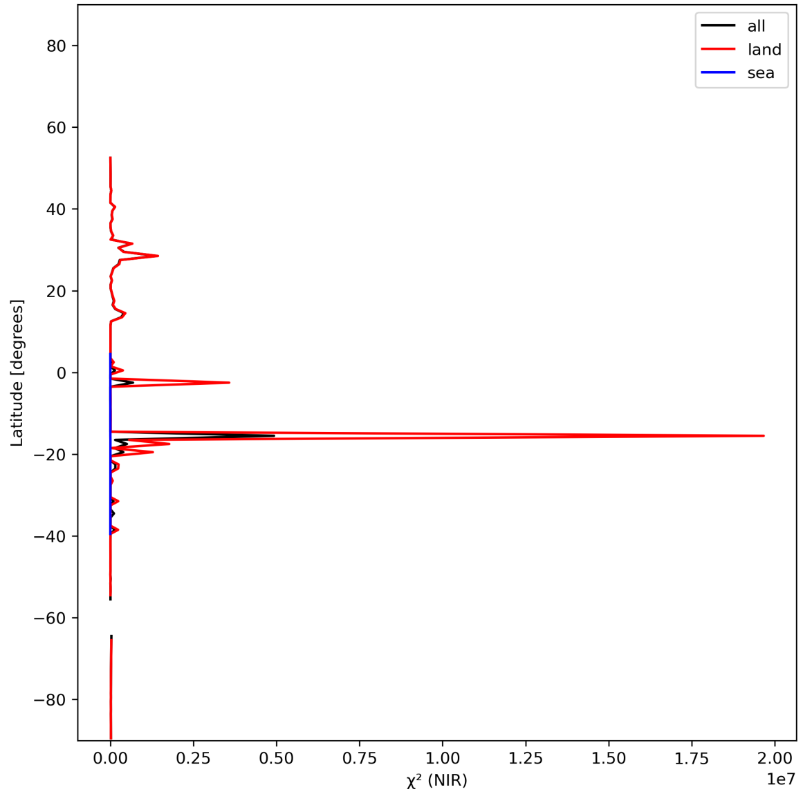
Figure 18: Zonal average of “ \chi^2 (NIR)” for 2024-01-07 to 2024-01-09.
