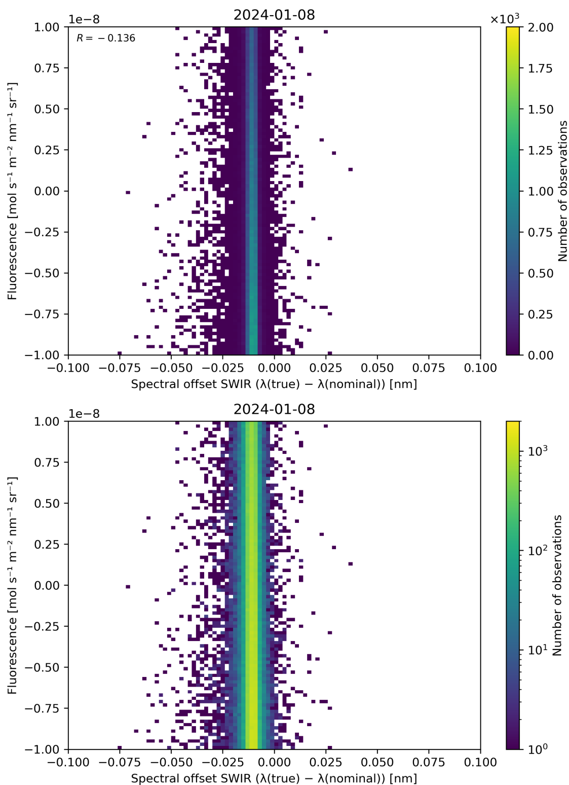
Figure 120: Scatter density plot of “Spectral offset SWIR ( \lambda(\text{true}) - \lambda(\text{nominal}) )” against “Fluorescence” for 2024-01-07 to 2024-01-09.
