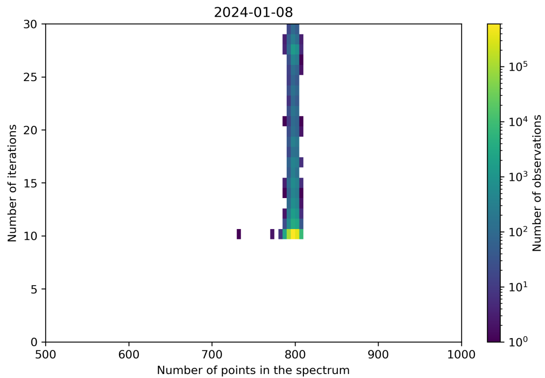
Figure 92: Scatter density plot of “Number of points in the spectrum” against “Number of iterations” for 2024-01-07 to 2024-01-09.
