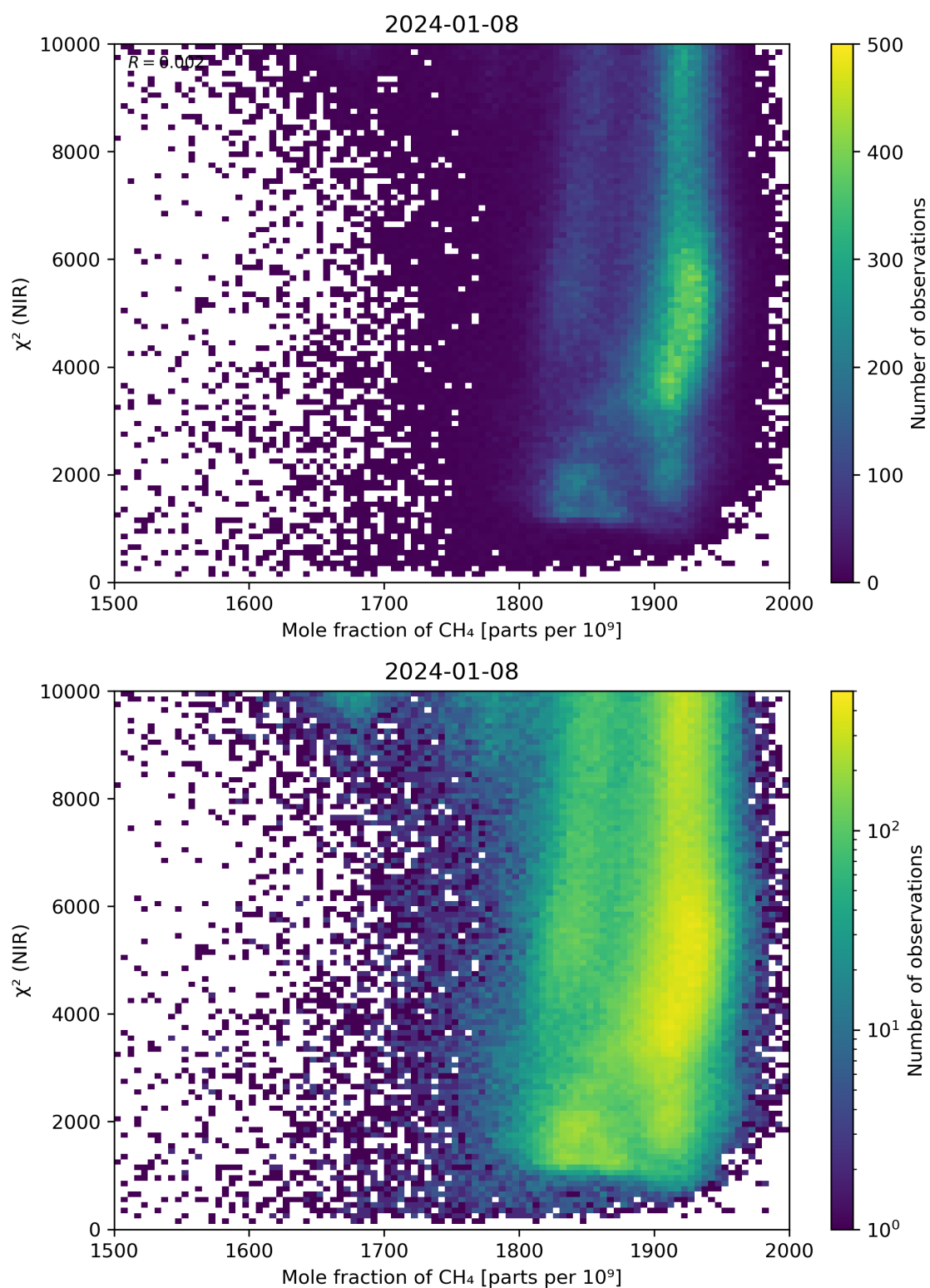
Figure 70: Scatter density plot of “Mole fraction of \text{CH}_4 ” against “ \chi^2 (NIR)” for 2024-01-07 to 2024-01-09.
