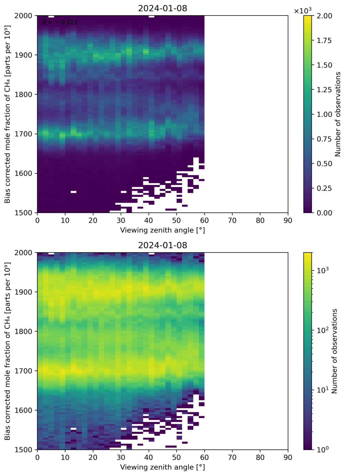
Figure 111: Scatter density plot of “Viewing zenith angle” against “Bias corrected mole fraction of CH 4 ” for 2024-01-07 to 2024-01-09.
