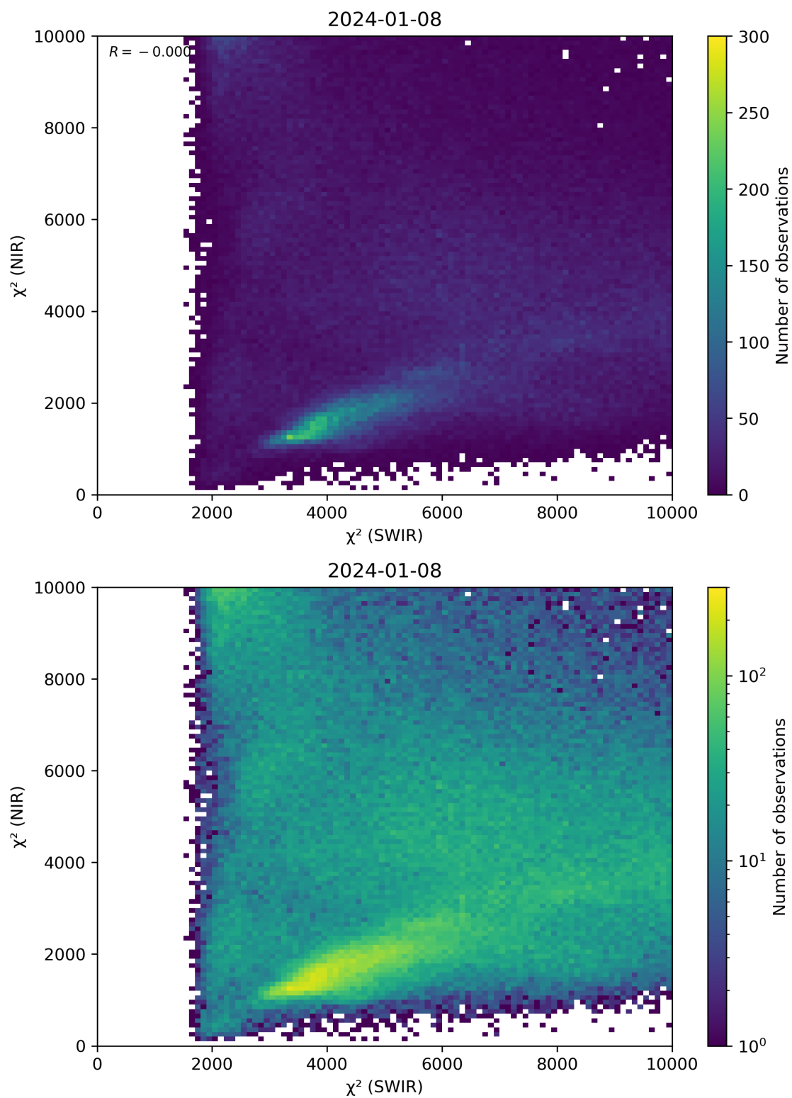
Figure 47: Scatter density plot of “ \chi^2 (SWIR)” against “ \chi^2 (NIR)” for 2024-01-07 to 2024-01-09.
