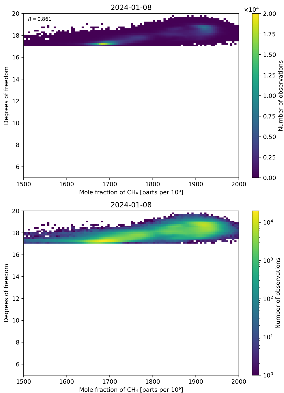
Figure 72: Scatter density plot of “Mole fraction of CH 4 ” against “Degrees of freedom” for 2024-01-07 to 2024-01-09.
