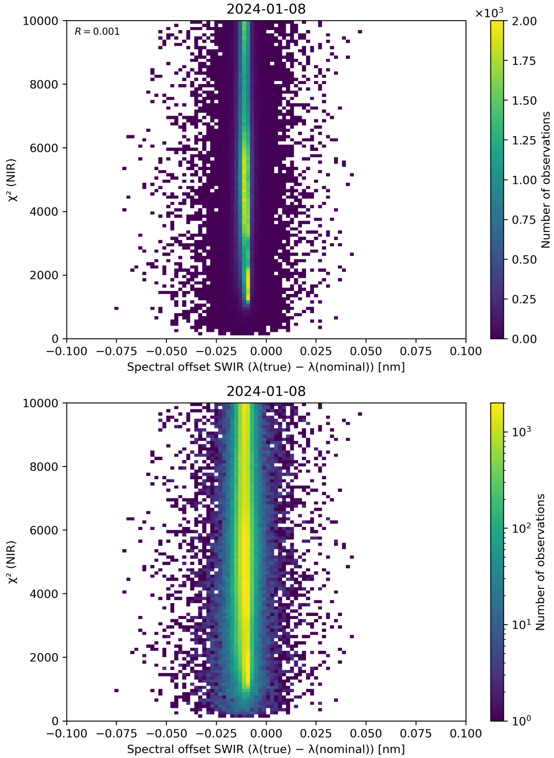
Figure 117: Scatter density plot of “Spectral offset SWIR ( \lambda(\text{true}) - \lambda(\text{nominal}) )” against “ \chi^2 (NIR)” for 2024-01-07 to 2024-01-09.
