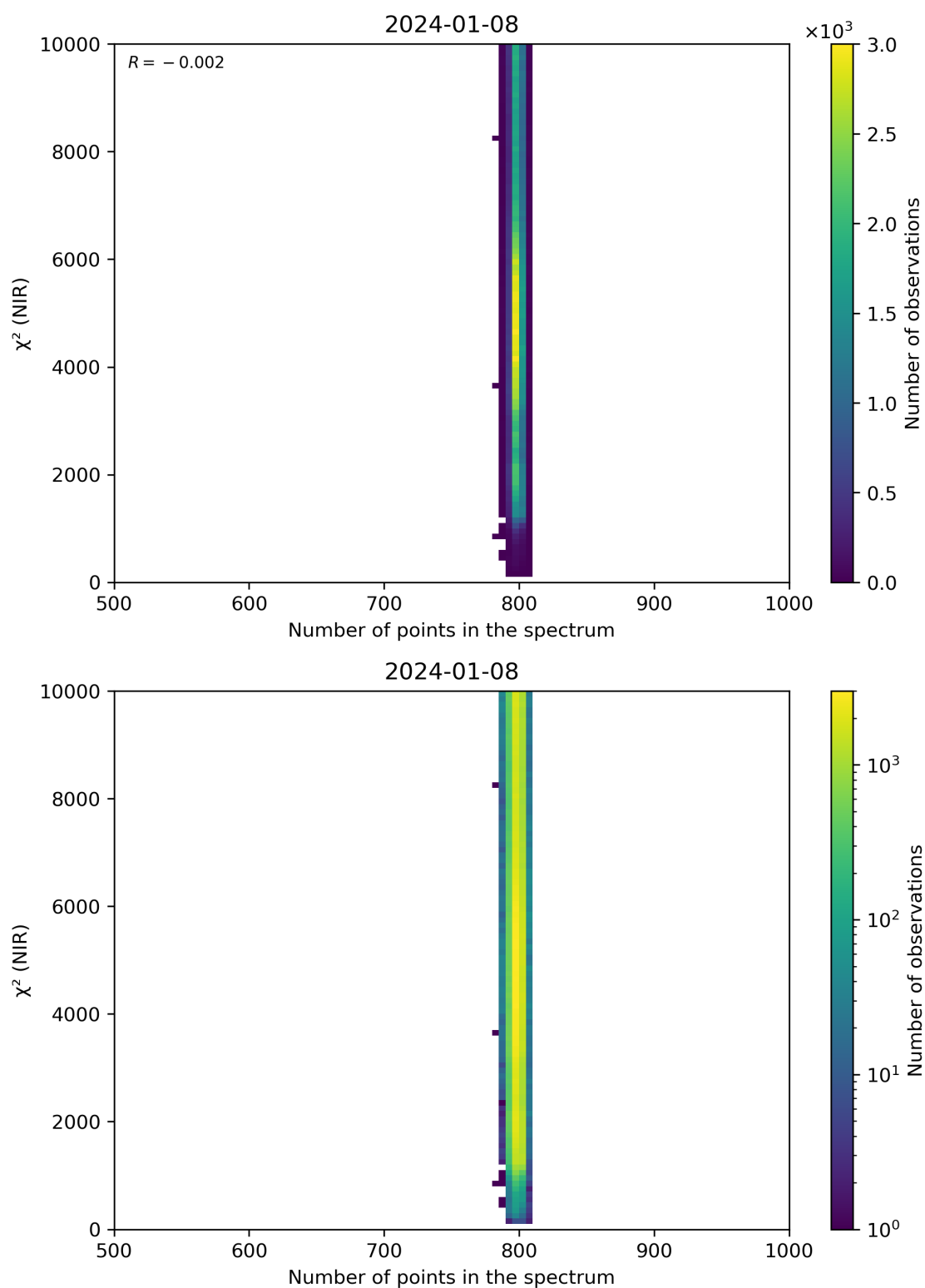
Figure 88: Scatter density plot of “Number of points in the spectrum” against “ \chi^2 (NIR)” for 2024-01-07 to 2024-01-09.
