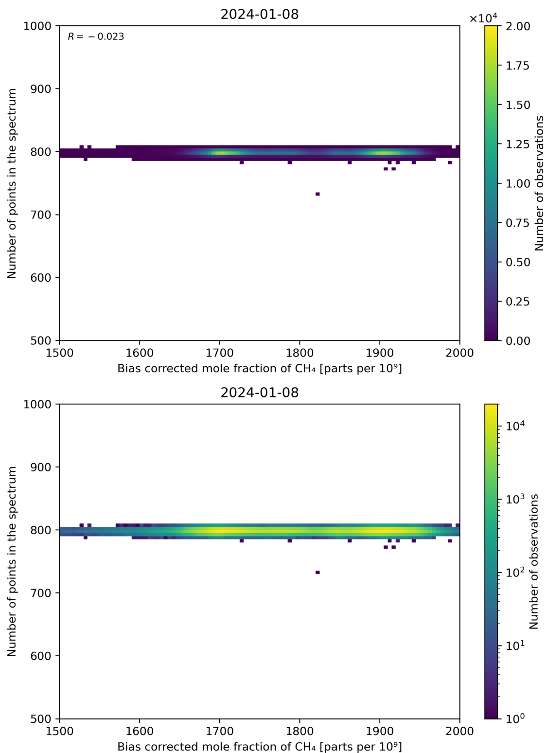
Figure 68: Scatter density plot of “Bias corrected mole fraction of CH 4 ” against “Number of points in the spectrum” for 2024-01-07 to 2024-01-09.
