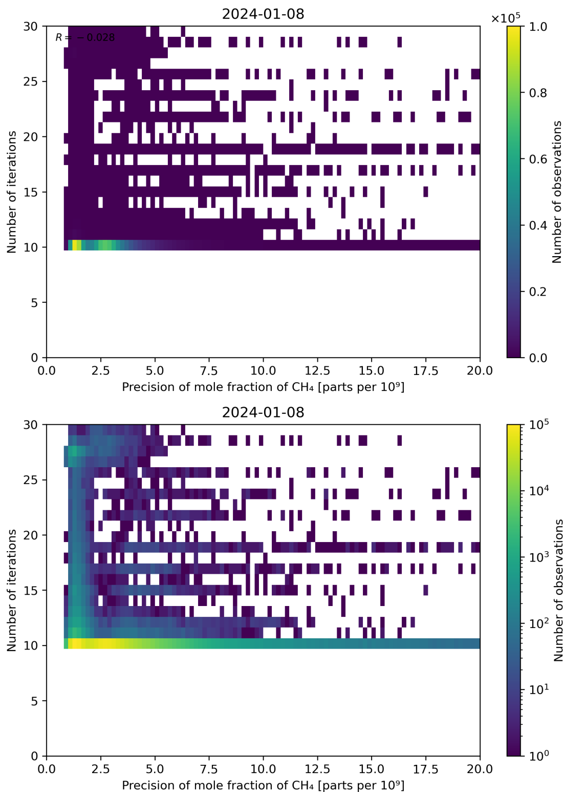
Figure 83: Scatter density plot of “Precision of mole fraction of CH 4 ” against “Number of iterations” for 2024-01-07 to 2024-01-09.
