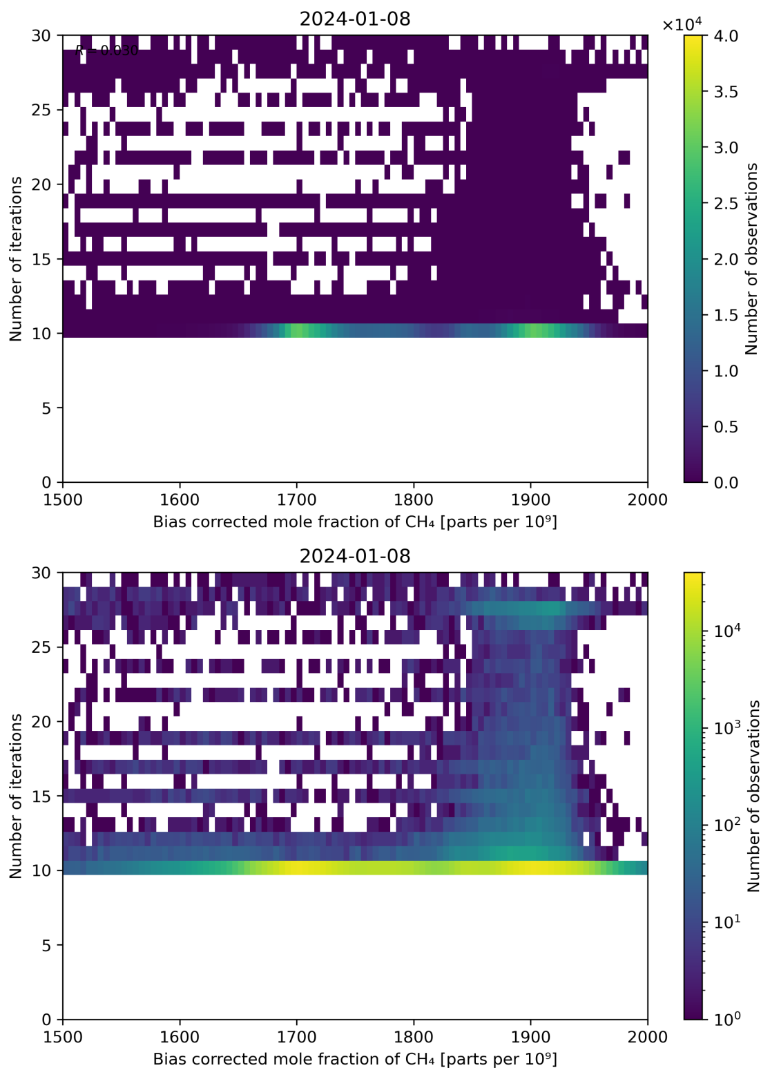
Figure 67: Scatter density plot of “Bias corrected mole fraction of CH 4 ” against “Number of iterations” for 2024-01-07 to 2024-01-09.
