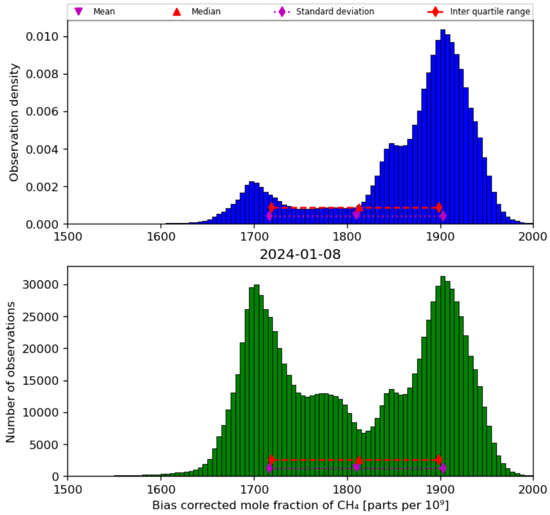
Figure 25: Histogram of “Bias corrected mole fraction of CH 4 ” for 2024-01-07 to 2024-01-09
