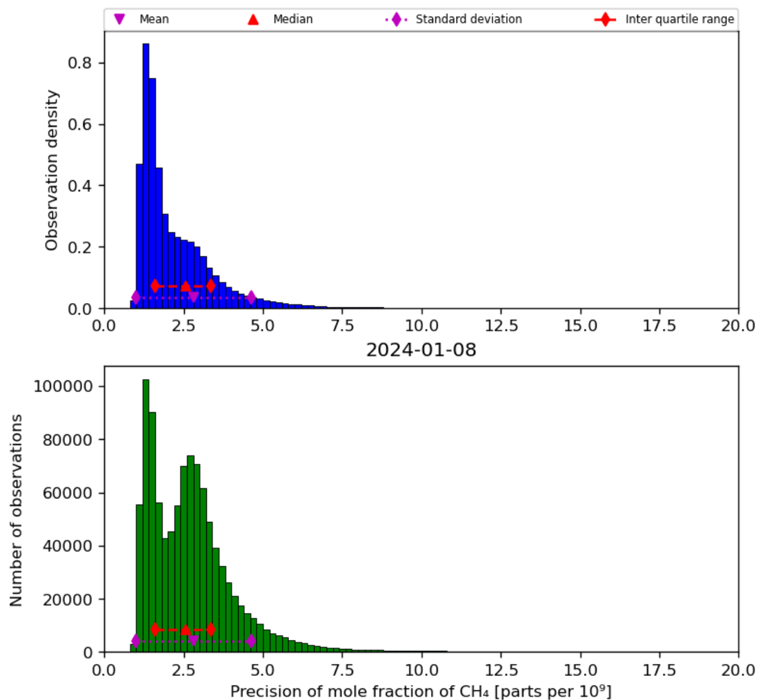
Figure 24: Histogram of “Precision of mole fraction of CH 4 ” for 2024-01-07 to 2024-01-09
