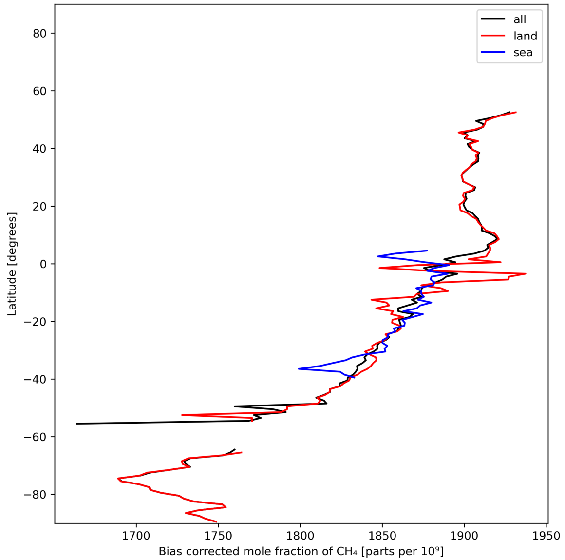
Figure 14: Zonal average of “Bias corrected mole fraction of CH 4 ” for 2024-01-07 to 2024-01-09.
