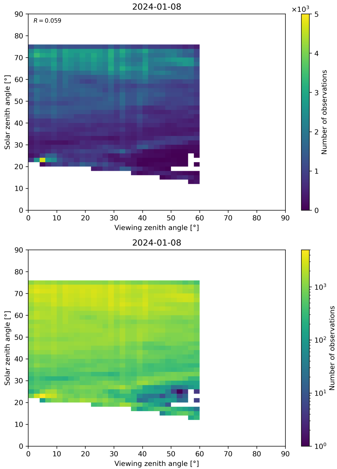
Figure 115: Scatter density plot of “Viewing zenith angle” against “Solar zenith angle” for 2024-01-07 to 2024-01-09.
