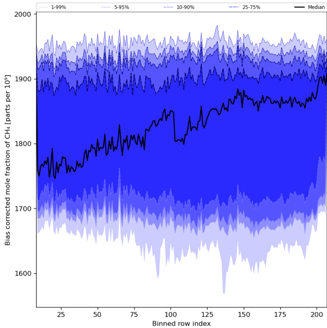
Figure 36: Along track statistics of “Bias corrected mole fraction of CH 4 ” for 2024-01-07 to 2024-01-09
