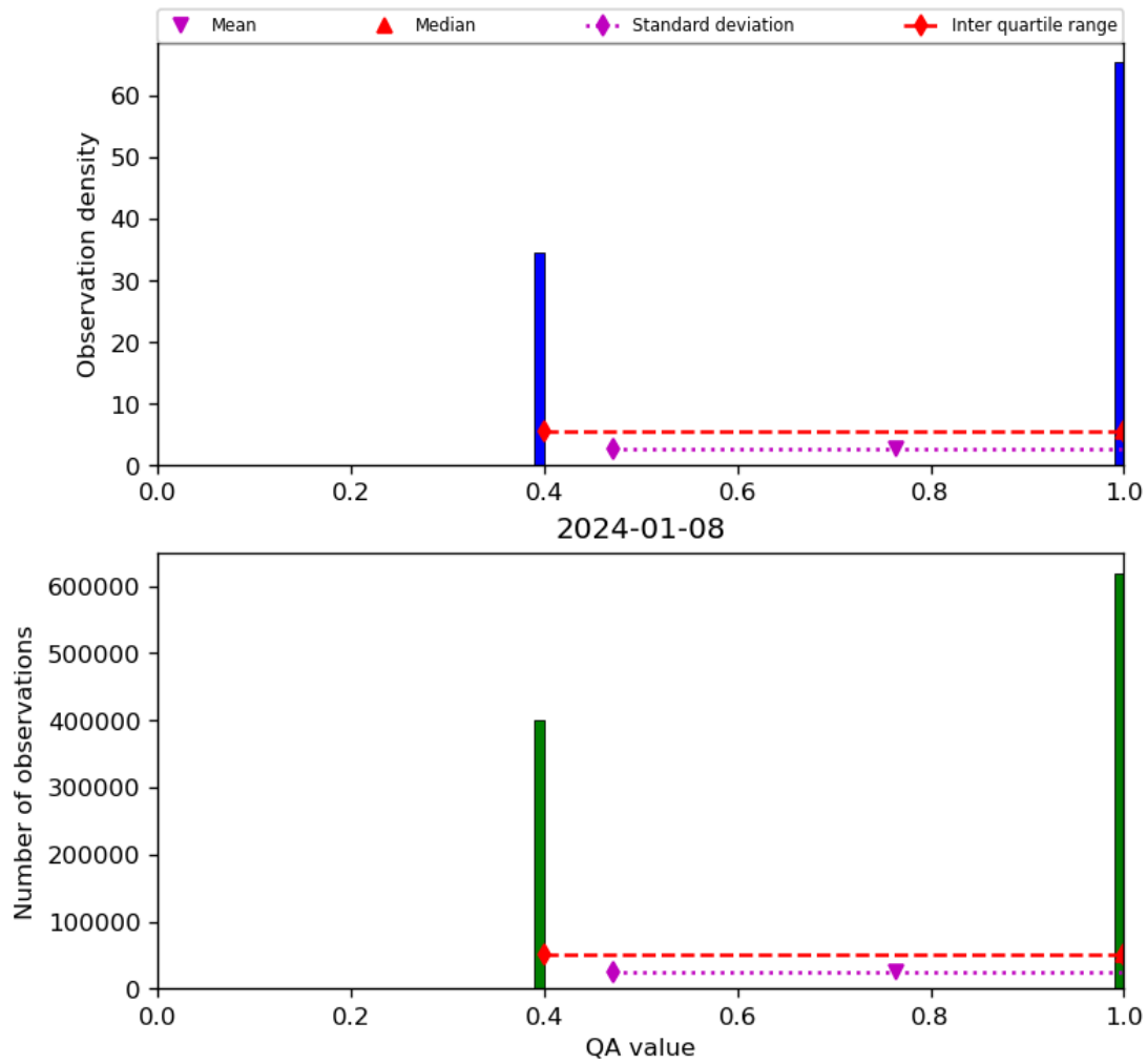
Figure 22: Histogram of “QA value” for 2024-01-07 to 2024-01-09
