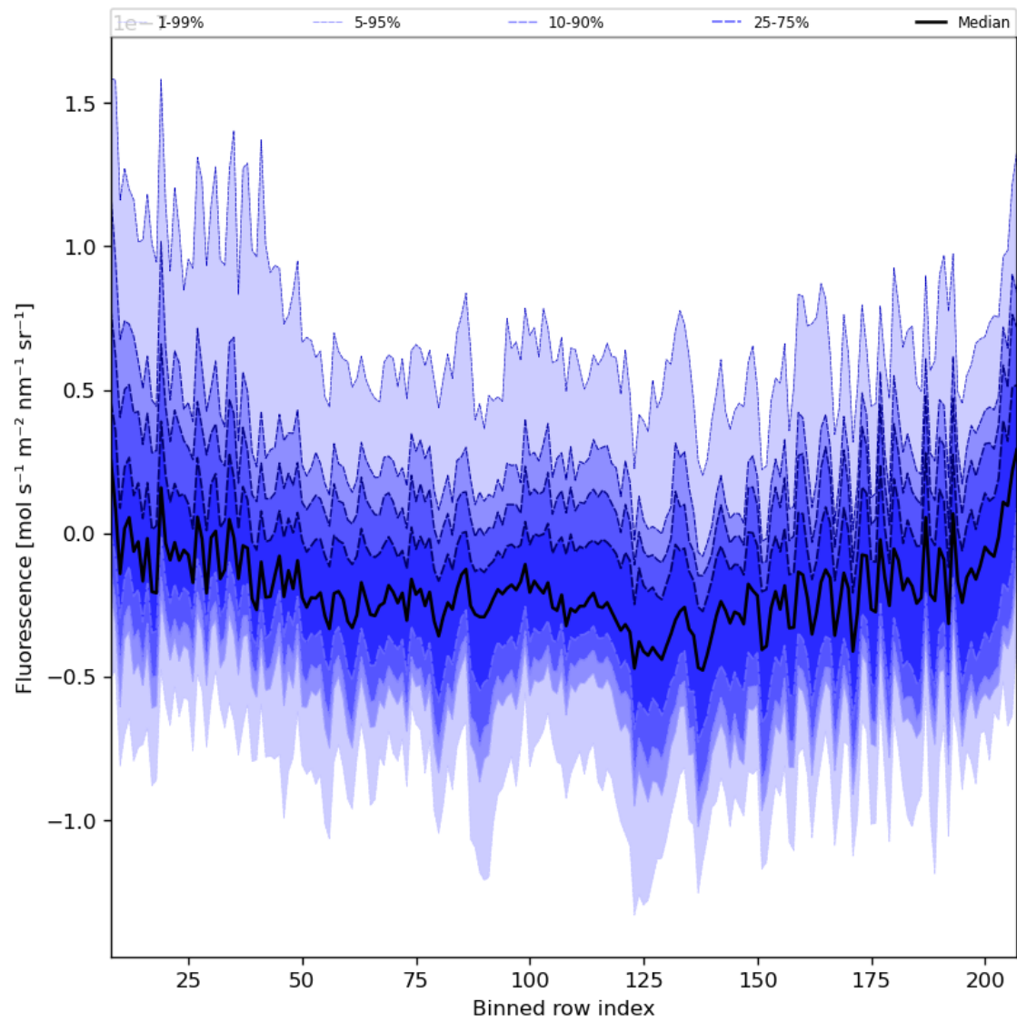
Figure 43: Along track statistics of “Fluorescence” for 2024-01-07 to 2024-01-09
