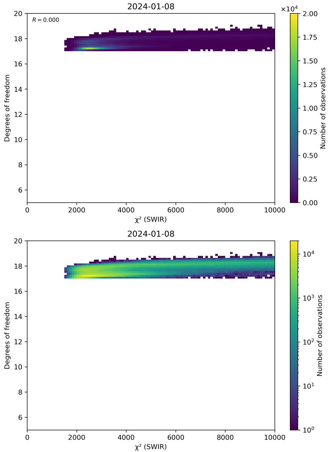
Figure 48: Scatter density plot of “ \chi^2 (SWIR)” against “Degrees of freedom” for 2024-01-07 to 2024-01-09.
