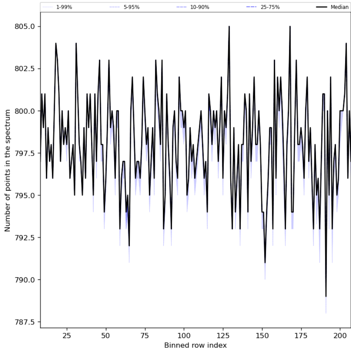
Figure 37: Along track statistics of “Number of points in the spectrum” for 2024-01-07 to 2024-01-09
