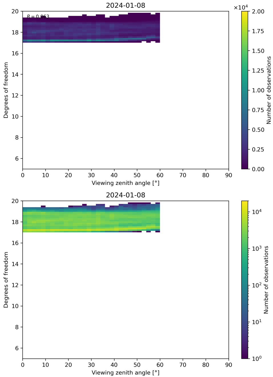
Figure 107: Scatter density plot of “Viewing zenith angle” against “Degrees of freedom” for 2024-01-07 to 2024-01-09.
