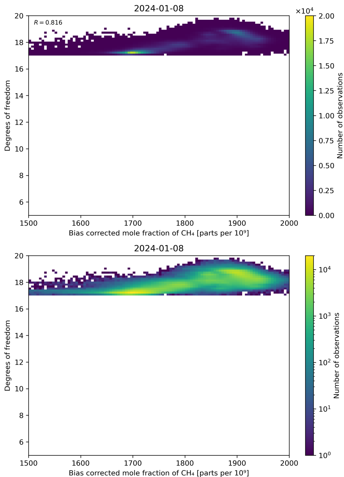
Figure 65: Scatter density plot of “Bias corrected mole fraction of CH 4 ” against “Degrees of freedom” for 2024-01-07 to 2024-01-09.
