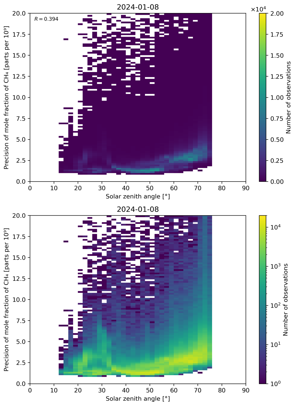
Figure 101: Scatter density plot of “Solar zenith angle” against “Precision of mole fraction of \text{CH}_4 ” for 2024-01-07 to 2024-01-09.
