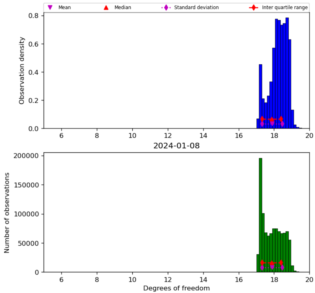
Figure 30: Histogram of “Degrees of freedom” for 2024-01-07 to 2024-01-09
