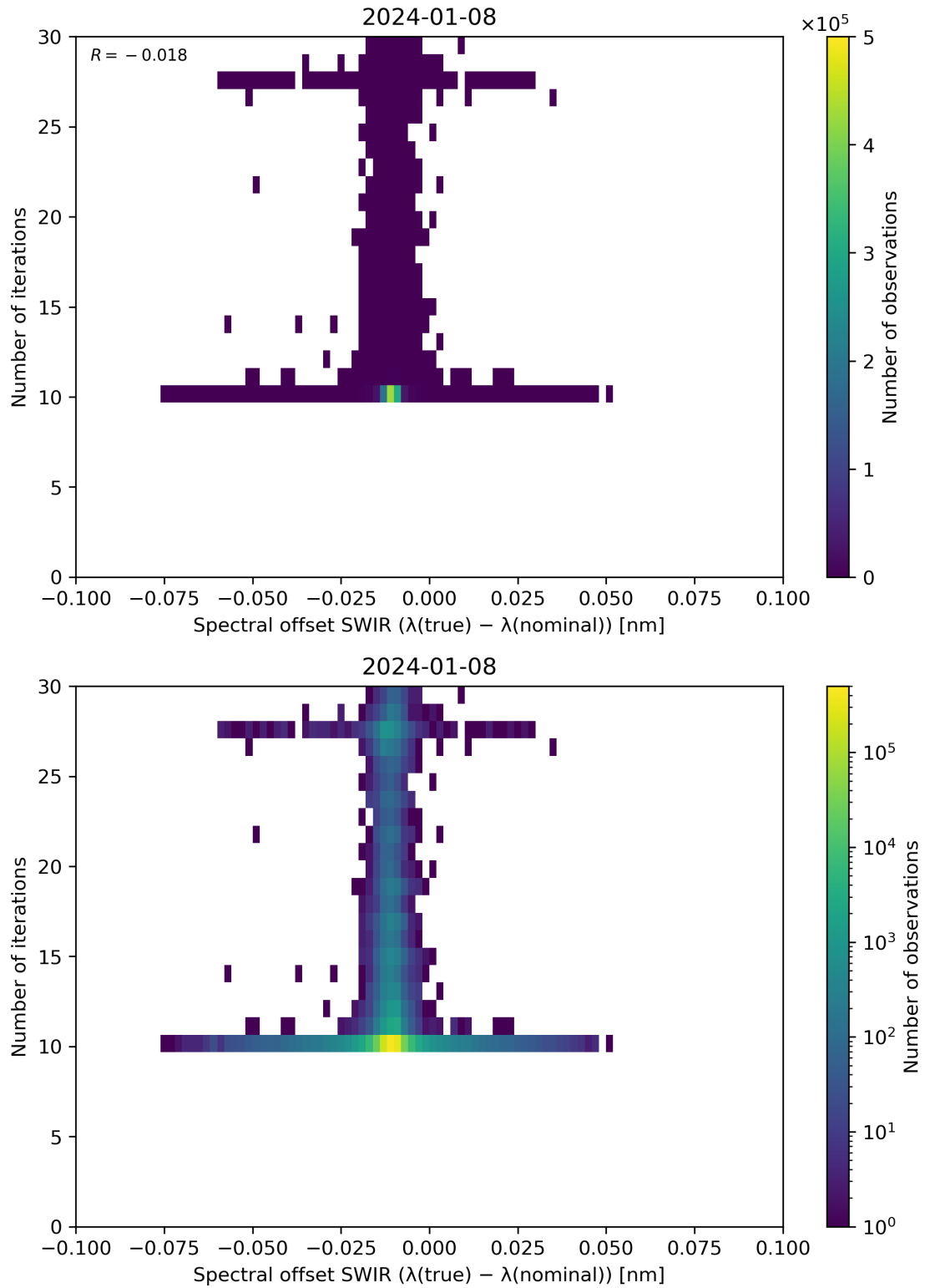
Figure 121: Scatter density plot of “Spectral offset SWIR ( \lambda(\text{true}) - \lambda(\text{nominal}) )” against “Number of iterations” for 2024-01-07 to 2024-01-09.
