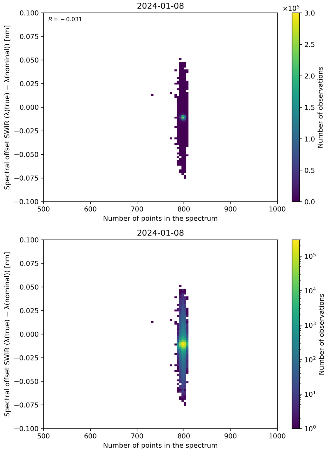
Figure 93: Scatter density plot of “Number of points in the spectrum” against “Spectral offset SWIR ( \lambda(\text{true}) - \lambda(\text{nominal}) )” for 2024-01-07 to 2024-01-09.
