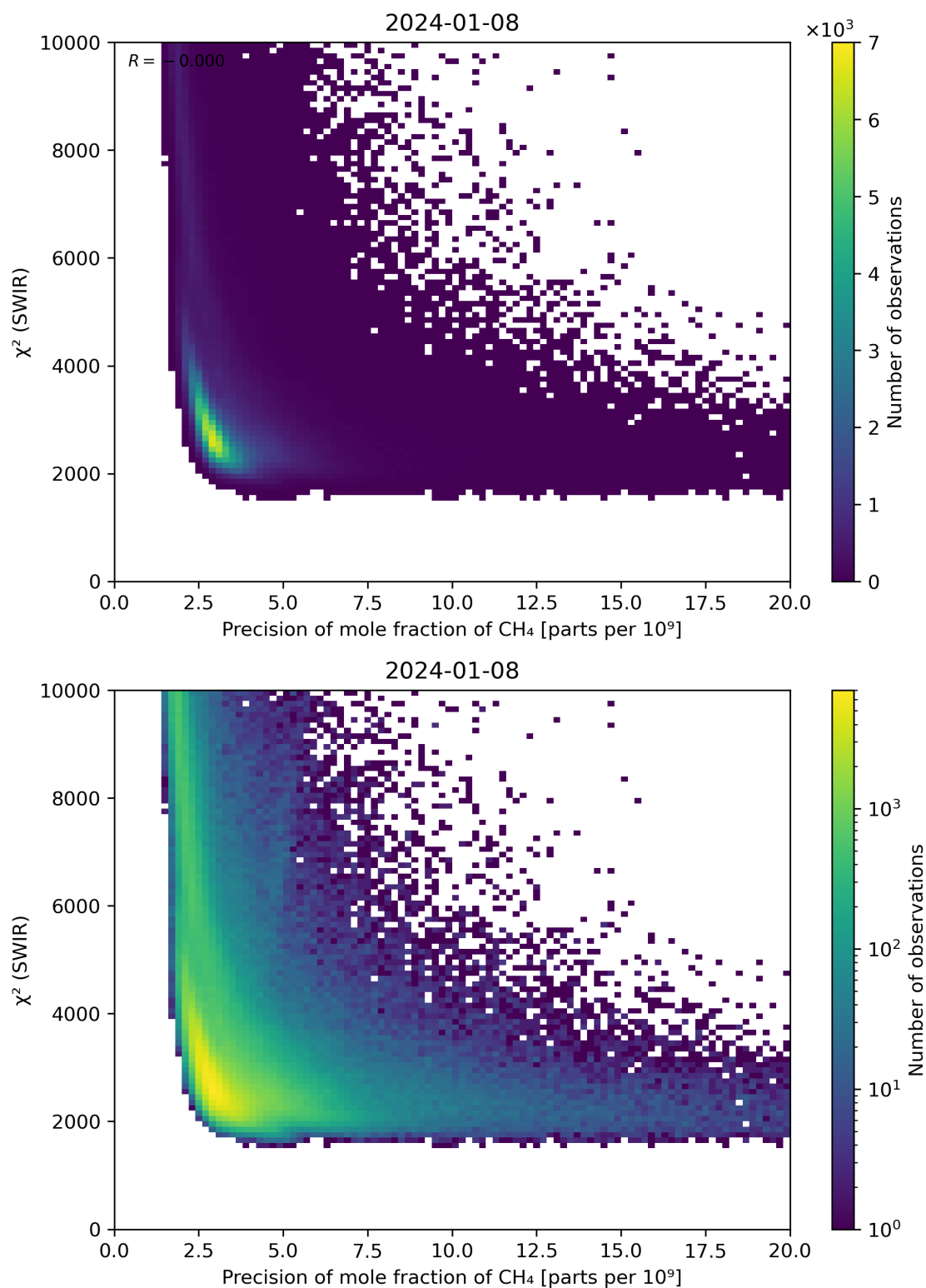
Figure 79: Scatter density plot of “Precision of mole fraction of \text{CH}_4 ” against “ \chi^2 (SWIR)” for 2024-01-07 to 2024-01-09.
