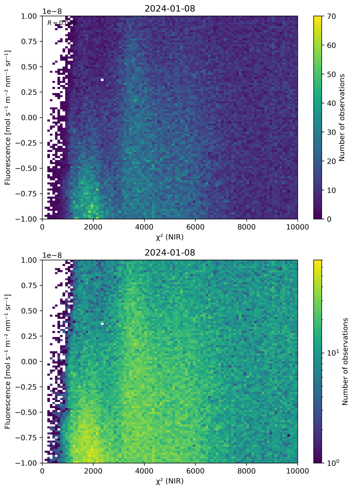
Figure 45: Scatter density plot of “ \chi^2 (NIR)” against “Fluorescence” for 2024-01-07 to 2024-01-09.
