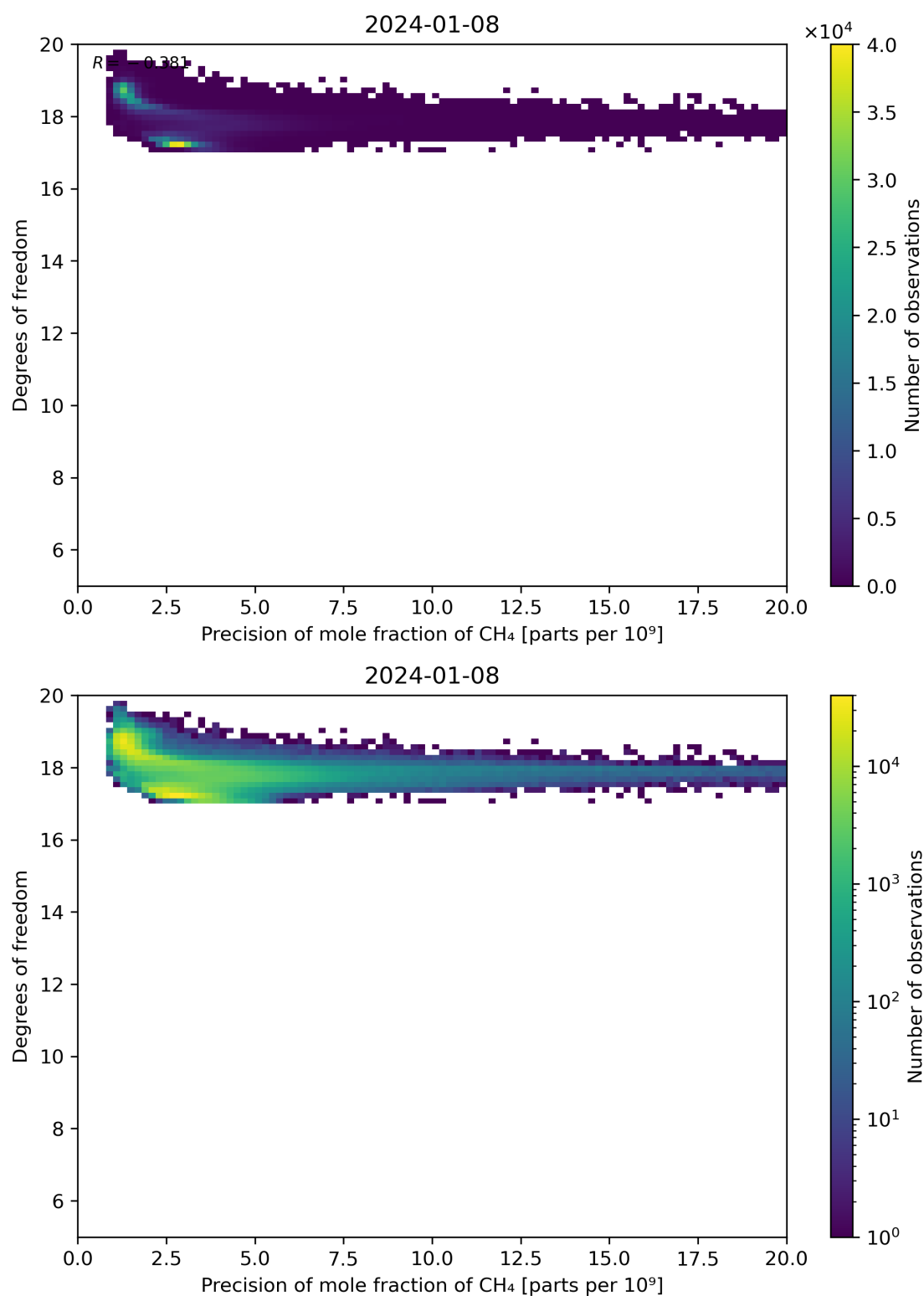
Figure 80: Scatter density plot of “Precision of mole fraction of CH 4 ” against “Degrees of freedom” for 2024-01-07 to 2024-01-09.
