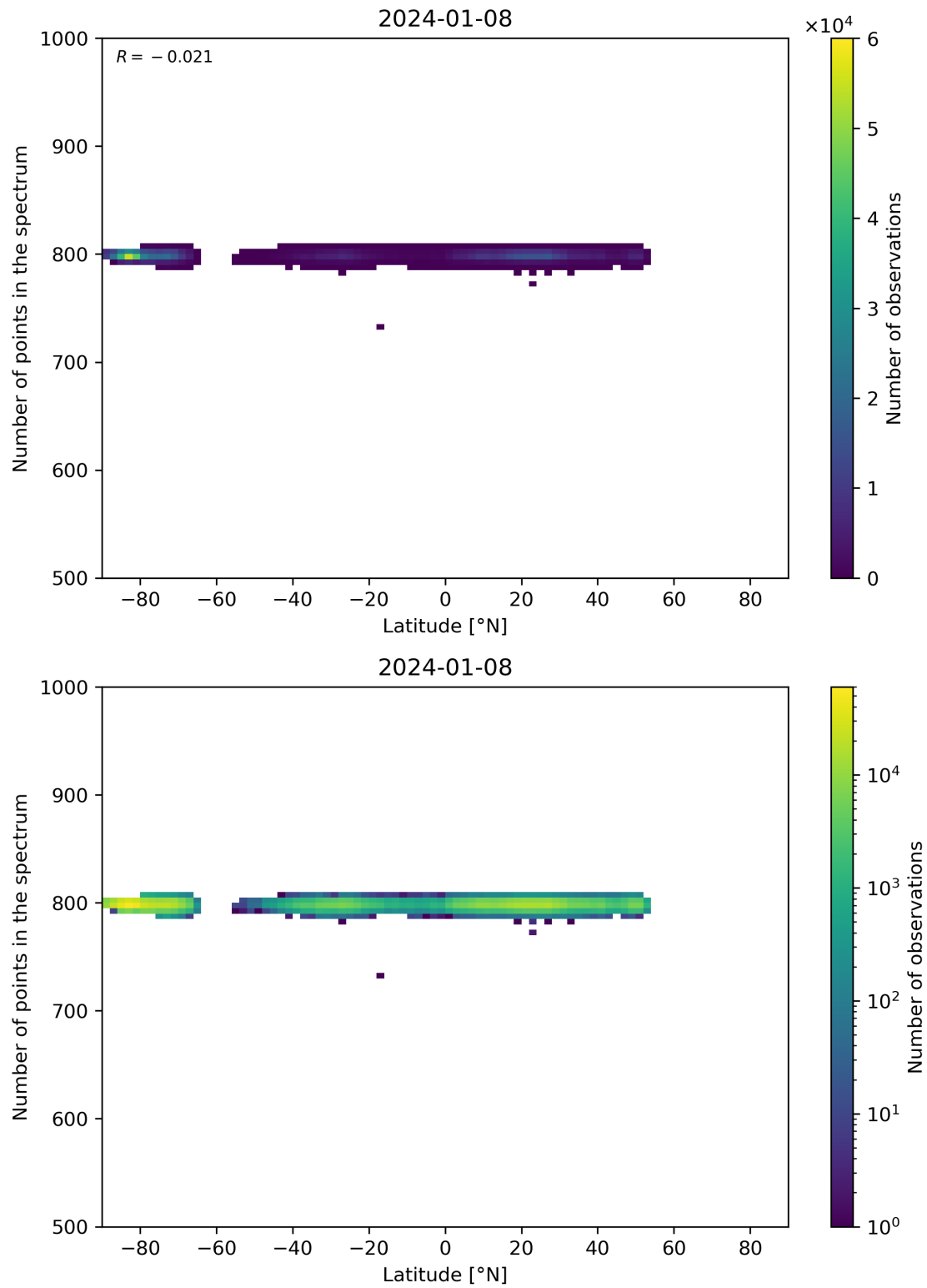
Figure 61: Scatter density plot of “Latitude” against “Number of points in the spectrum” for 2024-01-07 to 2024-01-09.
