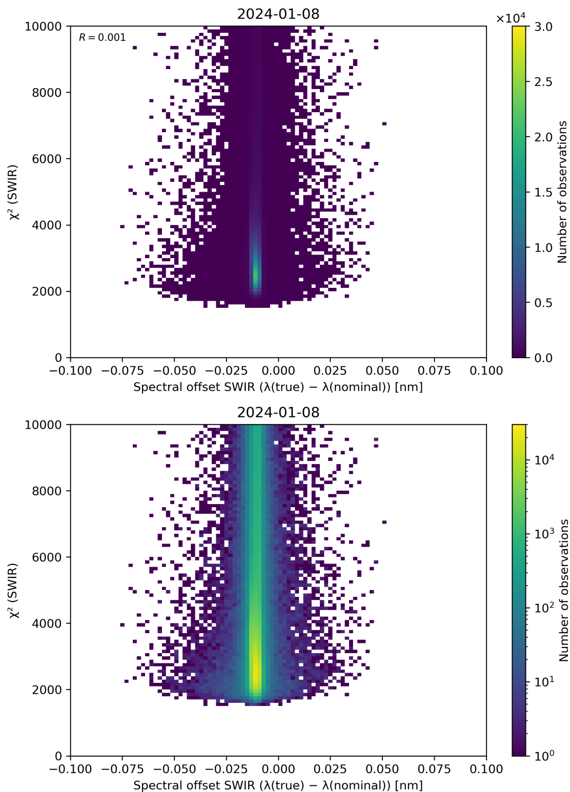
Figure 118: Scatter density plot of “Spectral offset SWIR ( \lambda(\text{true}) - \lambda(\text{nominal}) )” against “ \chi^2 (SWIR)” for 2024-01-07 to 2024-01-09.
