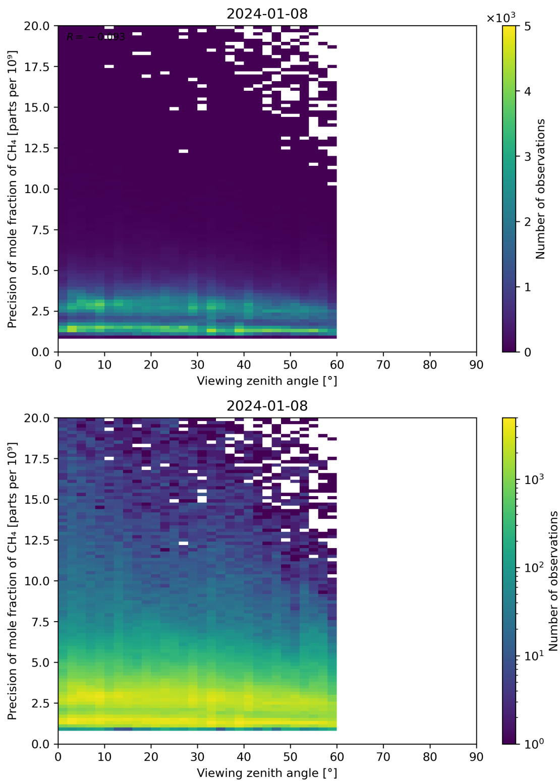
Figure 112: Scatter density plot of “Viewing zenith angle” against “Precision of mole fraction of CH 4 ” for 2024-01-07 to 2024-01-09.
