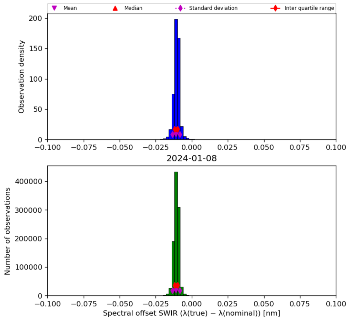
Figure 27: Histogram of “Spectral offset SWIR ( \lambda(\text{true}) - \lambda(\text{nominal}) )” for 2024-01-07 to 2024-01-09
