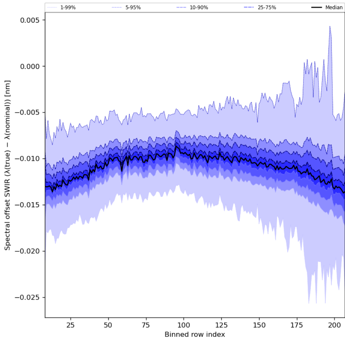
Figure 38: Along track statistics of “Spectral offset SWIR ( \lambda(\text{true}) - \lambda(\text{nominal}) )” for 2024-01-07 to 2024-01-09
