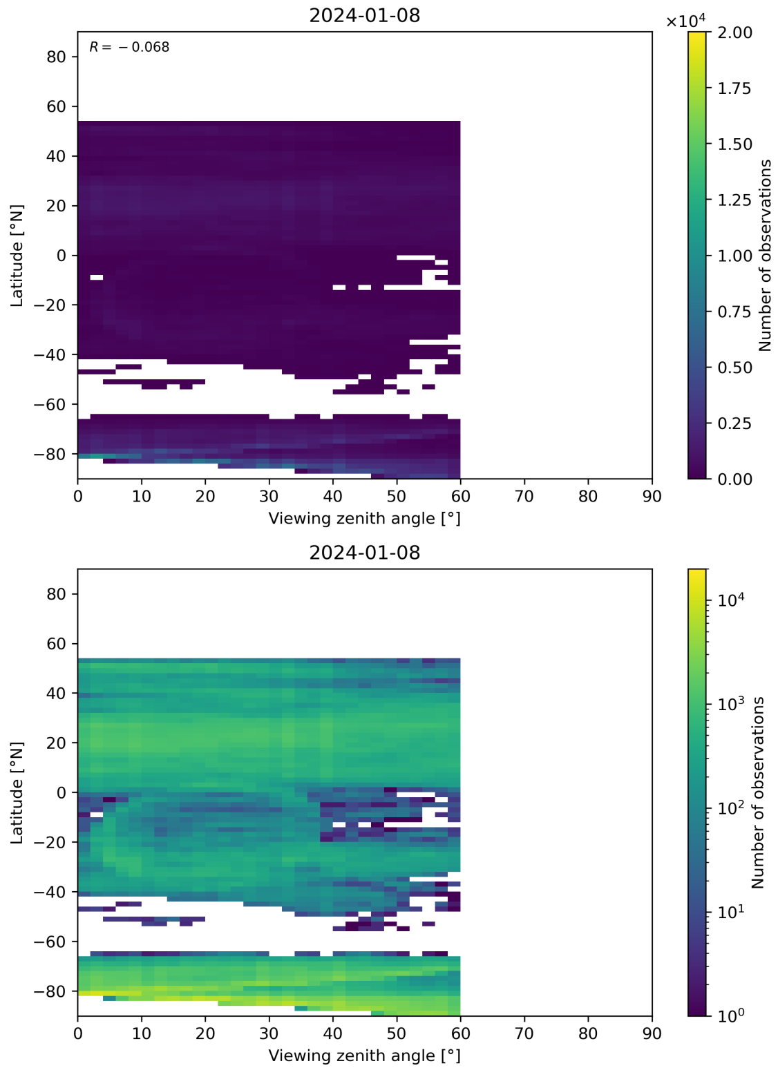
Figure 109: Scatter density plot of “Viewing zenith angle” against “Latitude” for 2024-01-07 to 2024-01-09.
