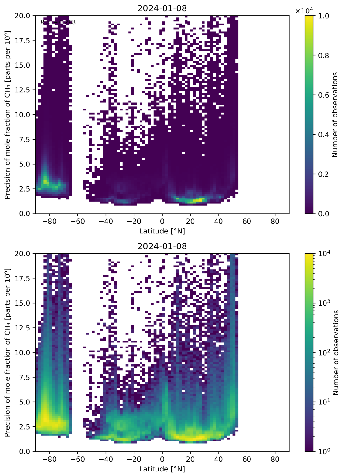
Figure 59: Scatter density plot of “Latitude” against “Precision of mole fraction of CH 4 ” for 2024-01-07 to 2024-01-09.
