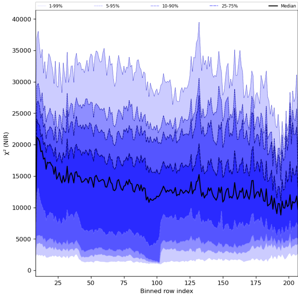
Figure 40: Along track statistics of “ \chi^2 (NIR)” for 2024-01-07 to 2024-01-09
