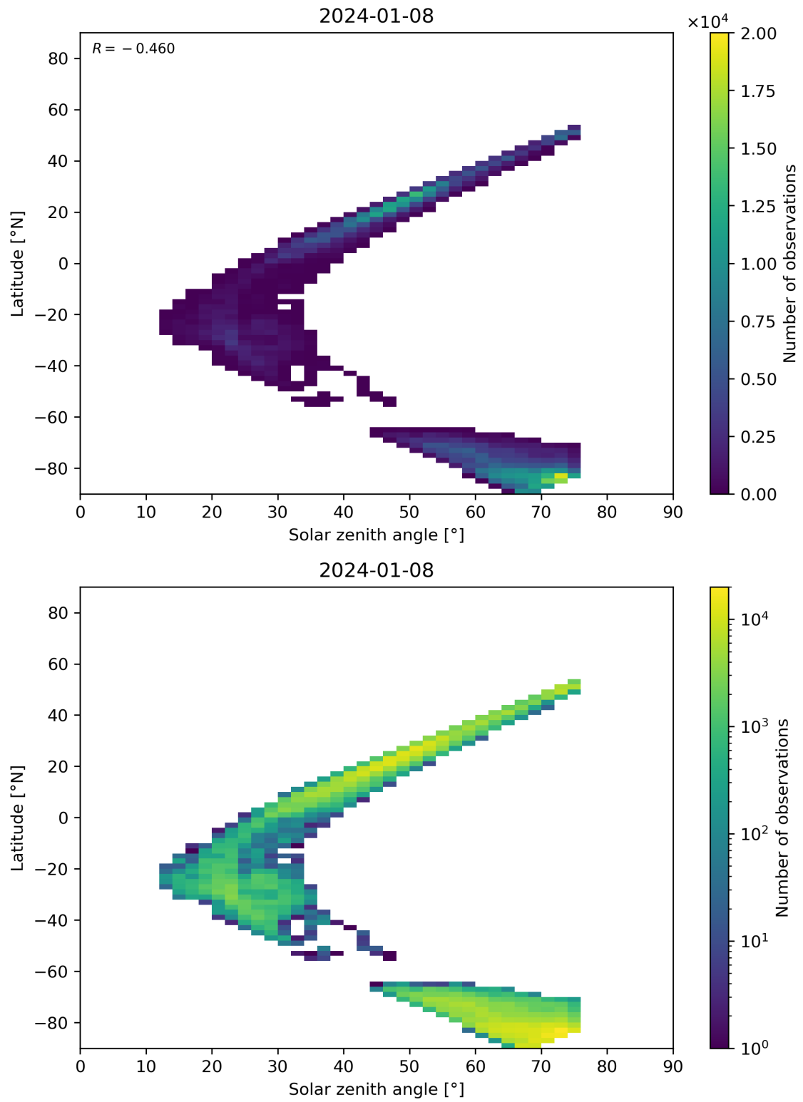
Figure 98: Scatter density plot of “Solar zenith angle” against “Latitude” for 2024-01-07 to 2024-01-09.
