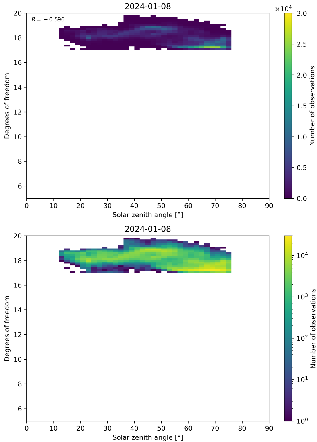
Figure 96: Scatter density plot of “Solar zenith angle” against “Degrees of freedom” for 2024-01-07 to 2024-01-09.
