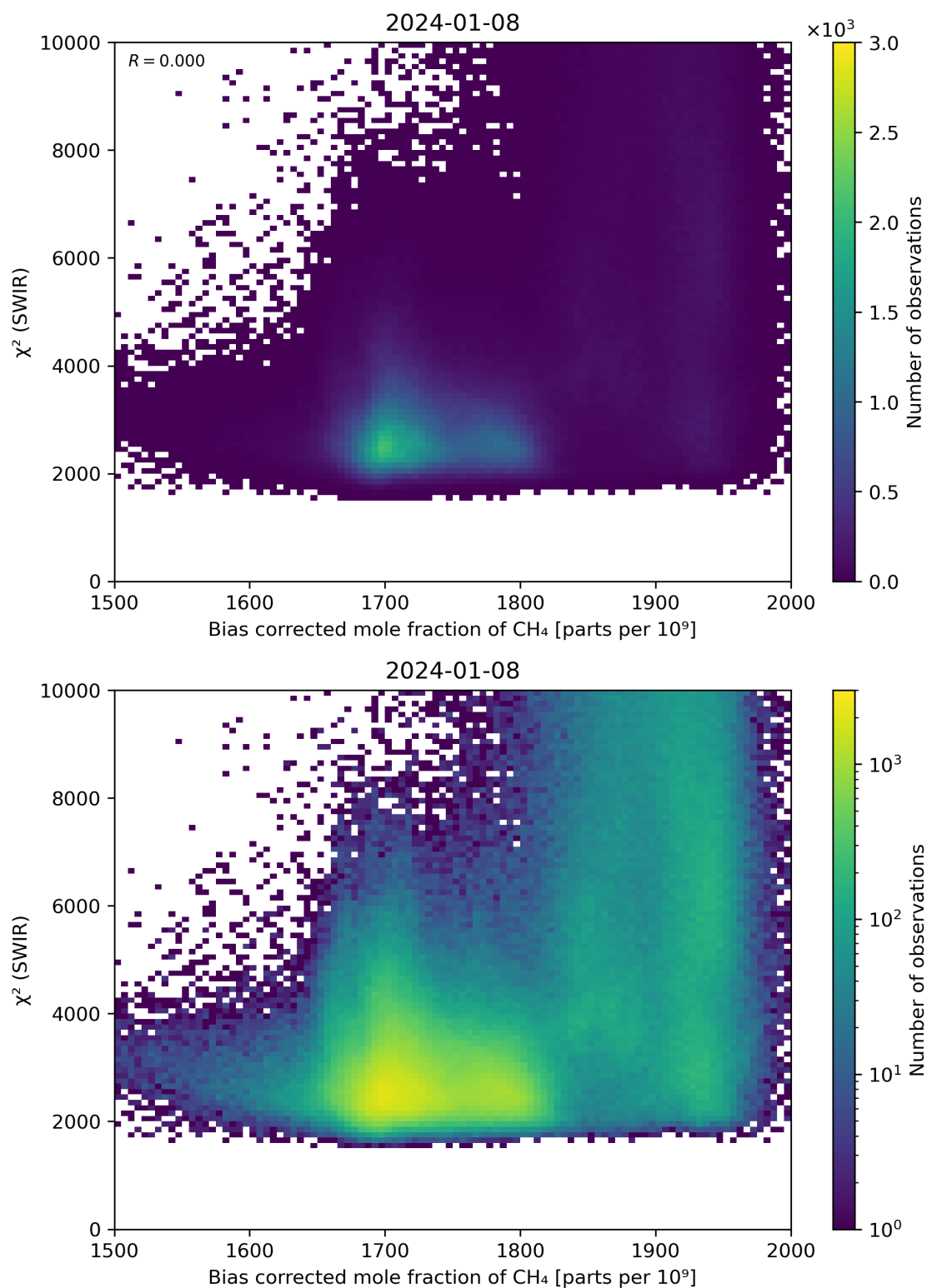
Figure 64: Scatter density plot of “Bias corrected mole fraction of \text{CH}_4 ” against “ \chi^2 (SWIR)” for 2024-01-07 to 2024-01-09.
