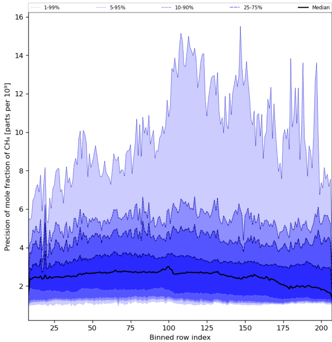
Figure 35: Along track statistics of “Precision of mole fraction of CH 4 ” for 2024-01-07 to 2024-01-09
