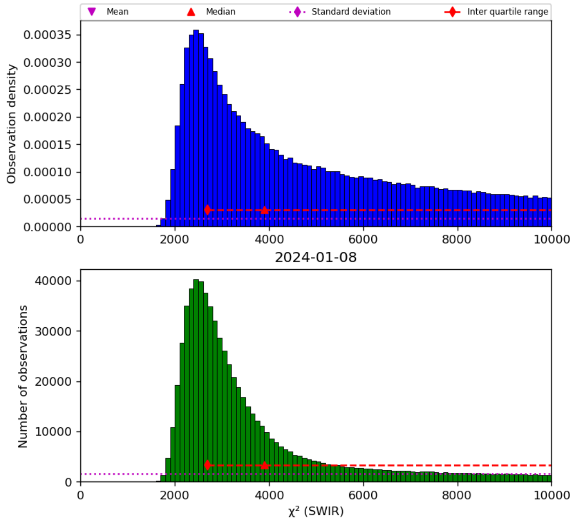
Figure 28: Histogram of “ \chi^2 (SWIR)” for 2024-01-07 to 2024-01-09
