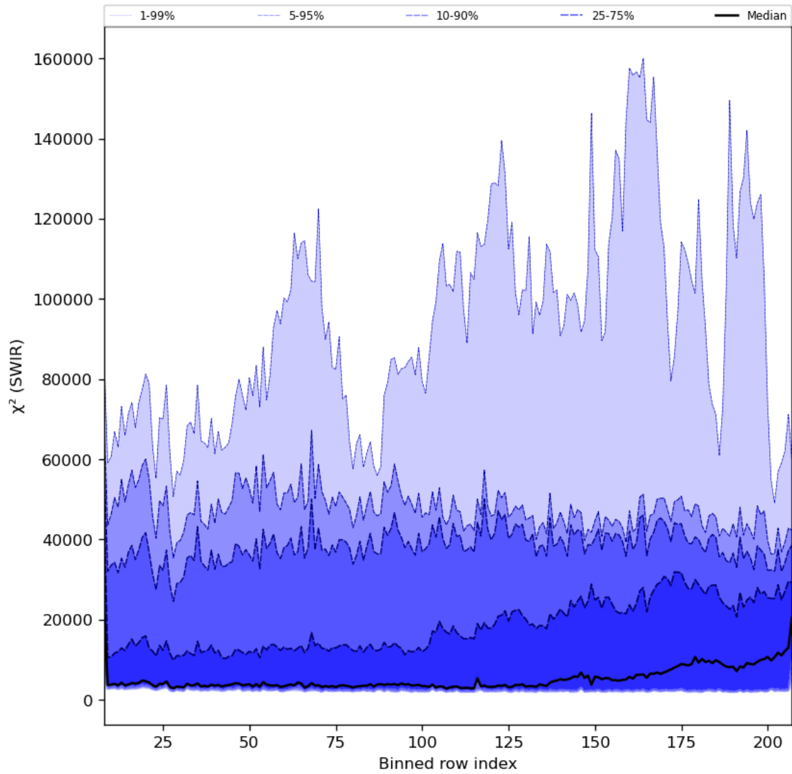
Figure 39: Along track statistics of “ \chi^2 (SWIR)” for 2024-01-07 to 2024-01-09
