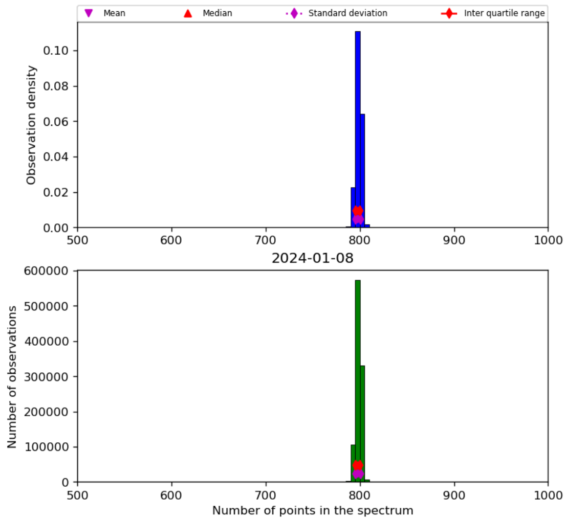
Figure 26: Histogram of “Number of points in the spectrum” for 2024-01-07 to 2024-01-09
