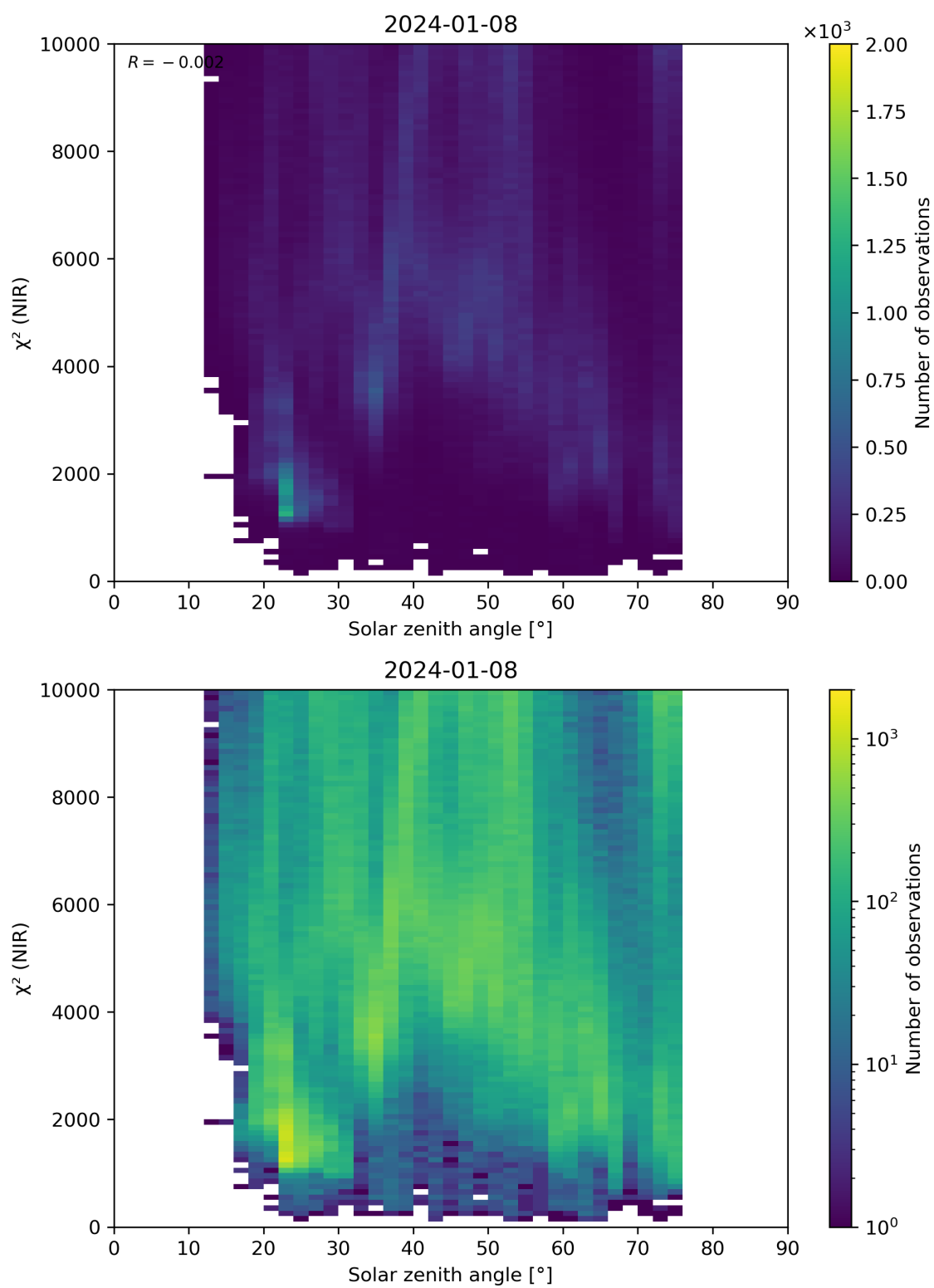
Figure 94: Scatter density plot of “Solar zenith angle” against “ \chi^2 (NIR)” for 2024-01-07 to 2024-01-09.
