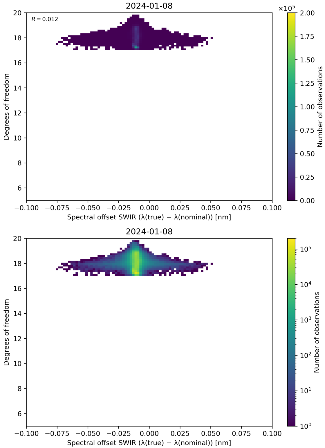
Figure 119: Scatter density plot of “Spectral offset SWIR ( \lambda(\text{true}) - \lambda(\text{nominal}) )” against “Degrees of freedom” for 2024-01-07 to 2024-01-09.
