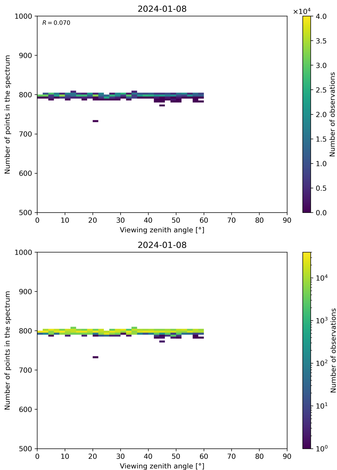
Figure 114: Scatter density plot of “Viewing zenith angle” against “Number of points in the spectrum” for 2024-01-07 to 2024-01-09.
