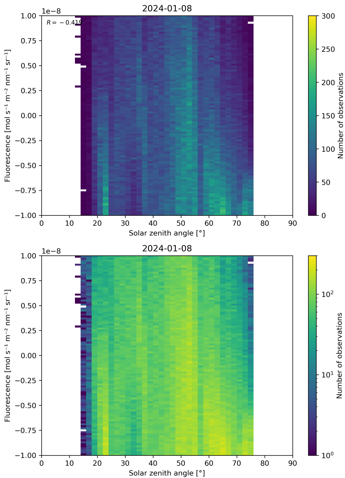
Figure 97: Scatter density plot of “Solar zenith angle” against “Fluorescence” for 2024-01-07 to 2024-01-09.
