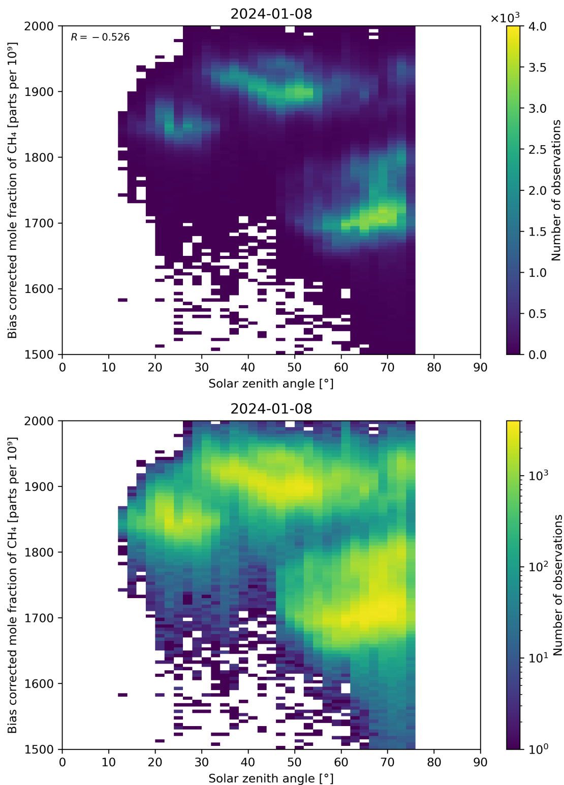
Figure 100: Scatter density plot of “Solar zenith angle” against “Bias corrected mole fraction of CH 4 ” for 2024-01-07 to 2024-01-09.
