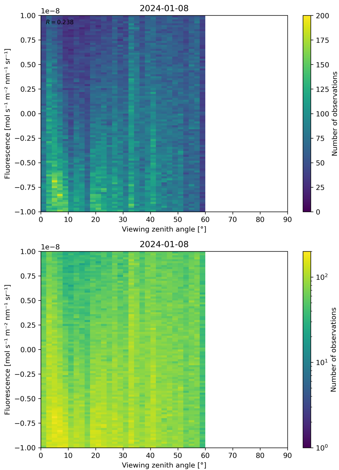
Figure 108: Scatter density plot of “Viewing zenith angle” against “Fluorescence” for 2024-01-07 to 2024-01-09.
