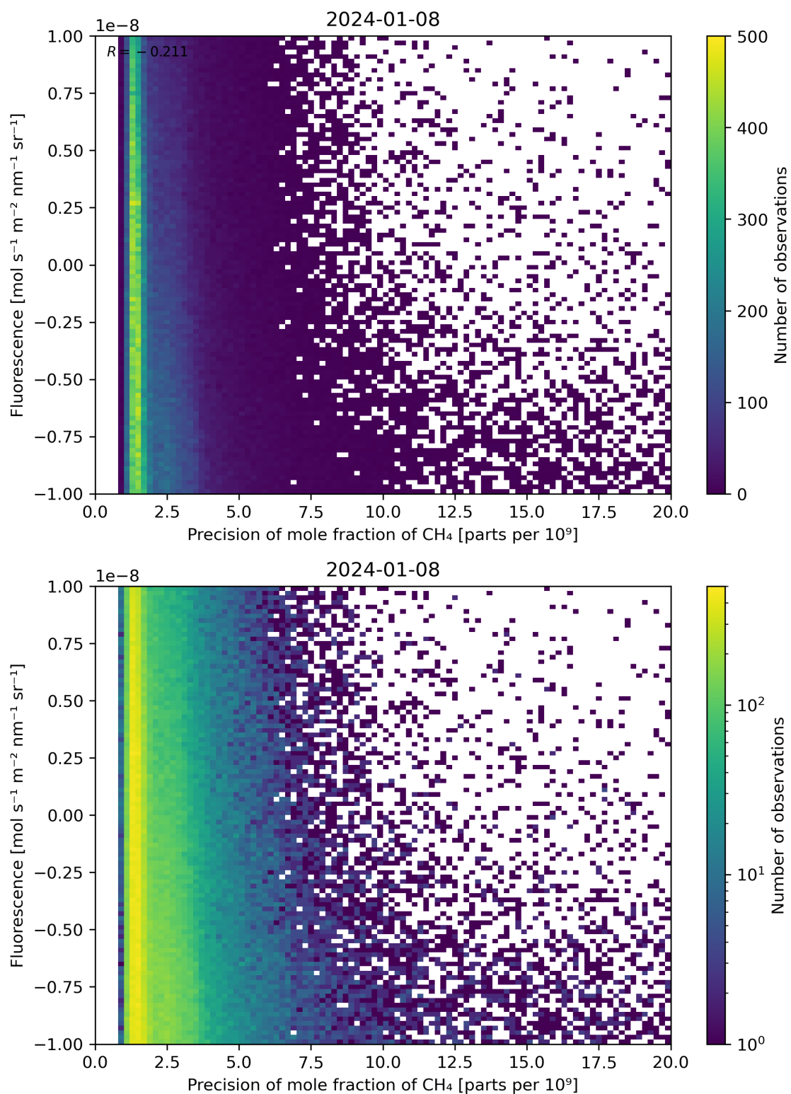
Figure 81: Scatter density plot of “Precision of mole fraction of \text{CH}_4 ” against “Fluorescence” for 2024-01-07 to 2024-01-09.
