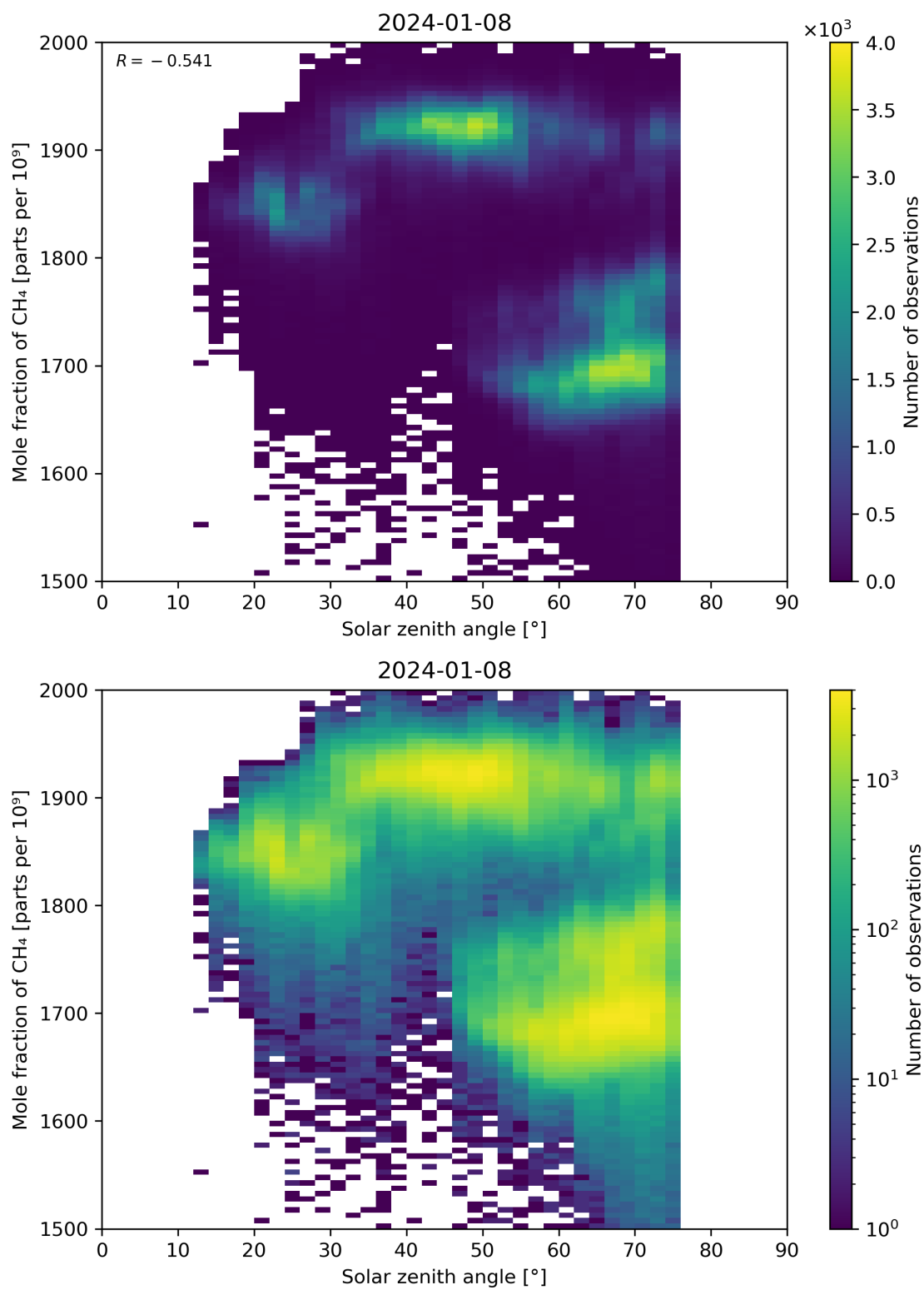
Figure 99: Scatter density plot of “Solar zenith angle” against “Mole fraction of CH 4 ” for 2024-01-07 to 2024-01-09.
