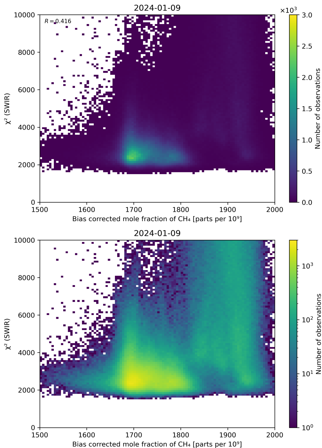
Figure 64: Scatter density plot of “Bias corrected mole fraction of CH 4 ” against “ \chi^2 (SWIR)” for 2024-01-08 to 2024-01-10.
