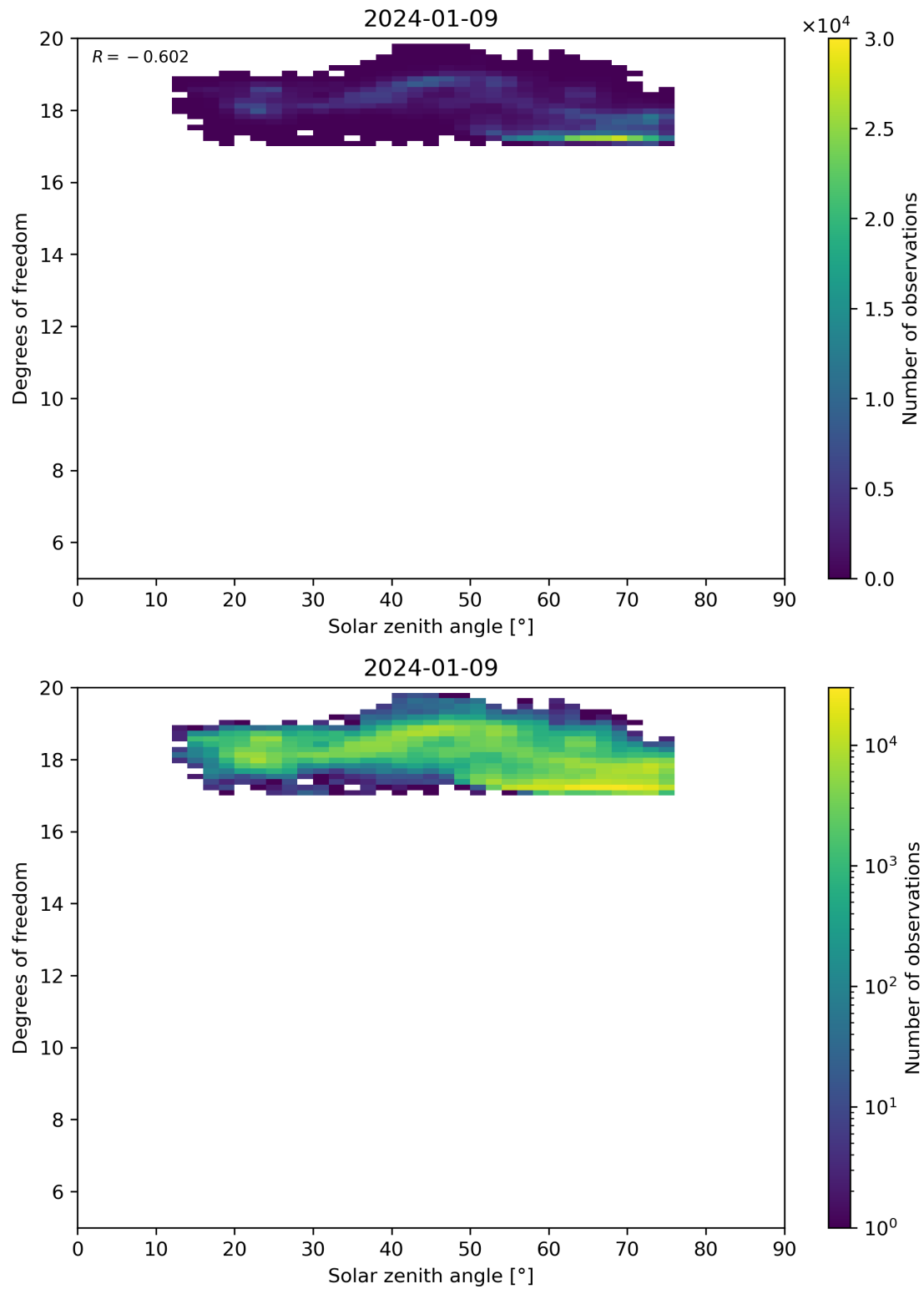
Figure 96: Scatter density plot of “Solar zenith angle” against “Degrees of freedom” for 2024-01-08 to 2024-01-10.
