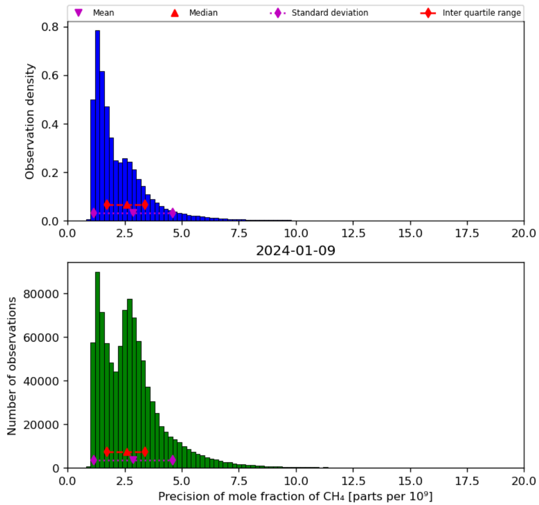
Figure 24: Histogram of “Precision of mole fraction of CH 4 ” for 2024-01-08 to 2024-01-10
