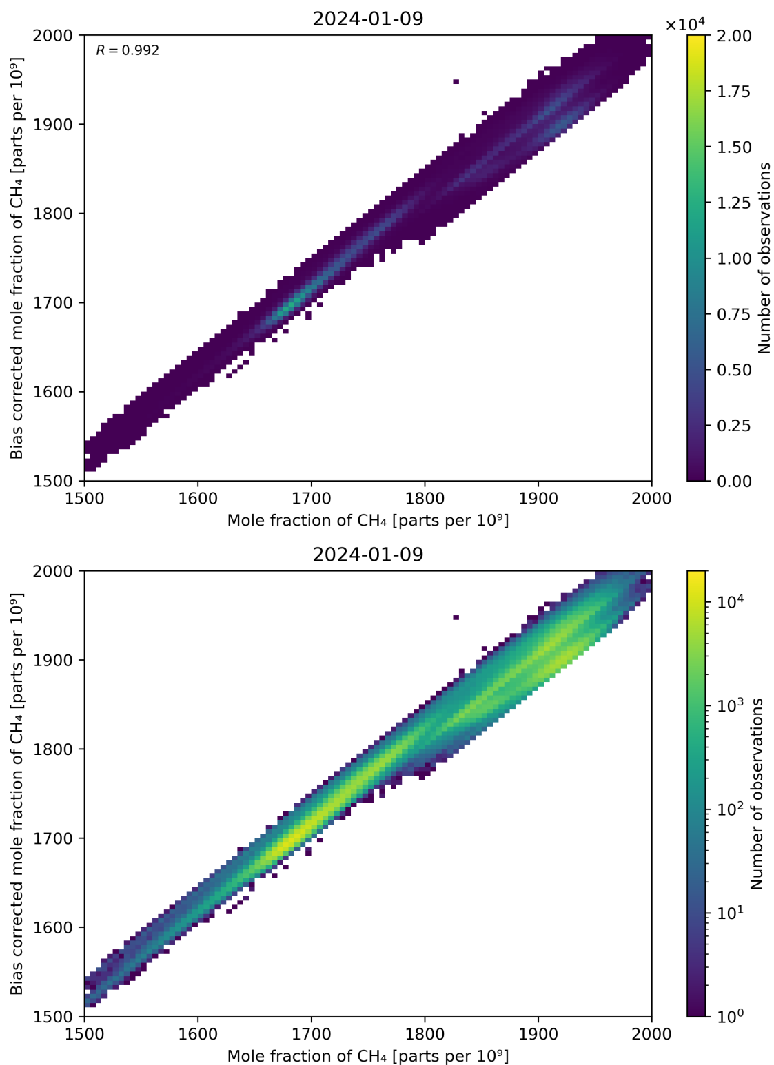
Figure 74: Scatter density plot of “Mole fraction of CH 4 ” against “Bias corrected mole fraction of CH 4 ” for 2024-01-08 to 2024-01-10.
