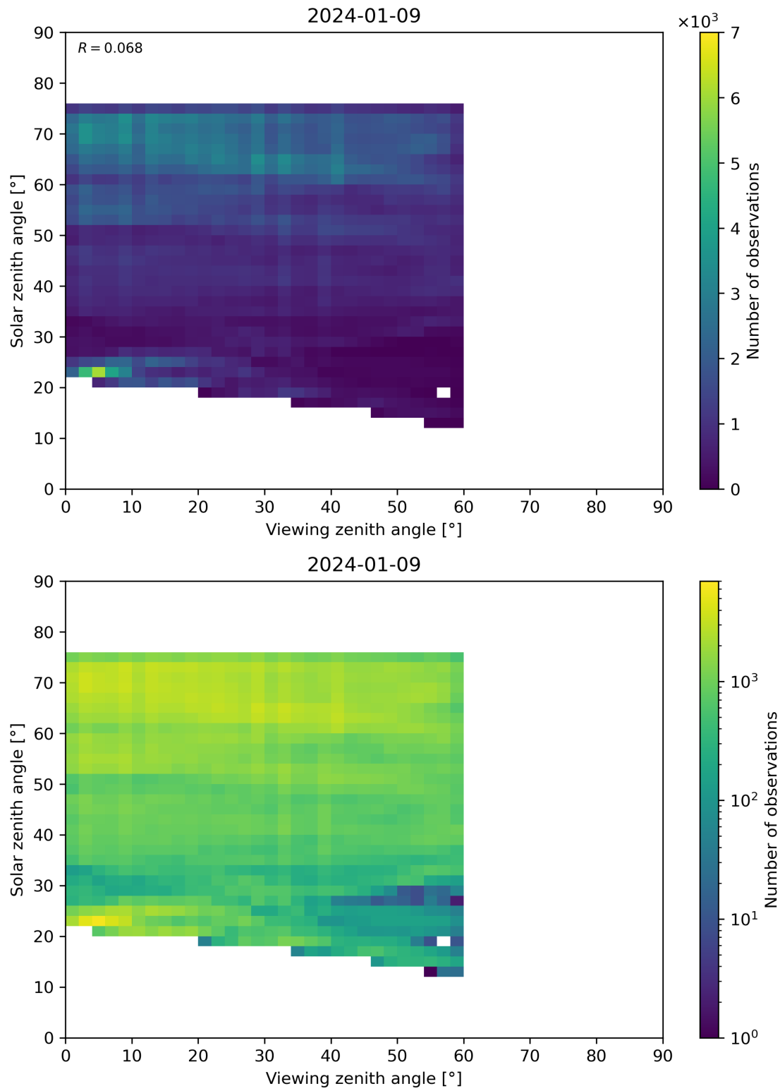
Figure 115: Scatter density plot of “Viewing zenith angle” against “Solar zenith angle” for 2024-01-08 to 2024-01-10.
