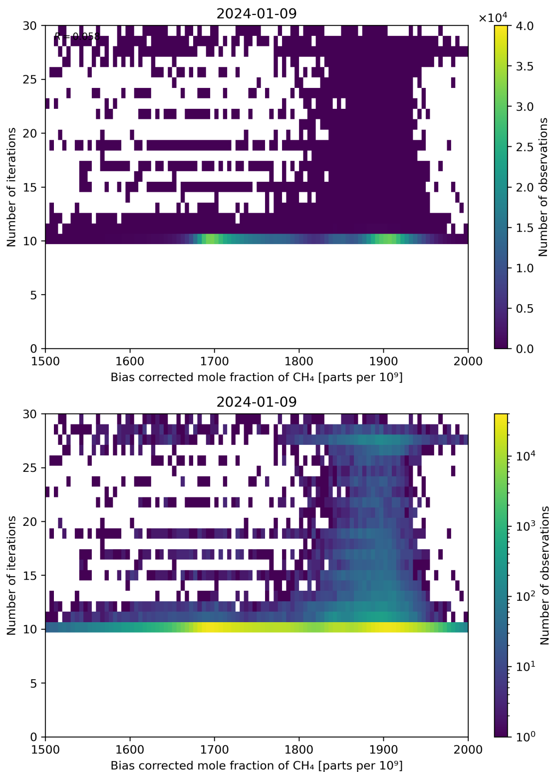
Figure 67: Scatter density plot of “Bias corrected mole fraction of CH 4 ” against “Number of iterations” for 2024-01-08 to 2024-01-10.
