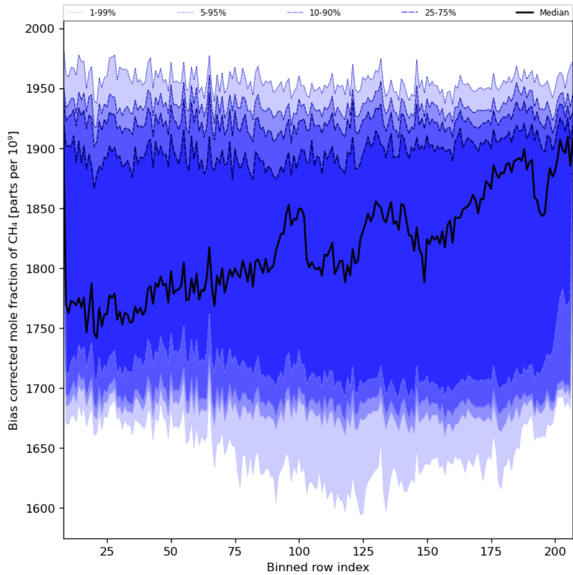
Figure 36: Along track statistics of “Bias corrected mole fraction of CH 4 ” for 2024-01-08 to 2024-01-10
