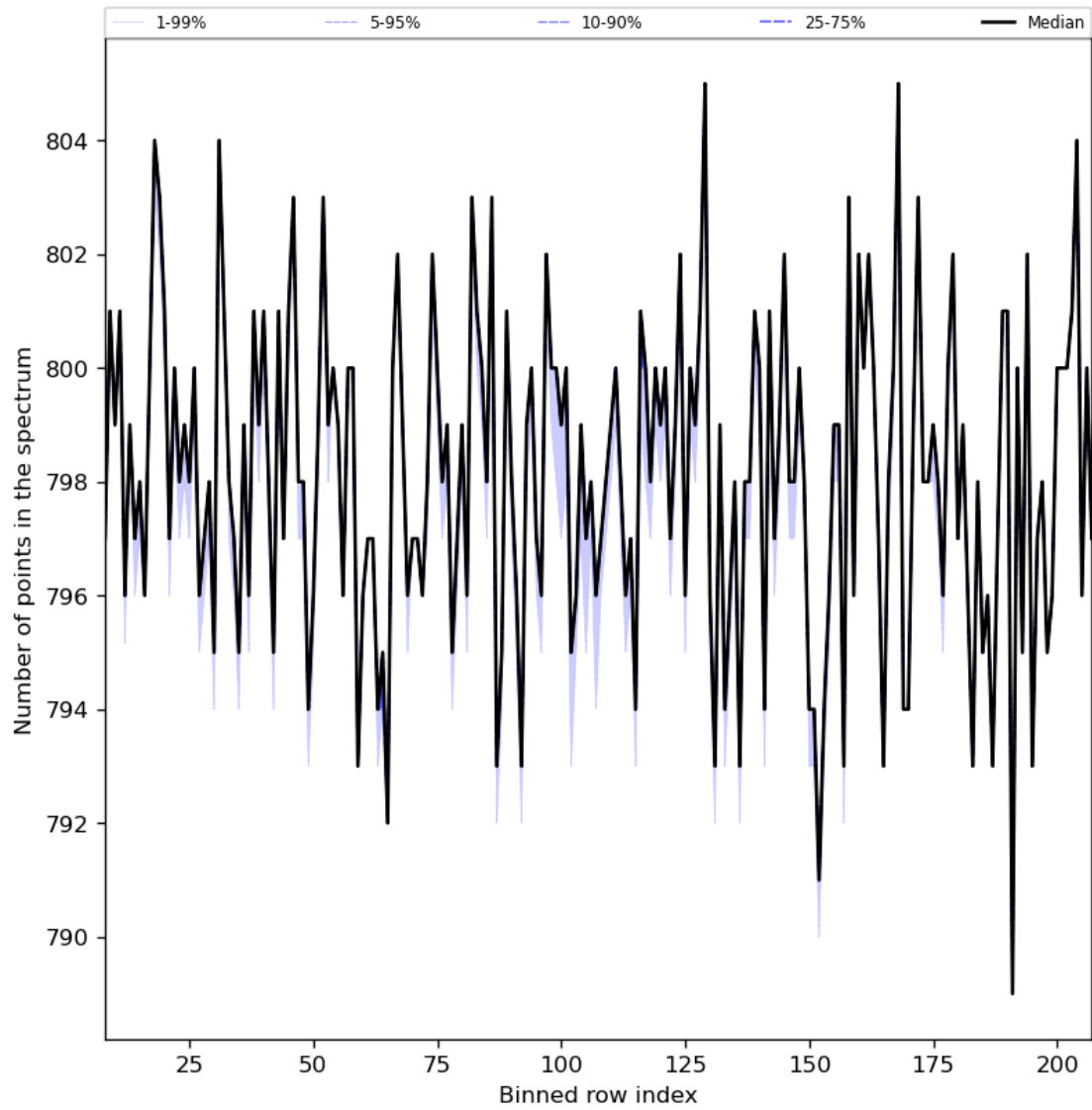
Figure 37: Along track statistics of “Number of points in the spectrum” for 2024-01-08 to 2024-01-10
