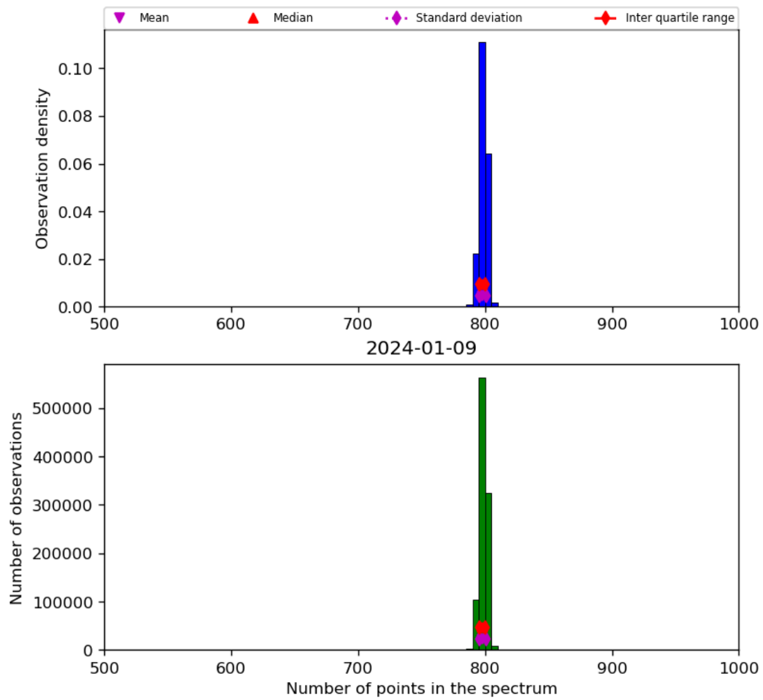
Figure 26: Histogram of “Number of points in the spectrum” for 2024-01-08 to 2024-01-10
