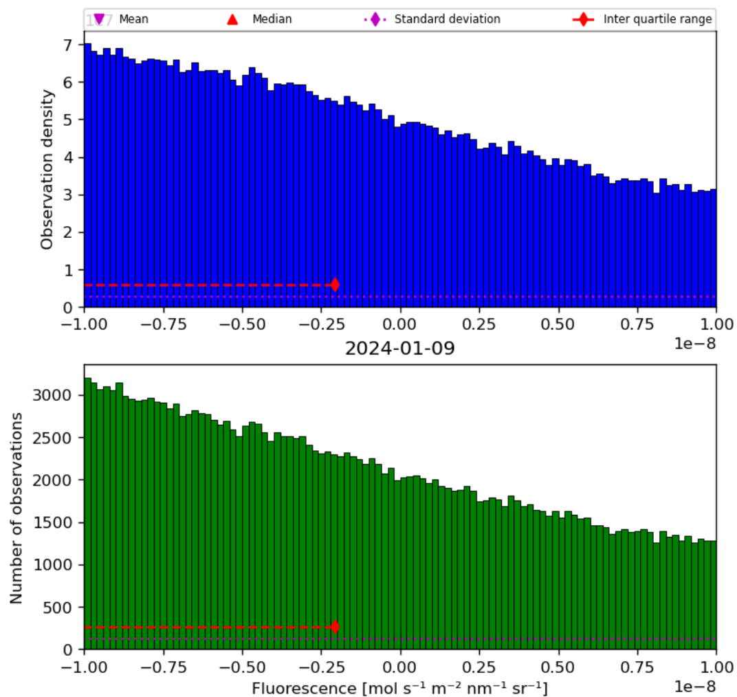
Figure 32: Histogram of “Fluorescence” for 2024-01-08 to 2024-01-10
