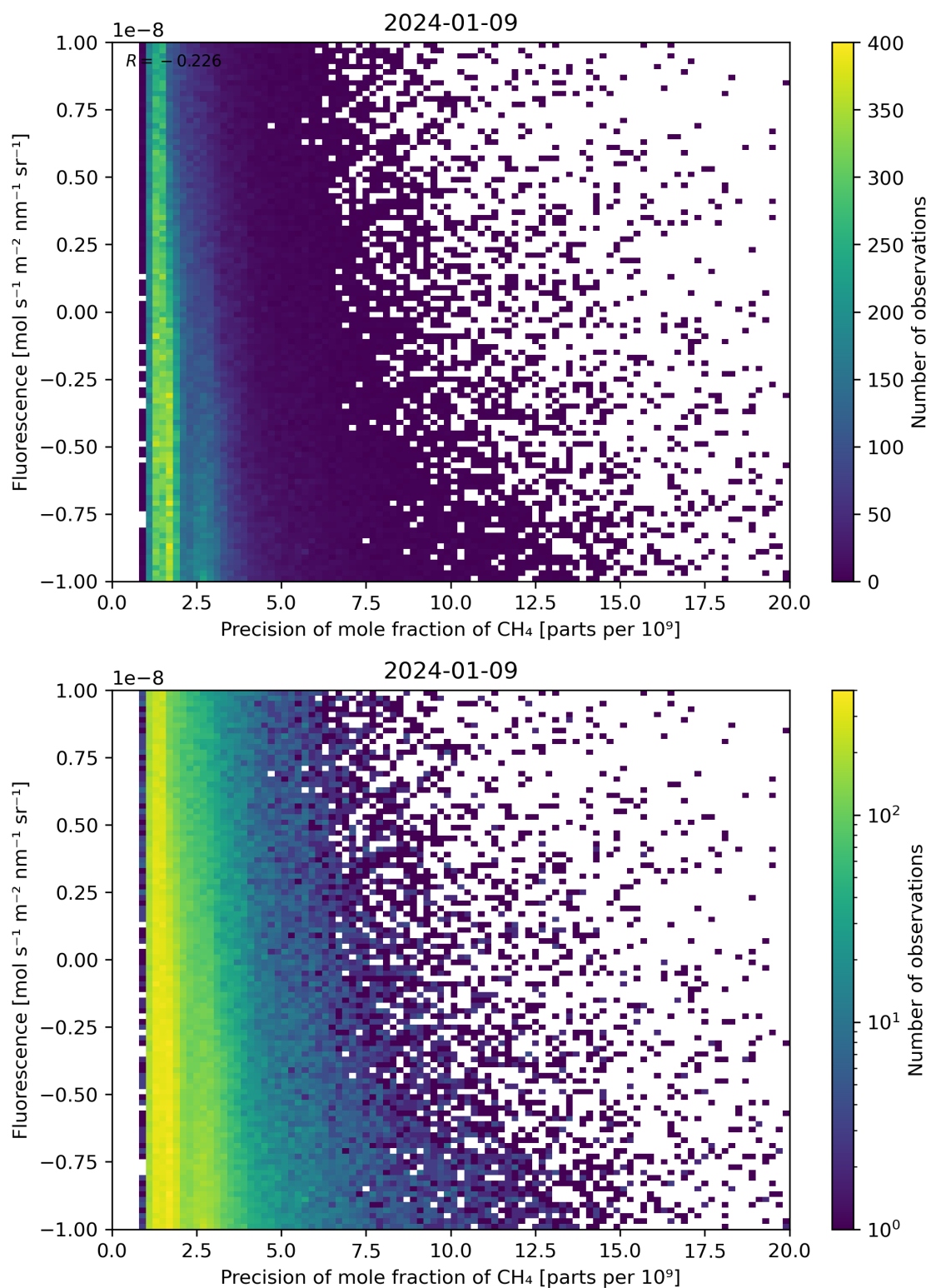
Figure 81: Scatter density plot of “Precision of mole fraction of CH 4 ” against “Fluorescence” for 2024-01-08 to 2024-01-10.
