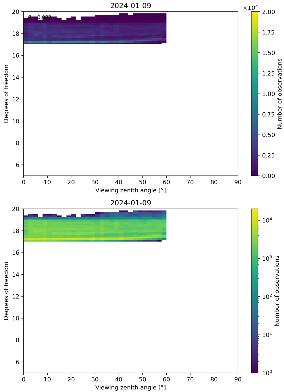
Figure 107: Scatter density plot of “Viewing zenith angle” against “Degrees of freedom” for 2024-01-08 to 2024-01-10.
