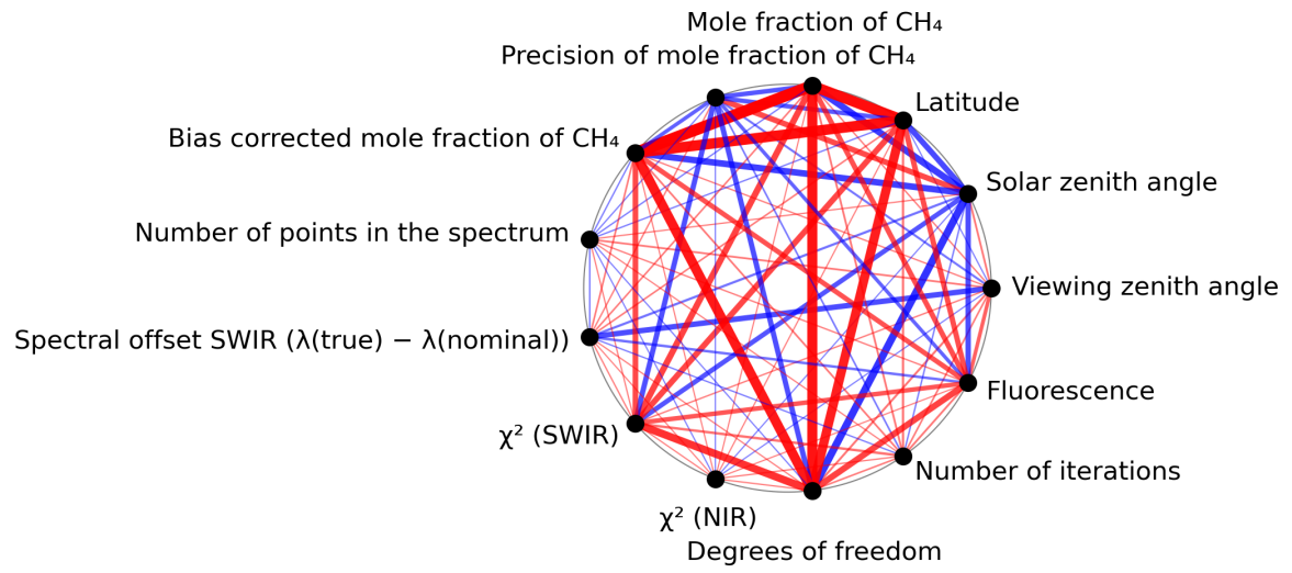
Figure 1: Map of correlation graph for 2024-01-08 to 2024-01-10.
