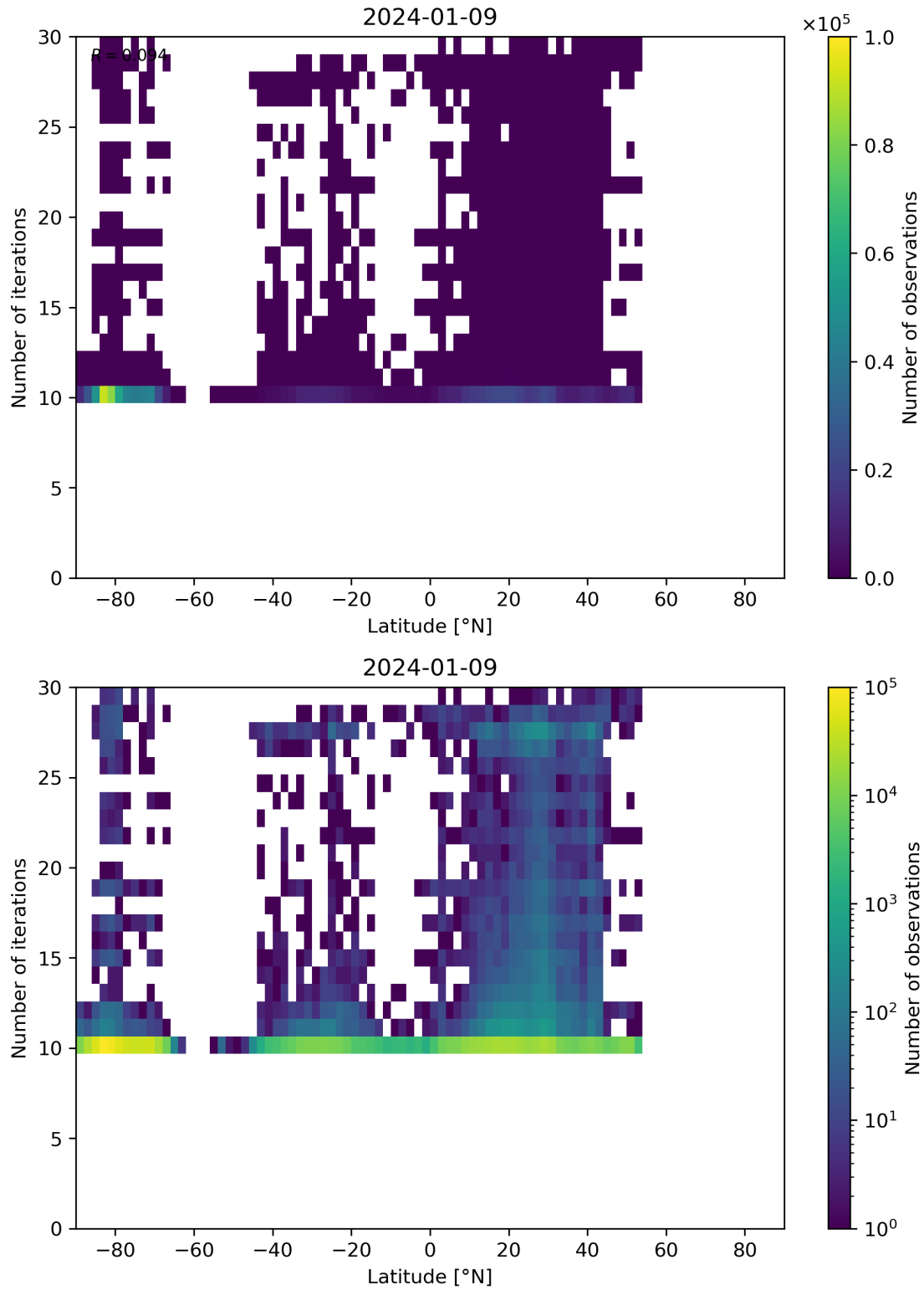
Figure 60: Scatter density plot of “Latitude” against “Number of iterations” for 2024-01-08 to 2024-01-10.
