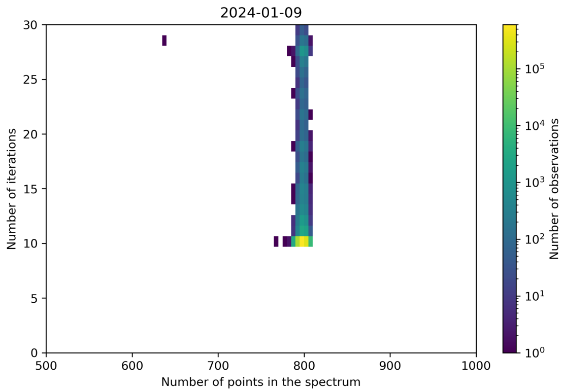
Figure 92: Scatter density plot of “Number of points in the spectrum” against “Number of iterations” for 2024-01-08 to 2024-01-10.
