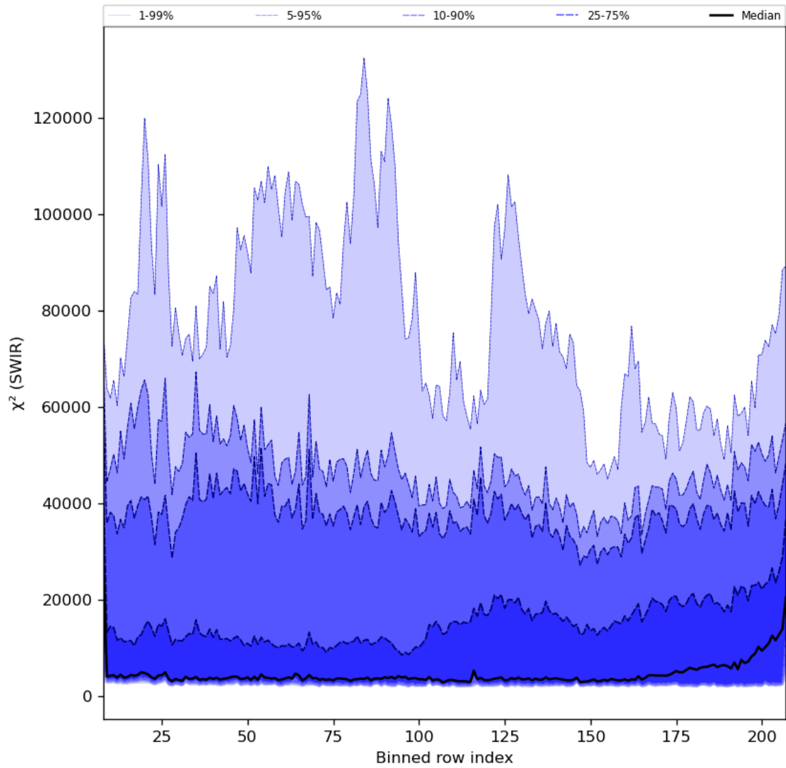
Figure 39: Along track statistics of “ \chi^2 (SWIR)” for 2024-01-08 to 2024-01-10
