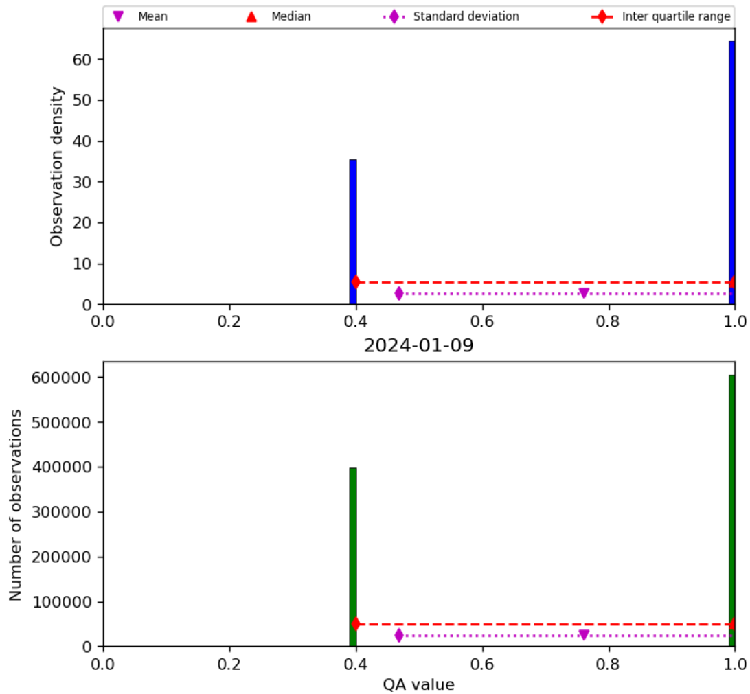
Figure 22: Histogram of “QA value” for 2024-01-08 to 2024-01-10
