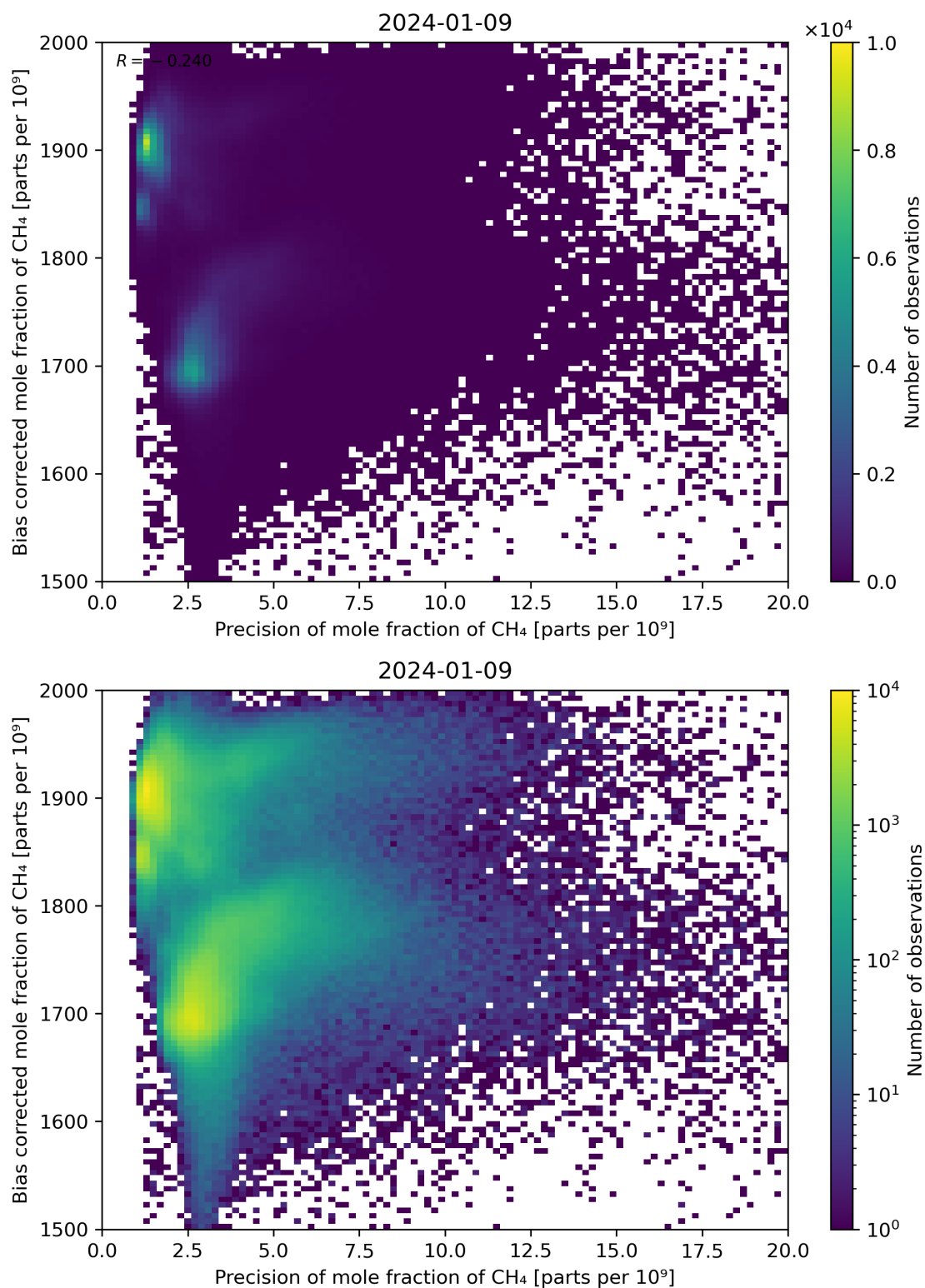
Figure 82: Scatter density plot of “Precision of mole fraction of CH 4 ” against “Bias corrected mole fraction of CH 4 ” for 2024-01-08 to 2024-01-10.
