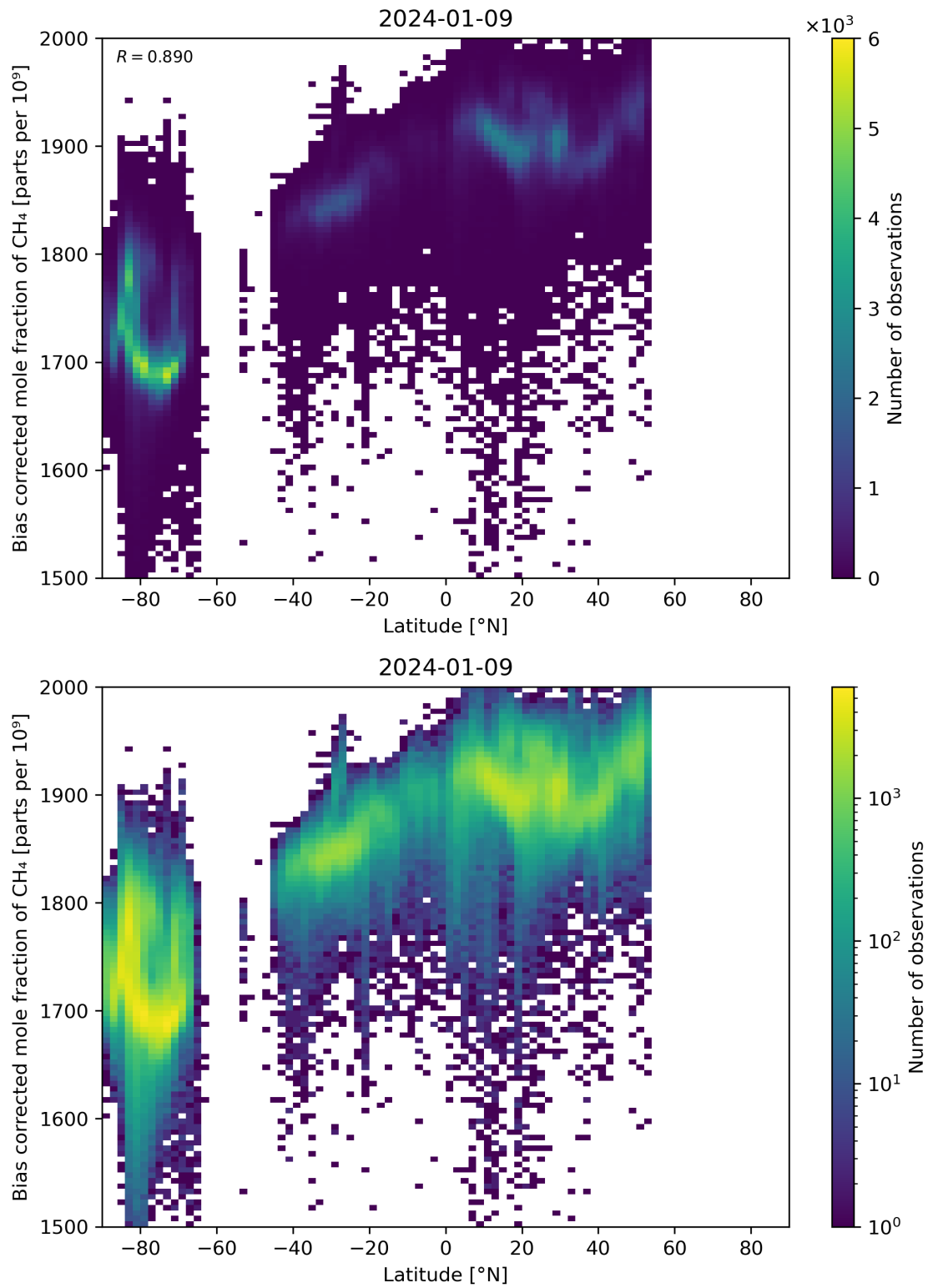
Figure 58: Scatter density plot of “Latitude” against “Bias corrected mole fraction of CH 4 ” for 2024-01-08 to 2024-01-10.
