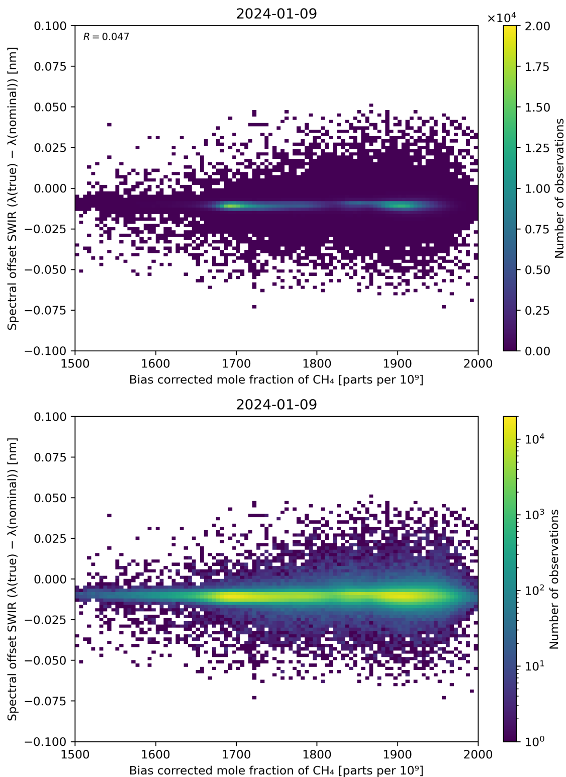
Figure 69: Scatter density plot of “Bias corrected mole fraction of \text{CH}_4 ” against “Spectral offset SWIR ( \lambda(\text{true}) - \lambda(\text{nominal}) )” for 2024-01-08 to 2024-01-10.
