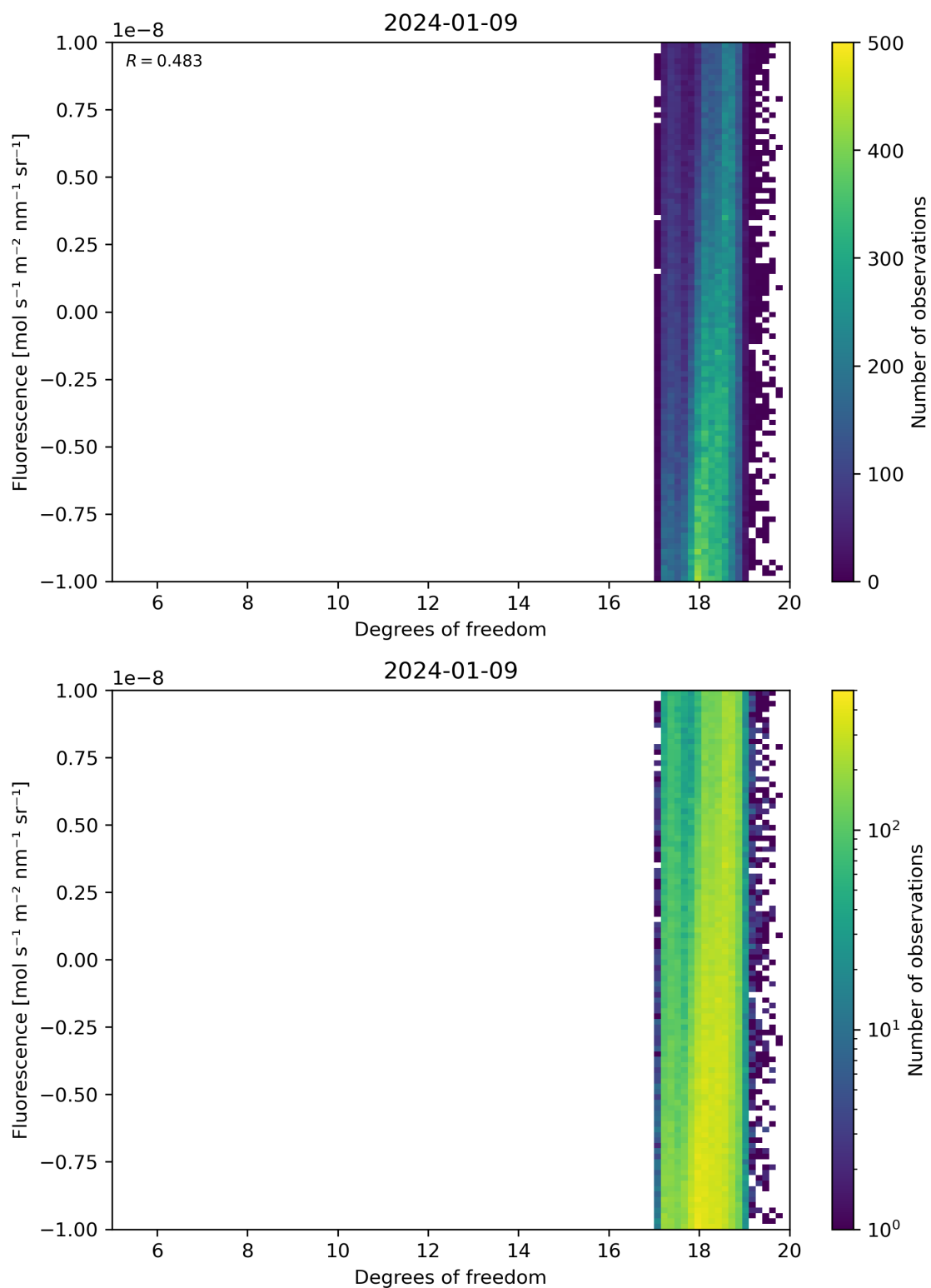
Figure 51: Scatter density plot of “Degrees of freedom” against “Fluorescence” for 2024-01-08 to 2024-01-10.
