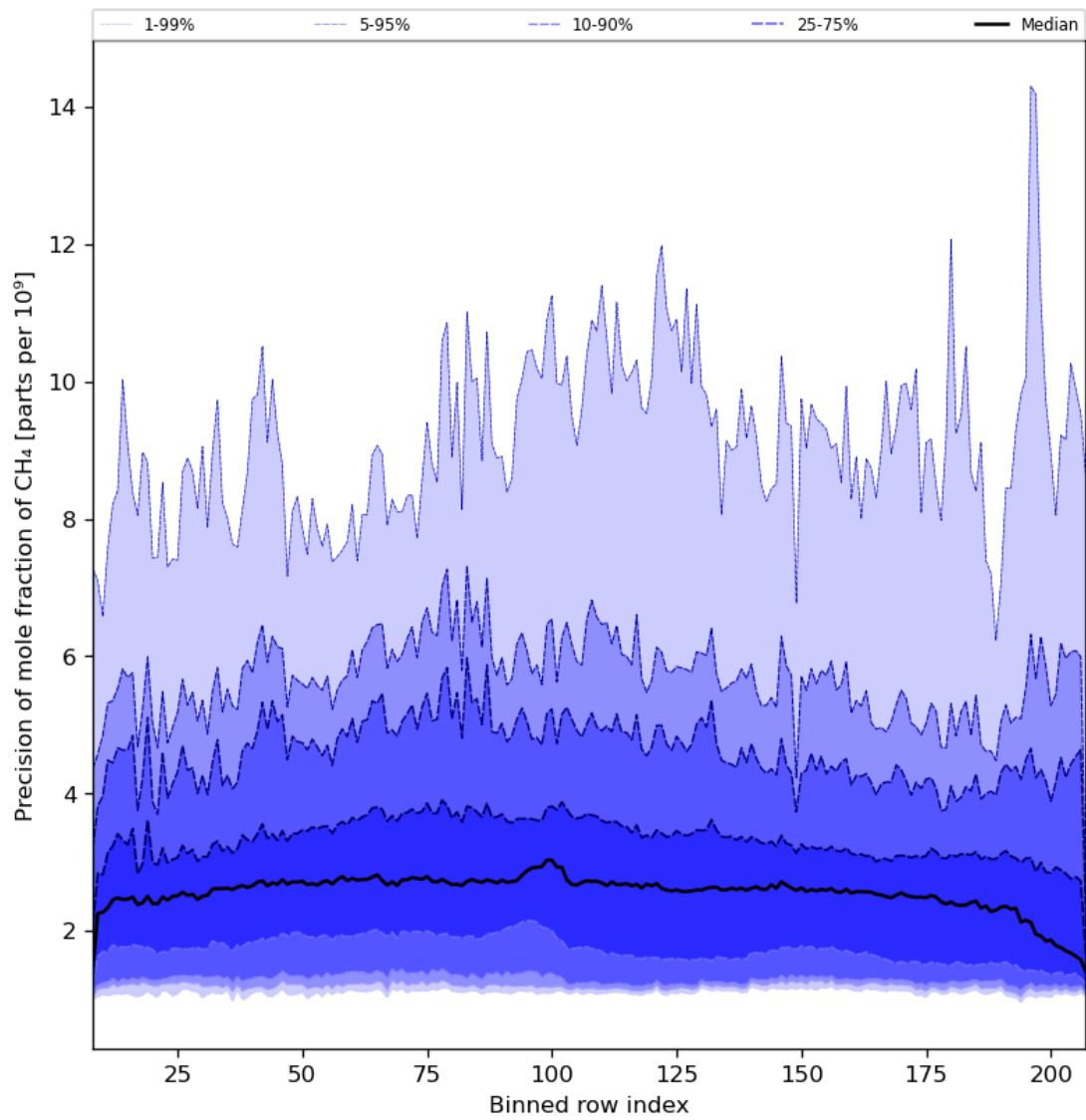
Figure 35: Along track statistics of “Precision of mole fraction of CH 4 ” for 2024-01-08 to 2024-01-10
