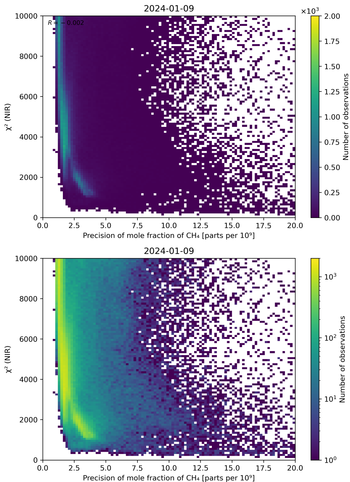
Figure 78: Scatter density plot of “Precision of mole fraction of \text{CH}_4 ” against “ \chi^2 (NIR)” for 2024-01-08 to 2024-01-10.
