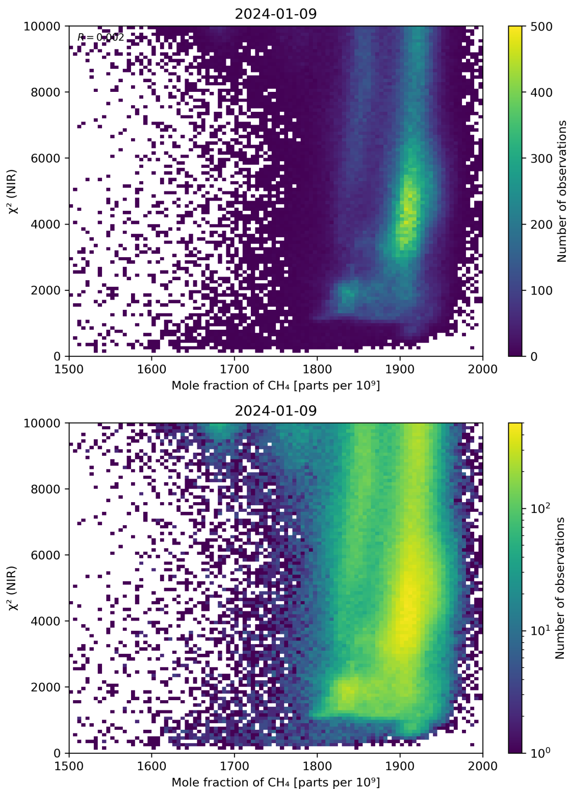
Figure 70: Scatter density plot of “Mole fraction of CH 4 ” against “ \chi^2 (NIR)” for 2024-01-08 to 2024-01-10.
