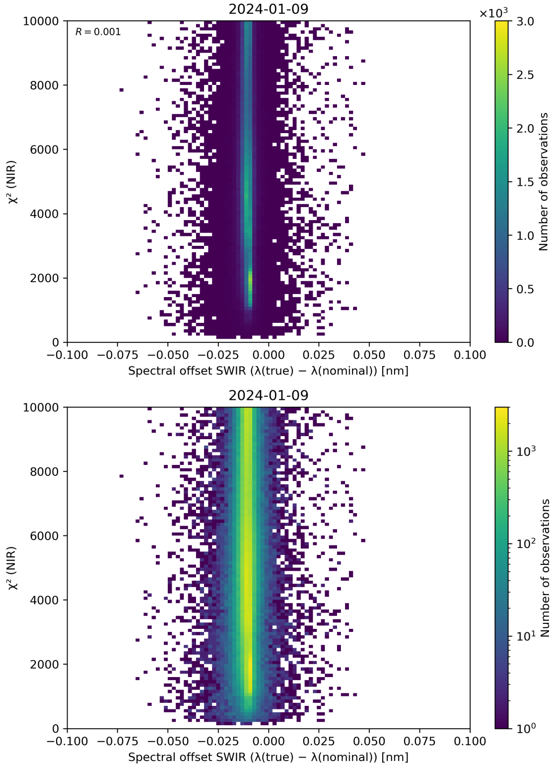
Figure 117: Scatter density plot of “Spectral offset SWIR ( \lambda(\text{true}) - \lambda(\text{nominal}) )” against “ \chi^2 (NIR)” for 2024-01-08 to 2024-01-10.
