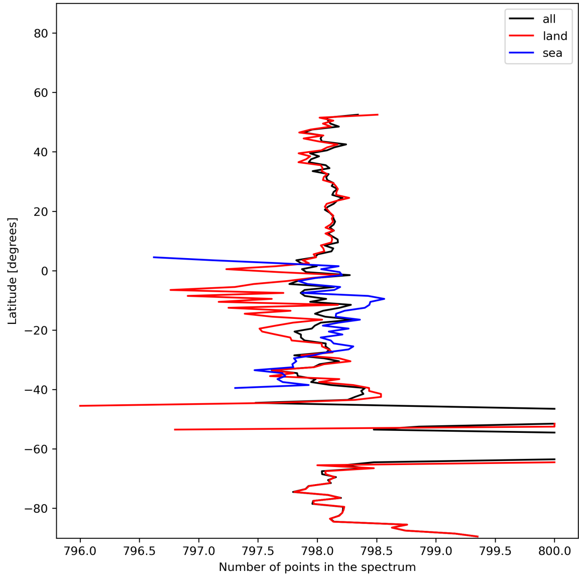
Figure 15: Zonal average of “Number of points in the spectrum” for 2024-01-08 to 2024-01-10.
