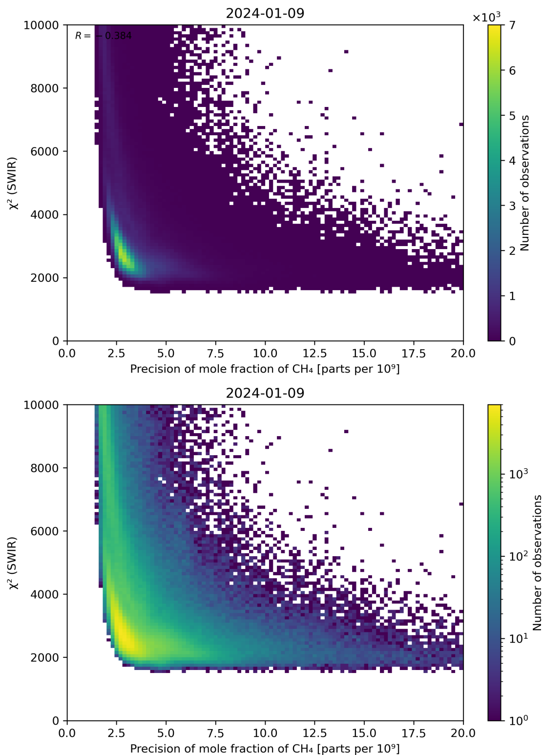
Figure 79: Scatter density plot of “Precision of mole fraction of \text{CH}_4 ” against “ \chi^2 (SWIR)” for 2024-01-08 to 2024-01-10.
