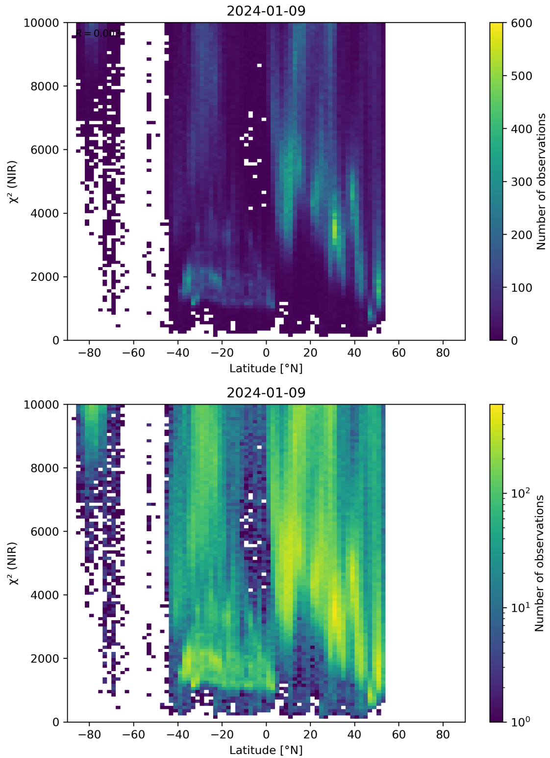
Figure 53: Scatter density plot of “Latitude” against “ \chi^2 (NIR)” for 2024-01-08 to 2024-01-10.
