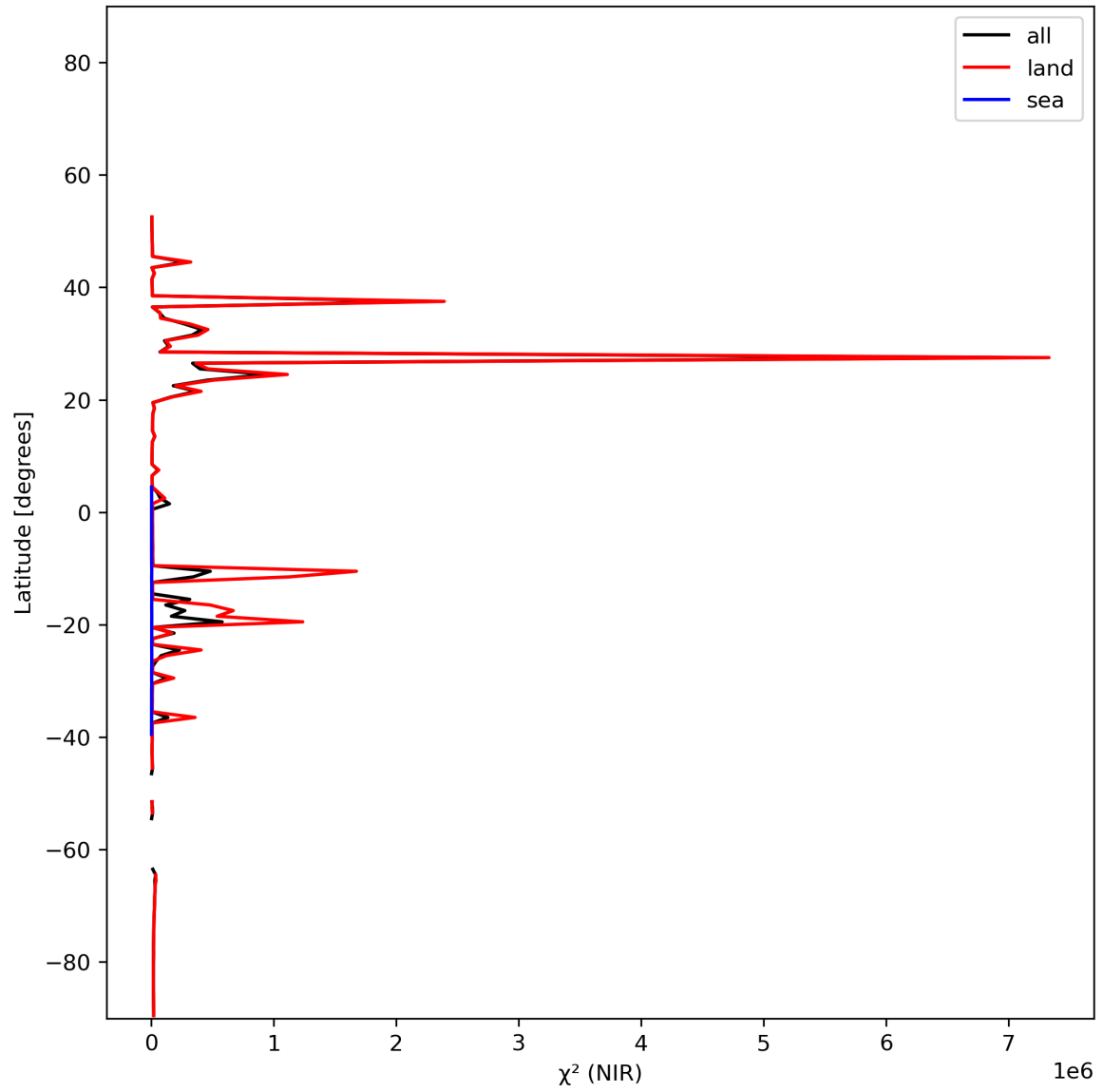
Figure 18: Zonal average of “ \chi^2 (NIR)” for 2024-01-08 to 2024-01-10.
