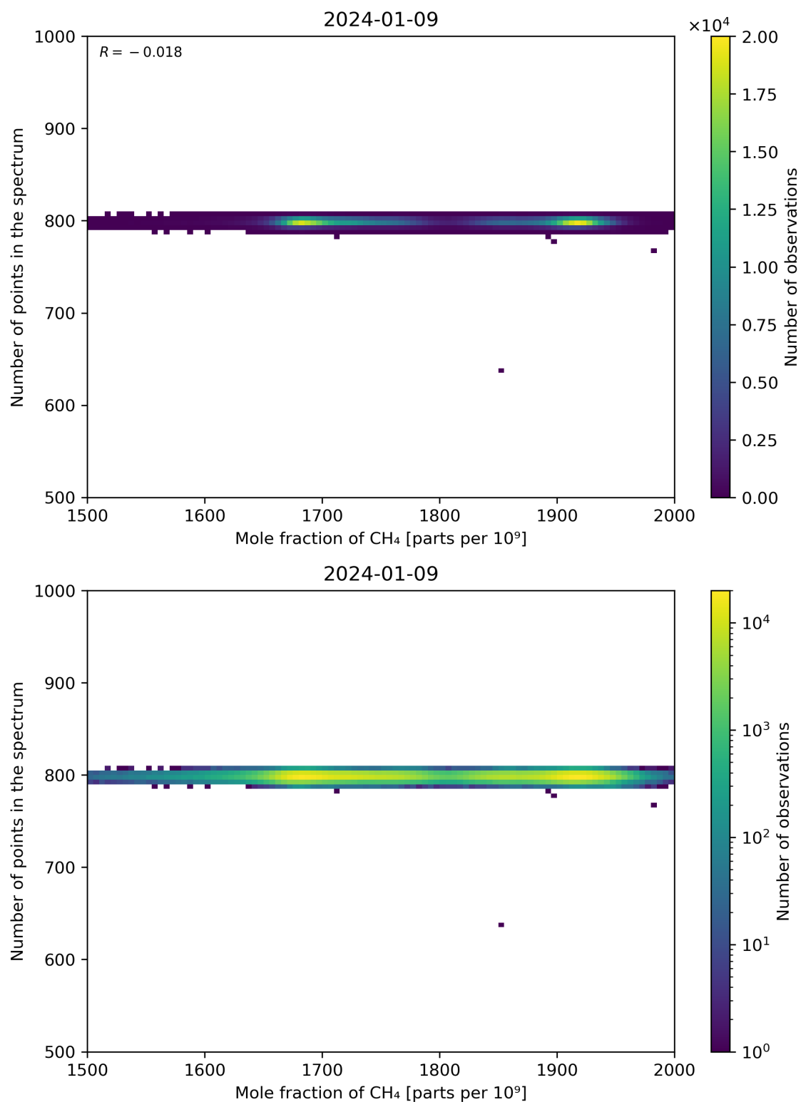
Figure 77: Scatter density plot of “Mole fraction of CH 4 ” against “Number of points in the spectrum” for 2024-01-08 to 2024-01-10.
