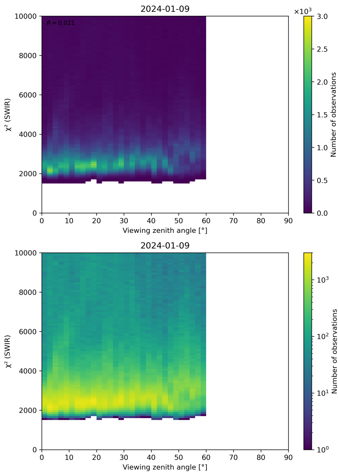
Figure 106: Scatter density plot of “Viewing zenith angle” against “ \chi^2 (SWIR)” for 2024-01-08 to 2024-01-10.
