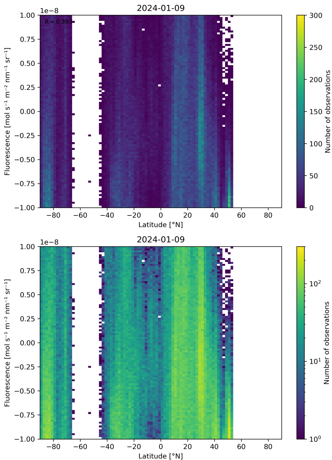
Figure 56: Scatter density plot of “Latitude” against “Fluorescence” for 2024-01-08 to 2024-01-10.
