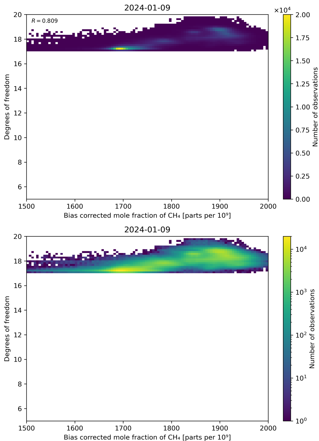
Figure 65: Scatter density plot of “Bias corrected mole fraction of CH 4 ” against “Degrees of freedom” for 2024-01-08 to 2024-01-10.
