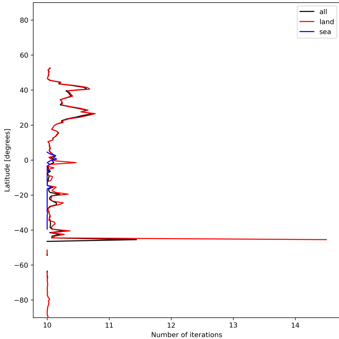
Figure 20: Zonal average of “Number of iterations” for 2024-01-08 to 2024-01-10.
