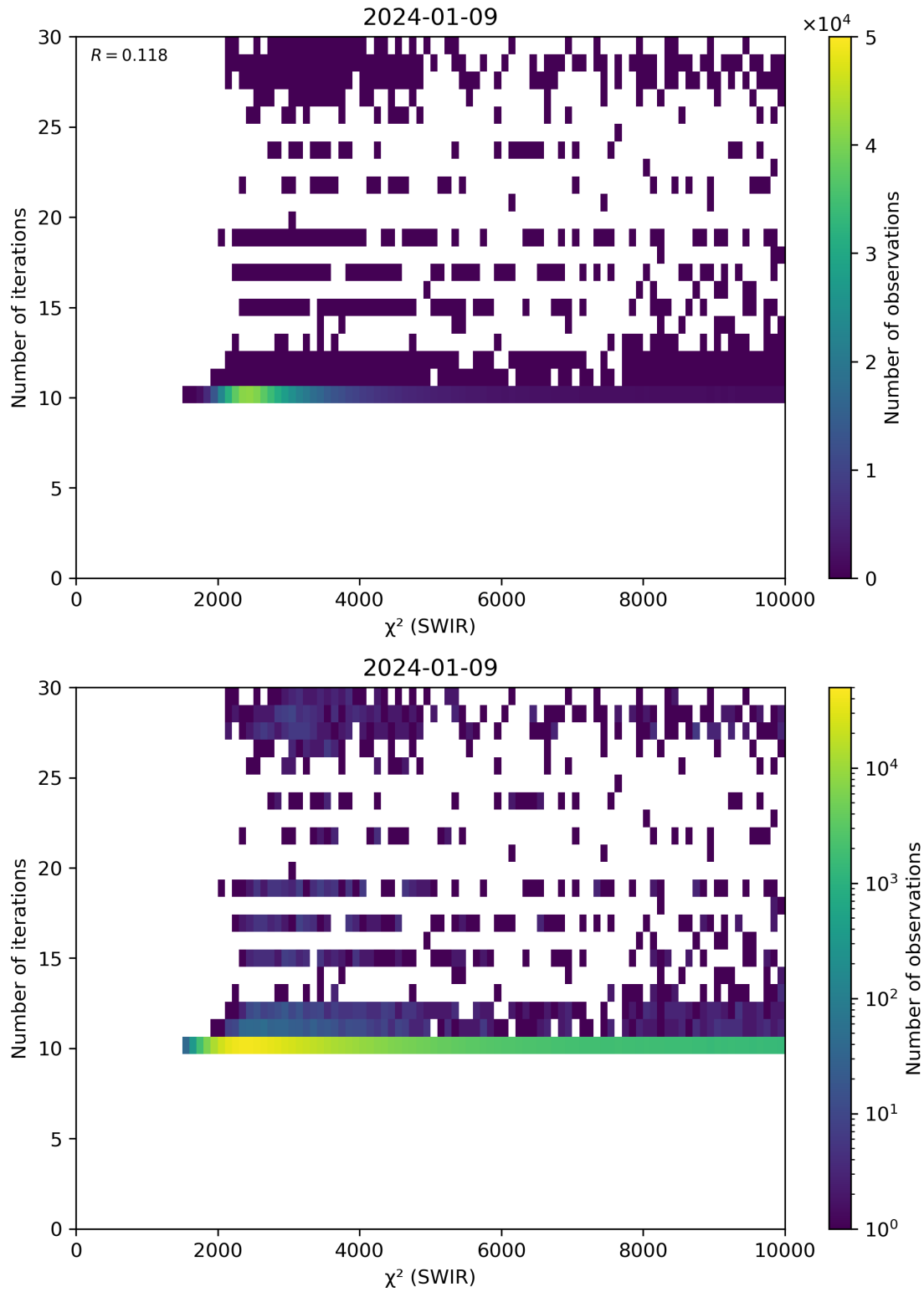
Figure 50: Scatter density plot of “ \chi^2 (SWIR)” against “Number of iterations” for 2024-01-08 to 2024-01-10.
