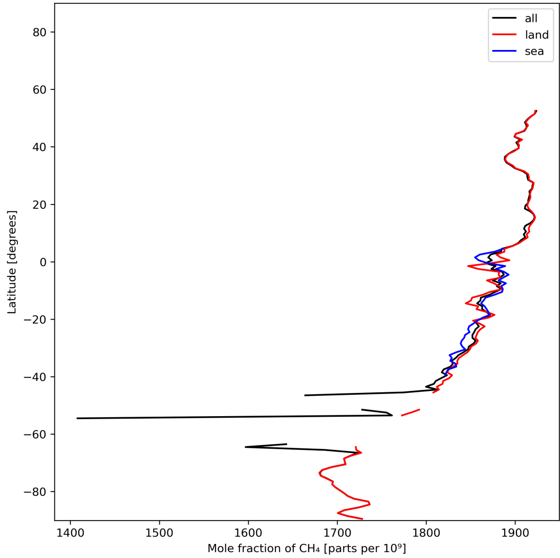
Figure 12: Zonal average of “Mole fraction of \text{CH}_4 ” for 2024-01-08 to 2024-01-10.
