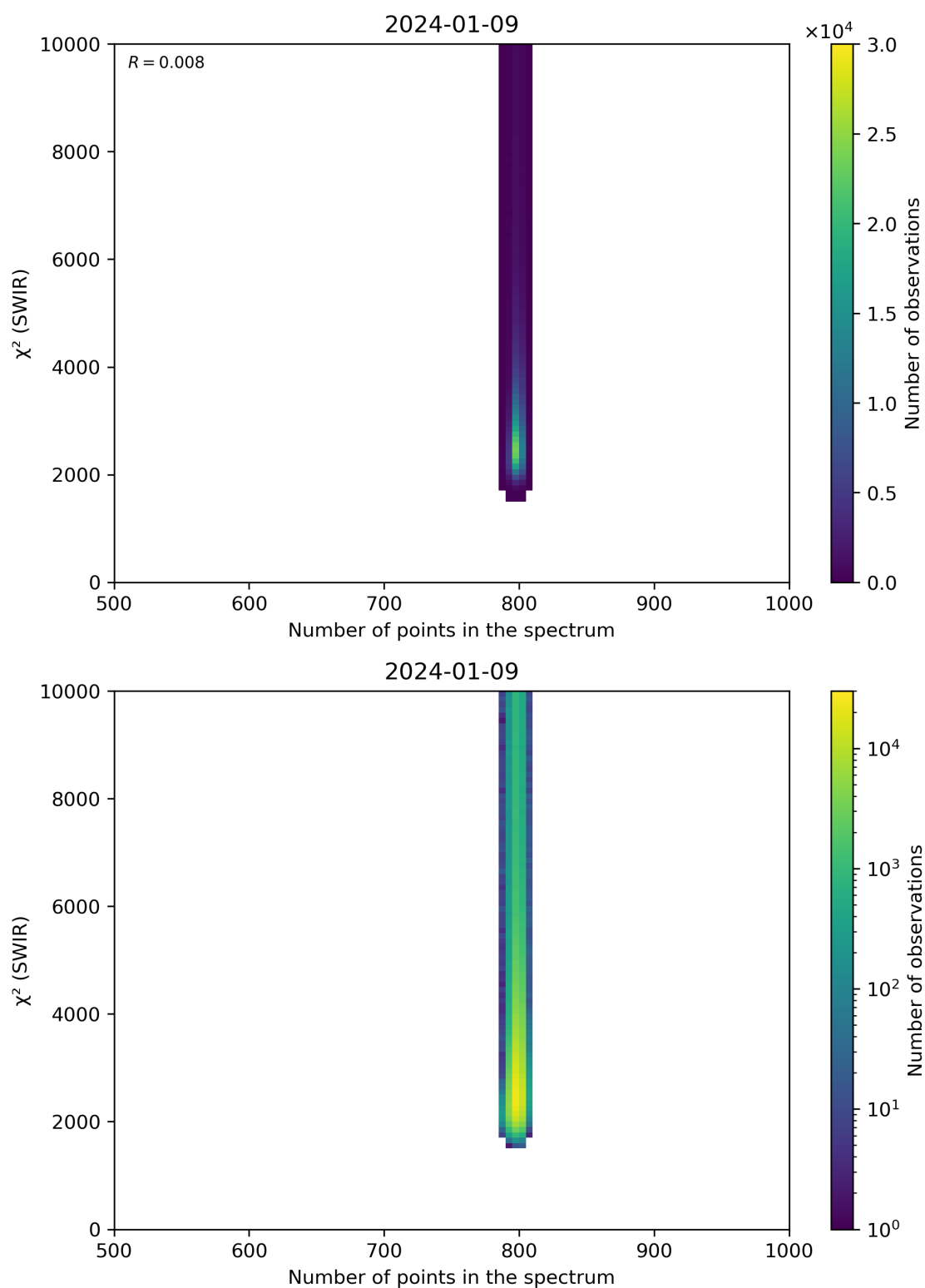
Figure 89: Scatter density plot of “Number of points in the spectrum” against “ \chi^2 (SWIR)” for 2024-01-08 to 2024-01-10.
