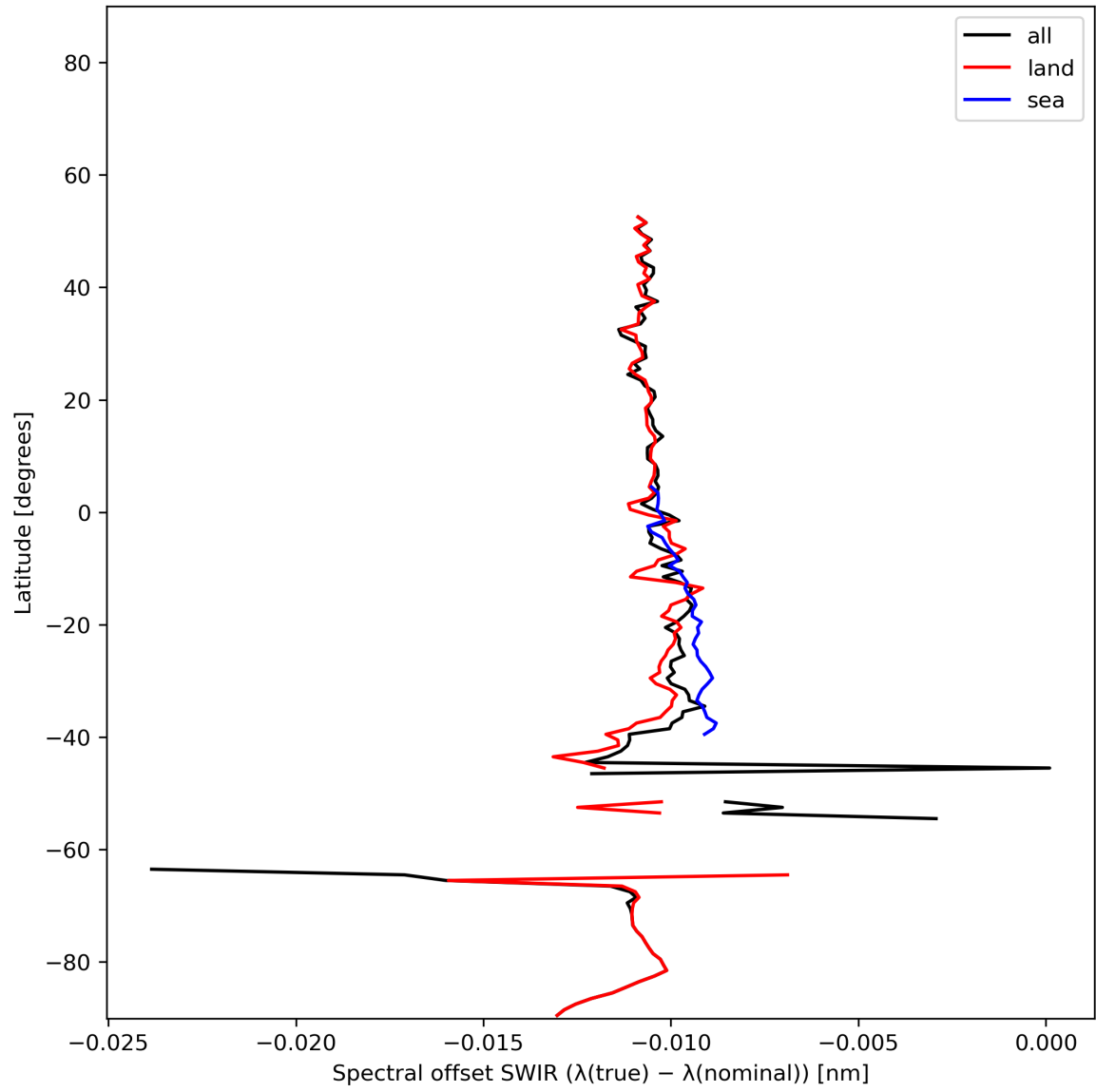
Figure 16: Zonal average of “Spectral offset SWIR ( \lambda(\text{true}) - \lambda(\text{nominal}) )” for 2024-01-08 to 2024-01-10.
