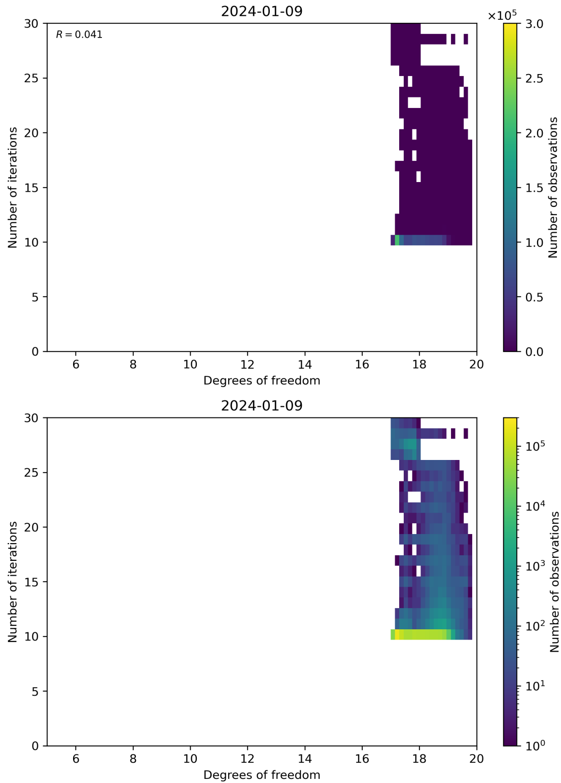
Figure 52: Scatter density plot of “Degrees of freedom” against “Number of iterations” for 2024-01-08 to 2024-01-10.
