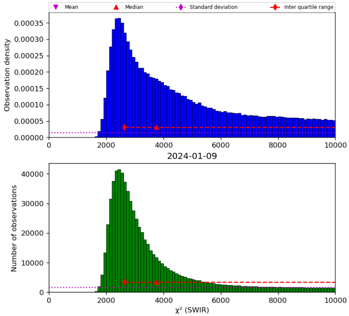
Figure 28: Histogram of “ \chi^2 (SWIR)” for 2024-01-08 to 2024-01-10
