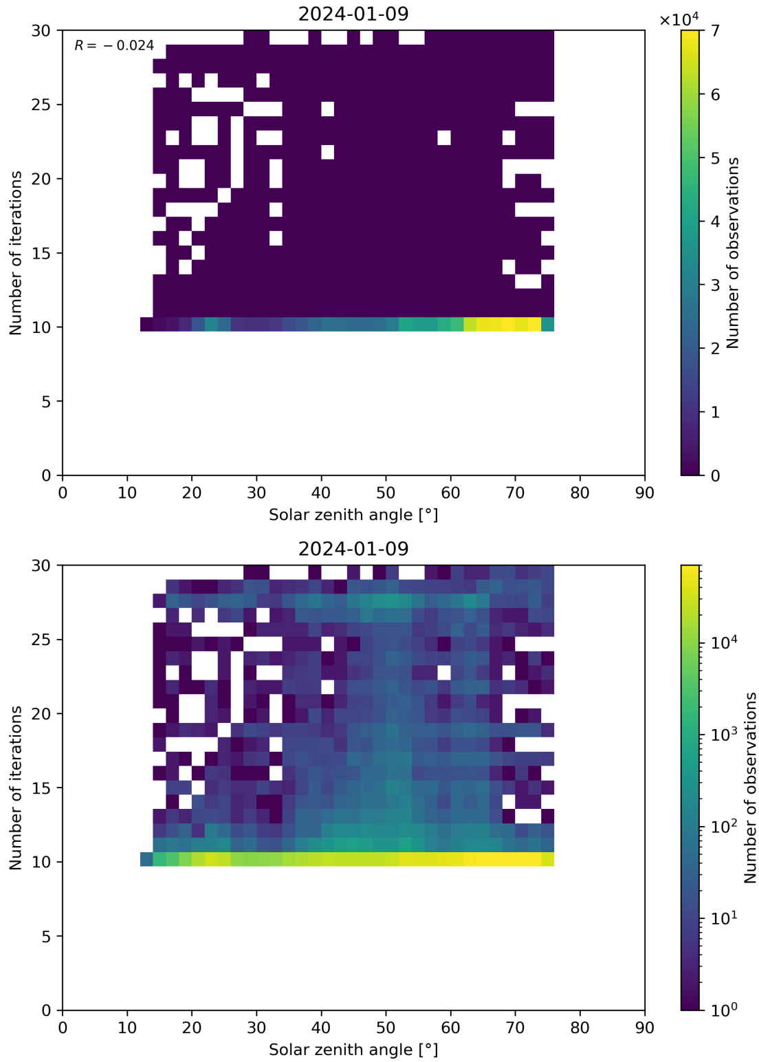
Figure 102: Scatter density plot of “Solar zenith angle” against “Number of iterations” for 2024-01-08 to 2024-01-10.
