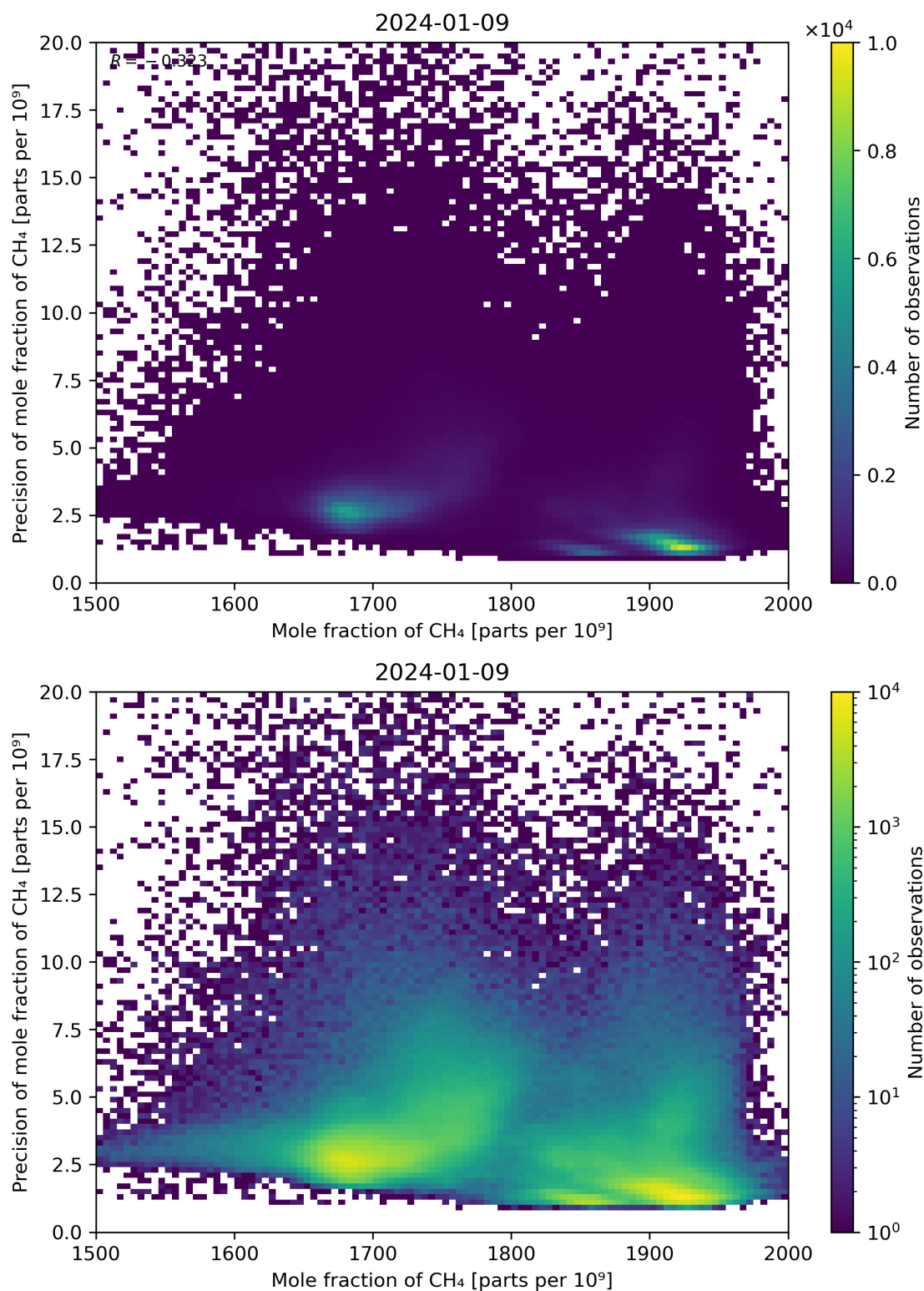
Figure 75: Scatter density plot of “Mole fraction of CH 4 ” against “Precision of mole fraction of CH 4 ” for 2024-01-08 to 2024-01-10.
