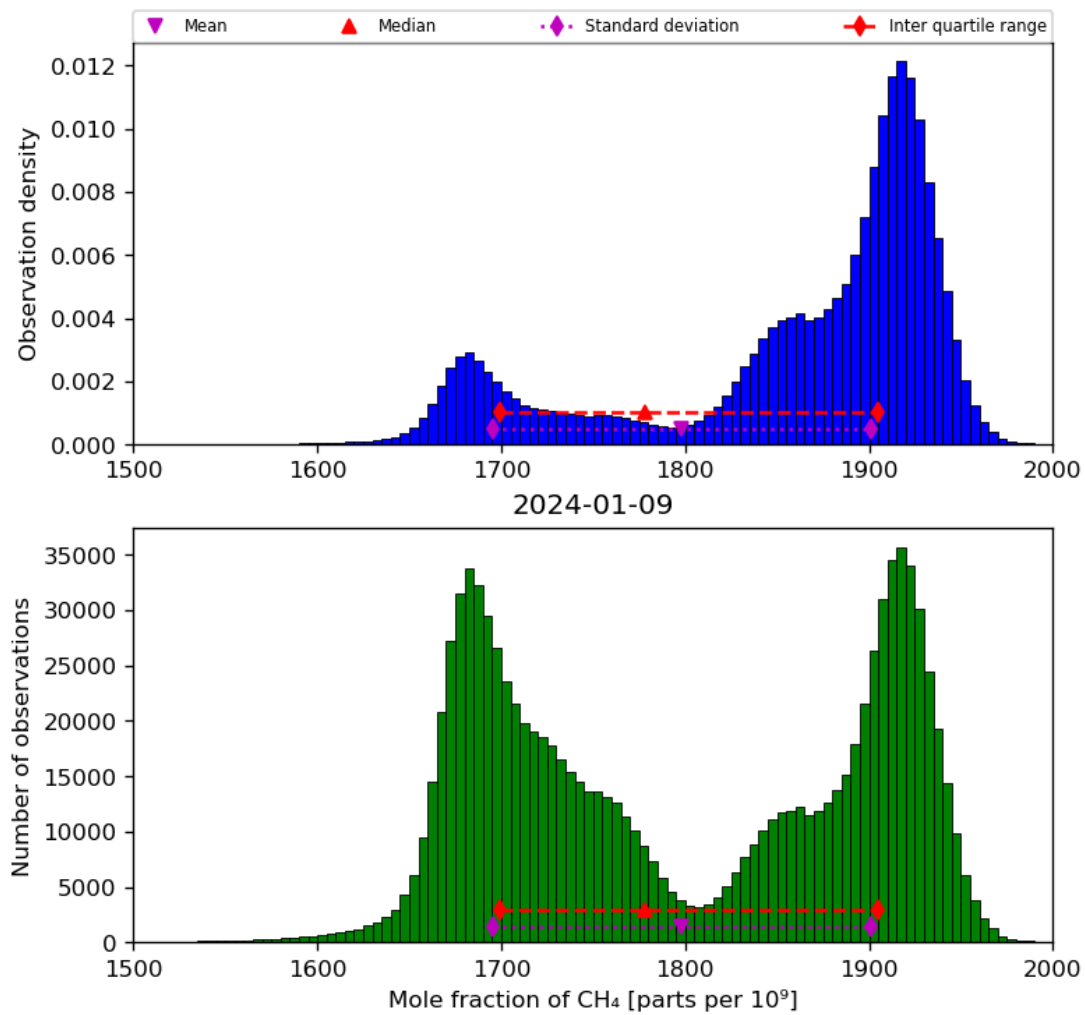
Figure 23: Histogram of “Mole fraction of CH 4 ” for 2024-01-08 to 2024-01-10
