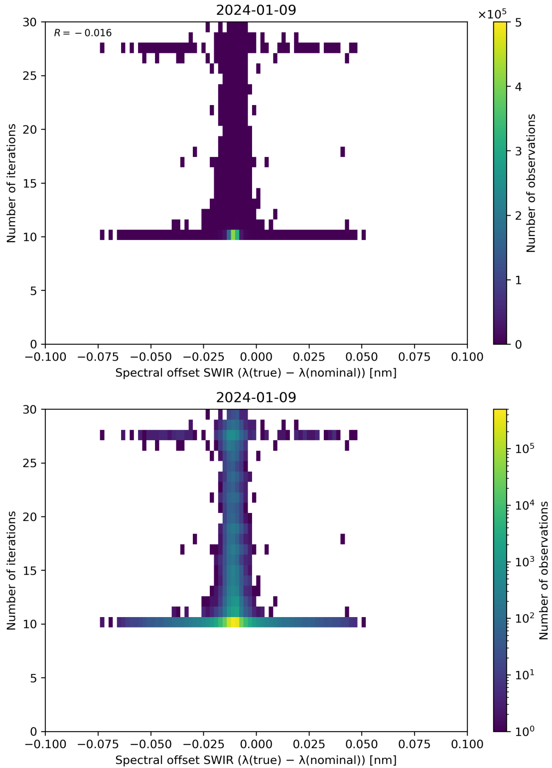
Figure 121: Scatter density plot of “Spectral offset SWIR ( \lambda(\text{true}) - \lambda(\text{nominal}) )” against “Number of iterations” for 2024-01-08 to 2024-01-10.
