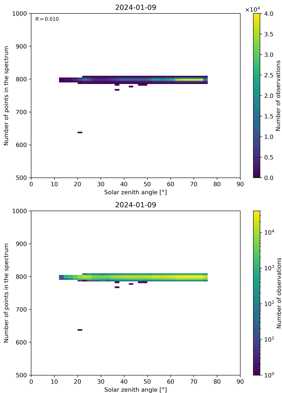
Figure 103: Scatter density plot of “Solar zenith angle” against “Number of points in the spectrum” for 2024-01-08 to 2024-01-10.
