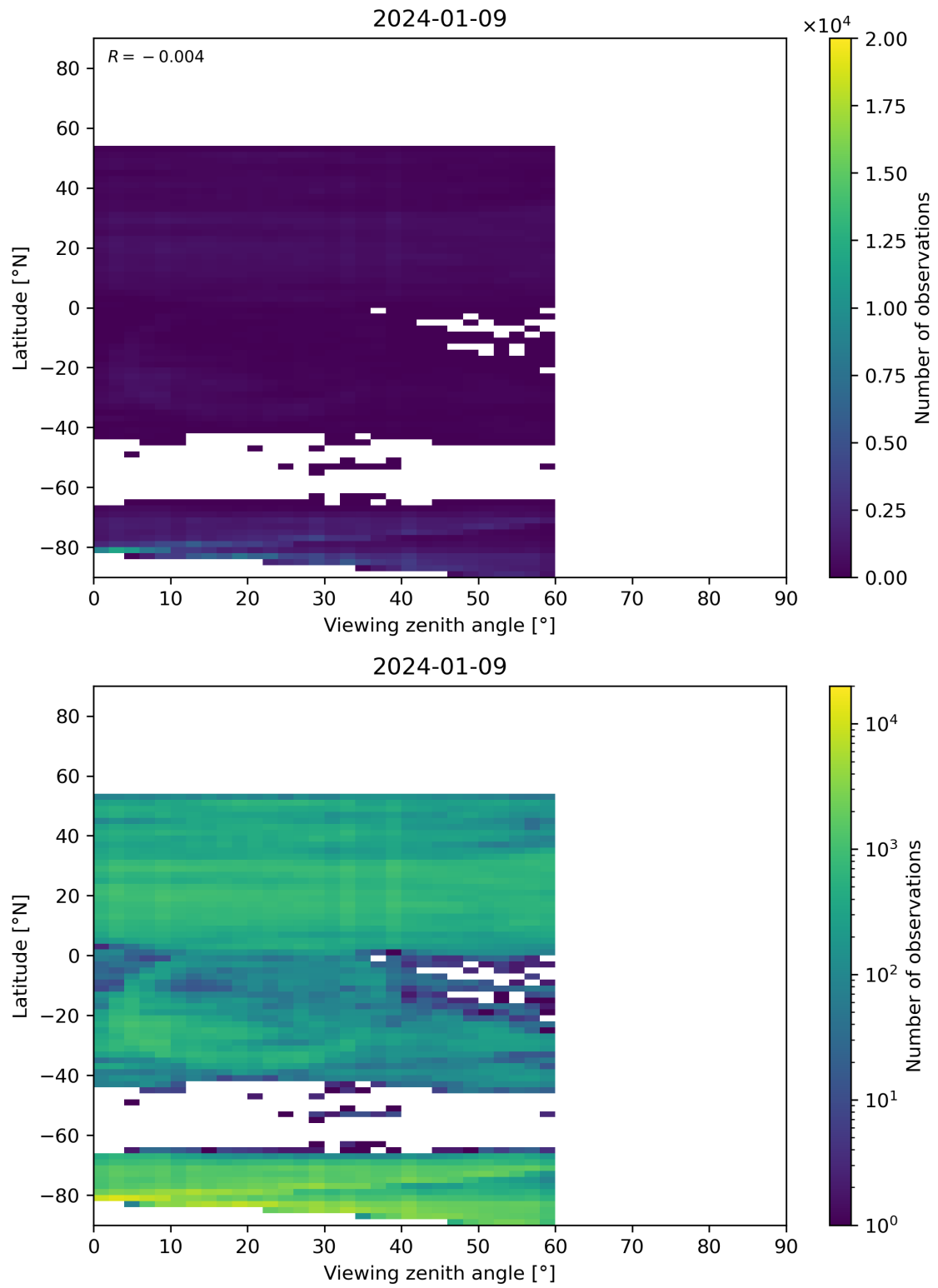
Figure 109: Scatter density plot of “Viewing zenith angle” against “Latitude” for 2024-01-08 to 2024-01-10.
