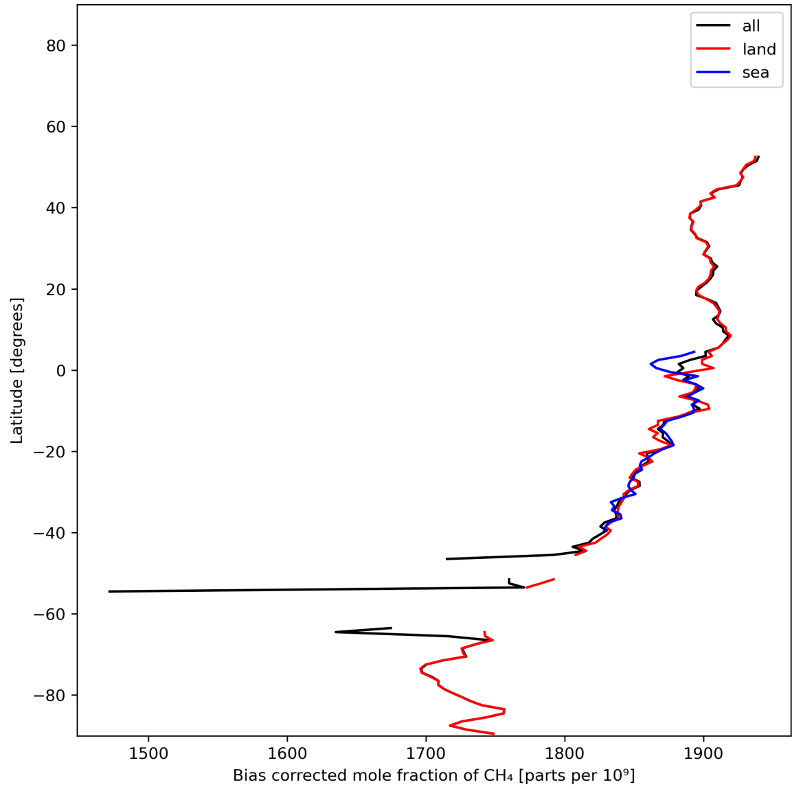
Figure 14: Zonal average of “Bias corrected mole fraction of CH 4 ” for 2024-01-08 to 2024-01-10.
