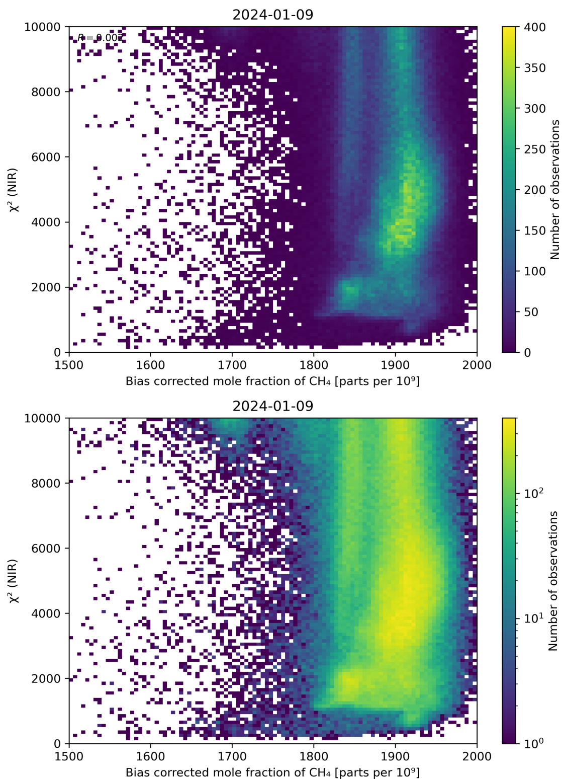
Figure 63: Scatter density plot of “Bias corrected mole fraction of \text{CH}_4 ” against “ \chi^2 (NIR)” for 2024-01-08 to 2024-01-10.
