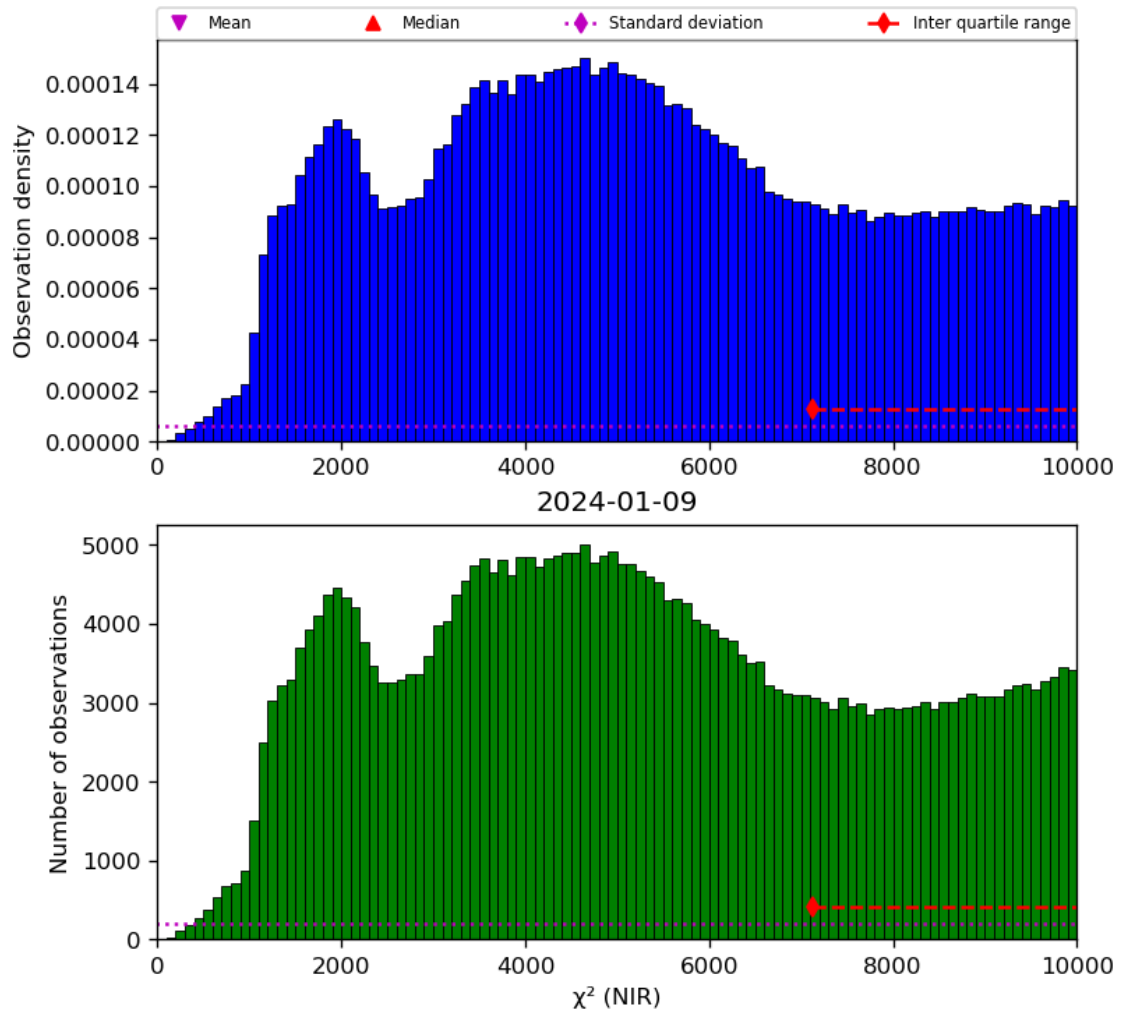
Figure 29: Histogram of “ \chi^2 (NIR)” for 2024-01-08 to 2024-01-10
