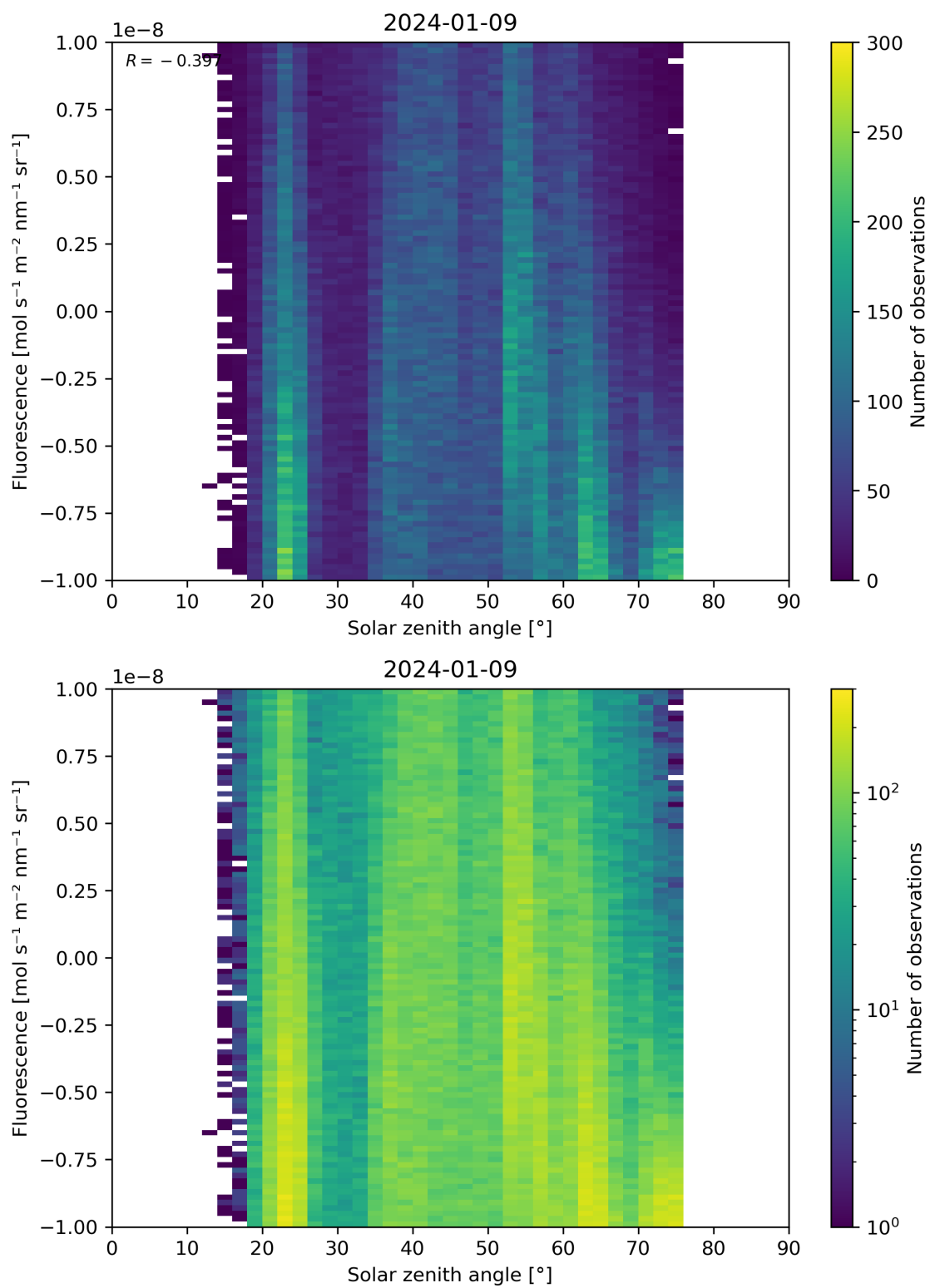
Figure 97: Scatter density plot of “Solar zenith angle” against “Fluorescence” for 2024-01-08 to 2024-01-10.
