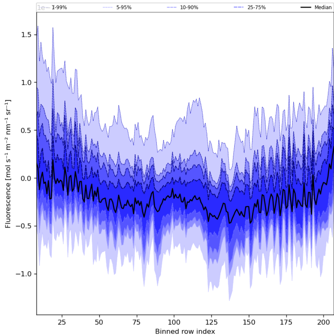
Figure 43: Along track statistics of “Fluorescence” for 2024-01-08 to 2024-01-10
