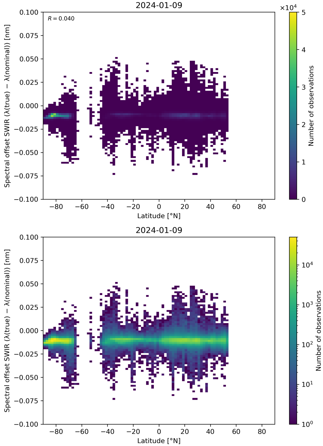
Figure 62: Scatter density plot of “Latitude” against “Spectral offset SWIR ( \lambda(\text{true}) - \lambda(\text{nominal}) )” for 2024-01-08 to 2024-01-10.
