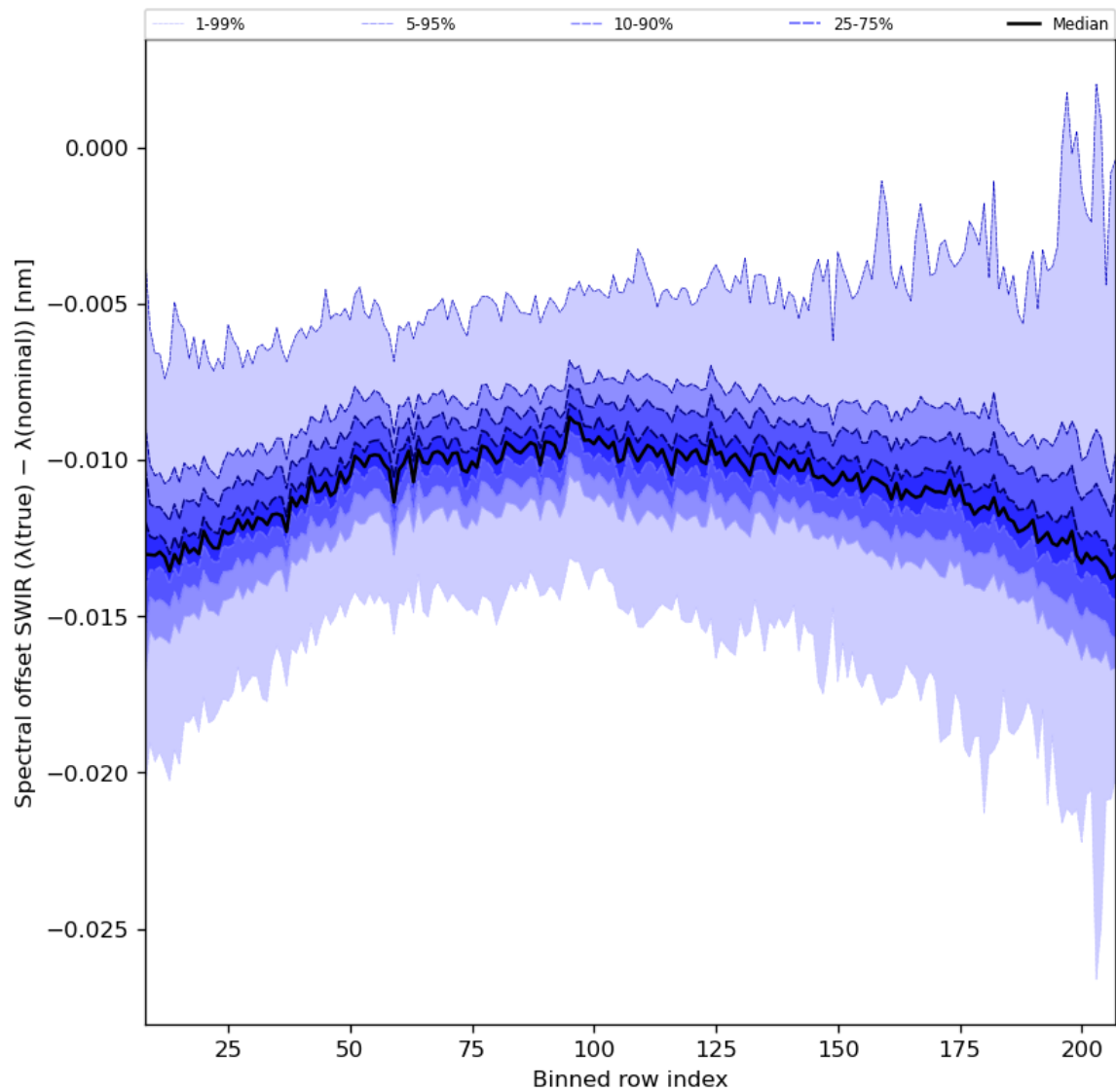
Figure 38: Along track statistics of “Spectral offset SWIR ( \lambda(\text{true}) - \lambda(\text{nominal}) )” for 2024-01-08 to 2024-01-10
