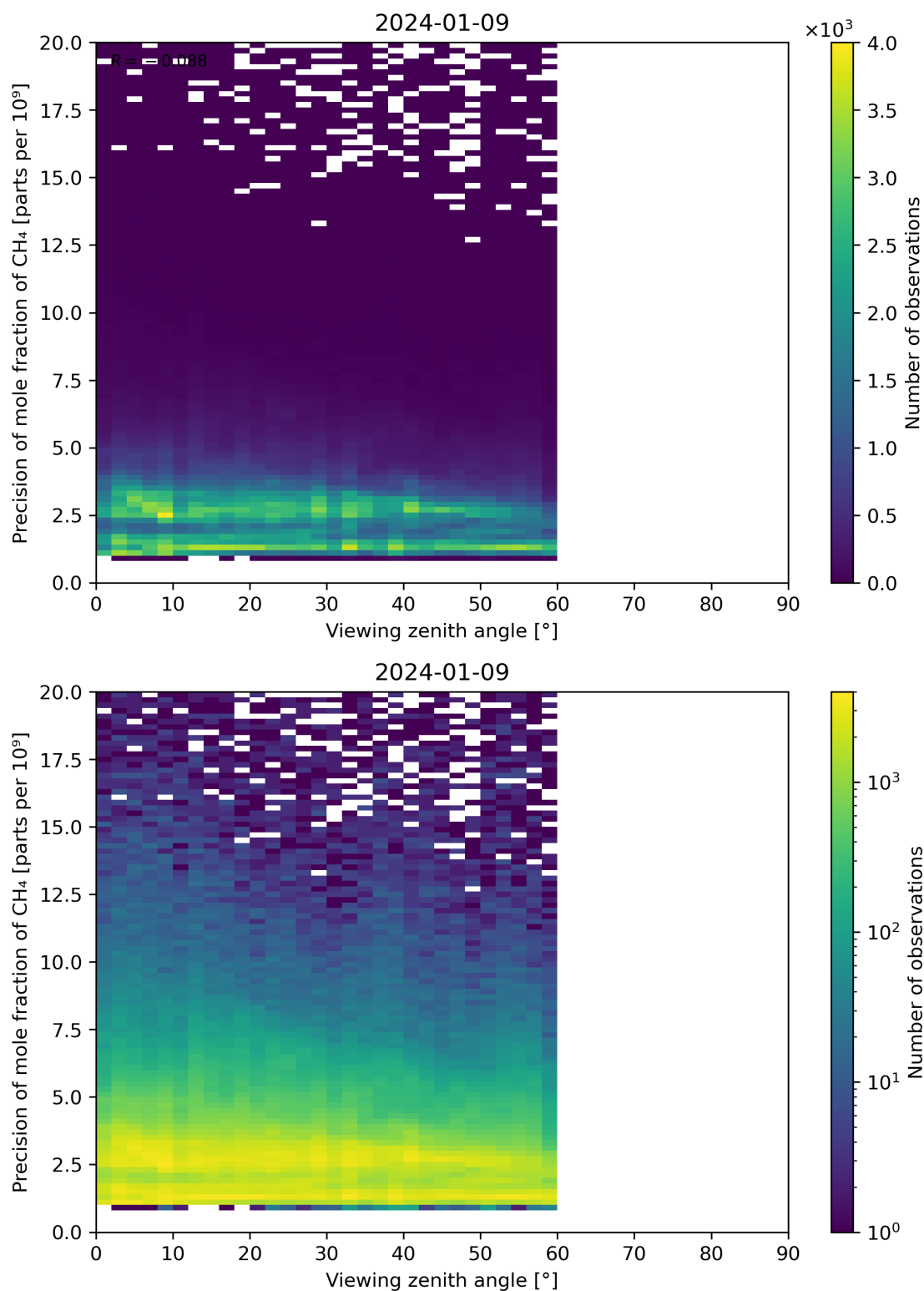
Figure 112: Scatter density plot of “Viewing zenith angle” against “Precision of mole fraction of CH 4 ” for 2024-01-08 to 2024-01-10.
