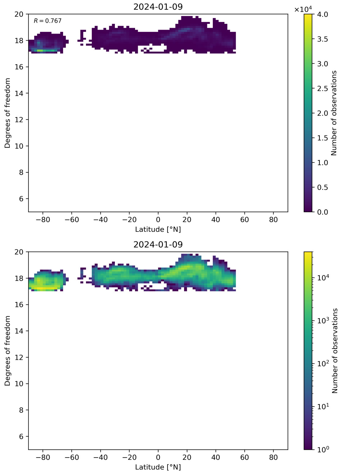
Figure 55: Scatter density plot of “Latitude” against “Degrees of freedom” for 2024-01-08 to 2024-01-10.
