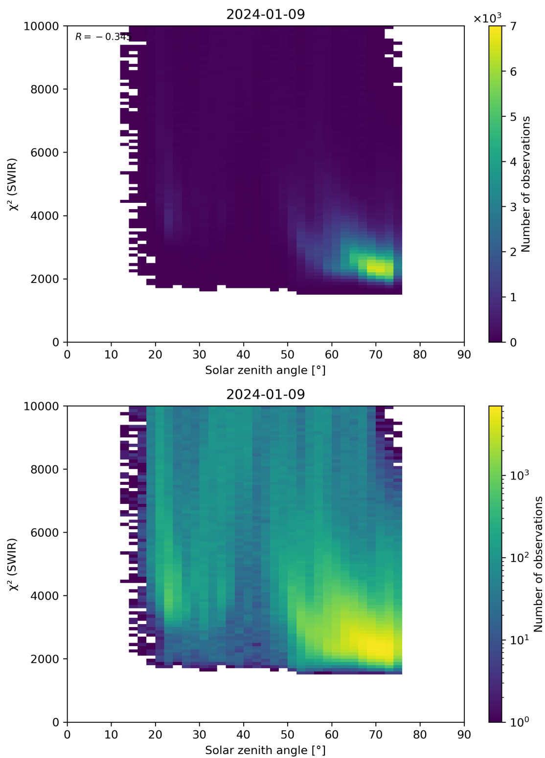
Figure 95: Scatter density plot of “Solar zenith angle” against “ \chi^2 (SWIR)” for 2024-01-08 to 2024-01-10.
