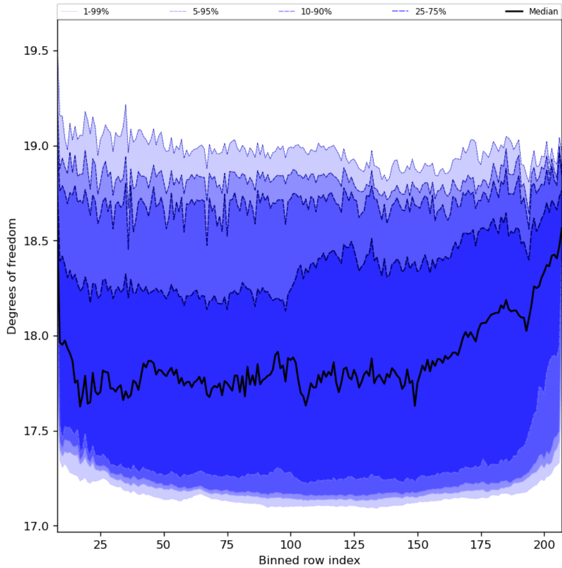
Figure 41: Along track statistics of “Degrees of freedom” for 2024-01-08 to 2024-01-10
