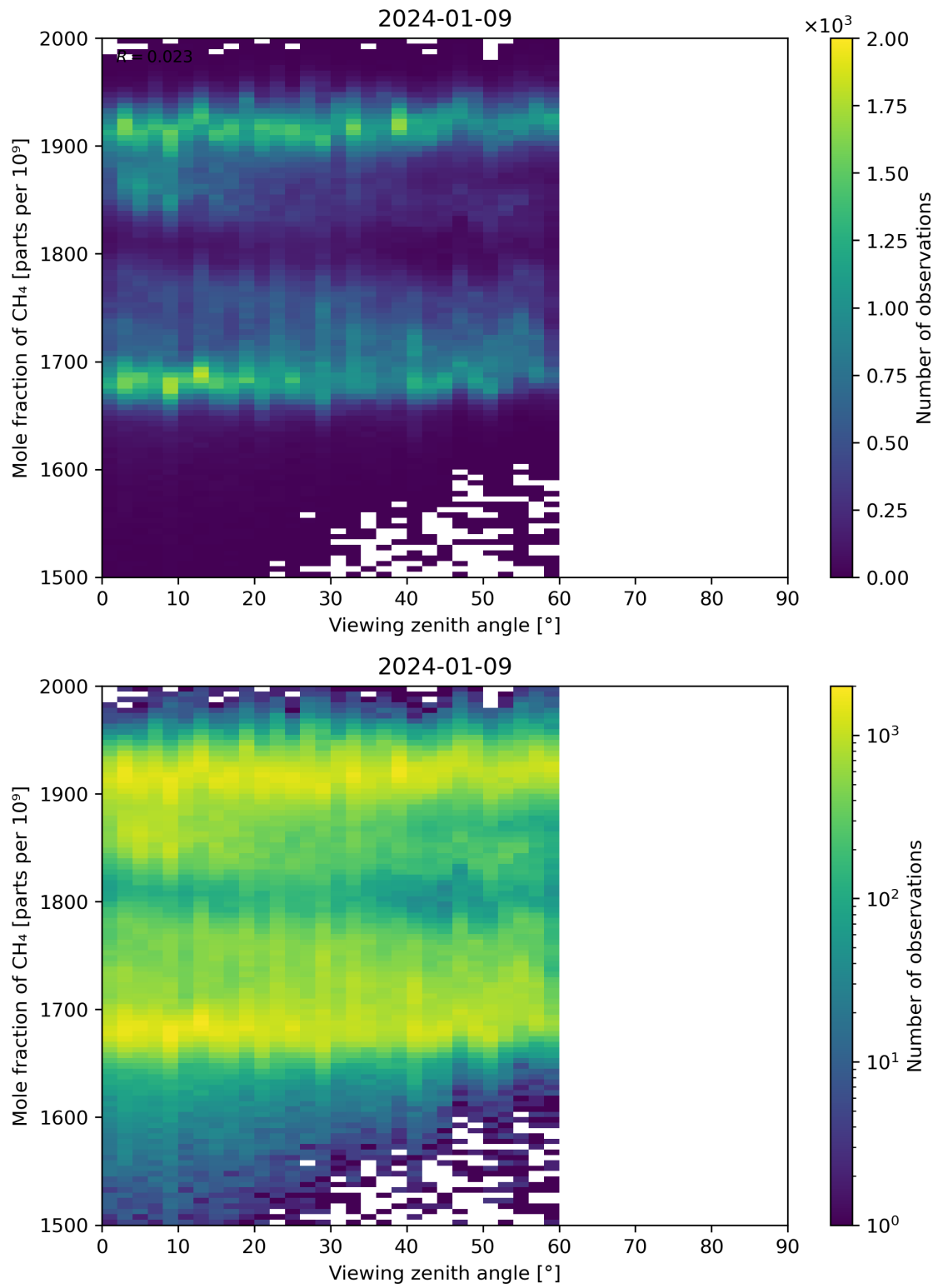
Figure 110: Scatter density plot of “Viewing zenith angle” against “Mole fraction of CH 4 ” for 2024-01-08 to 2024-01-10.
