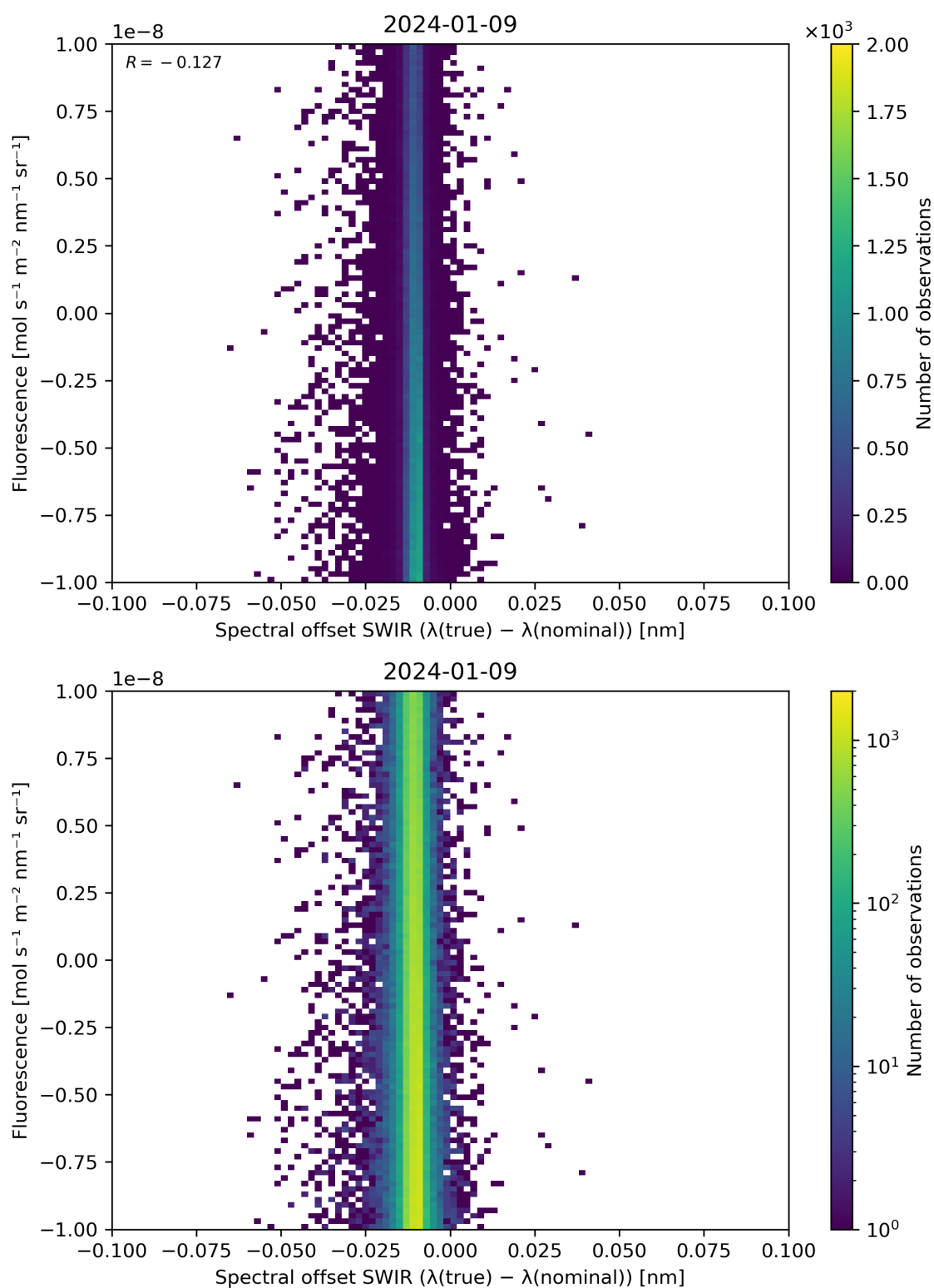
Figure 120: Scatter density plot of “Spectral offset SWIR ( \lambda(\text{true}) - \lambda(\text{nominal}) )” against “Fluorescence” for 2024-01-08 to 2024-01-10.
