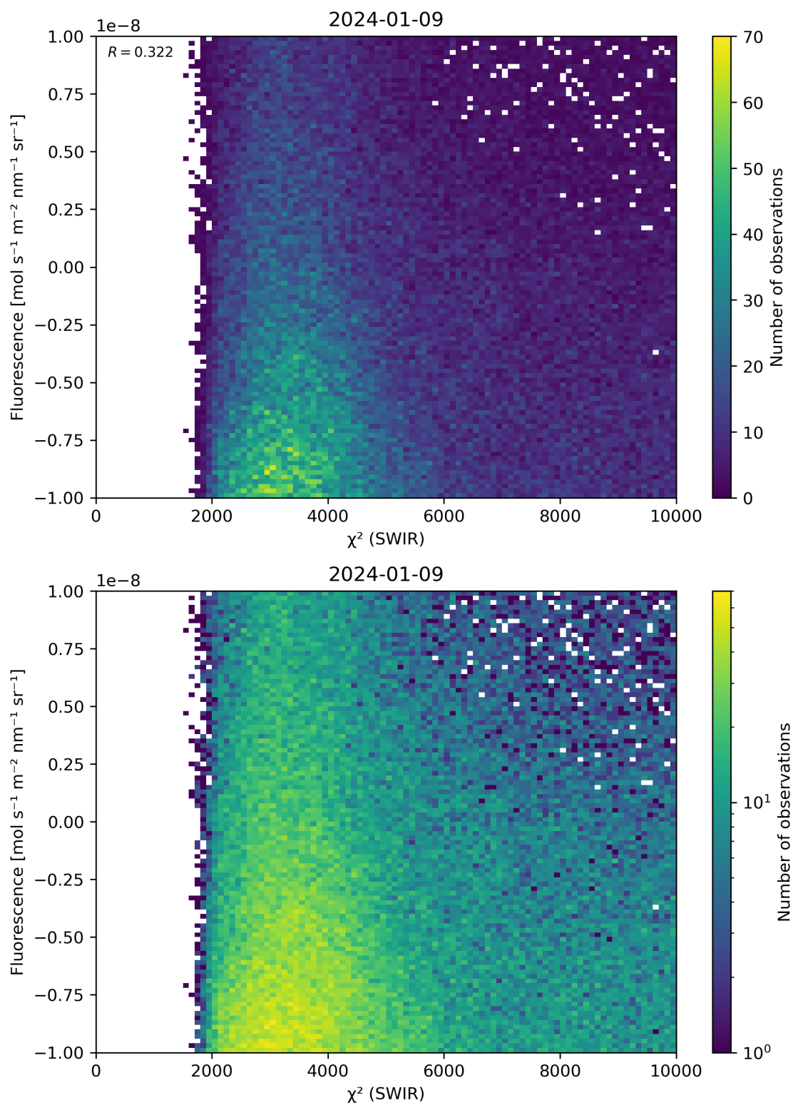
Figure 49: Scatter density plot of “ \chi^2 (SWIR)” against “Fluorescence” for 2024-01-08 to 2024-01-10.
