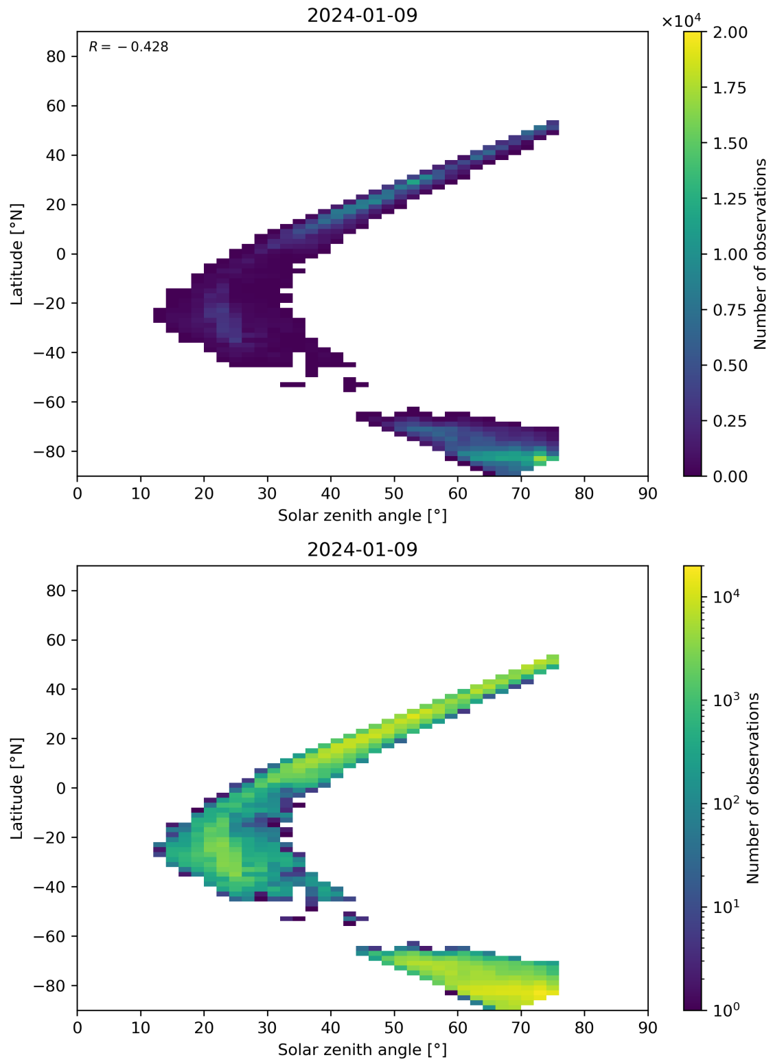
Figure 98: Scatter density plot of “Solar zenith angle” against “Latitude” for 2024-01-08 to 2024-01-10.
