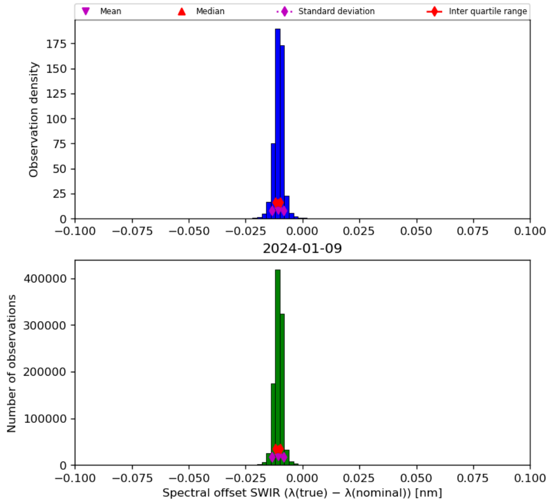
Figure 27: Histogram of “Spectral offset SWIR ( \lambda(\text{true}) - \lambda(\text{nominal}) )” for 2024-01-08 to 2024-01-10
