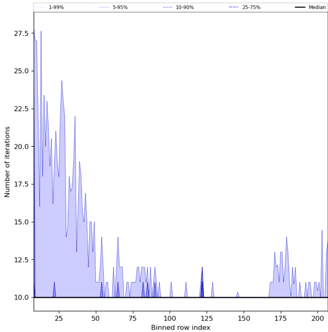
Figure 42: Along track statistics of “Number of iterations” for 2024-01-08 to 2024-01-10
