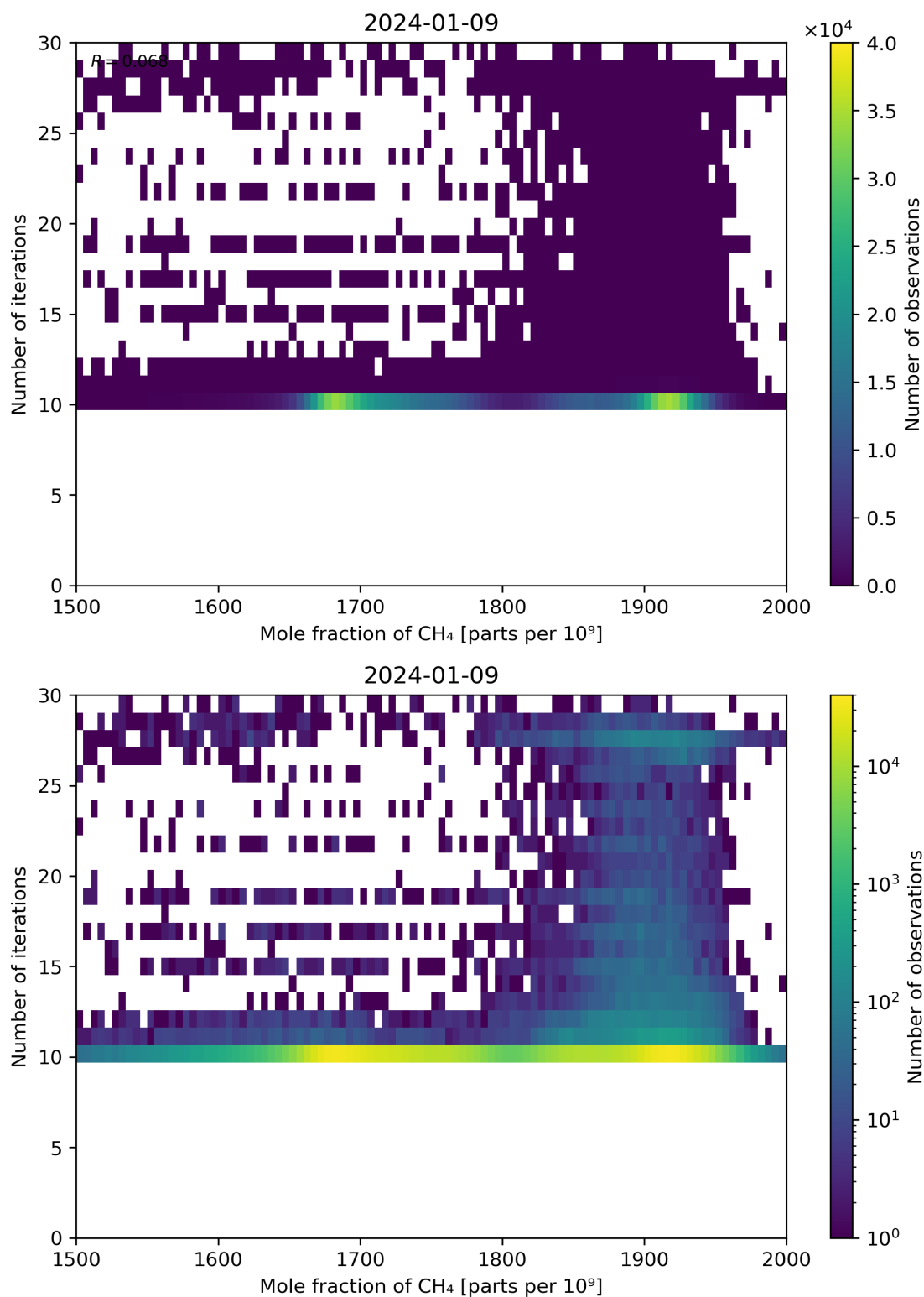
Figure 76: Scatter density plot of “Mole fraction of CH 4 ” against “Number of iterations” for 2024-01-08 to 2024-01-10.
