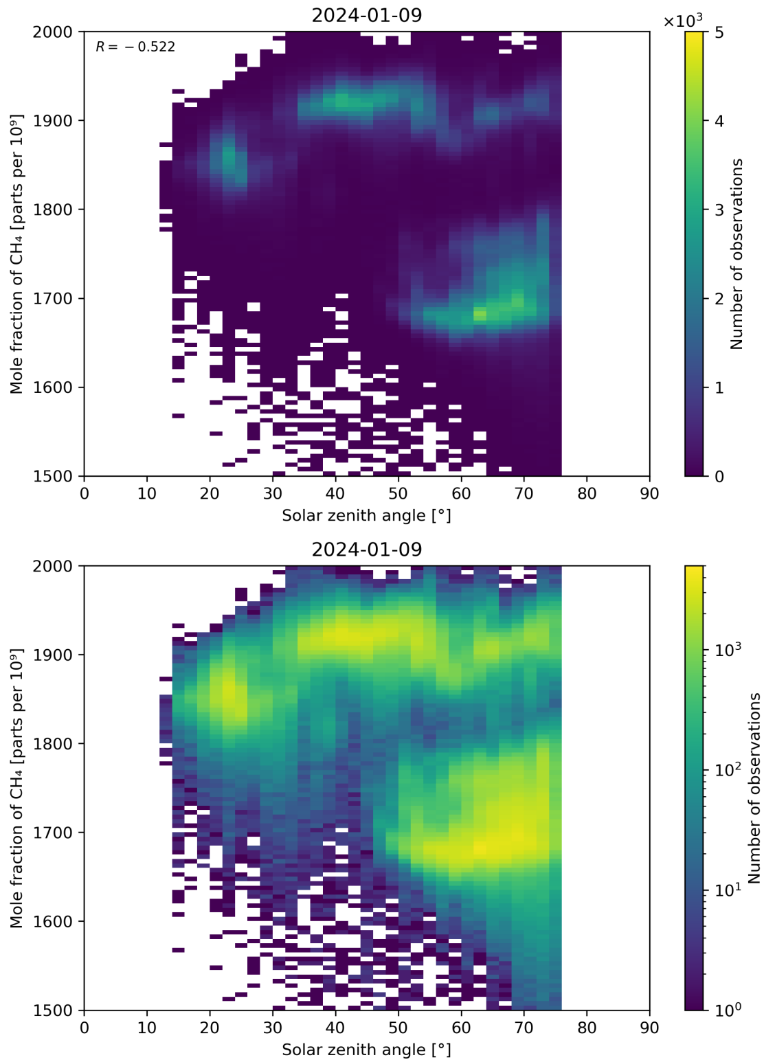
Figure 99: Scatter density plot of “Solar zenith angle” against “Mole fraction of CH 4 ” for 2024-01-08 to 2024-01-10.
