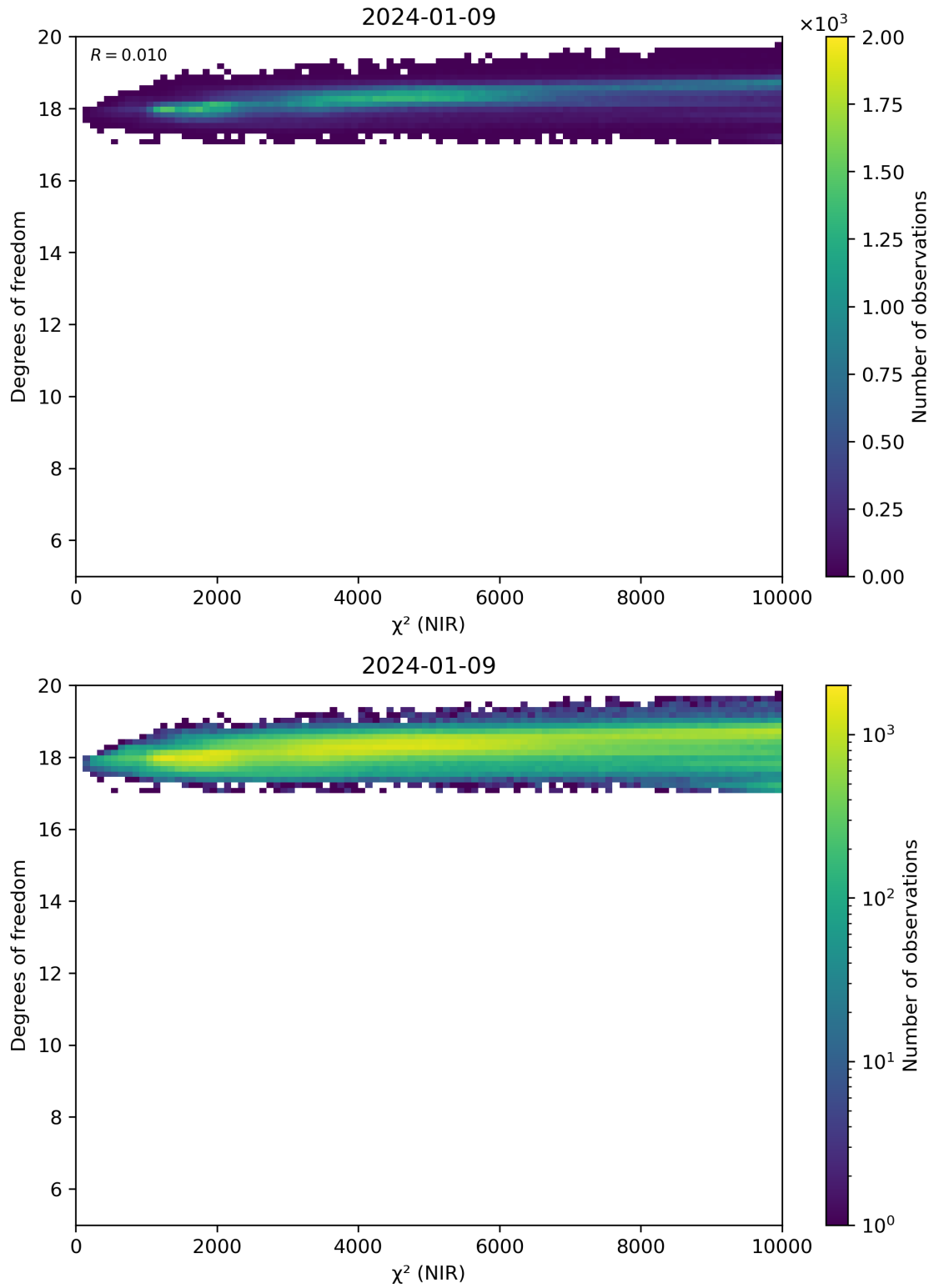
Figure 44: Scatter density plot of “ \chi^2 (NIR)” against “Degrees of freedom” for 2024-01-08 to 2024-01-10.
