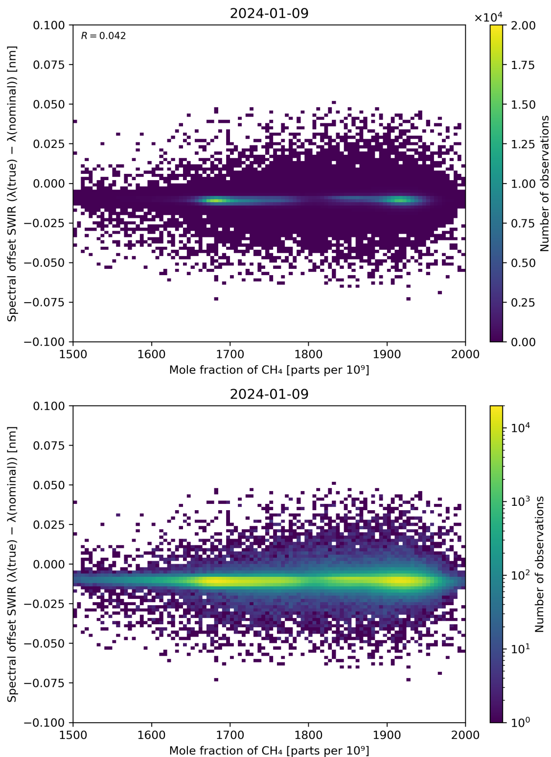
Figure 86: Scatter density plot of “Mole fraction of CH 4 ” against “Spectral offset SWIR ( \lambda(\text{true}) - \lambda(\text{nominal}) )” for 2024-01-08 to 2024-01-10.
