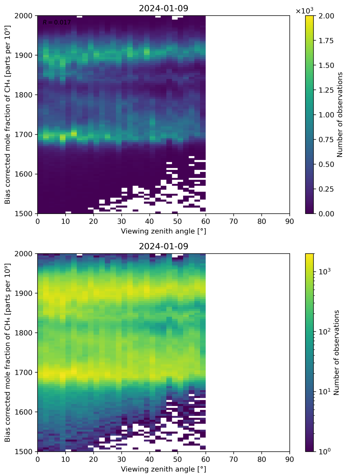
Figure 111: Scatter density plot of “Viewing zenith angle” against “Bias corrected mole fraction of CH 4 ” for 2024-01-08 to 2024-01-10.
