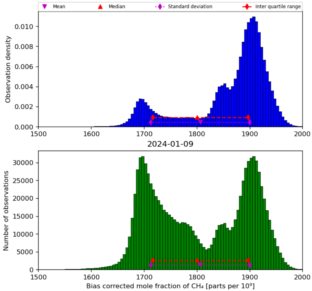
Figure 25: Histogram of “Bias corrected mole fraction of CH 4 ” for 2024-01-08 to 2024-01-10
