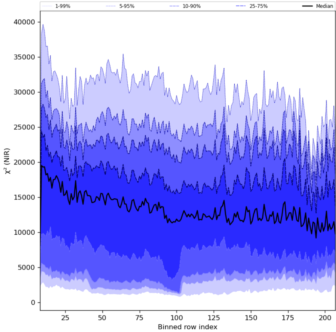
Figure 40: Along track statistics of “ \chi^2 (NIR)” for 2024-01-08 to 2024-01-10
