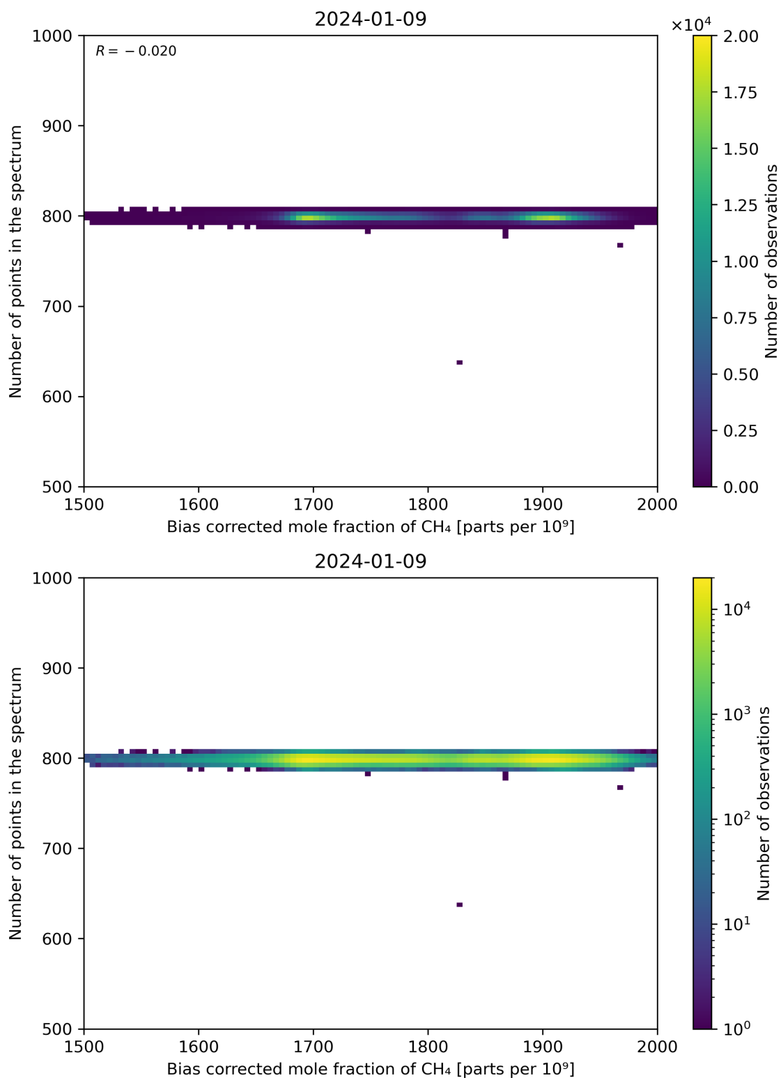
Figure 68: Scatter density plot of “Bias corrected mole fraction of CH 4 ” against “Number of points in the spectrum” for 2024-01-08 to 2024-01-10.
