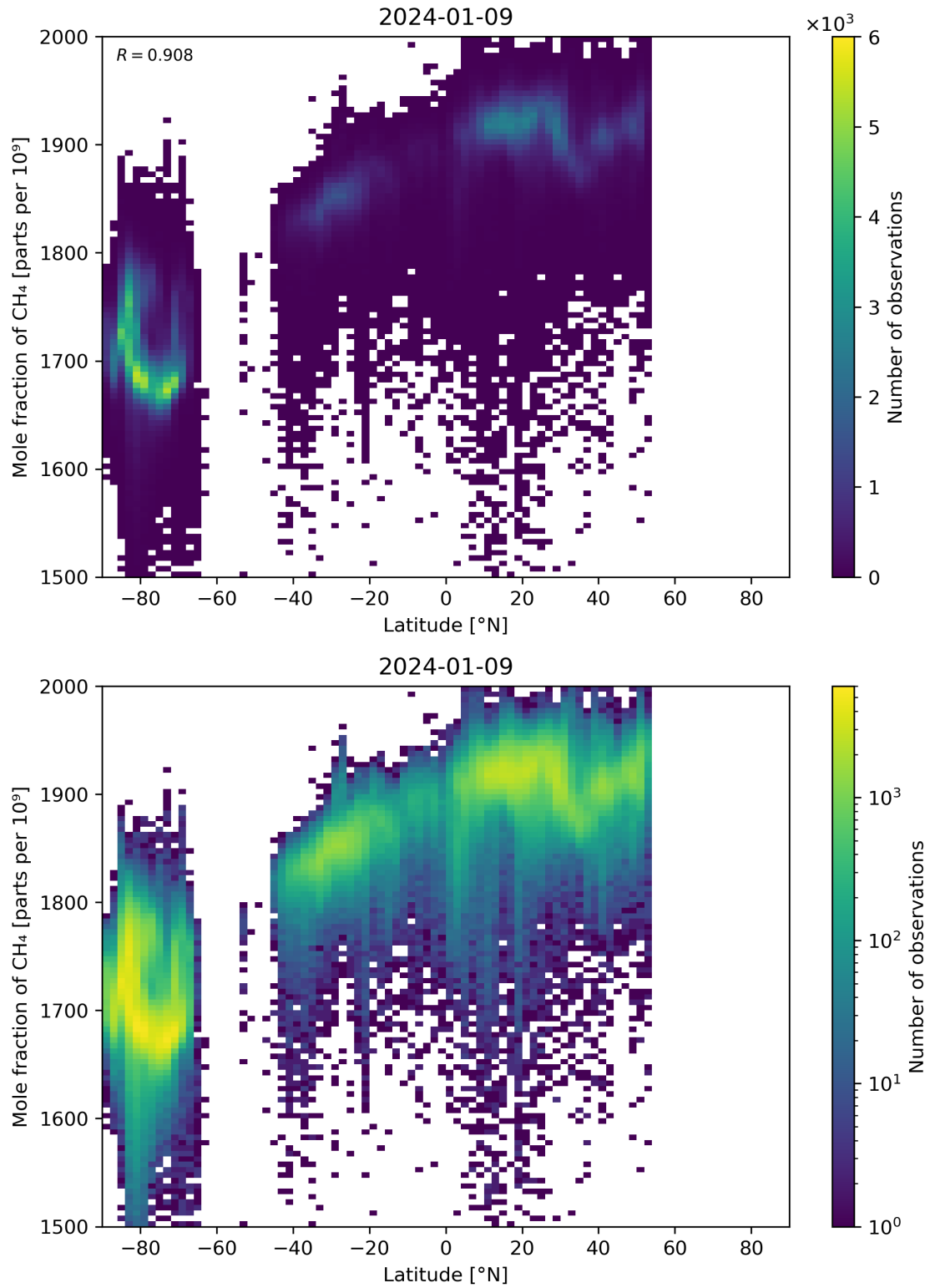
Figure 57: Scatter density plot of “Latitude” against “Mole fraction of CH 4 ” for 2024-01-08 to 2024-01-10.
