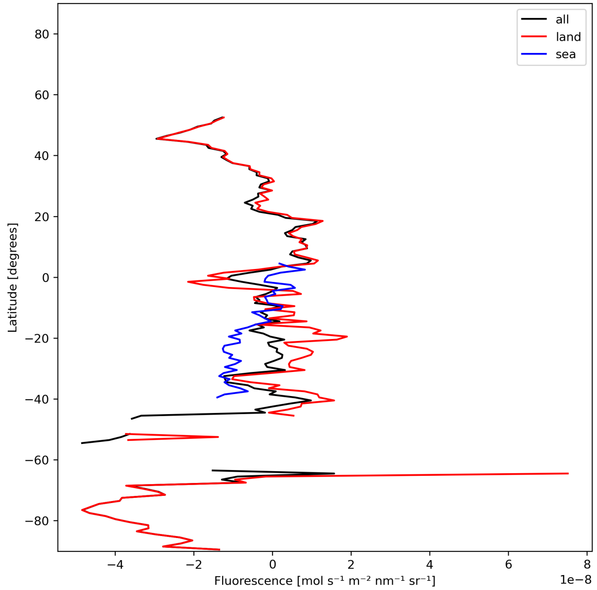
Figure 21: Zonal average of “Fluorescence” for 2024-01-08 to 2024-01-10.
