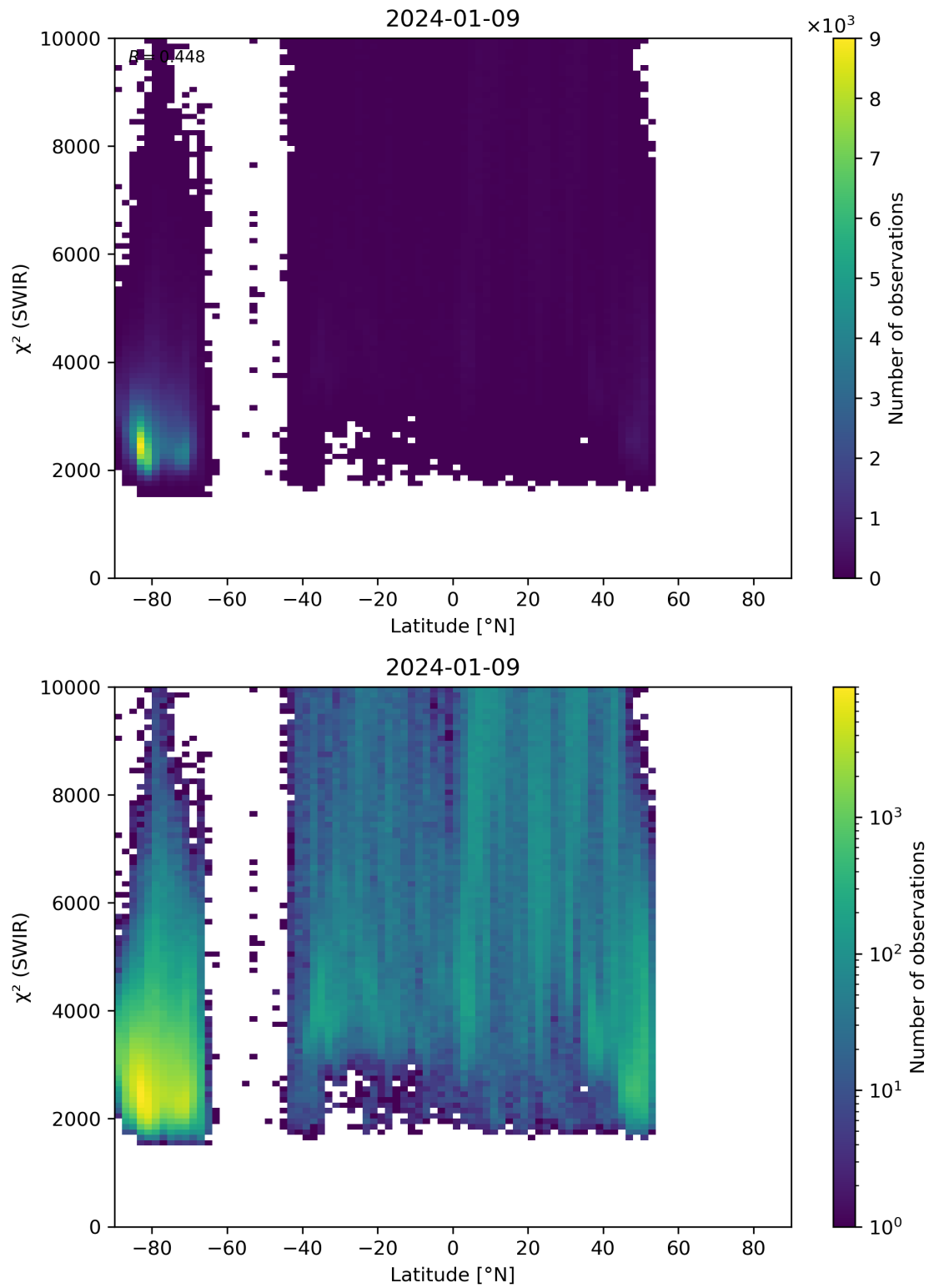
Figure 54: Scatter density plot of “Latitude” against “ \chi^2 (SWIR)” for 2024-01-08 to 2024-01-10.
