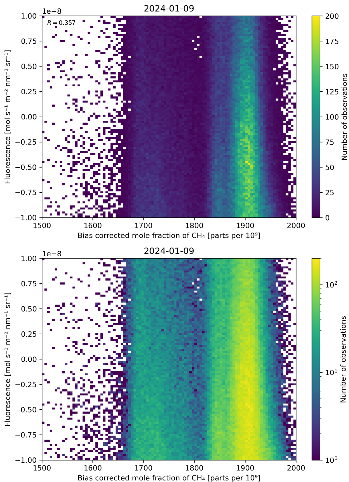
Figure 66: Scatter density plot of “Bias corrected mole fraction of \text{CH}_4 ” against “Fluorescence” for 2024-01-08 to 2024-01-10.
