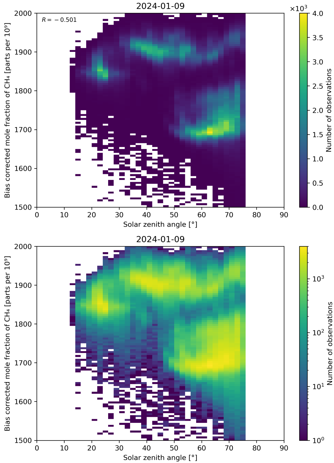
Figure 100: Scatter density plot of “Solar zenith angle” against “Bias corrected mole fraction of CH 4 ” for 2024-01-08 to 2024-01-10.
