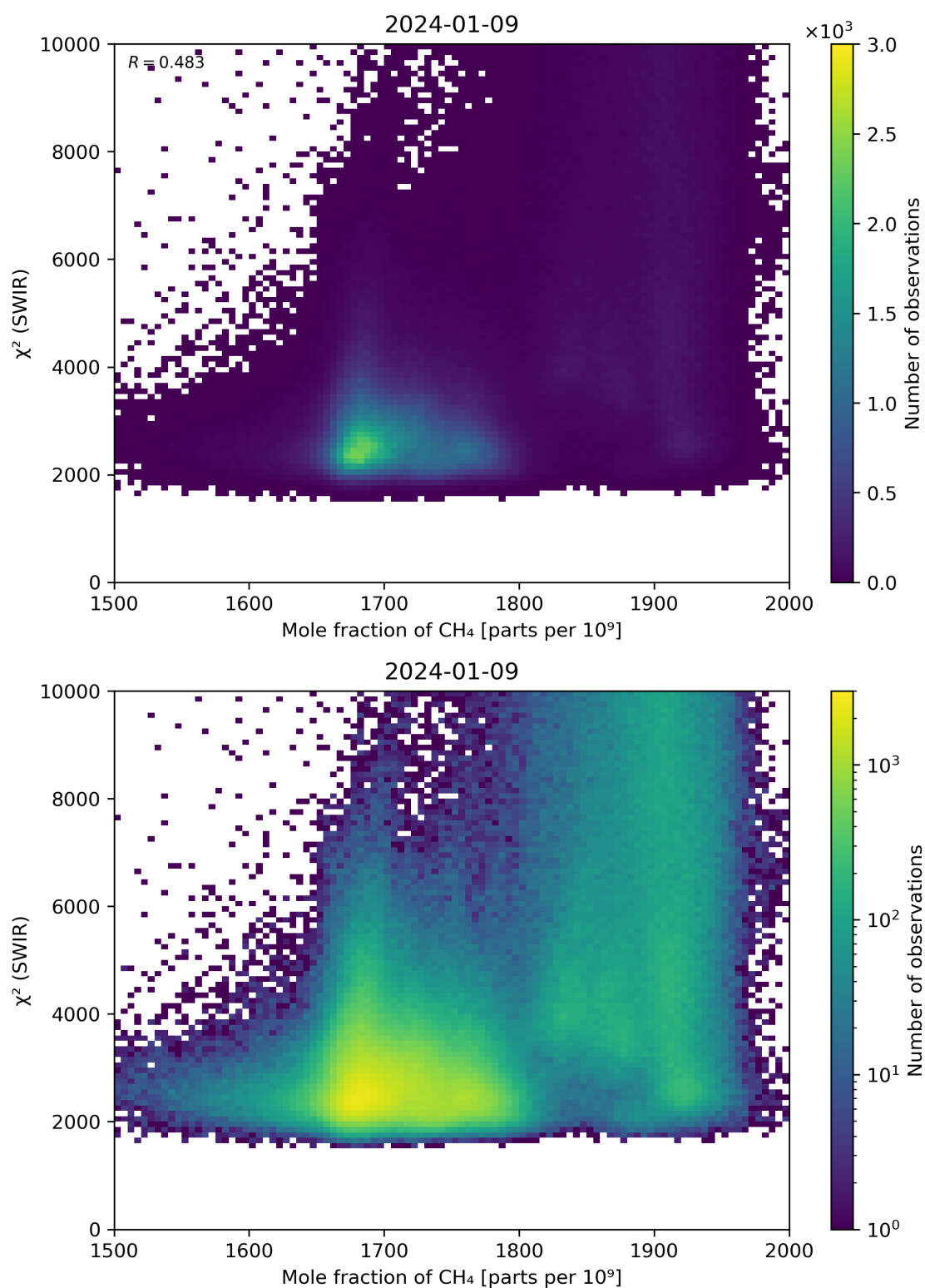
Figure 71: Scatter density plot of “Mole fraction of CH 4 ” against “ \chi^2 (SWIR)” for 2024-01-08 to 2024-01-10.
