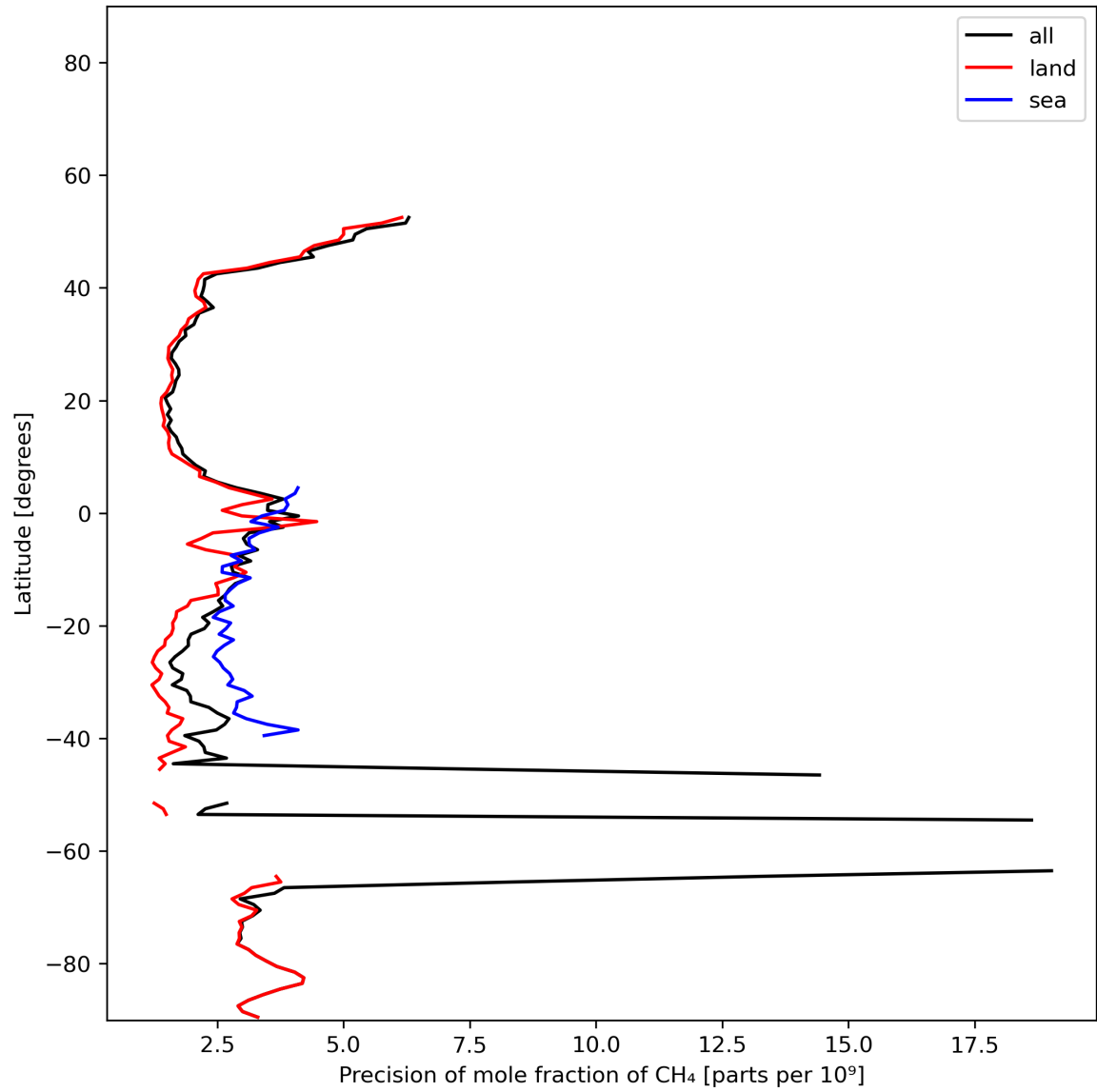
Figure 13: Zonal average of “Precision of mole fraction of CH 4 ” for 2024-01-08 to 2024-01-10.
