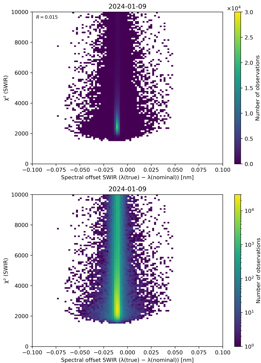
Figure 118: Scatter density plot of “Spectral offset SWIR ( \lambda(\text{true}) - \lambda(\text{nominal}) )” against “ \chi^2 (SWIR)” for 2024-01-08 to 2024-01-10.
