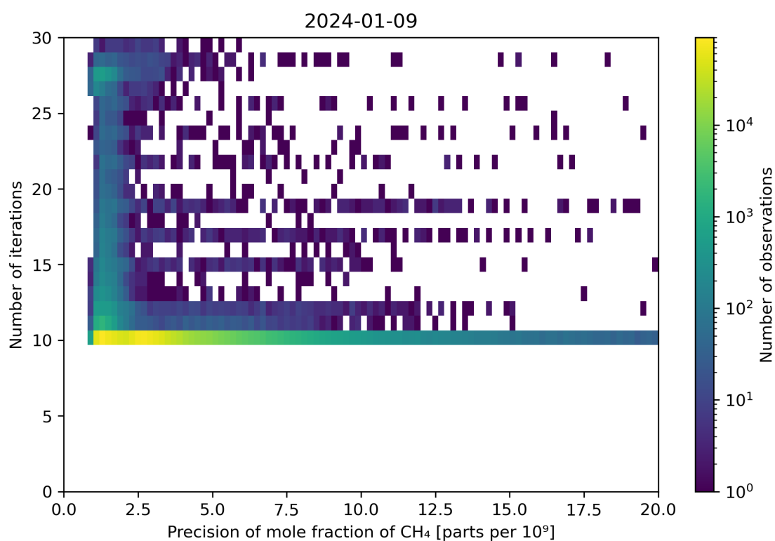
Figure 83: Scatter density plot of “Precision of mole fraction of \text{CH}_4 ” against “Number of iterations” for 2024-01-08 to 2024-01-10.
