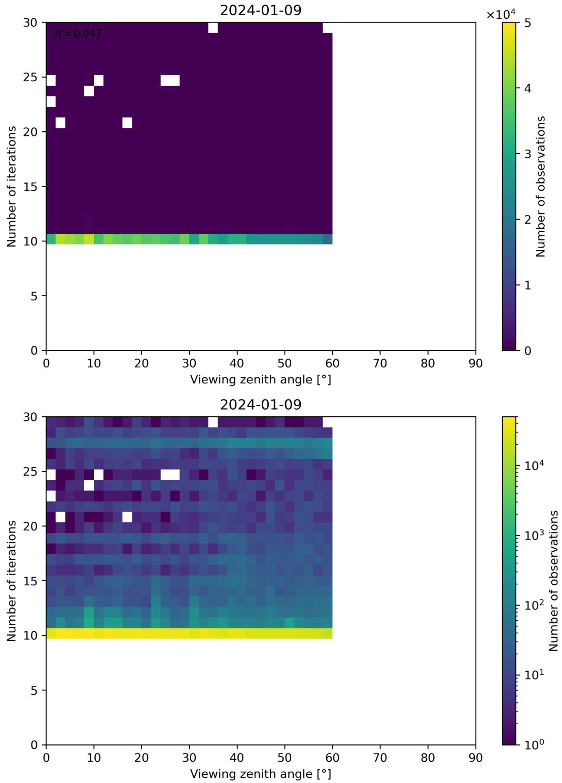
Figure 113: Scatter density plot of “Viewing zenith angle” against “Number of iterations” for 2024-01-08 to 2024-01-10.
