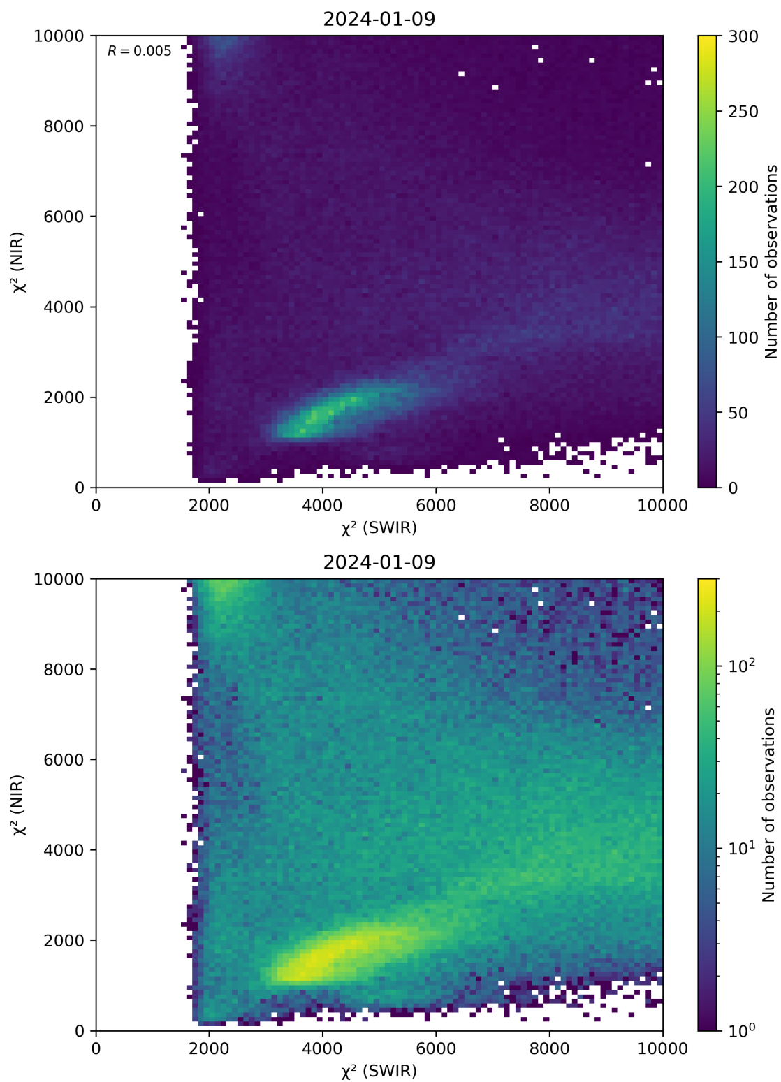
Figure 47: Scatter density plot of “ \chi^2 (SWIR)” against “ \chi^2 (NIR)” for 2024-01-08 to 2024-01-10.
