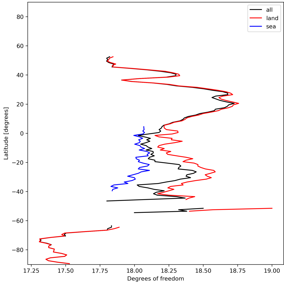
Figure 19: Zonal average of “Degrees of freedom” for 2024-01-08 to 2024-01-10.
