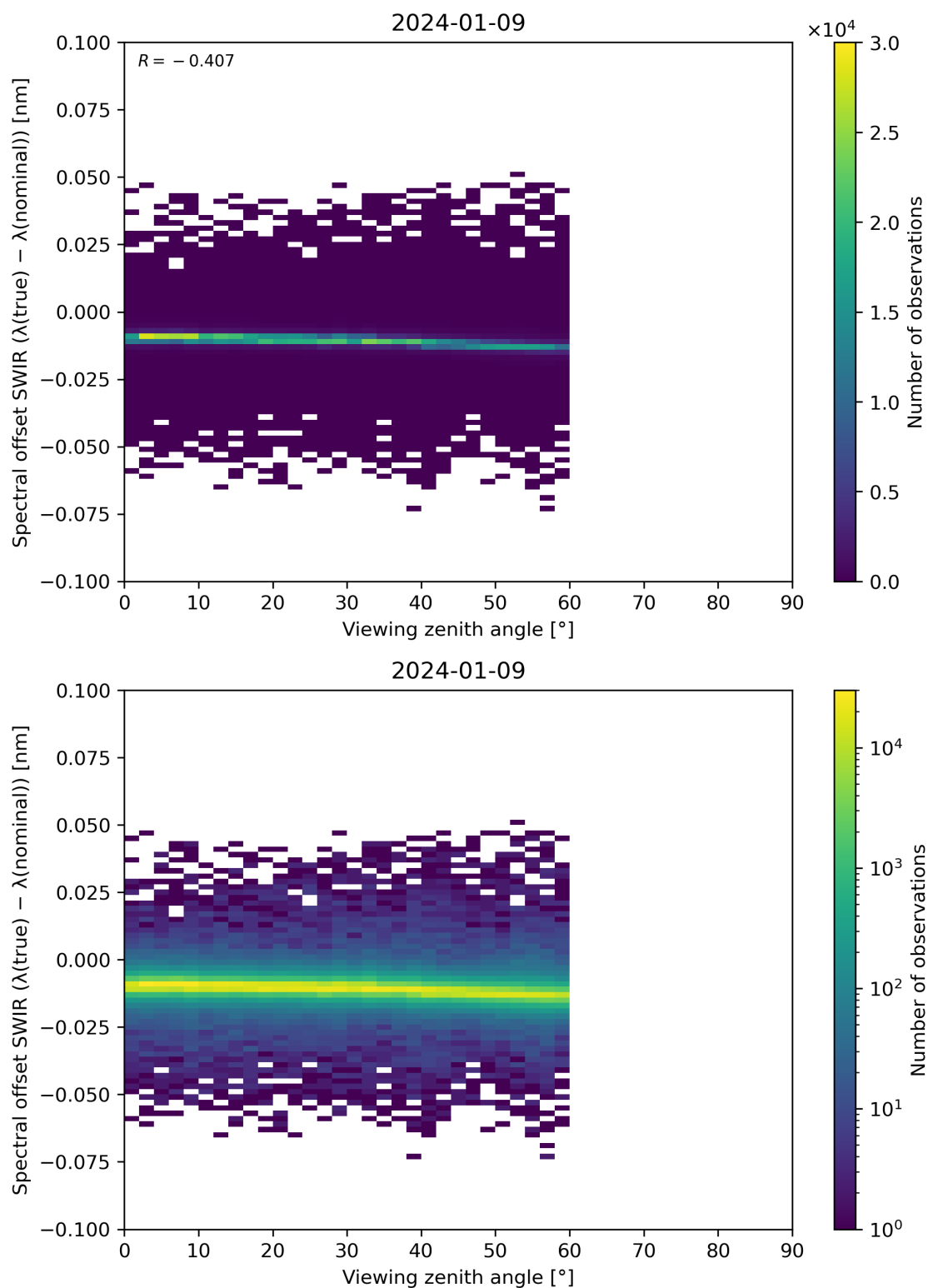
Figure 116: Scatter density plot of “Viewing zenith angle” against “Spectral offset SWIR ( \lambda(\text{true}) - \lambda(\text{nominal}) )” for 2024-01-08 to 2024-01-10.
