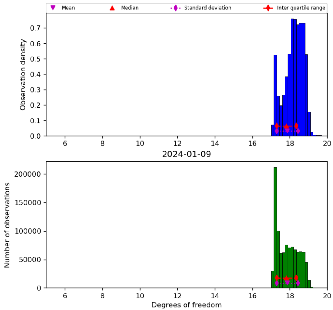
Figure 30: Histogram of “Degrees of freedom” for 2024-01-08 to 2024-01-10
