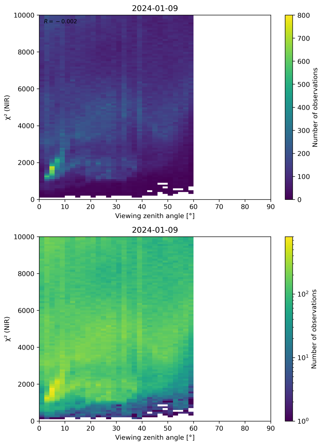
Figure 105: Scatter density plot of “Viewing zenith angle” against “ \chi^2 (NIR)” for 2024-01-08 to 2024-01-10.
