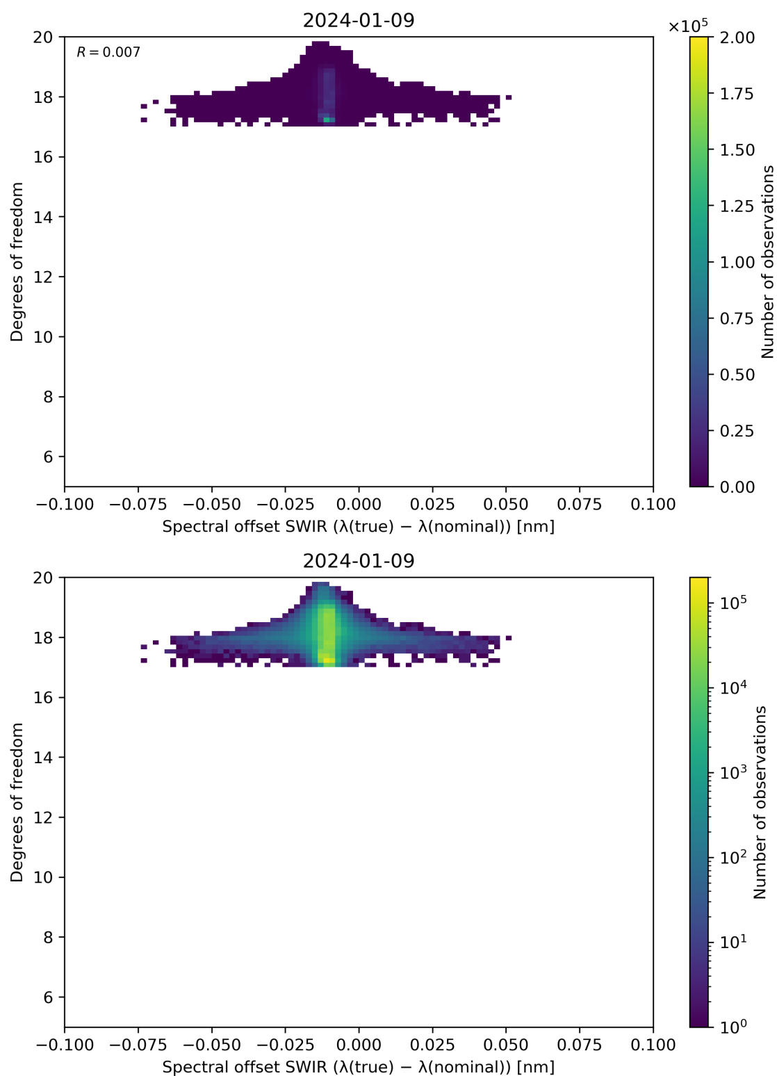
Figure 119: Scatter density plot of “Spectral offset SWIR ( \lambda(\text{true}) - \lambda(\text{nominal}) )” against “Degrees of freedom” for 2024-01-08 to 2024-01-10.
