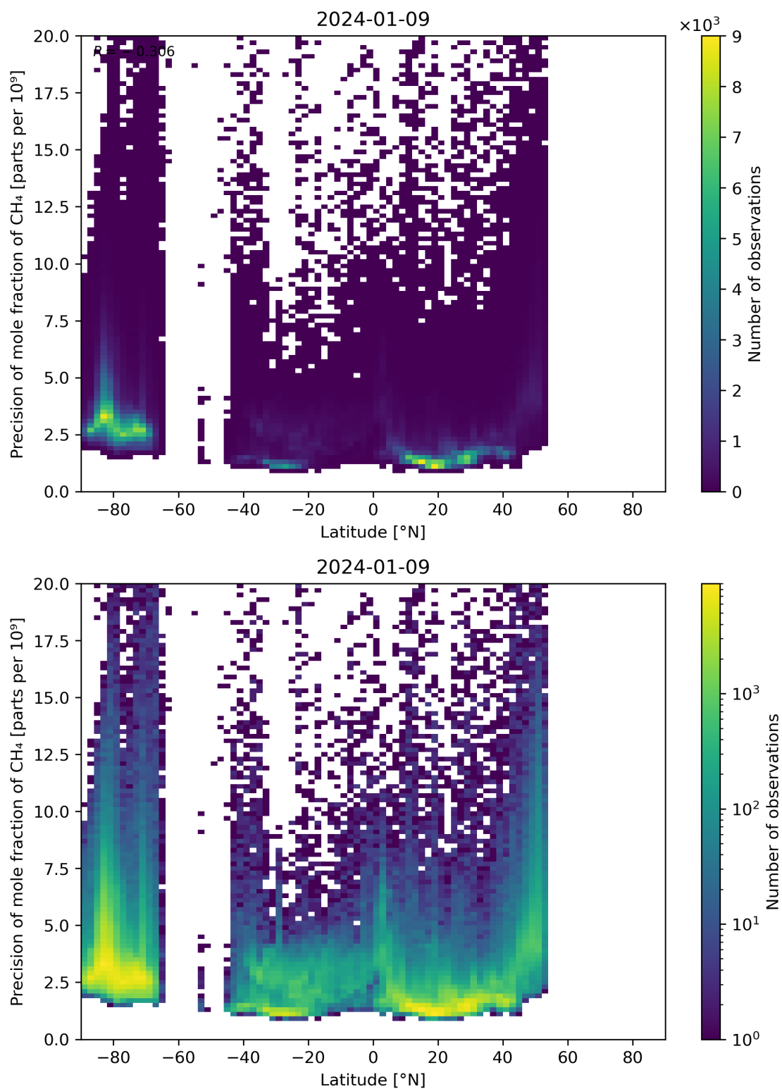
Figure 59: Scatter density plot of “Latitude” against “Precision of mole fraction of CH 4 ” for 2024-01-08 to 2024-01-10.
