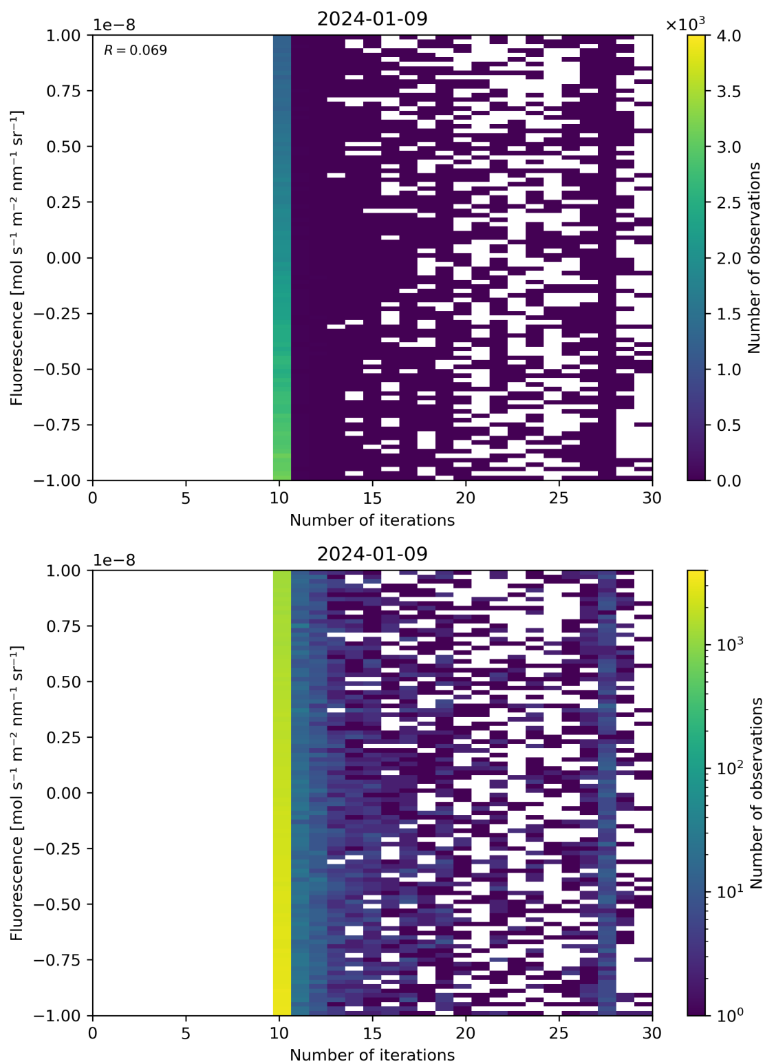
Figure 87: Scatter density plot of “Number of iterations” against “Fluorescence” for 2024-01-08 to 2024-01-10.
