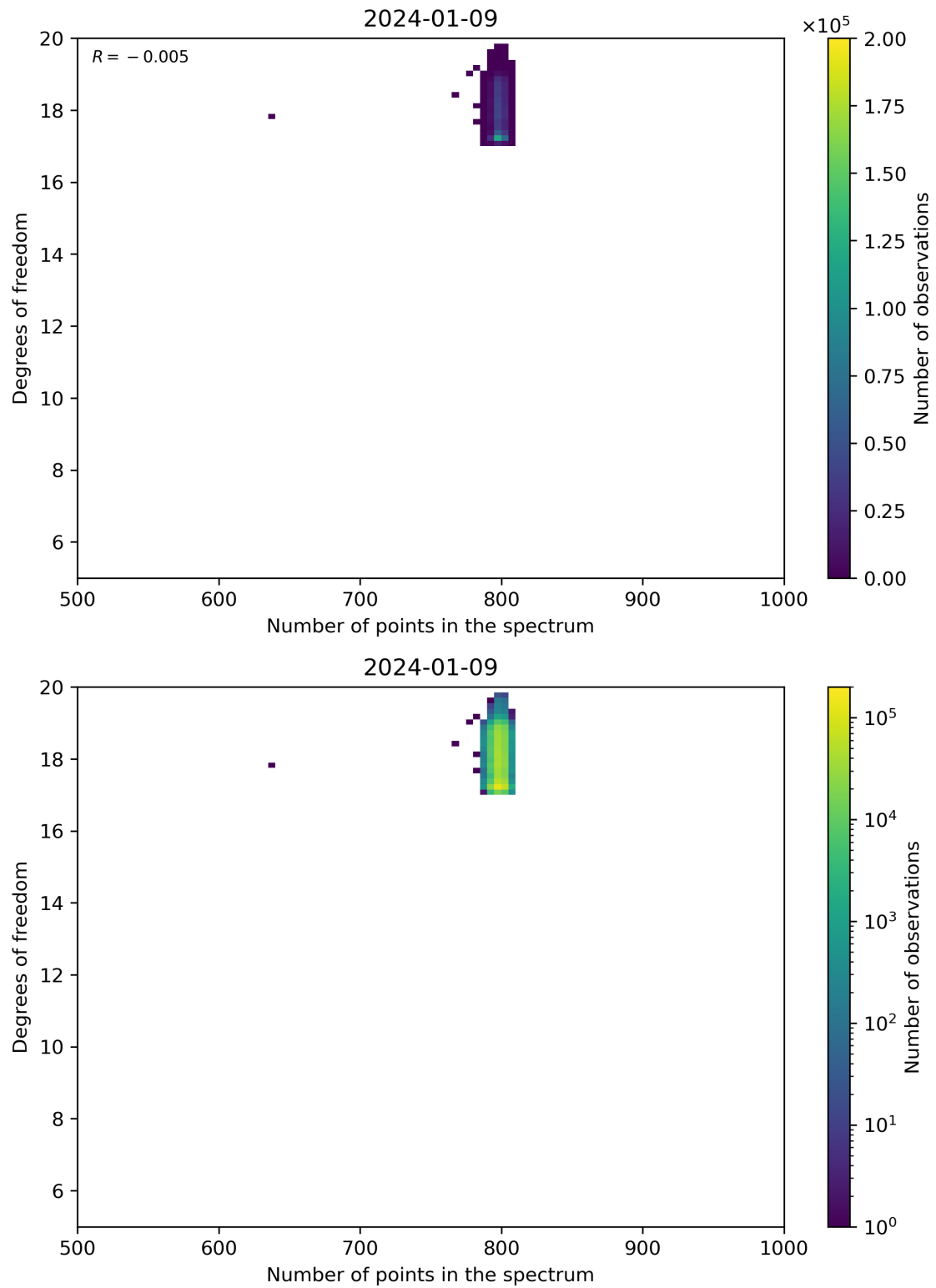
Figure 90: Scatter density plot of “Number of points in the spectrum” against “Degrees of freedom” for 2024-01-08 to 2024-01-10.
