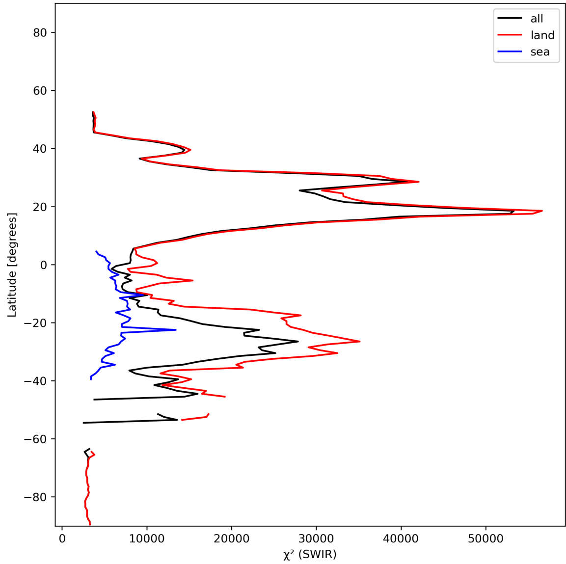
Figure 17: Zonal average of “ \chi^2 (SWIR)” for 2024-01-08 to 2024-01-10.
