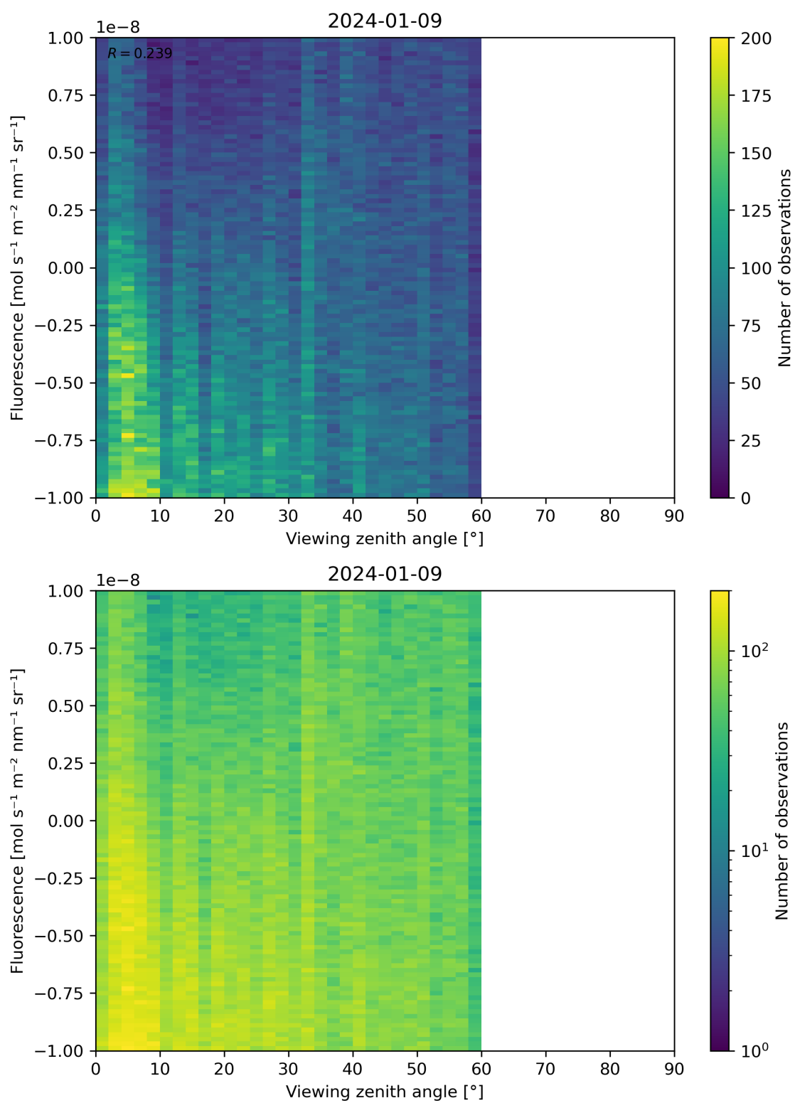
Figure 108: Scatter density plot of “Viewing zenith angle” against “Fluorescence” for 2024-01-08 to 2024-01-10.
