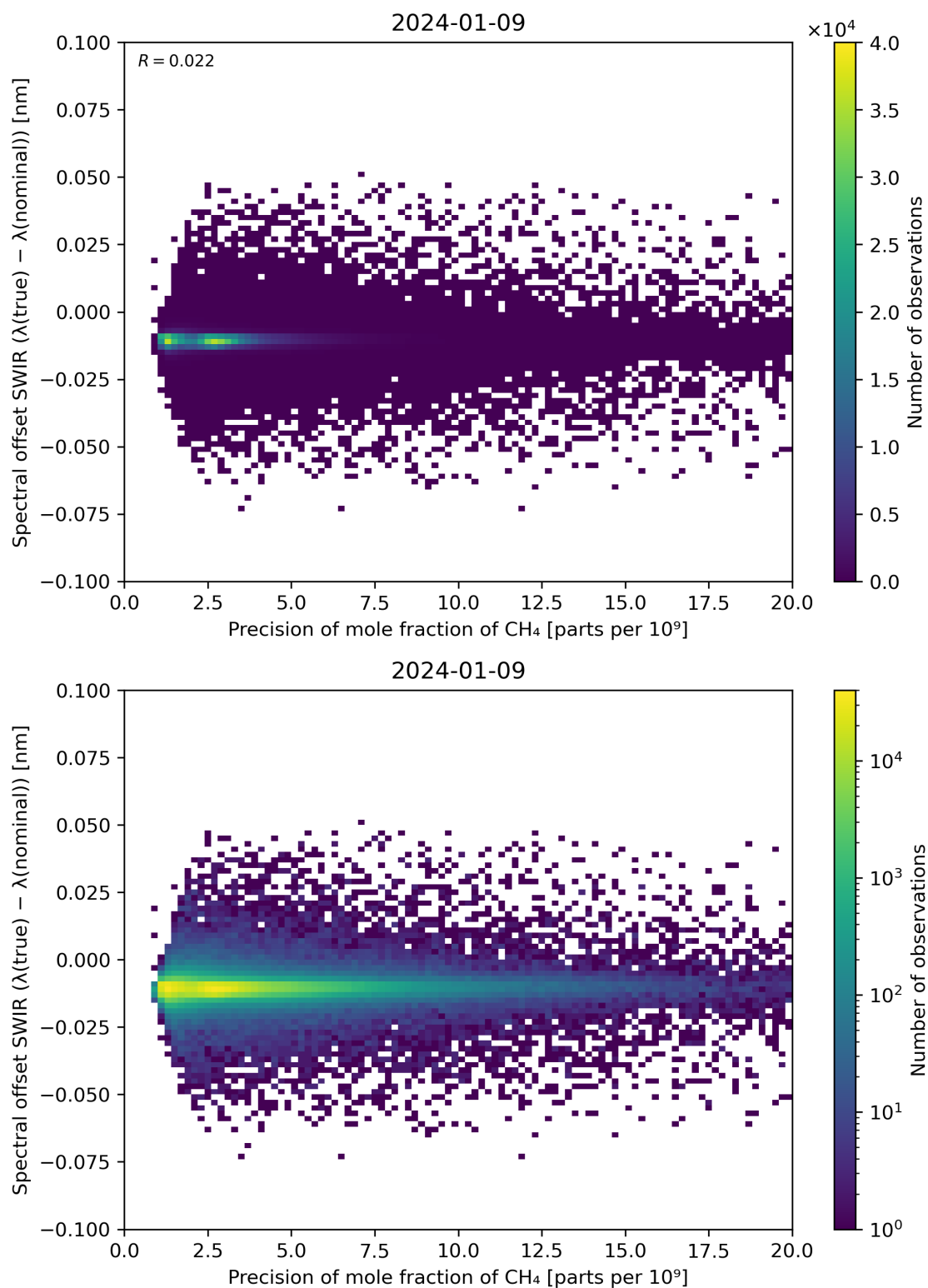
Figure 85: Scatter density plot of “Precision of mole fraction of CH 4 ” against “Spectral offset SWIR ( \lambda(\text{true}) - \lambda(\text{nominal}) )” for 2024-01-08 to 2024-01-10.
