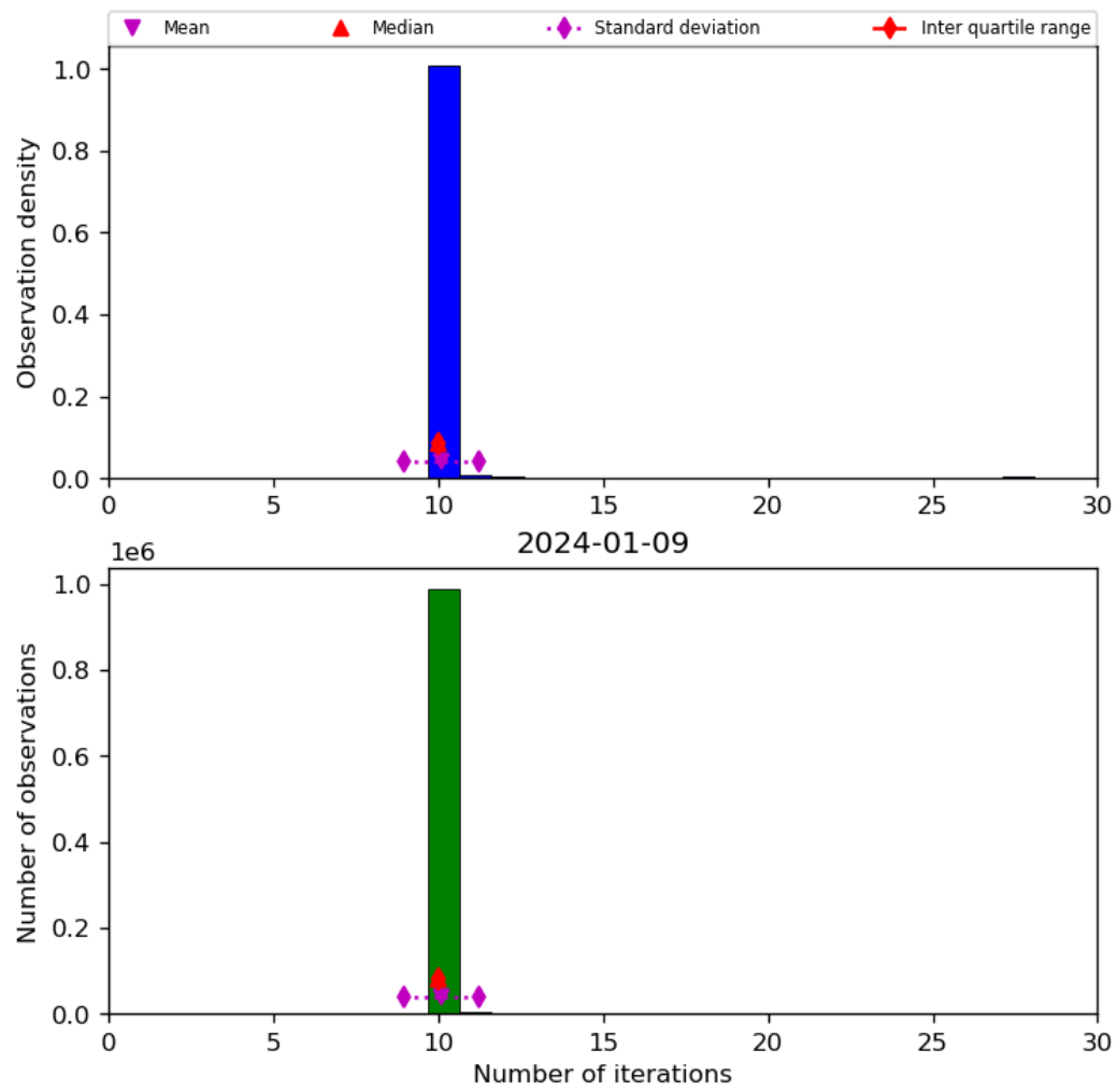
Figure 31: Histogram of “Number of iterations” for 2024-01-08 to 2024-01-10
