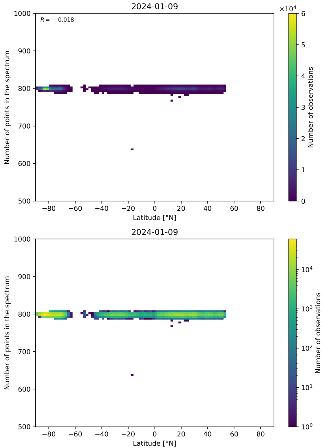
Figure 61: Scatter density plot of “Latitude” against “Number of points in the spectrum” for 2024-01-08 to 2024-01-10.
