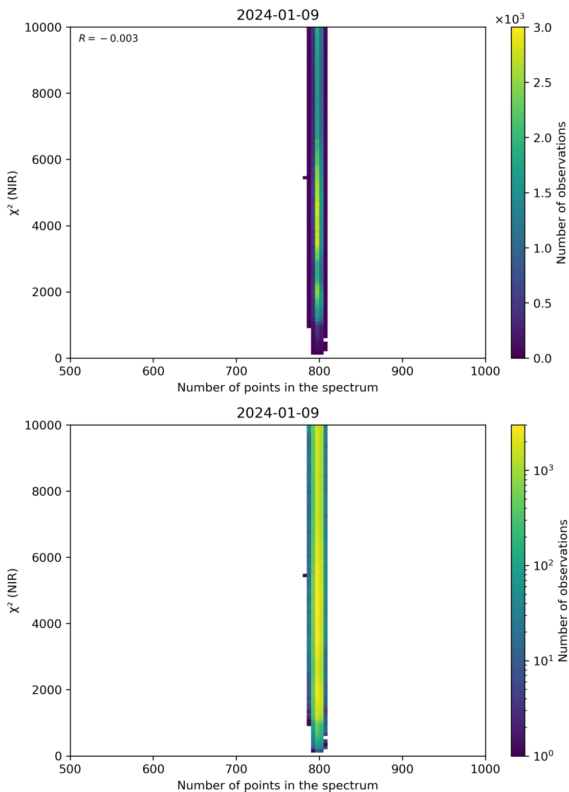
Figure 88: Scatter density plot of “Number of points in the spectrum” against “ \chi^2 (NIR)” for 2024-01-08 to 2024-01-10.
