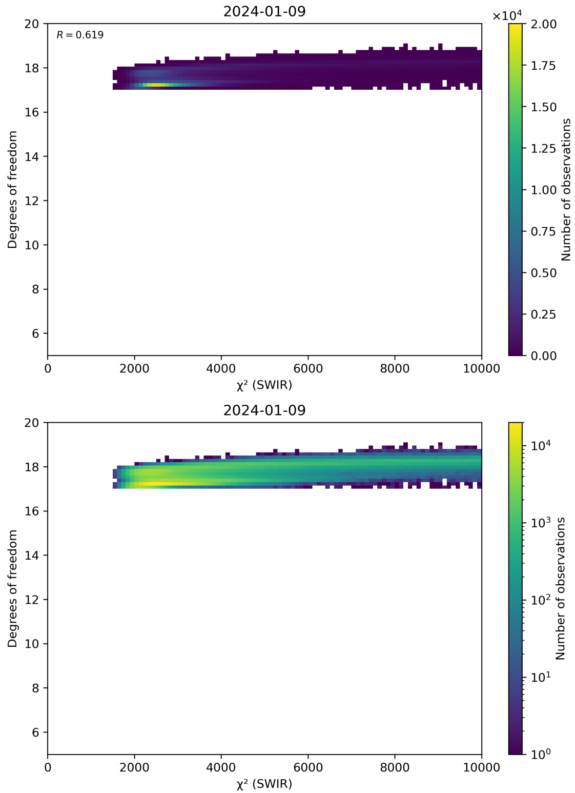
Figure 48: Scatter density plot of “ \chi^2 (SWIR)” against “Degrees of freedom” for 2024-01-08 to 2024-01-10.
