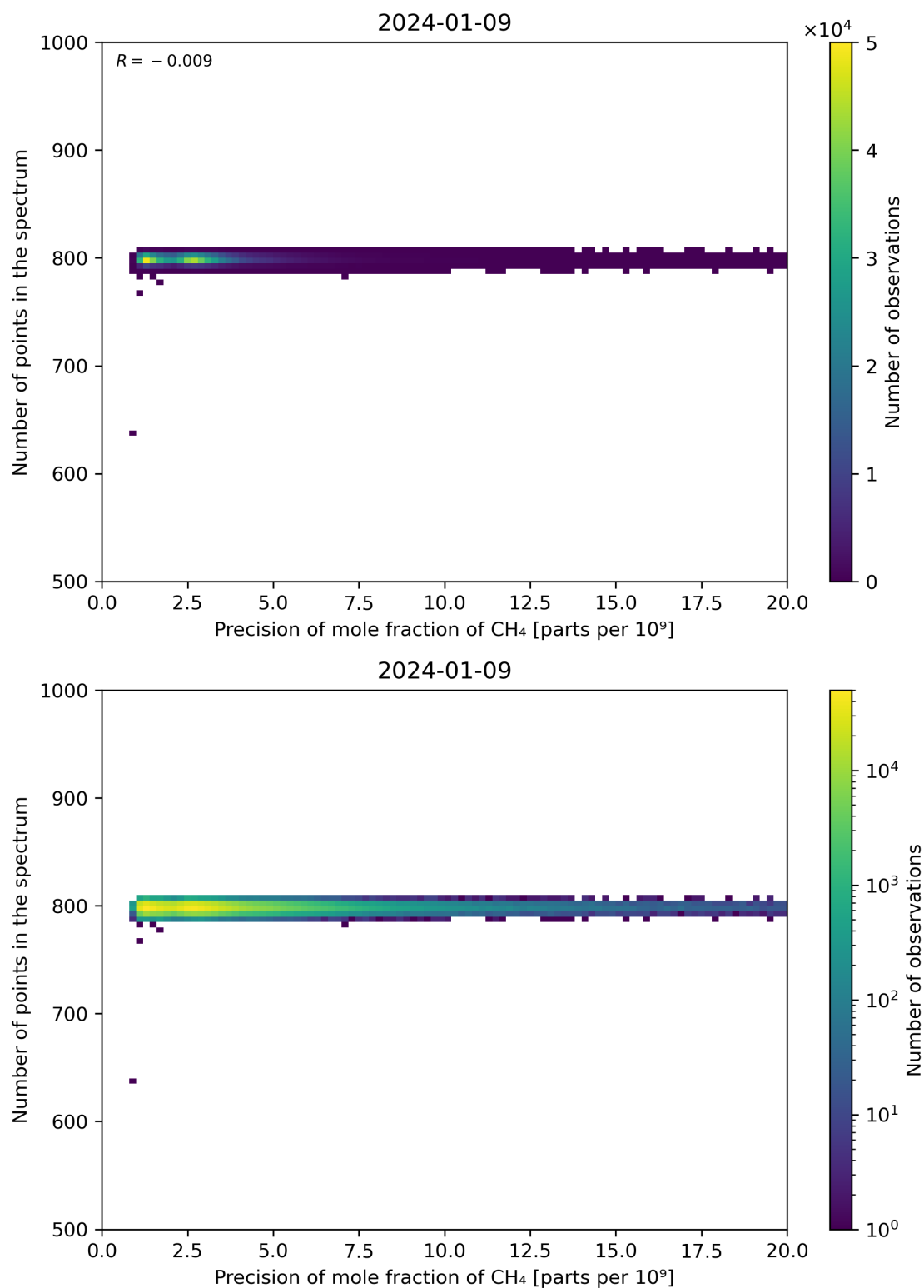
Figure 84: Scatter density plot of “Precision of mole fraction of CH 4 ” against “Number of points in the spectrum” for 2024-01-08 to 2024-01-10.
