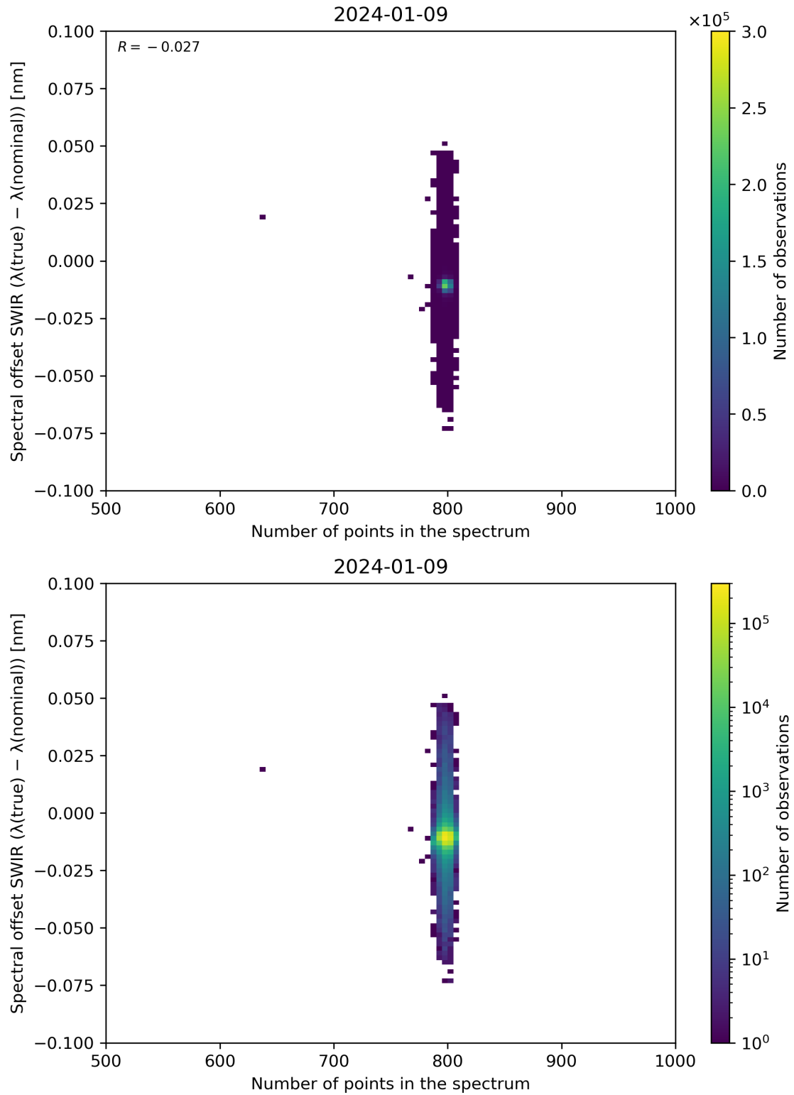
Figure 93: Scatter density plot of “Number of points in the spectrum” against “Spectral offset SWIR ( \lambda(\text{true}) - \lambda(\text{nominal}) )” for 2024-01-08 to 2024-01-10.
