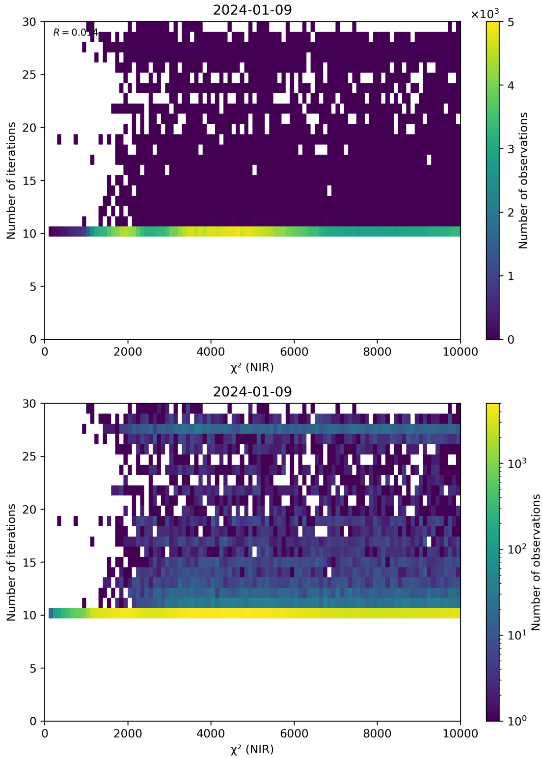
Figure 46: Scatter density plot of “ \chi^2 (NIR)” against “Number of iterations” for 2024-01-08 to 2024-01-10.
