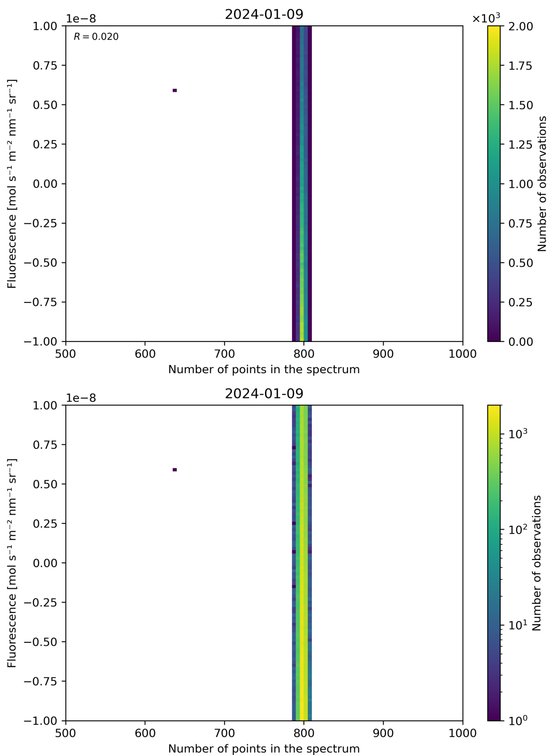
Figure 91: Scatter density plot of “Number of points in the spectrum” against “Fluorescence” for 2024-01-08 to 2024-01-10.
