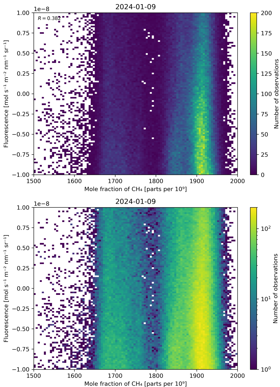
Figure 73: Scatter density plot of “Mole fraction of \text{CH}_4 ” against “Fluorescence” for 2024-01-08 to 2024-01-10.
