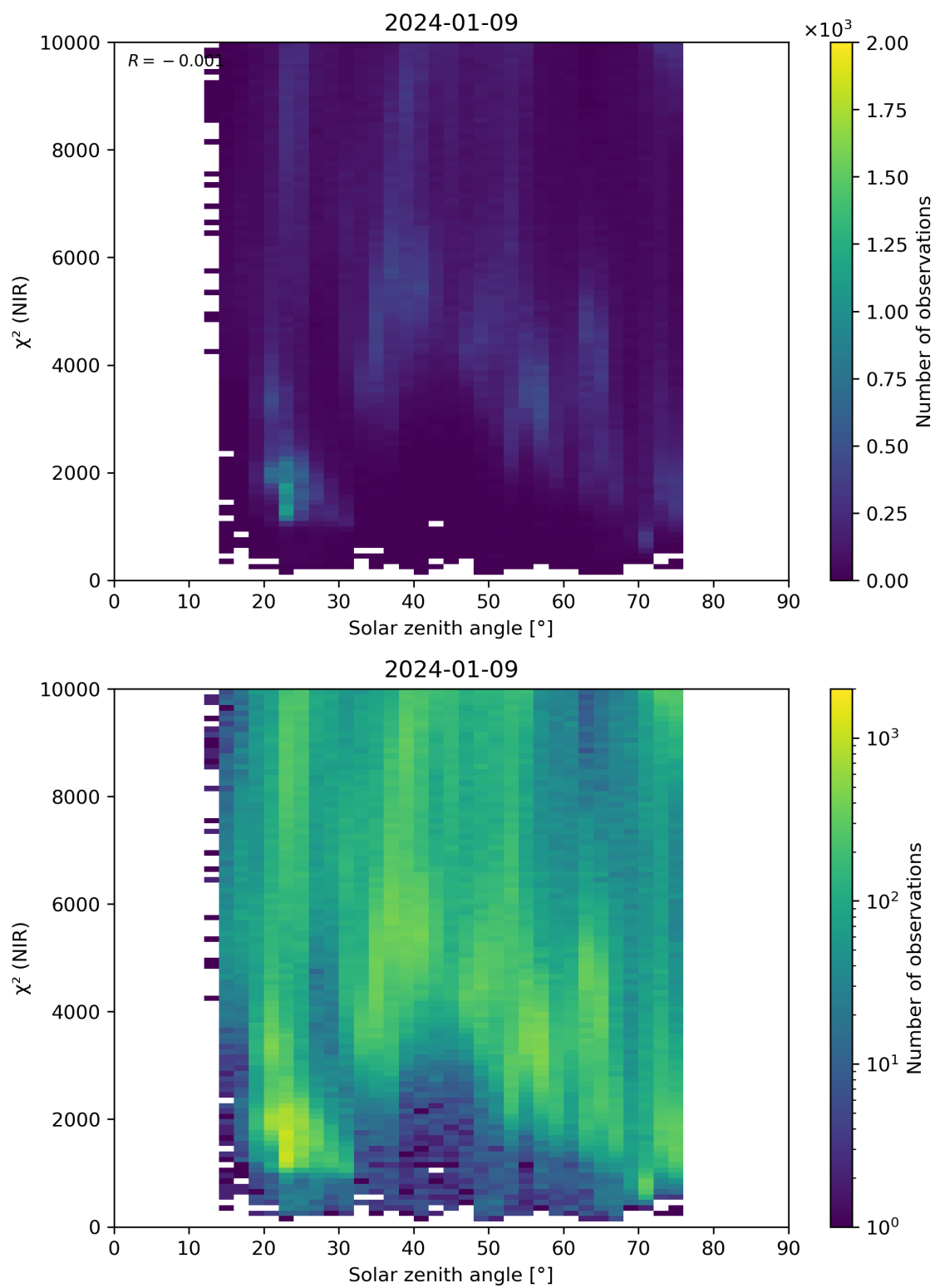
Figure 94: Scatter density plot of “Solar zenith angle” against “ \chi^2 (NIR)” for 2024-01-08 to 2024-01-10.
