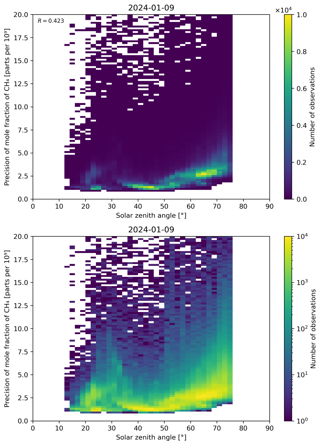
Figure 101: Scatter density plot of “Solar zenith angle” against “Precision of mole fraction of \text{CH}_4 ” for 2024-01-08 to 2024-01-10.
