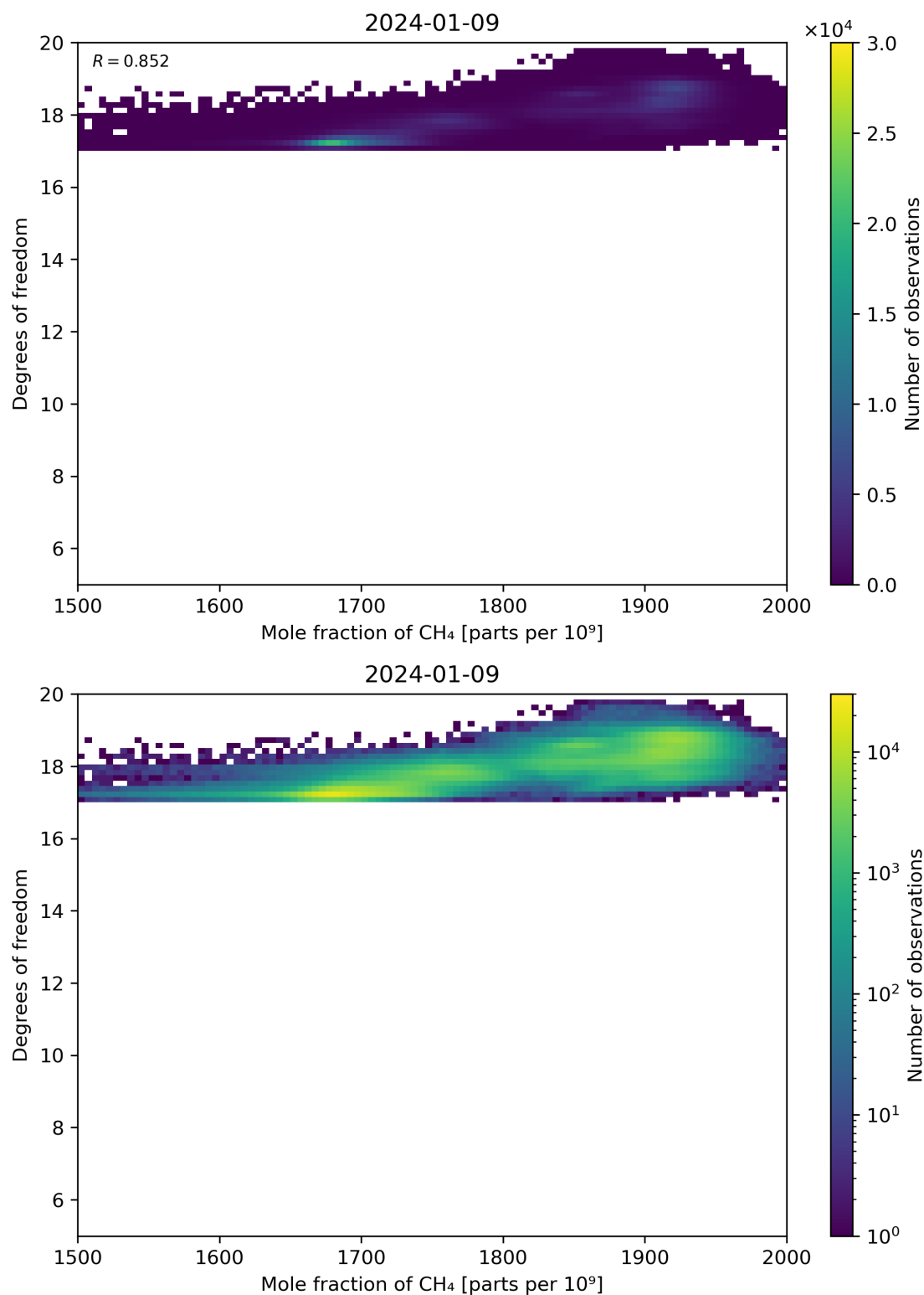
Figure 72: Scatter density plot of “Mole fraction of CH 4 ” against “Degrees of freedom” for 2024-01-08 to 2024-01-10.
