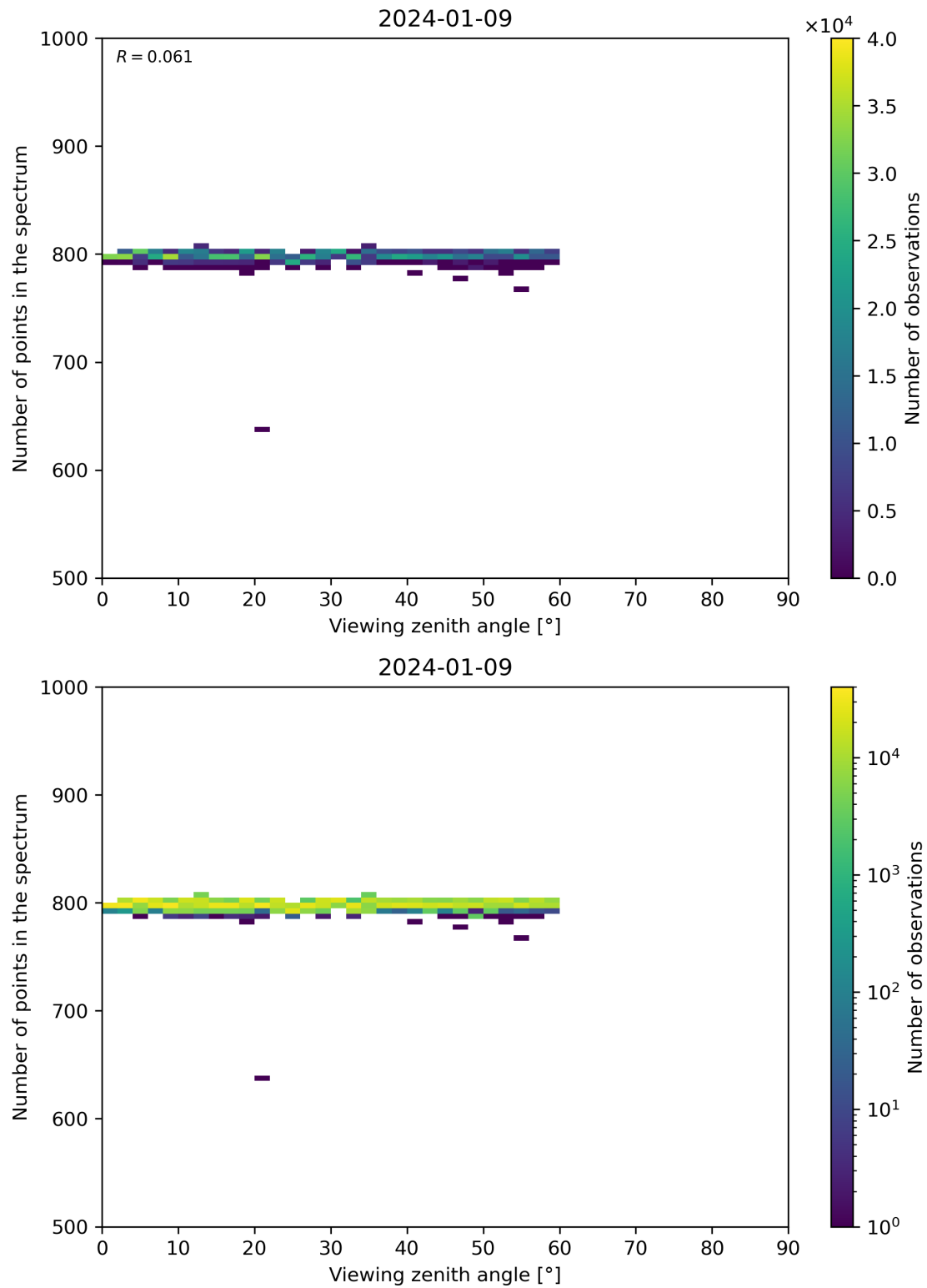
Figure 114: Scatter density plot of “Viewing zenith angle” against “Number of points in the spectrum” for 2024-01-08 to 2024-01-10.
