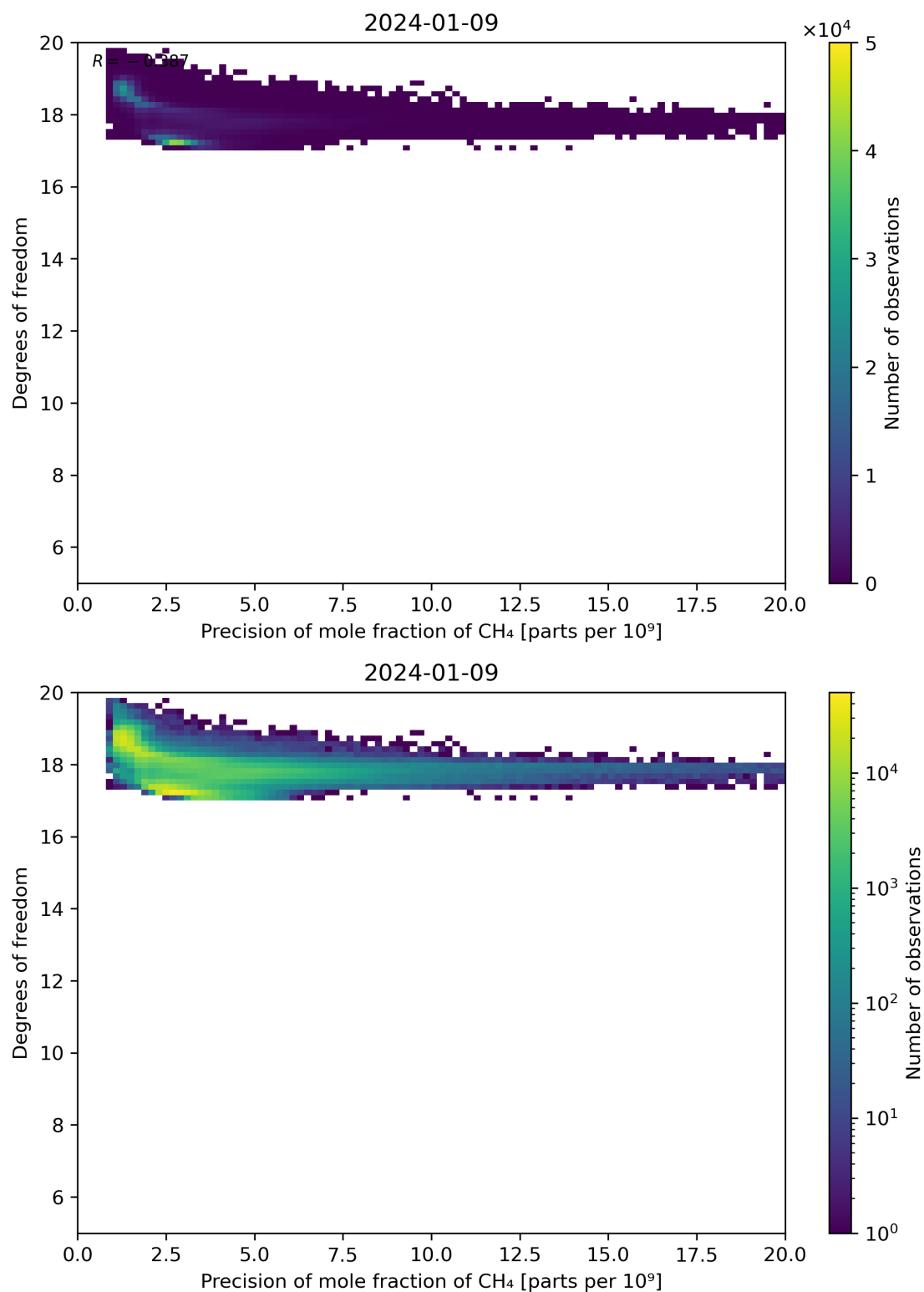
Figure 80: Scatter density plot of “Precision of mole fraction of CH 4 ” against “Degrees of freedom” for 2024-01-08 to 2024-01-10.
