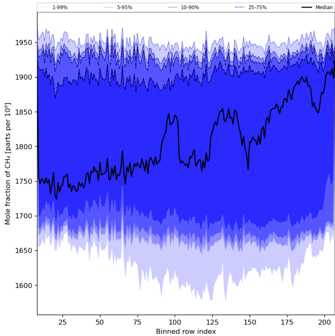
Figure 34: Along track statistics of “Mole fraction of CH 4 ” for 2024-01-08 to 2024-01-10
