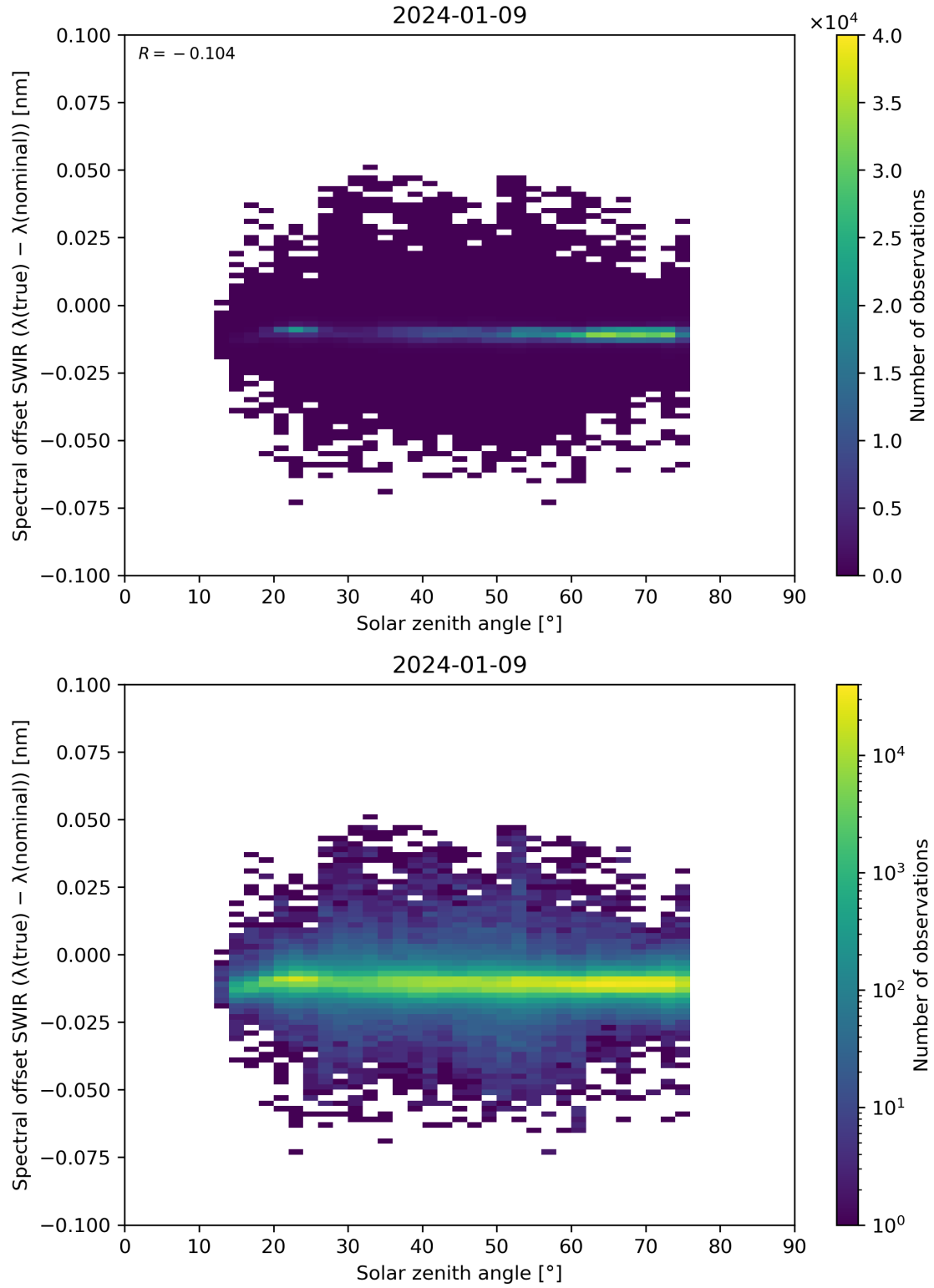
Figure 104: Scatter density plot of “Solar zenith angle” against “Spectral offset SWIR ( \lambda(\text{true}) - \lambda(\text{nominal}) )” for 2024-01-08 to 2024-01-10.
