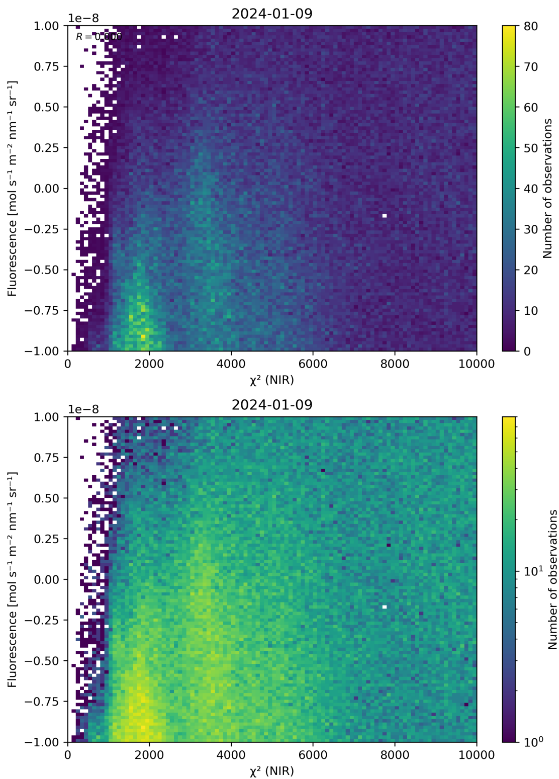
Figure 45: Scatter density plot of “ \chi^2 (NIR)” against “Fluorescence” for 2024-01-08 to 2024-01-10.
