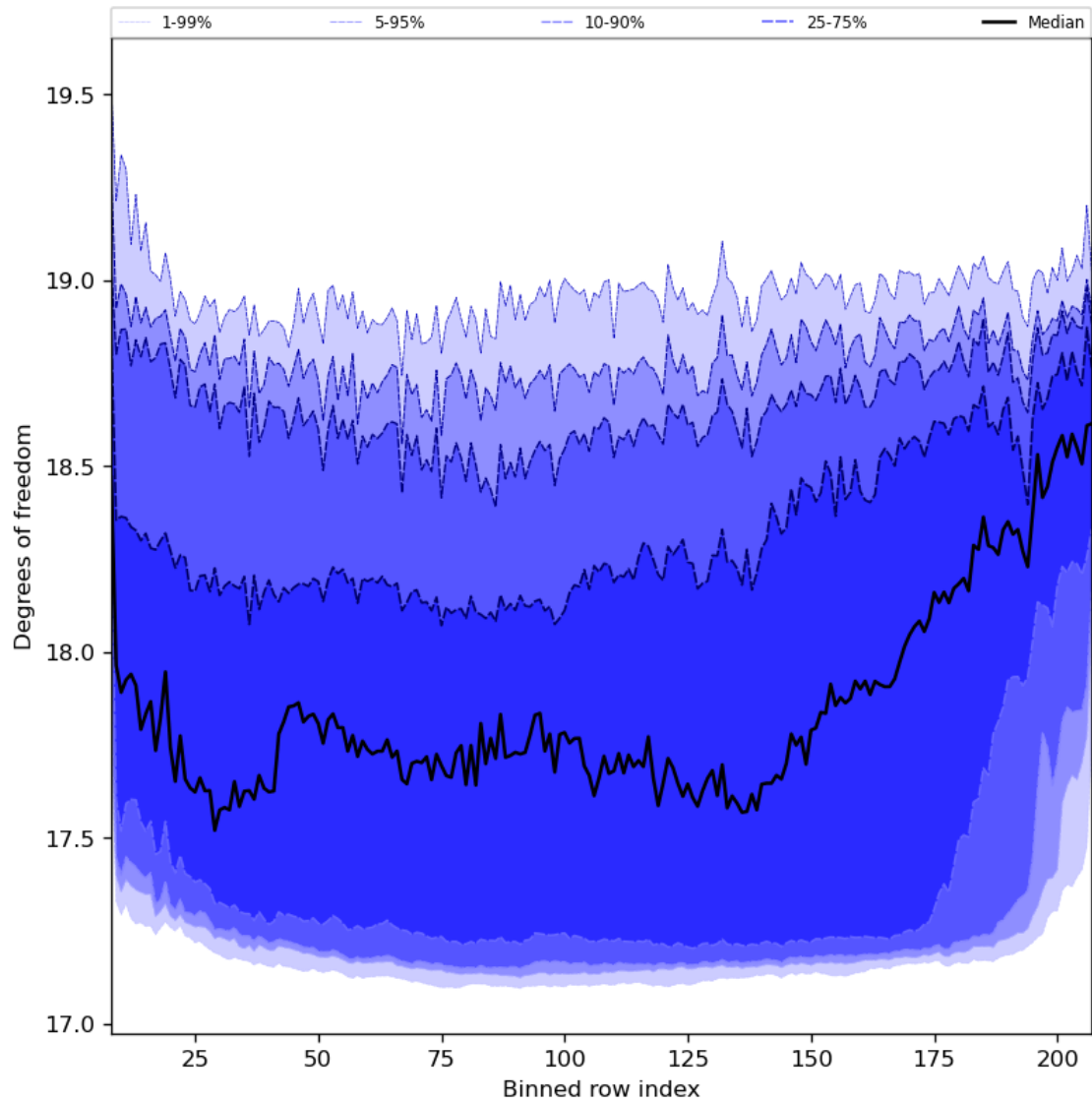
Figure 41: Along track statistics of “Degrees of freedom” for 2024-01-10 to 2024-01-12
