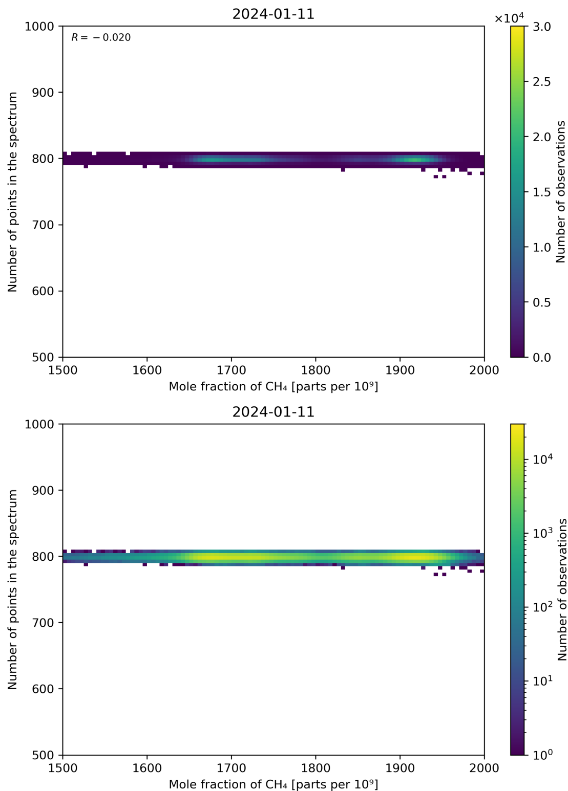
Figure 77: Scatter density plot of “Mole fraction of CH 4 ” against “Number of points in the spectrum” for 2024-01-10 to 2024-01-12.
