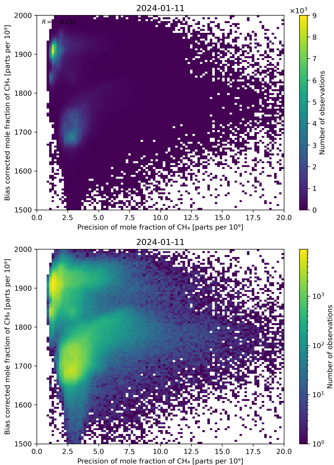
Figure 82: Scatter density plot of “Precision of mole fraction of CH 4 ” against “Bias corrected mole fraction of CH 4 ” for 2024-01-10 to 2024-01-12.
