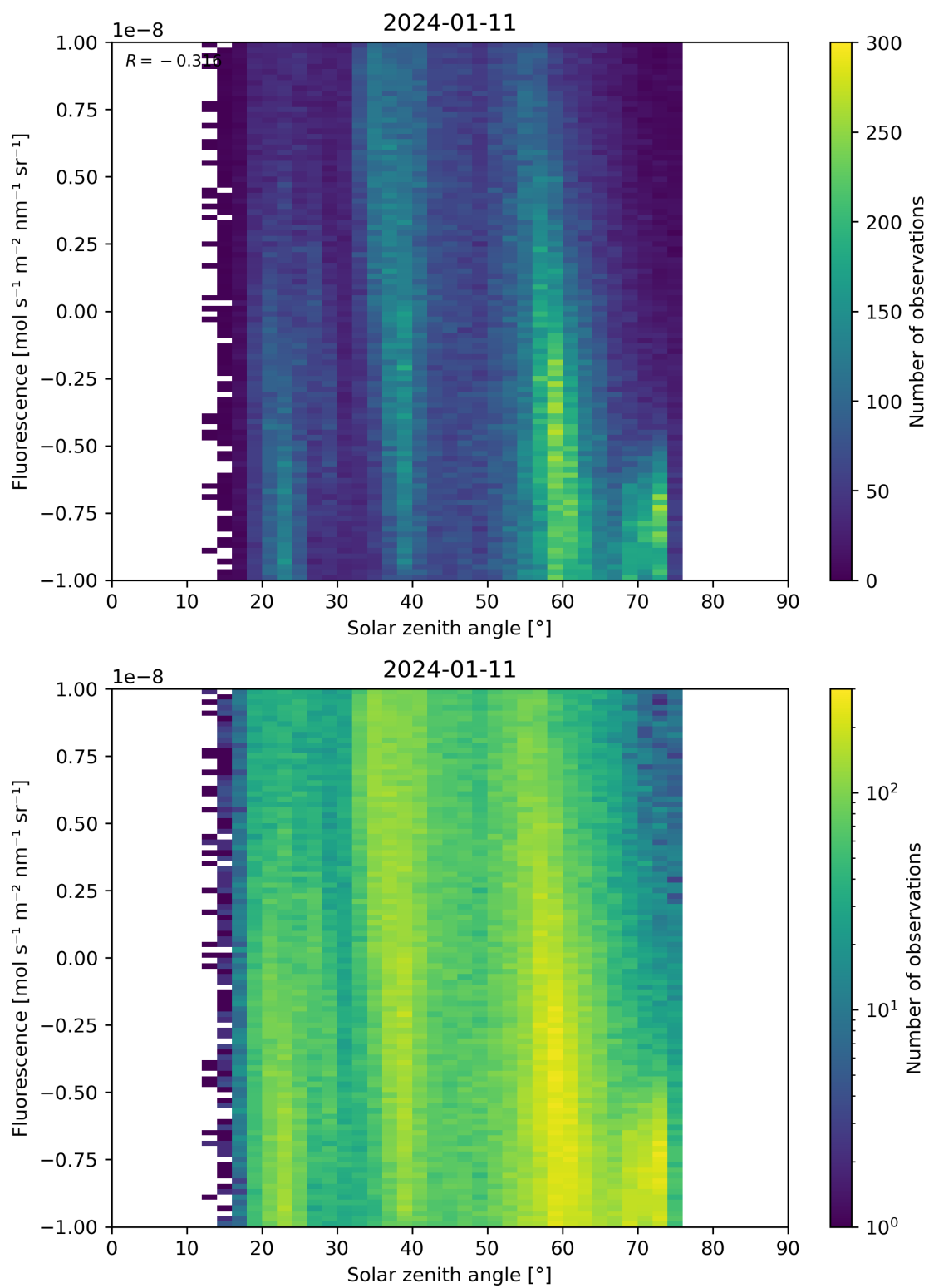
Figure 97: Scatter density plot of “Solar zenith angle” against “Fluorescence” for 2024-01-10 to 2024-01-12.
