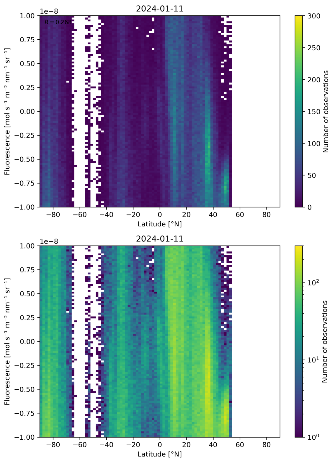
Figure 56: Scatter density plot of “Latitude” against “Fluorescence” for 2024-01-10 to 2024-01-12.
