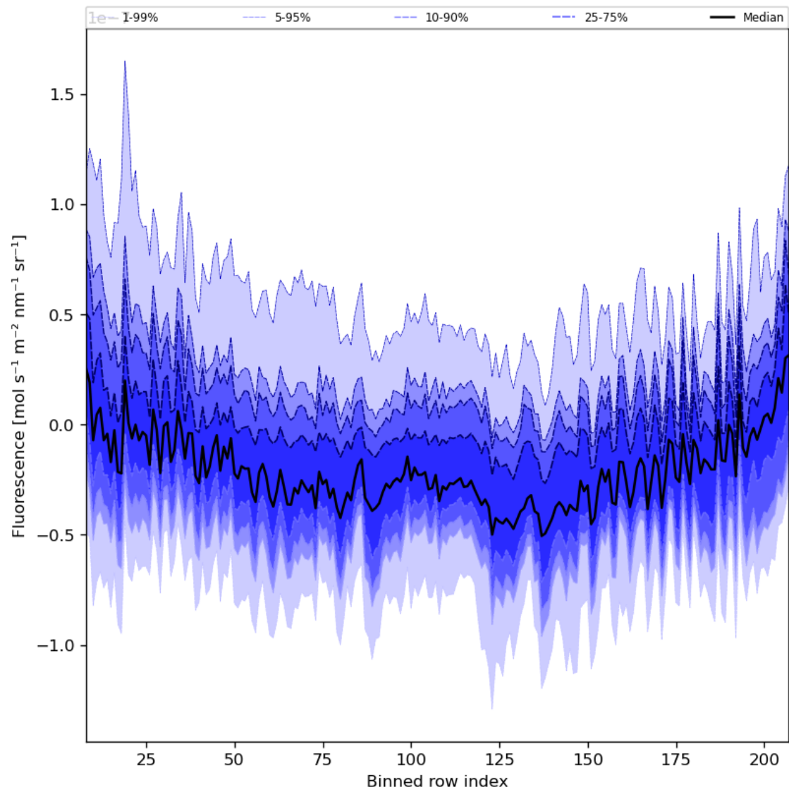
Figure 43: Along track statistics of “Fluorescence” for 2024-01-10 to 2024-01-12
