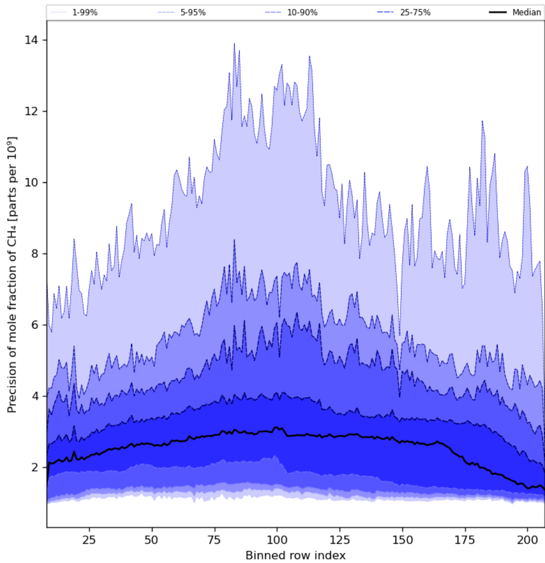
Figure 35: Along track statistics of “Precision of mole fraction of CH 4 ” for 2024-01-10 to 2024-01-12
