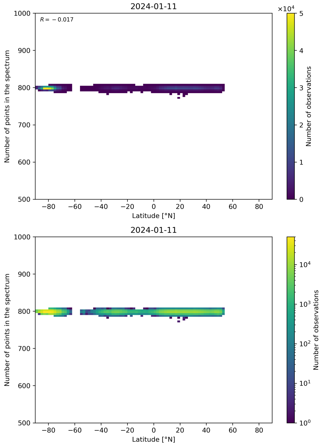
Figure 61: Scatter density plot of “Latitude” against “Number of points in the spectrum” for 2024-01-10 to 2024-01-12.
