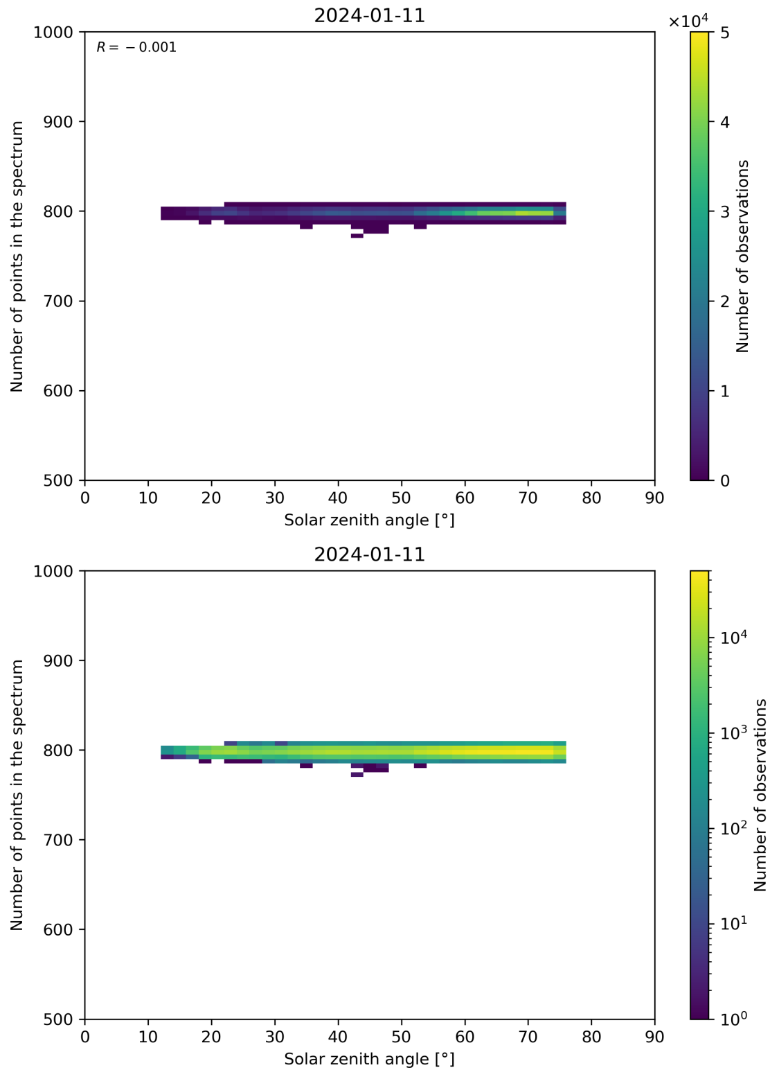
Figure 103: Scatter density plot of “Solar zenith angle” against “Number of points in the spectrum” for 2024-01-10 to 2024-01-12.
