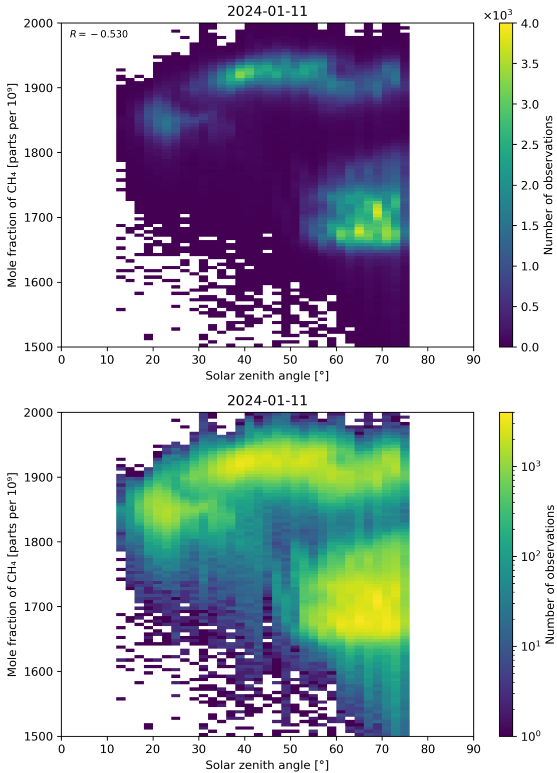
Figure 99: Scatter density plot of “Solar zenith angle” against “Mole fraction of \text{CH}_4 ” for 2024-01-10 to 2024-01-12.
