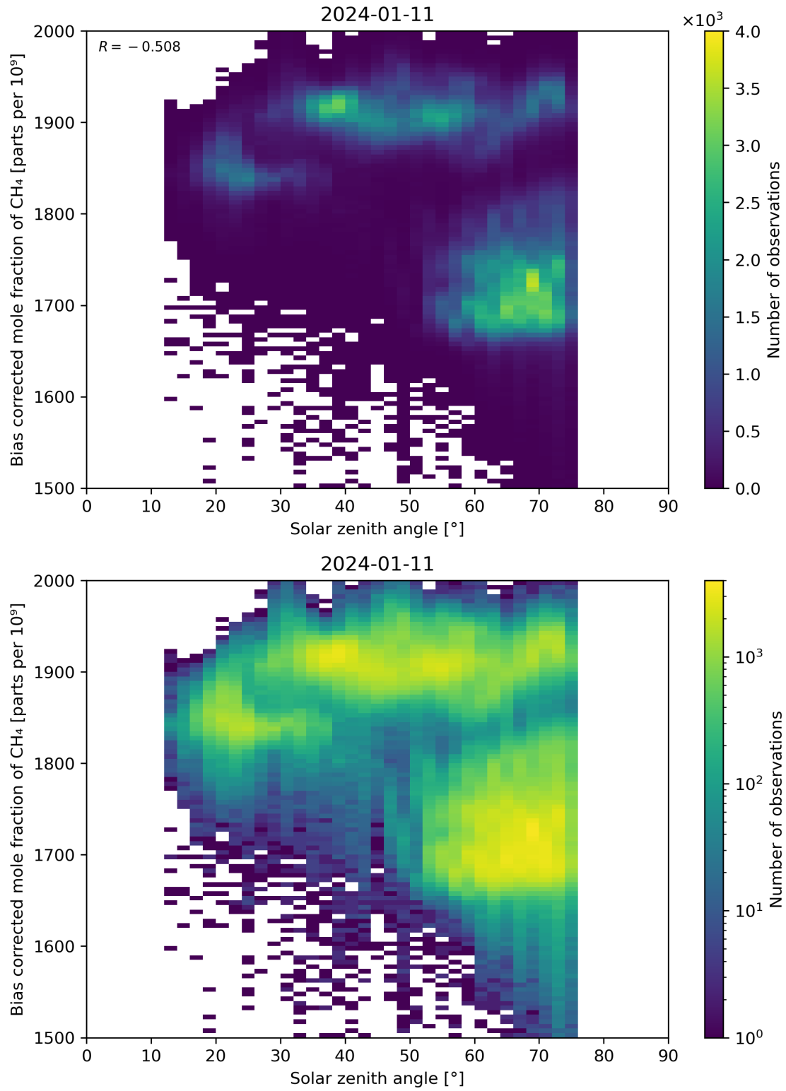
Figure 100: Scatter density plot of “Solar zenith angle” against “Bias corrected mole fraction of \text{CH}_4 ” for 2024-01-10 to 2024-01-12.
