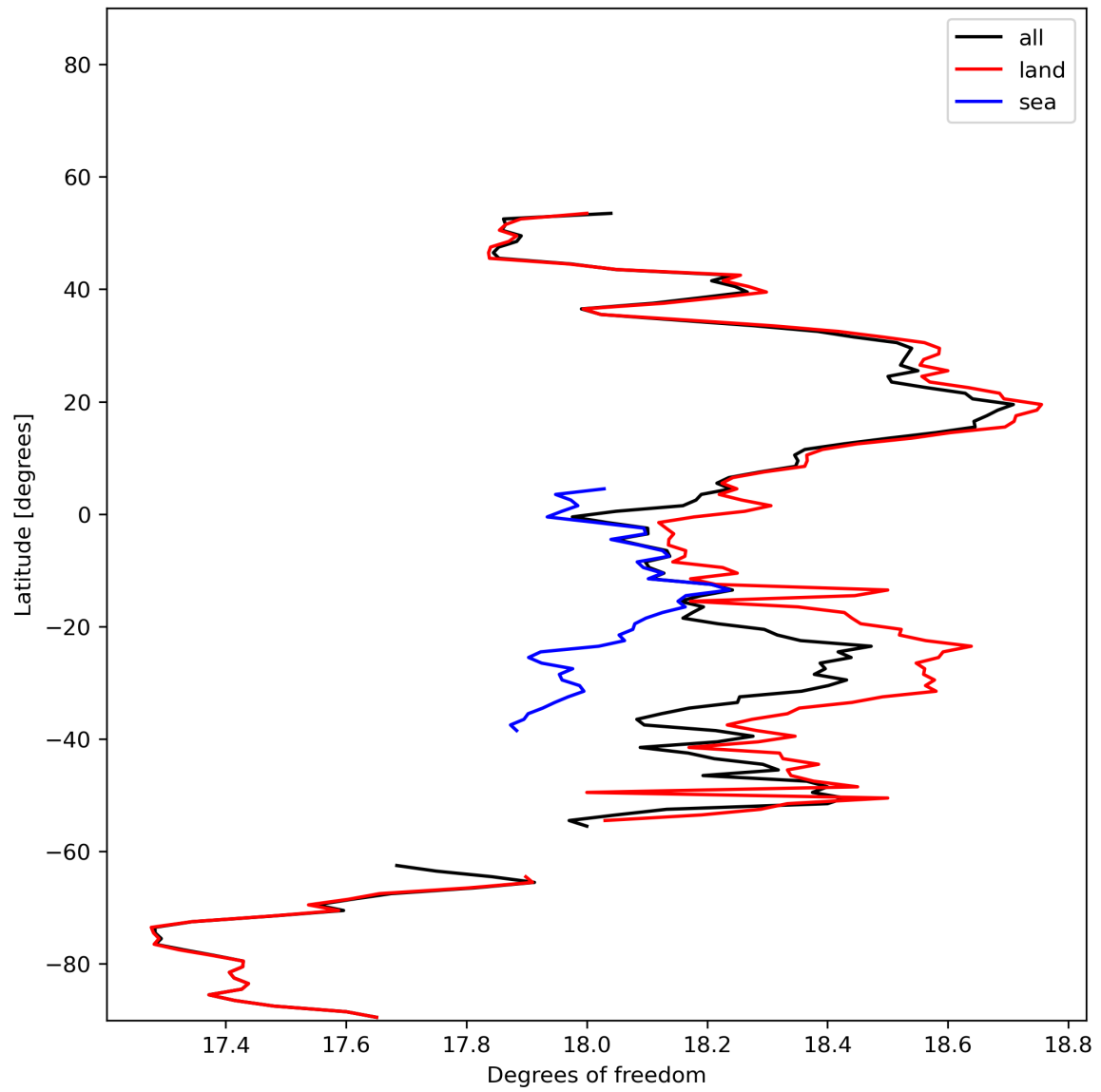
Figure 19: Zonal average of “Degrees of freedom” for 2024-01-10 to 2024-01-12.
