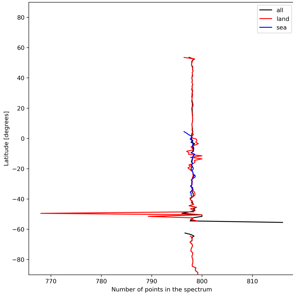
Figure 15: Zonal average of “Number of points in the spectrum” for 2024-01-10 to 2024-01-12.
