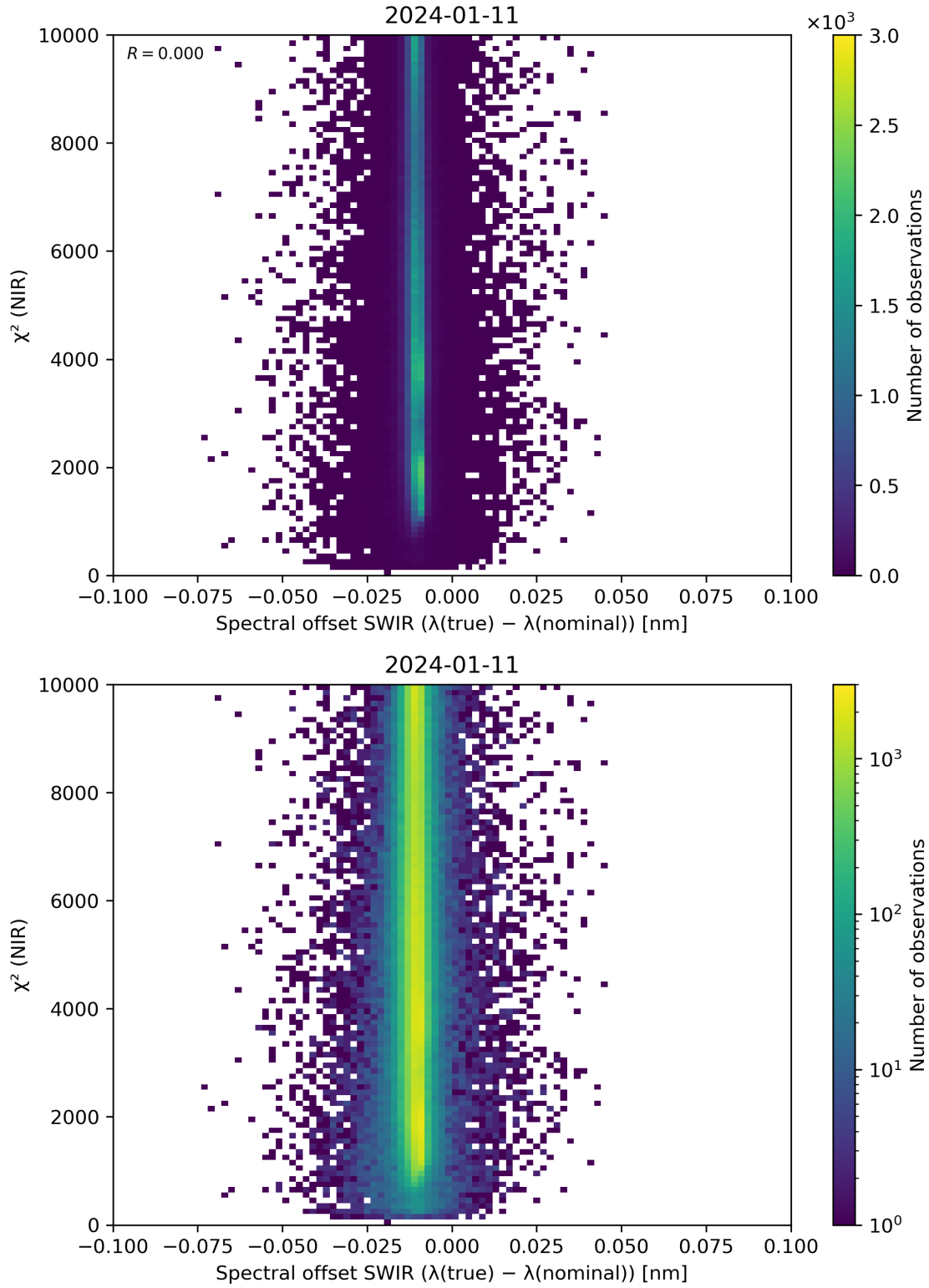
Figure 117: Scatter density plot of “Spectral offset SWIR ( \lambda(\text{true}) - \lambda(\text{nominal}) )” against “ \chi^2 (NIR)” for 2024-01-10 to 2024-01-12.
