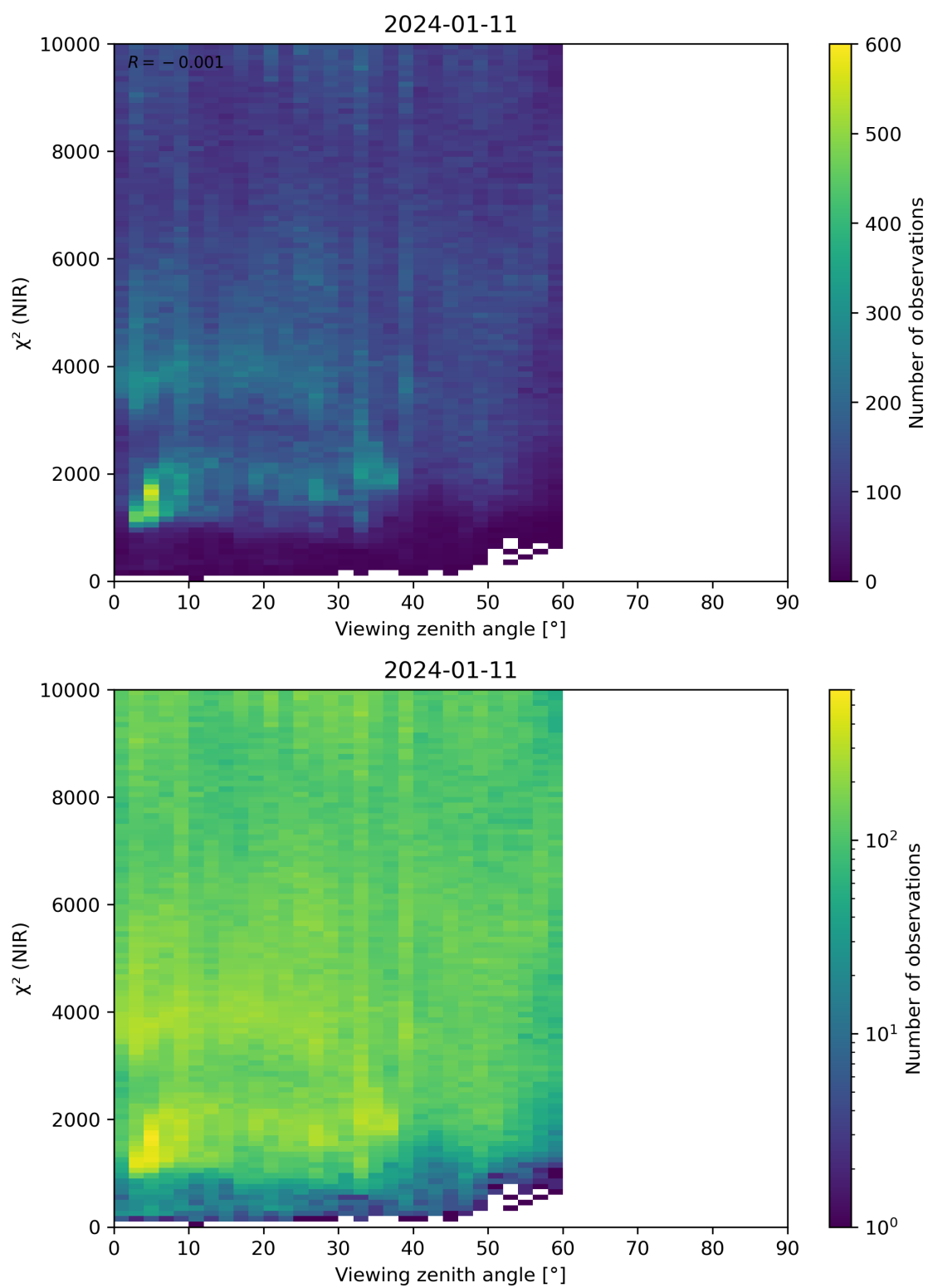
Figure 105: Scatter density plot of “Viewing zenith angle” against “ \chi^2 (NIR)” for 2024-01-10 to 2024-01-12.
