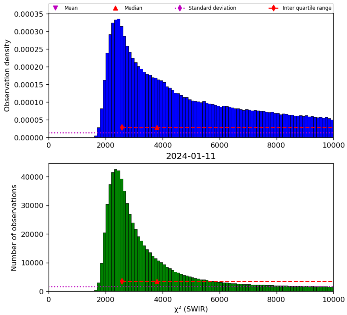
Figure 28: Histogram of “ \chi^2 (SWIR)” for 2024-01-10 to 2024-01-12
