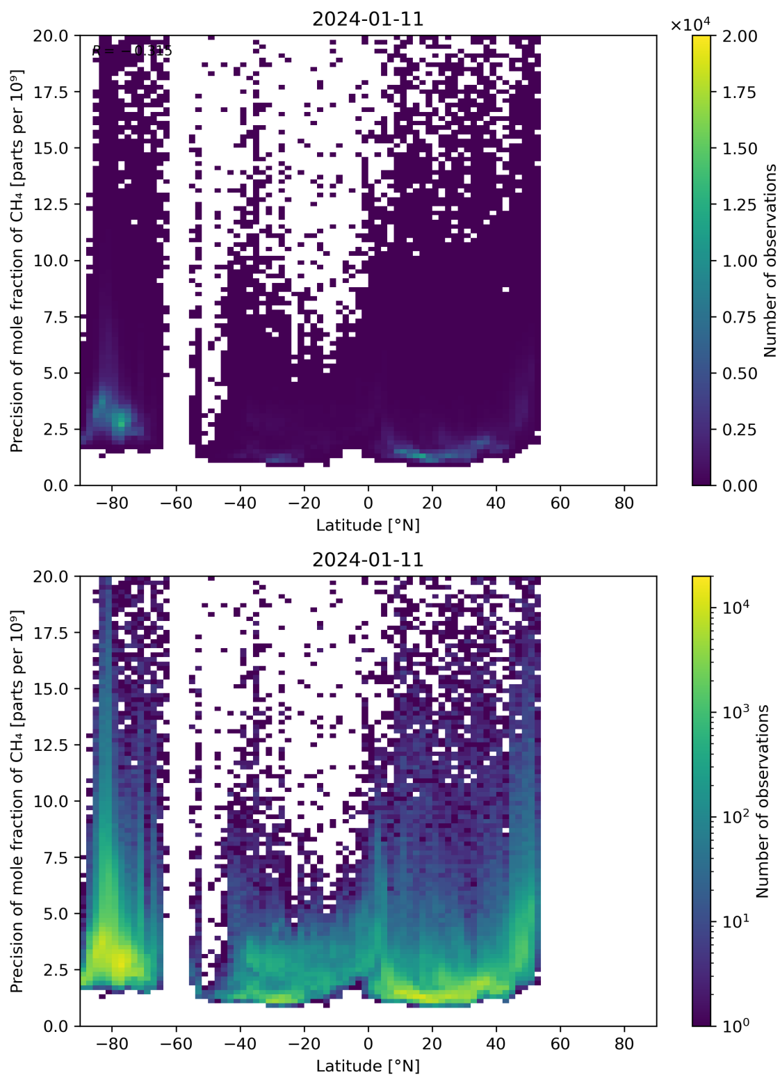
Figure 59: Scatter density plot of “Latitude” against “Precision of mole fraction of CH 4 ” for 2024-01-10 to 2024-01-12.
