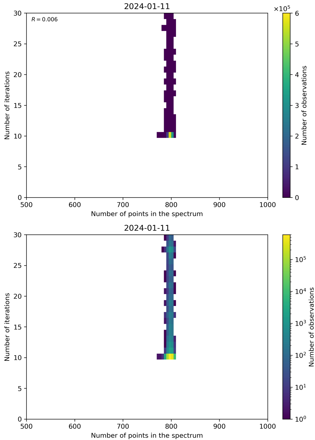
Figure 92: Scatter density plot of “Number of points in the spectrum” against “Number of iterations” for 2024-01-10 to 2024-01-12.
