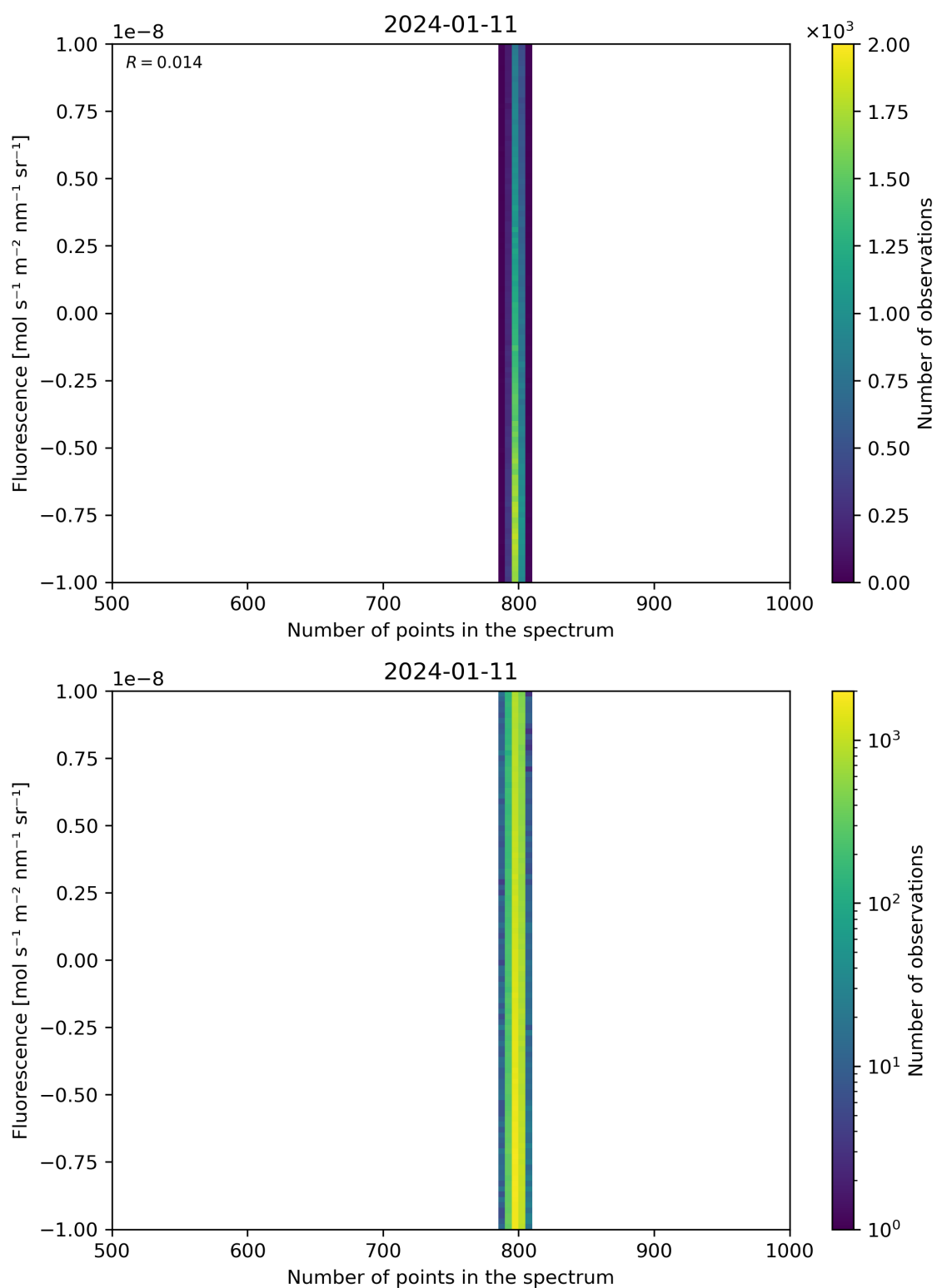
Figure 91: Scatter density plot of “Number of points in the spectrum” against “Fluorescence” for 2024-01-10 to 2024-01-12.
