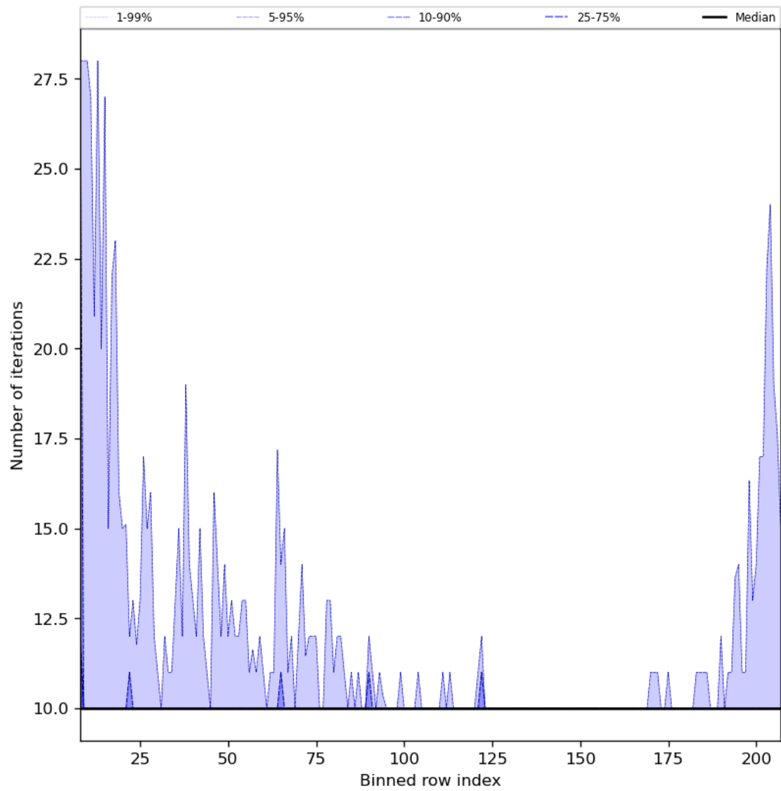
Figure 42: Along track statistics of “Number of iterations” for 2024-01-10 to 2024-01-12
