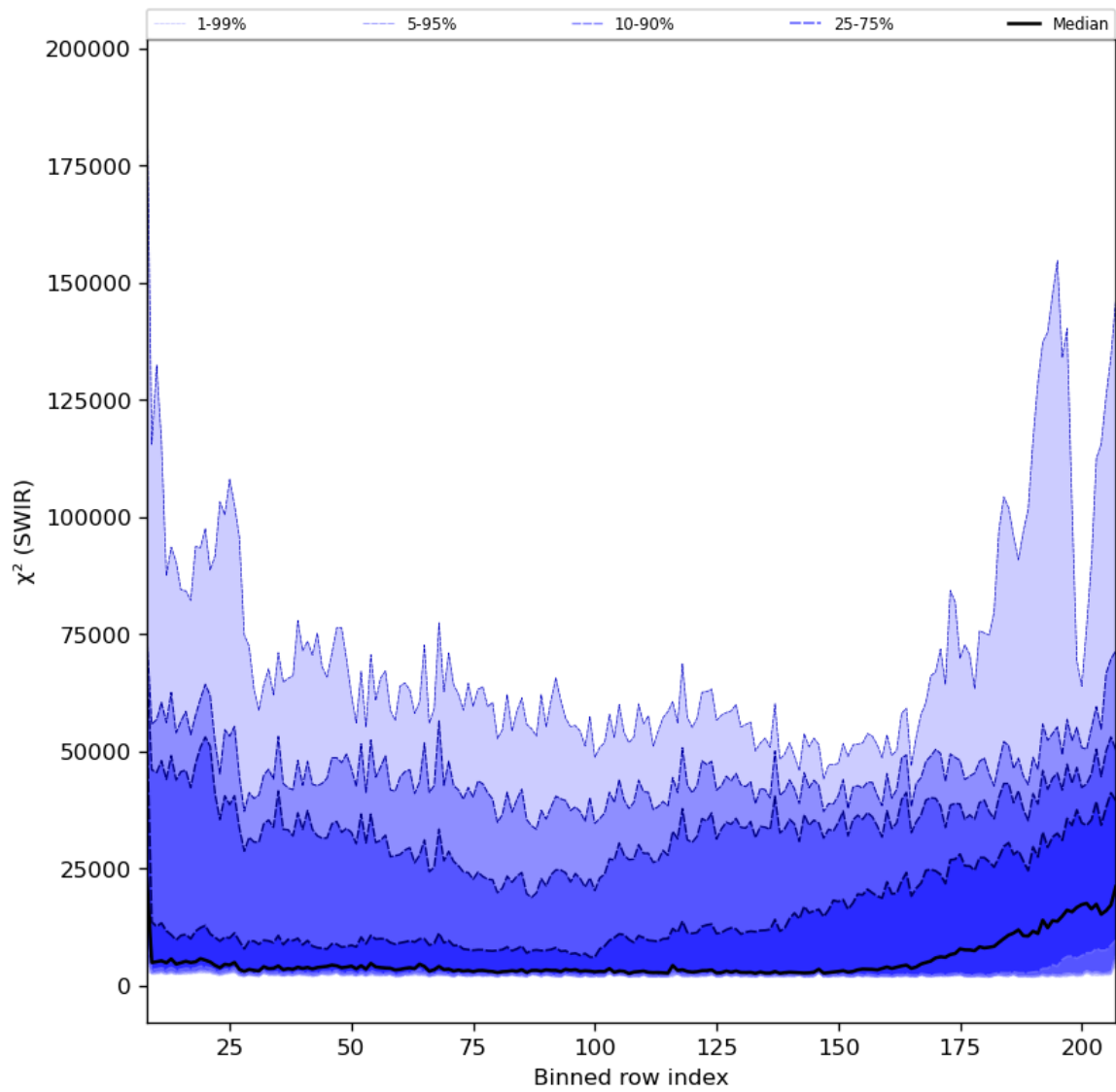
Figure 39: Along track statistics of “ \chi^2 (SWIR)” for 2024-01-10 to 2024-01-12
