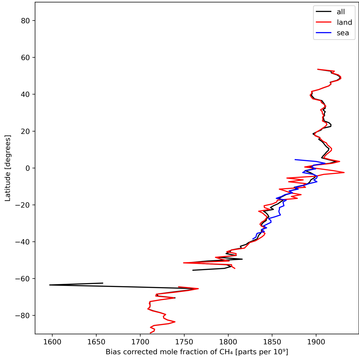
Figure 14: Zonal average of “Bias corrected mole fraction of CH 4 ” for 2024-01-10 to 2024-01-12.
