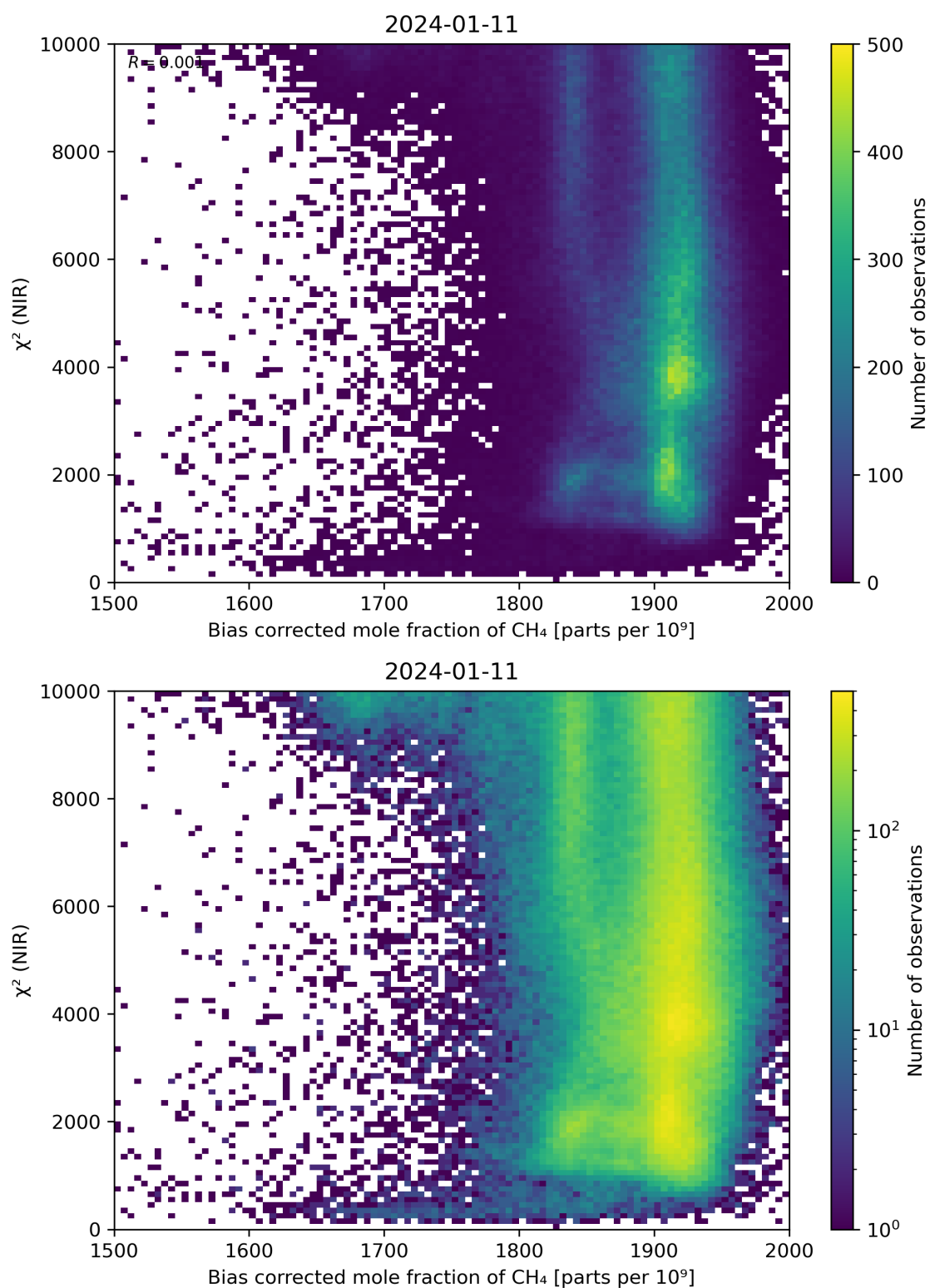
Figure 63: Scatter density plot of “Bias corrected mole fraction of CH 4 ” against “ \chi^2 (NIR)” for 2024-01-10 to 2024-01-12.
