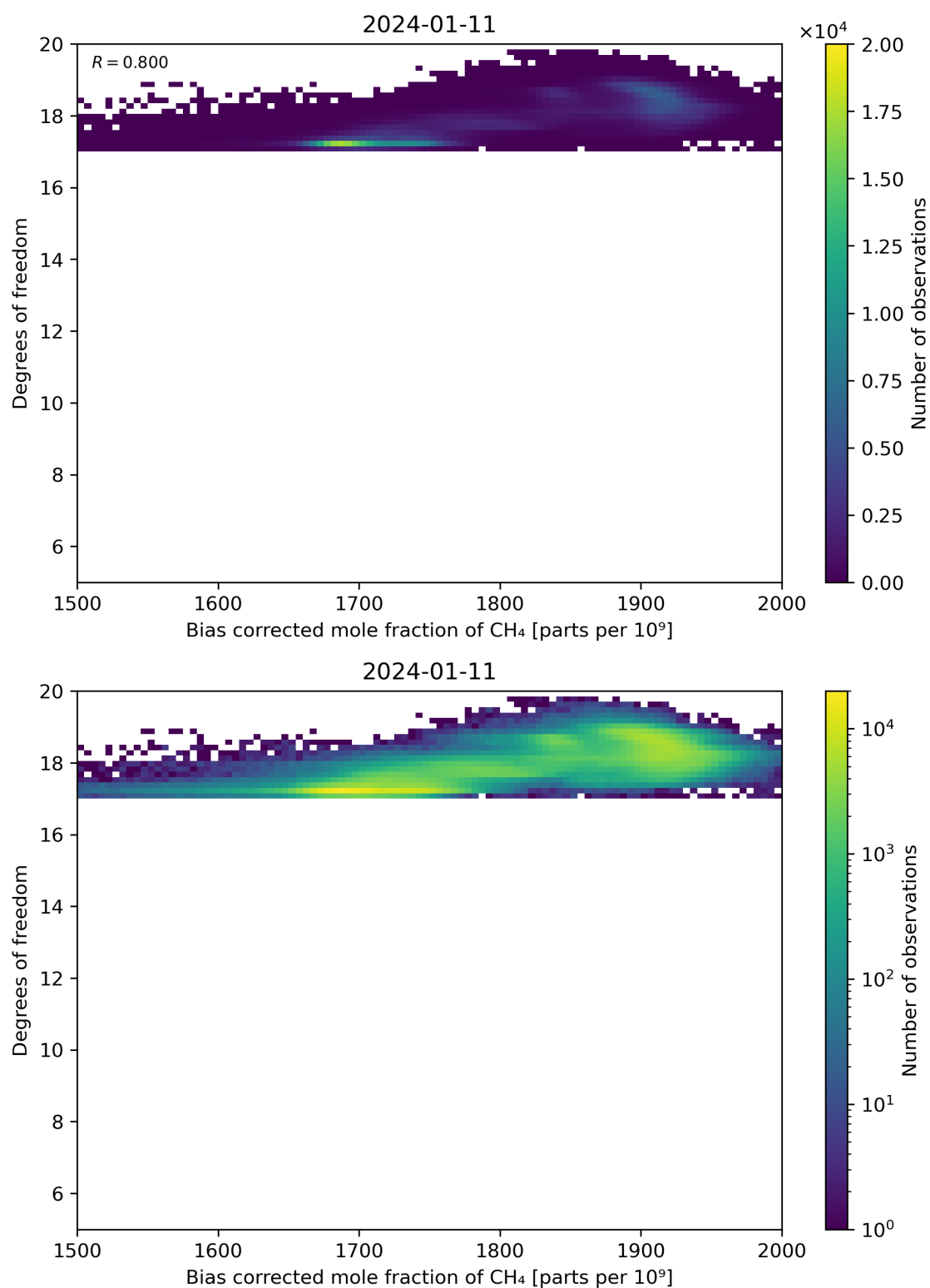
Figure 65: Scatter density plot of “Bias corrected mole fraction of CH 4 ” against “Degrees of freedom” for 2024-01-10 to 2024-01-12.
