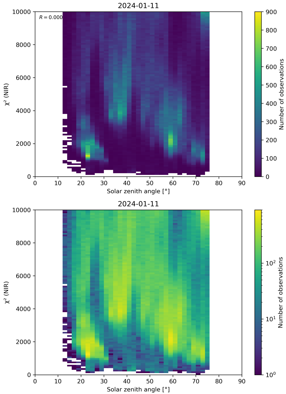
Figure 94: Scatter density plot of “Solar zenith angle” against “ \chi^2 (NIR)” for 2024-01-10 to 2024-01-12.
