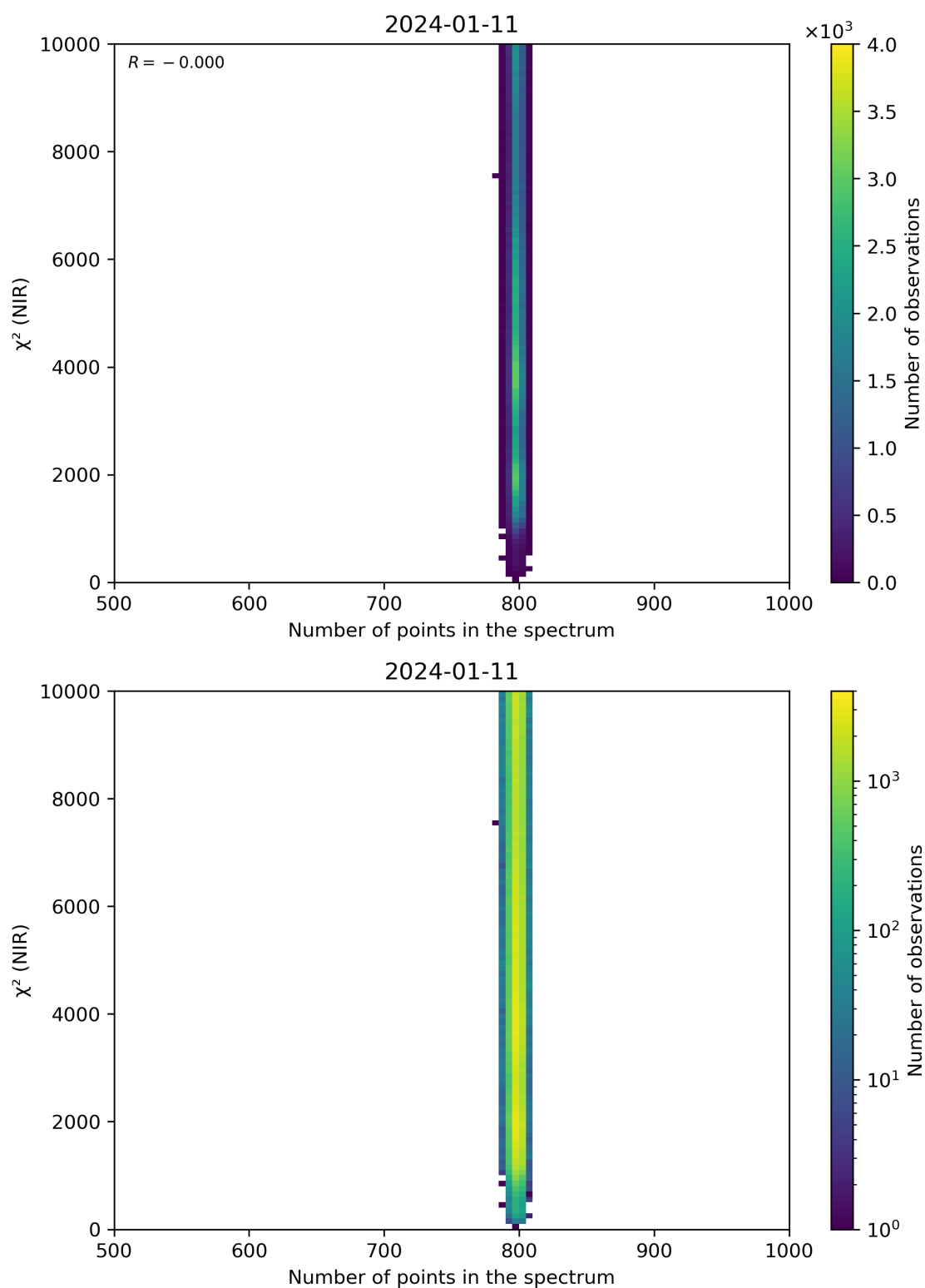
Figure 88: Scatter density plot of “Number of points in the spectrum” against “ \chi^2 (NIR)” for 2024-01-10 to 2024-01-12.
