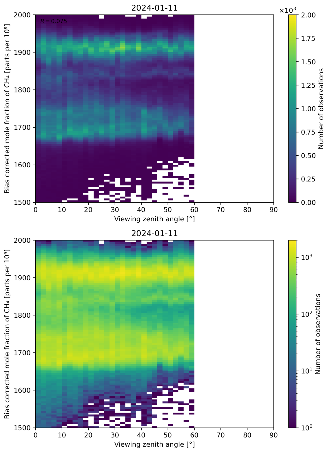
Figure 111: Scatter density plot of “Viewing zenith angle” against “Bias corrected mole fraction of CH 4 ” for 2024-01-10 to 2024-01-12.
