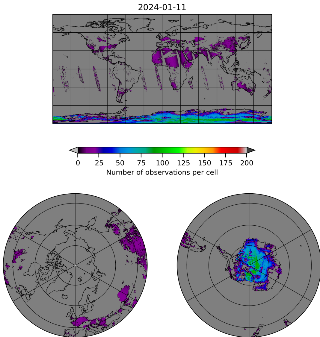
Figure 10: Map of the number of observations for 2024-01-10 to 2024-01-12
