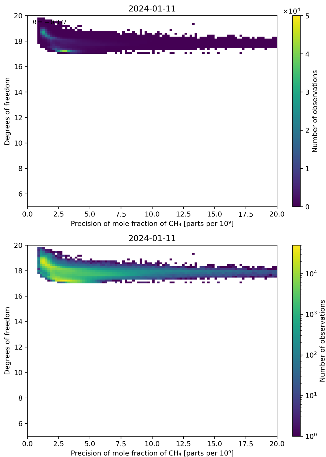
Figure 80: Scatter density plot of “Precision of mole fraction of CH 4 ” against “Degrees of freedom” for 2024-01-10 to 2024-01-12.
