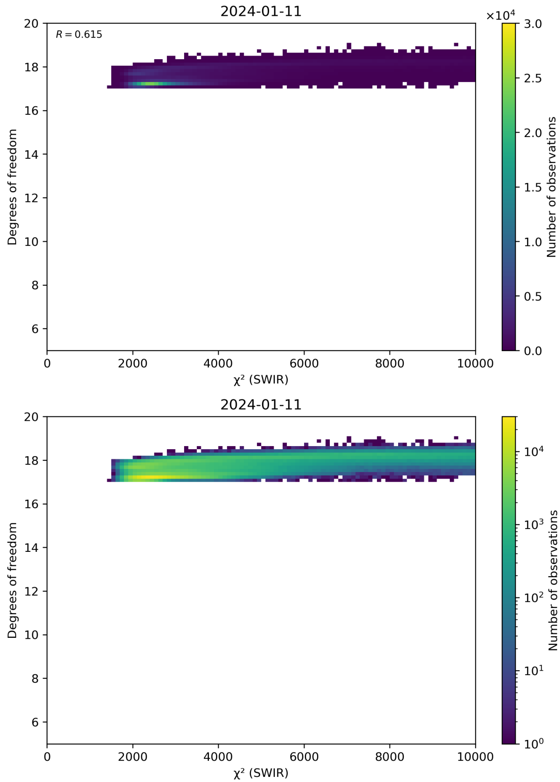
Figure 48: Scatter density plot of “ \chi^2 (SWIR)” against “Degrees of freedom” for 2024-01-10 to 2024-01-12.
