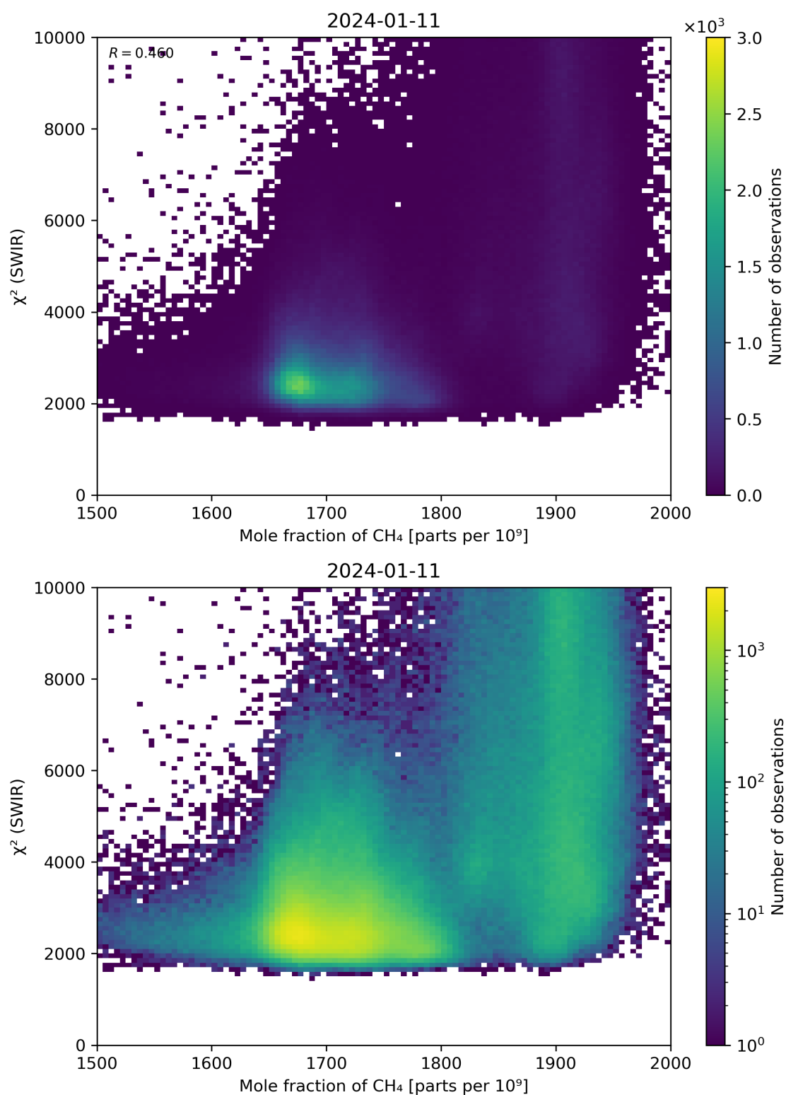
Figure 71: Scatter density plot of “Mole fraction of \text{CH}_4 ” against “ \chi^2 (SWIR)” for 2024-01-10 to 2024-01-12.
