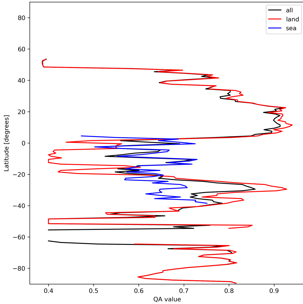
Figure 11: Zonal average of “QA value” for 2024-01-10 to 2024-01-12.
