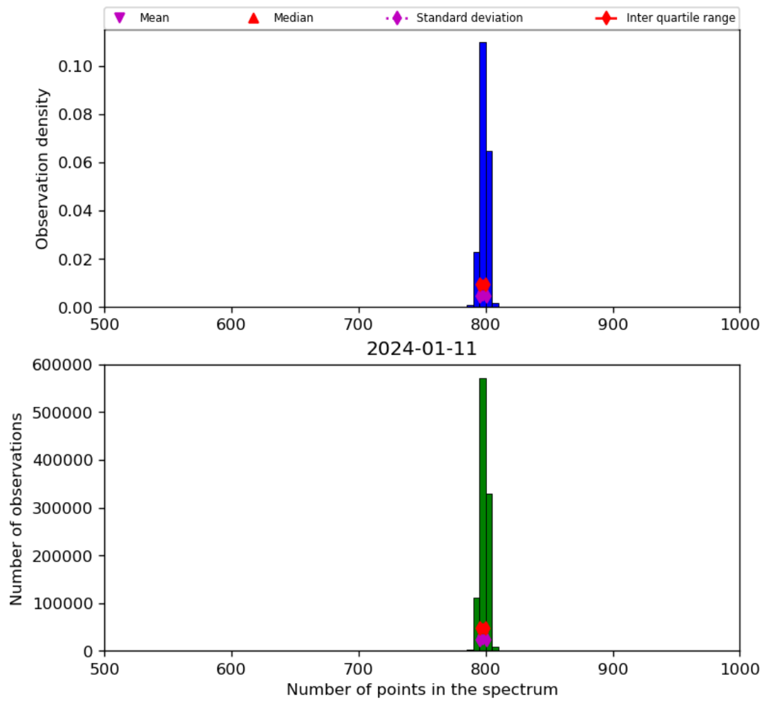
Figure 26: Histogram of “Number of points in the spectrum” for 2024-01-10 to 2024-01-12
