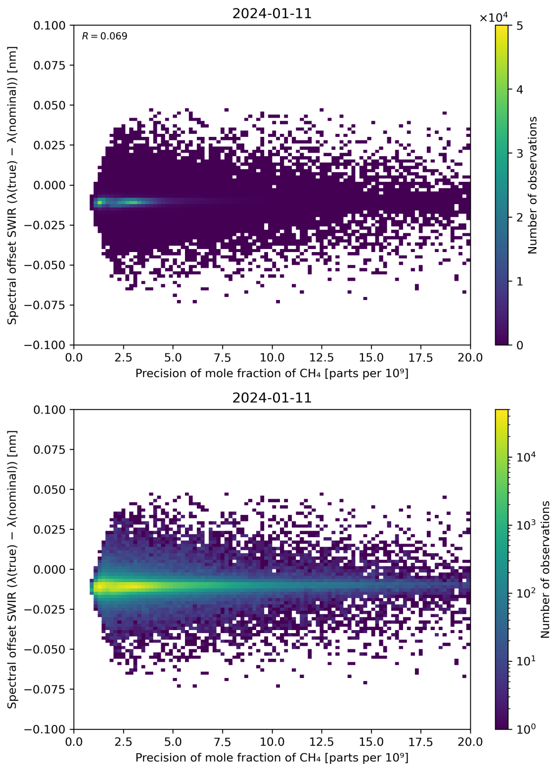
Figure 85: Scatter density plot of “Precision of mole fraction of CH 4 ” against “Spectral offset SWIR ( \lambda(\text{true}) - \lambda(\text{nominal}) )” for 2024-01-10 to 2024-01-12.
