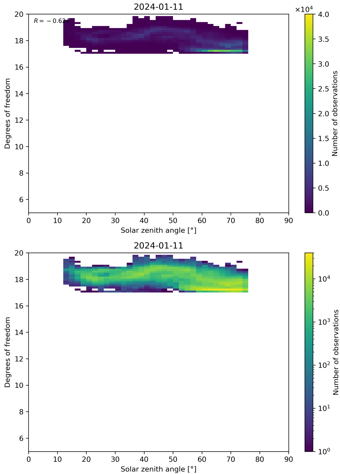
Figure 96: Scatter density plot of “Solar zenith angle” against “Degrees of freedom” for 2024-01-10 to 2024-01-12.
