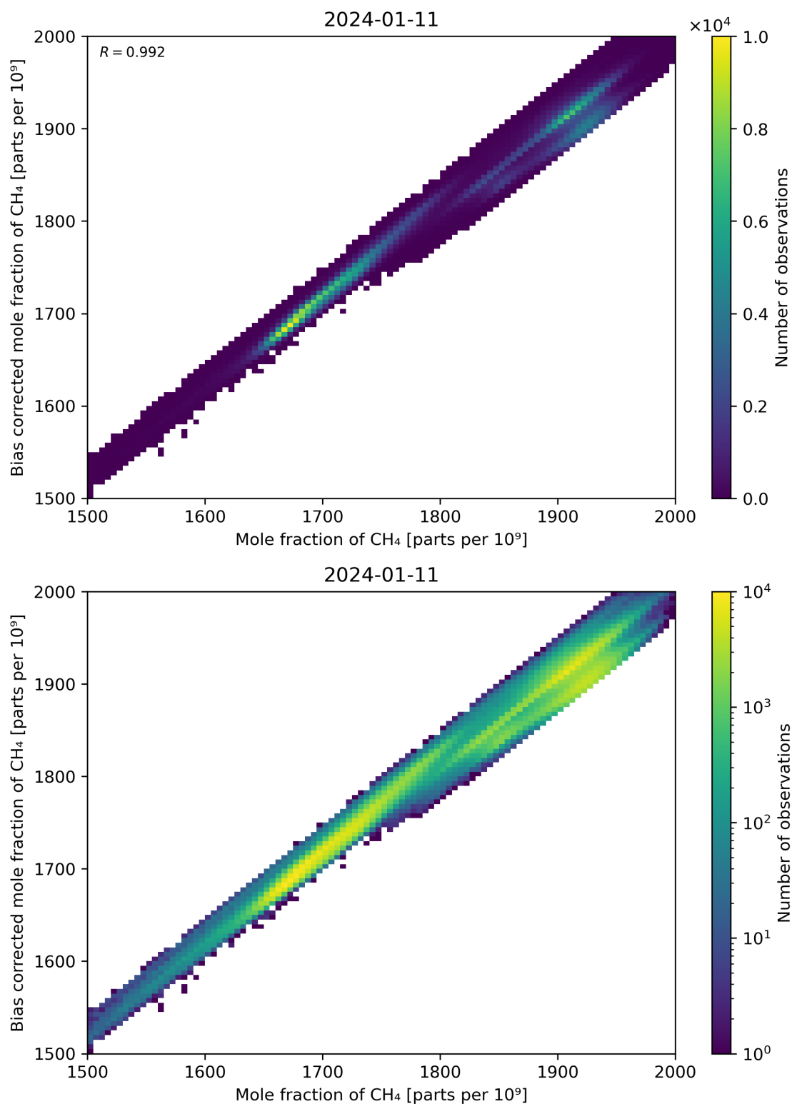
Figure 74: Scatter density plot of “Mole fraction of CH 4 ” against “Bias corrected mole fraction of CH 4 ” for 2024-01-10 to 2024-01-12.
