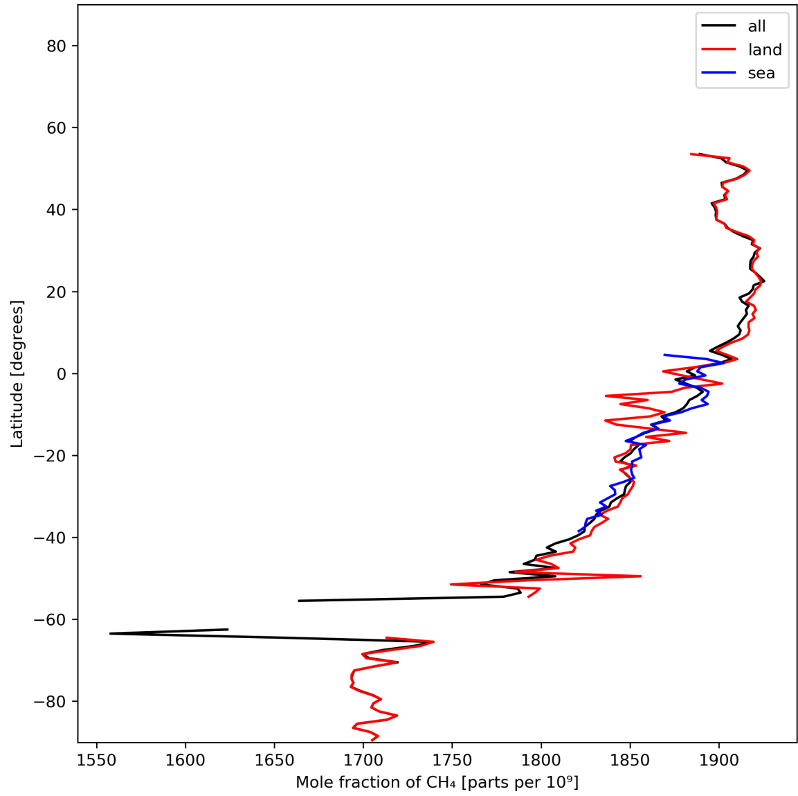
Figure 12: Zonal average of “Mole fraction of CH 4 ” for 2024-01-10 to 2024-01-12.
