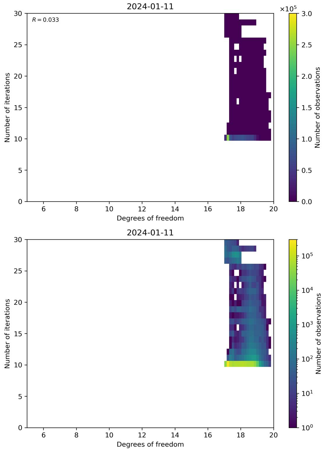
Figure 52: Scatter density plot of “Degrees of freedom” against “Number of iterations” for 2024-01-10 to 2024-01-12.
