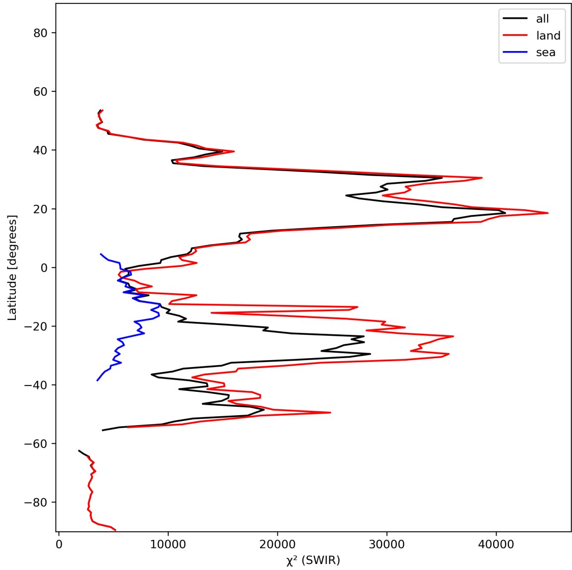
Figure 17: Zonal average of “ \chi^2 (SWIR)” for 2024-01-10 to 2024-01-12.
