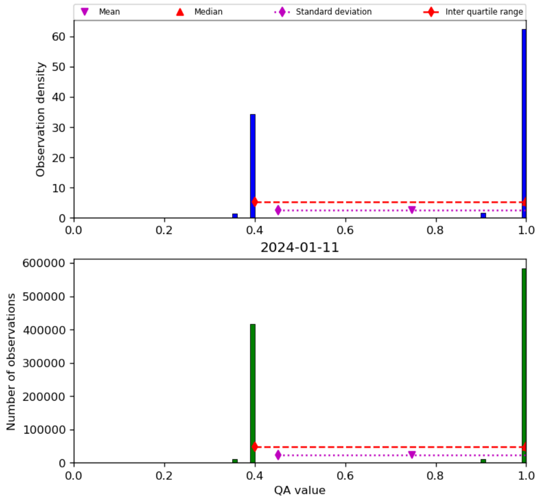
Figure 22: Histogram of “QA value” for 2024-01-10 to 2024-01-12
