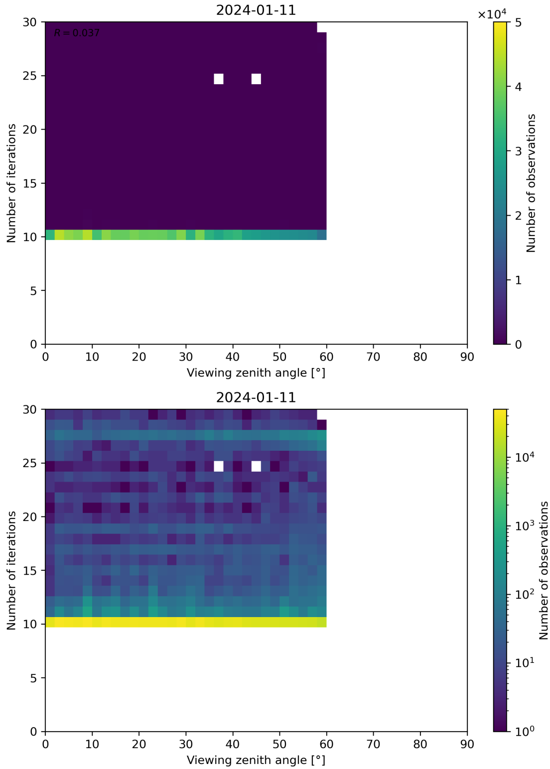
Figure 113: Scatter density plot of “Viewing zenith angle” against “Number of iterations” for 2024-01-10 to 2024-01-12.
