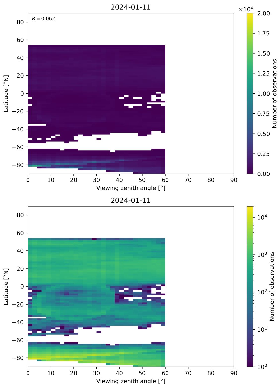
Figure 109: Scatter density plot of “Viewing zenith angle” against “Latitude” for 2024-01-10 to 2024-01-12.
