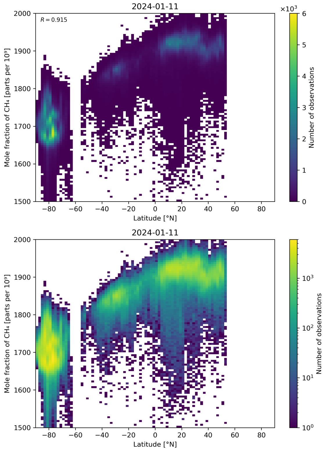
Figure 57: Scatter density plot of “Latitude” against “Mole fraction of \text{CH}_4 ” for 2024-01-10 to 2024-01-12.
