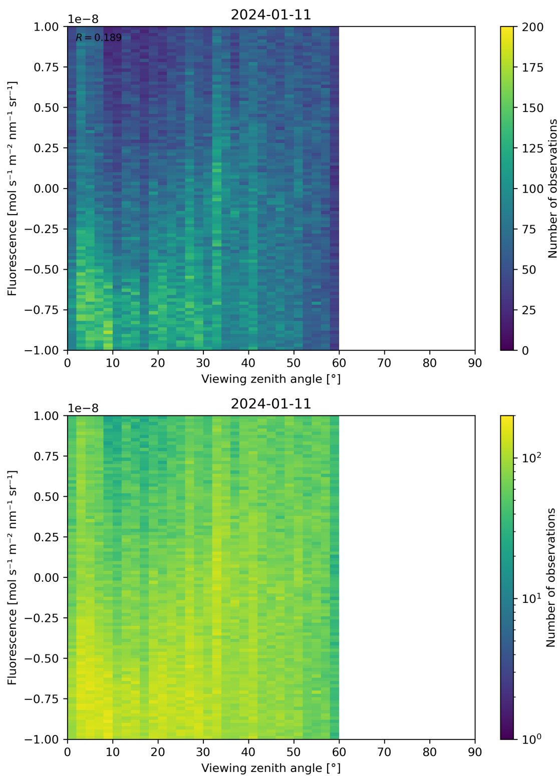
Figure 108: Scatter density plot of “Viewing zenith angle” against “Fluorescence” for 2024-01-10 to 2024-01-12.
