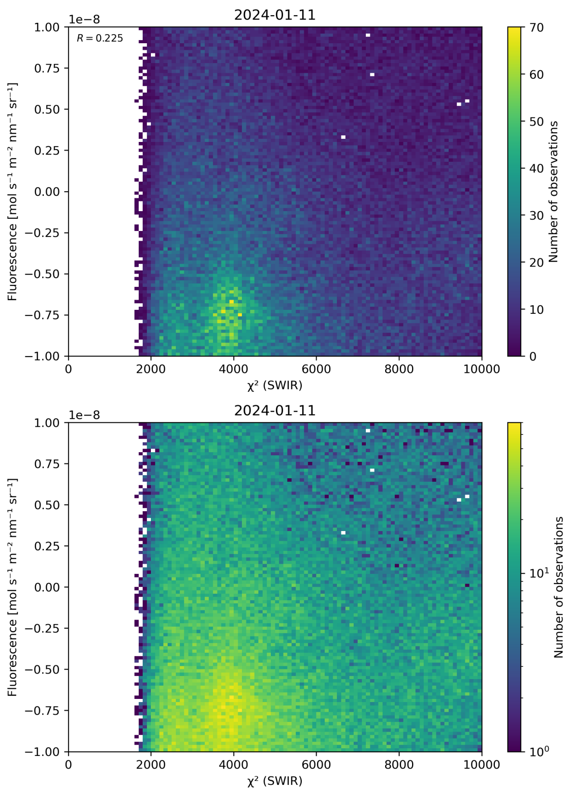
Figure 49: Scatter density plot of “ \chi^2 (SWIR)” against “Fluorescence” for 2024-01-10 to 2024-01-12.
