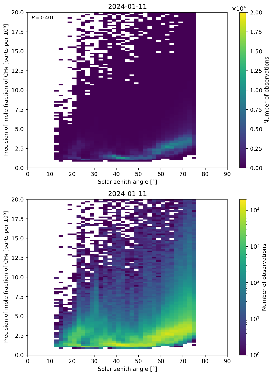
Figure 101: Scatter density plot of “Solar zenith angle” against “Precision of mole fraction of CH 4 ” for 2024-01-10 to 2024-01-12.
