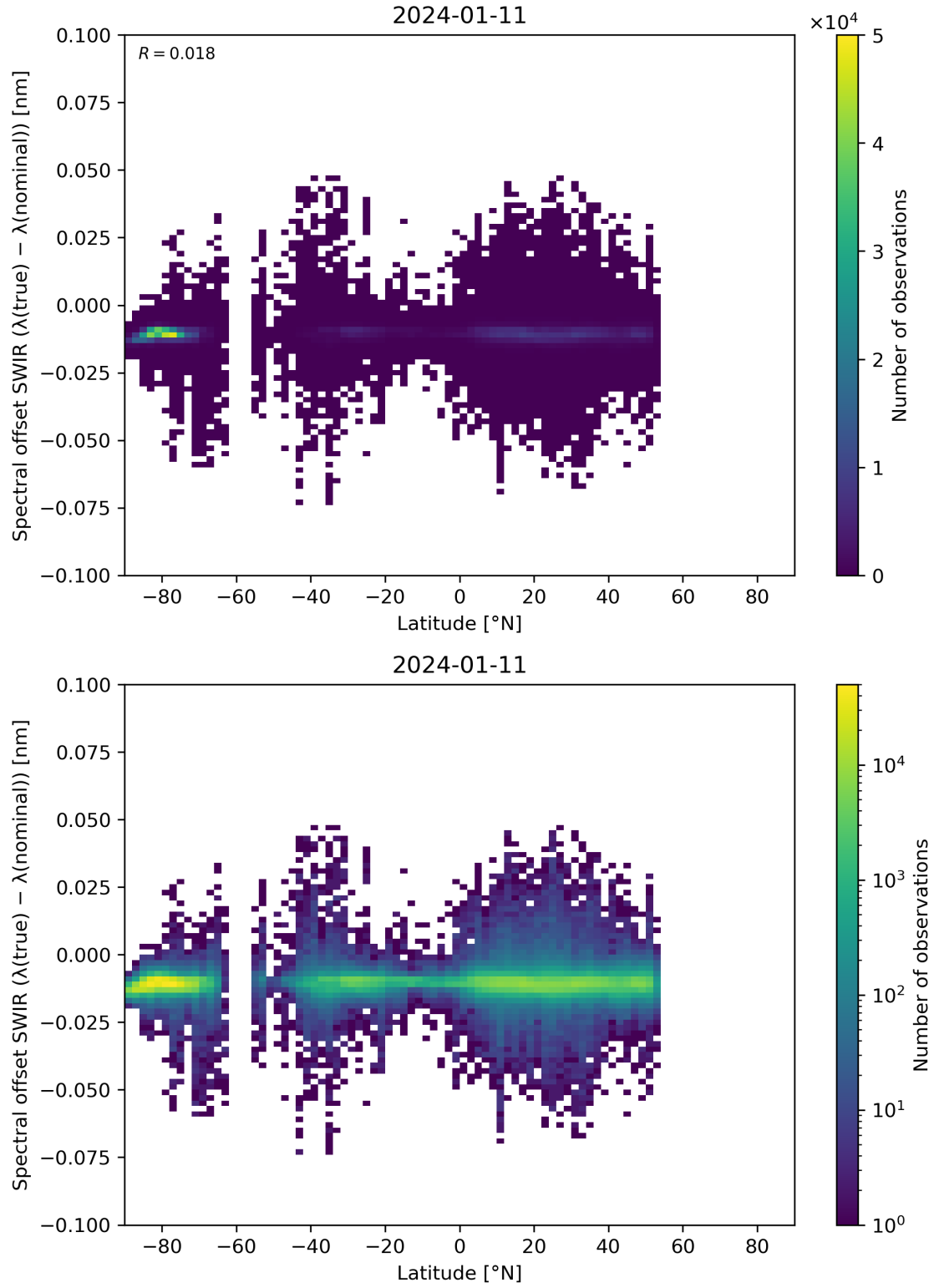
Figure 62: Scatter density plot of “Latitude” against “Spectral offset SWIR ( \lambda(\text{true}) - \lambda(\text{nominal}) )” for 2024-01-10 to 2024-01-12.
