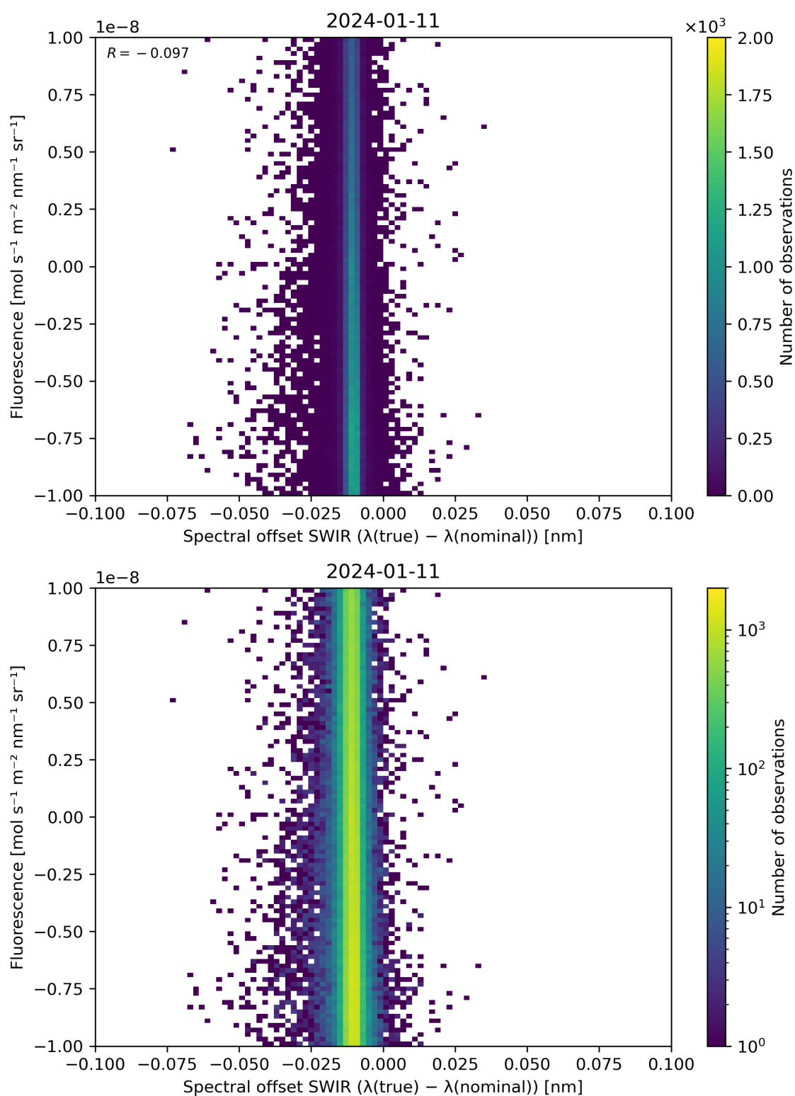
Figure 120: Scatter density plot of “Spectral offset SWIR ( \lambda(\text{true}) - \lambda(\text{nominal}) )” against “Fluorescence” for 2024-01-10 to 2024-01-12.
