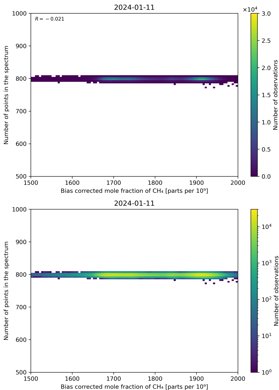
Figure 68: Scatter density plot of “Bias corrected mole fraction of CH 4 ” against “Number of points in the spectrum” for 2024-01-10 to 2024-01-12.
