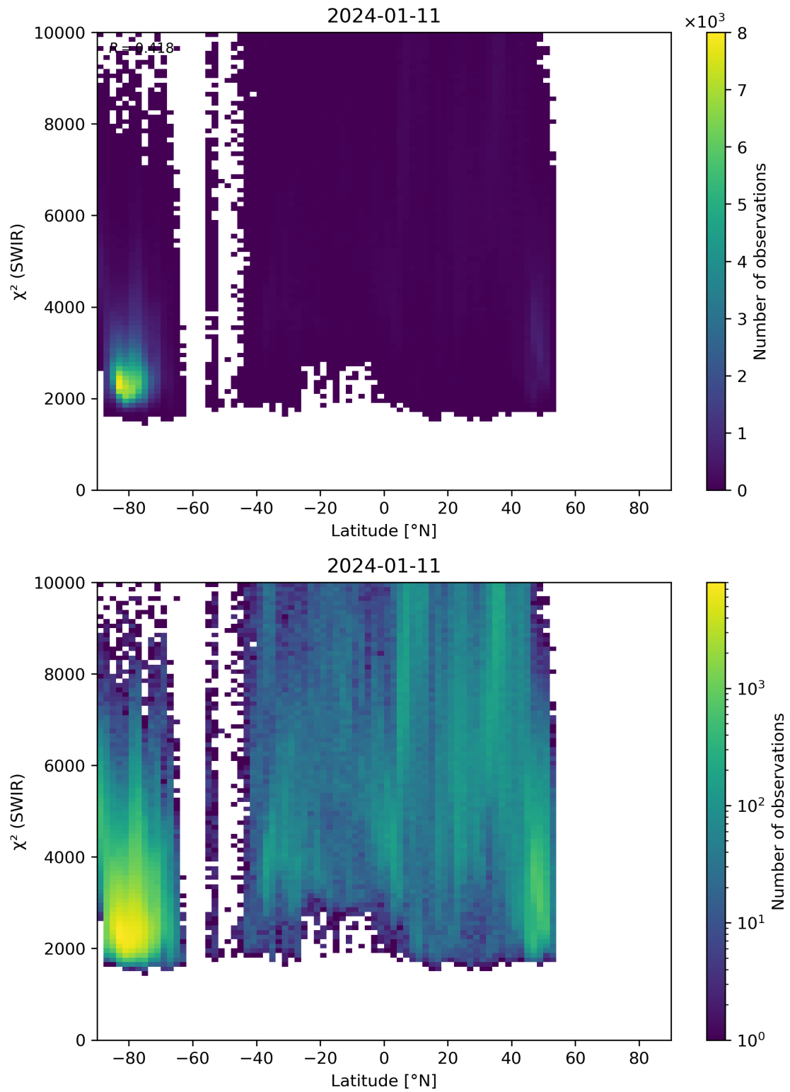
Figure 54: Scatter density plot of “Latitude” against “ \chi^2 (SWIR)” for 2024-01-10 to 2024-01-12.
