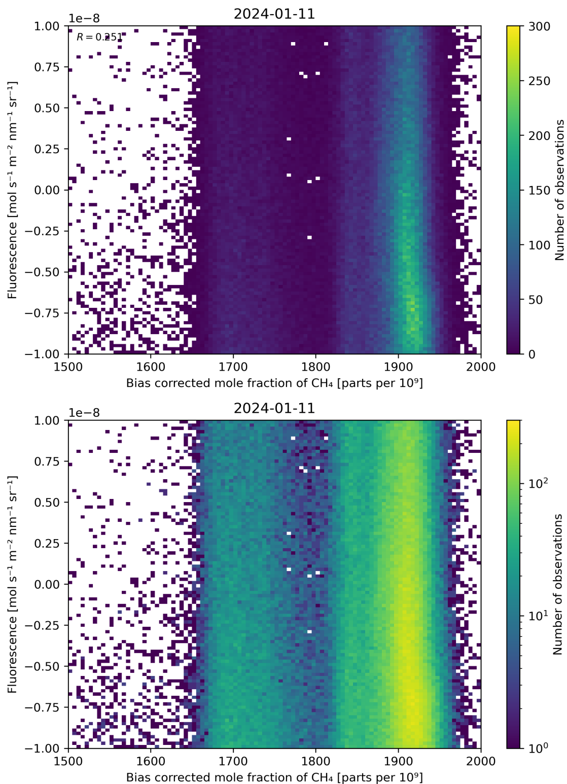
Figure 66: Scatter density plot of “Bias corrected mole fraction of \text{CH}_4 ” against “Fluorescence” for 2024-01-10 to 2024-01-12.
