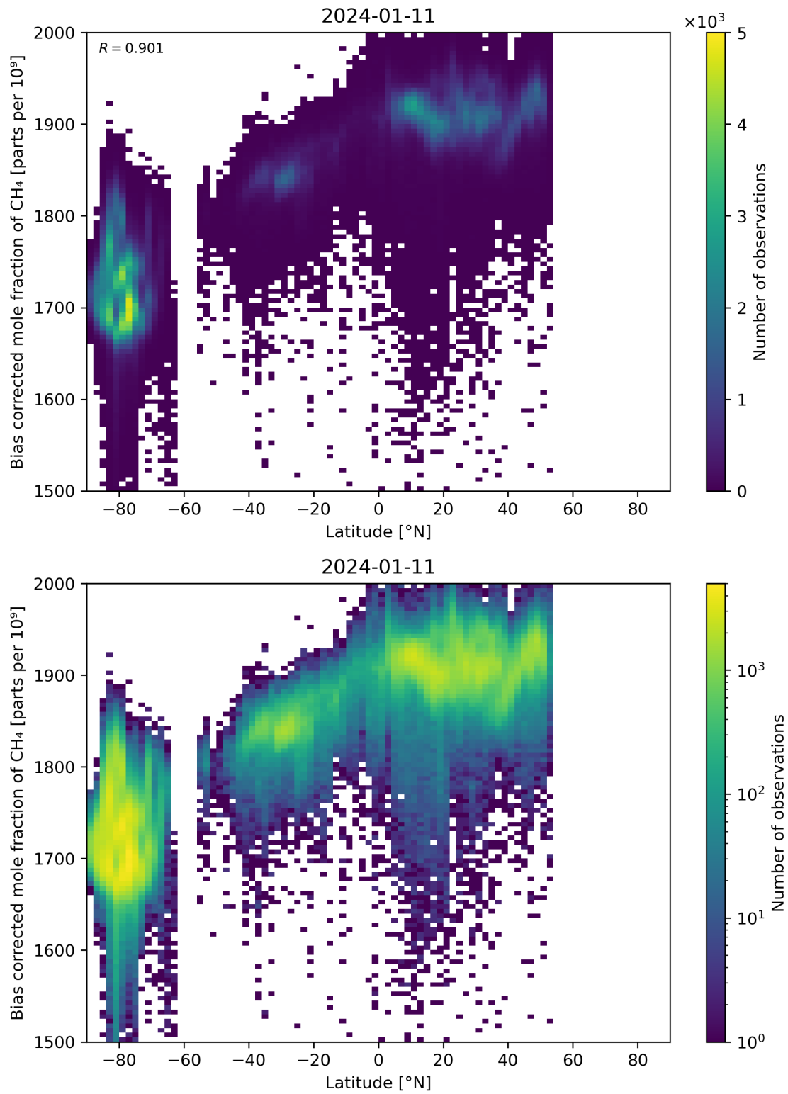
Figure 58: Scatter density plot of “Latitude” against “Bias corrected mole fraction of CH 4 ” for 2024-01-10 to 2024-01-12.
