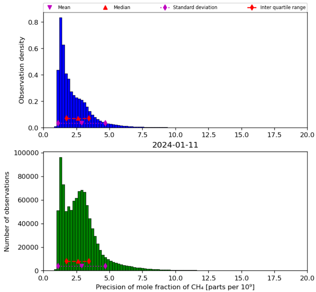
Figure 24: Histogram of “Precision of mole fraction of CH 4 ” for 2024-01-10 to 2024-01-12
