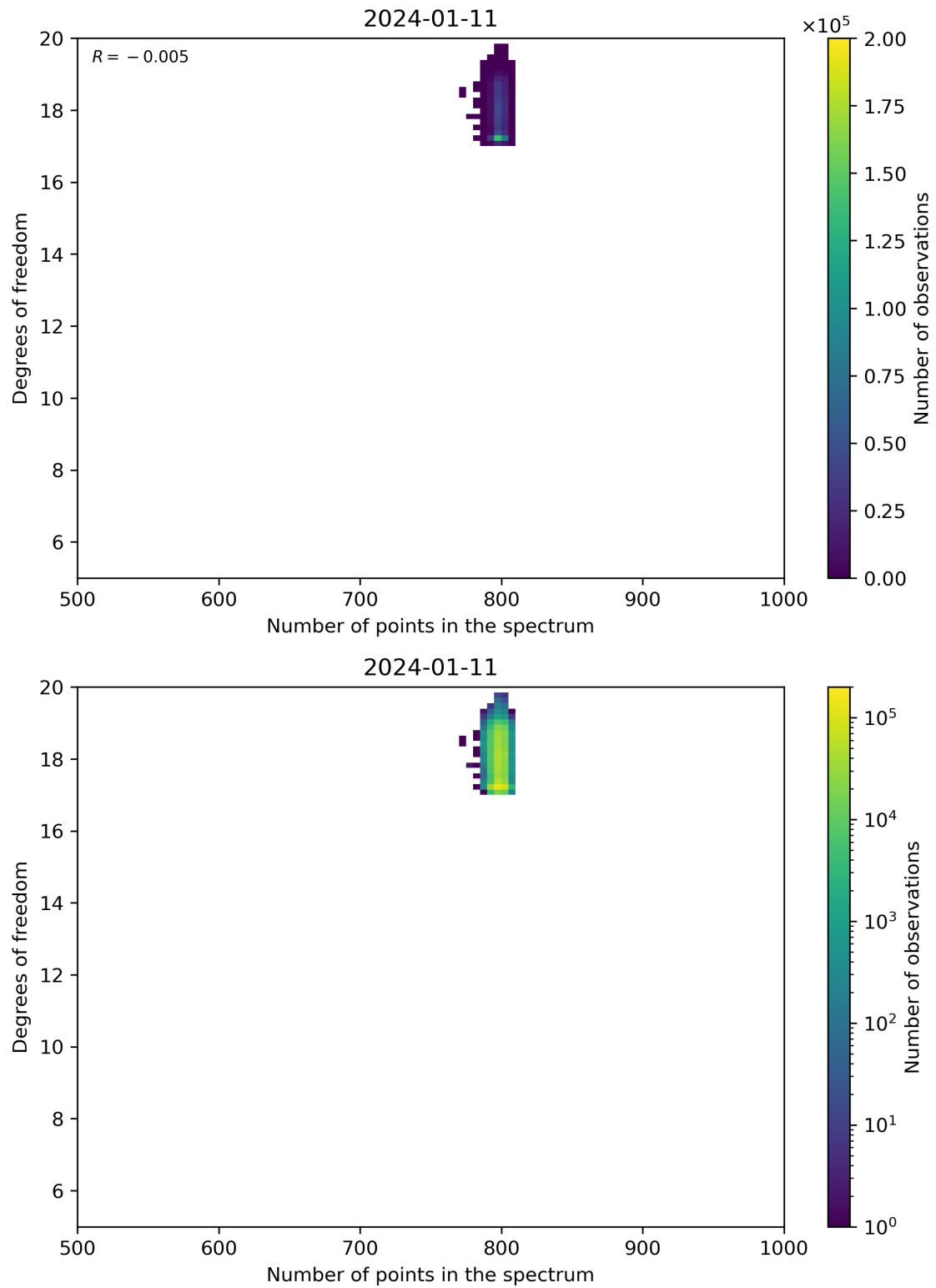
Figure 90: Scatter density plot of “Number of points in the spectrum” against “Degrees of freedom” for 2024-01-10 to 2024-01-12.
