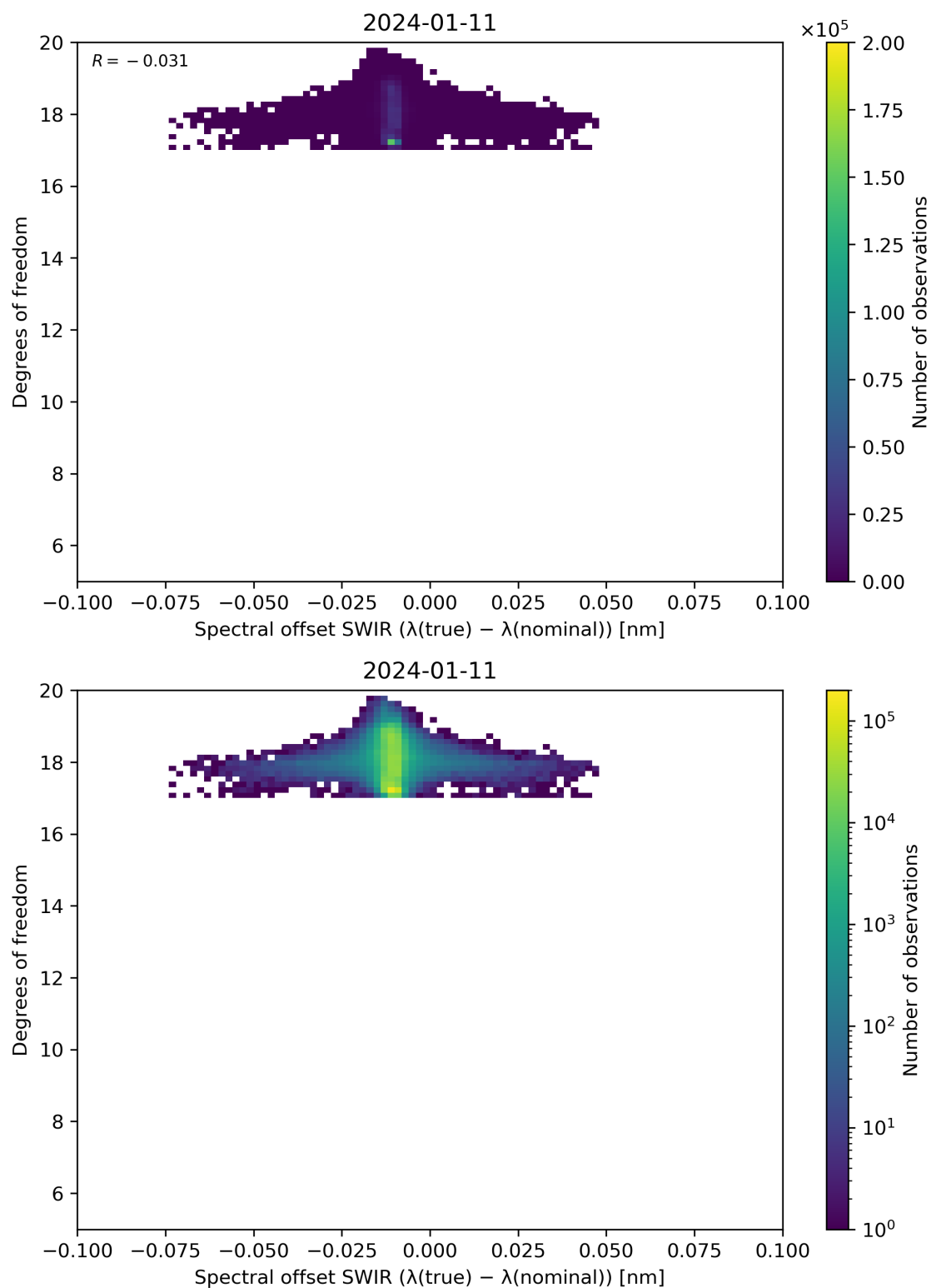
Figure 119: Scatter density plot of “Spectral offset SWIR ( \lambda(\text{true}) - \lambda(\text{nominal}) )” against “Degrees of freedom” for 2024-01-10 to 2024-01-12.
