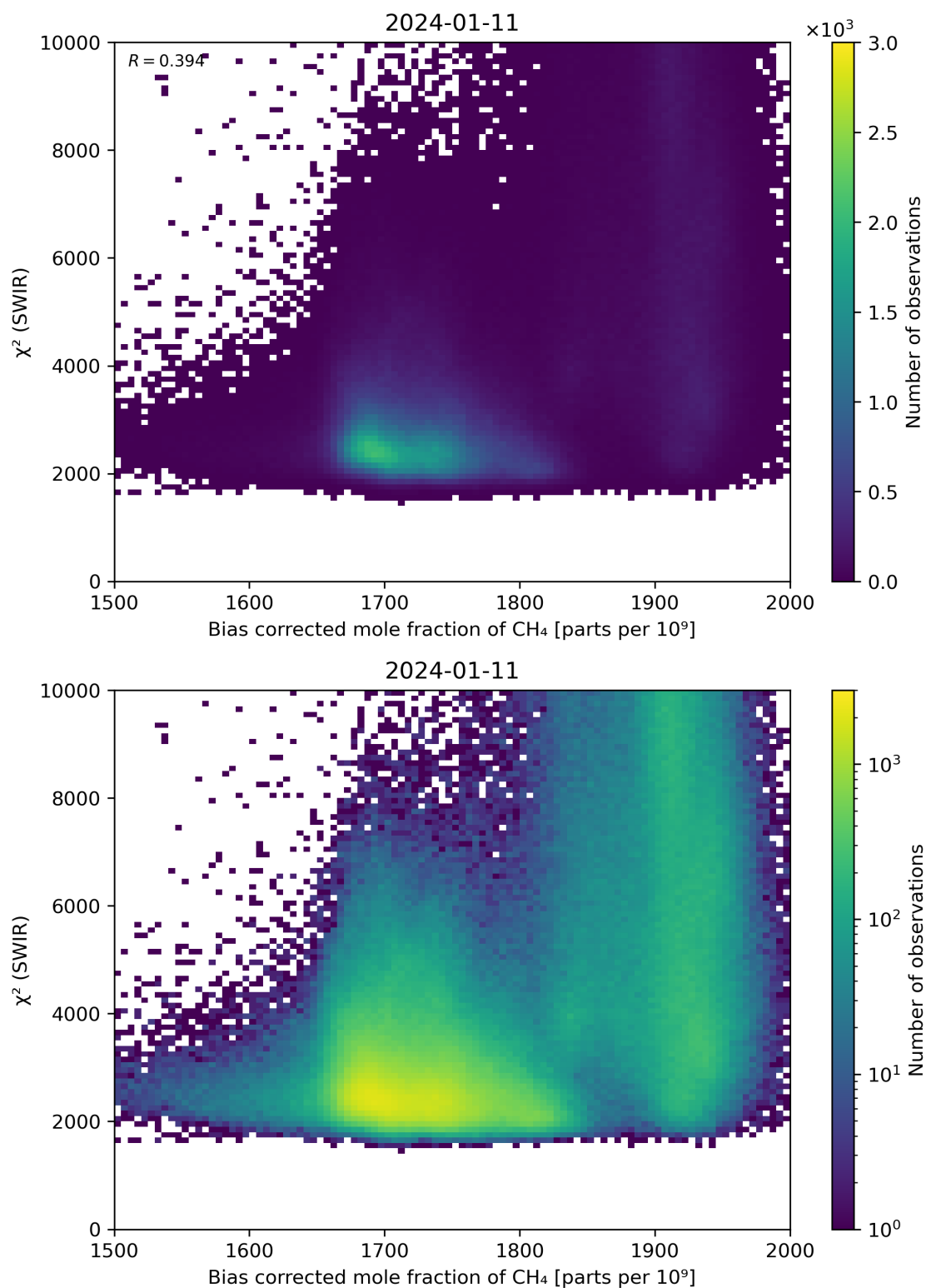
Figure 64: Scatter density plot of “Bias corrected mole fraction of \text{CH}_4 ” against “ \chi^2 (SWIR)” for 2024-01-10 to 2024-01-12.
