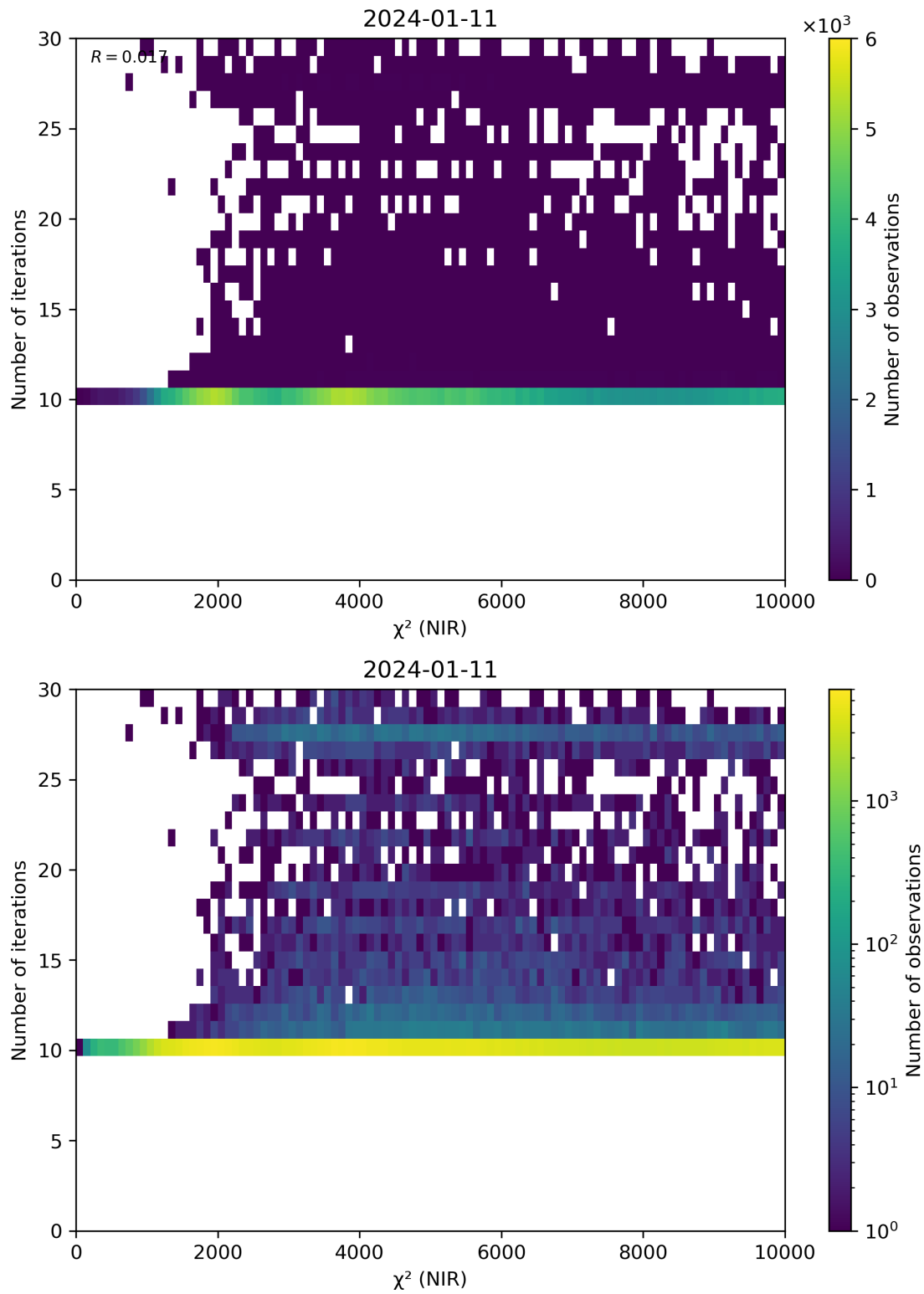
Figure 46: Scatter density plot of “ \chi^2 (NIR)” against “Number of iterations” for 2024-01-10 to 2024-01-12.
