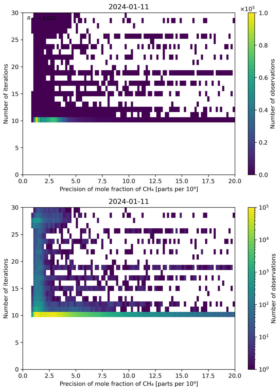
Figure 83: Scatter density plot of “Precision of mole fraction of CH 4 ” against “Number of iterations” for 2024-01-10 to 2024-01-12.
