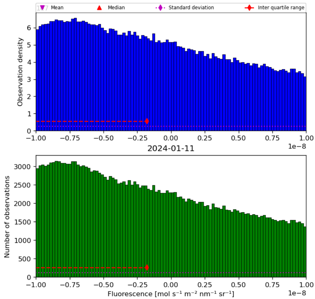
Figure 32: Histogram of “Fluorescence” for 2024-01-10 to 2024-01-12
