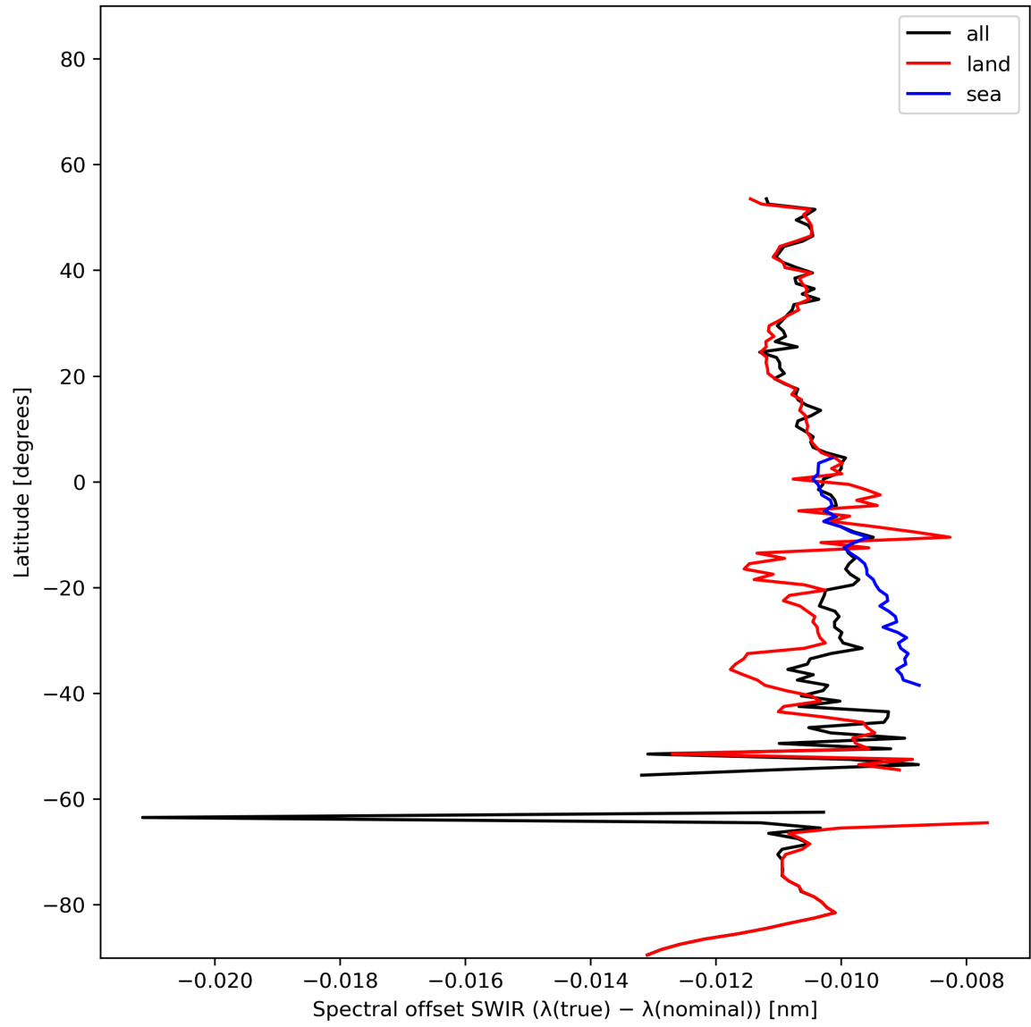
Figure 16: Zonal average of “Spectral offset SWIR ( \lambda(\text{true}) - \lambda(\text{nominal}) )” for 2024-01-10 to 2024-01-12.
