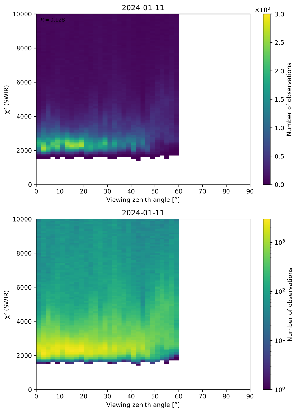
Figure 106: Scatter density plot of “Viewing zenith angle” against “ \chi^2 (SWIR)” for 2024-01-10 to 2024-01-12.
