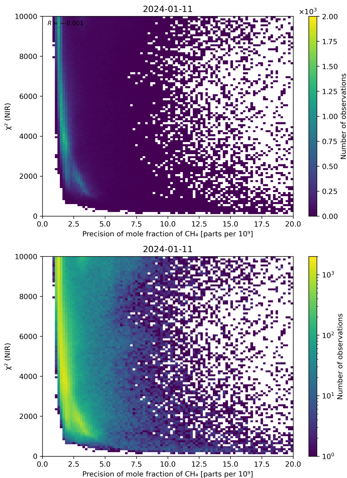
Figure 78: Scatter density plot of “Precision of mole fraction of CH 4 ” against “ \chi^2 (NIR)” for 2024-01-10 to 2024-01-12.
