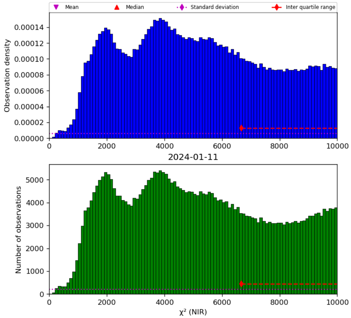
Figure 29: Histogram of “ \chi^2 (NIR)” for 2024-01-10 to 2024-01-12
