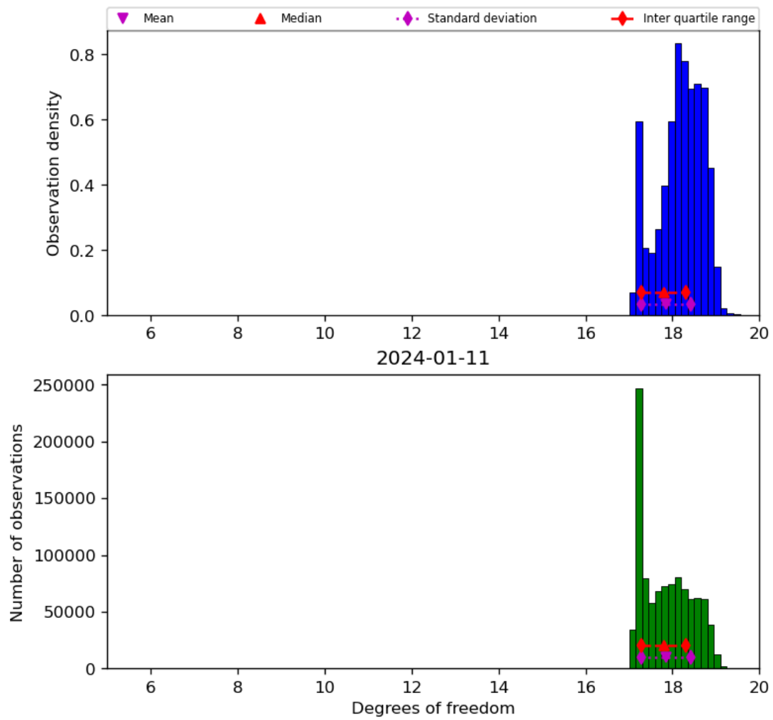
Figure 30: Histogram of “Degrees of freedom” for 2024-01-10 to 2024-01-12
