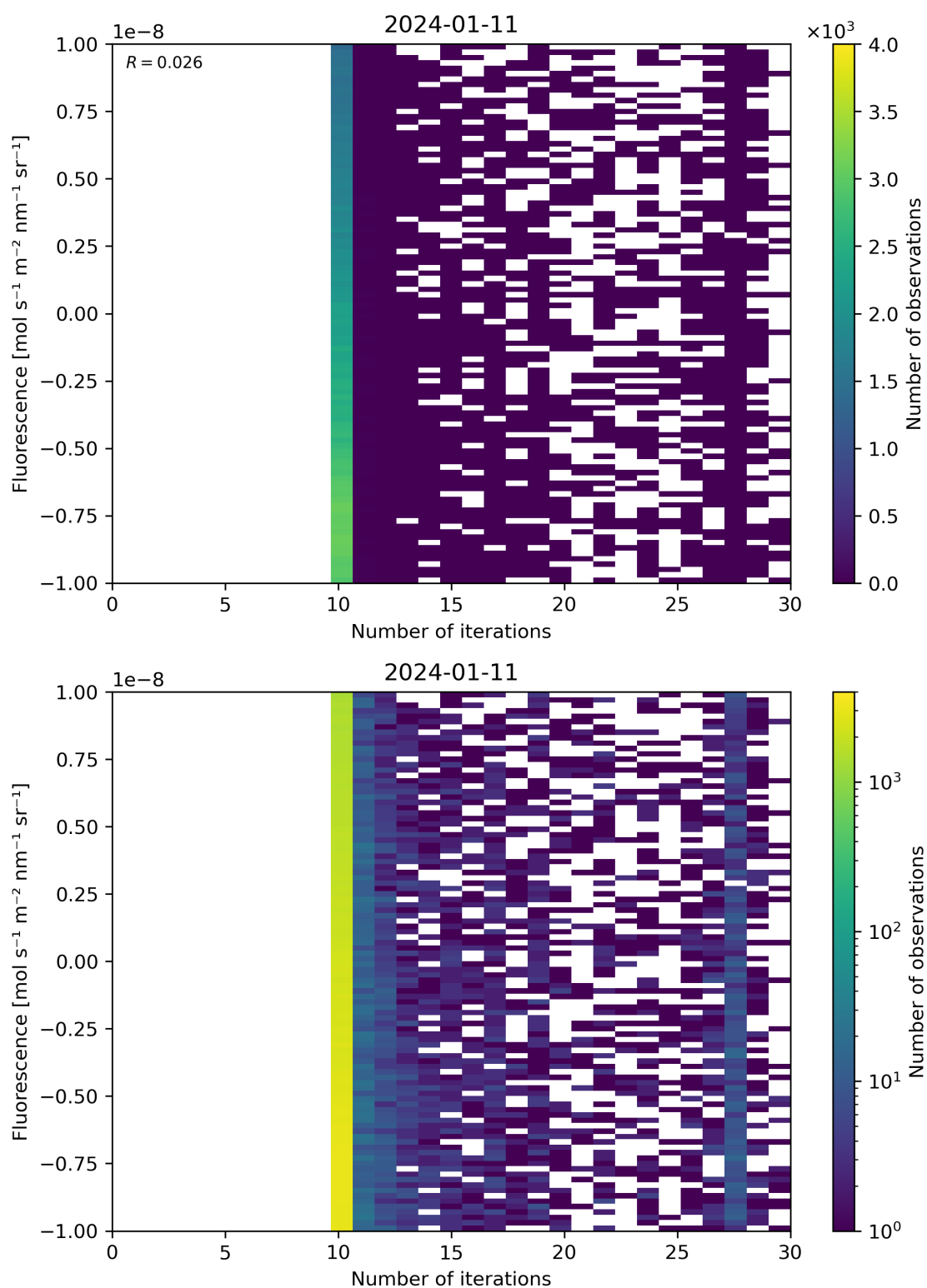
Figure 87: Scatter density plot of “Number of iterations” against “Fluorescence” for 2024-01-10 to 2024-01-12.
