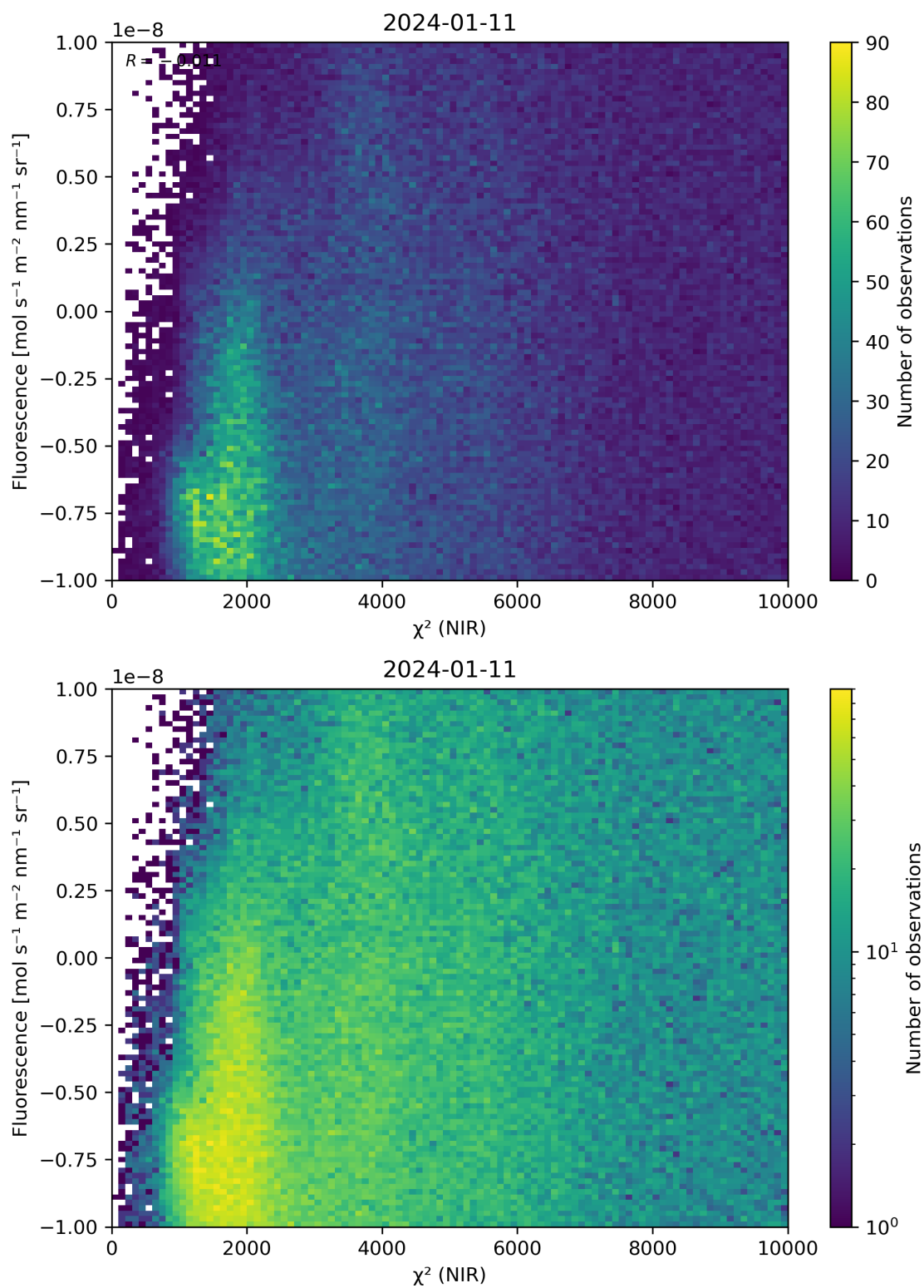
Figure 45: Scatter density plot of “ \chi^2 (NIR)” against “Fluorescence” for 2024-01-10 to 2024-01-12.
