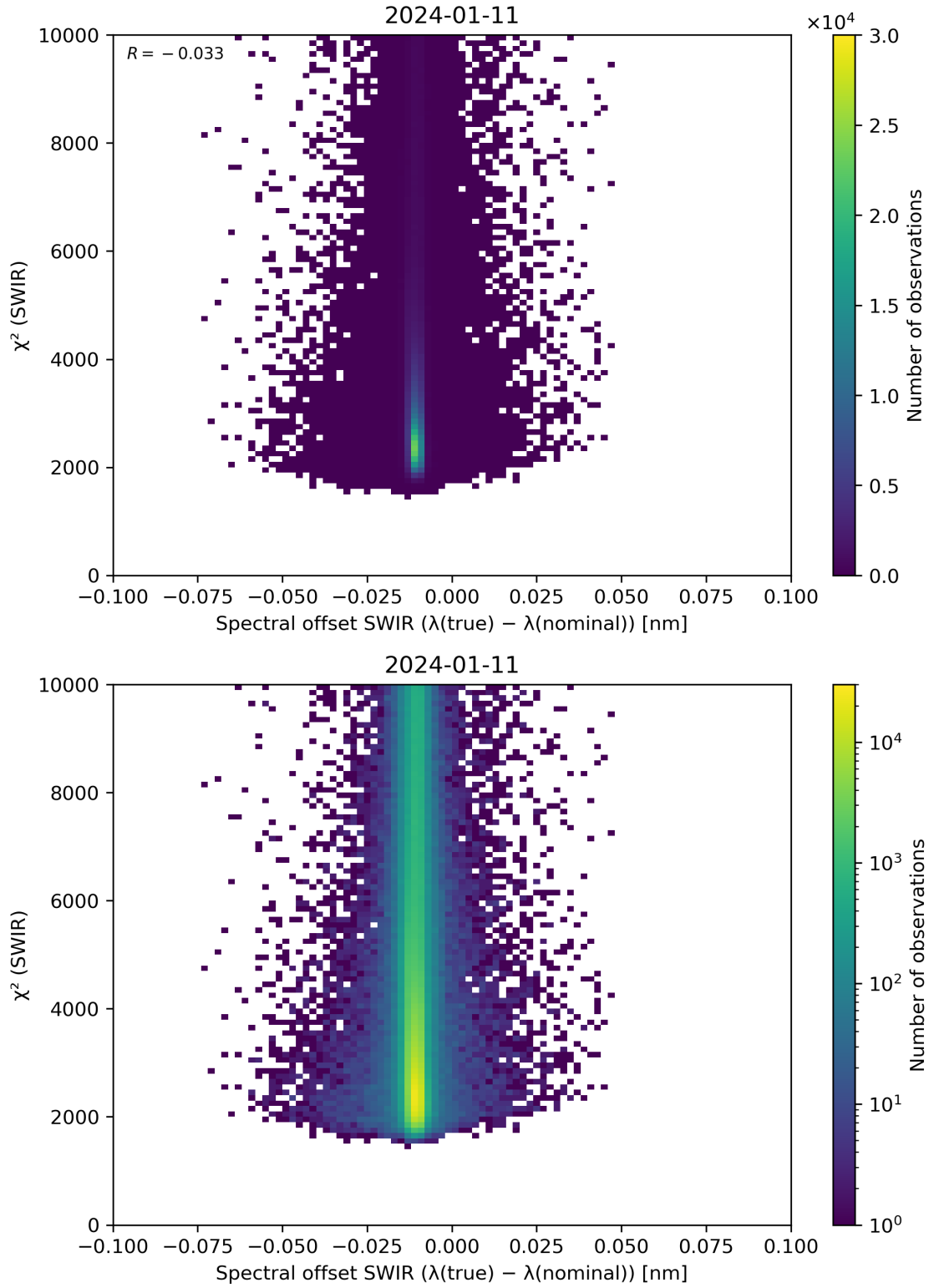
Figure 118: Scatter density plot of “Spectral offset SWIR ( \lambda(\text{true}) - \lambda(\text{nominal}) )” against “ \chi^2 (SWIR)” for 2024-01-10 to 2024-01-12.
