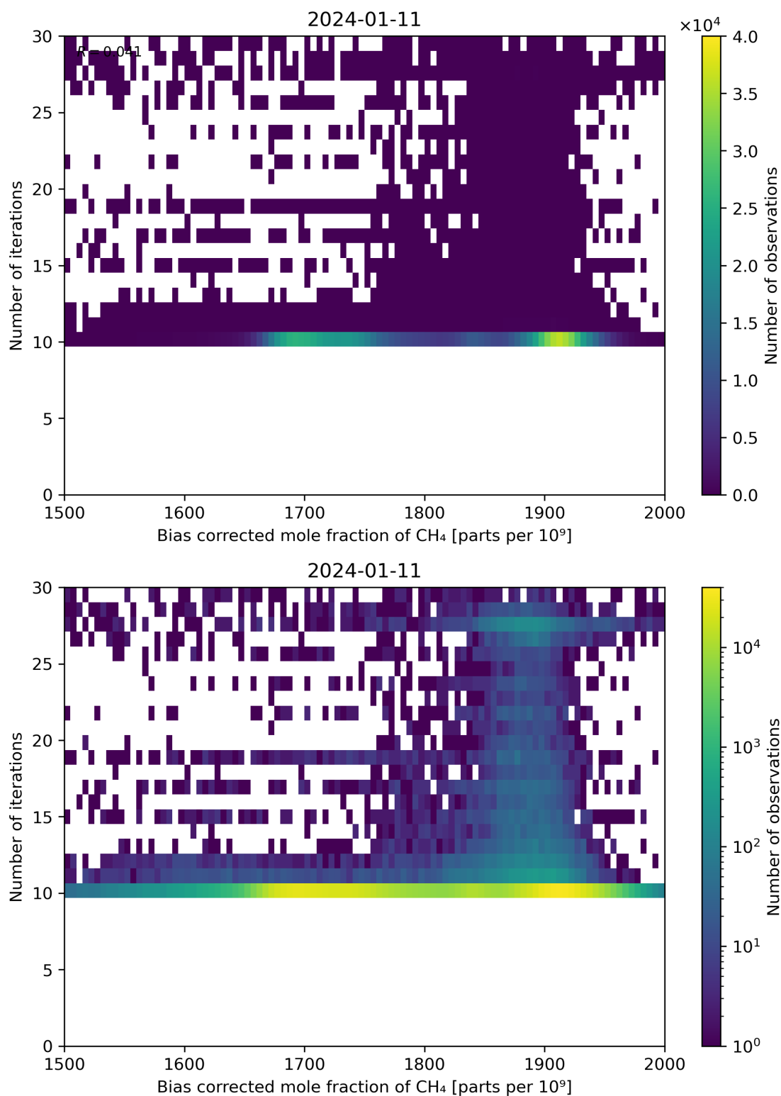
Figure 67: Scatter density plot of “Bias corrected mole fraction of \text{CH}_4 ” against “Number of iterations” for 2024-01-10 to 2024-01-12.
