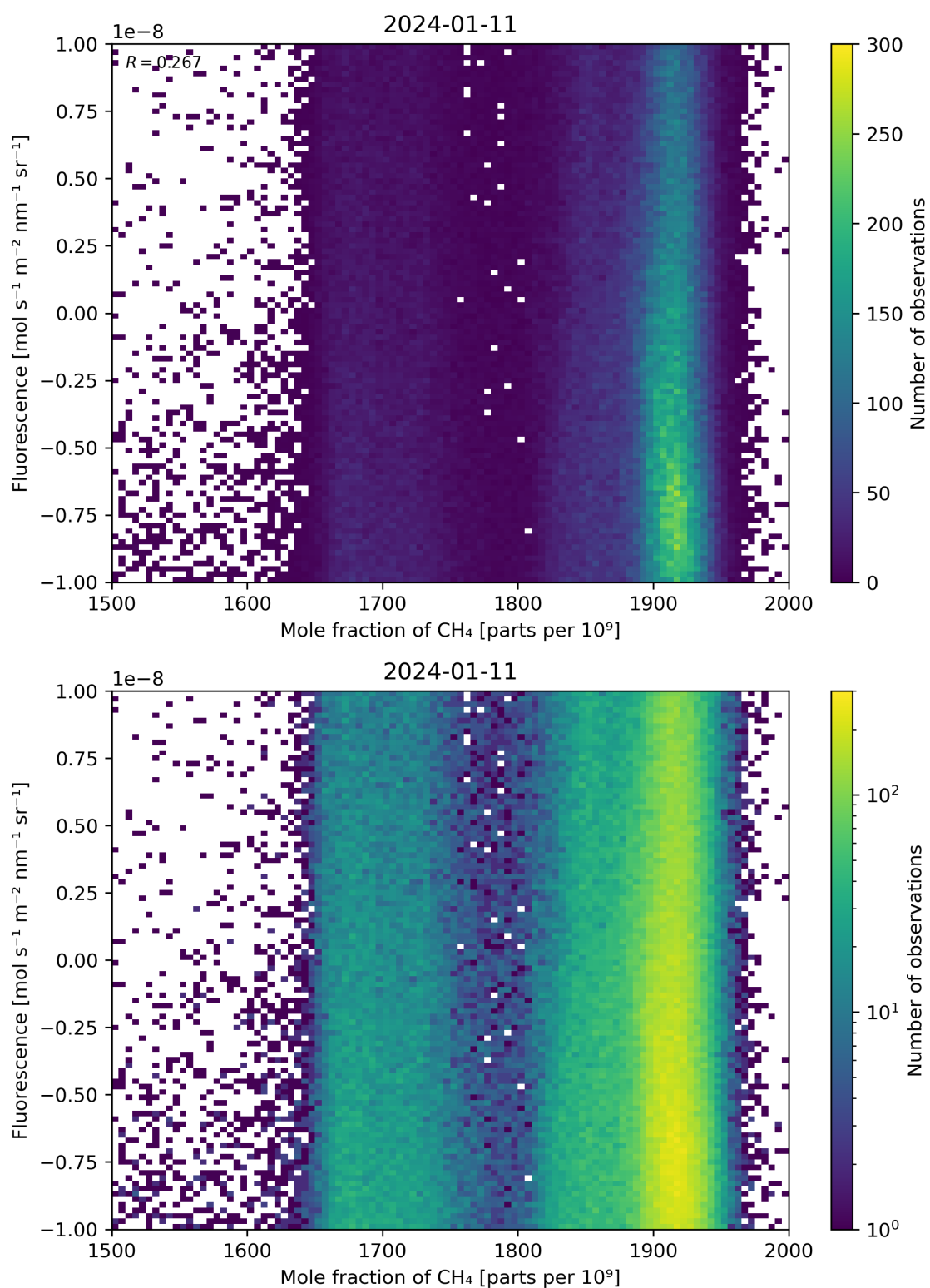
Figure 73: Scatter density plot of “Mole fraction of \text{CH}_4 ” against “Fluorescence” for 2024-01-10 to 2024-01-12.
