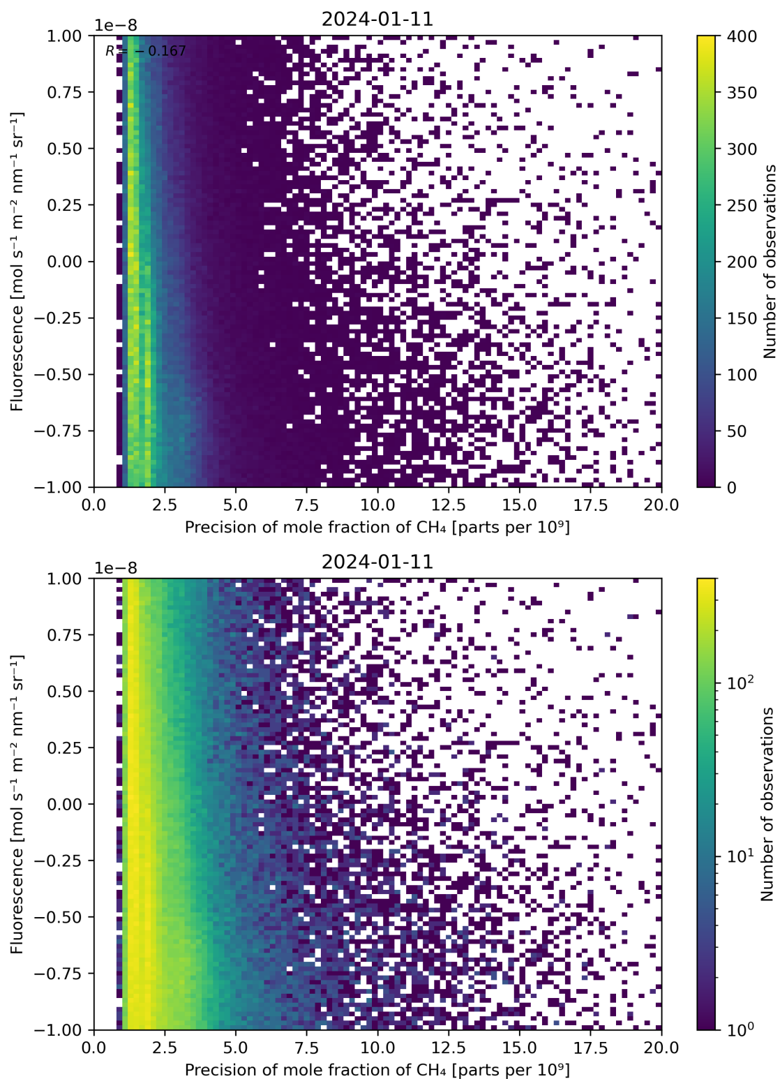
Figure 81: Scatter density plot of “Precision of mole fraction of CH 4 ” against “Fluorescence” for 2024-01-10 to 2024-01-12.
