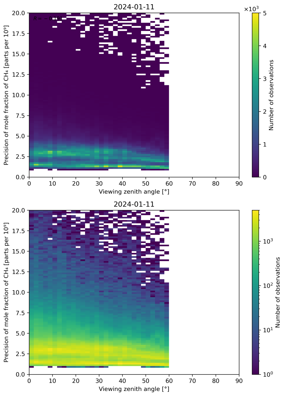
Figure 112: Scatter density plot of “Viewing zenith angle” against “Precision of mole fraction of \text{CH}_4 ” for 2024-01-10 to 2024-01-12.
