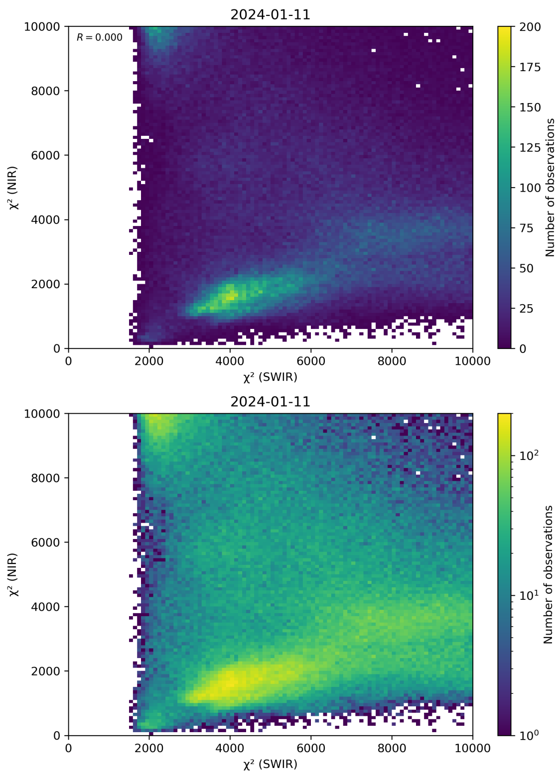
Figure 47: Scatter density plot of “ \chi^2 (SWIR)” against “ \chi^2 (NIR)” for 2024-01-10 to 2024-01-12.
