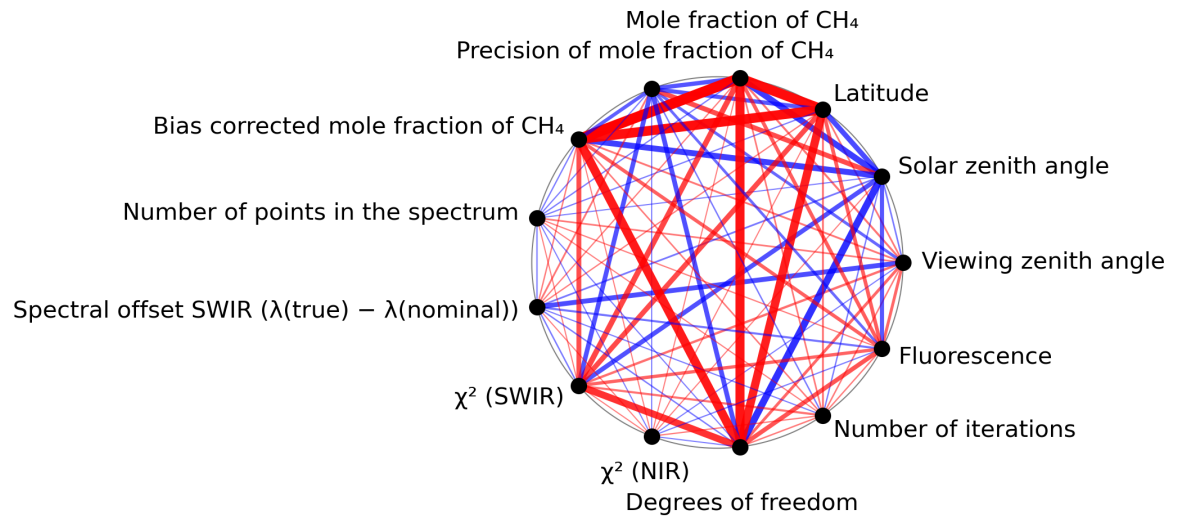
Figure 1: Map of correlation graph for 2024-01-10 to 2024-01-12.
