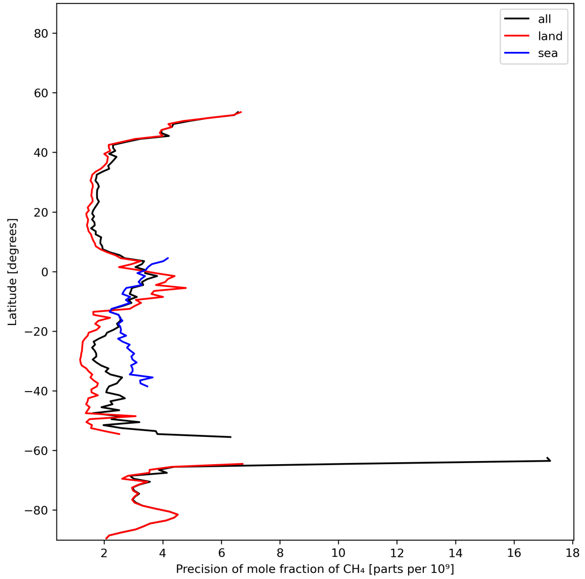
Figure 13: Zonal average of “Precision of mole fraction of CH 4 ” for 2024-01-10 to 2024-01-12.
