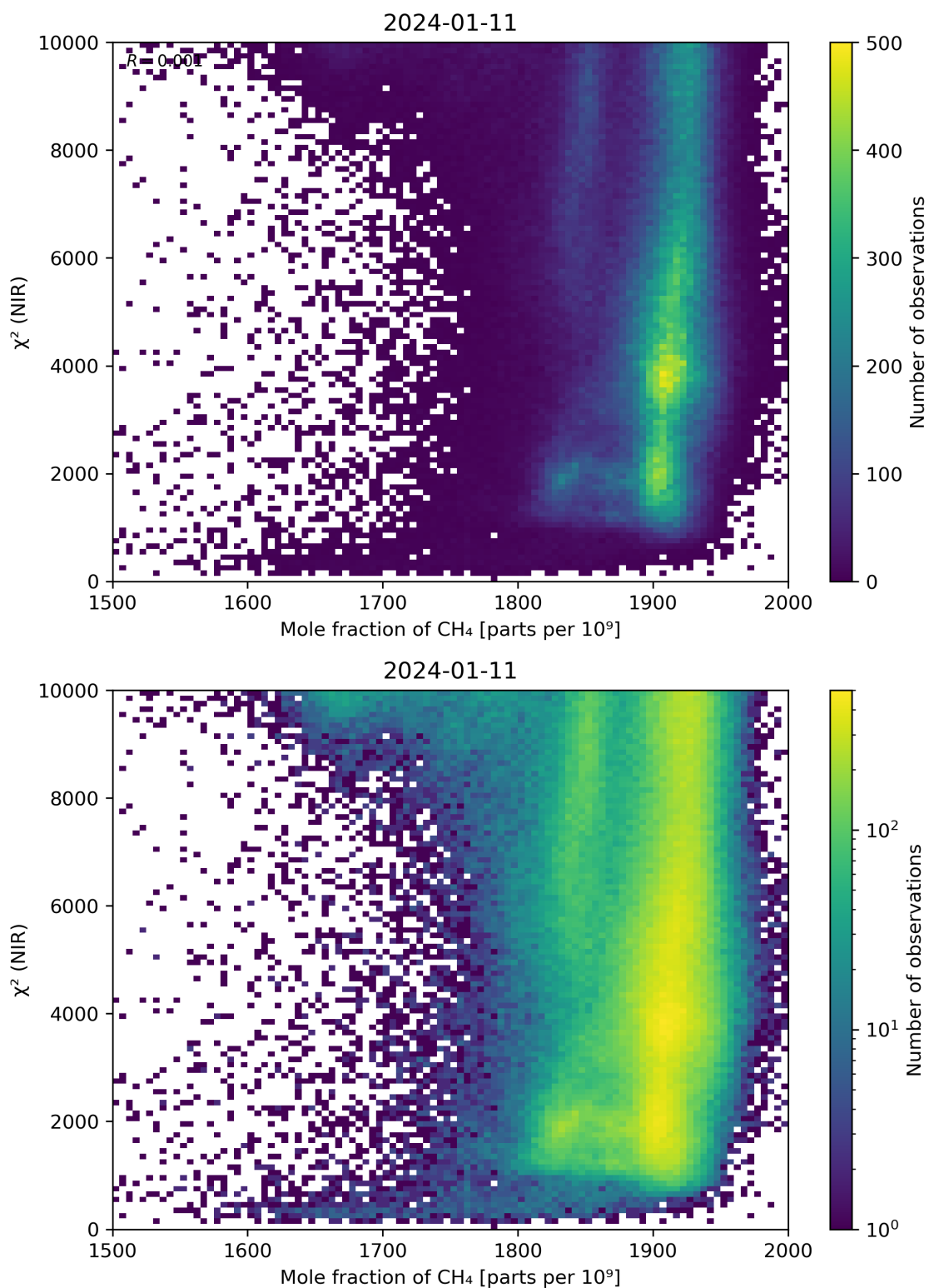
Figure 70: Scatter density plot of “Mole fraction of \text{CH}_4 ” against “ \chi^2 (NIR)” for 2024-01-10 to 2024-01-12.
