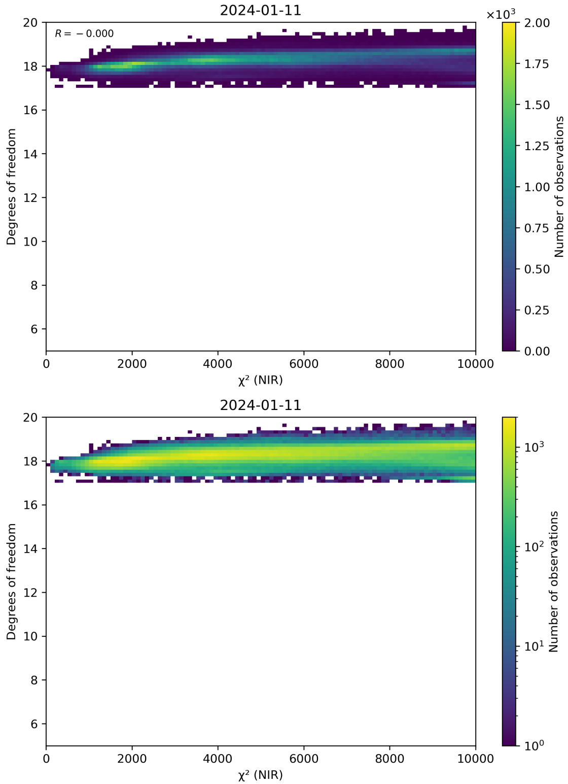
Figure 44: Scatter density plot of “ \chi^2 (NIR)” against “Degrees of freedom” for 2024-01-10 to 2024-01-12.
