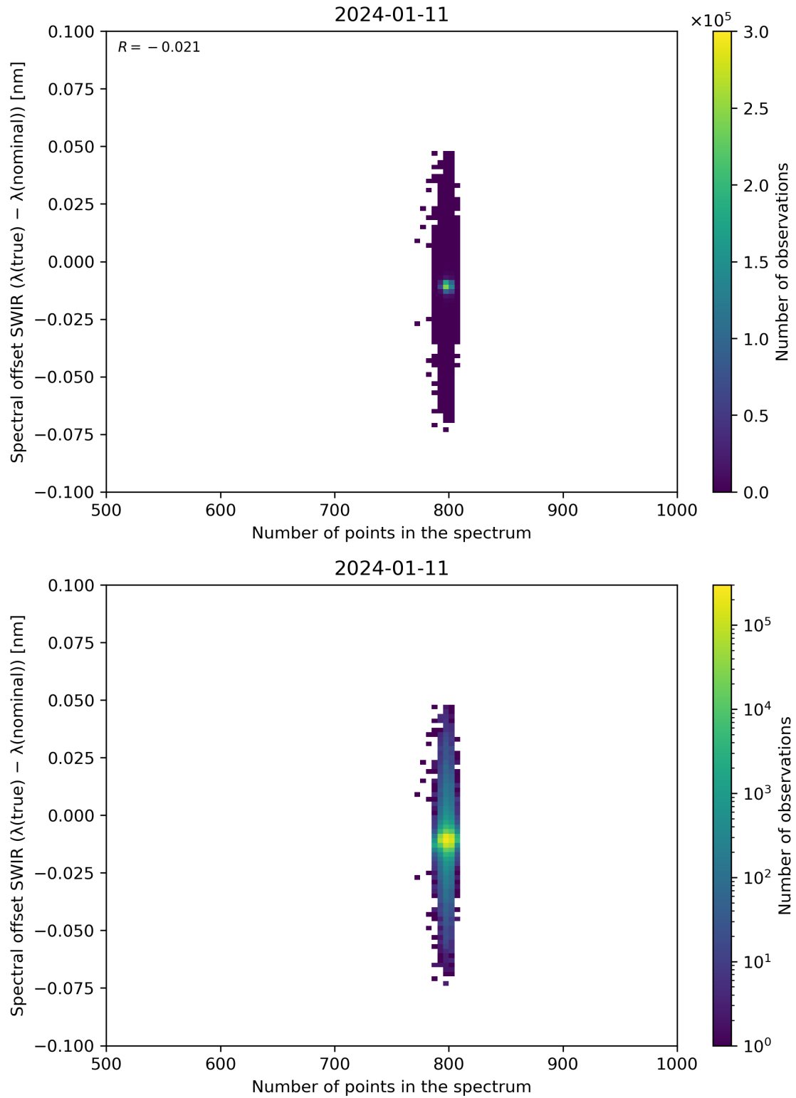
Figure 93: Scatter density plot of “Number of points in the spectrum” against “Spectral offset SWIR ( \lambda(\text{true}) - \lambda(\text{nominal}) )” for 2024-01-10 to 2024-01-12.
