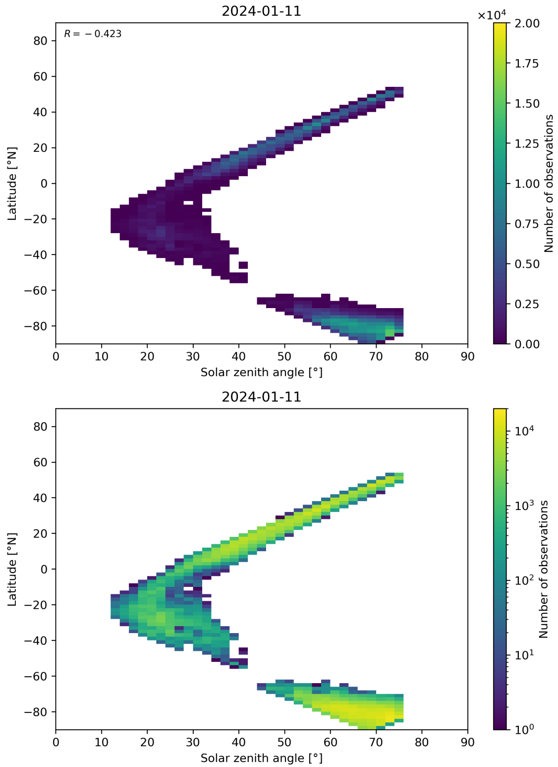
Figure 98: Scatter density plot of “Solar zenith angle” against “Latitude” for 2024-01-10 to 2024-01-12.
