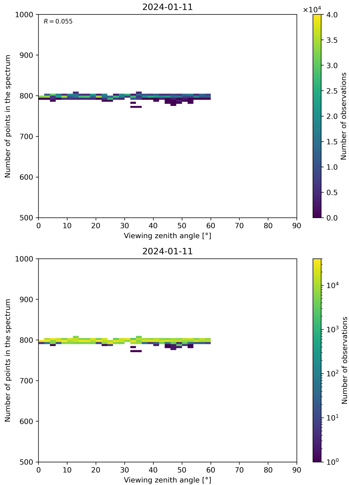
Figure 114: Scatter density plot of “Viewing zenith angle” against “Number of points in the spectrum” for 2024-01-10 to 2024-01-12.
