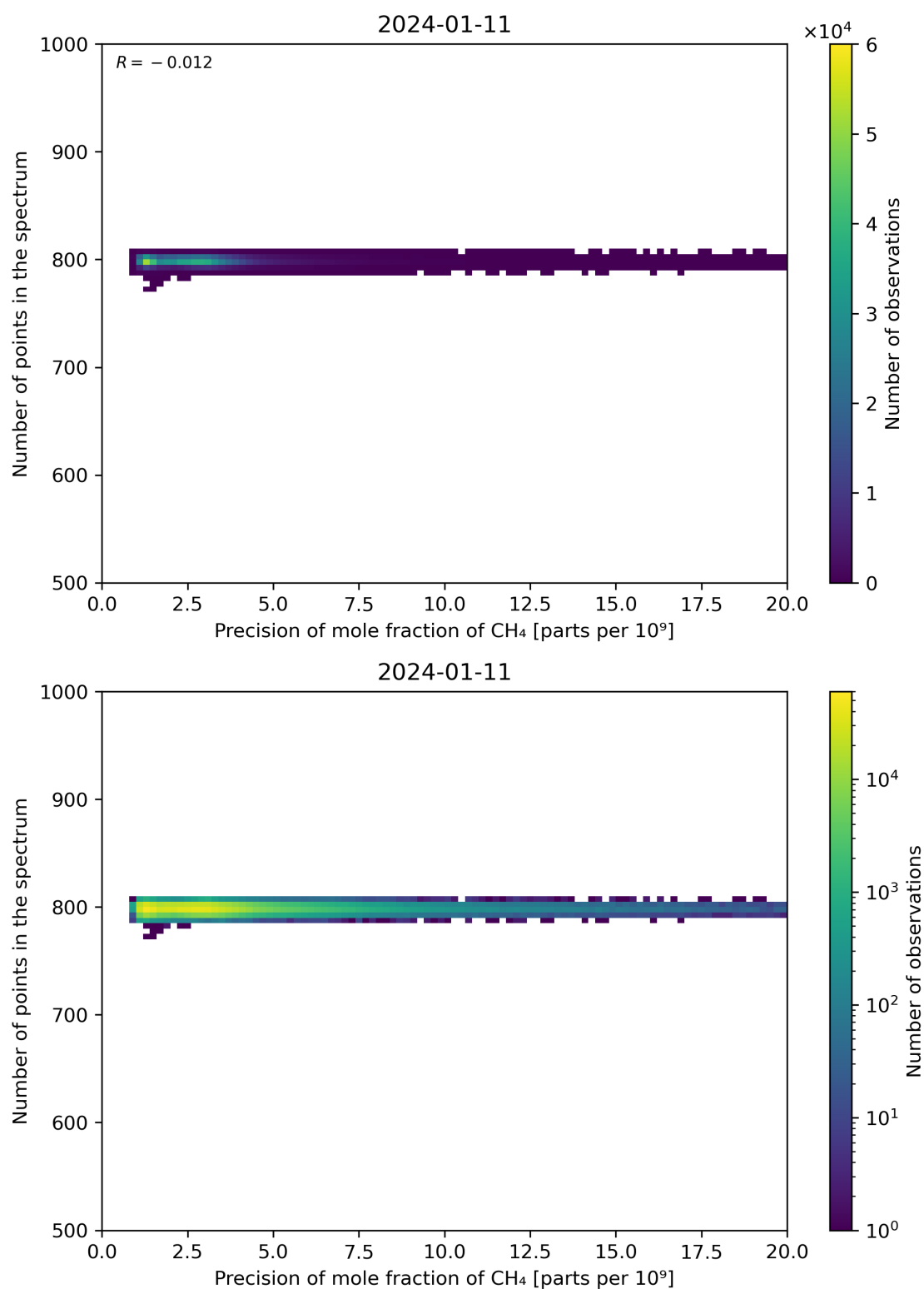
Figure 84: Scatter density plot of “Precision of mole fraction of CH 4 ” against “Number of points in the spectrum” for 2024-01-10 to 2024-01-12.
