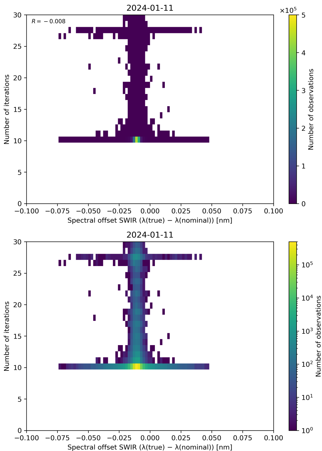
Figure 121: Scatter density plot of “Spectral offset SWIR ( \lambda(\text{true}) - \lambda(\text{nominal}) )” against “Number of iterations” for 2024-01-10 to 2024-01-12.
