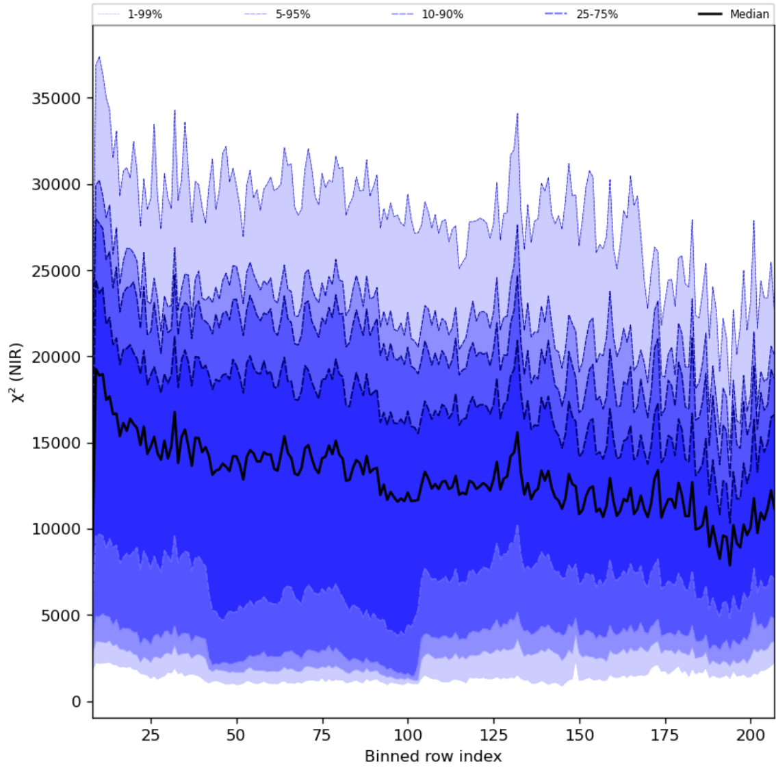
Figure 40: Along track statistics of “ \chi^2 (NIR)” for 2024-01-10 to 2024-01-12
