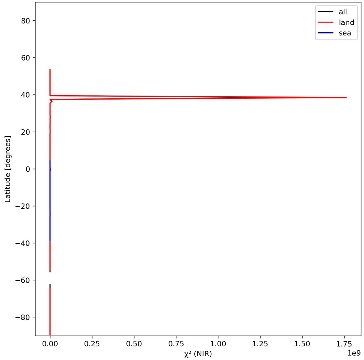
Figure 18: Zonal average of “ \chi^2 (NIR)” for 2024-01-10 to 2024-01-12.
