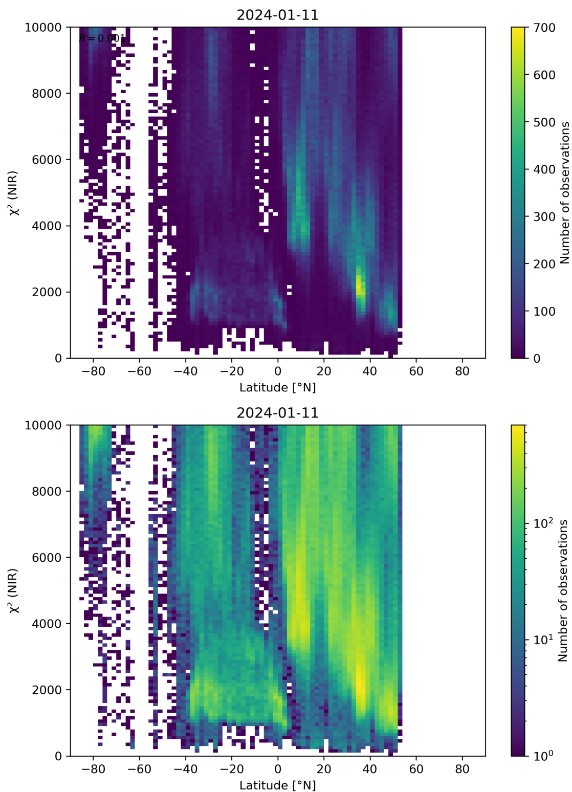
Figure 53: Scatter density plot of “Latitude” against “ \chi^2 (NIR)” for 2024-01-10 to 2024-01-12.
