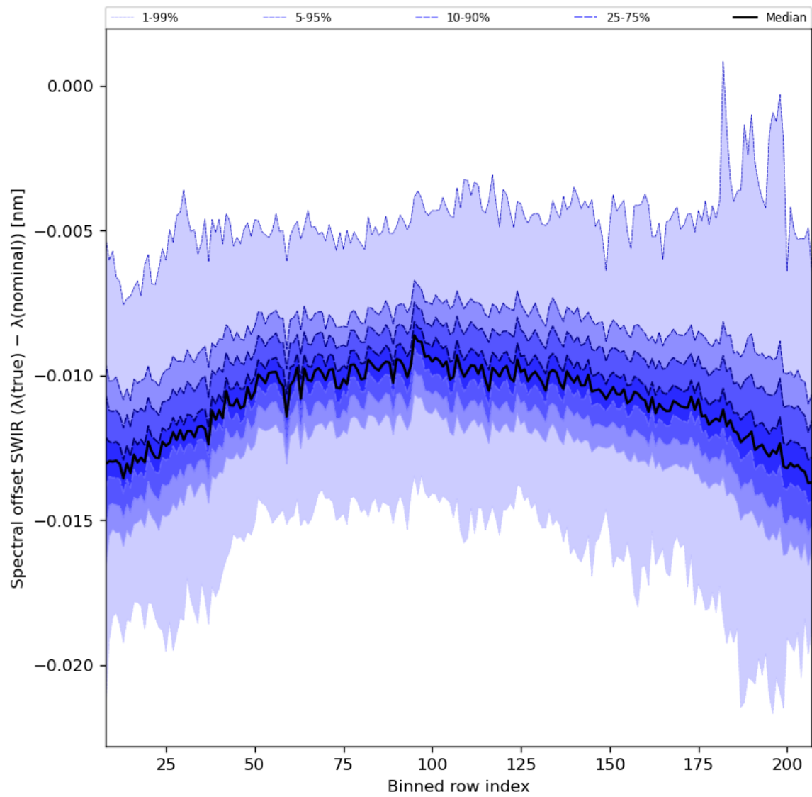
Figure 38: Along track statistics of “Spectral offset SWIR ( \lambda(\text{true}) - \lambda(\text{nominal}) )” for 2024-01-10 to 2024-01-12
