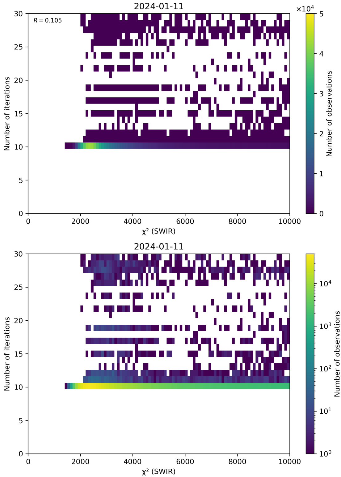
Figure 50: Scatter density plot of “ \chi^2 (SWIR)” against “Number of iterations” for 2024-01-10 to 2024-01-12.
