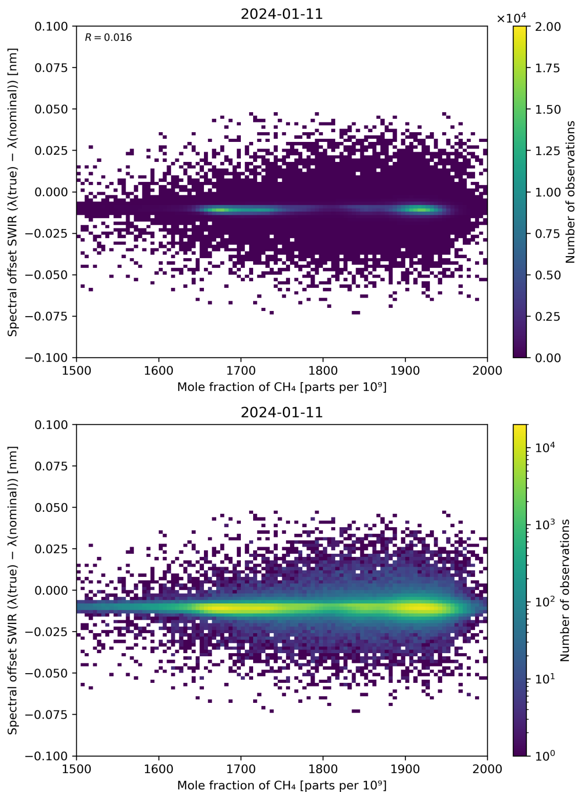
Figure 86: Scatter density plot of “Mole fraction of CH 4 ” against “Spectral offset SWIR ( \lambda(\text{true}) - \lambda(\text{nominal}) )” for 2024-01-10 to 2024-01-12.
