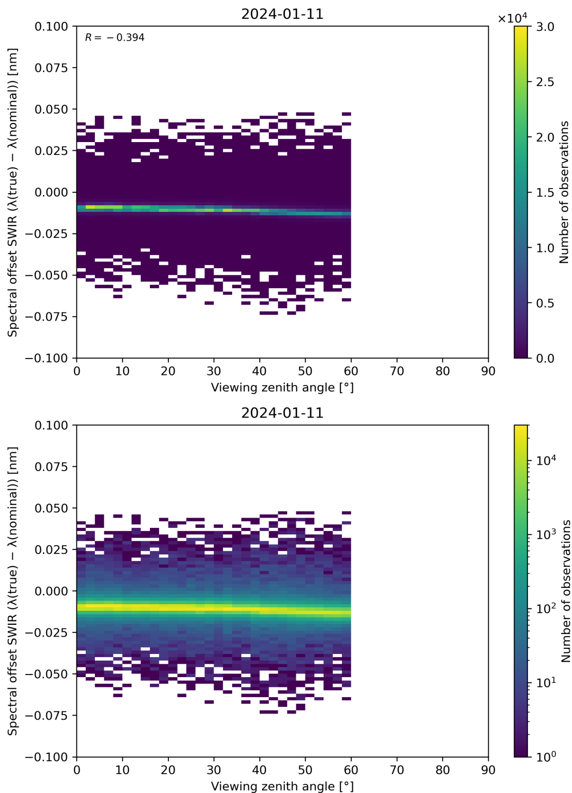
Figure 116: Scatter density plot of “Viewing zenith angle” against “Spectral offset SWIR ( \lambda(\text{true}) - \lambda(\text{nominal}) )” for 2024-01-10 to 2024-01-12.
