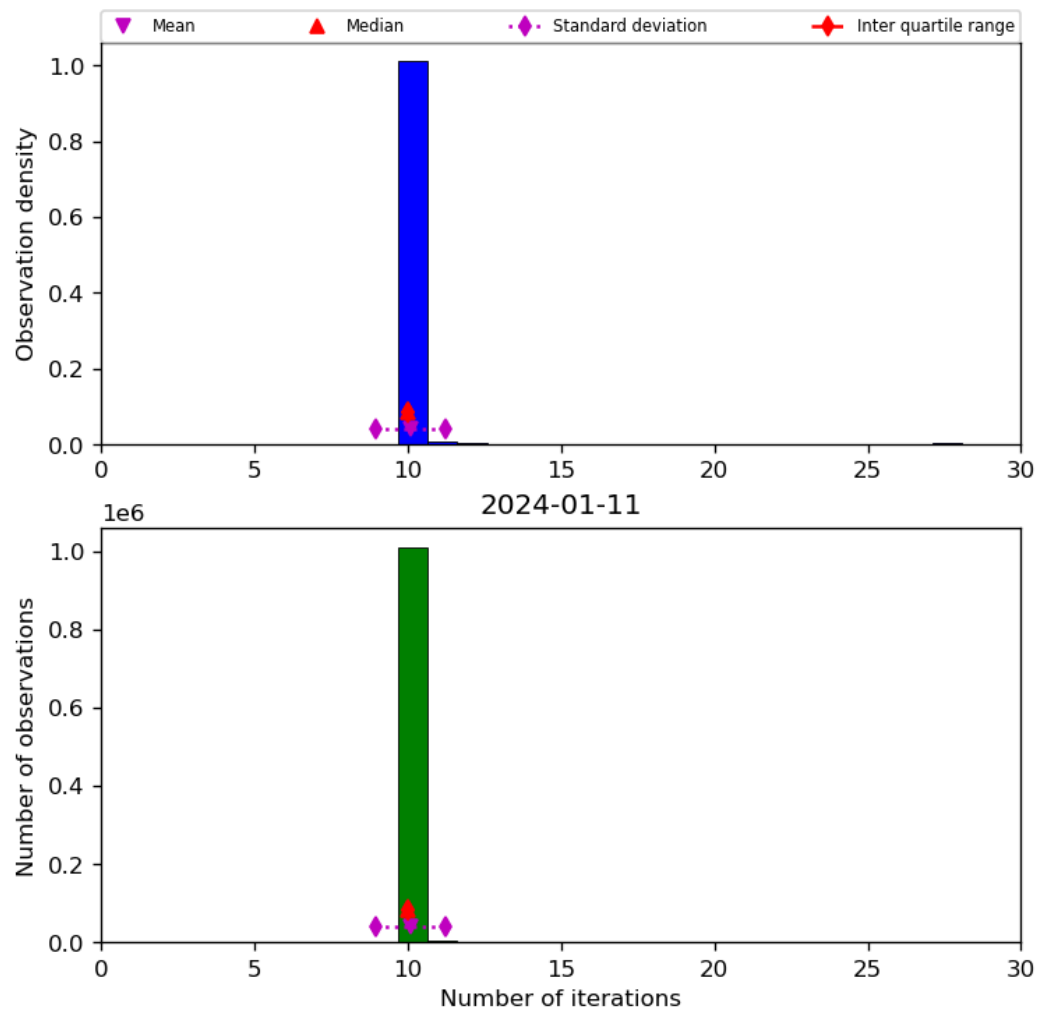
Figure 31: Histogram of “Number of iterations” for 2024-01-10 to 2024-01-12
