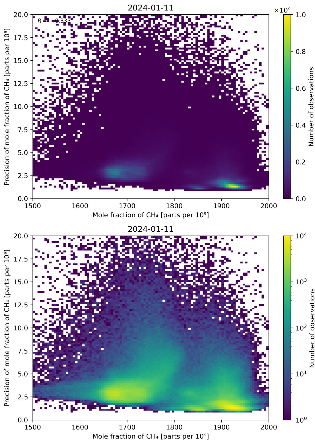
Figure 75: Scatter density plot of “Mole fraction of CH 4 ” against “Precision of mole fraction of CH 4 ” for 2024-01-10 to 2024-01-12.
