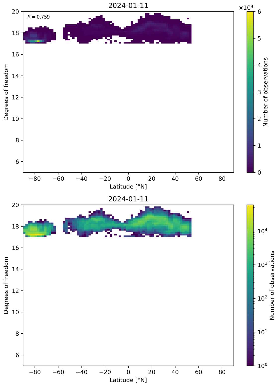
Figure 55: Scatter density plot of “Latitude” against “Degrees of freedom” for 2024-01-10 to 2024-01-12.
