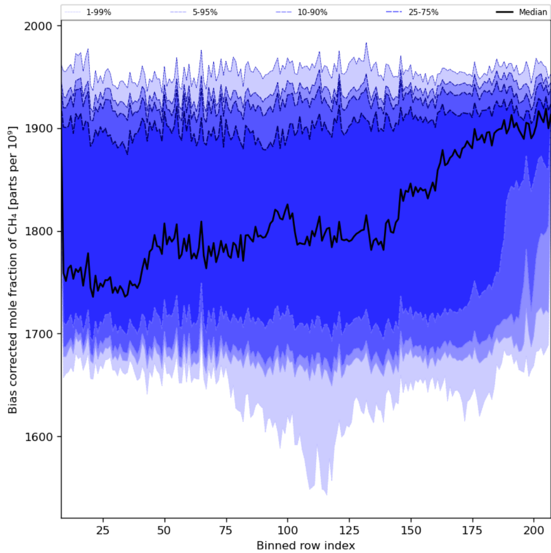
Figure 36: Along track statistics of “Bias corrected mole fraction of CH 4 ” for 2024-01-10 to 2024-01-12
