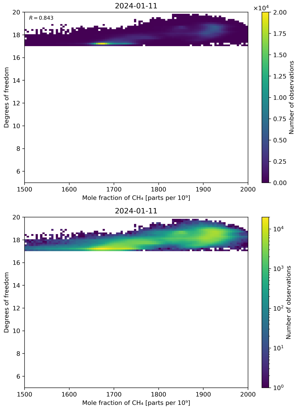
Figure 72: Scatter density plot of “Mole fraction of CH 4 ” against “Degrees of freedom” for 2024-01-10 to 2024-01-12.
