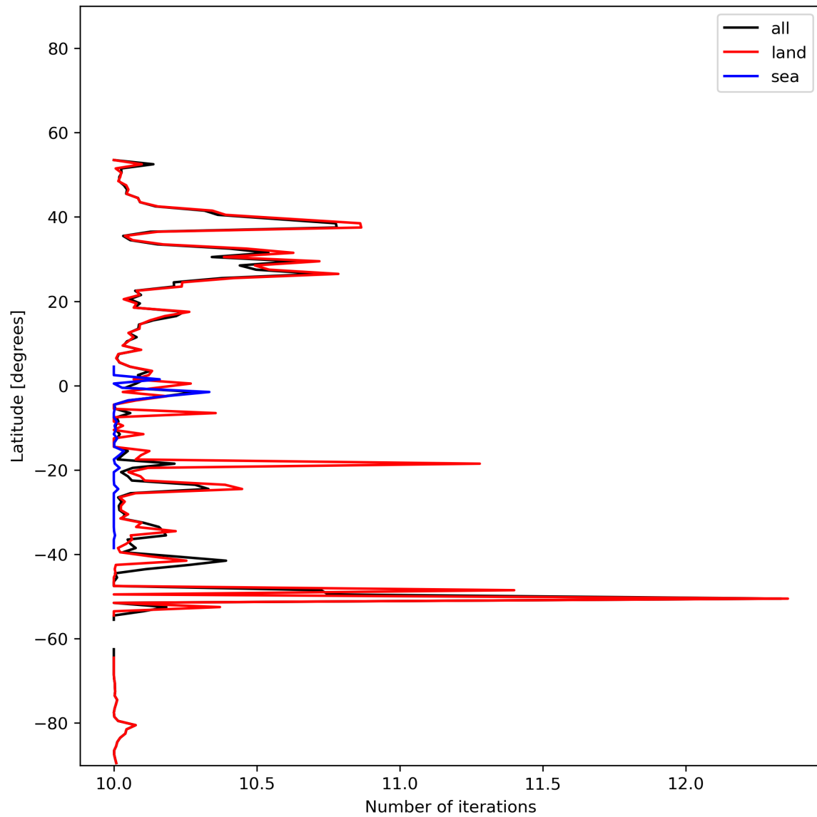
Figure 20: Zonal average of “Number of iterations” for 2024-01-10 to 2024-01-12.
