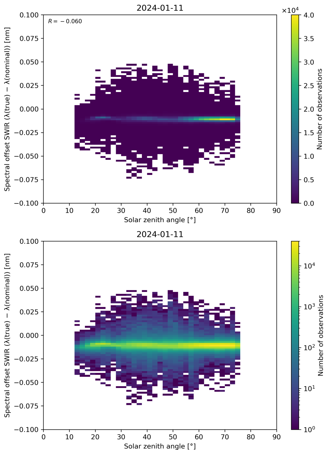
Figure 104: Scatter density plot of “Solar zenith angle” against “Spectral offset SWIR ( \lambda(\text{true}) - \lambda(\text{nominal}) )” for 2024-01-10 to 2024-01-12.
