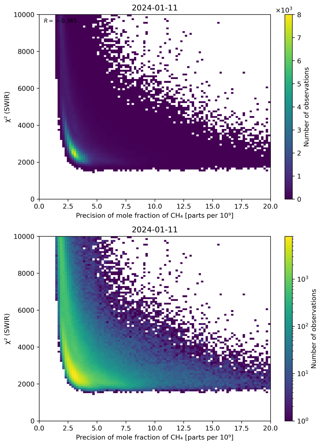
Figure 79: Scatter density plot of “Precision of mole fraction of \text{CH}_4 ” against “ \chi^2 (SWIR)” for 2024-01-10 to 2024-01-12.
