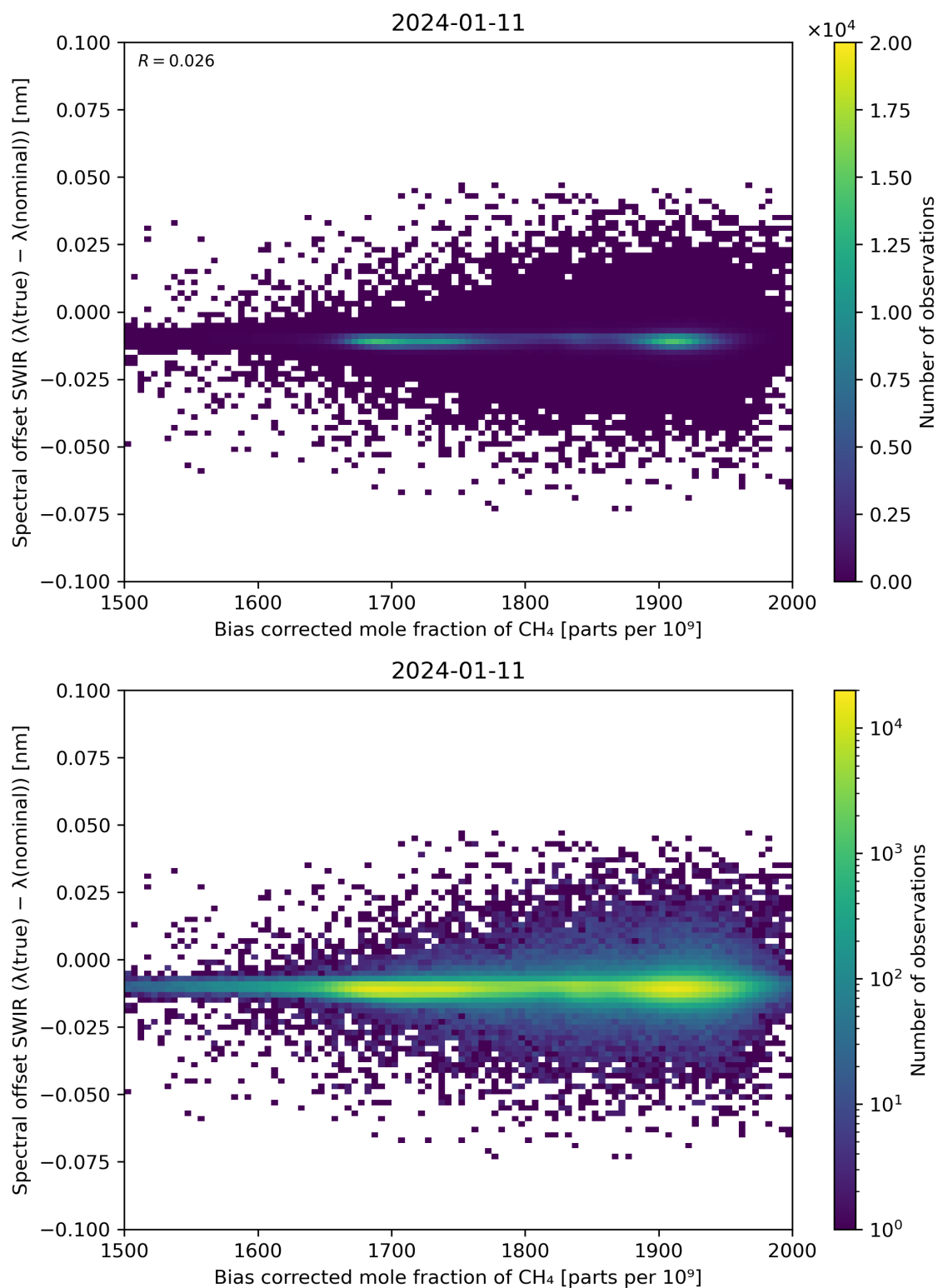
Figure 69: Scatter density plot of “Bias corrected mole fraction of \text{CH}_4 ” against “Spectral offset SWIR ( \lambda(\text{true}) - \lambda(\text{nominal}) )” for 2024-01-10 to 2024-01-12.
