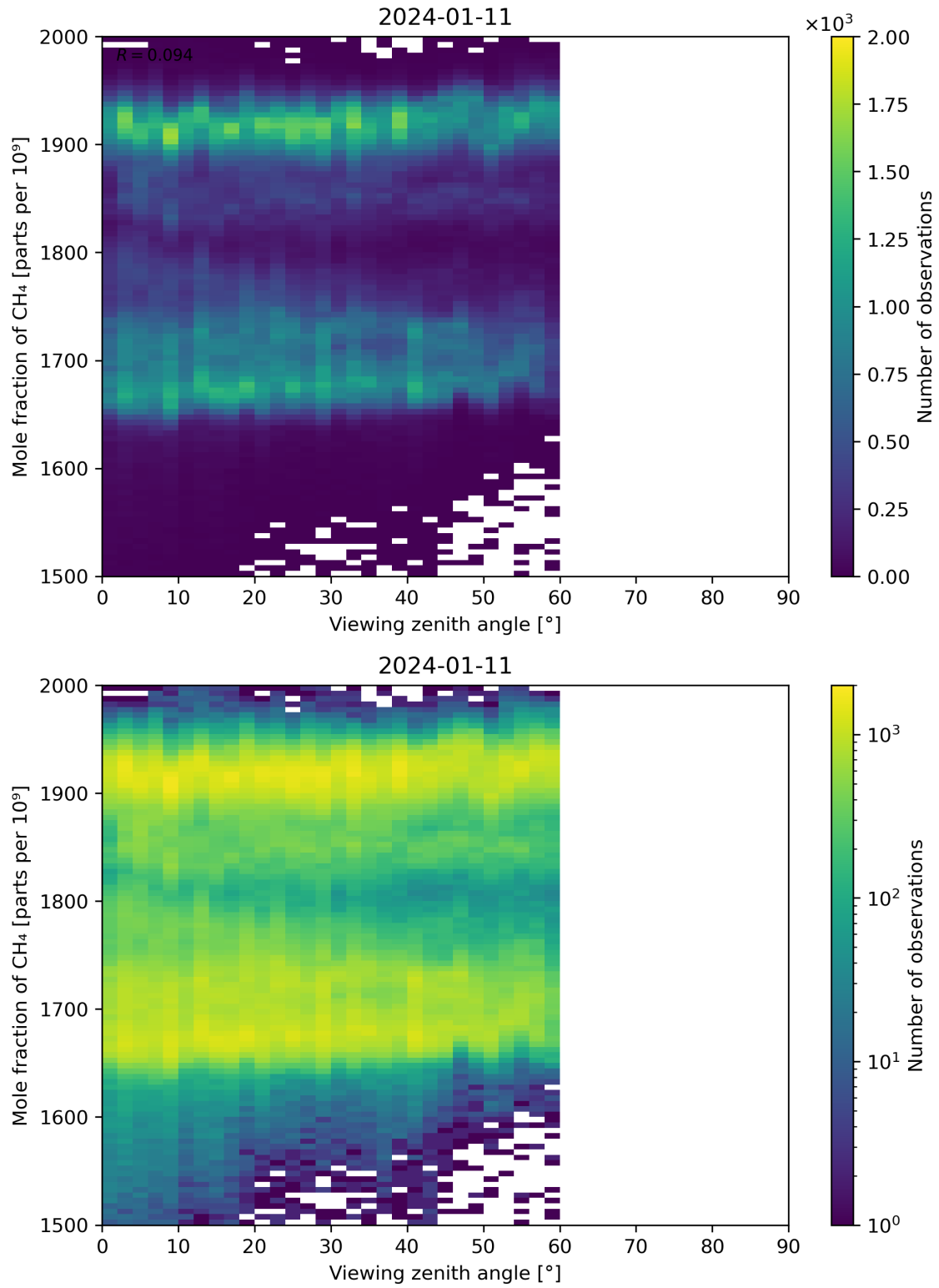
Figure 110: Scatter density plot of “Viewing zenith angle” against “Mole fraction of \text{CH}_4 ” for 2024-01-10 to 2024-01-12.
