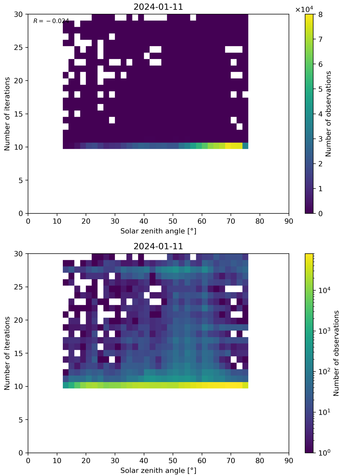
Figure 102: Scatter density plot of “Solar zenith angle” against “Number of iterations” for 2024-01-10 to 2024-01-12.
