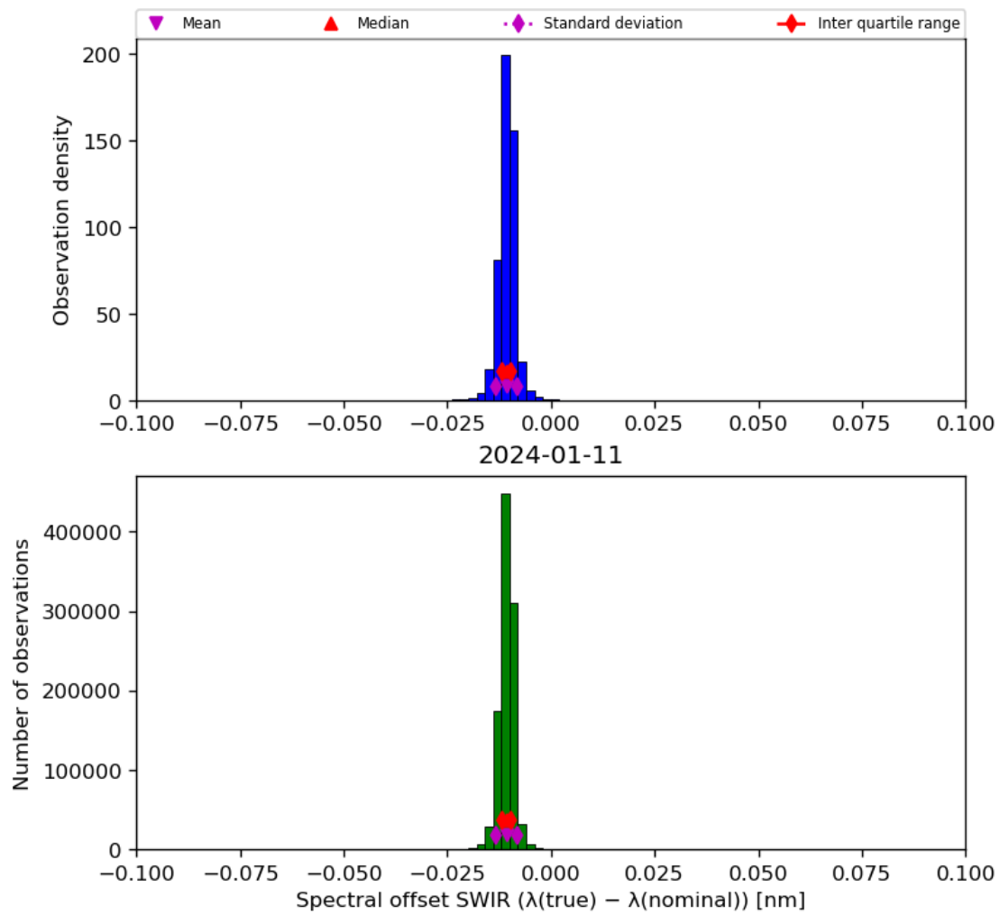
Figure 27: Histogram of “Spectral offset SWIR ( \lambda(\text{true}) - \lambda(\text{nominal}) )” for 2024-01-10 to 2024-01-12
