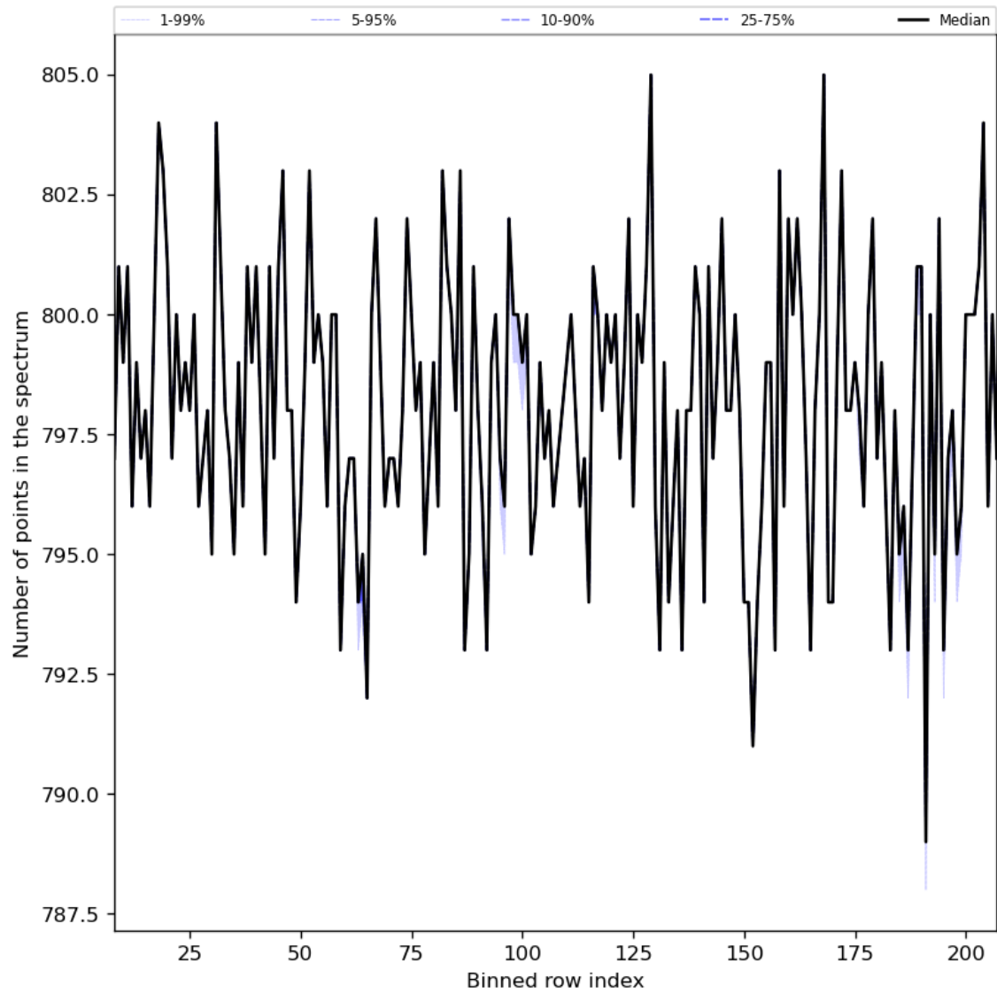
Figure 37: Along track statistics of “Number of points in the spectrum” for 2024-01-10 to 2024-01-12
