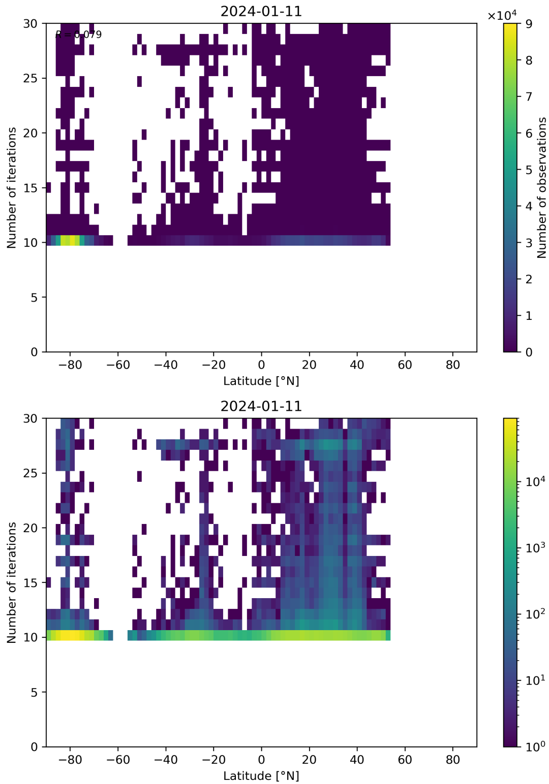
Figure 60: Scatter density plot of “Latitude” against “Number of iterations” for 2024-01-10 to 2024-01-12.
