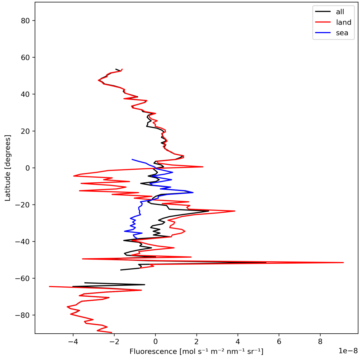
Figure 21: Zonal average of “Fluorescence” for 2024-01-10 to 2024-01-12.
