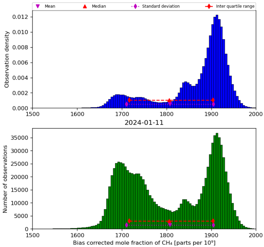
Figure 25: Histogram of “Bias corrected mole fraction of CH 4 ” for 2024-01-10 to 2024-01-12
