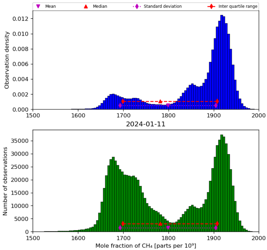
Figure 23: Histogram of “Mole fraction of CH 4 ” for 2024-01-10 to 2024-01-12
