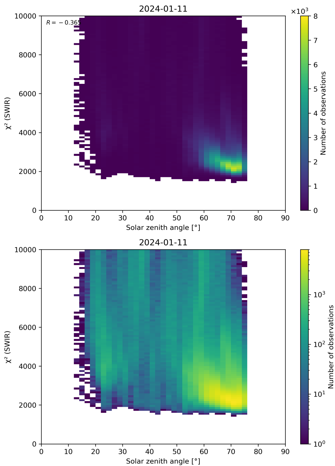
Figure 95: Scatter density plot of “Solar zenith angle” against “ \chi^2 (SWIR)” for 2024-01-10 to 2024-01-12.
