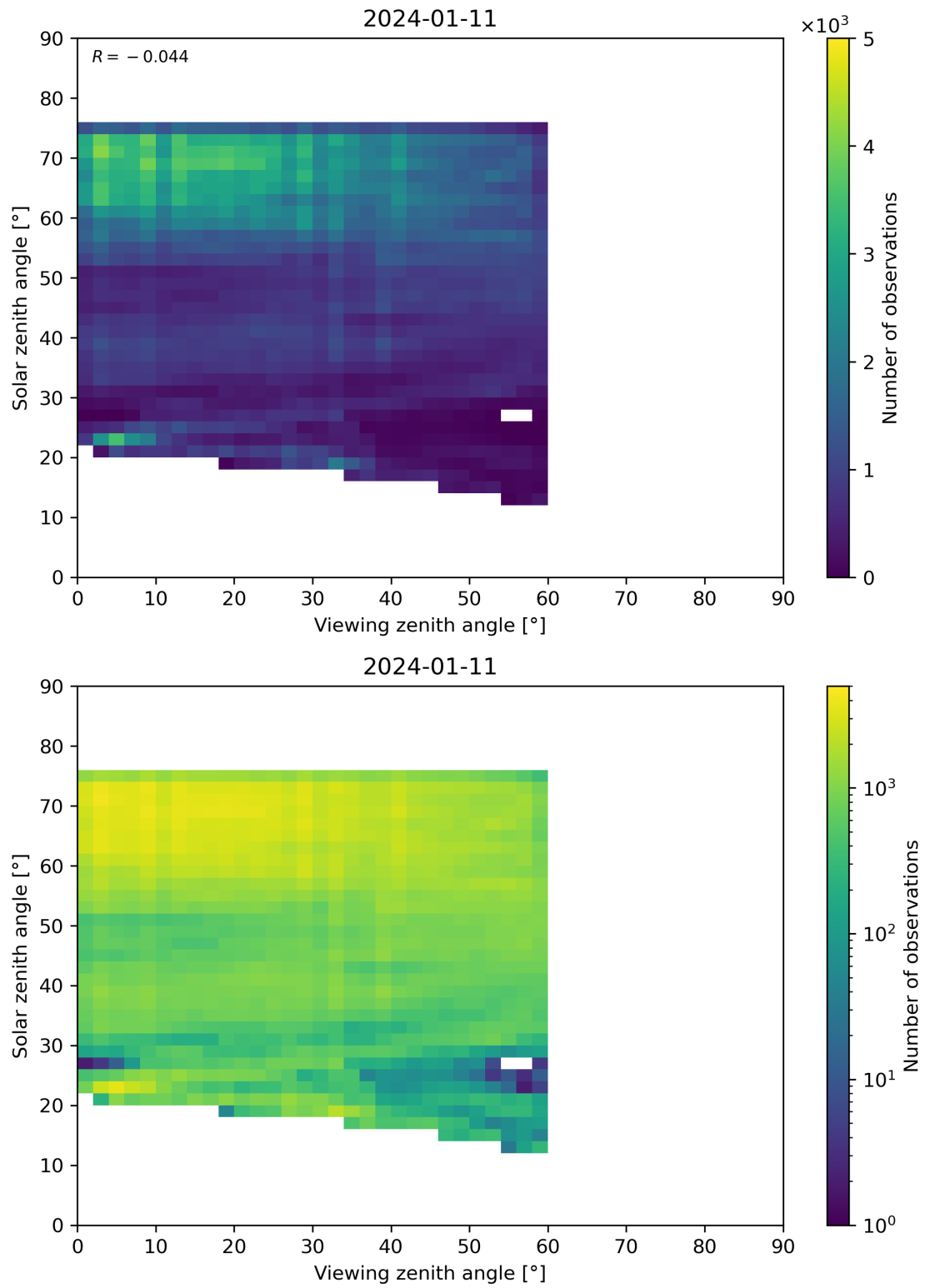
Figure 115: Scatter density plot of “Viewing zenith angle” against “Solar zenith angle” for 2024-01-10 to 2024-01-12.
