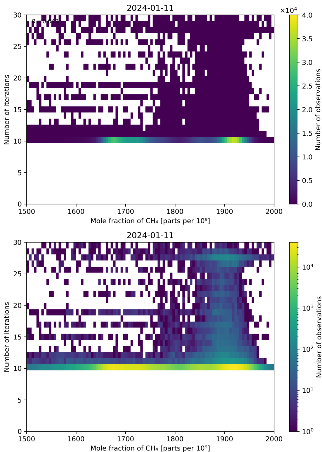
Figure 76: Scatter density plot of “Mole fraction of CH 4 ” against “Number of iterations” for 2024-01-10 to 2024-01-12.
