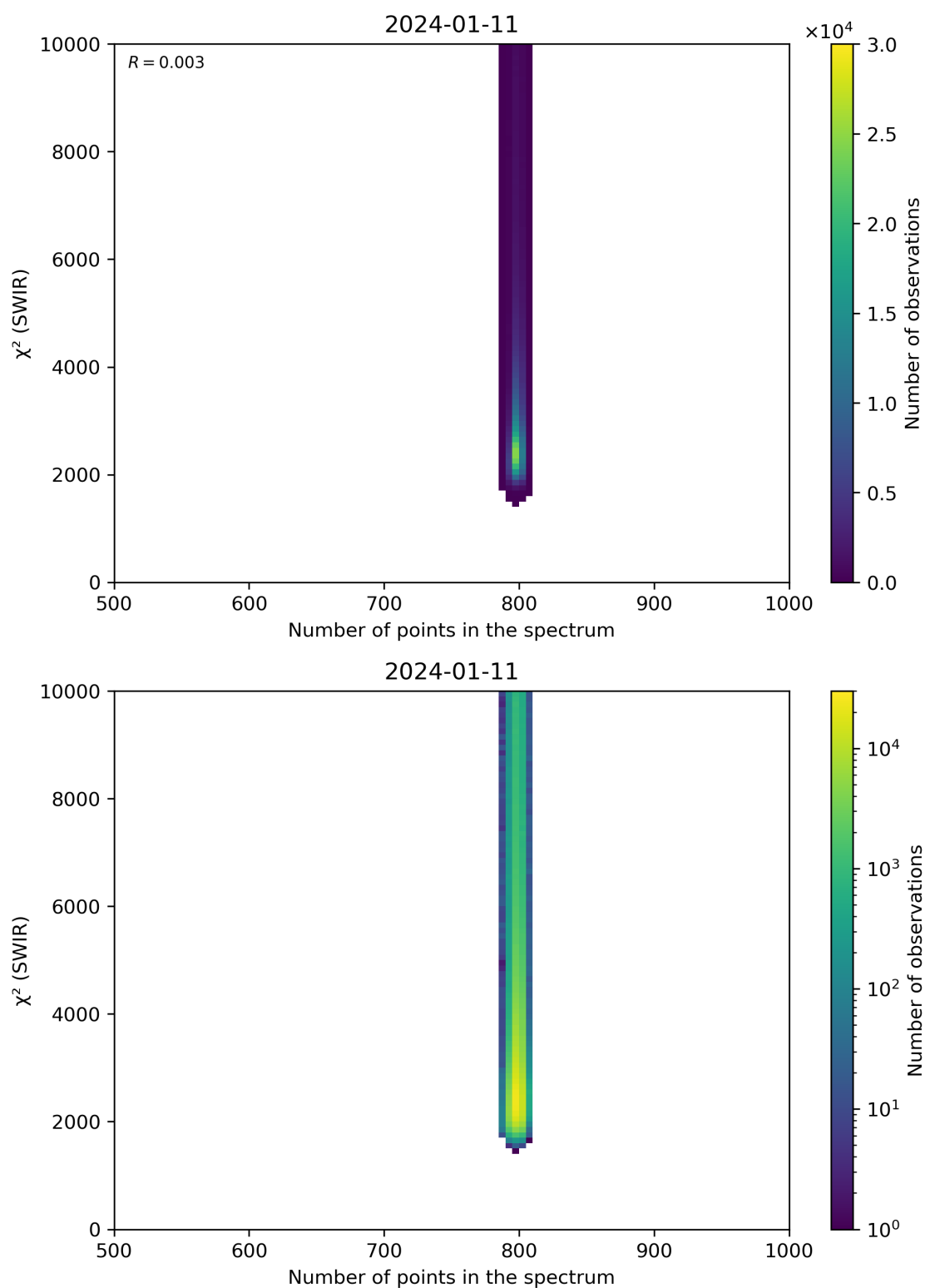
Figure 89: Scatter density plot of “Number of points in the spectrum” against “ \chi^2 (SWIR)” for 2024-01-10 to 2024-01-12.
