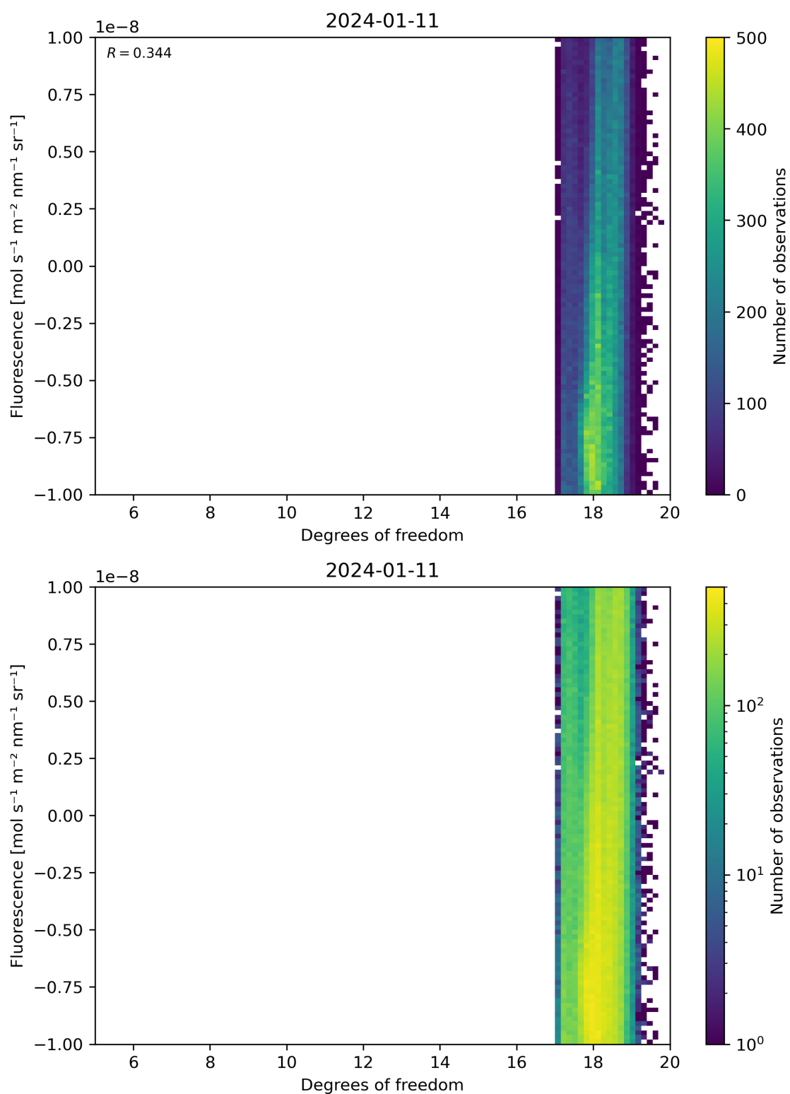
Figure 51: Scatter density plot of “Degrees of freedom” against “Fluorescence” for 2024-01-10 to 2024-01-12.
