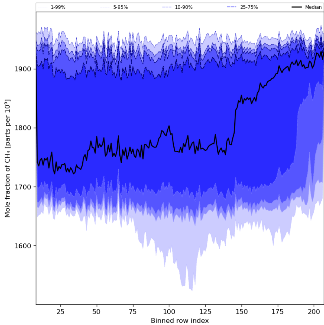
Figure 34: Along track statistics of “Mole fraction of CH 4 ” for 2024-01-10 to 2024-01-12
