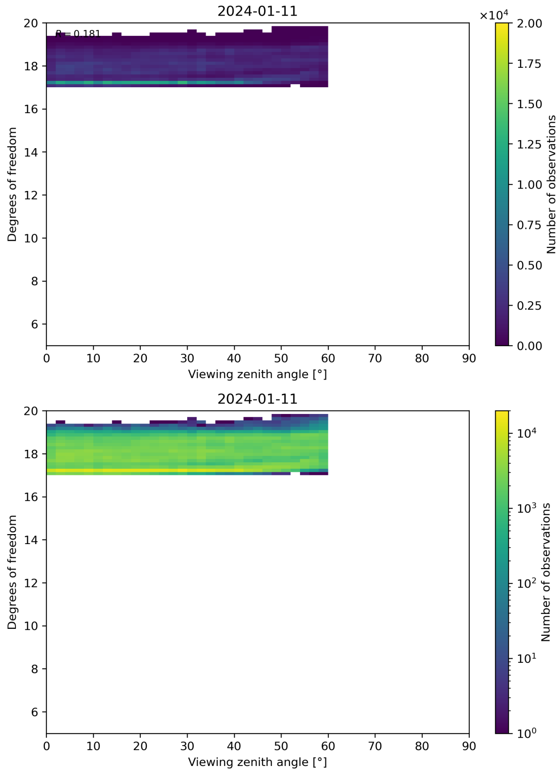
Figure 107: Scatter density plot of “Viewing zenith angle” against “Degrees of freedom” for 2024-01-10 to 2024-01-12.
