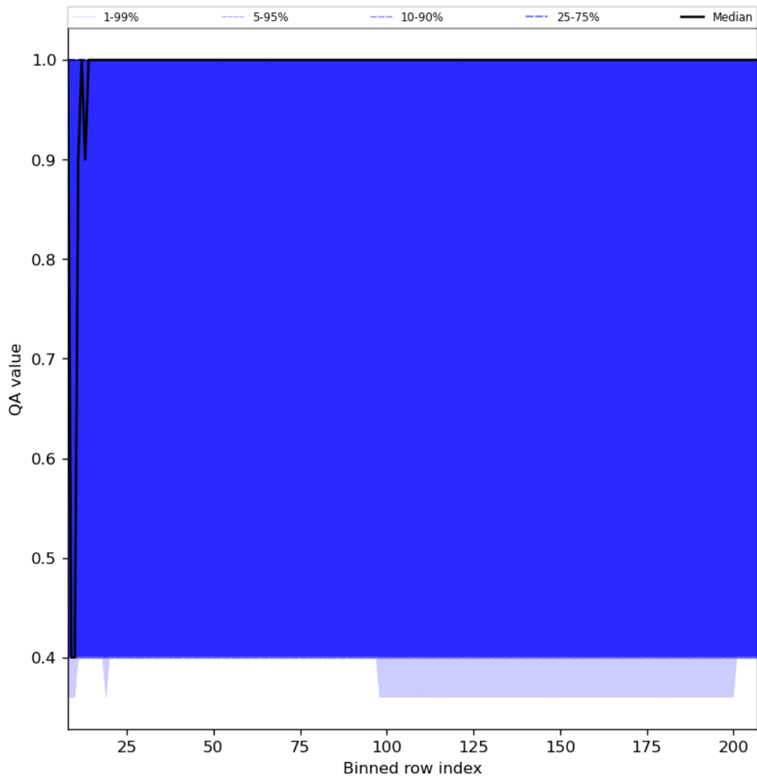
Figure 33: Along track statistics of “QA value” for 2024-01-10 to 2024-01-12
