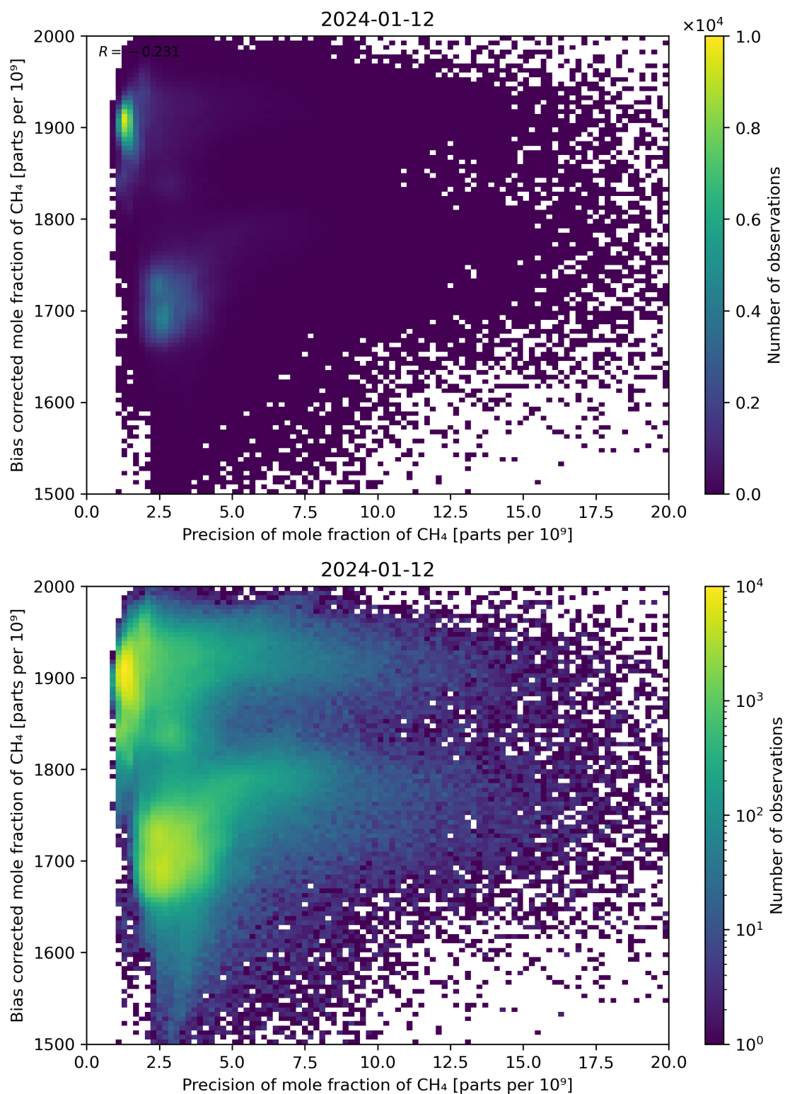
Figure 82: Scatter density plot of “Precision of mole fraction of CH 4 ” against “Bias corrected mole fraction of CH 4 ” for 2024-01-11 to 2024-01-13.
