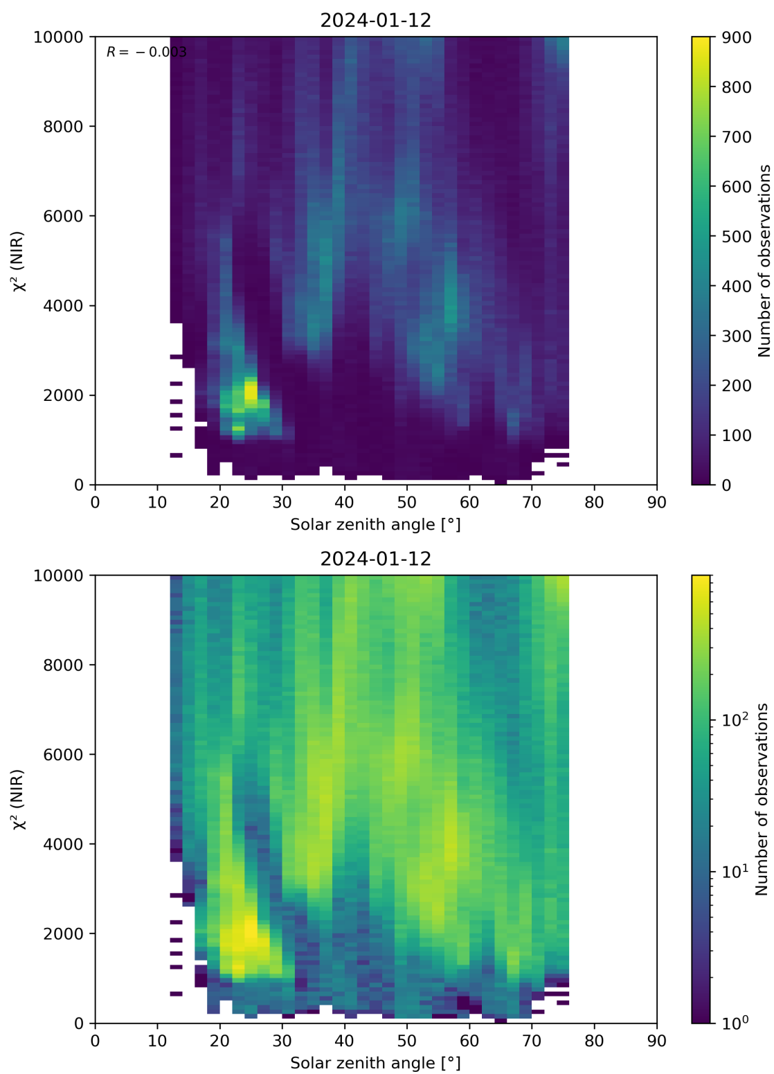
Figure 94: Scatter density plot of “Solar zenith angle” against “ \chi^2 (NIR)” for 2024-01-11 to 2024-01-13.
