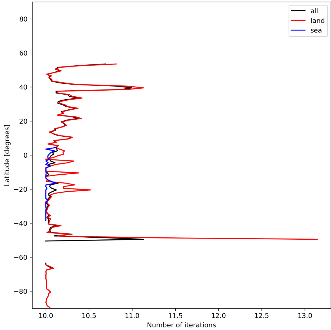
Figure 20: Zonal average of “Number of iterations” for 2024-01-11 to 2024-01-13.
