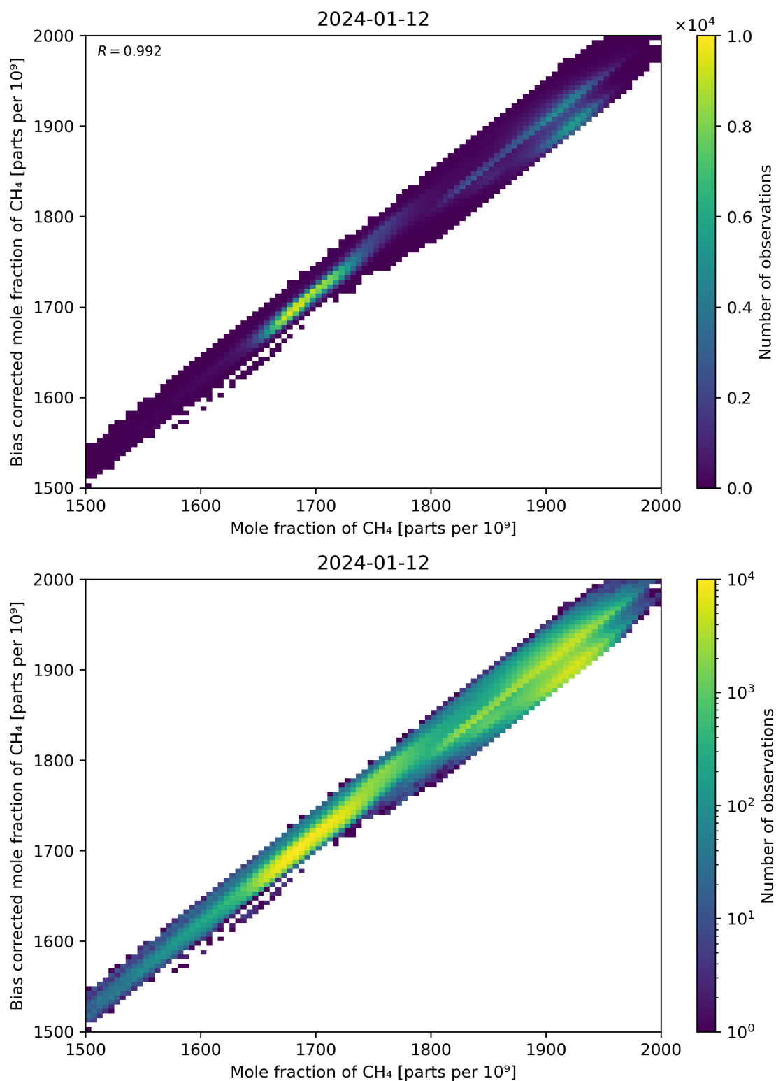
Figure 74: Scatter density plot of “Mole fraction of CH 4 ” against “Bias corrected mole fraction of CH 4 ” for 2024-01-11 to 2024-01-13.
