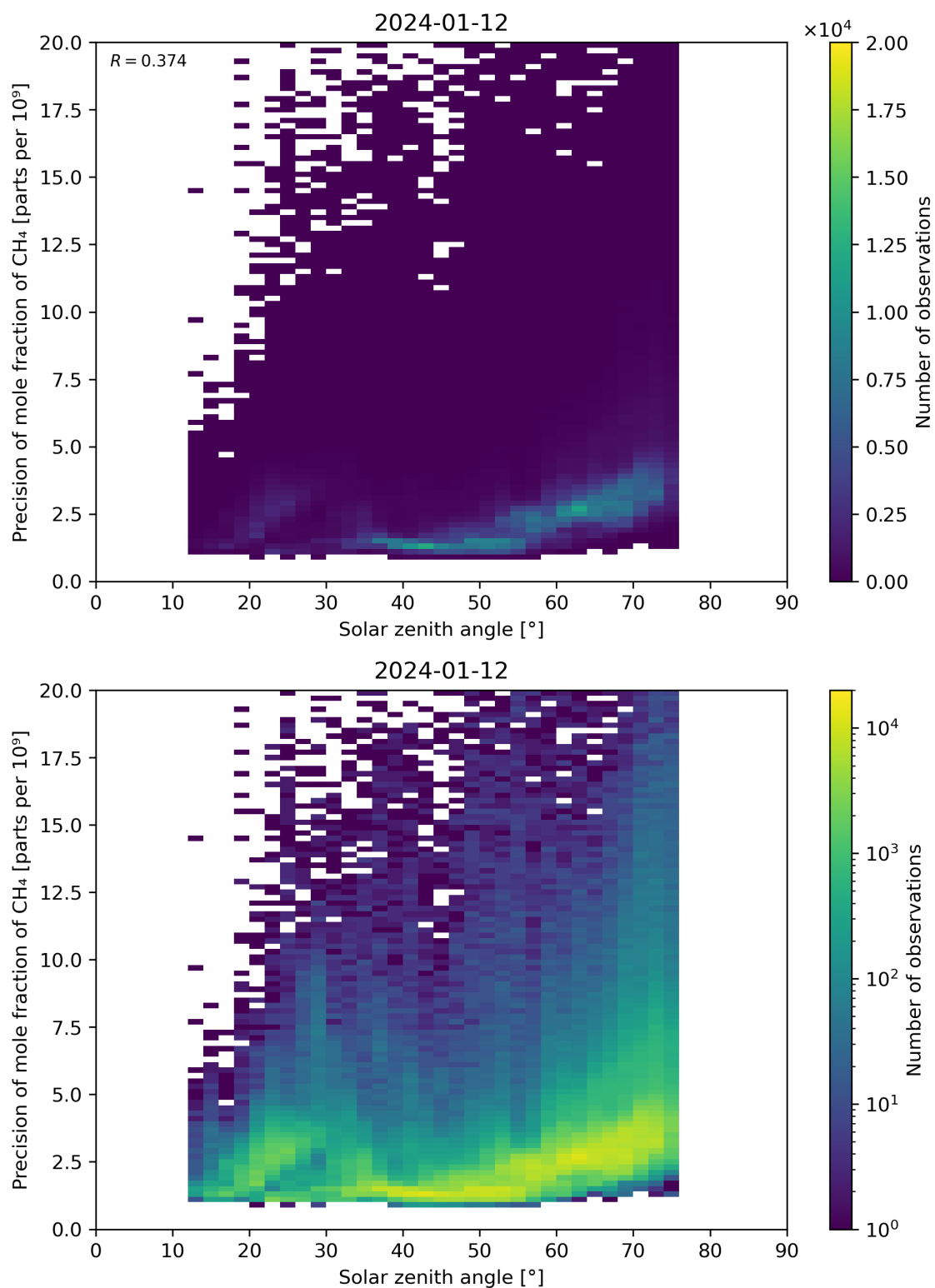
Figure 101: Scatter density plot of “Solar zenith angle” against “Precision of mole fraction of CH 4 ” for 2024-01-11 to 2024-01-13.
