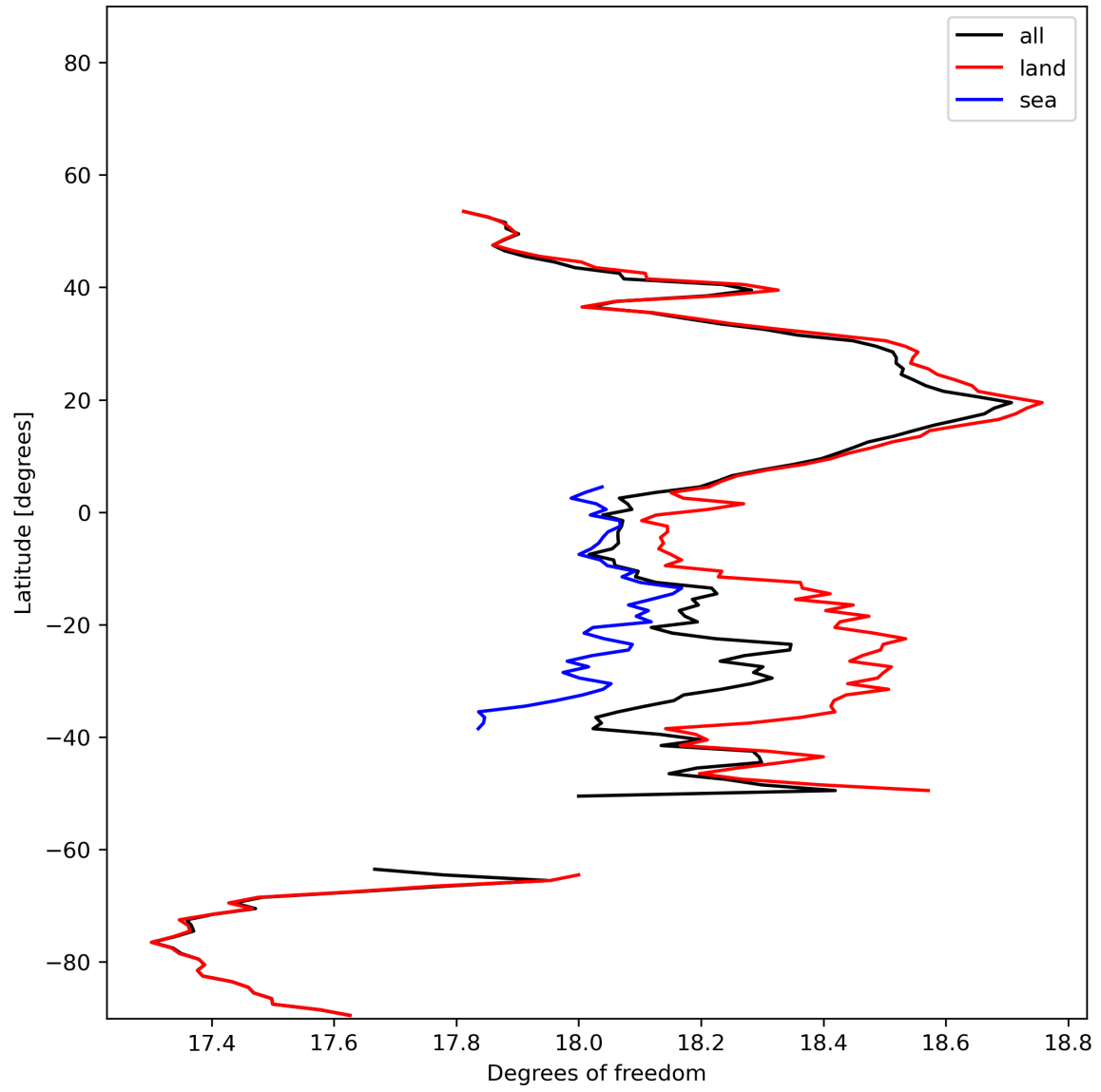
Figure 19: Zonal average of “Degrees of freedom” for 2024-01-11 to 2024-01-13.
