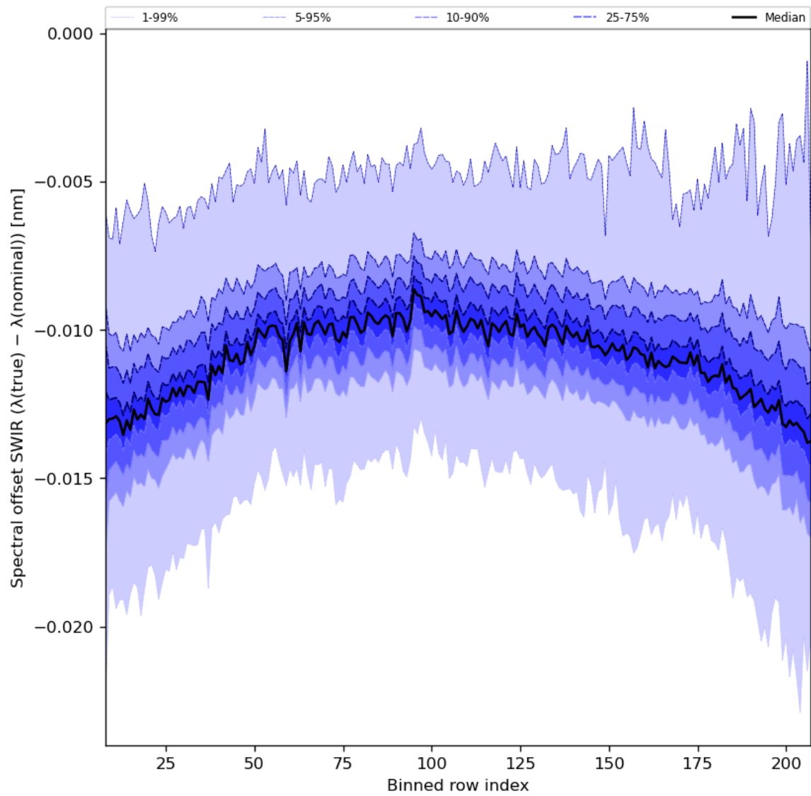
Figure 38: Along track statistics of “Spectral offset SWIR ( \lambda(\text{true}) - \lambda(\text{nominal}) )” for 2024-01-11 to 2024-01-13
