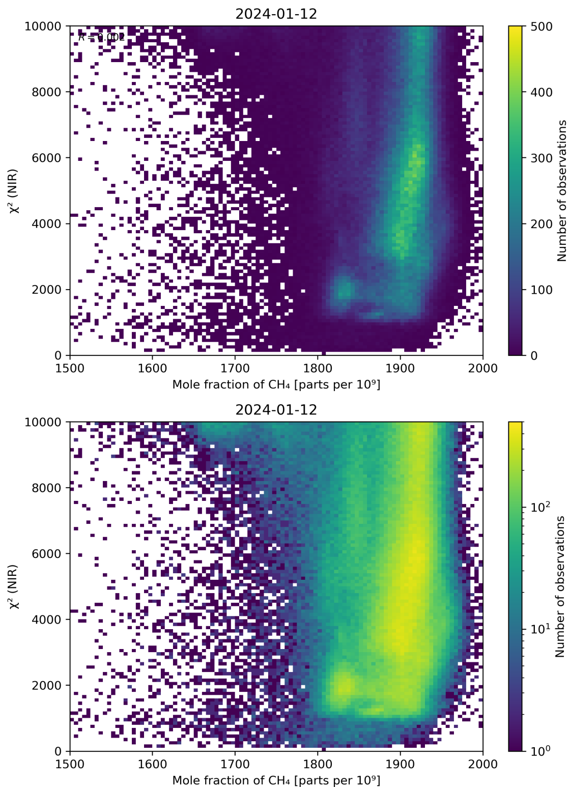
Figure 70: Scatter density plot of “Mole fraction of \text{CH}_4 ” against “ \chi^2 (NIR)” for 2024-01-11 to 2024-01-13.
