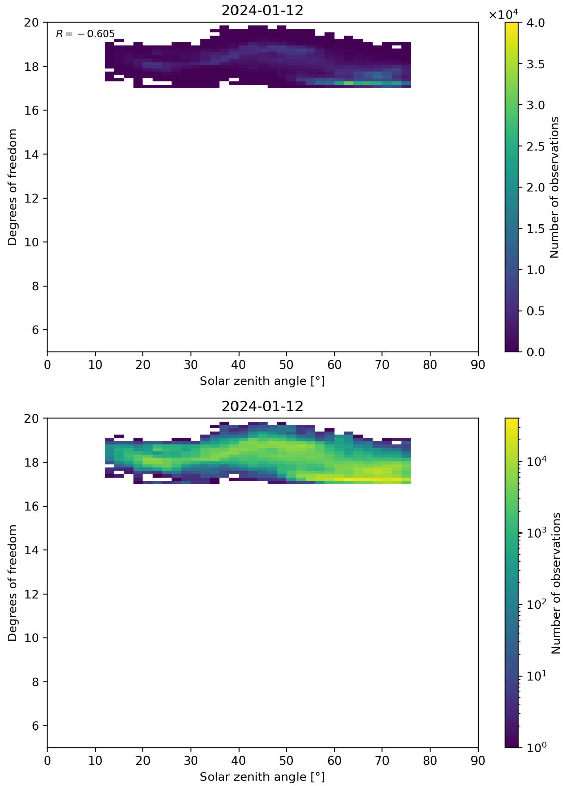
Figure 96: Scatter density plot of “Solar zenith angle” against “Degrees of freedom” for 2024-01-11 to 2024-01-13.
