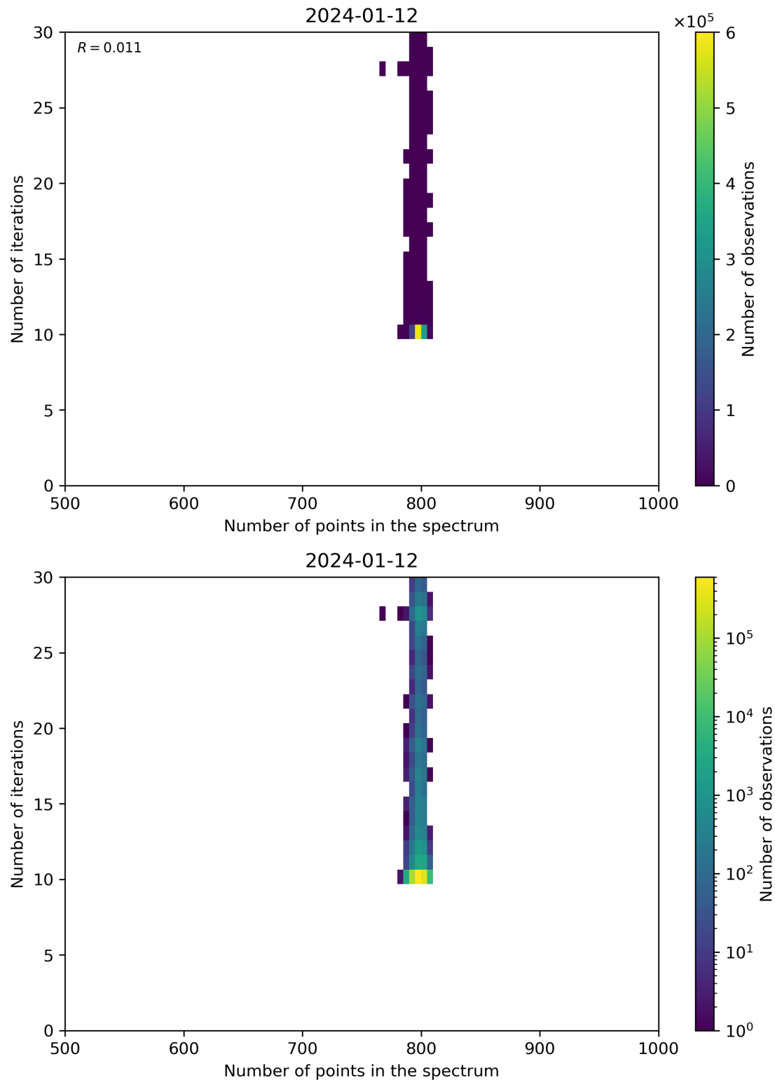
Figure 92: Scatter density plot of “Number of points in the spectrum” against “Number of iterations” for 2024-01-11 to 2024-01-13.
