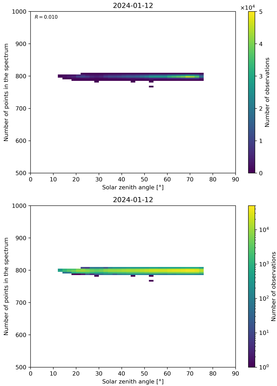
Figure 103: Scatter density plot of “Solar zenith angle” against “Number of points in the spectrum” for 2024-01-11 to 2024-01-13.
