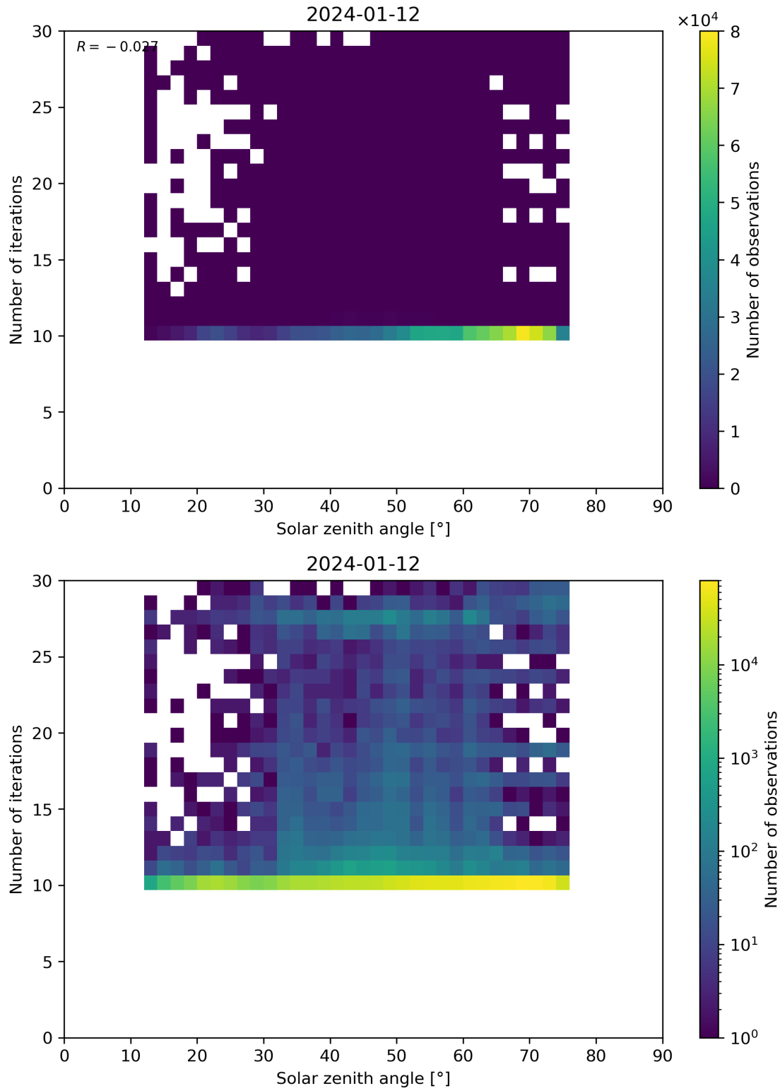
Figure 102: Scatter density plot of “Solar zenith angle” against “Number of iterations” for 2024-01-11 to 2024-01-13.
