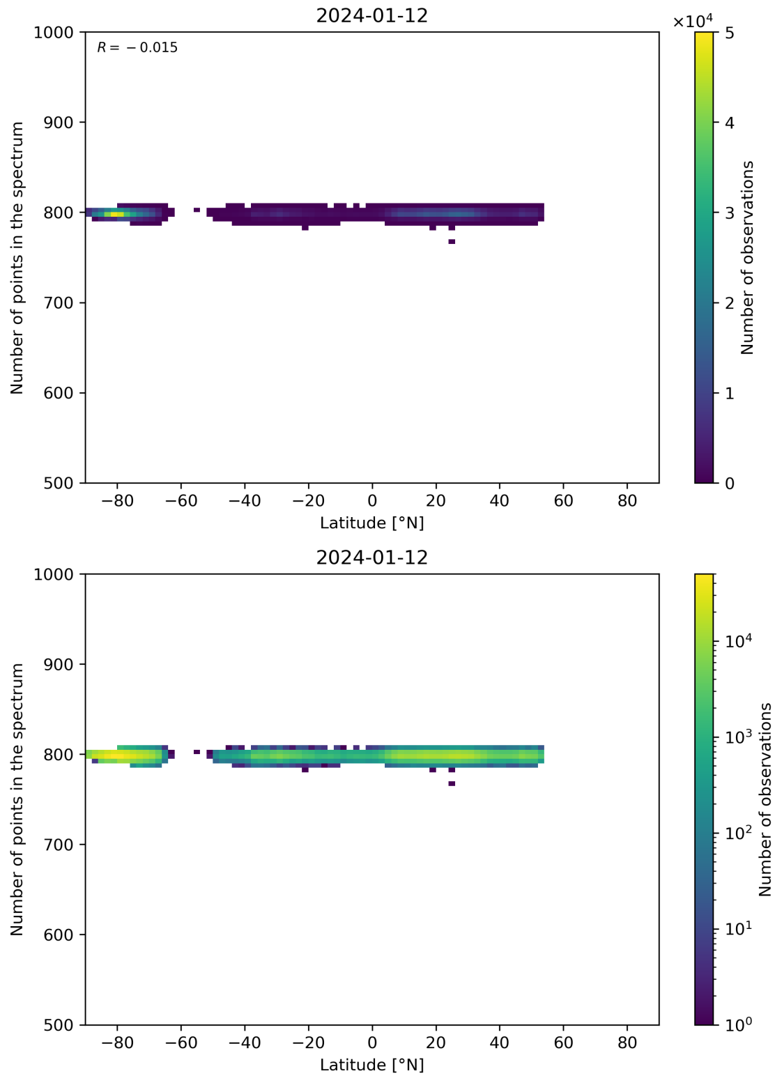
Figure 61: Scatter density plot of “Latitude” against “Number of points in the spectrum” for 2024-01-11 to 2024-01-13.
