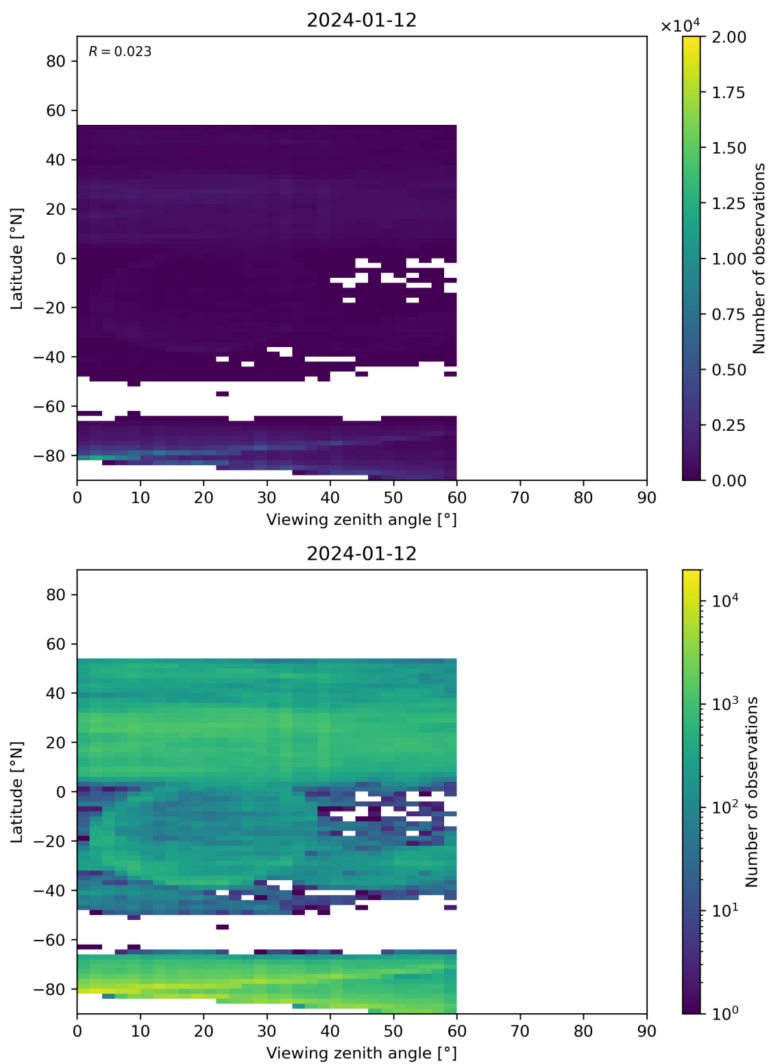
Figure 109: Scatter density plot of “Viewing zenith angle” against “Latitude” for 2024-01-11 to 2024-01-13.
