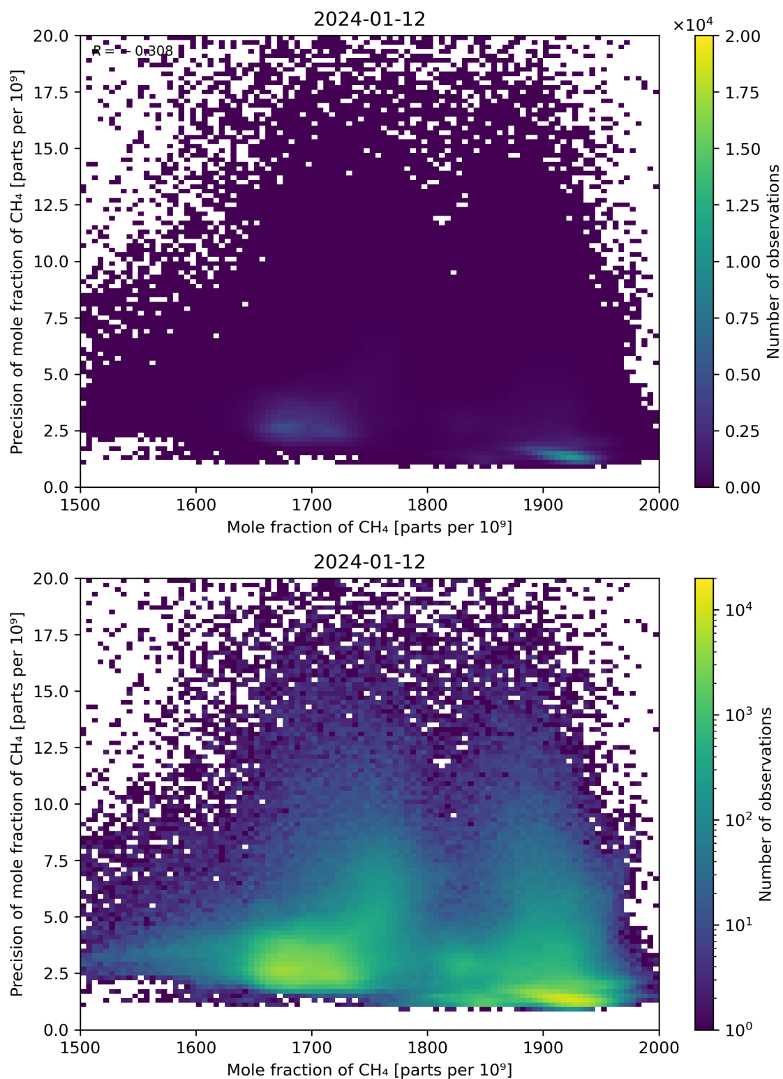
Figure 75: Scatter density plot of “Mole fraction of CH 4 ” against “Precision of mole fraction of CH 4 ” for 2024-01-11 to 2024-01-13.
