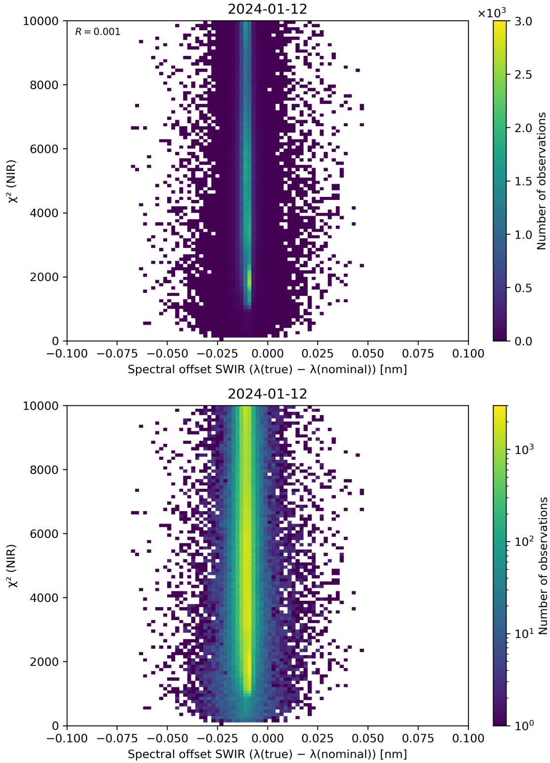
Figure 117: Scatter density plot of “Spectral offset SWIR ( \lambda(\text{true}) - \lambda(\text{nominal}) )” against “ \chi^2 (NIR)” for 2024-01-11 to 2024-01-13.
