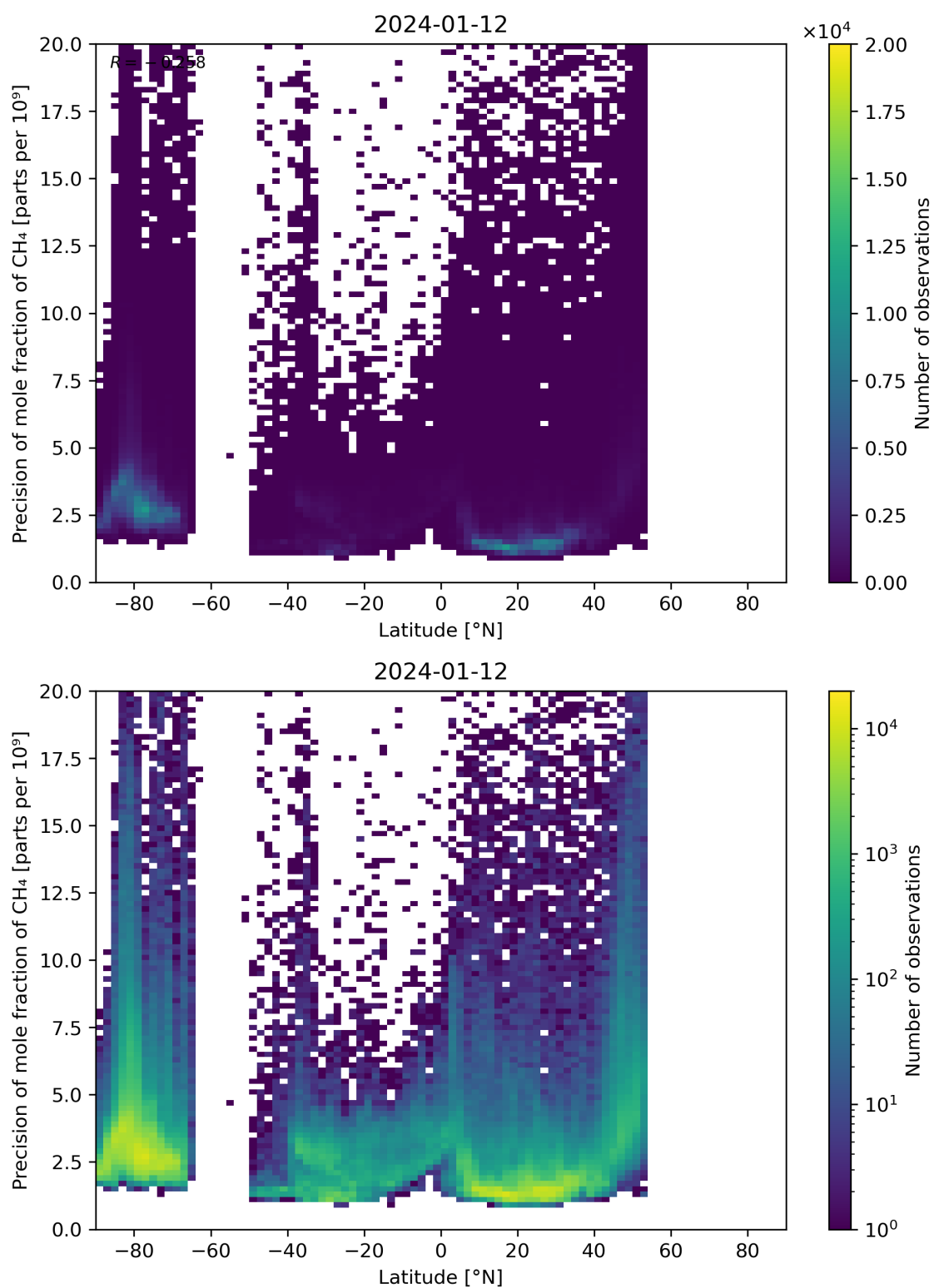
Figure 59: Scatter density plot of “Latitude” against “Precision of mole fraction of CH 4 ” for 2024-01-11 to 2024-01-13.
