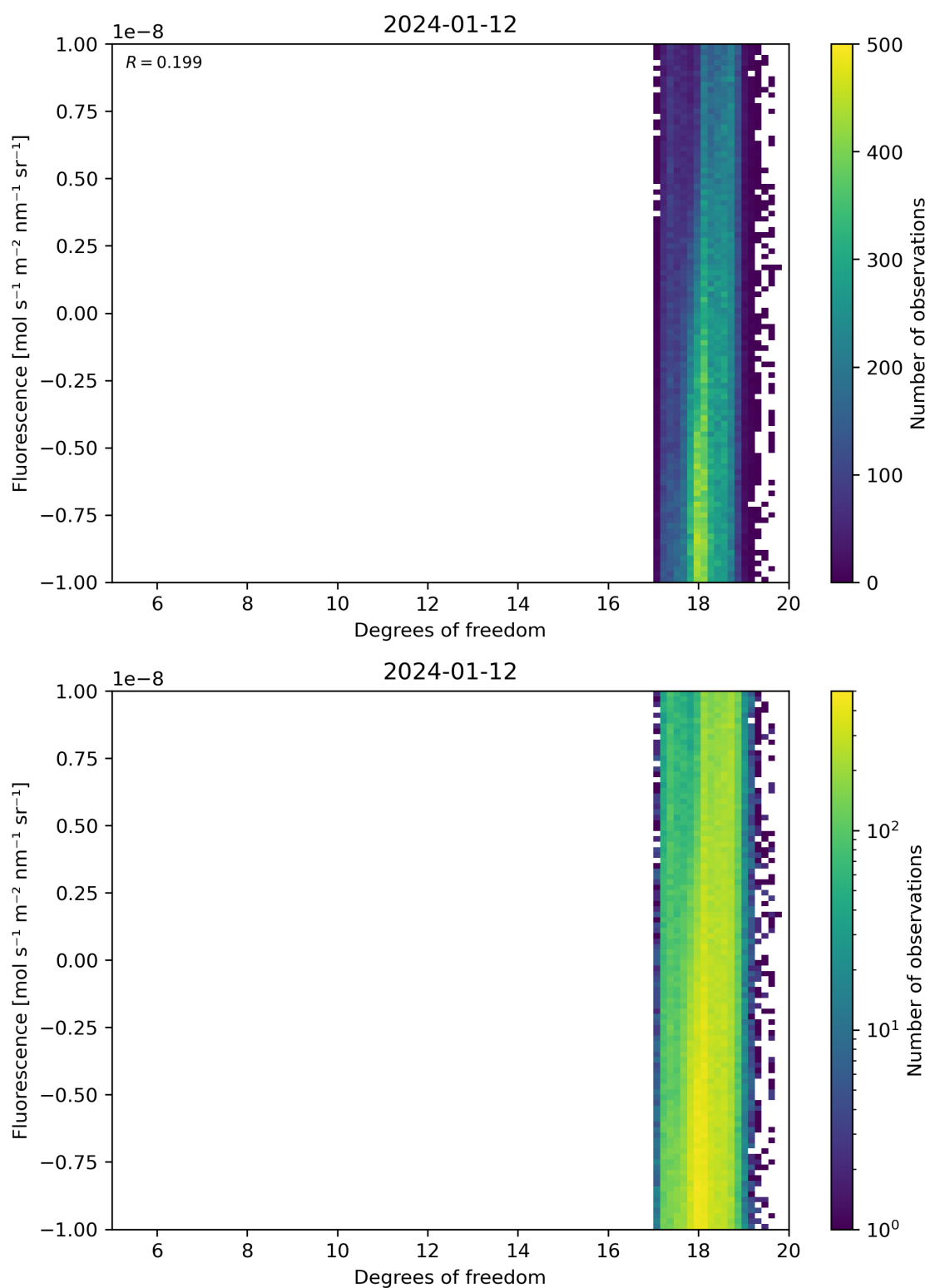
Figure 51: Scatter density plot of “Degrees of freedom” against “Fluorescence” for 2024-01-11 to 2024-01-13.
