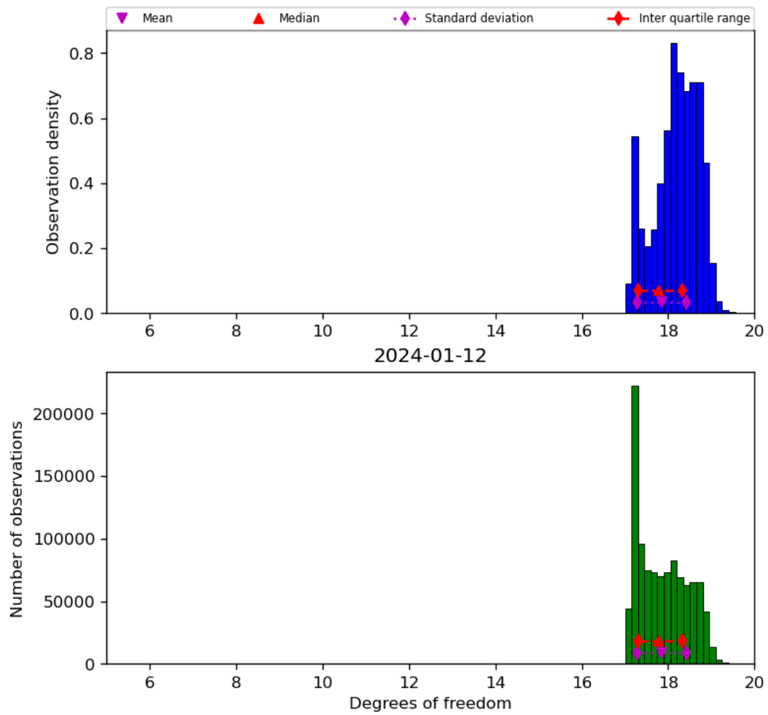
Figure 30: Histogram of “Degrees of freedom” for 2024-01-11 to 2024-01-13
