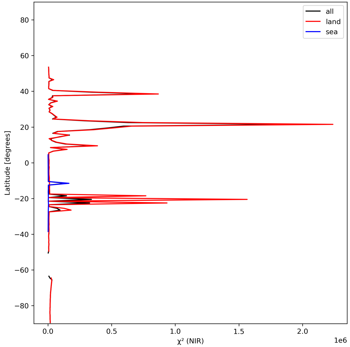
Figure 18: Zonal average of “ \chi^2 (NIR)” for 2024-01-11 to 2024-01-13.
