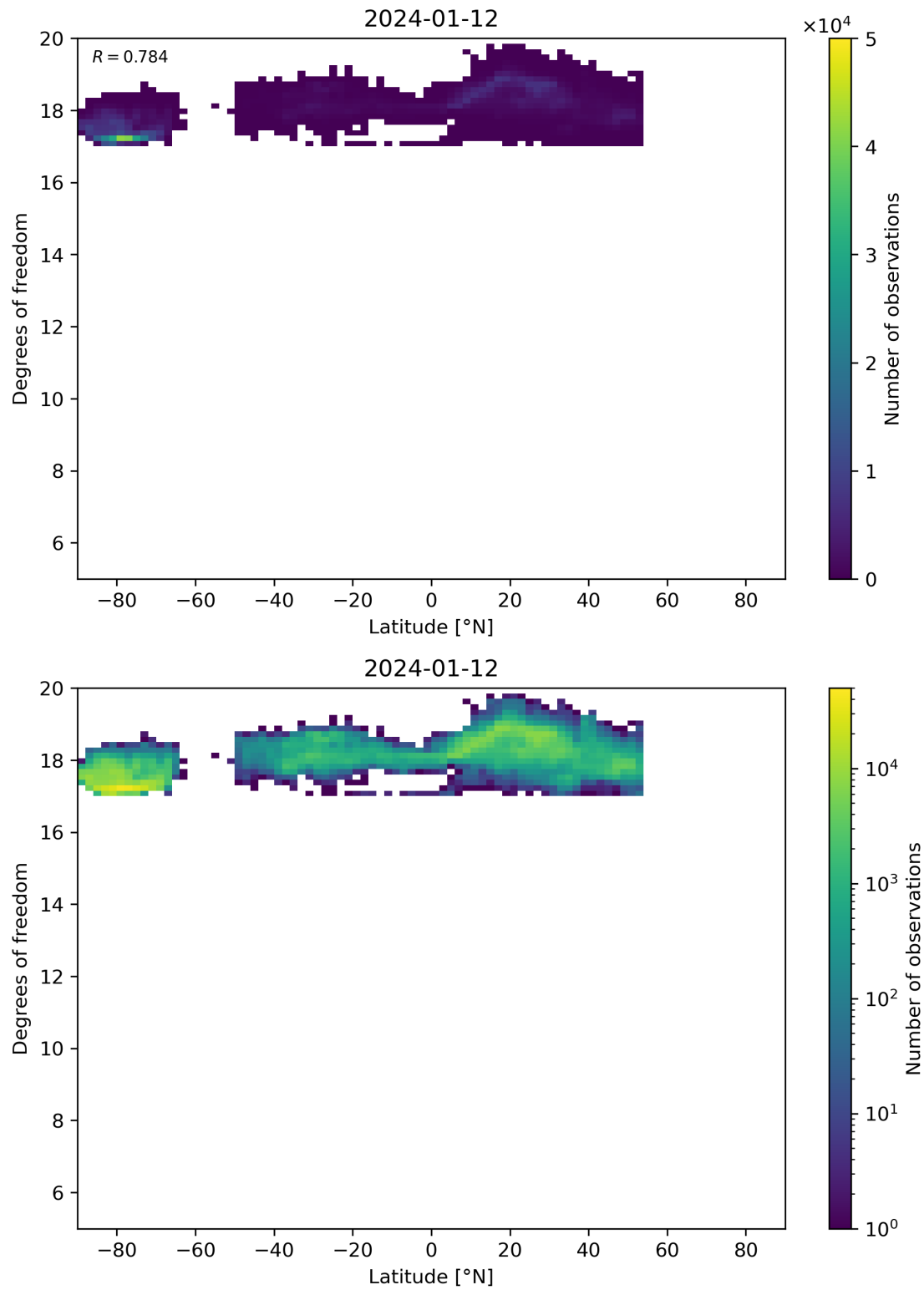
Figure 55: Scatter density plot of “Latitude” against “Degrees of freedom” for 2024-01-11 to 2024-01-13.
