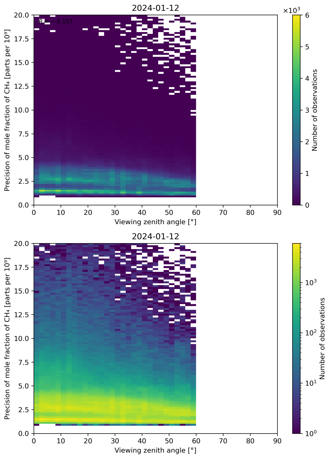
Figure 112: Scatter density plot of “Viewing zenith angle” against “Precision of mole fraction of CH 4 ” for 2024-01-11 to 2024-01-13.
