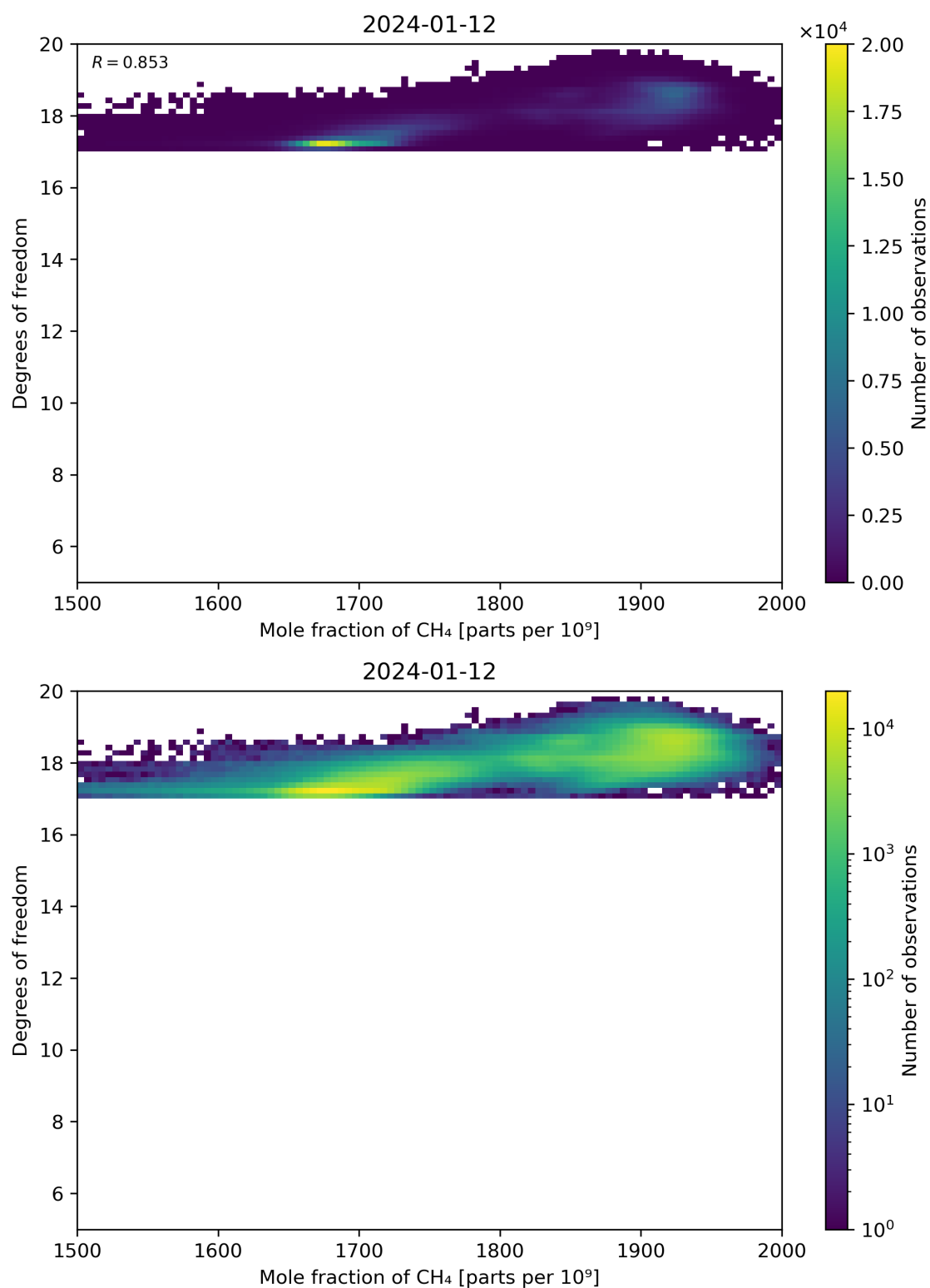
Figure 72: Scatter density plot of “Mole fraction of CH 4 ” against “Degrees of freedom” for 2024-01-11 to 2024-01-13.
