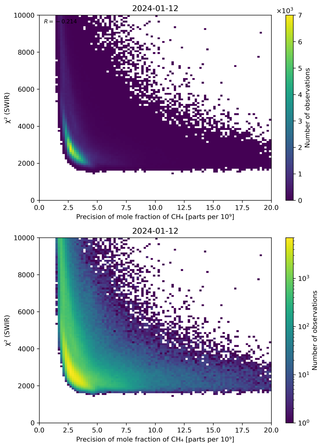
Figure 79: Scatter density plot of “Precision of mole fraction of \text{CH}_4 ” against “ \chi^2 (SWIR)” for 2024-01-11 to 2024-01-13.
