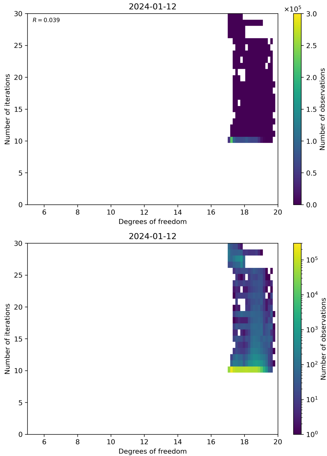
Figure 52: Scatter density plot of “Degrees of freedom” against “Number of iterations” for 2024-01-11 to 2024-01-13.
