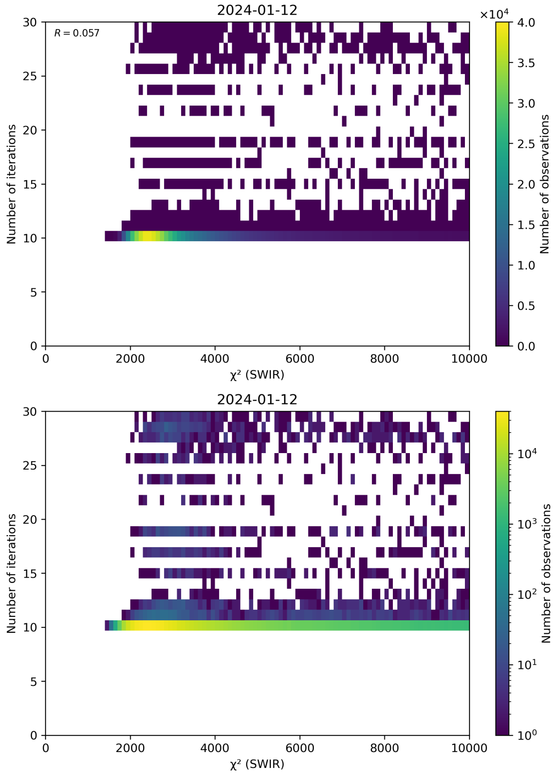
Figure 50: Scatter density plot of “ \chi^2 (SWIR)” against “Number of iterations” for 2024-01-11 to 2024-01-13.
