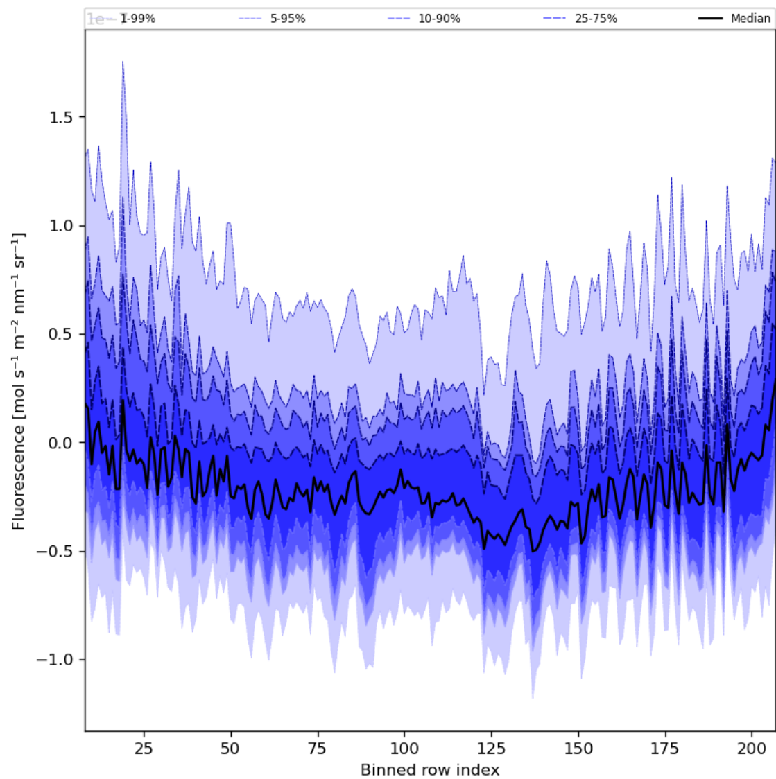
Figure 43: Along track statistics of “Fluorescence” for 2024-01-11 to 2024-01-13
