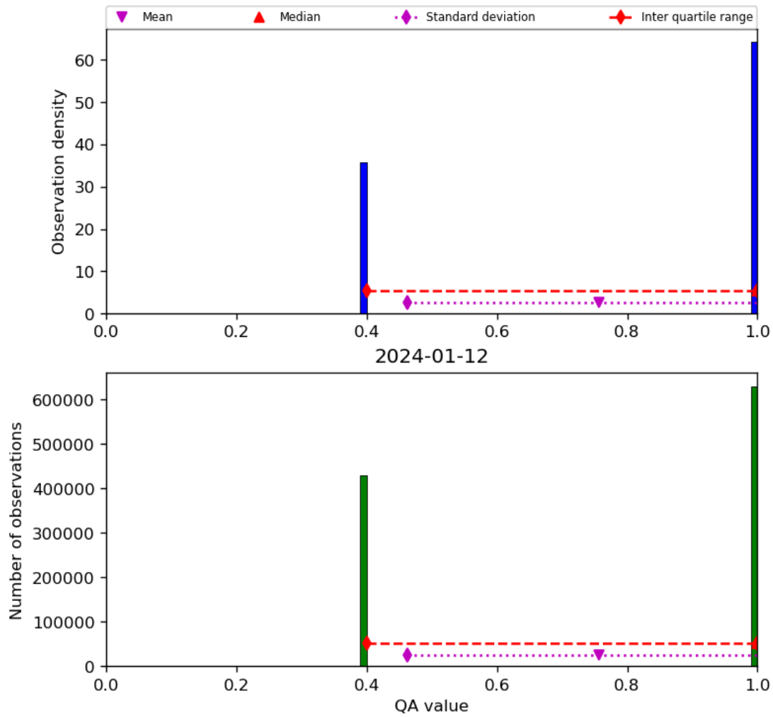
Figure 22: Histogram of “QA value” for 2024-01-11 to 2024-01-13
