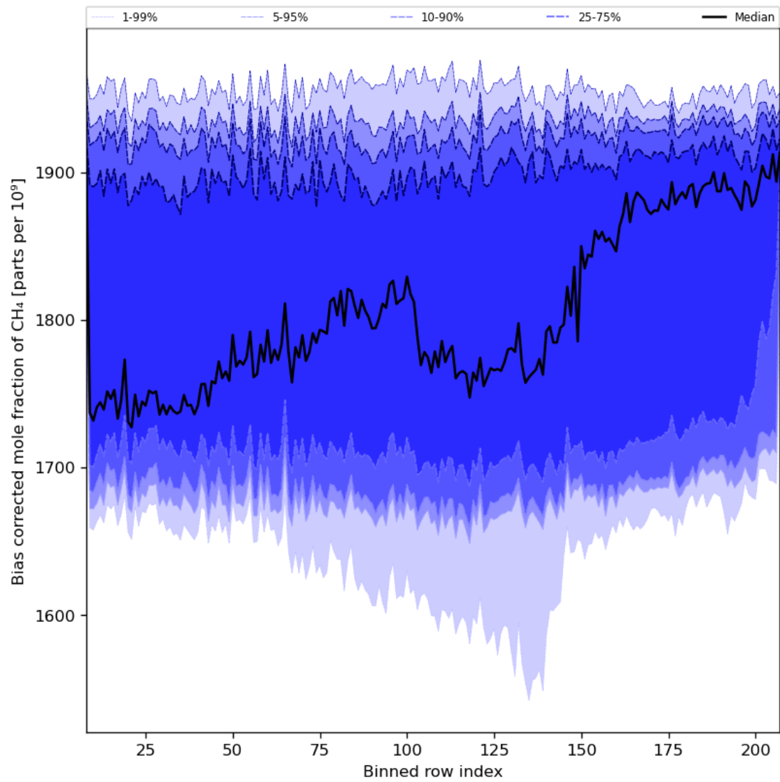
Figure 36: Along track statistics of “Bias corrected mole fraction of CH 4 ” for 2024-01-11 to 2024-01-13
