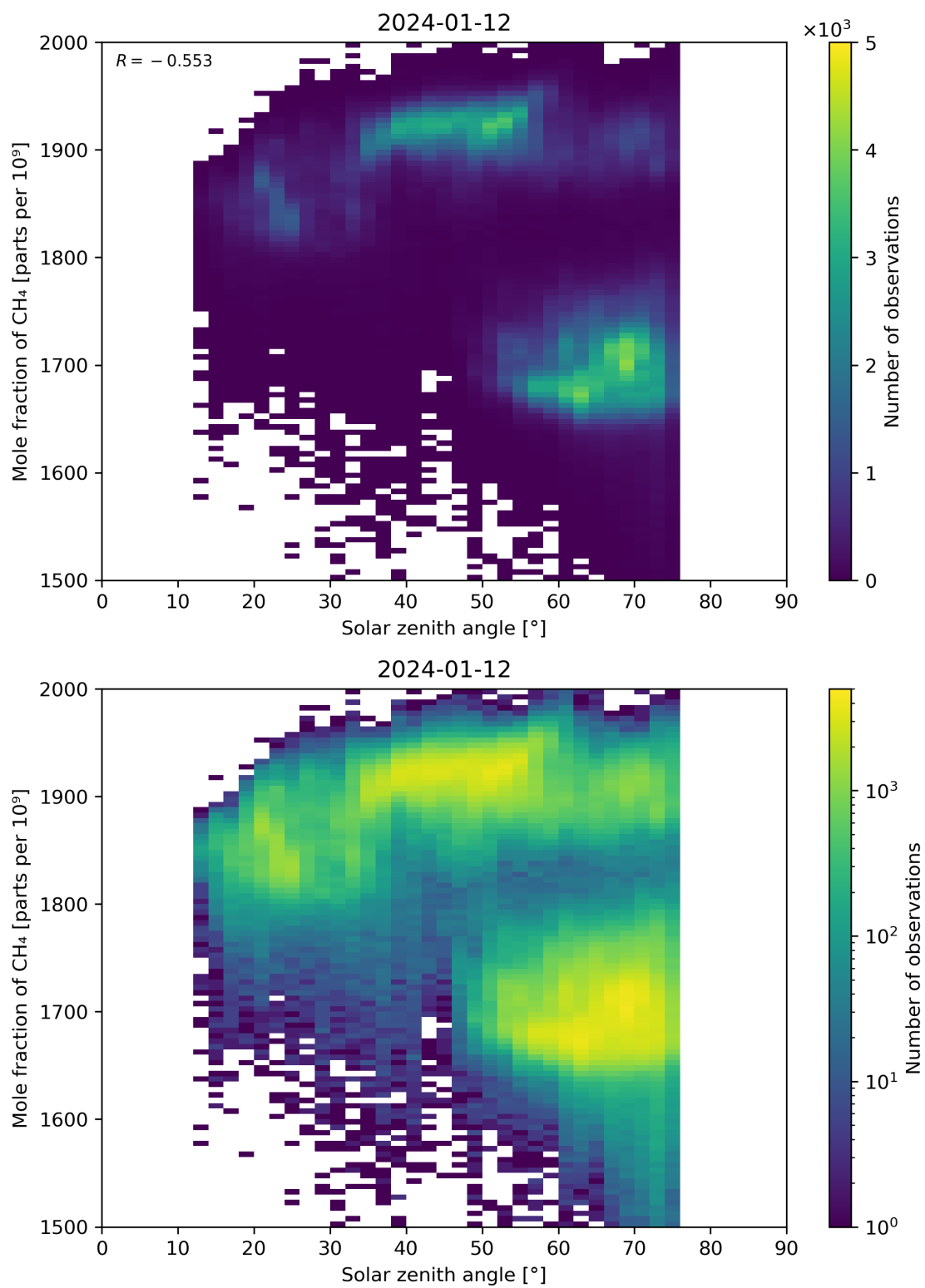
Figure 99: Scatter density plot of “Solar zenith angle” against “Mole fraction of \text{CH}_4 ” for 2024-01-11 to 2024-01-13.
