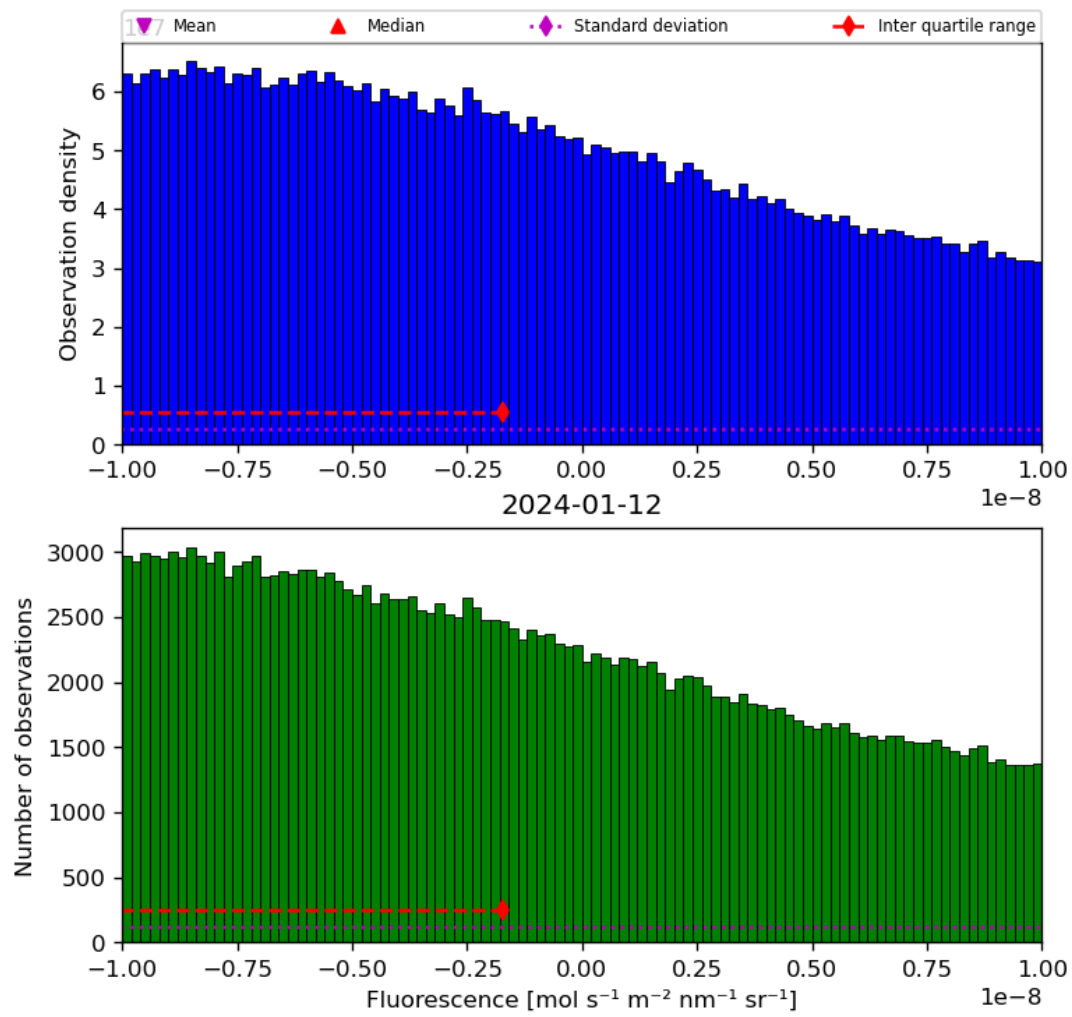
Figure 32: Histogram of “Fluorescence” for 2024-01-11 to 2024-01-13
