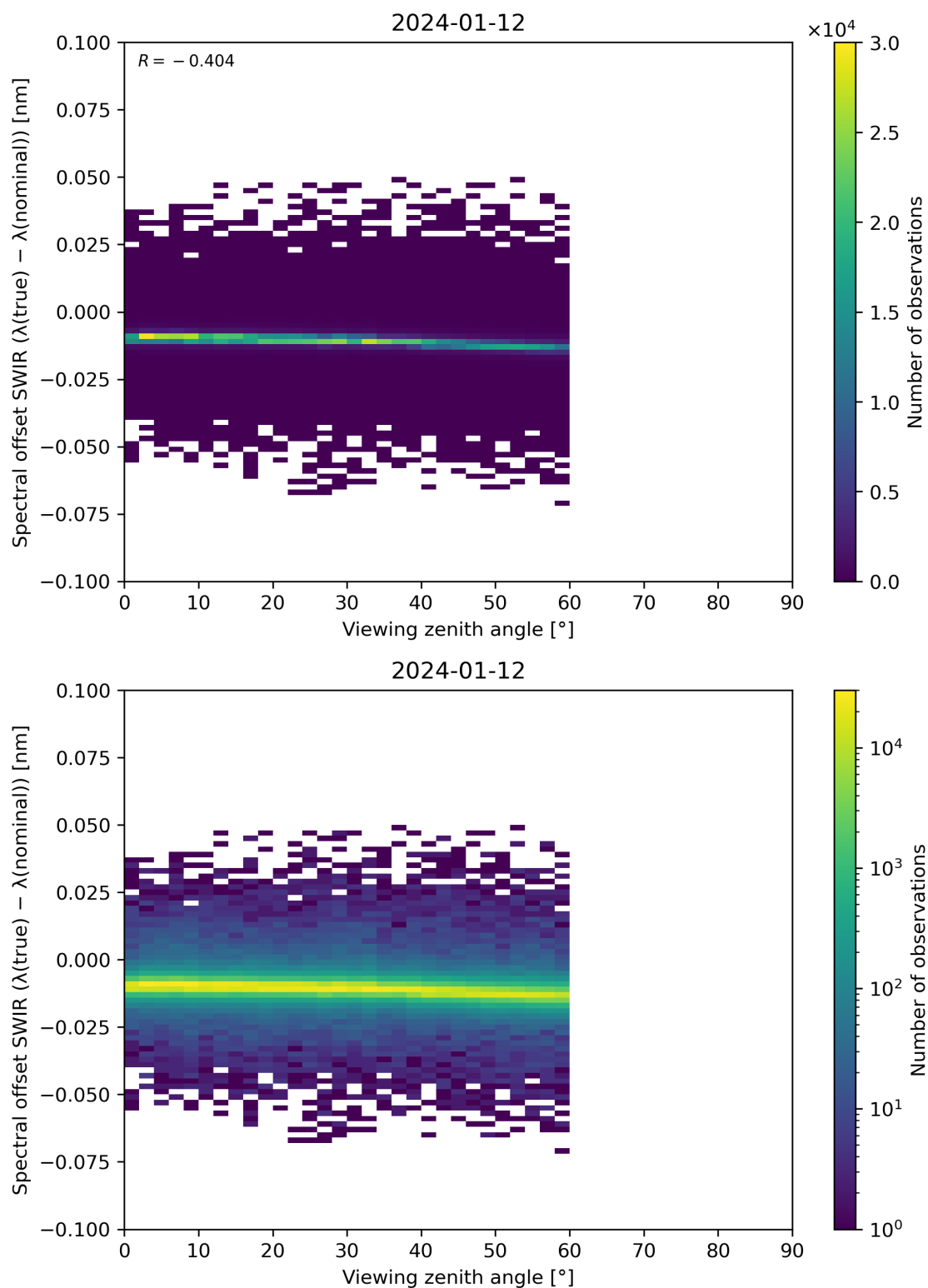
Figure 116: Scatter density plot of “Viewing zenith angle” against “Spectral offset SWIR ( \lambda(\text{true}) - \lambda(\text{nominal}) )” for 2024-01-11 to 2024-01-13.
