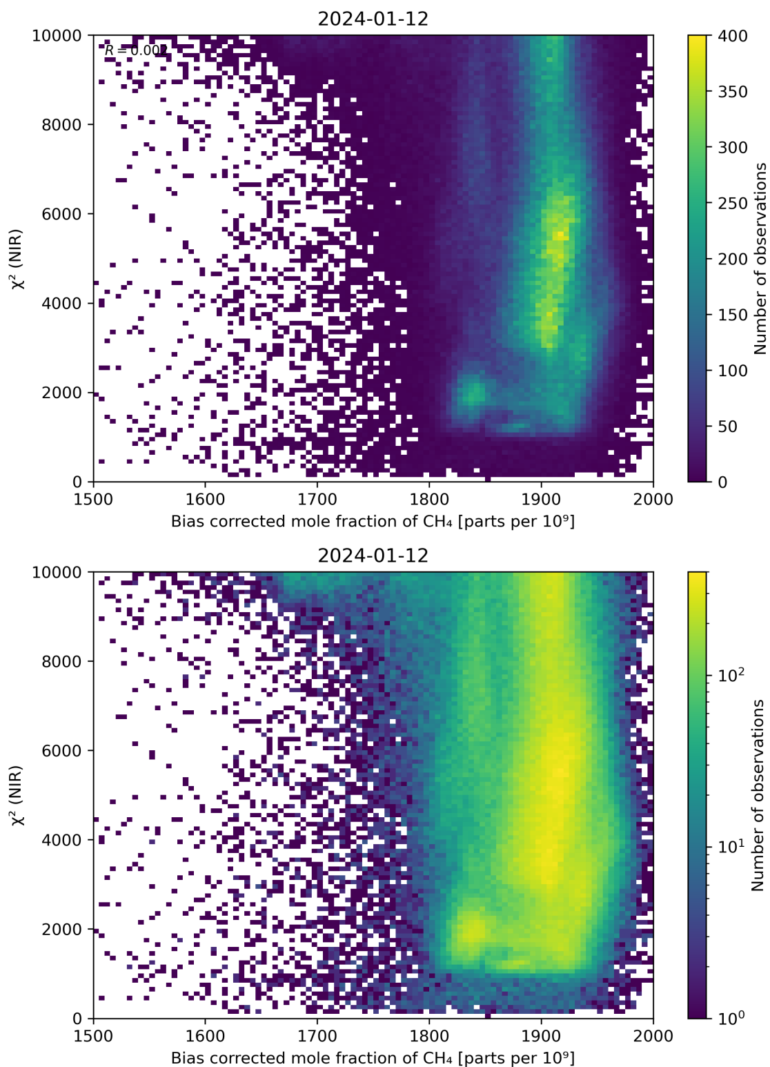
Figure 63: Scatter density plot of “Bias corrected mole fraction of CH 4 ” against “ \chi^2 (NIR)” for 2024-01-11 to 2024-01-13.
