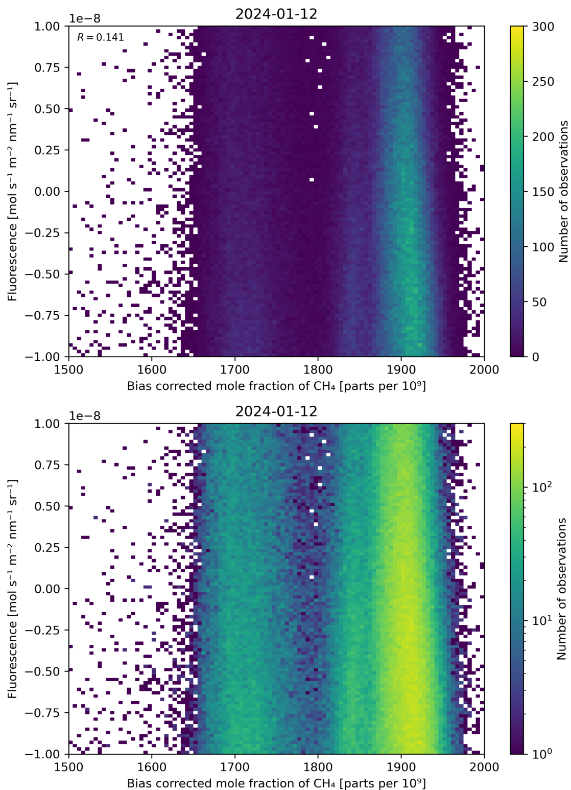
Figure 66: Scatter density plot of “Bias corrected mole fraction of \text{CH}_4 ” against “Fluorescence” for 2024-01-11 to 2024-01-13.
