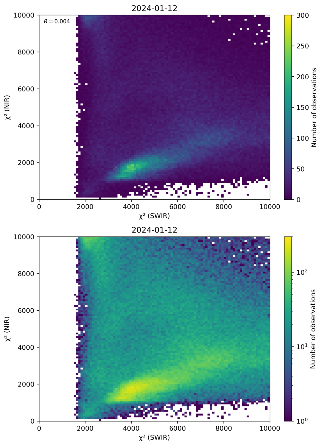
Figure 47: Scatter density plot of “ \chi^2 (SWIR)” against “ \chi^2 (NIR)” for 2024-01-11 to 2024-01-13.
