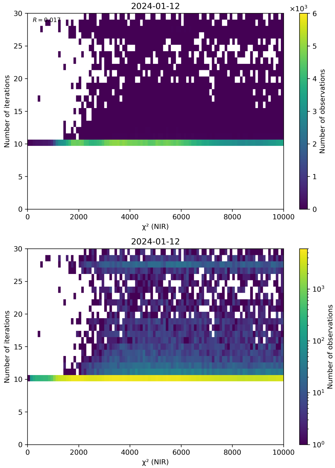
Figure 46: Scatter density plot of “ \chi^2 (NIR)” against “Number of iterations” for 2024-01-11 to 2024-01-13.
