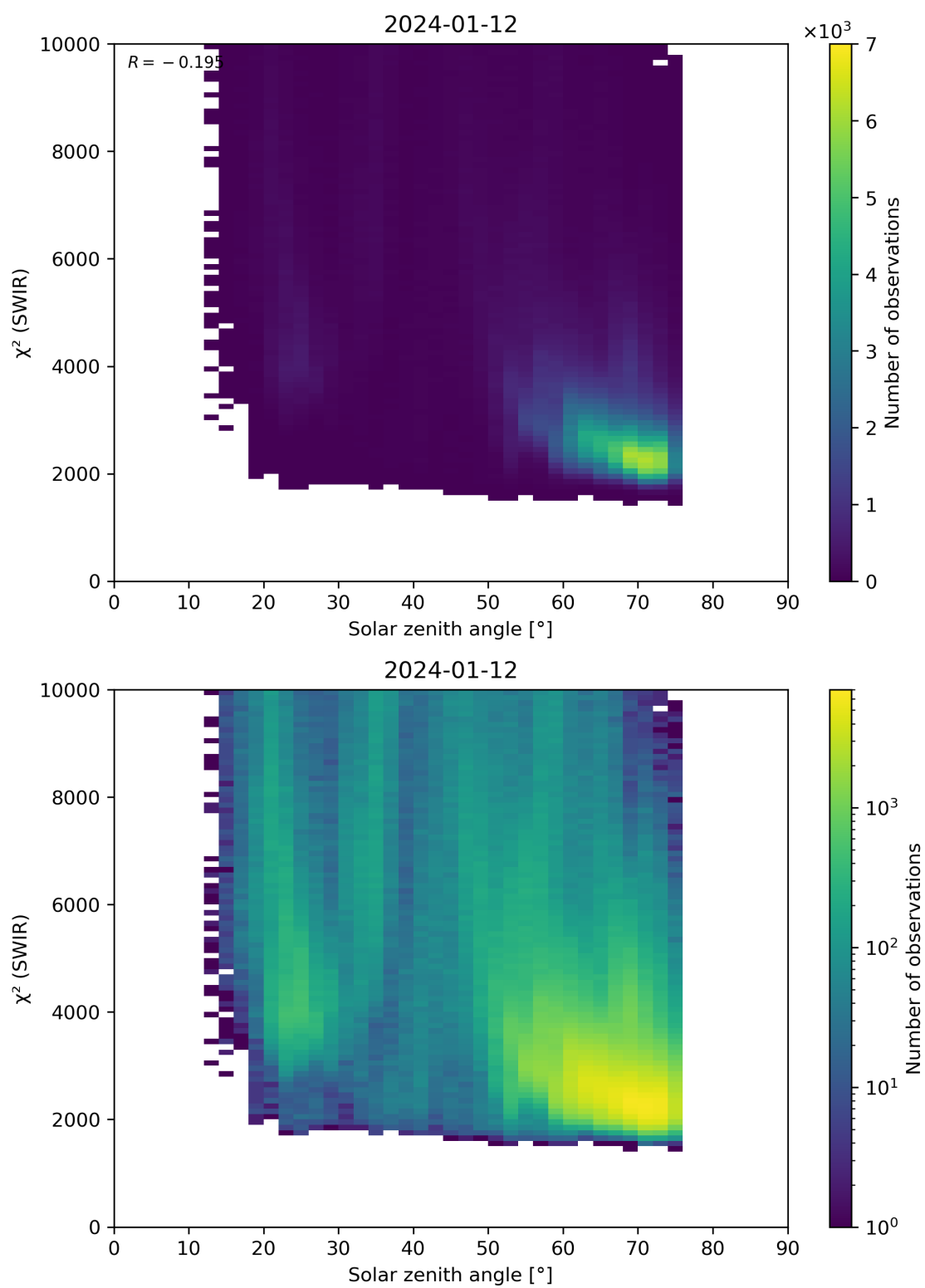
Figure 95: Scatter density plot of “Solar zenith angle” against “ \chi^2 (SWIR)” for 2024-01-11 to 2024-01-13.
