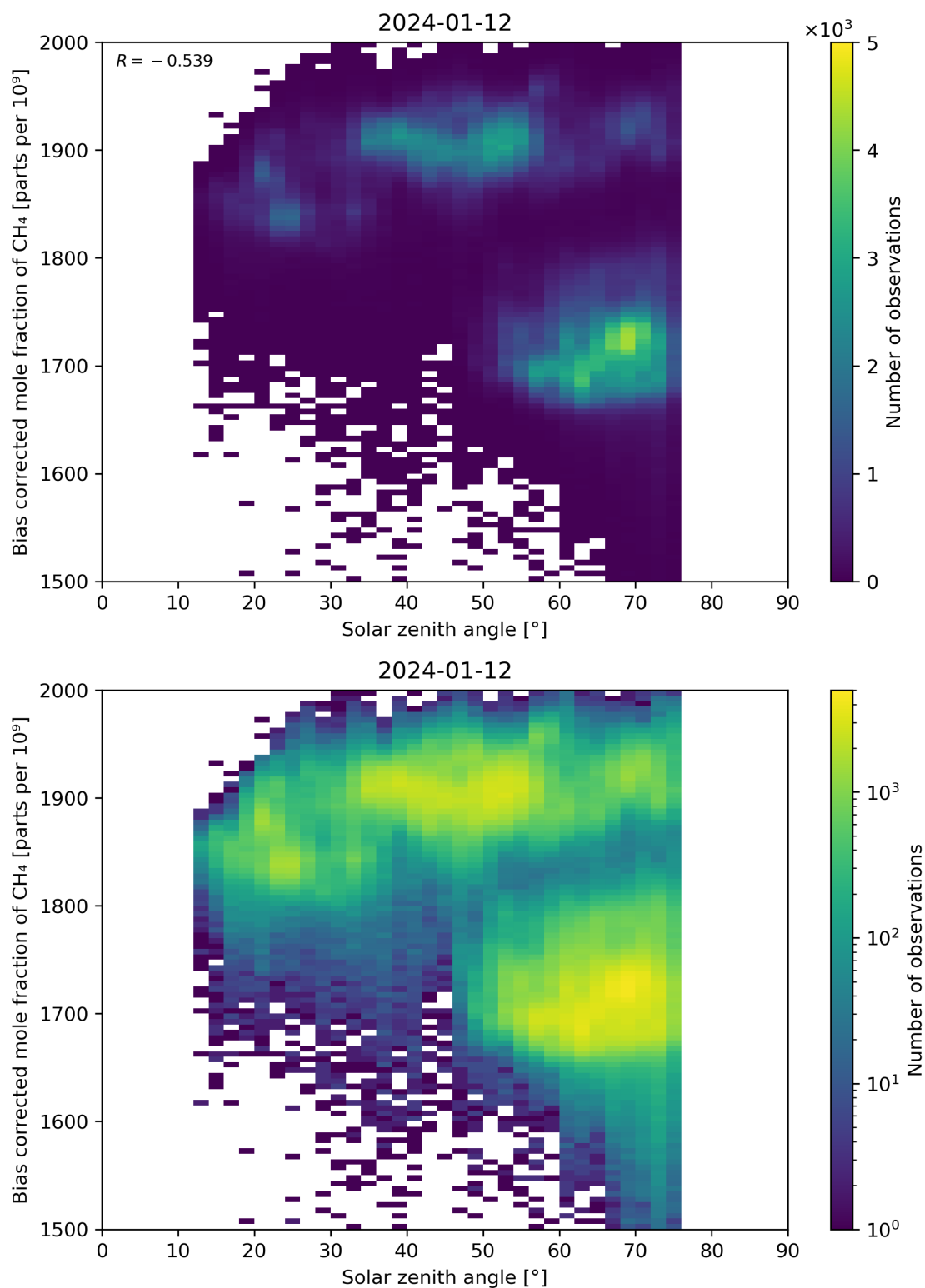
Figure 100: Scatter density plot of “Solar zenith angle” against “Bias corrected mole fraction of CH 4 ” for 2024-01-11 to 2024-01-13.
