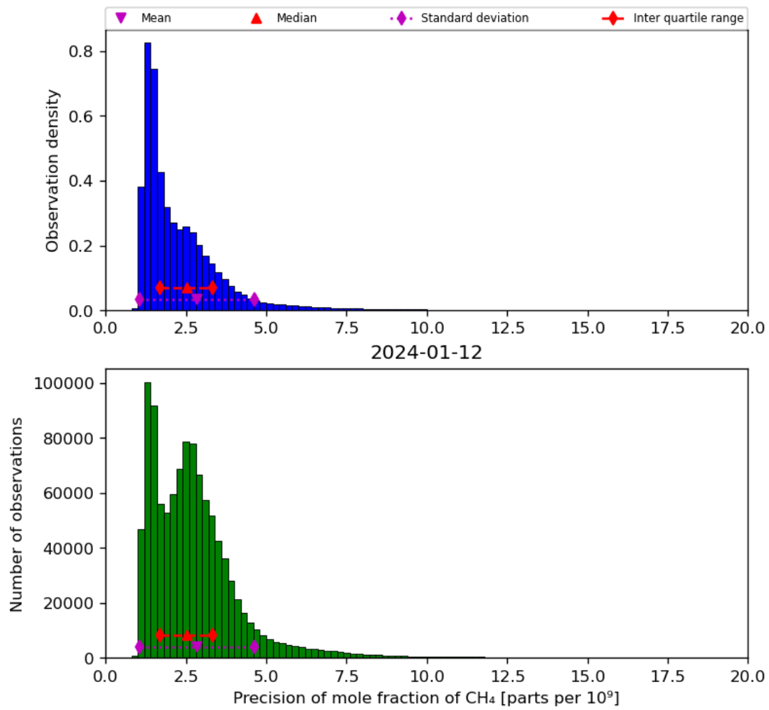
Figure 24: Histogram of “Precision of mole fraction of CH 4 ” for 2024-01-11 to 2024-01-13
