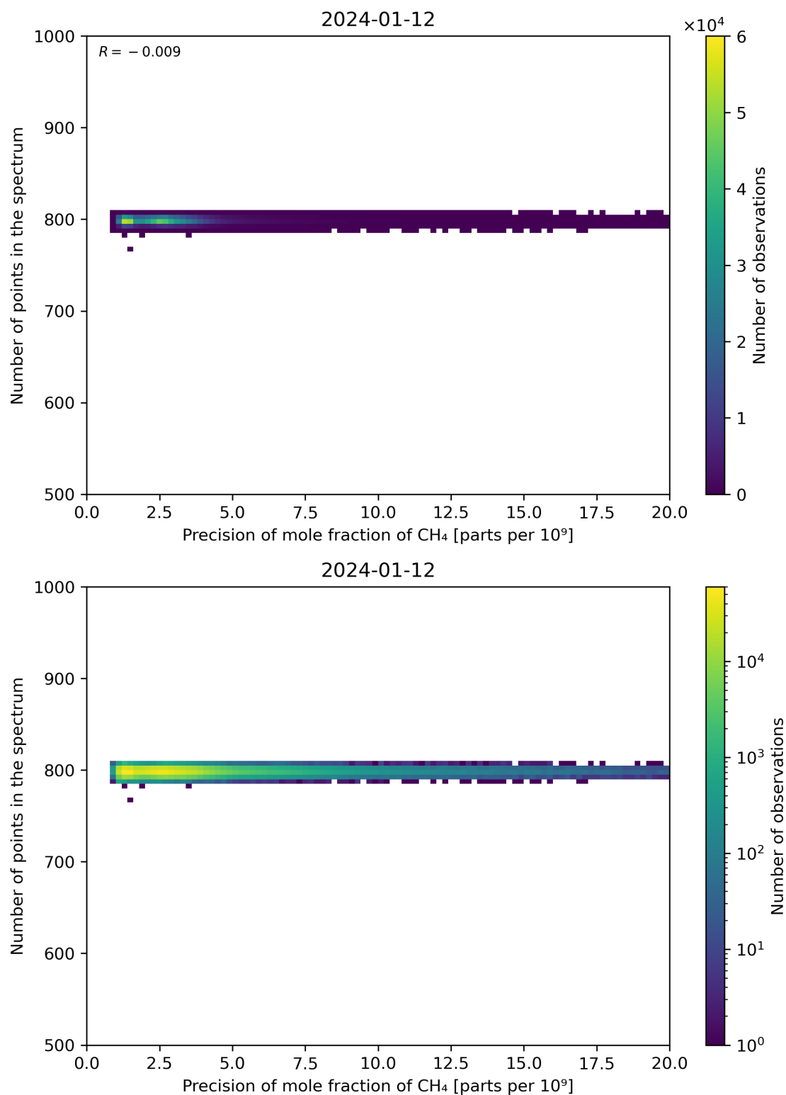
Figure 84: Scatter density plot of “Precision of mole fraction of CH 4 ” against “Number of points in the spectrum” for 2024-01-11 to 2024-01-13.
