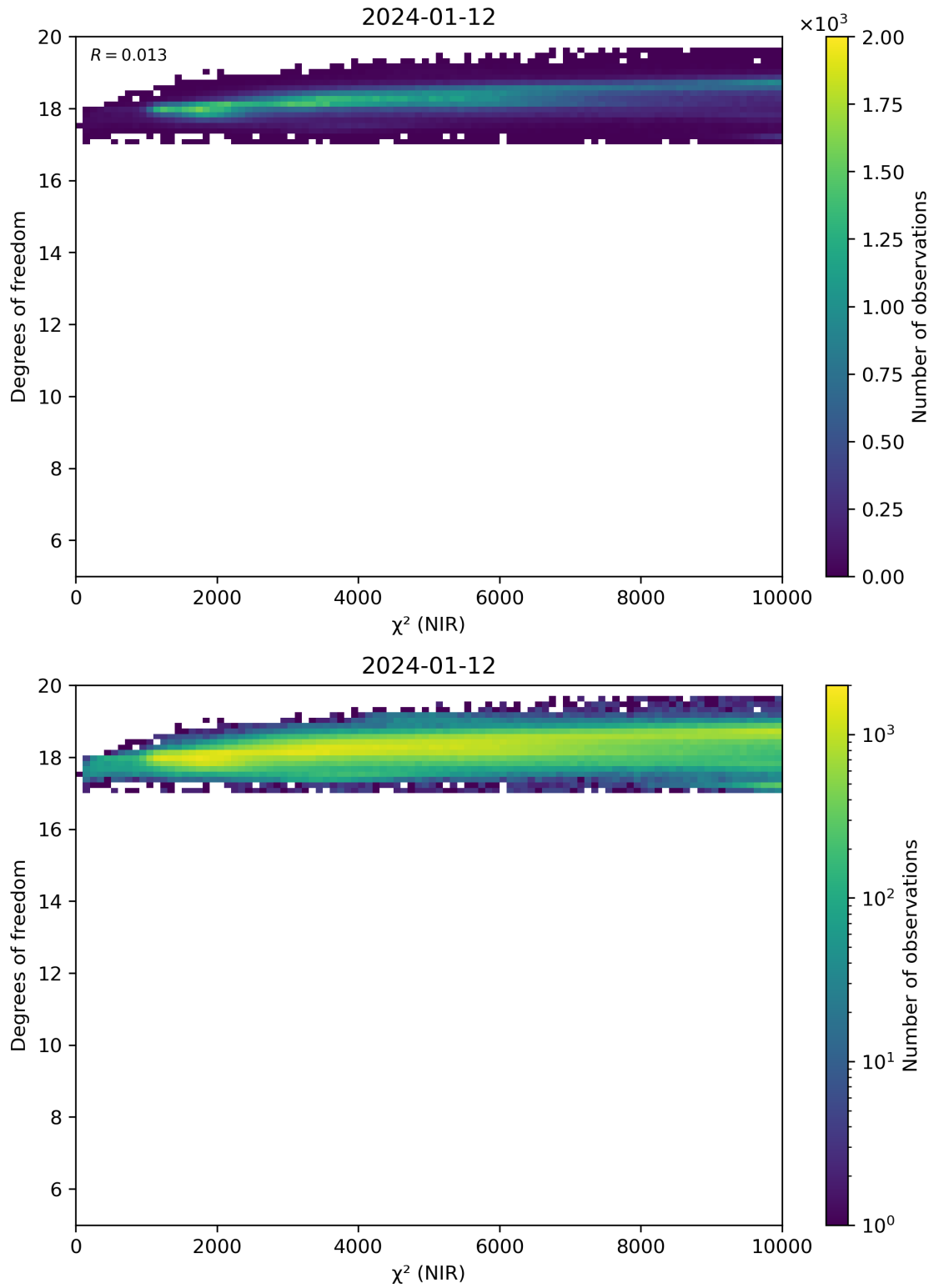
Figure 44: Scatter density plot of “ \chi^2 (NIR)” against “Degrees of freedom” for 2024-01-11 to 2024-01-13.
