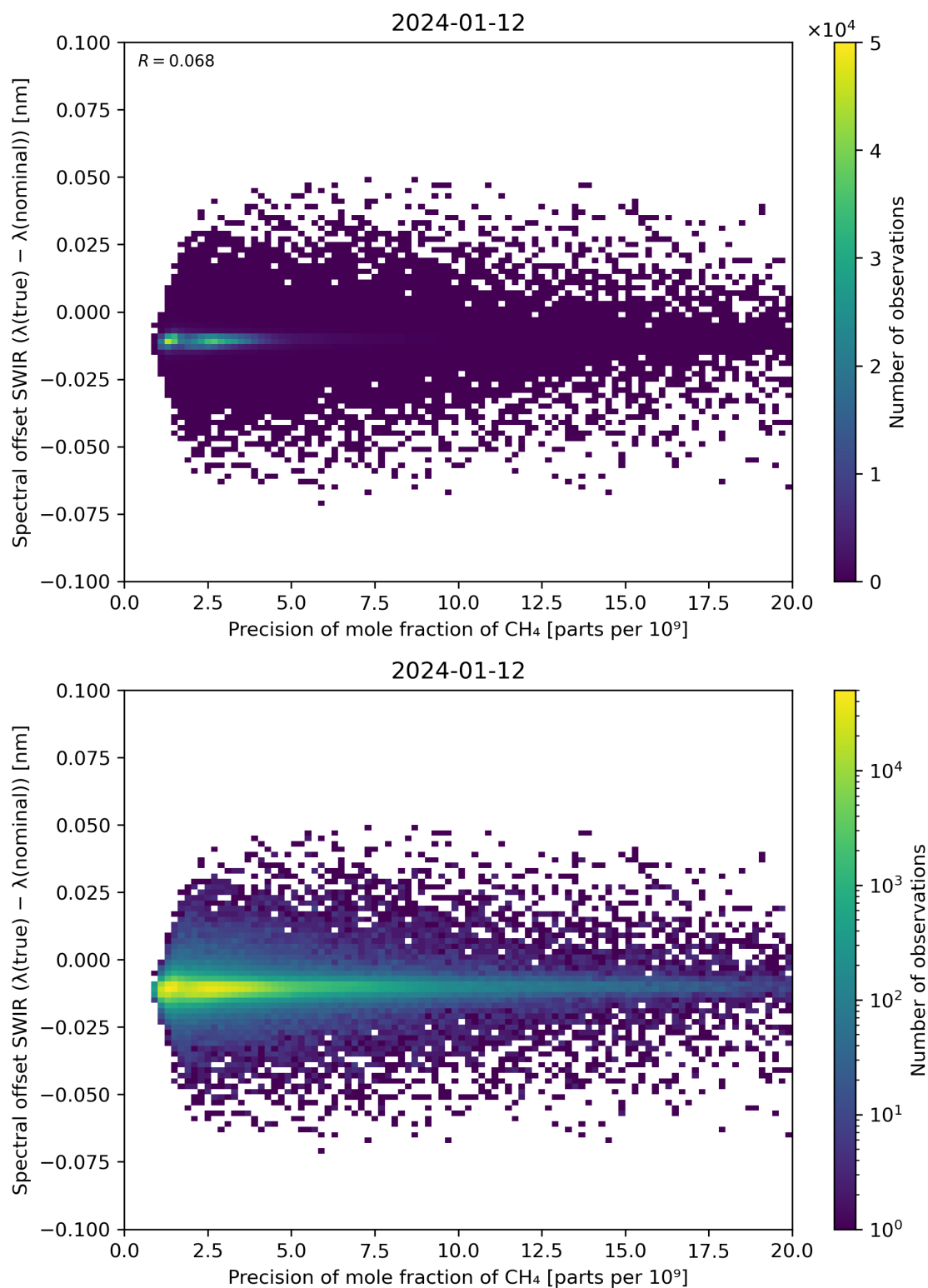
Figure 85: Scatter density plot of “Precision of mole fraction of CH 4 ” against “Spectral offset SWIR ( \lambda(\text{true}) - \lambda(\text{nominal}) )” for 2024-01-11 to 2024-01-13.
