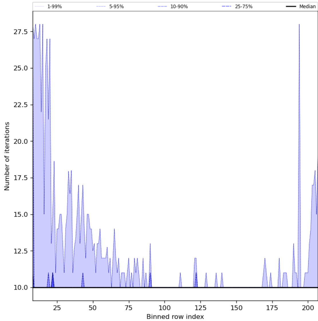
Figure 42: Along track statistics of “Number of iterations” for 2024-01-11 to 2024-01-13
