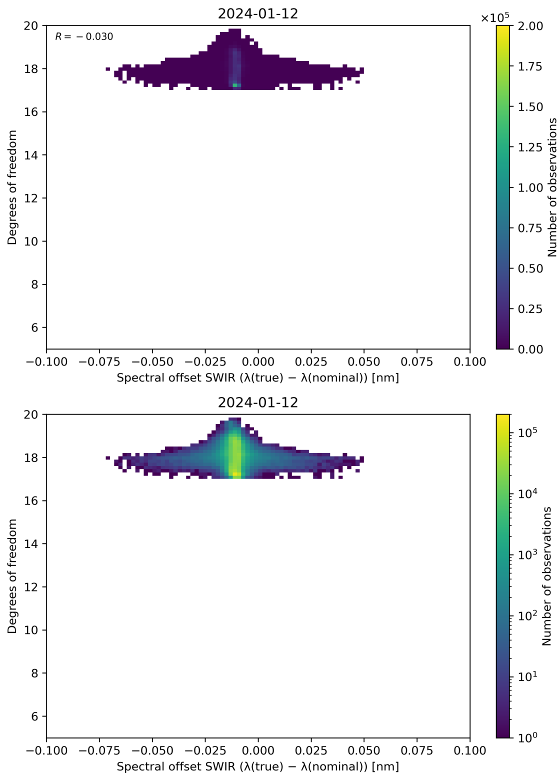
Figure 119: Scatter density plot of “Spectral offset SWIR ( \lambda(\text{true}) - \lambda(\text{nominal}) )” against “Degrees of freedom” for 2024-01-11 to 2024-01-13.
