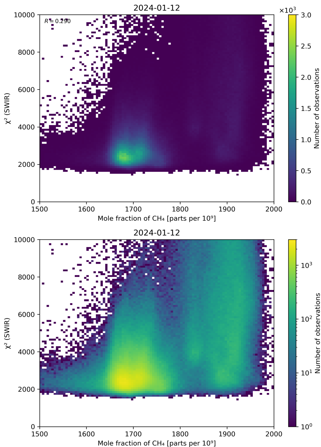
Figure 71: Scatter density plot of “Mole fraction of \text{CH}_4 ” against “ \chi^2 (SWIR)” for 2024-01-11 to 2024-01-13.
