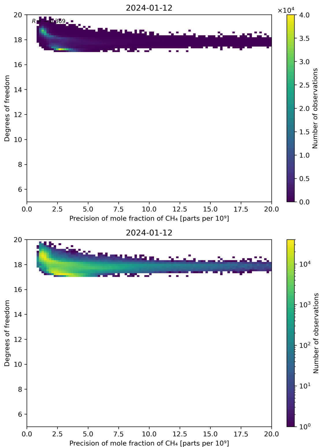
Figure 80: Scatter density plot of “Precision of mole fraction of CH 4 ” against “Degrees of freedom” for 2024-01-11 to 2024-01-13.
