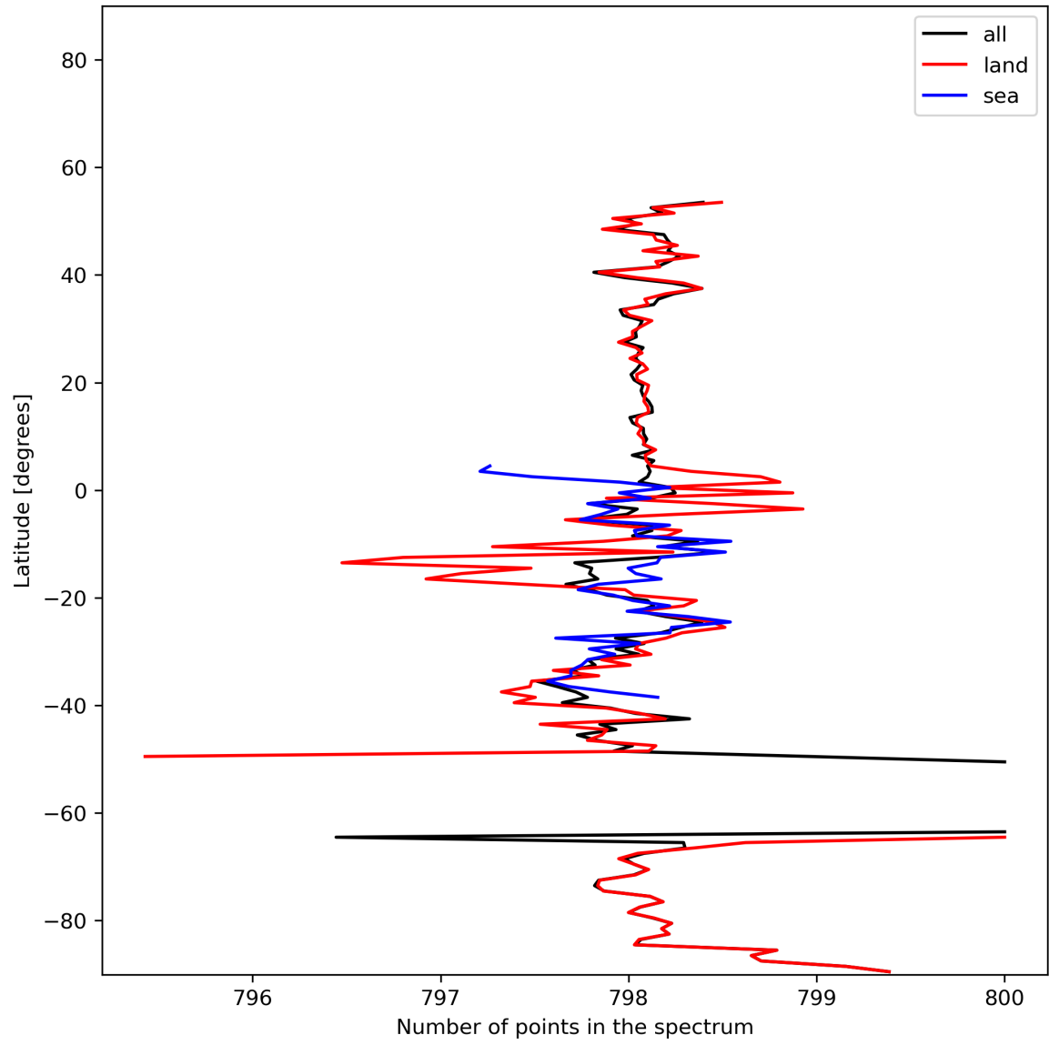
Figure 15: Zonal average of “Number of points in the spectrum” for 2024-01-11 to 2024-01-13.
