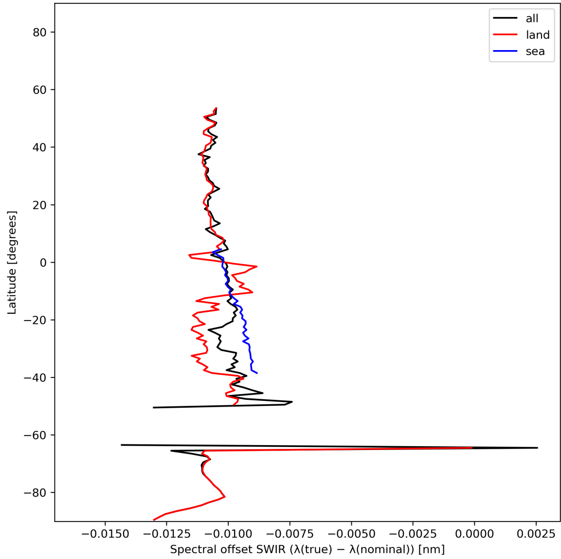
Figure 16: Zonal average of “Spectral offset SWIR ( \lambda(\text{true}) - \lambda(\text{nominal}) )” for 2024-01-11 to 2024-01-13.
