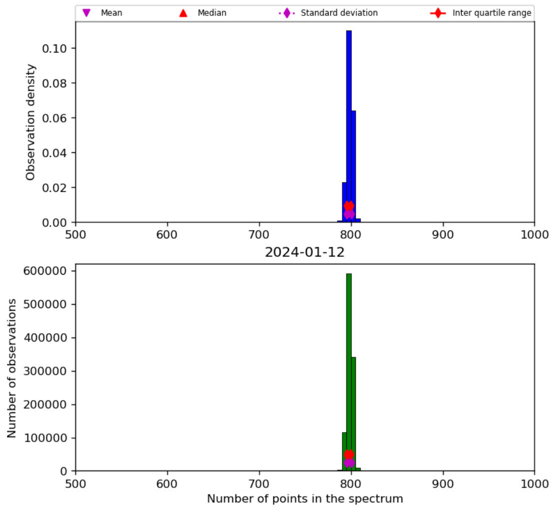
Figure 26: Histogram of “Number of points in the spectrum” for 2024-01-11 to 2024-01-13
