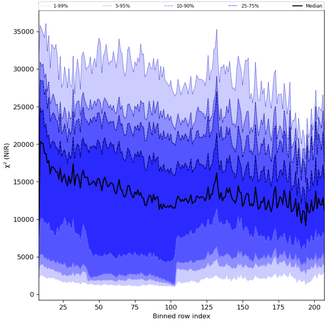
Figure 40: Along track statistics of “ \chi^2 (NIR)” for 2024-01-11 to 2024-01-13
