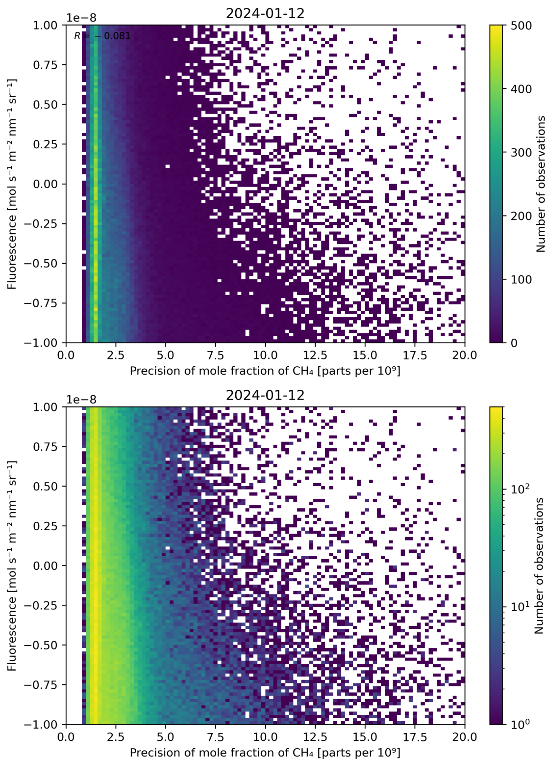
Figure 81: Scatter density plot of “Precision of mole fraction of CH 4 ” against “Fluorescence” for 2024-01-11 to 2024-01-13.
