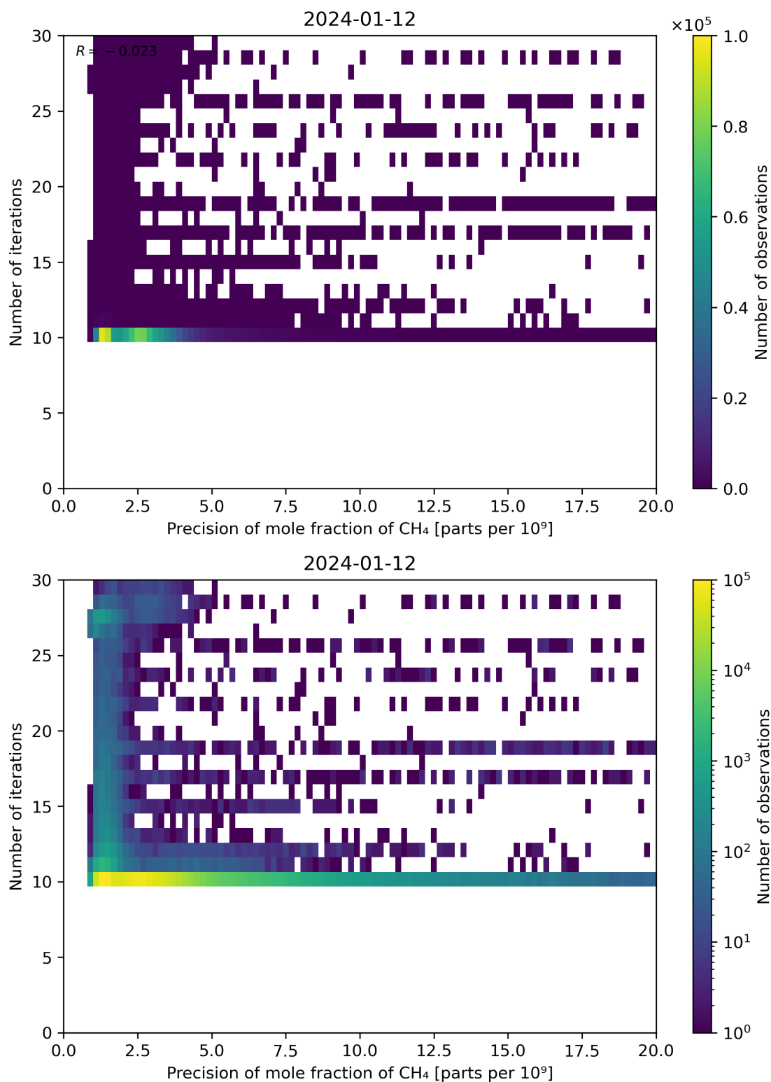
Figure 83: Scatter density plot of “Precision of mole fraction of CH 4 ” against “Number of iterations” for 2024-01-11 to 2024-01-13.
