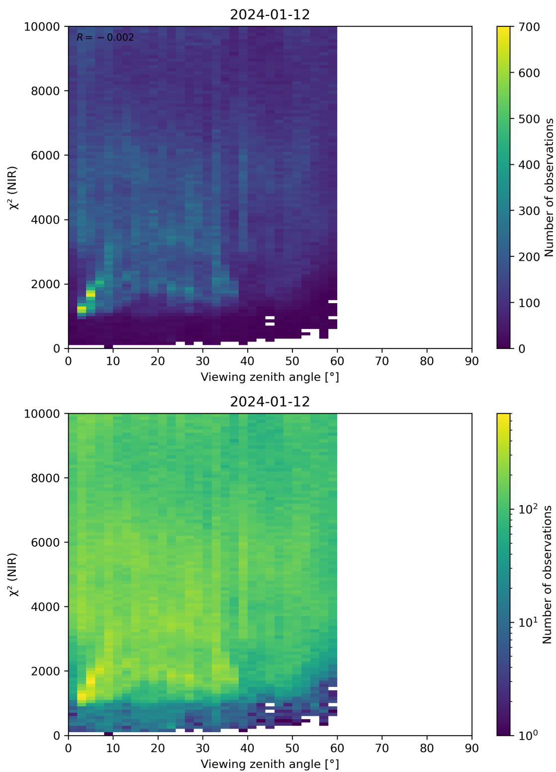
Figure 105: Scatter density plot of “Viewing zenith angle” against “ \chi^2 (NIR)” for 2024-01-11 to 2024-01-13.
