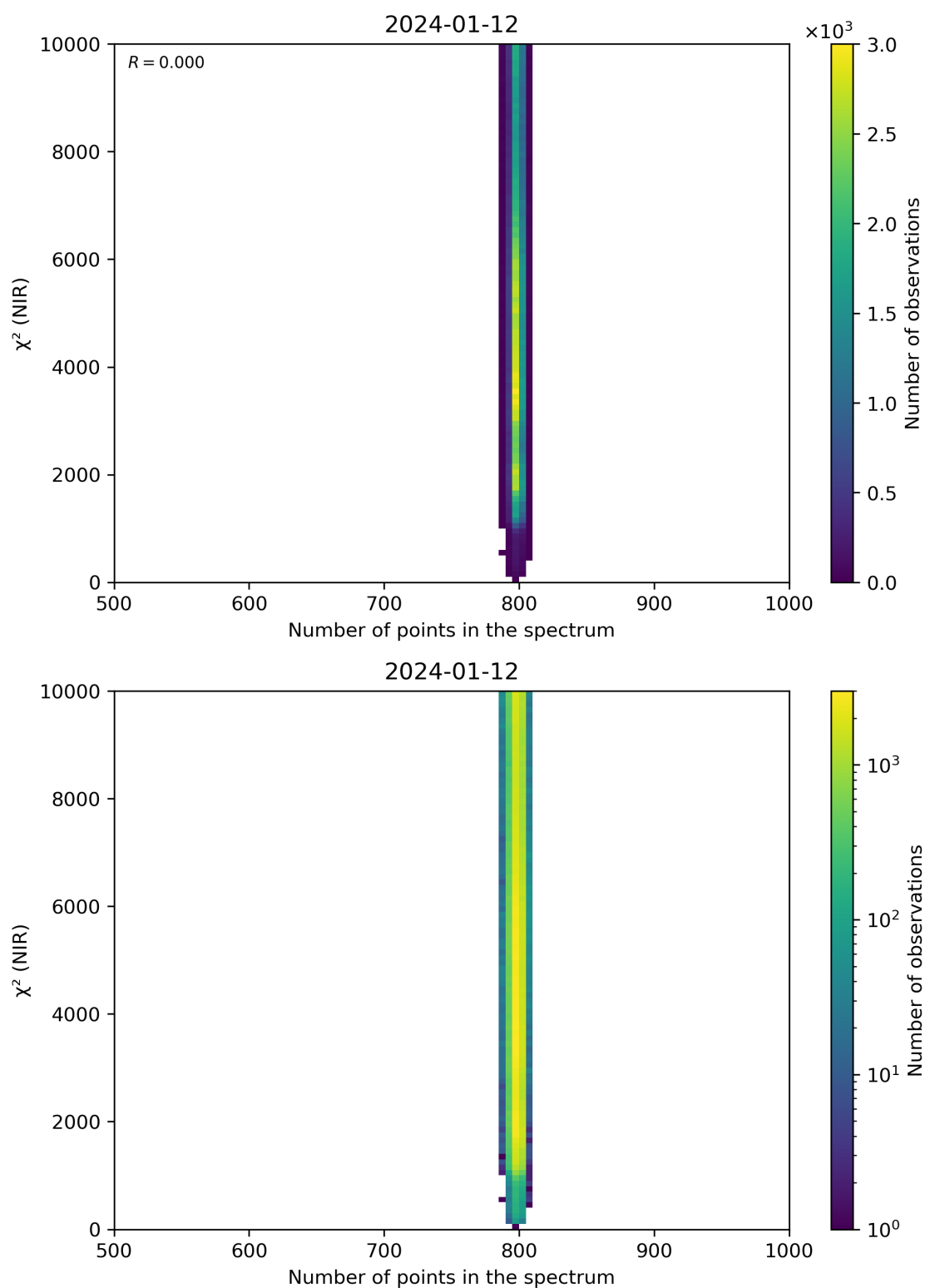
Figure 88: Scatter density plot of “Number of points in the spectrum” against “ \chi^2 (NIR)” for 2024-01-11 to 2024-01-13.
