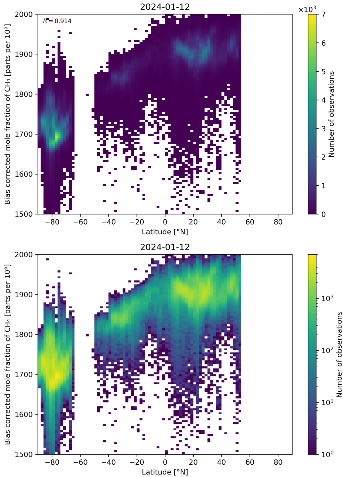
Figure 58: Scatter density plot of “Latitude” against “Bias corrected mole fraction of CH 4 ” for 2024-01-11 to 2024-01-13.
