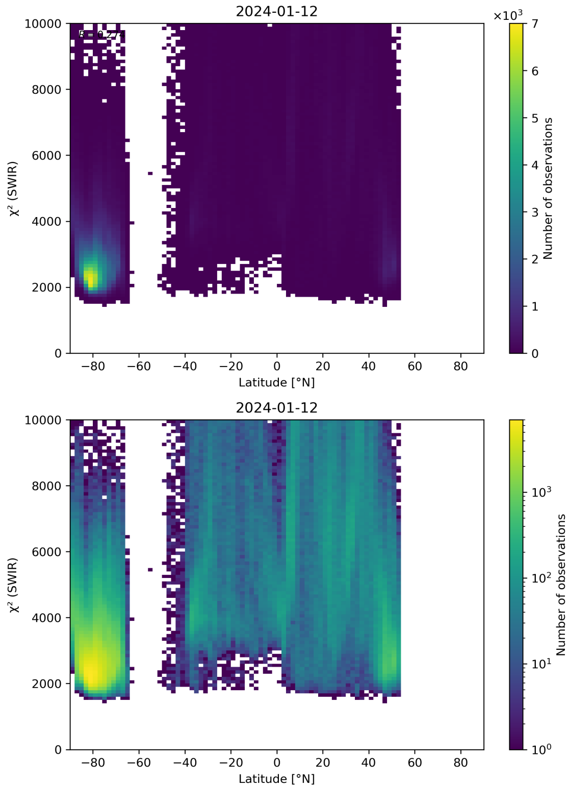
Figure 54: Scatter density plot of “Latitude” against “ \chi^2 (SWIR)” for 2024-01-11 to 2024-01-13.
