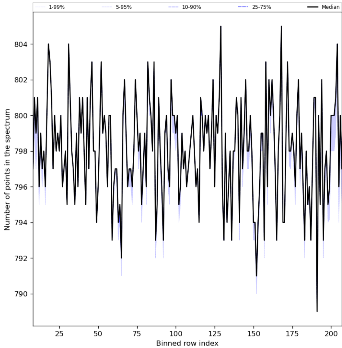
Figure 37: Along track statistics of “Number of points in the spectrum” for 2024-01-11 to 2024-01-13
