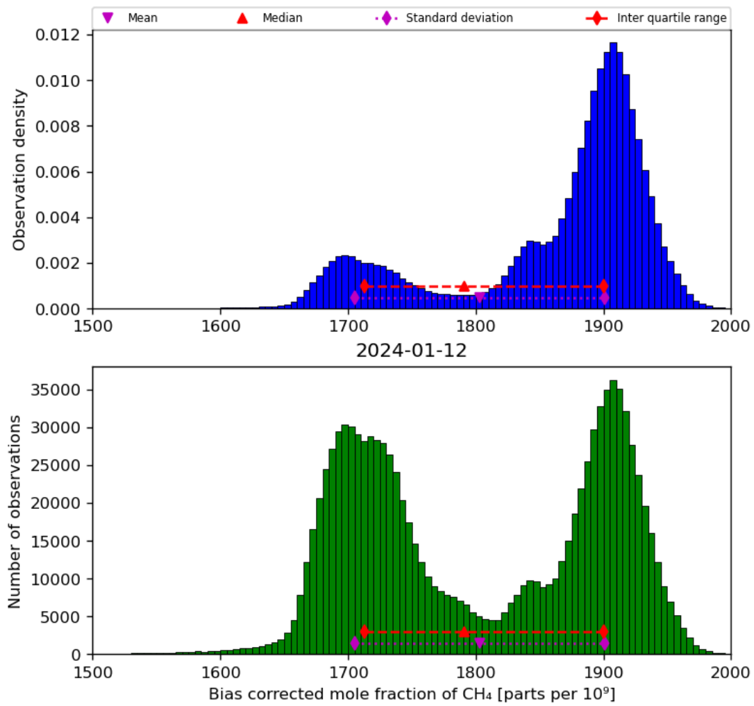
Figure 25: Histogram of “Bias corrected mole fraction of CH 4 ” for 2024-01-11 to 2024-01-13
