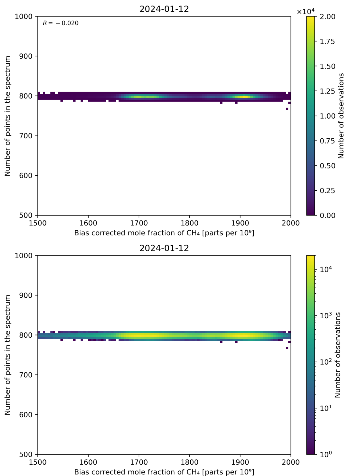
Figure 68: Scatter density plot of “Bias corrected mole fraction of CH 4 ” against “Number of points in the spectrum” for 2024-01-11 to 2024-01-13.
