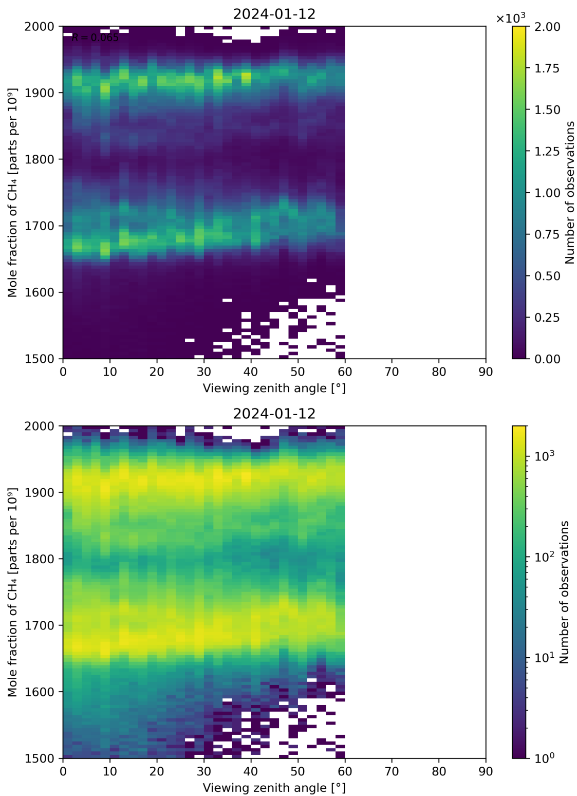
Figure 110: Scatter density plot of “Viewing zenith angle” against “Mole fraction of \text{CH}_4 ” for 2024-01-11 to 2024-01-13.
