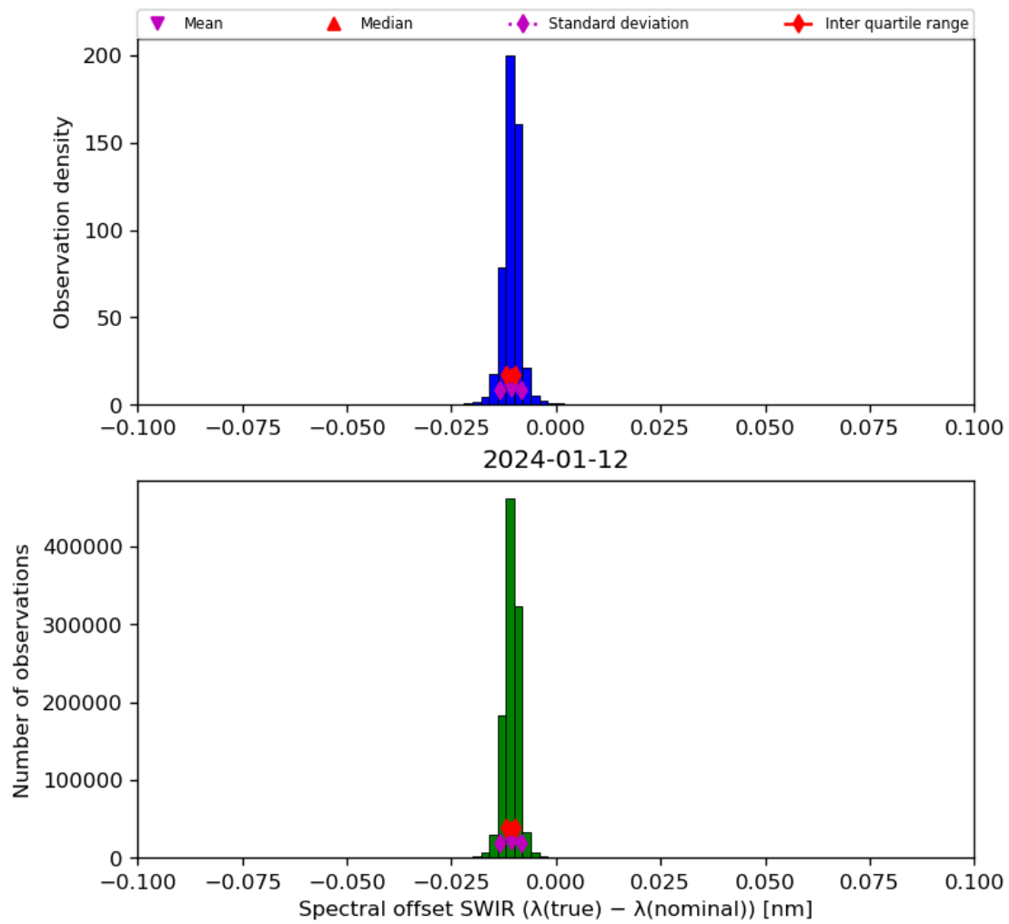
Figure 27: Histogram of “Spectral offset SWIR ( \lambda(\text{true}) - \lambda(\text{nominal}) )” for 2024-01-11 to 2024-01-13
