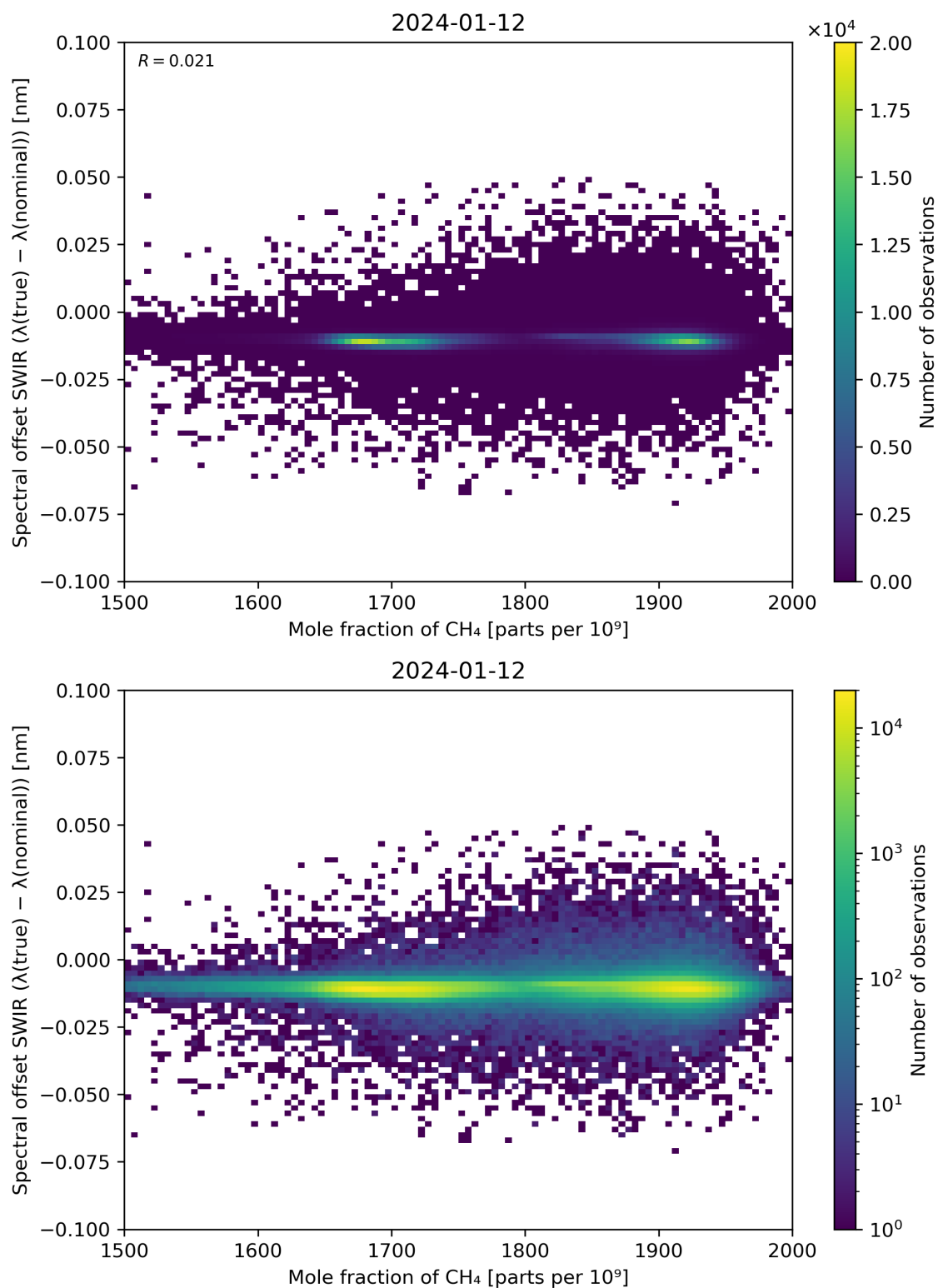
Figure 86: Scatter density plot of “Mole fraction of CH 4 ” against “Spectral offset SWIR ( \lambda(\text{true}) - \lambda(\text{nominal}) )” for 2024-01-11 to 2024-01-13.
