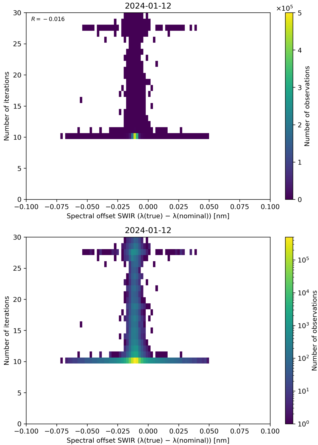
Figure 121: Scatter density plot of “Spectral offset SWIR ( \lambda(\text{true}) - \lambda(\text{nominal}) )” against “Number of iterations” for 2024-01-11 to 2024-01-13.
