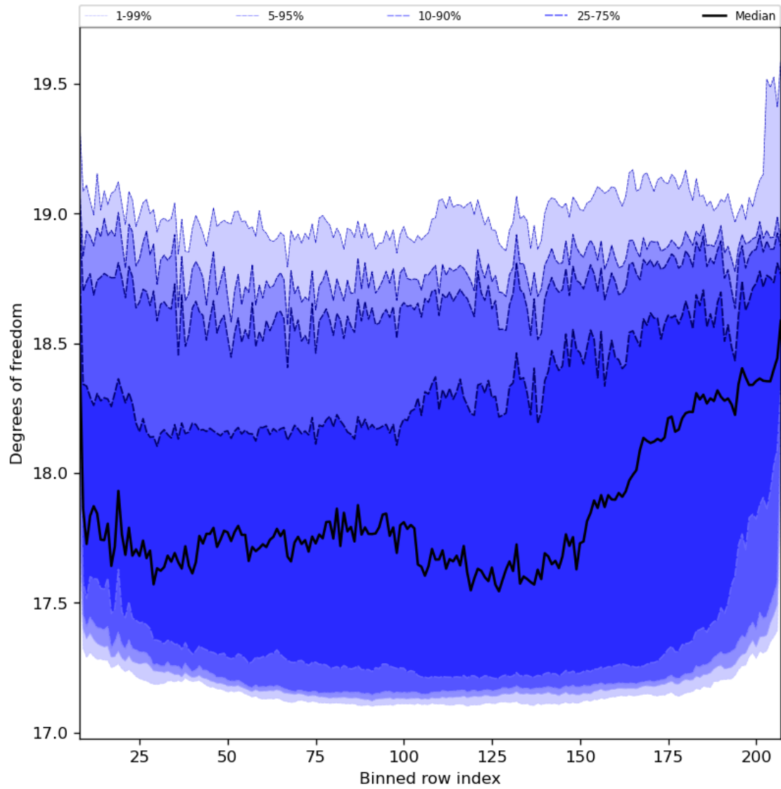
Figure 41: Along track statistics of “Degrees of freedom” for 2024-01-11 to 2024-01-13
