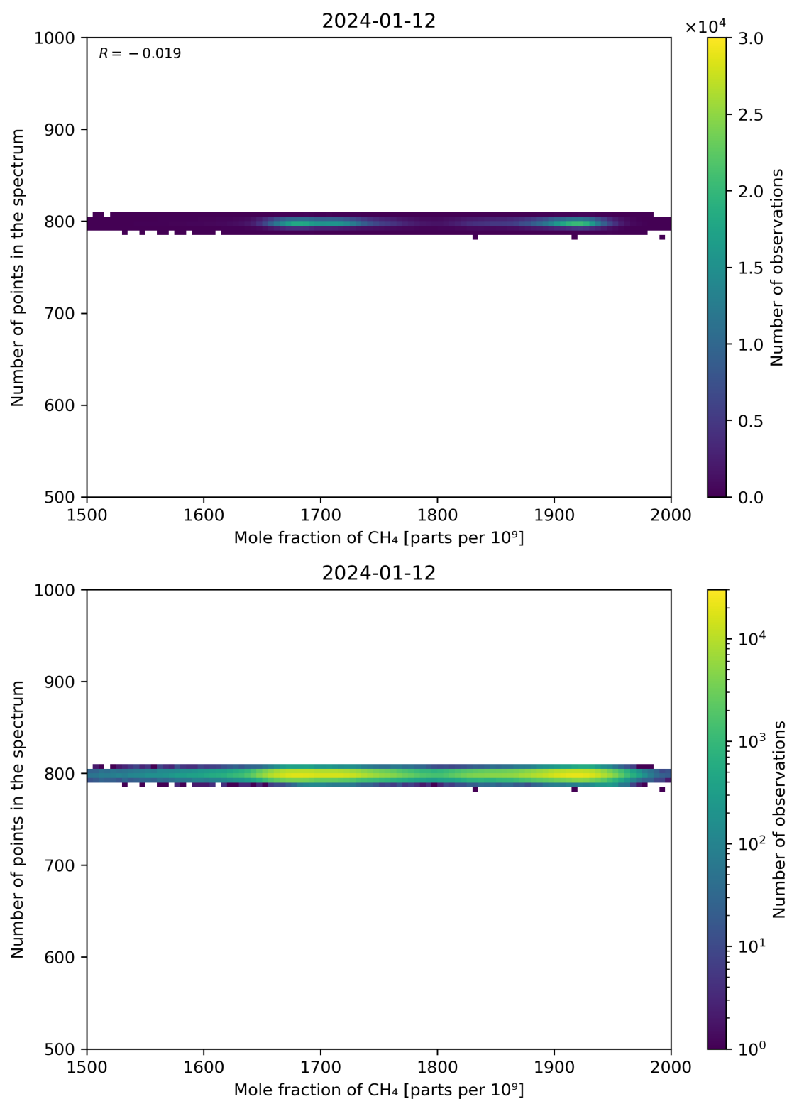
Figure 77: Scatter density plot of “Mole fraction of CH 4 ” against “Number of points in the spectrum” for 2024-01-11 to 2024-01-13.
