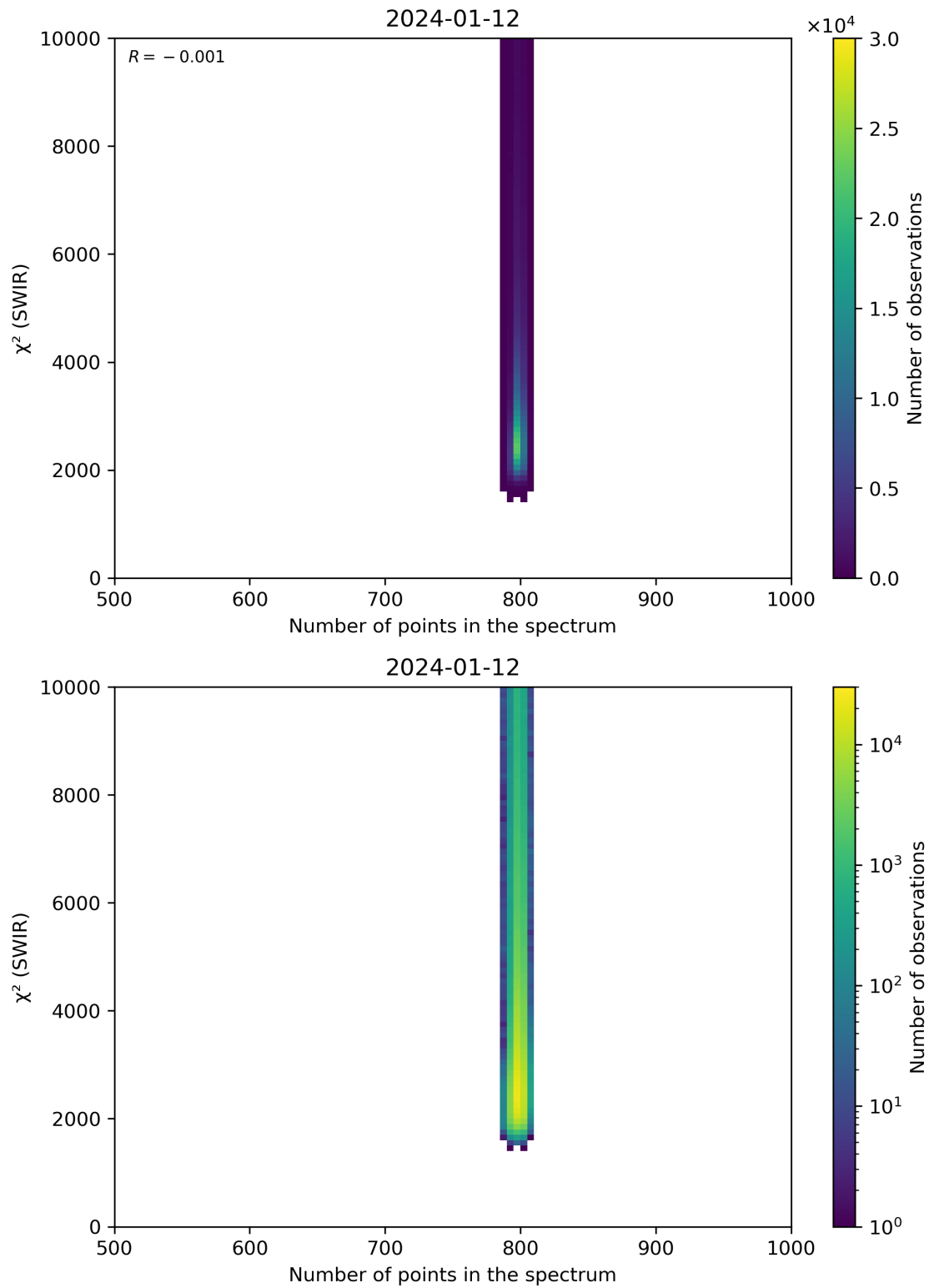
Figure 89: Scatter density plot of “Number of points in the spectrum” against “ \chi^2 (SWIR)” for 2024-01-11 to 2024-01-13.
