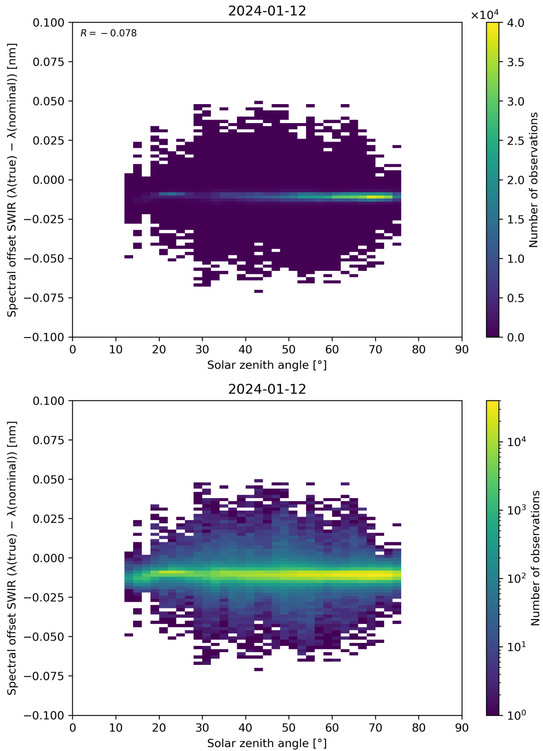
Figure 104: Scatter density plot of “Solar zenith angle” against “Spectral offset SWIR ( \lambda(\text{true}) - \lambda(\text{nominal}) )” for 2024-01-11 to 2024-01-13.
