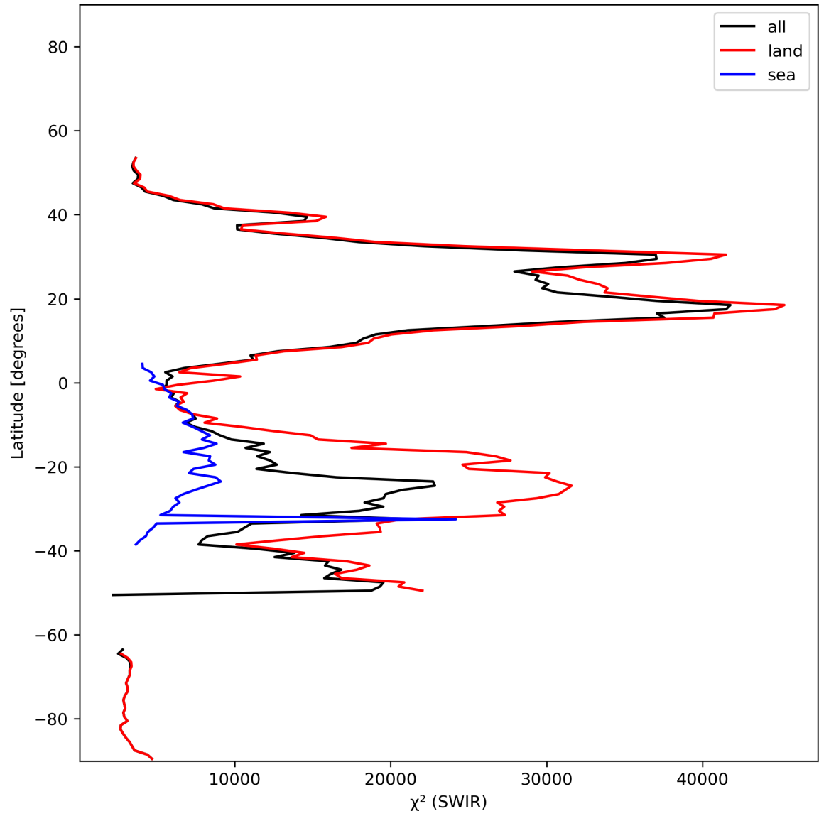
Figure 17: Zonal average of “ \chi^2 (SWIR)” for 2024-01-11 to 2024-01-13.
