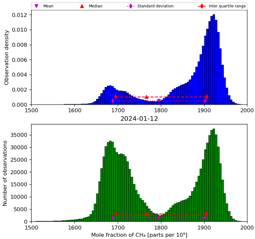
Figure 23: Histogram of “Mole fraction of CH 4 ” for 2024-01-11 to 2024-01-13
