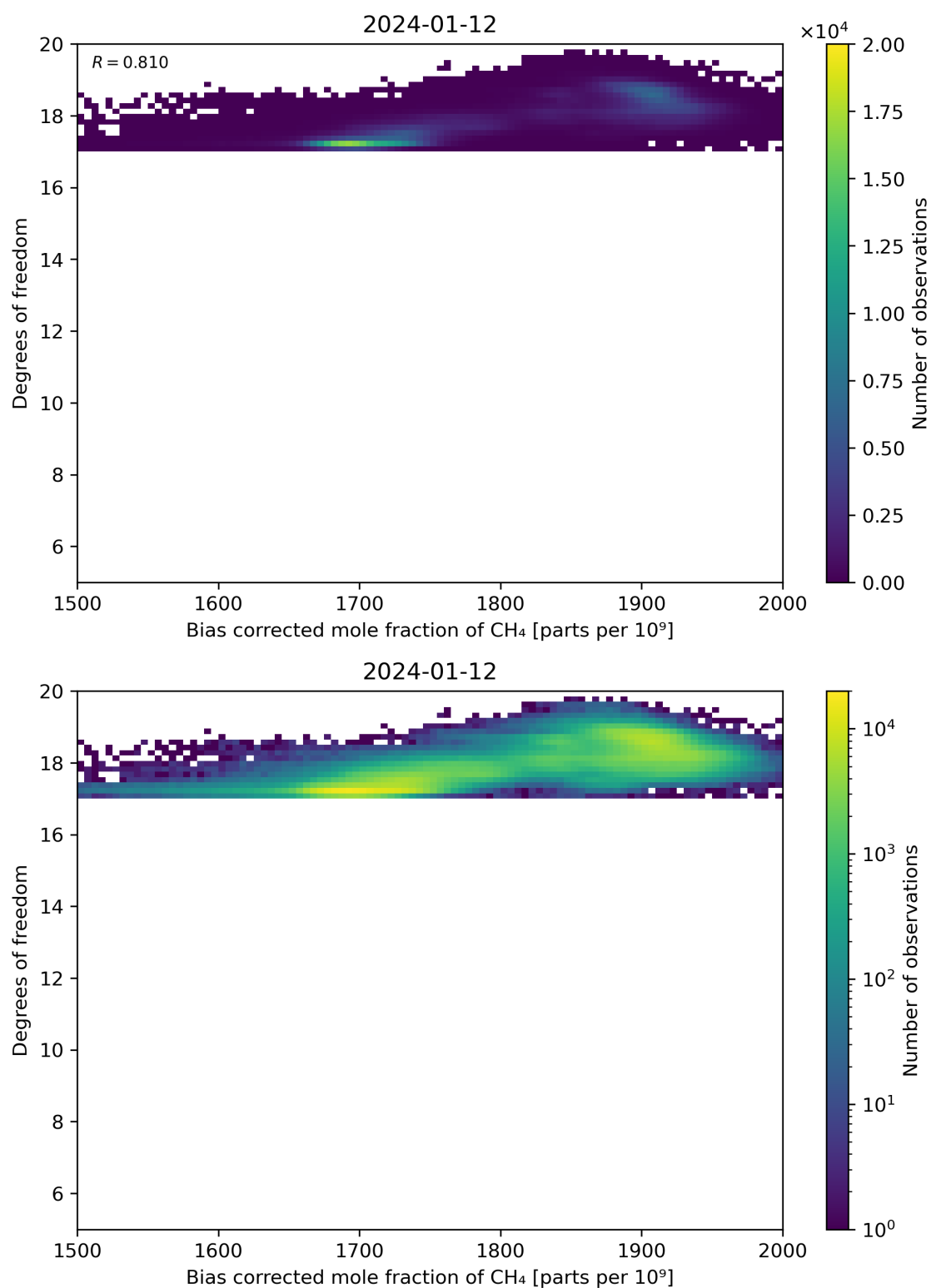
Figure 65: Scatter density plot of “Bias corrected mole fraction of CH 4 ” against “Degrees of freedom” for 2024-01-11 to 2024-01-13.
