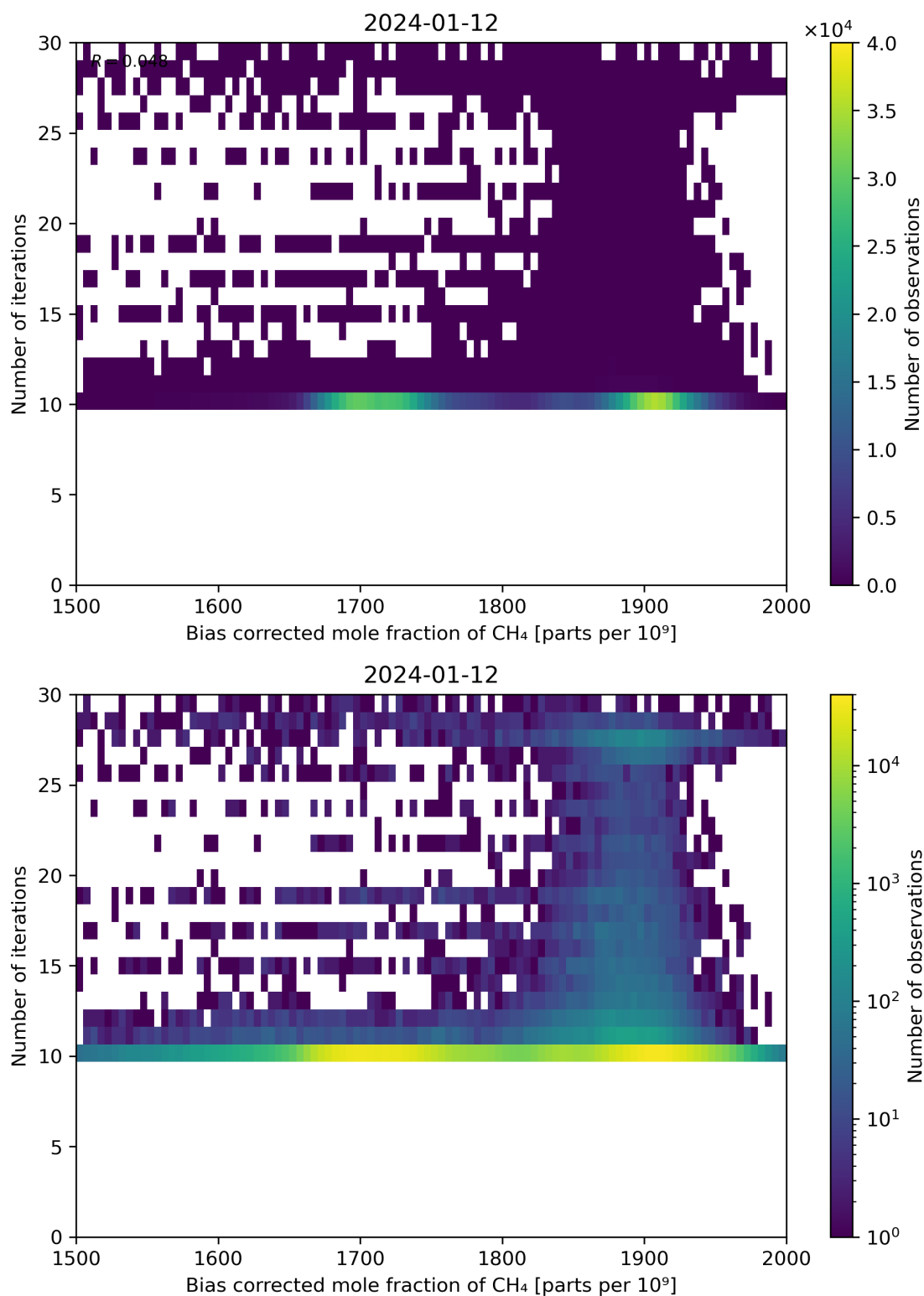
Figure 67: Scatter density plot of “Bias corrected mole fraction of \text{CH}_4 ” against “Number of iterations” for 2024-01-11 to 2024-01-13.
