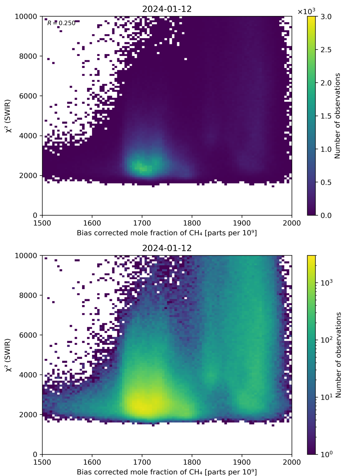
Figure 64: Scatter density plot of “Bias corrected mole fraction of \text{CH}_4 ” against “ \chi^2 (SWIR)” for 2024-01-11 to 2024-01-13.
