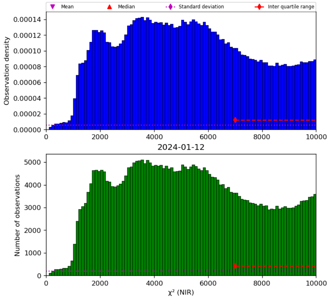
Figure 29: Histogram of “ \chi^2 (NIR)” for 2024-01-11 to 2024-01-13
