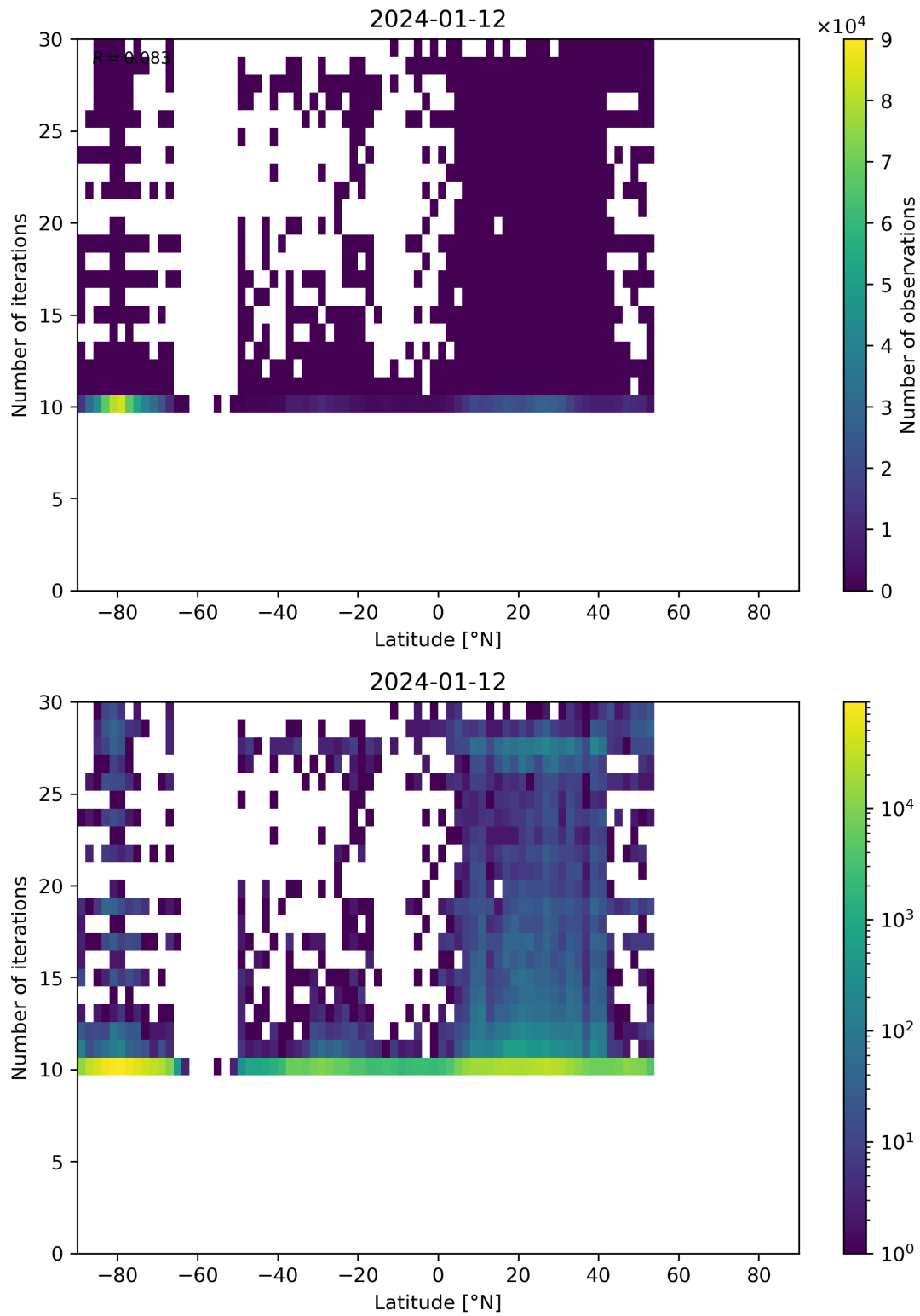
Figure 60: Scatter density plot of “Latitude” against “Number of iterations” for 2024-01-11 to 2024-01-13.
