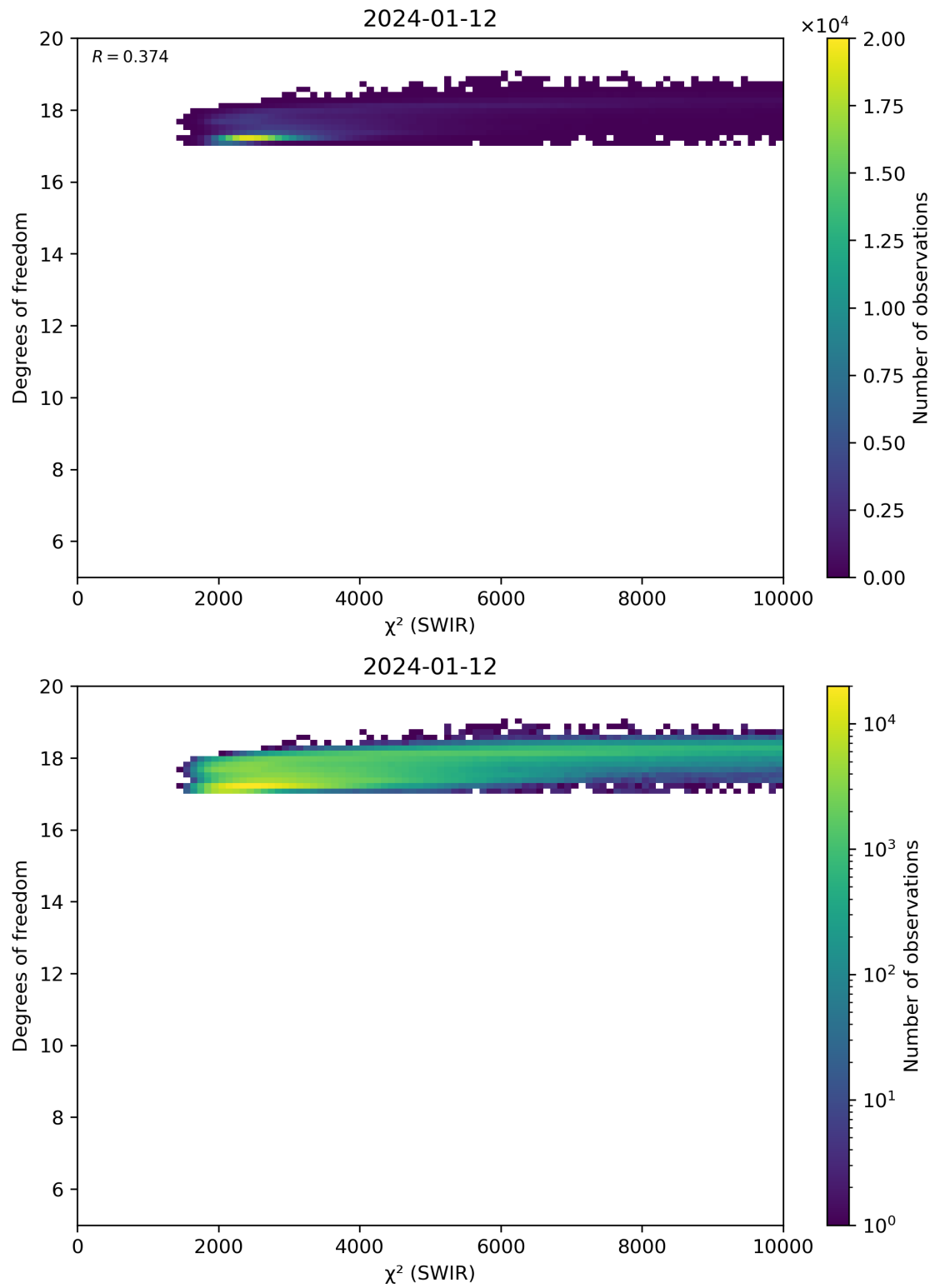
Figure 48: Scatter density plot of “ \chi^2 (SWIR)” against “Degrees of freedom” for 2024-01-11 to 2024-01-13.
