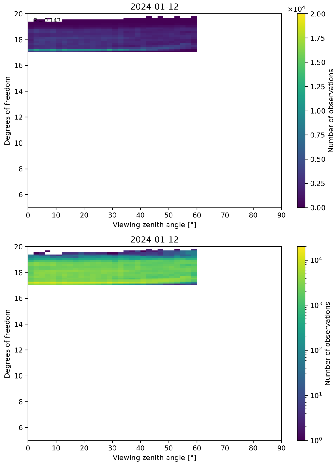
Figure 107: Scatter density plot of “Viewing zenith angle” against “Degrees of freedom” for 2024-01-11 to 2024-01-13.
