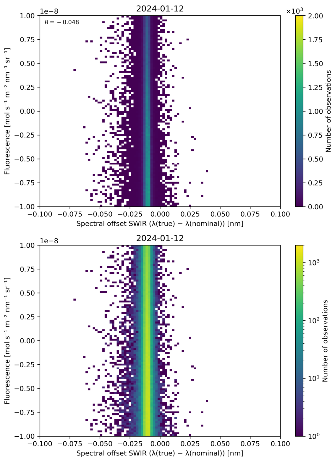
Figure 120: Scatter density plot of “Spectral offset SWIR ( \lambda(\text{true}) - \lambda(\text{nominal}) )” against “Fluorescence” for 2024-01-11 to 2024-01-13.
