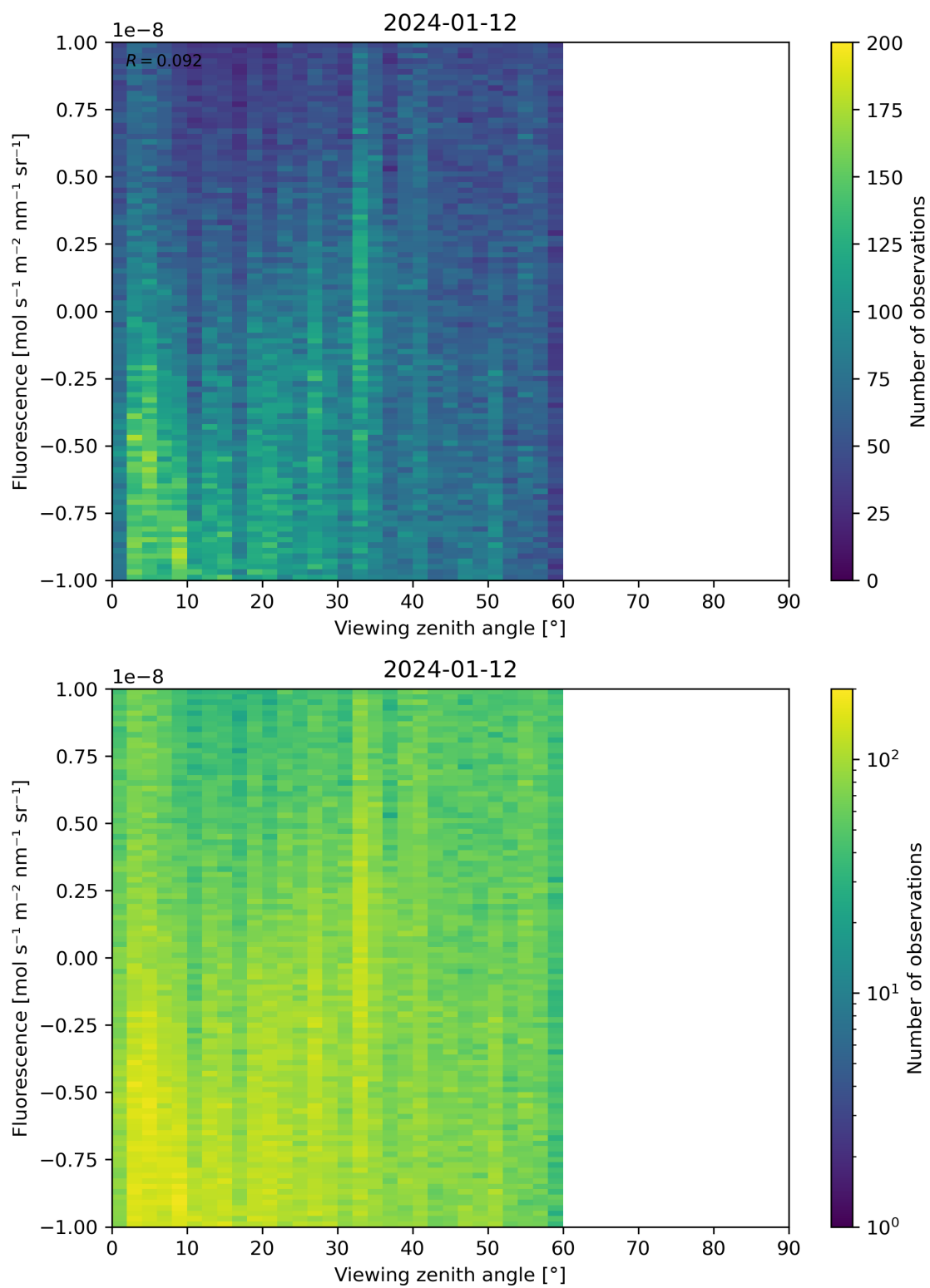
Figure 108: Scatter density plot of “Viewing zenith angle” against “Fluorescence” for 2024-01-11 to 2024-01-13.
