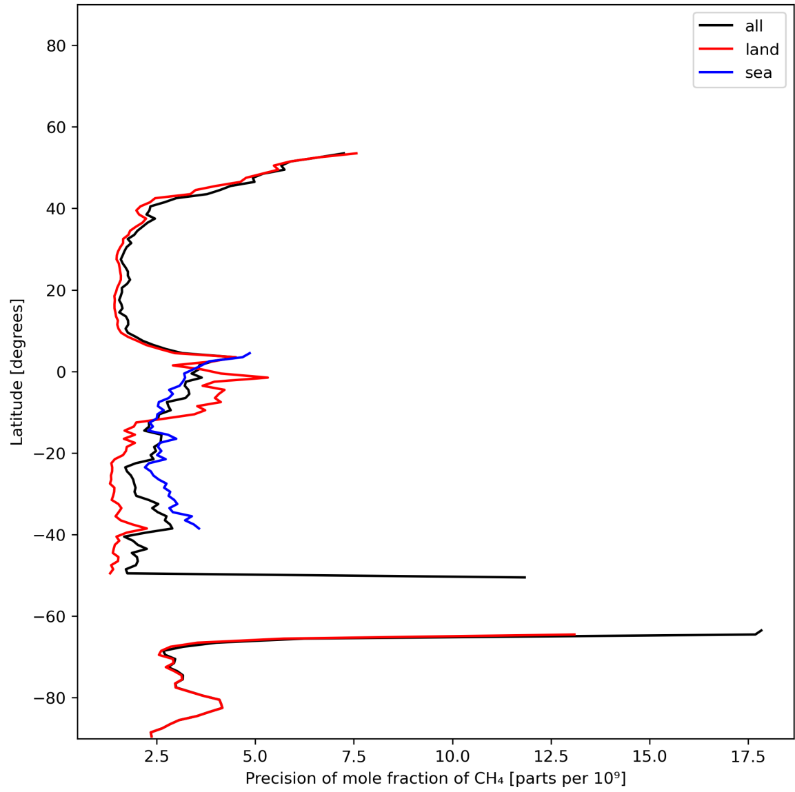
Figure 13: Zonal average of “Precision of mole fraction of CH 4 ” for 2024-01-11 to 2024-01-13.
