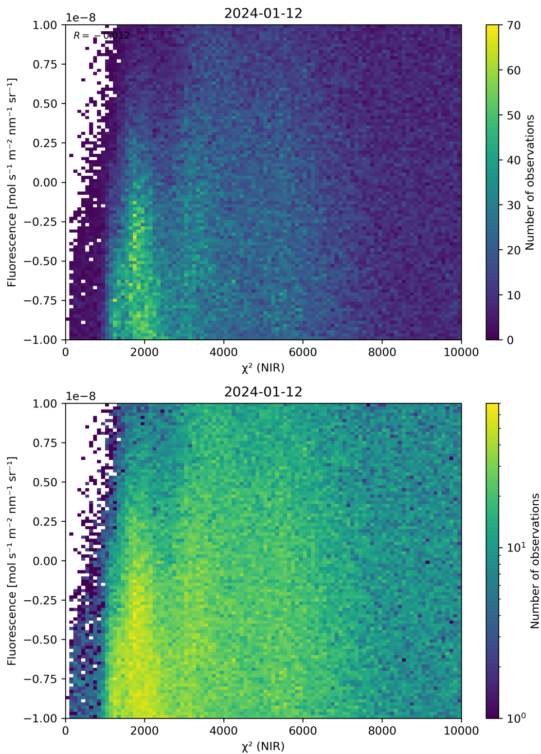
Figure 45: Scatter density plot of “ \chi^2 (NIR)” against “Fluorescence” for 2024-01-11 to 2024-01-13.
