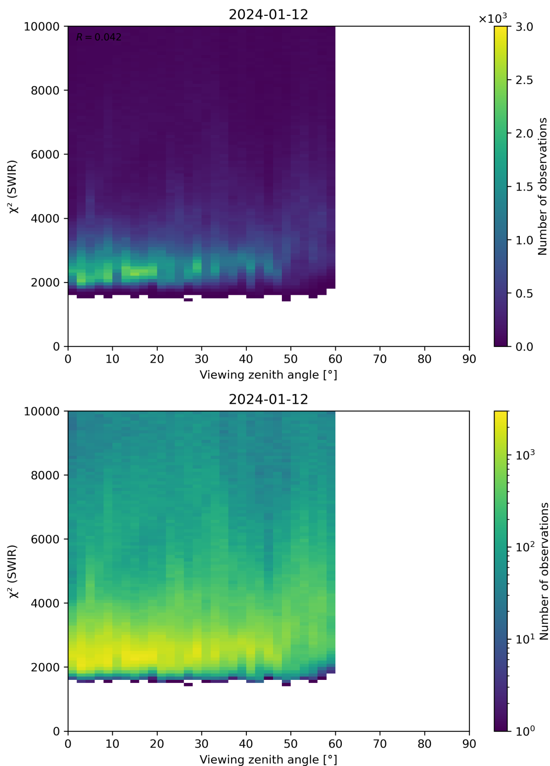
Figure 106: Scatter density plot of “Viewing zenith angle” against “ \chi^2 (SWIR)” for 2024-01-11 to 2024-01-13.
