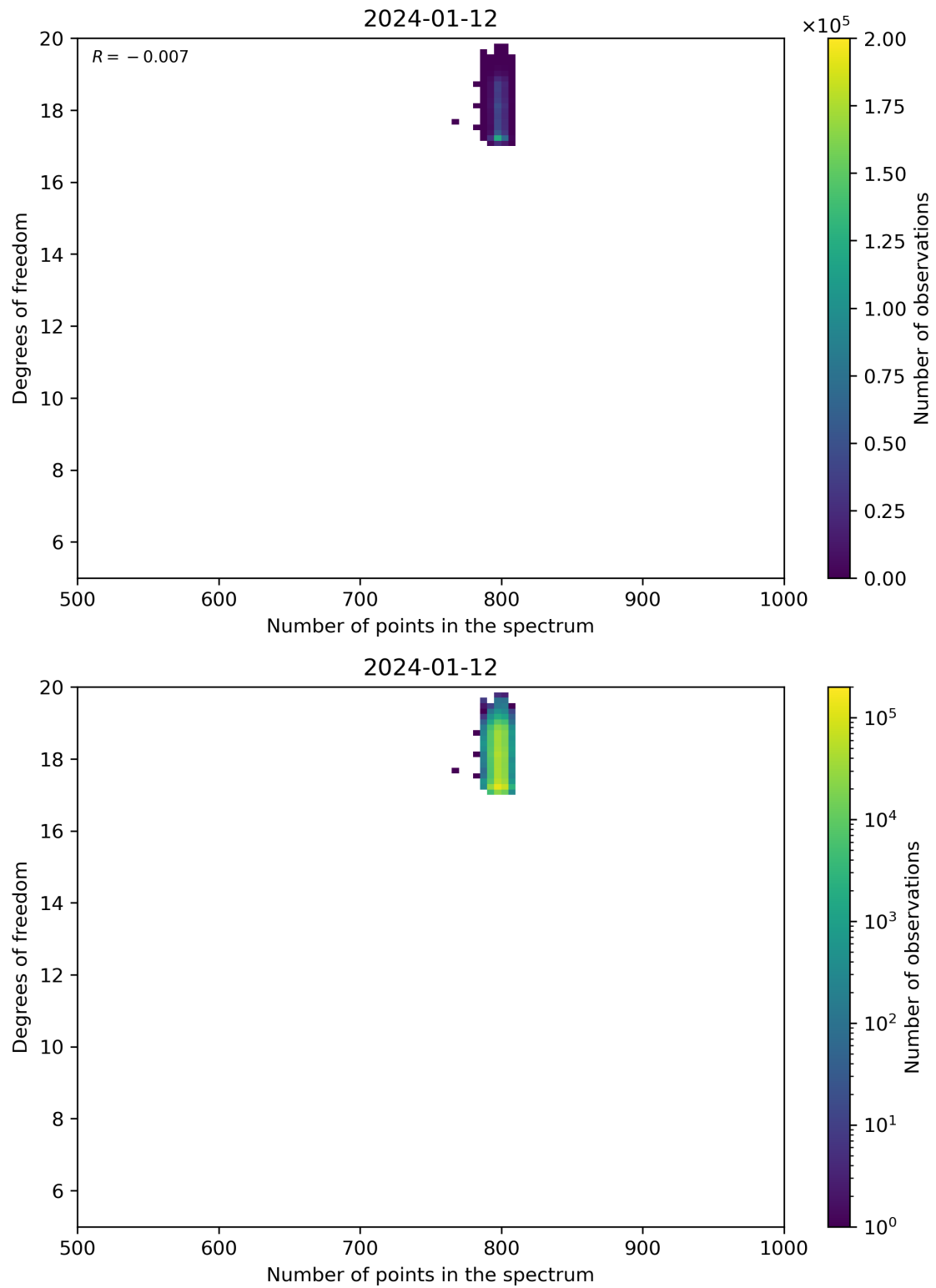
Figure 90: Scatter density plot of “Number of points in the spectrum” against “Degrees of freedom” for 2024-01-11 to 2024-01-13.
