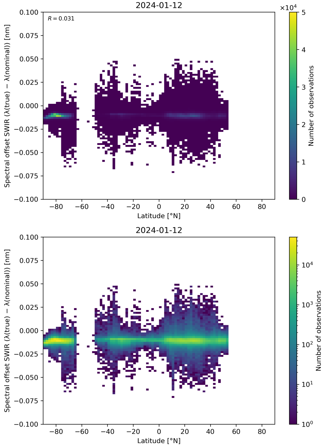
Figure 62: Scatter density plot of “Latitude” against “Spectral offset SWIR ( \lambda(\text{true}) - \lambda(\text{nominal}) )” for 2024-01-11 to 2024-01-13.
