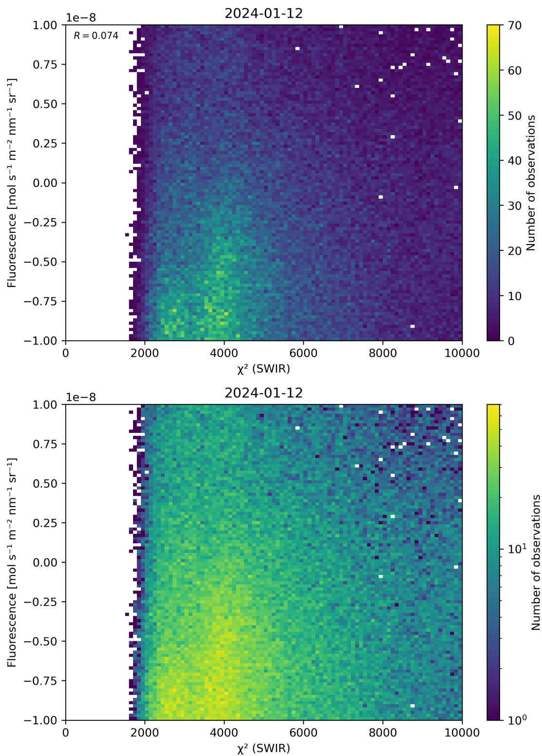
Figure 49: Scatter density plot of “ \chi^2 (SWIR)” against “Fluorescence” for 2024-01-11 to 2024-01-13.
