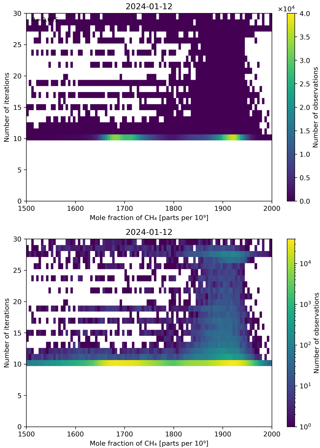
Figure 76: Scatter density plot of “Mole fraction of CH 4 ” against “Number of iterations” for 2024-01-11 to 2024-01-13.
