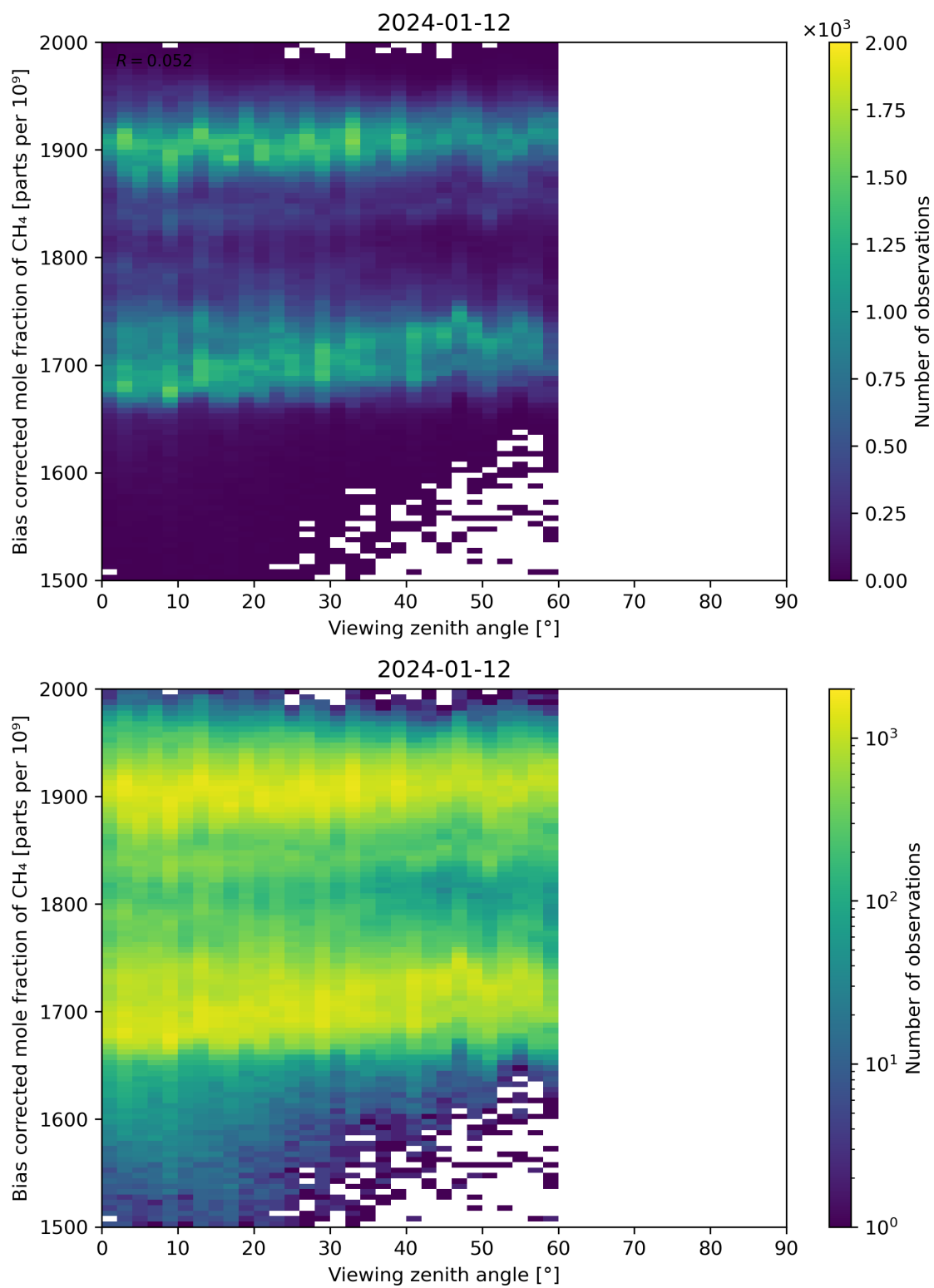
Figure 111: Scatter density plot of “Viewing zenith angle” against “Bias corrected mole fraction of CH 4 ” for 2024-01-11 to 2024-01-13.
