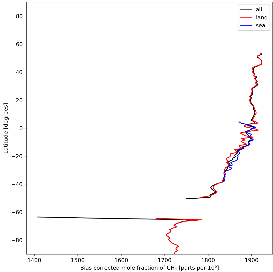
Figure 14: Zonal average of “Bias corrected mole fraction of CH 4 ” for 2024-01-11 to 2024-01-13.
