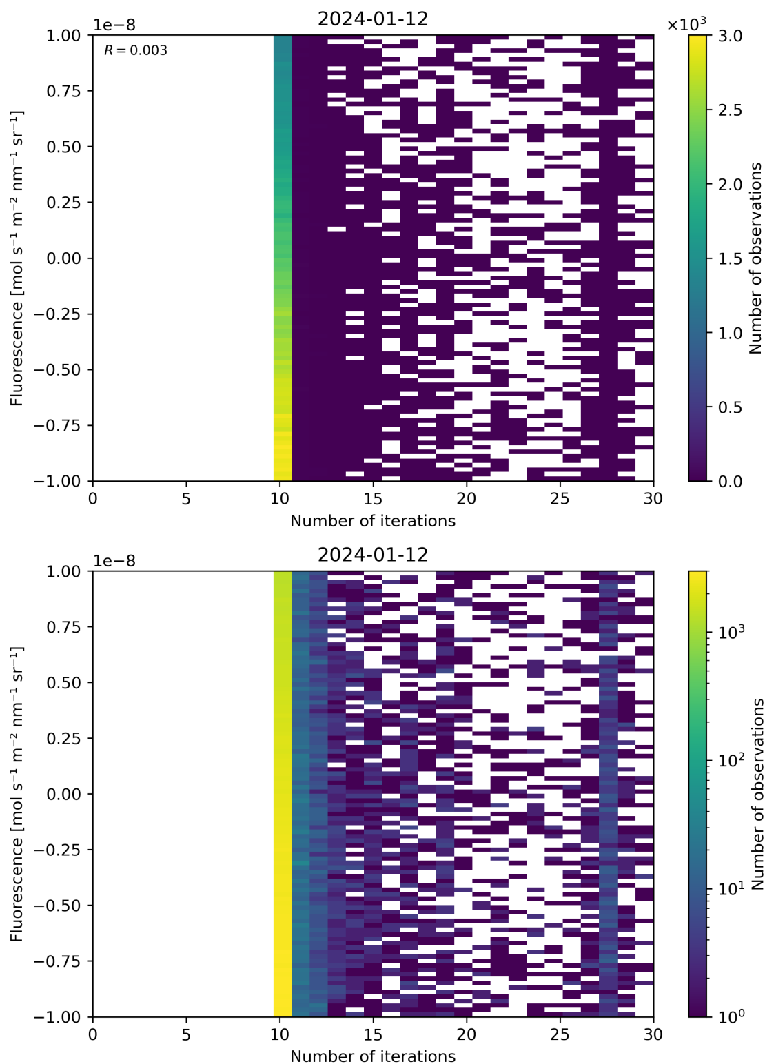
Figure 87: Scatter density plot of “Number of iterations” against “Fluorescence” for 2024-01-11 to 2024-01-13.
