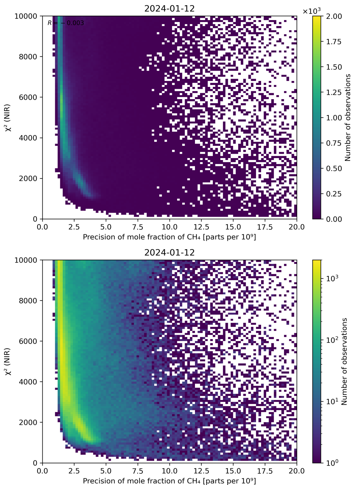
Figure 78: Scatter density plot of “Precision of mole fraction of CH 4 ” against “ \chi^2 (NIR)” for 2024-01-11 to 2024-01-13.
