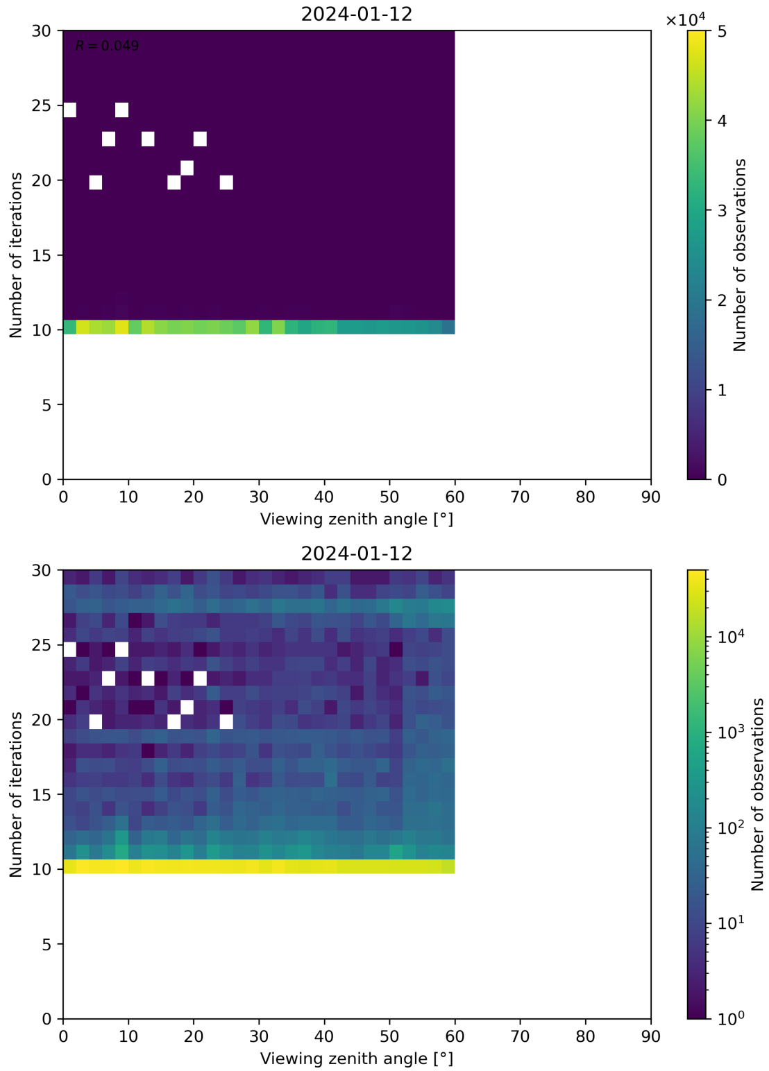
Figure 113: Scatter density plot of “Viewing zenith angle” against “Number of iterations” for 2024-01-11 to 2024-01-13.
