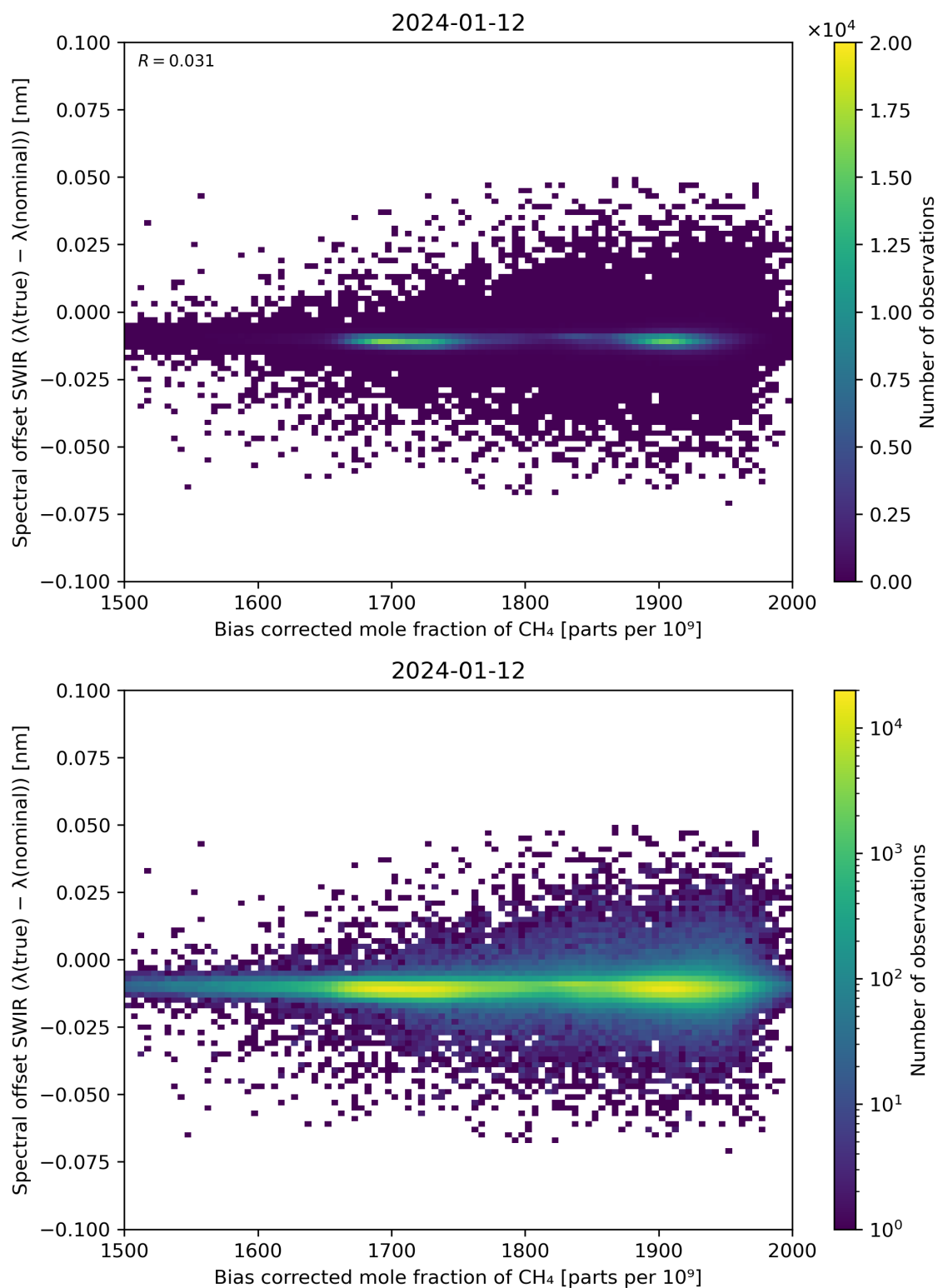
Figure 69: Scatter density plot of “Bias corrected mole fraction of \text{CH}_4 ” against “Spectral offset SWIR ( \lambda(\text{true}) - \lambda(\text{nominal}) )” for 2024-01-11 to 2024-01-13.
