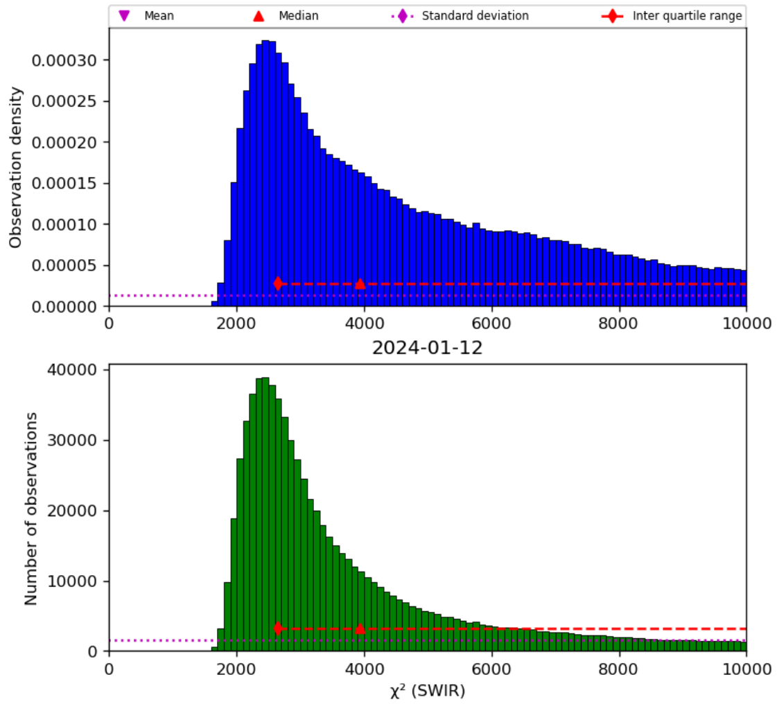
Figure 28: Histogram of “ \chi^2 (SWIR)” for 2024-01-11 to 2024-01-13
