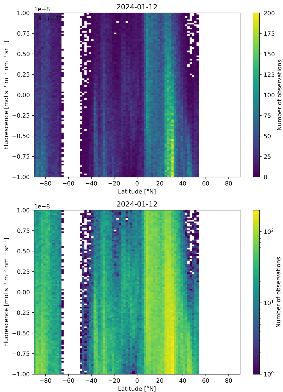
Figure 56: Scatter density plot of “Latitude” against “Fluorescence” for 2024-01-11 to 2024-01-13.
