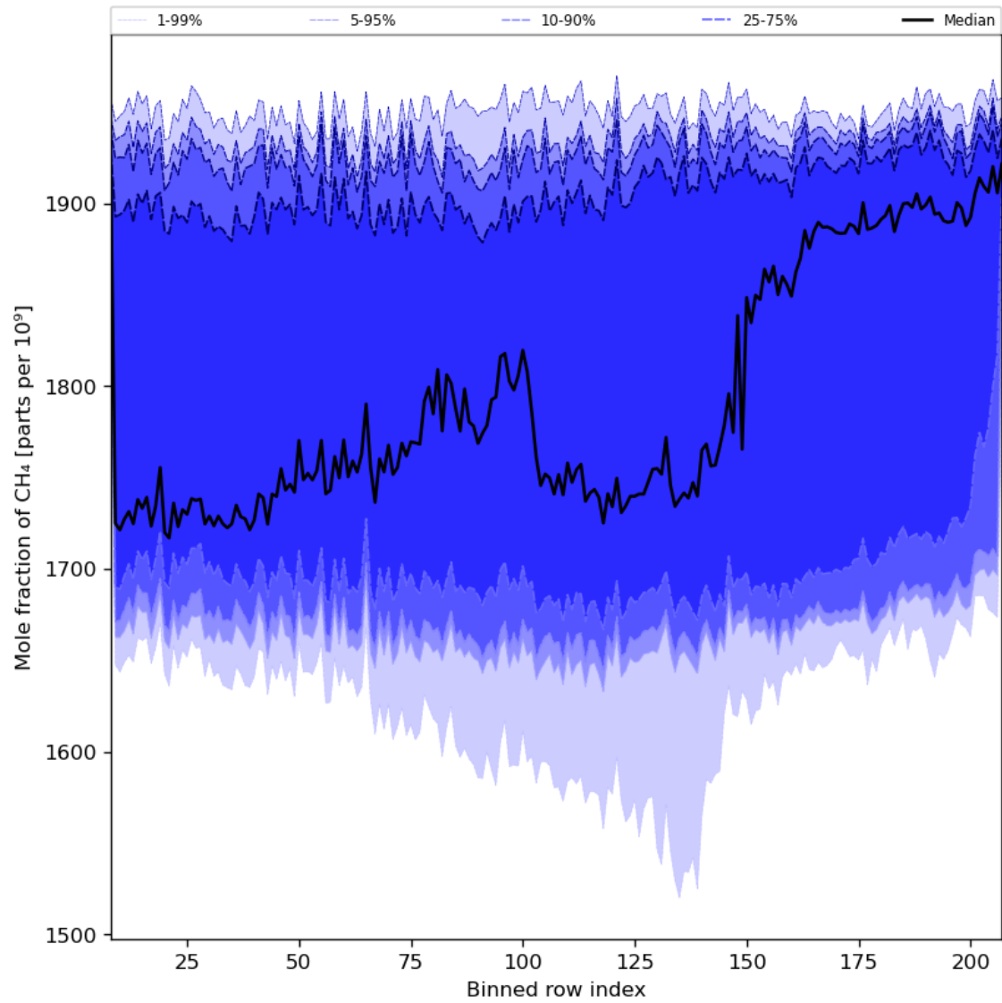
Figure 34: Along track statistics of “Mole fraction of CH 4 ” for 2024-01-11 to 2024-01-13
