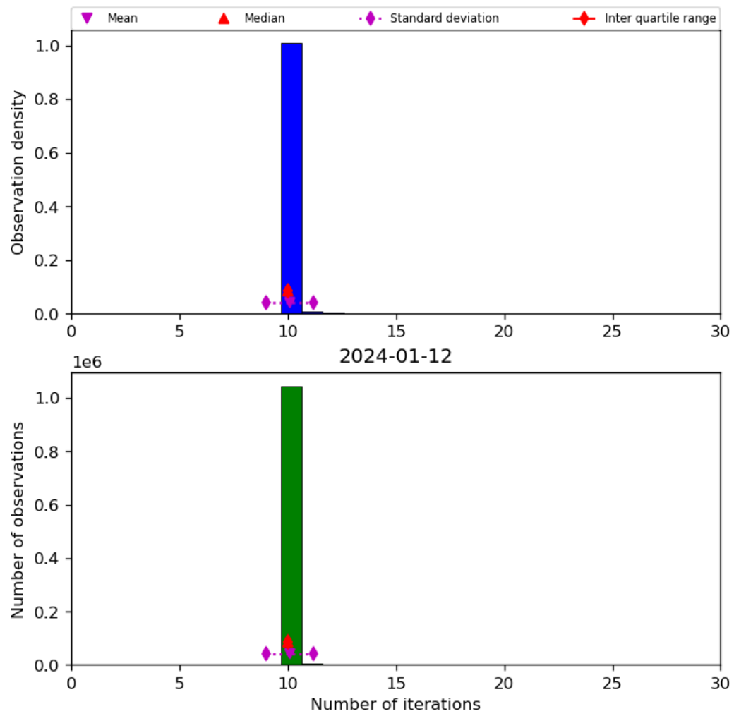
Figure 31: Histogram of “Number of iterations” for 2024-01-11 to 2024-01-13
