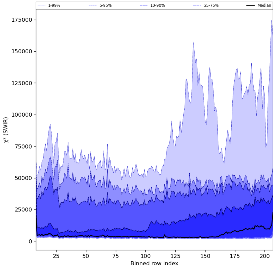
Figure 39: Along track statistics of “ \chi^2 (SWIR)” for 2024-01-11 to 2024-01-13
