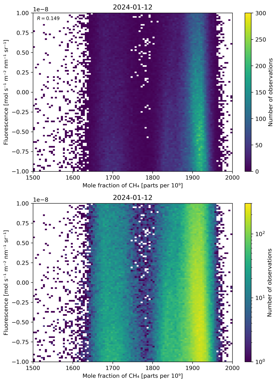
Figure 73: Scatter density plot of “Mole fraction of \text{CH}_4 ” against “Fluorescence” for 2024-01-11 to 2024-01-13.
