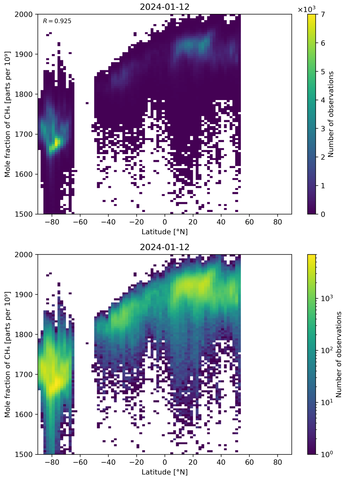
Figure 57: Scatter density plot of “Latitude” against “Mole fraction of \text{CH}_4 ” for 2024-01-11 to 2024-01-13.
