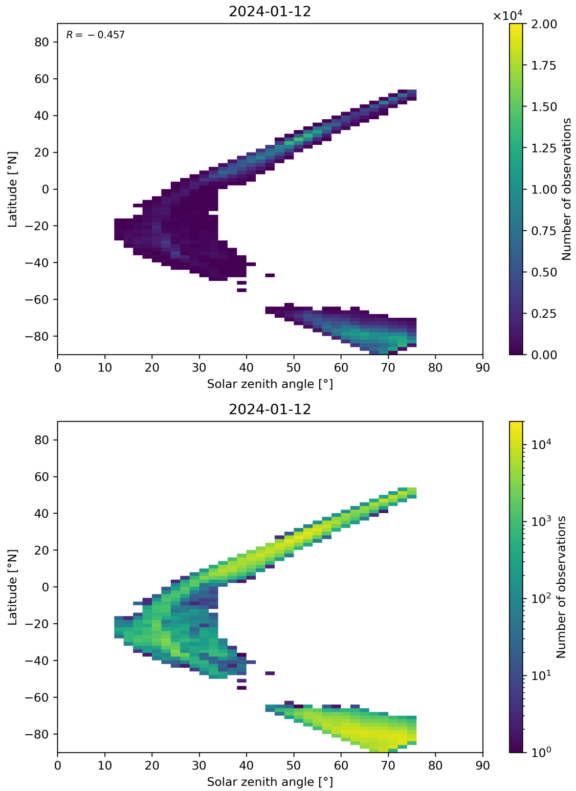
Figure 98: Scatter density plot of “Solar zenith angle” against “Latitude” for 2024-01-11 to 2024-01-13.
