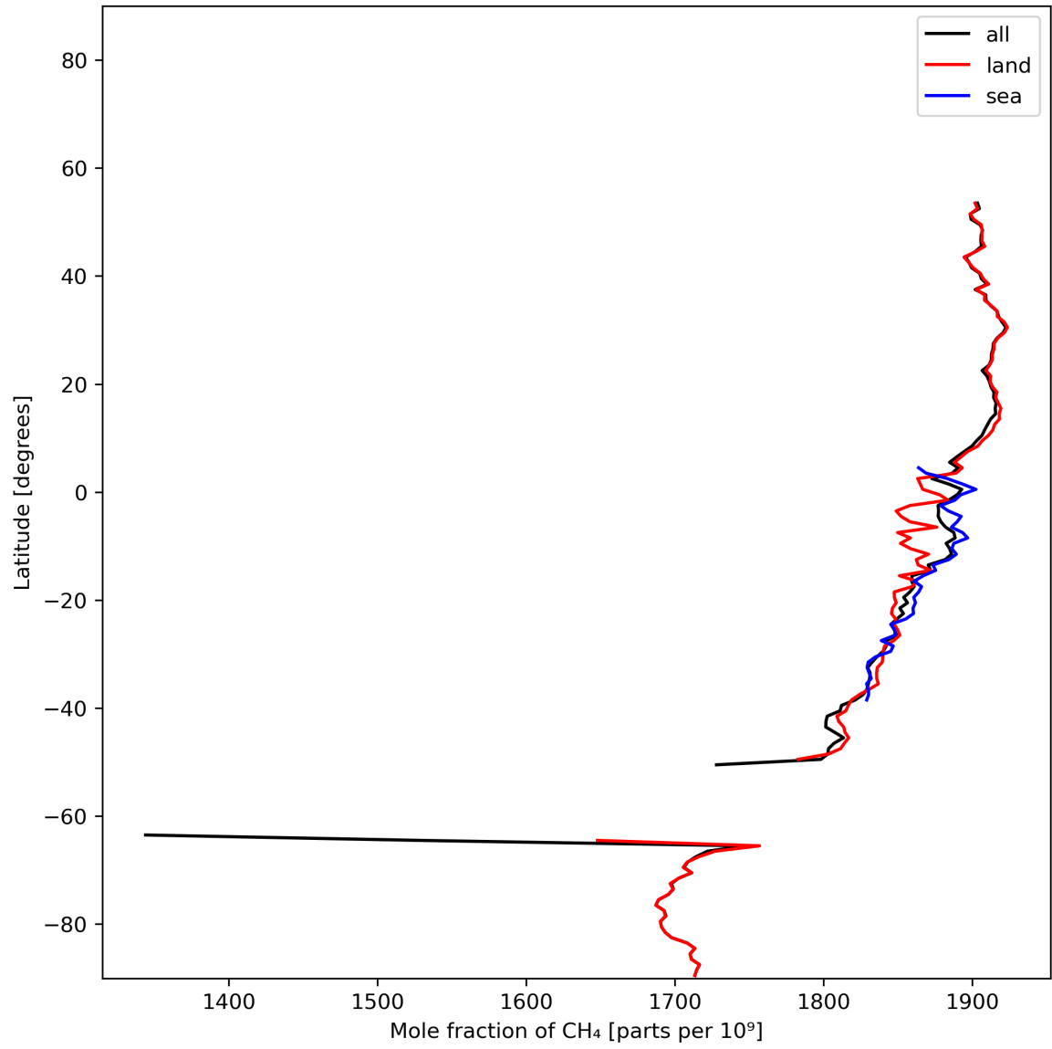
Figure 12: Zonal average of “Mole fraction of \text{CH}_4 ” for 2024-01-11 to 2024-01-13.
