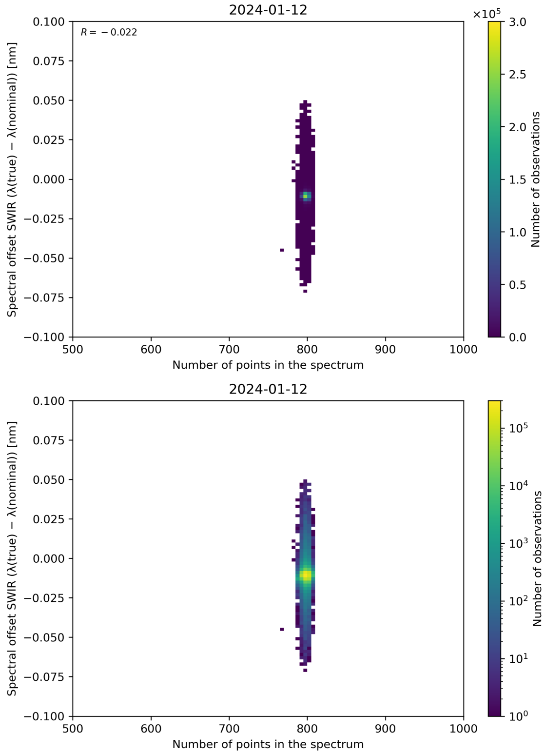
Figure 93: Scatter density plot of “Number of points in the spectrum” against “Spectral offset SWIR ( \lambda(\text{true}) - \lambda(\text{nominal}) )” for 2024-01-11 to 2024-01-13.
