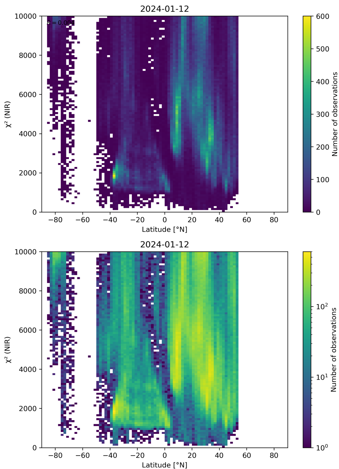
Figure 53: Scatter density plot of “Latitude” against “ \chi^2 (NIR)” for 2024-01-11 to 2024-01-13.
