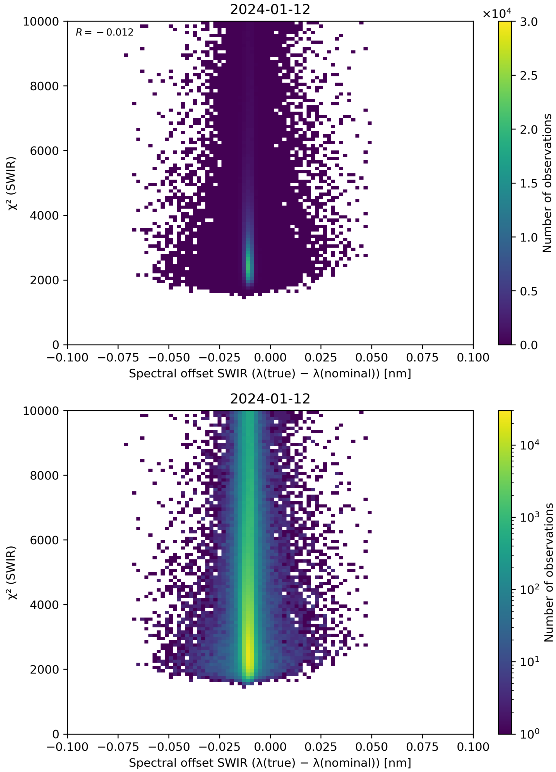
Figure 118: Scatter density plot of “Spectral offset SWIR ( \lambda(\text{true}) - \lambda(\text{nominal}) )” against “ \chi^2 (SWIR)” for 2024-01-11 to 2024-01-13.
