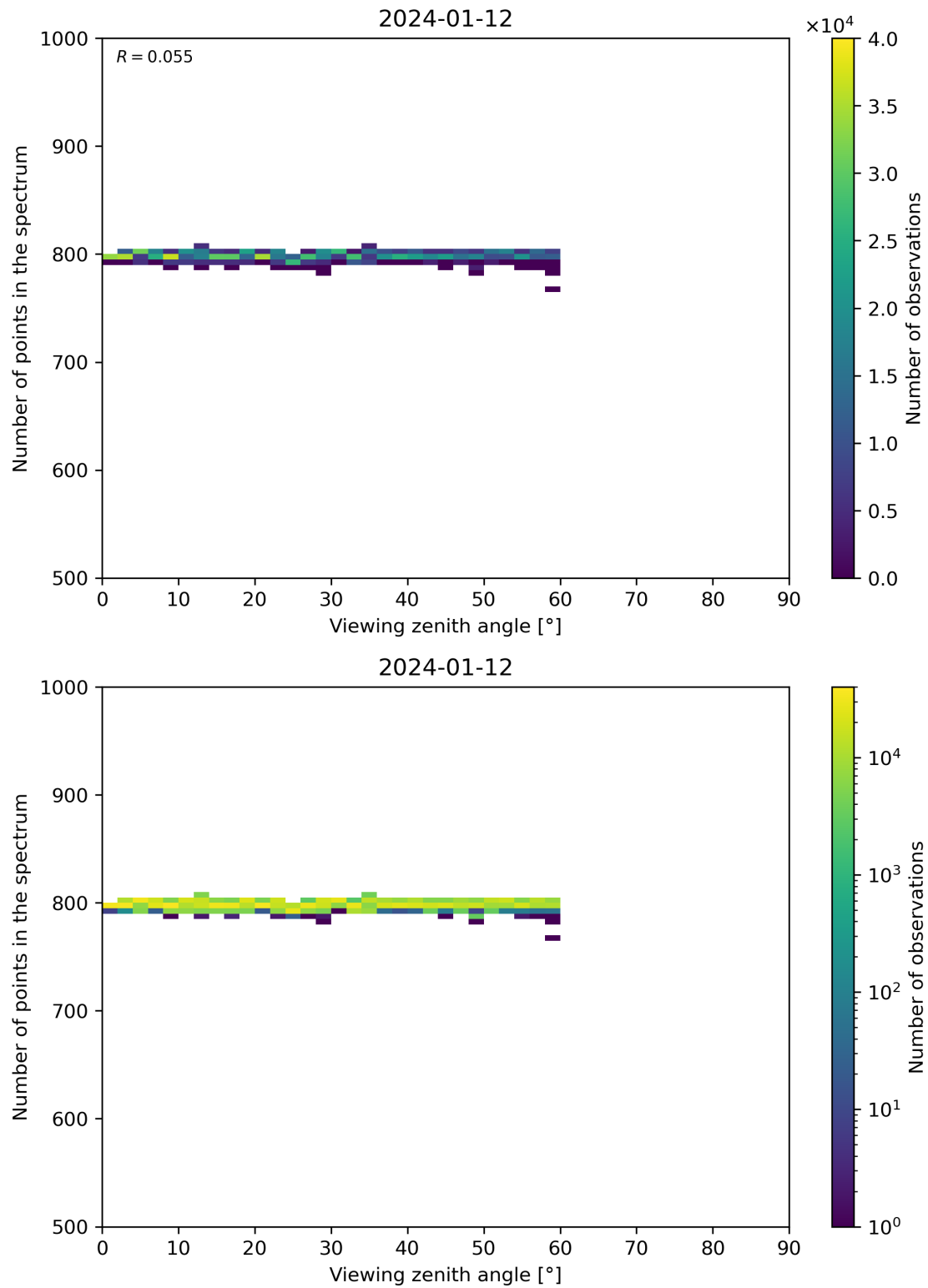
Figure 114: Scatter density plot of “Viewing zenith angle” against “Number of points in the spectrum” for 2024-01-11 to 2024-01-13.
