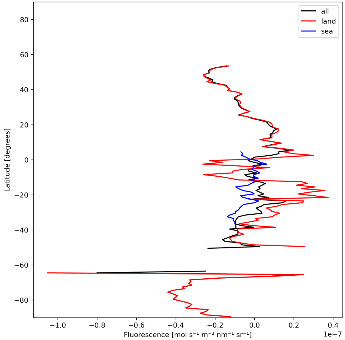
Figure 21: Zonal average of “Fluorescence” for 2024-01-11 to 2024-01-13.
