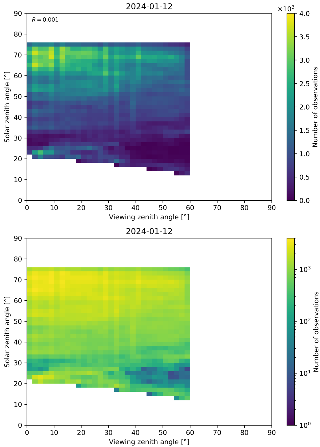
Figure 115: Scatter density plot of “Viewing zenith angle” against “Solar zenith angle” for 2024-01-11 to 2024-01-13.
