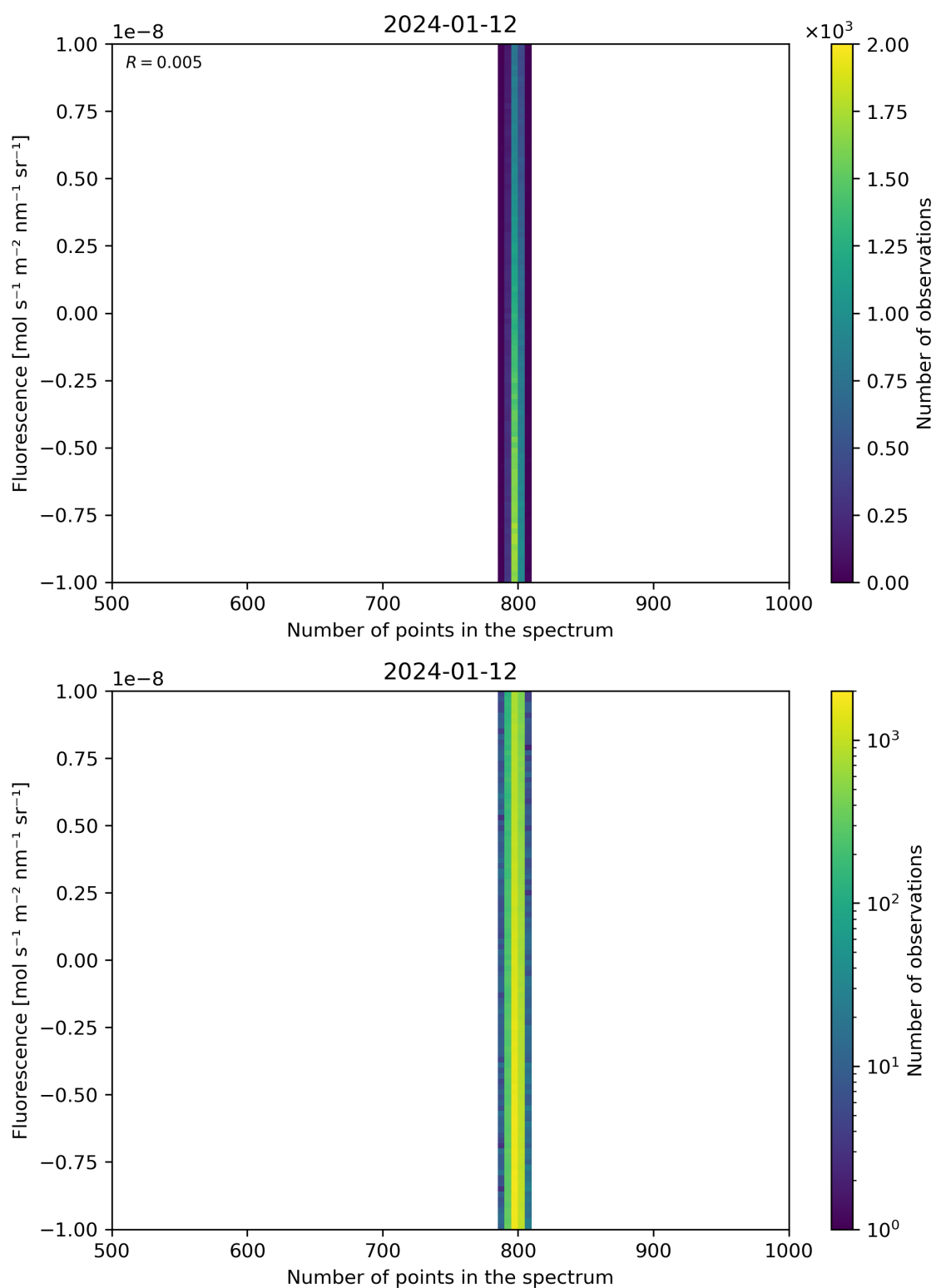
Figure 91: Scatter density plot of “Number of points in the spectrum” against “Fluorescence” for 2024-01-11 to 2024-01-13.
