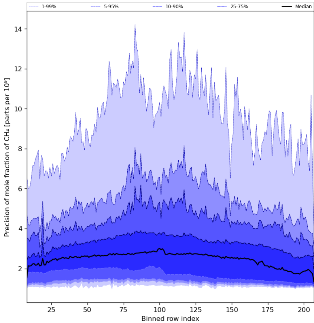
Figure 35: Along track statistics of “Precision of mole fraction of CH 4 ” for 2024-01-11 to 2024-01-13
