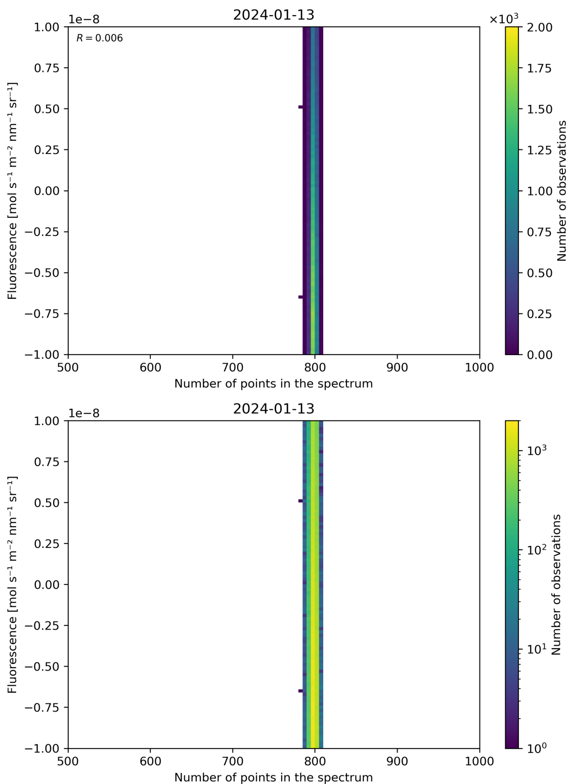
Figure 91: Scatter density plot of “Number of points in the spectrum” against “Fluorescence” for 2024-01-12 to 2024-01-14.
