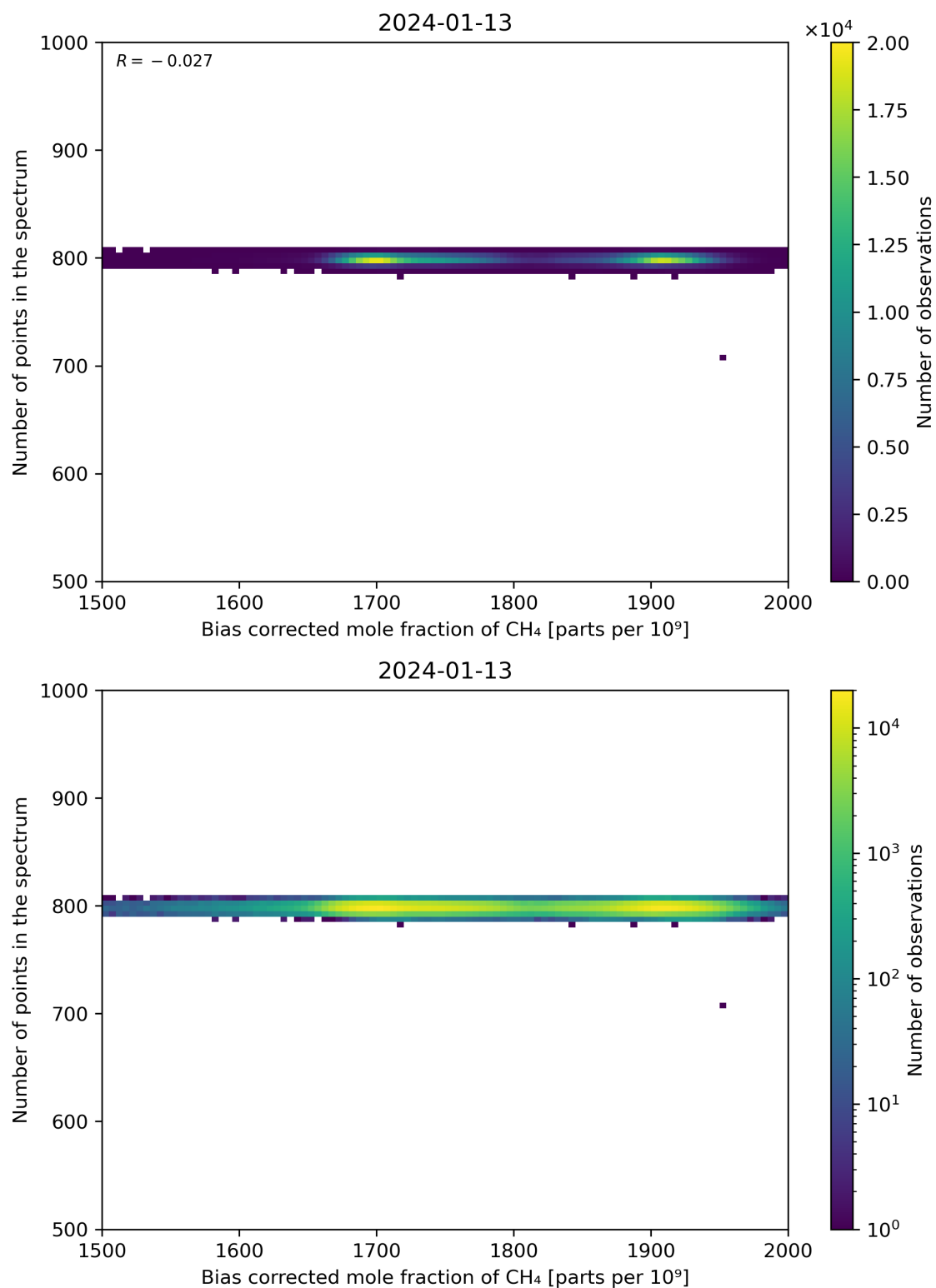
Figure 68: Scatter density plot of “Bias corrected mole fraction of CH 4 ” against “Number of points in the spectrum” for 2024-01-12 to 2024-01-14.
