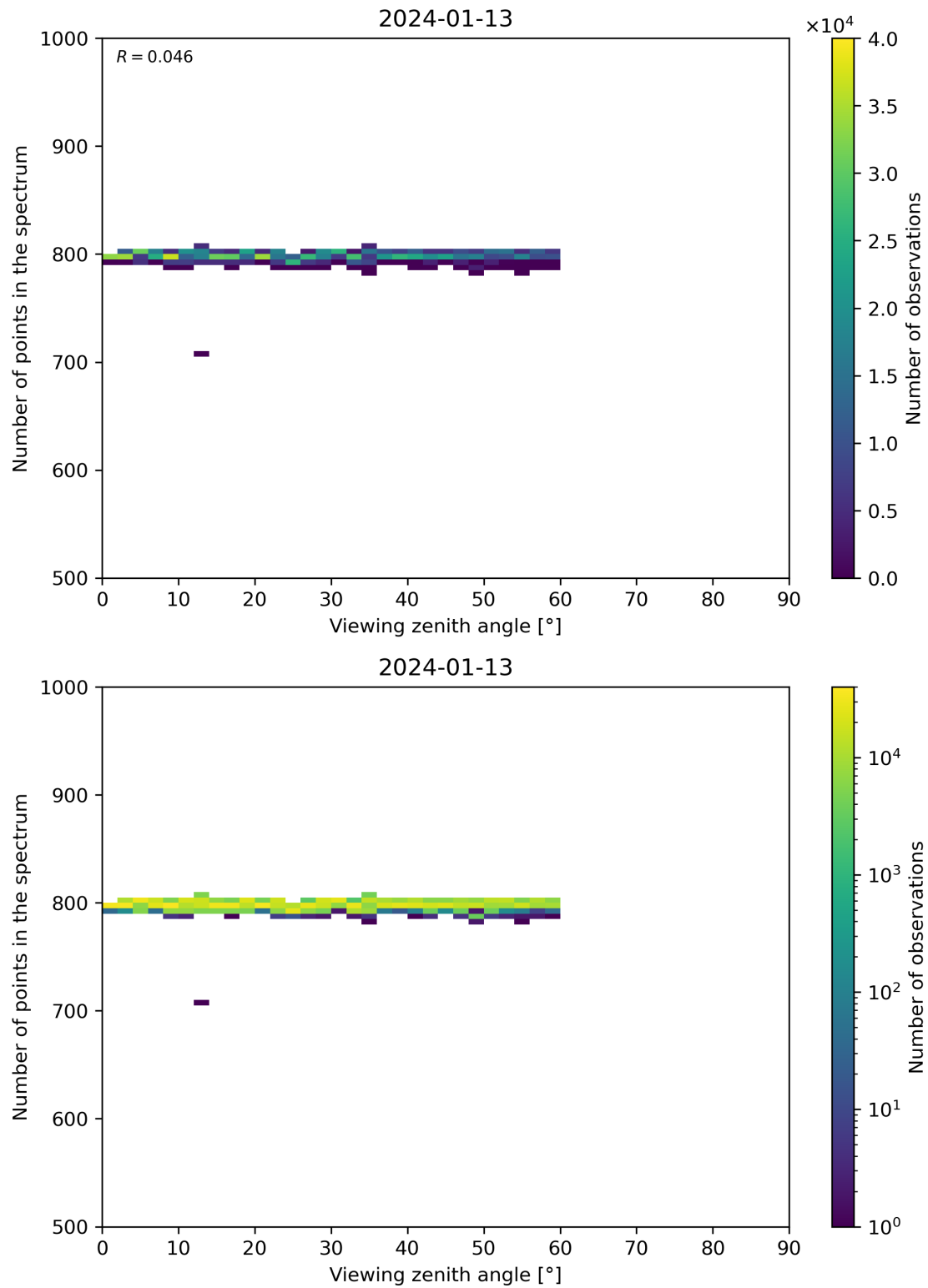
Figure 114: Scatter density plot of “Viewing zenith angle” against “Number of points in the spectrum” for 2024-01-12 to 2024-01-14.
