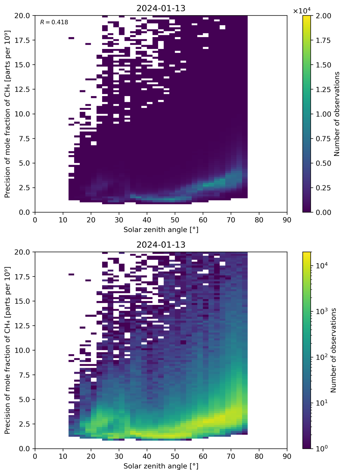
Figure 101: Scatter density plot of “Solar zenith angle” against “Precision of mole fraction of CH 4 ” for 2024-01-12 to 2024-01-14.
