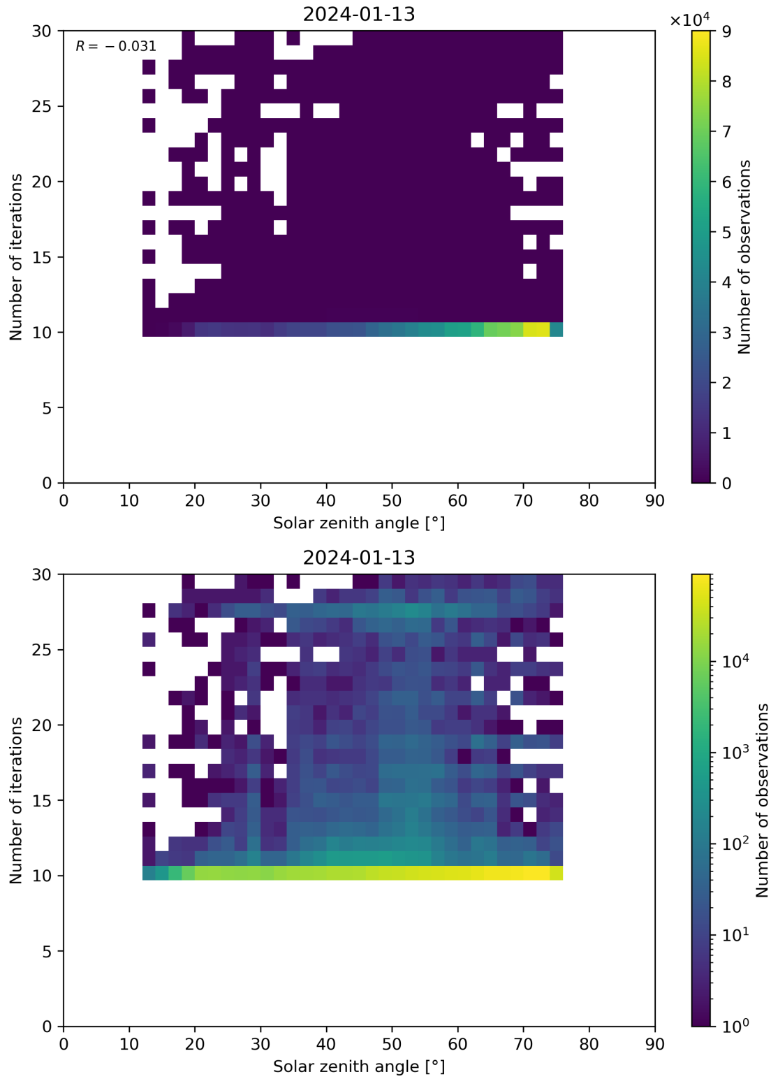
Figure 102: Scatter density plot of “Solar zenith angle” against “Number of iterations” for 2024-01-12 to 2024-01-14.
