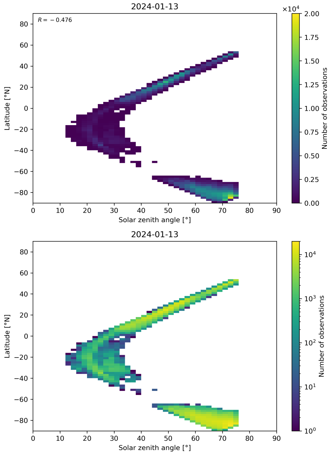
Figure 98: Scatter density plot of “Solar zenith angle” against “Latitude” for 2024-01-12 to 2024-01-14.
