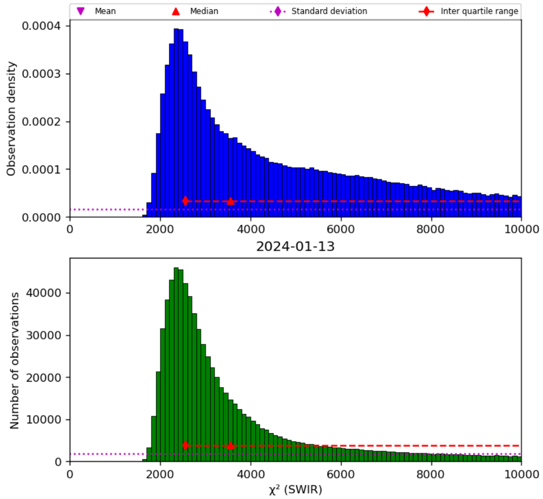
Figure 28: Histogram of “ \chi^2 (SWIR)” for 2024-01-12 to 2024-01-14
