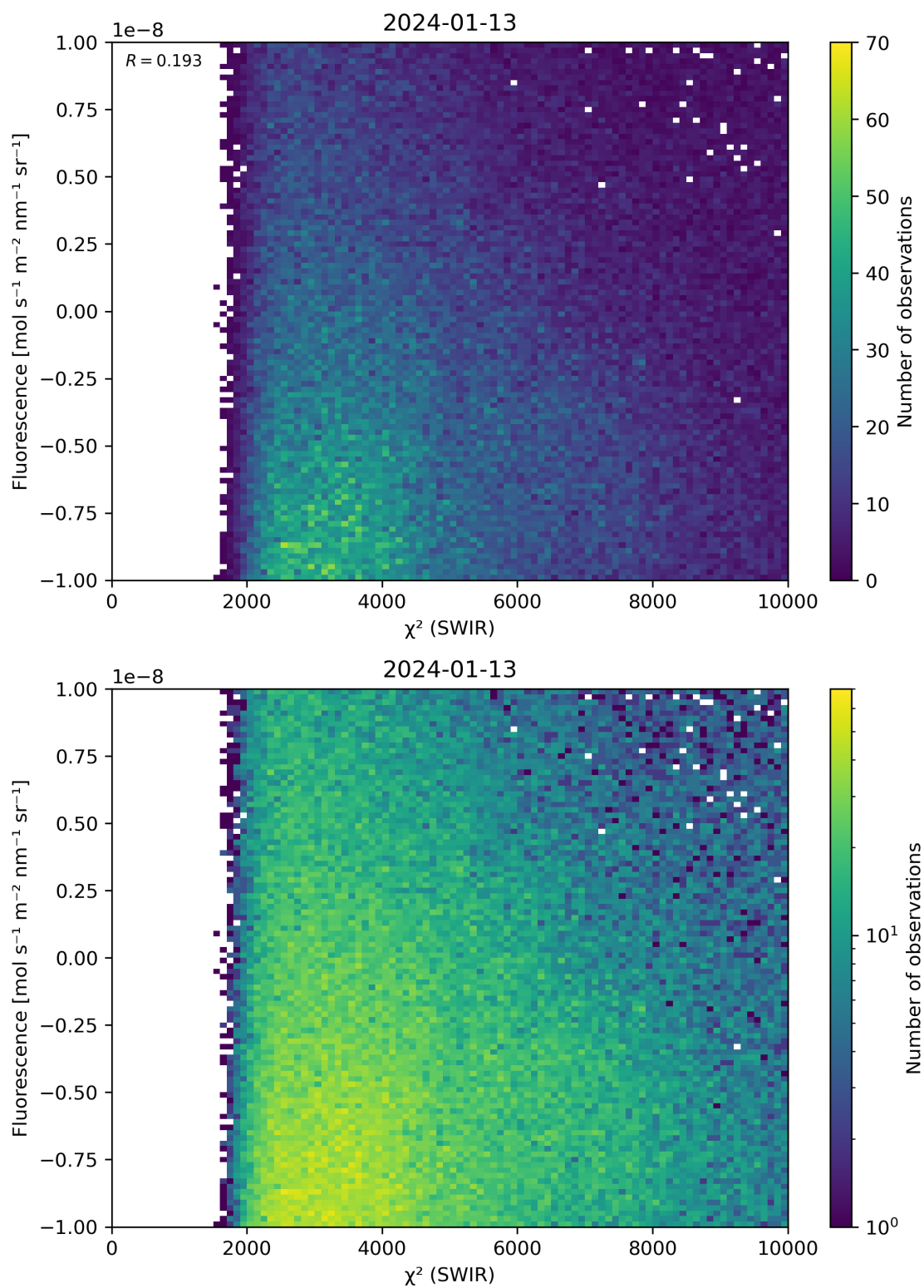
Figure 49: Scatter density plot of “ \chi^2 (SWIR)” against “Fluorescence” for 2024-01-12 to 2024-01-14.
