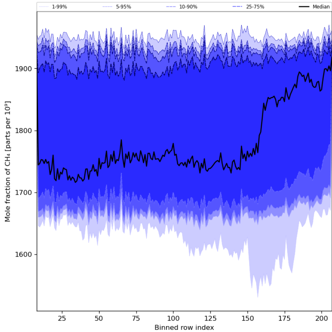
Figure 34: Along track statistics of “Mole fraction of CH 4 ” for 2024-01-12 to 2024-01-14
