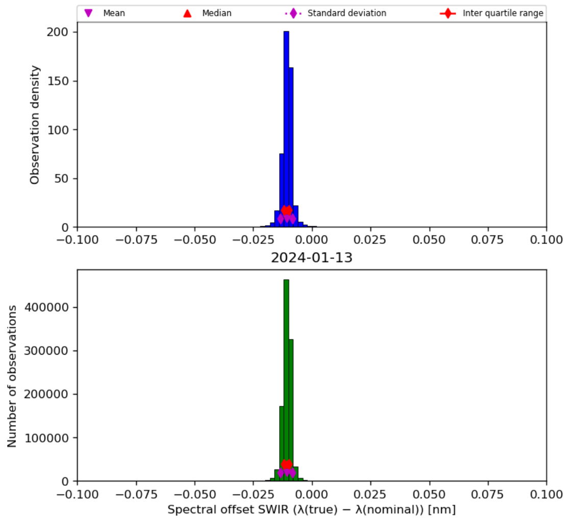
Figure 27: Histogram of “Spectral offset SWIR ( \lambda(\text{true}) - \lambda(\text{nominal}) )” for 2024-01-12 to 2024-01-14
