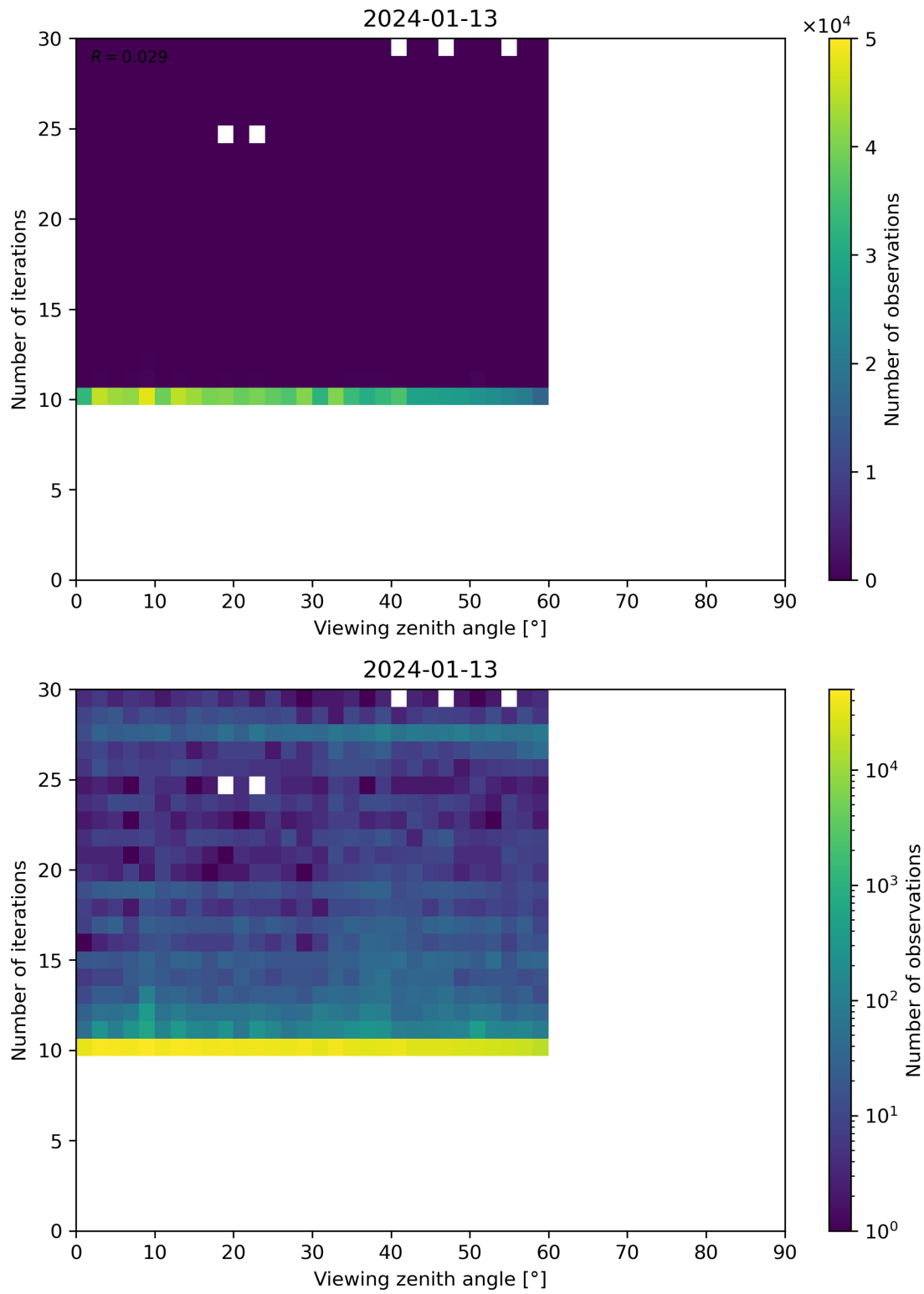
Figure 113: Scatter density plot of “Viewing zenith angle” against “Number of iterations” for 2024-01-12 to 2024-01-14.
