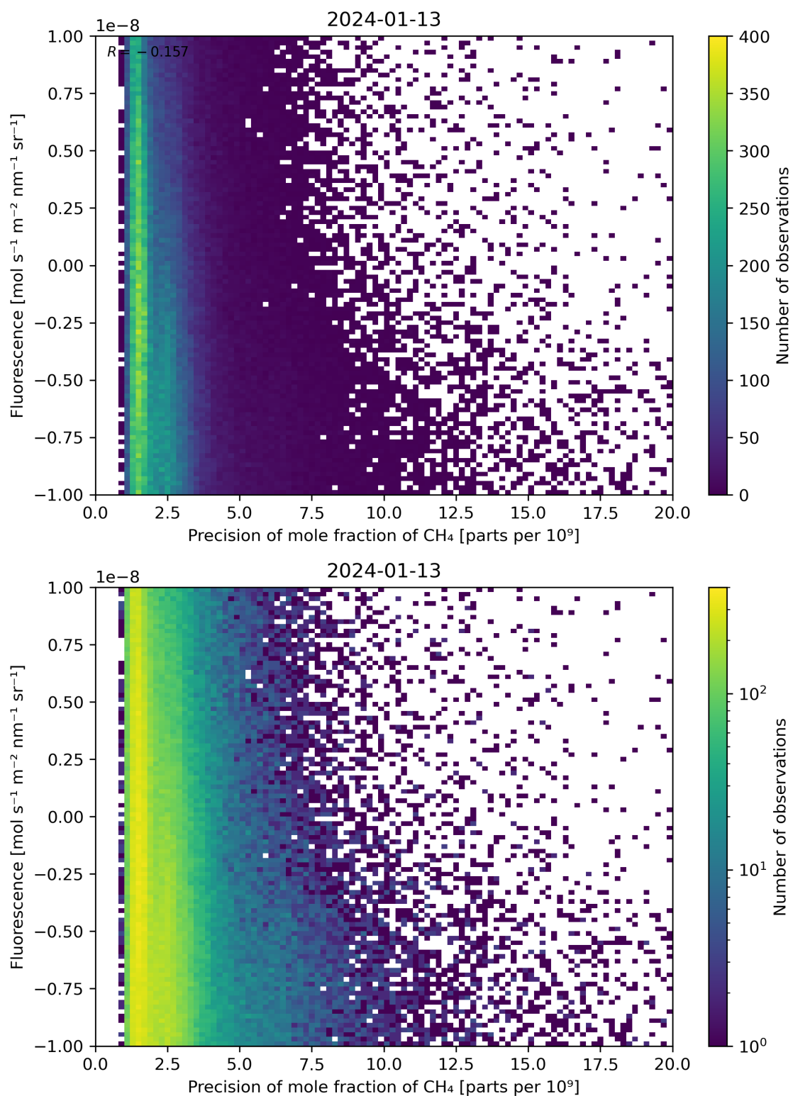
Figure 81: Scatter density plot of “Precision of mole fraction of CH 4 ” against “Fluorescence” for 2024-01-12 to 2024-01-14.
