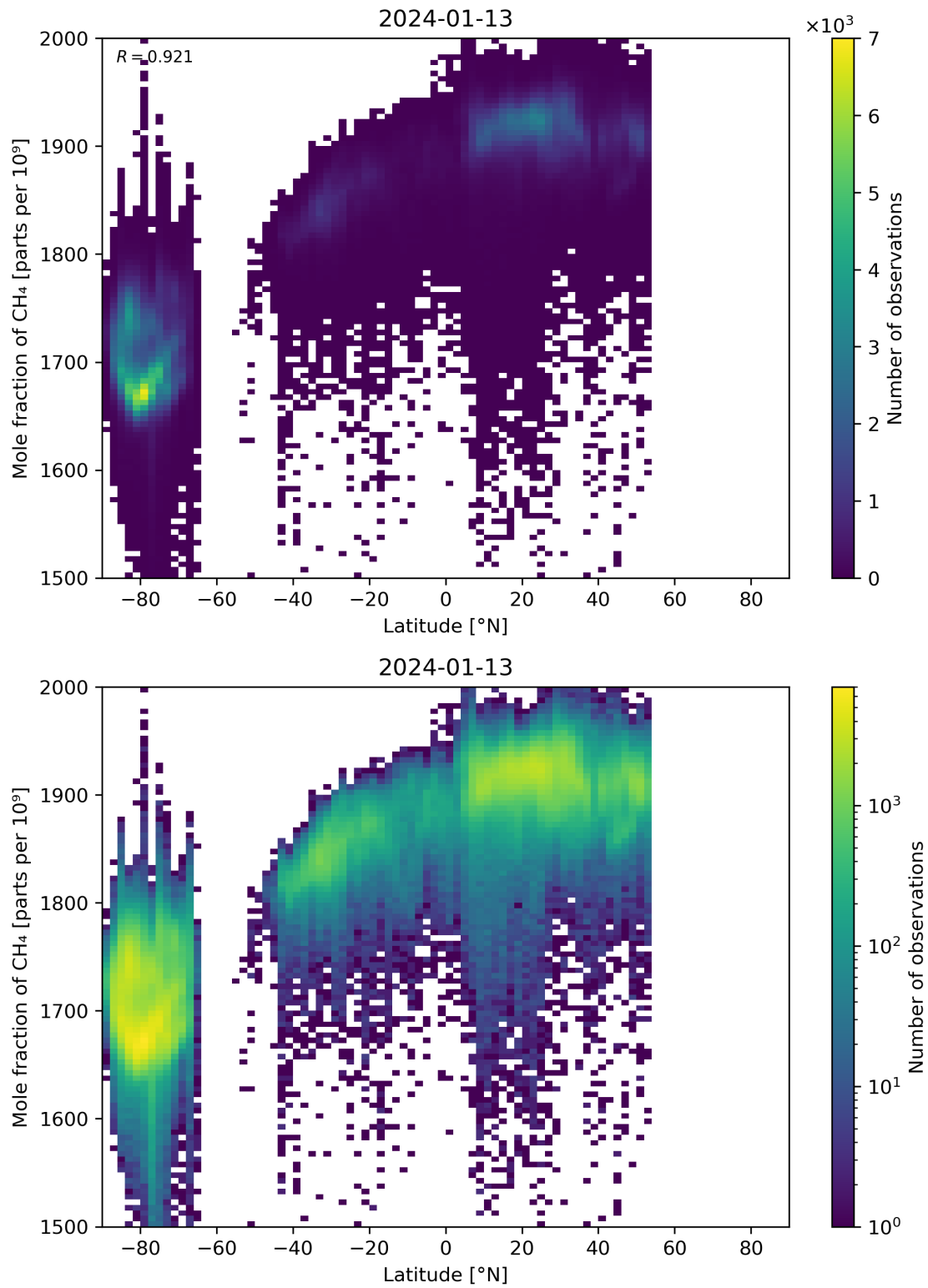
Figure 57: Scatter density plot of “Latitude” against “Mole fraction of CH 4 ” for 2024-01-12 to 2024-01-14.
