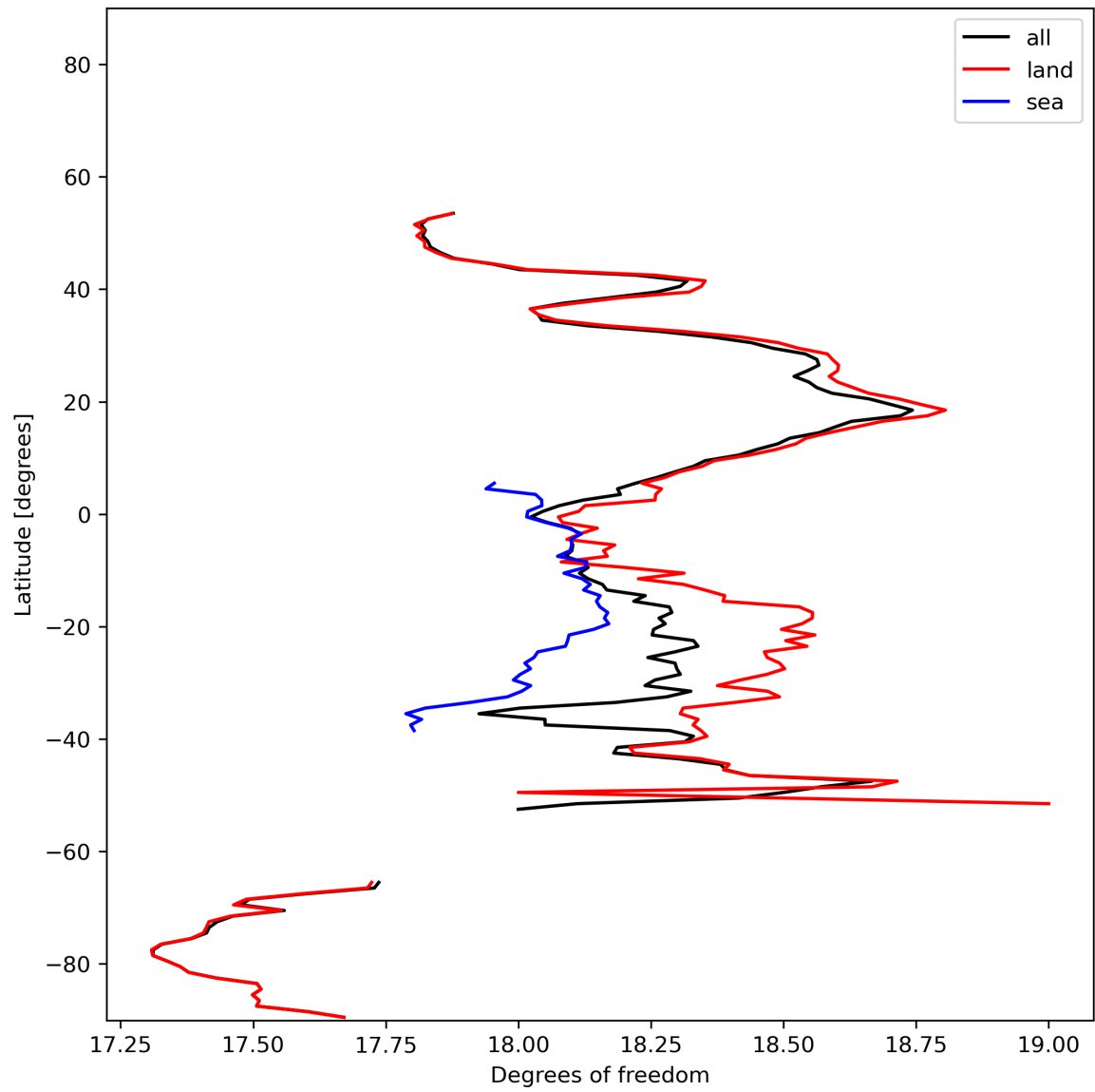
Figure 19: Zonal average of “Degrees of freedom” for 2024-01-12 to 2024-01-14.
