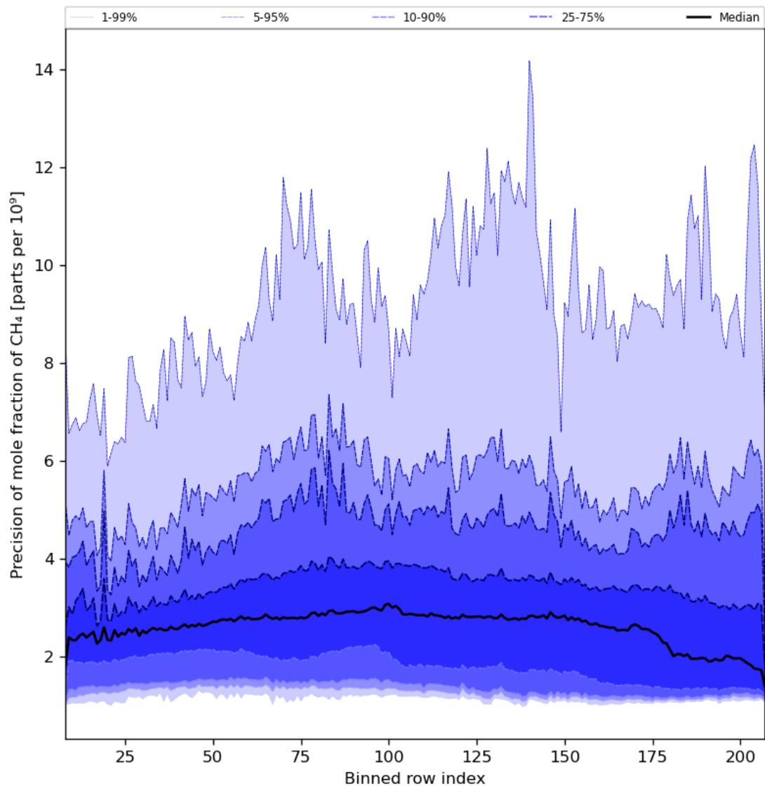
Figure 35: Along track statistics of “Precision of mole fraction of CH 4 ” for 2024-01-12 to 2024-01-14
