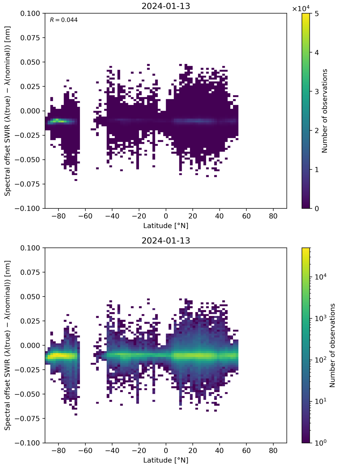
Figure 62: Scatter density plot of “Latitude” against “Spectral offset SWIR ( \lambda(\text{true}) - \lambda(\text{nominal}) )” for 2024-01-12 to 2024-01-14.
