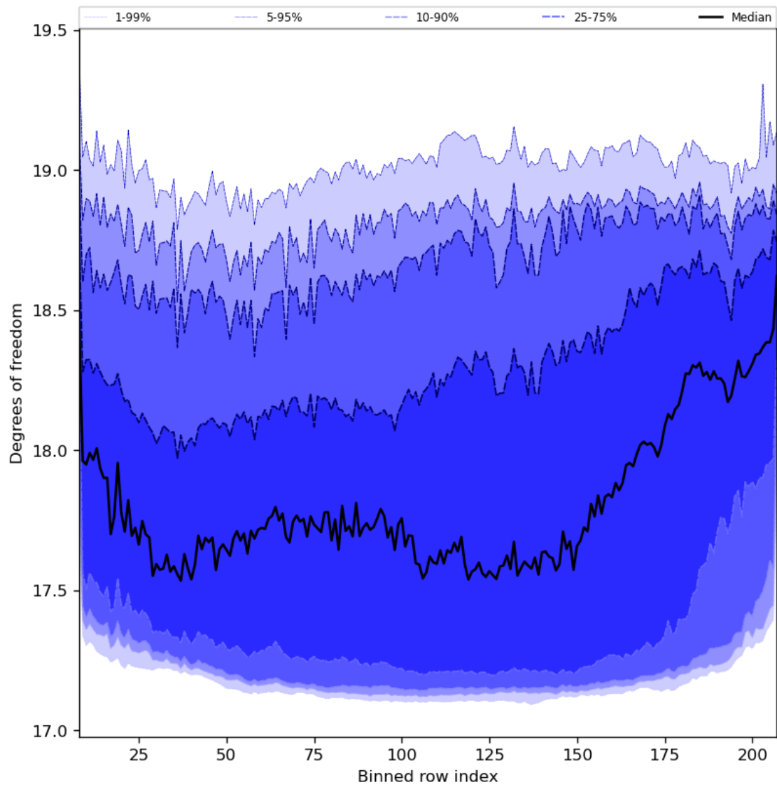
Figure 41: Along track statistics of “Degrees of freedom” for 2024-01-12 to 2024-01-14
