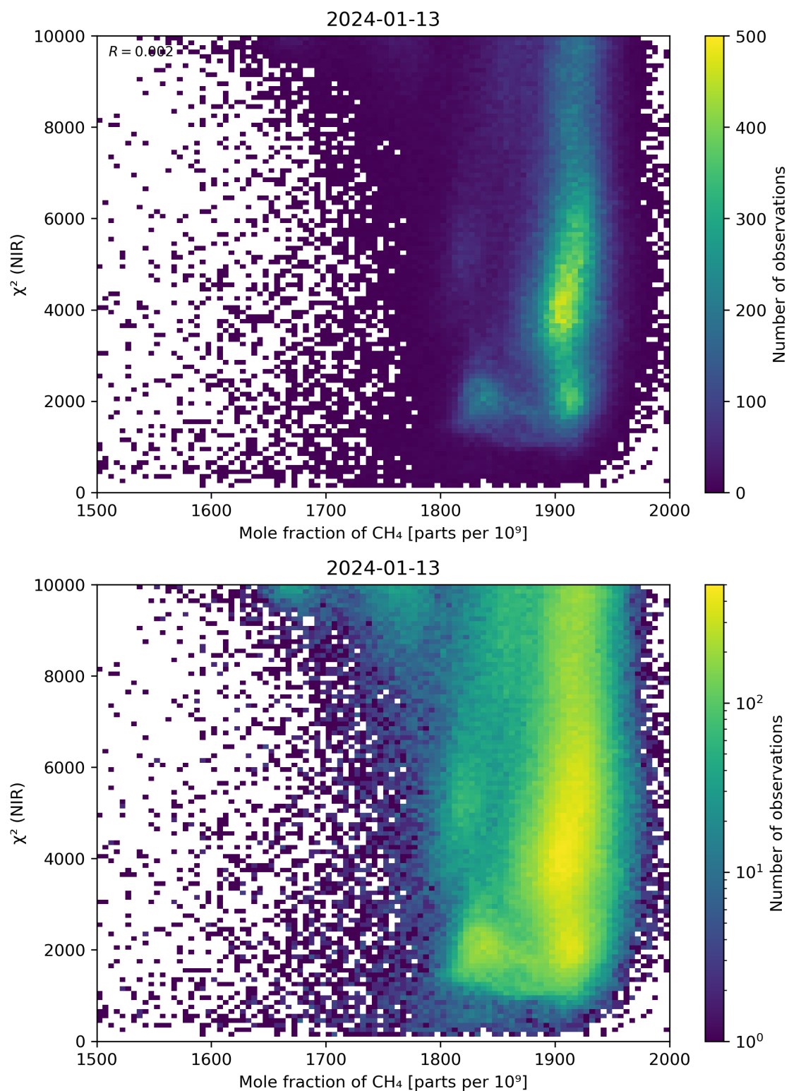
Figure 70: Scatter density plot of “Mole fraction of CH 4 ” against “ \chi^2 (NIR)” for 2024-01-12 to 2024-01-14.
