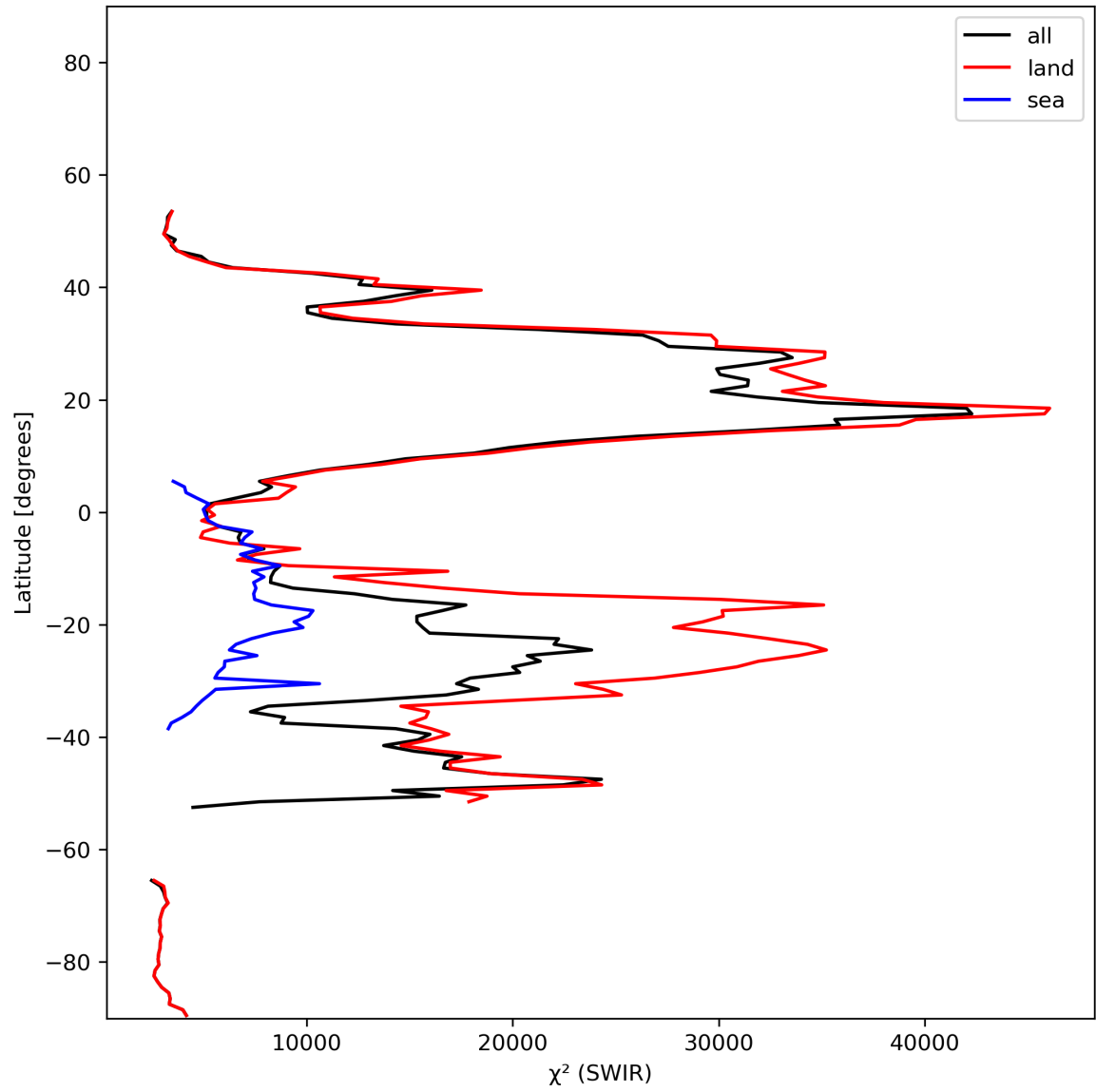
Figure 17: Zonal average of “ \chi^2 (SWIR)” for 2024-01-12 to 2024-01-14.
