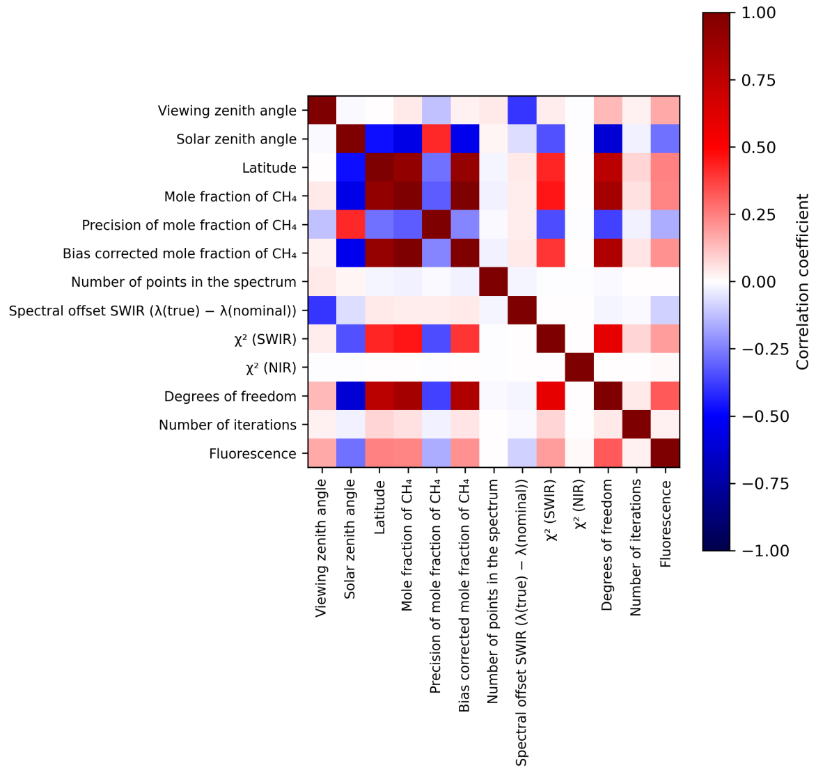
Figure 2: Map of correlation matrix for 2024-01-12 to 2024-01-14.
