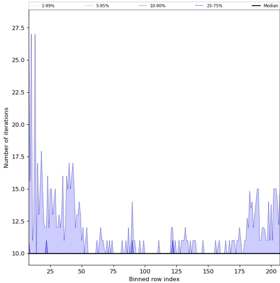
Figure 42: Along track statistics of “Number of iterations” for 2024-01-12 to 2024-01-14
