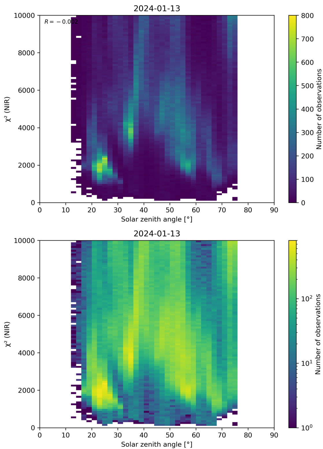
Figure 94: Scatter density plot of “Solar zenith angle” against “ \chi^2 (NIR)” for 2024-01-12 to 2024-01-14.
