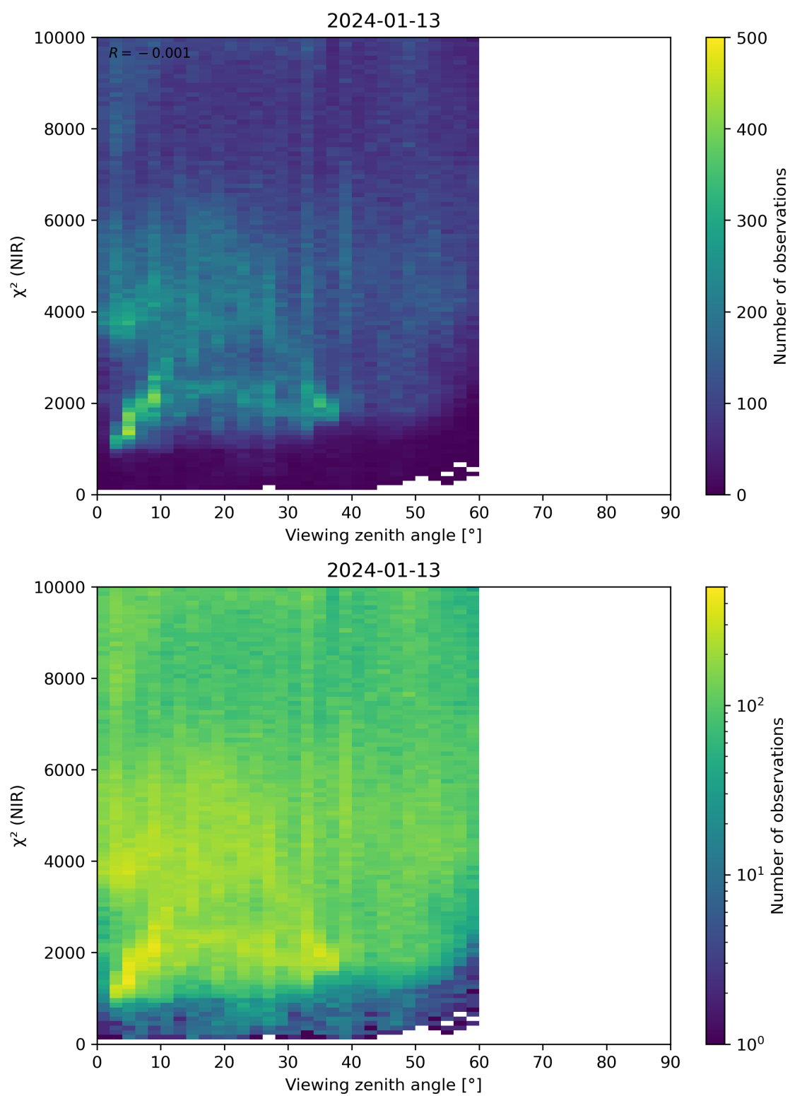
Figure 105: Scatter density plot of “Viewing zenith angle” against “ \chi^2 (NIR)” for 2024-01-12 to 2024-01-14.
