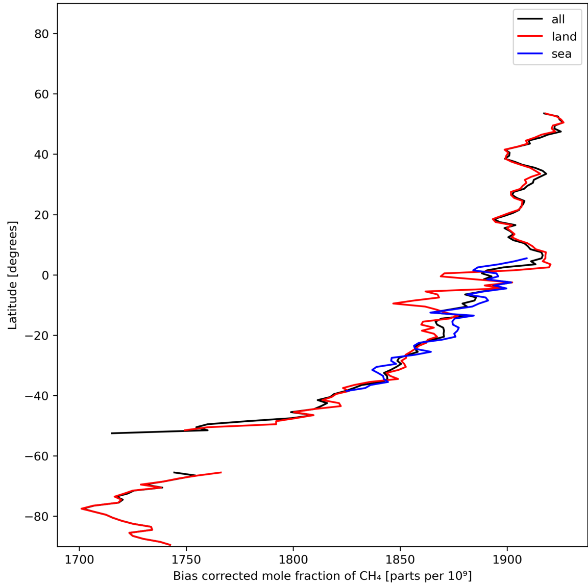
Figure 14: Zonal average of “Bias corrected mole fraction of CH 4 ” for 2024-01-12 to 2024-01-14.
