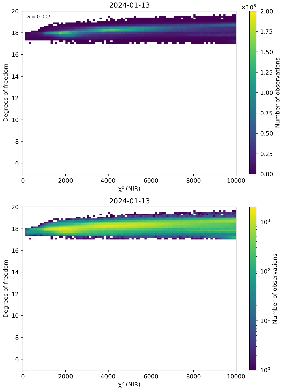
Figure 44: Scatter density plot of “ \chi^2 (NIR)” against “Degrees of freedom” for 2024-01-12 to 2024-01-14.
