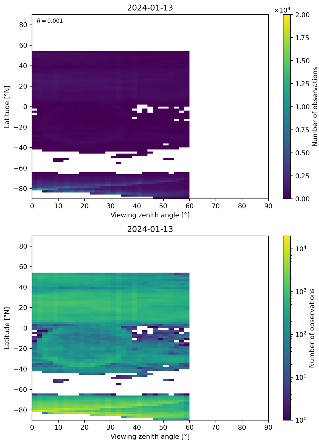
Figure 109: Scatter density plot of “Viewing zenith angle” against “Latitude” for 2024-01-12 to 2024-01-14.
