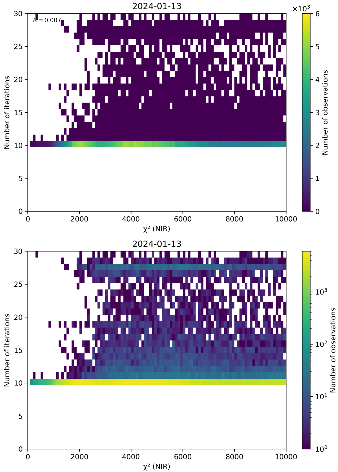
Figure 46: Scatter density plot of “ \chi^2 (NIR)” against “Number of iterations” for 2024-01-12 to 2024-01-14.
