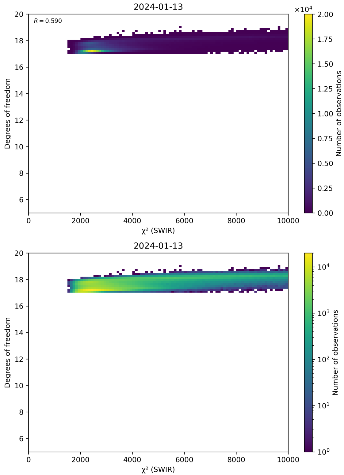
Figure 48: Scatter density plot of “ \chi^2 (SWIR)” against “Degrees of freedom” for 2024-01-12 to 2024-01-14.
