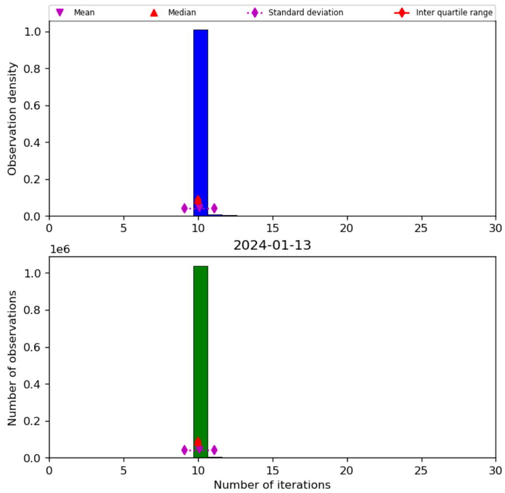
Figure 31: Histogram of “Number of iterations” for 2024-01-12 to 2024-01-14
