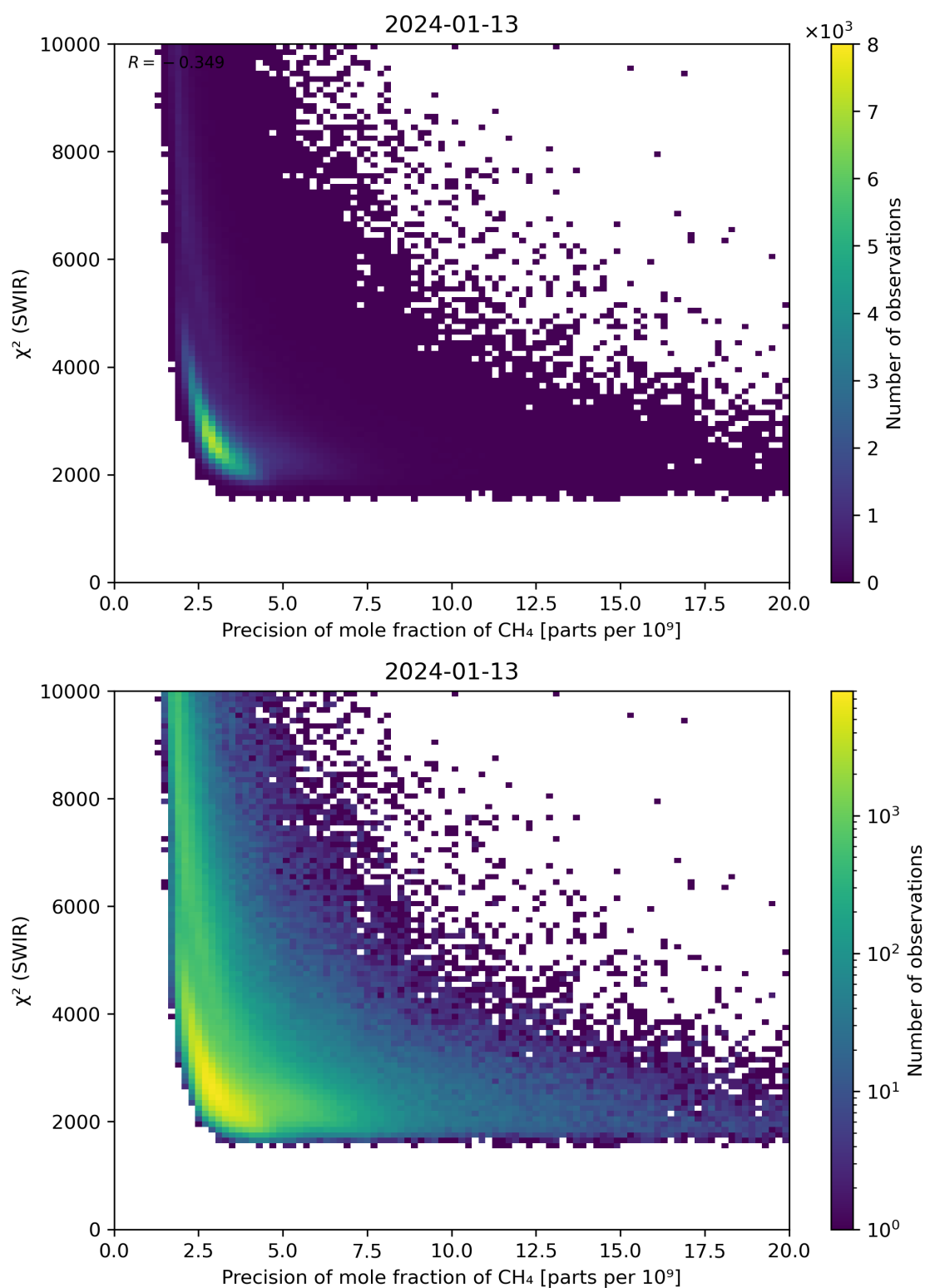
Figure 79: Scatter density plot of “Precision of mole fraction of \text{CH}_4 ” against “ \chi^2 (SWIR)” for 2024-01-12 to 2024-01-14.
