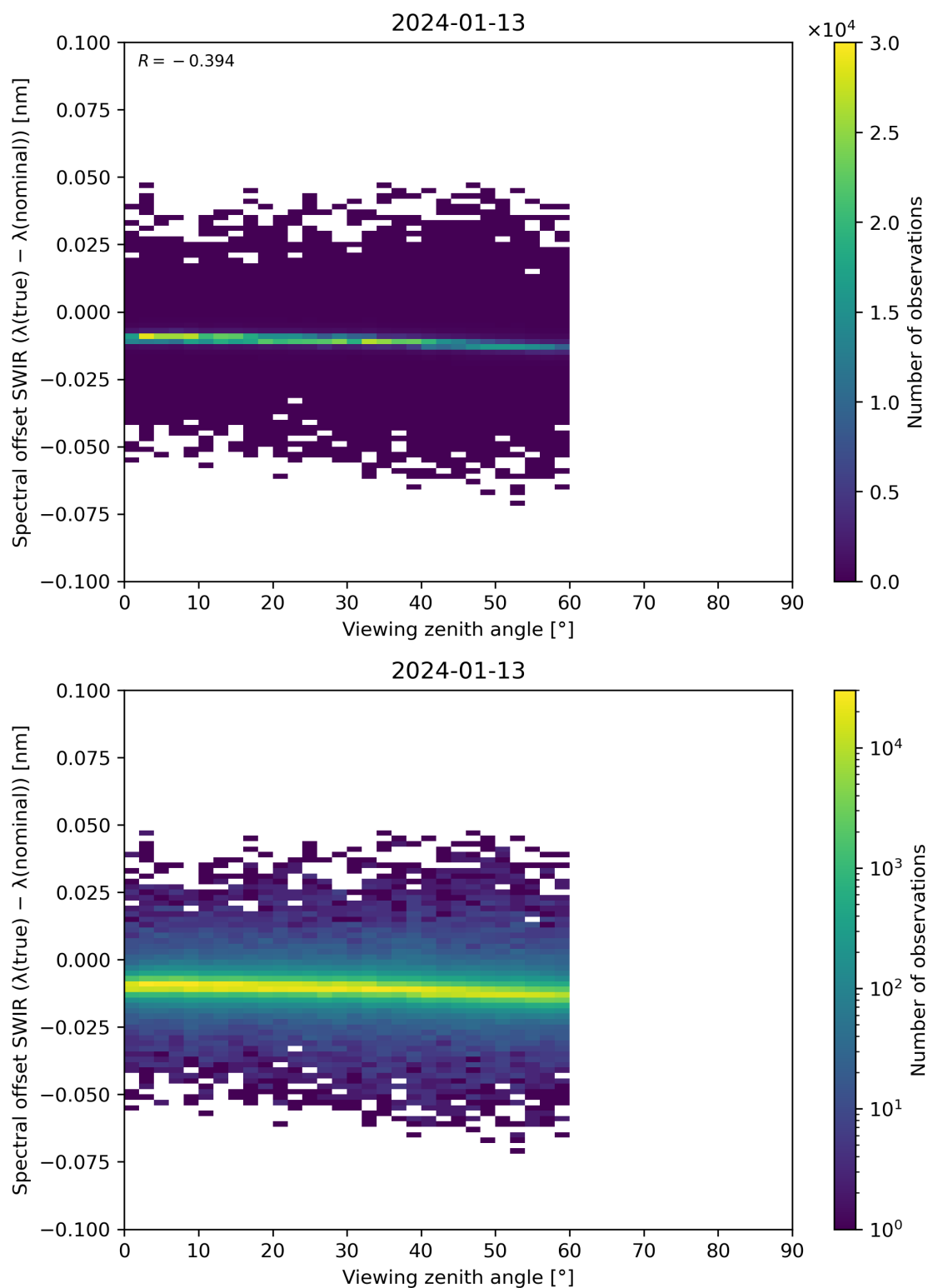
Figure 116: Scatter density plot of “Viewing zenith angle” against “Spectral offset SWIR ( \lambda(\text{true}) - \lambda(\text{nominal}) )” for 2024-01-12 to 2024-01-14.
