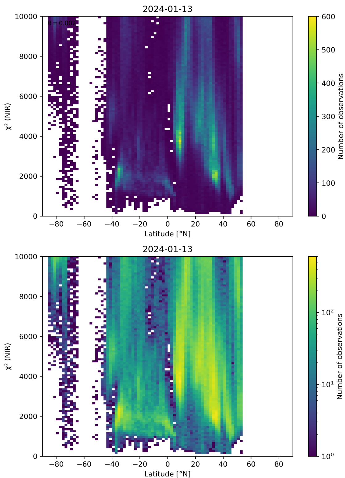
Figure 53: Scatter density plot of “Latitude” against “ \chi^2 (NIR)” for 2024-01-12 to 2024-01-14.
