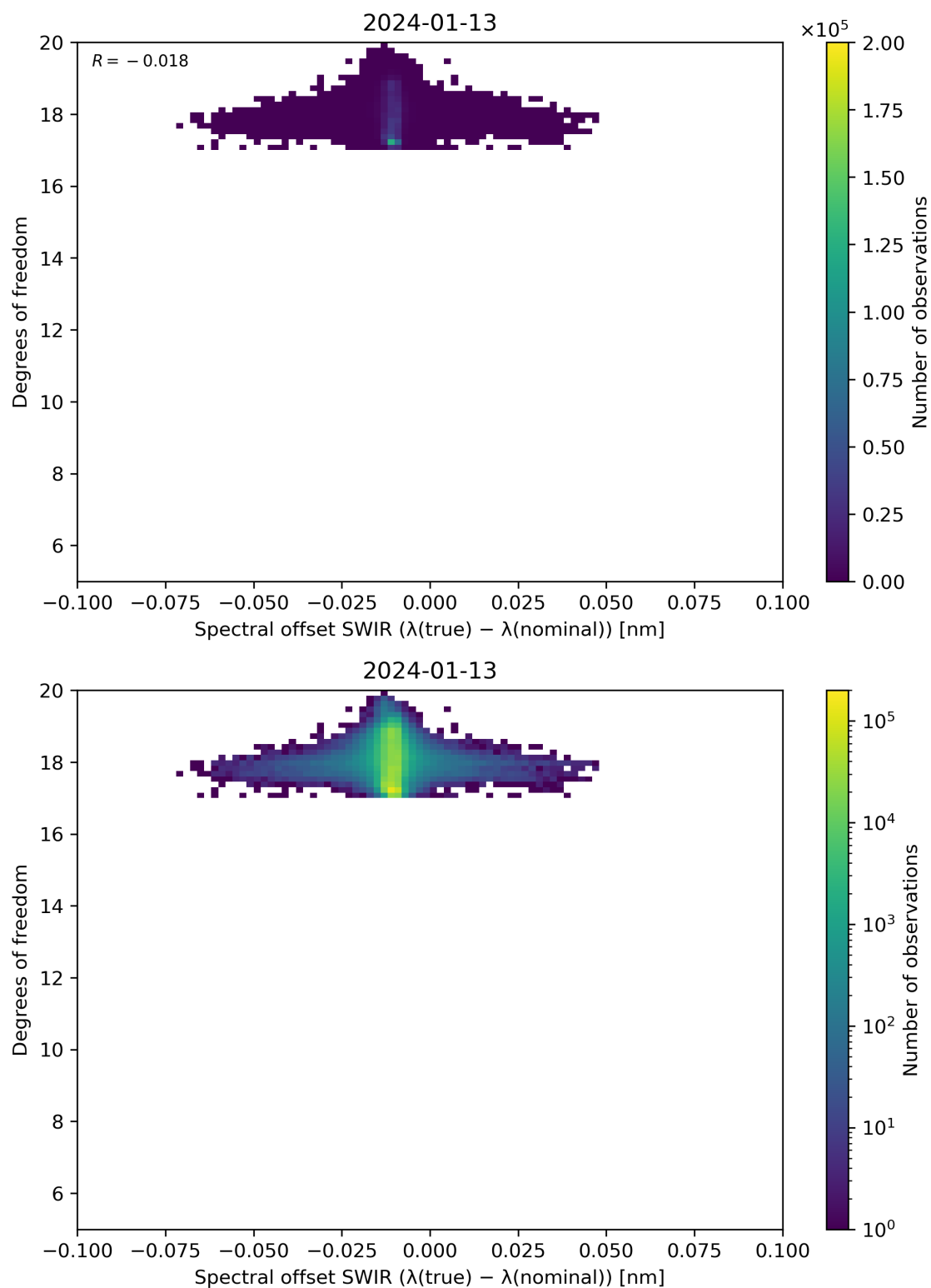
Figure 119: Scatter density plot of “Spectral offset SWIR ( \lambda(\text{true}) - \lambda(\text{nominal}) )” against “Degrees of freedom” for 2024-01-12 to 2024-01-14.
