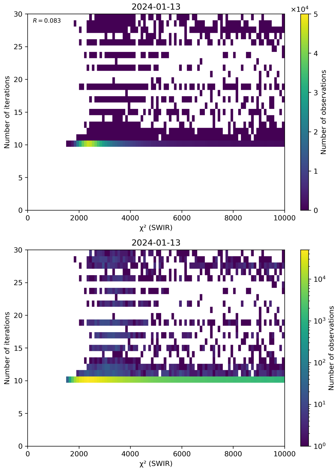
Figure 50: Scatter density plot of “ \chi^2 (SWIR)” against “Number of iterations” for 2024-01-12 to 2024-01-14.
