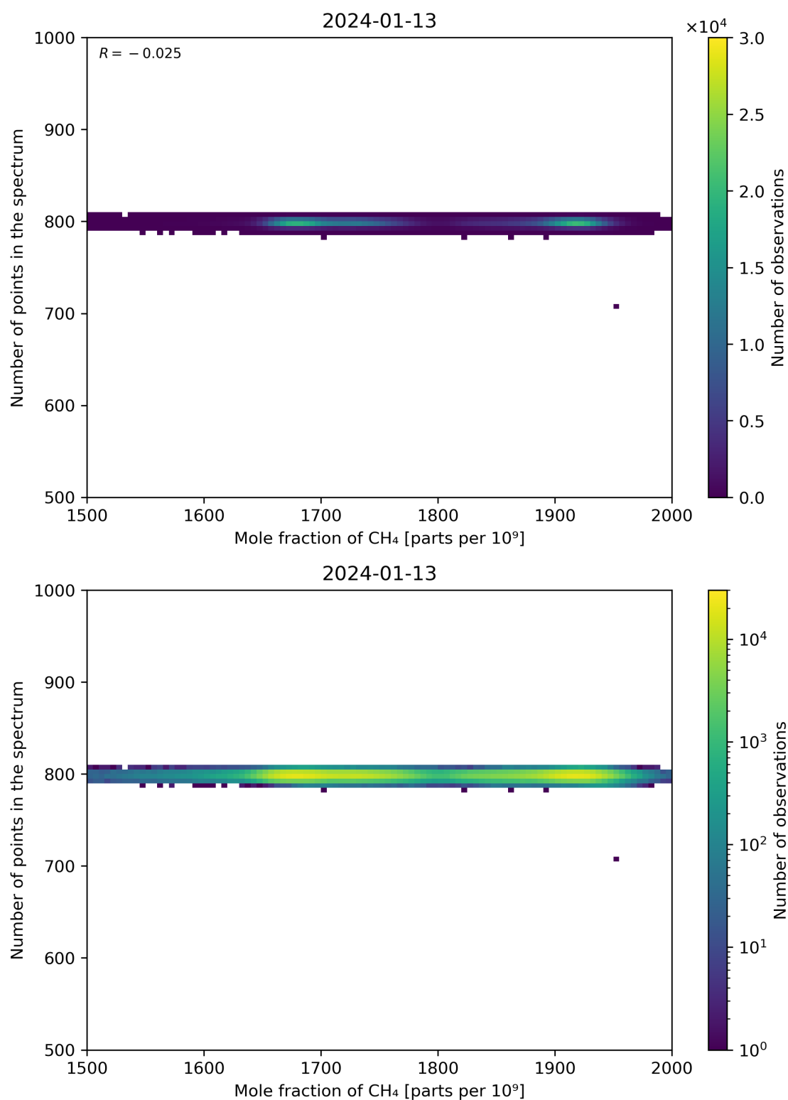
Figure 77: Scatter density plot of “Mole fraction of CH 4 ” against “Number of points in the spectrum” for 2024-01-12 to 2024-01-14.
