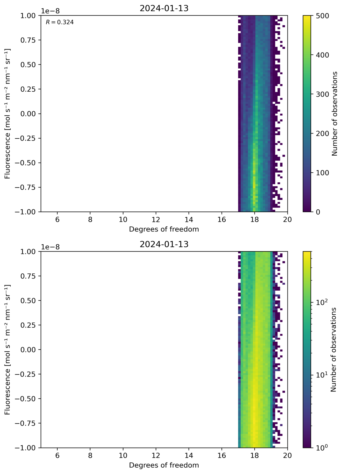
Figure 51: Scatter density plot of “Degrees of freedom” against “Fluorescence” for 2024-01-12 to 2024-01-14.
