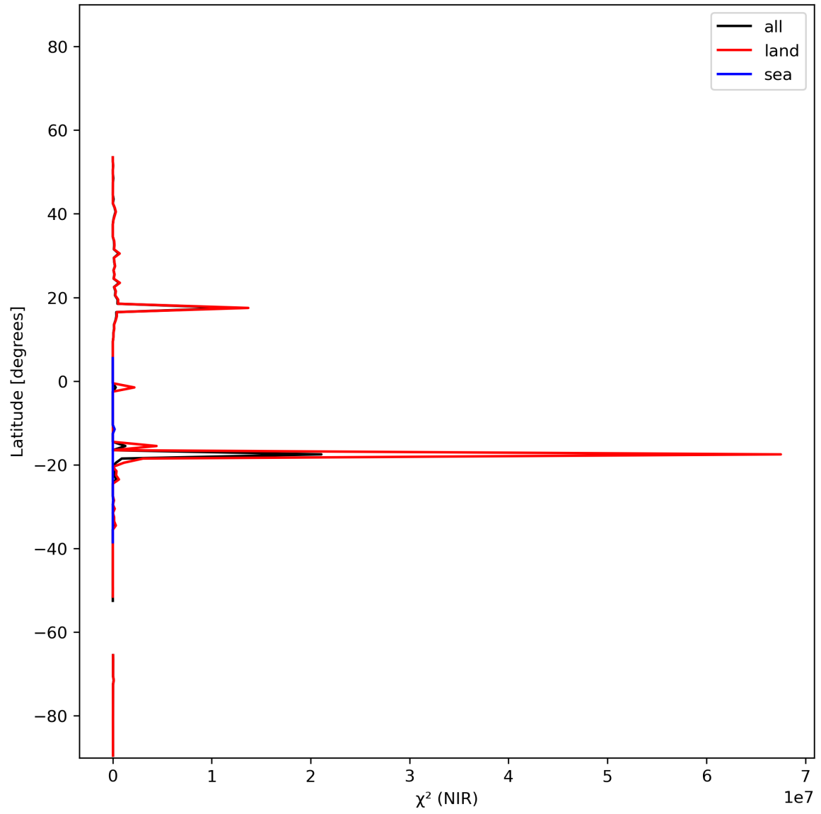
Figure 18: Zonal average of “ \chi^2 (NIR)” for 2024-01-12 to 2024-01-14.
