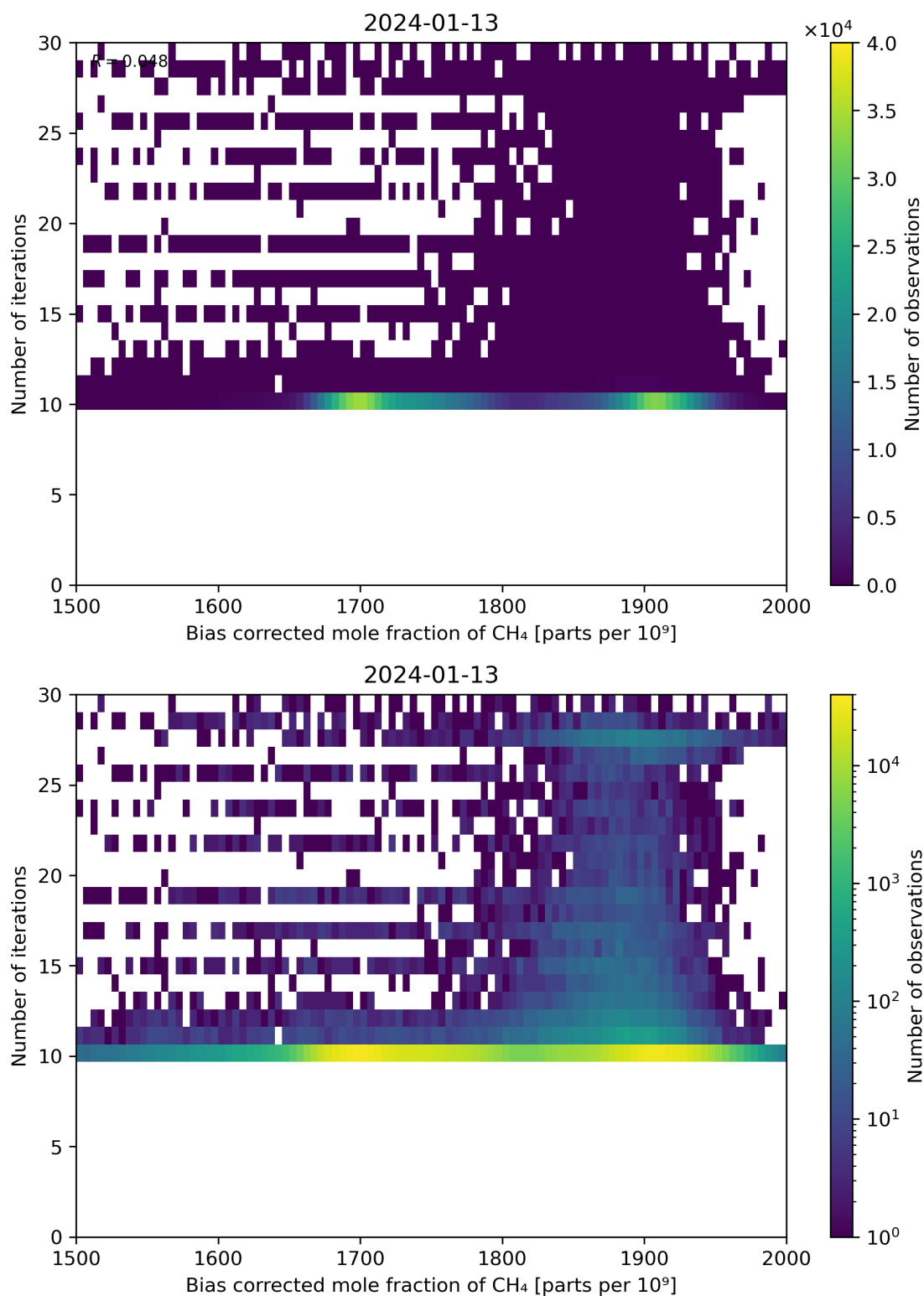
Figure 67: Scatter density plot of “Bias corrected mole fraction of \text{CH}_4 ” against “Number of iterations” for 2024-01-12 to 2024-01-14.
