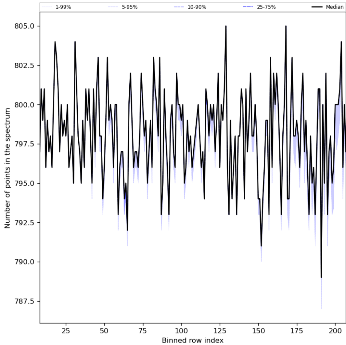
Figure 37: Along track statistics of “Number of points in the spectrum” for 2024-01-12 to 2024-01-14
