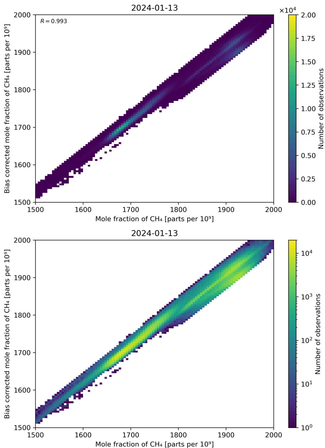
Figure 74: Scatter density plot of “Mole fraction of CH 4 ” against “Bias corrected mole fraction of CH 4 ” for 2024-01-12 to 2024-01-14.
