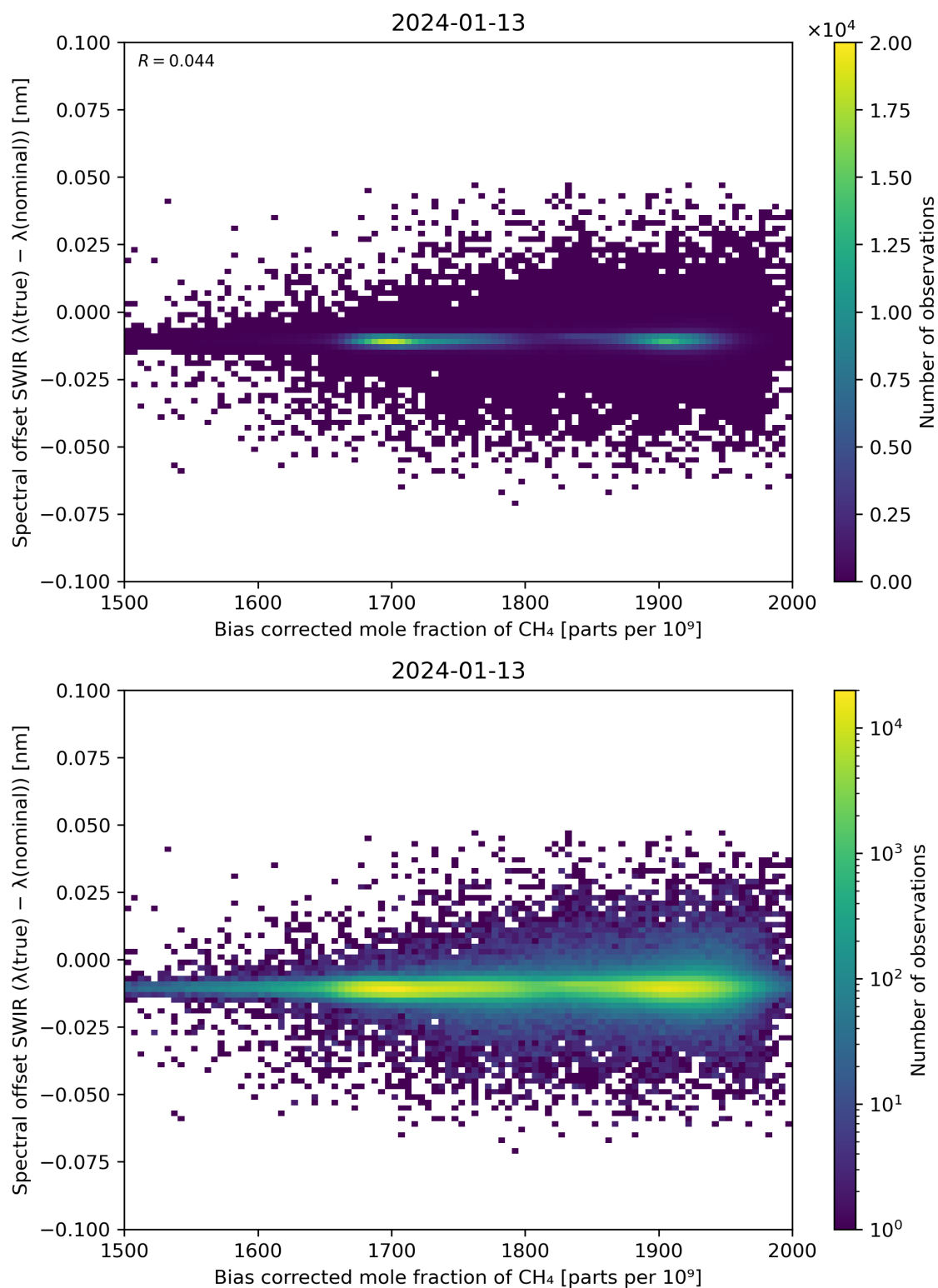
Figure 69: Scatter density plot of “Bias corrected mole fraction of \text{CH}_4 ” against “Spectral offset SWIR ( \lambda(\text{true}) - \lambda(\text{nominal}) )” for 2024-01-12 to 2024-01-14.
