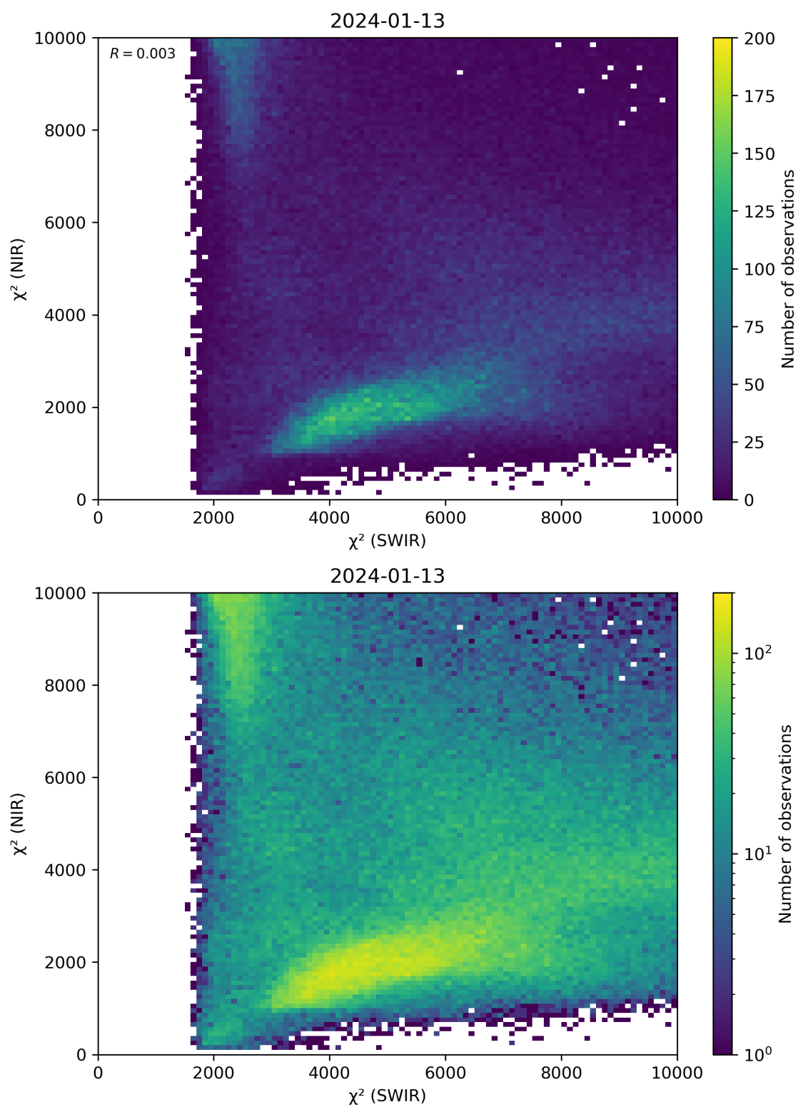
Figure 47: Scatter density plot of “ \chi^2 (SWIR)” against “ \chi^2 (NIR)” for 2024-01-12 to 2024-01-14.
