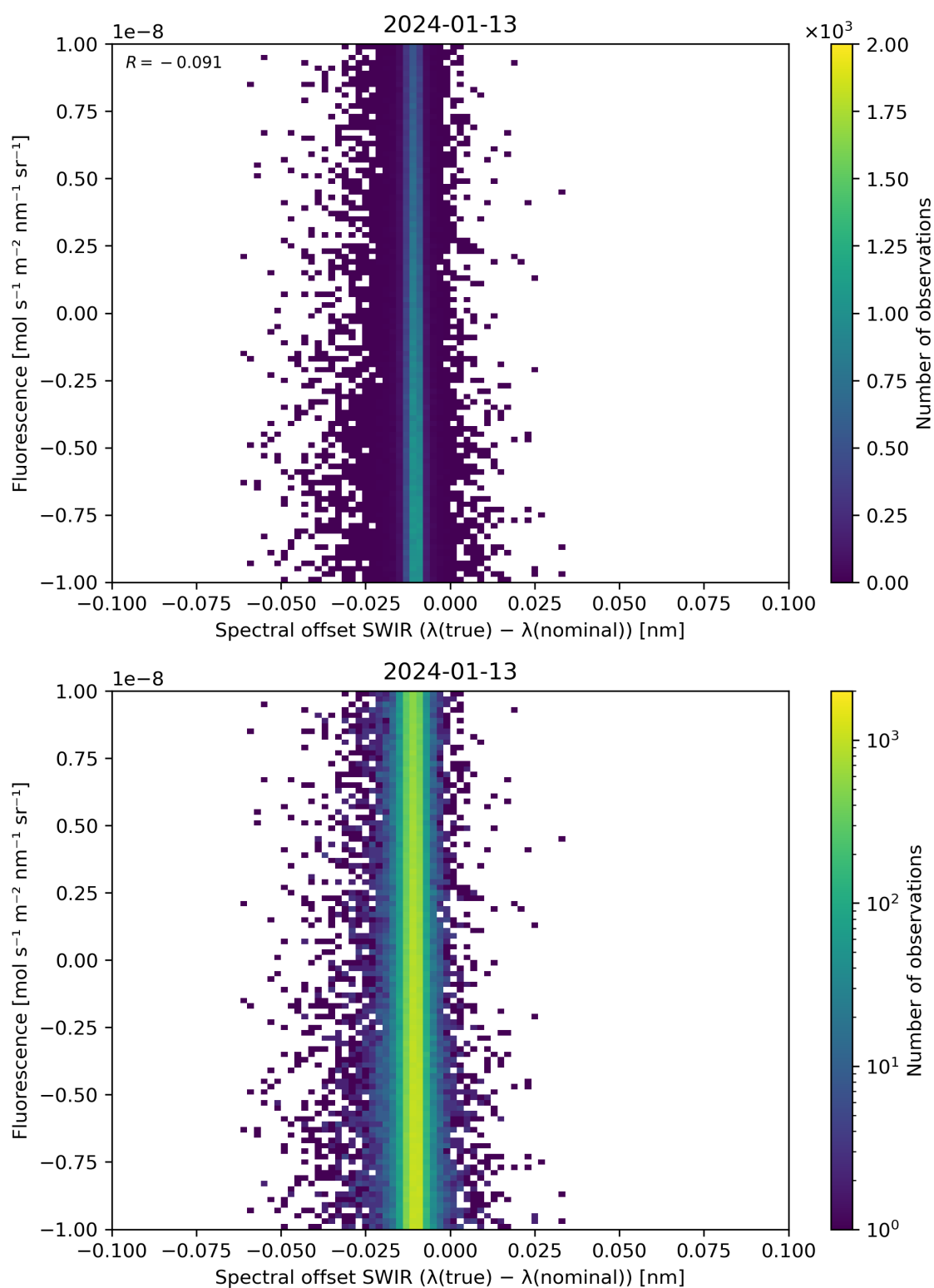
Figure 120: Scatter density plot of “Spectral offset SWIR ( \lambda(\text{true}) - \lambda(\text{nominal}) )” against “Fluorescence” for 2024-01-12 to 2024-01-14.
