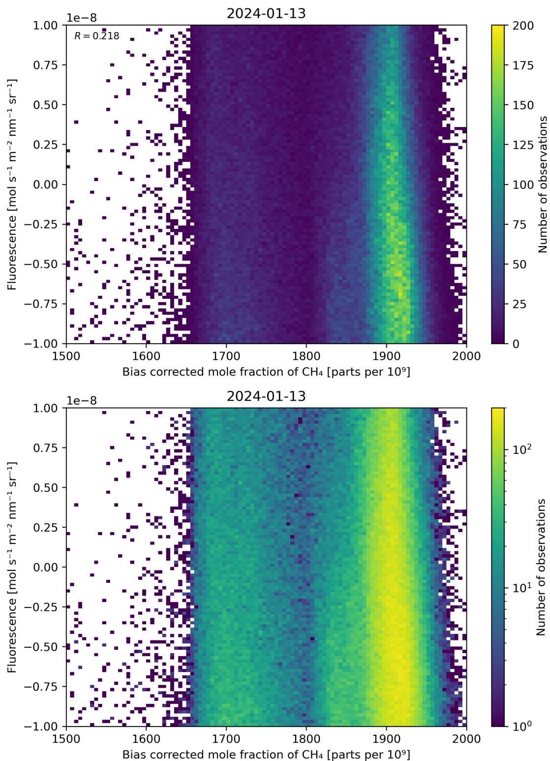
Figure 66: Scatter density plot of “Bias corrected mole fraction of \text{CH}_4 ” against “Fluorescence” for 2024-01-12 to 2024-01-14.
