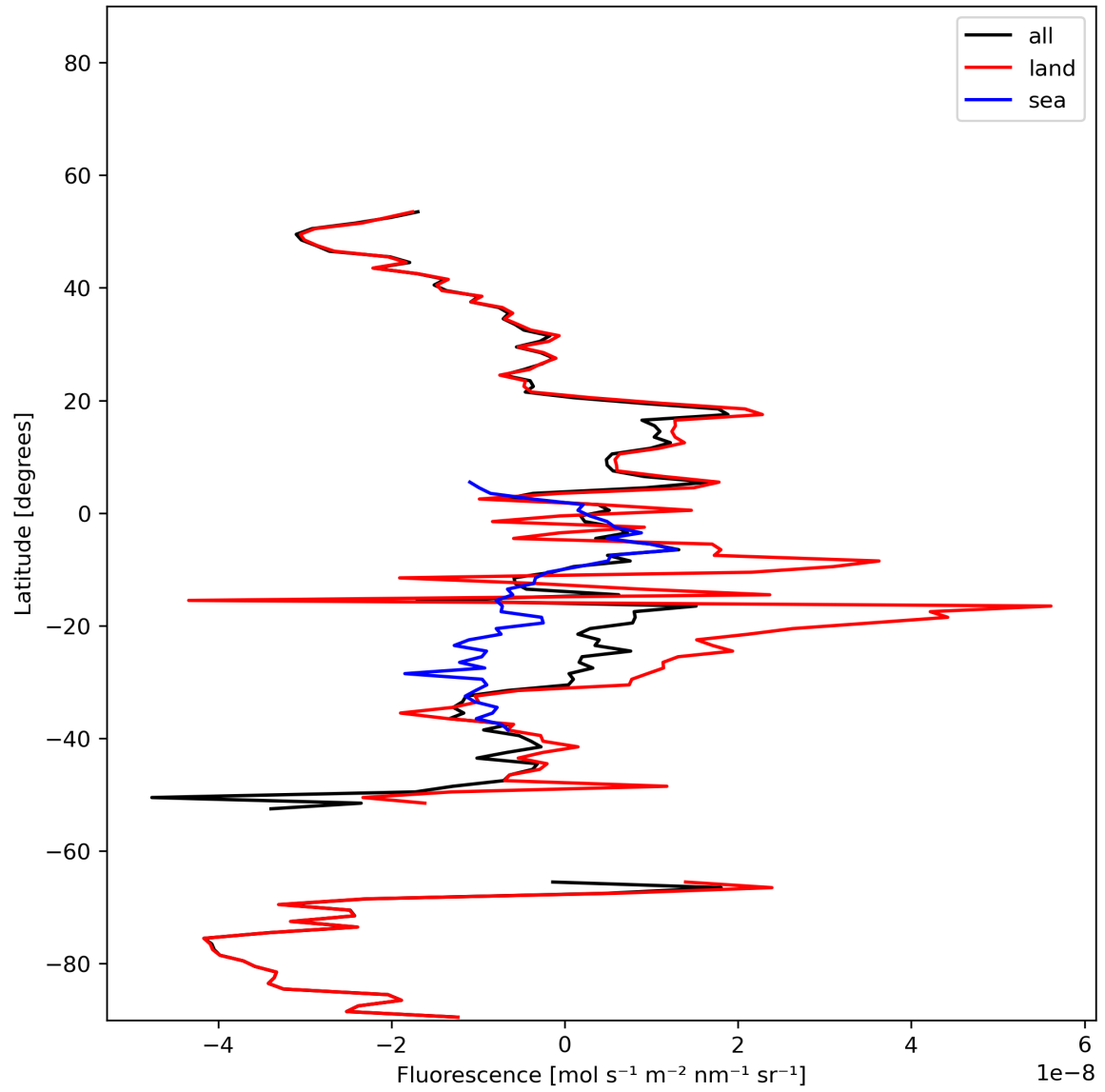
Figure 21: Zonal average of “Fluorescence” for 2024-01-12 to 2024-01-14.
