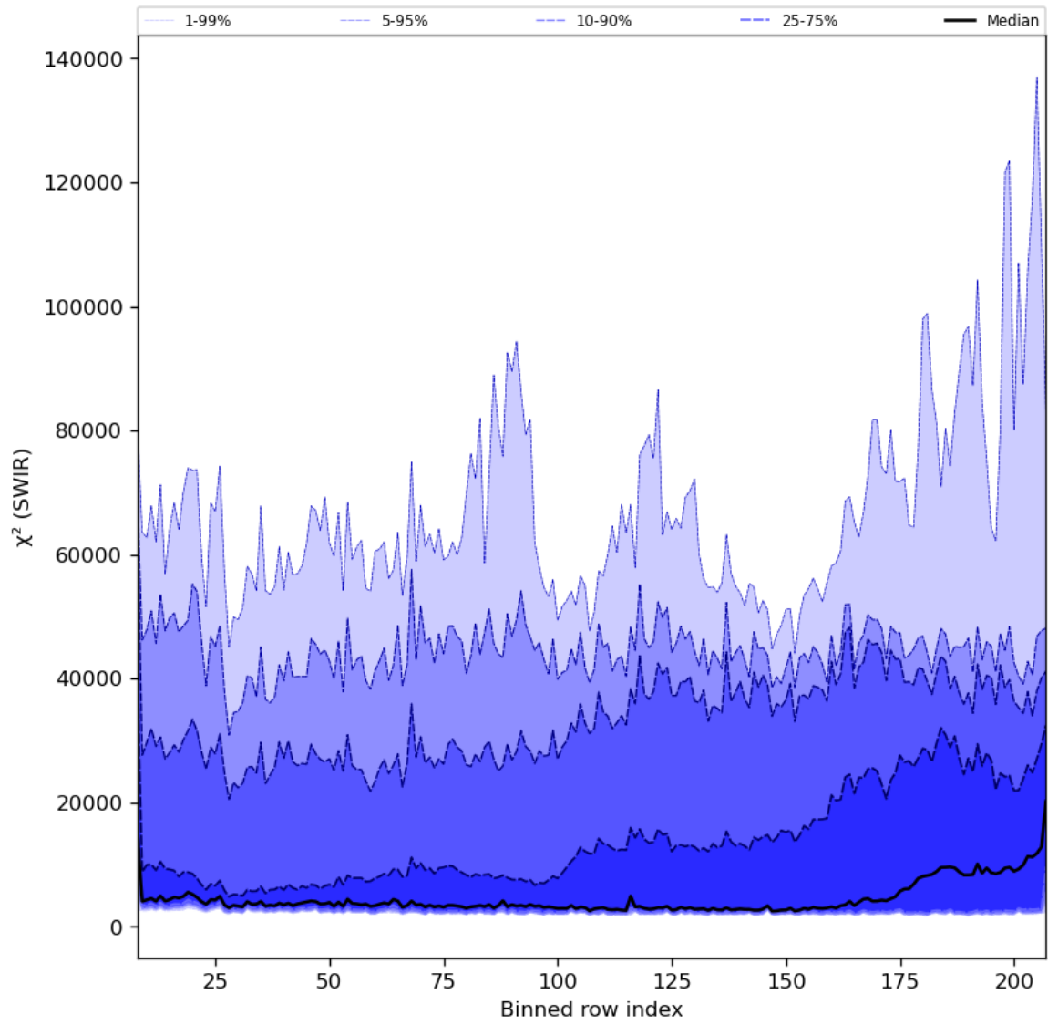
Figure 39: Along track statistics of “ \chi^2 (SWIR)” for 2024-01-12 to 2024-01-14
