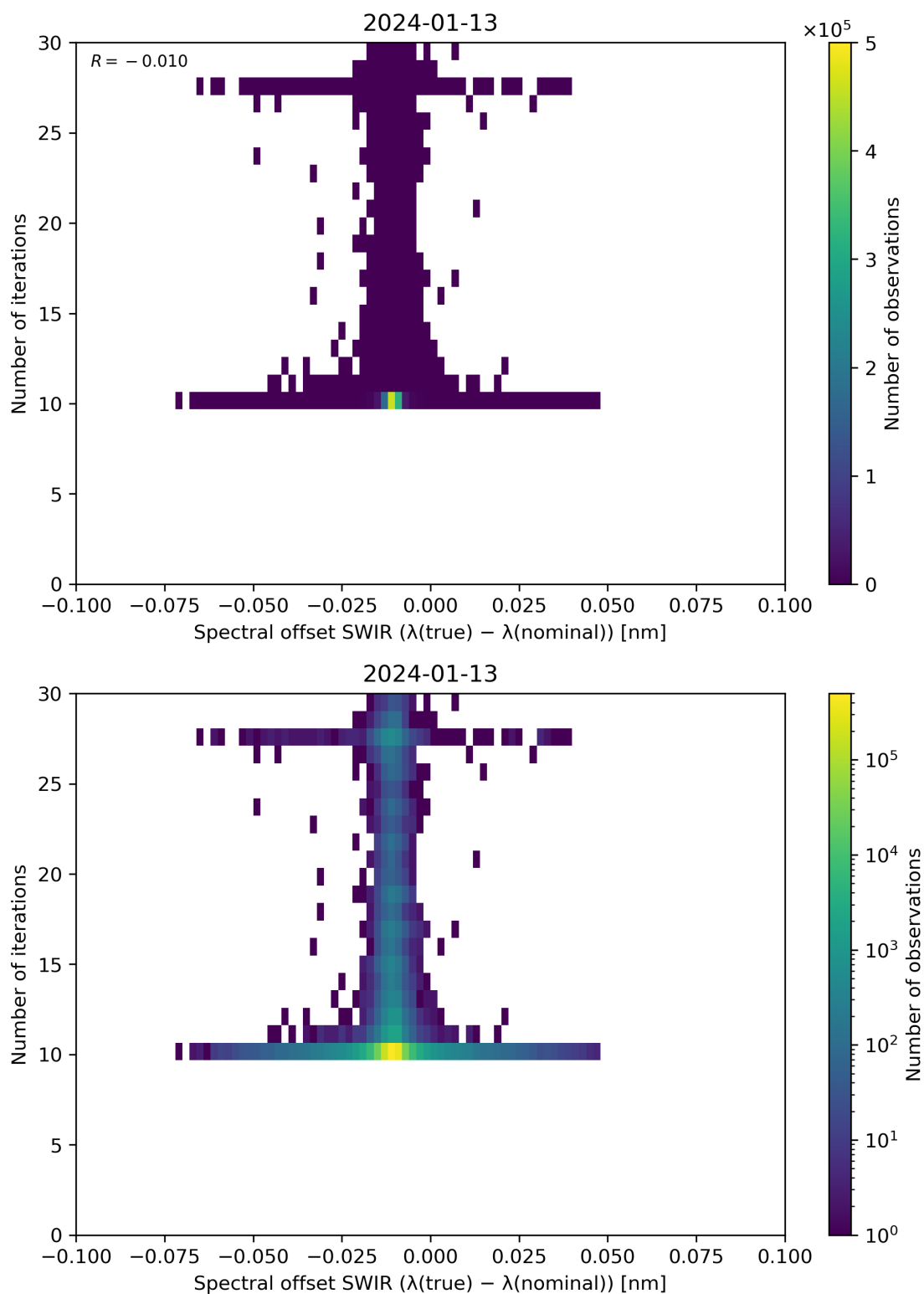
Figure 121: Scatter density plot of “Spectral offset SWIR ( \lambda(\text{true}) - \lambda(\text{nominal}) )” against “Number of iterations” for 2024-01-12 to 2024-01-14.
