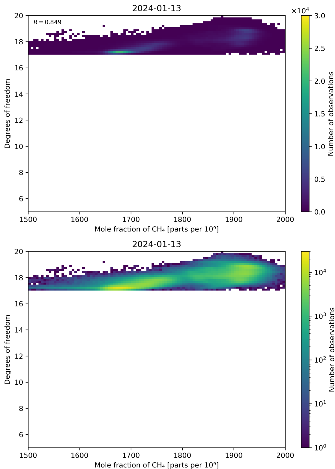
Figure 72: Scatter density plot of “Mole fraction of CH 4 ” against “Degrees of freedom” for 2024-01-12 to 2024-01-14.
