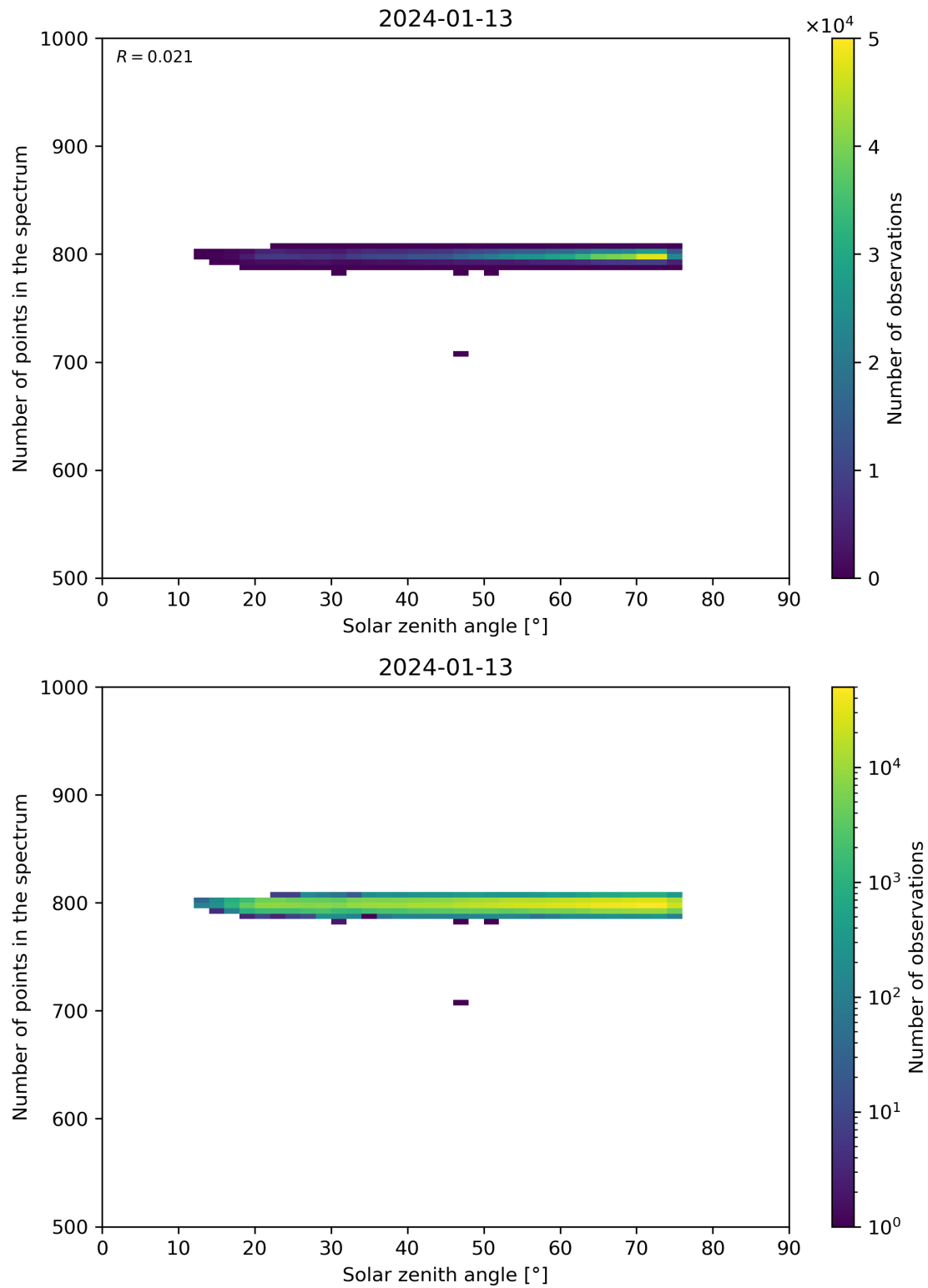
Figure 103: Scatter density plot of “Solar zenith angle” against “Number of points in the spectrum” for 2024-01-12 to 2024-01-14.
