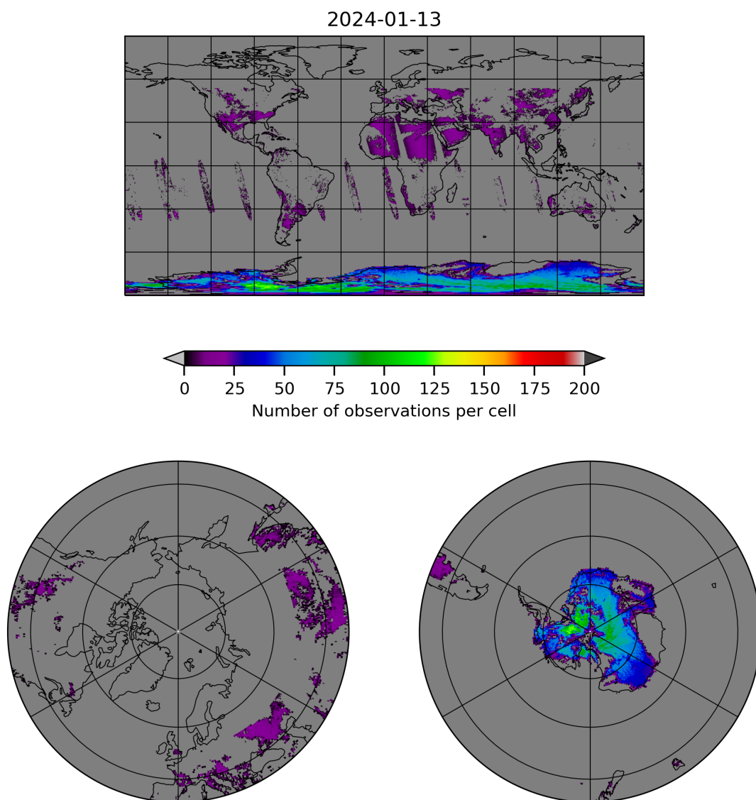
Figure 10: Map of the number of observations for 2024-01-12 to 2024-01-14
