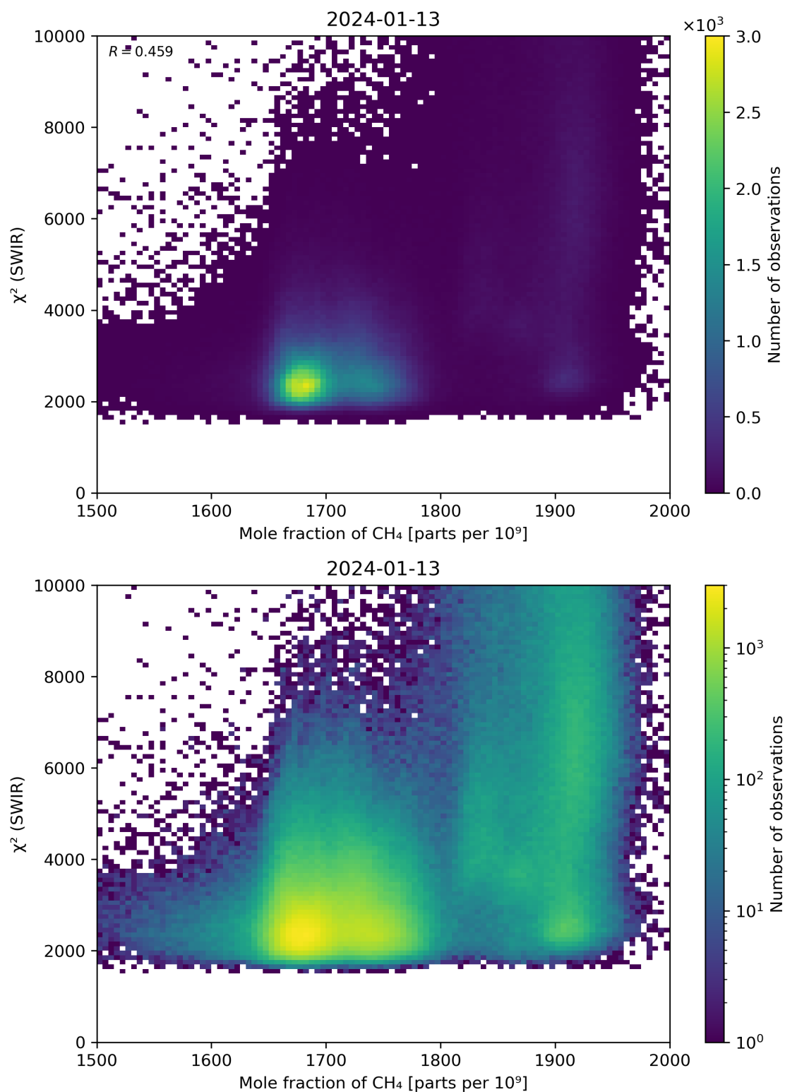
Figure 71: Scatter density plot of “Mole fraction of \text{CH}_4 ” against “ \chi^2 (SWIR)” for 2024-01-12 to 2024-01-14.
