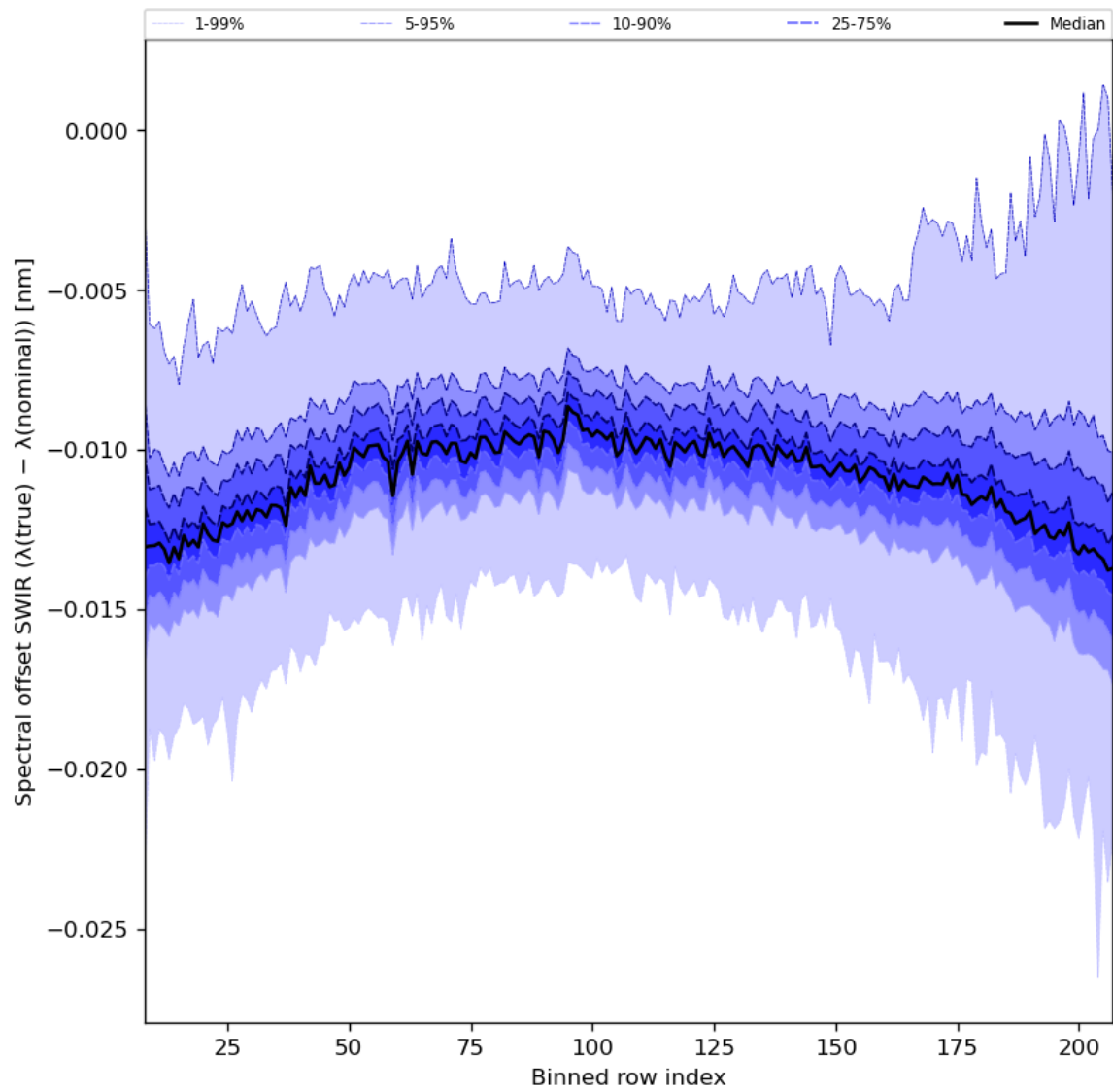
Figure 38: Along track statistics of “Spectral offset SWIR ( \lambda(\text{true}) - \lambda(\text{nominal}) )” for 2024-01-12 to 2024-01-14
