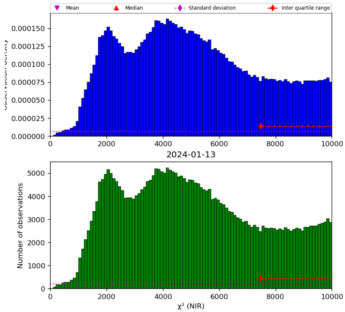
Figure 29: Histogram of “ \chi^2 (NIR)” for 2024-01-12 to 2024-01-14
