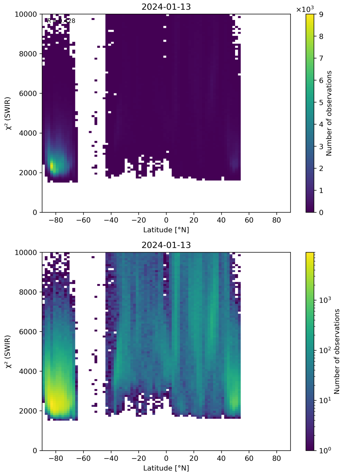
Figure 54: Scatter density plot of “Latitude” against “ \chi^2 (SWIR)” for 2024-01-12 to 2024-01-14.
