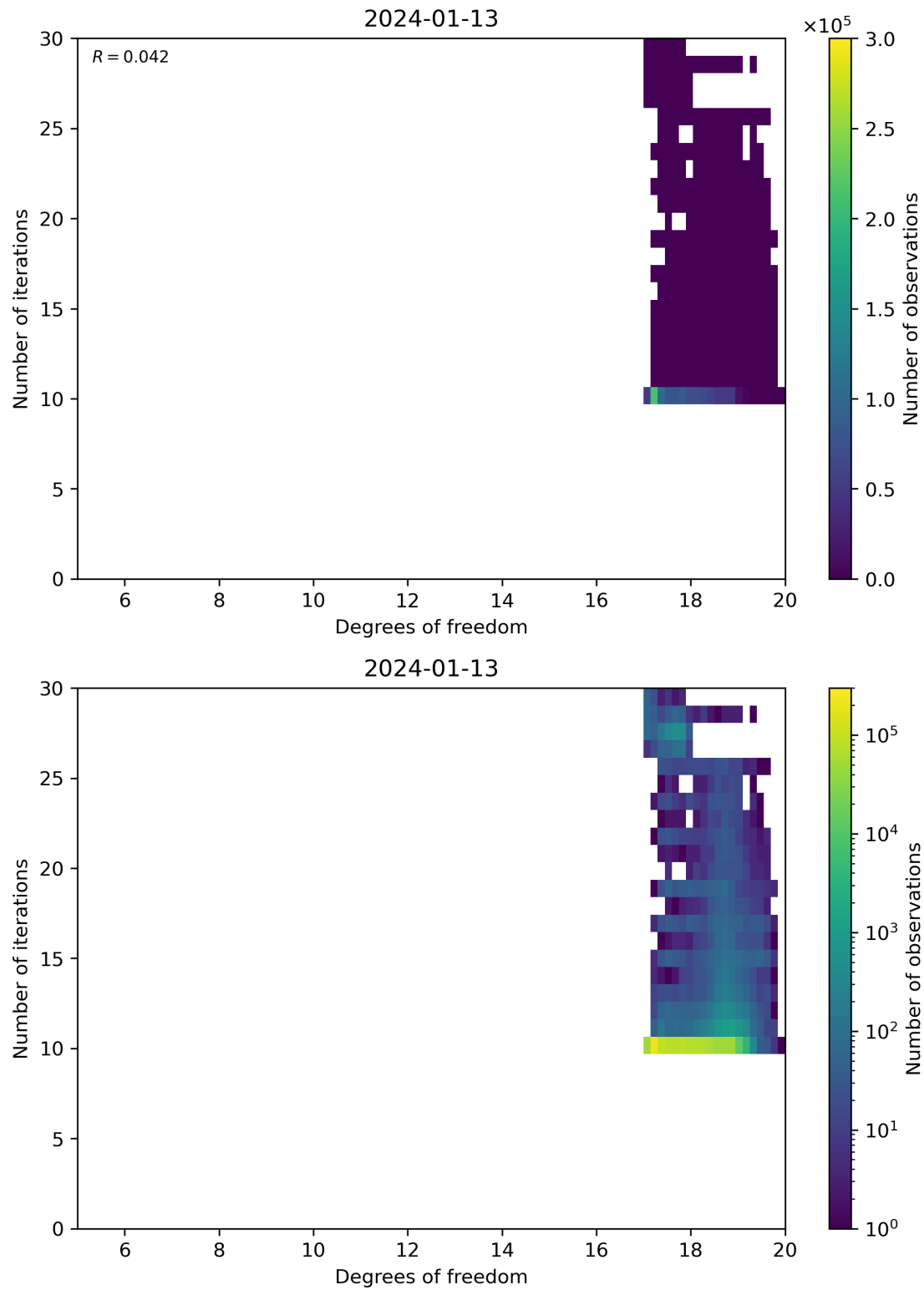
Figure 52: Scatter density plot of “Degrees of freedom” against “Number of iterations” for 2024-01-12 to 2024-01-14.
