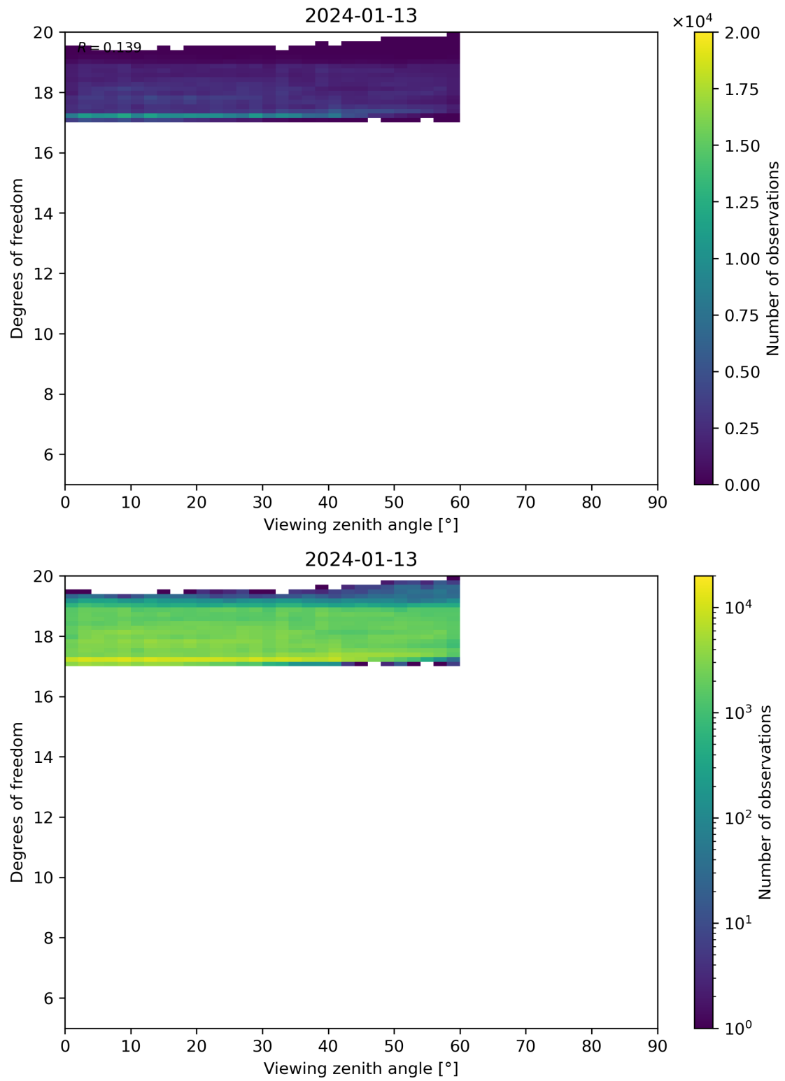
Figure 107: Scatter density plot of “Viewing zenith angle” against “Degrees of freedom” for 2024-01-12 to 2024-01-14.
