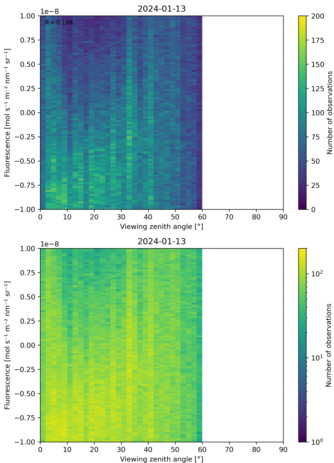
Figure 108: Scatter density plot of “Viewing zenith angle” against “Fluorescence” for 2024-01-12 to 2024-01-14.
