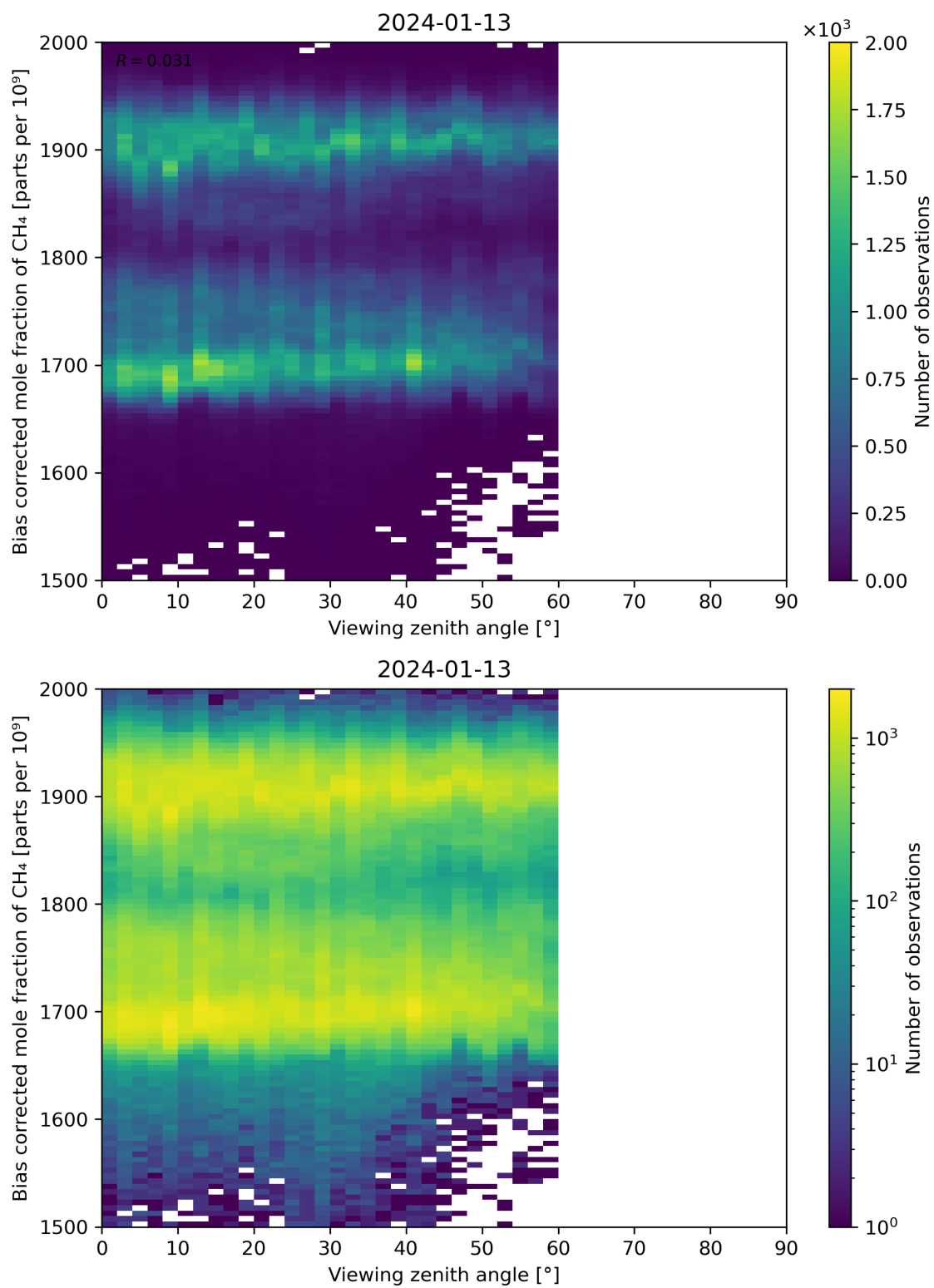
Figure 111: Scatter density plot of “Viewing zenith angle” against “Bias corrected mole fraction of CH 4 ” for 2024-01-12 to 2024-01-14.
