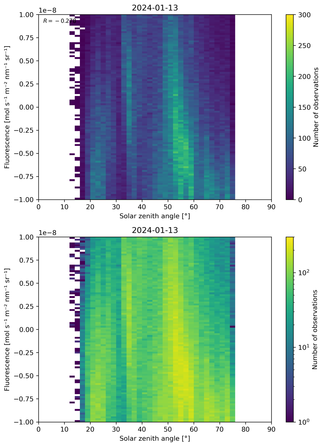
Figure 97: Scatter density plot of “Solar zenith angle” against “Fluorescence” for 2024-01-12 to 2024-01-14.
