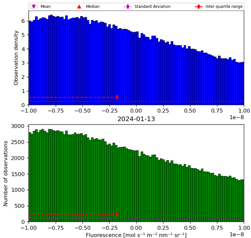
Figure 32: Histogram of “Fluorescence” for 2024-01-12 to 2024-01-14
