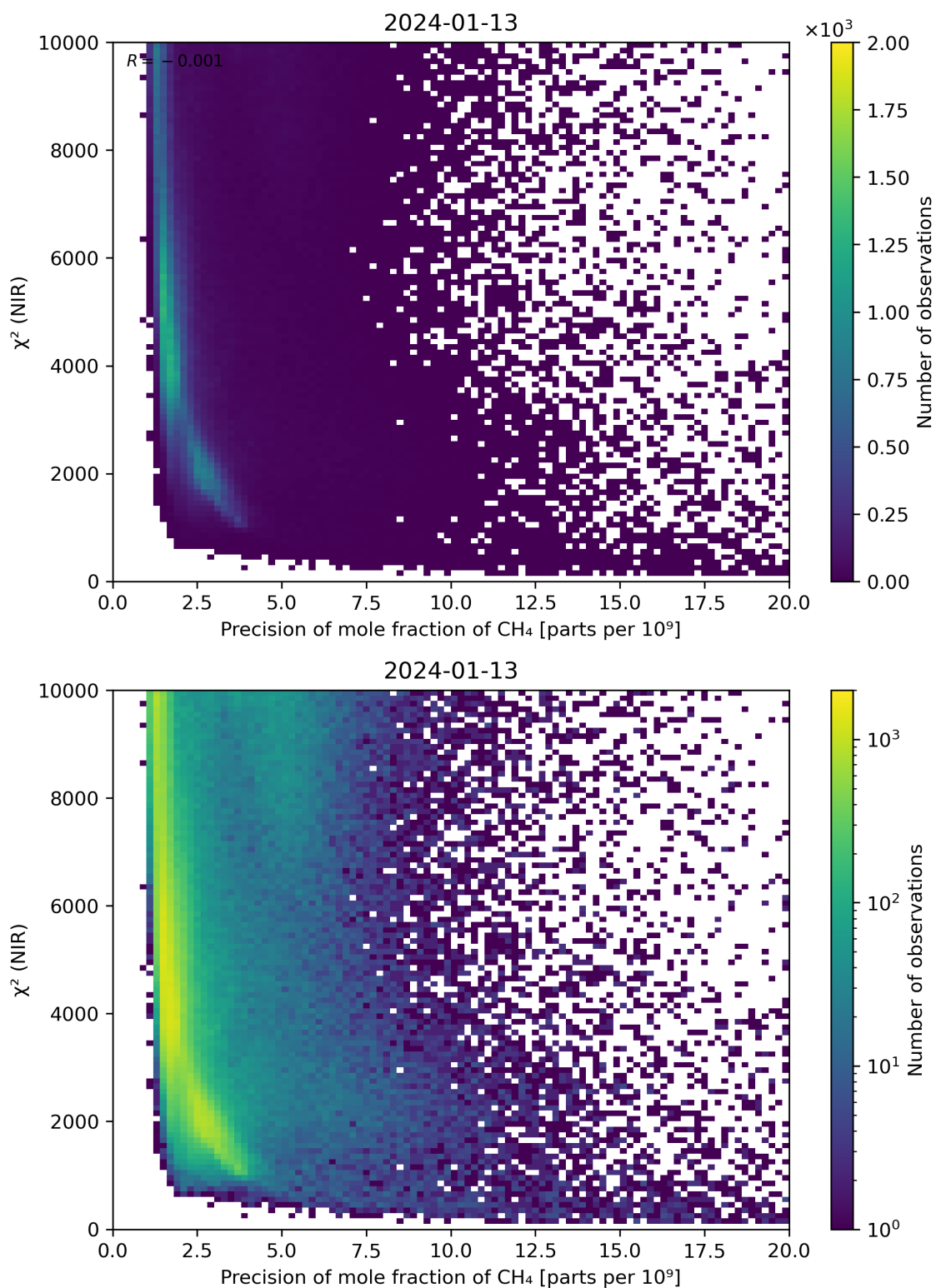
Figure 78: Scatter density plot of “Precision of mole fraction of CH 4 ” against “ \chi^2 (NIR)” for 2024-01-12 to 2024-01-14.
