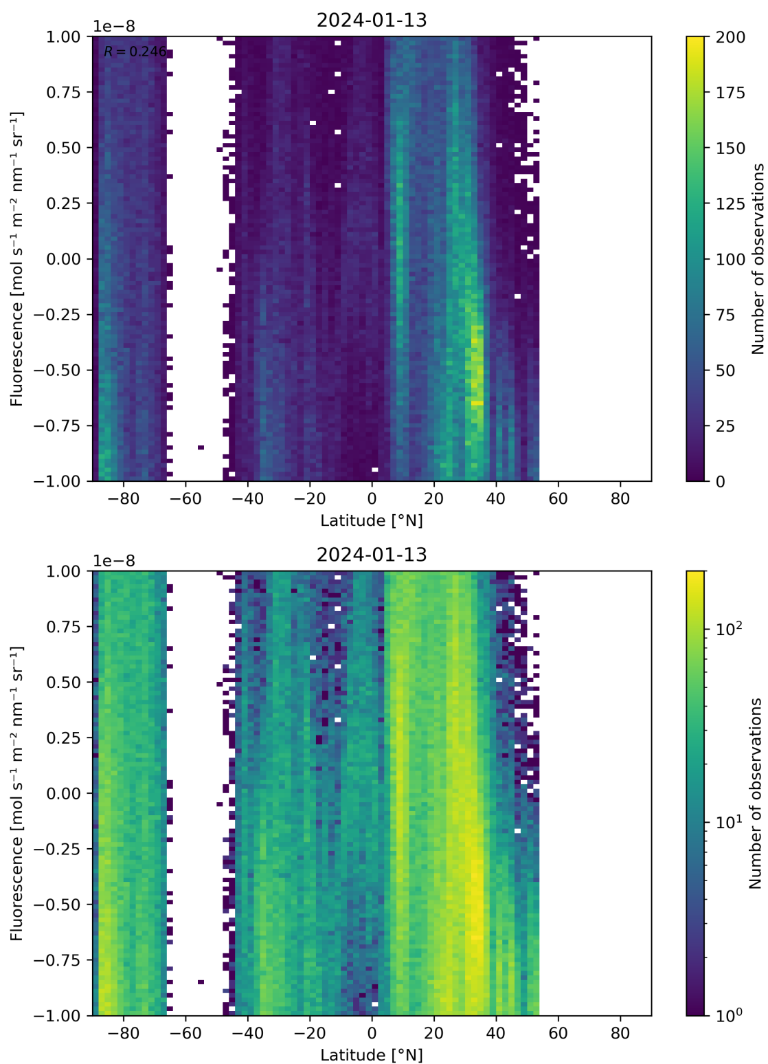
Figure 56: Scatter density plot of “Latitude” against “Fluorescence” for 2024-01-12 to 2024-01-14.
