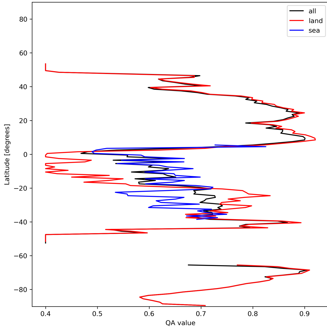
Figure 11: Zonal average of “QA value” for 2024-01-12 to 2024-01-14.
