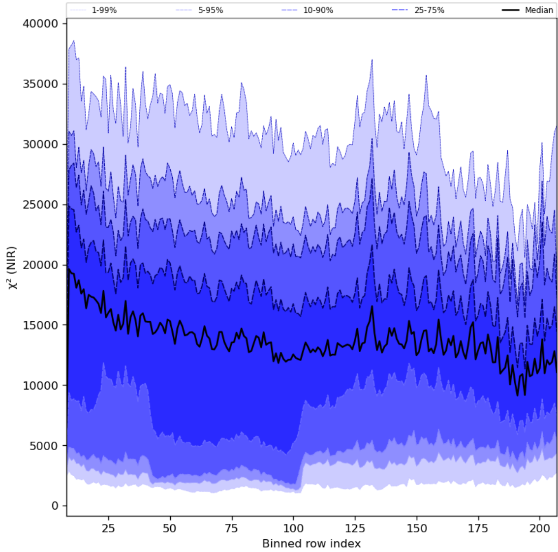
Figure 40: Along track statistics of " \chi^2 (NIR)" for 2024-01-12 to 2024-01-14
