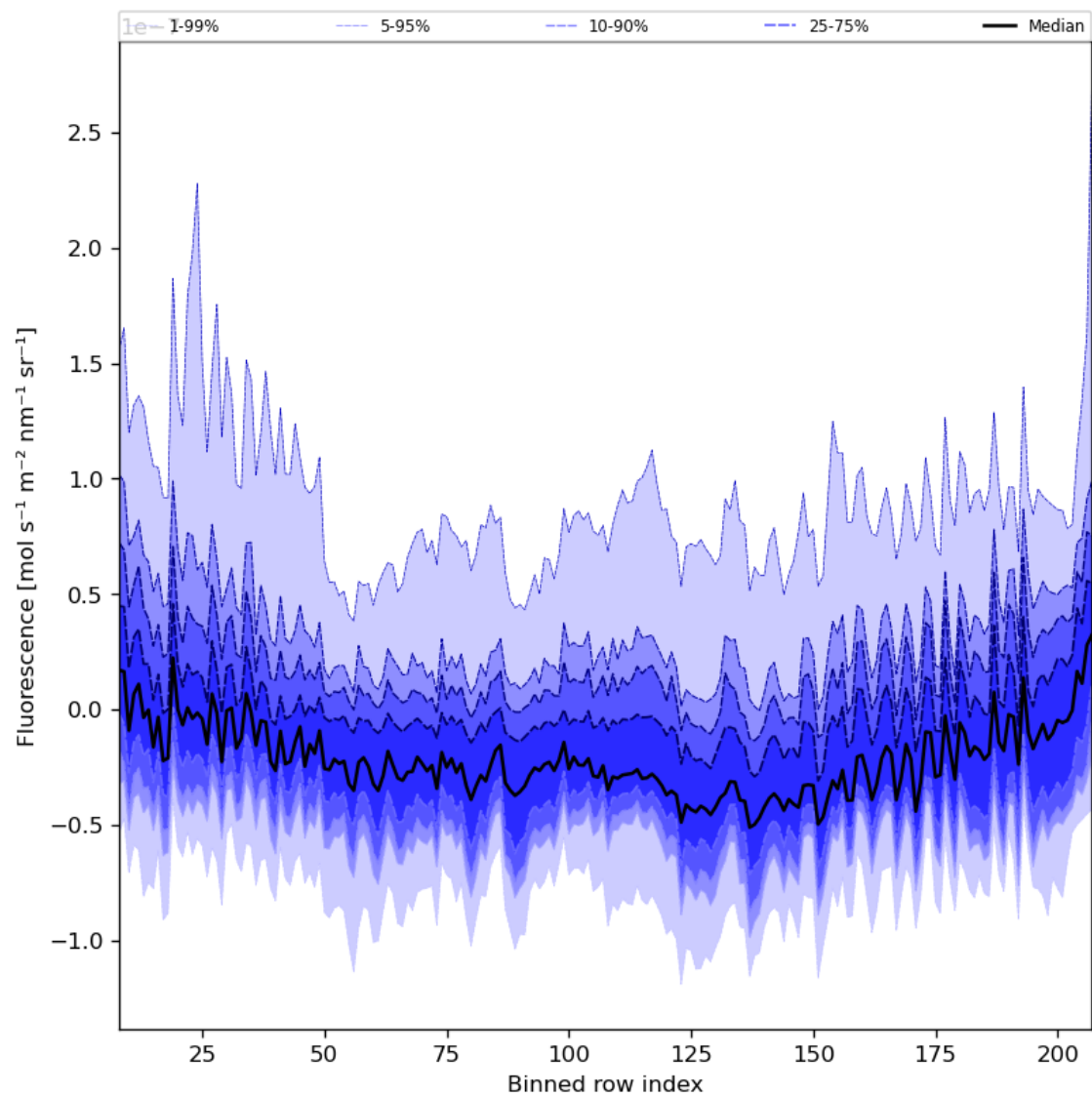
Figure 43: Along track statistics of “Fluorescence” for 2024-01-12 to 2024-01-14
