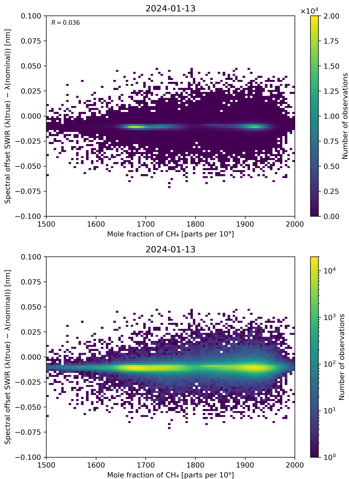
Figure 86: Scatter density plot of “Mole fraction of CH 4 ” against “Spectral offset SWIR ( \lambda(\text{true}) - \lambda(\text{nominal}) )” for 2024-01-12 to 2024-01-14.
