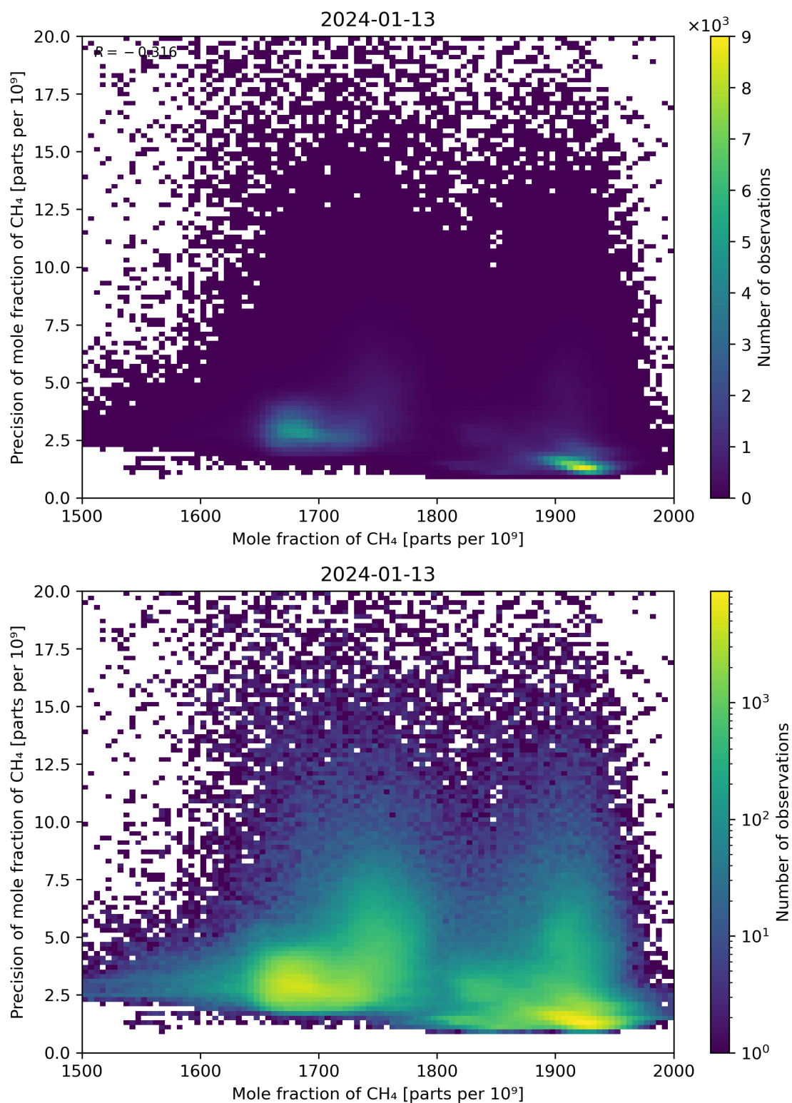
Figure 75: Scatter density plot of “Mole fraction of CH 4 ” against “Precision of mole fraction of CH 4 ” for 2024-01-12 to 2024-01-14.
