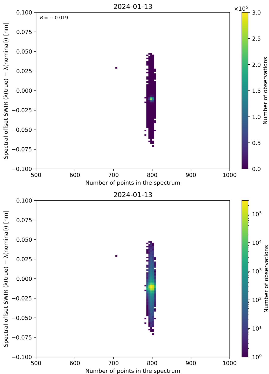
Figure 93: Scatter density plot of “Number of points in the spectrum” against “Spectral offset SWIR ( \lambda(\text{true}) - \lambda(\text{nominal}) )” for 2024-01-12 to 2024-01-14.
