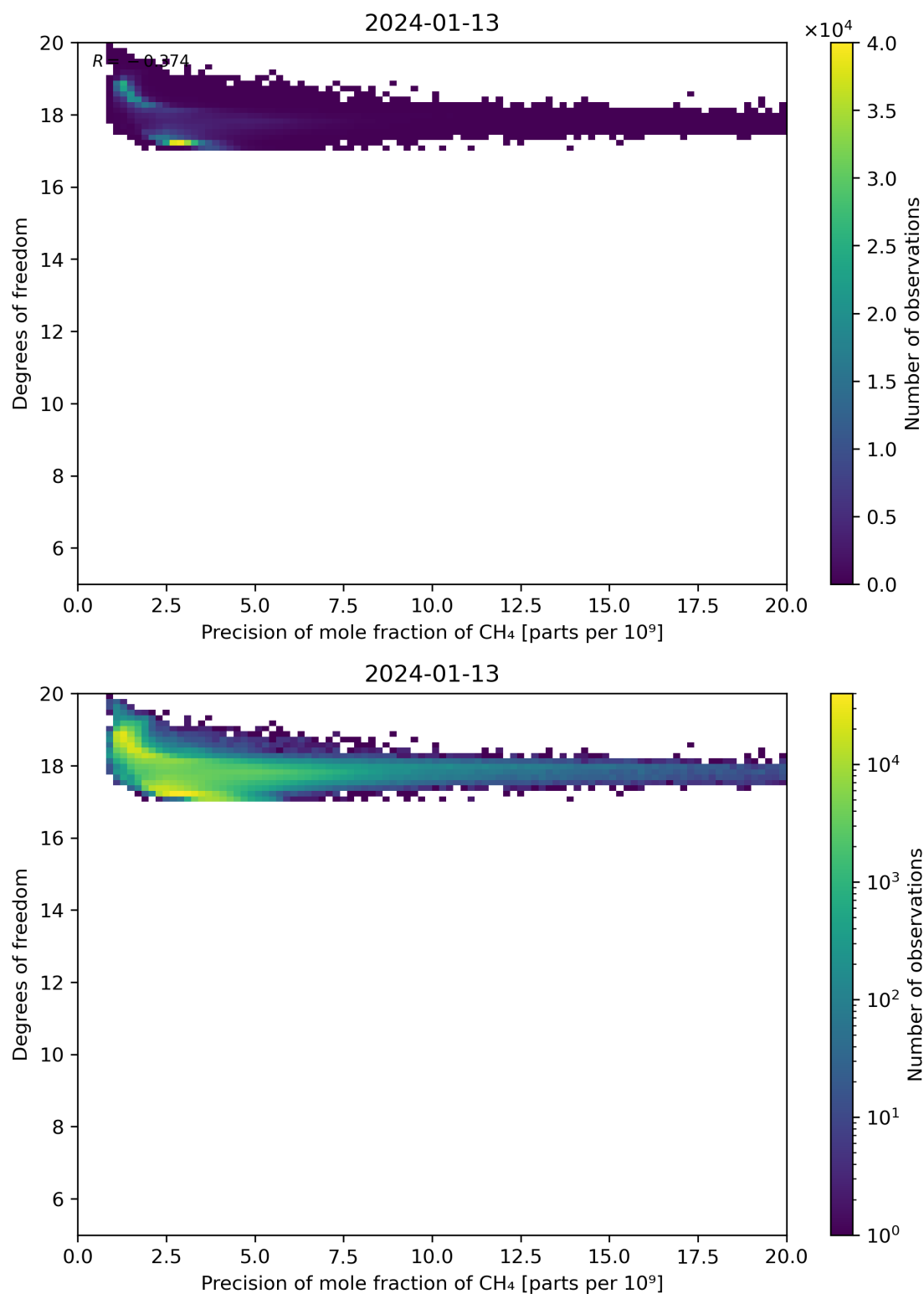
Figure 80: Scatter density plot of “Precision of mole fraction of CH 4 ” against “Degrees of freedom” for 2024-01-12 to 2024-01-14.
