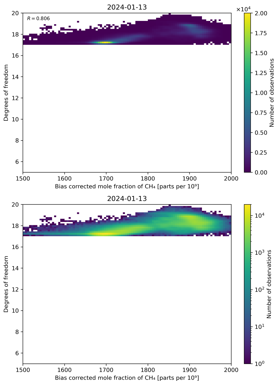
Figure 65: Scatter density plot of “Bias corrected mole fraction of CH 4 ” against “Degrees of freedom” for 2024-01-12 to 2024-01-14.
