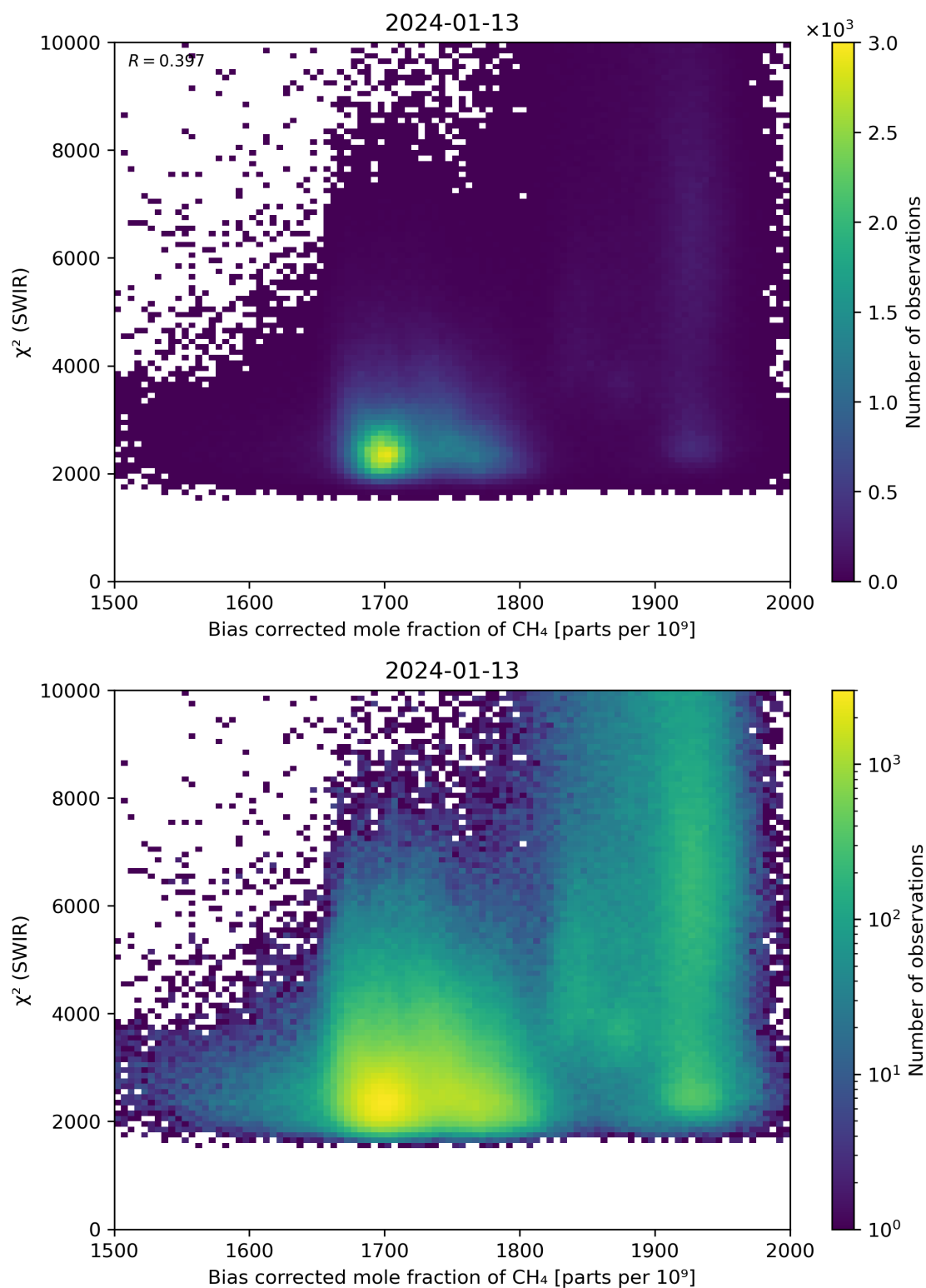
Figure 64: Scatter density plot of “Bias corrected mole fraction of \text{CH}_4 ” against “ \chi^2 (SWIR)” for 2024-01-12 to 2024-01-14.
