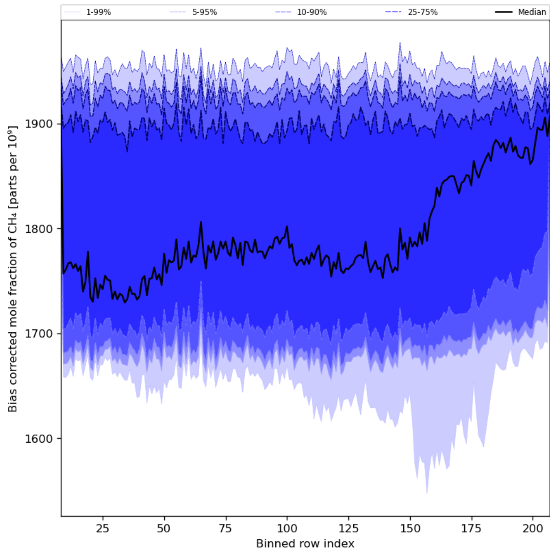
Figure 36: Along track statistics of “Bias corrected mole fraction of CH 4 ” for 2024-01-12 to 2024-01-14
