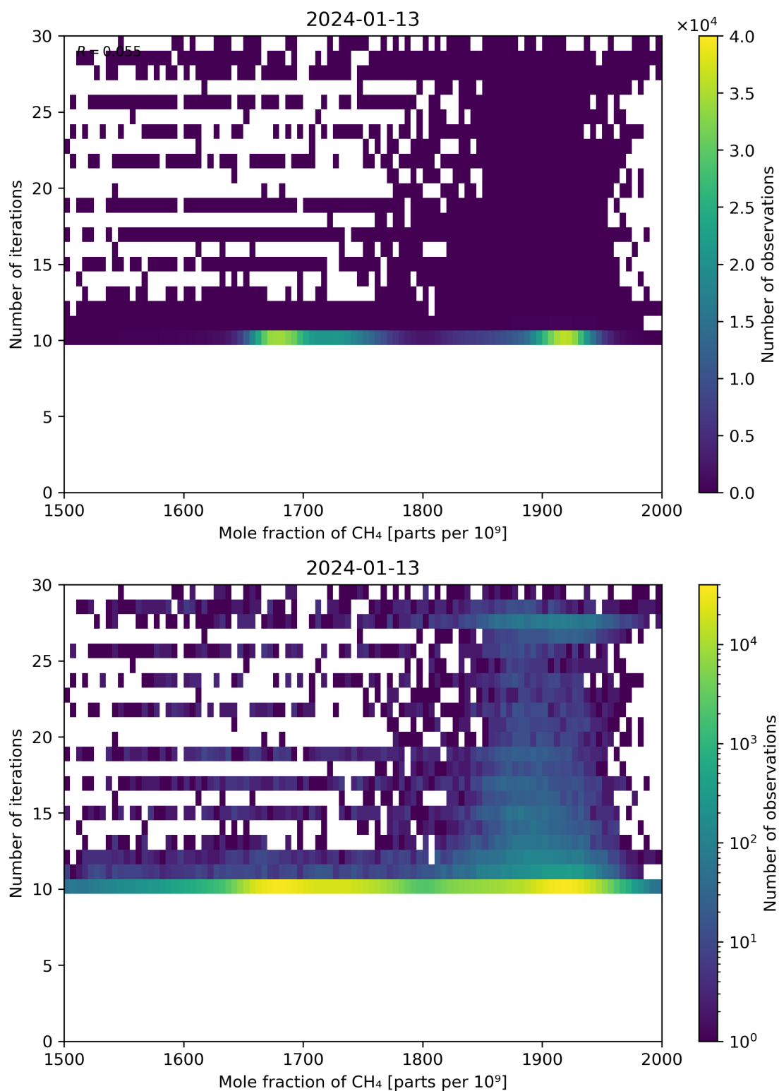
Figure 76: Scatter density plot of “Mole fraction of CH 4 ” against “Number of iterations” for 2024-01-12 to 2024-01-14.
