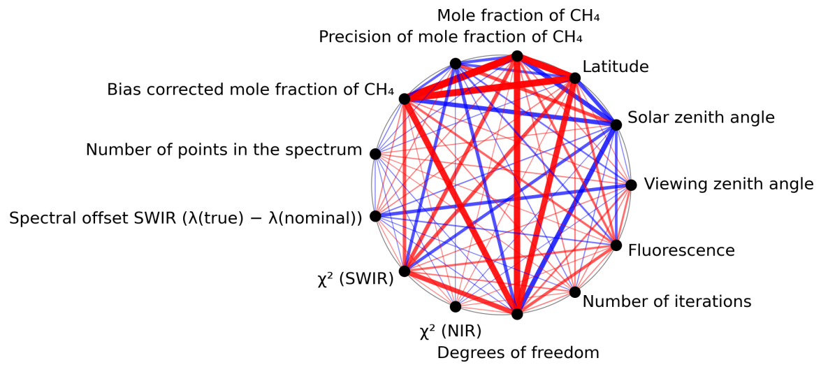
Figure 1: Map of correlation graph for 2024-01-12 to 2024-01-14.
