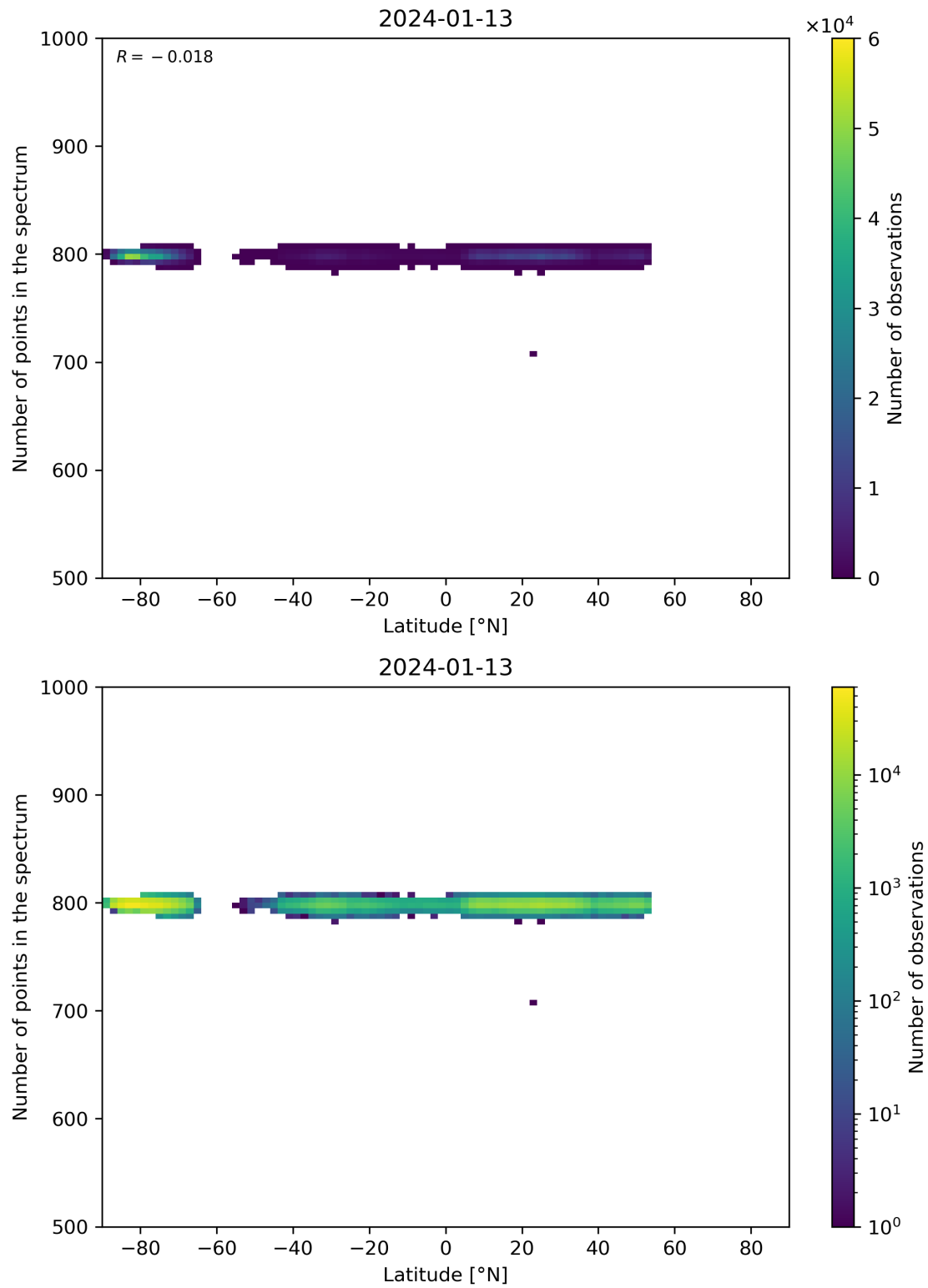
Figure 61: Scatter density plot of “Latitude” against “Number of points in the spectrum” for 2024-01-12 to 2024-01-14.
