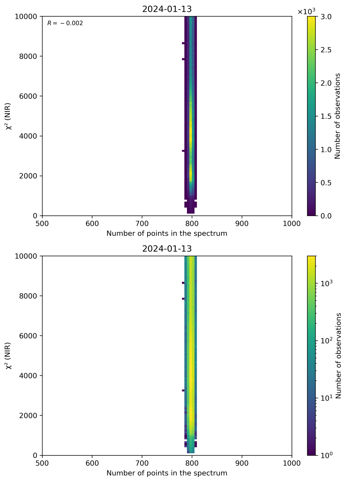
Figure 88: Scatter density plot of “Number of points in the spectrum” against “ \chi^2 (NIR)” for 2024-01-12 to 2024-01-14.
