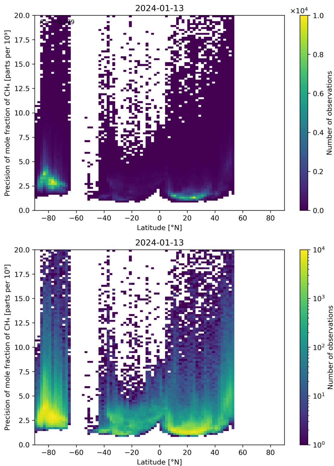
Figure 59: Scatter density plot of “Latitude” against “Precision of mole fraction of CH 4 ” for 2024-01-12 to 2024-01-14.
