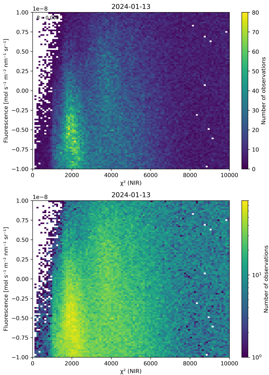
Figure 45: Scatter density plot of “ \chi^2 (NIR)” against “Fluorescence” for 2024-01-12 to 2024-01-14.
