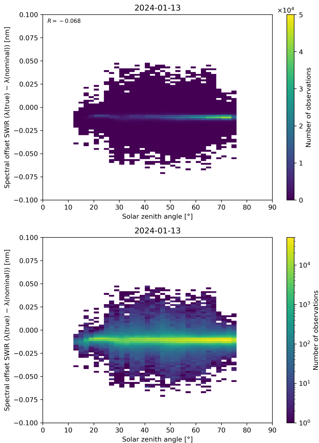
Figure 104: Scatter density plot of “Solar zenith angle” against “Spectral offset SWIR ( \lambda(\text{true}) - \lambda(\text{nominal}) )” for 2024-01-12 to 2024-01-14.
