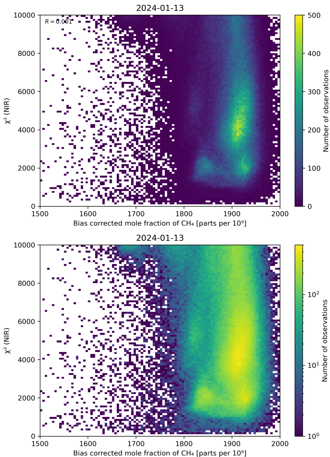
Figure 63: Scatter density plot of “Bias corrected mole fraction of CH 4 ” against “ \chi^2 (NIR)” for 2024-01-12 to 2024-01-14.
