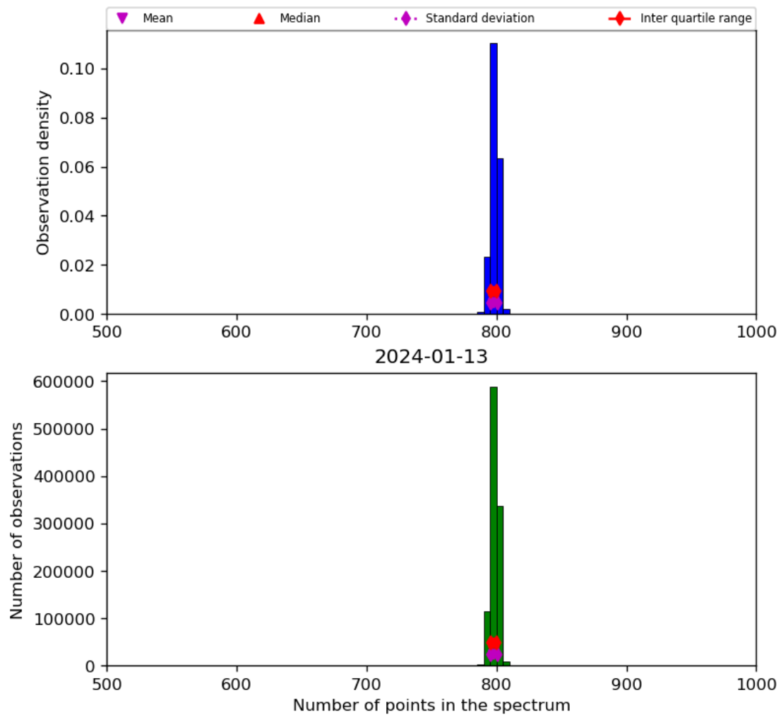
Figure 26: Histogram of “Number of points in the spectrum” for 2024-01-12 to 2024-01-14
