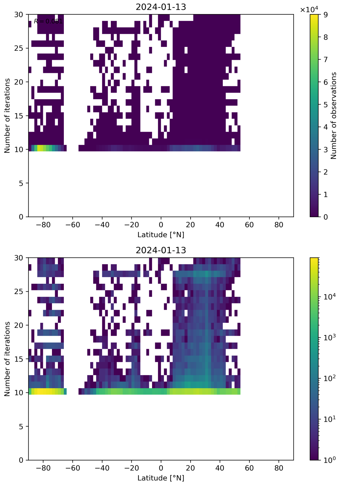
Figure 60: Scatter density plot of “Latitude” against “Number of iterations” for 2024-01-12 to 2024-01-14.
