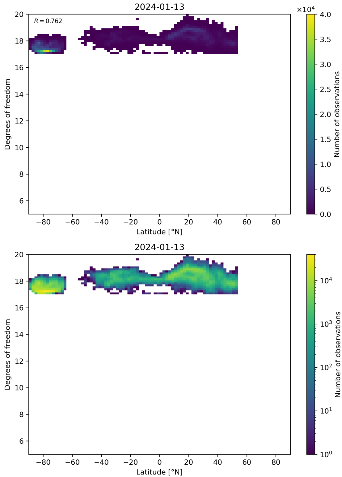
Figure 55: Scatter density plot of “Latitude” against “Degrees of freedom” for 2024-01-12 to 2024-01-14.
