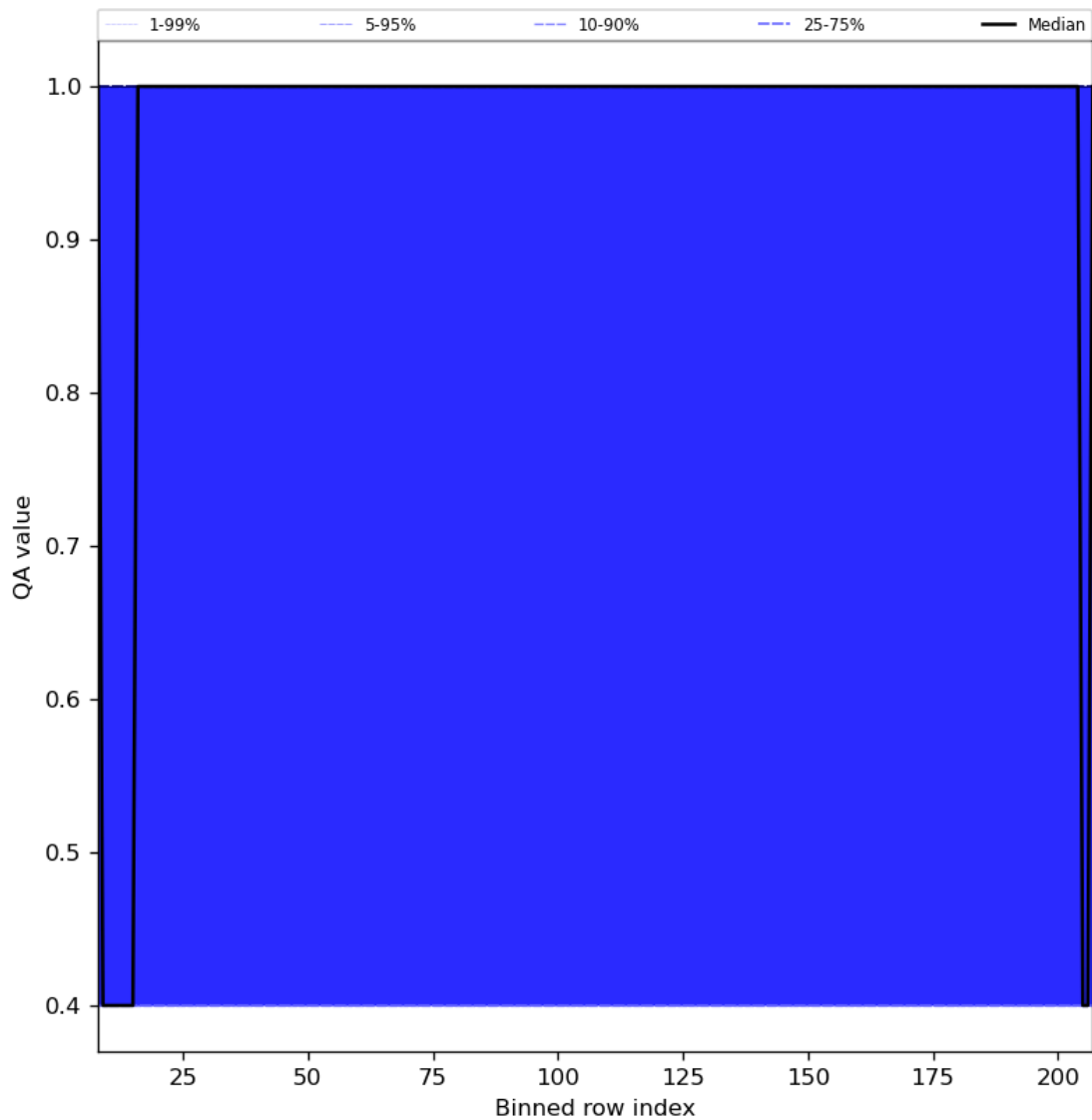
Figure 33: Along track statistics of “QA value” for 2024-01-12 to 2024-01-14
