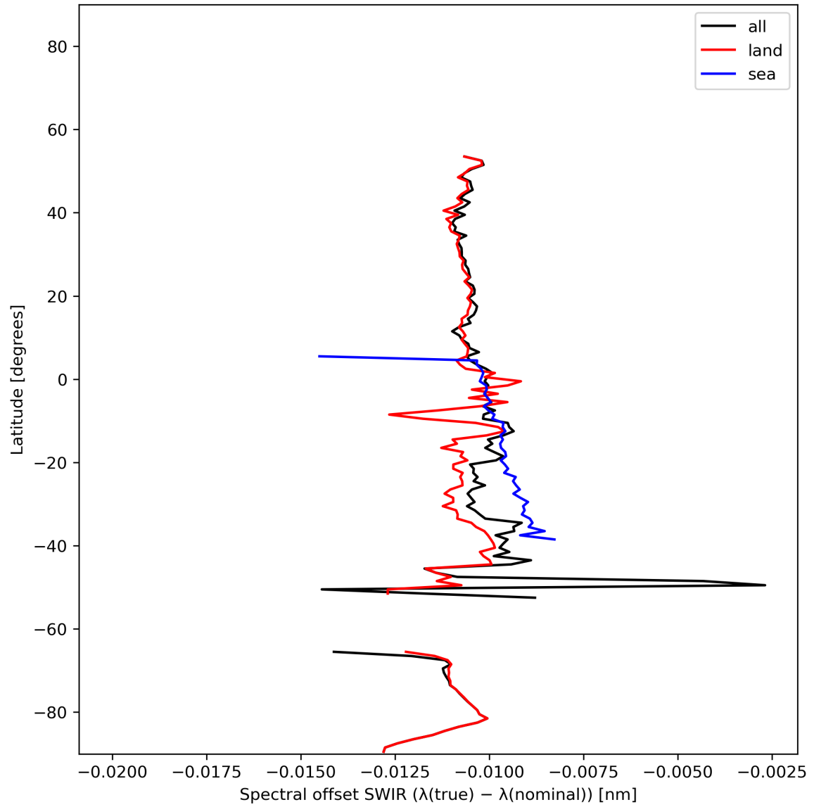
Figure 16: Zonal average of “Spectral offset SWIR ( \lambda(\text{true}) - \lambda(\text{nominal}) )” for 2024-01-12 to 2024-01-14.
