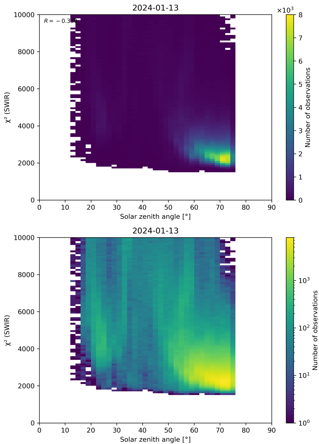
Figure 95: Scatter density plot of “Solar zenith angle” against “ \chi^2 (SWIR)” for 2024-01-12 to 2024-01-14.
