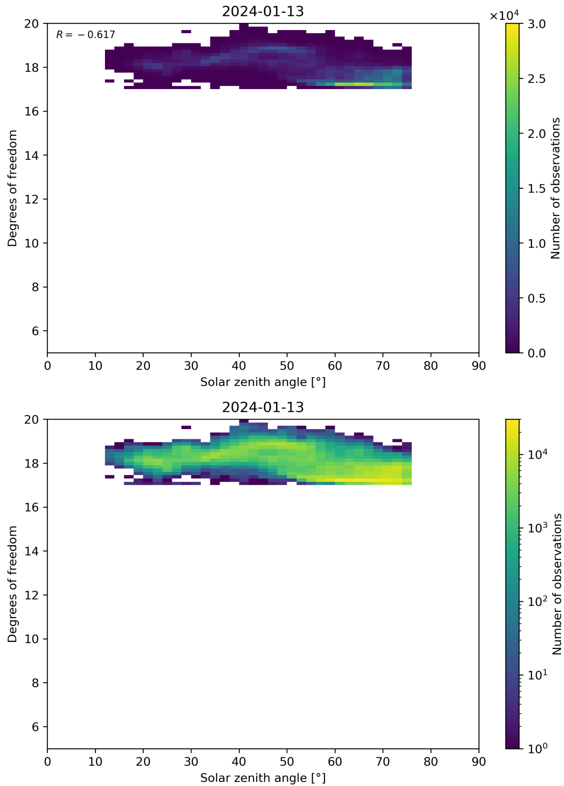
Figure 96: Scatter density plot of “Solar zenith angle” against “Degrees of freedom” for 2024-01-12 to 2024-01-14.
