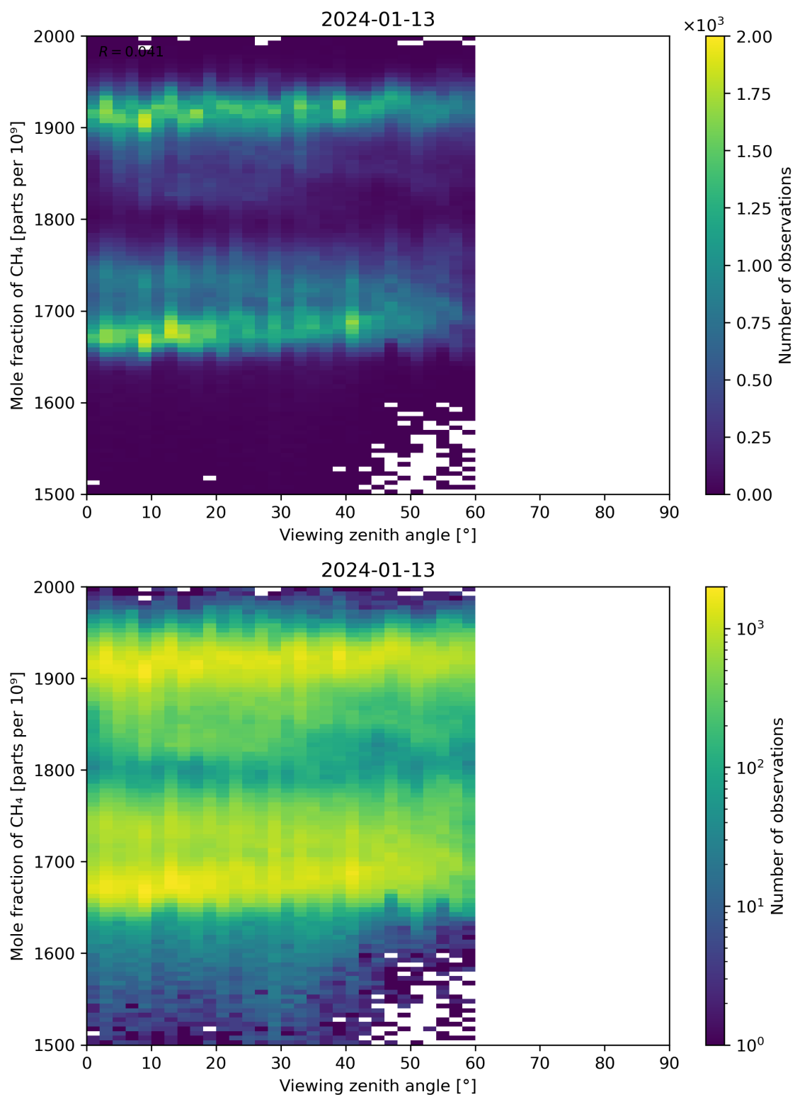
Figure 110: Scatter density plot of “Viewing zenith angle” against “Mole fraction of CH 4 ” for 2024-01-12 to 2024-01-14.
