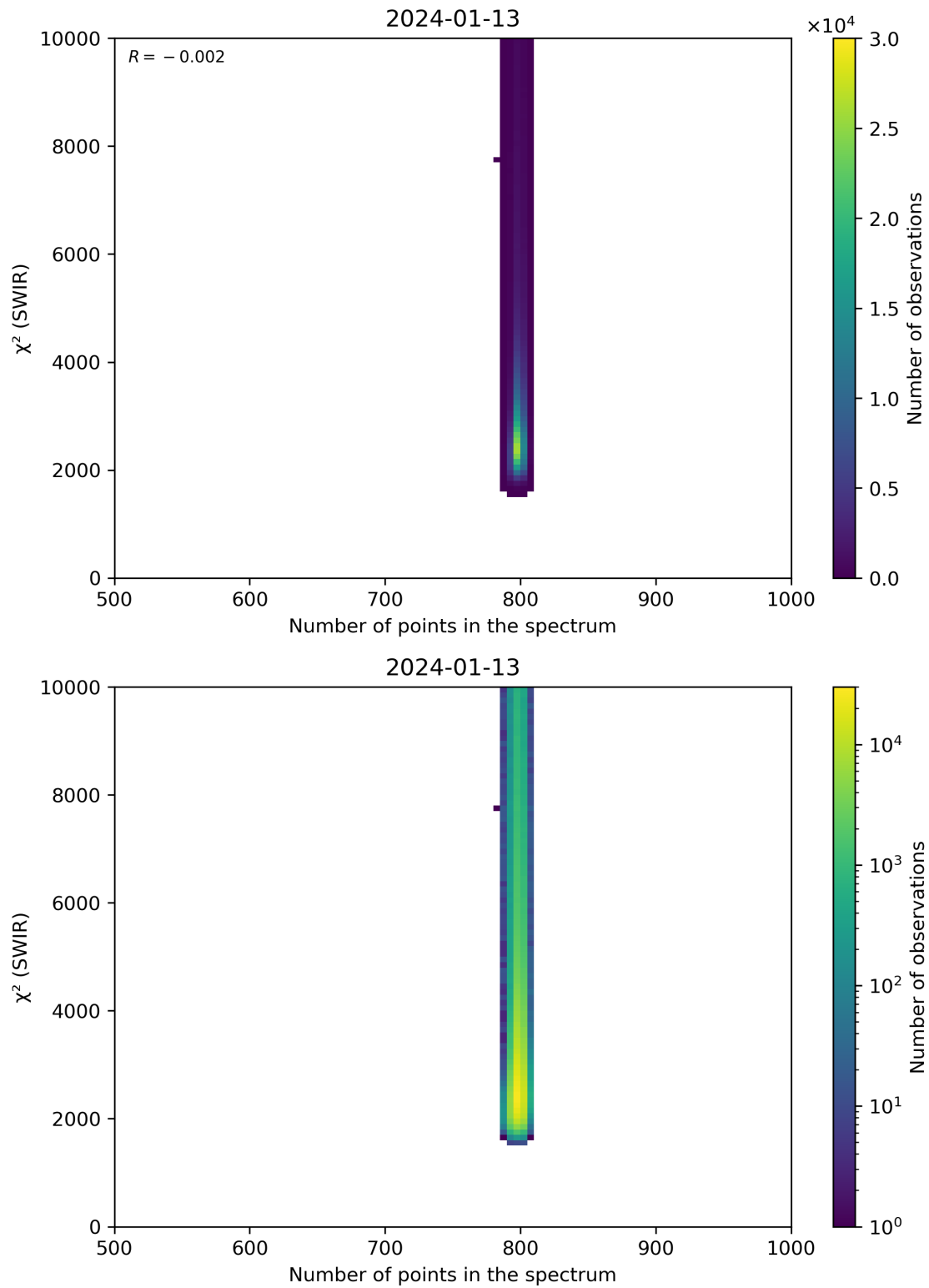
Figure 89: Scatter density plot of “Number of points in the spectrum” against “ \chi^2 (SWIR)” for 2024-01-12 to 2024-01-14.
