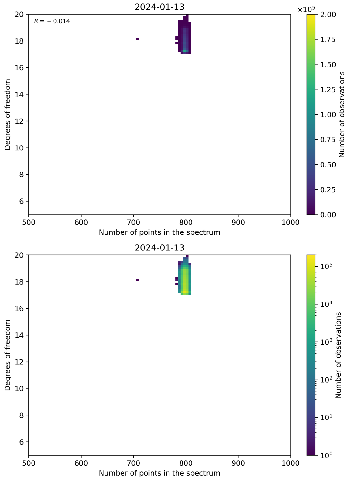
Figure 90: Scatter density plot of “Number of points in the spectrum” against “Degrees of freedom” for 2024-01-12 to 2024-01-14.
