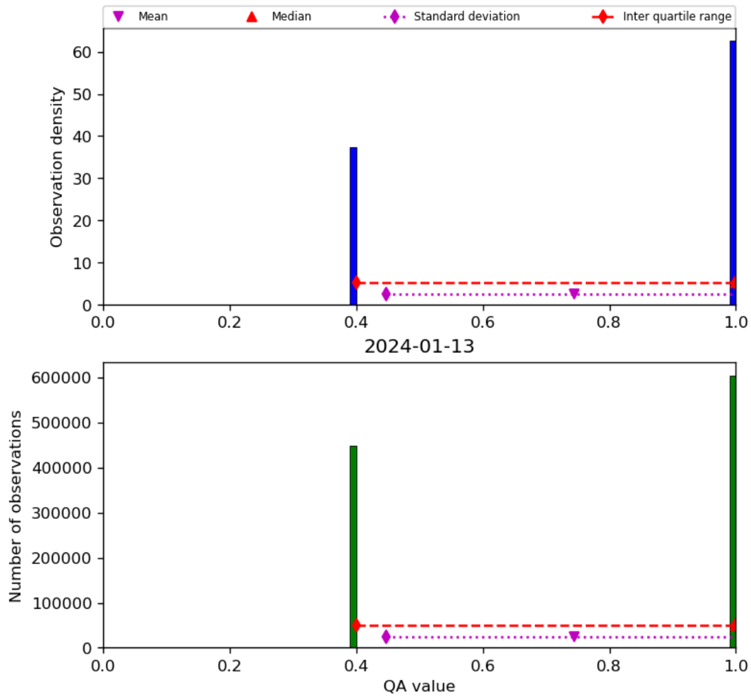
Figure 22: Histogram of “QA value” for 2024-01-12 to 2024-01-14
