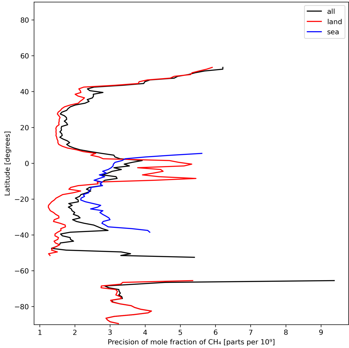
Figure 13: Zonal average of “Precision of mole fraction of CH 4 ” for 2024-01-12 to 2024-01-14.
