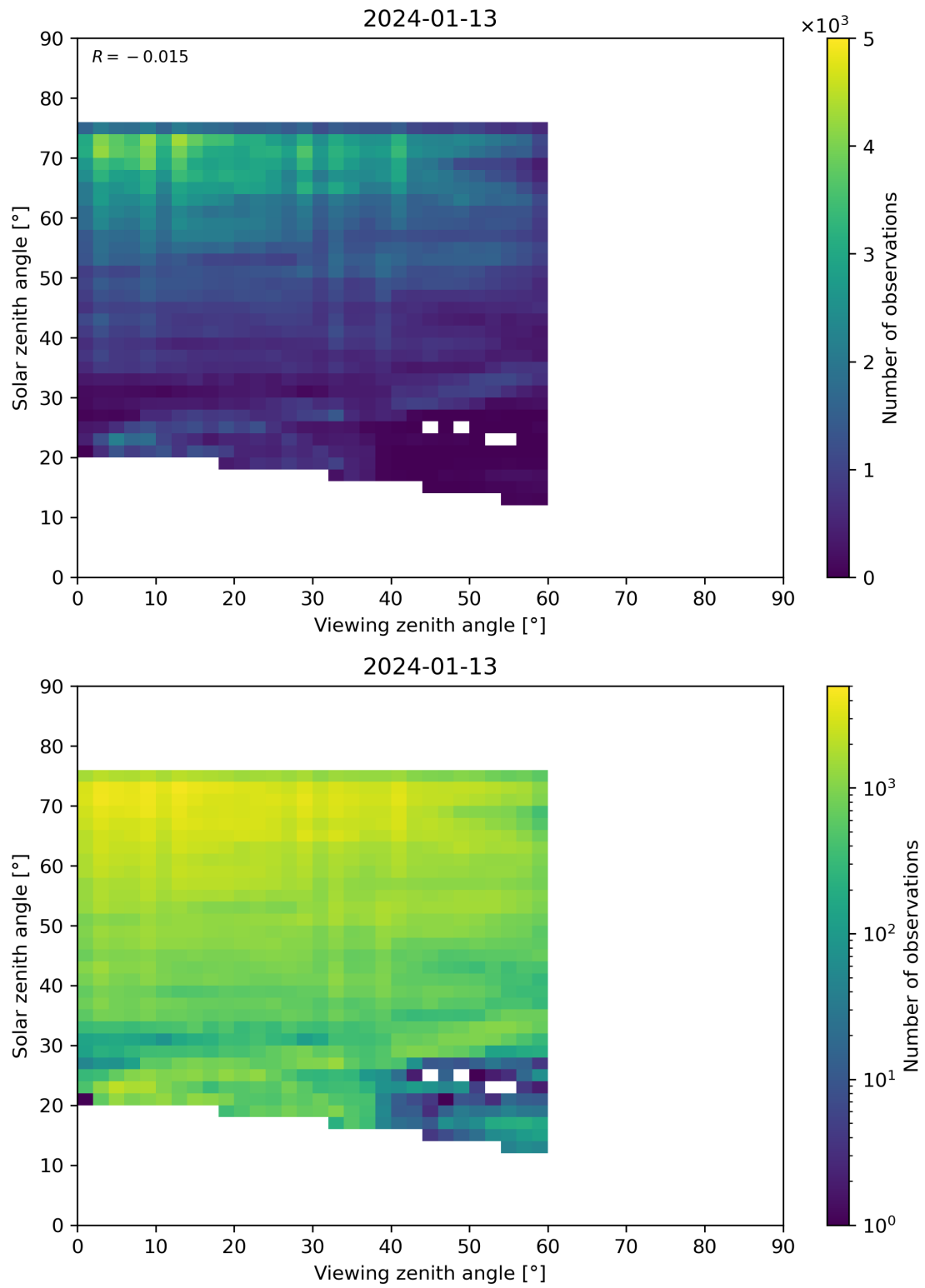
Figure 115: Scatter density plot of “Viewing zenith angle” against “Solar zenith angle” for 2024-01-12 to 2024-01-14.
