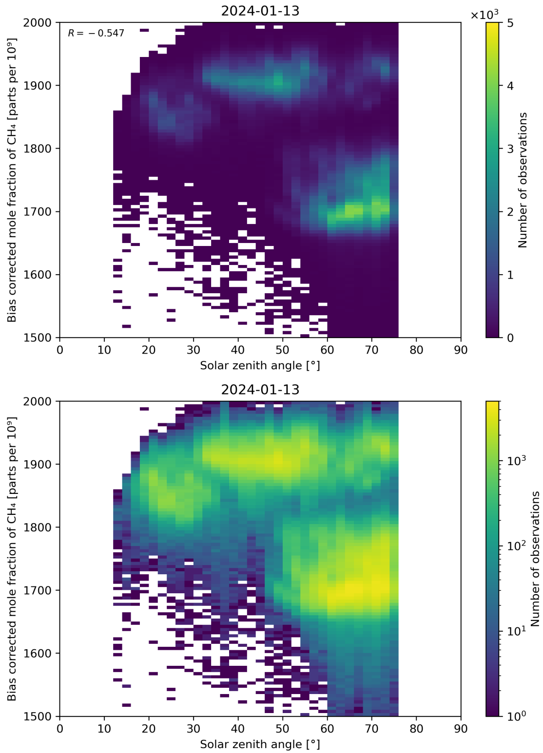
Figure 100: Scatter density plot of “Solar zenith angle” against “Bias corrected mole fraction of \text{CH}_4 ” for 2024-01-12 to 2024-01-14.
