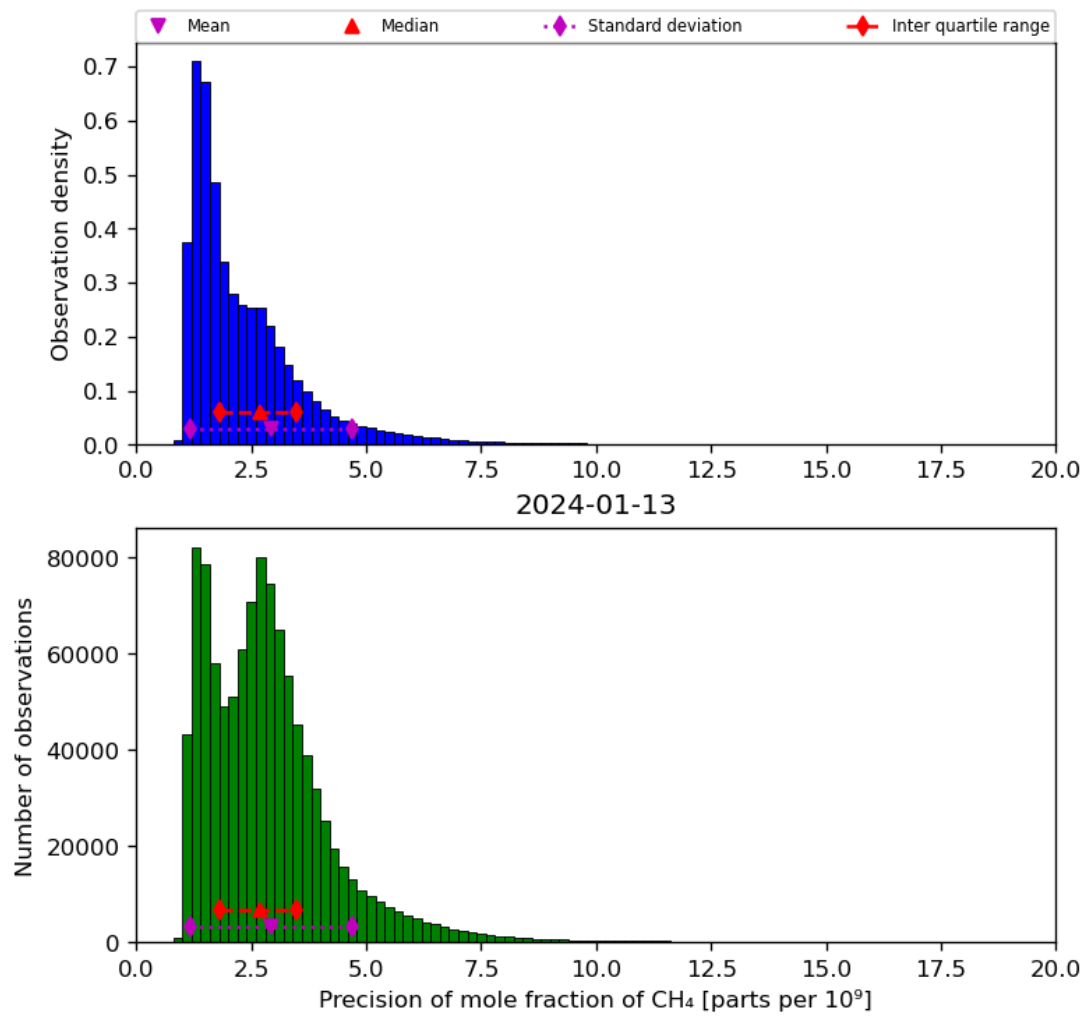
Figure 24: Histogram of “Precision of mole fraction of CH 4 ” for 2024-01-12 to 2024-01-14
