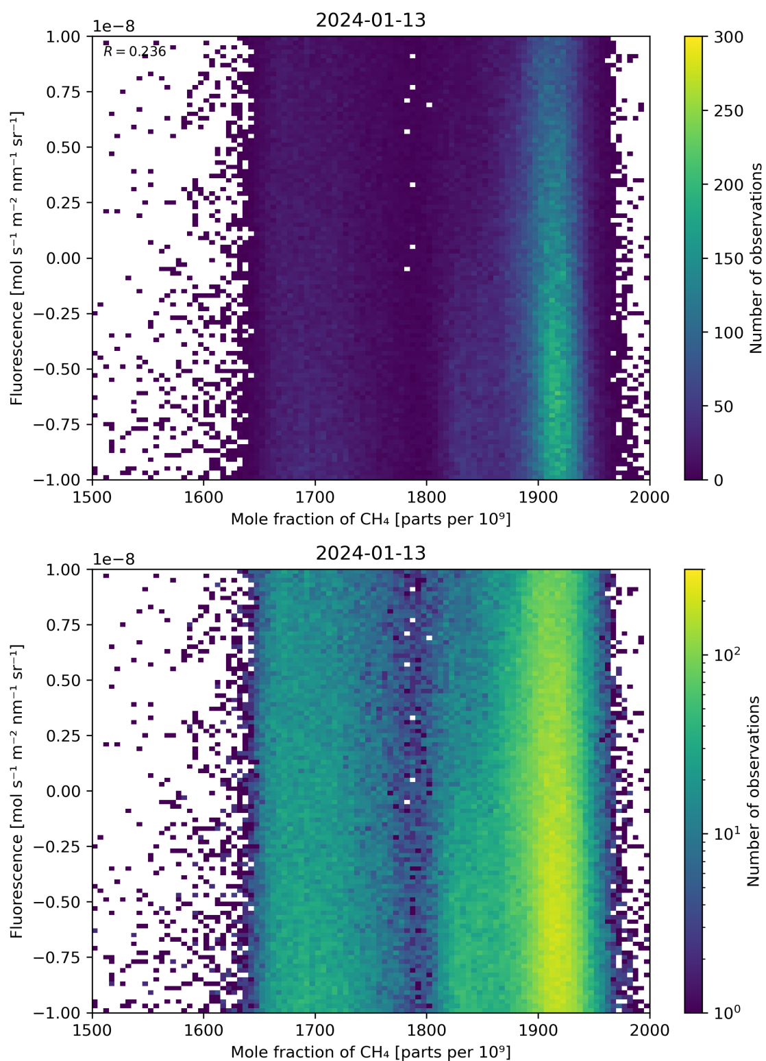
Figure 73: Scatter density plot of “Mole fraction of \text{CH}_4 ” against “Fluorescence” for 2024-01-12 to 2024-01-14.
