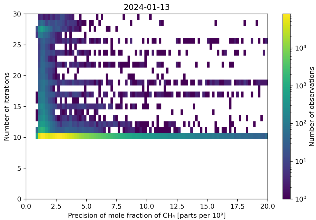
Figure 83: Scatter density plot of “Precision of mole fraction of CH 4 ” against “Number of iterations” for 2024-01-12 to 2024-01-14.
