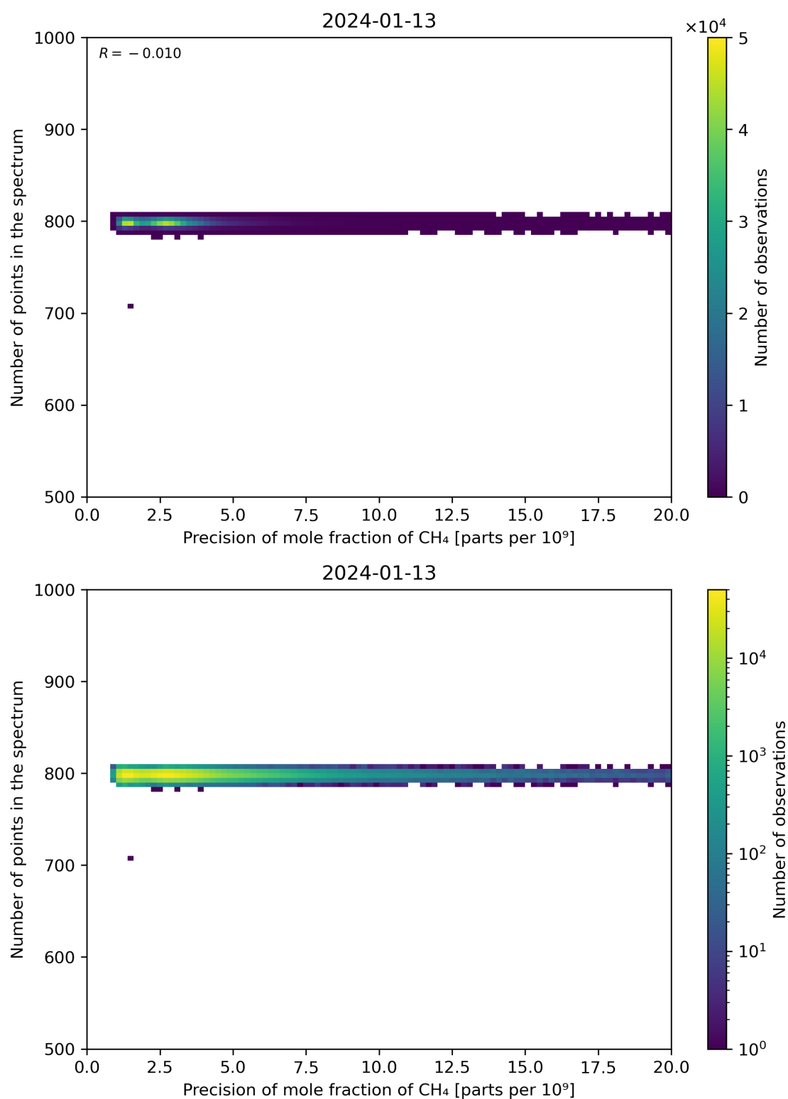
Figure 84: Scatter density plot of “Precision of mole fraction of CH 4 ” against “Number of points in the spectrum” for 2024-01-12 to 2024-01-14.
