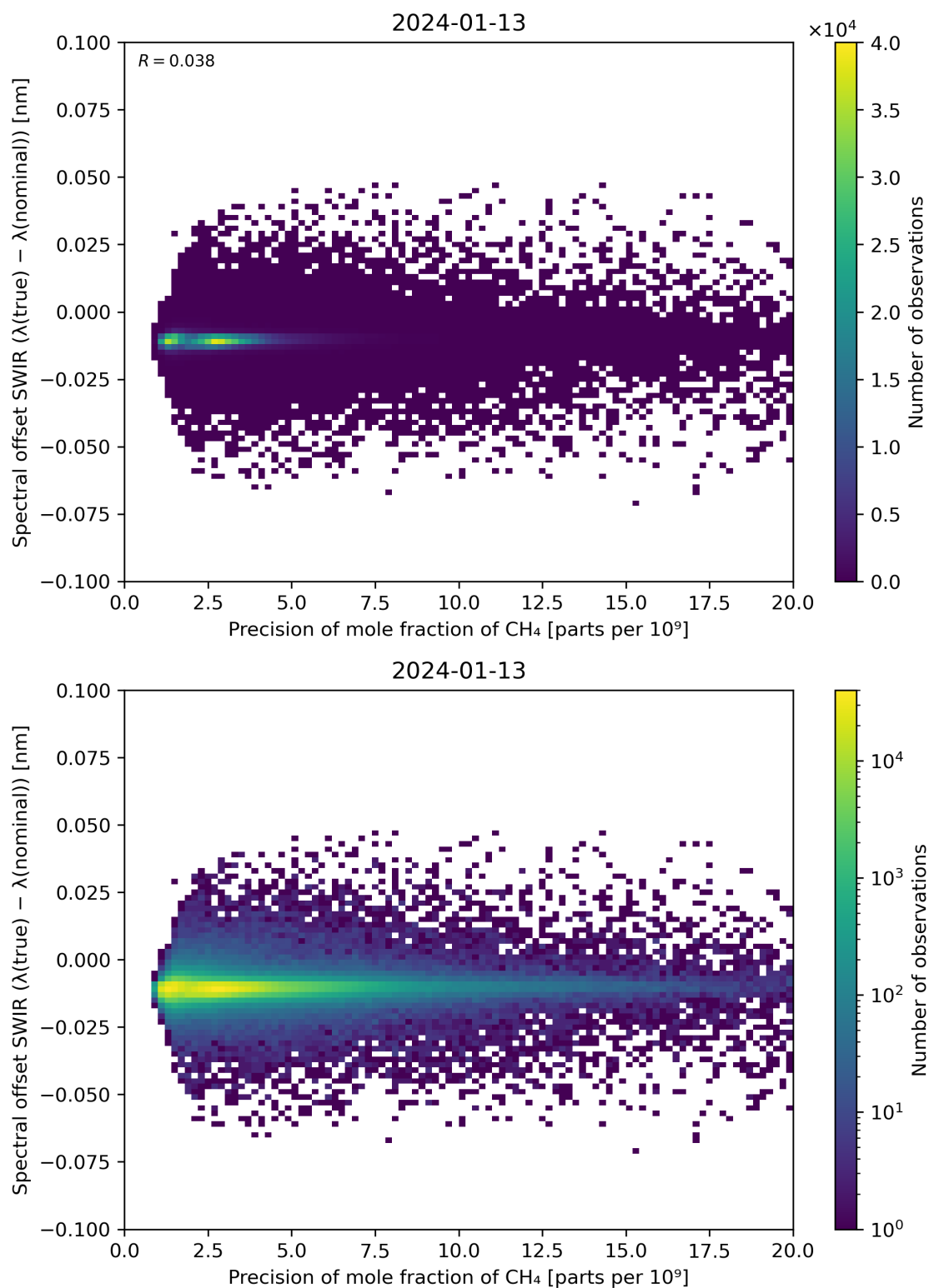
Figure 85: Scatter density plot of “Precision of mole fraction of \text{CH}_4 ” against “Spectral offset SWIR ( \lambda(\text{true}) - \lambda(\text{nominal}) )” for 2024-01-12 to 2024-01-14.
