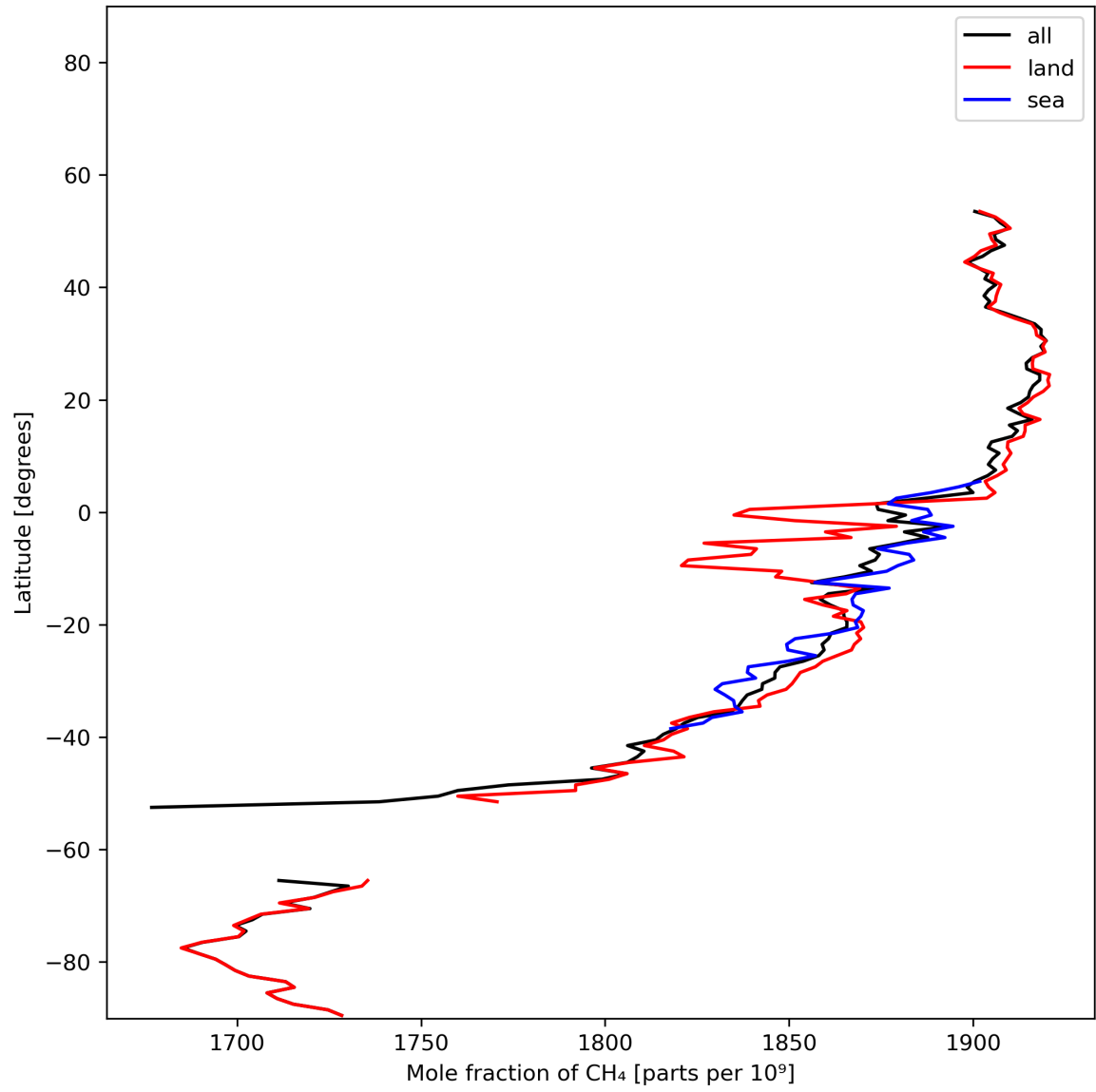
Figure 12: Zonal average of “Mole fraction of \text{CH}_4 ” for 2024-01-12 to 2024-01-14.
