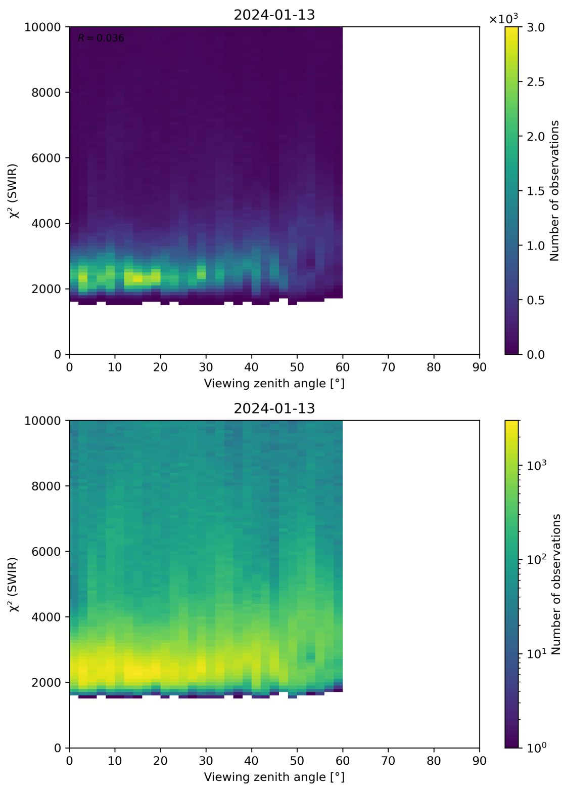
Figure 106: Scatter density plot of “Viewing zenith angle” against “ \chi^2 (SWIR)” for 2024-01-12 to 2024-01-14.
