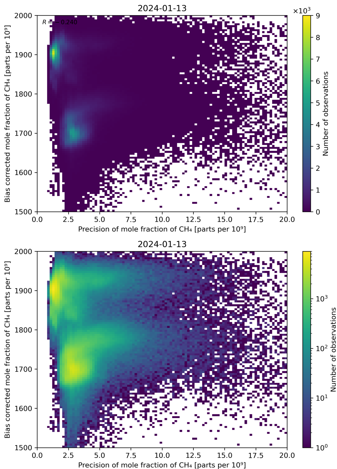
Figure 82: Scatter density plot of “Precision of mole fraction of CH 4 ” against “Bias corrected mole fraction of CH 4 ” for 2024-01-12 to 2024-01-14.
