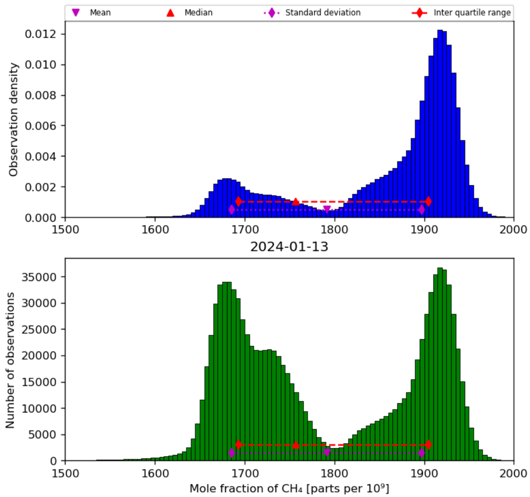
Figure 23: Histogram of “Mole fraction of CH 4 ” for 2024-01-12 to 2024-01-14
