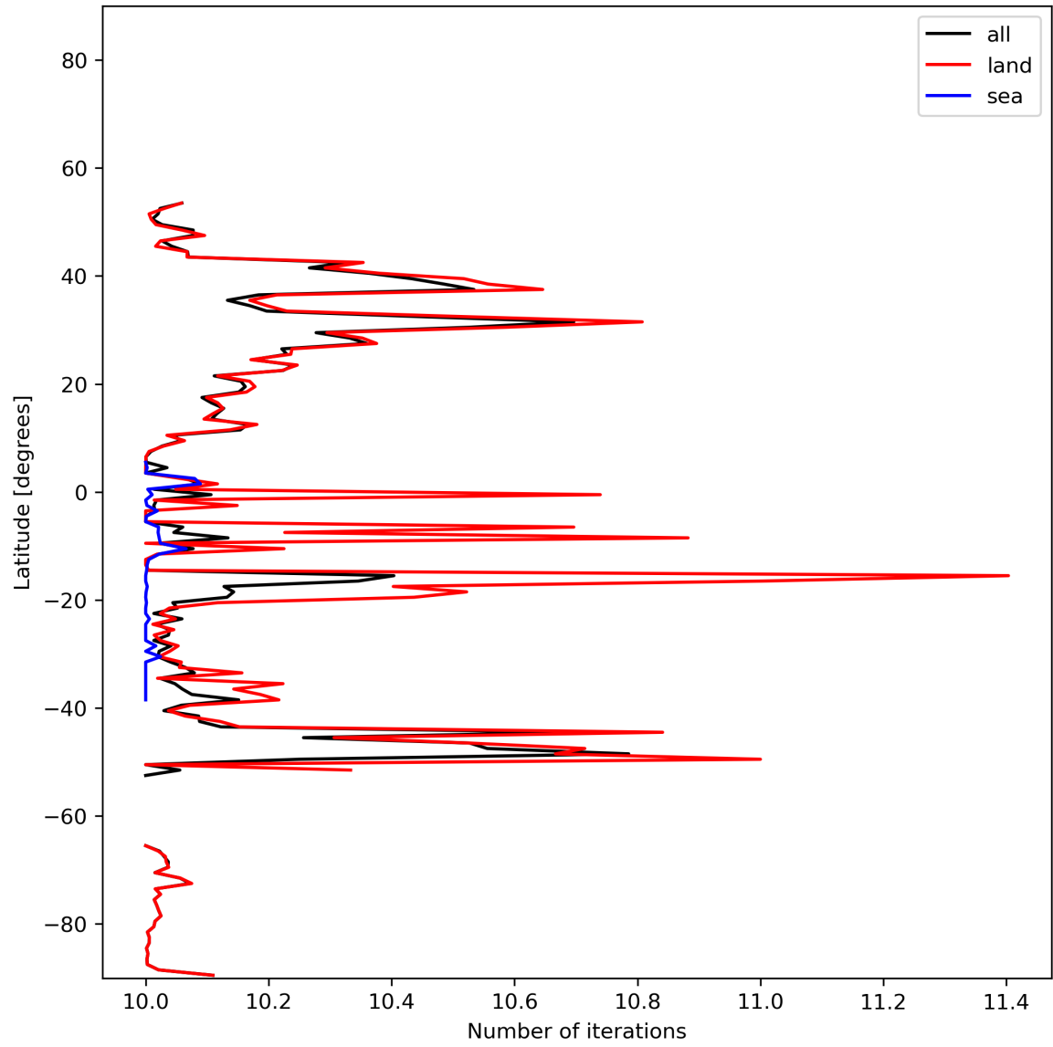
Figure 20: Zonal average of “Number of iterations” for 2024-01-12 to 2024-01-14.
