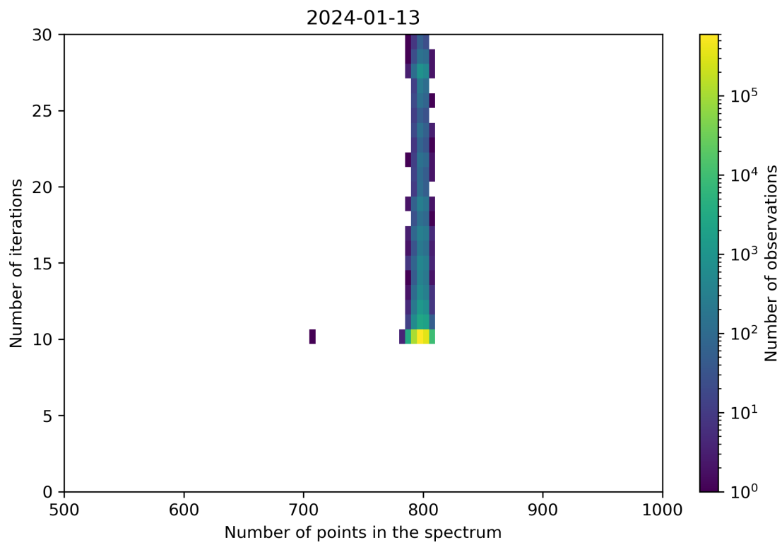
Figure 92: Scatter density plot of “Number of points in the spectrum” against “Number of iterations” for 2024-01-12 to 2024-01-14.
