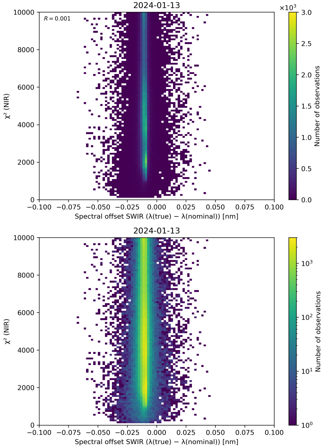
Figure 117: Scatter density plot of “Spectral offset SWIR ( \lambda(\text{true}) - \lambda(\text{nominal}) )” against “ \chi^2 (NIR)” for 2024-01-12 to 2024-01-14.
