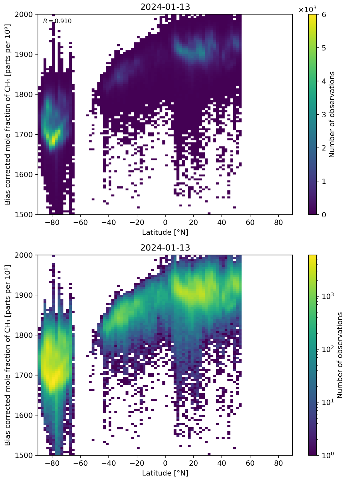
Figure 58: Scatter density plot of “Latitude” against “Bias corrected mole fraction of CH 4 ” for 2024-01-12 to 2024-01-14.
