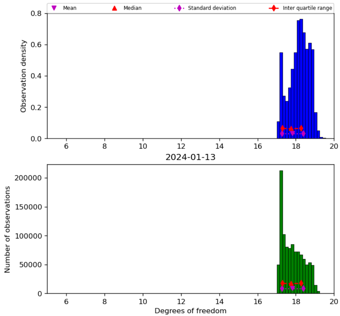
Figure 30: Histogram of “Degrees of freedom” for 2024-01-12 to 2024-01-14
