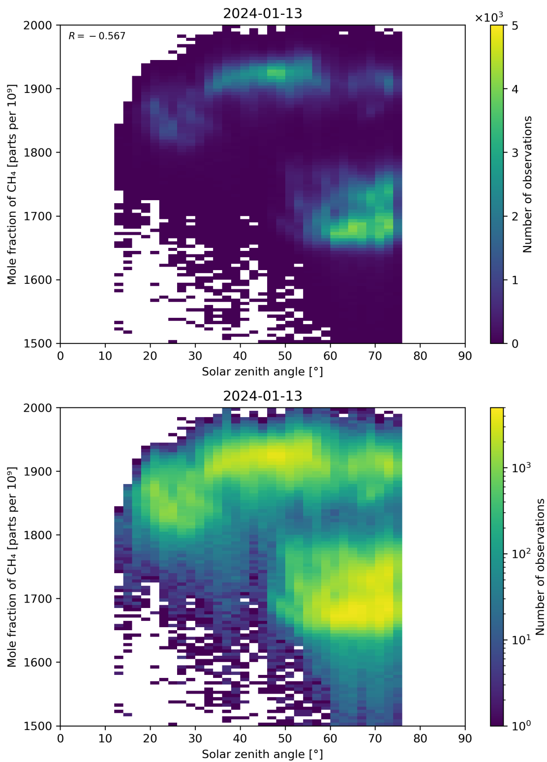
Figure 99: Scatter density plot of “Solar zenith angle” against “Mole fraction of CH 4 ” for 2024-01-12 to 2024-01-14.
