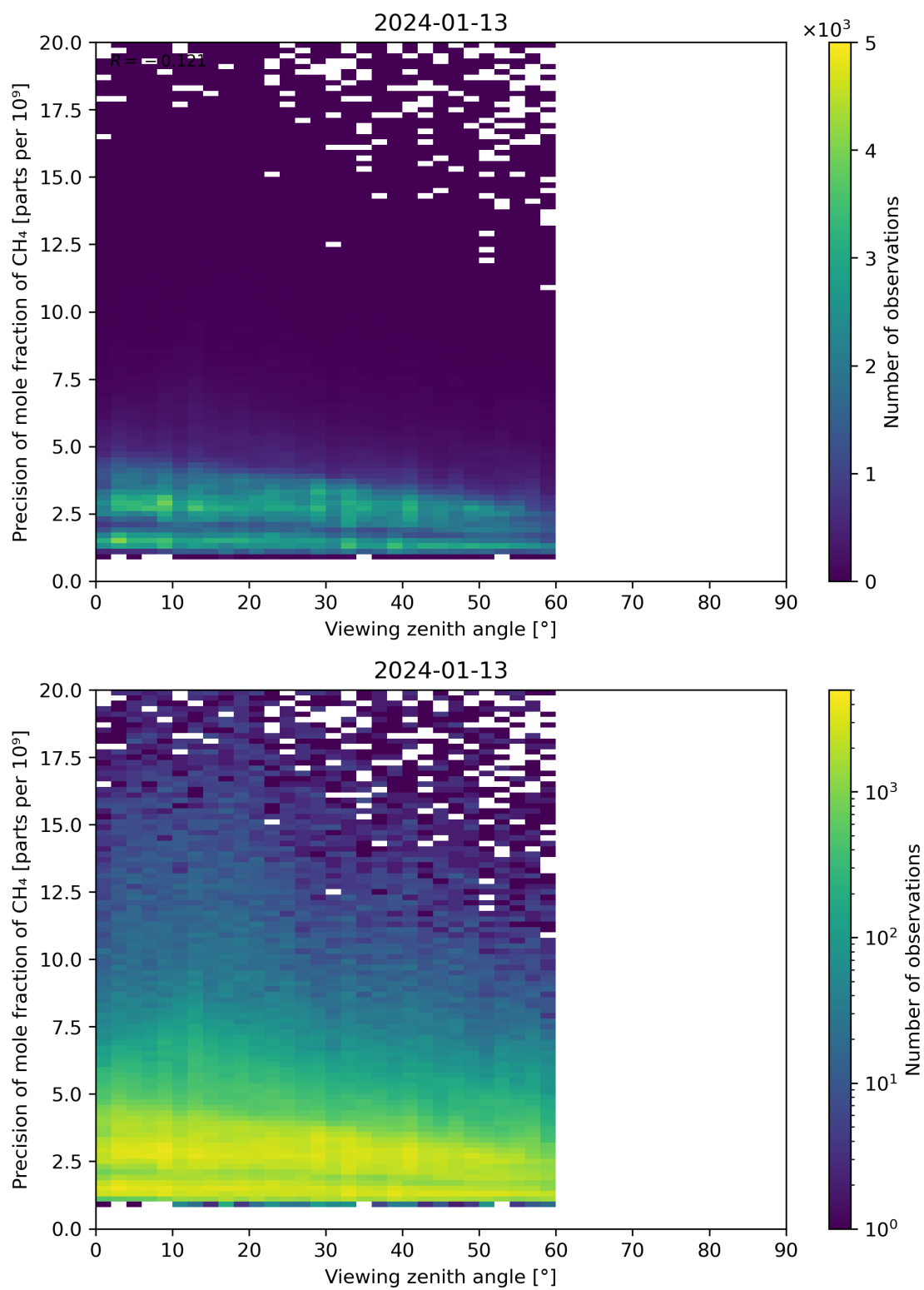
Figure 112: Scatter density plot of “Viewing zenith angle” against “Precision of mole fraction of CH 4 ” for 2024-01-12 to 2024-01-14.
