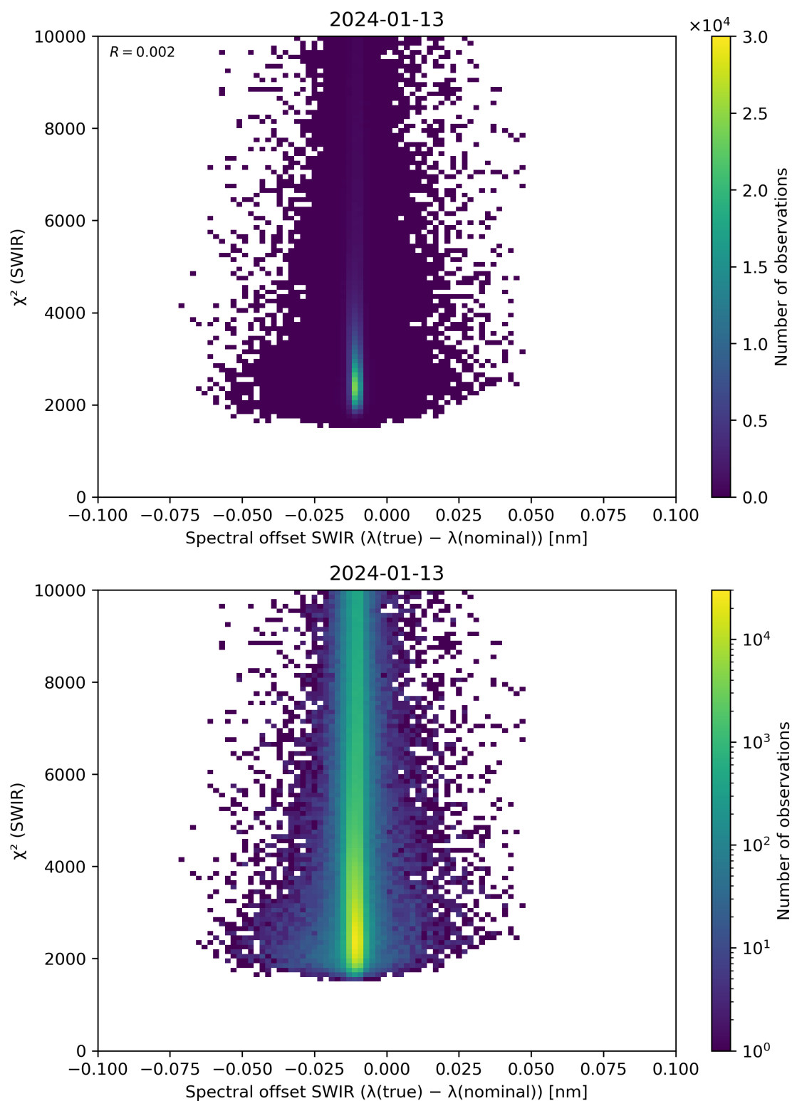
Figure 118: Scatter density plot of “Spectral offset SWIR ( \lambda(\text{true}) - \lambda(\text{nominal}) )” against “ \chi^2 (SWIR)” for 2024-01-12 to 2024-01-14.
