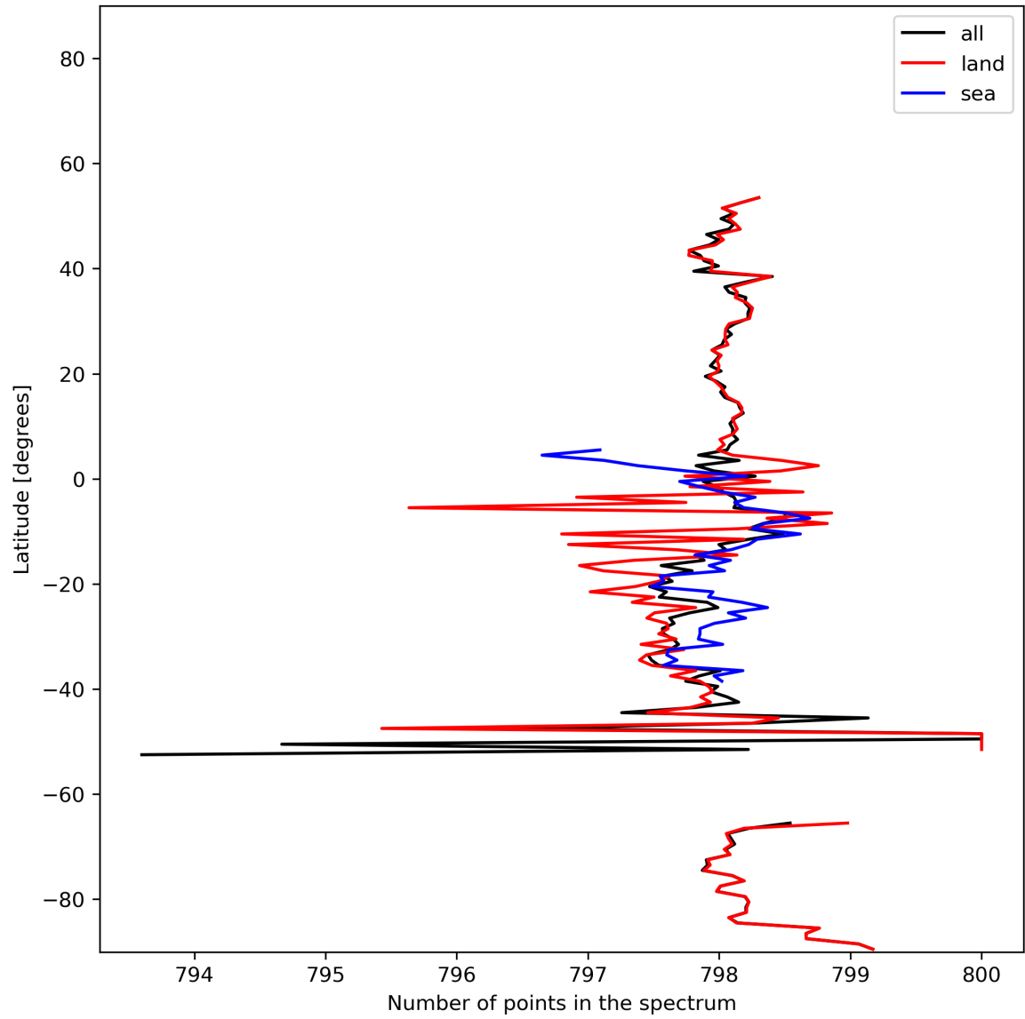
Figure 15: Zonal average of “Number of points in the spectrum” for 2024-01-12 to 2024-01-14.
