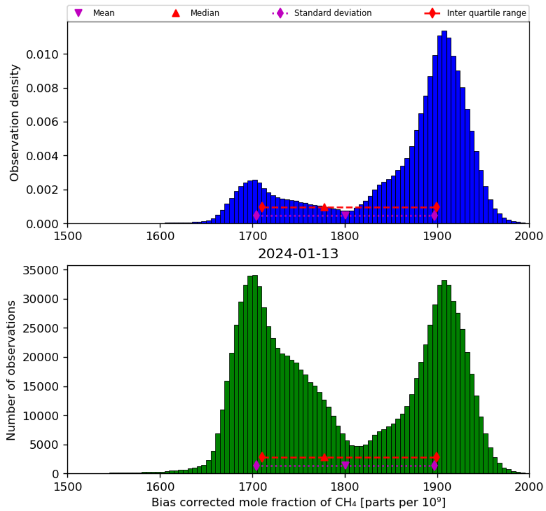
Figure 25: Histogram of “Bias corrected mole fraction of CH 4 ” for 2024-01-12 to 2024-01-14
