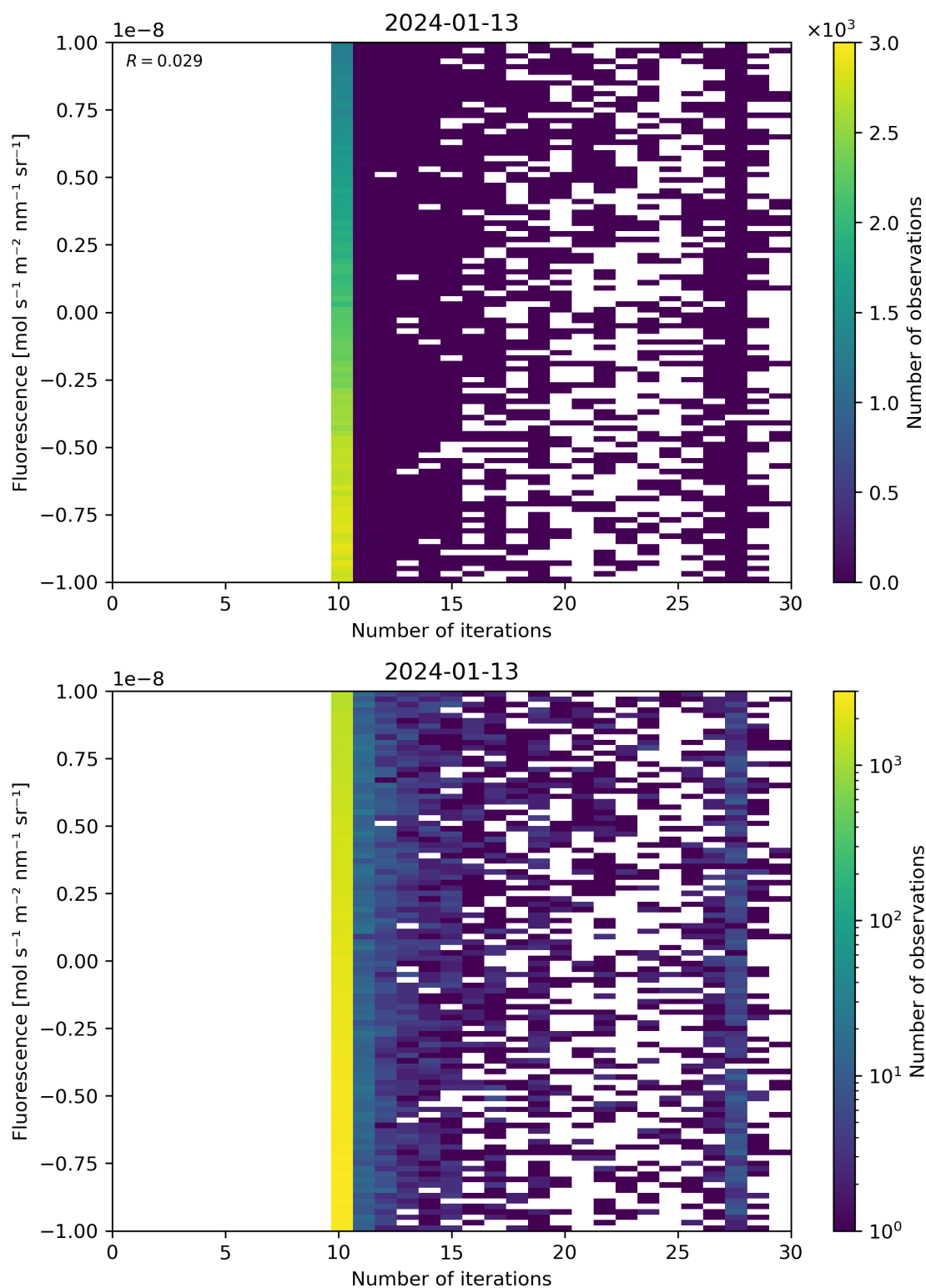
Figure 87: Scatter density plot of “Number of iterations” against “Fluorescence” for 2024-01-12 to 2024-01-14.
