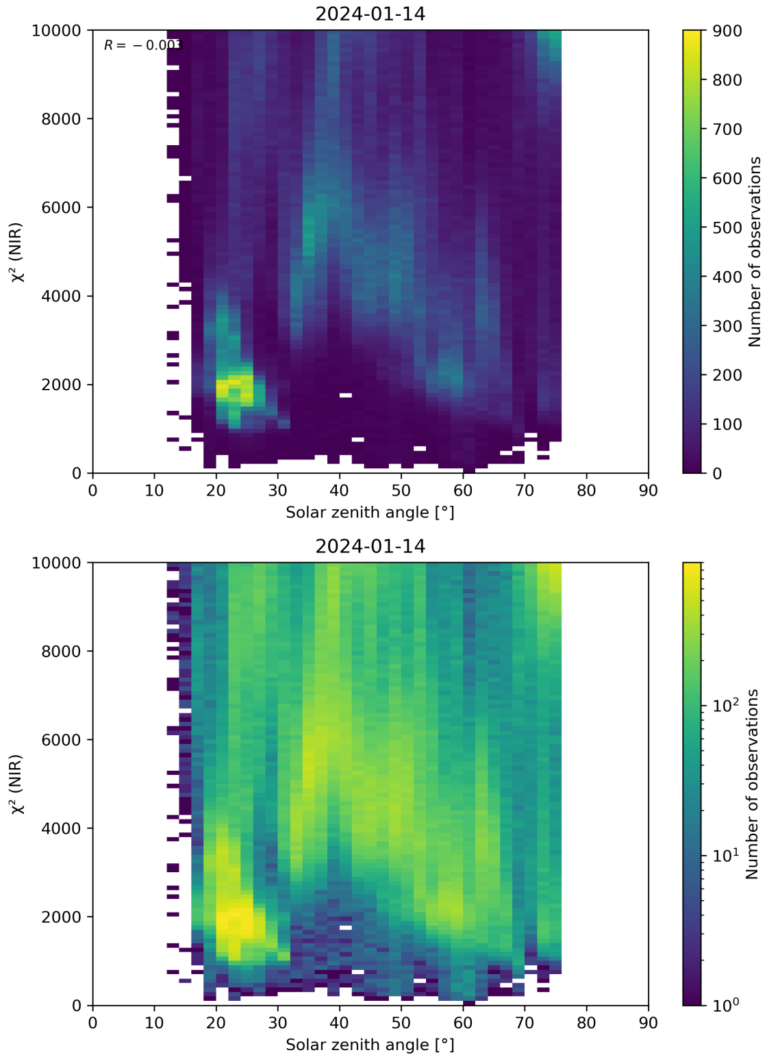
Figure 94: Scatter density plot of “Solar zenith angle” against “ \chi^2 (NIR)” for 2024-01-13 to 2024-01-15.
