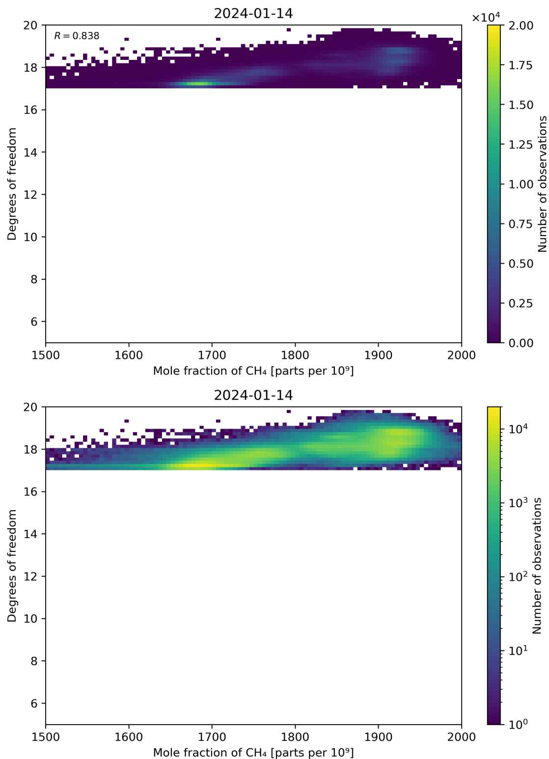
Figure 72: Scatter density plot of “Mole fraction of CH 4 ” against “Degrees of freedom” for 2024-01-13 to 2024-01-15.
