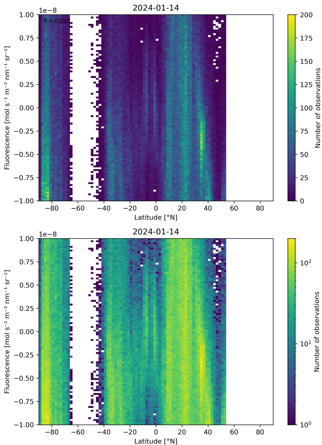
Figure 56: Scatter density plot of “Latitude” against “Fluorescence” for 2024-01-13 to 2024-01-15.
