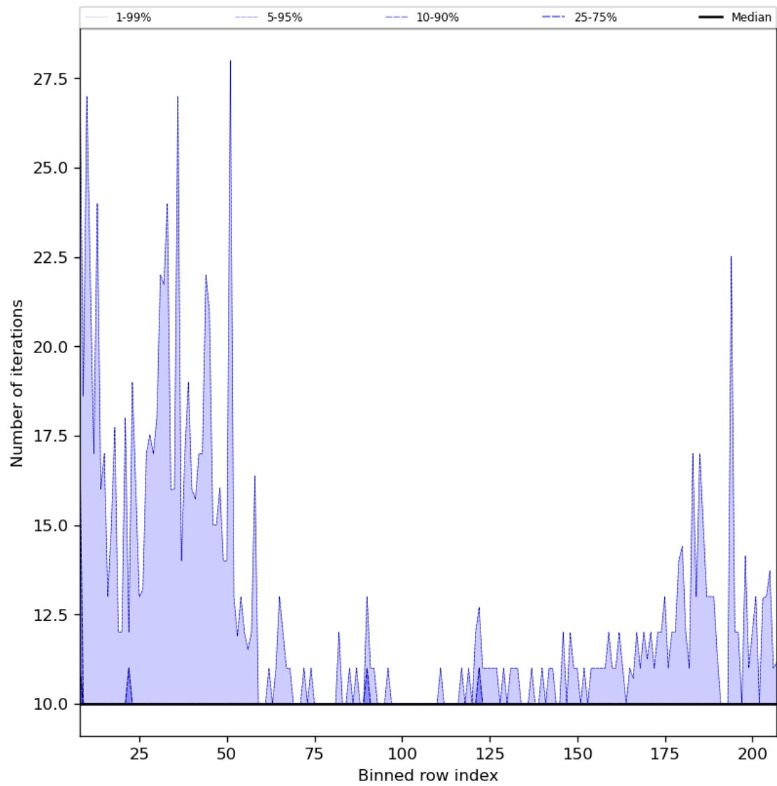
Figure 42: Along track statistics of “Number of iterations” for 2024-01-13 to 2024-01-15
