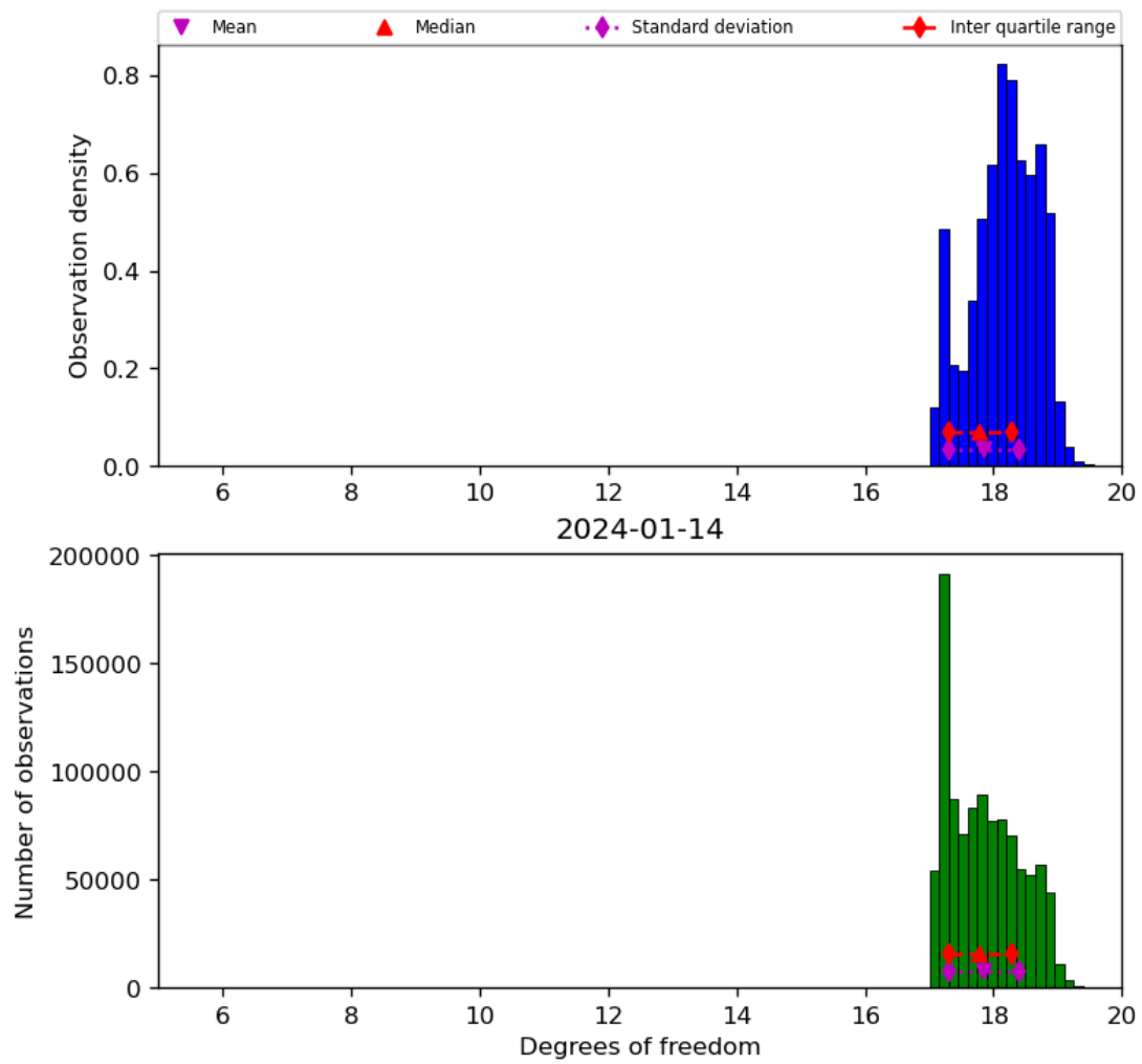
Figure 30: Histogram of “Degrees of freedom” for 2024-01-13 to 2024-01-15
