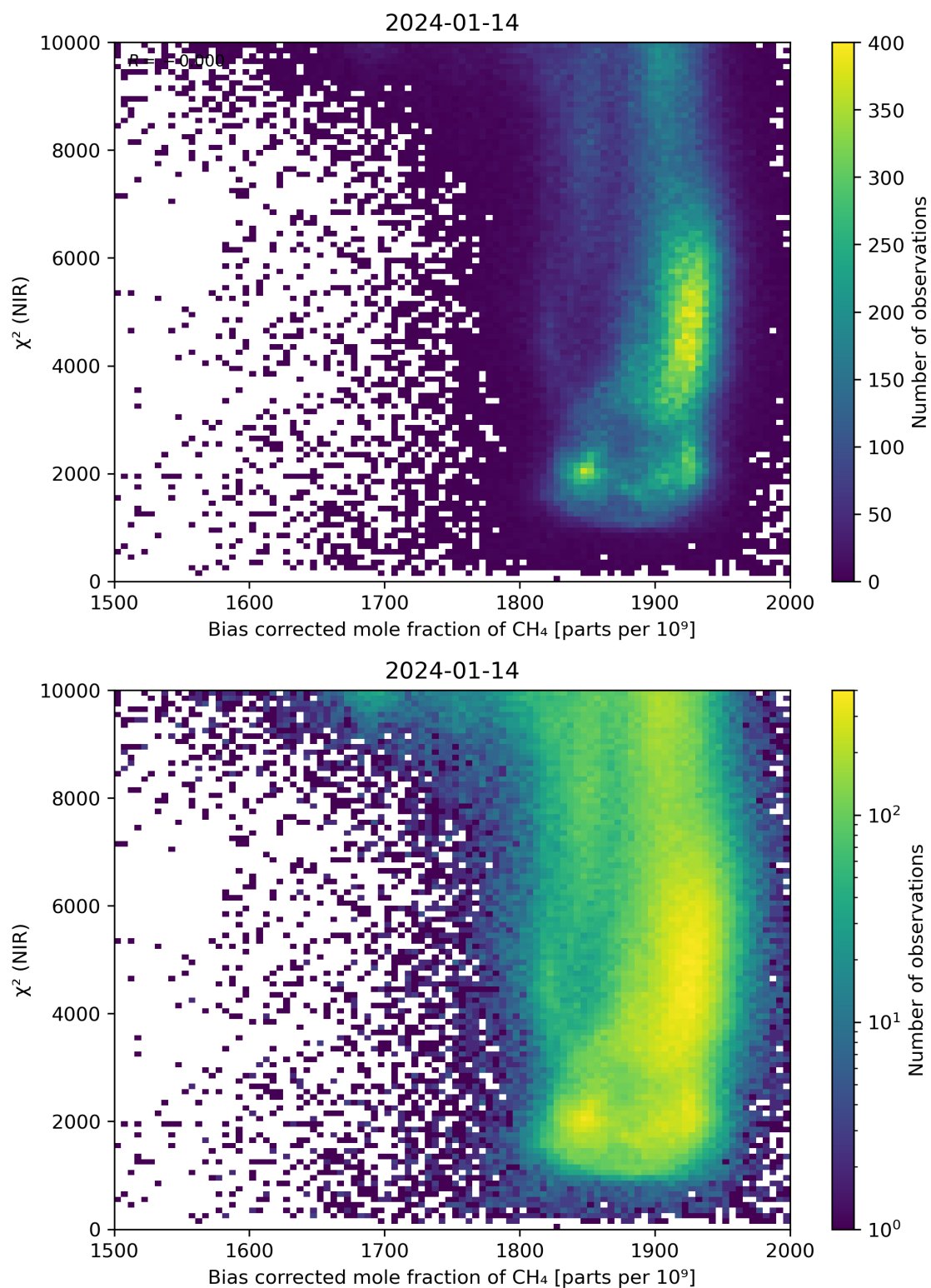
Figure 63: Scatter density plot of “Bias corrected mole fraction of \text{CH}_4 ” against “ \chi^2 (NIR)” for 2024-01-13 to 2024-01-15.
