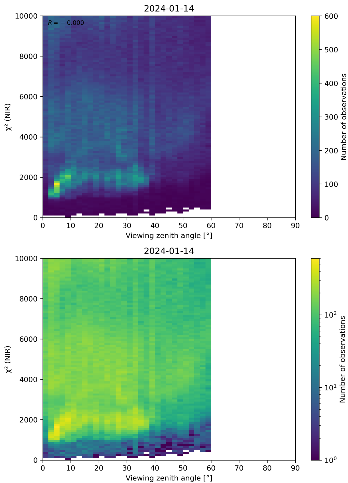
Figure 105: Scatter density plot of “Viewing zenith angle” against “ \chi^2 (NIR)” for 2024-01-13 to 2024-01-15.
