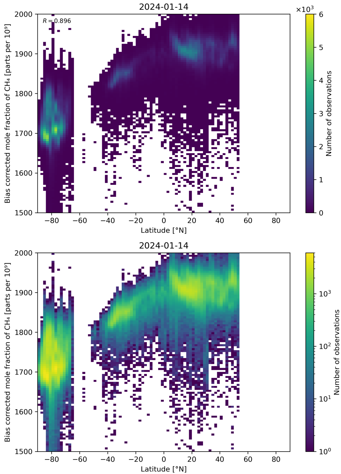
Figure 58: Scatter density plot of “Latitude” against “Bias corrected mole fraction of CH 4 ” for 2024-01-13 to 2024-01-15.
