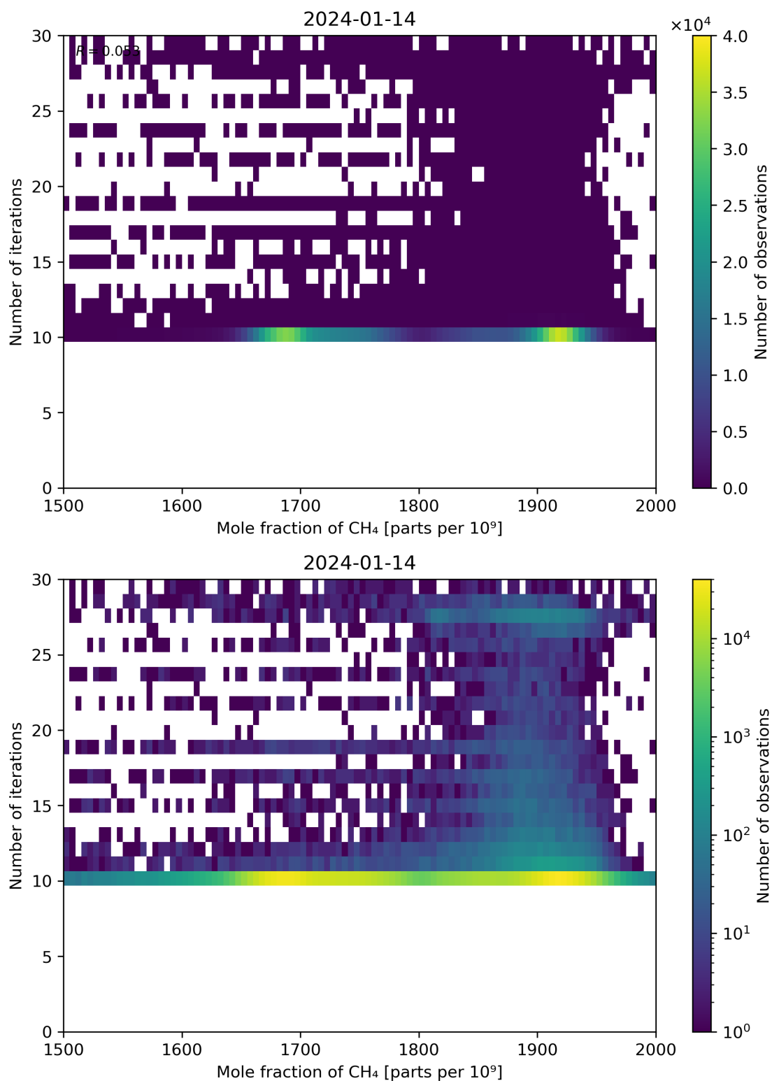
Figure 76: Scatter density plot of “Mole fraction of CH 4 ” against “Number of iterations” for 2024-01-13 to 2024-01-15.
