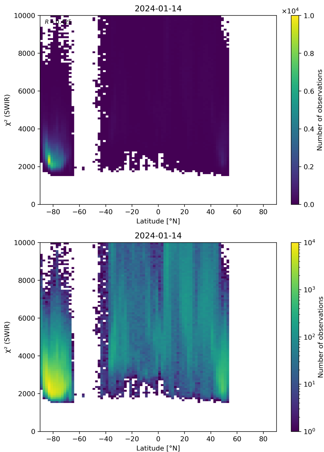
Figure 54: Scatter density plot of “Latitude” against “ \chi^2 (SWIR)” for 2024-01-13 to 2024-01-15.
