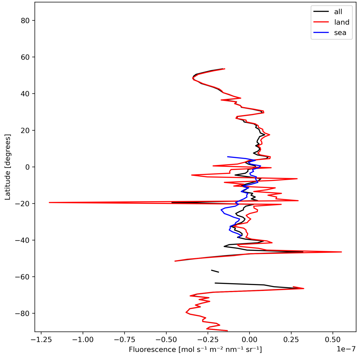
Figure 21: Zonal average of “Fluorescence” for 2024-01-13 to 2024-01-15.
