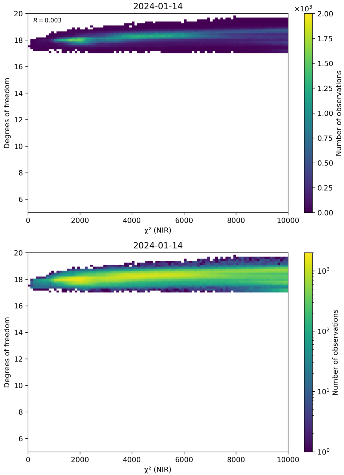
Figure 44: Scatter density plot of “ \chi^2 (NIR)” against “Degrees of freedom” for 2024-01-13 to 2024-01-15.
