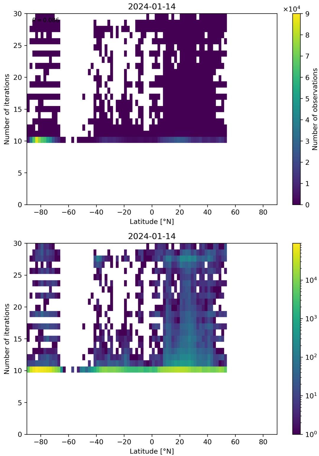
Figure 60: Scatter density plot of “Latitude” against “Number of iterations” for 2024-01-13 to 2024-01-15.
