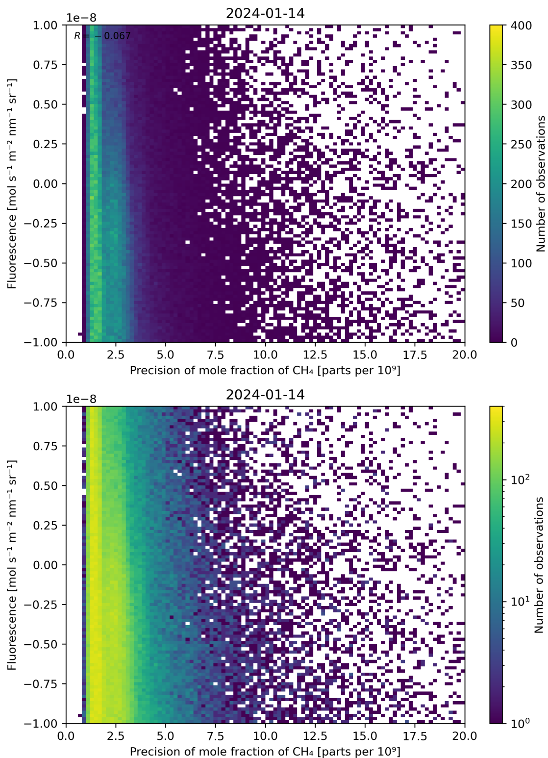
Figure 81: Scatter density plot of “Precision of mole fraction of \text{CH}_4 ” against “Fluorescence” for 2024-01-13 to 2024-01-15.
