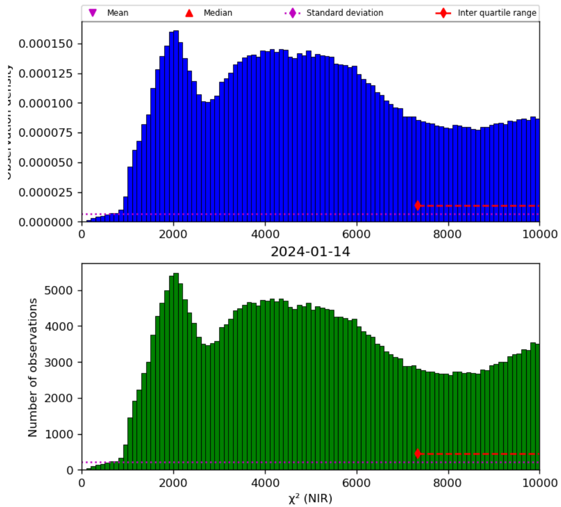
Figure 29: Histogram of “ \chi^2 (NIR)” for 2024-01-13 to 2024-01-15
