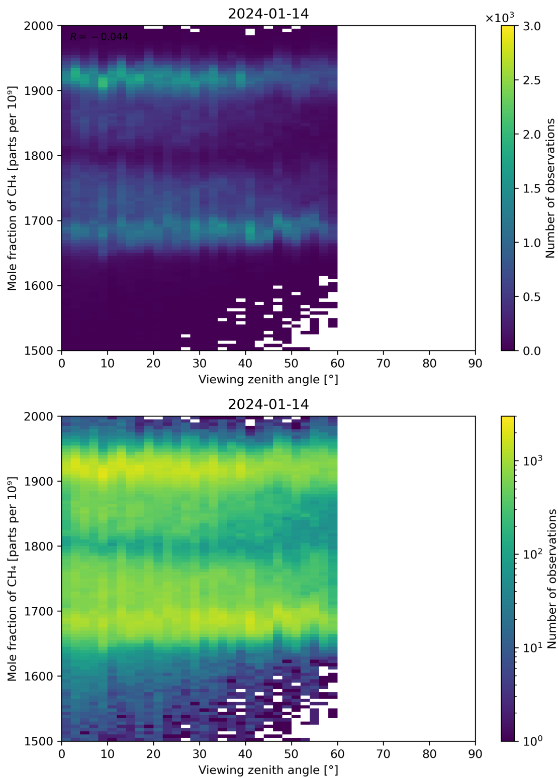
Figure 110: Scatter density plot of “Viewing zenith angle” against “Mole fraction of CH 4 ” for 2024-01-13 to 2024-01-15.
