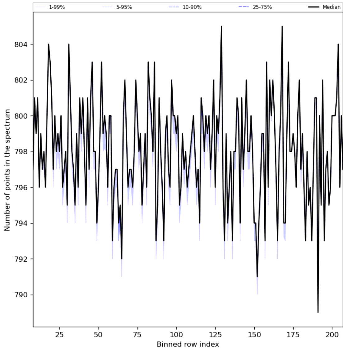
Figure 37: Along track statistics of “Number of points in the spectrum” for 2024-01-13 to 2024-01-15
