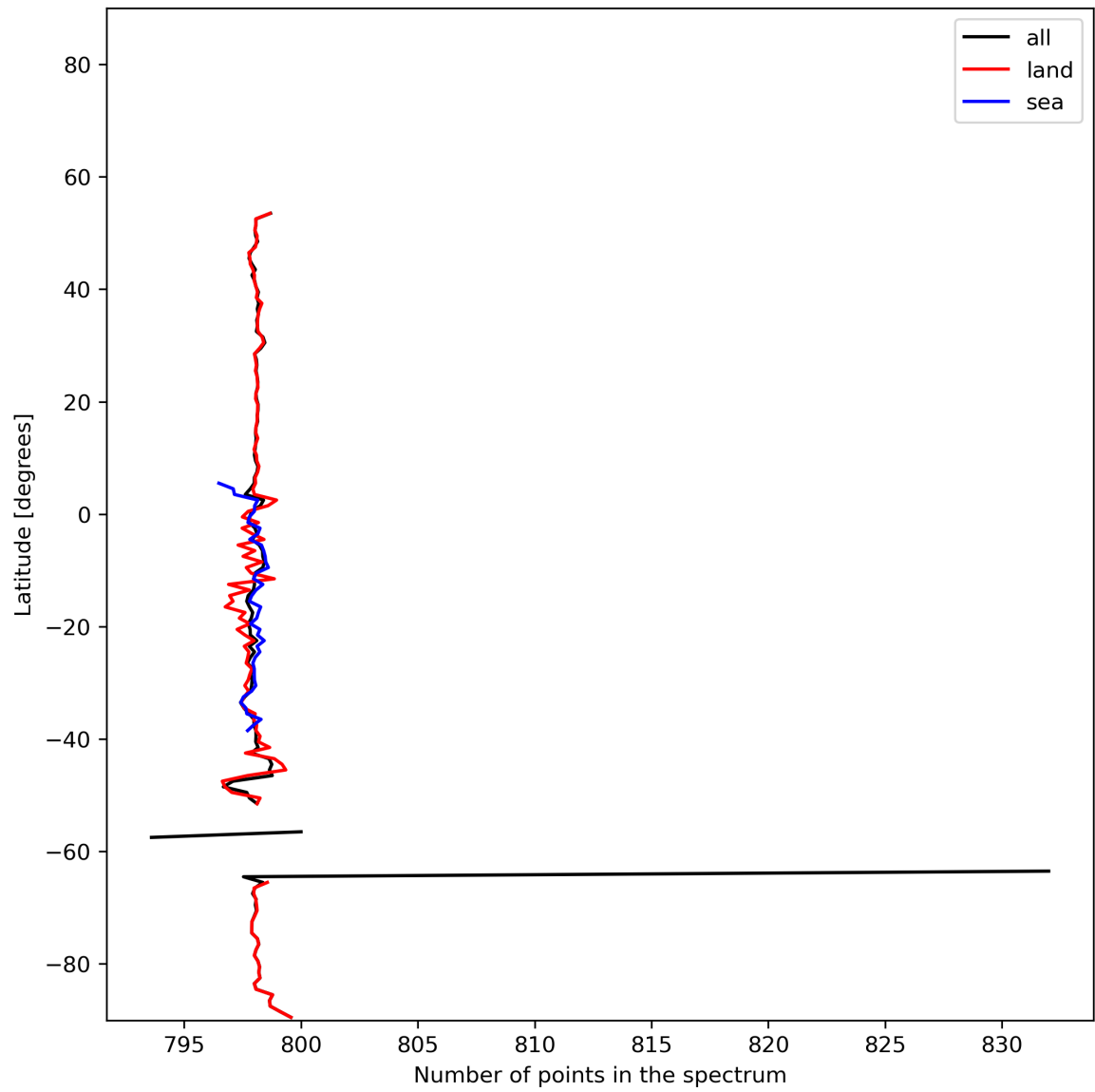
Figure 15: Zonal average of “Number of points in the spectrum” for 2024-01-13 to 2024-01-15.
