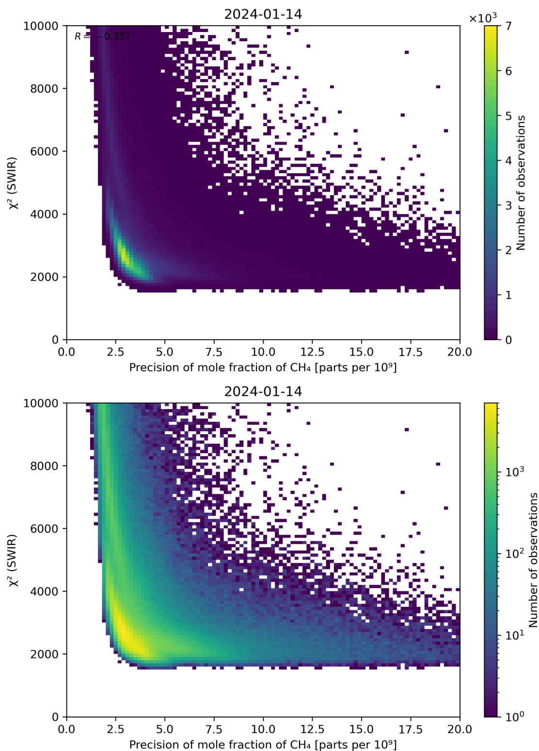
Figure 79: Scatter density plot of “Precision of mole fraction of CH 4 ” against “ \chi^2 (SWIR)” for 2024-01-13 to 2024-01-15.
