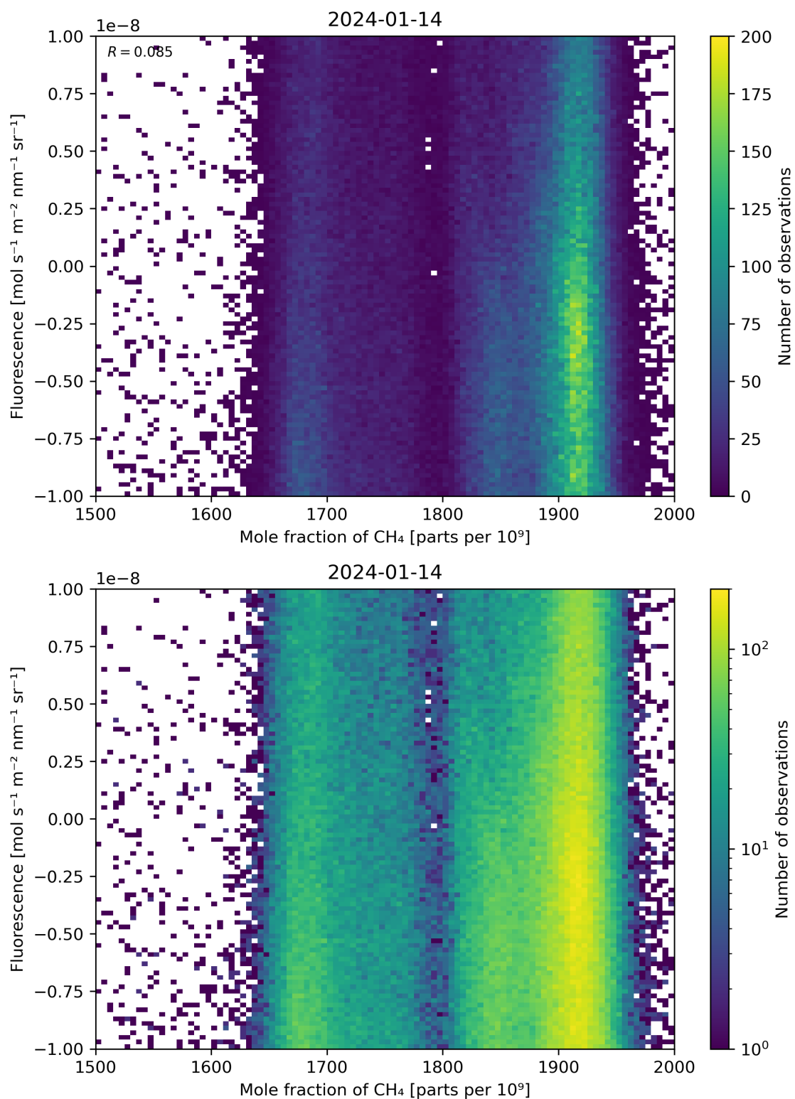
Figure 73: Scatter density plot of “Mole fraction of \text{CH}_4 ” against “Fluorescence” for 2024-01-13 to 2024-01-15.
