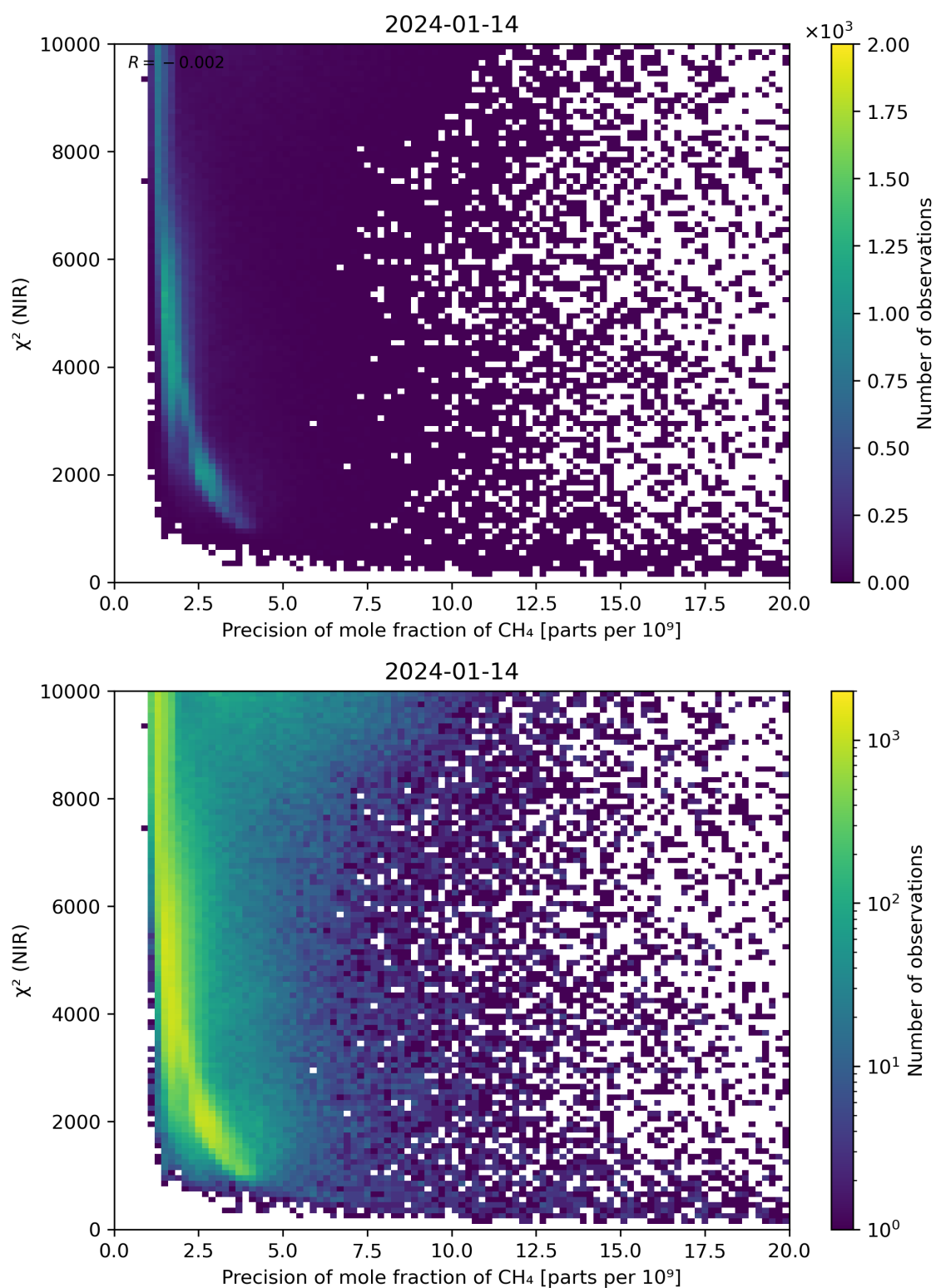
Figure 78: Scatter density plot of “Precision of mole fraction of CH 4 ” against “ \chi^2 (NIR)” for 2024-01-13 to 2024-01-15.
