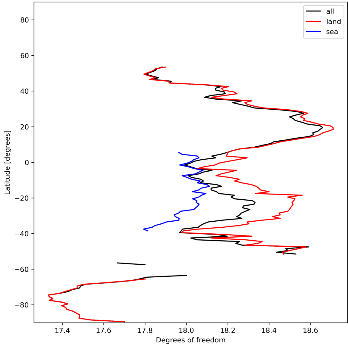
Figure 19: Zonal average of “Degrees of freedom” for 2024-01-13 to 2024-01-15.
