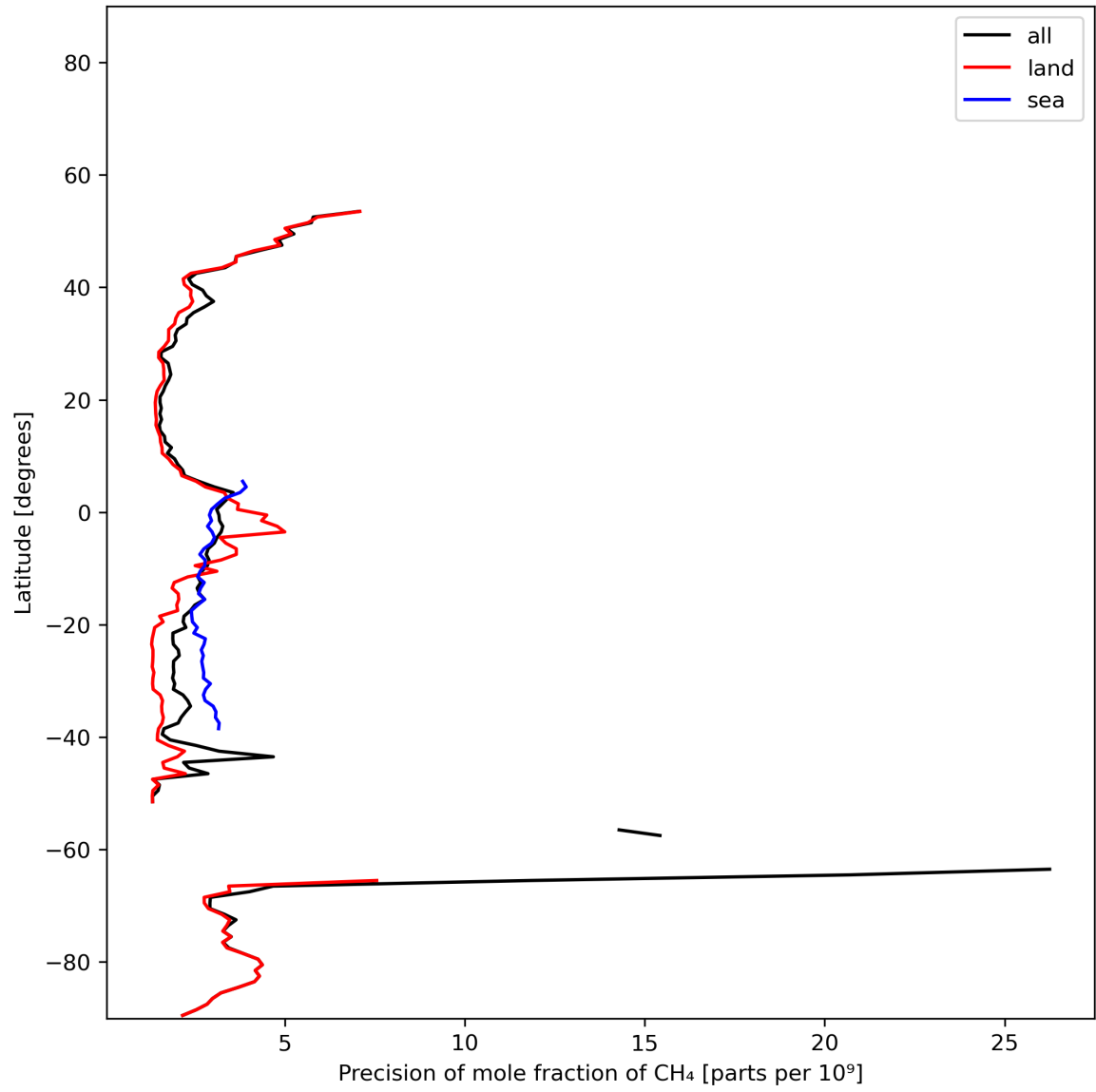
Figure 13: Zonal average of “Precision of mole fraction of \text{CH}_4 ” for 2024-01-13 to 2024-01-15.
