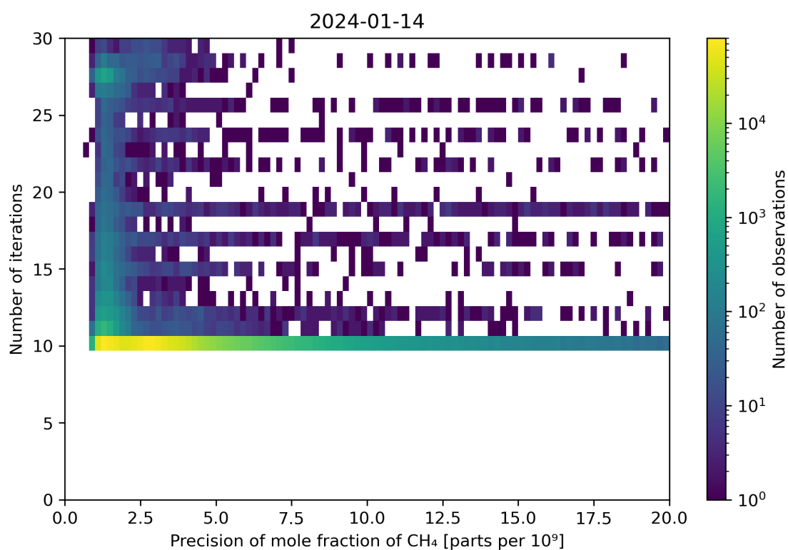
Figure 83: Scatter density plot of “Precision of mole fraction of CH 4 ” against “Number of iterations” for 2024-01-13 to 2024-01-15.
