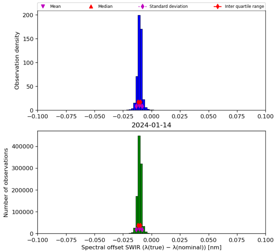
Figure 27: Histogram of “Spectral offset SWIR ( \lambda(\text{true}) - \lambda(\text{nominal}) )” for 2024-01-13 to 2024-01-15
