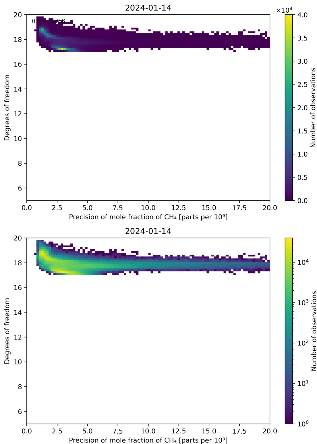
Figure 80: Scatter density plot of “Precision of mole fraction of CH 4 ” against “Degrees of freedom” for 2024-01-13 to 2024-01-15.
