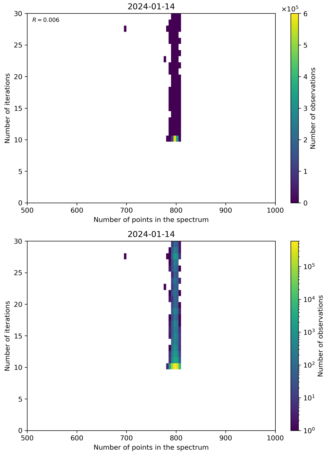
Figure 92: Scatter density plot of “Number of points in the spectrum” against “Number of iterations” for 2024-01-13 to 2024-01-15.
