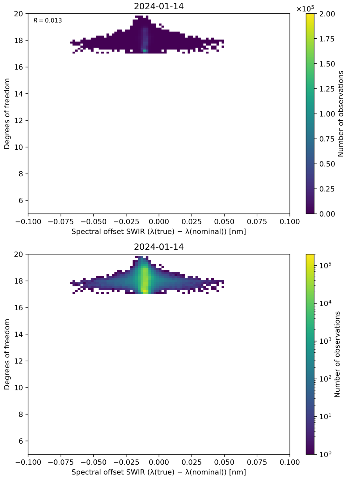
Figure 119: Scatter density plot of “Spectral offset SWIR ( \lambda(\text{true}) - \lambda(\text{nominal}) )” against “Degrees of freedom” for 2024-01-13 to 2024-01-15.
