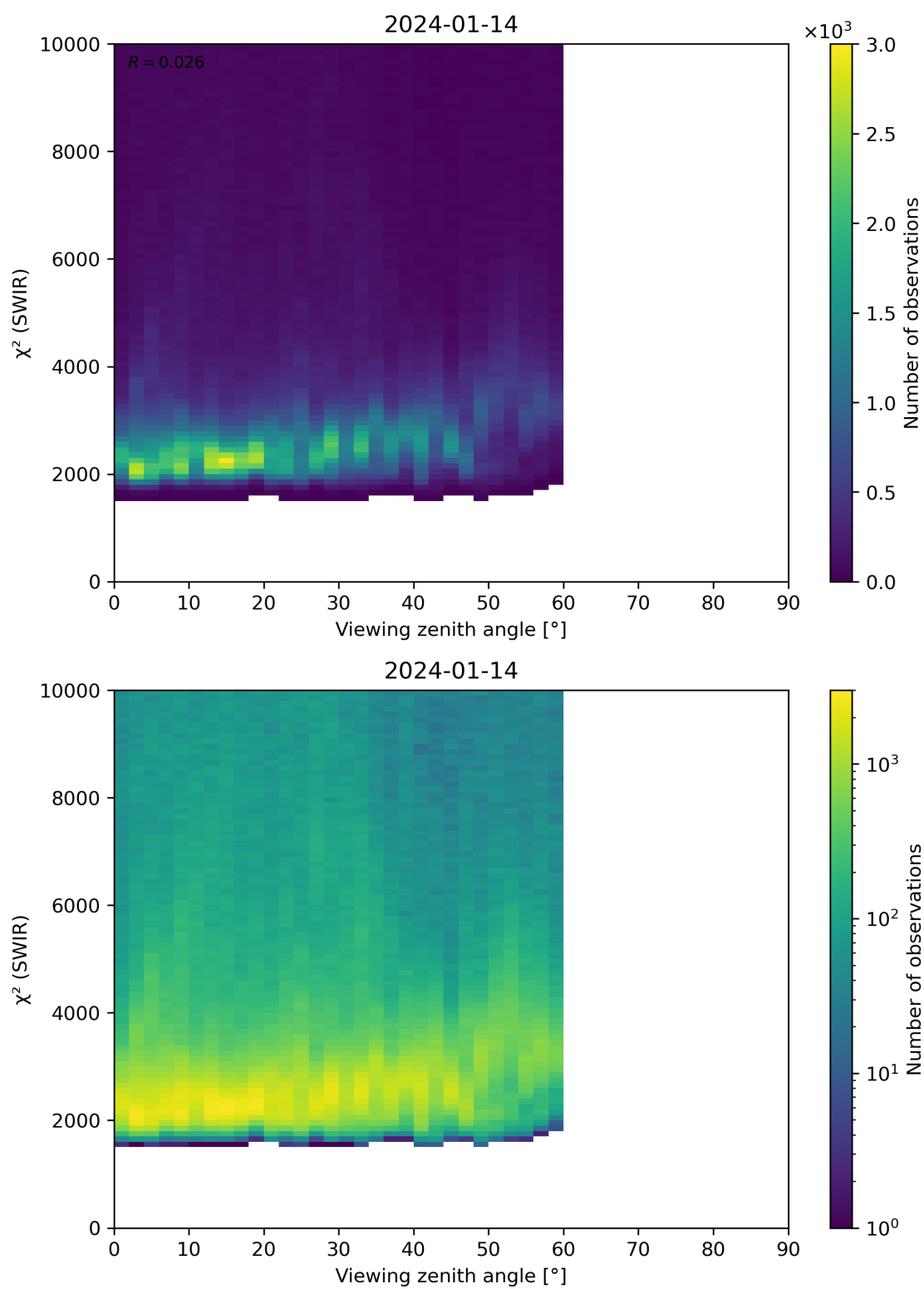
Figure 106: Scatter density plot of “Viewing zenith angle” against “ \chi^2 (SWIR)” for 2024-01-13 to 2024-01-15.
