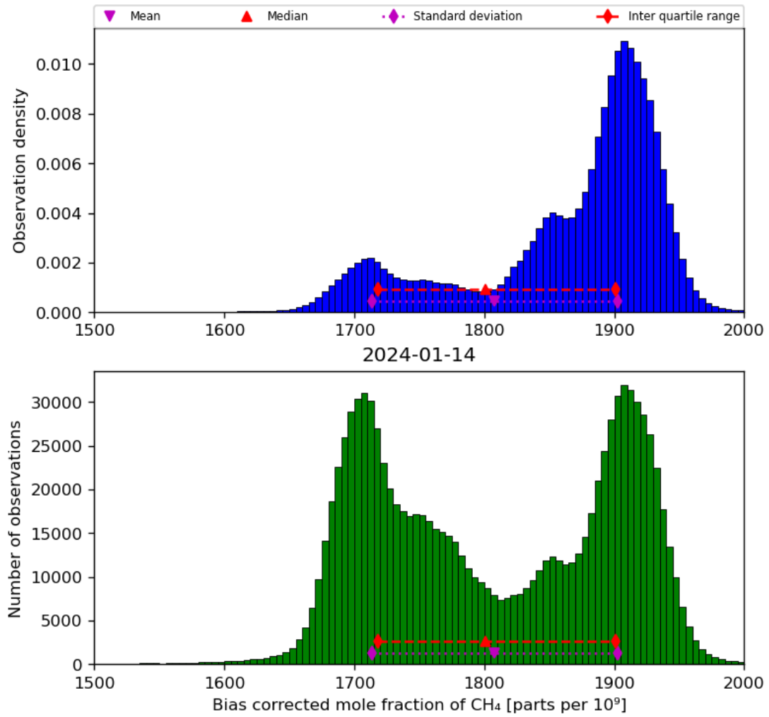
Figure 25: Histogram of “Bias corrected mole fraction of CH 4 ” for 2024-01-13 to 2024-01-15
