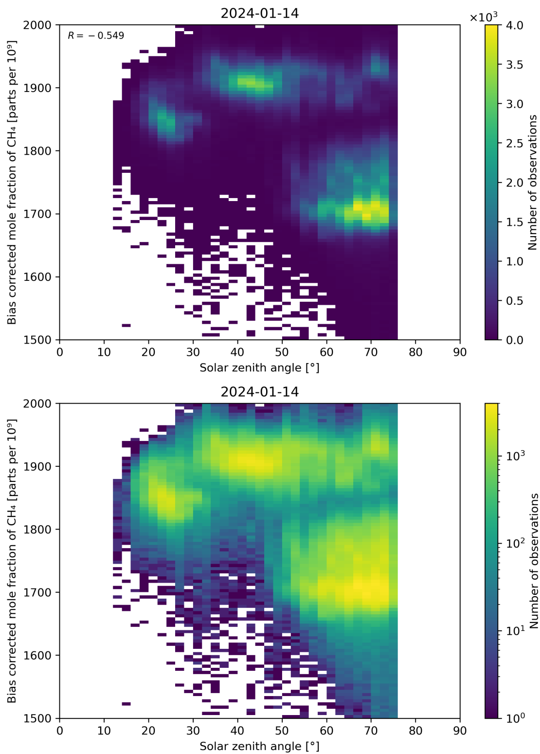
Figure 100: Scatter density plot of “Solar zenith angle” against “Bias corrected mole fraction of CH 4 ” for 2024-01-13 to 2024-01-15.
