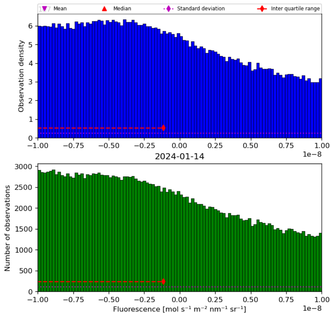
Figure 32: Histogram of “Fluorescence” for 2024-01-13 to 2024-01-15
