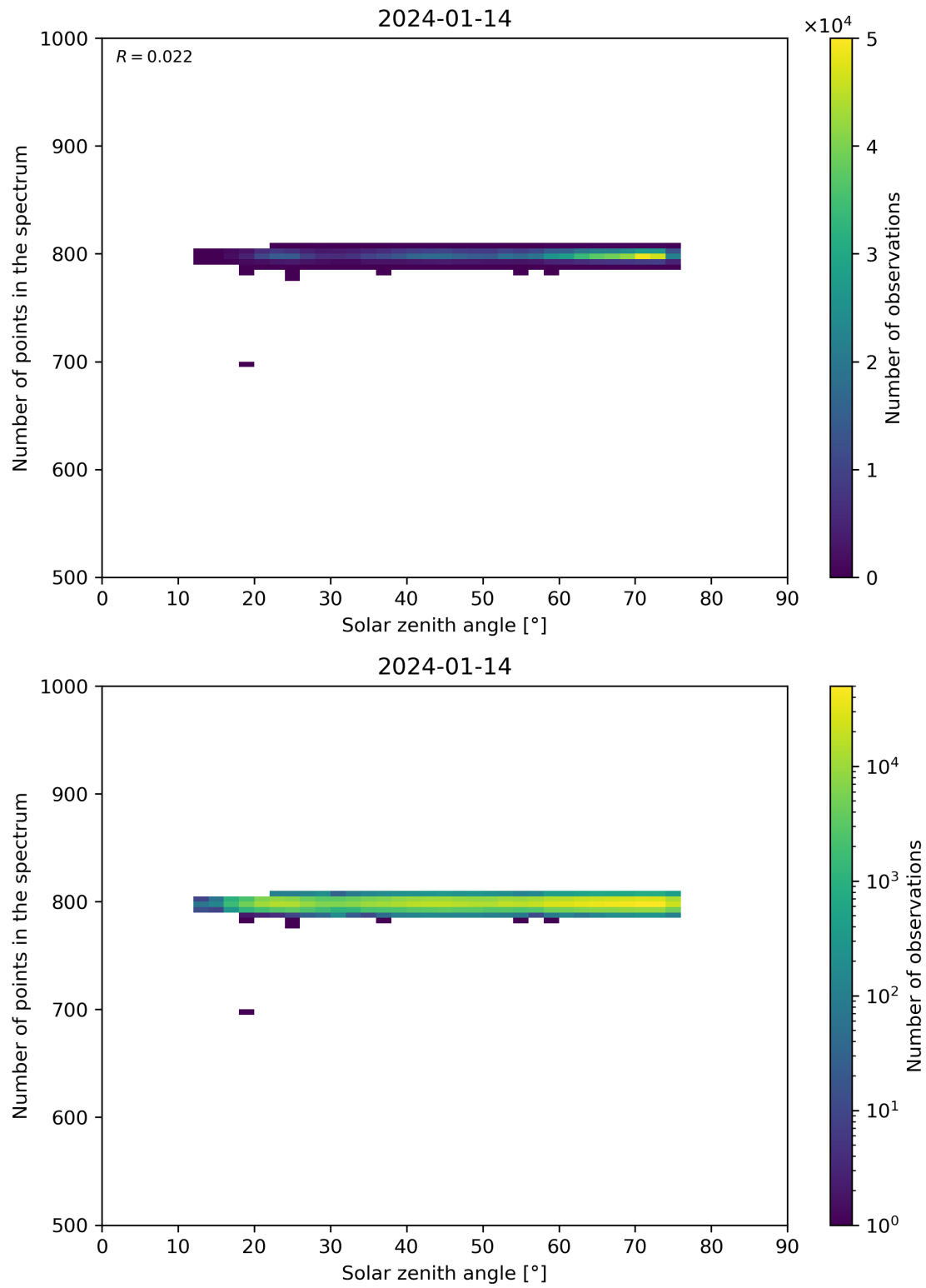
Figure 103: Scatter density plot of “Solar zenith angle” against “Number of points in the spectrum” for 2024-01-13 to 2024-01-15.
