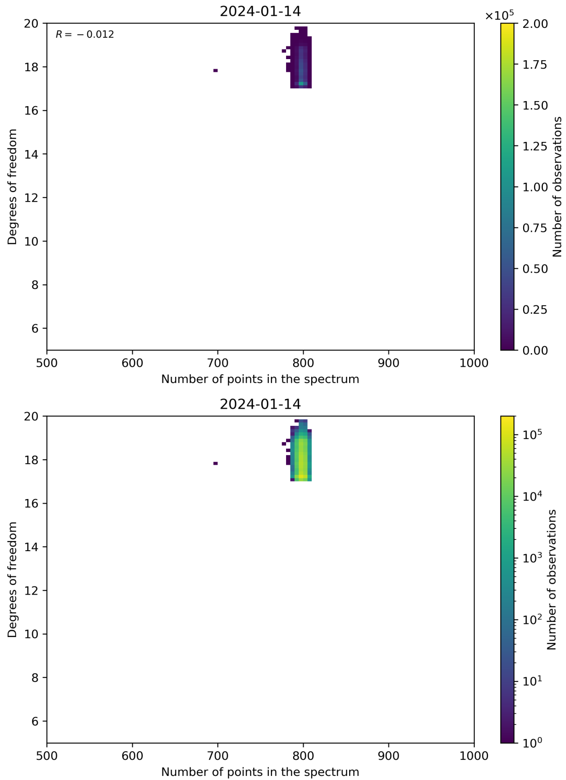
Figure 90: Scatter density plot of “Number of points in the spectrum” against “Degrees of freedom” for 2024-01-13 to 2024-01-15.
