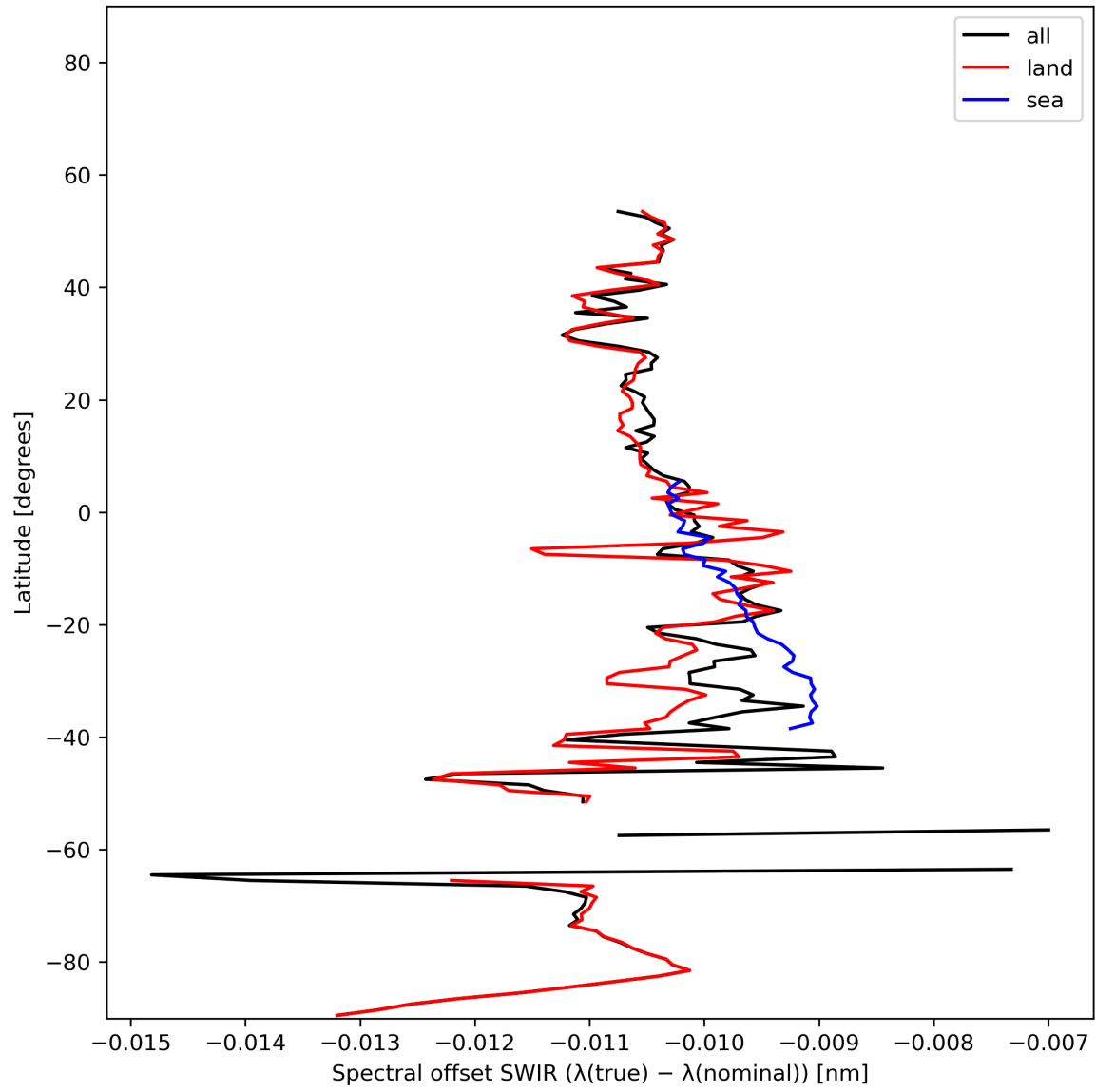
Figure 16: Zonal average of “Spectral offset SWIR ( \lambda(\text{true}) - \lambda(\text{nominal}) )” for 2024-01-13 to 2024-01-15.
