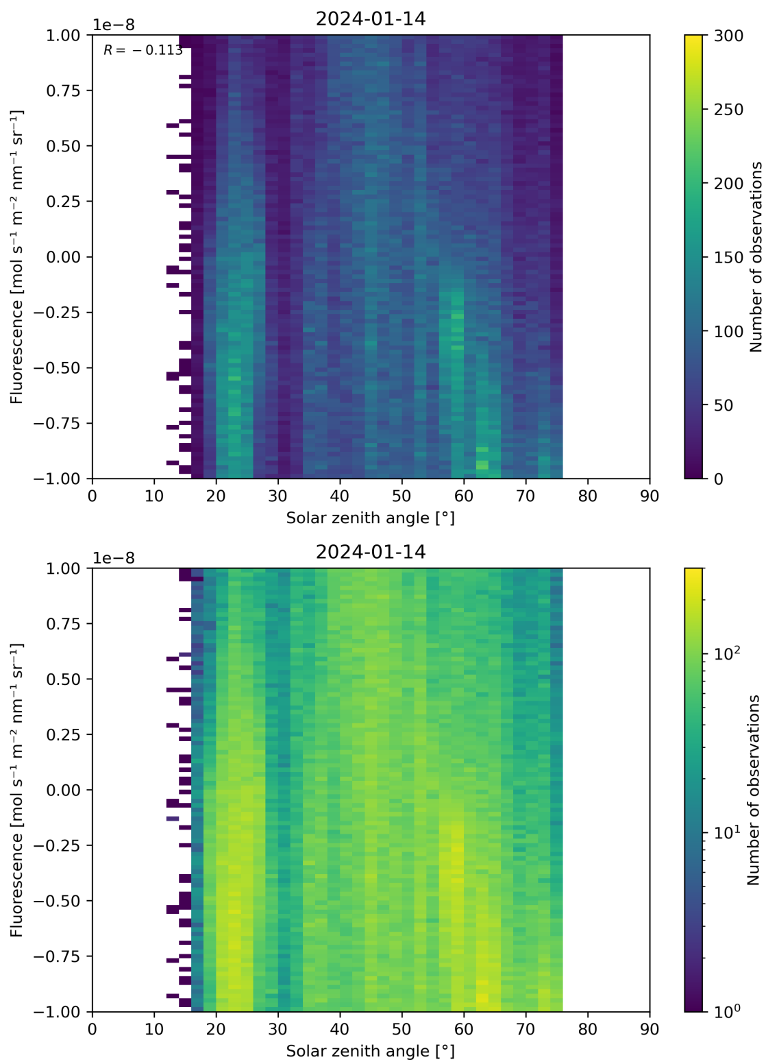
Figure 97: Scatter density plot of “Solar zenith angle” against “Fluorescence” for 2024-01-13 to 2024-01-15.
