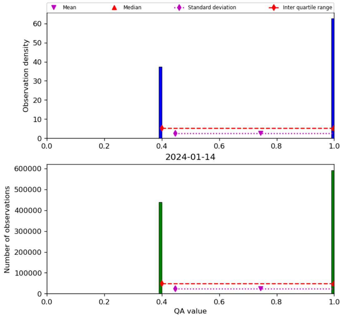
Figure 22: Histogram of “QA value” for 2024-01-13 to 2024-01-15
