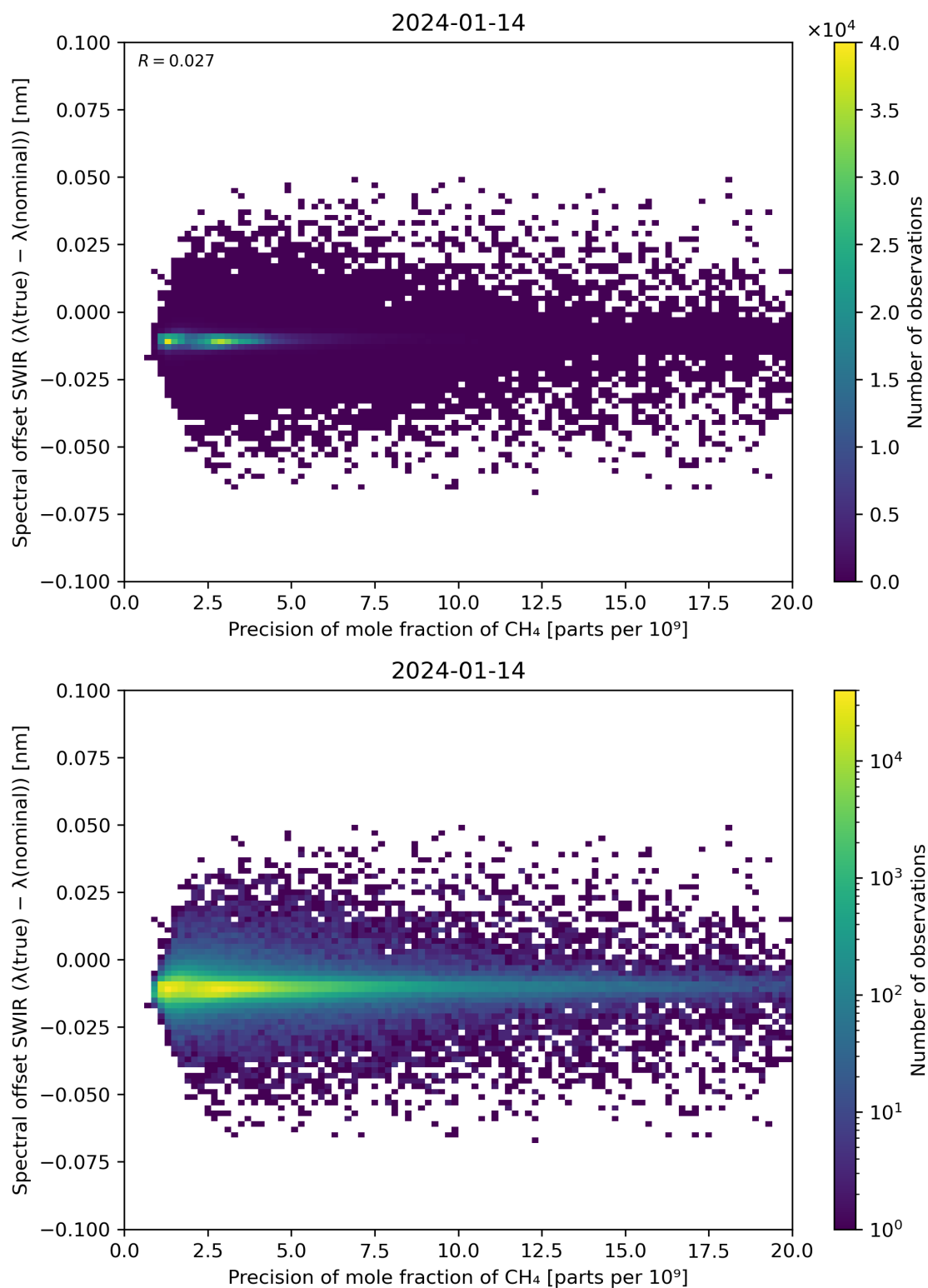
Figure 85: Scatter density plot of “Precision of mole fraction of \text{CH}_4 ” against “Spectral offset SWIR ( \lambda(\text{true}) - \lambda(\text{nominal}) )” for 2024-01-13 to 2024-01-15.
