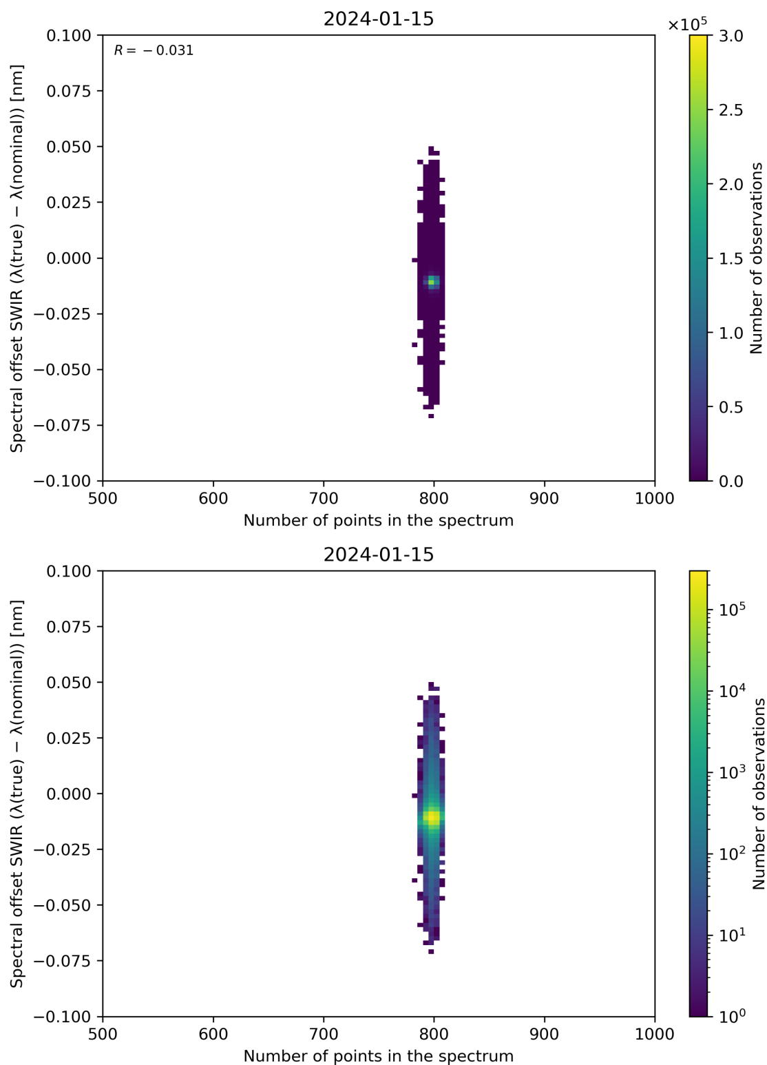
Figure 93: Scatter density plot of “Number of points in the spectrum” against “Spectral offset SWIR ( \lambda(\text{true}) - \lambda(\text{nominal}) )” for 2024-01-15 to 2024-01-16.
