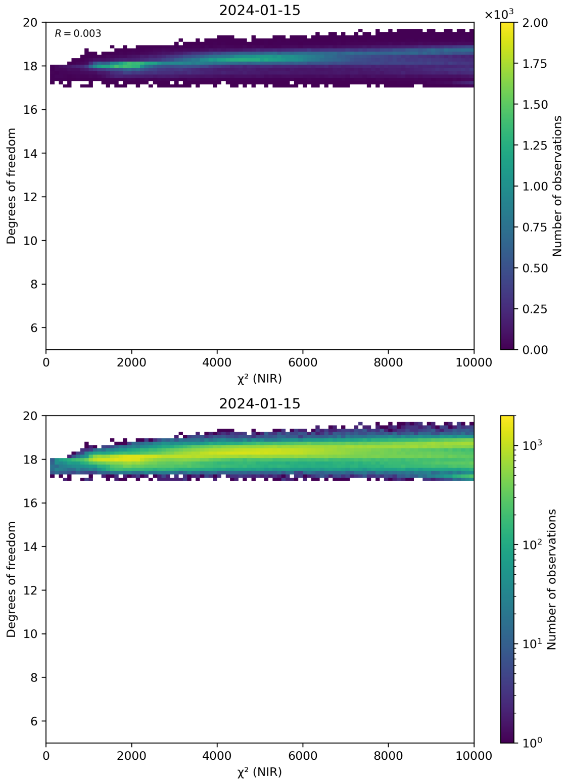
Figure 44: Scatter density plot of “ \chi^2 (NIR)” against “Degrees of freedom” for 2024-01-15 to 2024-01-16.
