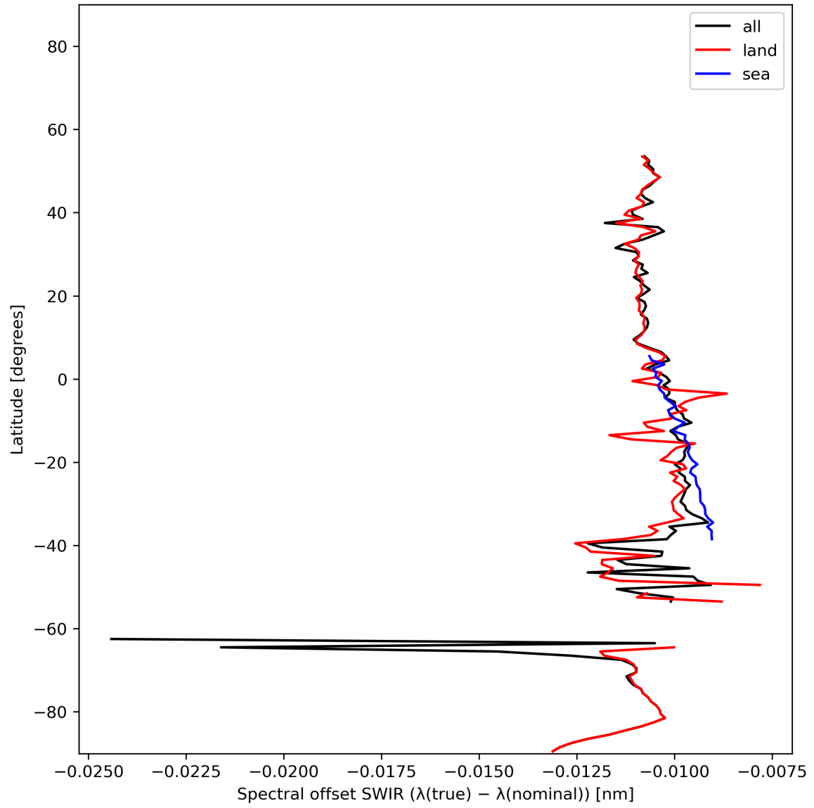
Figure 16: Zonal average of “Spectral offset SWIR ( \lambda(\text{true}) - \lambda(\text{nominal}) )” for 2024-01-15 to 2024-01-16.
