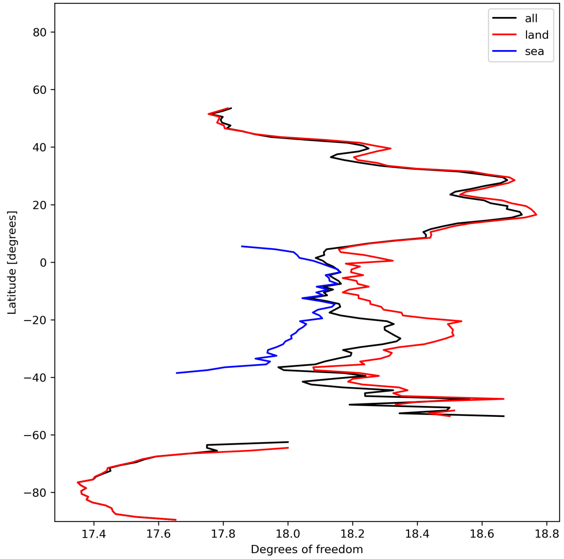
Figure 19: Zonal average of “Degrees of freedom” for 2024-01-15 to 2024-01-16.
