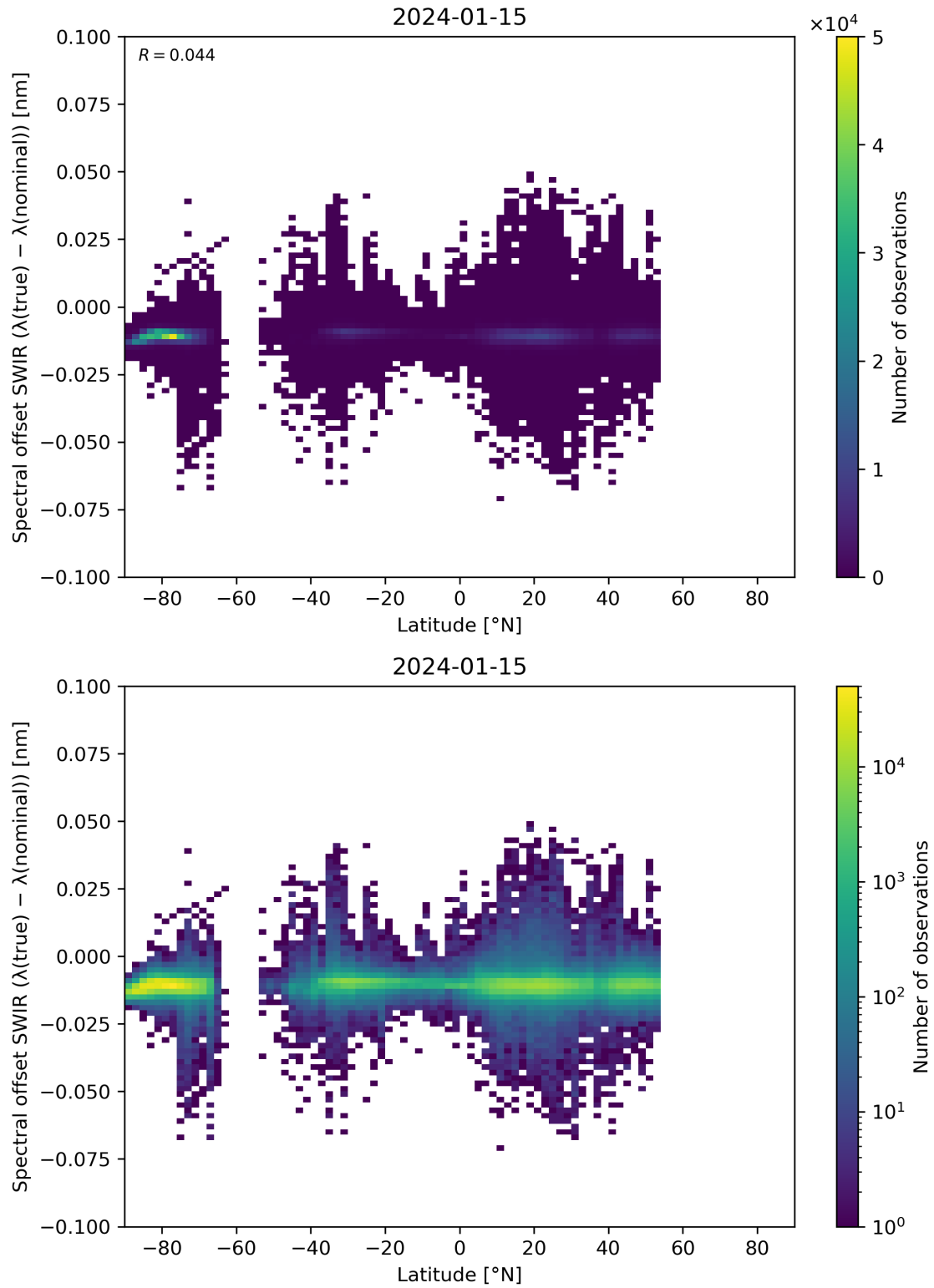
Figure 62: Scatter density plot of “Latitude” against “Spectral offset SWIR ( \lambda(\text{true}) - \lambda(\text{nominal}) )” for 2024-01-15 to 2024-01-16.
