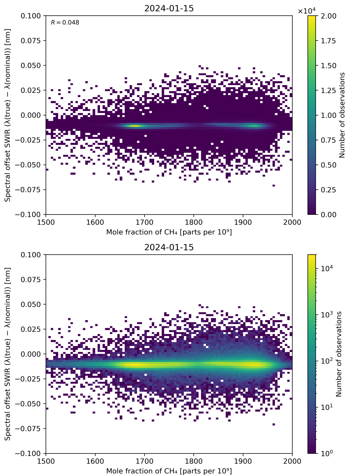
Figure 86: Scatter density plot of “Mole fraction of CH 4 ” against “Spectral offset SWIR ( \lambda(\text{true}) - \lambda(\text{nominal}) )” for 2024-01-15 to 2024-01-16.
