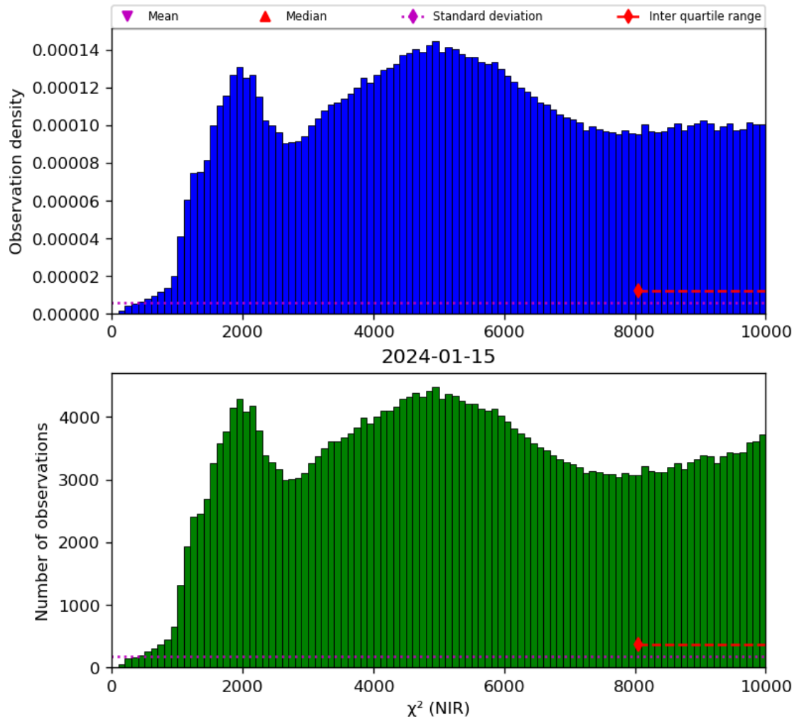
Figure 29: Histogram of “ \chi^2 (NIR)” for 2024-01-15 to 2024-01-16
