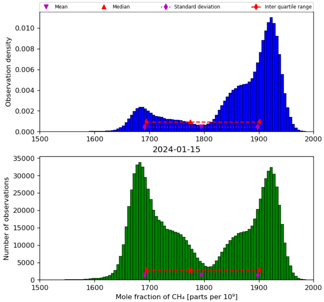
Figure 23: Histogram of “Mole fraction of CH 4 ” for 2024-01-15 to 2024-01-16
