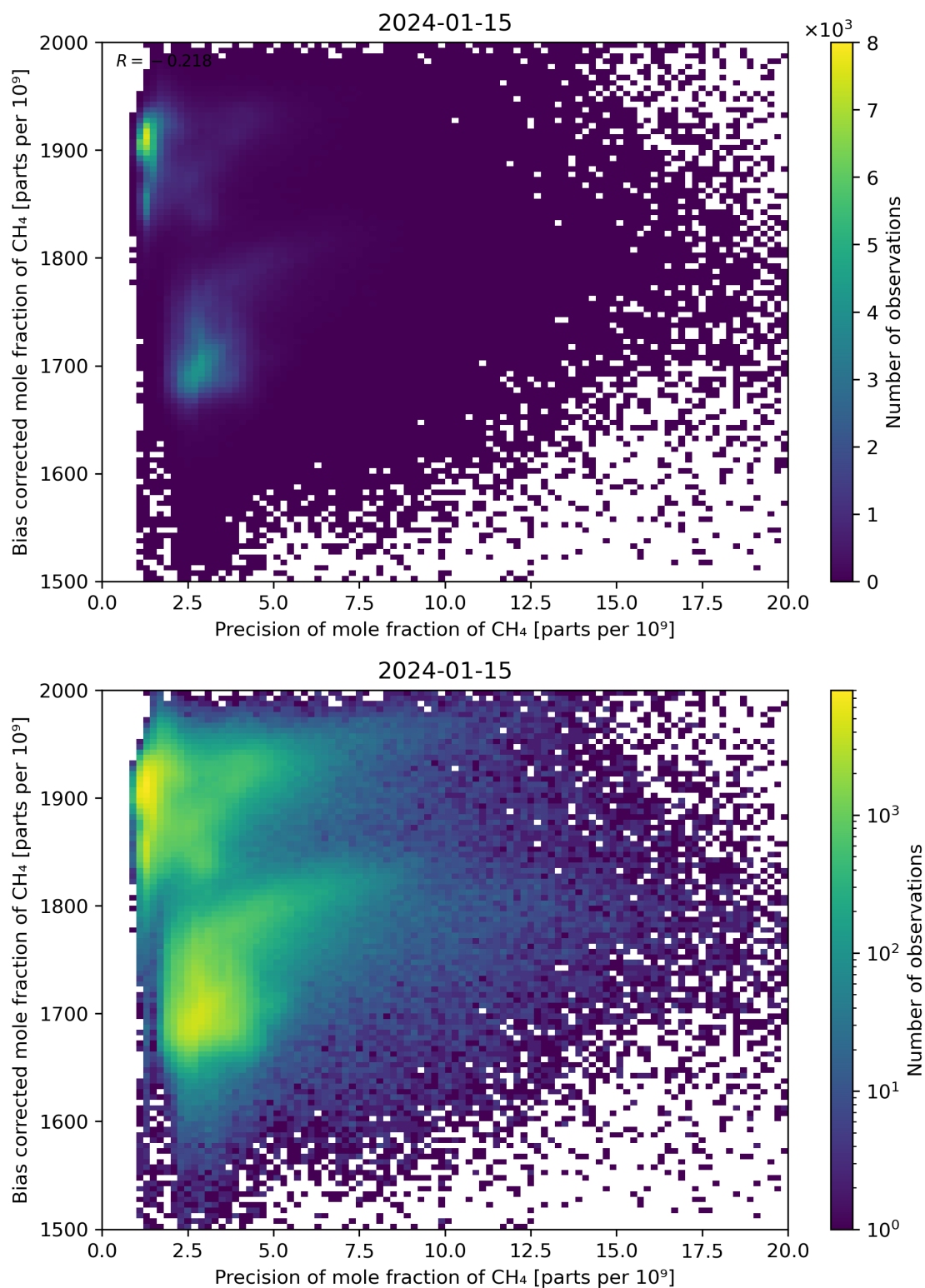
Figure 82: Scatter density plot of “Precision of mole fraction of \text{CH}_4 ” against “Bias corrected mole fraction of \text{CH}_4 ” for 2024-01-15 to 2024-01-16.
