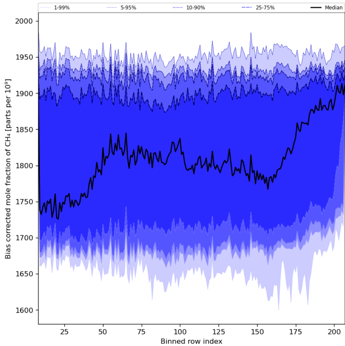
Figure 36: Along track statistics of “Bias corrected mole fraction of CH 4 ” for 2024-01-15 to 2024-01-16
