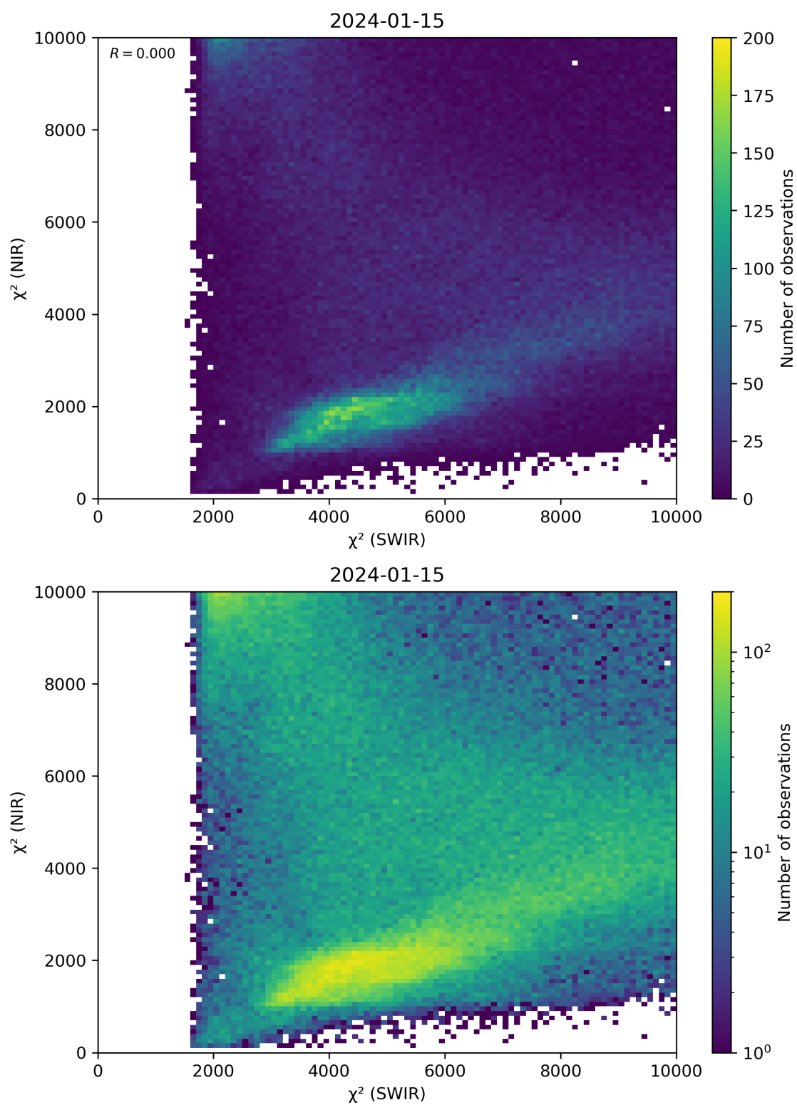
Figure 47: Scatter density plot of “ \chi^2 (SWIR)” against “ \chi^2 (NIR)” for 2024-01-15 to 2024-01-16.
