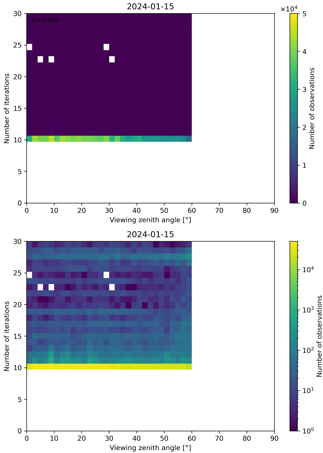
Figure 113: Scatter density plot of “Viewing zenith angle” against “Number of iterations” for 2024-01-15 to 2024-01-16.
