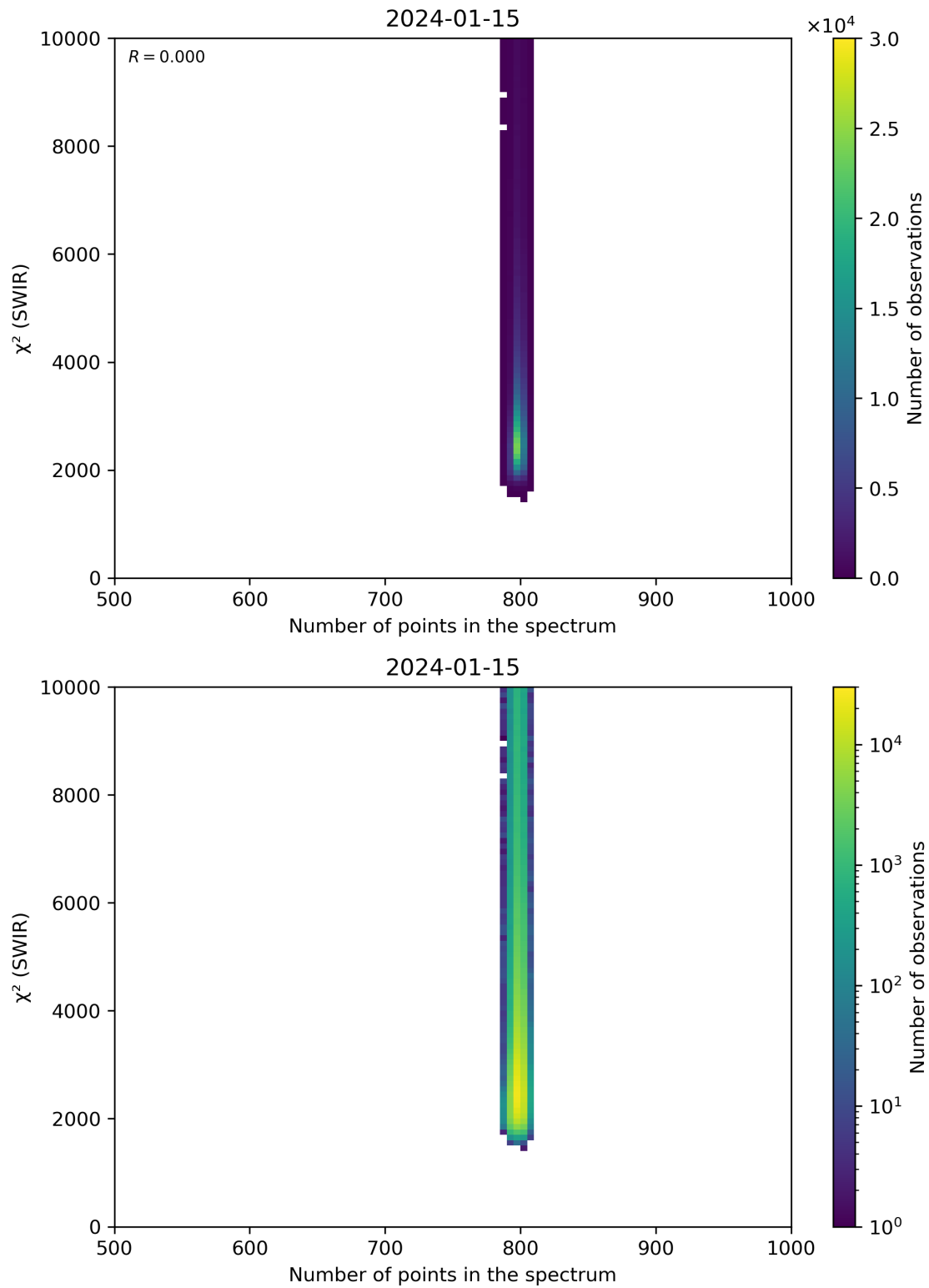
Figure 89: Scatter density plot of “Number of points in the spectrum” against “ \chi^2 (SWIR)” for 2024-01-15 to 2024-01-16.
