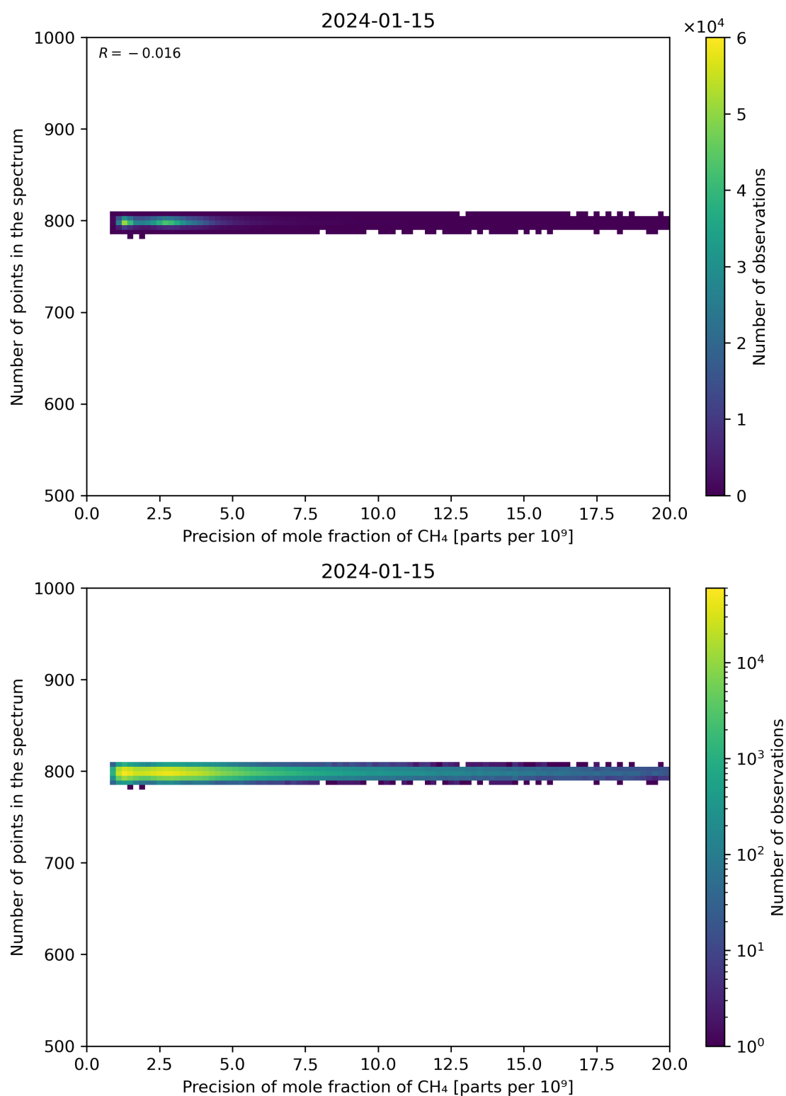
Figure 84: Scatter density plot of “Precision of mole fraction of CH 4 ” against “Number of points in the spectrum” for 2024-01-15 to 2024-01-16.
