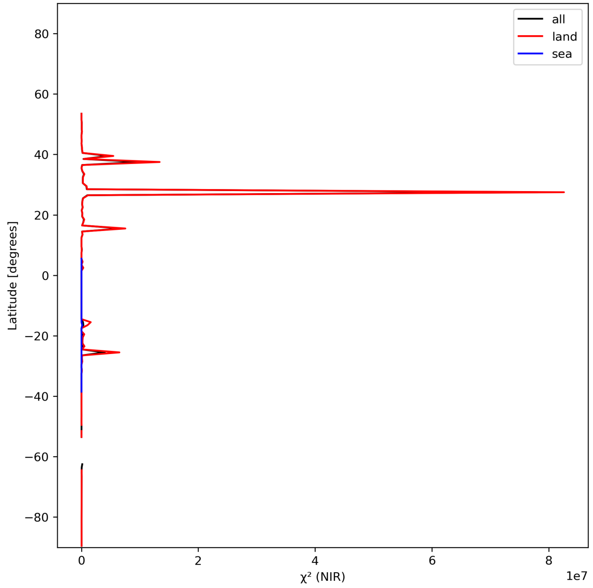
Figure 18: Zonal average of “ \chi^2 (NIR)” for 2024-01-15 to 2024-01-16.
