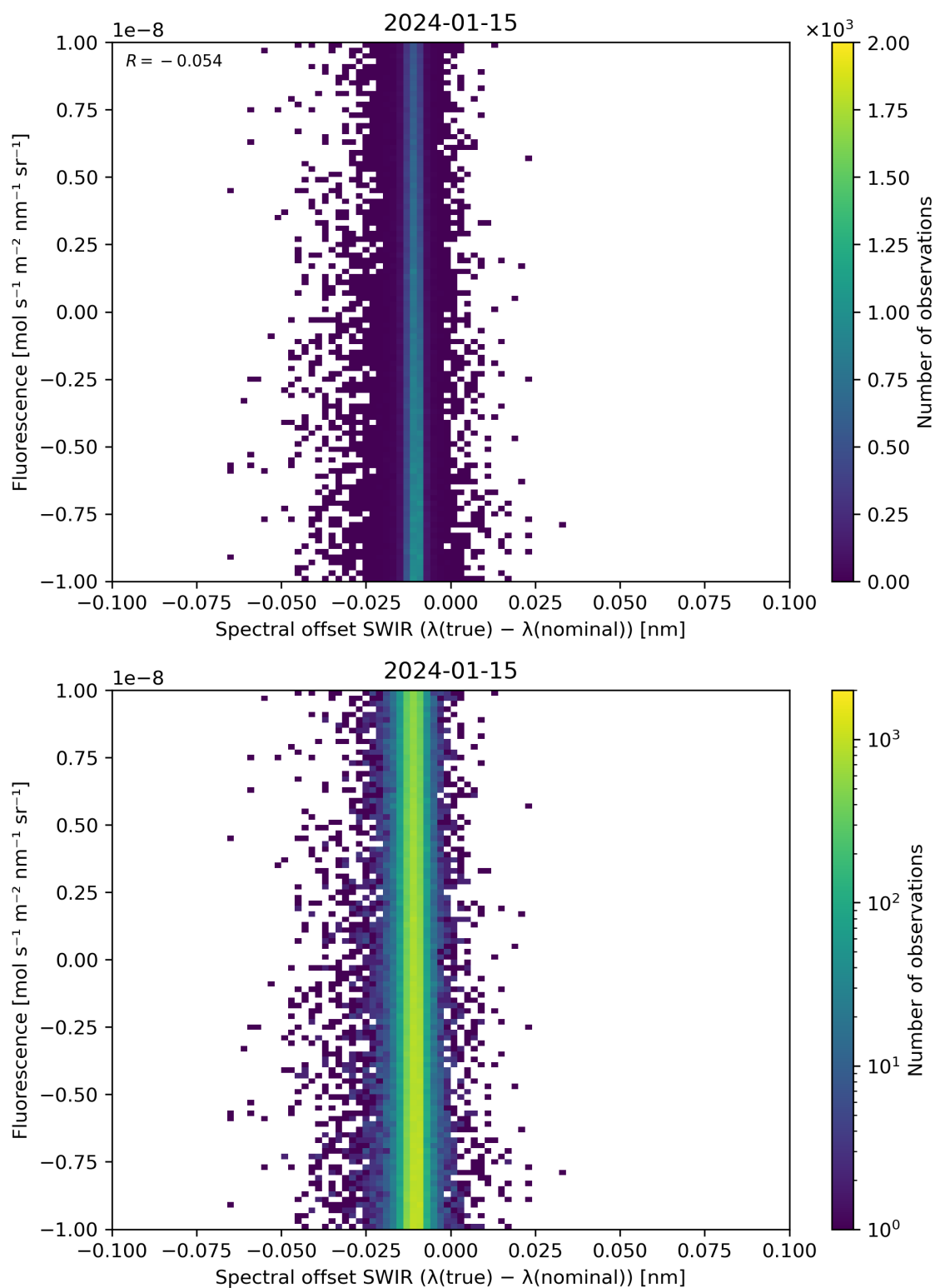
Figure 120: Scatter density plot of “Spectral offset SWIR ( \lambda(\text{true}) - \lambda(\text{nominal}) )” against “Fluorescence” for 2024-01-15 to 2024-01-16.
