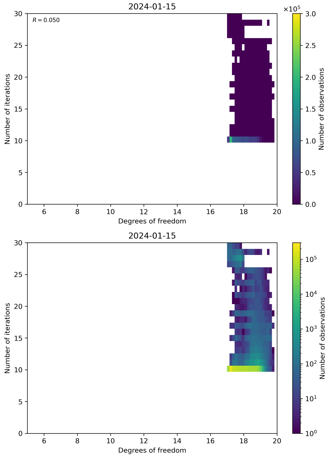
Figure 52: Scatter density plot of “Degrees of freedom” against “Number of iterations” for 2024-01-15 to 2024-01-16.
