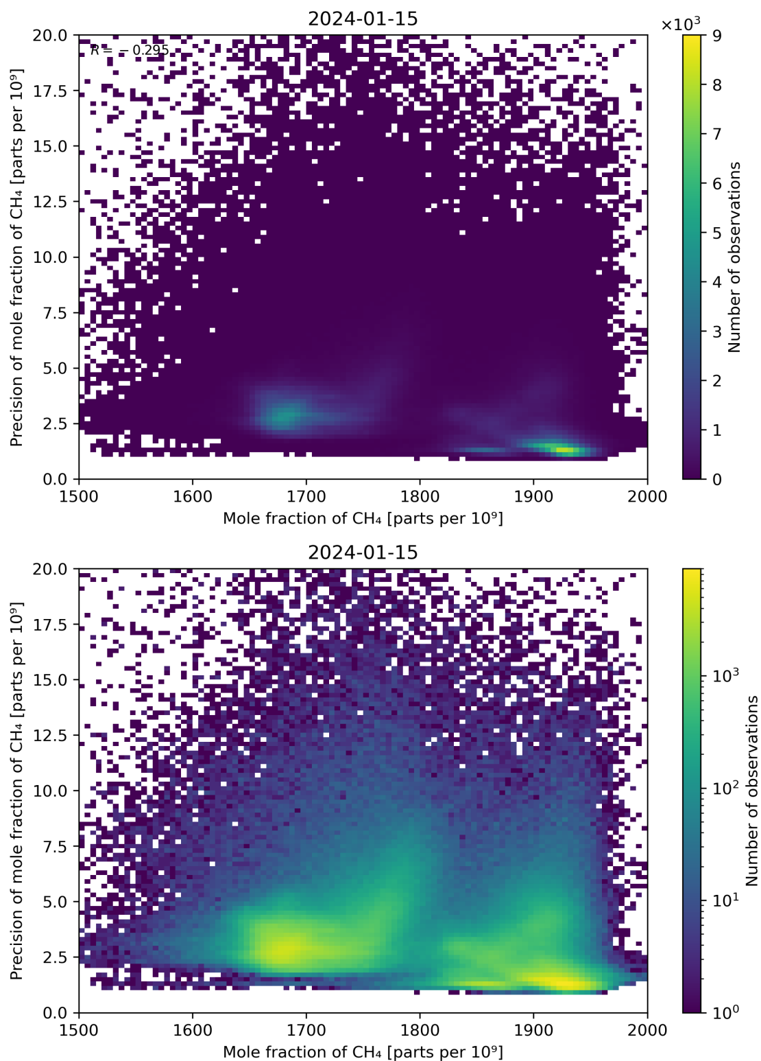
Figure 75: Scatter density plot of “Mole fraction of CH 4 ” against “Precision of mole fraction of CH 4 ” for 2024-01-15 to 2024-01-16.
