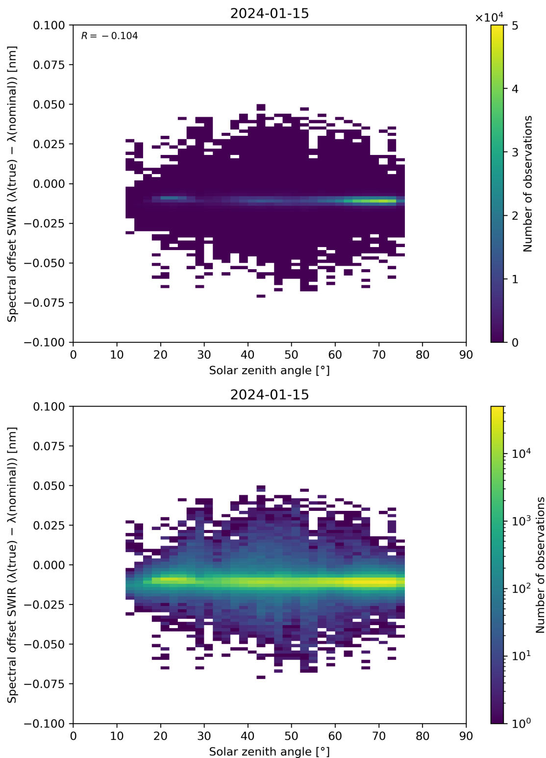
Figure 104: Scatter density plot of “Solar zenith angle” against “Spectral offset SWIR ( \lambda(\text{true}) - \lambda(\text{nominal}) )” for 2024-01-15 to 2024-01-16.
