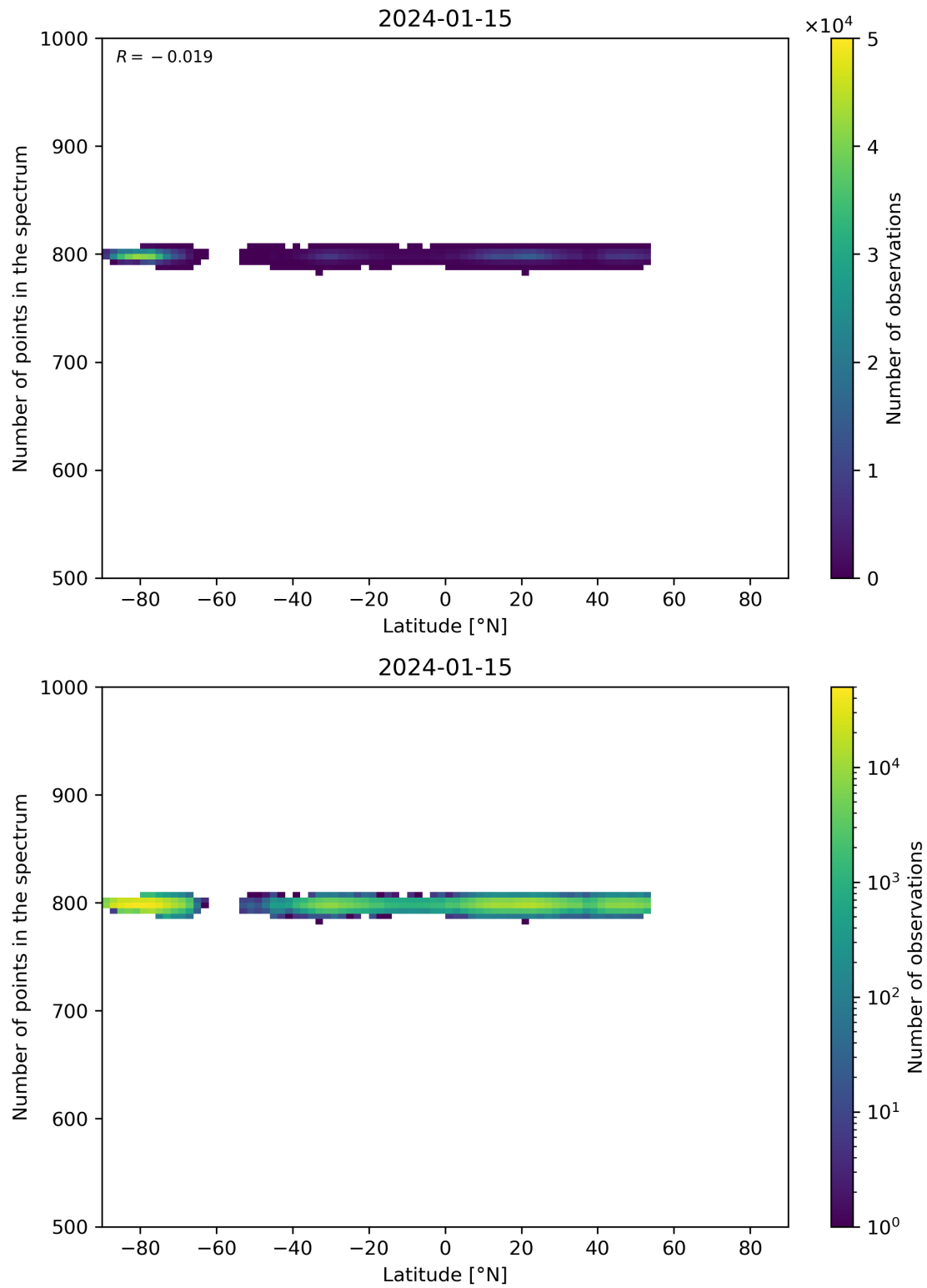
Figure 61: Scatter density plot of “Latitude” against “Number of points in the spectrum” for 2024-01-15 to 2024-01-16.
