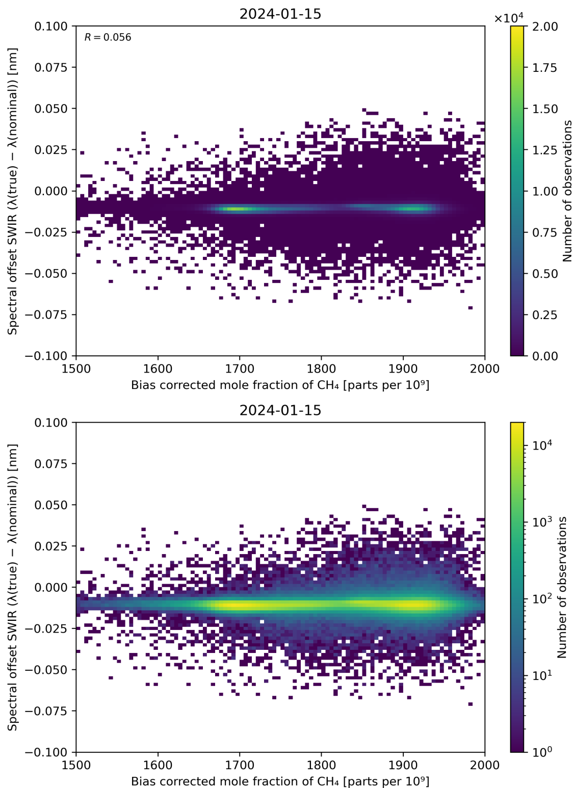
Figure 69: Scatter density plot of “Bias corrected mole fraction of \text{CH}_4 ” against “Spectral offset SWIR ( \lambda(\text{true}) - \lambda(\text{nominal}) )” for 2024-01-15 to 2024-01-16.
