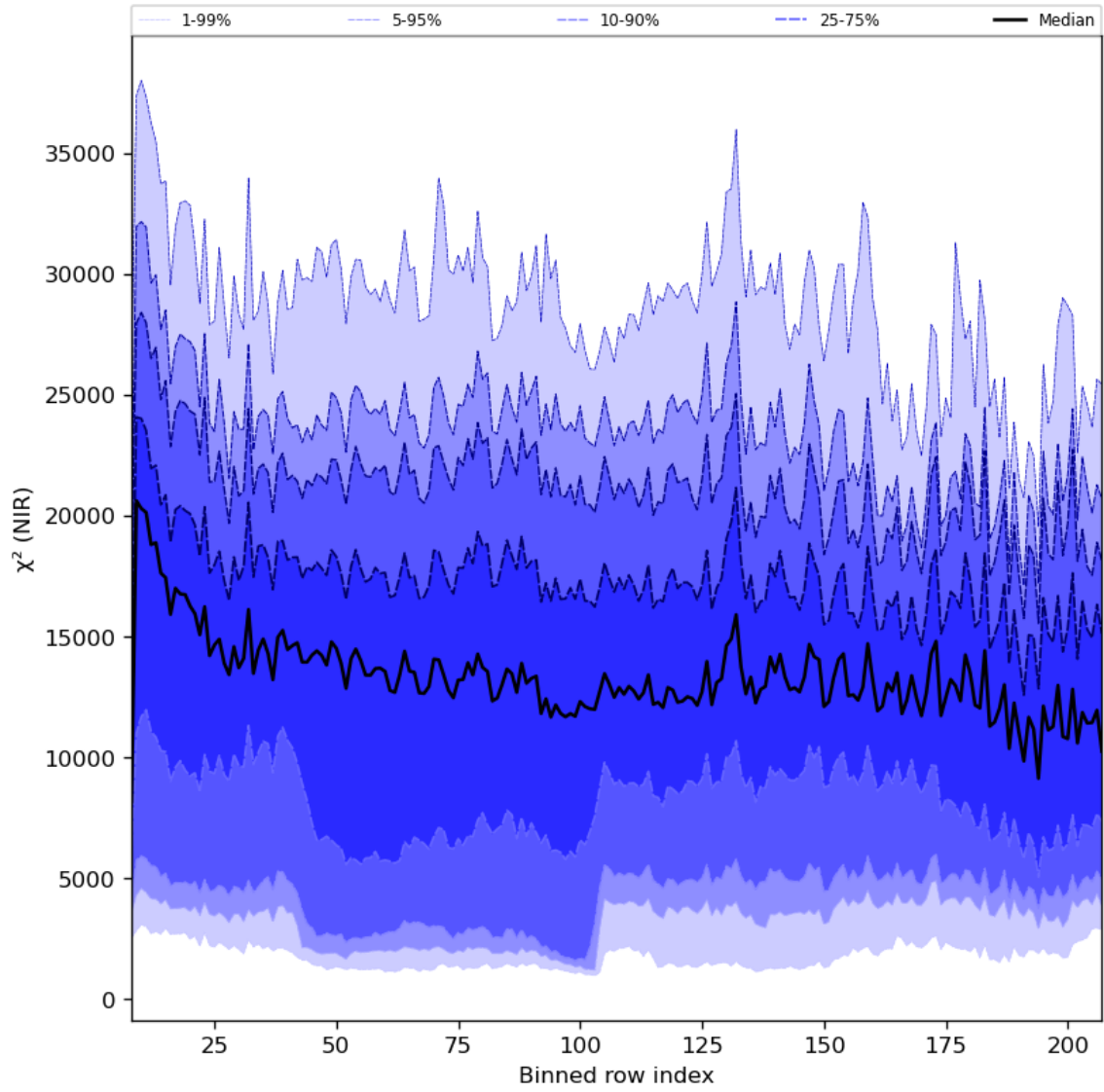
Figure 40: Along track statistics of " \chi^2 (NIR)" for 2024-01-15 to 2024-01-16
