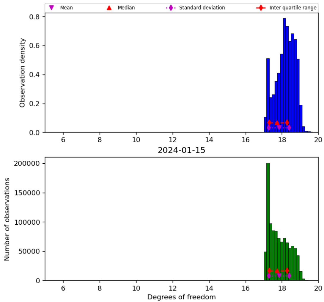
Figure 30: Histogram of “Degrees of freedom” for 2024-01-15 to 2024-01-16
