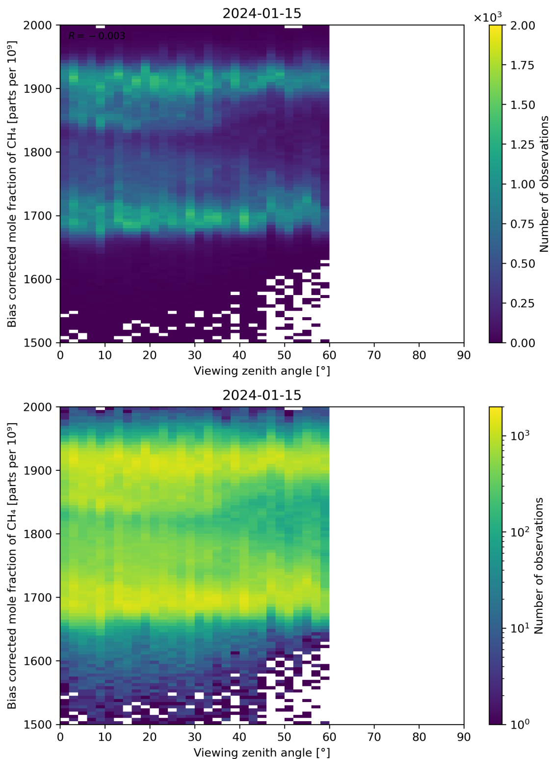
Figure 111: Scatter density plot of “Viewing zenith angle” against “Bias corrected mole fraction of CH 4 ” for 2024-01-15 to 2024-01-16.
