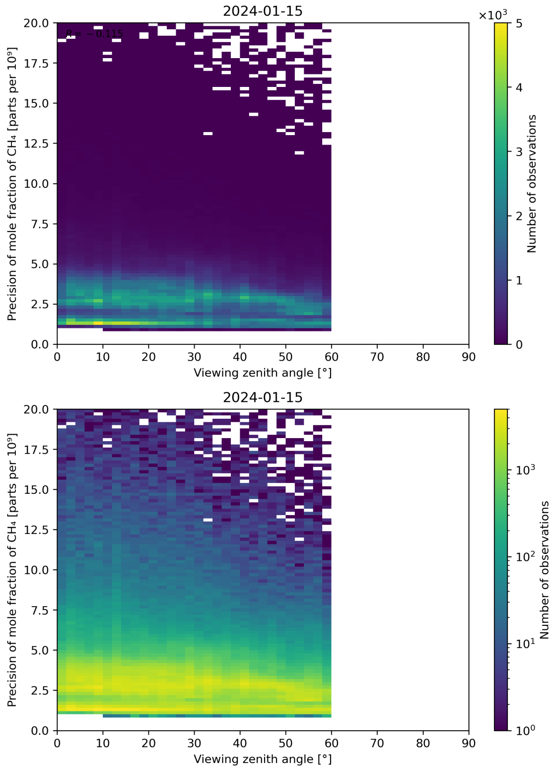
Figure 112: Scatter density plot of “Viewing zenith angle” against “Precision of mole fraction of CH 4 ” for 2024-01-15 to 2024-01-16.
