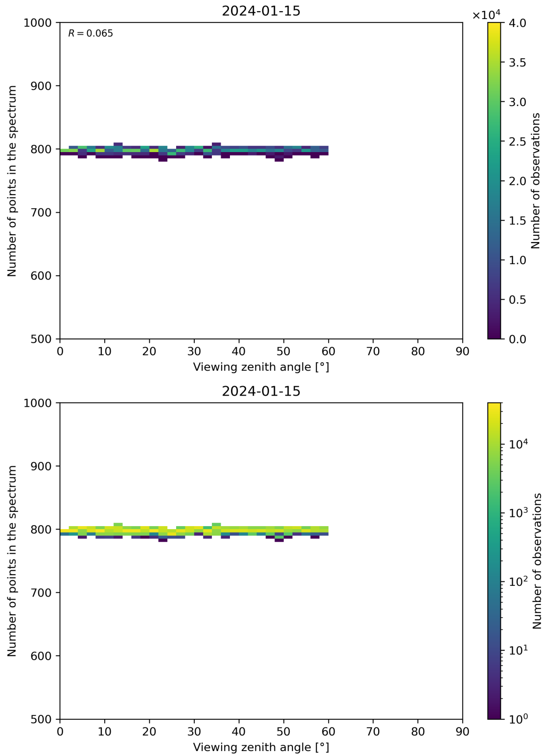
Figure 114: Scatter density plot of “Viewing zenith angle” against “Number of points in the spectrum” for 2024-01-15 to 2024-01-16.
