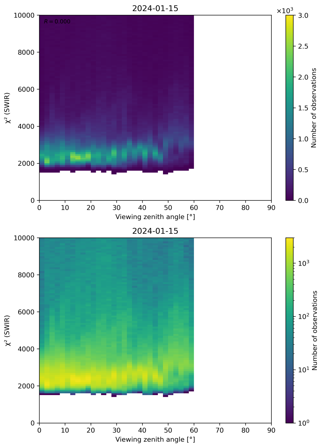
Figure 106: Scatter density plot of “Viewing zenith angle” against “ \chi^2 (SWIR)” for 2024-01-15 to 2024-01-16.
