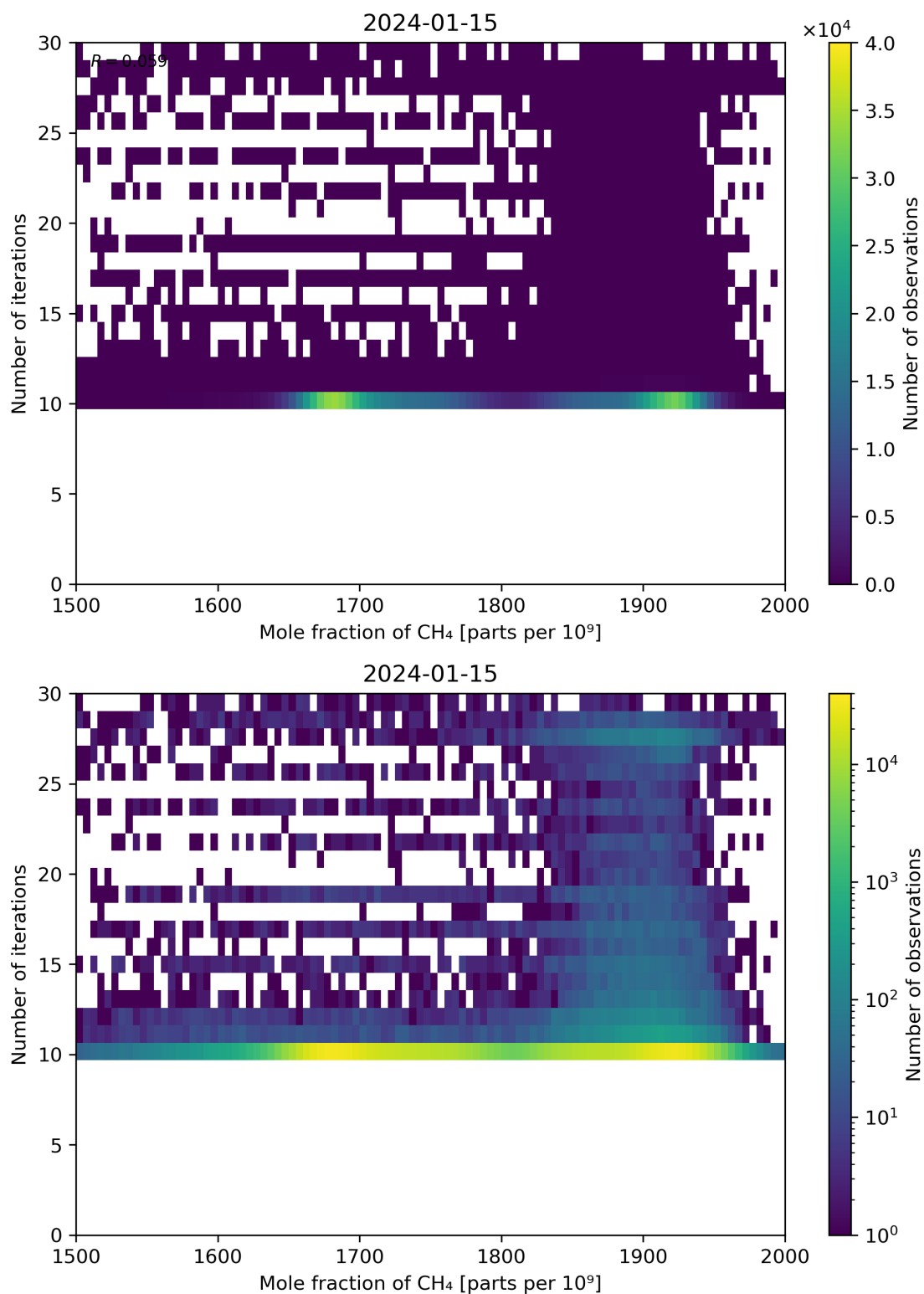
Figure 76: Scatter density plot of “Mole fraction of CH 4 ” against “Number of iterations” for 2024-01-15 to 2024-01-16.
