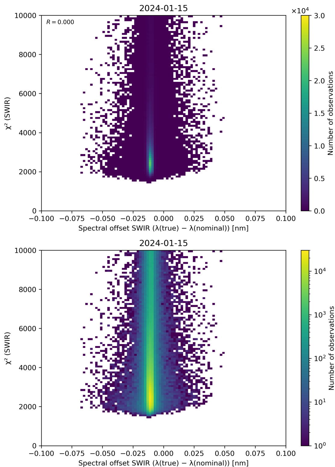
Figure 118: Scatter density plot of “Spectral offset SWIR ( \lambda(\text{true}) - \lambda(\text{nominal}) )” against “ \chi^2 (SWIR)” for 2024-01-15 to 2024-01-16.
