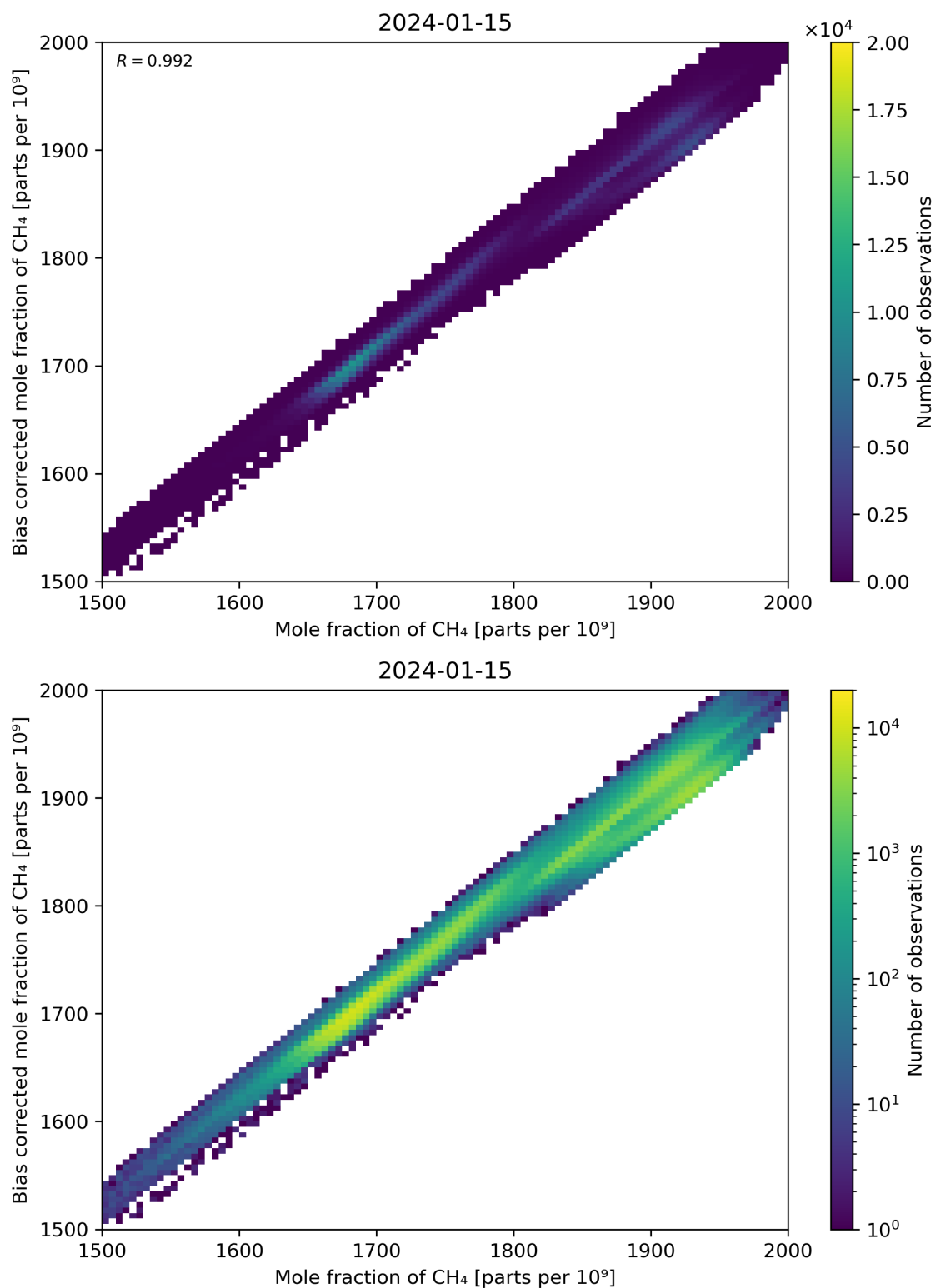
Figure 74: Scatter density plot of “Mole fraction of CH 4 ” against “Bias corrected mole fraction of CH 4 ” for 2024-01-15 to 2024-01-16.
