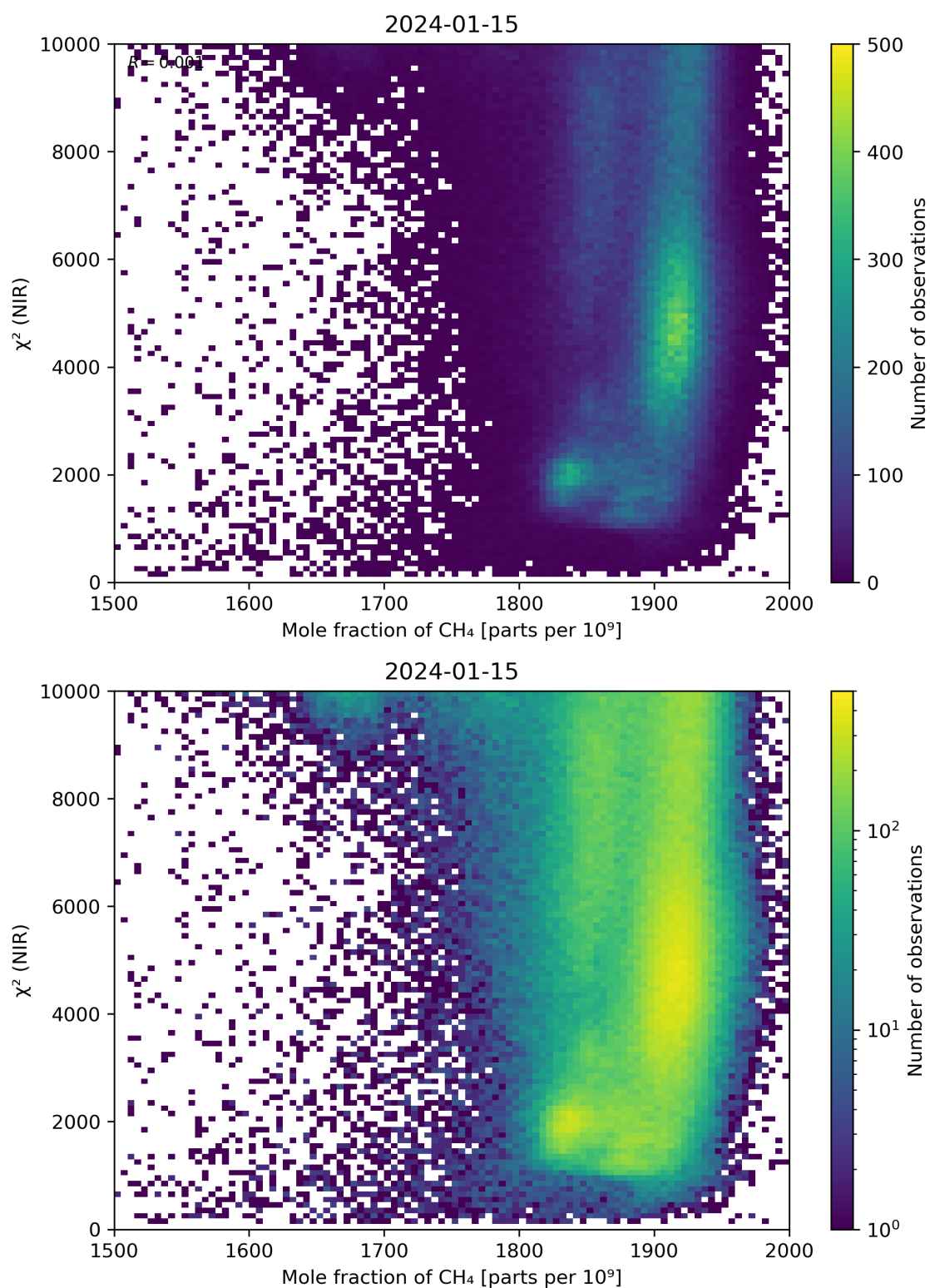
Figure 70: Scatter density plot of “Mole fraction of \text{CH}_4 ” against “ \chi^2 (NIR)” for 2024-01-15 to 2024-01-16.
