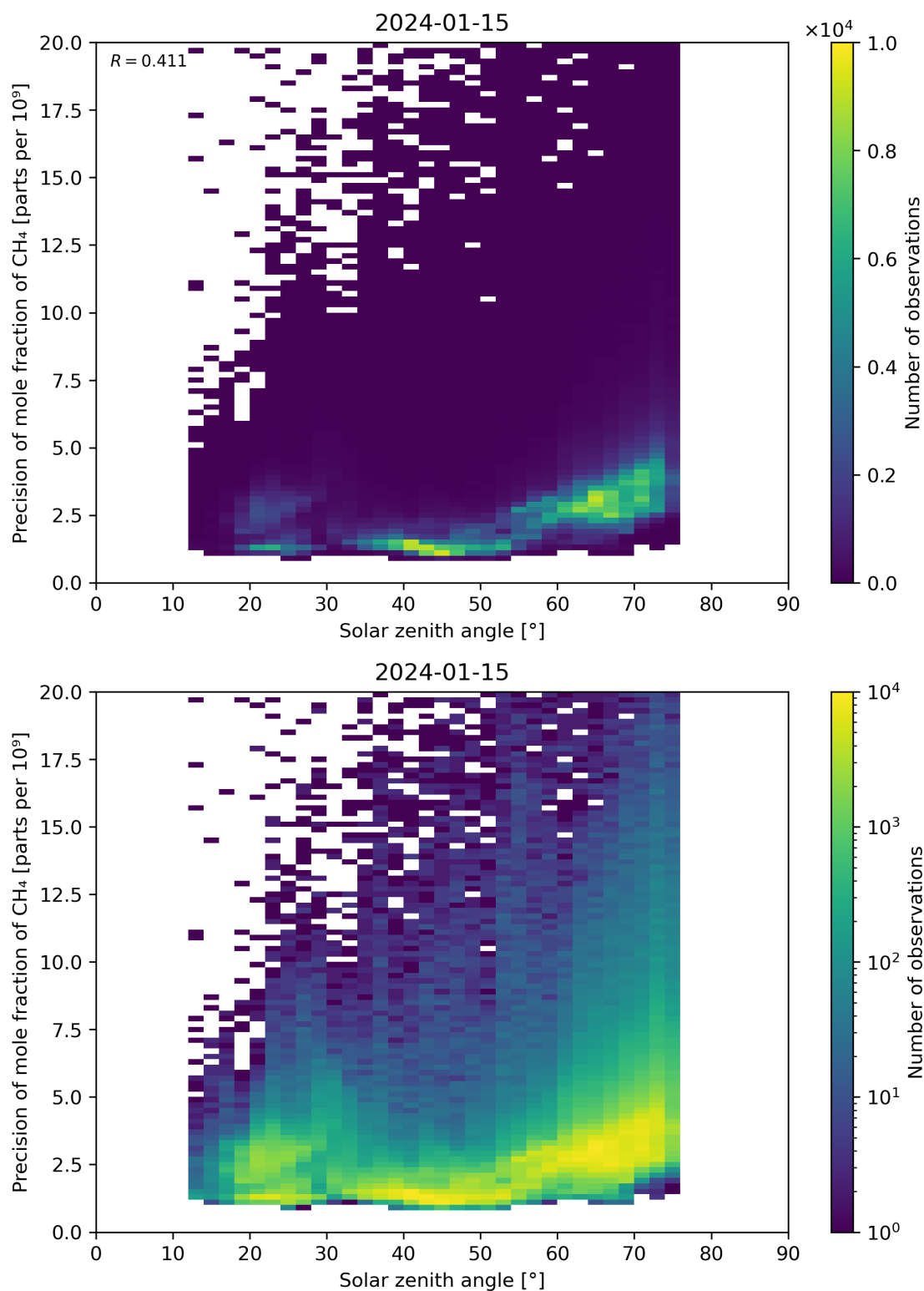
Figure 101: Scatter density plot of “Solar zenith angle” against “Precision of mole fraction of CH 4 ” for 2024-01-15 to 2024-01-16.
