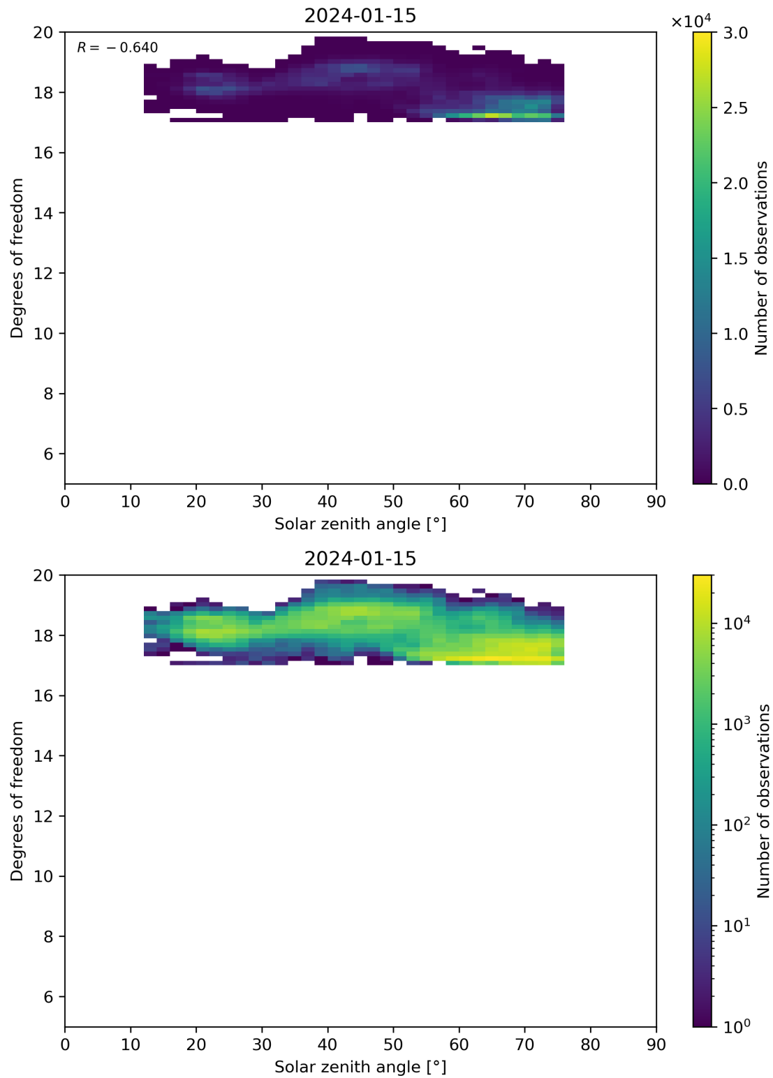
Figure 96: Scatter density plot of “Solar zenith angle” against “Degrees of freedom” for 2024-01-15 to 2024-01-16.
