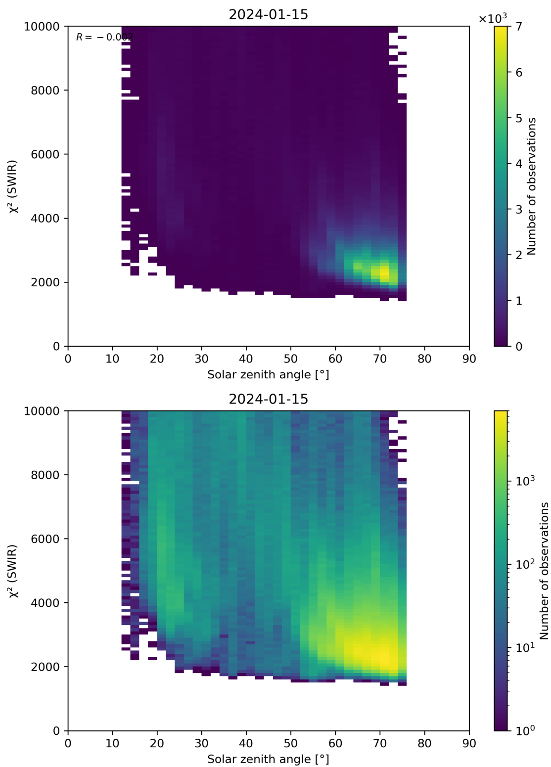
Figure 95: Scatter density plot of “Solar zenith angle” against “ \chi^2 (SWIR)” for 2024-01-15 to 2024-01-16.
