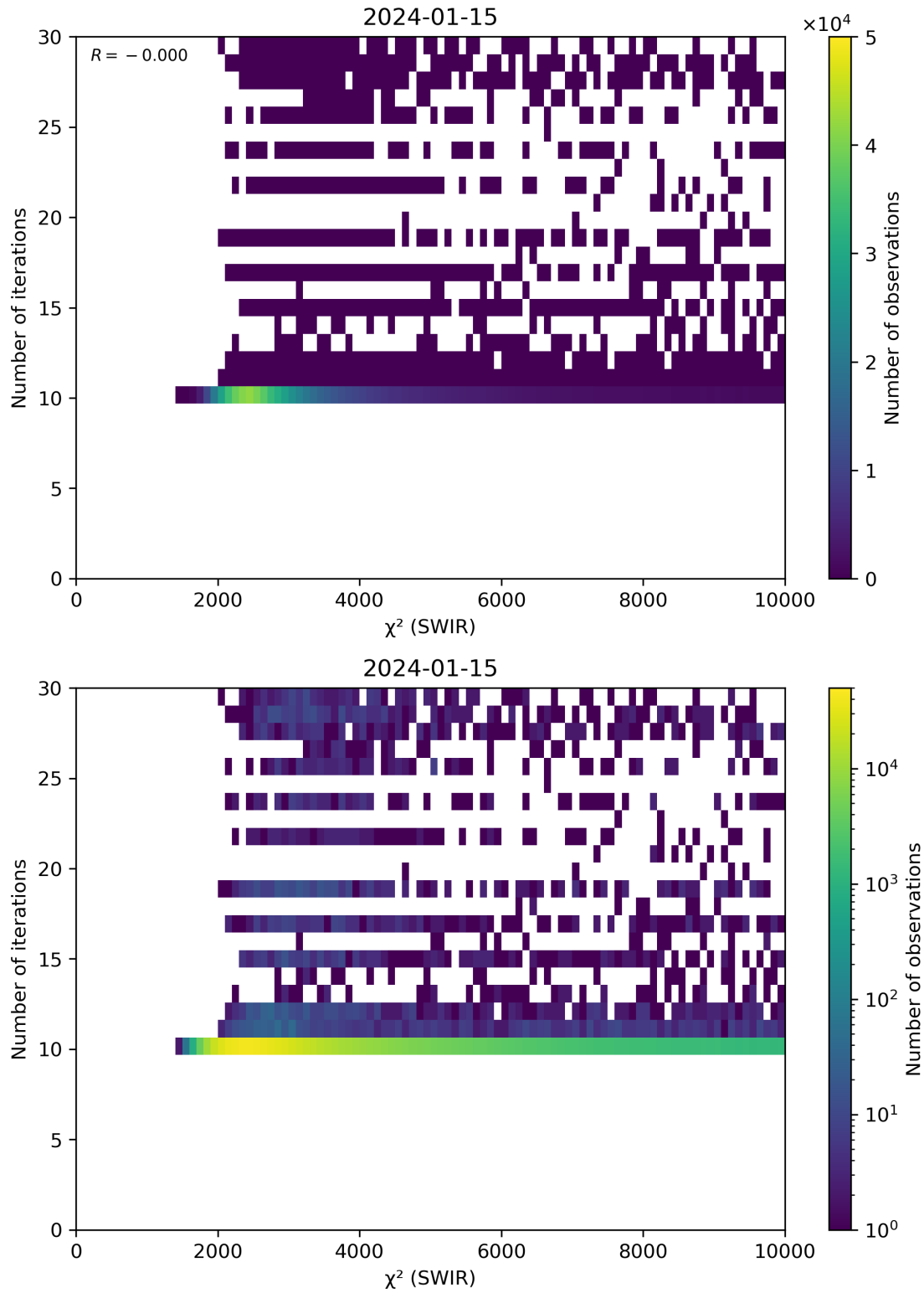
Figure 50: Scatter density plot of “ \chi^2 (SWIR)” against “Number of iterations” for 2024-01-15 to 2024-01-16.
