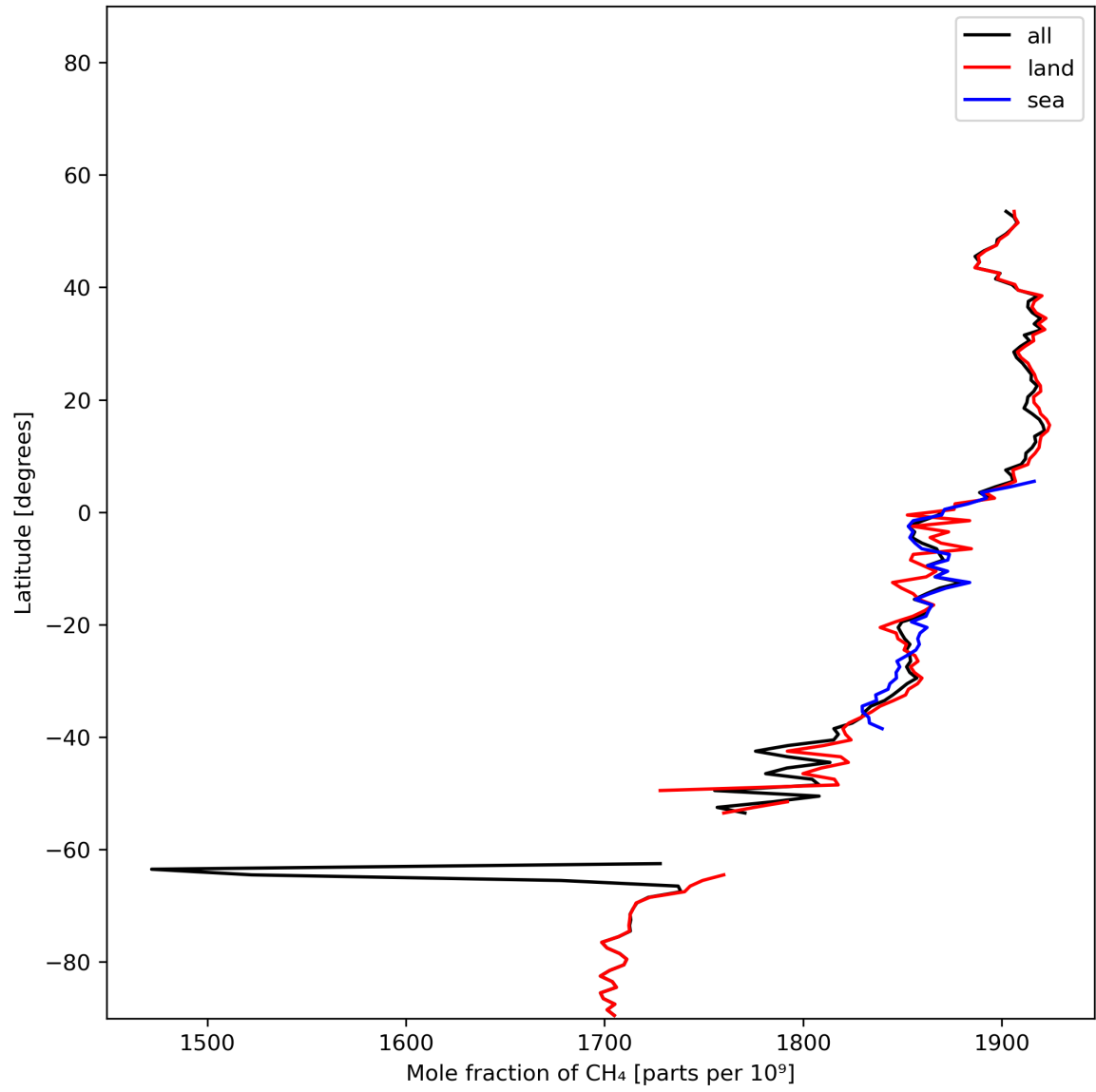
Figure 12: Zonal average of “Mole fraction of \text{CH}_4 ” for 2024-01-15 to 2024-01-16.
