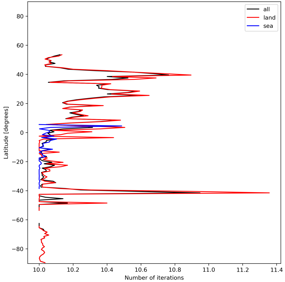
Figure 20: Zonal average of “Number of iterations” for 2024-01-15 to 2024-01-16.
