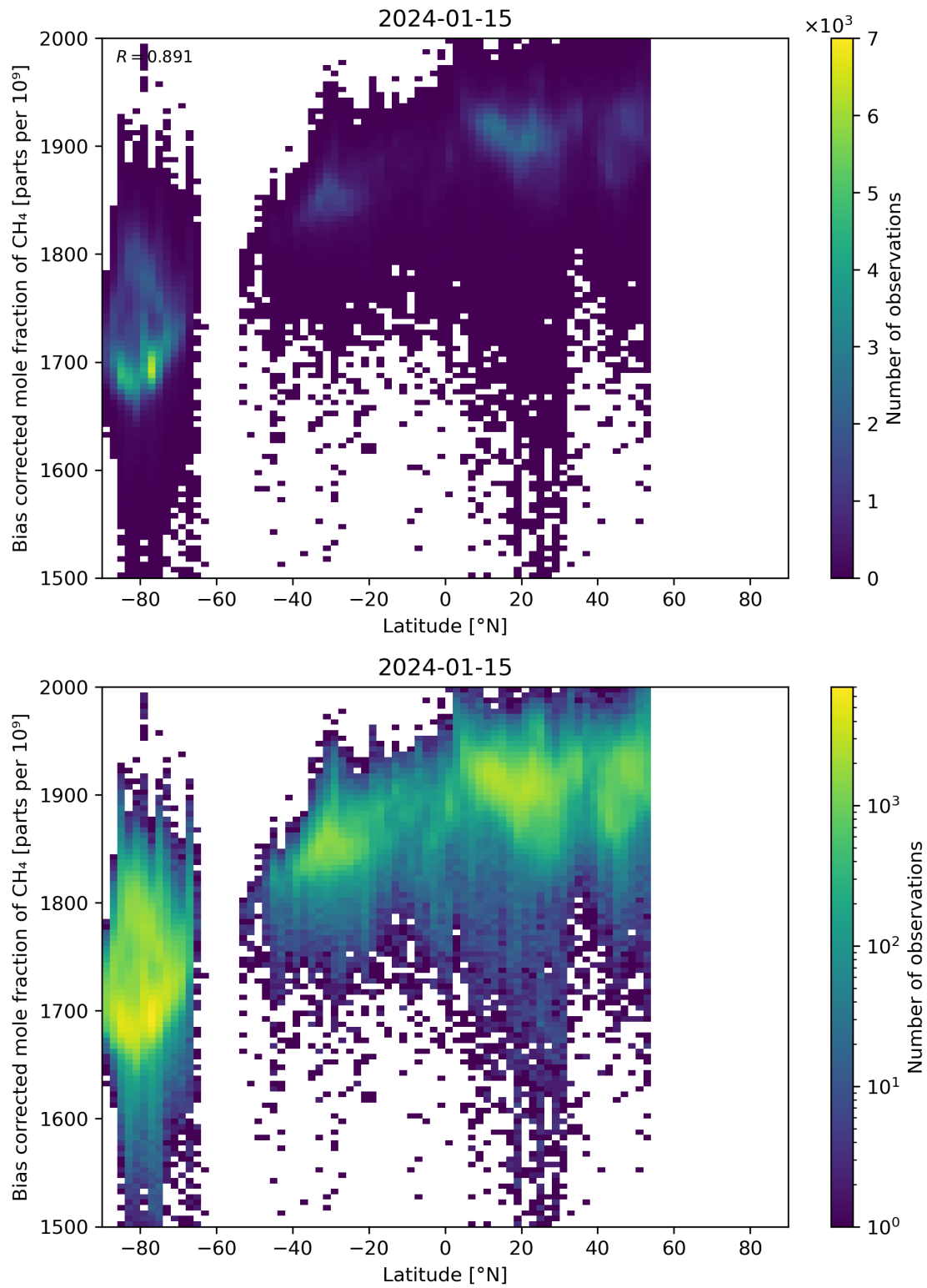
Figure 58: Scatter density plot of “Latitude” against “Bias corrected mole fraction of CH 4 ” for 2024-01-15 to 2024-01-16.
