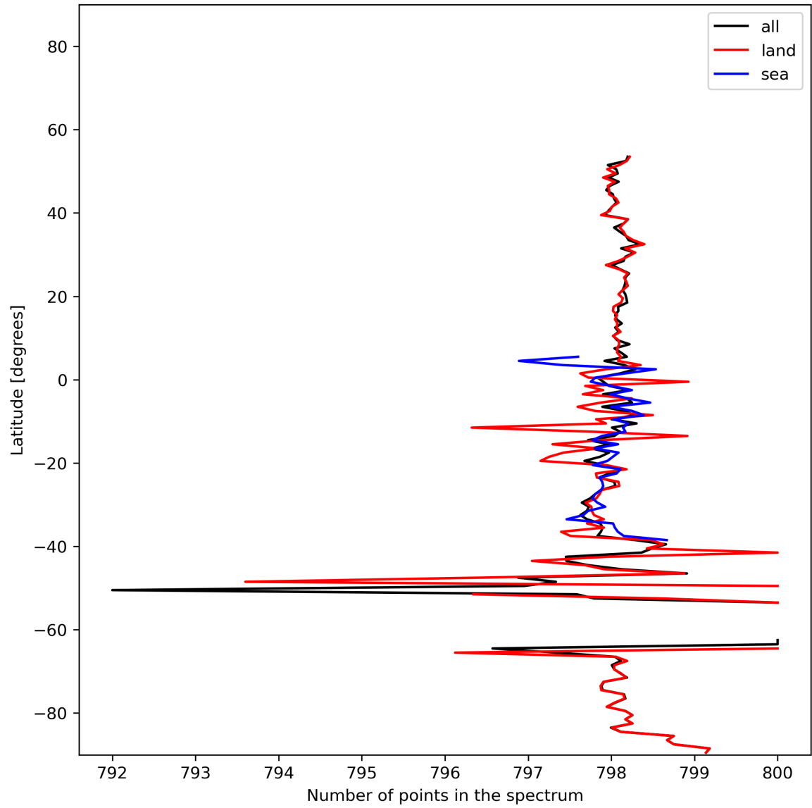
Figure 15: Zonal average of “Number of points in the spectrum” for 2024-01-15 to 2024-01-16.
