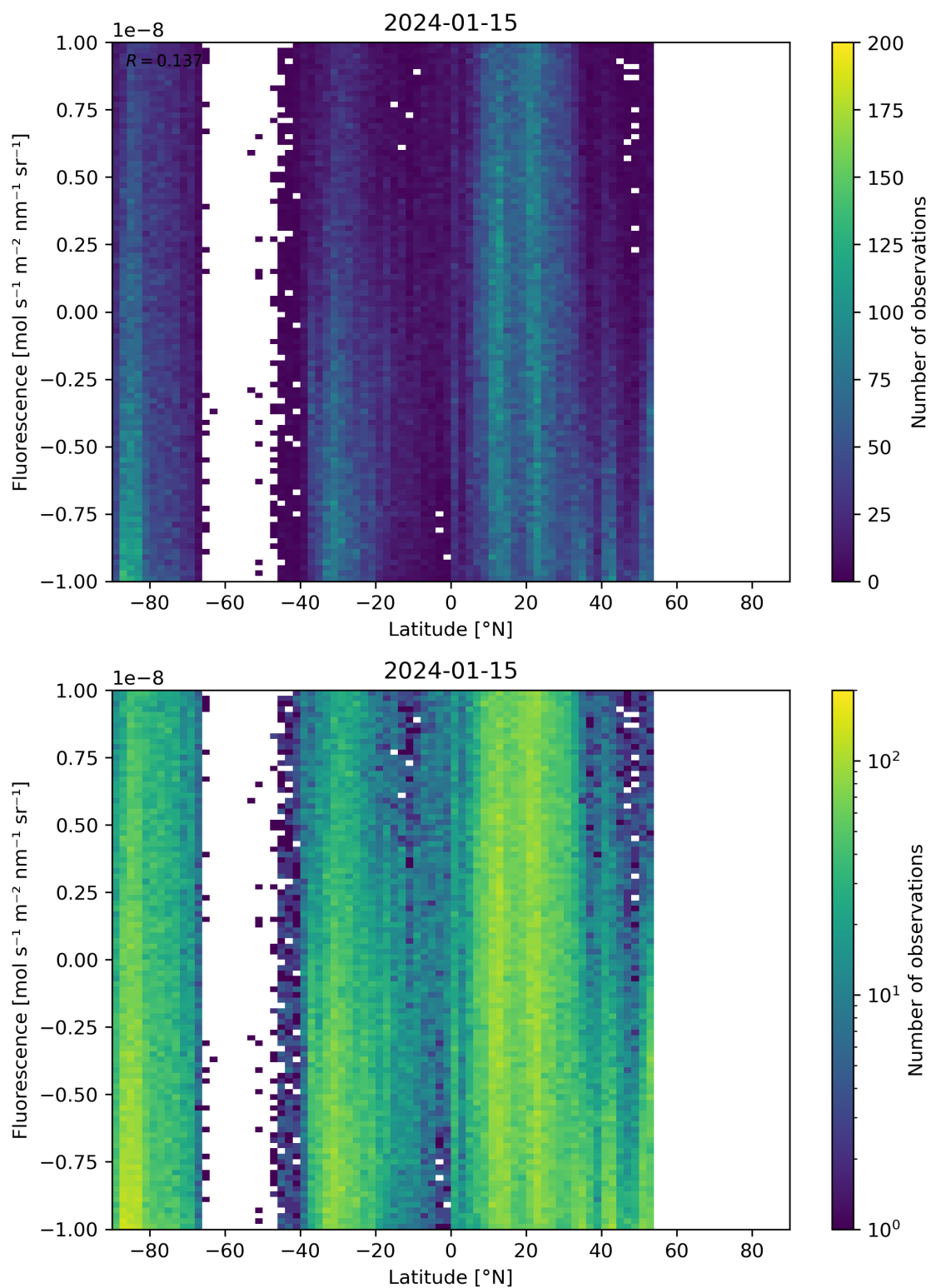
Figure 56: Scatter density plot of “Latitude” against “Fluorescence” for 2024-01-15 to 2024-01-16.
