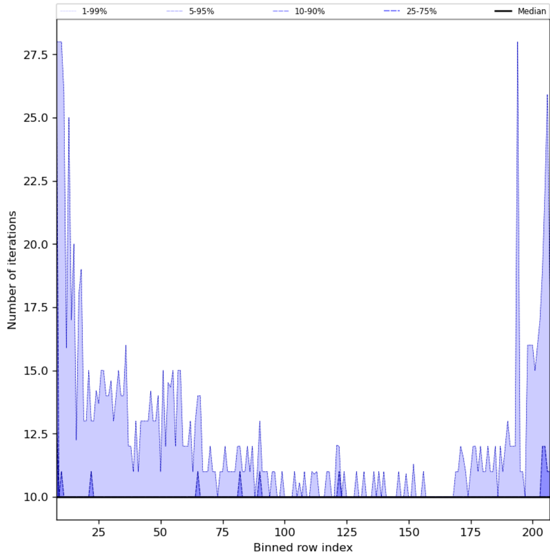
Figure 42: Along track statistics of “Number of iterations” for 2024-01-15 to 2024-01-16
