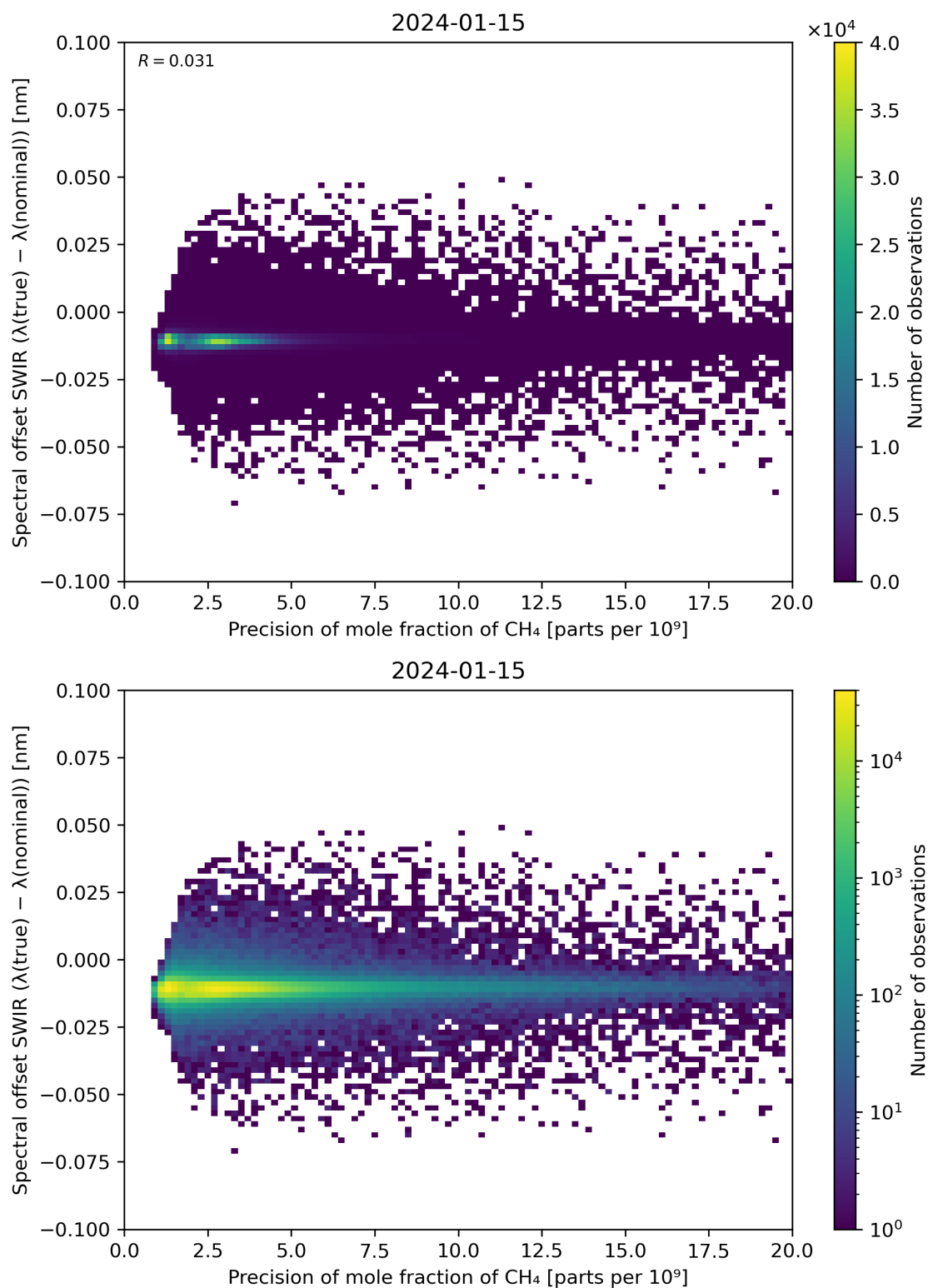
Figure 85: Scatter density plot of “Precision of mole fraction of CH 4 ” against “Spectral offset SWIR ( \lambda(\text{true}) - \lambda(\text{nominal}) )” for 2024-01-15 to 2024-01-16.
