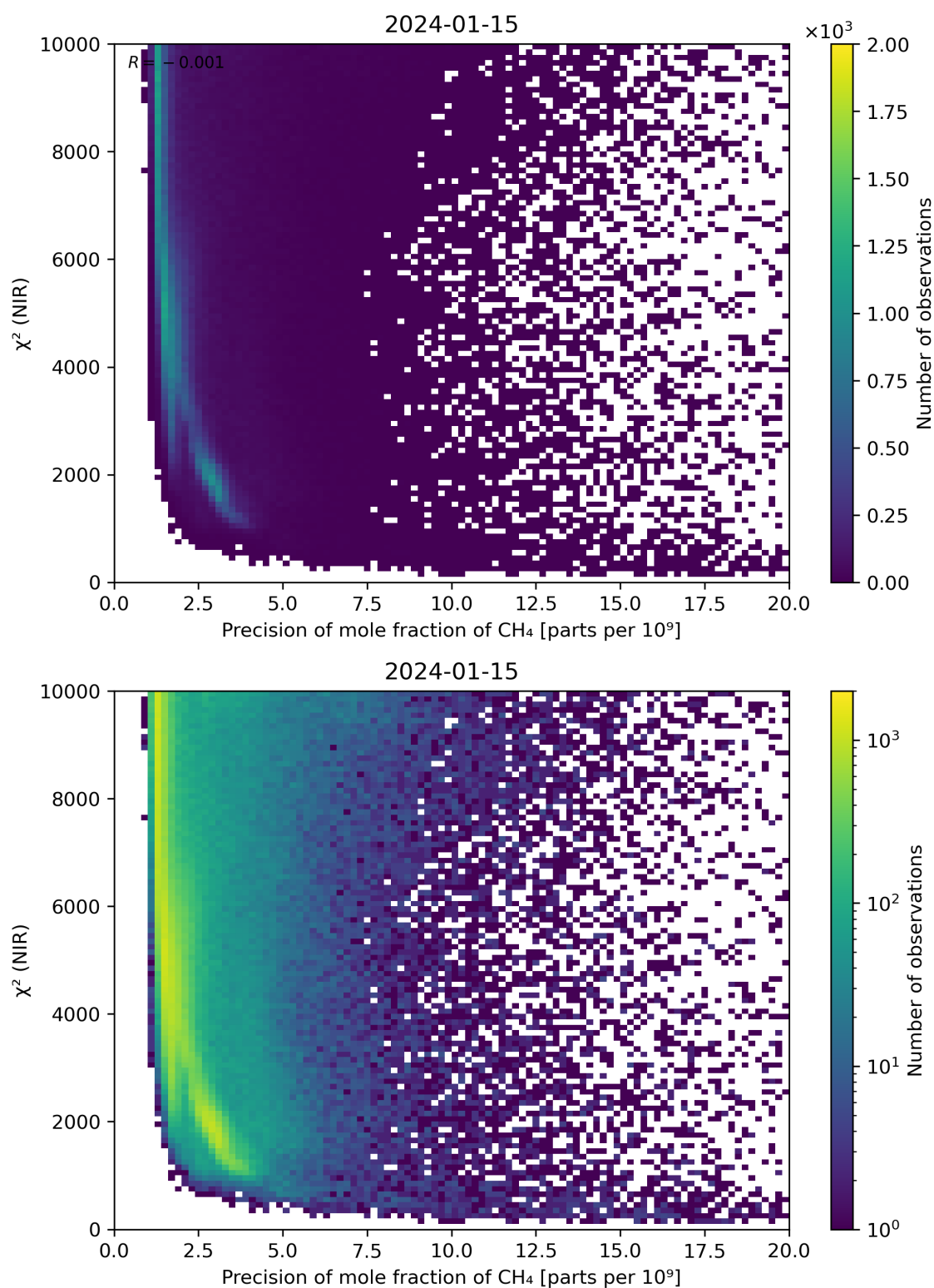
Figure 78: Scatter density plot of “Precision of mole fraction of CH 4 ” against “ \chi^2 (NIR)” for 2024-01-15 to 2024-01-16.
