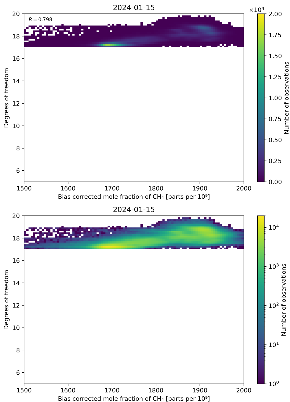
Figure 65: Scatter density plot of “Bias corrected mole fraction of CH 4 ” against “Degrees of freedom” for 2024-01-15 to 2024-01-16.
