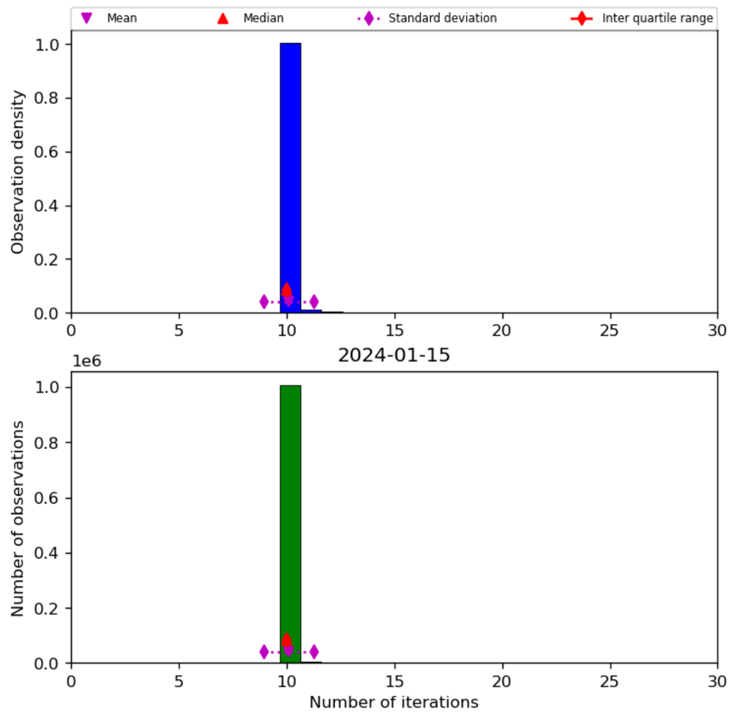
Figure 31: Histogram of “Number of iterations” for 2024-01-15 to 2024-01-16
