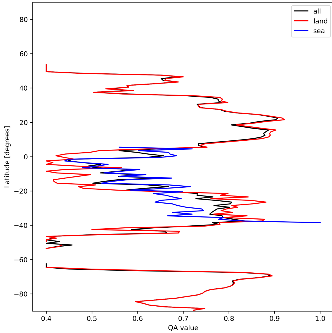
Figure 11: Zonal average of “QA value” for 2024-01-15 to 2024-01-16.
