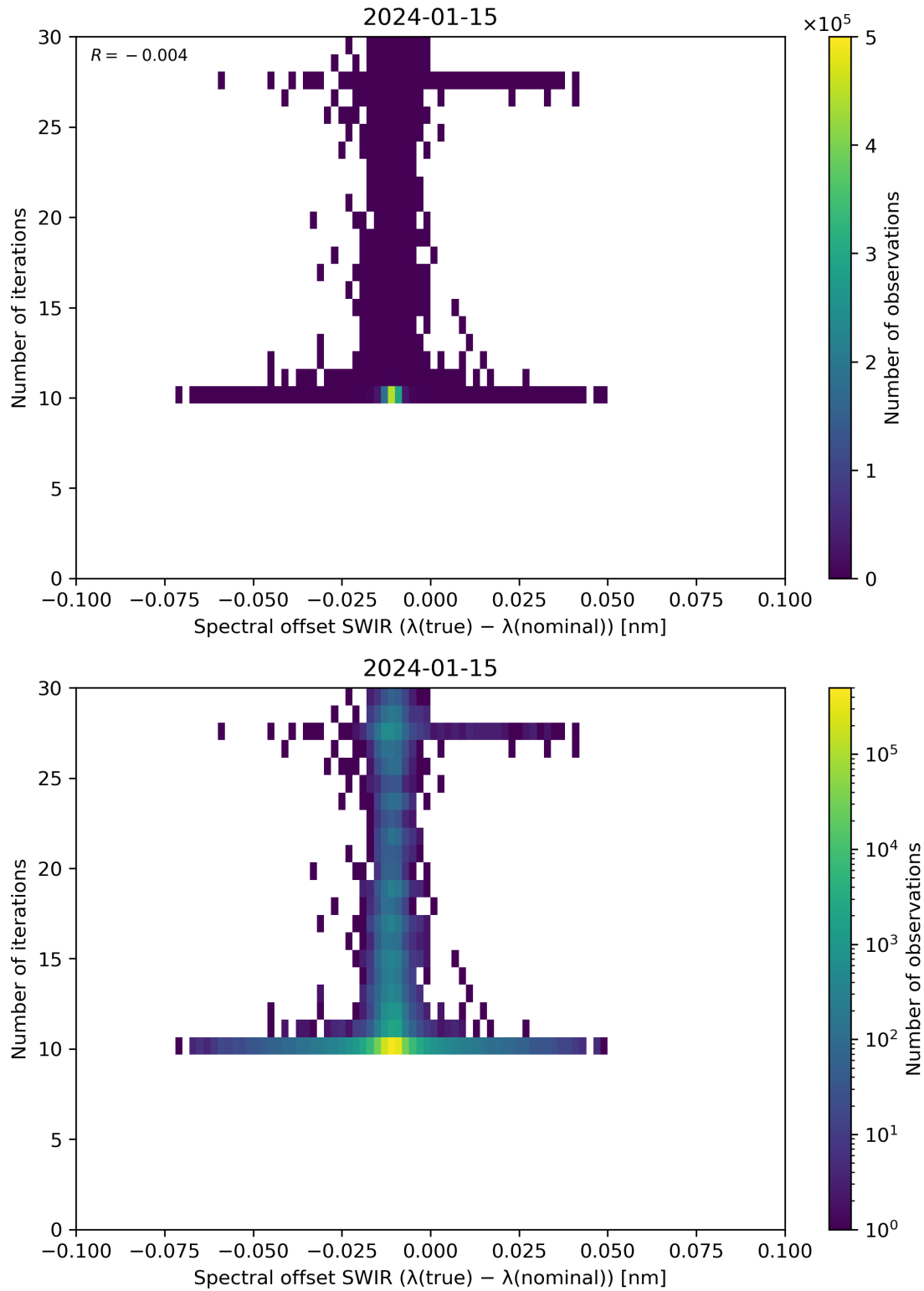
Figure 121: Scatter density plot of “Spectral offset SWIR ( \lambda(\text{true}) - \lambda(\text{nominal}) )” against “Number of iterations” for 2024-01-15 to 2024-01-16.
