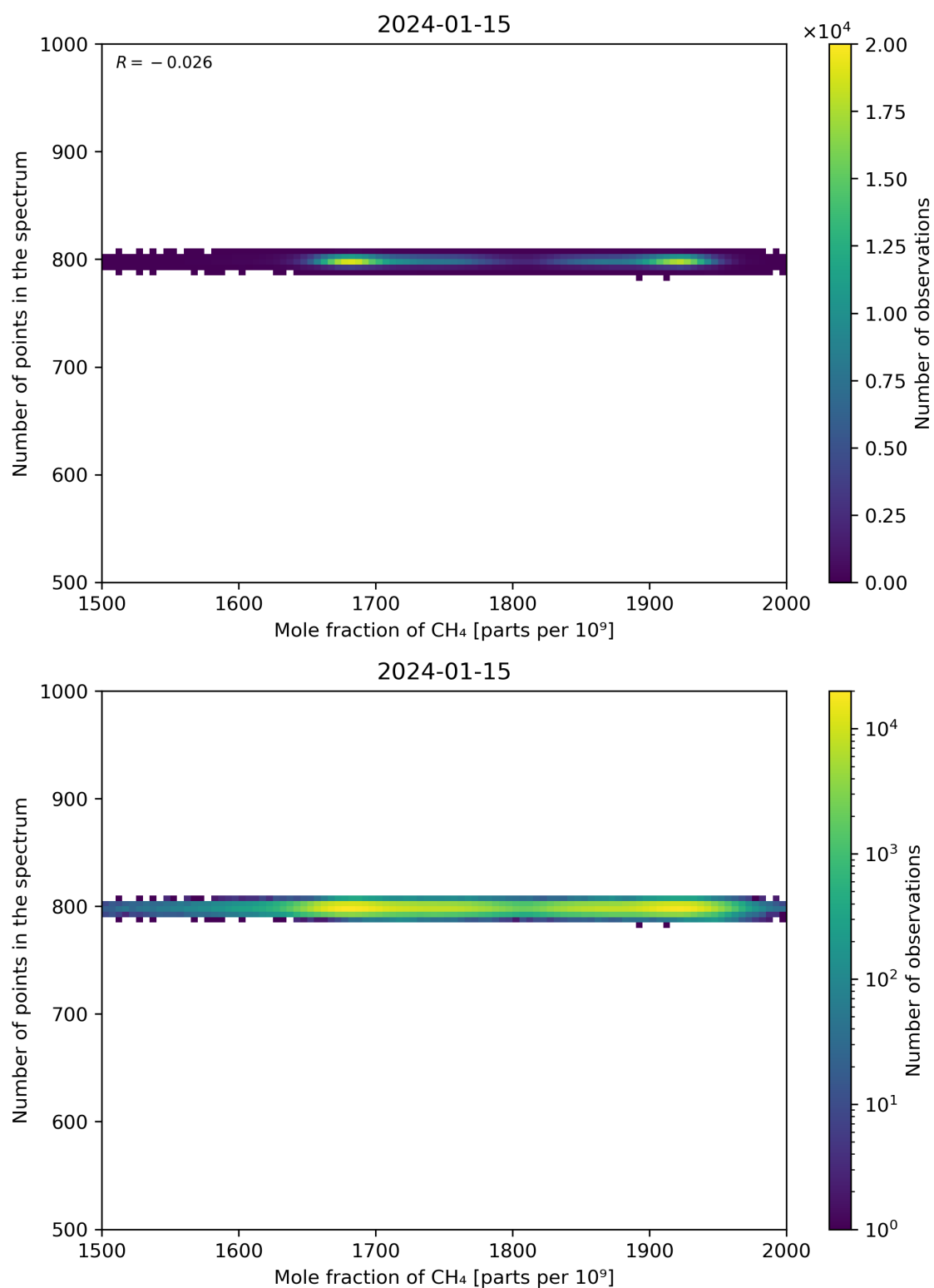
Figure 77: Scatter density plot of “Mole fraction of CH 4 ” against “Number of points in the spectrum” for 2024-01-15 to 2024-01-16.
