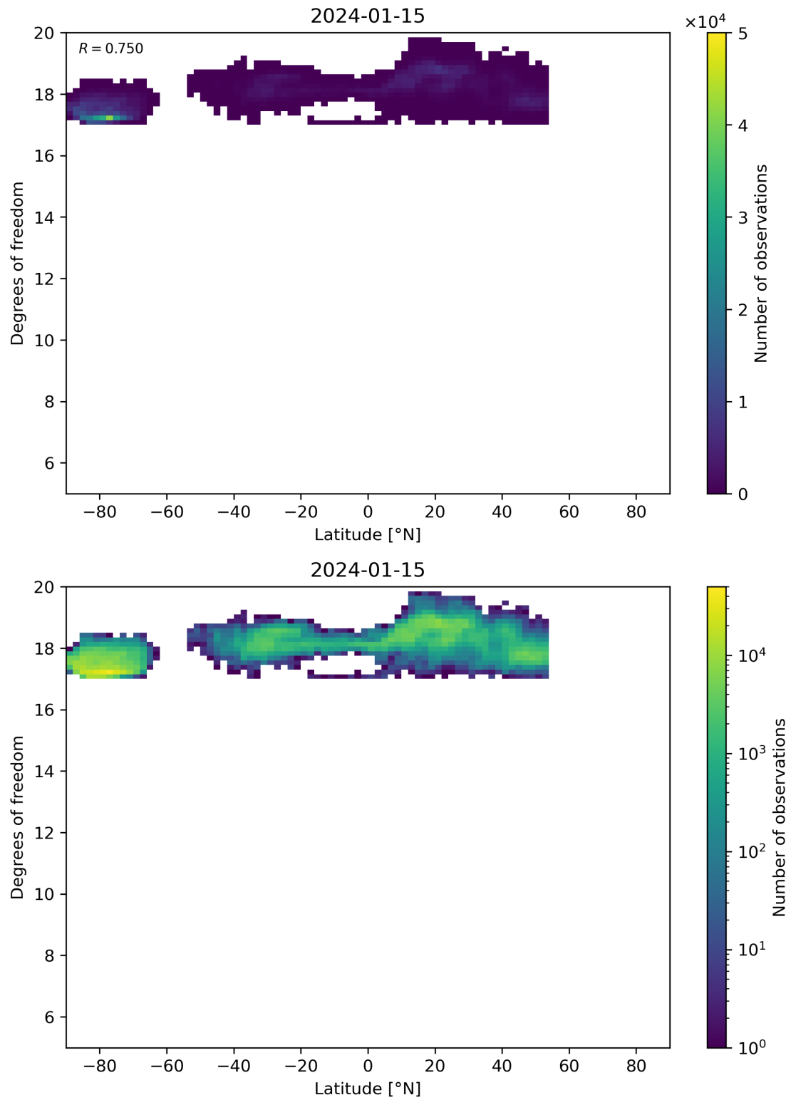
Figure 55: Scatter density plot of “Latitude” against “Degrees of freedom” for 2024-01-15 to 2024-01-16.
