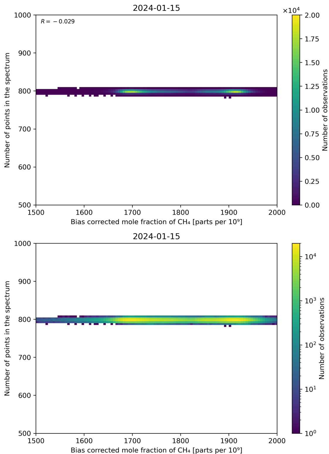
Figure 68: Scatter density plot of “Bias corrected mole fraction of CH 4 ” against “Number of points in the spectrum” for 2024-01-15 to 2024-01-16.
