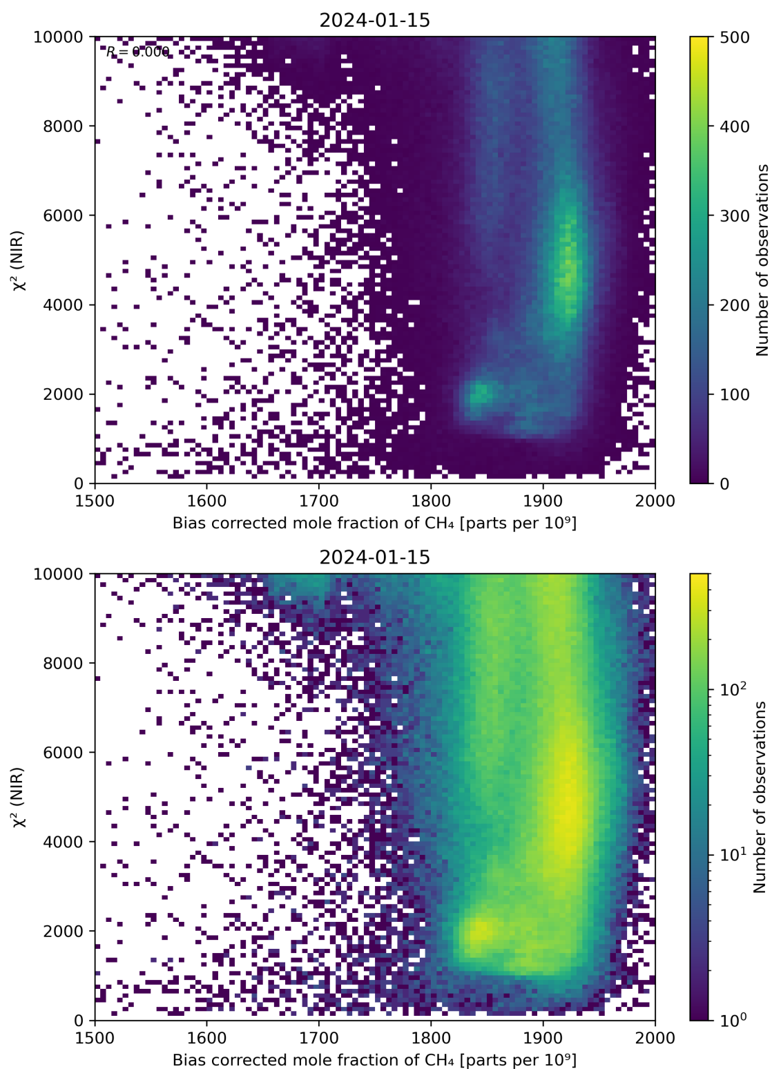
Figure 63: Scatter density plot of “Bias corrected mole fraction of \text{CH}_4 ” against “ \chi^2 (NIR)” for 2024-01-15 to 2024-01-16.
