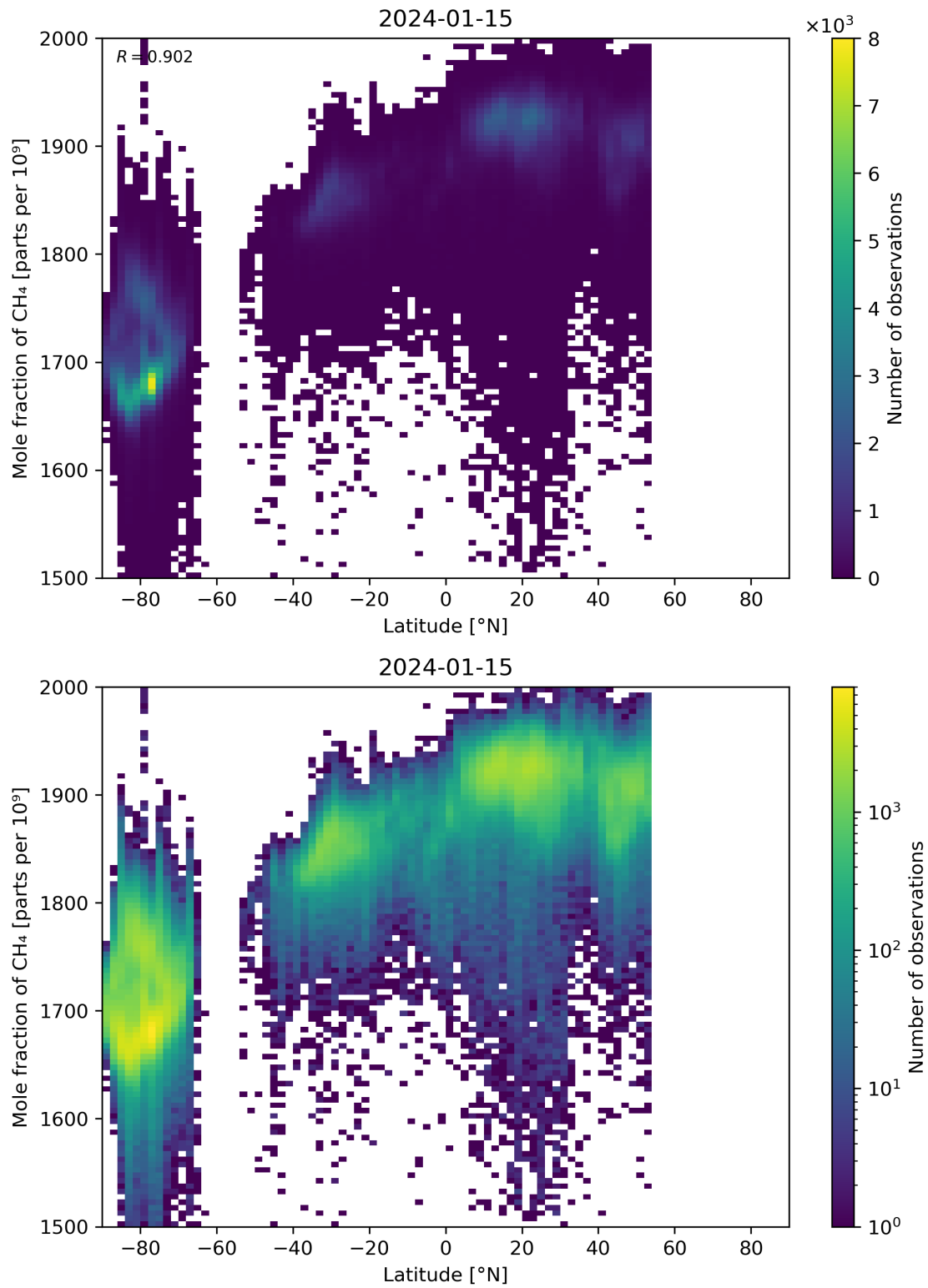
Figure 57: Scatter density plot of “Latitude” against “Mole fraction of CH 4 ” for 2024-01-15 to 2024-01-16.
