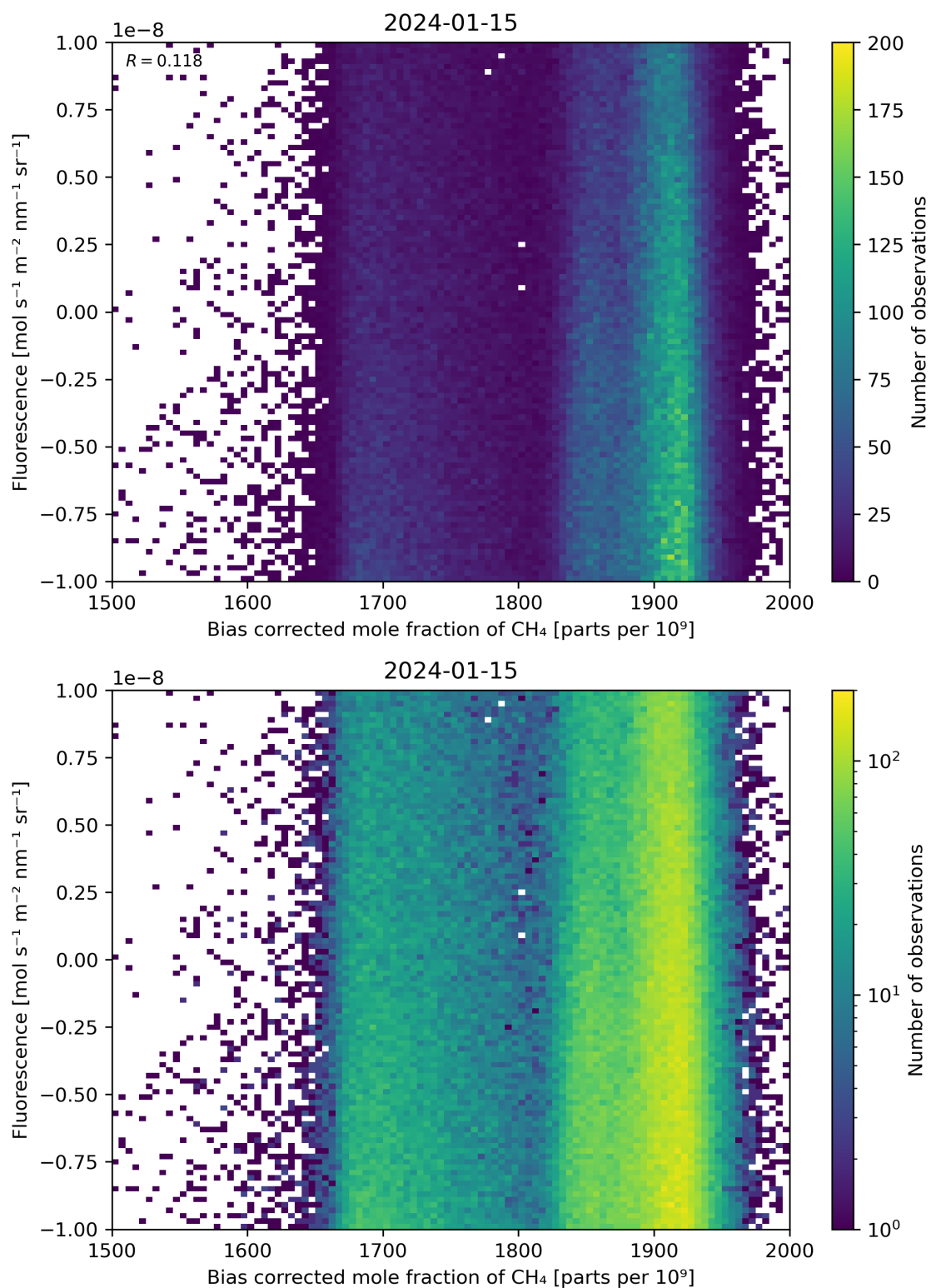
Figure 66: Scatter density plot of “Bias corrected mole fraction of \text{CH}_4 ” against “Fluorescence” for 2024-01-15 to 2024-01-16.
