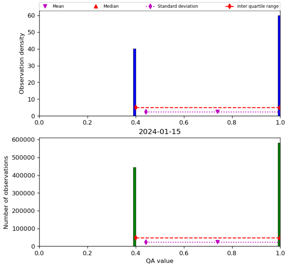
Figure 22: Histogram of “QA value” for 2024-01-15 to 2024-01-16
