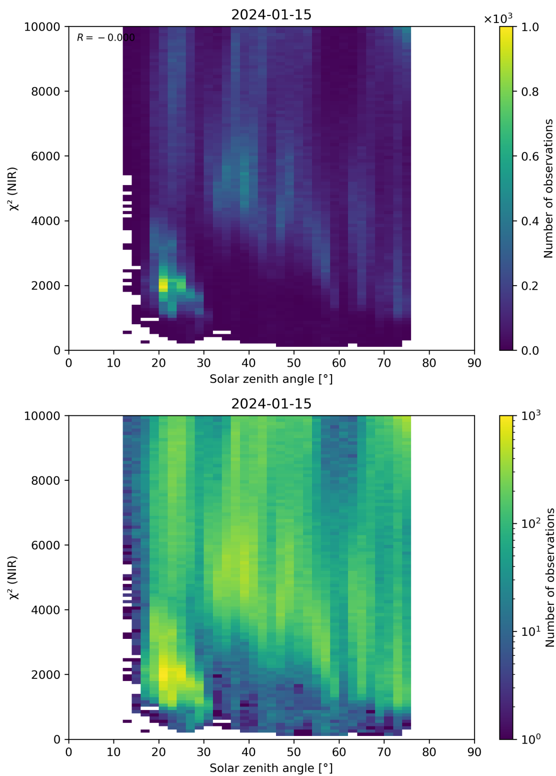
Figure 94: Scatter density plot of “Solar zenith angle” against “ \chi^2 (NIR)” for 2024-01-15 to 2024-01-16.
