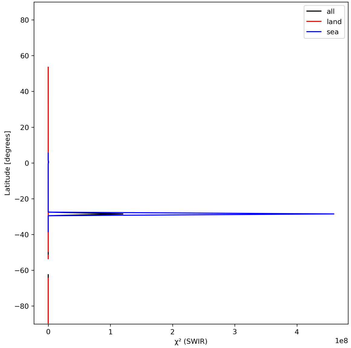
Figure 17: Zonal average of “ \chi^2 (SWIR)” for 2024-01-15 to 2024-01-16.
