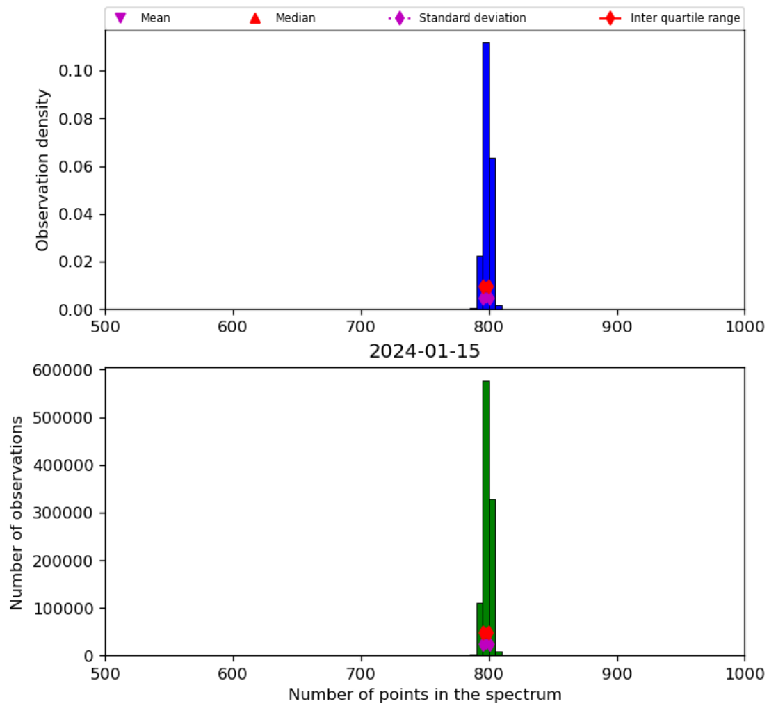
Figure 26: Histogram of “Number of points in the spectrum” for 2024-01-15 to 2024-01-16
