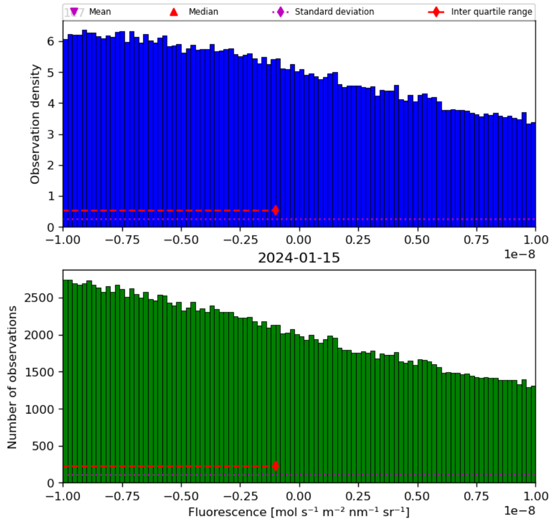
Figure 32: Histogram of “Fluorescence” for 2024-01-15 to 2024-01-16
