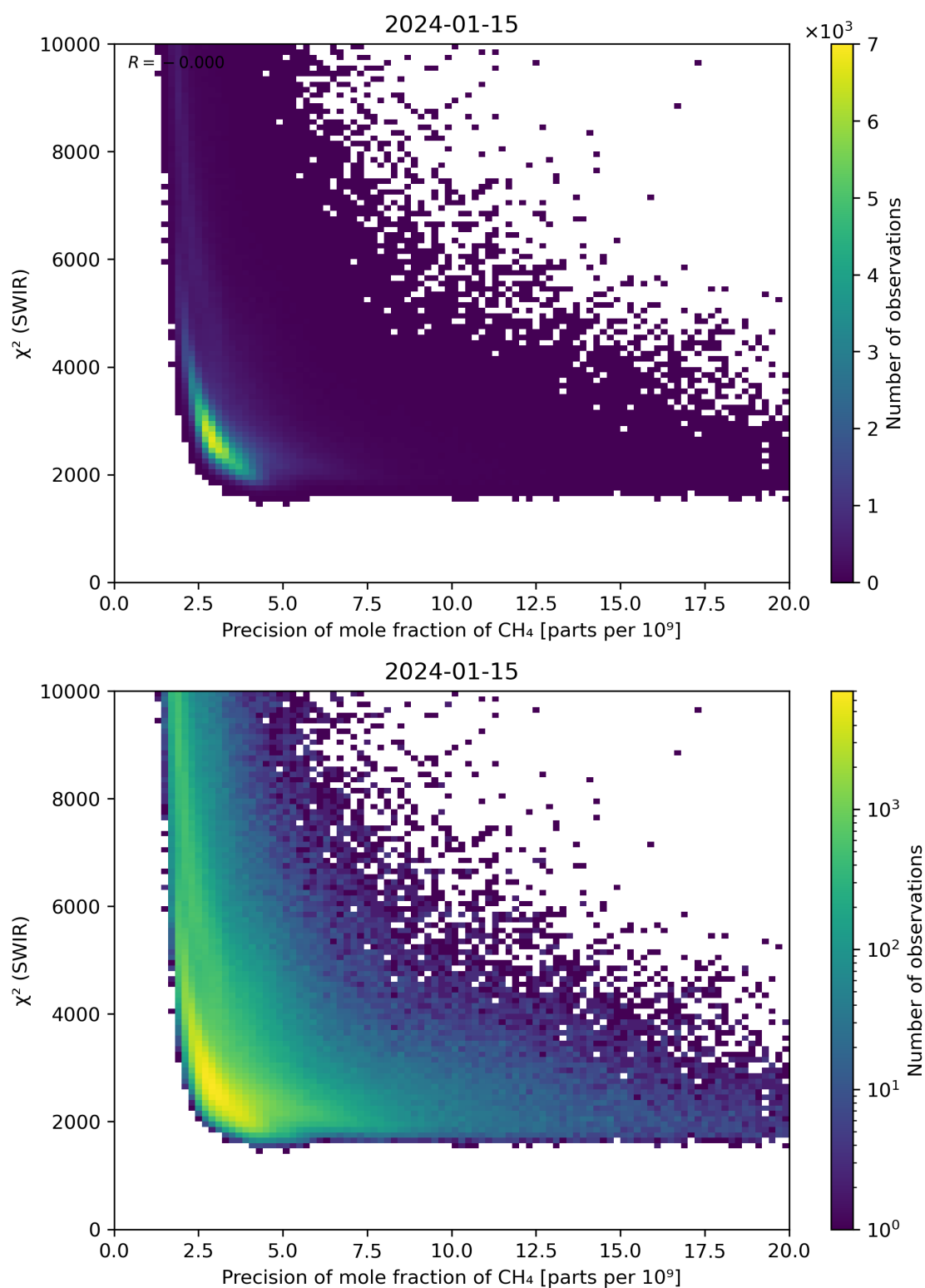
Figure 79: Scatter density plot of “Precision of mole fraction of \text{CH}_4 ” against “ \chi^2 (SWIR)” for 2024-01-15 to 2024-01-16.
