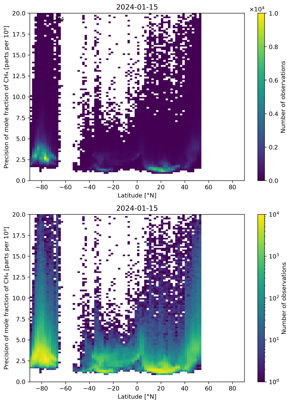
Figure 59: Scatter density plot of “Latitude” against “Precision of mole fraction of CH 4 ” for 2024-01-15 to 2024-01-16.
