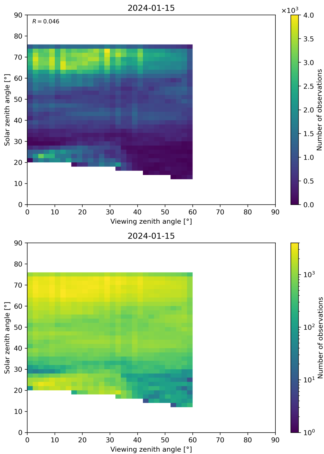
Figure 115: Scatter density plot of “Viewing zenith angle” against “Solar zenith angle” for 2024-01-15 to 2024-01-16.
