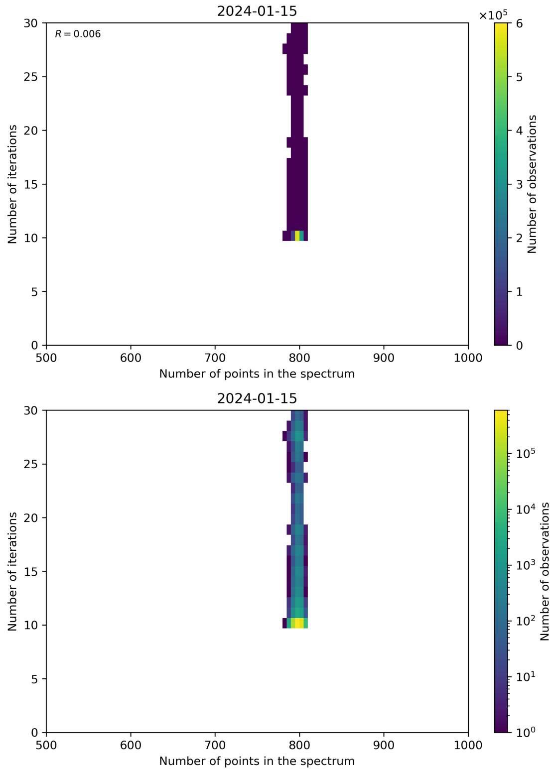
Figure 92: Scatter density plot of “Number of points in the spectrum” against “Number of iterations” for 2024-01-15 to 2024-01-16.
