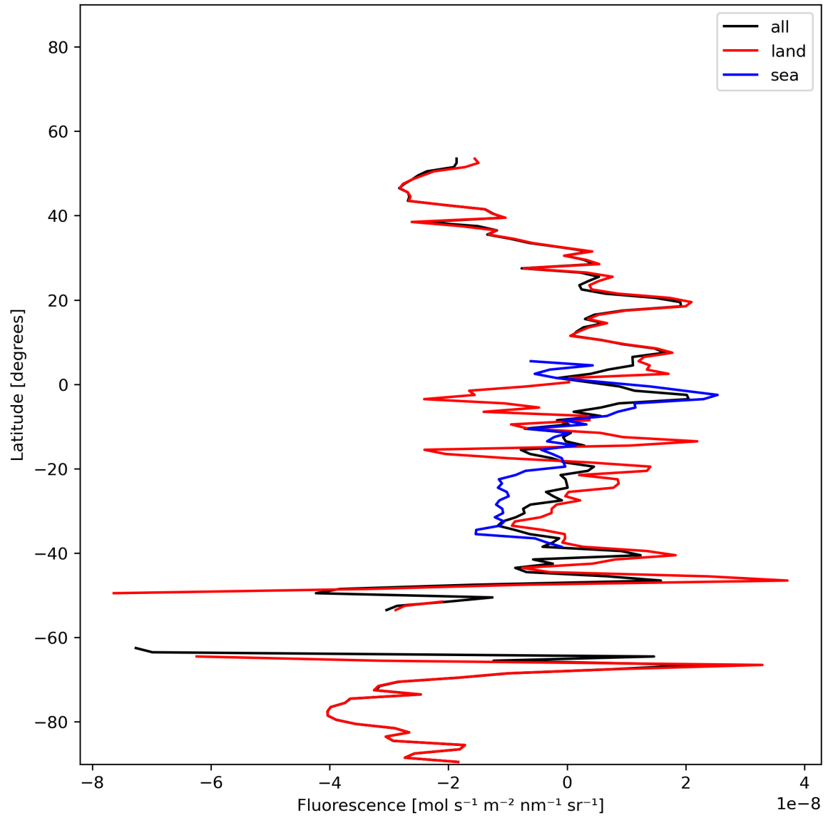
Figure 21: Zonal average of “Fluorescence” for 2024-01-15 to 2024-01-16.
