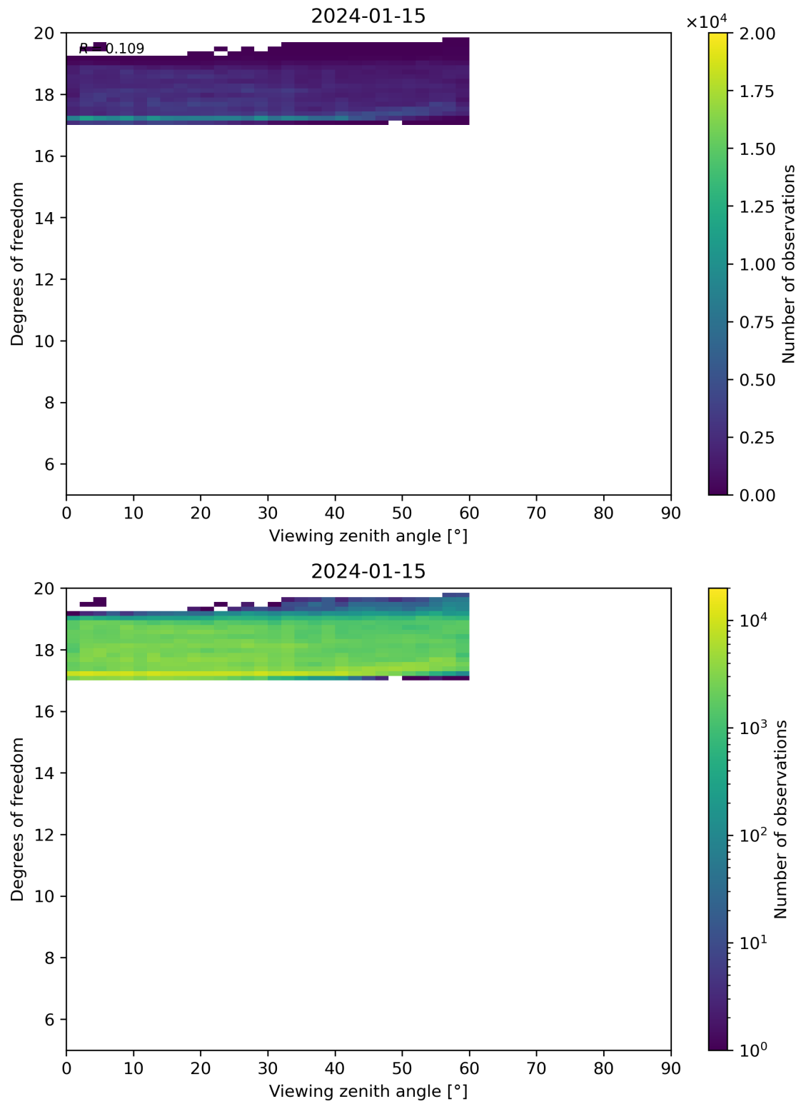
Figure 107: Scatter density plot of “Viewing zenith angle” against “Degrees of freedom” for 2024-01-15 to 2024-01-16.
