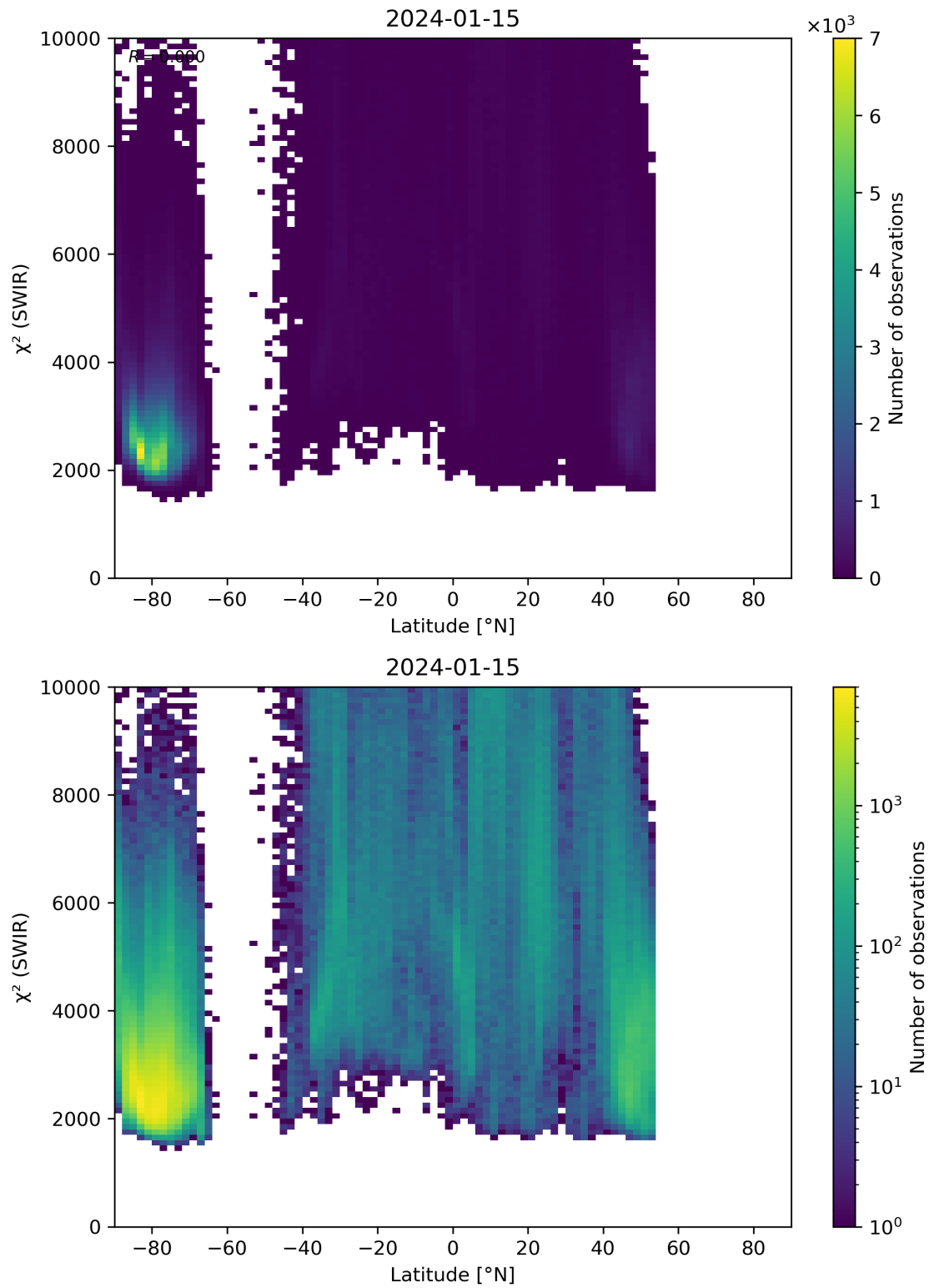
Figure 54: Scatter density plot of “Latitude” against “ \chi^2 (SWIR)” for 2024-01-15 to 2024-01-16.
