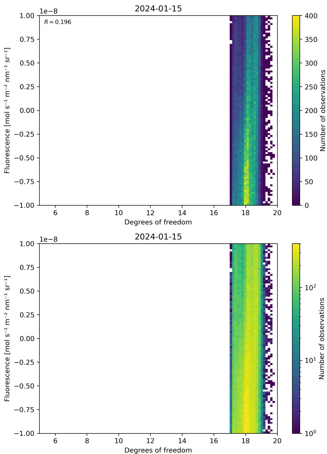
Figure 51: Scatter density plot of “Degrees of freedom” against “Fluorescence” for 2024-01-15 to 2024-01-16.
