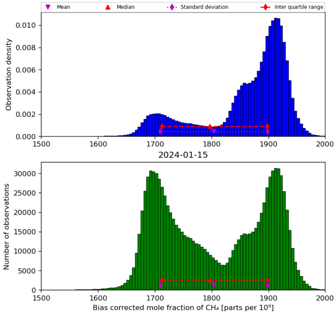
Figure 25: Histogram of “Bias corrected mole fraction of CH 4 ” for 2024-01-15 to 2024-01-16
