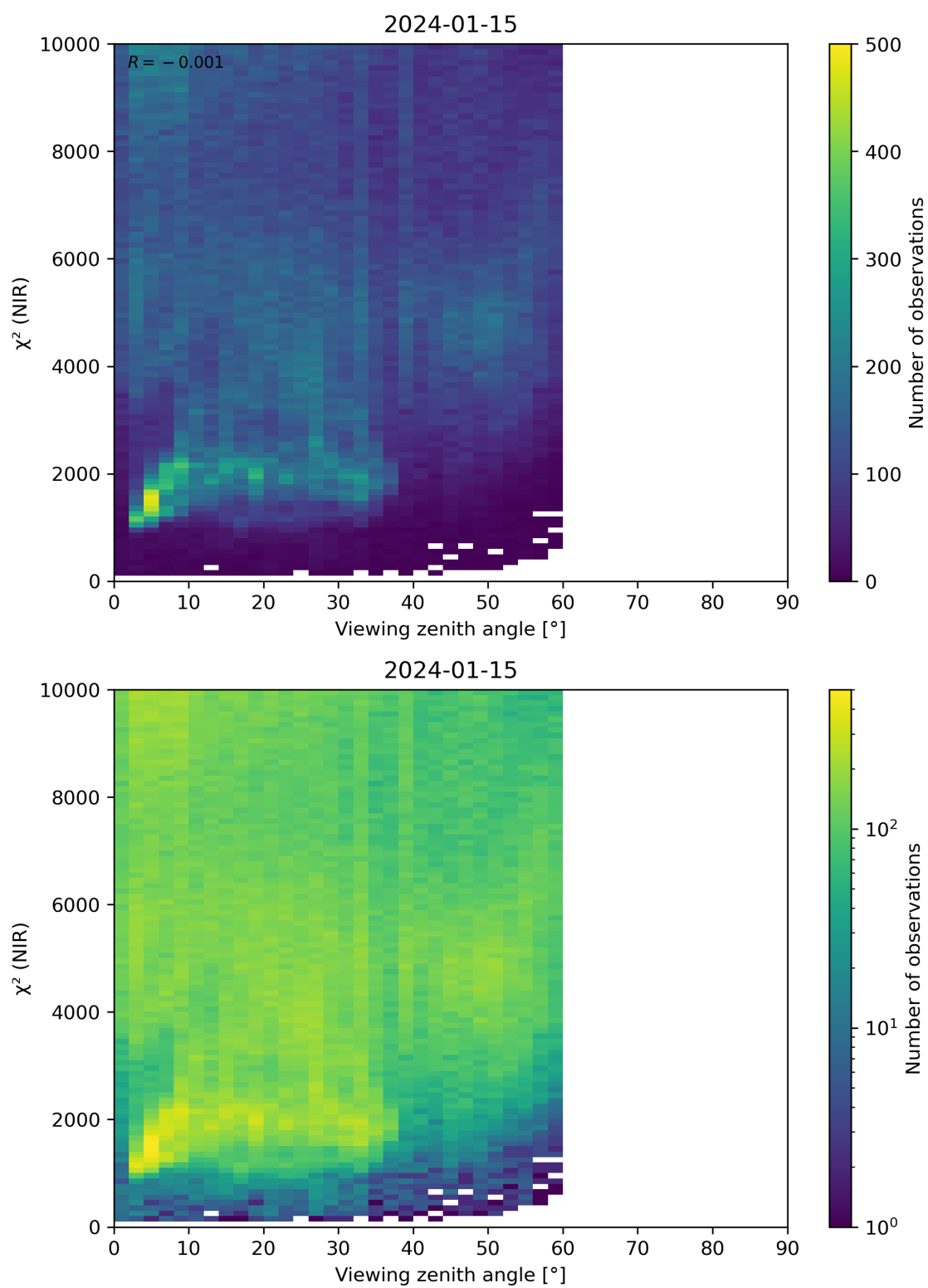
Figure 105: Scatter density plot of “Viewing zenith angle” against “ \chi^2 (NIR)” for 2024-01-15 to 2024-01-16.
