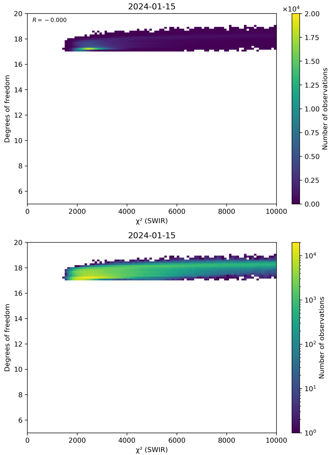
Figure 48: Scatter density plot of “ \chi^2 (SWIR)” against “Degrees of freedom” for 2024-01-15 to 2024-01-16.
