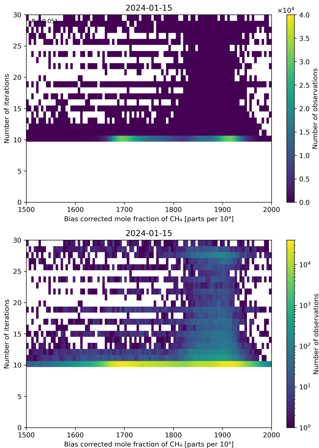
Figure 67: Scatter density plot of “Bias corrected mole fraction of CH 4 ” against “Number of iterations” for 2024-01-15 to 2024-01-16.
