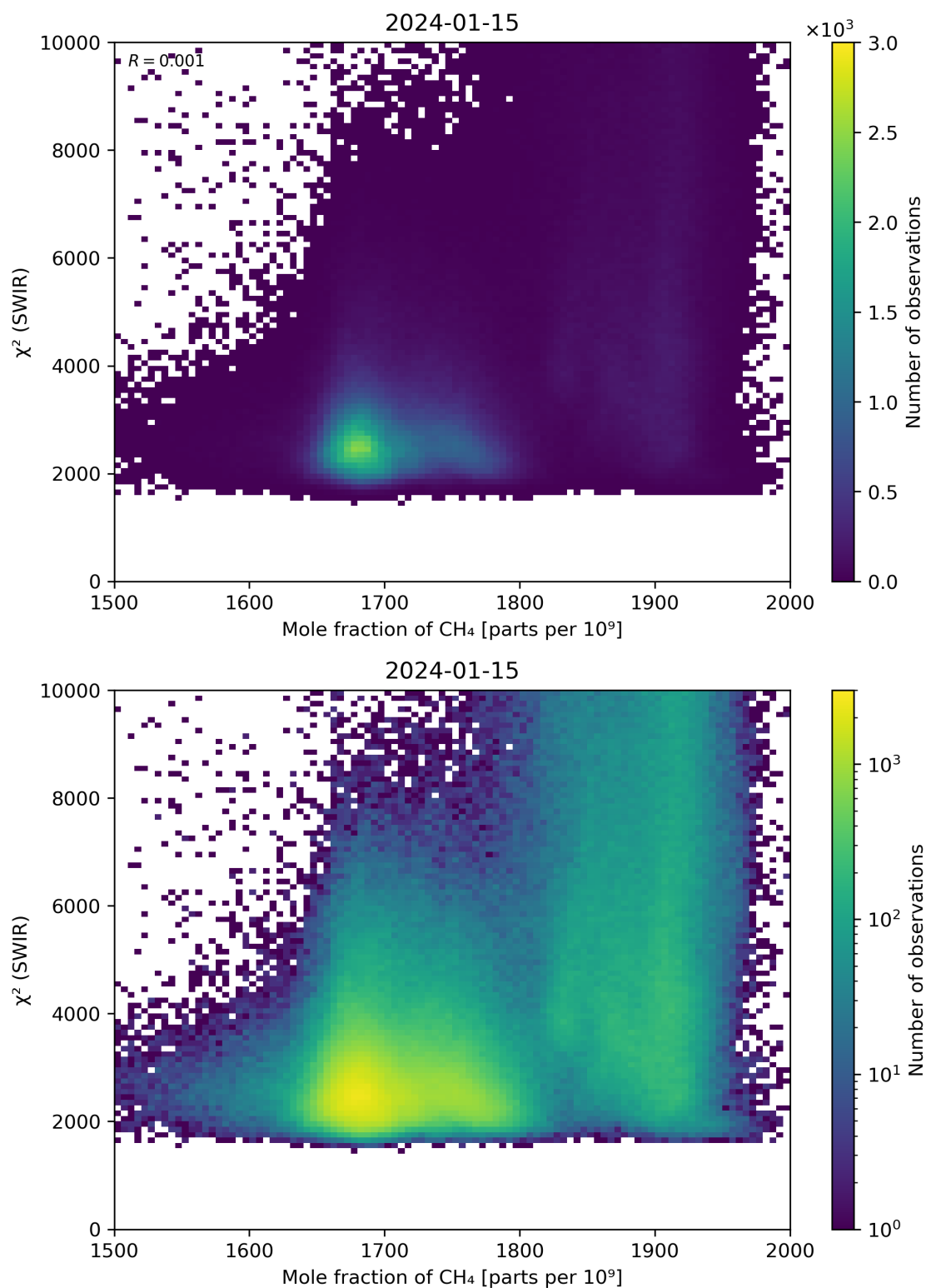
Figure 71: Scatter density plot of “Mole fraction of \text{CH}_4 ” against “ \chi^2 (SWIR)” for 2024-01-15 to 2024-01-16.
