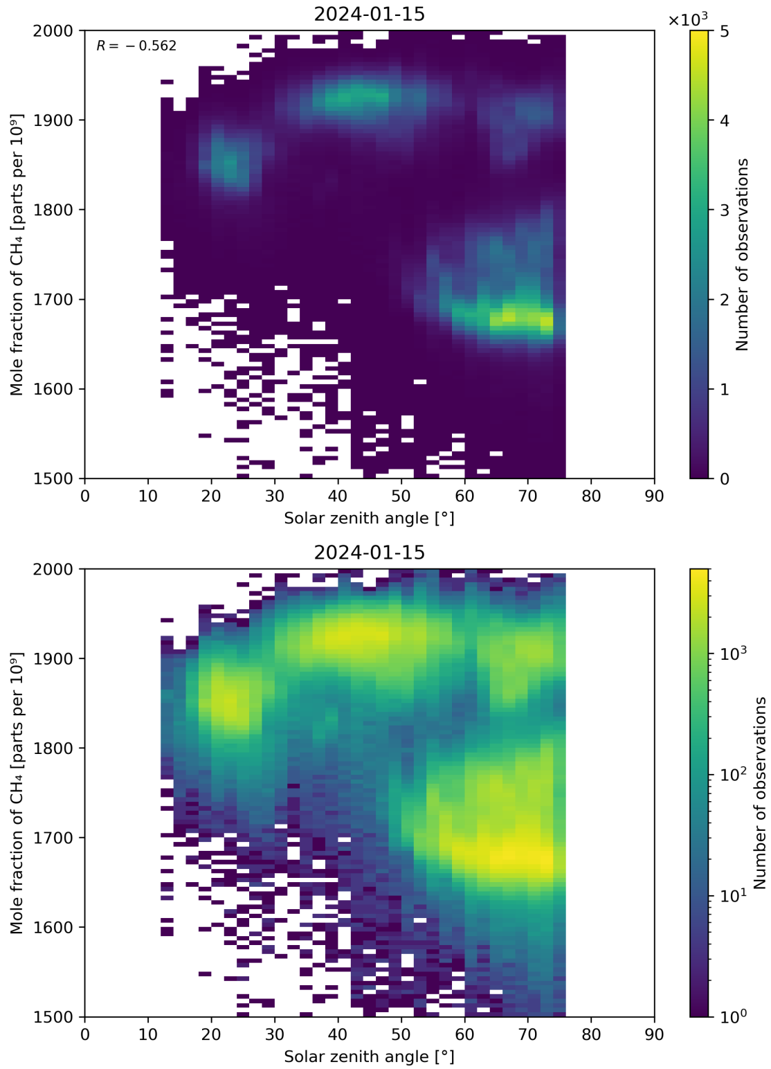
Figure 99: Scatter density plot of “Solar zenith angle” against “Mole fraction of CH 4 ” for 2024-01-15 to 2024-01-16.
