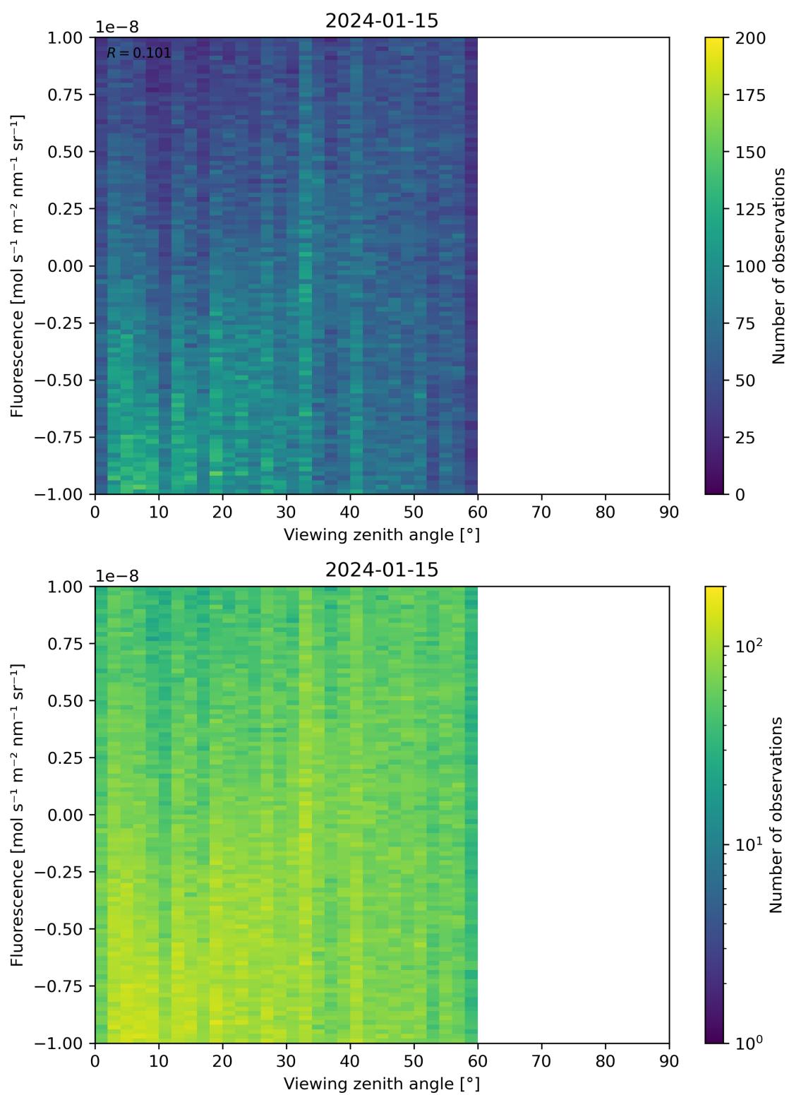
Figure 108: Scatter density plot of “Viewing zenith angle” against “Fluorescence” for 2024-01-15 to 2024-01-16.
