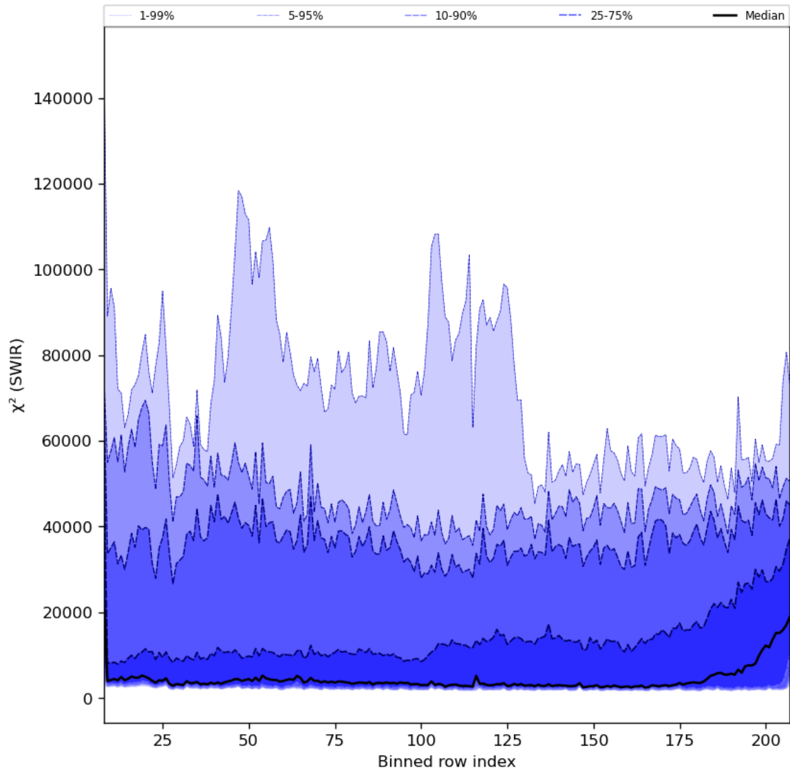
Figure 39: Along track statistics of " \chi^2 (SWIR)" for 2024-01-15 to 2024-01-16
