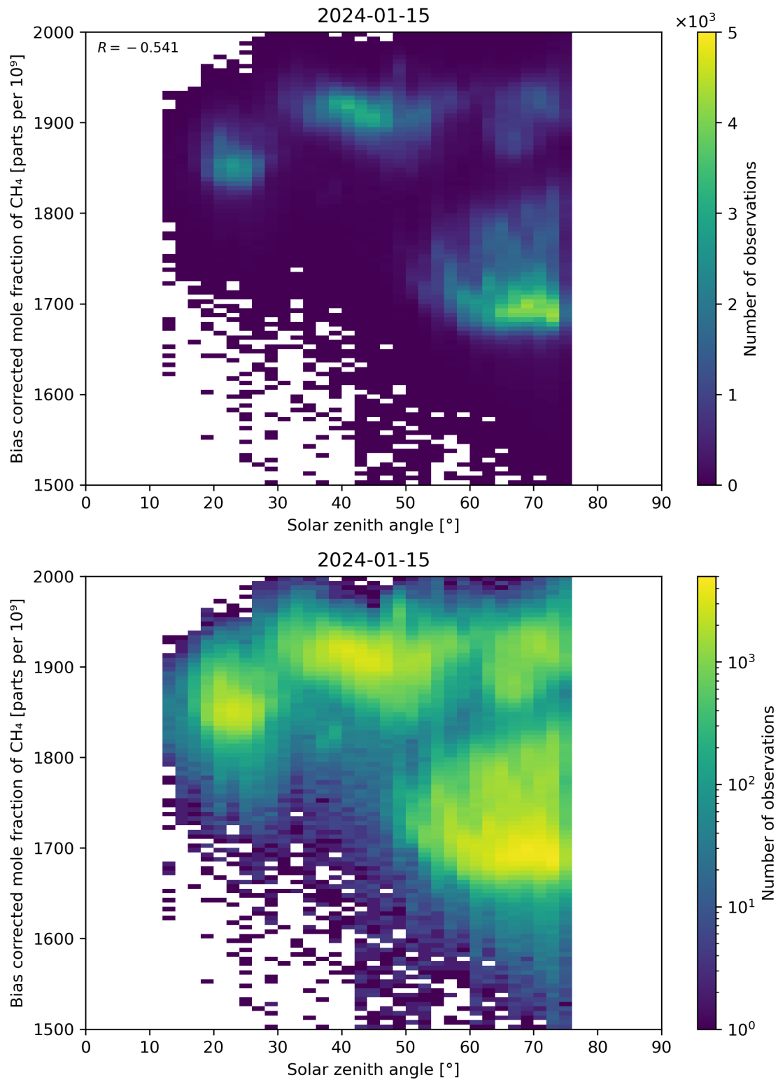
Figure 100: Scatter density plot of “Solar zenith angle” against “Bias corrected mole fraction of CH 4 ” for 2024-01-15 to 2024-01-16.
