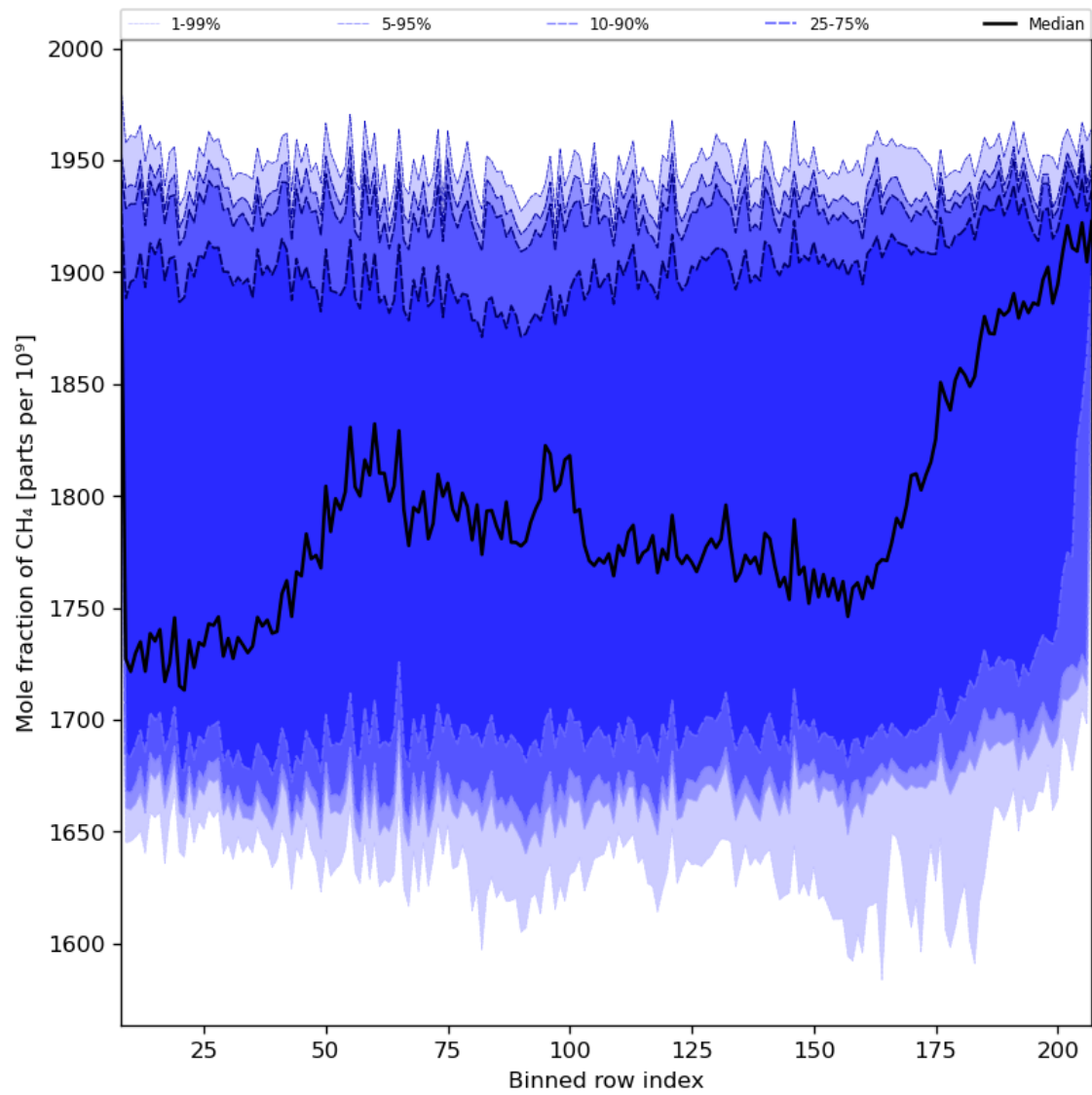
Figure 34: Along track statistics of “Mole fraction of CH 4 ” for 2024-01-15 to 2024-01-16
