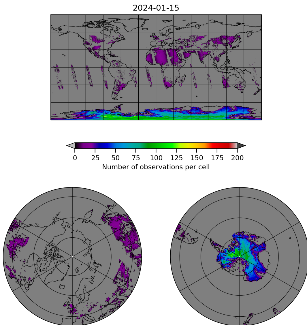
Figure 10: Map of the number of observations for 2024-01-15 to 2024-01-16
