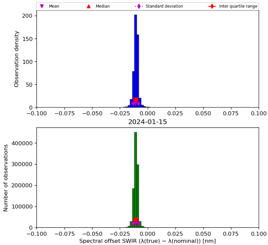
Figure 27: Histogram of “Spectral offset SWIR ( \lambda(\text{true}) - \lambda(\text{nominal}) )” for 2024-01-15 to 2024-01-16
