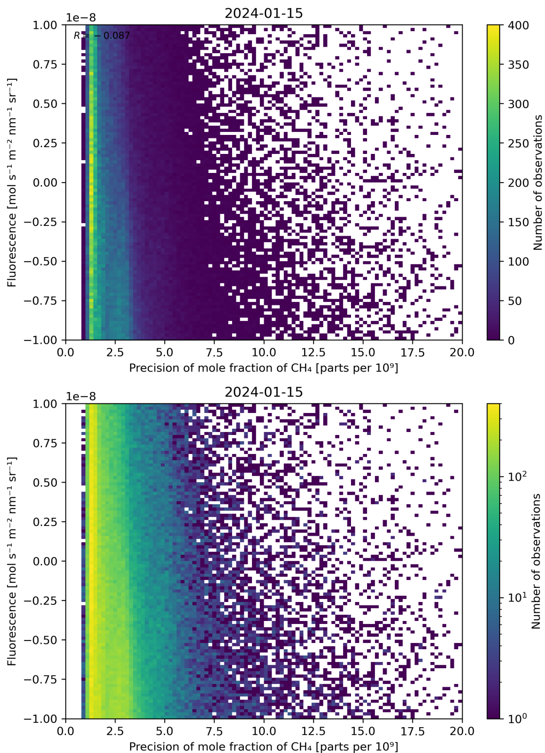
Figure 81: Scatter density plot of “Precision of mole fraction of CH 4 ” against “Fluorescence” for 2024-01-15 to 2024-01-16.
