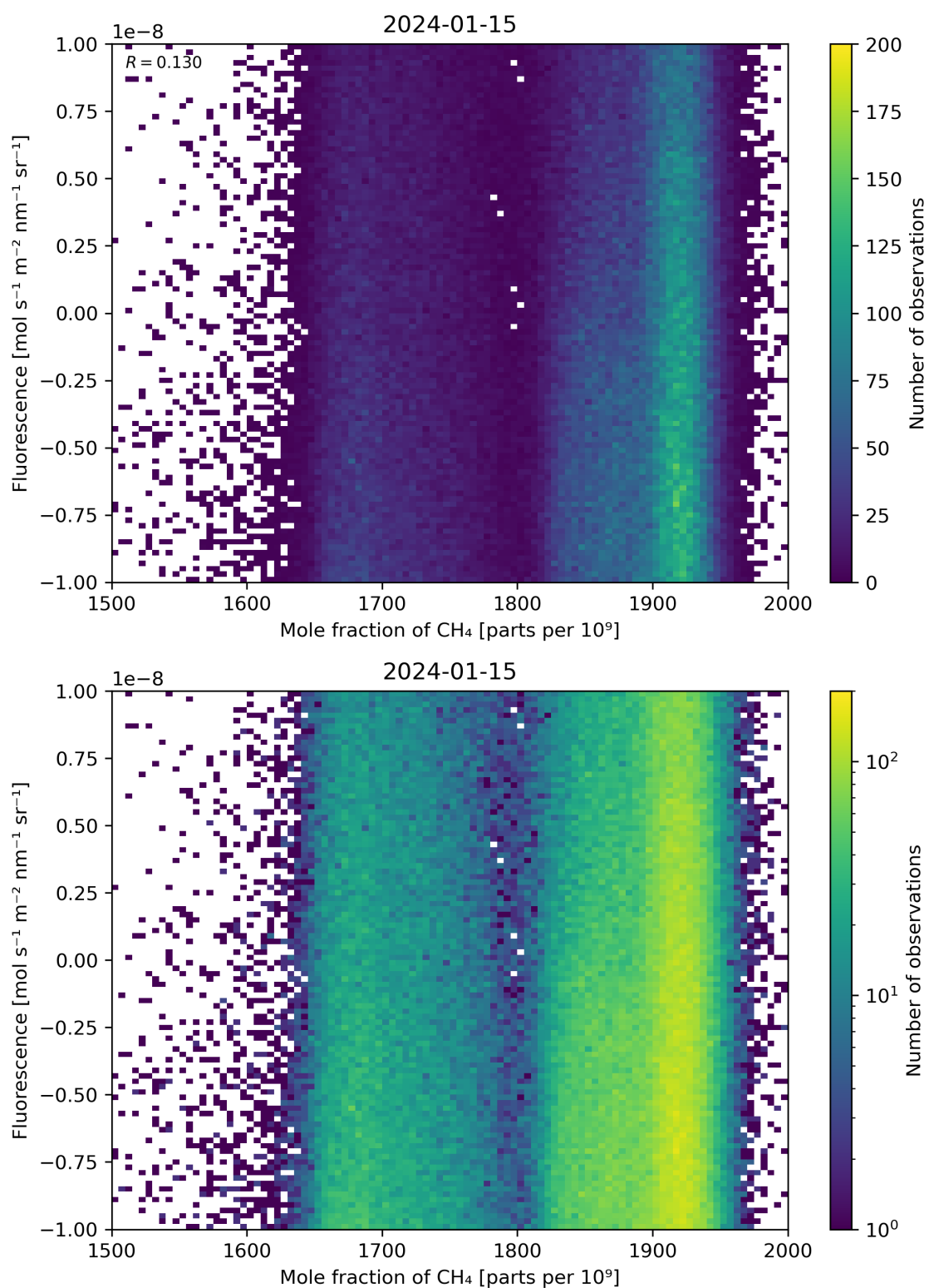
Figure 73: Scatter density plot of “Mole fraction of \text{CH}_4 ” against “Fluorescence” for 2024-01-15 to 2024-01-16.
