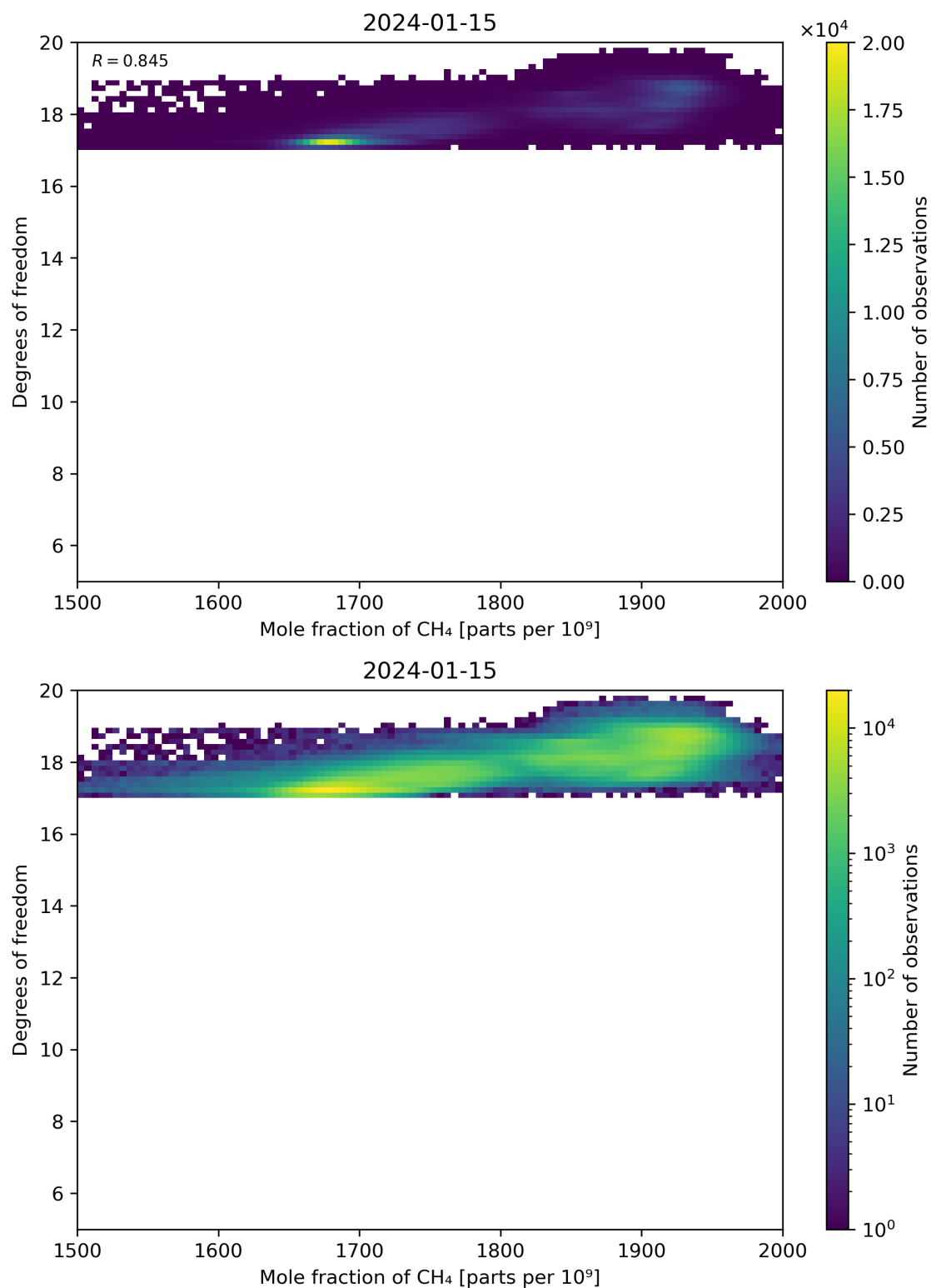
Figure 72: Scatter density plot of “Mole fraction of CH 4 ” against “Degrees of freedom” for 2024-01-15 to 2024-01-16.
