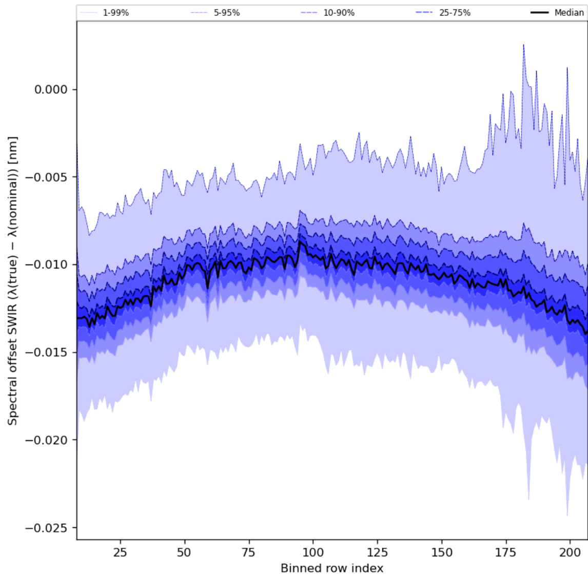
Figure 38: Along track statistics of “Spectral offset SWIR ( \lambda(\text{true}) - \lambda(\text{nominal}) )” for 2024-01-15 to 2024-01-16
