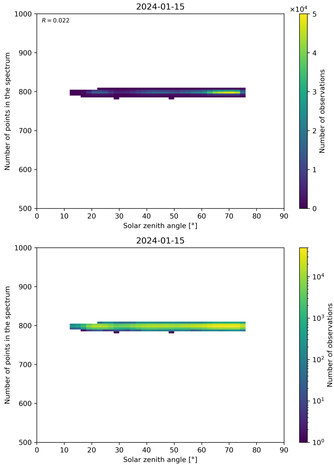
Figure 103: Scatter density plot of “Solar zenith angle” against “Number of points in the spectrum” for 2024-01-15 to 2024-01-16.
