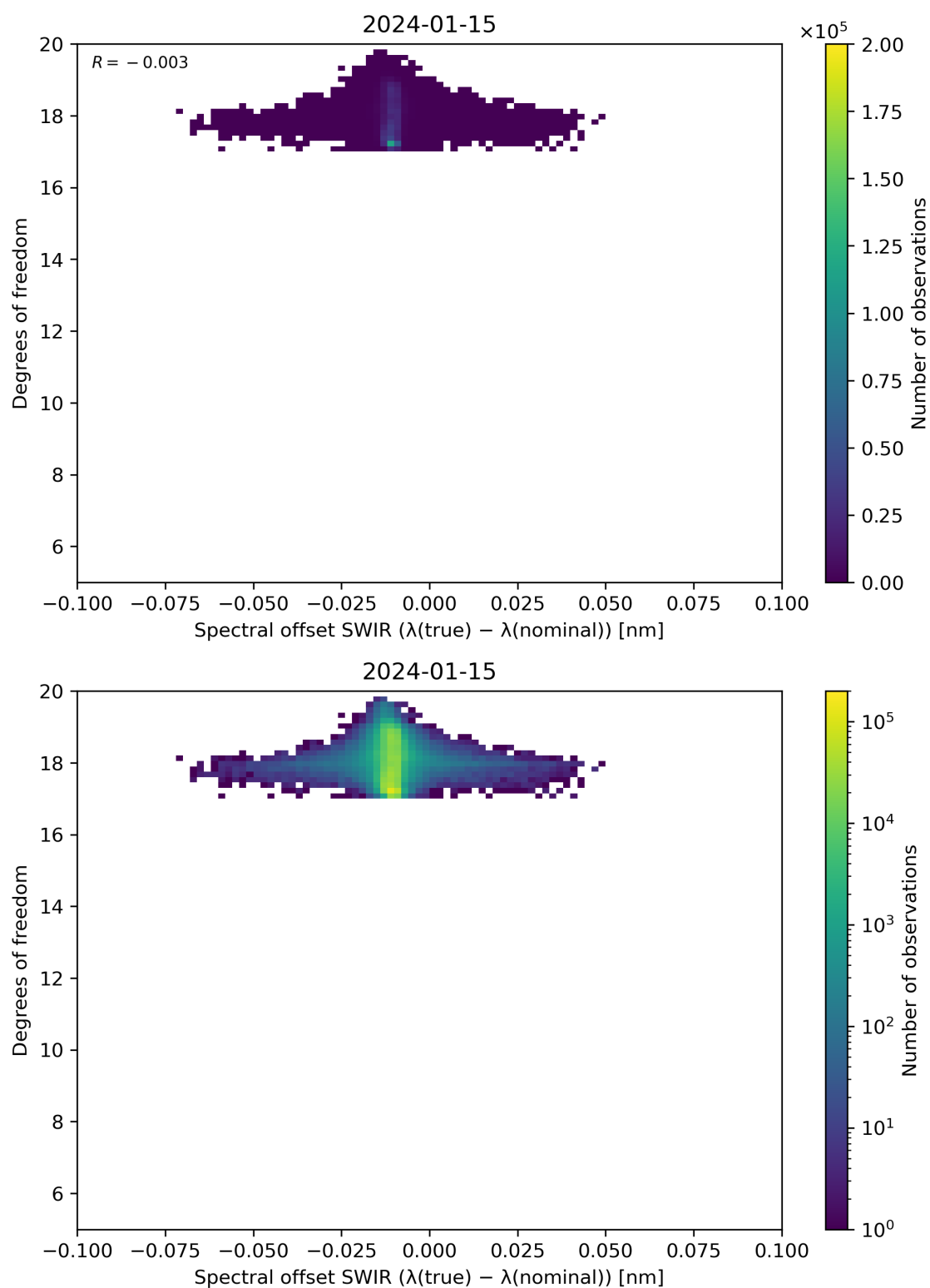
Figure 119: Scatter density plot of “Spectral offset SWIR ( \lambda(\text{true}) - \lambda(\text{nominal}) )” against “Degrees of freedom” for 2024-01-15 to 2024-01-16.
