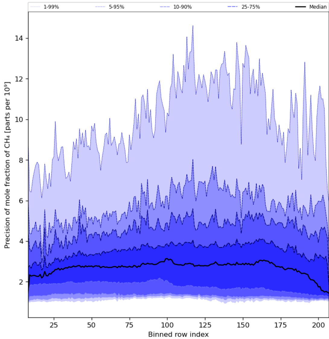
Figure 35: Along track statistics of “Precision of mole fraction of CH 4 ” for 2024-01-15 to 2024-01-16
