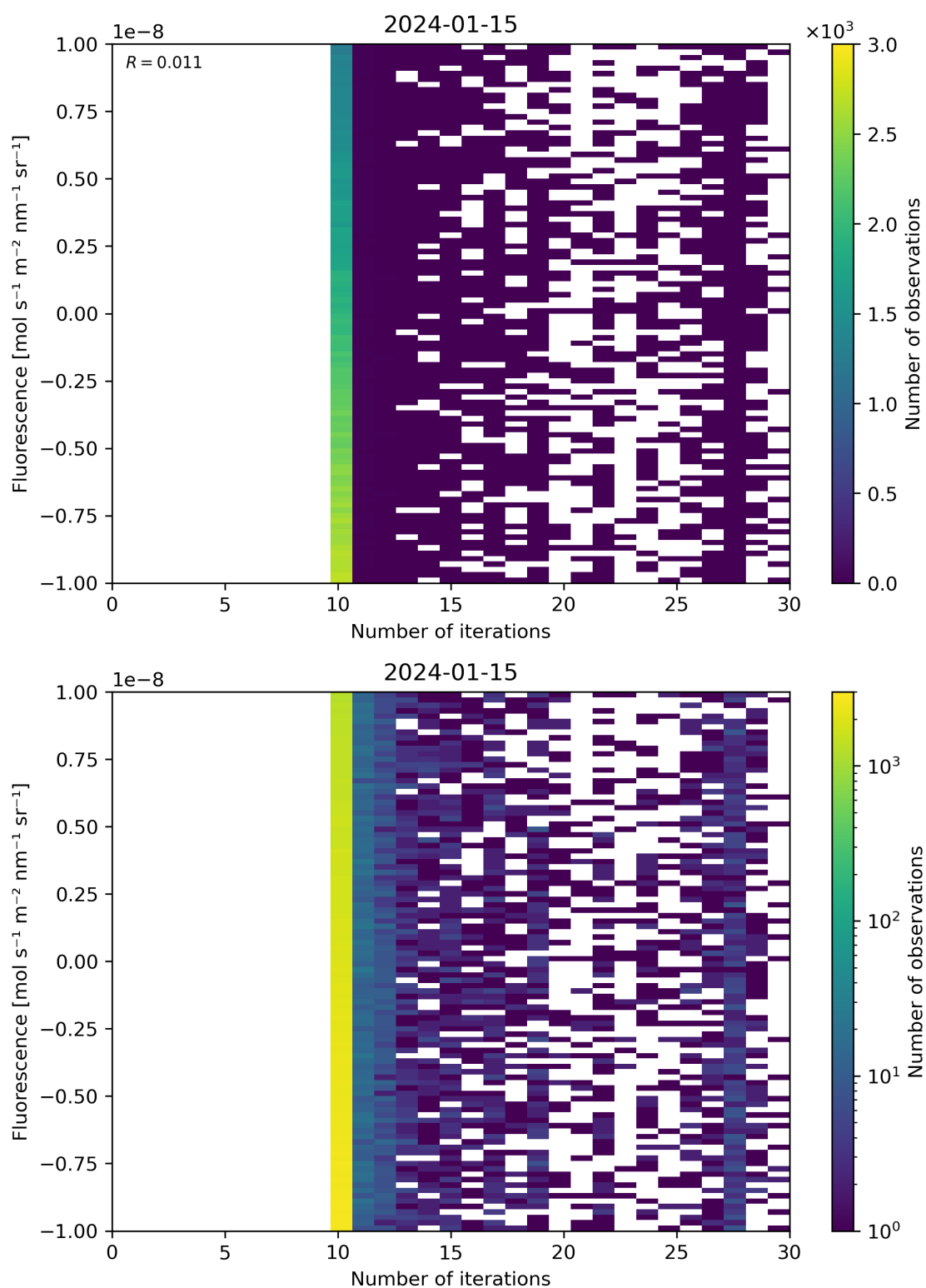
Figure 87: Scatter density plot of “Number of iterations” against “Fluorescence” for 2024-01-15 to 2024-01-16.
