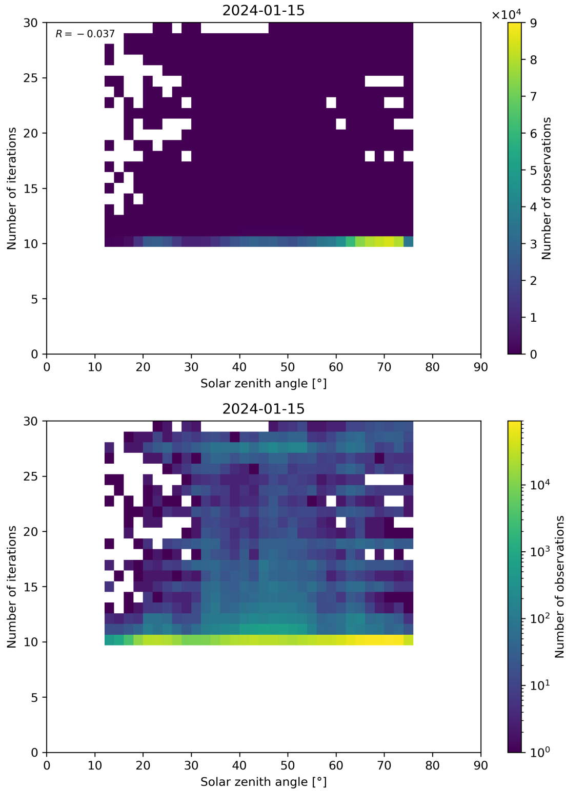
Figure 102: Scatter density plot of “Solar zenith angle” against “Number of iterations” for 2024-01-15 to 2024-01-16.
