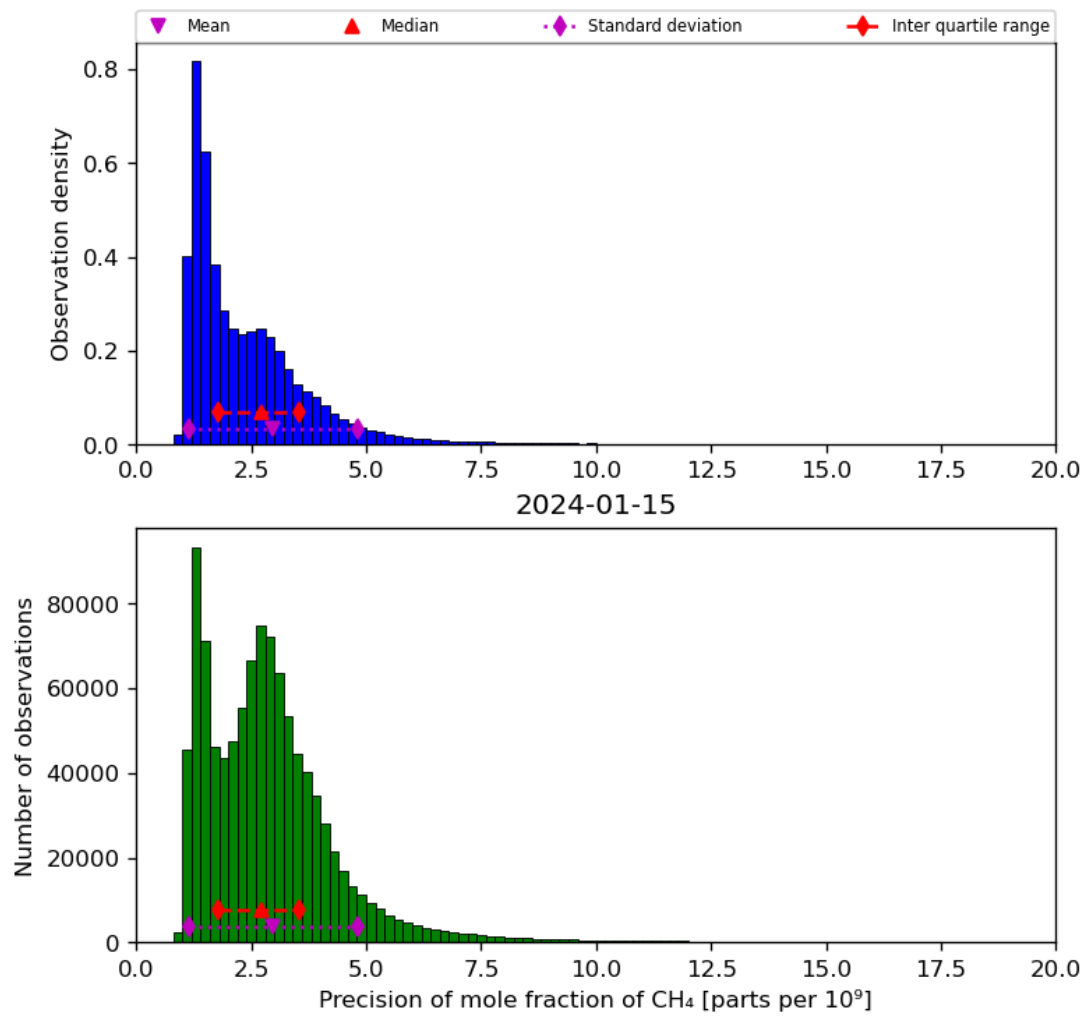
Figure 24: Histogram of “Precision of mole fraction of CH 4 ” for 2024-01-15 to 2024-01-16
