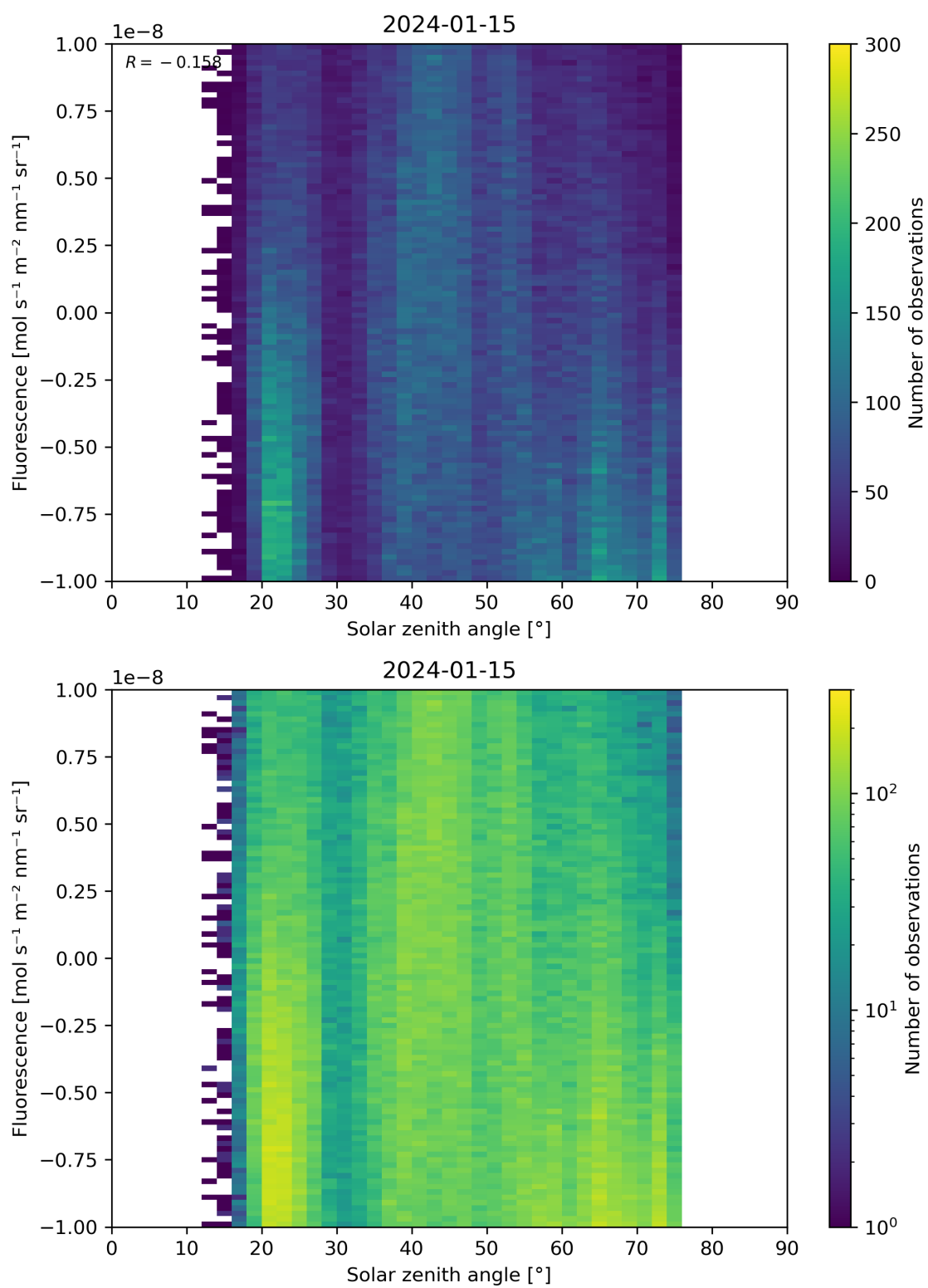
Figure 97: Scatter density plot of “Solar zenith angle” against “Fluorescence” for 2024-01-15 to 2024-01-16.
