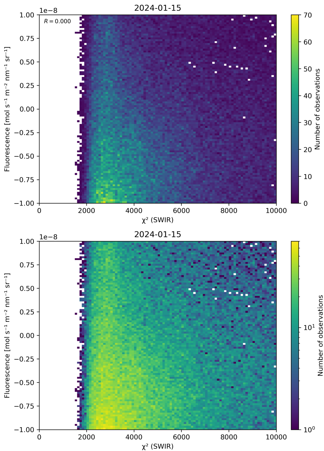
Figure 49: Scatter density plot of “ \chi^2 (SWIR)” against “Fluorescence” for 2024-01-15 to 2024-01-16.
