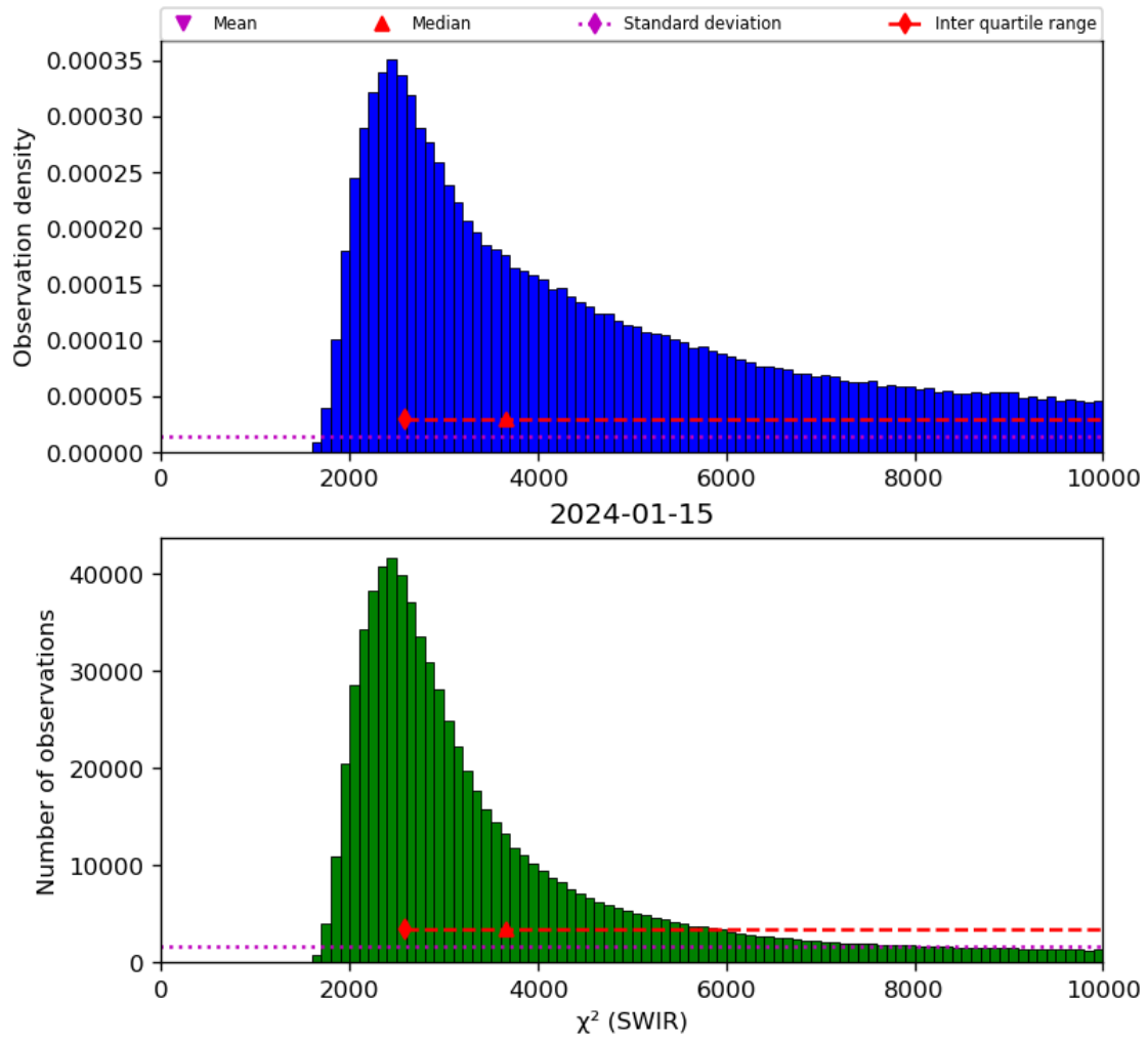
Figure 28: Histogram of “ \chi^2 (SWIR)” for 2024-01-15 to 2024-01-16
