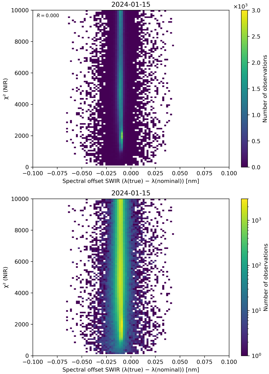
Figure 117: Scatter density plot of “Spectral offset SWIR ( \lambda(\text{true}) - \lambda(\text{nominal}) )” against “ \chi^2 (NIR)” for 2024-01-15 to 2024-01-16.
