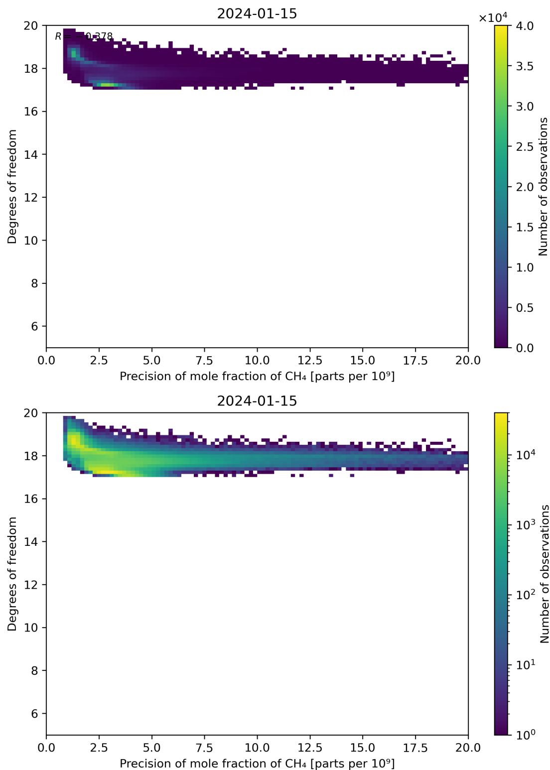
Figure 80: Scatter density plot of “Precision of mole fraction of CH 4 ” against “Degrees of freedom” for 2024-01-15 to 2024-01-16.
