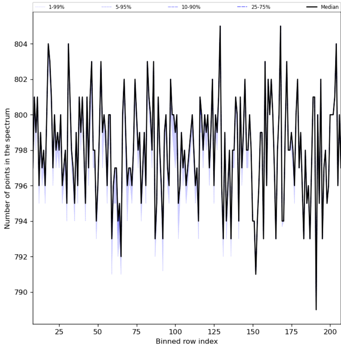
Figure 37: Along track statistics of “Number of points in the spectrum” for 2024-01-15 to 2024-01-16
