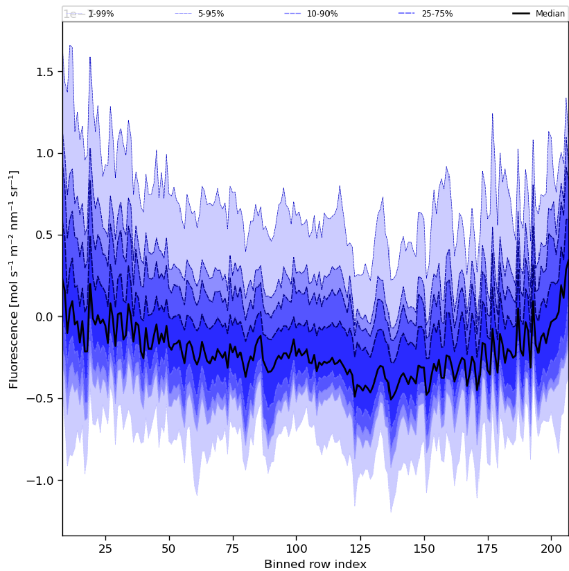
Figure 43: Along track statistics of “Fluorescence” for 2024-01-15 to 2024-01-16
