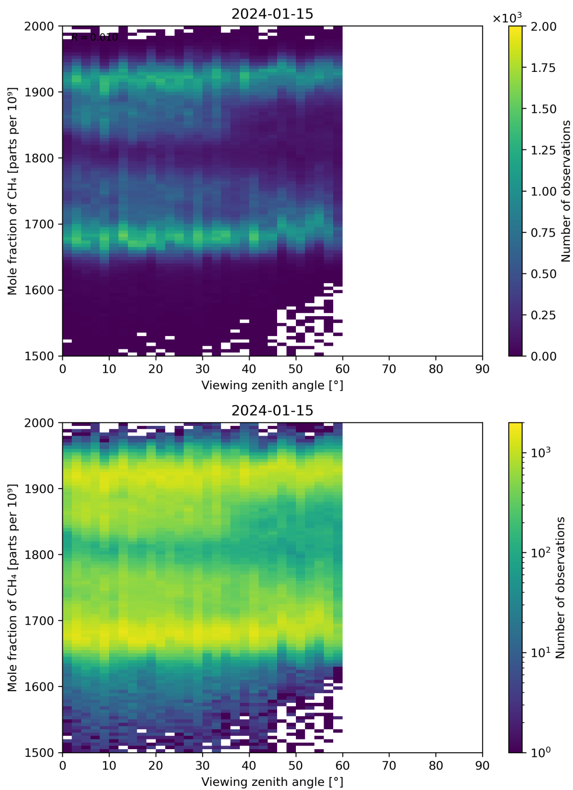
Figure 110: Scatter density plot of “Viewing zenith angle” against “Mole fraction of CH 4 ” for 2024-01-15 to 2024-01-16.
