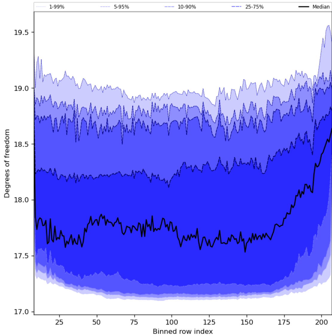
Figure 41: Along track statistics of “Degrees of freedom” for 2024-01-15 to 2024-01-16
