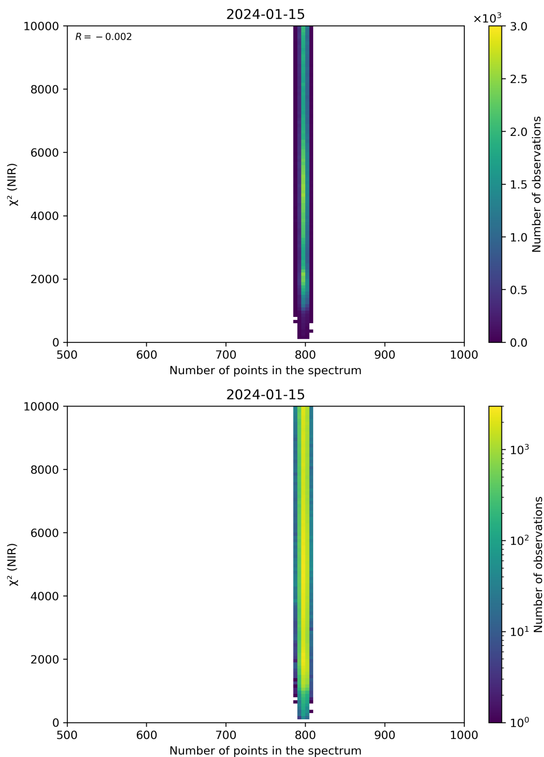
Figure 88: Scatter density plot of “Number of points in the spectrum” against “ \chi^2 (NIR)” for 2024-01-15 to 2024-01-16.
