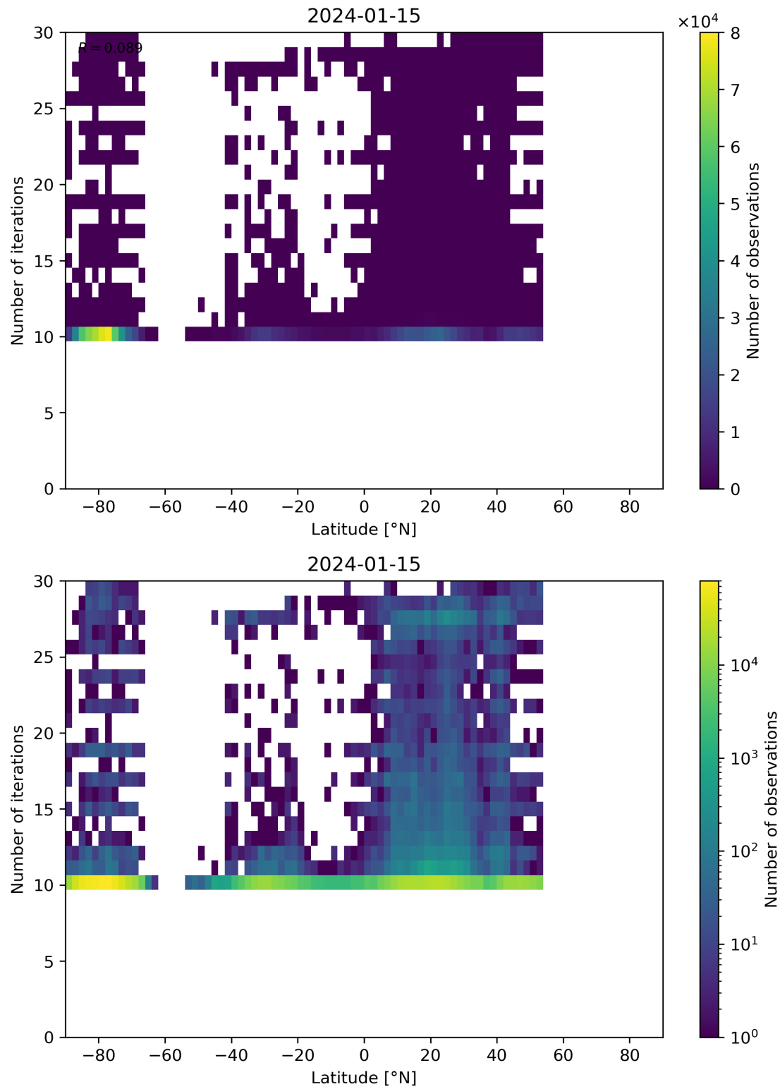
Figure 60: Scatter density plot of “Latitude” against “Number of iterations” for 2024-01-15 to 2024-01-16.
