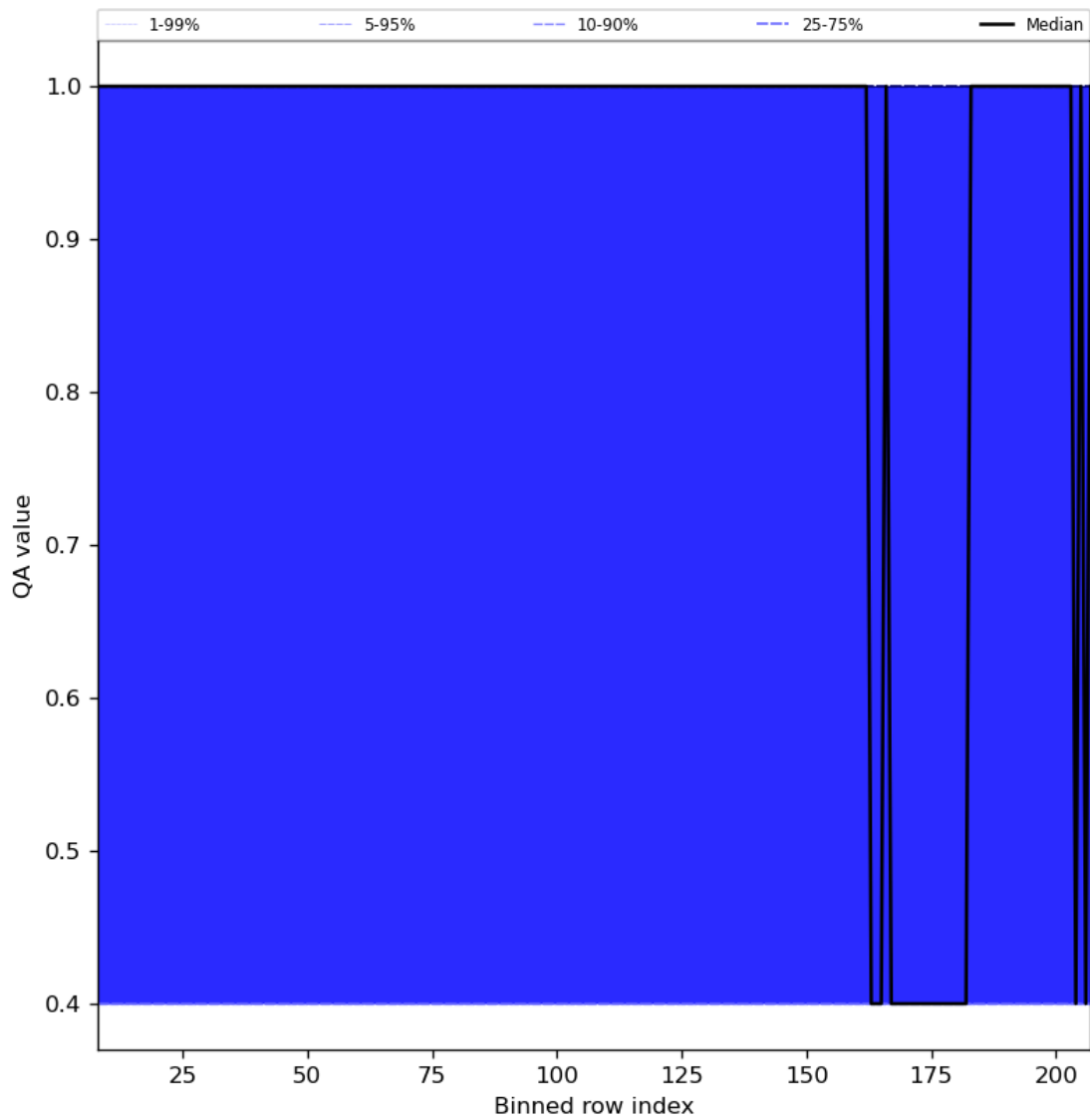
Figure 33: Along track statistics of “QA value” for 2024-01-15 to 2024-01-16
