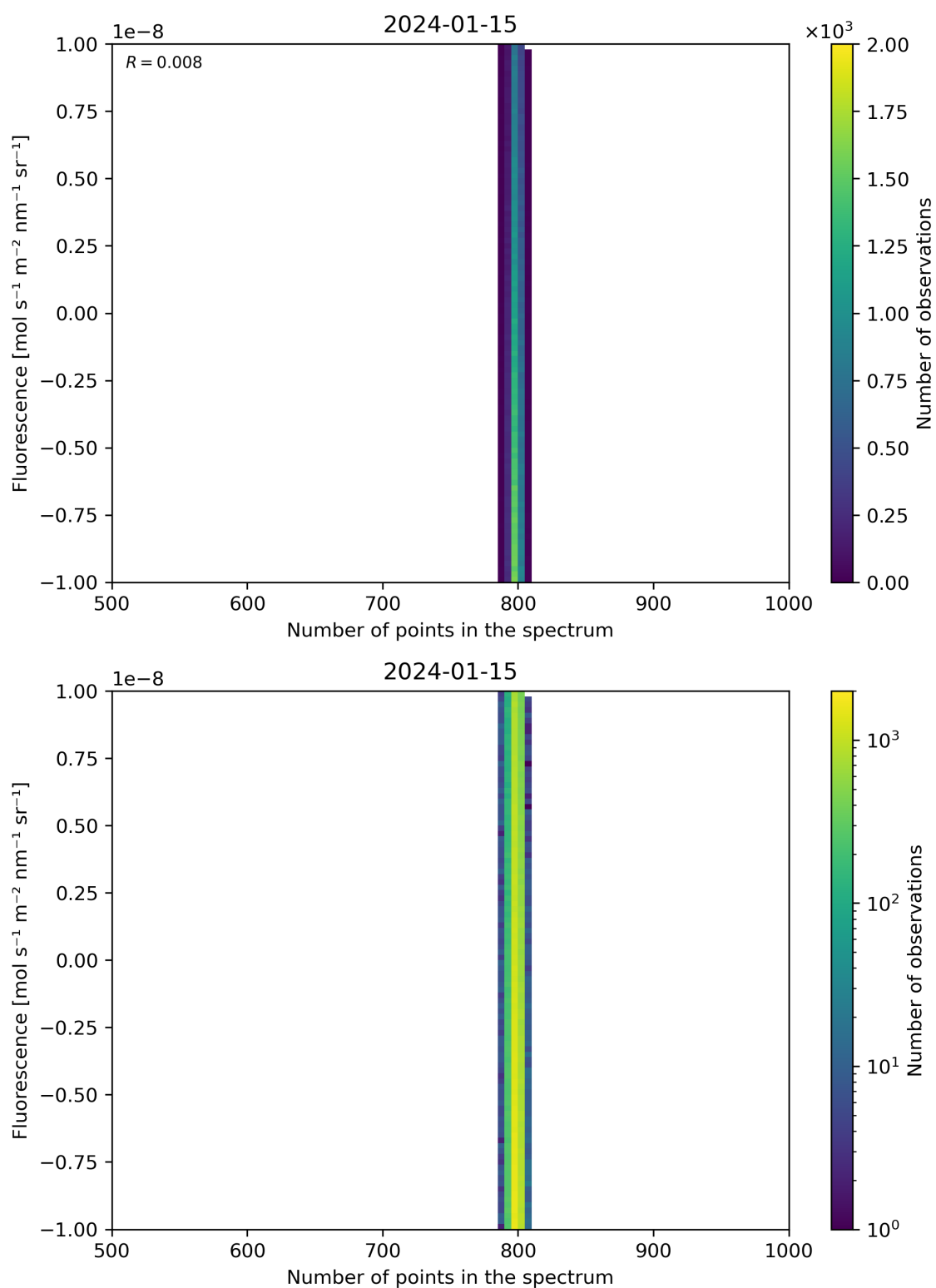
Figure 91: Scatter density plot of “Number of points in the spectrum” against “Fluorescence” for 2024-01-15 to 2024-01-16.
