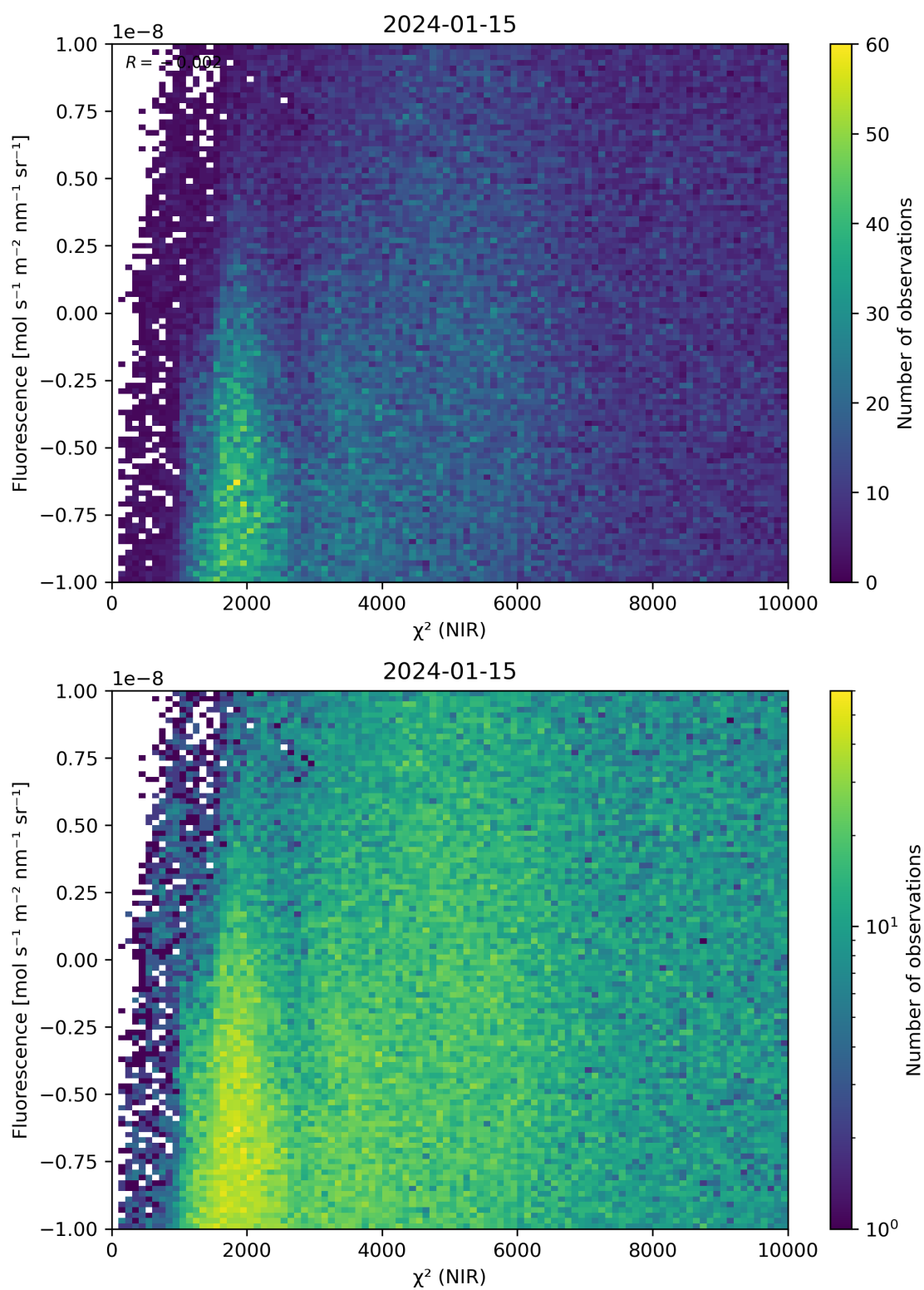
Figure 45: Scatter density plot of “ \chi^2 (NIR)” against “Fluorescence” for 2024-01-15 to 2024-01-16.
