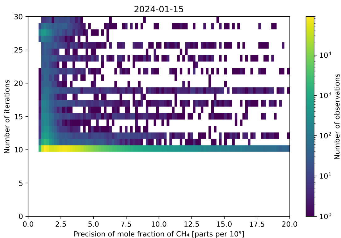
Figure 83: Scatter density plot of “Precision of mole fraction of CH 4 ” against “Number of iterations” for 2024-01-15 to 2024-01-16.
