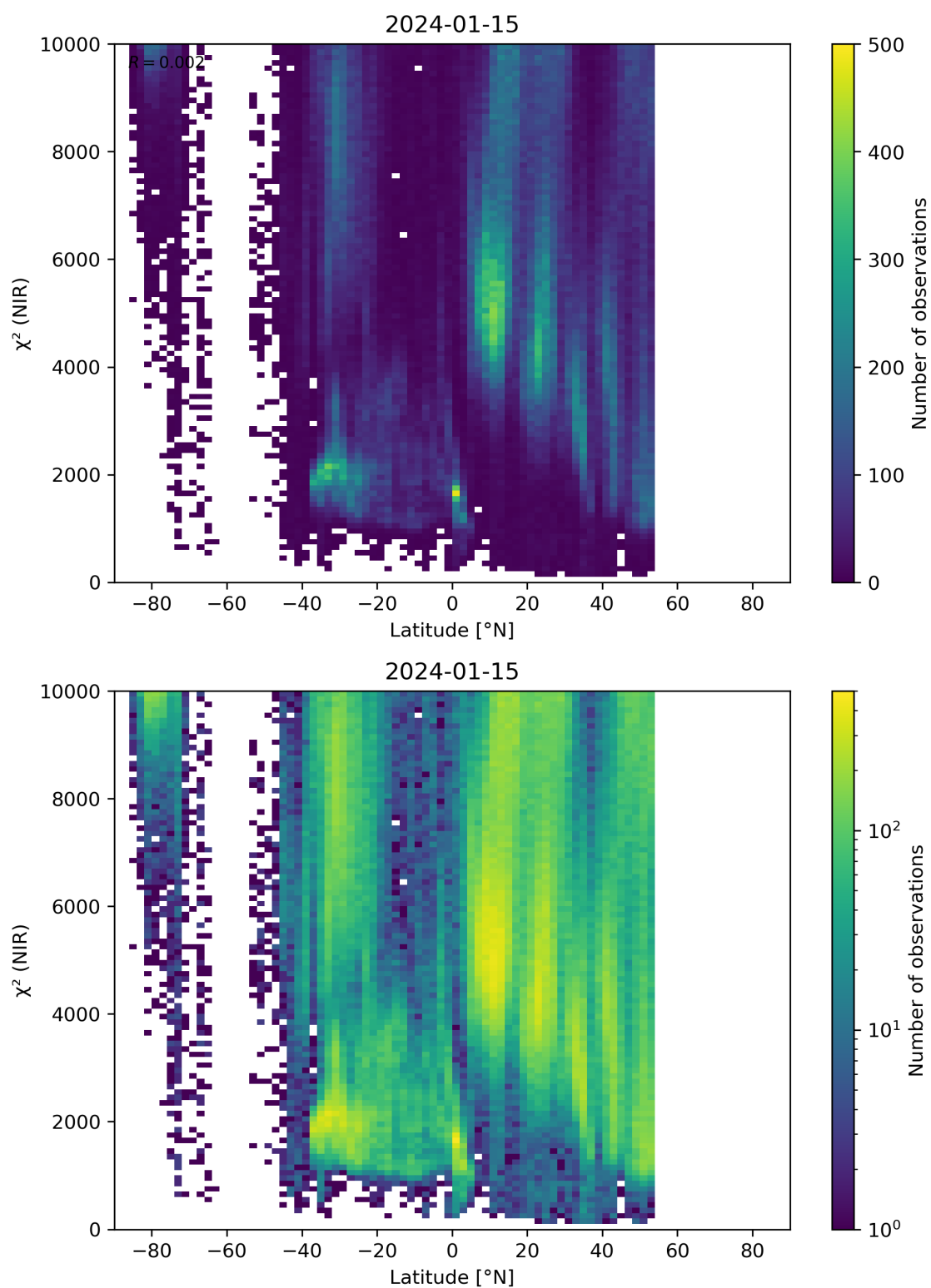
Figure 53: Scatter density plot of “Latitude” against “ \chi^2 (NIR)” for 2024-01-15 to 2024-01-16.
