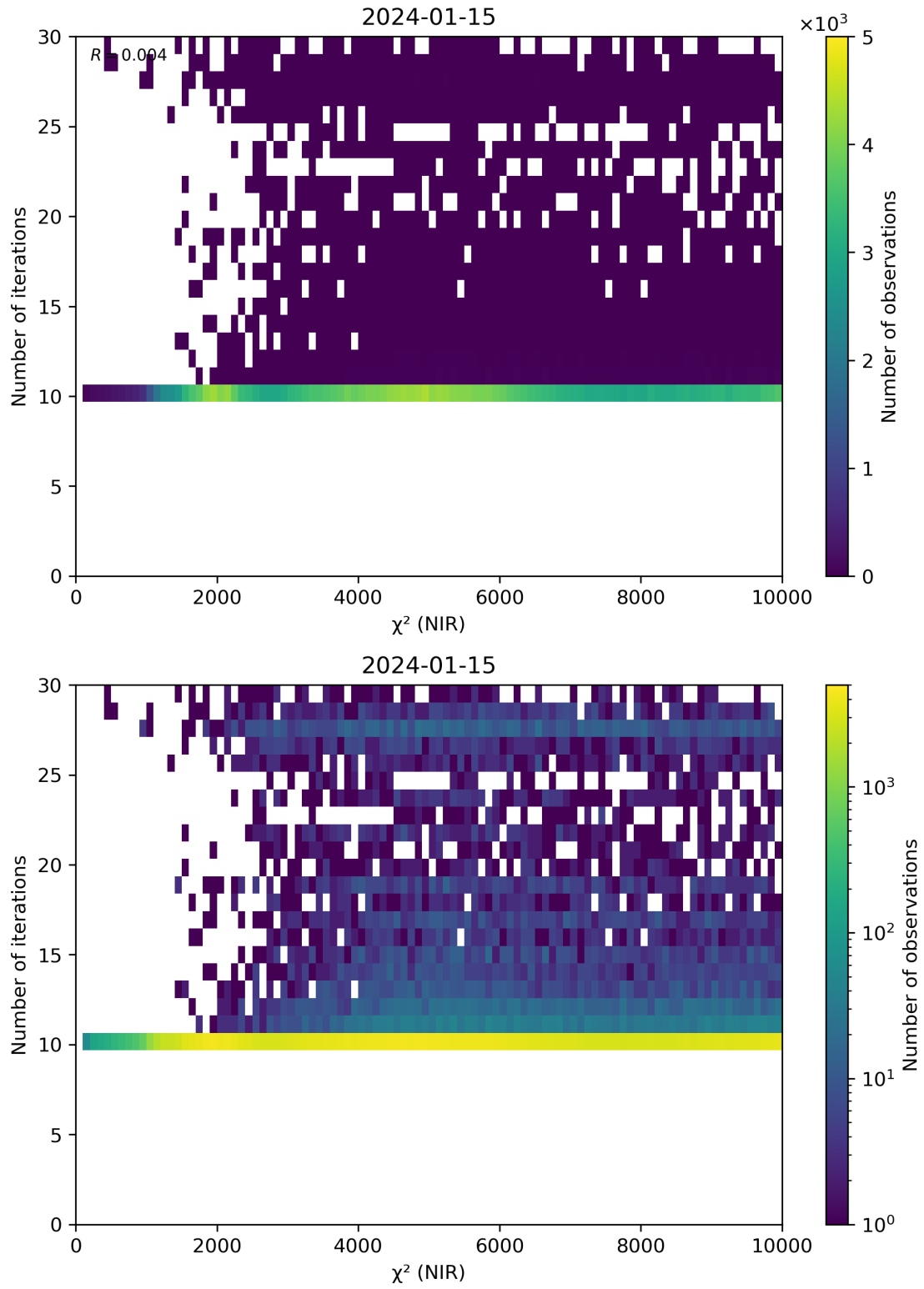
Figure 46: Scatter density plot of “ \chi^2 (NIR)” against “Number of iterations” for 2024-01-15 to 2024-01-16.
