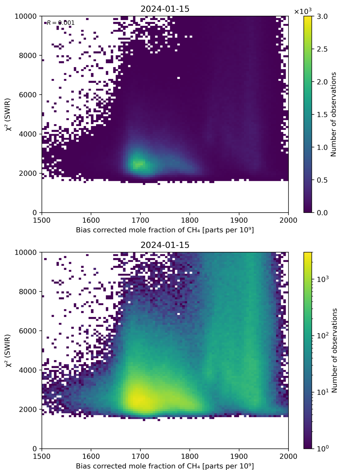
Figure 64: Scatter density plot of “Bias corrected mole fraction of CH 4 ” against “ \chi^2 (SWIR)” for 2024-01-15 to 2024-01-16.
