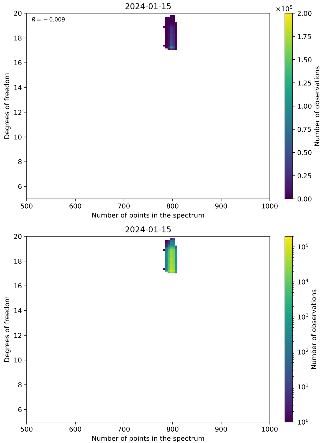
Figure 90: Scatter density plot of “Number of points in the spectrum” against “Degrees of freedom” for 2024-01-15 to 2024-01-16.
