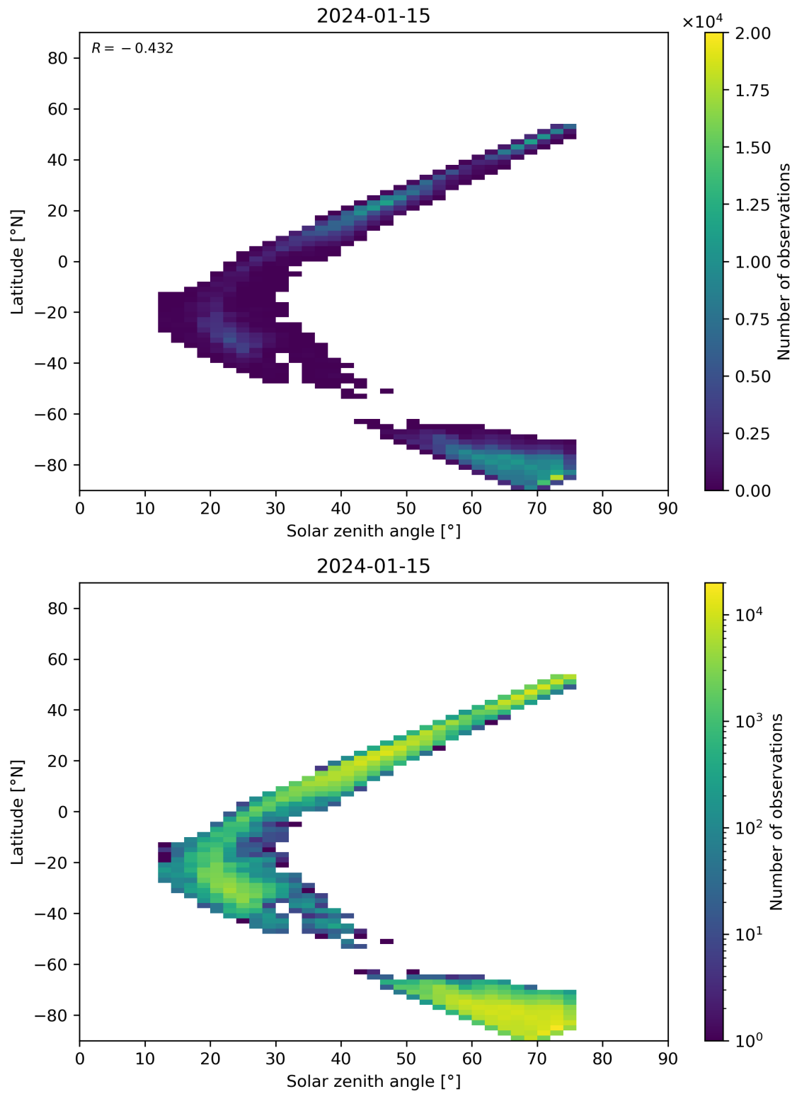
Figure 98: Scatter density plot of “Solar zenith angle” against “Latitude” for 2024-01-15 to 2024-01-16.
