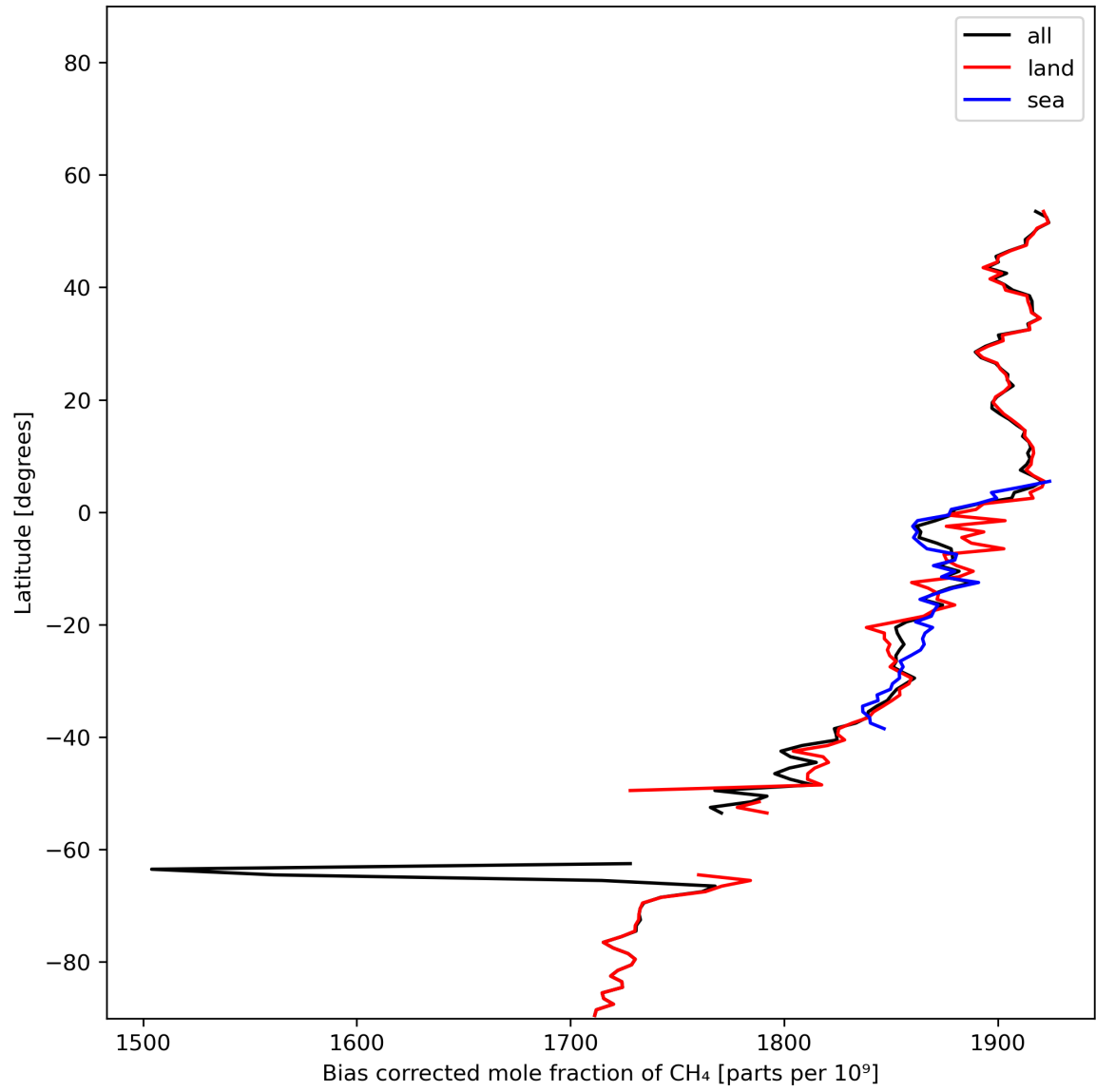
Figure 14: Zonal average of “Bias corrected mole fraction of CH 4 ” for 2024-01-15 to 2024-01-16.
