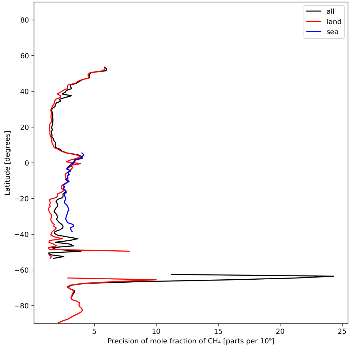
Figure 13: Zonal average of “Precision of mole fraction of CH 4 ” for 2024-01-15 to 2024-01-16.
