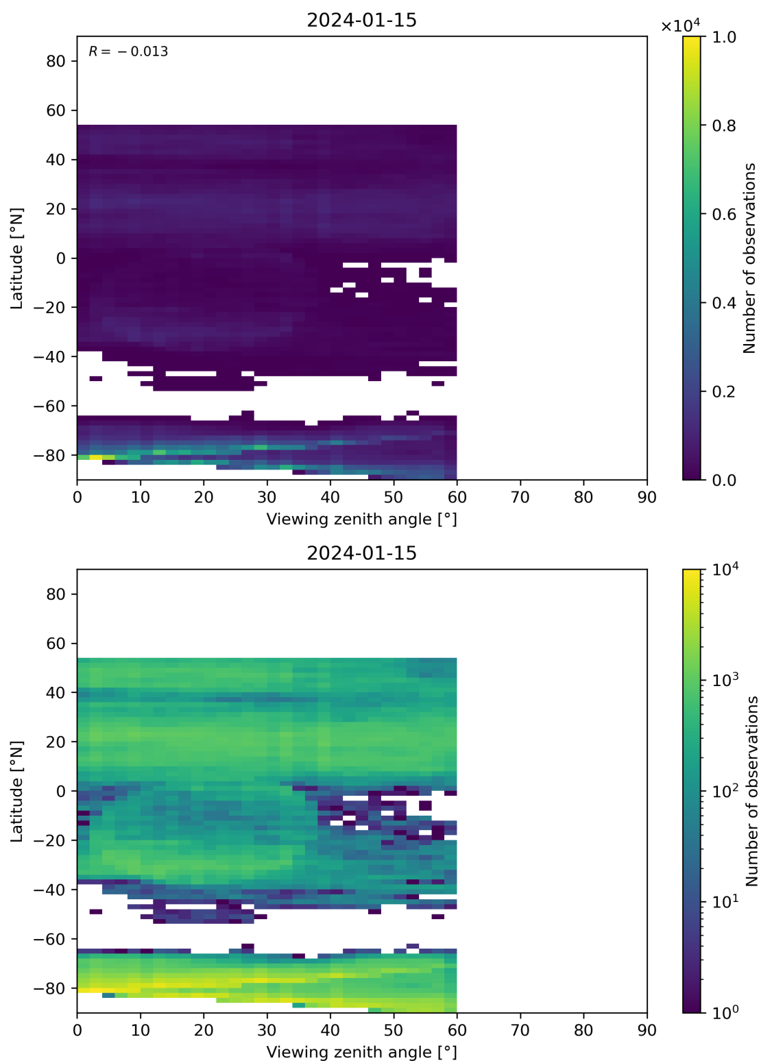
Figure 109: Scatter density plot of “Viewing zenith angle” against “Latitude” for 2024-01-15 to 2024-01-16.
