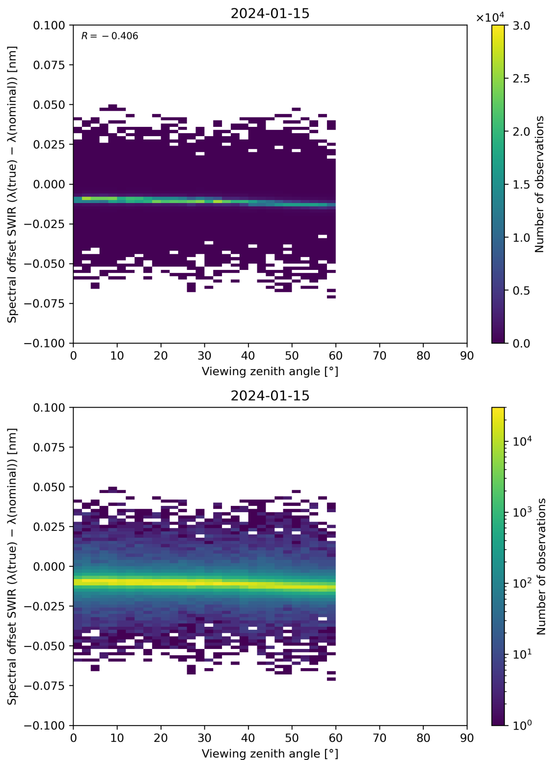
Figure 116: Scatter density plot of “Viewing zenith angle” against “Spectral offset SWIR ( \lambda(\text{true}) - \lambda(\text{nominal}) )” for 2024-01-15 to 2024-01-16.
