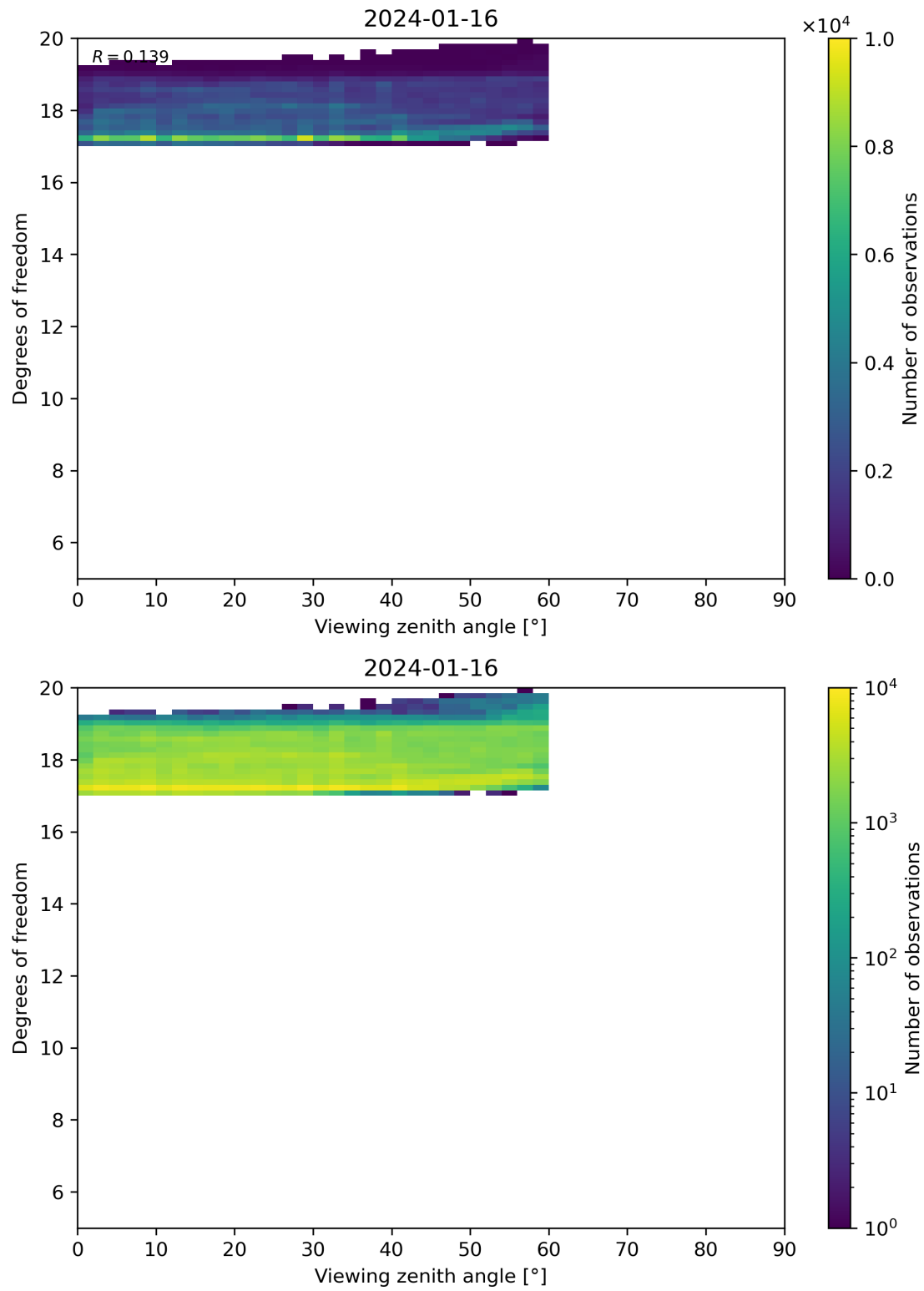
Figure 107: Scatter density plot of “Viewing zenith angle” against “Degrees of freedom” for 2024-01-15 to 2024-01-17.
