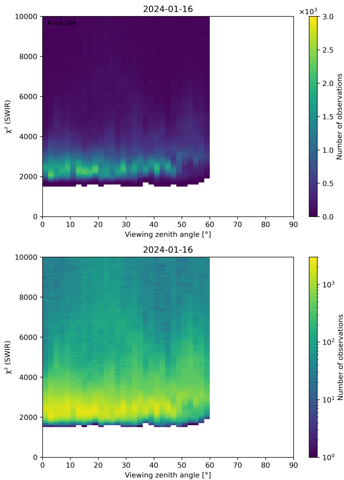
Figure 106: Scatter density plot of “Viewing zenith angle” against “ \chi^2 (SWIR)” for 2024-01-15 to 2024-01-17.
