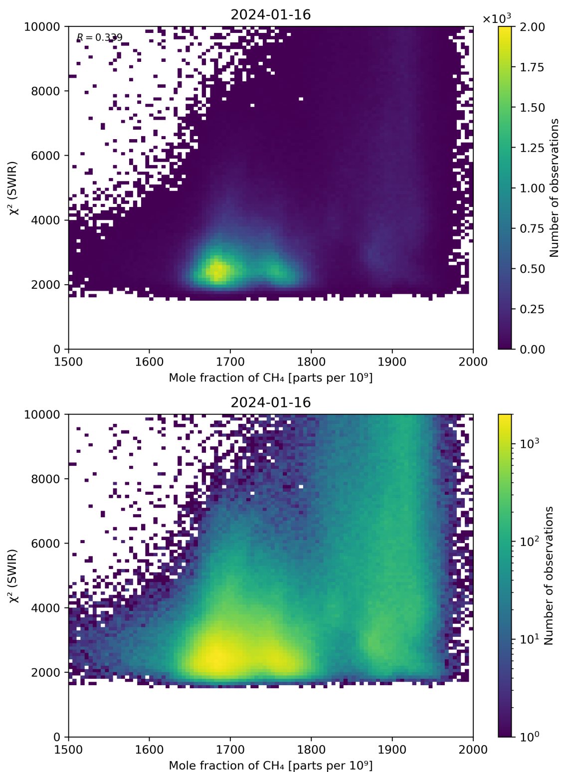
Figure 71: Scatter density plot of “Mole fraction of \text{CH}_4 ” against “ \chi^2 (SWIR)” for 2024-01-15 to 2024-01-17.
