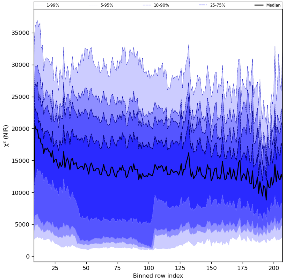
Figure 40: Along track statistics of “ \chi^2 (NIR)” for 2024-01-15 to 2024-01-17
