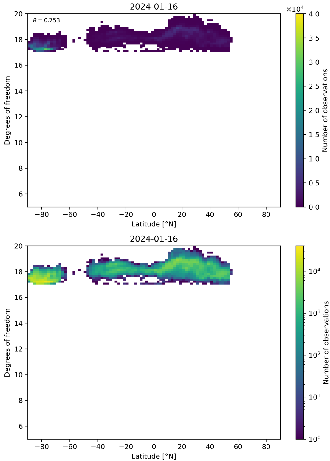
Figure 55: Scatter density plot of “Latitude” against “Degrees of freedom” for 2024-01-15 to 2024-01-17.
