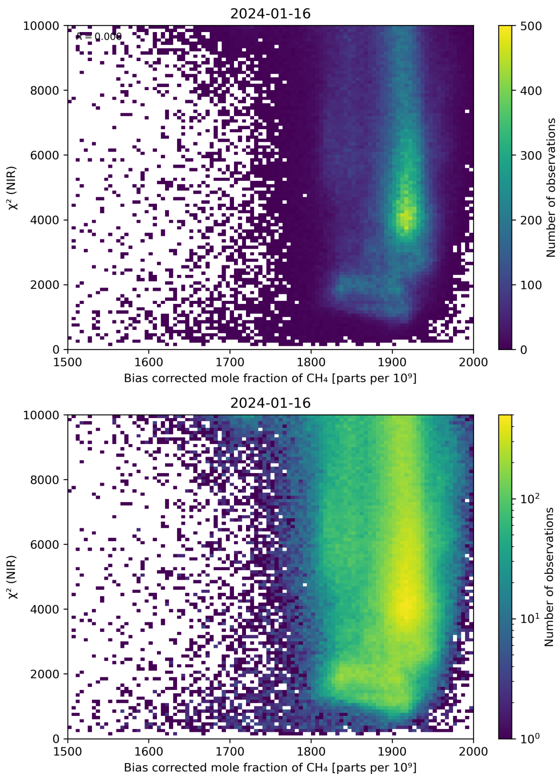
Figure 63: Scatter density plot of “Bias corrected mole fraction of CH 4 ” against “ \chi^2 (NIR)” for 2024-01-15 to 2024-01-17.
