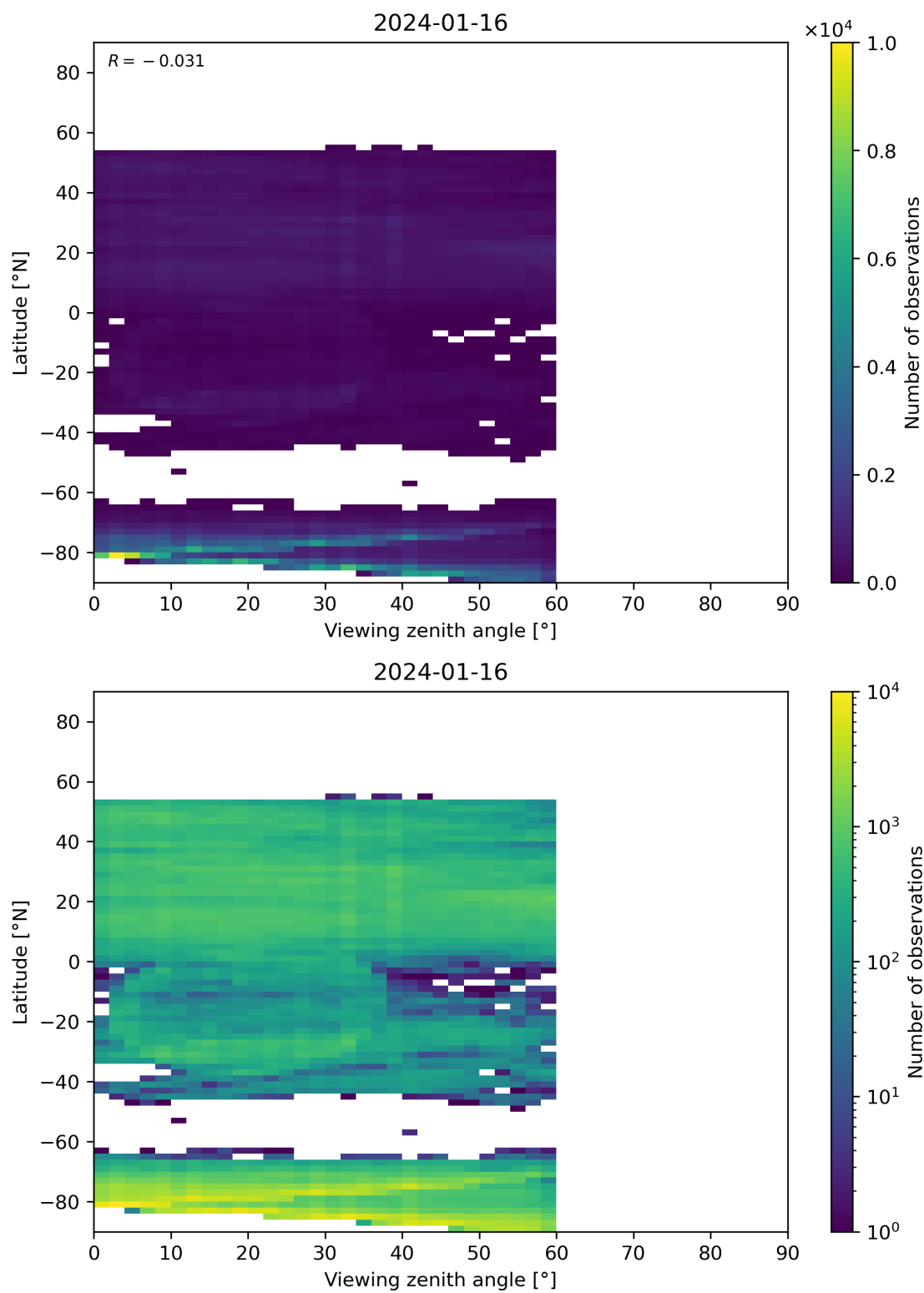
Figure 109: Scatter density plot of “Viewing zenith angle” against “Latitude” for 2024-01-15 to 2024-01-17.
