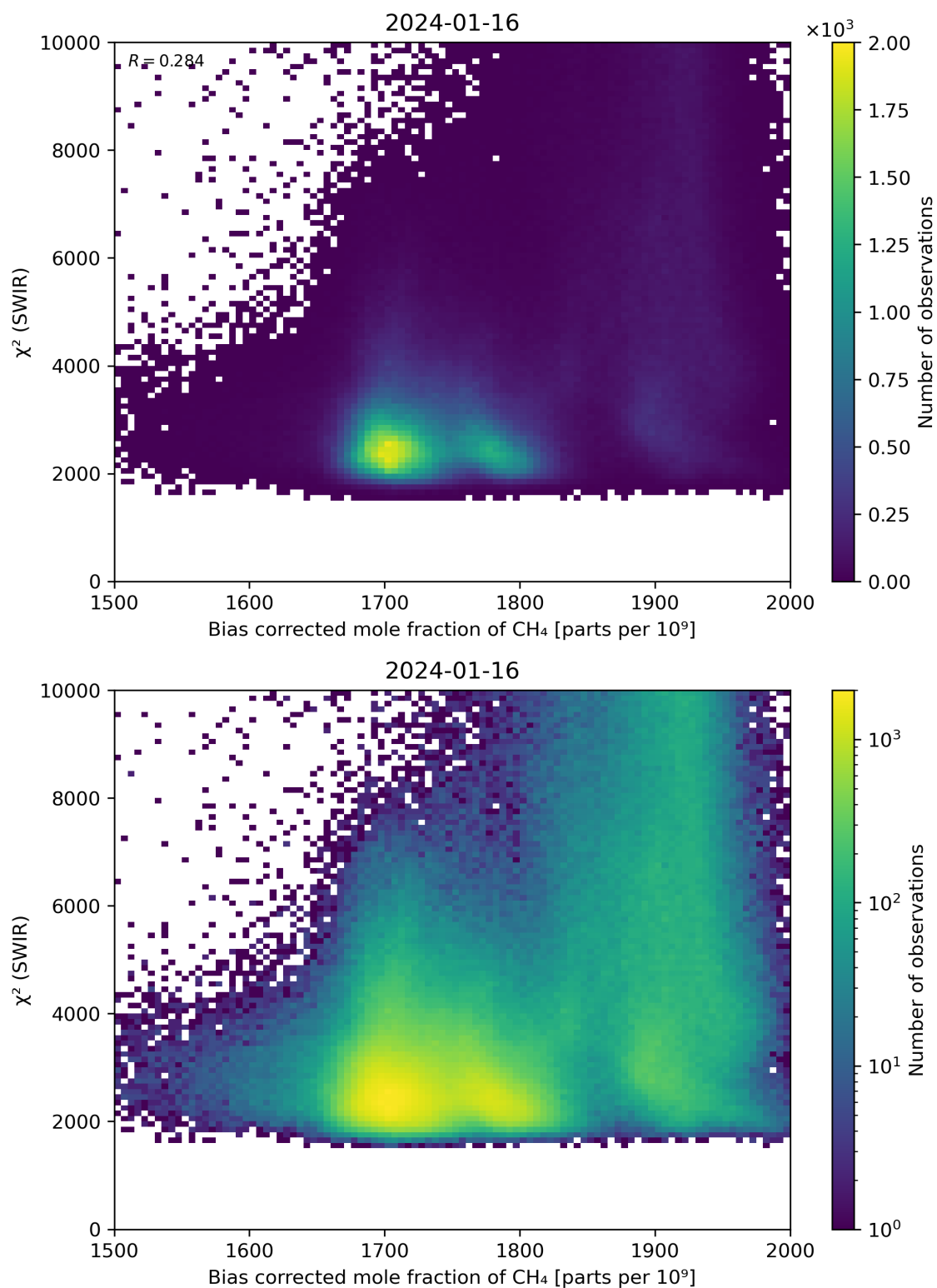
Figure 64: Scatter density plot of “Bias corrected mole fraction of \text{CH}_4 ” against “ \chi^2 (SWIR)” for 2024-01-15 to 2024-01-17.
