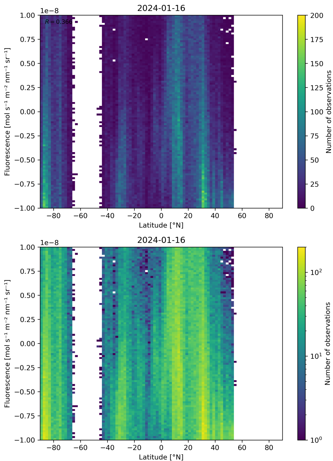
Figure 56: Scatter density plot of “Latitude” against “Fluorescence” for 2024-01-15 to 2024-01-17.
