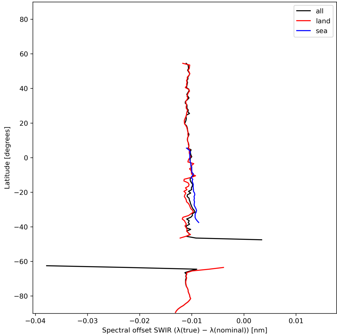
Figure 16: Zonal average of “Spectral offset SWIR ( \lambda(\text{true}) - \lambda(\text{nominal}) )” for 2024-01-15 to 2024-01-17.
