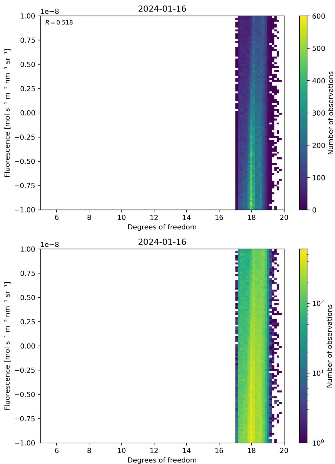
Figure 51: Scatter density plot of “Degrees of freedom” against “Fluorescence” for 2024-01-15 to 2024-01-17.
