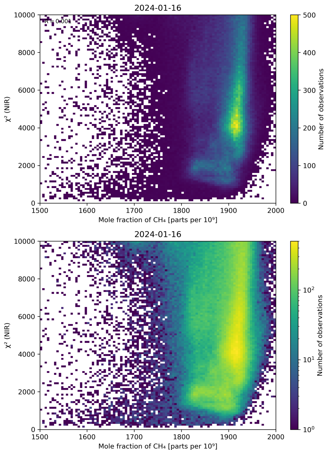
Figure 70: Scatter density plot of “Mole fraction of \text{CH}_4 ” against “ \chi^2 (NIR)” for 2024-01-15 to 2024-01-17.
