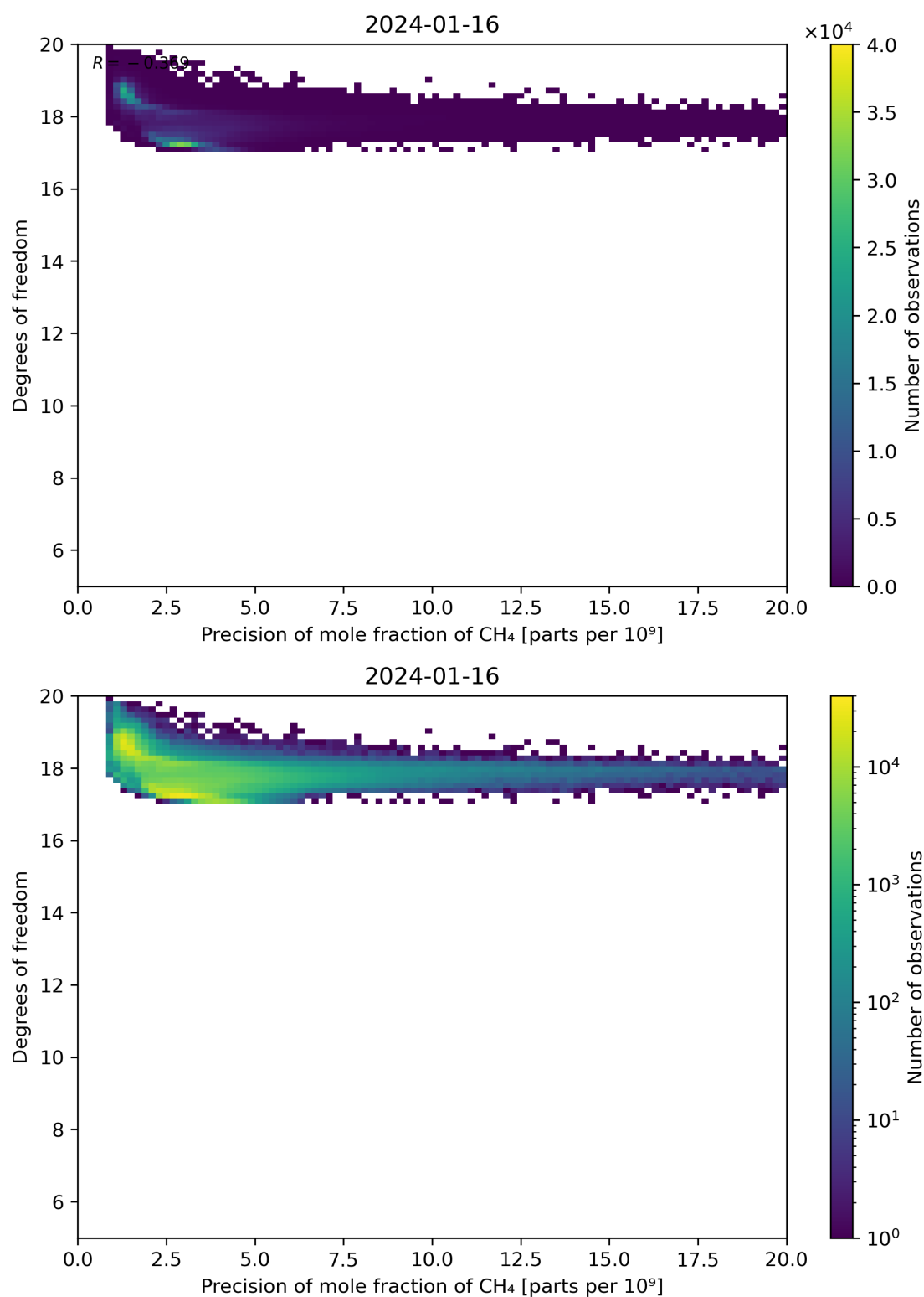
Figure 80: Scatter density plot of “Precision of mole fraction of CH 4 ” against “Degrees of freedom” for 2024-01-15 to 2024-01-17.
