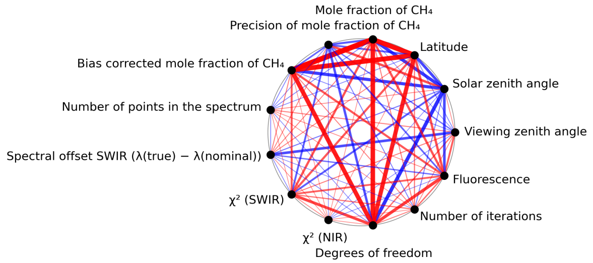
Figure 1: Map of correlation graph for 2024-01-15 to 2024-01-17.
