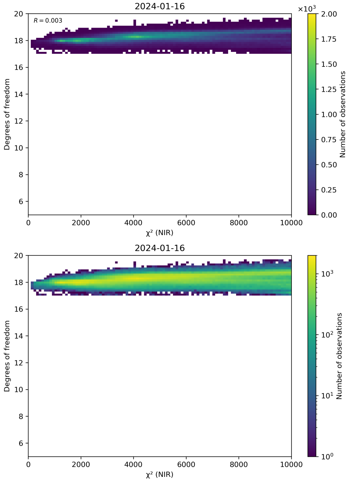
Figure 44: Scatter density plot of “ \chi^2 (NIR)” against “Degrees of freedom” for 2024-01-15 to 2024-01-17.
