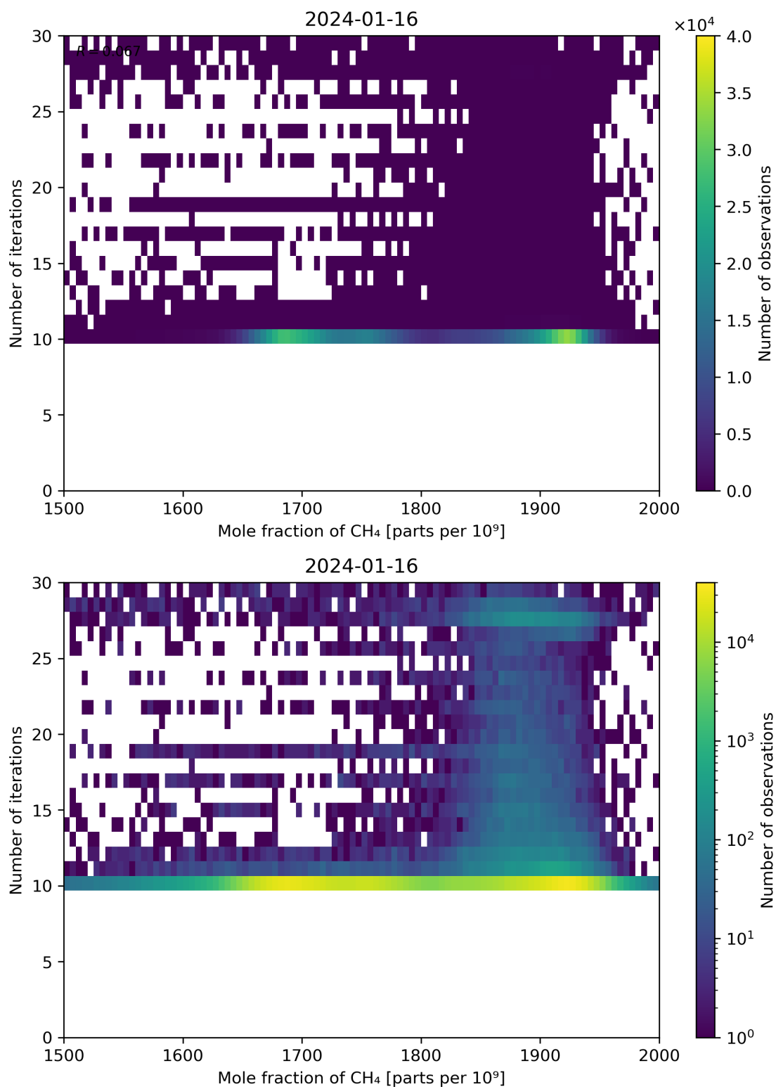
Figure 76: Scatter density plot of “Mole fraction of CH 4 ” against “Number of iterations” for 2024-01-15 to 2024-01-17.
