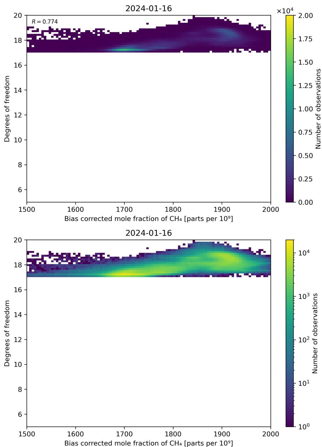
Figure 65: Scatter density plot of “Bias corrected mole fraction of CH 4 ” against “Degrees of freedom” for 2024-01-15 to 2024-01-17.
