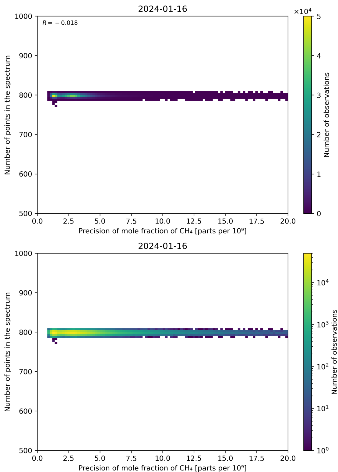
Figure 84: Scatter density plot of “Precision of mole fraction of CH 4 ” against “Number of points in the spectrum” for 2024-01-15 to 2024-01-17.
