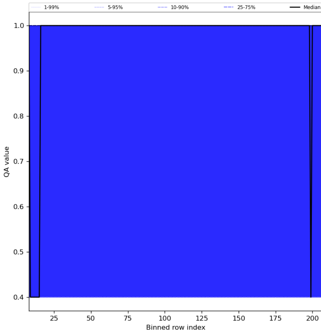
Figure 33: Along track statistics of “QA value” for 2024-01-15 to 2024-01-17
