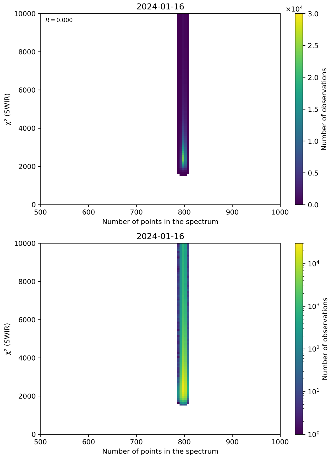
Figure 89: Scatter density plot of “Number of points in the spectrum” against “ \chi^2 (SWIR)” for 2024-01-15 to 2024-01-17.
