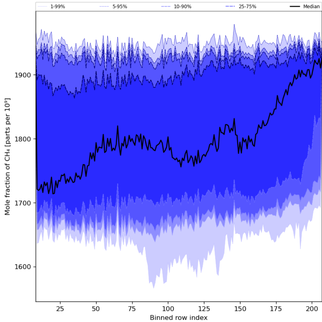
Figure 34: Along track statistics of “Mole fraction of CH 4 ” for 2024-01-15 to 2024-01-17
