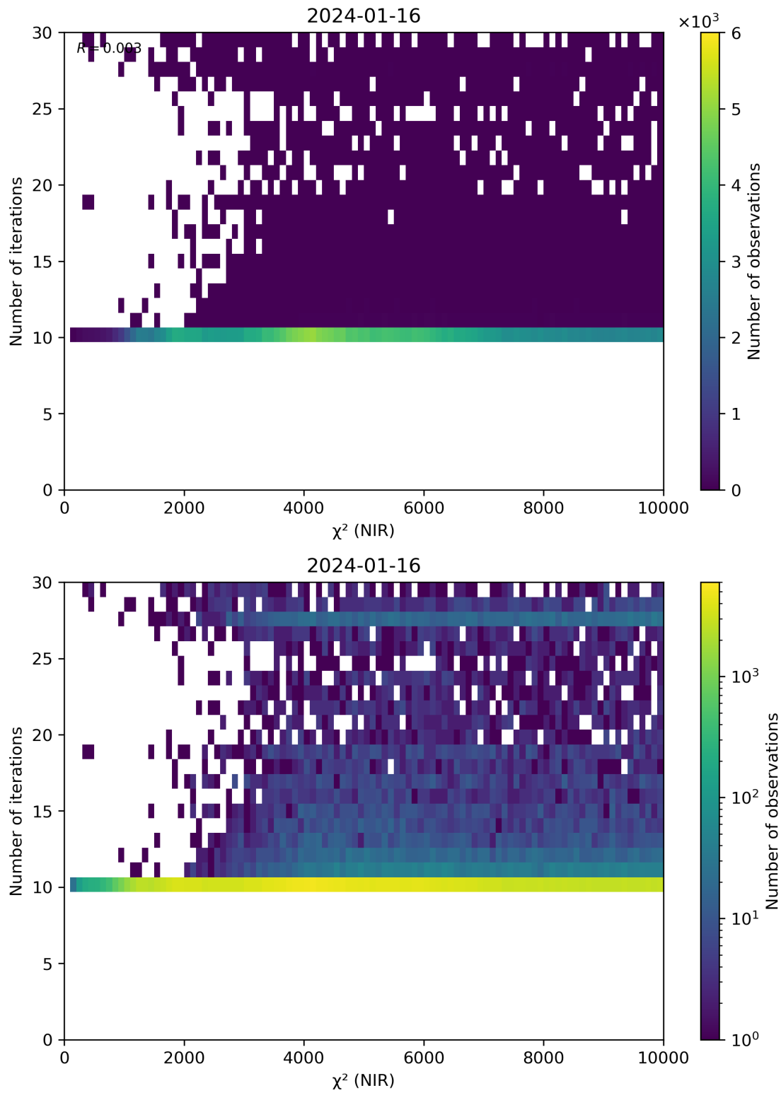
Figure 46: Scatter density plot of “ \chi^2 (NIR)” against “Number of iterations” for 2024-01-15 to 2024-01-17.
