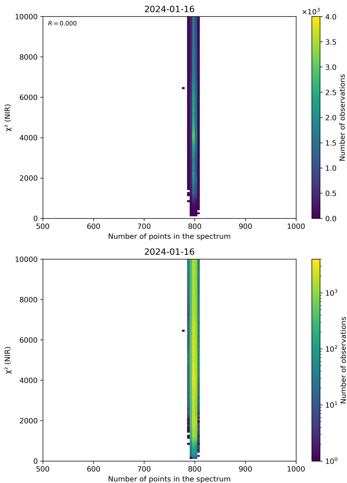
Figure 88: Scatter density plot of “Number of points in the spectrum” against “ \chi^2 (NIR)” for 2024-01-15 to 2024-01-17.
