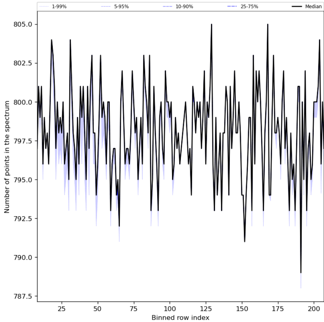
Figure 37: Along track statistics of “Number of points in the spectrum” for 2024-01-15 to 2024-01-17
