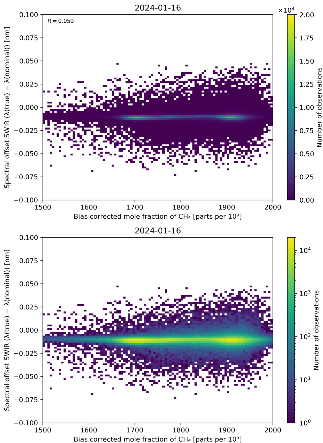
Figure 69: Scatter density plot of “Bias corrected mole fraction of \text{CH}_4 ” against “Spectral offset SWIR ( \lambda(\text{true}) - \lambda(\text{nominal}) )” for 2024-01-15 to 2024-01-17.
