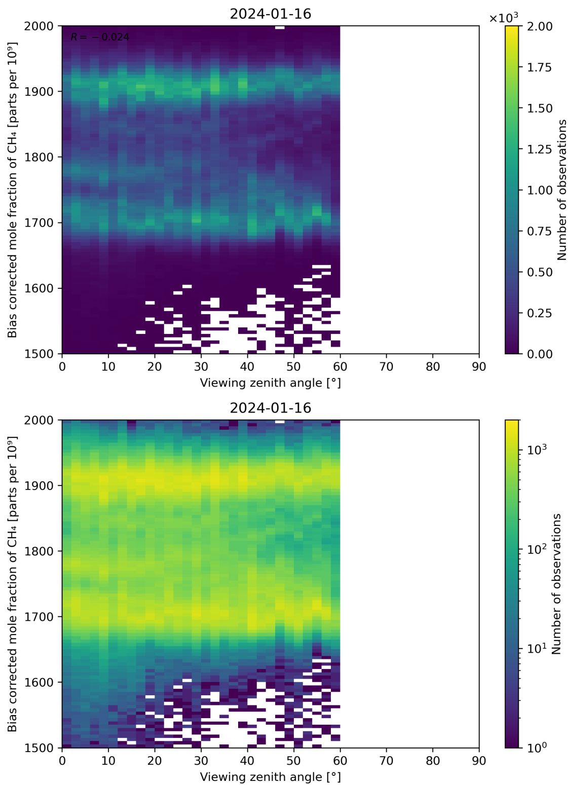
Figure 111: Scatter density plot of “Viewing zenith angle” against “Bias corrected mole fraction of CH 4 ” for 2024-01-15 to 2024-01-17.
