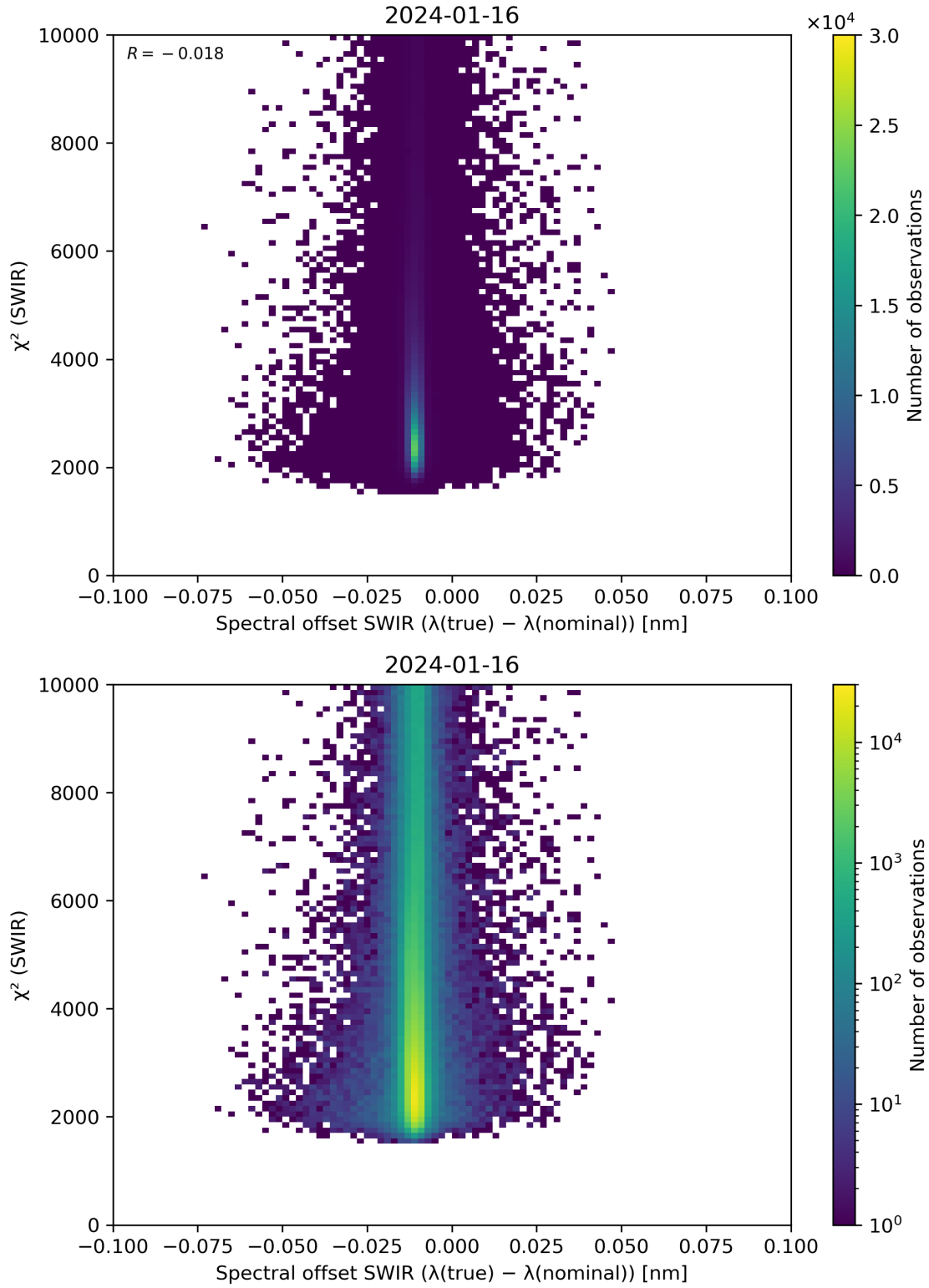
Figure 118: Scatter density plot of “Spectral offset SWIR ( \lambda(\text{true}) - \lambda(\text{nominal}) )” against “ \chi^2 (SWIR)” for 2024-01-15 to 2024-01-17.
