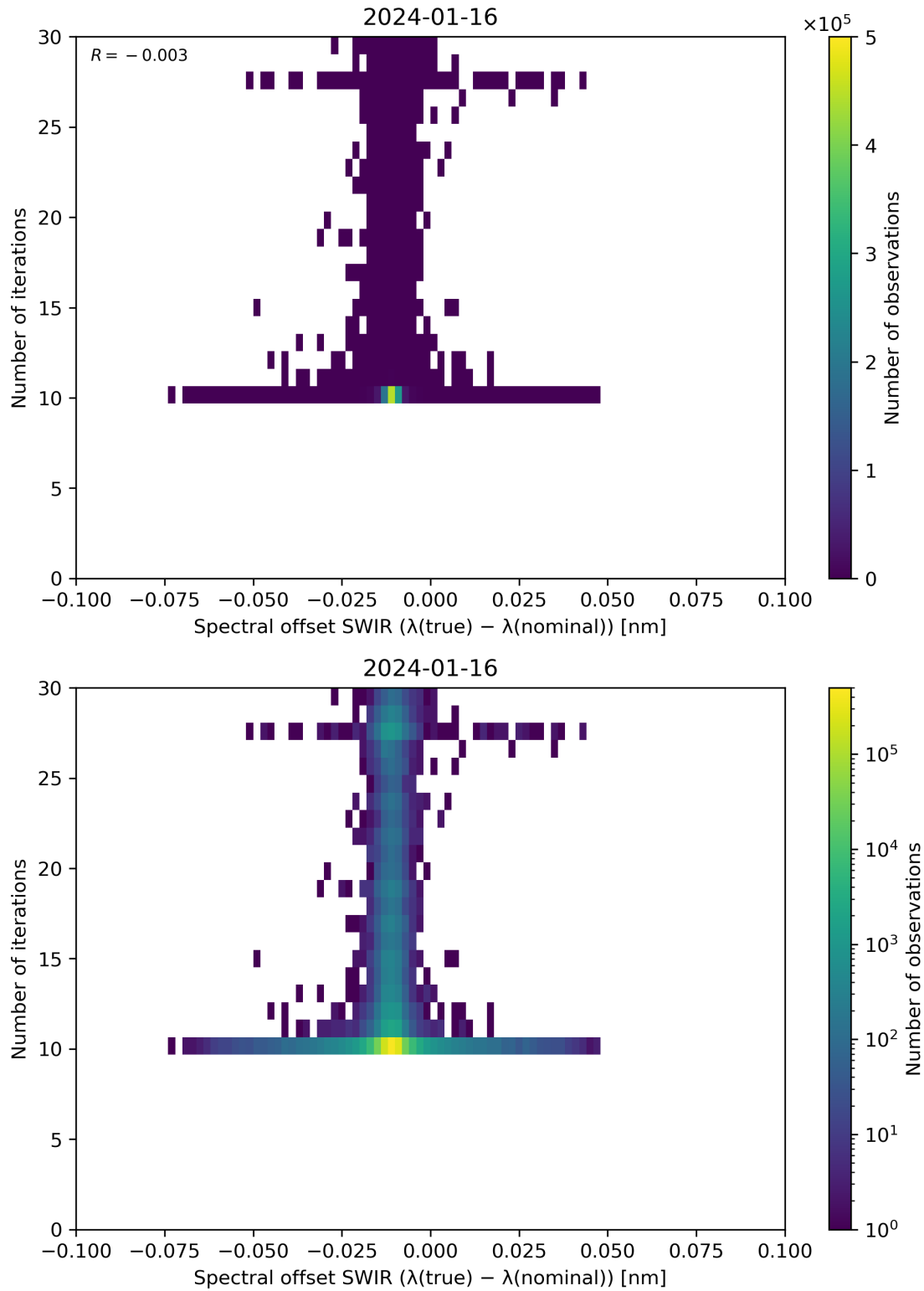
Figure 121: Scatter density plot of “Spectral offset SWIR ( \lambda(\text{true}) - \lambda(\text{nominal}) )” against “Number of iterations” for 2024-01-15 to 2024-01-17.
