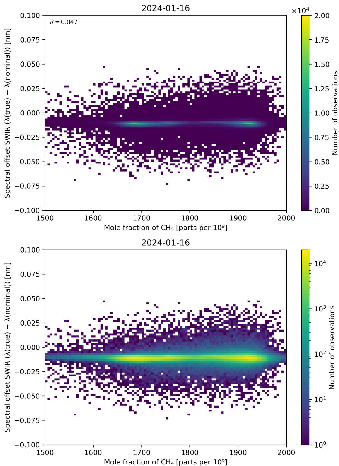
Figure 86: Scatter density plot of “Mole fraction of CH 4 ” against “Spectral offset SWIR ( \lambda(\text{true}) - \lambda(\text{nominal}) )” for 2024-01-15 to 2024-01-17.
