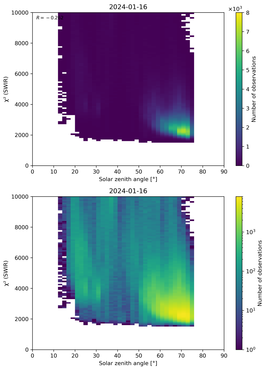
Figure 95: Scatter density plot of “Solar zenith angle” against “ \chi^2 (SWIR)” for 2024-01-15 to 2024-01-17.
