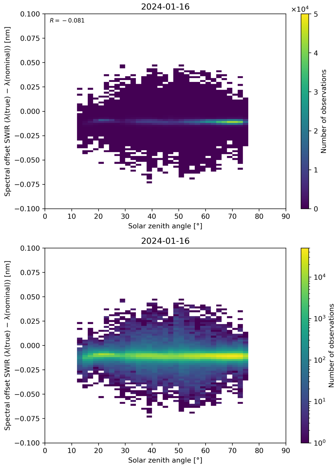
Figure 104: Scatter density plot of “Solar zenith angle” against “Spectral offset SWIR ( \lambda(\text{true}) - \lambda(\text{nominal}) )” for 2024-01-15 to 2024-01-17.
