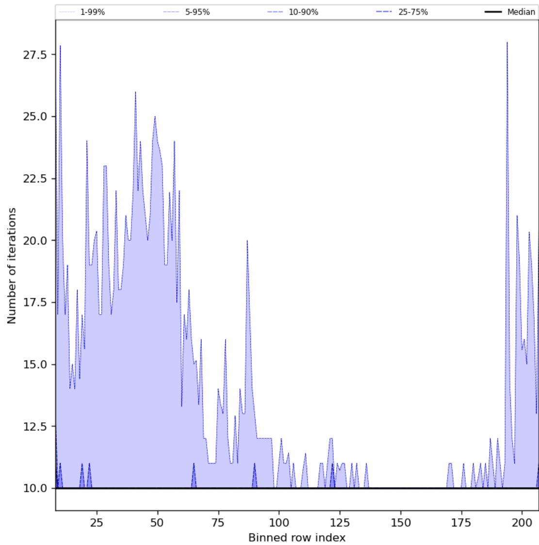
Figure 42: Along track statistics of “Number of iterations” for 2024-01-15 to 2024-01-17
