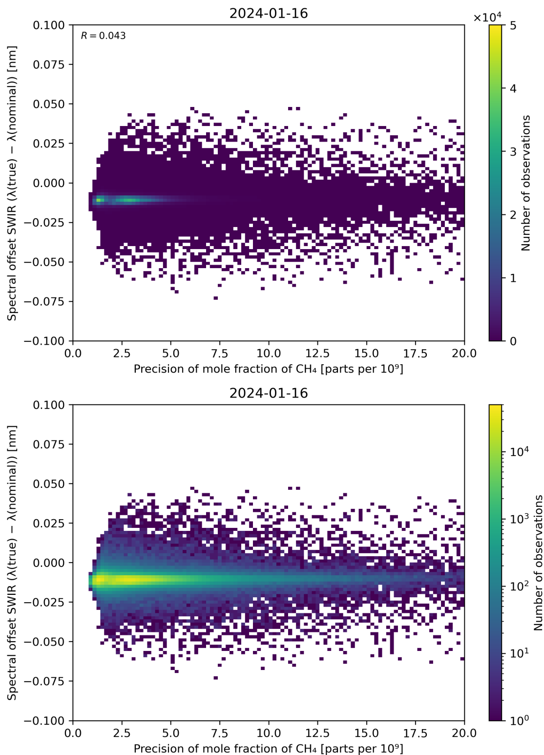
Figure 85: Scatter density plot of “Precision of mole fraction of \text{CH}_4 ” against “Spectral offset SWIR ( \lambda(\text{true}) - \lambda(\text{nominal}) )” for 2024-01-15 to 2024-01-17.
