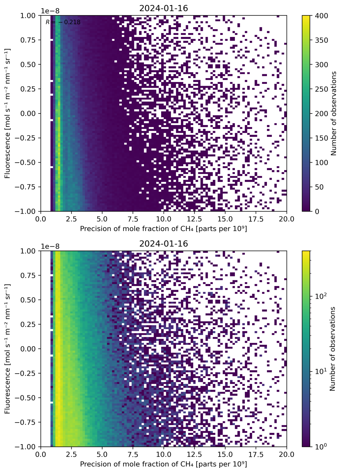
Figure 81: Scatter density plot of “Precision of mole fraction of \text{CH}_4 ” against “Fluorescence” for 2024-01-15 to 2024-01-17.
