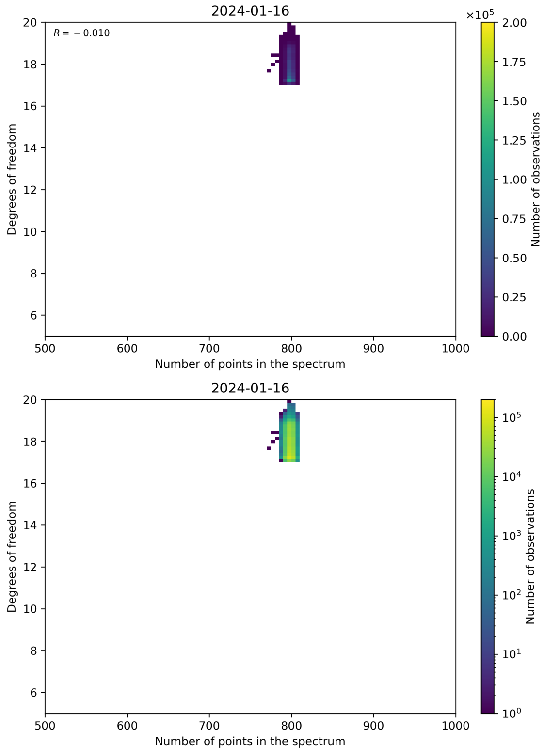
Figure 90: Scatter density plot of “Number of points in the spectrum” against “Degrees of freedom” for 2024-01-15 to 2024-01-17.
