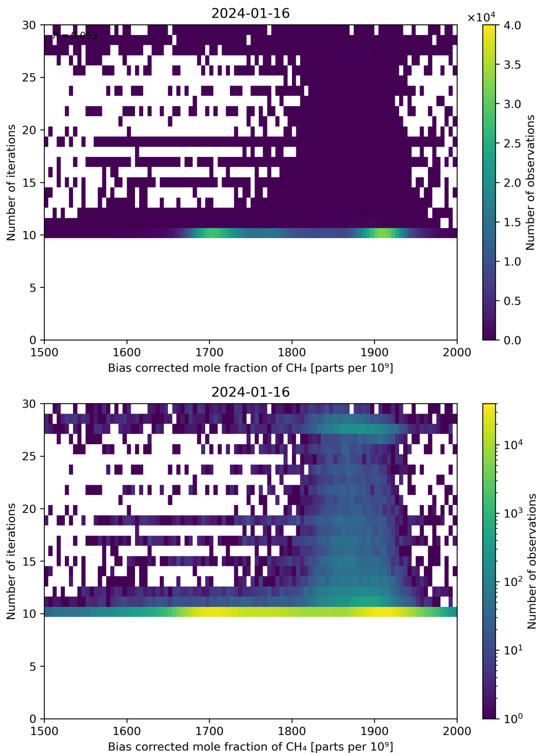
Figure 67: Scatter density plot of “Bias corrected mole fraction of CH 4 ” against “Number of iterations” for 2024-01-15 to 2024-01-17.
