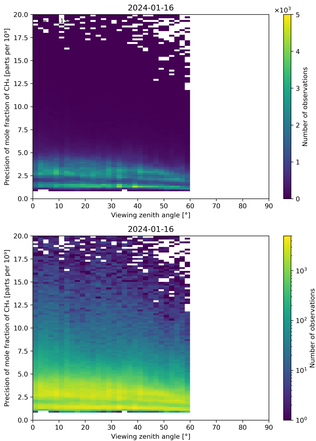
Figure 112: Scatter density plot of “Viewing zenith angle” against “Precision of mole fraction of CH 4 ” for 2024-01-15 to 2024-01-17.
