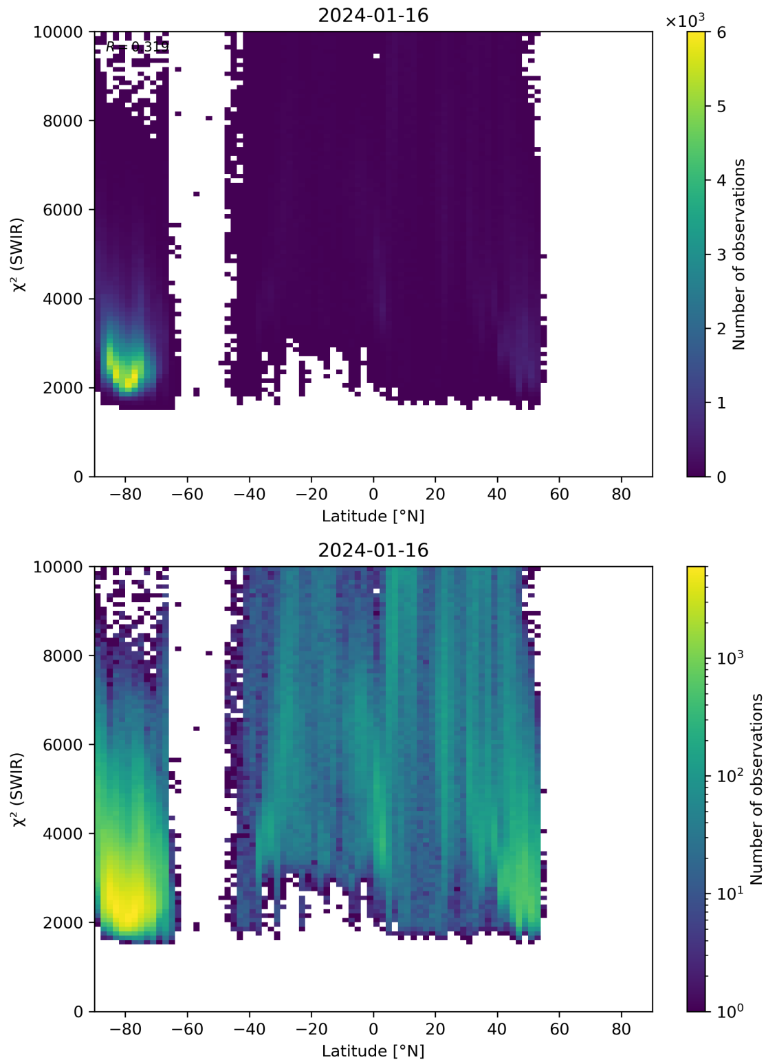
Figure 54: Scatter density plot of “Latitude” against “ \chi^2 (SWIR)” for 2024-01-15 to 2024-01-17.
