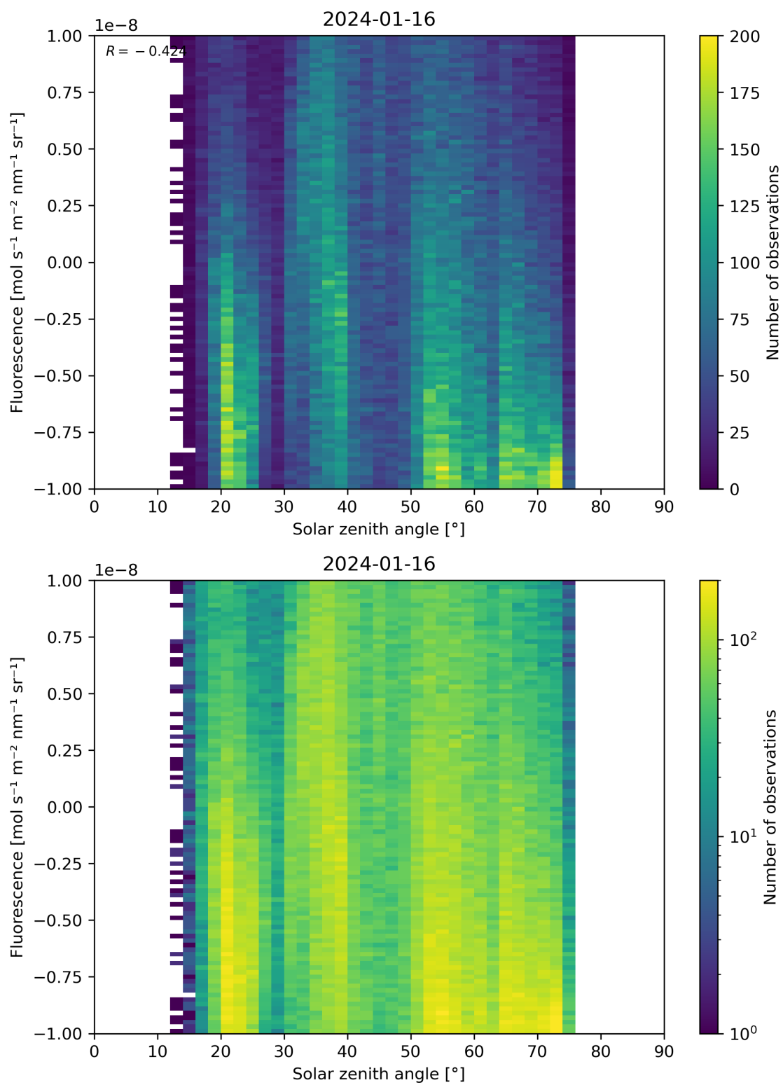
Figure 97: Scatter density plot of “Solar zenith angle” against “Fluorescence” for 2024-01-15 to 2024-01-17.
