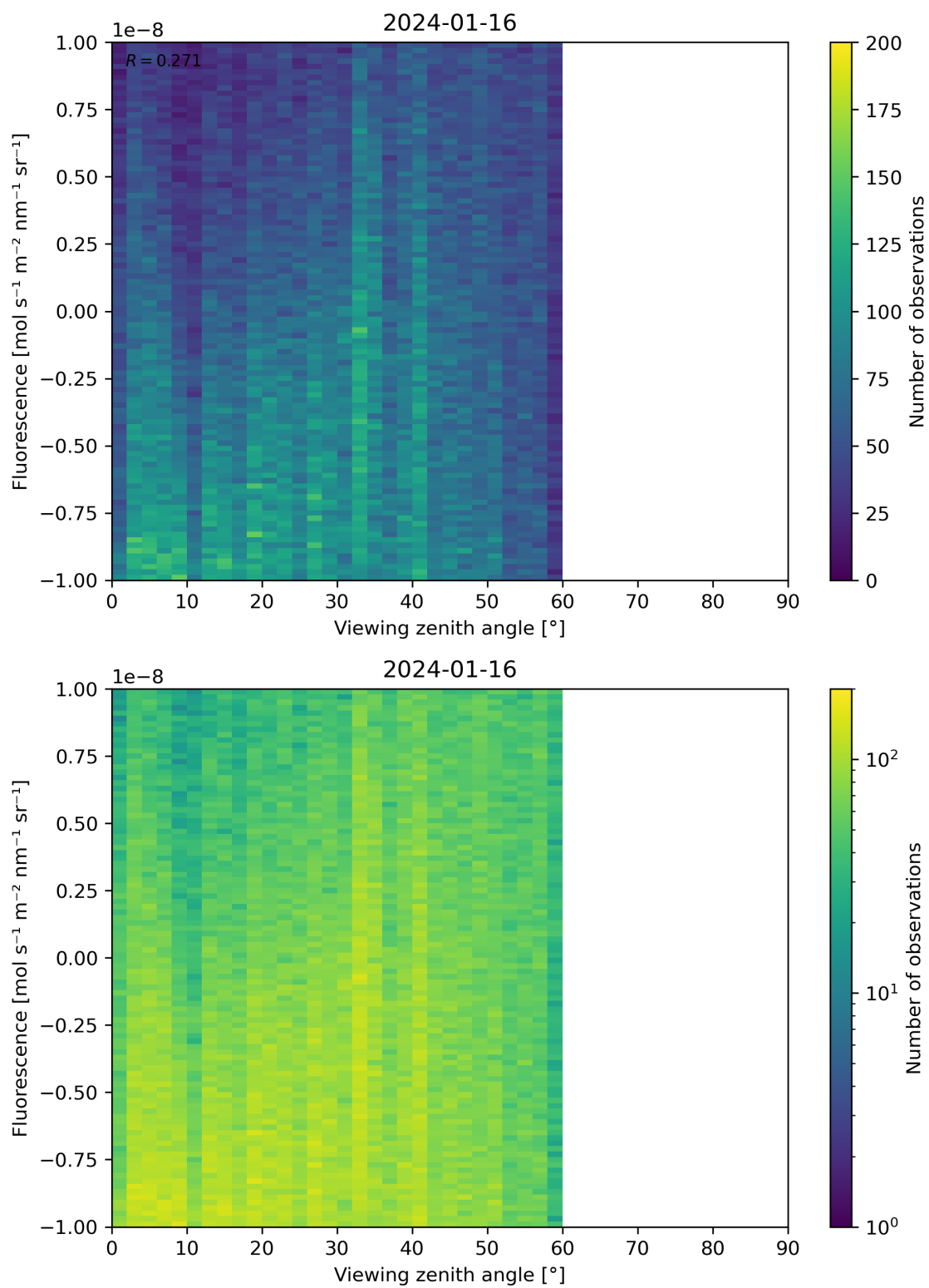
Figure 108: Scatter density plot of “Viewing zenith angle” against “Fluorescence” for 2024-01-15 to 2024-01-17.
