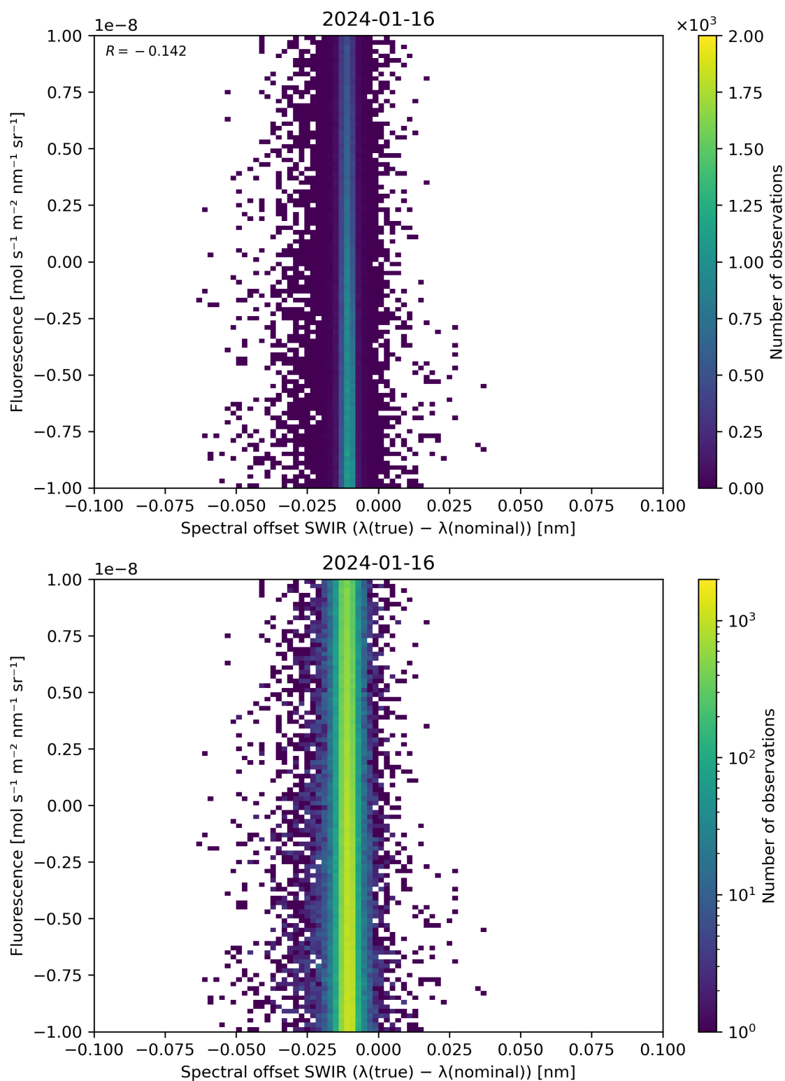
Figure 120: Scatter density plot of “Spectral offset SWIR ( \lambda(\text{true}) - \lambda(\text{nominal}) )” against “Fluorescence” for 2024-01-15 to 2024-01-17.
