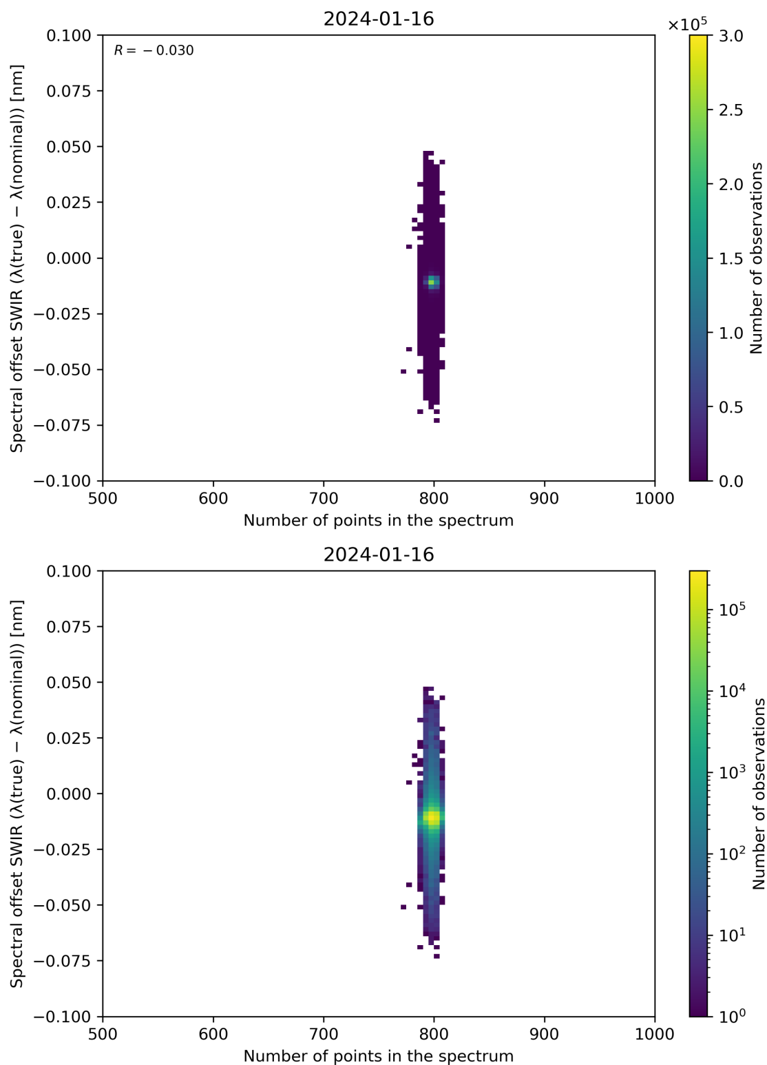
Figure 93: Scatter density plot of “Number of points in the spectrum” against “Spectral offset SWIR ( \lambda(\text{true}) - \lambda(\text{nominal}) )” for 2024-01-15 to 2024-01-17.
