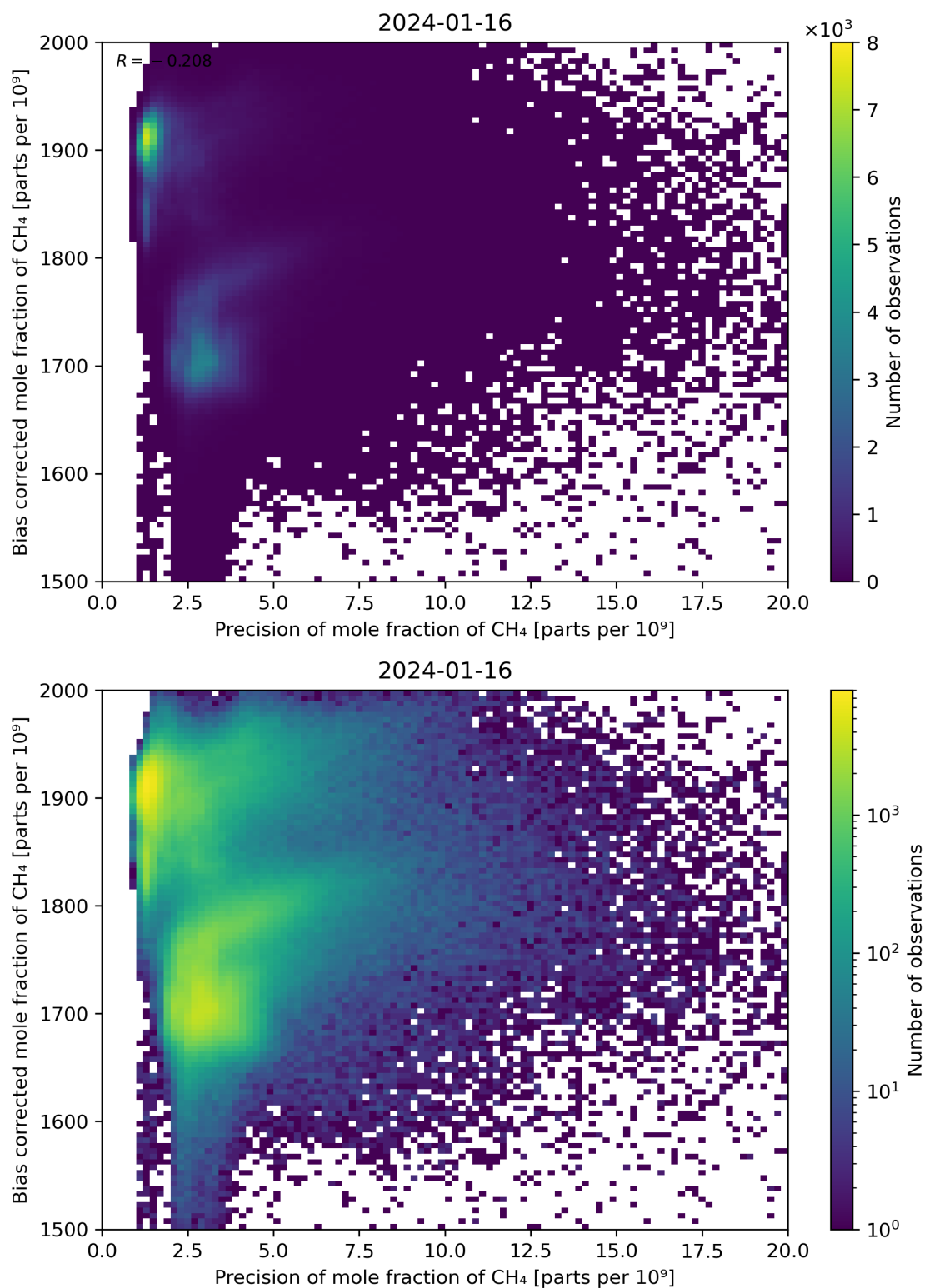
Figure 82: Scatter density plot of “Precision of mole fraction of CH 4 ” against “Bias corrected mole fraction of CH 4 ” for 2024-01-15 to 2024-01-17.
