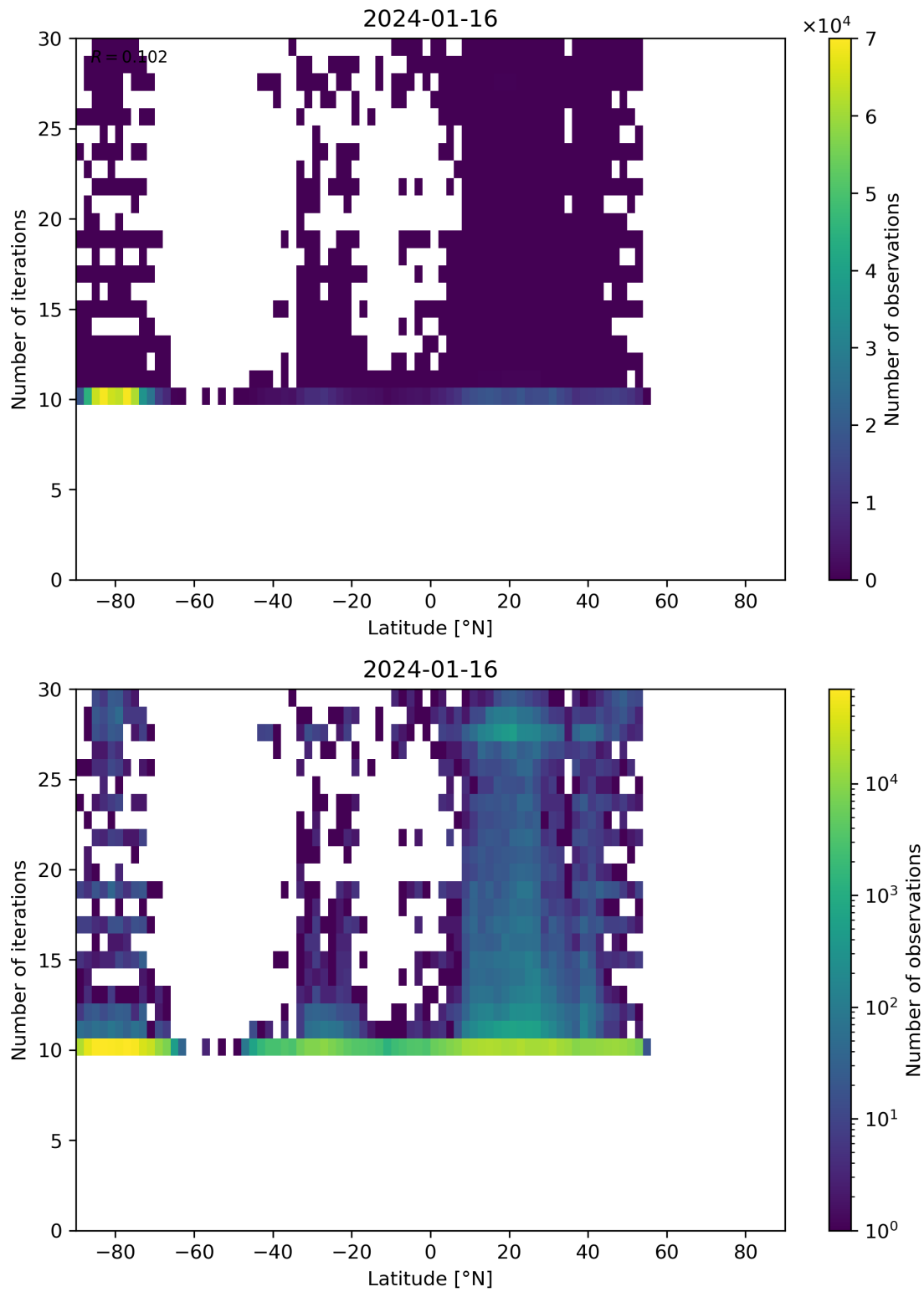
Figure 60: Scatter density plot of “Latitude” against “Number of iterations” for 2024-01-15 to 2024-01-17.
