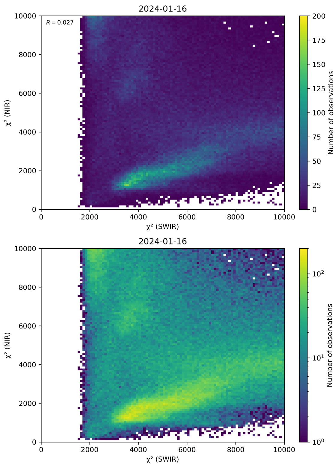
Figure 47: Scatter density plot of “ \chi^2 (SWIR)” against “ \chi^2 (NIR)” for 2024-01-15 to 2024-01-17.
