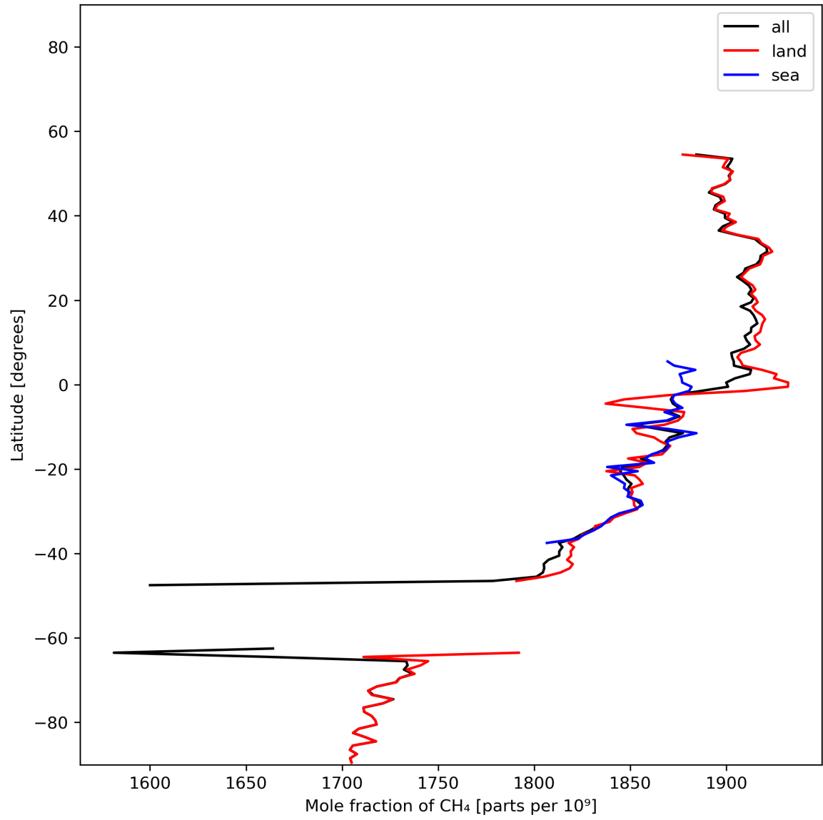
Figure 12: Zonal average of “Mole fraction of \text{CH}_4 ” for 2024-01-15 to 2024-01-17.
