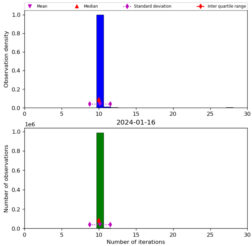
Figure 31: Histogram of "Number of iterations" for 2024-01-15 to 2024-01-17
