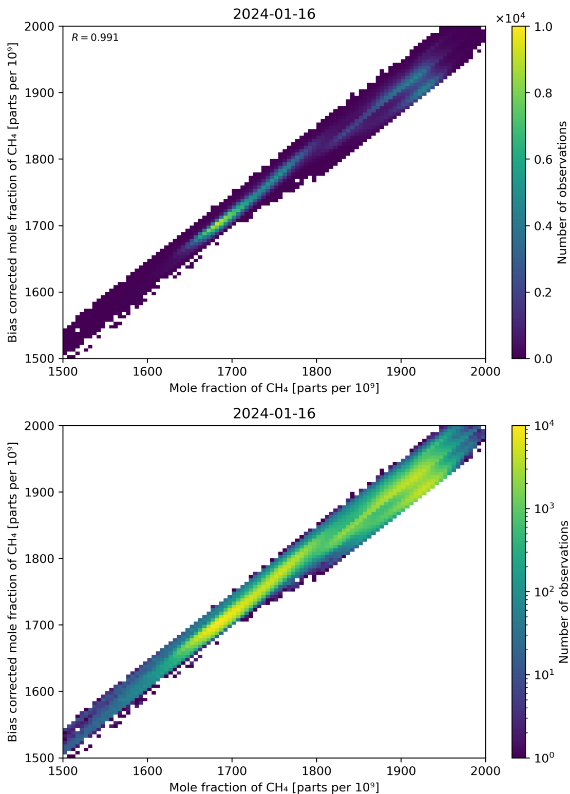
Figure 74: Scatter density plot of “Mole fraction of CH 4 ” against “Bias corrected mole fraction of CH 4 ” for 2024-01-15 to 2024-01-17.
