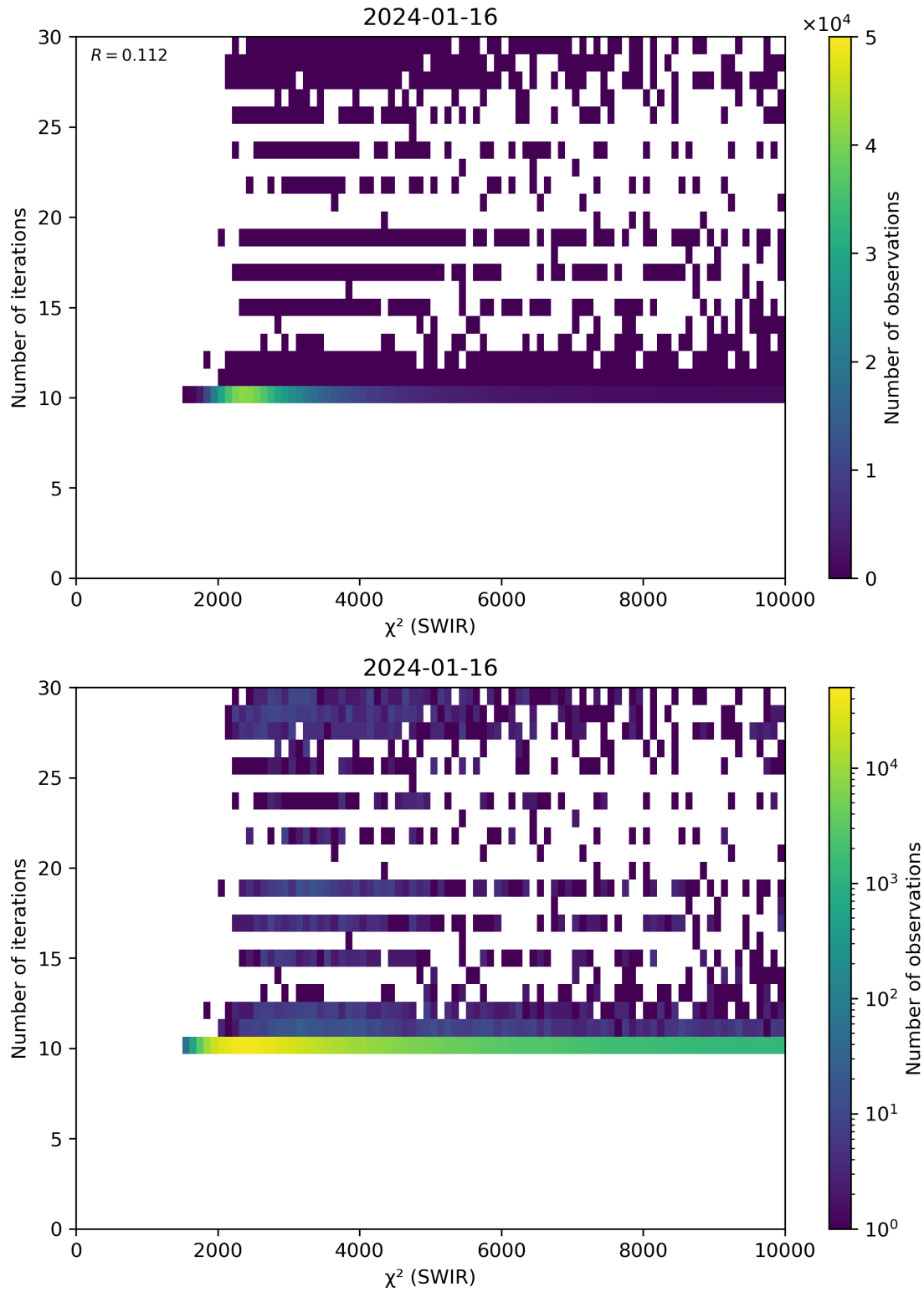
Figure 50: Scatter density plot of “ \chi^2 (SWIR)” against “Number of iterations” for 2024-01-15 to 2024-01-17.
