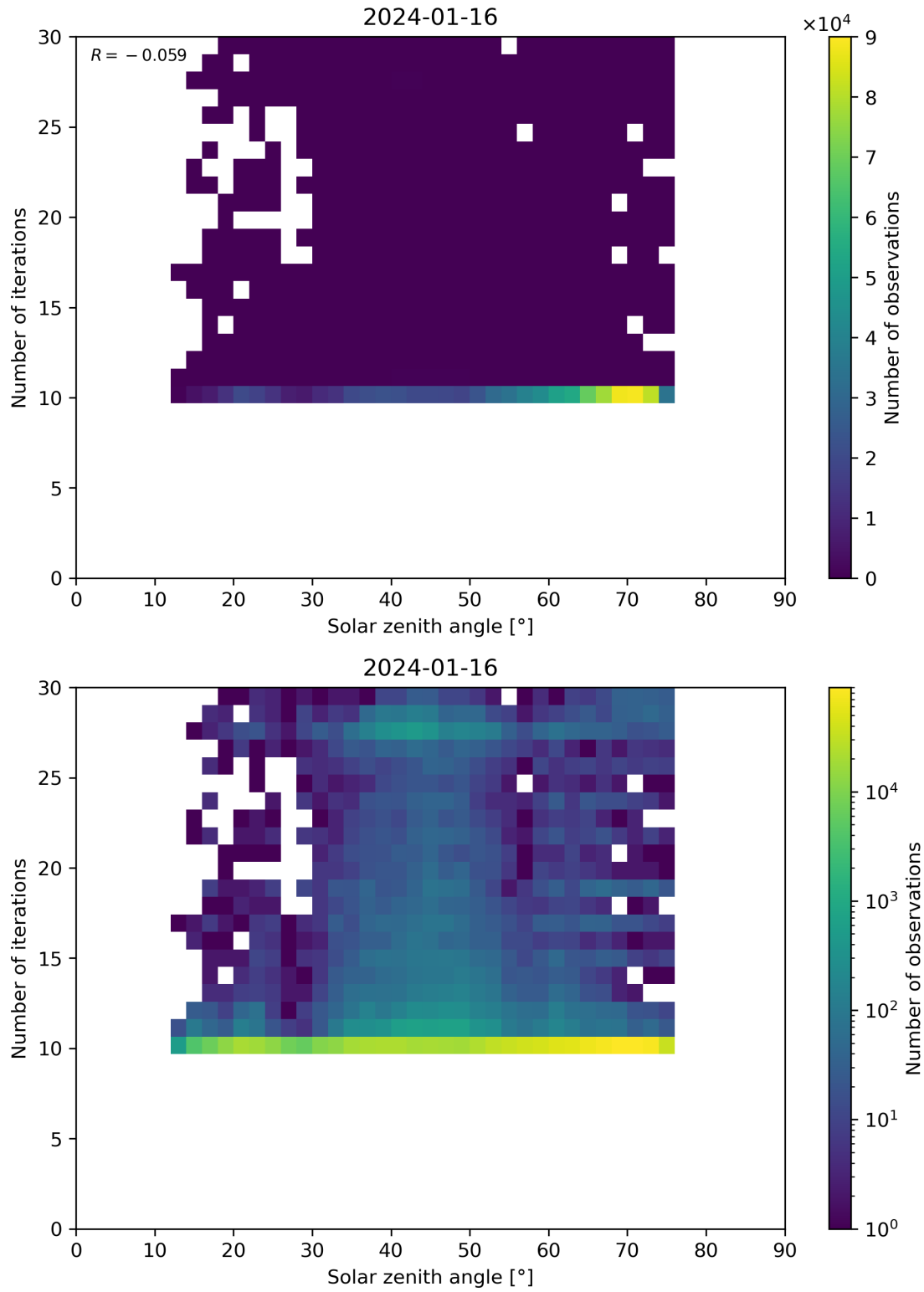
Figure 102: Scatter density plot of “Solar zenith angle” against “Number of iterations” for 2024-01-15 to 2024-01-17.
