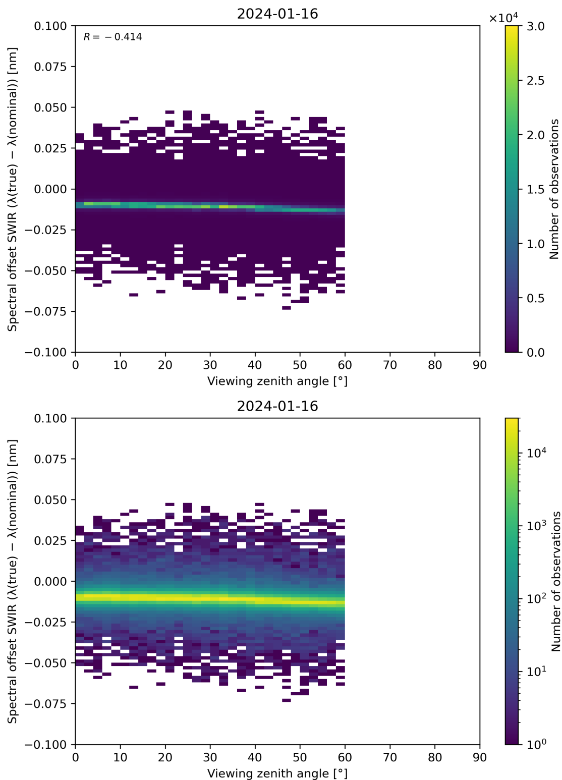
Figure 116: Scatter density plot of “Viewing zenith angle” against “Spectral offset SWIR ( \lambda(\text{true}) - \lambda(\text{nominal}) )” for 2024-01-15 to 2024-01-17.
