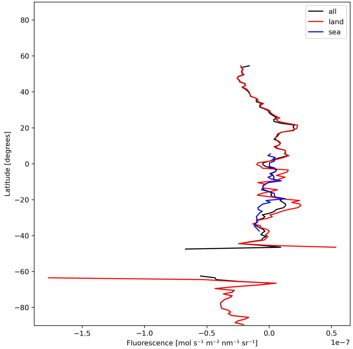
Figure 21: Zonal average of “Fluorescence” for 2024-01-15 to 2024-01-17.
