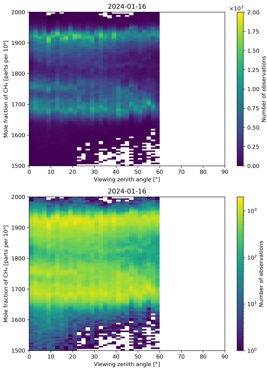
Figure 110: Scatter density plot of “Viewing zenith angle” against “Mole fraction of \text{CH}_4 ” for 2024-01-15 to 2024-01-17.
