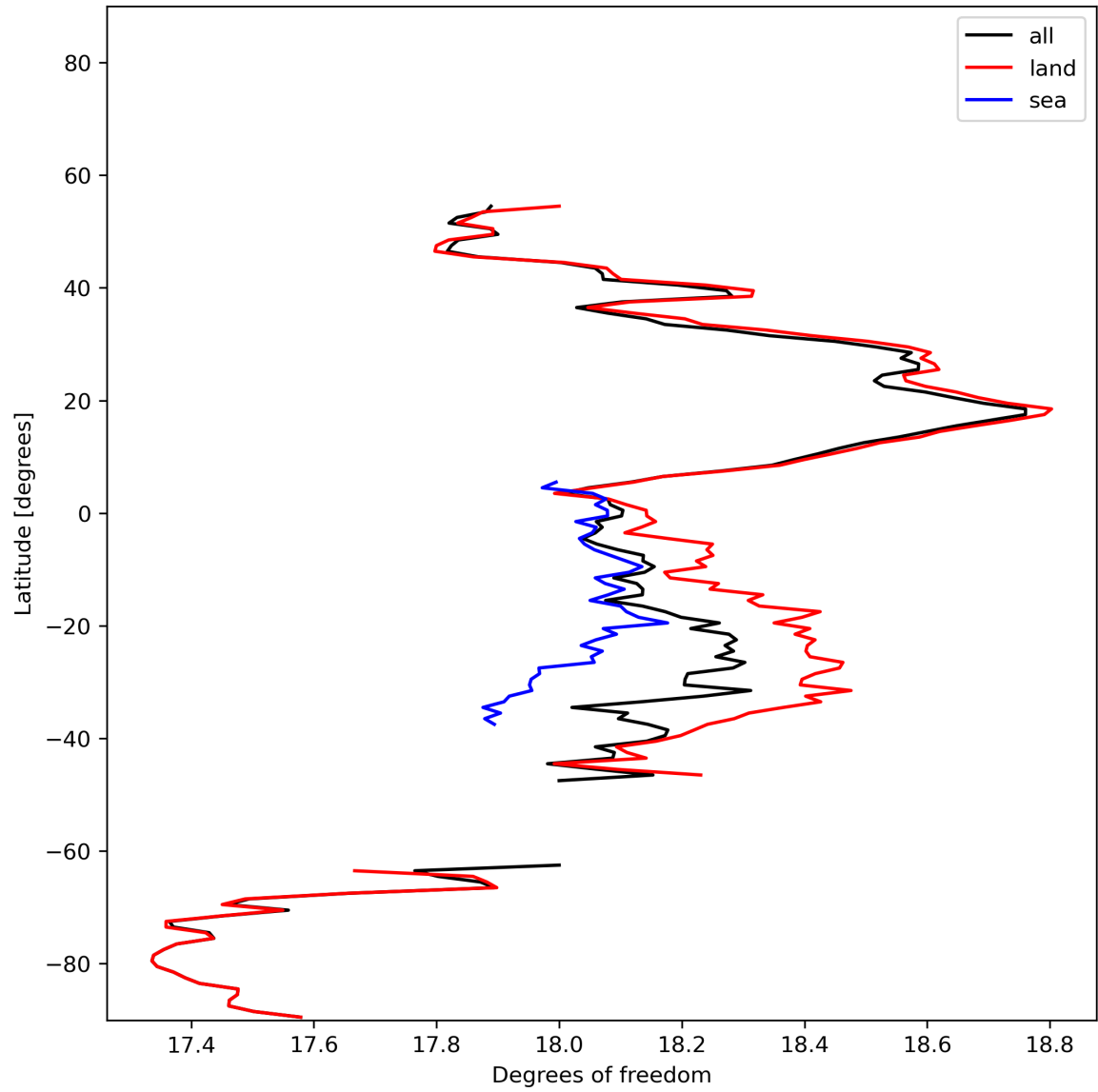
Figure 19: Zonal average of “Degrees of freedom” for 2024-01-15 to 2024-01-17.
