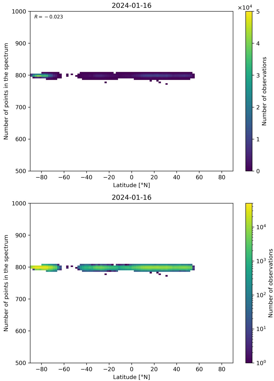
Figure 61: Scatter density plot of “Latitude” against “Number of points in the spectrum” for 2024-01-15 to 2024-01-17.
