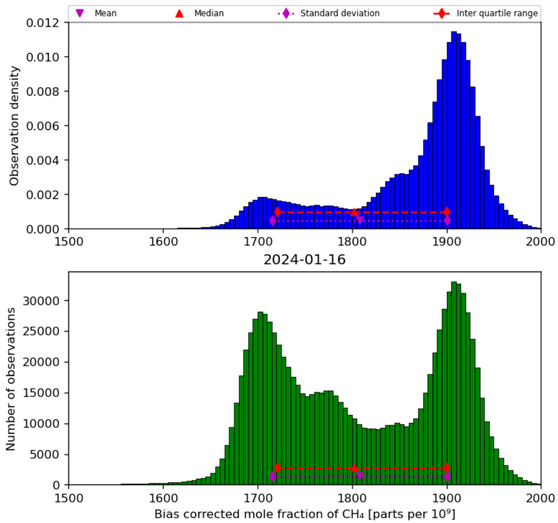
Figure 25: Histogram of “Bias corrected mole fraction of CH 4 ” for 2024-01-15 to 2024-01-17
