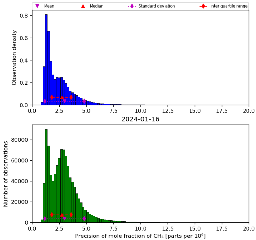
Figure 24: Histogram of “Precision of mole fraction of CH 4 ” for 2024-01-15 to 2024-01-17
