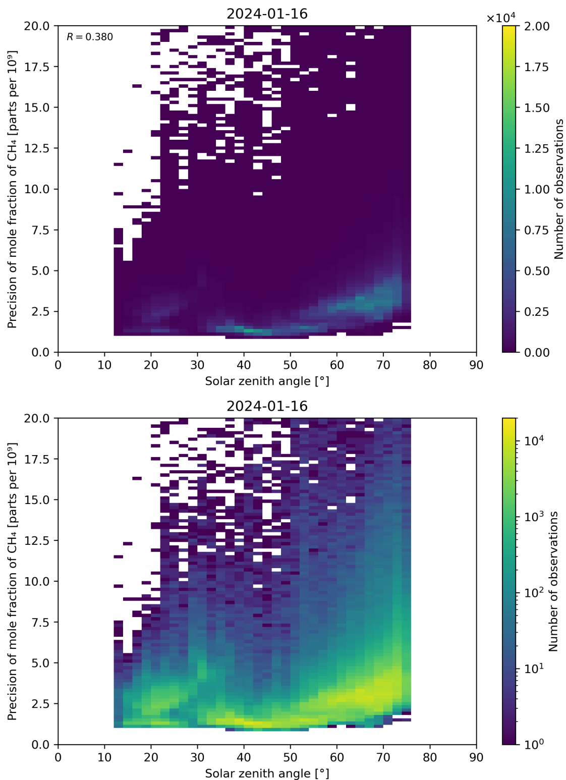
Figure 101: Scatter density plot of “Solar zenith angle” against “Precision of mole fraction of CH 4 ” for 2024-01-15 to 2024-01-17.
