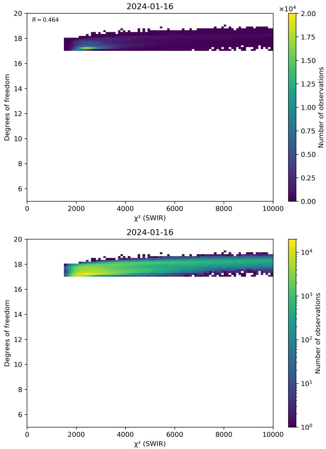
Figure 48: Scatter density plot of “ \chi^2 (SWIR)” against “Degrees of freedom” for 2024-01-15 to 2024-01-17.
