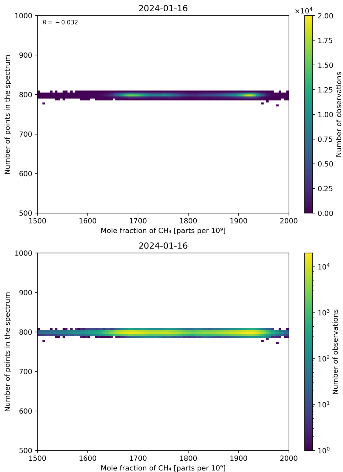
Figure 77: Scatter density plot of “Mole fraction of CH 4 ” against “Number of points in the spectrum” for 2024-01-15 to 2024-01-17.
