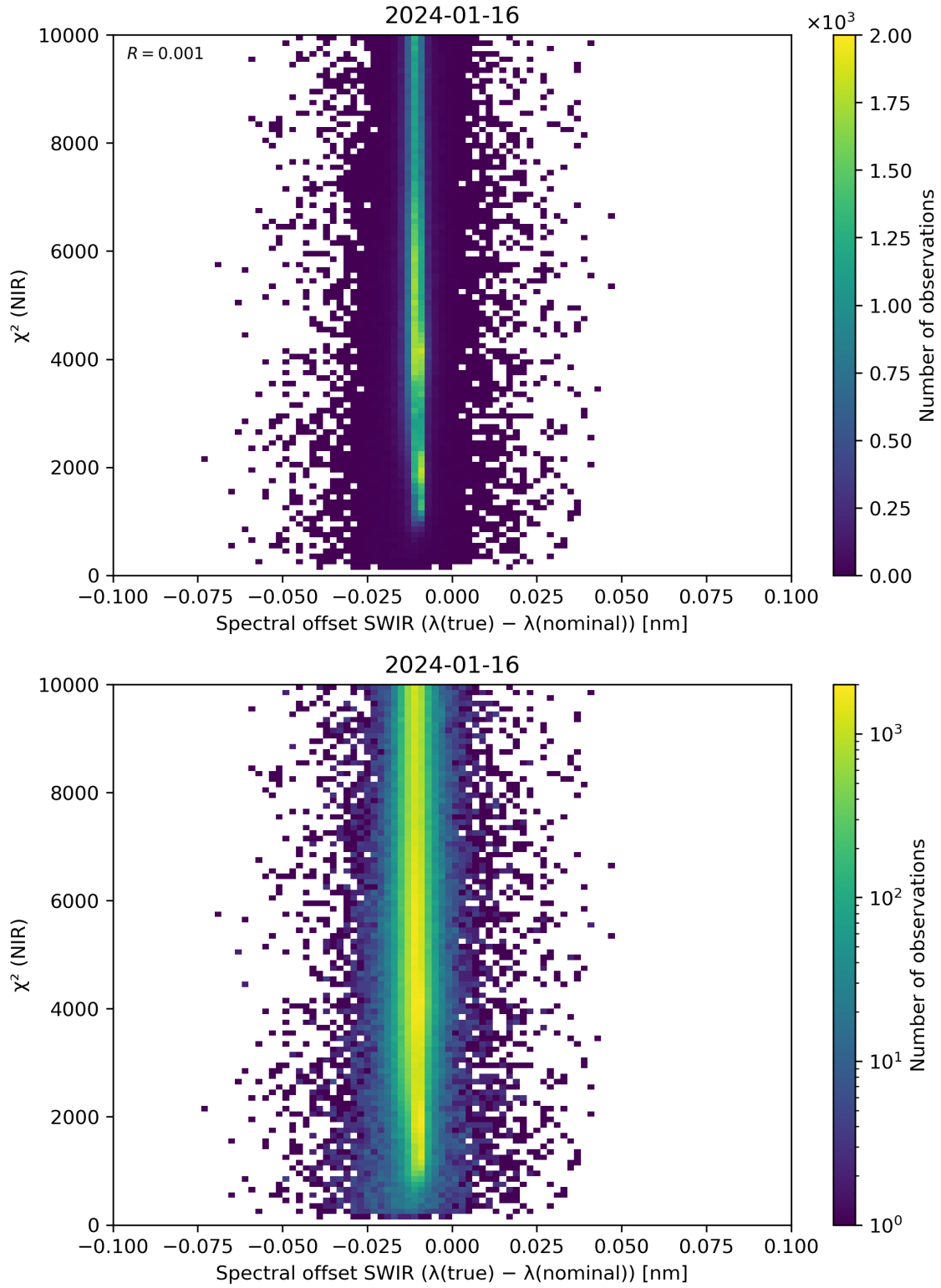
Figure 117: Scatter density plot of “Spectral offset SWIR ( \lambda(\text{true}) - \lambda(\text{nominal}) )” against “ \chi^2 (NIR)” for 2024-01-15 to 2024-01-17.
