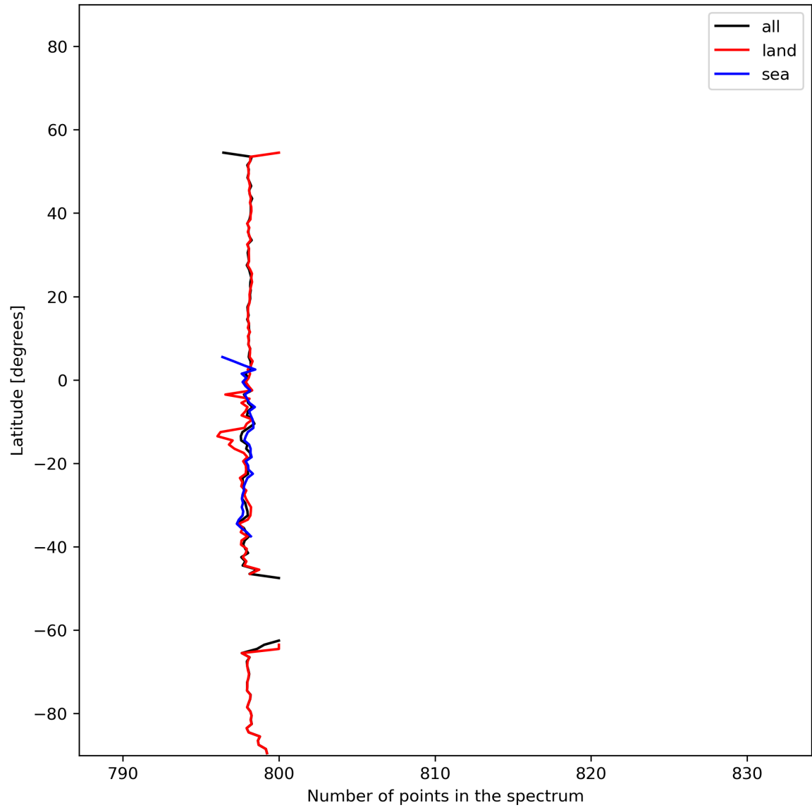
Figure 15: Zonal average of “Number of points in the spectrum” for 2024-01-15 to 2024-01-17.
