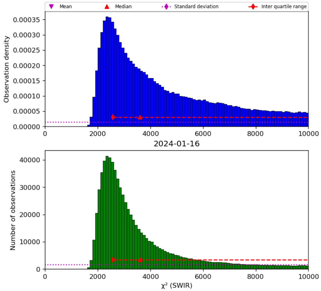
Figure 28: Histogram of “ \chi^2 (SWIR)” for 2024-01-15 to 2024-01-17
