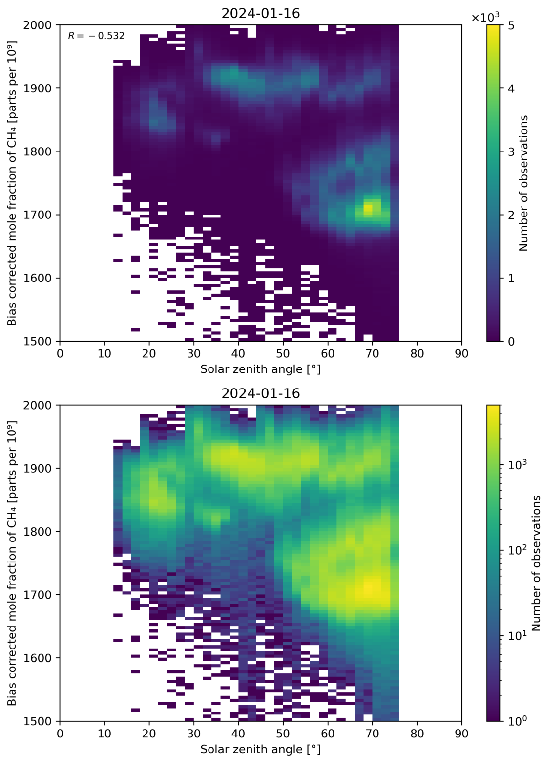
Figure 100: Scatter density plot of “Solar zenith angle” against “Bias corrected mole fraction of CH 4 ” for 2024-01-15 to 2024-01-17.
