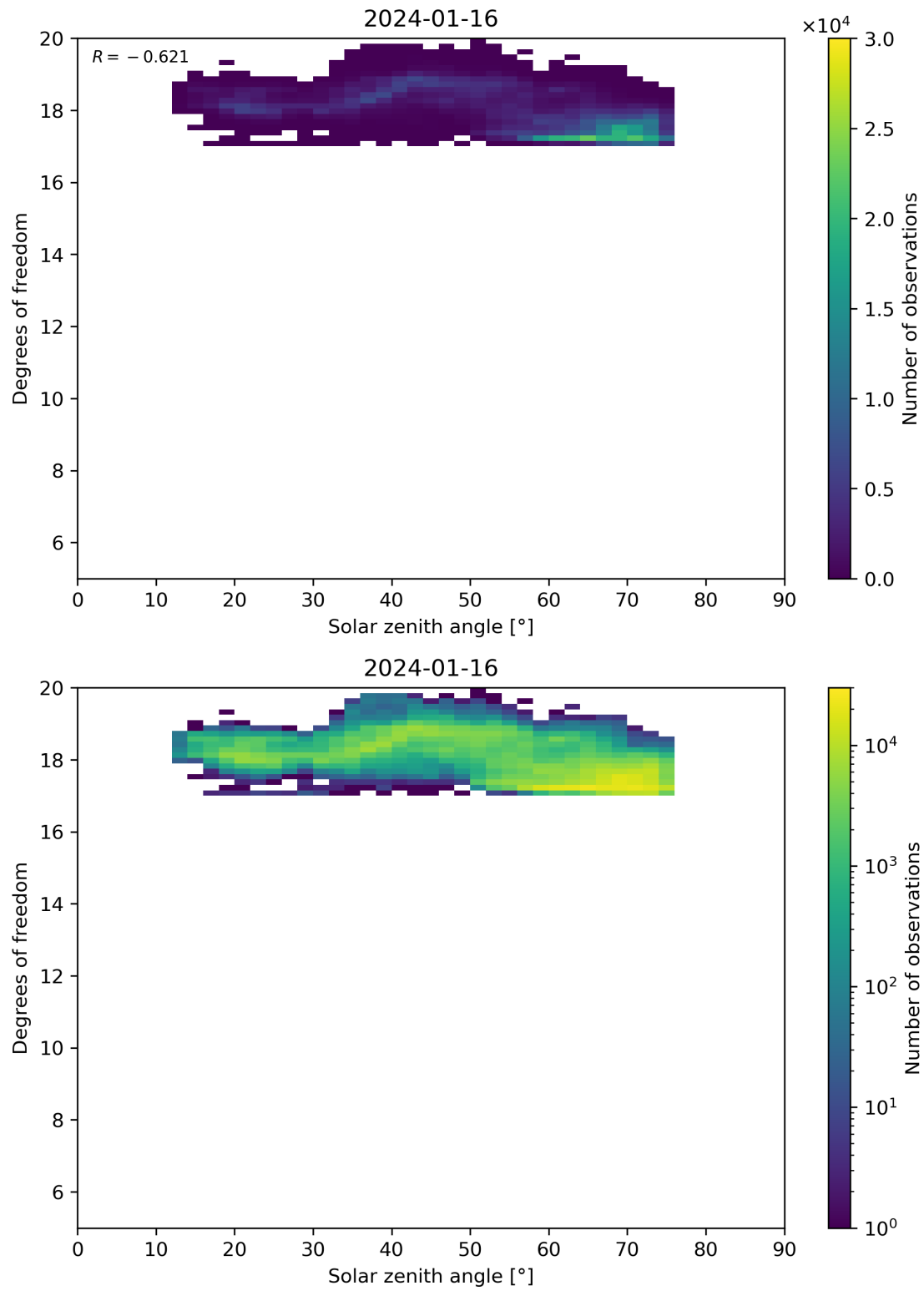
Figure 96: Scatter density plot of “Solar zenith angle” against “Degrees of freedom” for 2024-01-15 to 2024-01-17.
