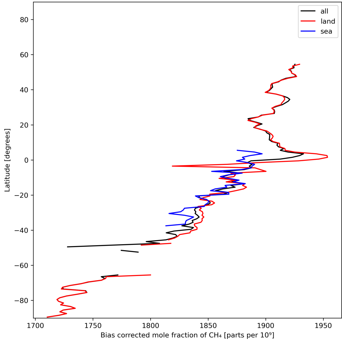
Figure 14: Zonal average of “Bias corrected mole fraction of CH 4 ” for 2024-01-16 to 2024-01-18.
