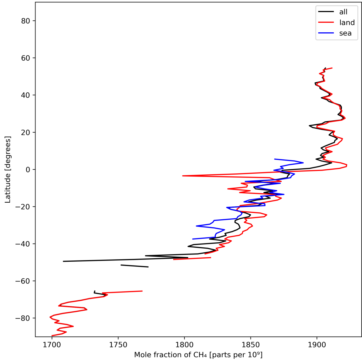
Figure 12: Zonal average of “Mole fraction of \text{CH}_4 ” for 2024-01-16 to 2024-01-18.
