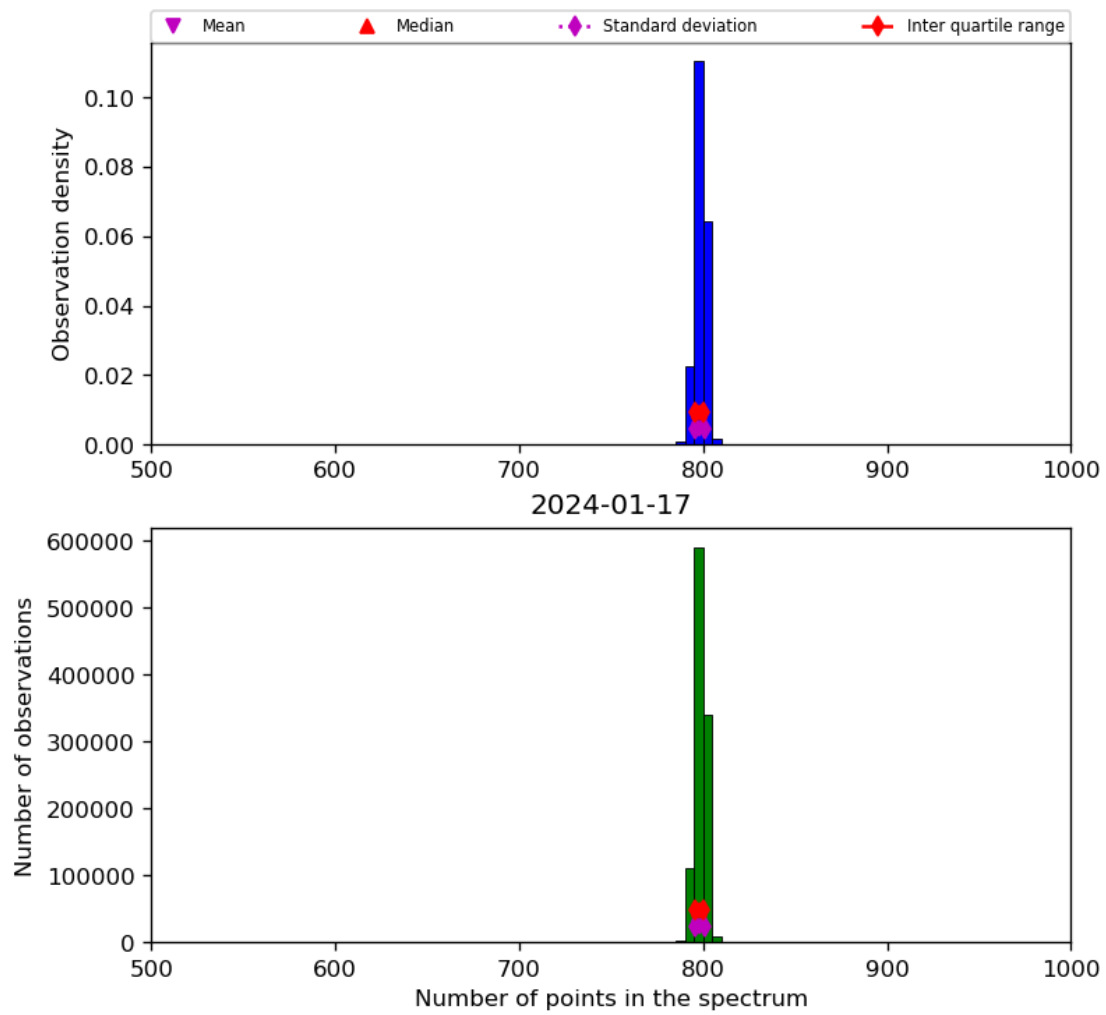
Figure 26: Histogram of “Number of points in the spectrum” for 2024-01-16 to 2024-01-18
