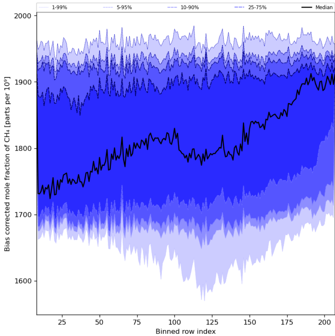
Figure 36: Along track statistics of “Bias corrected mole fraction of CH 4 ” for 2024-01-16 to 2024-01-18
