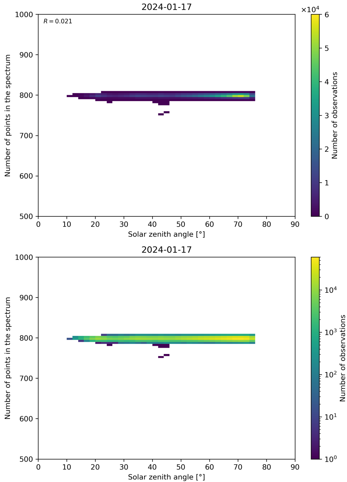
Figure 103: Scatter density plot of “Solar zenith angle” against “Number of points in the spectrum” for 2024-01-16 to 2024-01-18.
