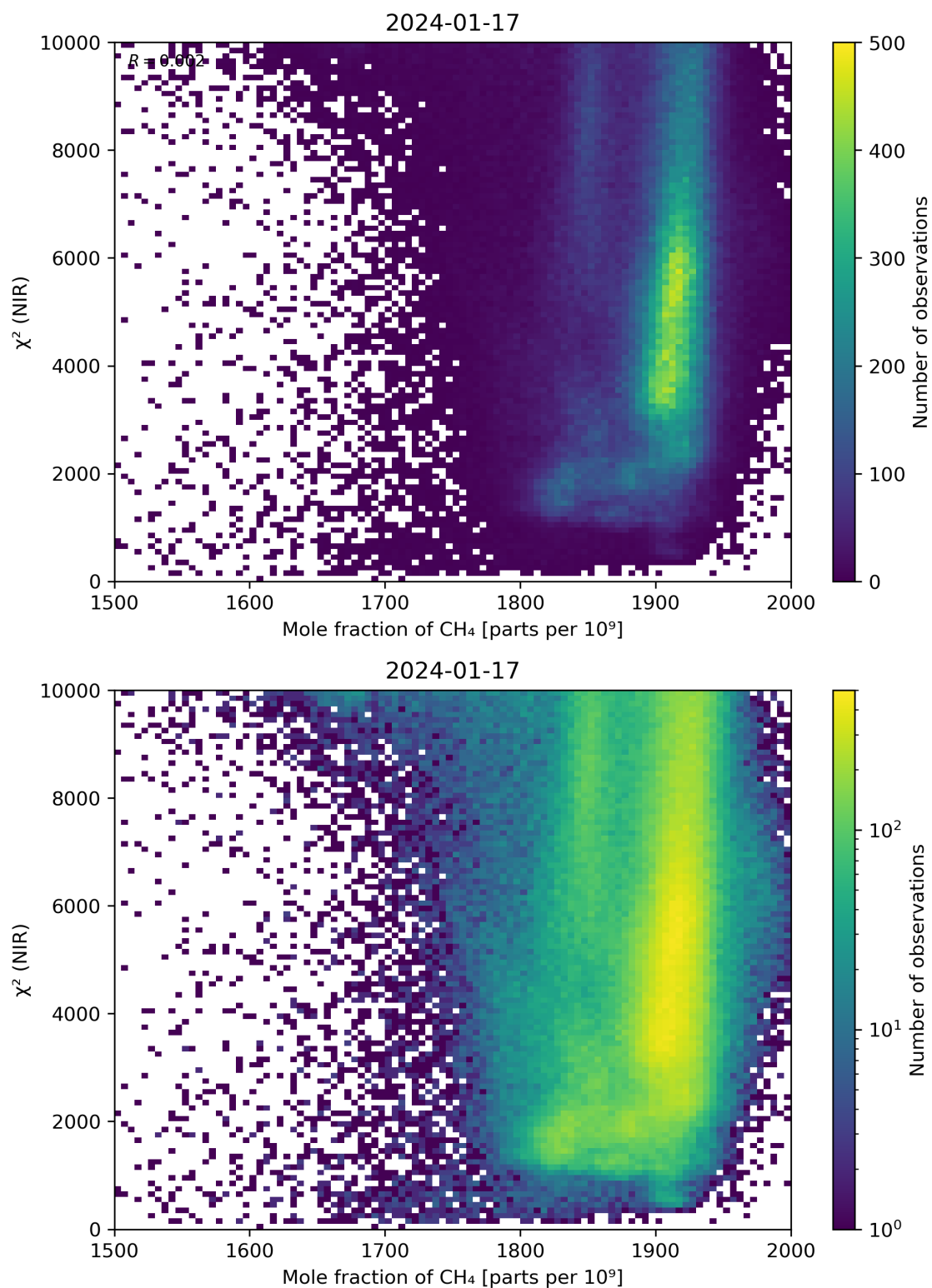
Figure 70: Scatter density plot of “Mole fraction of CH 4 ” against “ \chi^2 (NIR)” for 2024-01-16 to 2024-01-18.
