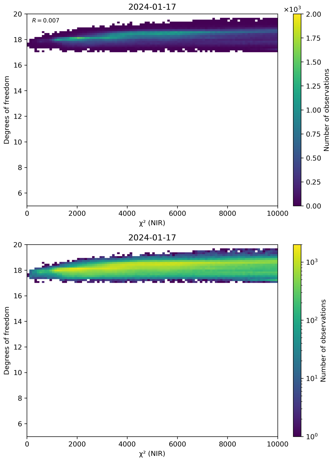
Figure 44: Scatter density plot of “ \chi^2 (NIR)” against “Degrees of freedom” for 2024-01-16 to 2024-01-18.
