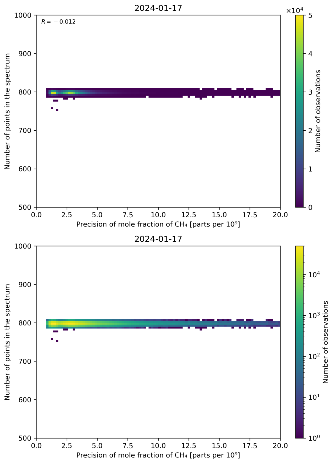
Figure 84: Scatter density plot of “Precision of mole fraction of CH 4 ” against “Number of points in the spectrum” for 2024-01-16 to 2024-01-18.
