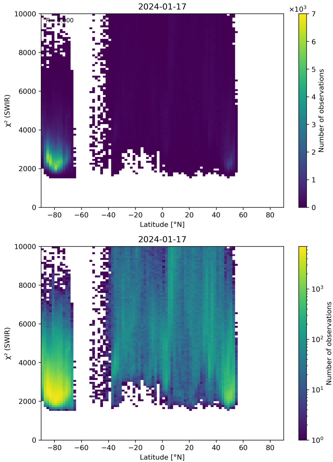
Figure 54: Scatter density plot of “Latitude” against “ \chi^2 (SWIR)” for 2024-01-16 to 2024-01-18.
