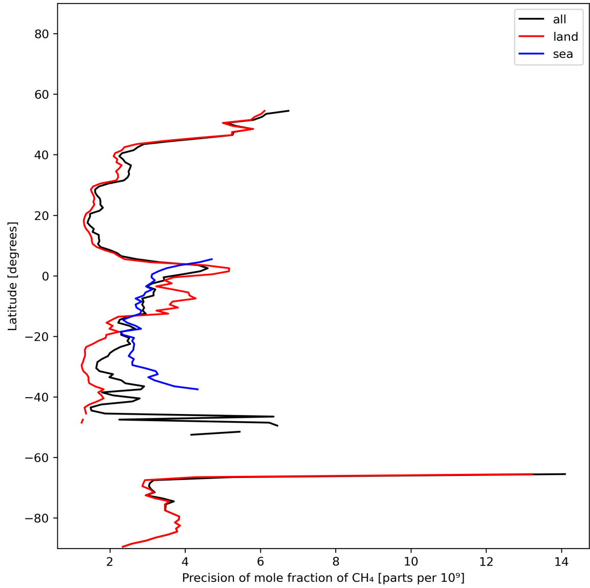
Figure 13: Zonal average of “Precision of mole fraction of CH 4 ” for 2024-01-16 to 2024-01-18.
