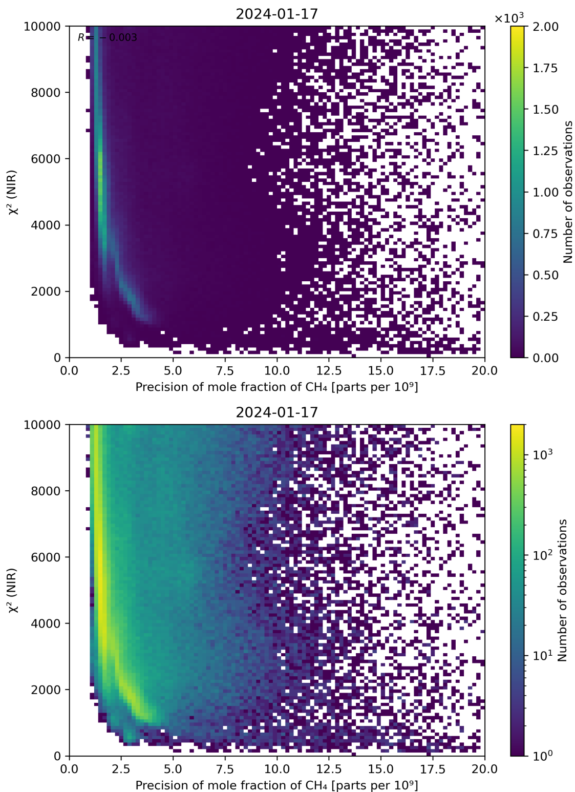
Figure 78: Scatter density plot of “Precision of mole fraction of CH 4 ” against “ \chi^2 (NIR)” for 2024-01-16 to 2024-01-18.
