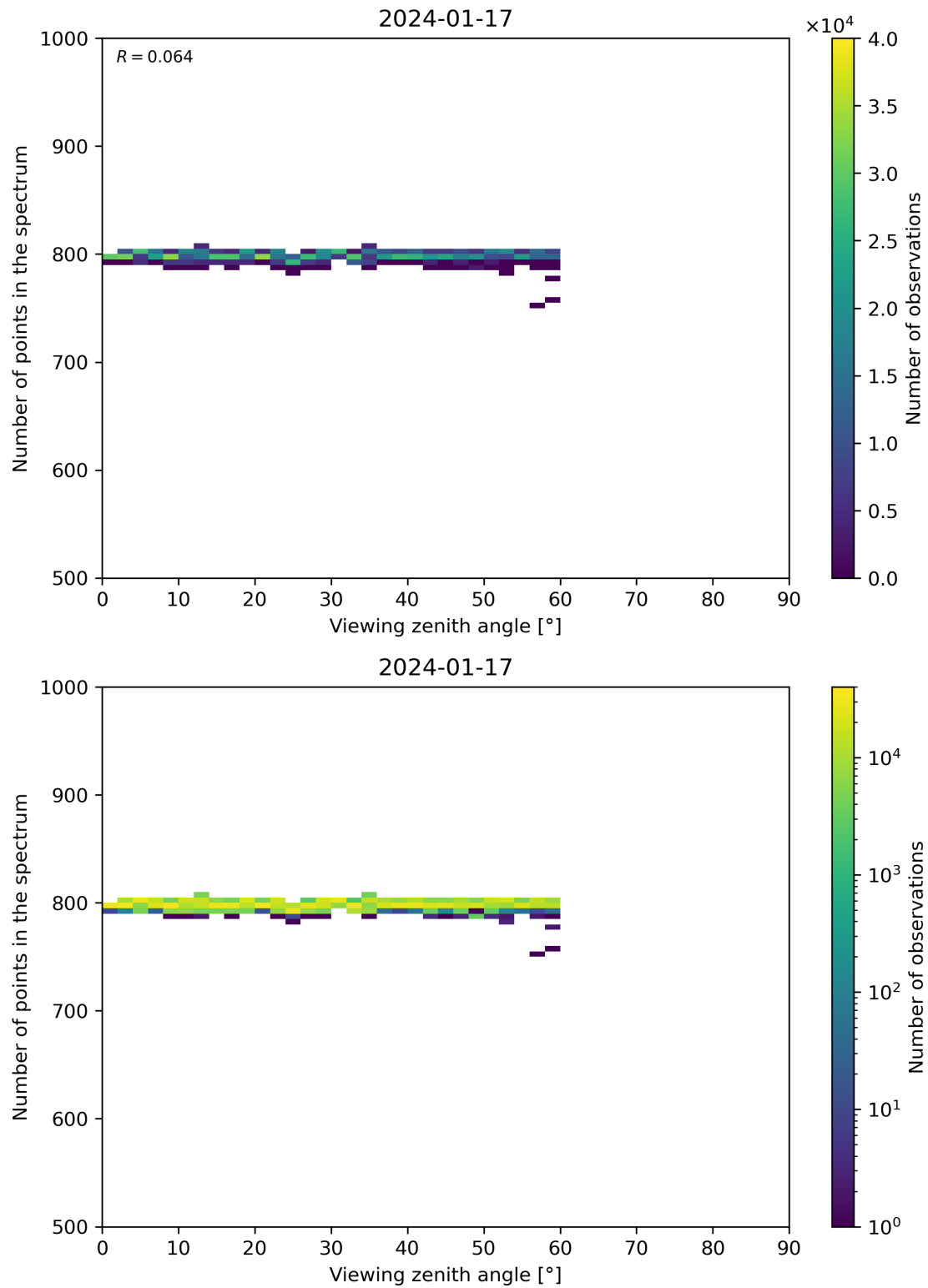
Figure 114: Scatter density plot of “Viewing zenith angle” against “Number of points in the spectrum” for 2024-01-16 to 2024-01-18.
