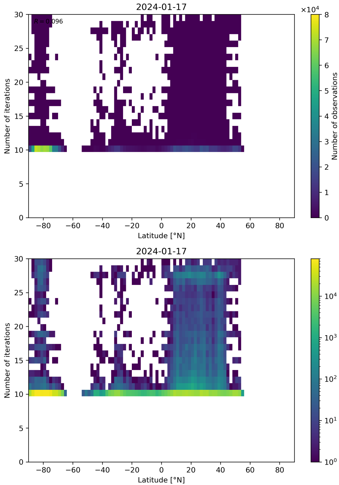
Figure 60: Scatter density plot of “Latitude” against “Number of iterations” for 2024-01-16 to 2024-01-18.
