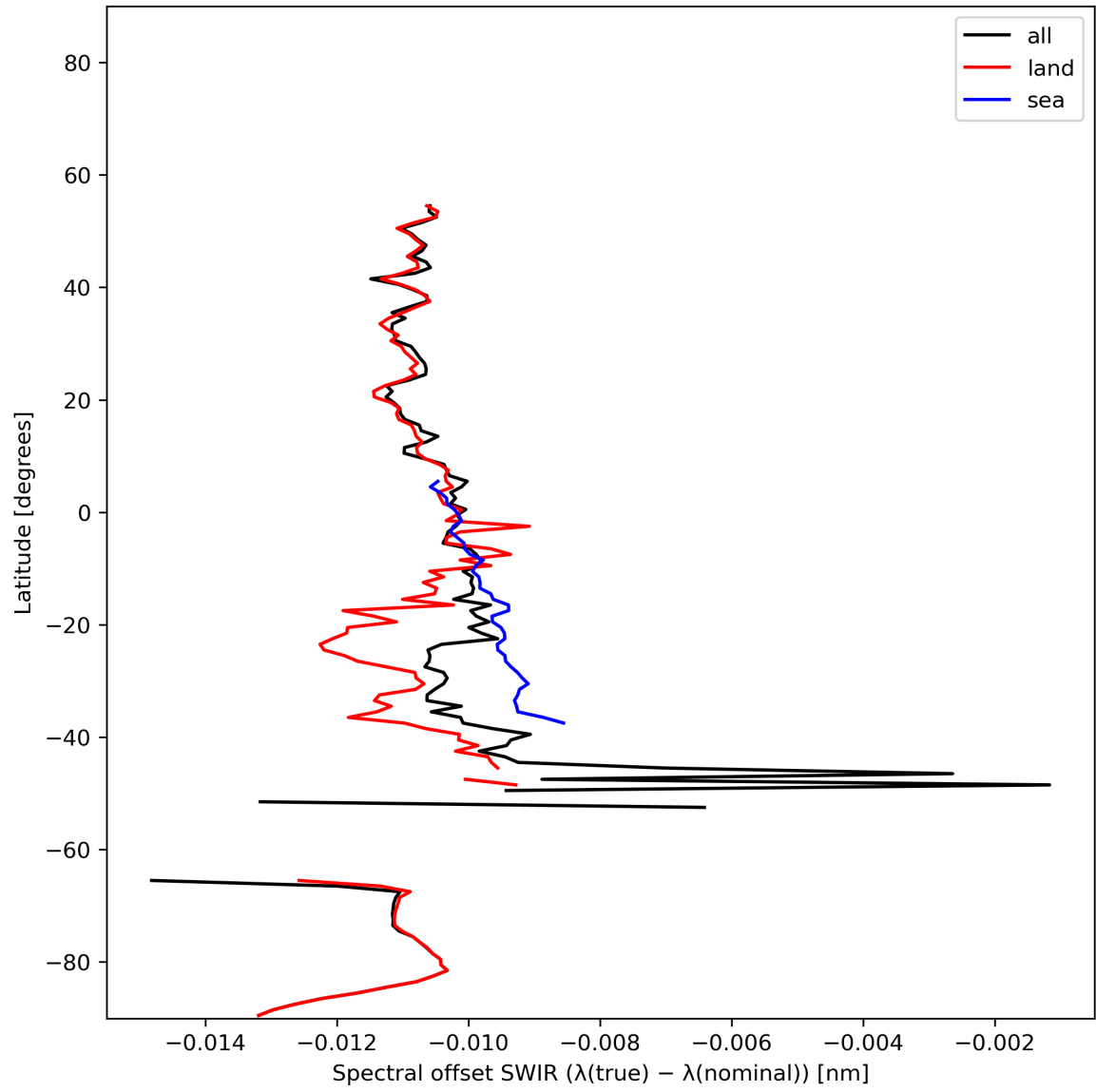
Figure 16: Zonal average of “Spectral offset SWIR ( \lambda(\text{true}) - \lambda(\text{nominal}) )” for 2024-01-16 to 2024-01-18.
