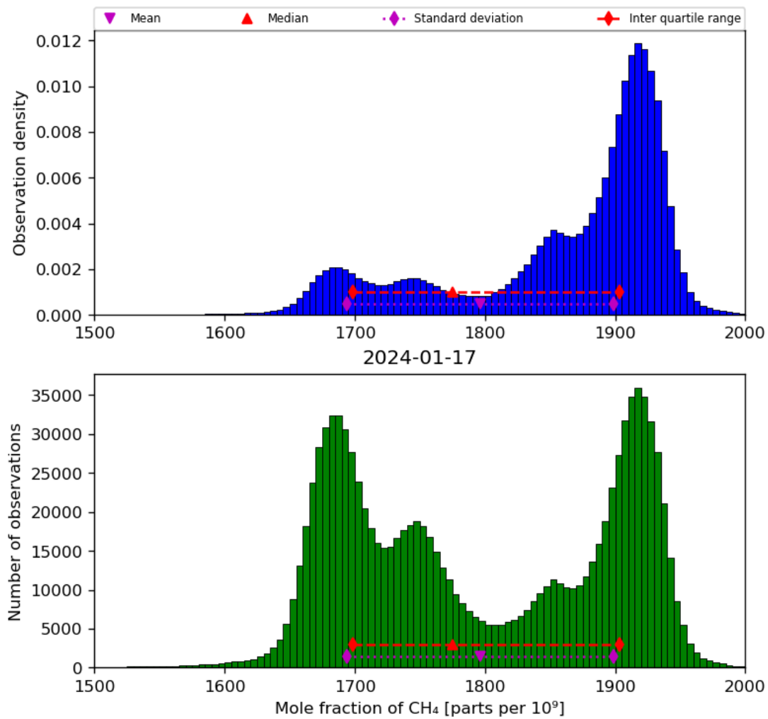
Figure 23: Histogram of “Mole fraction of CH 4 ” for 2024-01-16 to 2024-01-18
