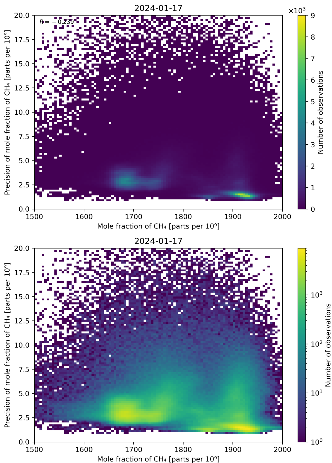
Figure 75: Scatter density plot of “Mole fraction of CH 4 ” against “Precision of mole fraction of CH 4 ” for 2024-01-16 to 2024-01-18.
