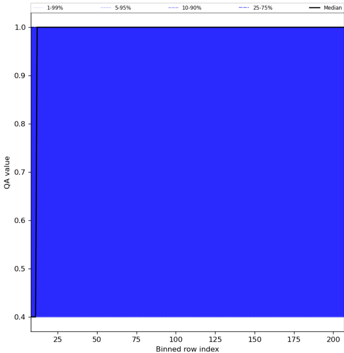
Figure 33: Along track statistics of “QA value” for 2024-01-16 to 2024-01-18
