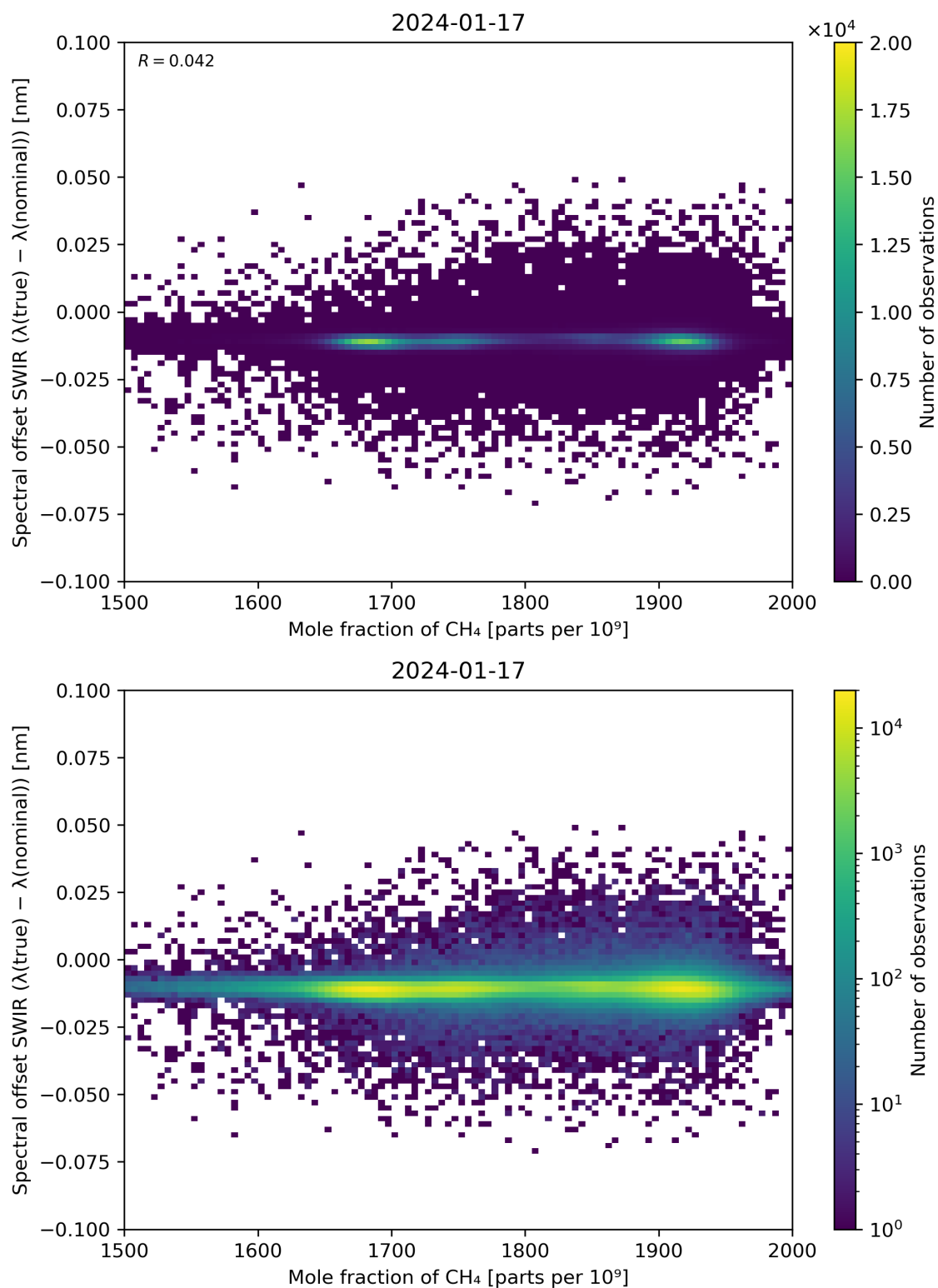
Figure 86: Scatter density plot of “Mole fraction of CH 4 ” against “Spectral offset SWIR ( \lambda(\text{true}) - \lambda(\text{nominal}) )” for 2024-01-16 to 2024-01-18.
