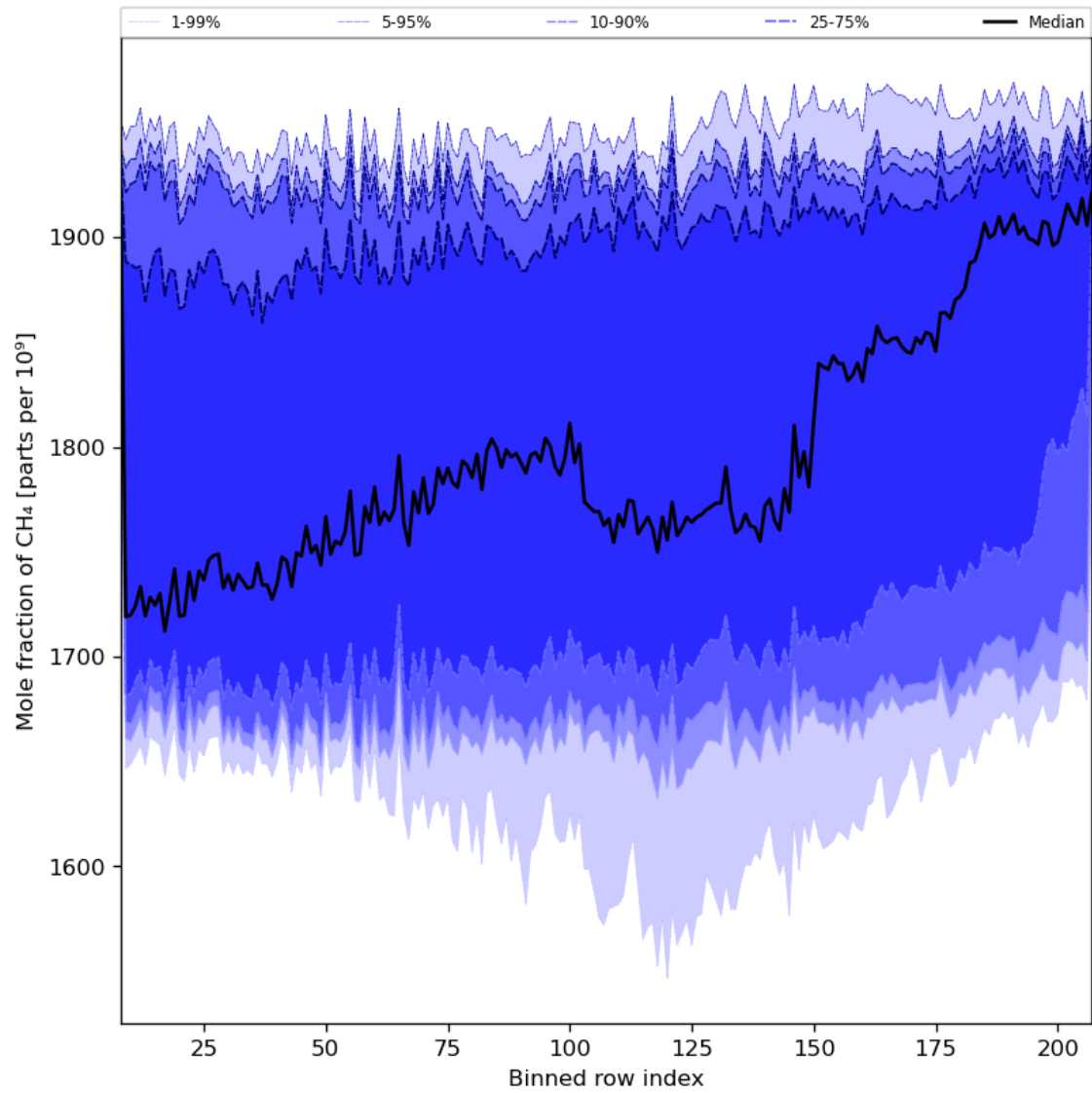
Figure 34: Along track statistics of “Mole fraction of CH 4 ” for 2024-01-16 to 2024-01-18
