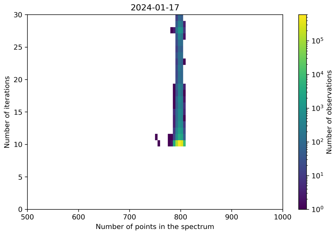
Figure 92: Scatter density plot of “Number of points in the spectrum” against “Number of iterations” for 2024-01-16 to 2024-01-18.
