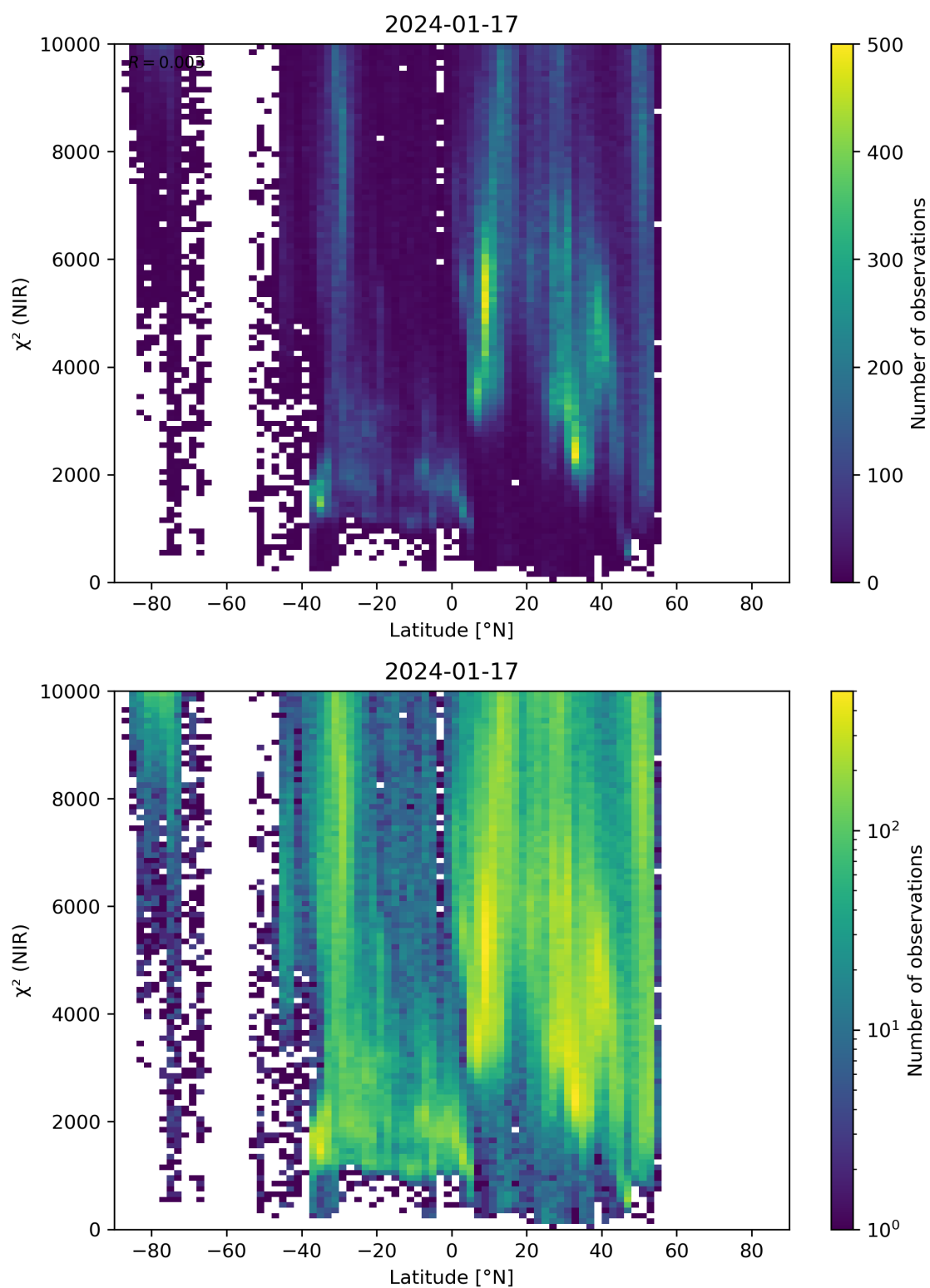
Figure 53: Scatter density plot of “Latitude” against “ \chi^2 (NIR)” for 2024-01-16 to 2024-01-18.
