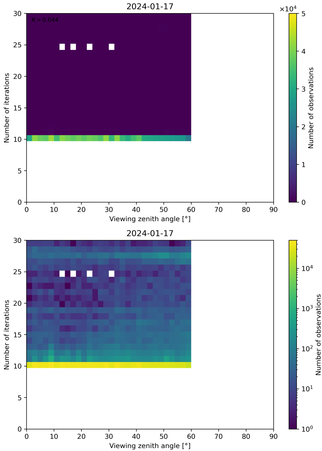
Figure 113: Scatter density plot of “Viewing zenith angle” against “Number of iterations” for 2024-01-16 to 2024-01-18.
