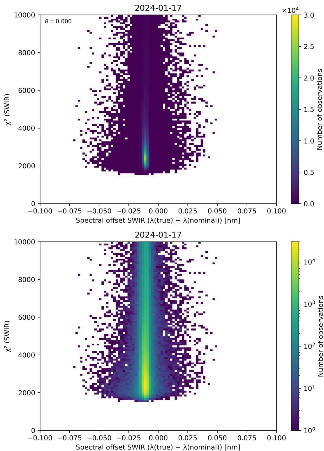
Figure 118: Scatter density plot of “Spectral offset SWIR ( \lambda(\text{true}) - \lambda(\text{nominal}) )” against “ \chi^2 (SWIR)” for 2024-01-16 to 2024-01-18.
