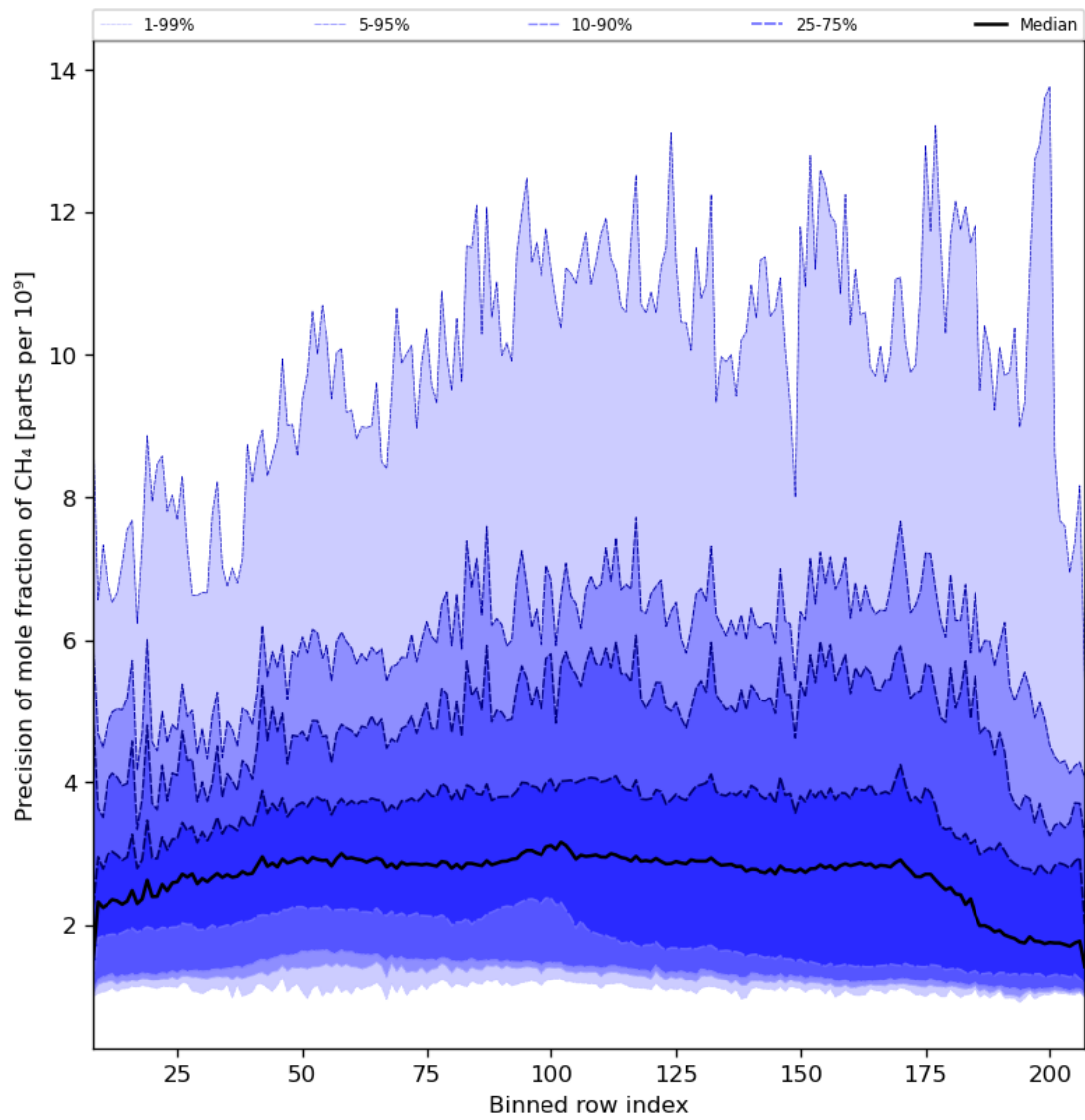
Figure 35: Along track statistics of “Precision of mole fraction of CH 4 ” for 2024-01-16 to 2024-01-18
