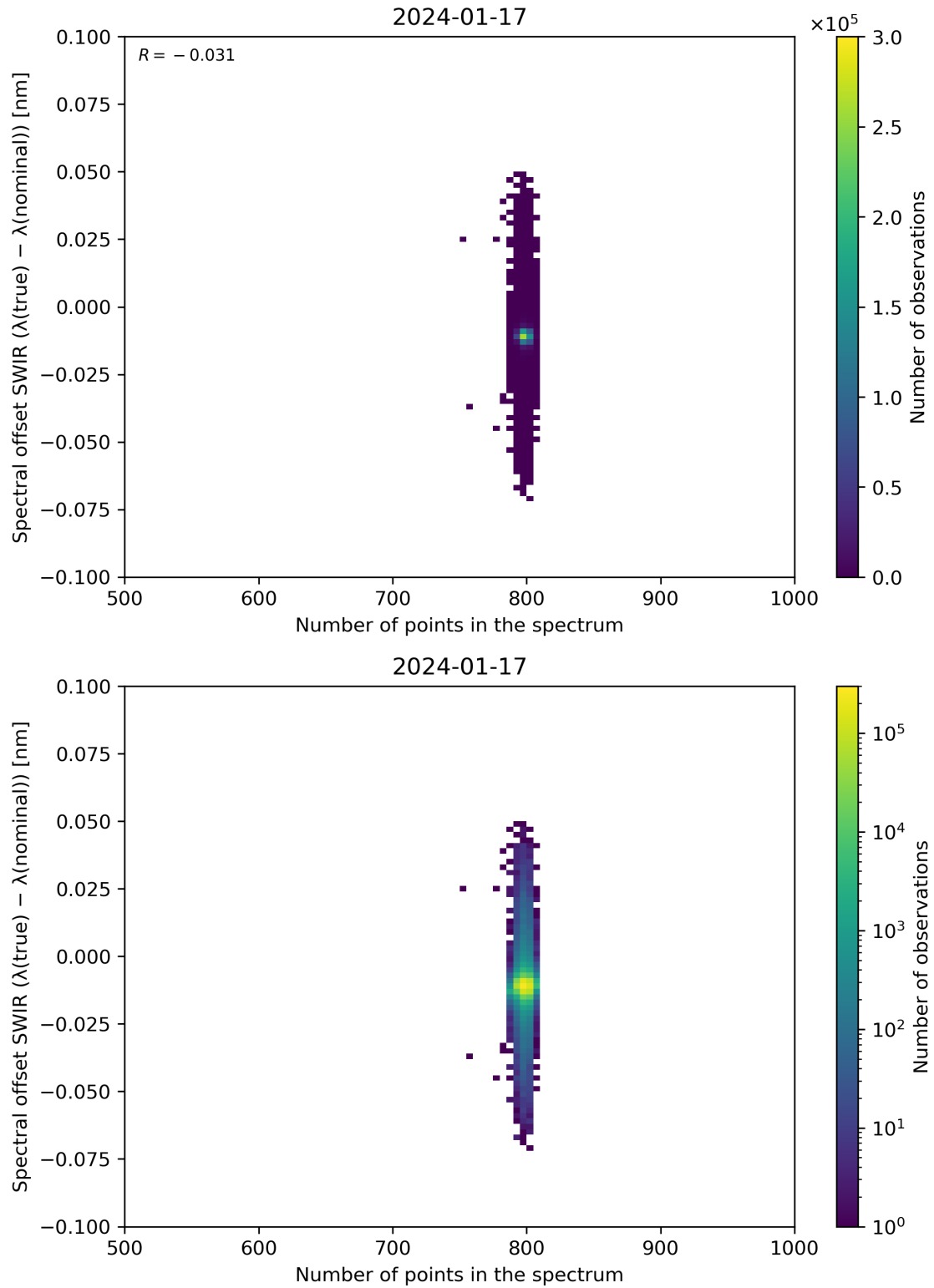
Figure 93: Scatter density plot of “Number of points in the spectrum” against “Spectral offset SWIR ( \lambda(\text{true}) - \lambda(\text{nominal}) )” for 2024-01-16 to 2024-01-18.
