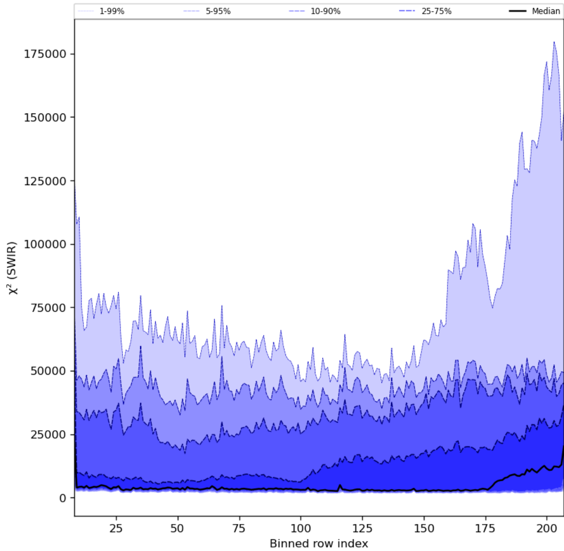
Figure 39: Along track statistics of “ \chi^2 (SWIR)” for 2024-01-16 to 2024-01-18
