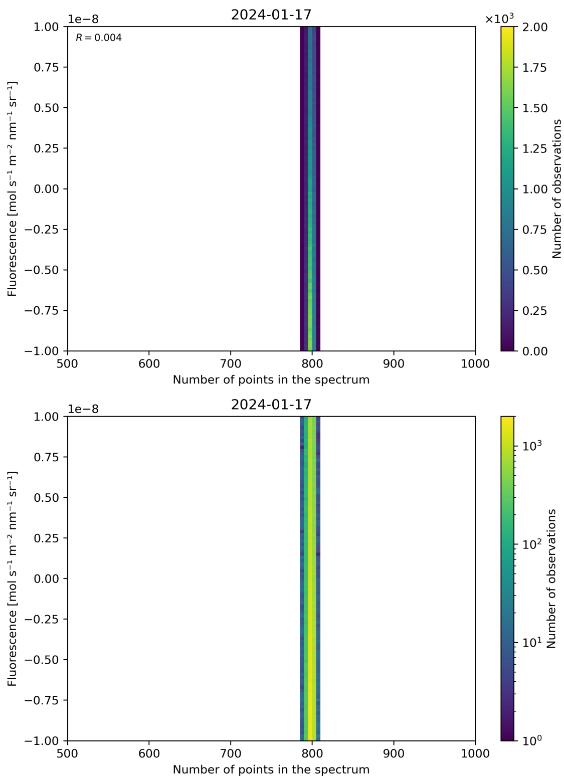
Figure 91: Scatter density plot of “Number of points in the spectrum” against “Fluorescence” for 2024-01-16 to 2024-01-18.
