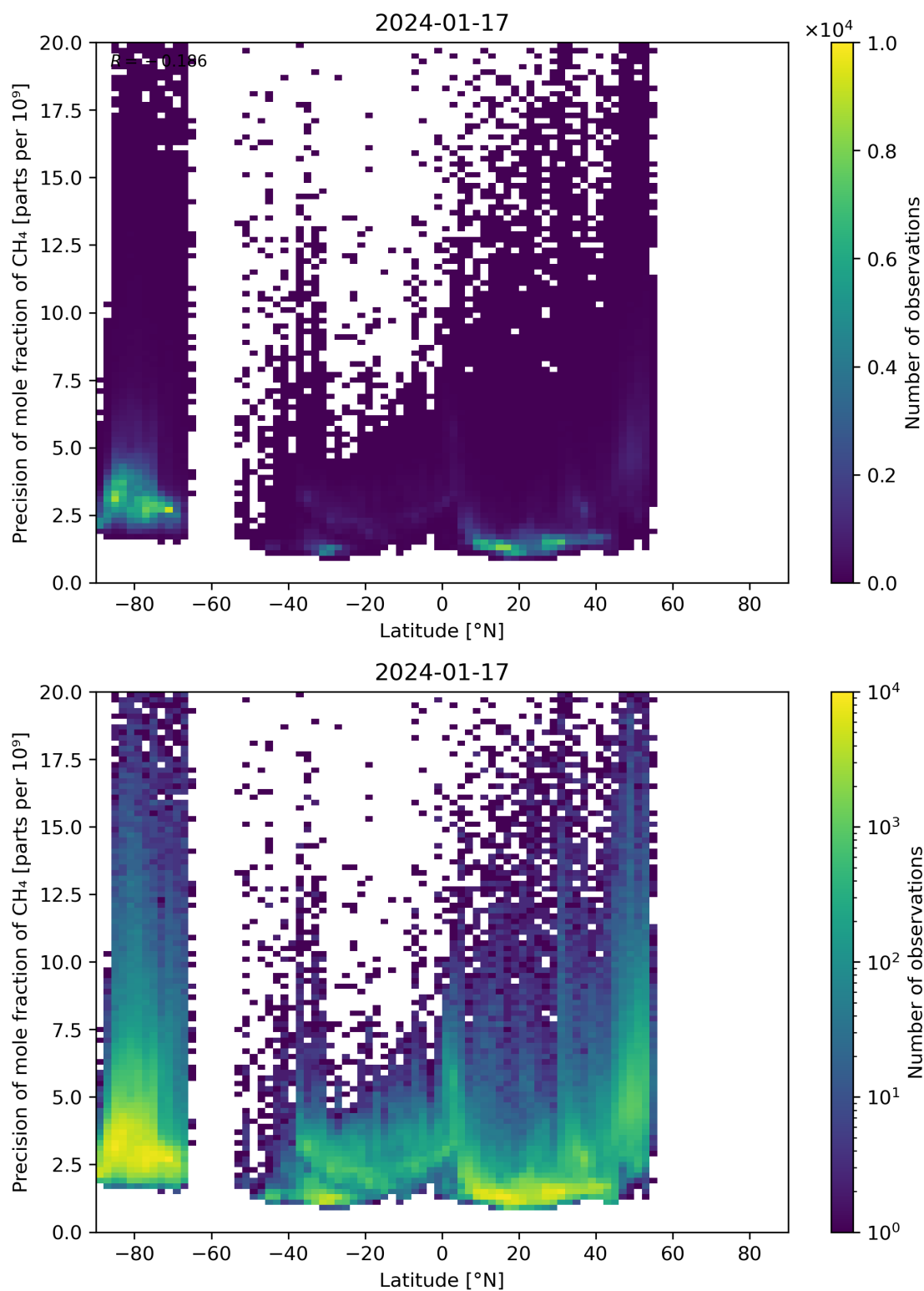
Figure 59: Scatter density plot of “Latitude” against “Precision of mole fraction of CH 4 ” for 2024-01-16 to 2024-01-18.
