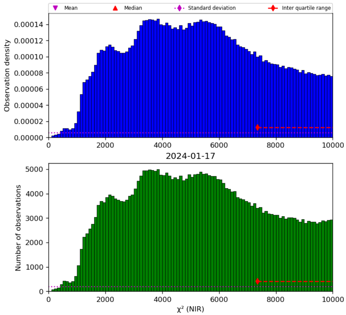
Figure 29: Histogram of “ \chi^2 (NIR)” for 2024-01-16 to 2024-01-18
