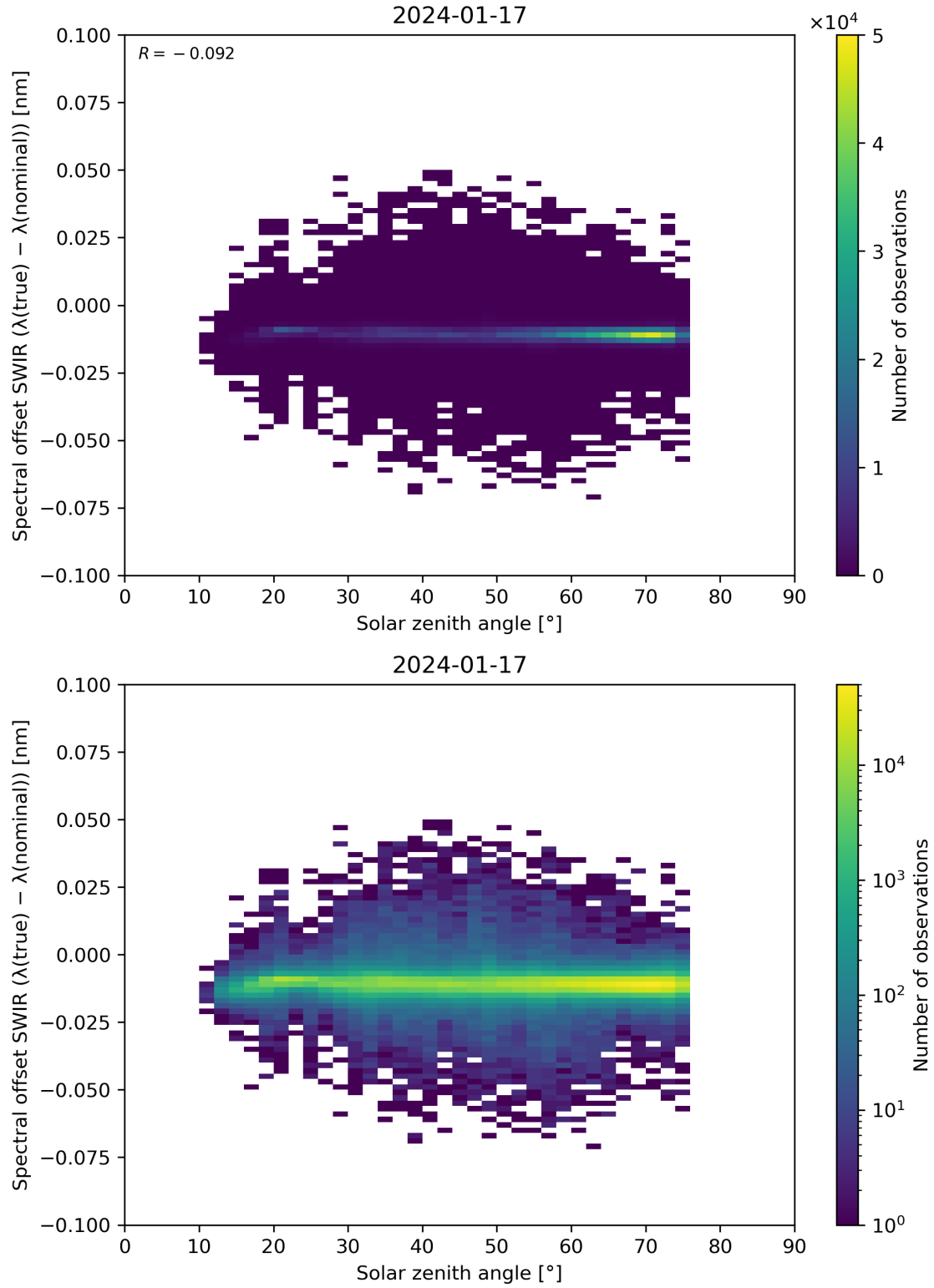
Figure 104: Scatter density plot of “Solar zenith angle” against “Spectral offset SWIR ( \lambda(\text{true}) - \lambda(\text{nominal}) )” for 2024-01-16 to 2024-01-18.
