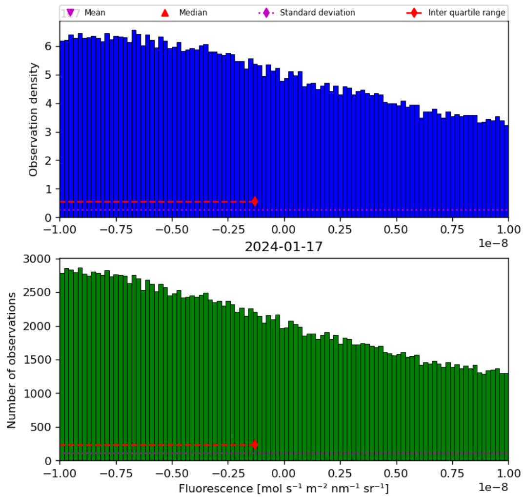
Figure 32: Histogram of “Fluorescence” for 2024-01-16 to 2024-01-18
