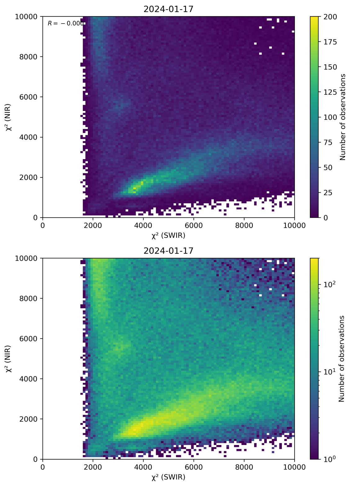
Figure 47: Scatter density plot of “ \chi^2 (SWIR)” against “ \chi^2 (NIR)” for 2024-01-16 to 2024-01-18.
