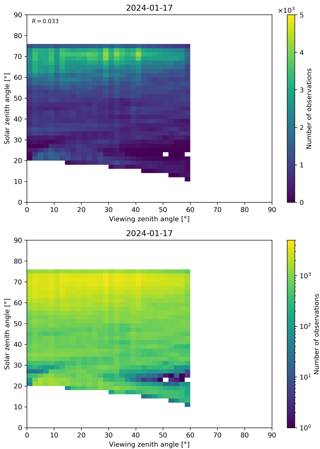
Figure 115: Scatter density plot of “Viewing zenith angle” against “Solar zenith angle” for 2024-01-16 to 2024-01-18.
