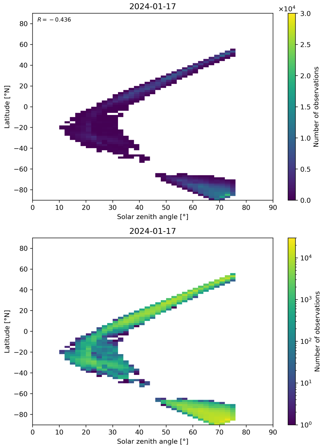
Figure 98: Scatter density plot of “Solar zenith angle” against “Latitude” for 2024-01-16 to 2024-01-18.
