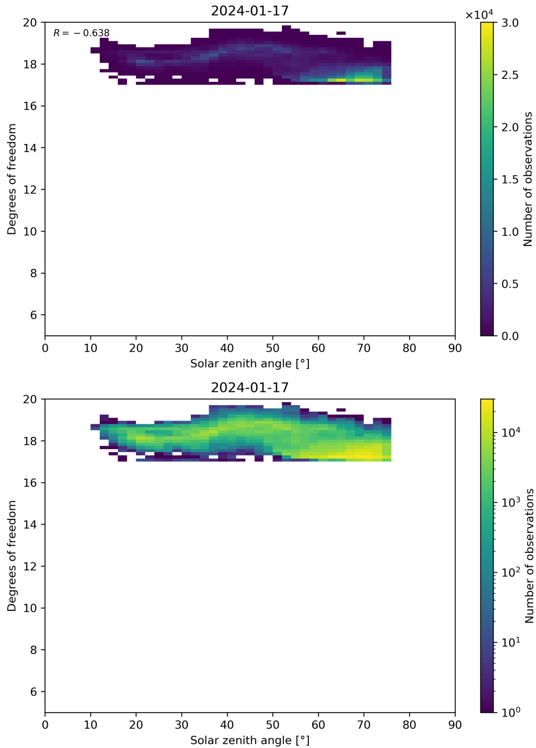
Figure 96: Scatter density plot of “Solar zenith angle” against “Degrees of freedom” for 2024-01-16 to 2024-01-18.
