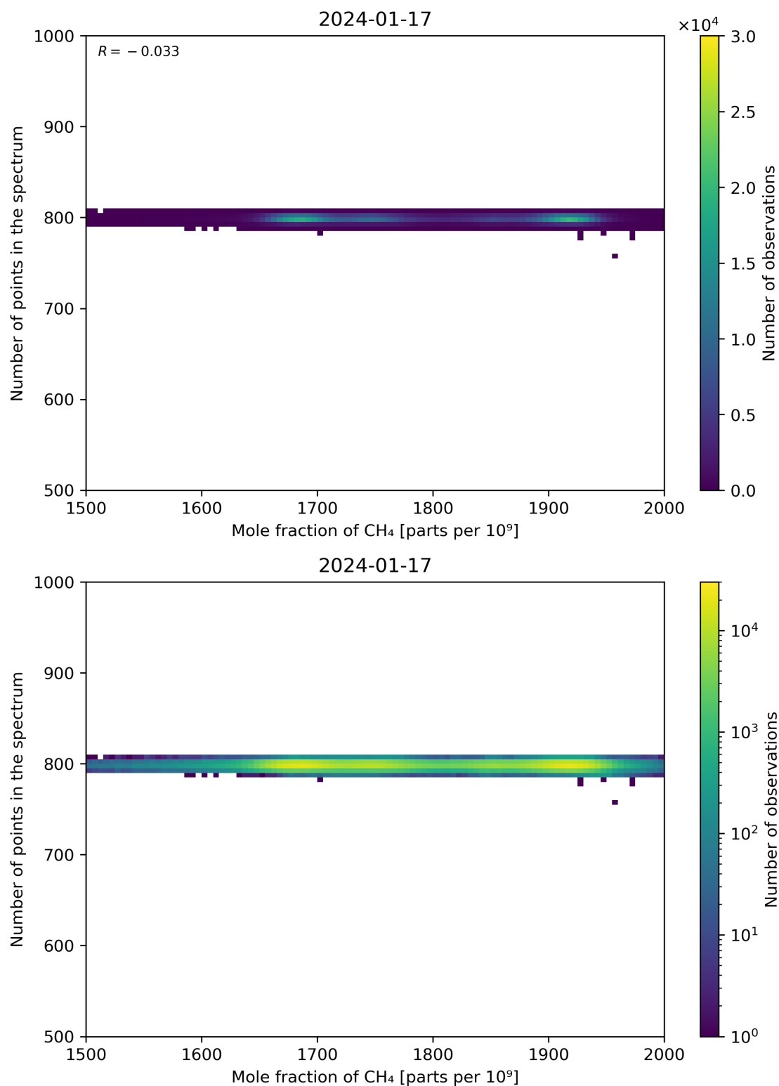
Figure 77: Scatter density plot of “Mole fraction of CH 4 ” against “Number of points in the spectrum” for 2024-01-16 to 2024-01-18.
