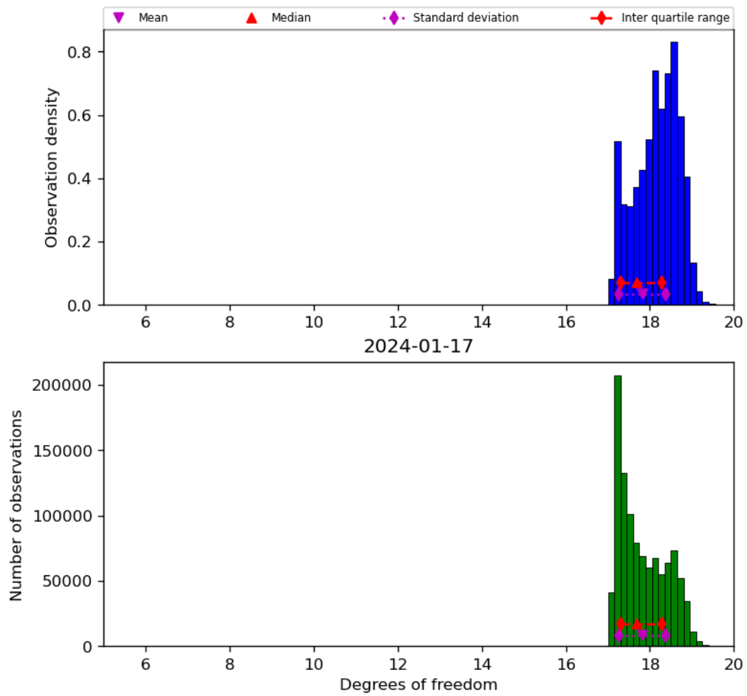
Figure 30: Histogram of “Degrees of freedom” for 2024-01-16 to 2024-01-18
