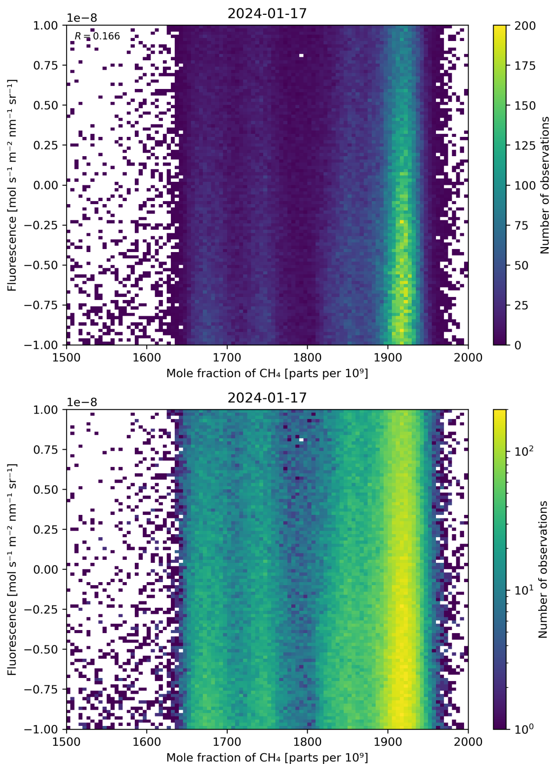
Figure 73: Scatter density plot of “Mole fraction of \text{CH}_4 ” against “Fluorescence” for 2024-01-16 to 2024-01-18.
