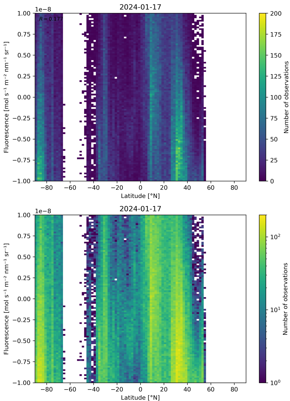
Figure 56: Scatter density plot of “Latitude” against “Fluorescence” for 2024-01-16 to 2024-01-18.
