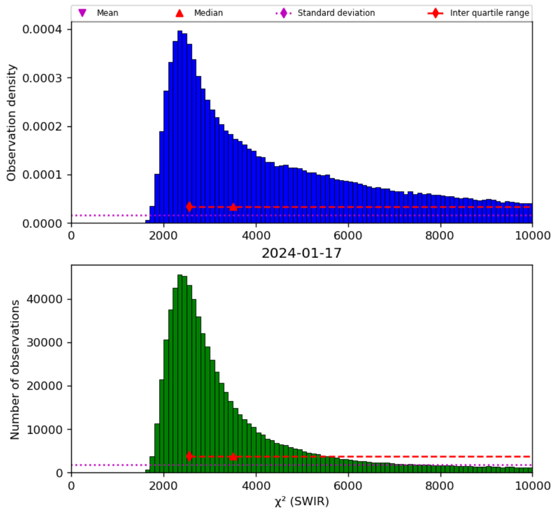
Figure 28: Histogram of “ \chi^2 (SWIR)” for 2024-01-16 to 2024-01-18
