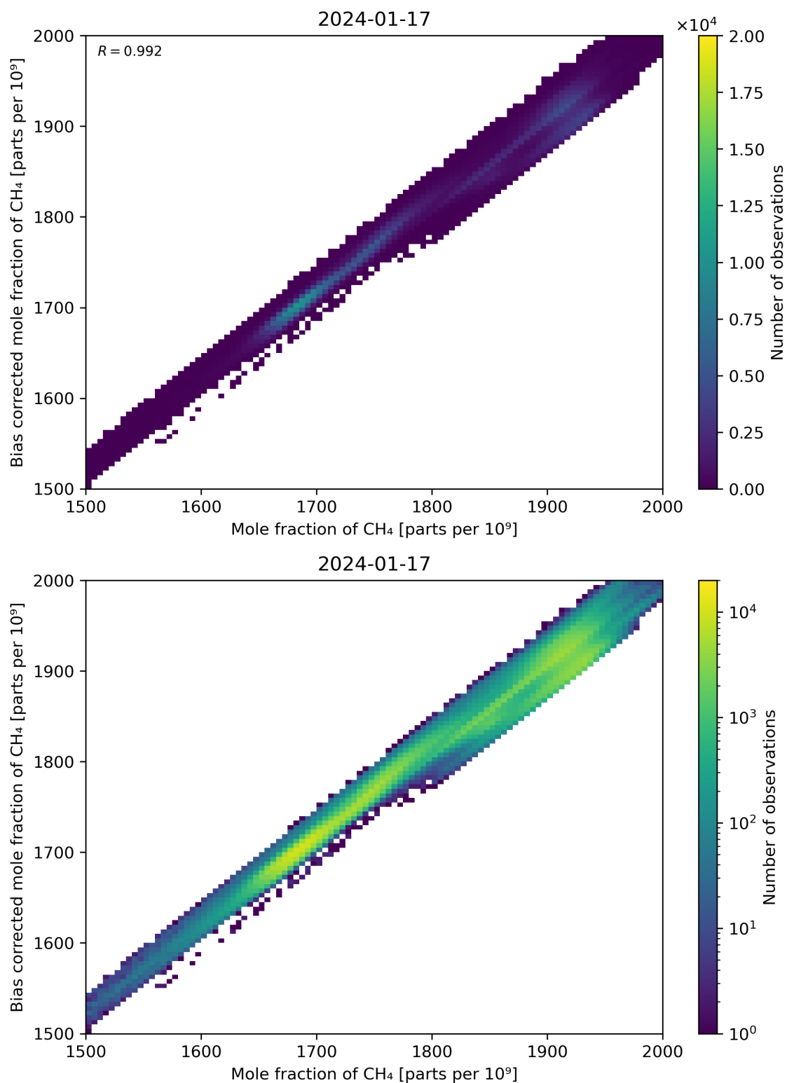
Figure 74: Scatter density plot of “Mole fraction of CH 4 ” against “Bias corrected mole fraction of CH 4 ” for 2024-01-16 to 2024-01-18.
