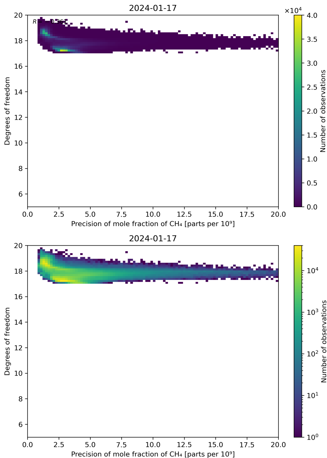
Figure 80: Scatter density plot of “Precision of mole fraction of CH 4 ” against “Degrees of freedom” for 2024-01-16 to 2024-01-18.
