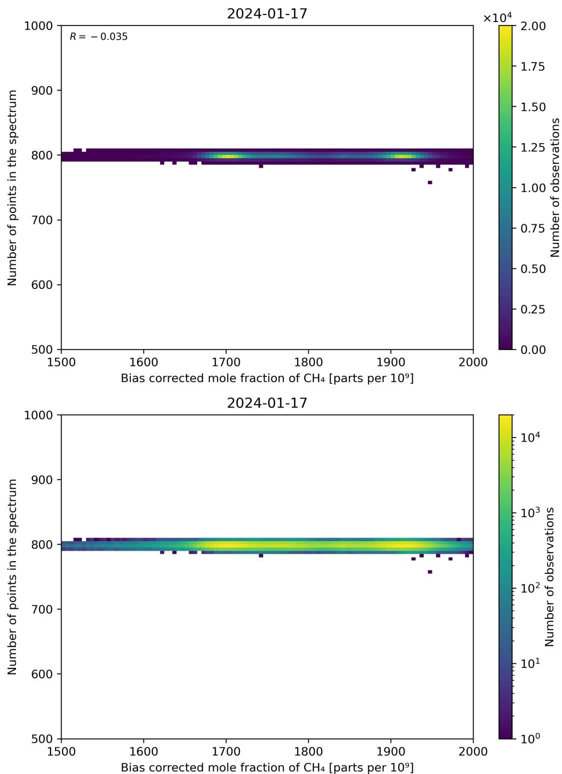
Figure 68: Scatter density plot of “Bias corrected mole fraction of CH 4 ” against “Number of points in the spectrum” for 2024-01-16 to 2024-01-18.
