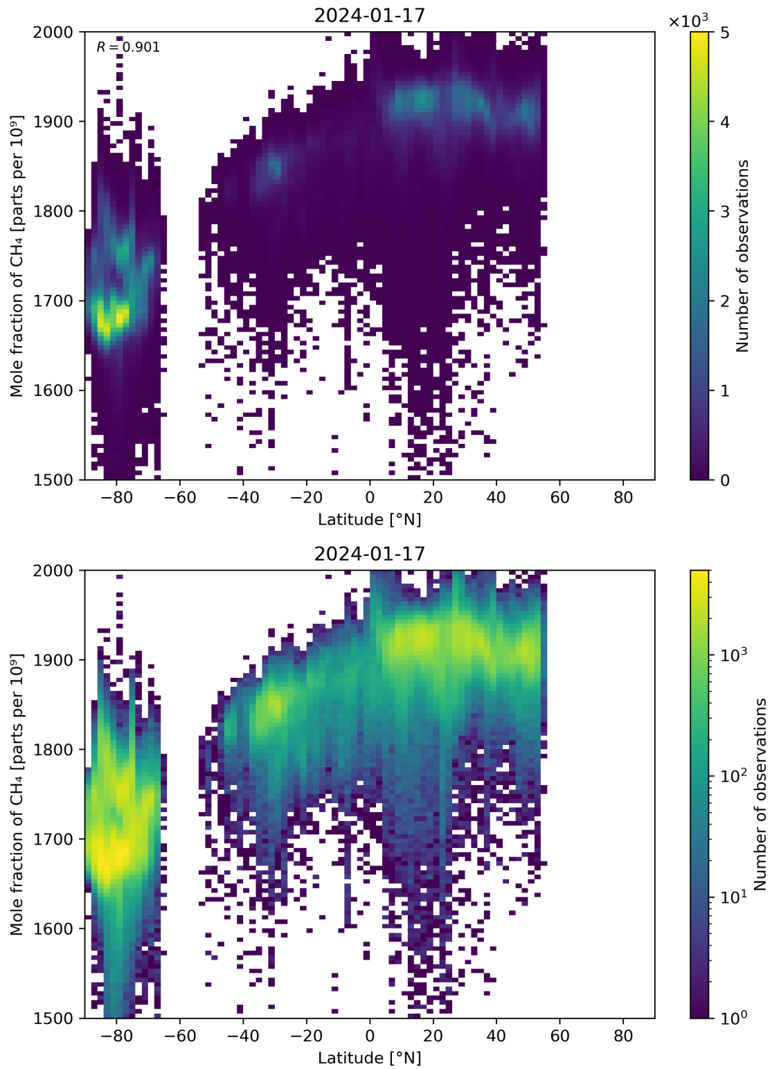
Figure 57: Scatter density plot of “Latitude” against “Mole fraction of \text{CH}_4 ” for 2024-01-16 to 2024-01-18.
