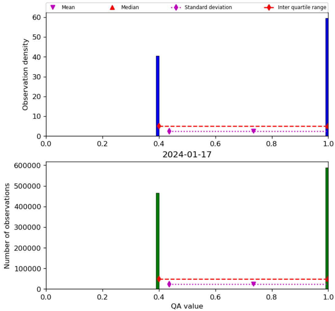
Figure 22: Histogram of “QA value” for 2024-01-16 to 2024-01-18
