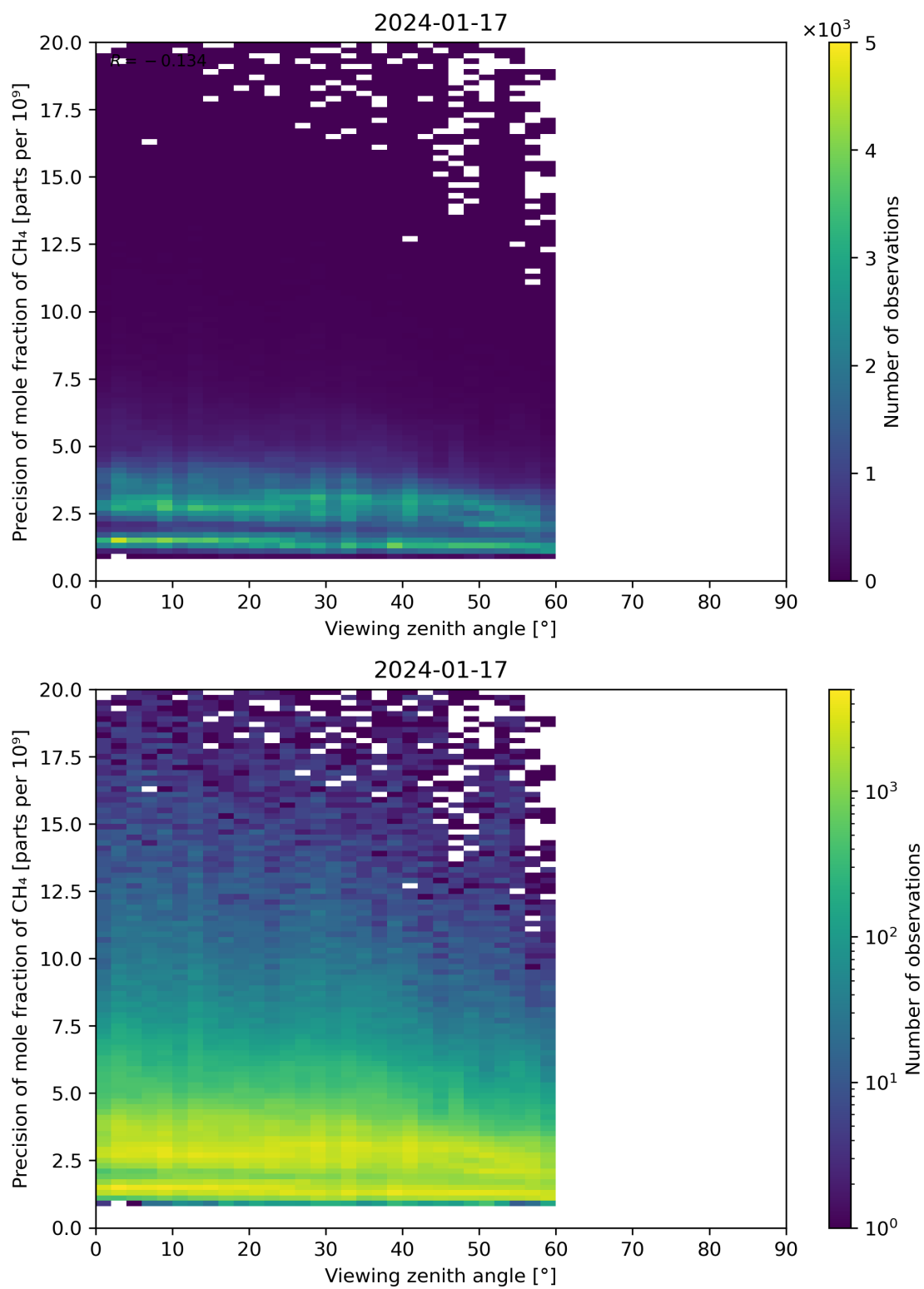
Figure 112: Scatter density plot of “Viewing zenith angle” against “Precision of mole fraction of CH 4 ” for 2024-01-16 to 2024-01-18.
