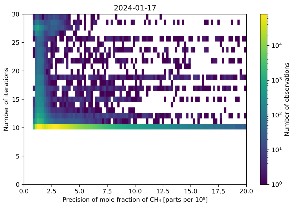
Figure 83: Scatter density plot of “Precision of mole fraction of CH 4 ” against “Number of iterations” for 2024-01-16 to 2024-01-18.
