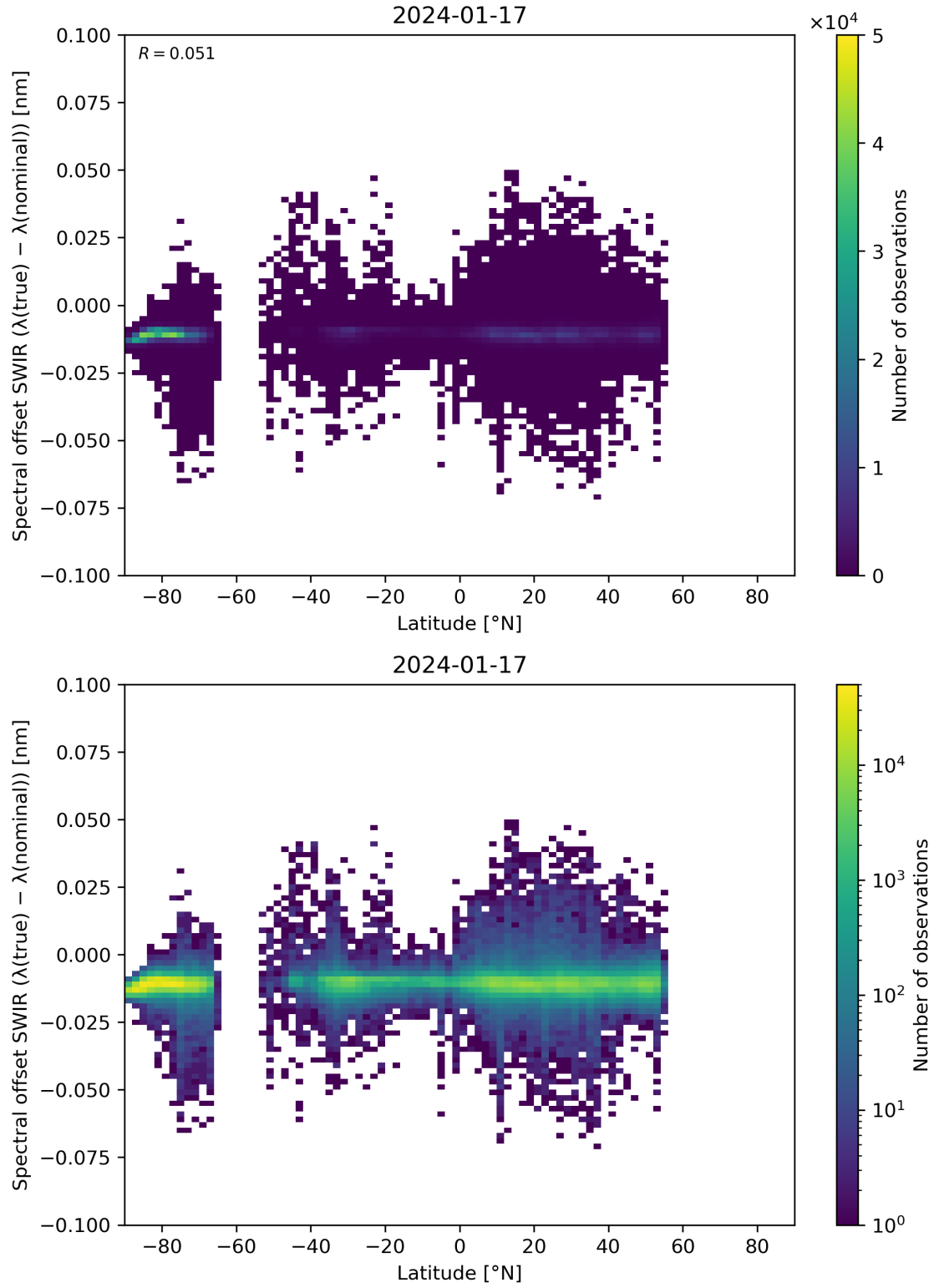
Figure 62: Scatter density plot of “Latitude” against “Spectral offset SWIR ( \lambda(\text{true}) - \lambda(\text{nominal}) )” for 2024-01-16 to 2024-01-18.
