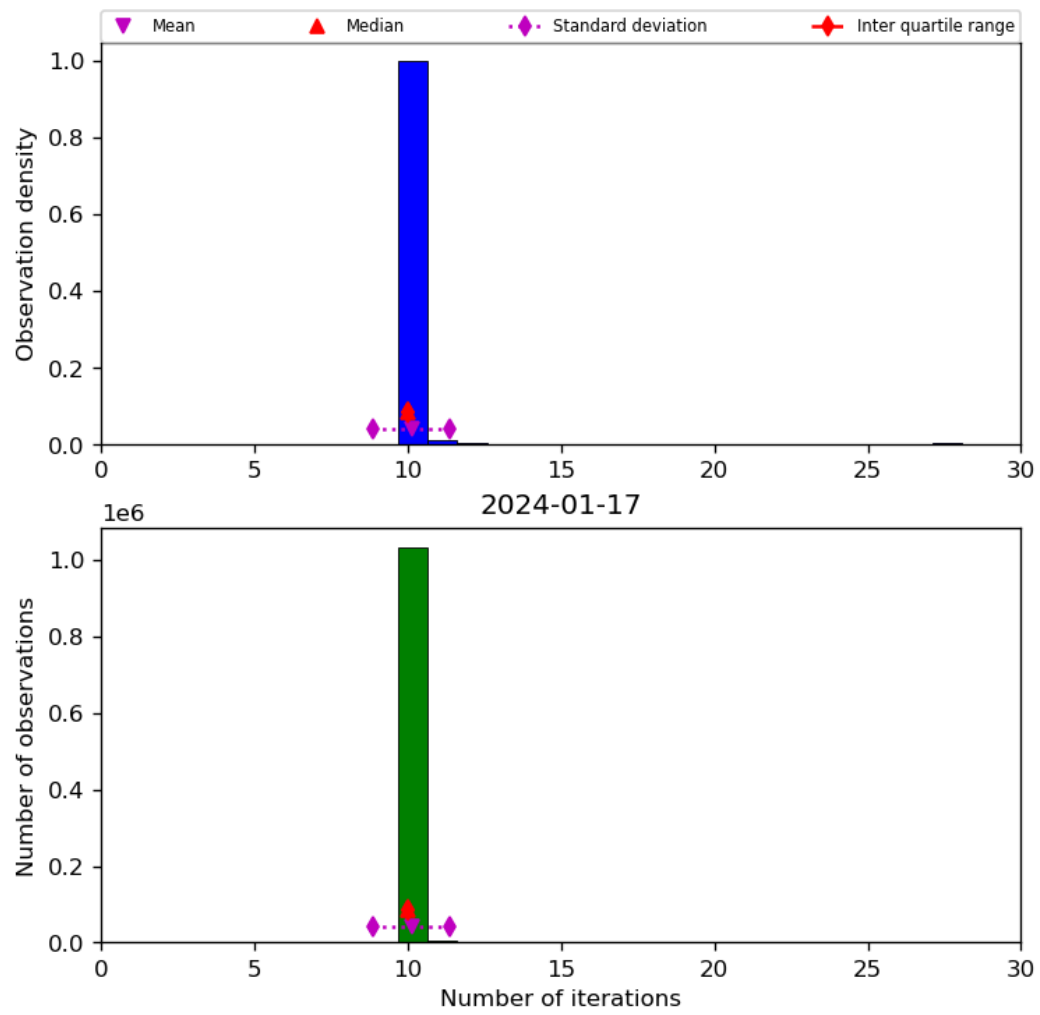
Figure 31: Histogram of “Number of iterations” for 2024-01-16 to 2024-01-18
