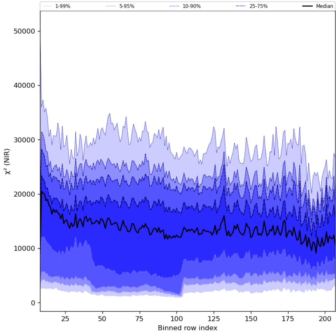
Figure 40: Along track statistics of “ \chi^2 (NIR)” for 2024-01-16 to 2024-01-18
