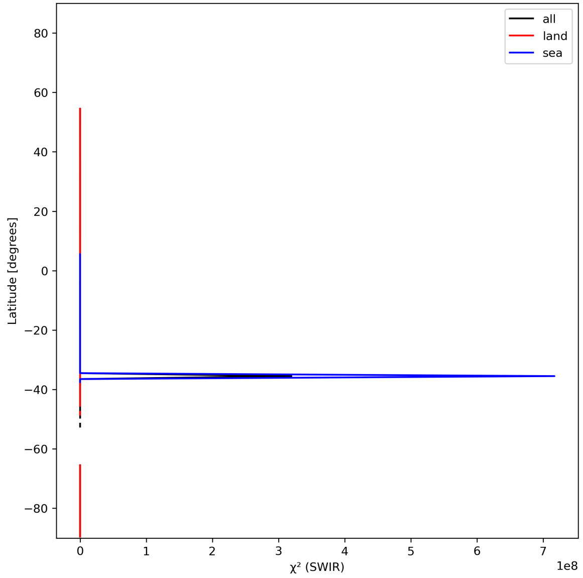
Figure 17: Zonal average of “ \chi^2 (SWIR)” for 2024-01-16 to 2024-01-18.
