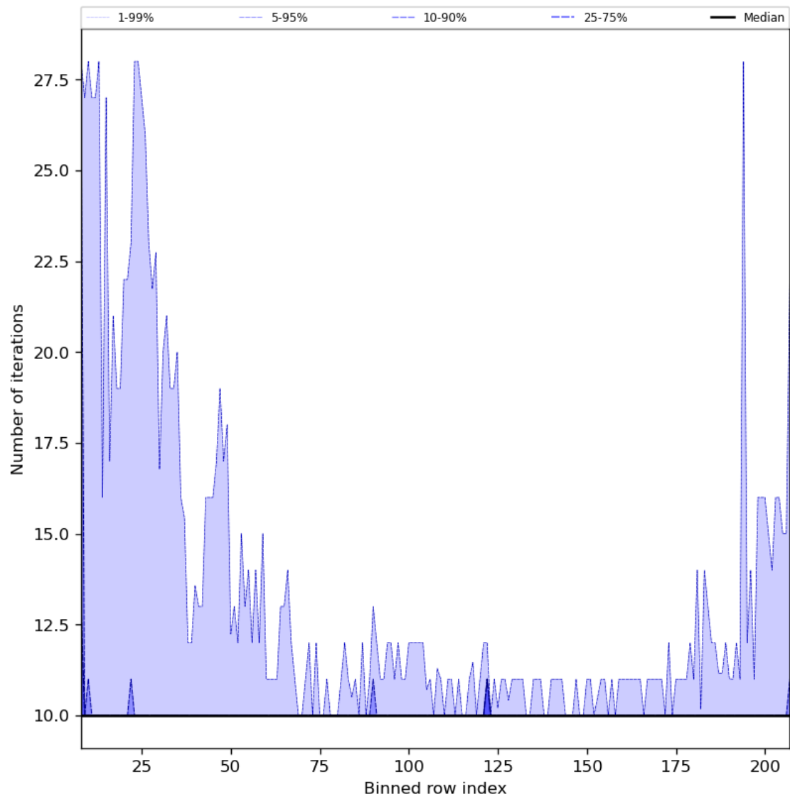
Figure 42: Along track statistics of “Number of iterations” for 2024-01-16 to 2024-01-18
