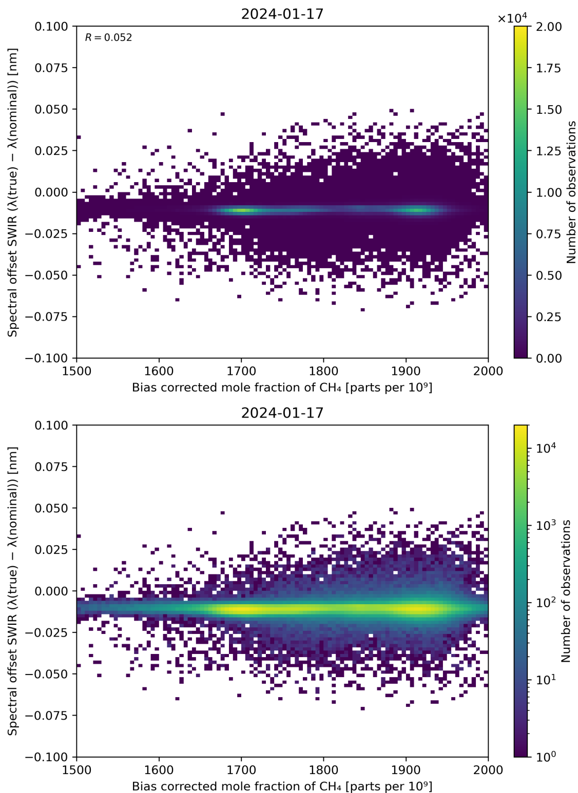
Figure 69: Scatter density plot of “Bias corrected mole fraction of \text{CH}_4 ” against “Spectral offset SWIR ( \lambda(\text{true}) - \lambda(\text{nominal}) )” for 2024-01-16 to 2024-01-18.
