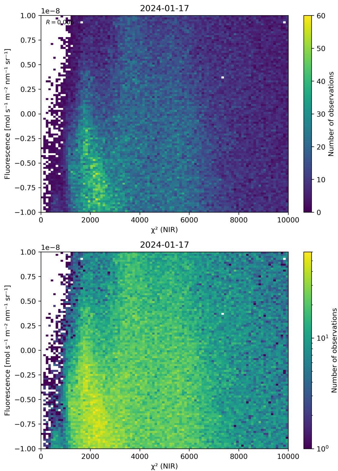
Figure 45: Scatter density plot of “ \chi^2 (NIR)” against “Fluorescence” for 2024-01-16 to 2024-01-18.
