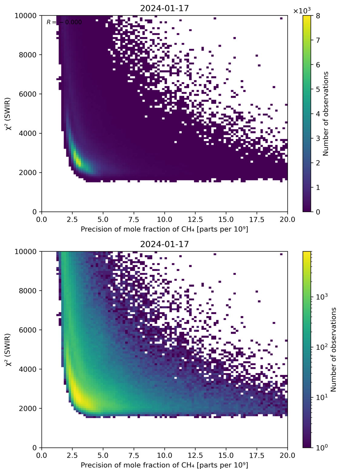
Figure 79: Scatter density plot of “Precision of mole fraction of CH 4 ” against “ \chi^2 (SWIR)” for 2024-01-16 to 2024-01-18.
