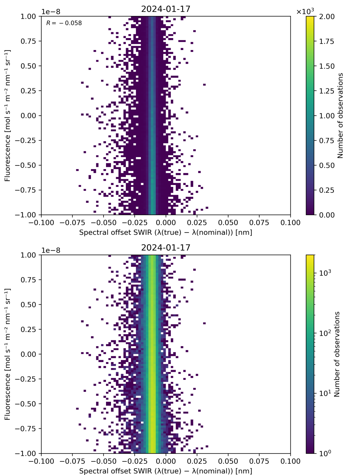
Figure 120: Scatter density plot of “Spectral offset SWIR ( \lambda(\text{true}) - \lambda(\text{nominal}) )” against “Fluorescence” for 2024-01-16 to 2024-01-18.
