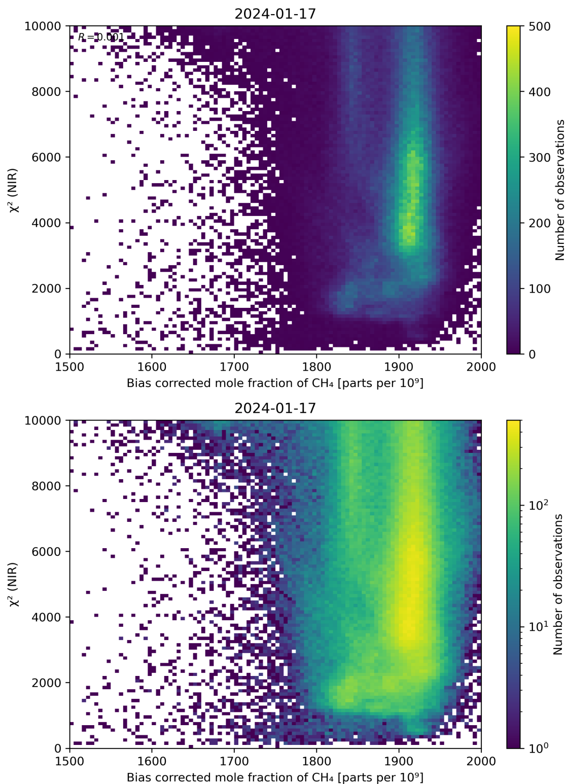
Figure 63: Scatter density plot of “Bias corrected mole fraction of CH 4 ” against “ \chi^2 (NIR)” for 2024-01-16 to 2024-01-18.
