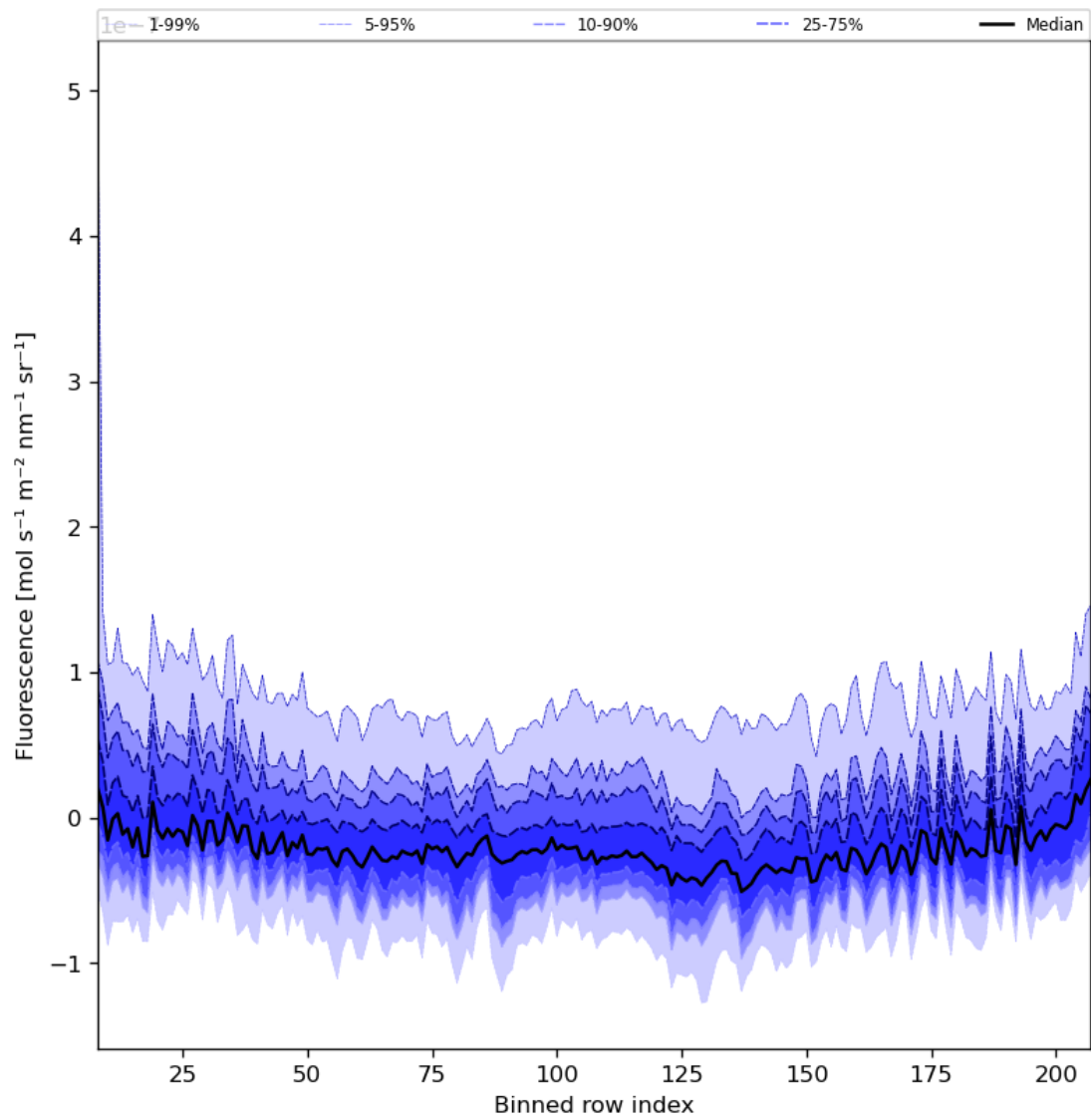
Figure 43: Along track statistics of “Fluorescence” for 2024-01-16 to 2024-01-18
