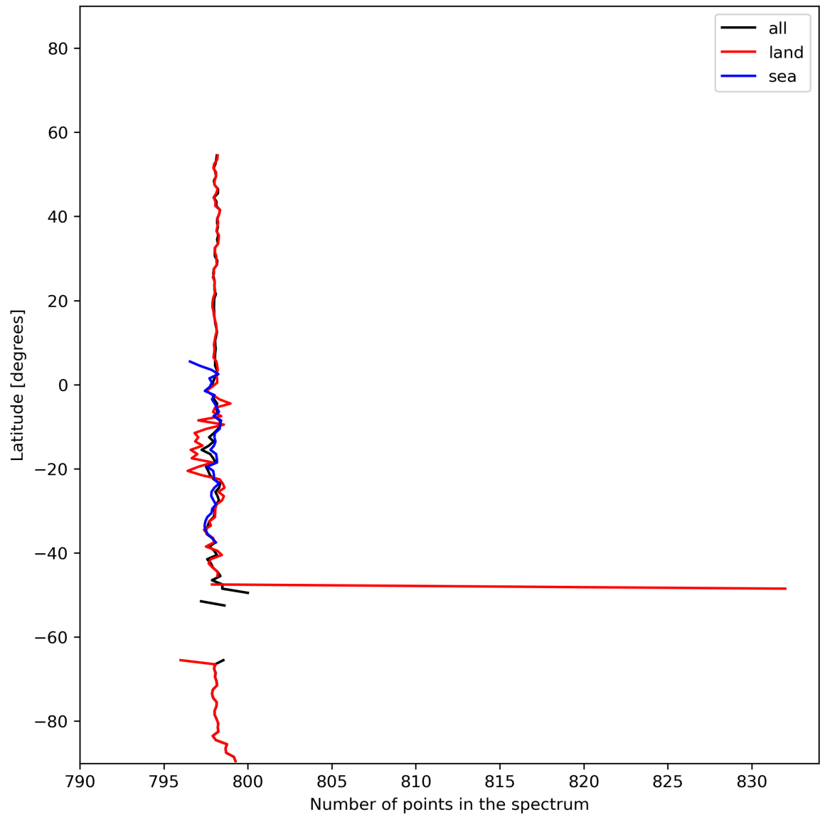
Figure 15: Zonal average of “Number of points in the spectrum” for 2024-01-16 to 2024-01-18.
