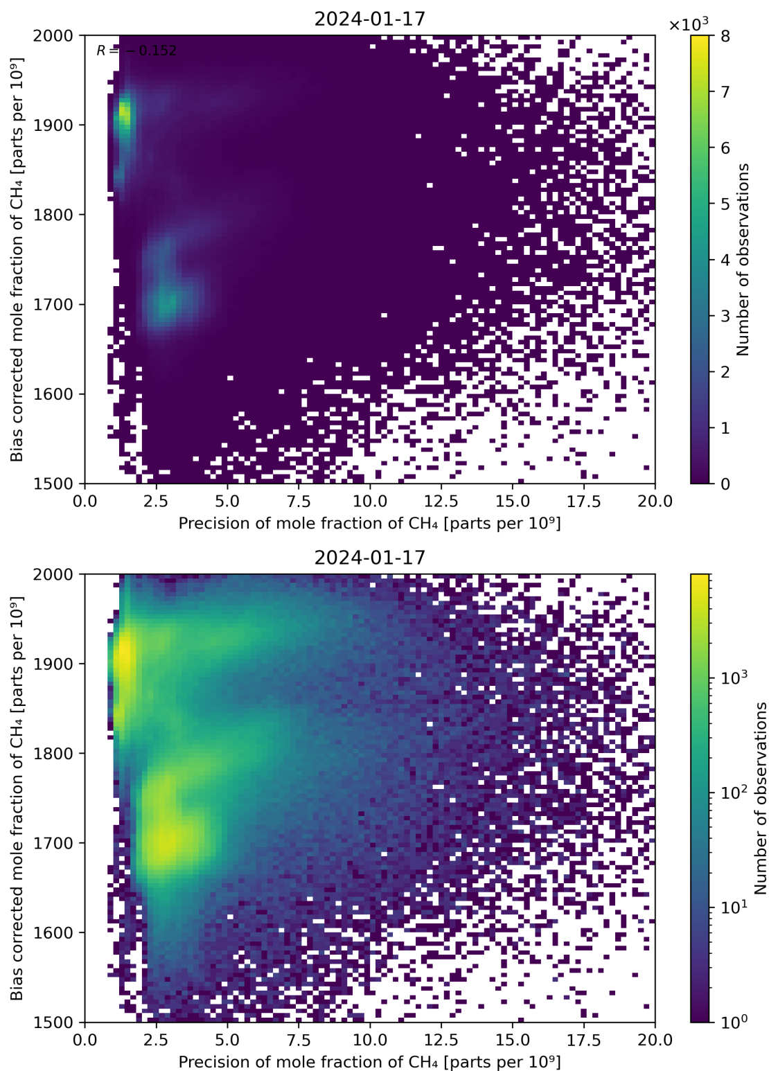
Figure 82: Scatter density plot of “Precision of mole fraction of \text{CH}_4 ” against “Bias corrected mole fraction of \text{CH}_4 ” for 2024-01-16 to 2024-01-18.
