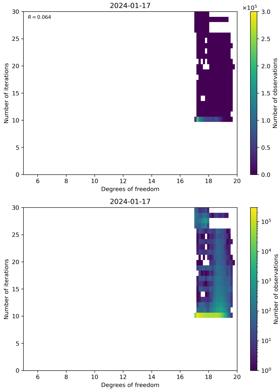
Figure 52: Scatter density plot of “Degrees of freedom” against “Number of iterations” for 2024-01-16 to 2024-01-18.
