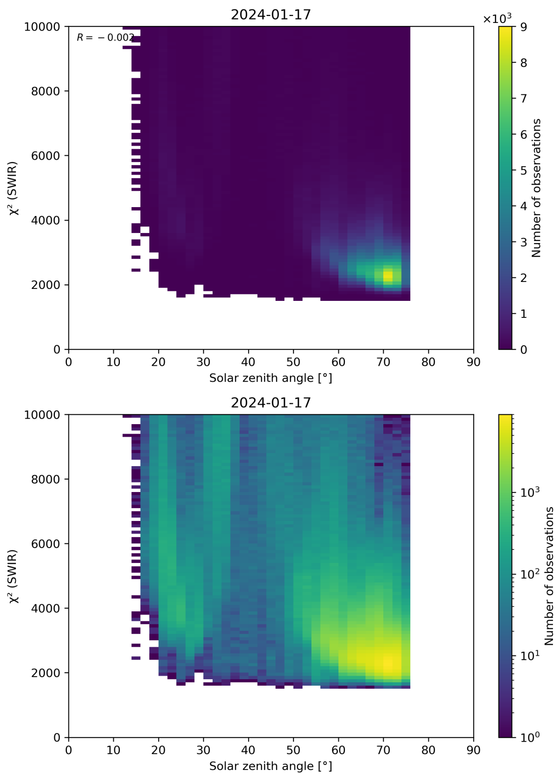
Figure 95: Scatter density plot of “Solar zenith angle” against “ \chi^2 (SWIR)” for 2024-01-16 to 2024-01-18.
