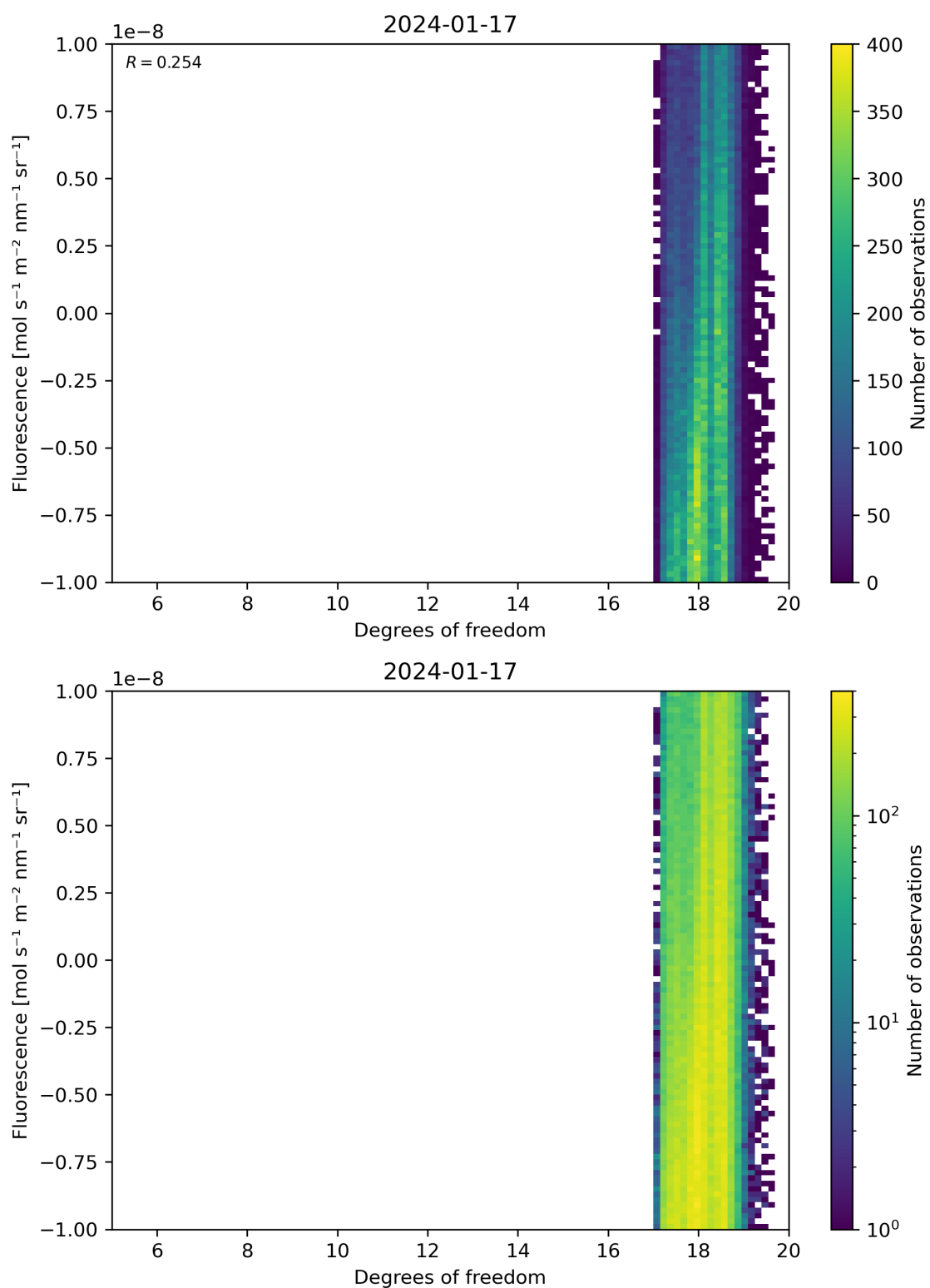
Figure 51: Scatter density plot of “Degrees of freedom” against “Fluorescence” for 2024-01-16 to 2024-01-18.
