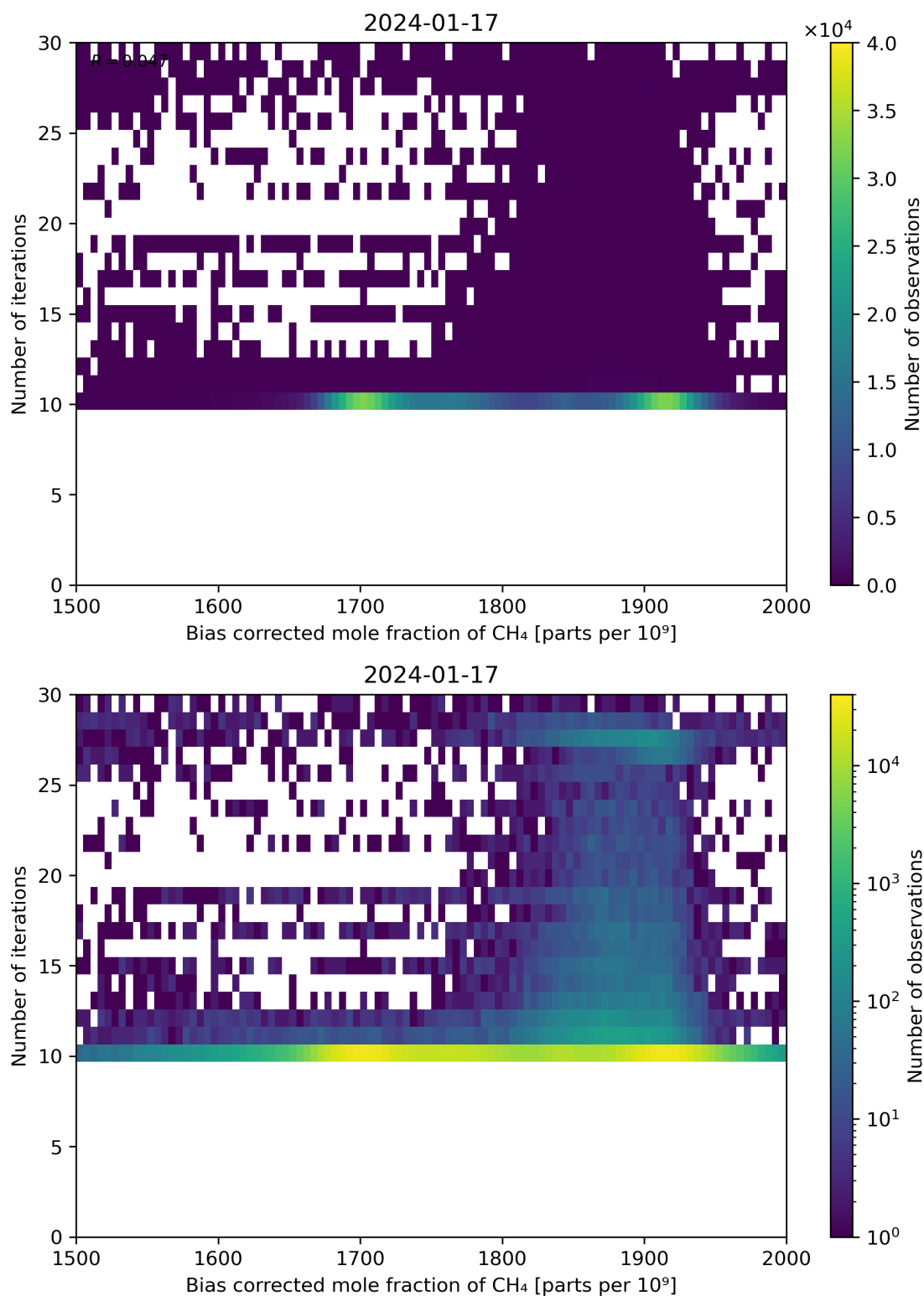
Figure 67: Scatter density plot of “Bias corrected mole fraction of CH 4 ” against “Number of iterations” for 2024-01-16 to 2024-01-18.
