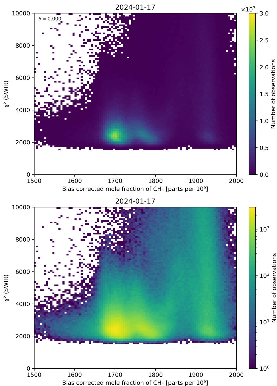
Figure 64: Scatter density plot of “Bias corrected mole fraction of CH 4 ” against “ \chi^2 (SWIR)” for 2024-01-16 to 2024-01-18.
