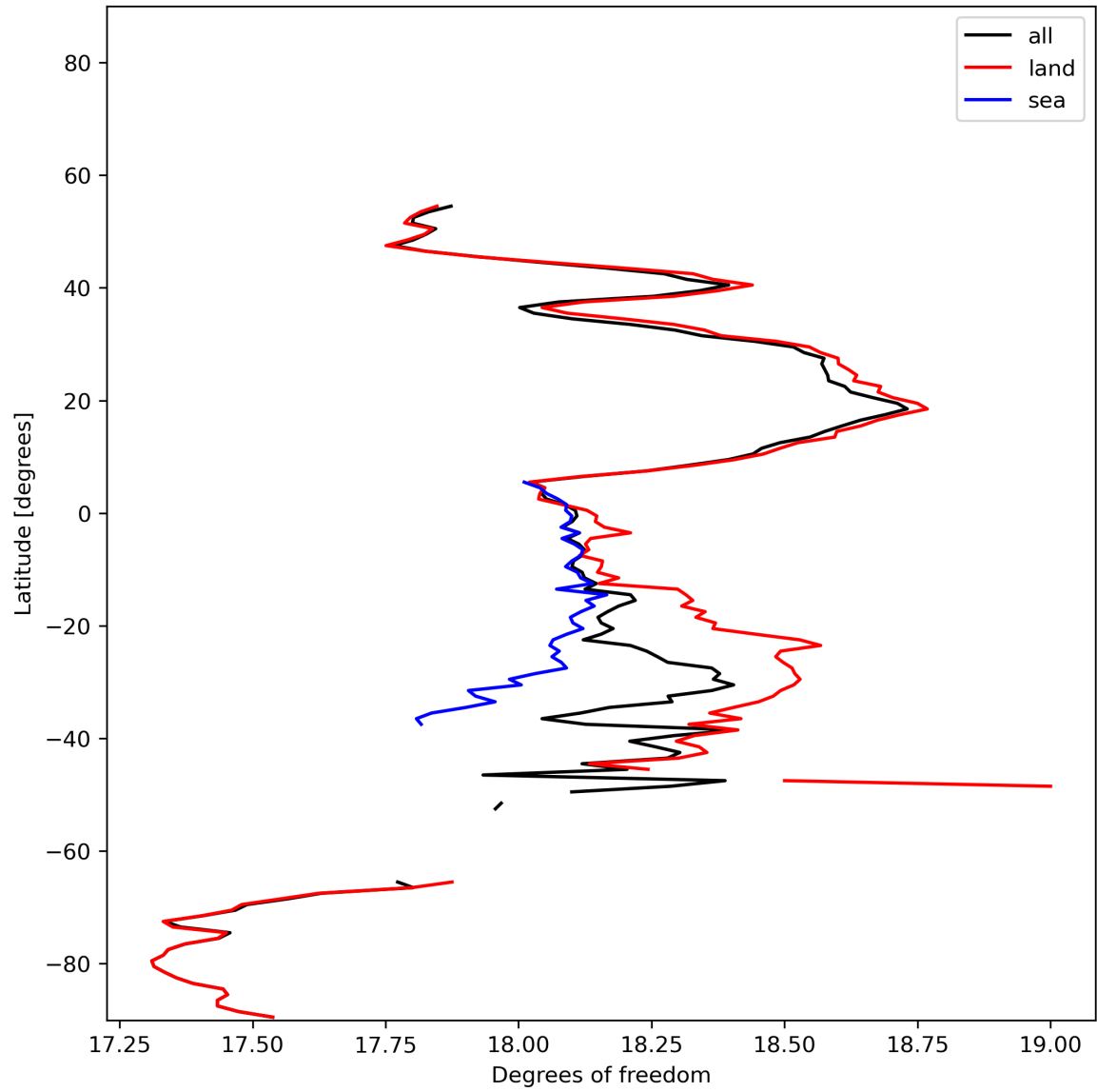
Figure 19: Zonal average of “Degrees of freedom” for 2024-01-16 to 2024-01-18.
