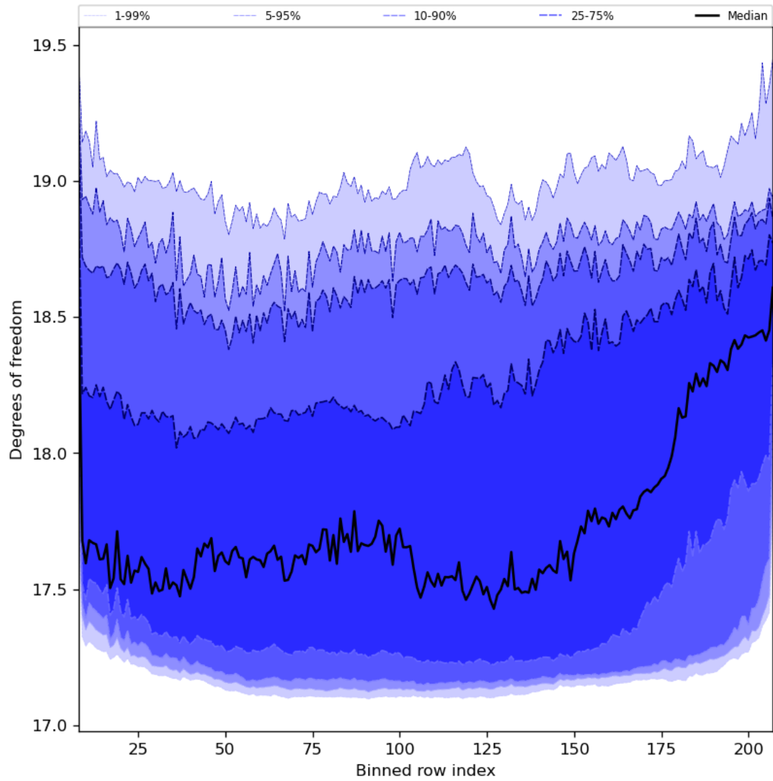
Figure 41: Along track statistics of “Degrees of freedom” for 2024-01-16 to 2024-01-18
