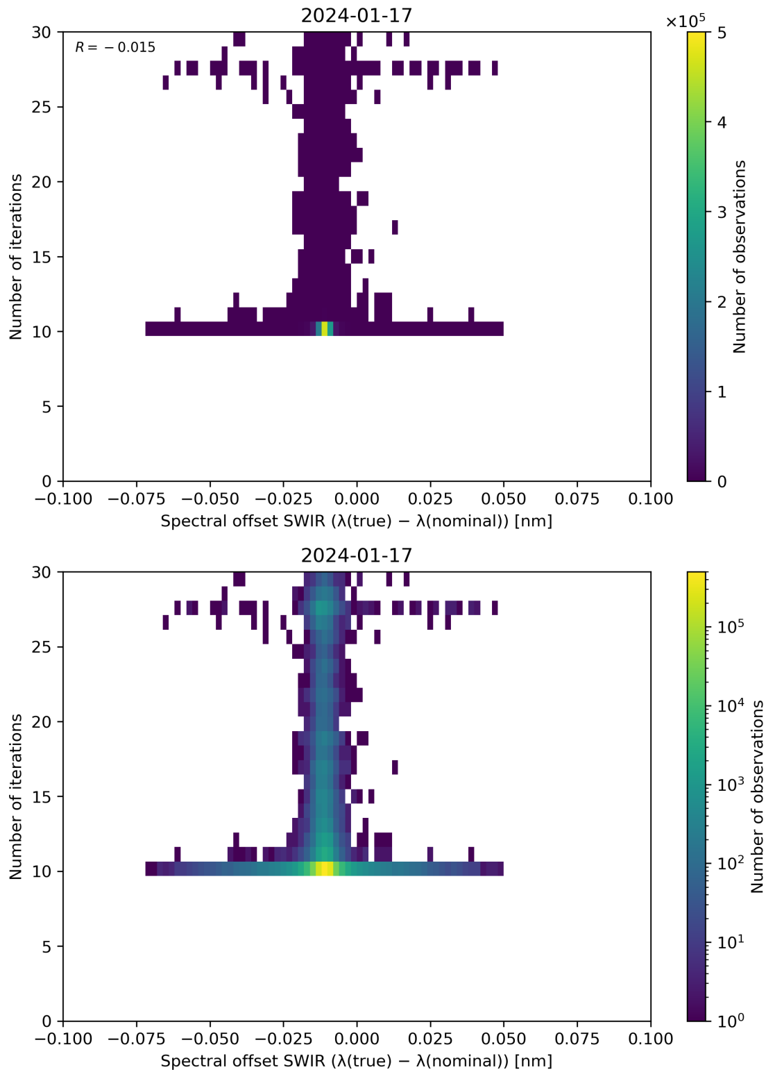
Figure 121: Scatter density plot of “Spectral offset SWIR ( \lambda(\text{true}) - \lambda(\text{nominal}) )” against “Number of iterations” for 2024-01-16 to 2024-01-18.
