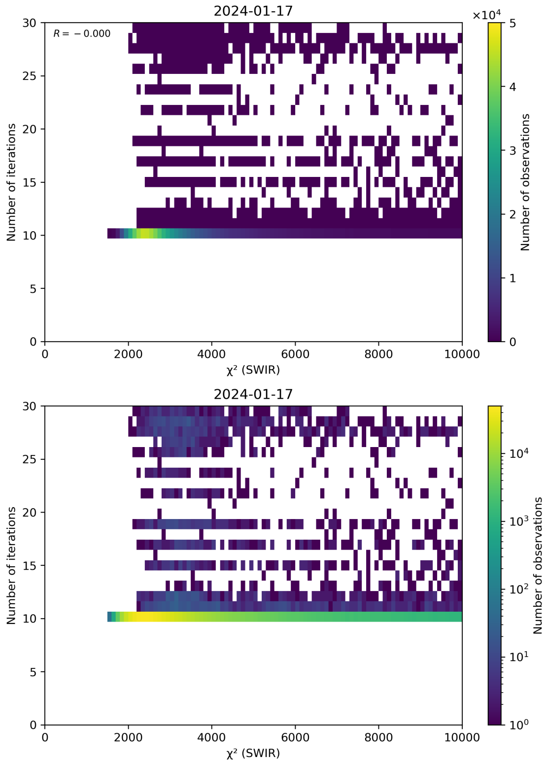
Figure 50: Scatter density plot of “ \chi^2 (SWIR)” against “Number of iterations” for 2024-01-16 to 2024-01-18.
