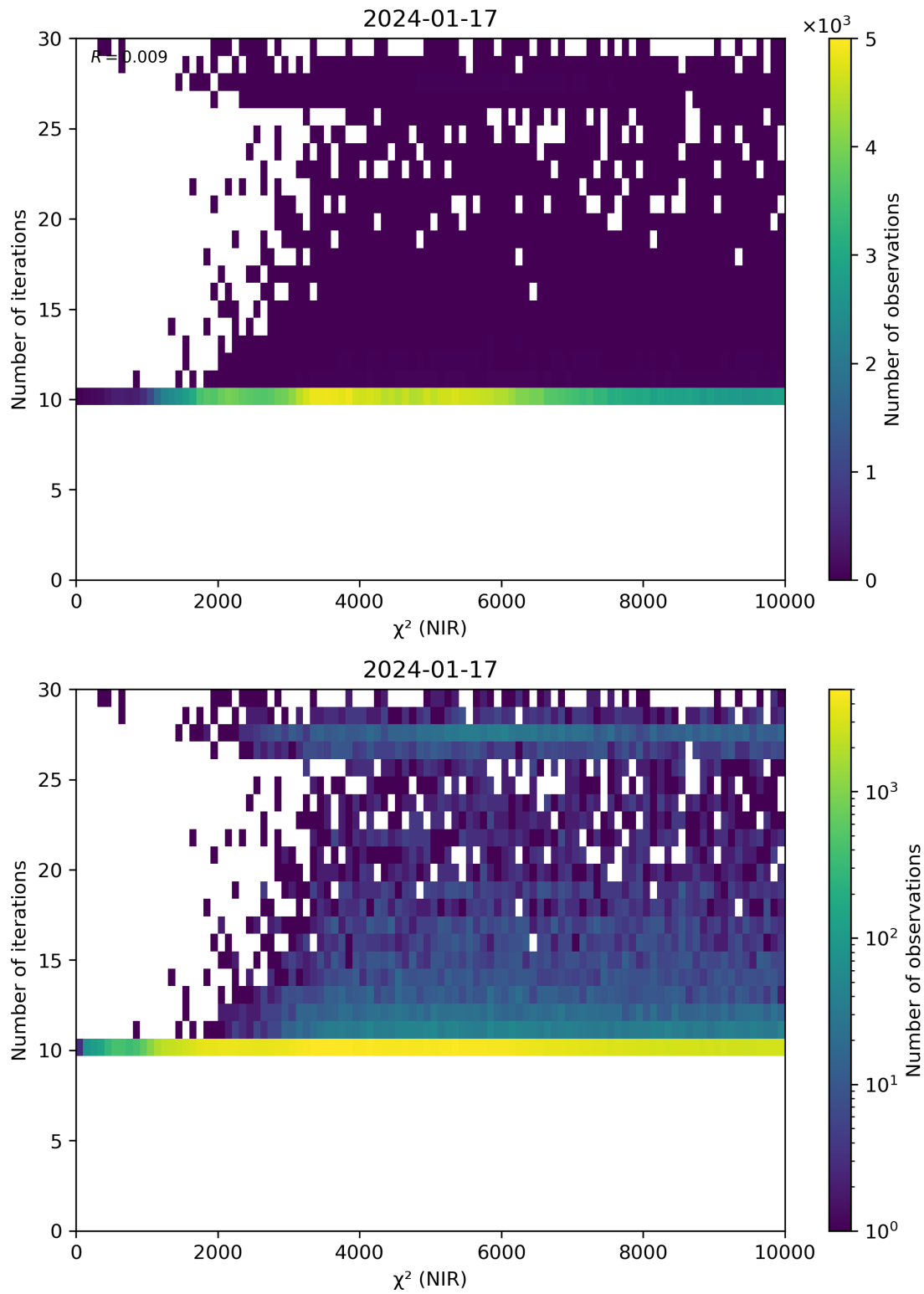
Figure 46: Scatter density plot of “ \chi^2 (NIR)” against “Number of iterations” for 2024-01-16 to 2024-01-18.
