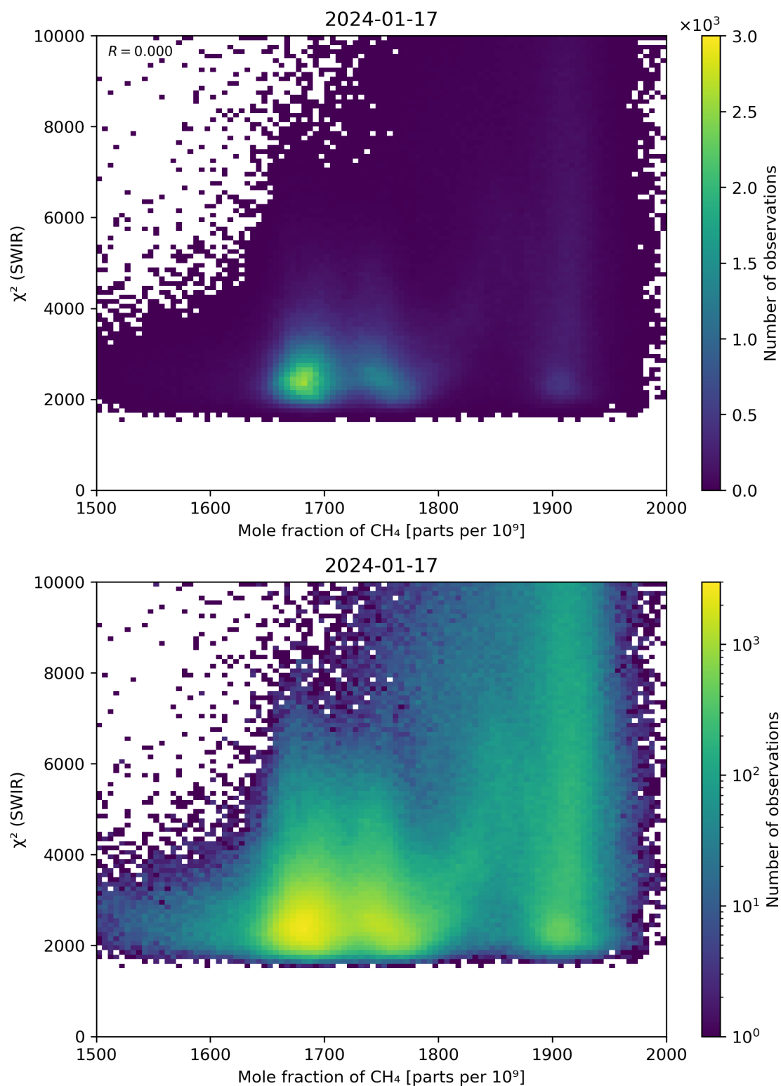
Figure 71: Scatter density plot of “Mole fraction of \text{CH}_4 ” against “ \chi^2 (SWIR)” for 2024-01-16 to 2024-01-18.
