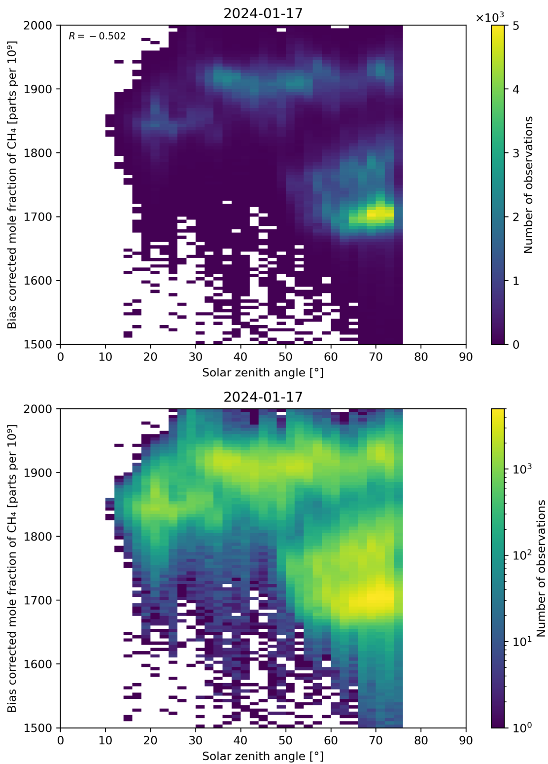
Figure 100: Scatter density plot of “Solar zenith angle” against “Bias corrected mole fraction of \text{CH}_4 ” for 2024-01-16 to 2024-01-18.
