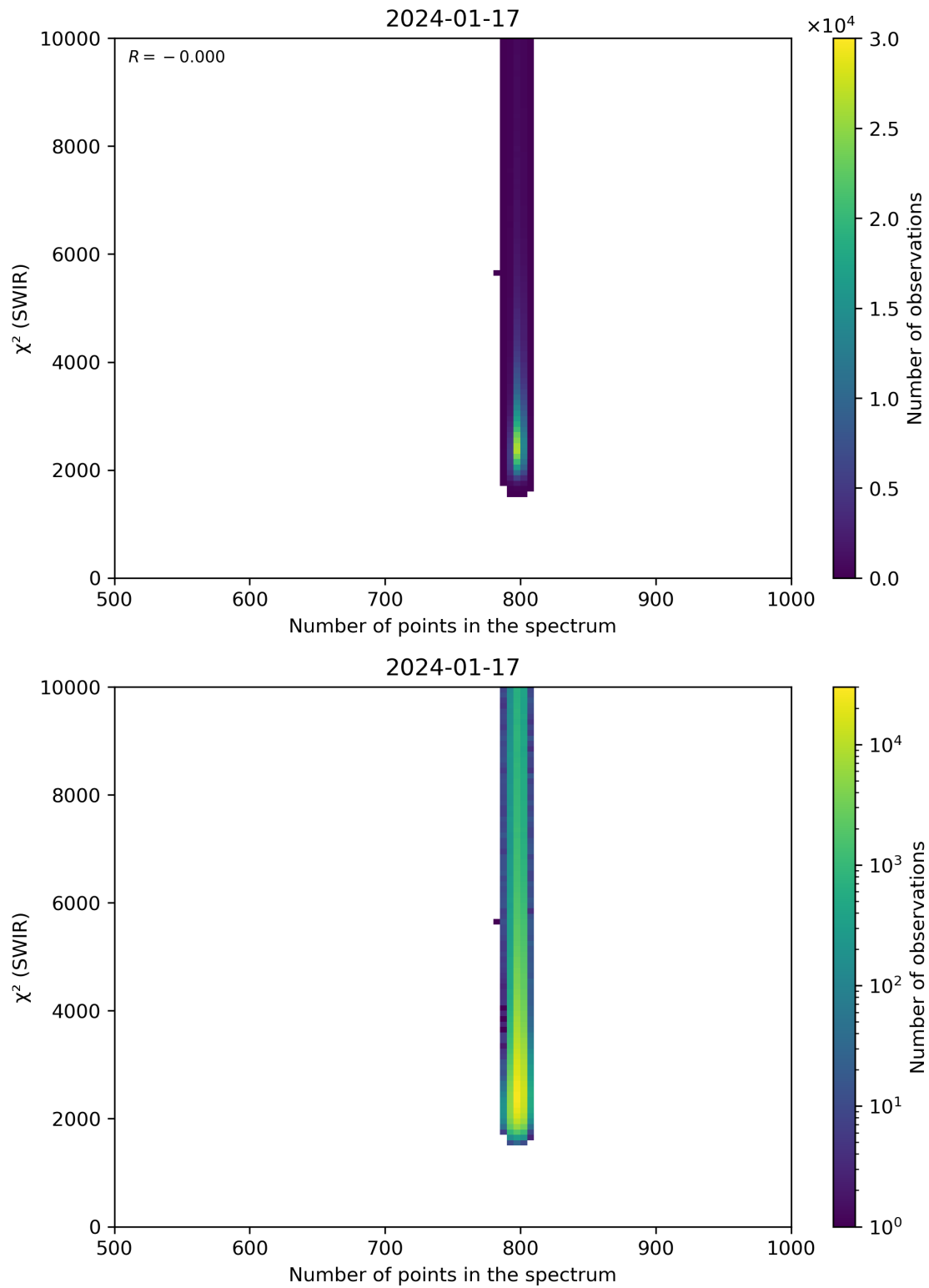
Figure 89: Scatter density plot of “Number of points in the spectrum” against “ \chi^2 (SWIR)” for 2024-01-16 to 2024-01-18.
