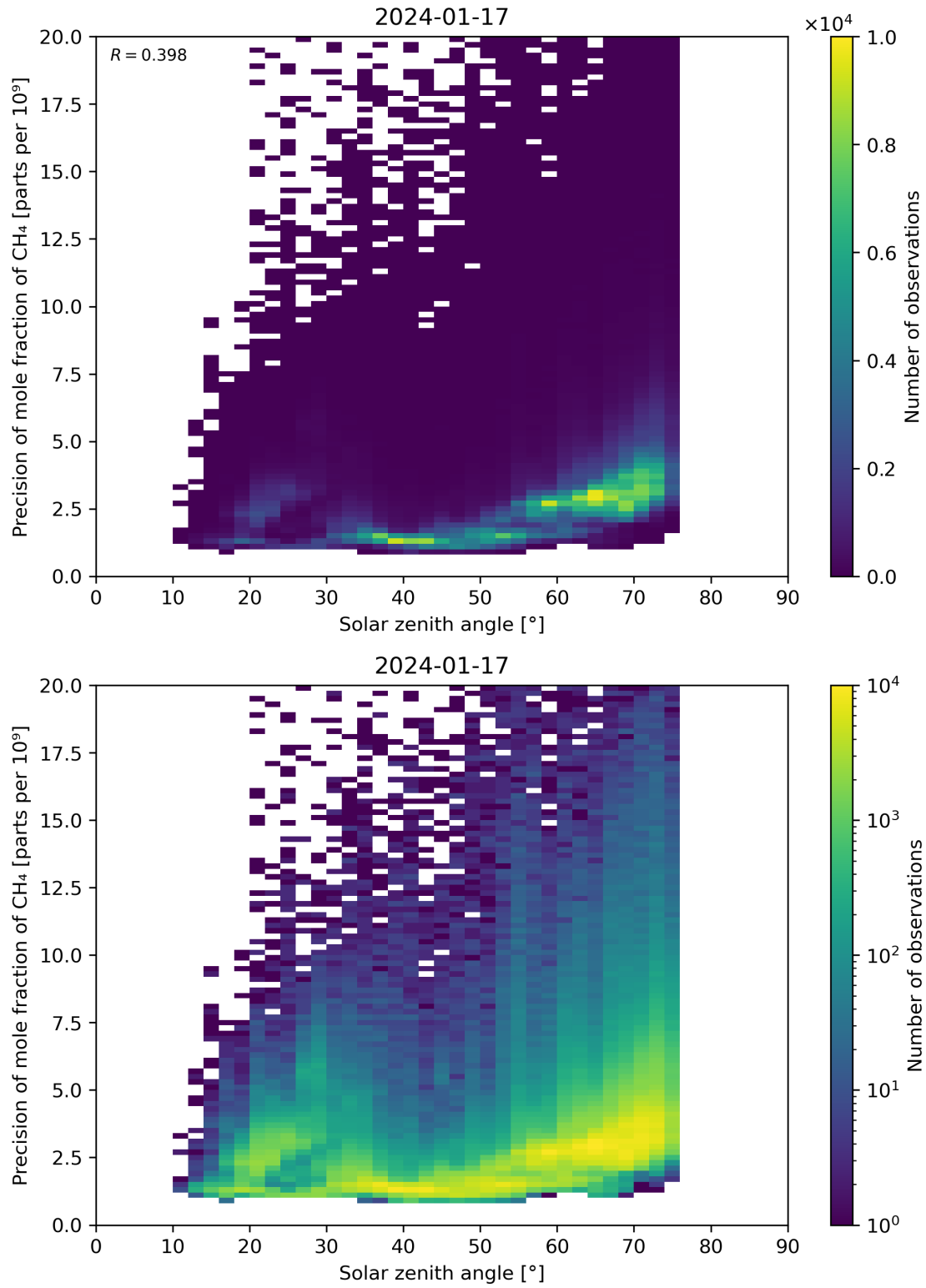
Figure 101: Scatter density plot of “Solar zenith angle” against “Precision of mole fraction of \text{CH}_4 ” for 2024-01-16 to 2024-01-18.
