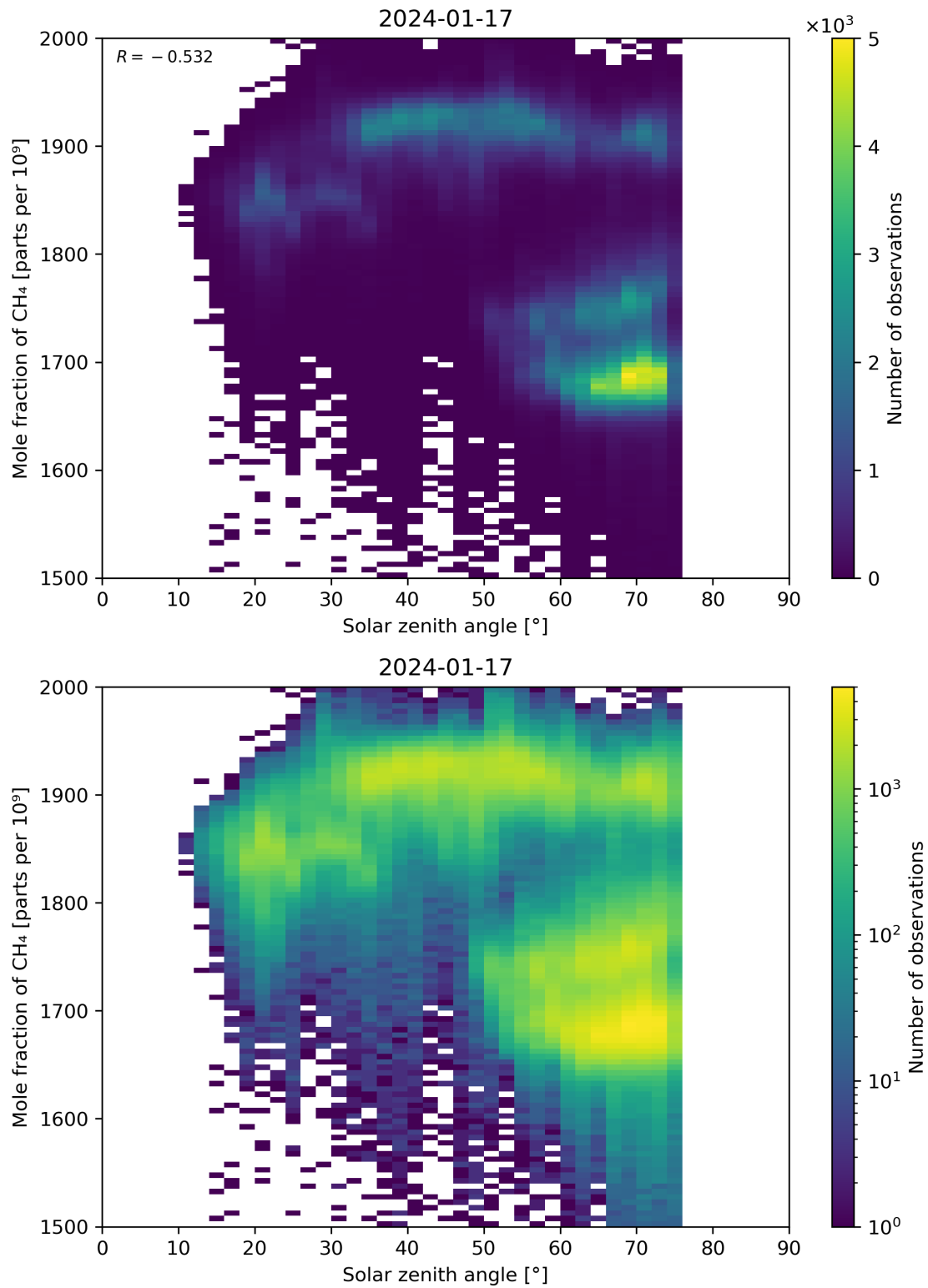
Figure 99: Scatter density plot of “Solar zenith angle” against “Mole fraction of CH 4 ” for 2024-01-16 to 2024-01-18.
