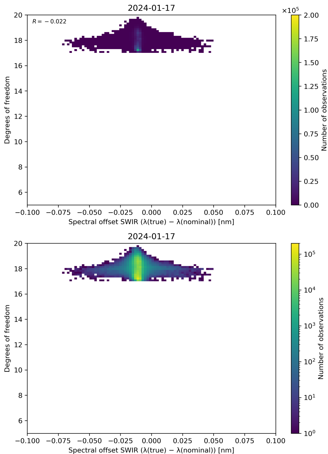
Figure 119: Scatter density plot of “Spectral offset SWIR ( \lambda(\text{true}) - \lambda(\text{nominal}) )” against “Degrees of freedom” for 2024-01-16 to 2024-01-18.
