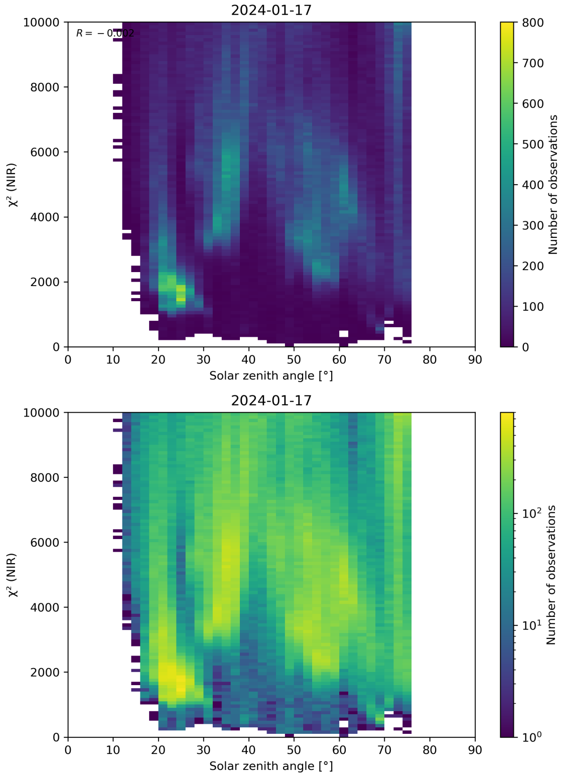
Figure 94: Scatter density plot of “Solar zenith angle” against “ \chi^2 (NIR)” for 2024-01-16 to 2024-01-18.
