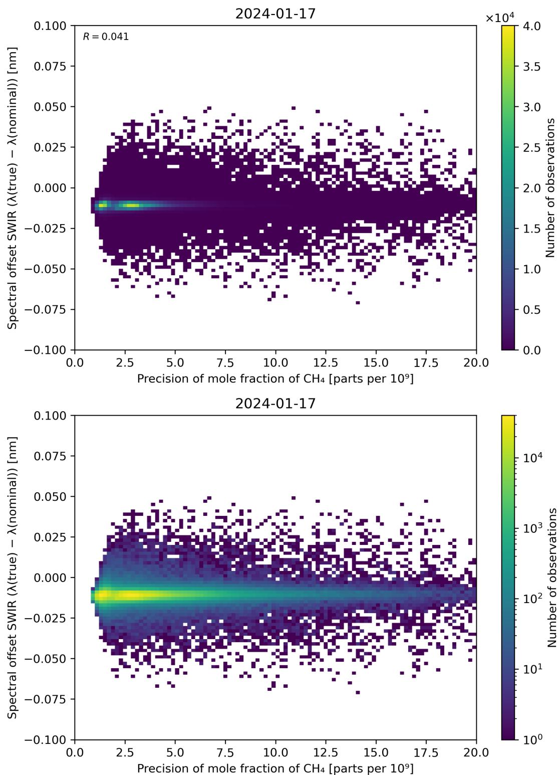
Figure 85: Scatter density plot of “Precision of mole fraction of \text{CH}_4 ” against “Spectral offset SWIR ( \lambda(\text{true}) - \lambda(\text{nominal}) )” for 2024-01-16 to 2024-01-18.
