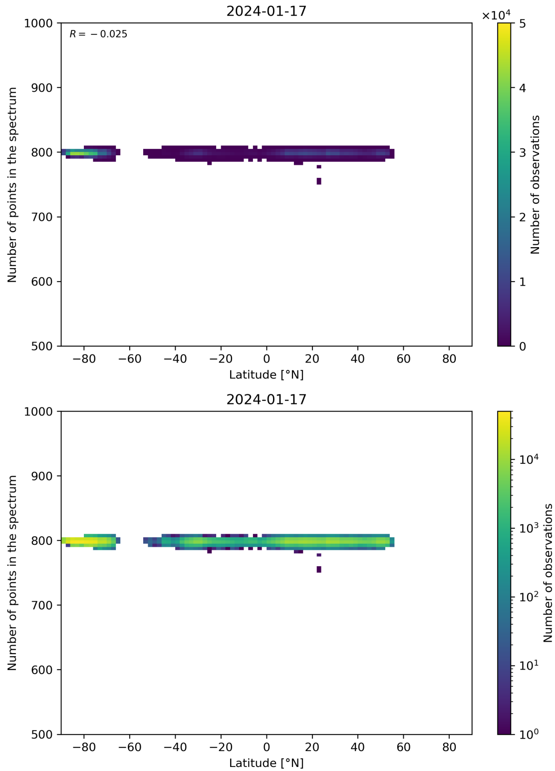
Figure 61: Scatter density plot of “Latitude” against “Number of points in the spectrum” for 2024-01-16 to 2024-01-18.
