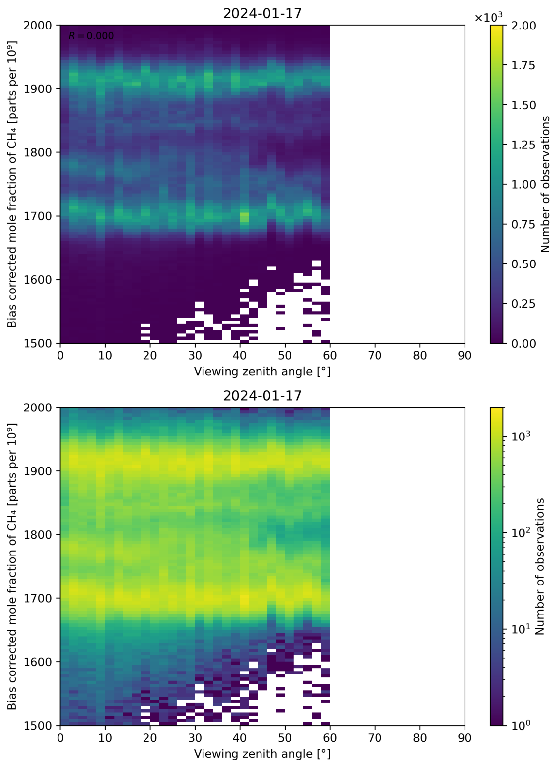
Figure 111: Scatter density plot of “Viewing zenith angle” against “Bias corrected mole fraction of CH 4 ” for 2024-01-16 to 2024-01-18.
