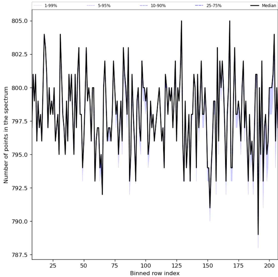
Figure 37: Along track statistics of “Number of points in the spectrum” for 2024-01-16 to 2024-01-18
