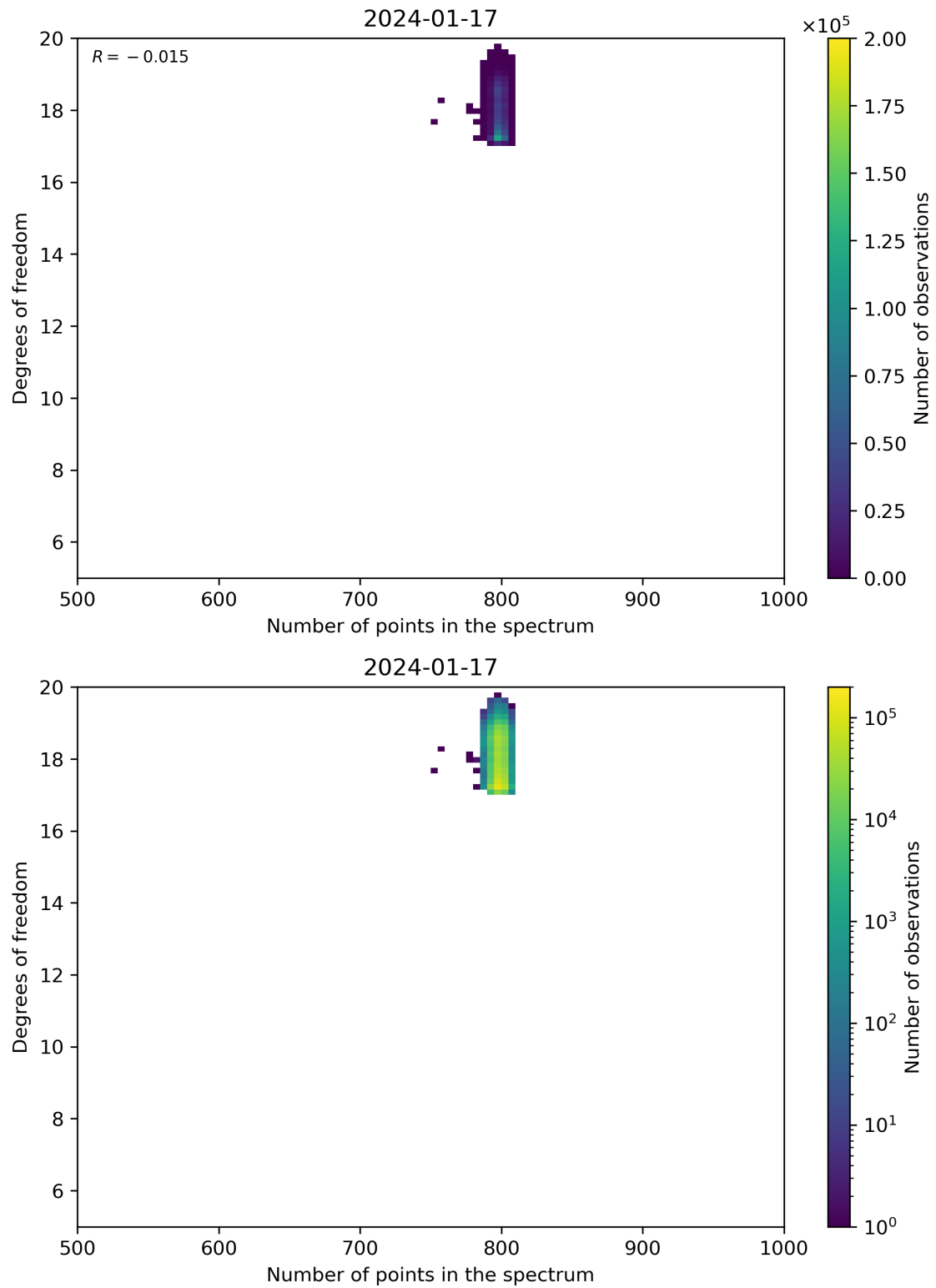
Figure 90: Scatter density plot of “Number of points in the spectrum” against “Degrees of freedom” for 2024-01-16 to 2024-01-18.
