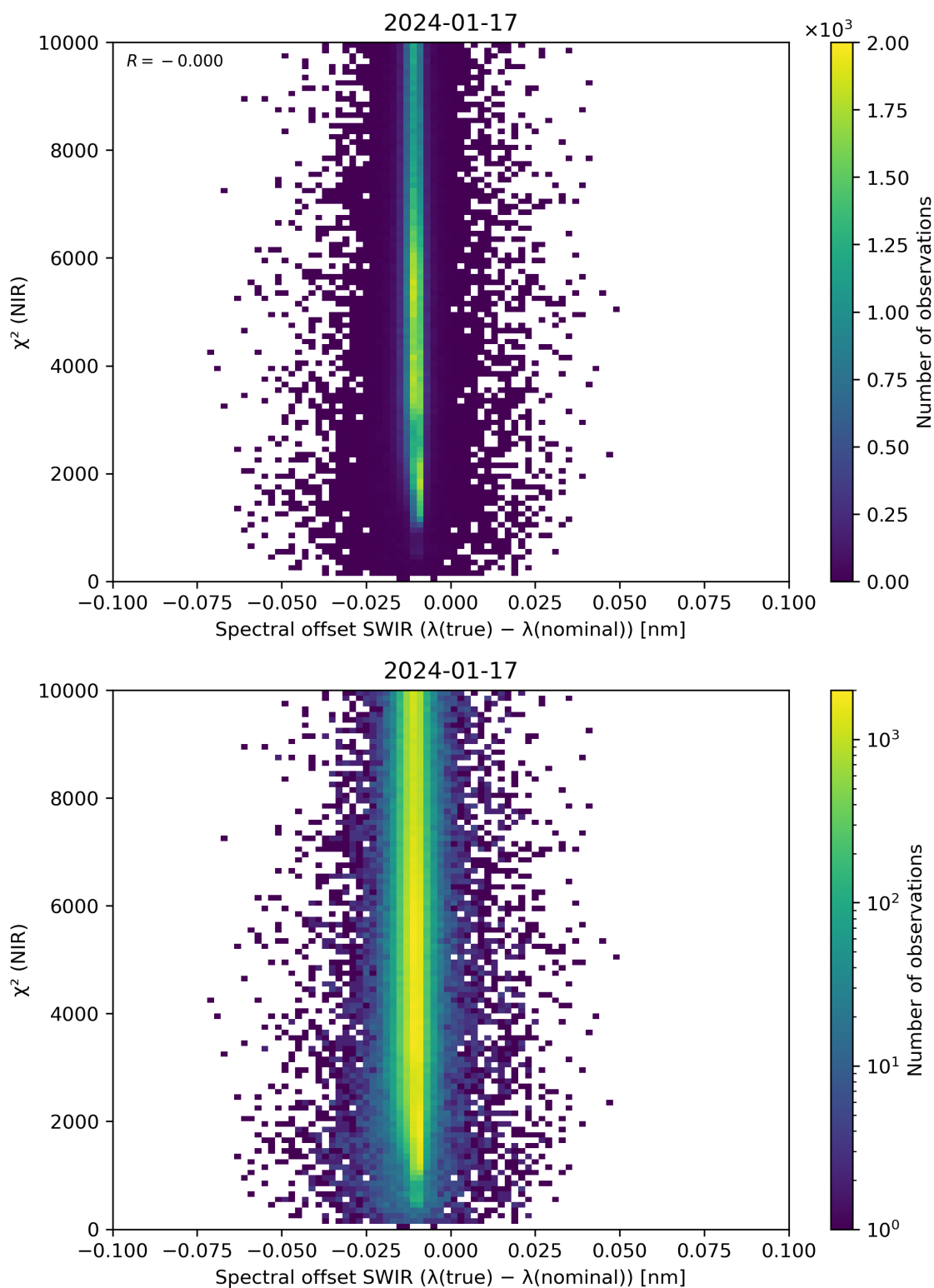
Figure 117: Scatter density plot of “Spectral offset SWIR ( \lambda(\text{true}) - \lambda(\text{nominal}) )” against “ \chi^2 (NIR)” for 2024-01-16 to 2024-01-18.
