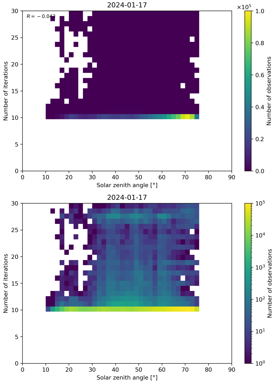
Figure 102: Scatter density plot of “Solar zenith angle” against “Number of iterations” for 2024-01-16 to 2024-01-18.
