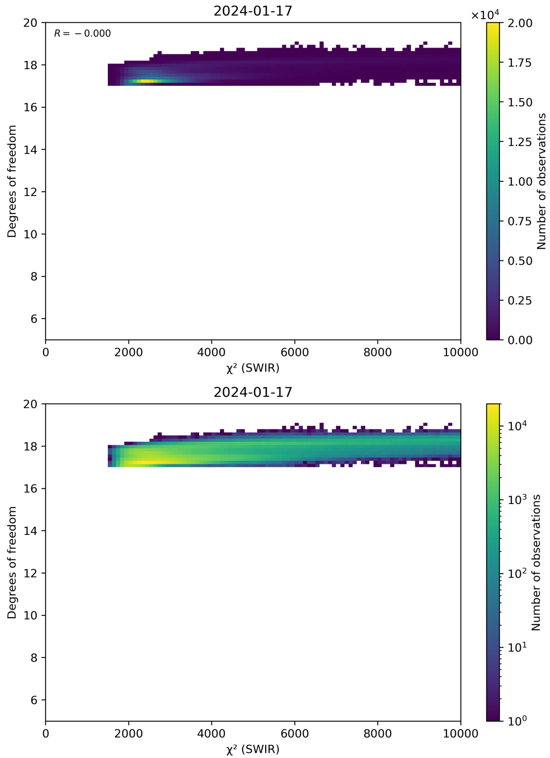
Figure 48: Scatter density plot of “ \chi^2 (SWIR)” against “Degrees of freedom” for 2024-01-16 to 2024-01-18.
