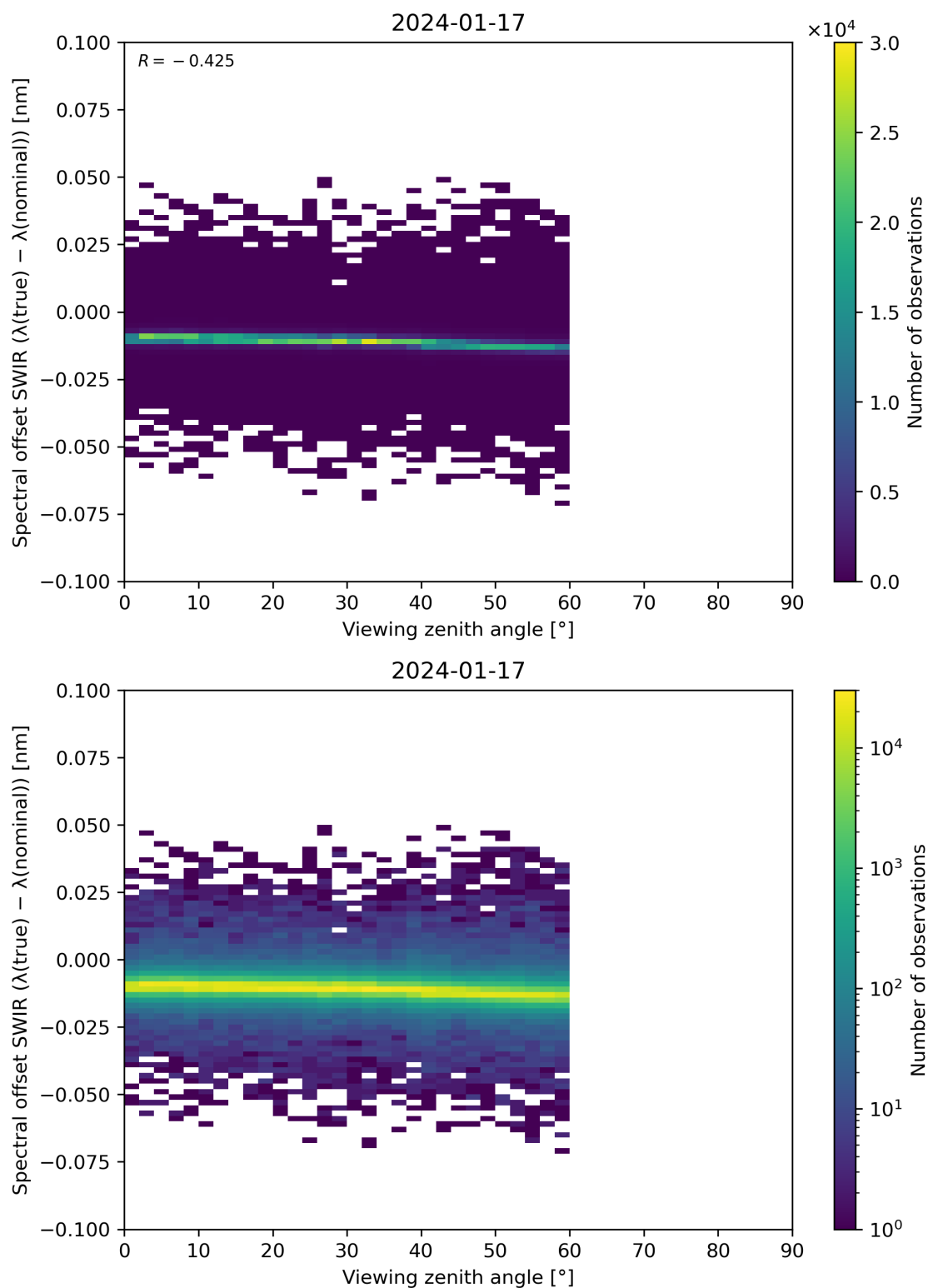
Figure 116: Scatter density plot of “Viewing zenith angle” against “Spectral offset SWIR ( \lambda(\text{true}) - \lambda(\text{nominal}) )” for 2024-01-16 to 2024-01-18.
