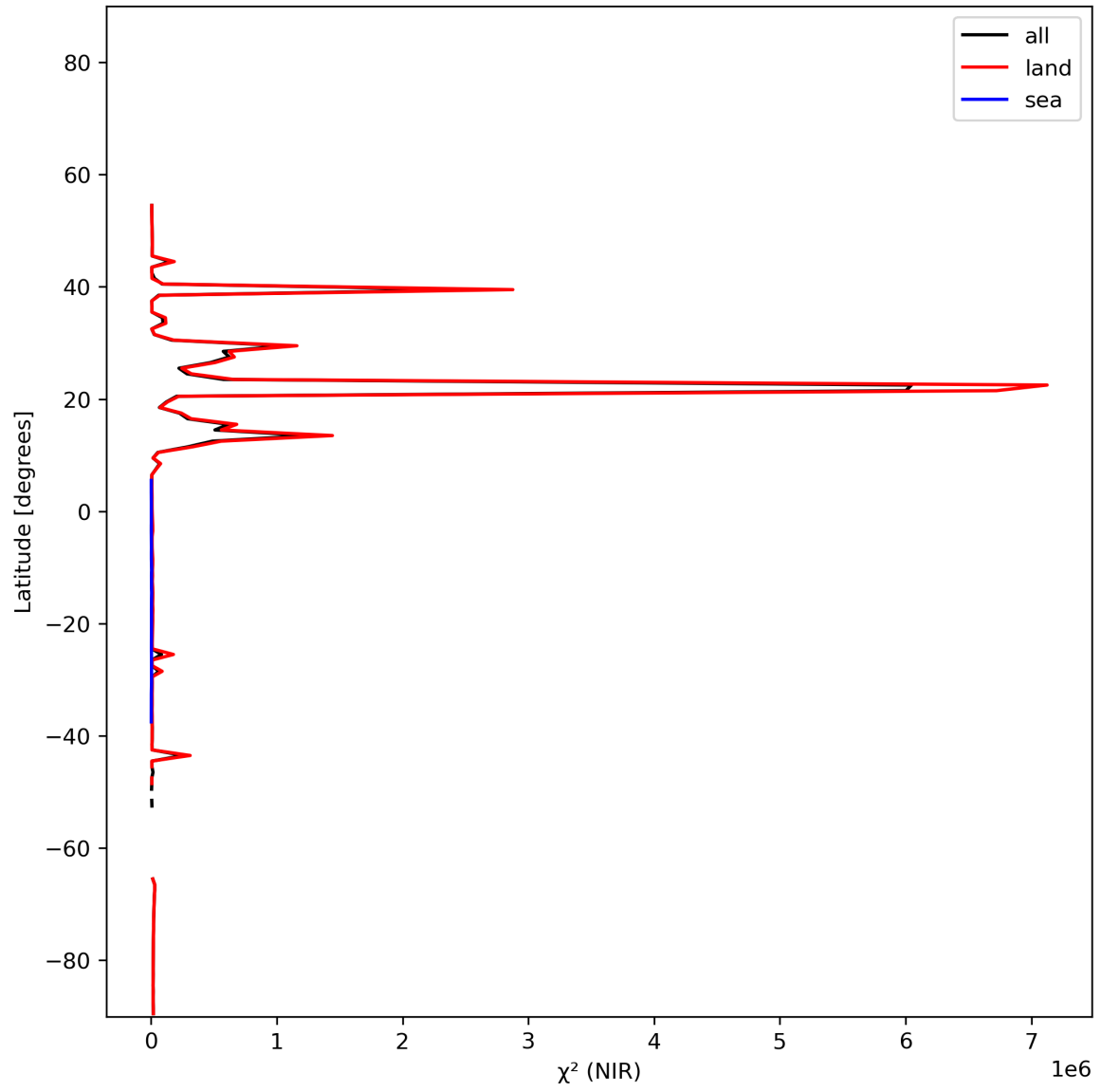
Figure 18: Zonal average of “ \chi^2 (NIR)” for 2024-01-16 to 2024-01-18.
