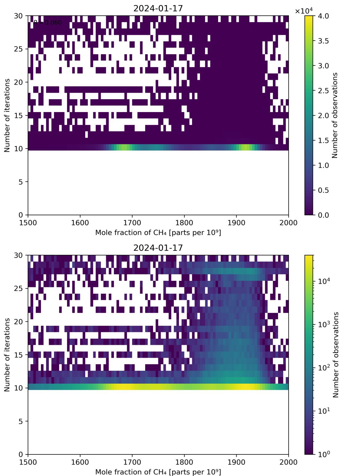
Figure 76: Scatter density plot of “Mole fraction of CH 4 ” against “Number of iterations” for 2024-01-16 to 2024-01-18.
