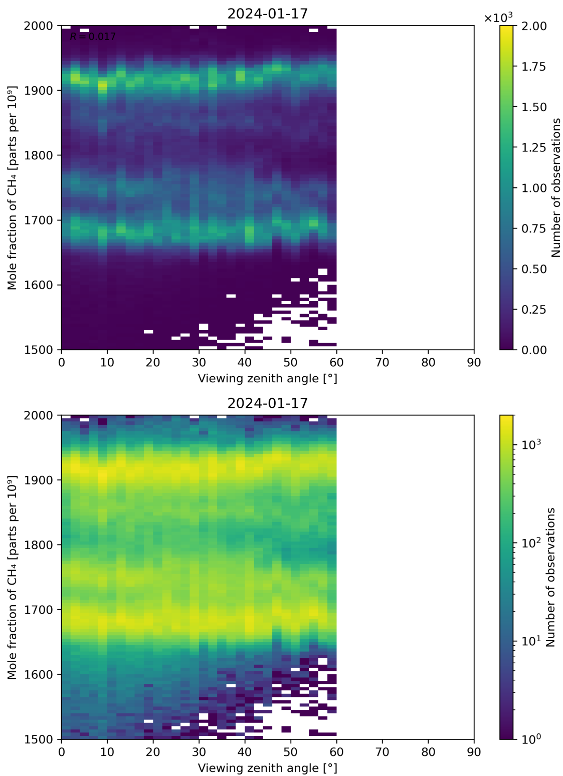
Figure 110: Scatter density plot of “Viewing zenith angle” against “Mole fraction of CH 4 ” for 2024-01-16 to 2024-01-18.
