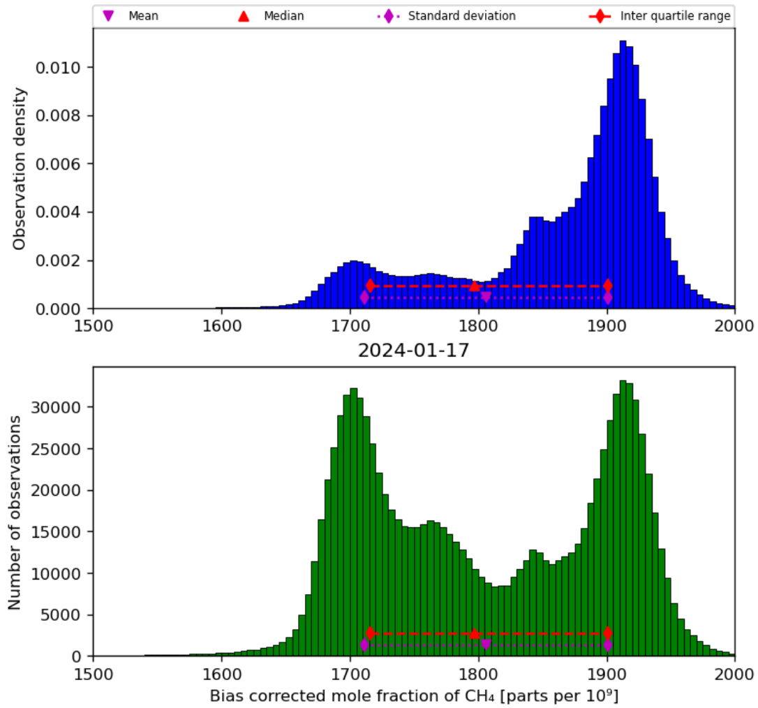
Figure 25: Histogram of “Bias corrected mole fraction of CH 4 ” for 2024-01-16 to 2024-01-18
