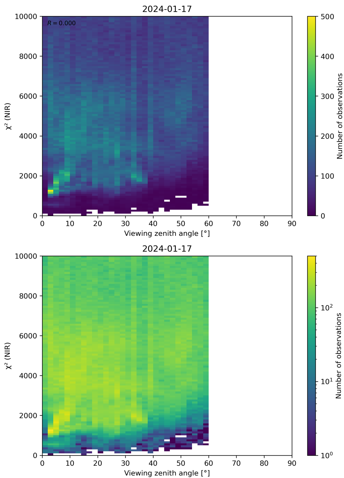
Figure 105: Scatter density plot of “Viewing zenith angle” against “ \chi^2 (NIR)” for 2024-01-16 to 2024-01-18.
