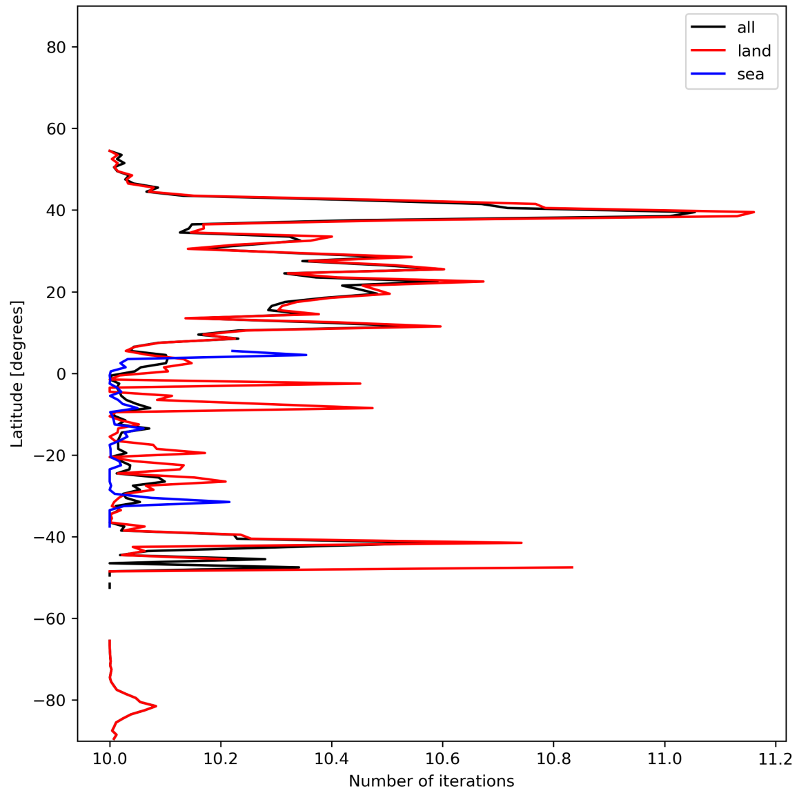
Figure 20: Zonal average of “Number of iterations” for 2024-01-16 to 2024-01-18.
