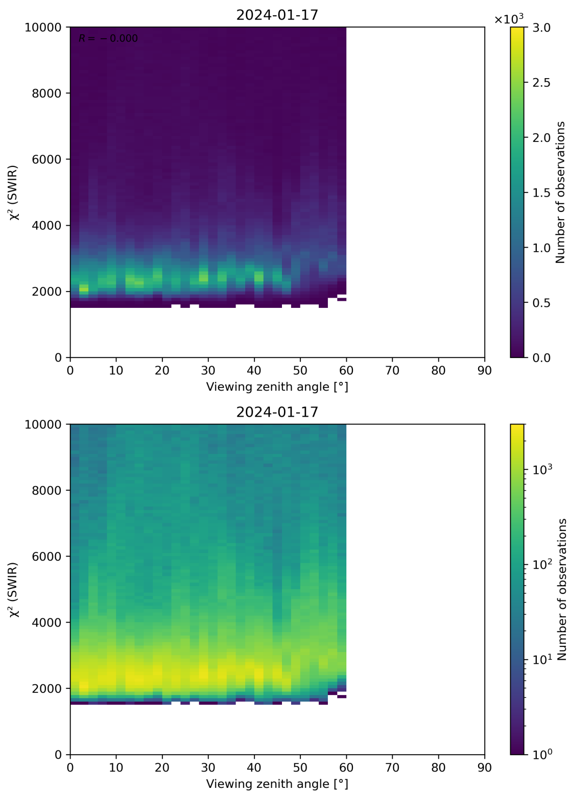
Figure 106: Scatter density plot of “Viewing zenith angle” against “ \chi^2 (SWIR)” for 2024-01-16 to 2024-01-18.
