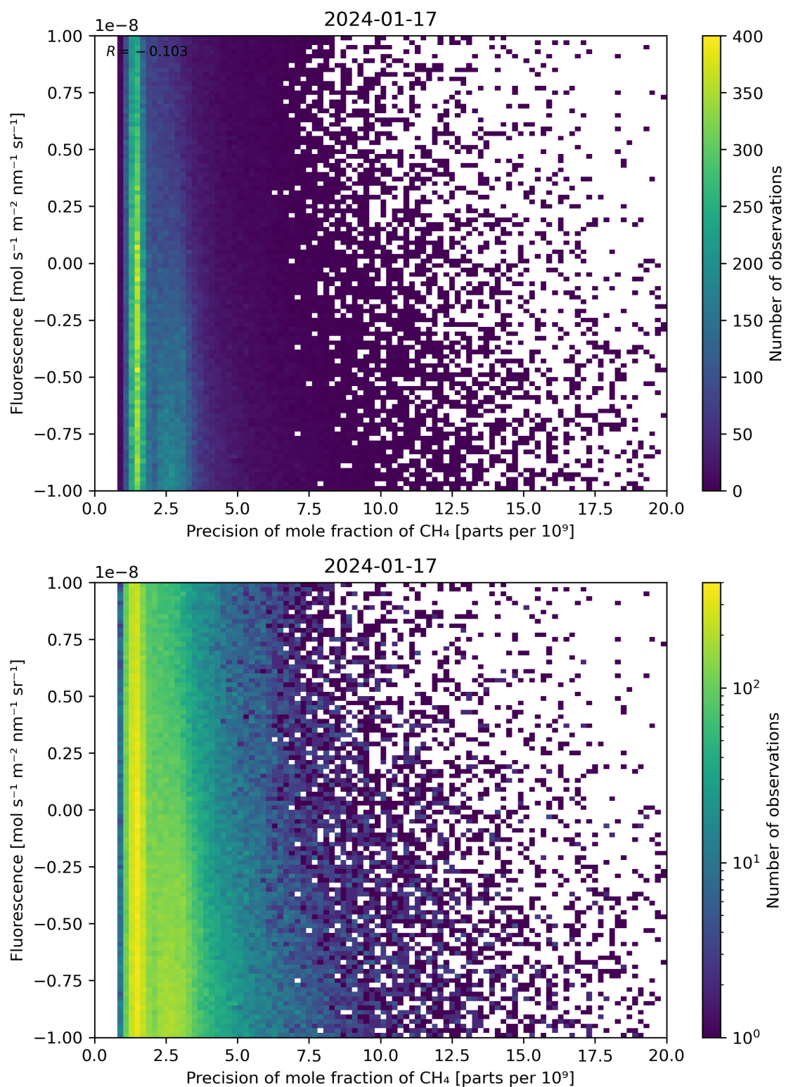
Figure 81: Scatter density plot of “Precision of mole fraction of \text{CH}_4 ” against “Fluorescence” for 2024-01-16 to 2024-01-18.
