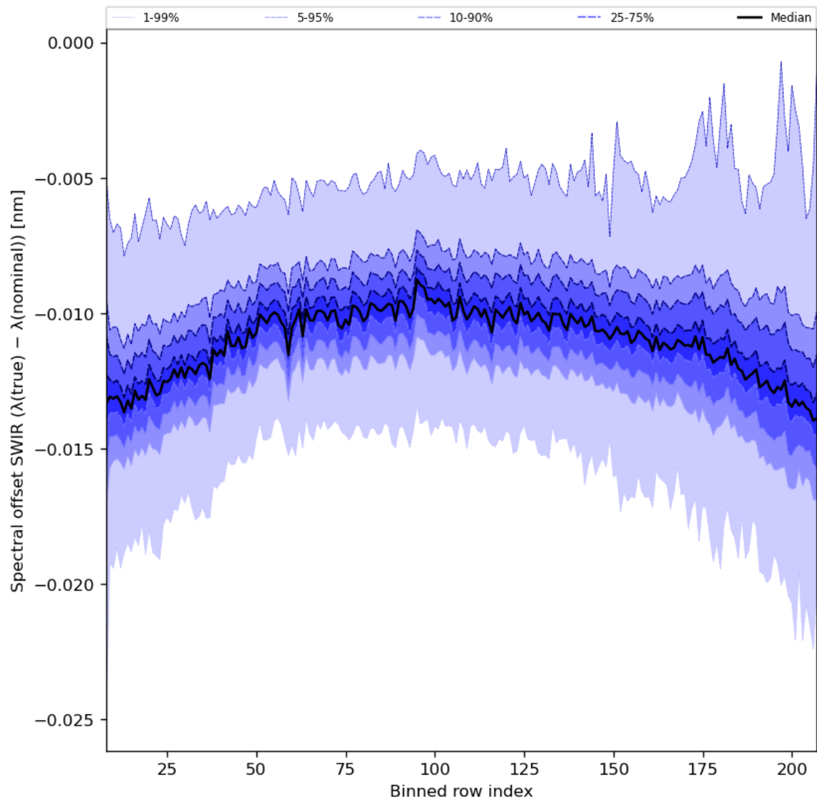
Figure 38: Along track statistics of “Spectral offset SWIR ( \lambda(\text{true}) - \lambda(\text{nominal}) )” for 2024-01-16 to 2024-01-18
