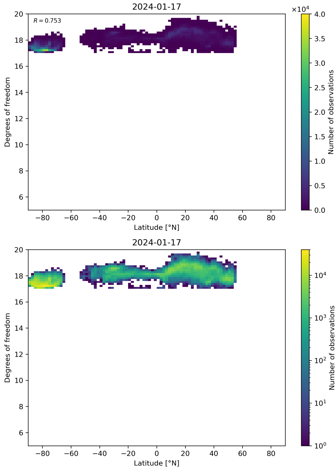
Figure 55: Scatter density plot of “Latitude” against “Degrees of freedom” for 2024-01-16 to 2024-01-18.
