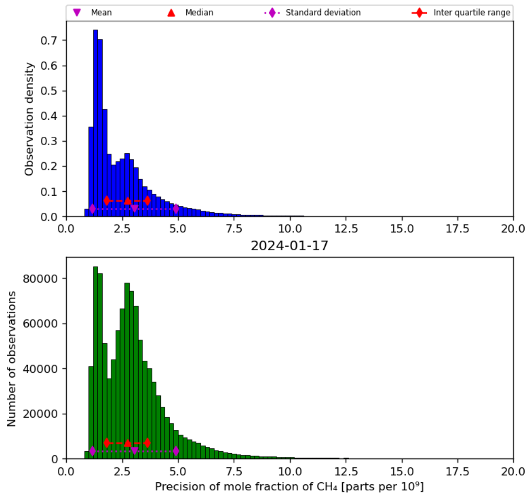
Figure 24: Histogram of “Precision of mole fraction of CH 4 ” for 2024-01-16 to 2024-01-18
