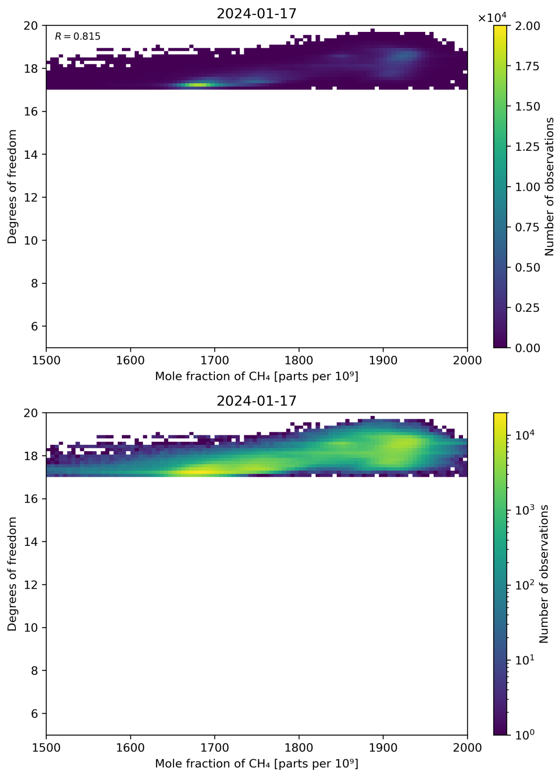
Figure 72: Scatter density plot of “Mole fraction of CH 4 ” against “Degrees of freedom” for 2024-01-16 to 2024-01-18.
