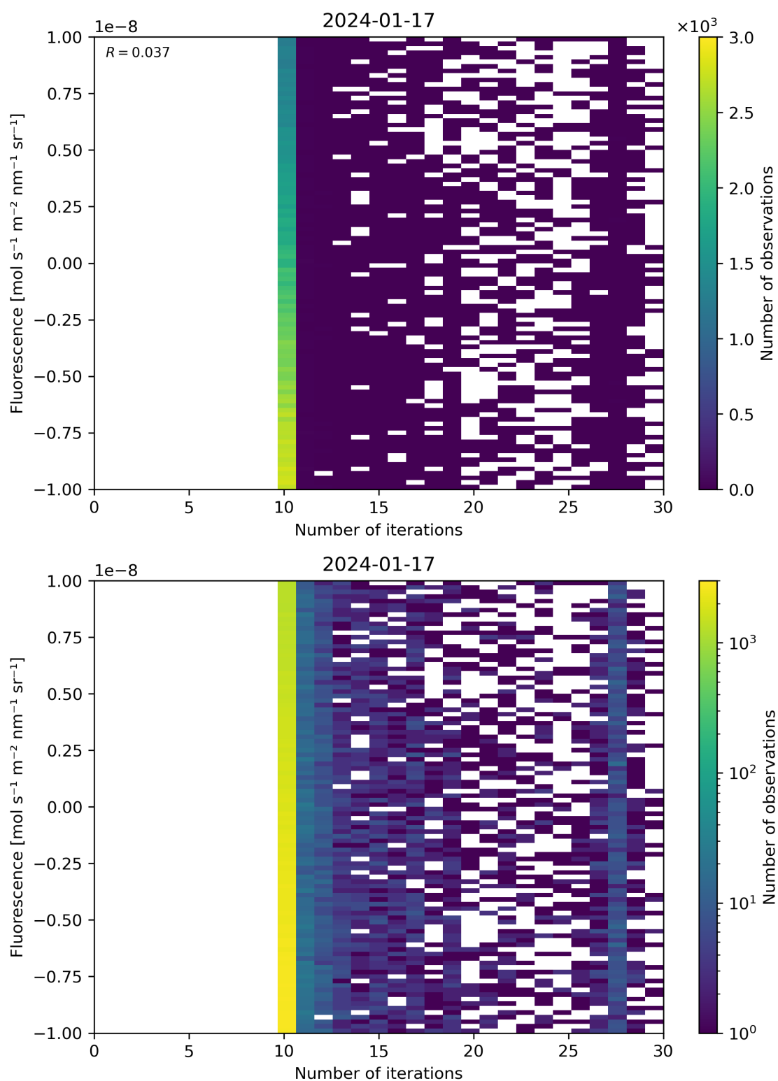
Figure 87: Scatter density plot of “Number of iterations” against “Fluorescence” for 2024-01-16 to 2024-01-18.
