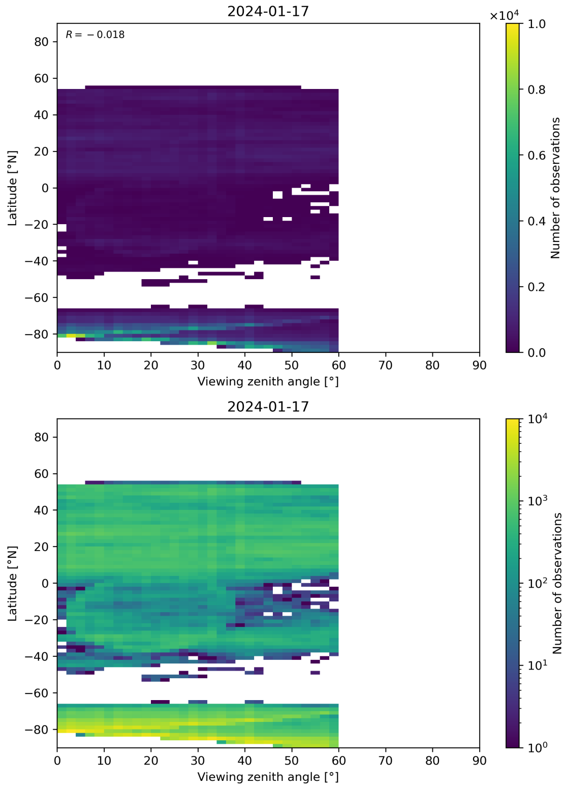
Figure 109: Scatter density plot of “Viewing zenith angle” against “Latitude” for 2024-01-16 to 2024-01-18.
