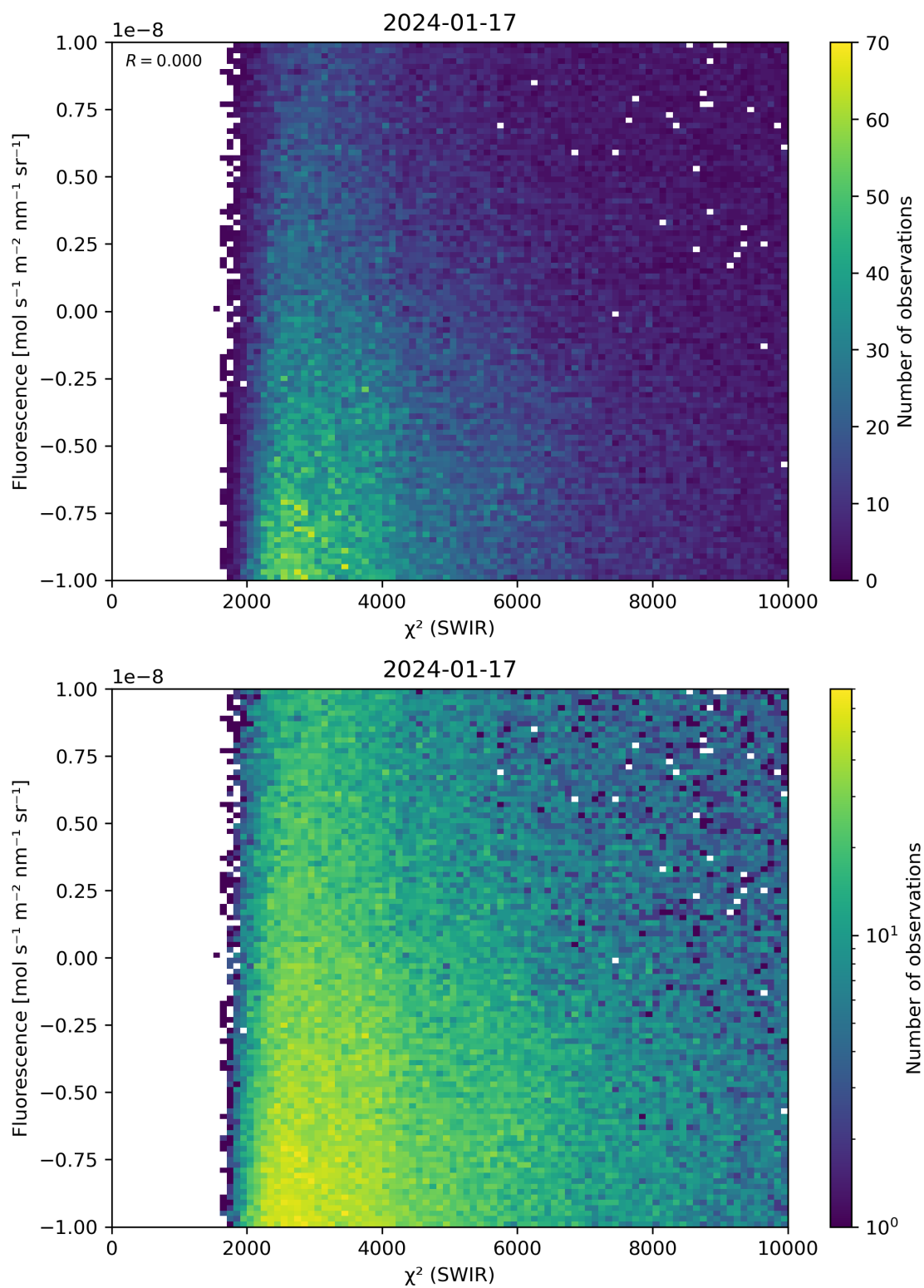
Figure 49: Scatter density plot of “ \chi^2 (SWIR)” against “Fluorescence” for 2024-01-16 to 2024-01-18.
