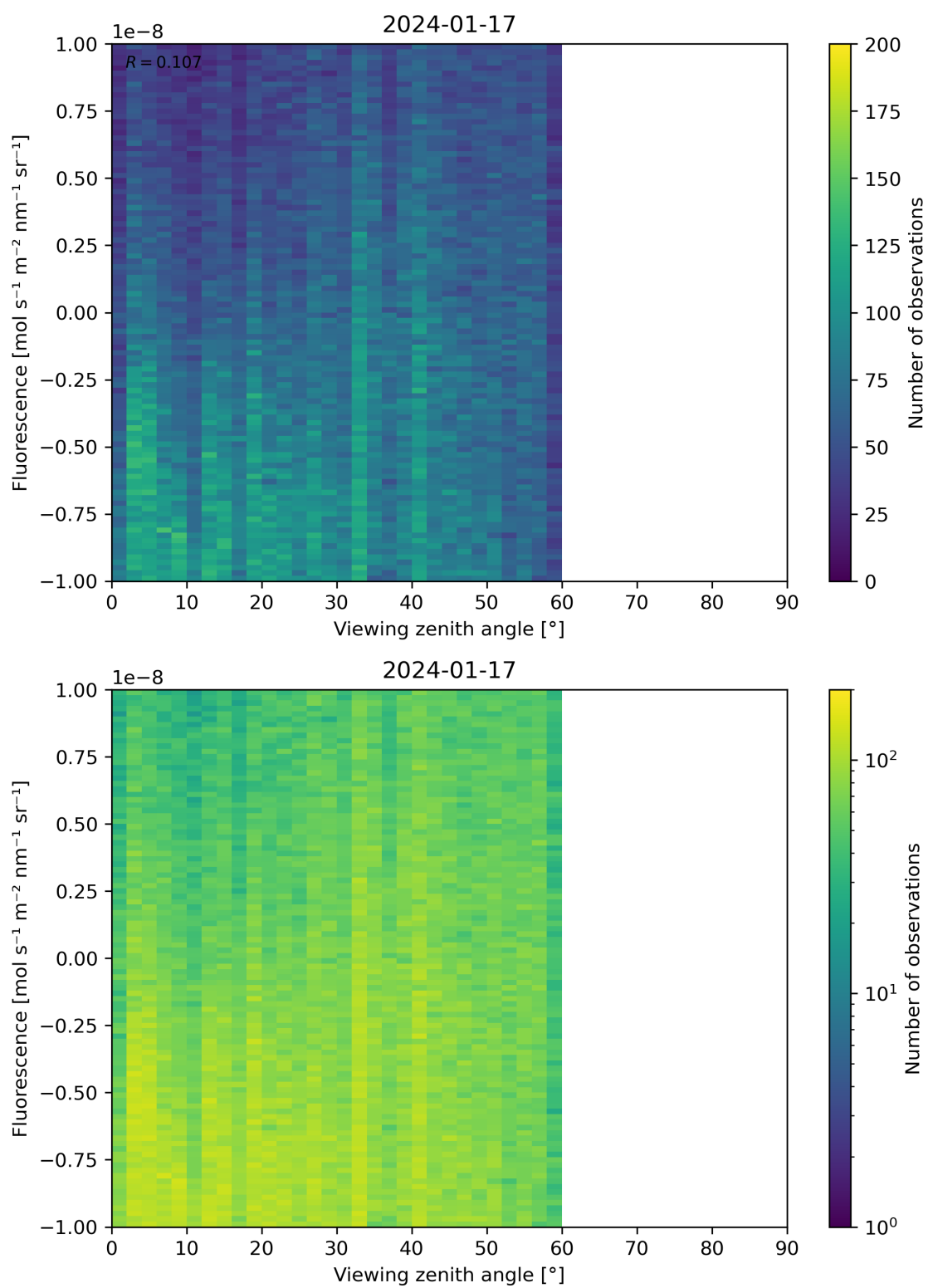
Figure 108: Scatter density plot of “Viewing zenith angle” against “Fluorescence” for 2024-01-16 to 2024-01-18.
