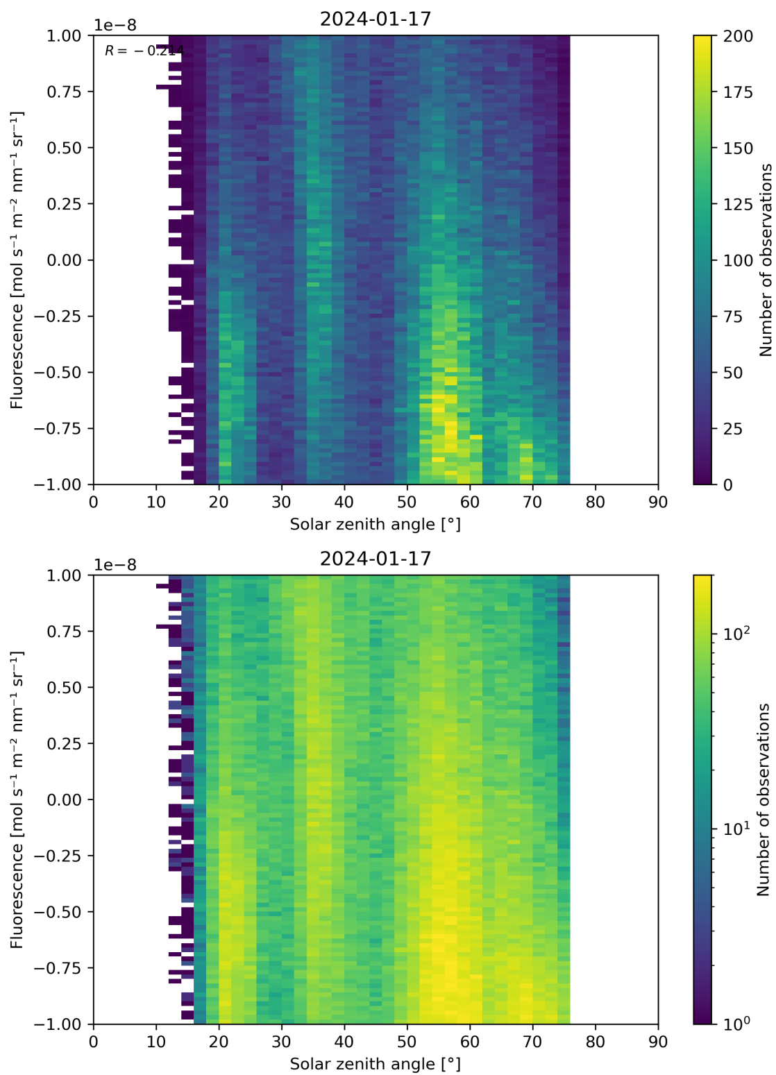
Figure 97: Scatter density plot of “Solar zenith angle” against “Fluorescence” for 2024-01-16 to 2024-01-18.
