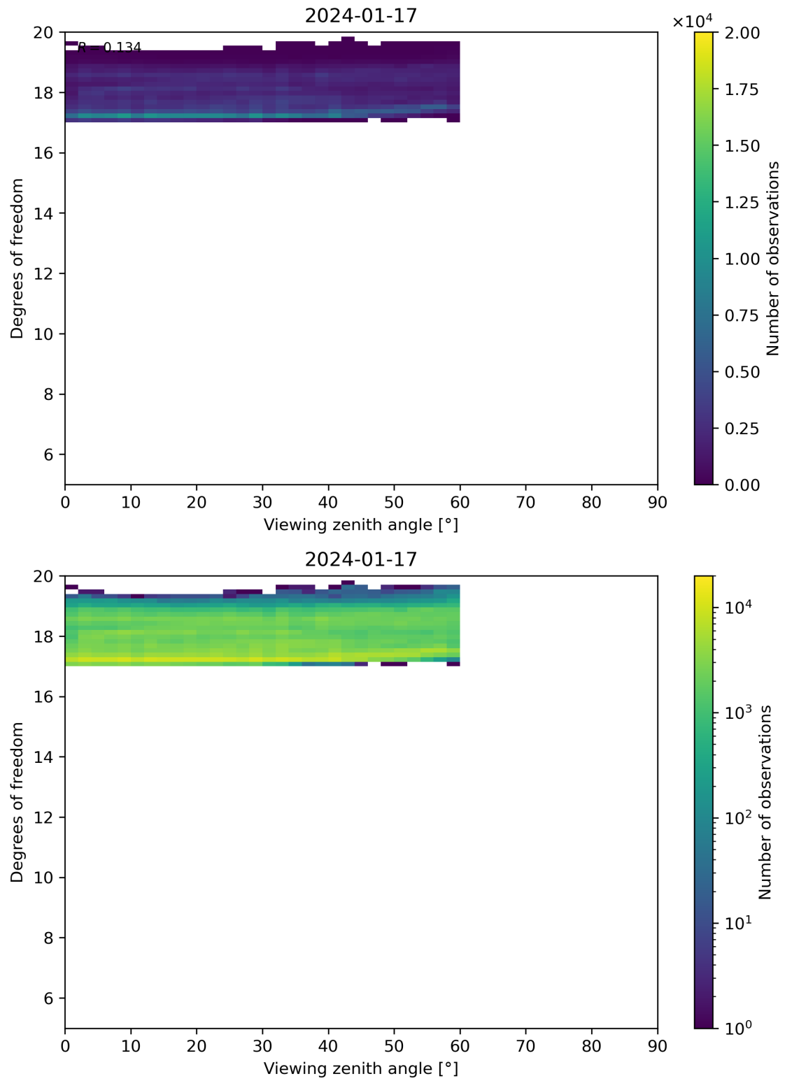
Figure 107: Scatter density plot of “Viewing zenith angle” against “Degrees of freedom” for 2024-01-16 to 2024-01-18.
