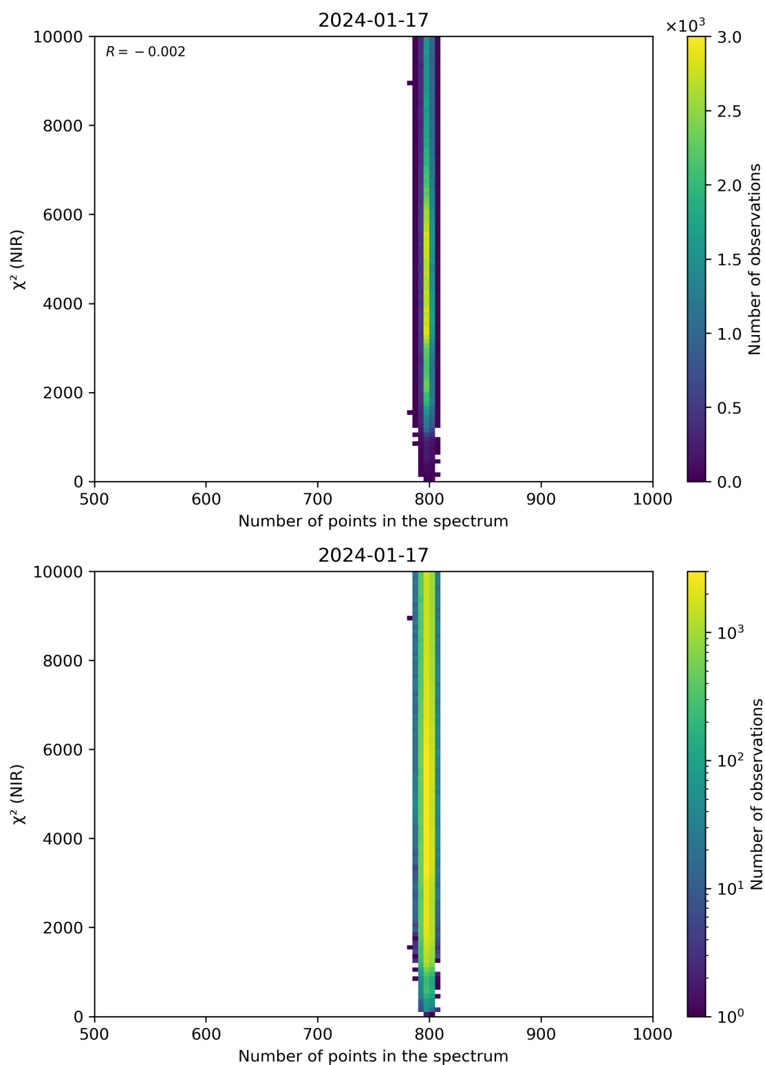
Figure 88: Scatter density plot of “Number of points in the spectrum” against “ \chi^2 (NIR)” for 2024-01-16 to 2024-01-18.
