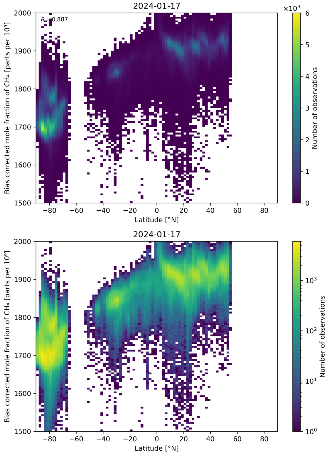
Figure 58: Scatter density plot of “Latitude” against “Bias corrected mole fraction of CH 4 ” for 2024-01-16 to 2024-01-18.
