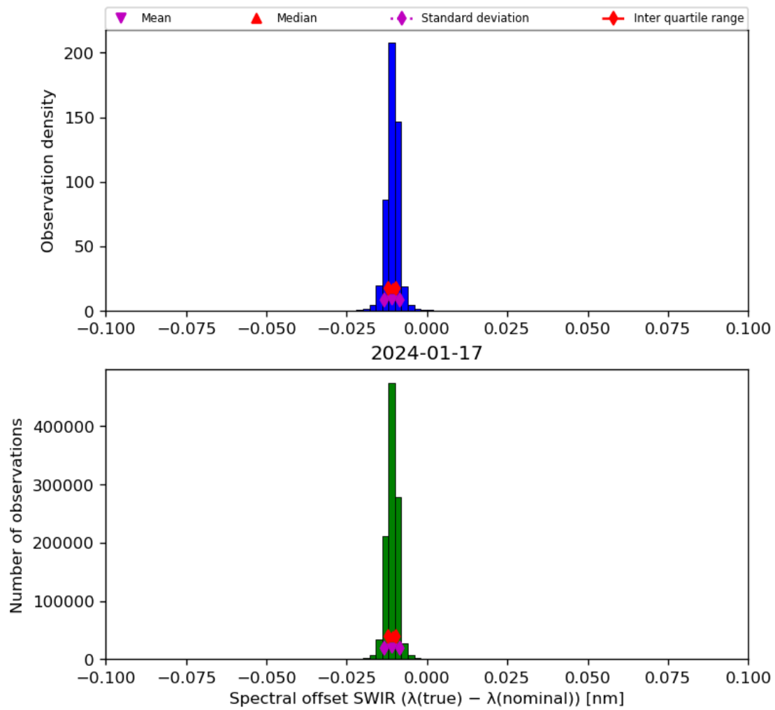
Figure 27: Histogram of “Spectral offset SWIR ( \lambda(\text{true}) - \lambda(\text{nominal}) )” for 2024-01-16 to 2024-01-18
