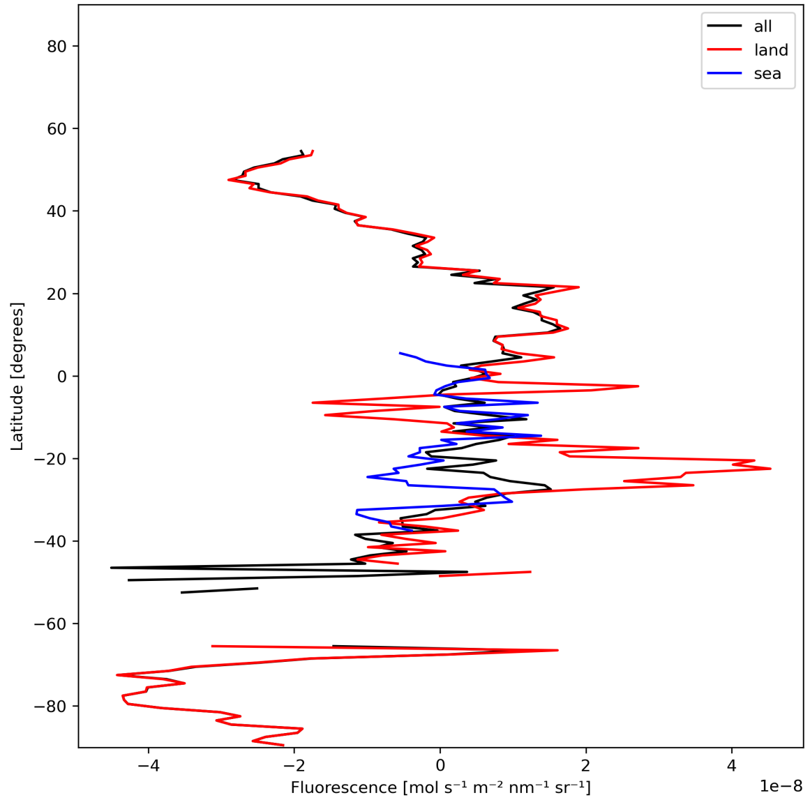
Figure 21: Zonal average of “Fluorescence” for 2024-01-16 to 2024-01-18.
