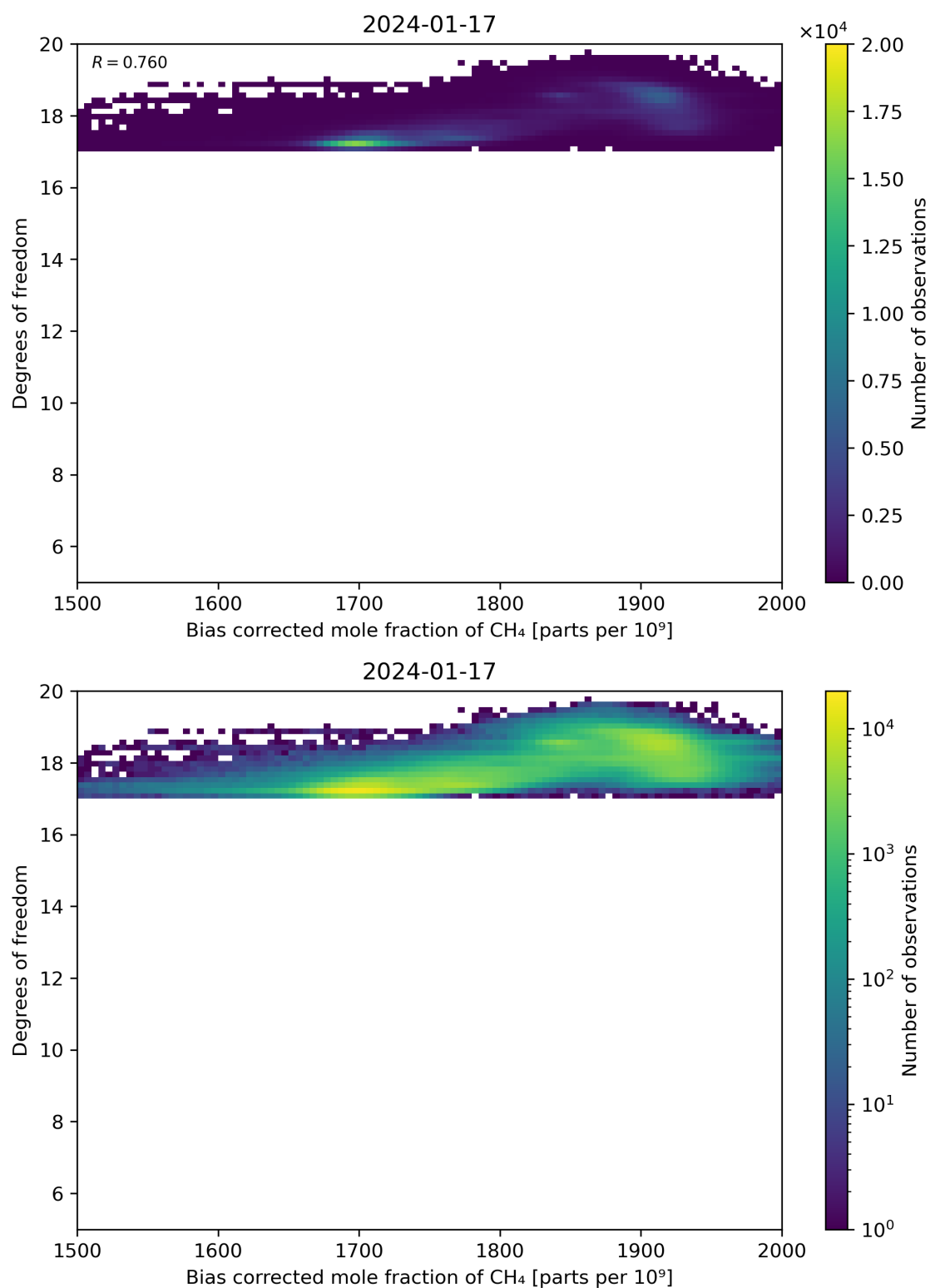
Figure 65: Scatter density plot of “Bias corrected mole fraction of CH 4 ” against “Degrees of freedom” for 2024-01-16 to 2024-01-18.
