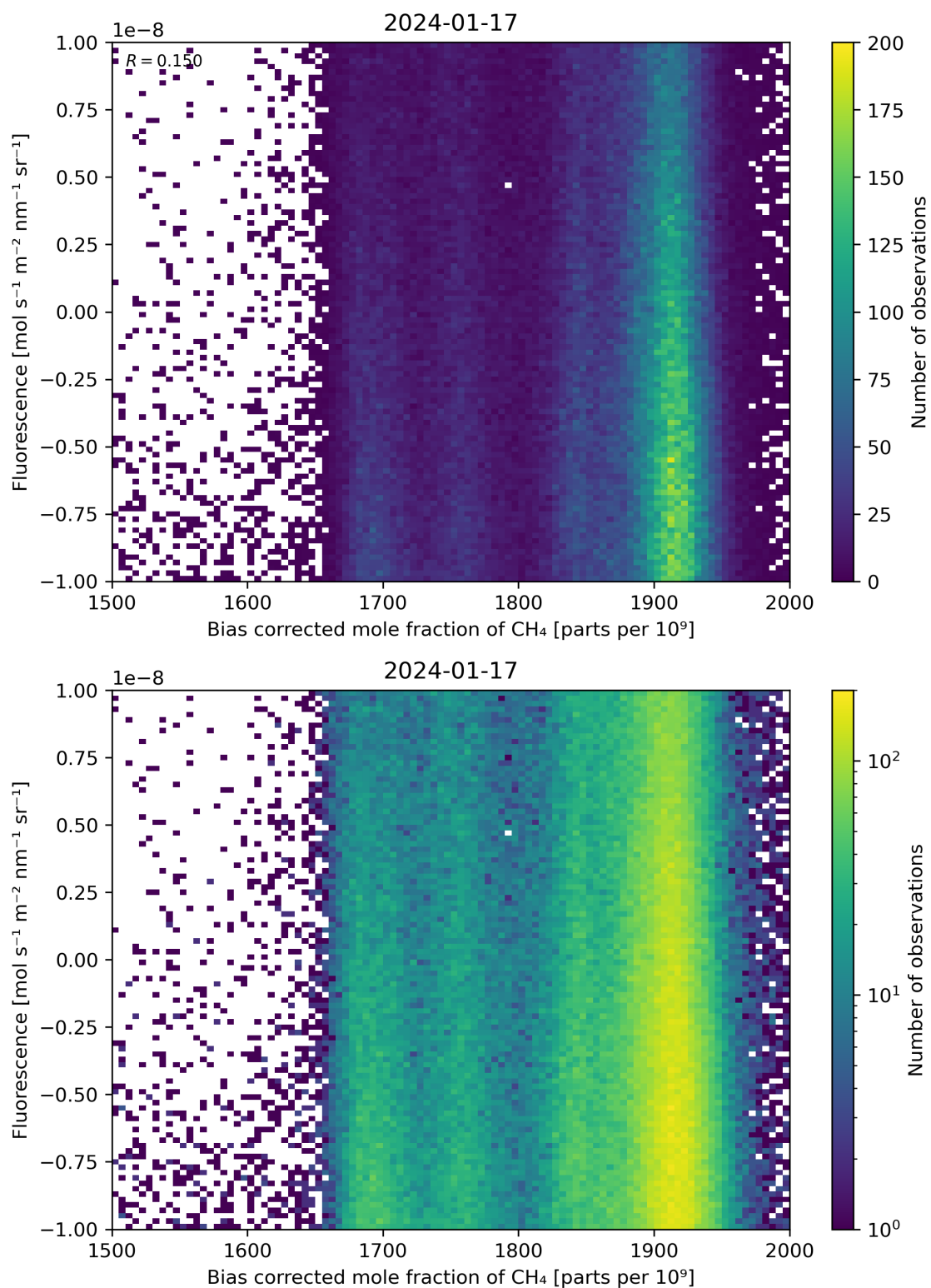
Figure 66: Scatter density plot of “Bias corrected mole fraction of \text{CH}_4 ” against “Fluorescence” for 2024-01-16 to 2024-01-18.
