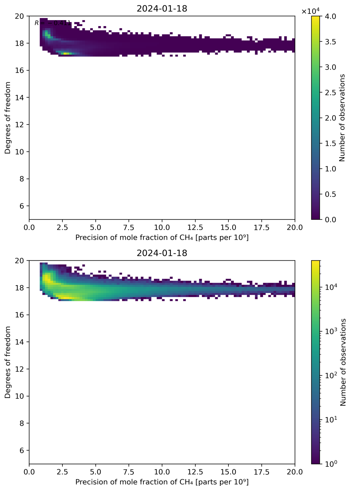
Figure 80: Scatter density plot of “Precision of mole fraction of CH 4 ” against “Degrees of freedom” for 2024-01-17 to 2024-01-19.
