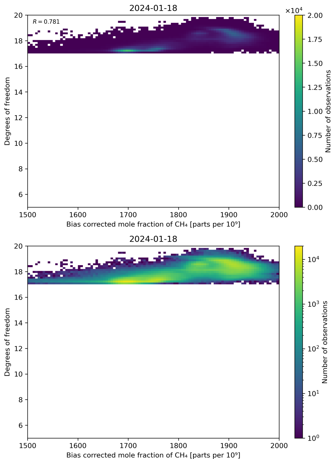
Figure 65: Scatter density plot of “Bias corrected mole fraction of CH 4 ” against “Degrees of freedom” for 2024-01-17 to 2024-01-19.
