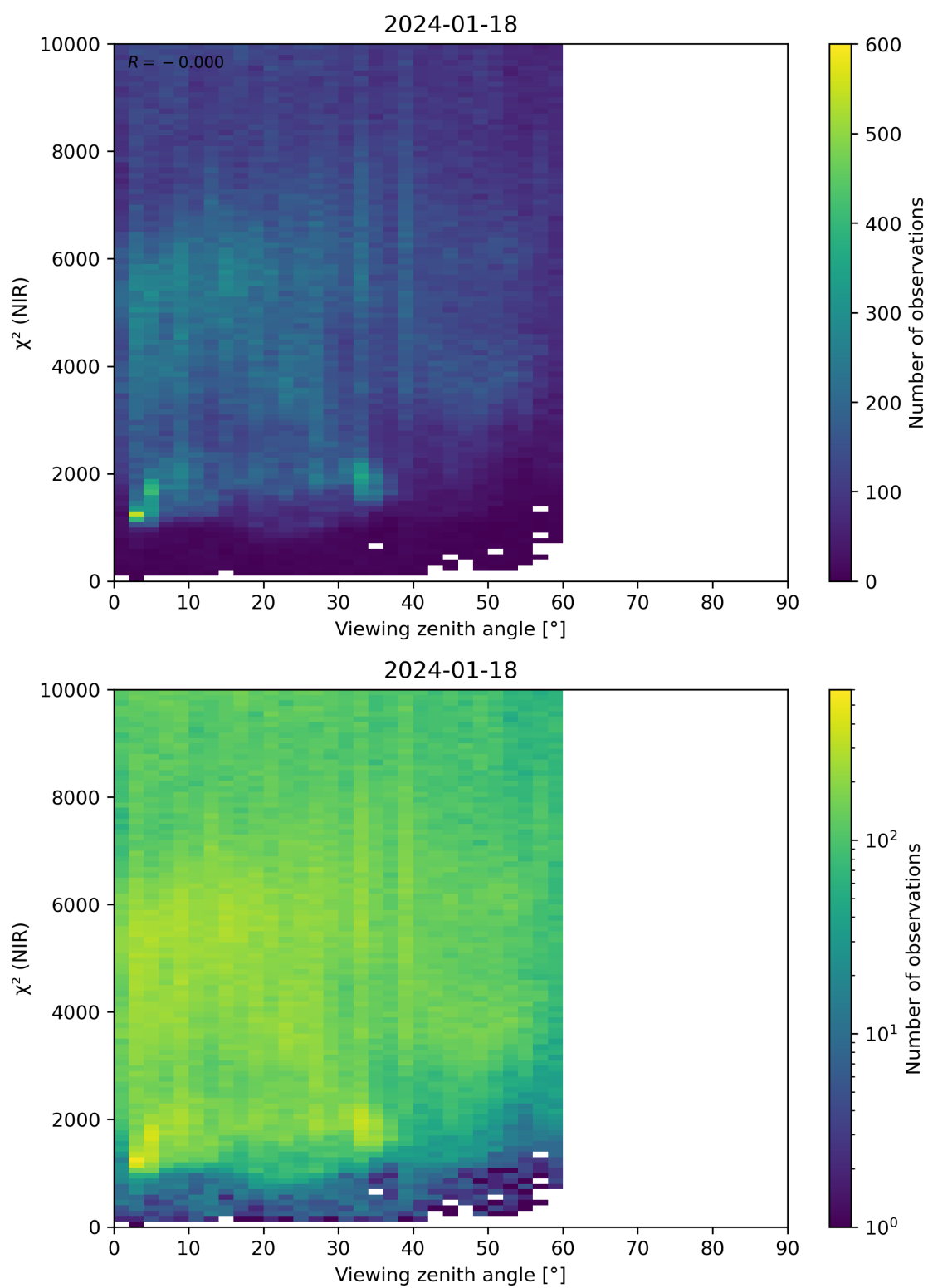
Figure 105: Scatter density plot of “Viewing zenith angle” against “ \chi^2 (NIR)” for 2024-01-17 to 2024-01-19.
