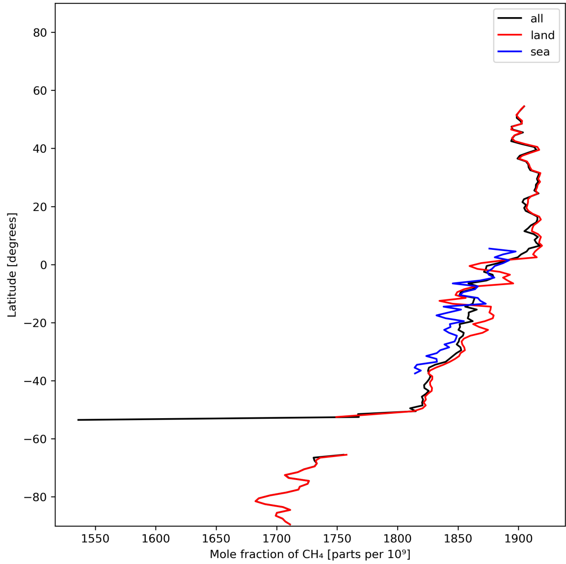
Figure 12: Zonal average of “Mole fraction of \text{CH}_4 ” for 2024-01-17 to 2024-01-19.
