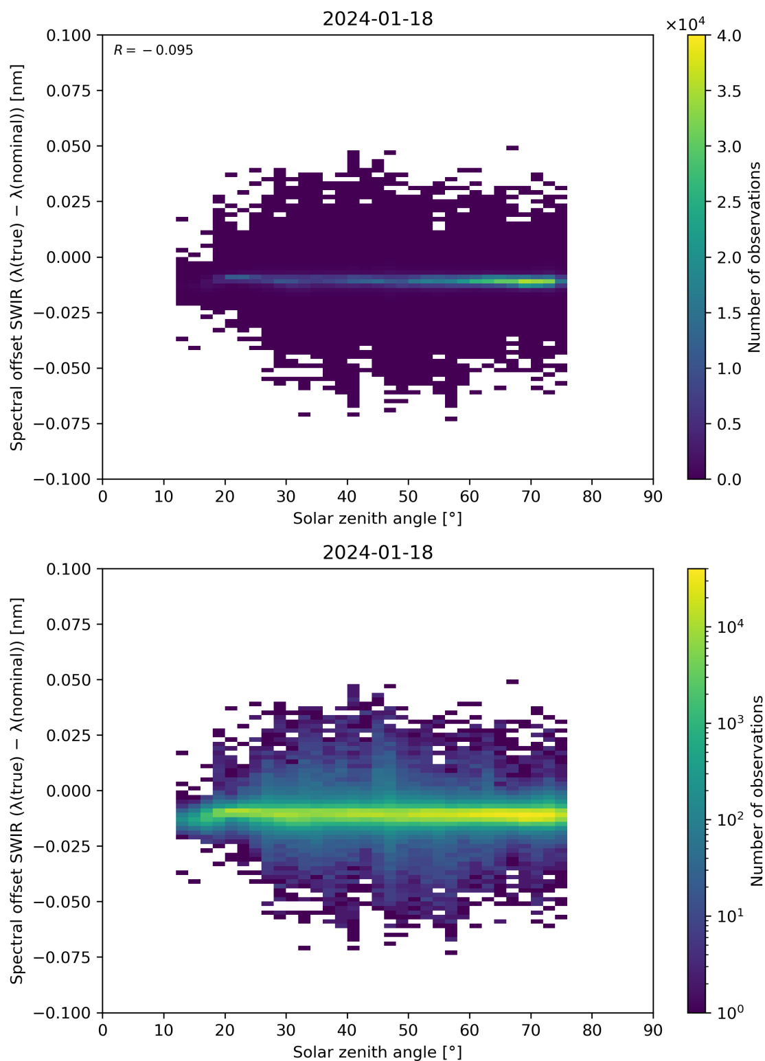
Figure 104: Scatter density plot of “Solar zenith angle” against “Spectral offset SWIR ( \lambda(\text{true}) - \lambda(\text{nominal}) )” for 2024-01-17 to 2024-01-19.
