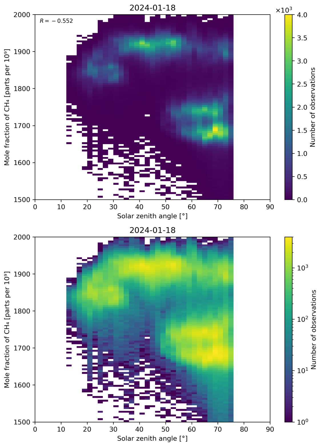
Figure 99: Scatter density plot of “Solar zenith angle” against “Mole fraction of CH 4 ” for 2024-01-17 to 2024-01-19.
