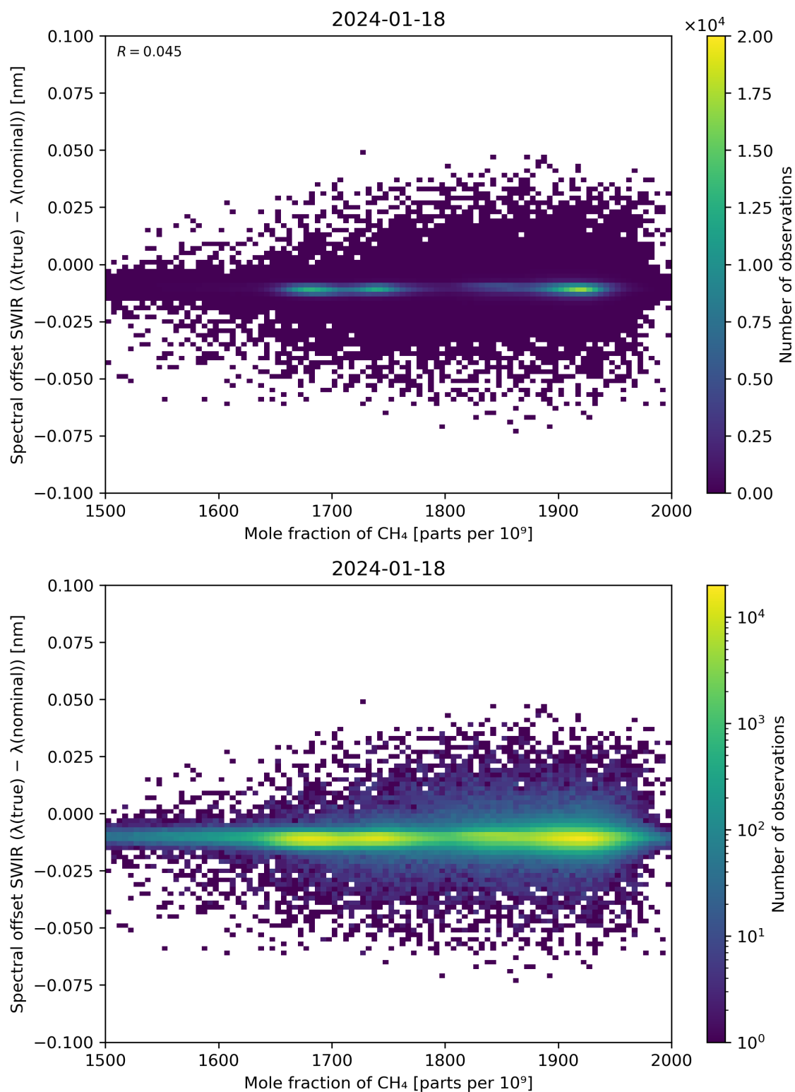
Figure 86: Scatter density plot of “Mole fraction of CH 4 ” against “Spectral offset SWIR ( \lambda(\text{true}) - \lambda(\text{nominal}) )” for 2024-01-17 to 2024-01-19.
