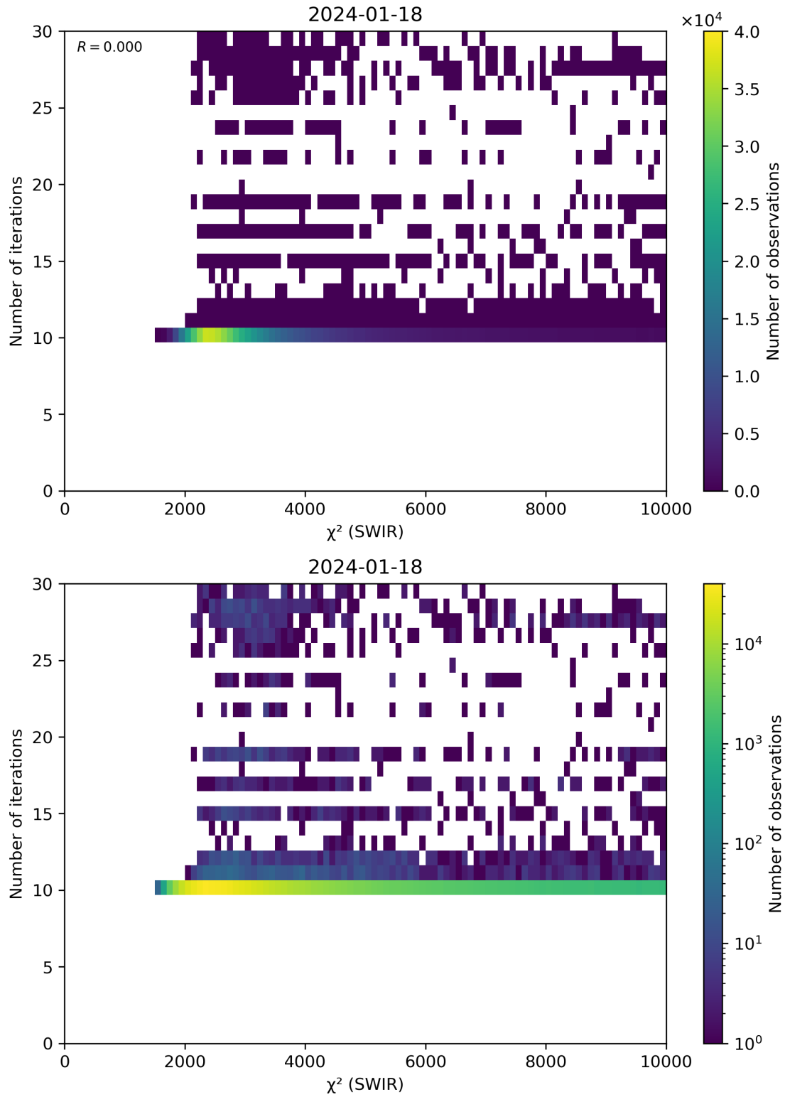
Figure 50: Scatter density plot of “ \chi^2 (SWIR)” against “Number of iterations” for 2024-01-17 to 2024-01-19.
