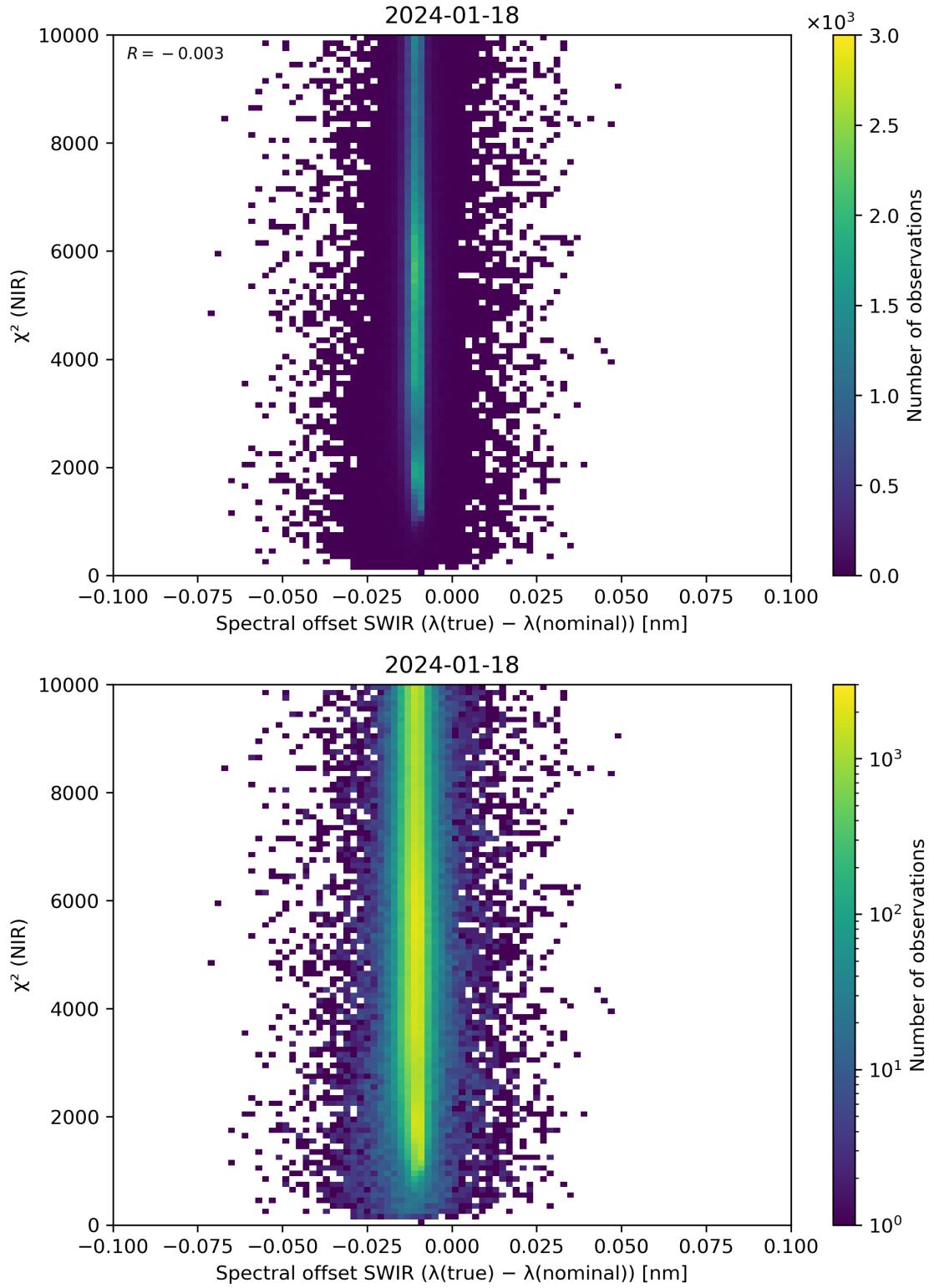
Figure 117: Scatter density plot of “Spectral offset SWIR ( \lambda(\text{true}) - \lambda(\text{nominal}) )” against “ \chi^2 (NIR)” for 2024-01-17 to 2024-01-19.
