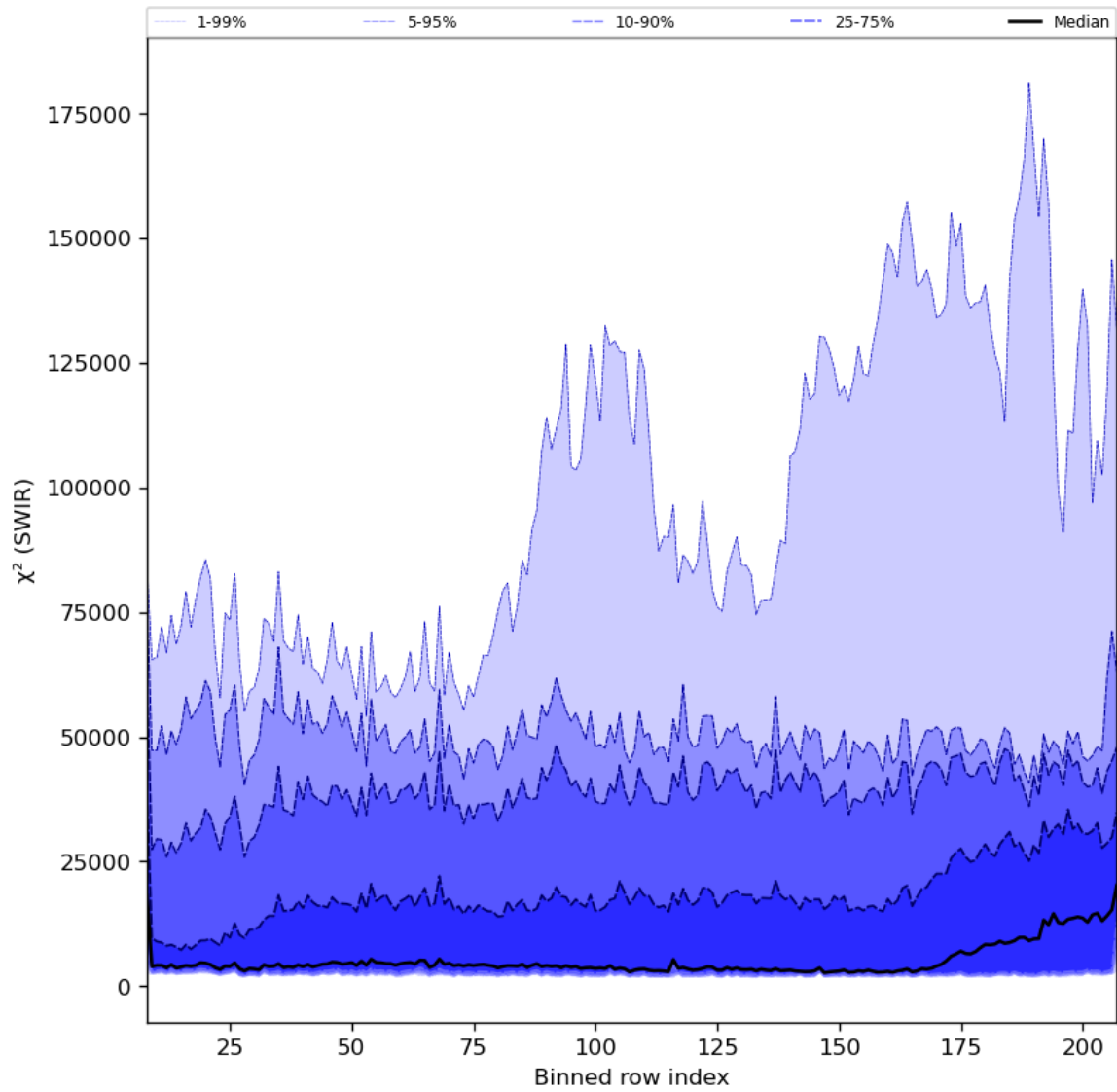
Figure 39: Along track statistics of “ \chi^2 (SWIR)” for 2024-01-17 to 2024-01-19
