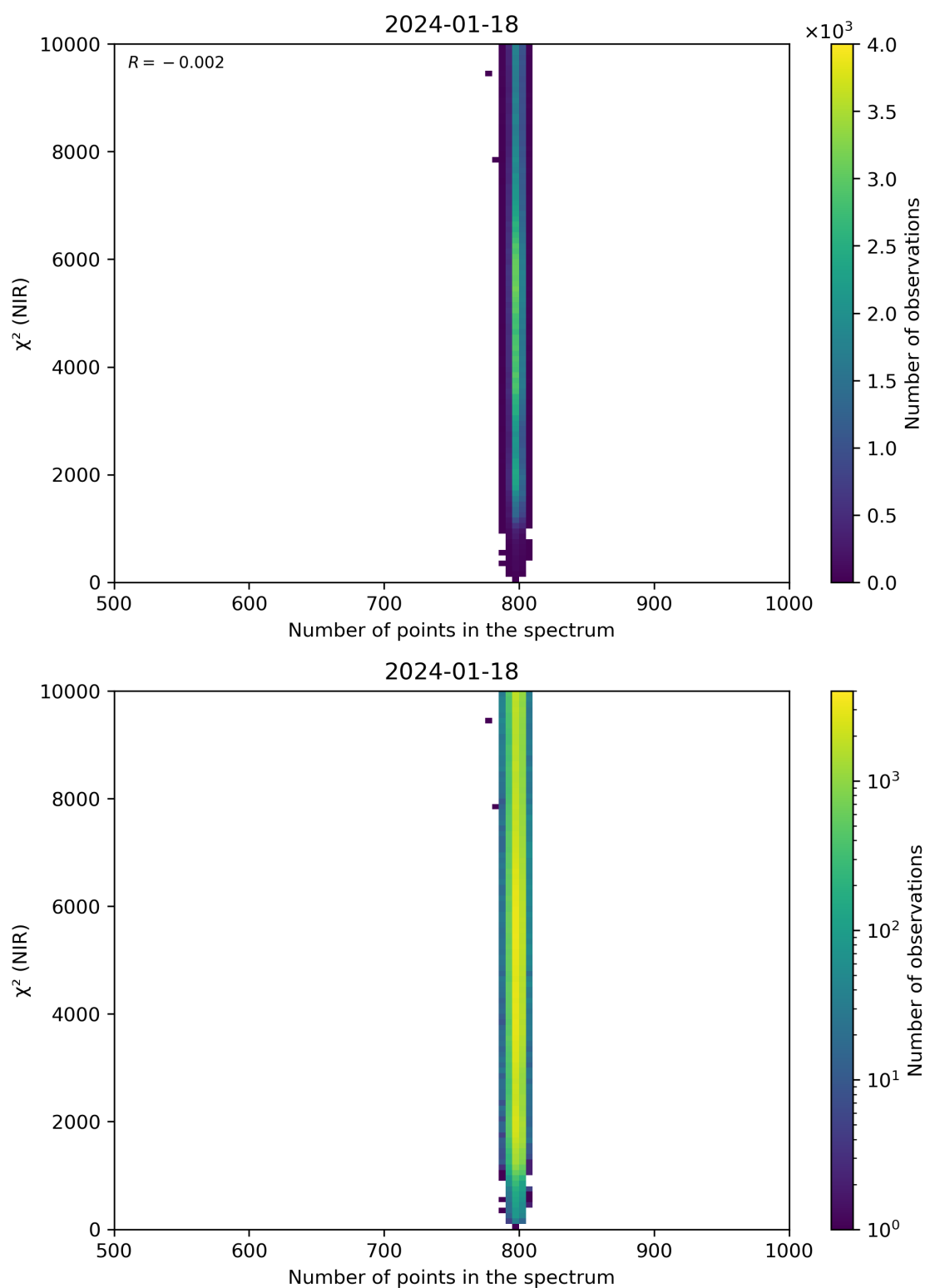
Figure 88: Scatter density plot of “Number of points in the spectrum” against “ \chi^2 (NIR)” for 2024-01-17 to 2024-01-19.
