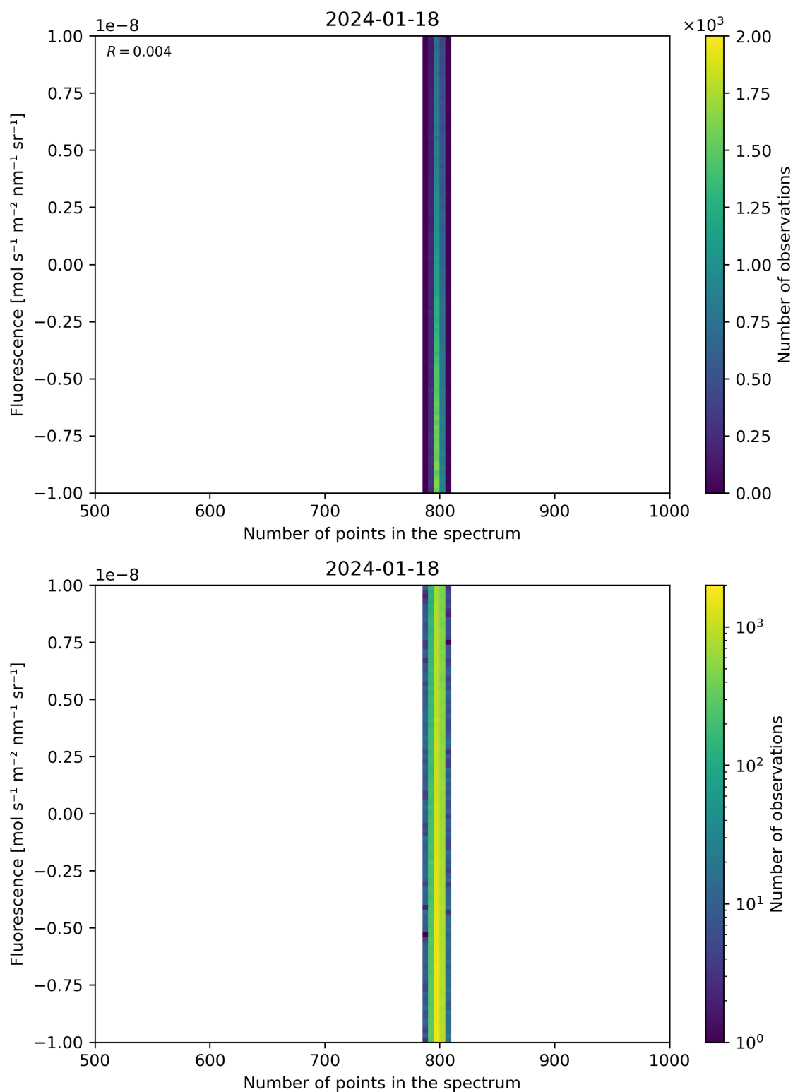
Figure 91: Scatter density plot of “Number of points in the spectrum” against “Fluorescence” for 2024-01-17 to 2024-01-19.
