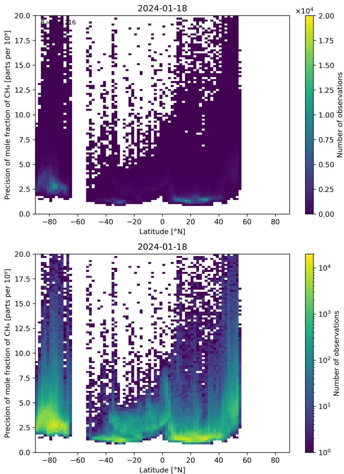
Figure 59: Scatter density plot of “Latitude” against “Precision of mole fraction of CH 4 ” for 2024-01-17 to 2024-01-19.
