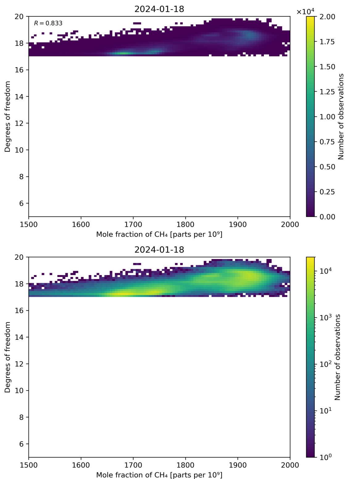
Figure 72: Scatter density plot of “Mole fraction of CH 4 ” against “Degrees of freedom” for 2024-01-17 to 2024-01-19.
