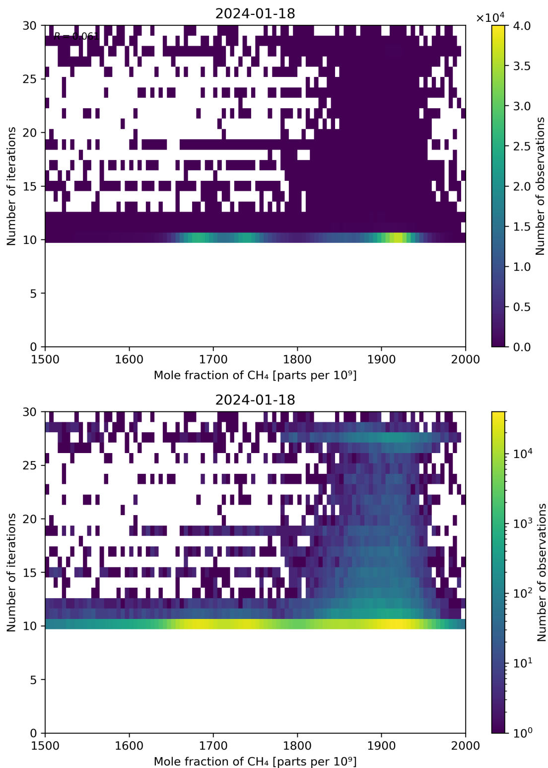
Figure 76: Scatter density plot of “Mole fraction of CH 4 ” against “Number of iterations” for 2024-01-17 to 2024-01-19.
