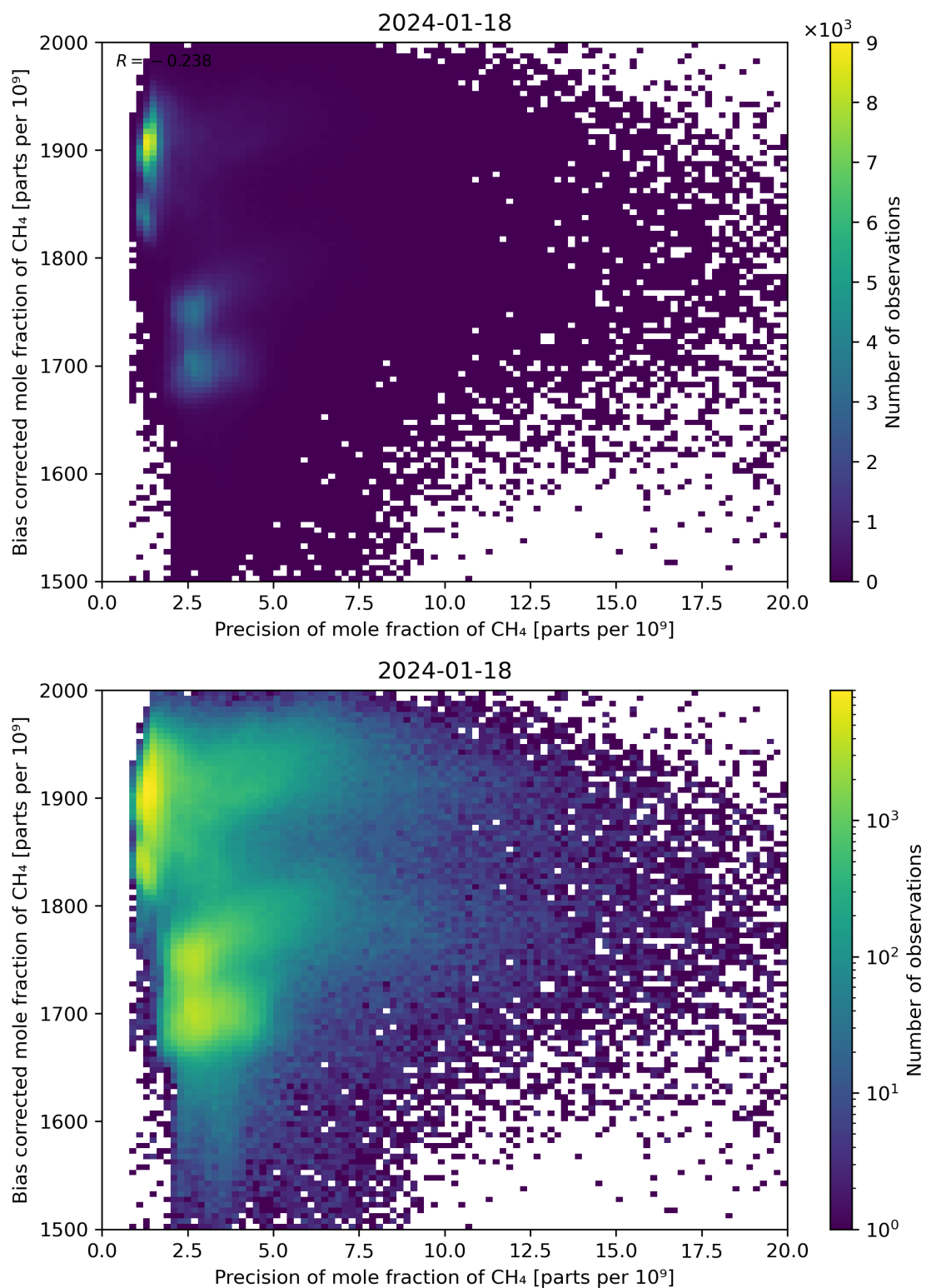
Figure 82: Scatter density plot of “Precision of mole fraction of CH 4 ” against “Bias corrected mole fraction of CH 4 ” for 2024-01-17 to 2024-01-19.
