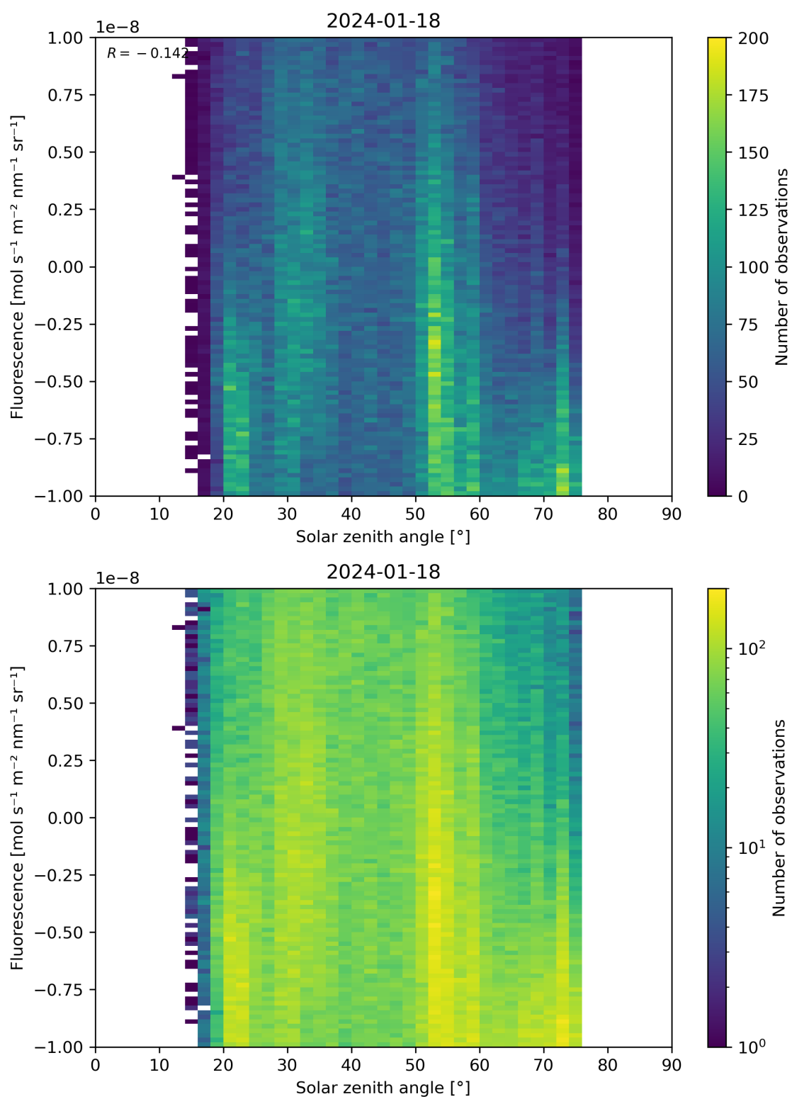
Figure 97: Scatter density plot of “Solar zenith angle” against “Fluorescence” for 2024-01-17 to 2024-01-19.
