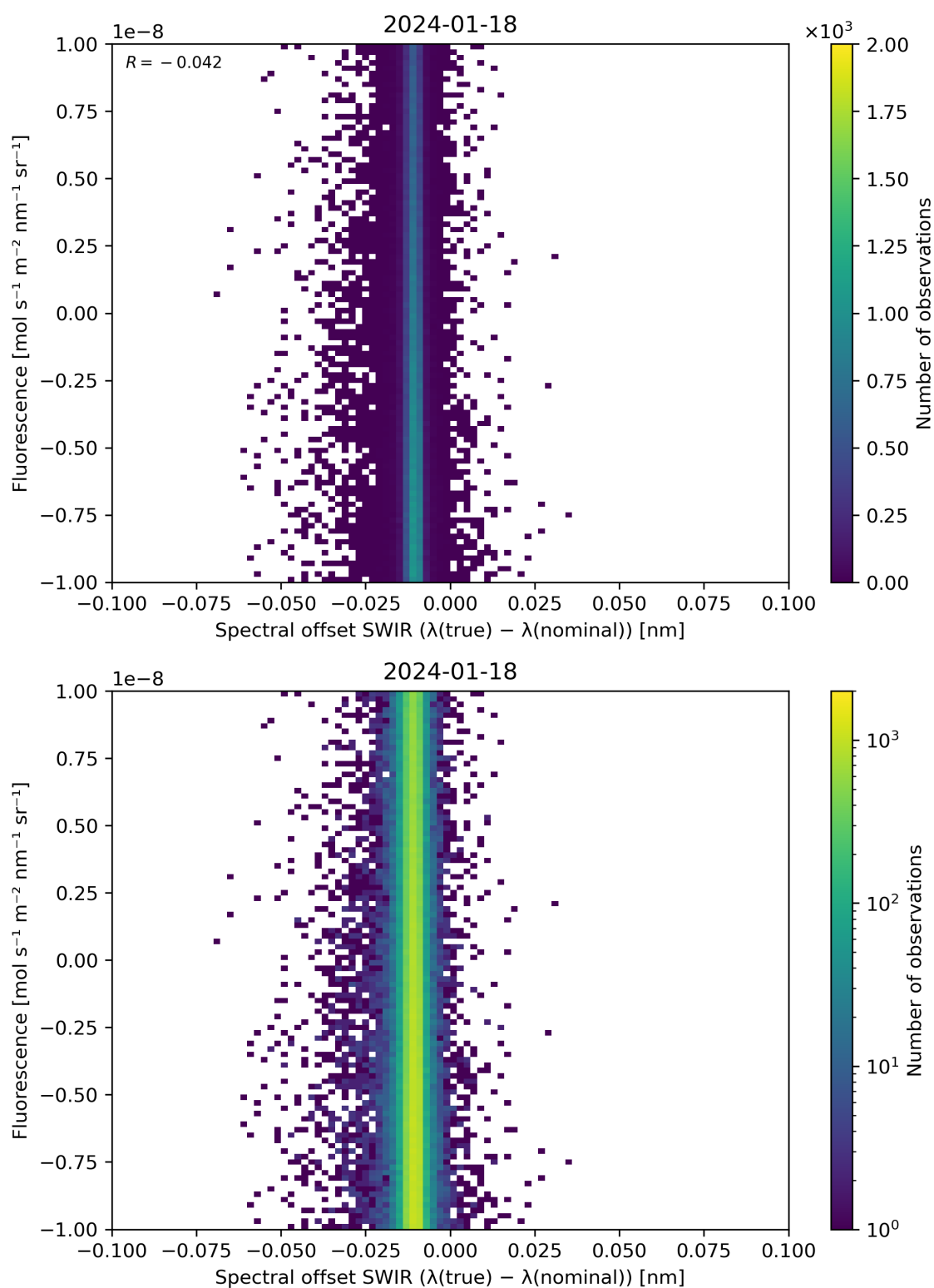
Figure 120: Scatter density plot of “Spectral offset SWIR ( \lambda(\text{true}) - \lambda(\text{nominal}) )” against “Fluorescence” for 2024-01-17 to 2024-01-19.
