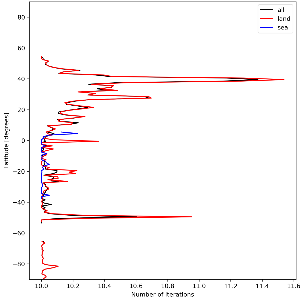
Figure 20: Zonal average of “Number of iterations” for 2024-01-17 to 2024-01-19.
