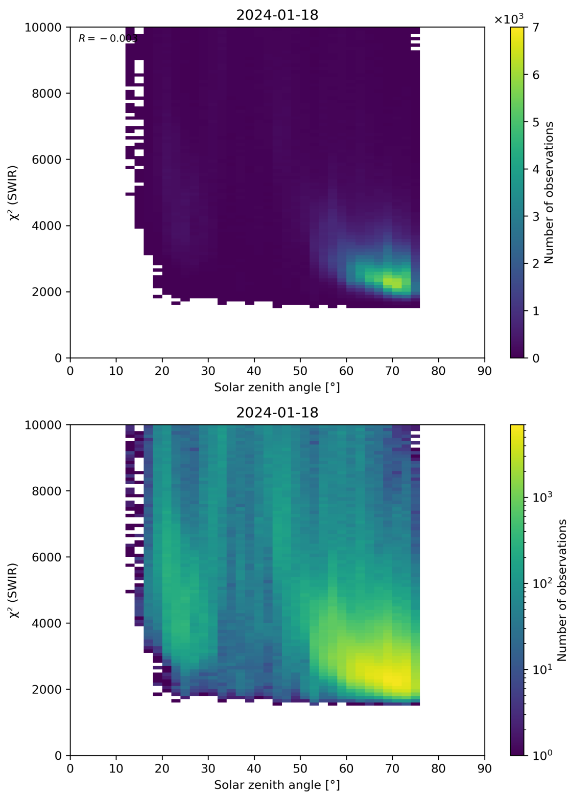
Figure 95: Scatter density plot of “Solar zenith angle” against “ \chi^2 (SWIR)” for 2024-01-17 to 2024-01-19.
