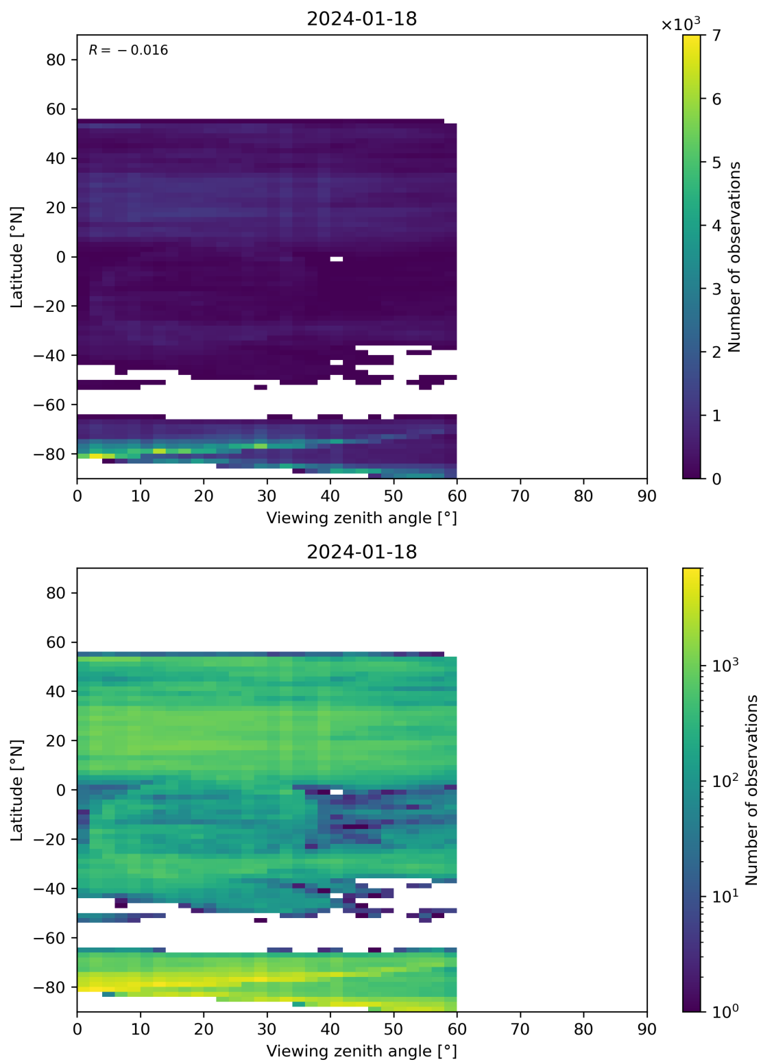
Figure 109: Scatter density plot of “Viewing zenith angle” against “Latitude” for 2024-01-17 to 2024-01-19.
