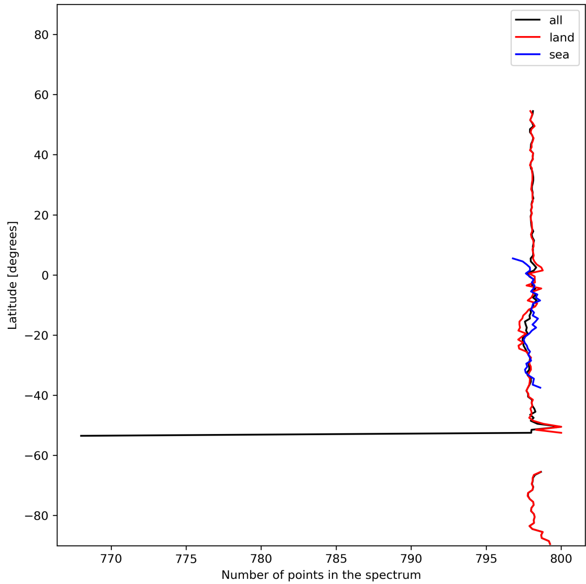
Figure 15: Zonal average of “Number of points in the spectrum” for 2024-01-17 to 2024-01-19.
