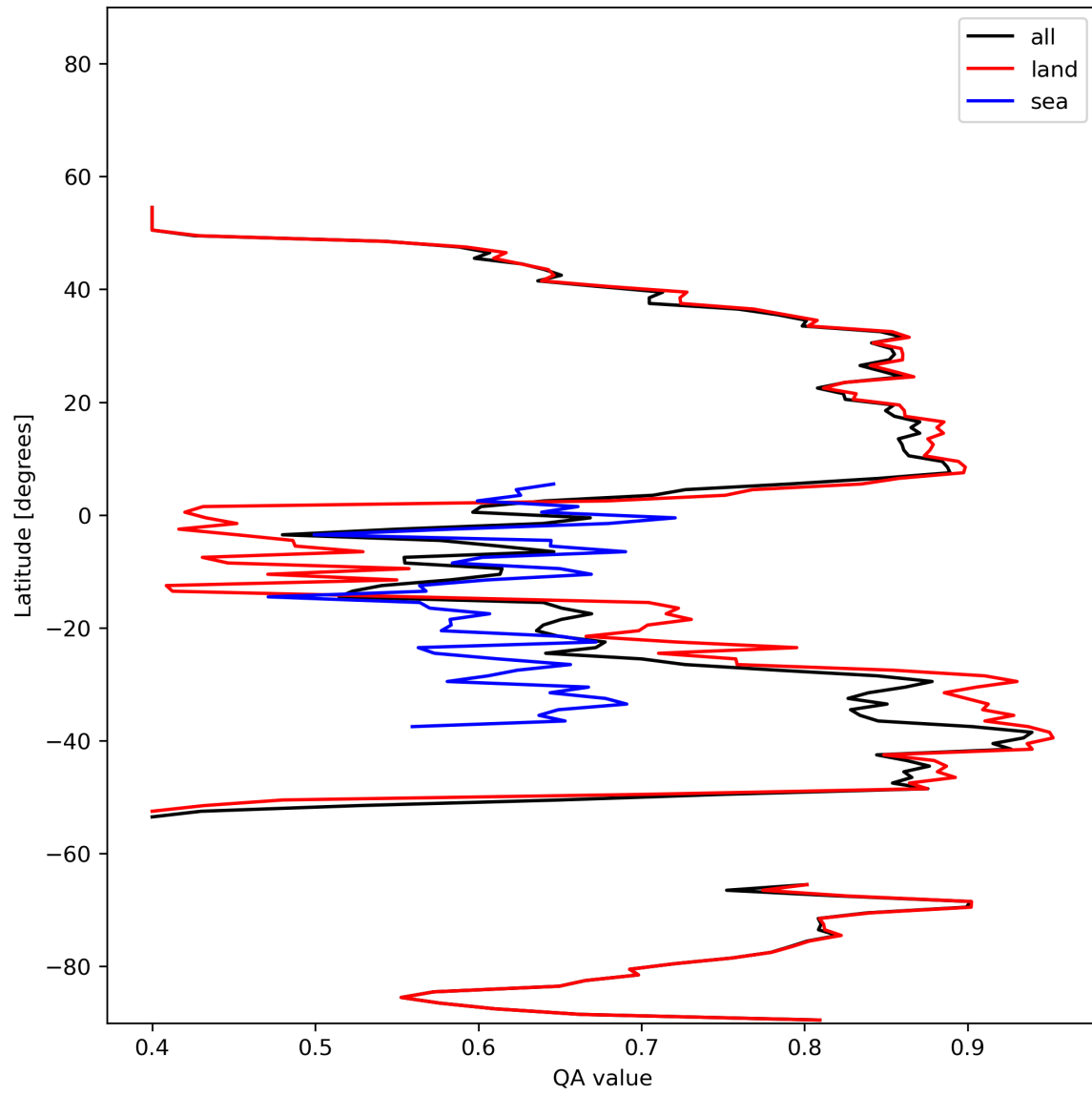
Figure 11: Zonal average of “QA value” for 2024-01-17 to 2024-01-19.
