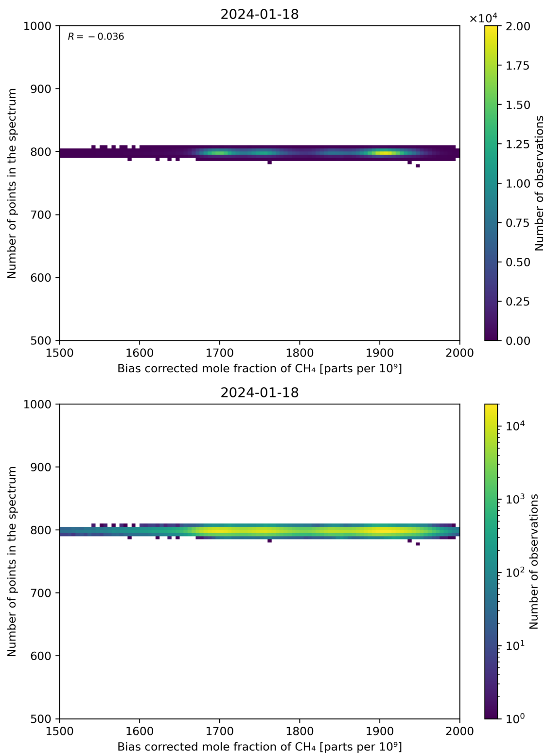
Figure 68: Scatter density plot of “Bias corrected mole fraction of CH 4 ” against “Number of points in the spectrum” for 2024-01-17 to 2024-01-19.
