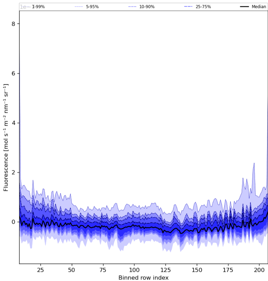
Figure 43: Along track statistics of “Fluorescence” for 2024-01-17 to 2024-01-19
