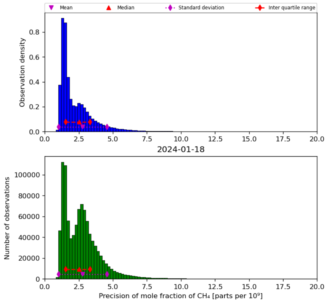
Figure 24: Histogram of “Precision of mole fraction of CH 4 ” for 2024-01-17 to 2024-01-19
