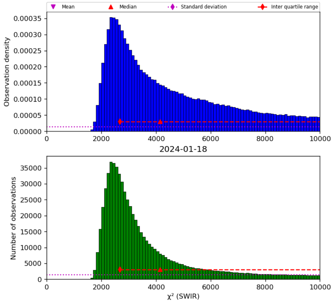
Figure 28: Histogram of “ \chi^2 (SWIR)” for 2024-01-17 to 2024-01-19
