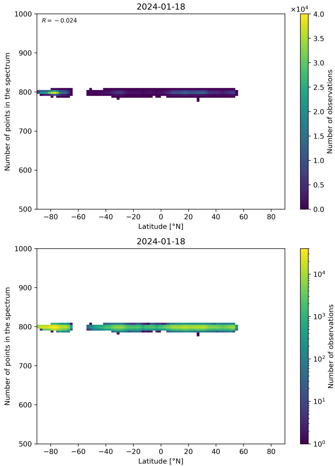
Figure 61: Scatter density plot of “Latitude” against “Number of points in the spectrum” for 2024-01-17 to 2024-01-19.
