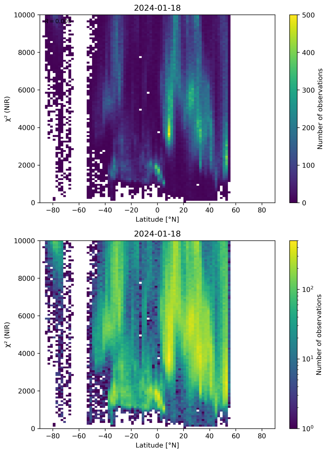
Figure 53: Scatter density plot of “Latitude” against “ \chi^2 (NIR)” for 2024-01-17 to 2024-01-19.
