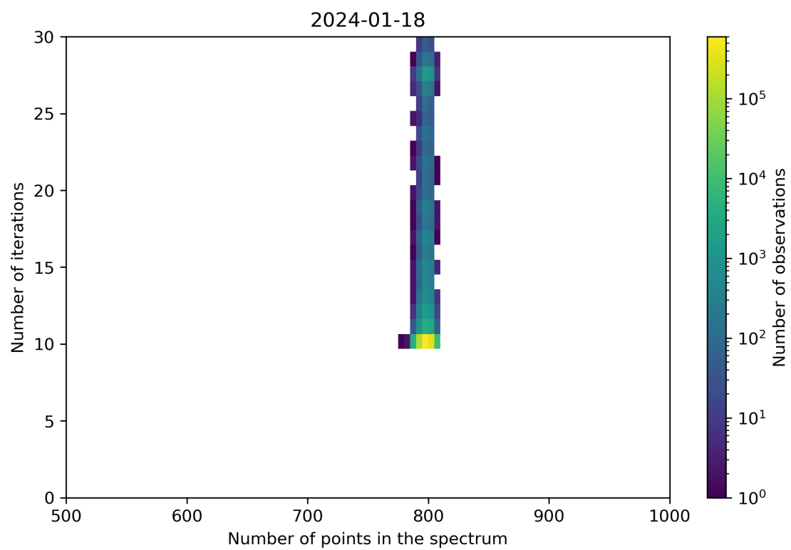
Figure 92: Scatter density plot of “Number of points in the spectrum” against “Number of iterations” for 2024-01-17 to 2024-01-19.
