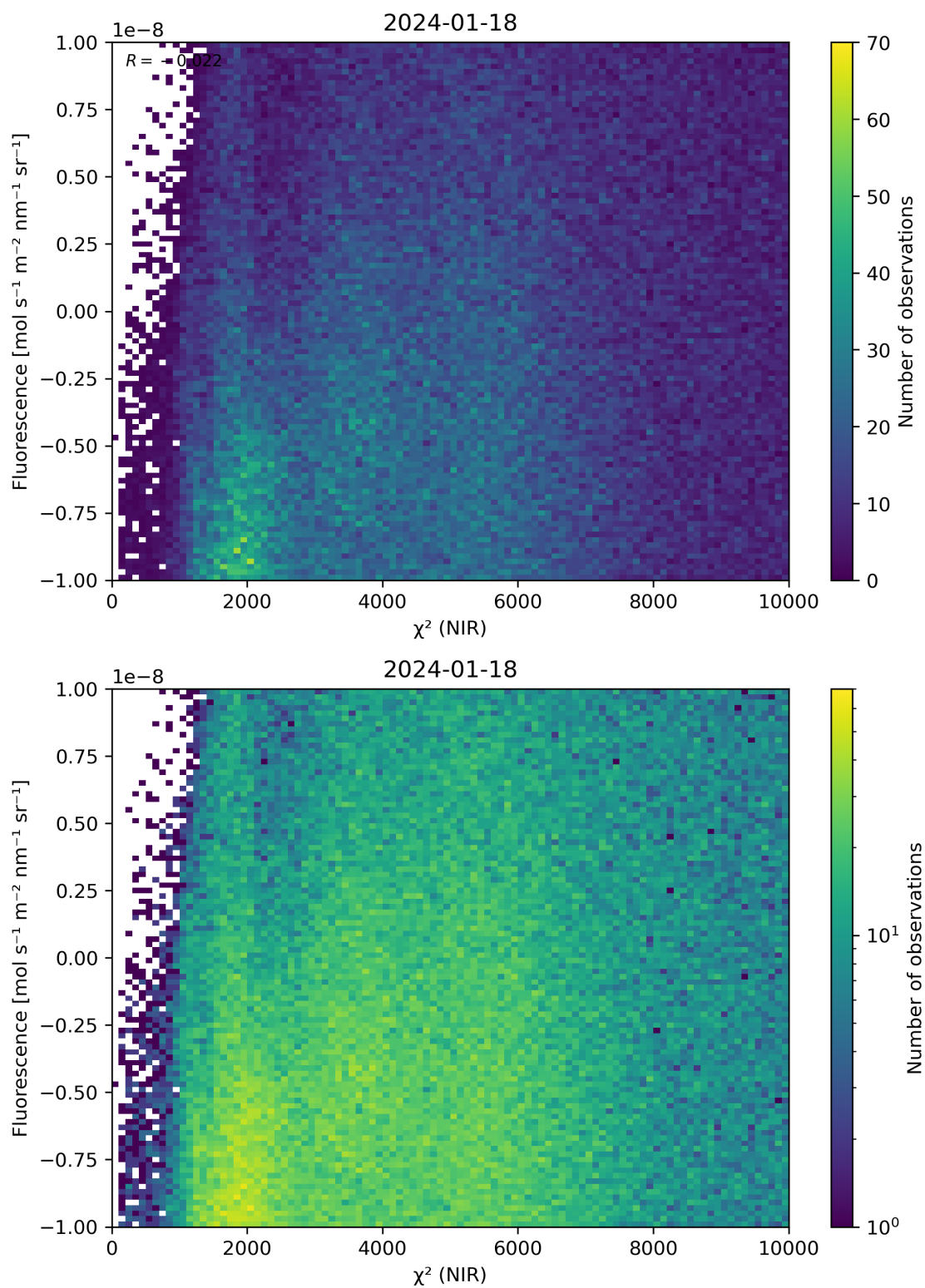
Figure 45: Scatter density plot of “ \chi^2 (NIR)” against “Fluorescence” for 2024-01-17 to 2024-01-19.
