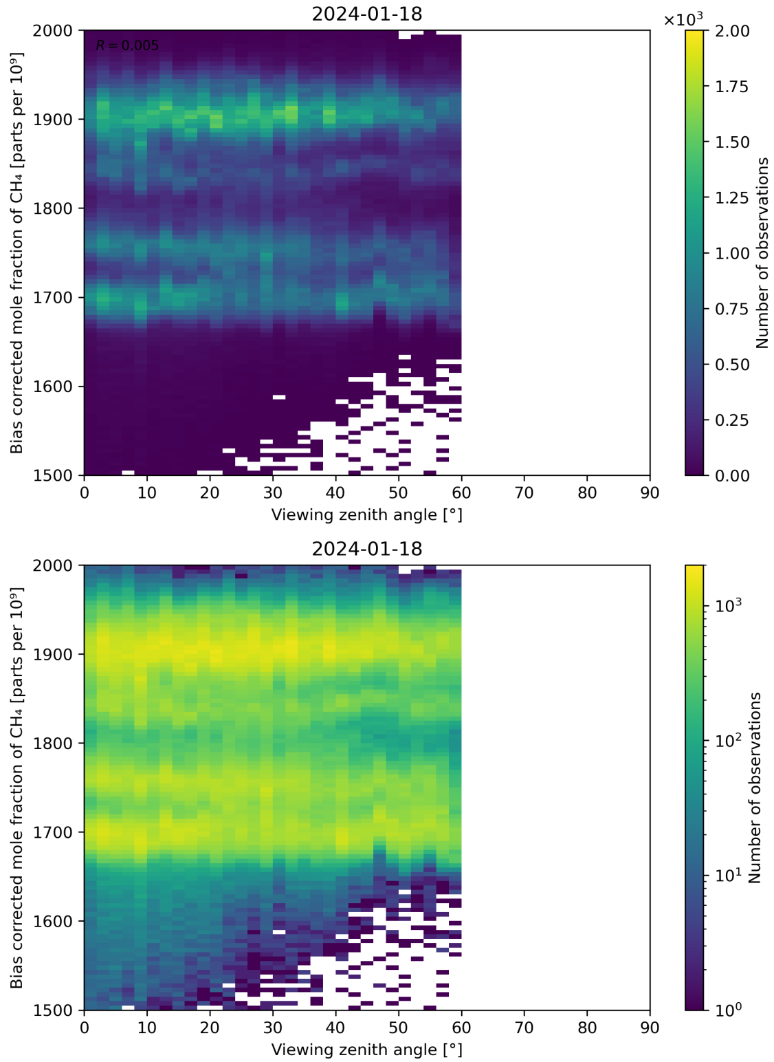
Figure 111: Scatter density plot of “Viewing zenith angle” against “Bias corrected mole fraction of CH 4 ” for 2024-01-17 to 2024-01-19.
