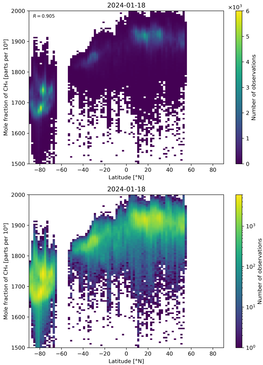
Figure 57: Scatter density plot of “Latitude” against “Mole fraction of \text{CH}_4 ” for 2024-01-17 to 2024-01-19.
