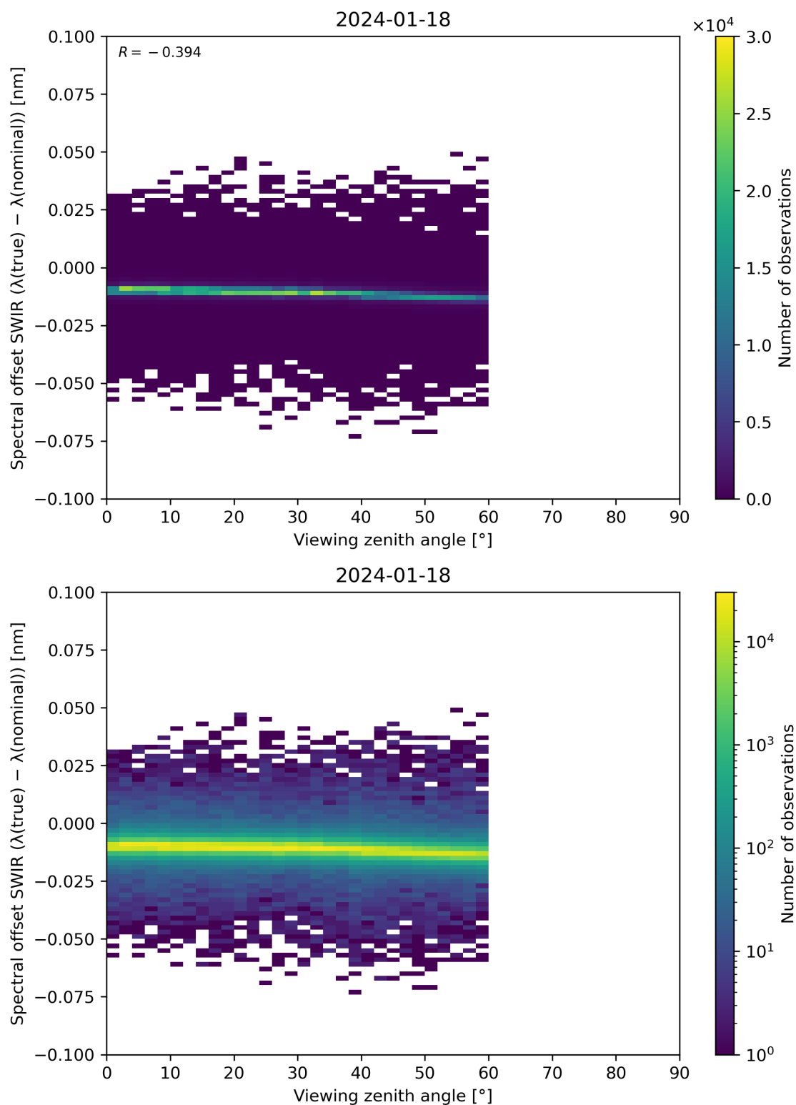
Figure 116: Scatter density plot of “Viewing zenith angle” against “Spectral offset SWIR ( \lambda(\text{true}) - \lambda(\text{nominal}) )” for 2024-01-17 to 2024-01-19.
