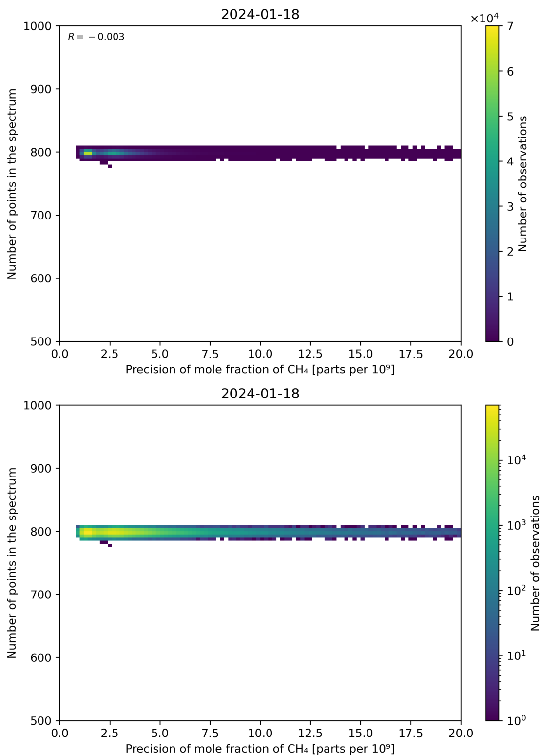
Figure 84: Scatter density plot of “Precision of mole fraction of CH 4 ” against “Number of points in the spectrum” for 2024-01-17 to 2024-01-19.
