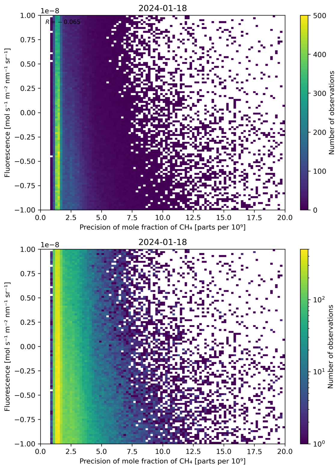
Figure 81: Scatter density plot of “Precision of mole fraction of \text{CH}_4 ” against “Fluorescence” for 2024-01-17 to 2024-01-19.
