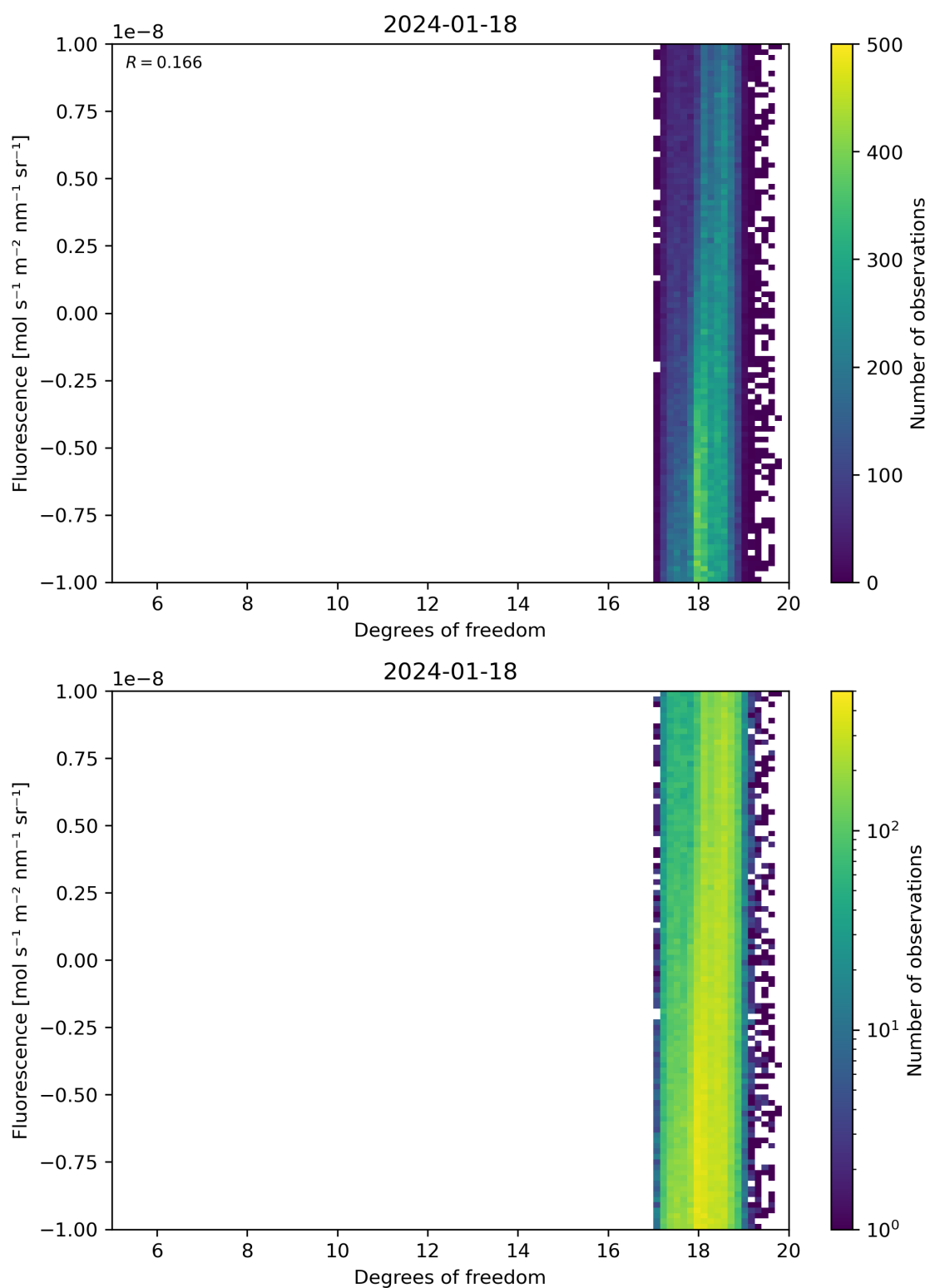
Figure 51: Scatter density plot of “Degrees of freedom” against “Fluorescence” for 2024-01-17 to 2024-01-19.
