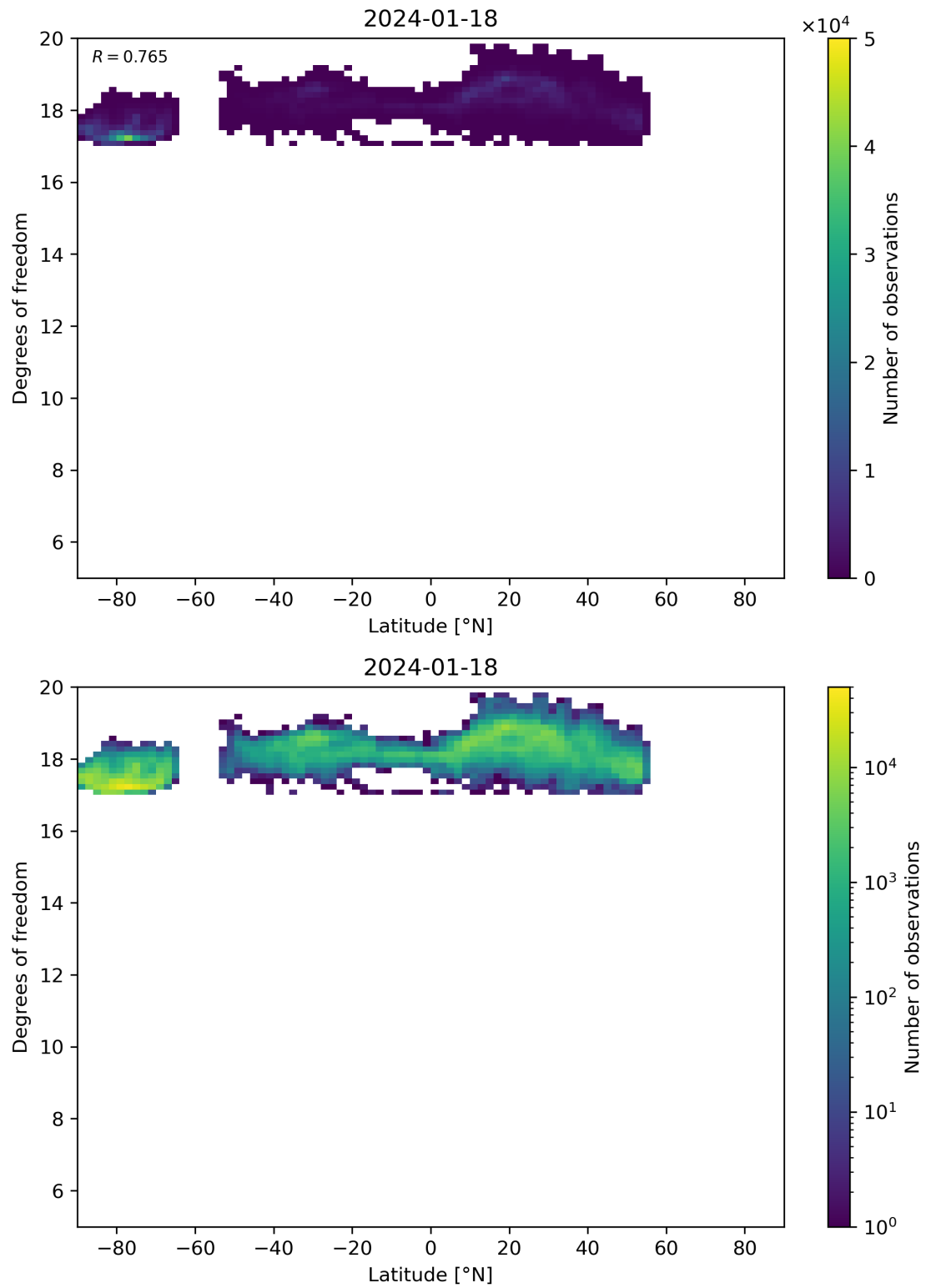
Figure 55: Scatter density plot of “Latitude” against “Degrees of freedom” for 2024-01-17 to 2024-01-19.
