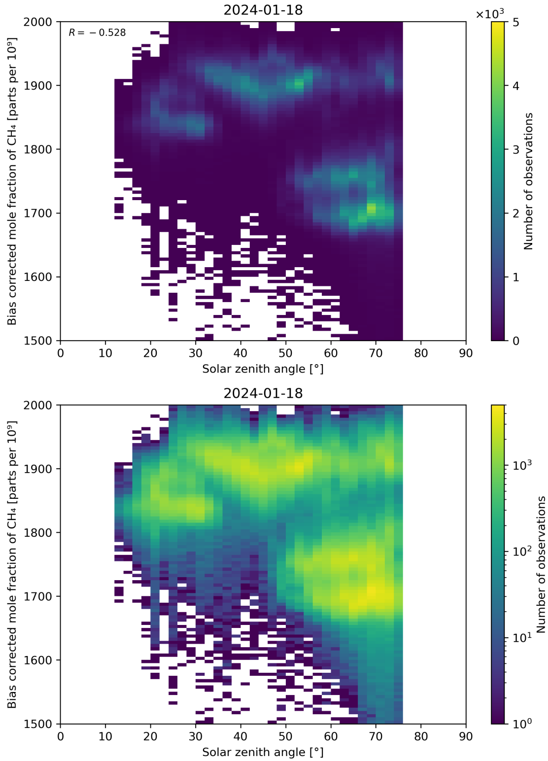
Figure 100: Scatter density plot of “Solar zenith angle” against “Bias corrected mole fraction of CH 4 ” for 2024-01-17 to 2024-01-19.
