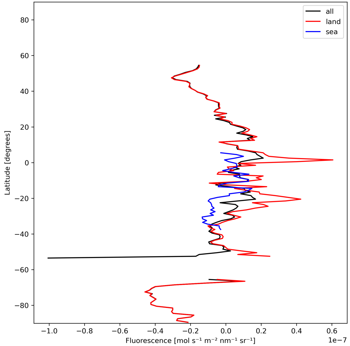
Figure 21: Zonal average of “Fluorescence” for 2024-01-17 to 2024-01-19.
