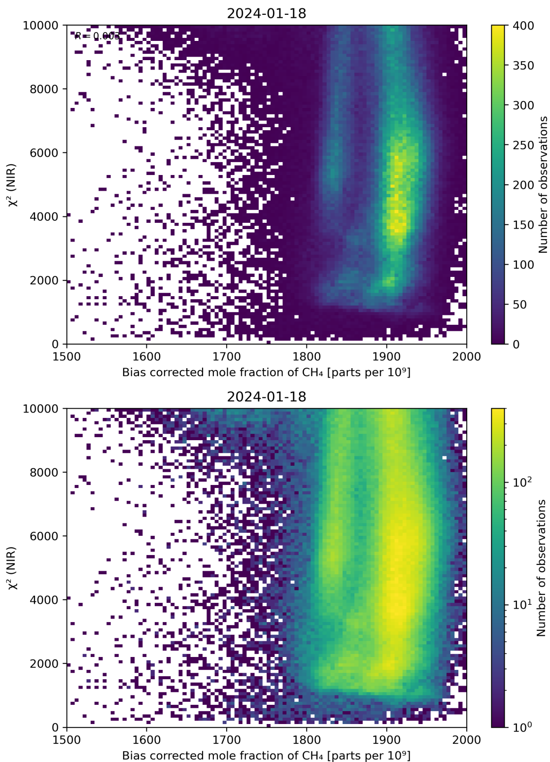
Figure 63: Scatter density plot of “Bias corrected mole fraction of \text{CH}_4 ” against “ \chi^2 (NIR)” for 2024-01-17 to 2024-01-19.
