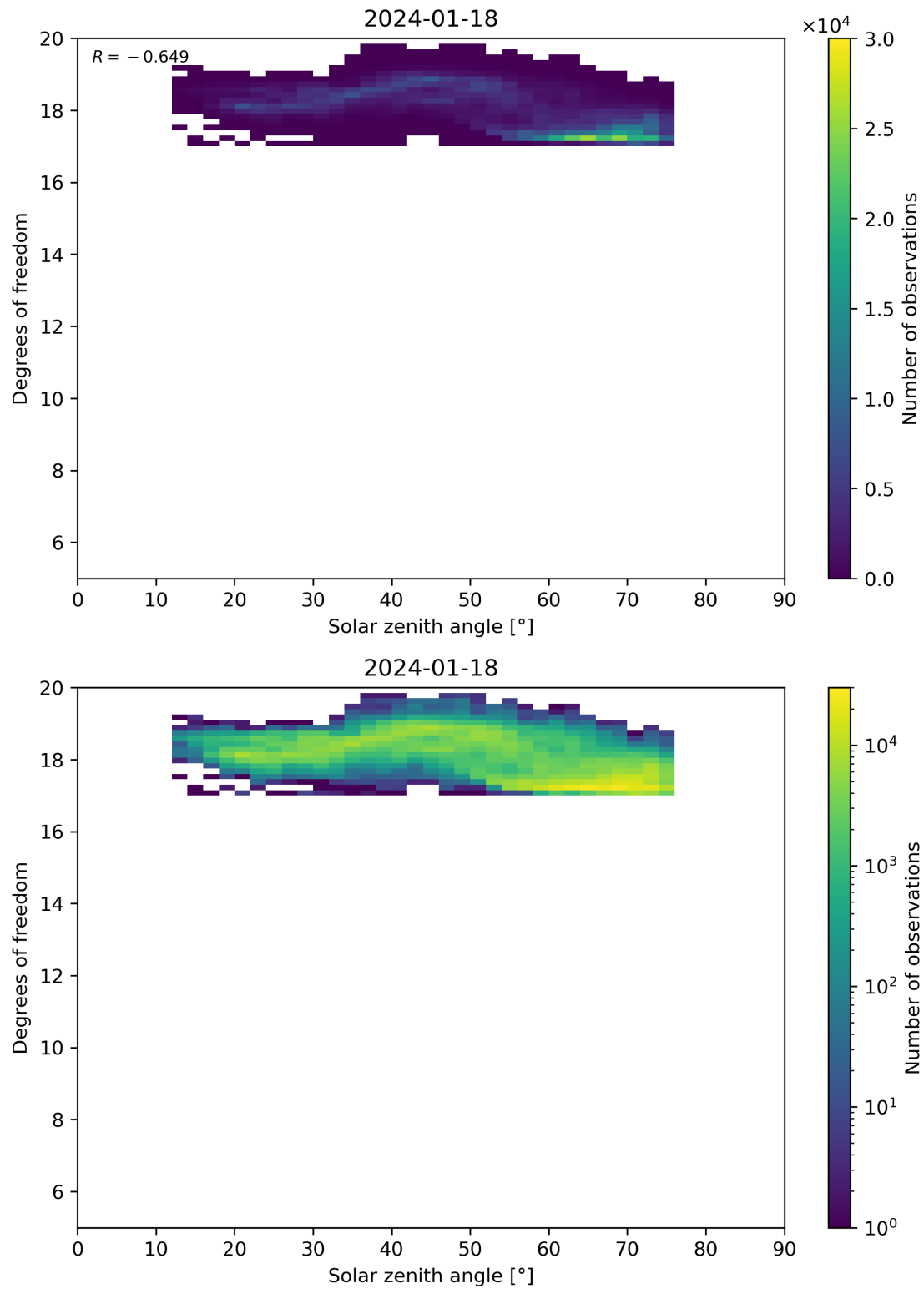
Figure 96: Scatter density plot of “Solar zenith angle” against “Degrees of freedom” for 2024-01-17 to 2024-01-19.
