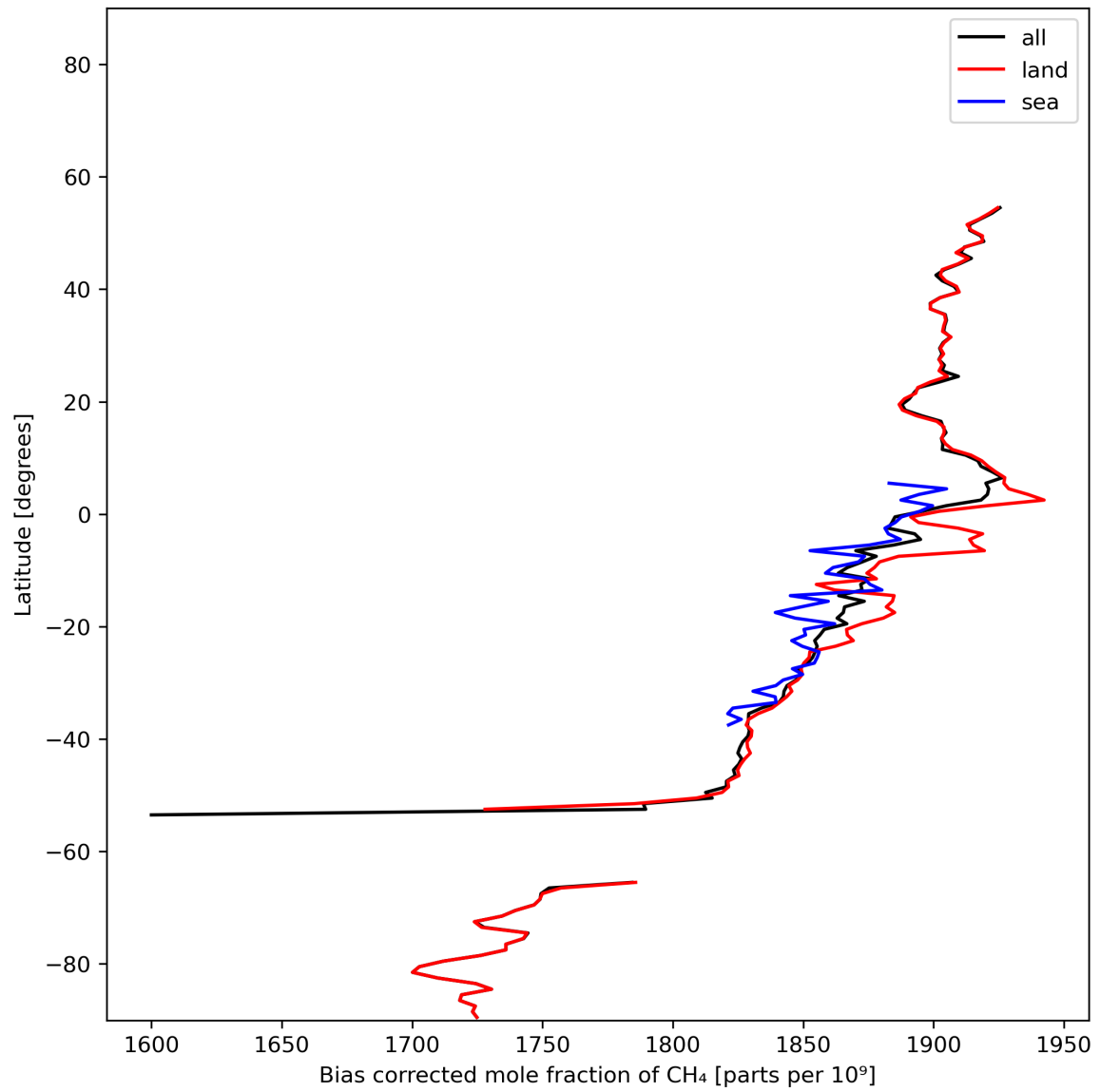
Figure 14: Zonal average of “Bias corrected mole fraction of CH 4 ” for 2024-01-17 to 2024-01-19.
