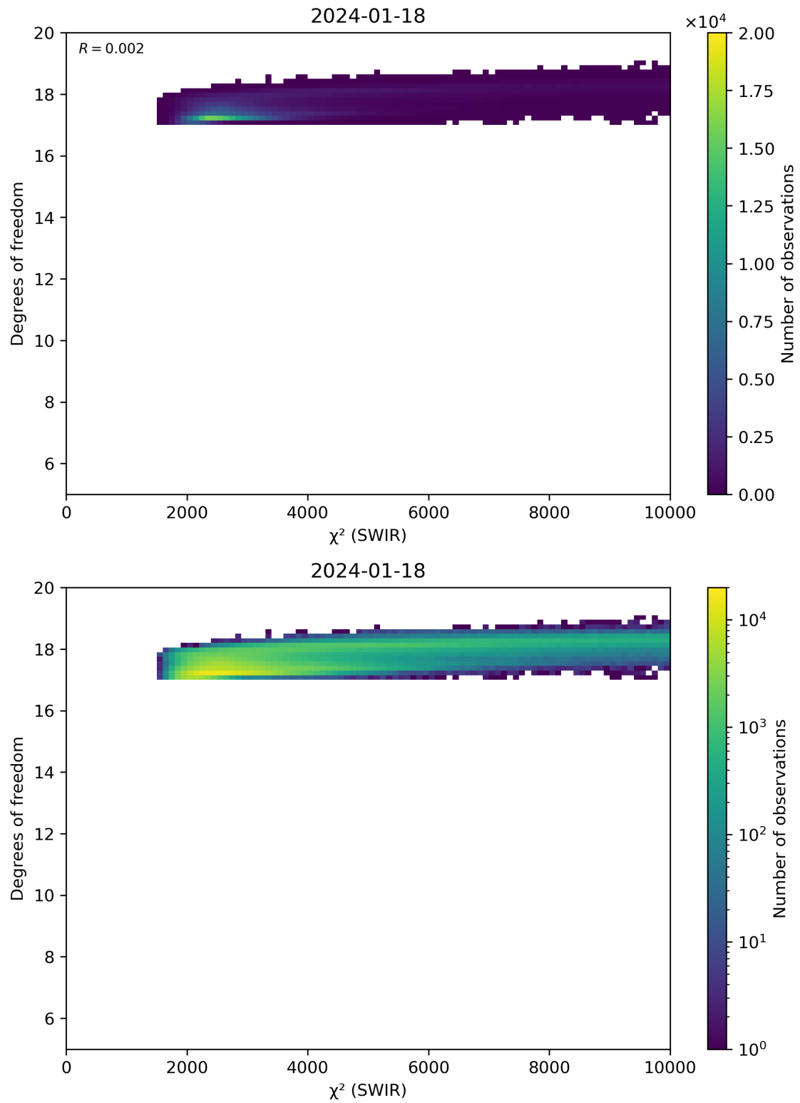
Figure 48: Scatter density plot of “ \chi^2 (SWIR)” against “Degrees of freedom” for 2024-01-17 to 2024-01-19.
