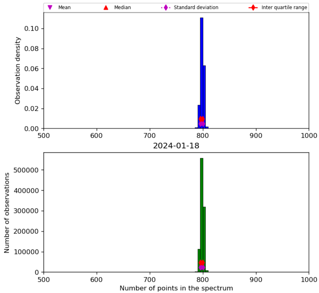
Figure 26: Histogram of “Number of points in the spectrum” for 2024-01-17 to 2024-01-19
