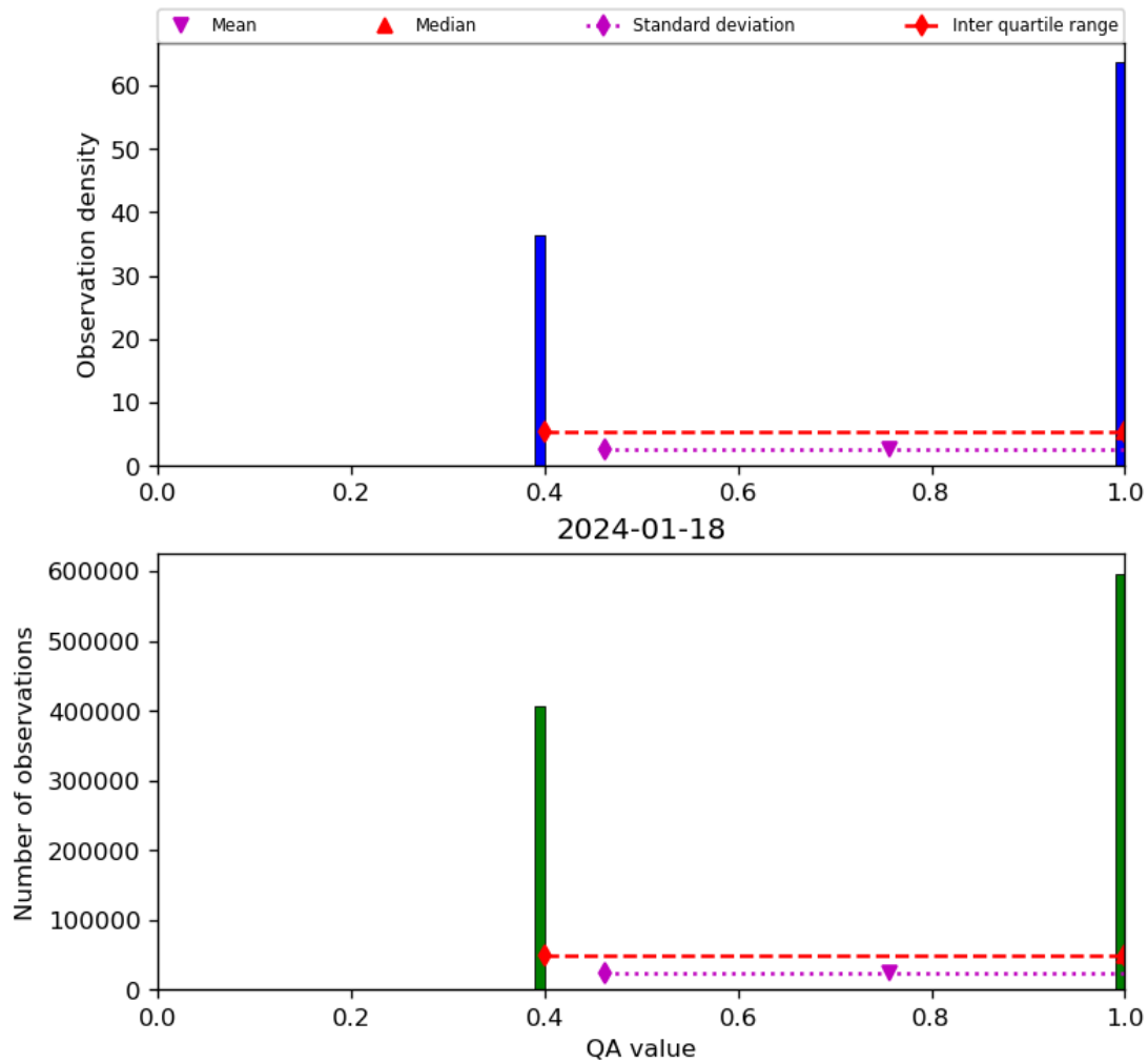
Figure 22: Histogram of “QA value” for 2024-01-17 to 2024-01-19
