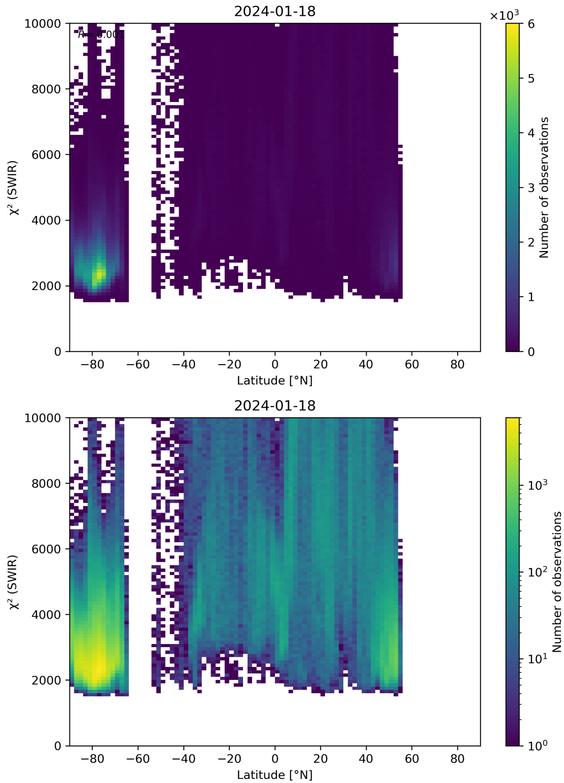
Figure 54: Scatter density plot of “Latitude” against “ \chi^2 (SWIR)” for 2024-01-17 to 2024-01-19.
