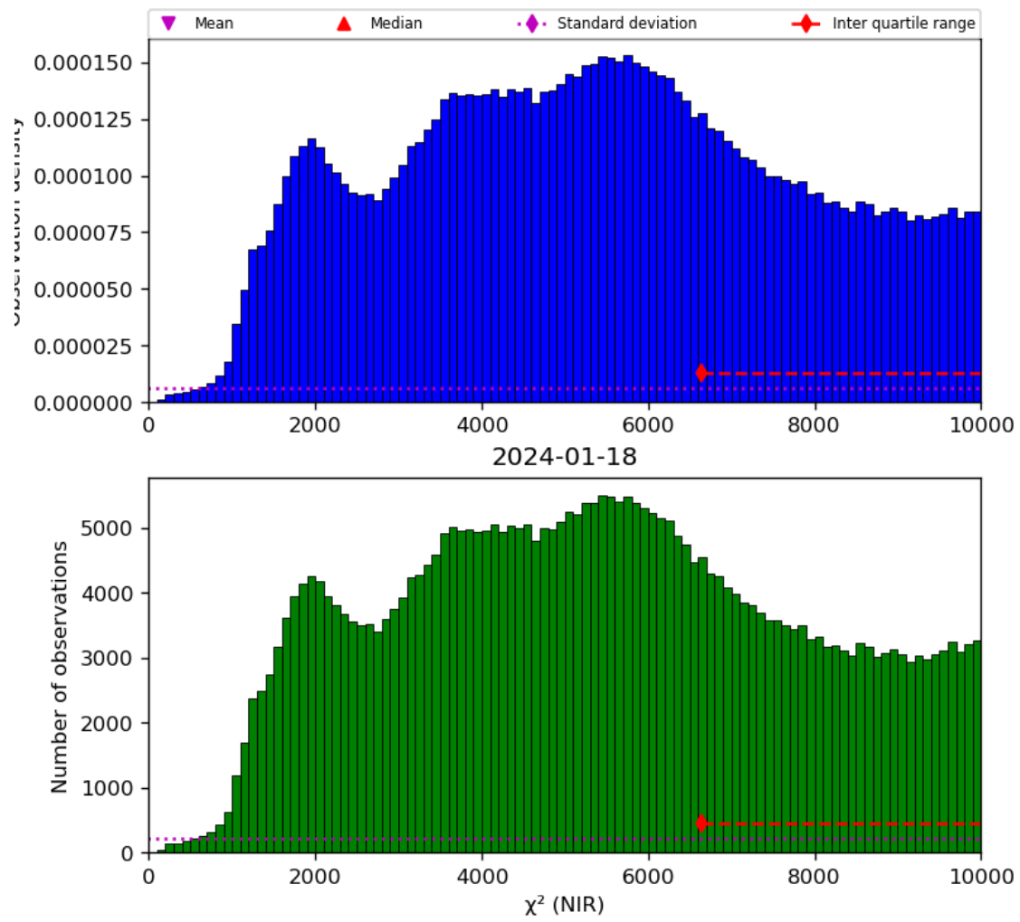
Figure 29: Histogram of “ \chi^2 (NIR)” for 2024-01-17 to 2024-01-19
