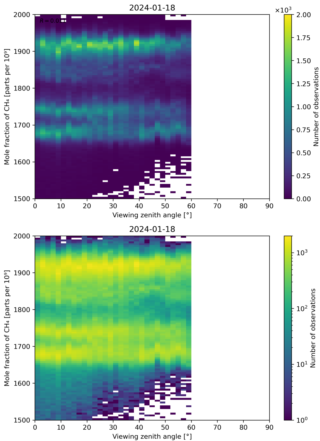
Figure 110: Scatter density plot of “Viewing zenith angle” against “Mole fraction of CH 4 ” for 2024-01-17 to 2024-01-19.
