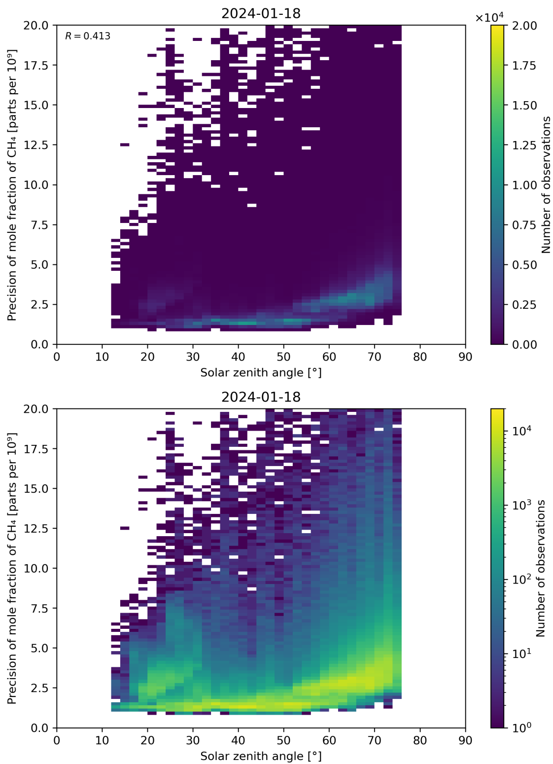
Figure 101: Scatter density plot of “Solar zenith angle” against “Precision of mole fraction of \text{CH}_4 ” for 2024-01-17 to 2024-01-19.
