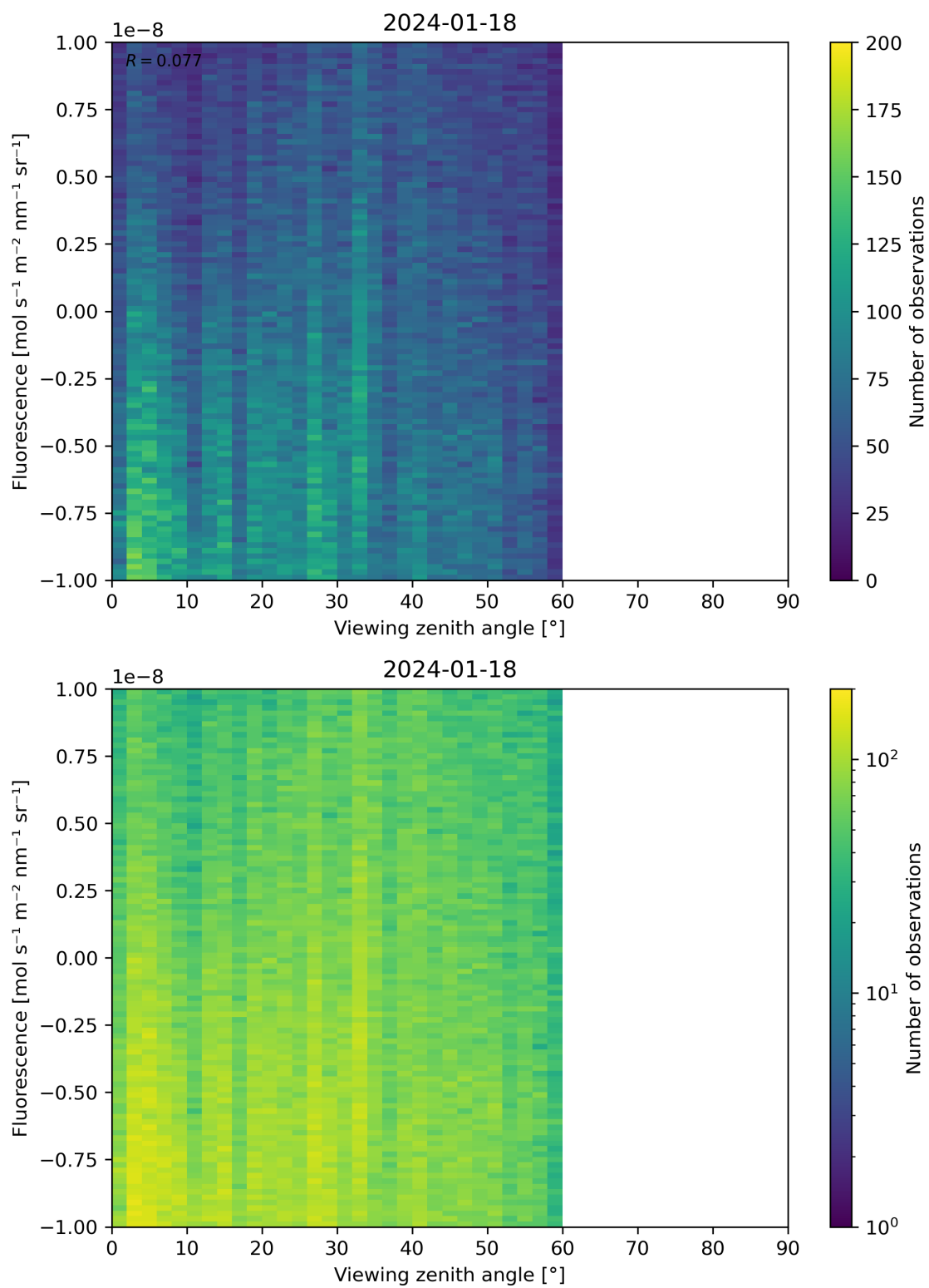
Figure 108: Scatter density plot of “Viewing zenith angle” against “Fluorescence” for 2024-01-17 to 2024-01-19.
