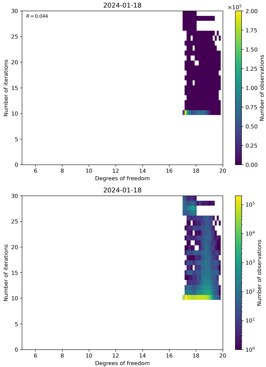
Figure 52: Scatter density plot of “Degrees of freedom” against “Number of iterations” for 2024-01-17 to 2024-01-19.
