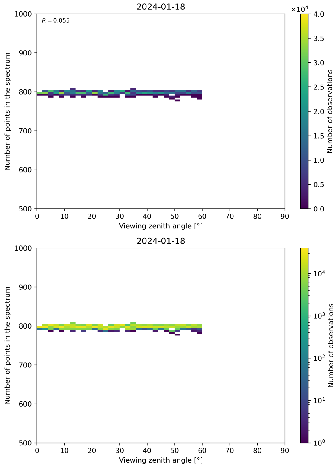
Figure 114: Scatter density plot of “Viewing zenith angle” against “Number of points in the spectrum” for 2024-01-17 to 2024-01-19.
