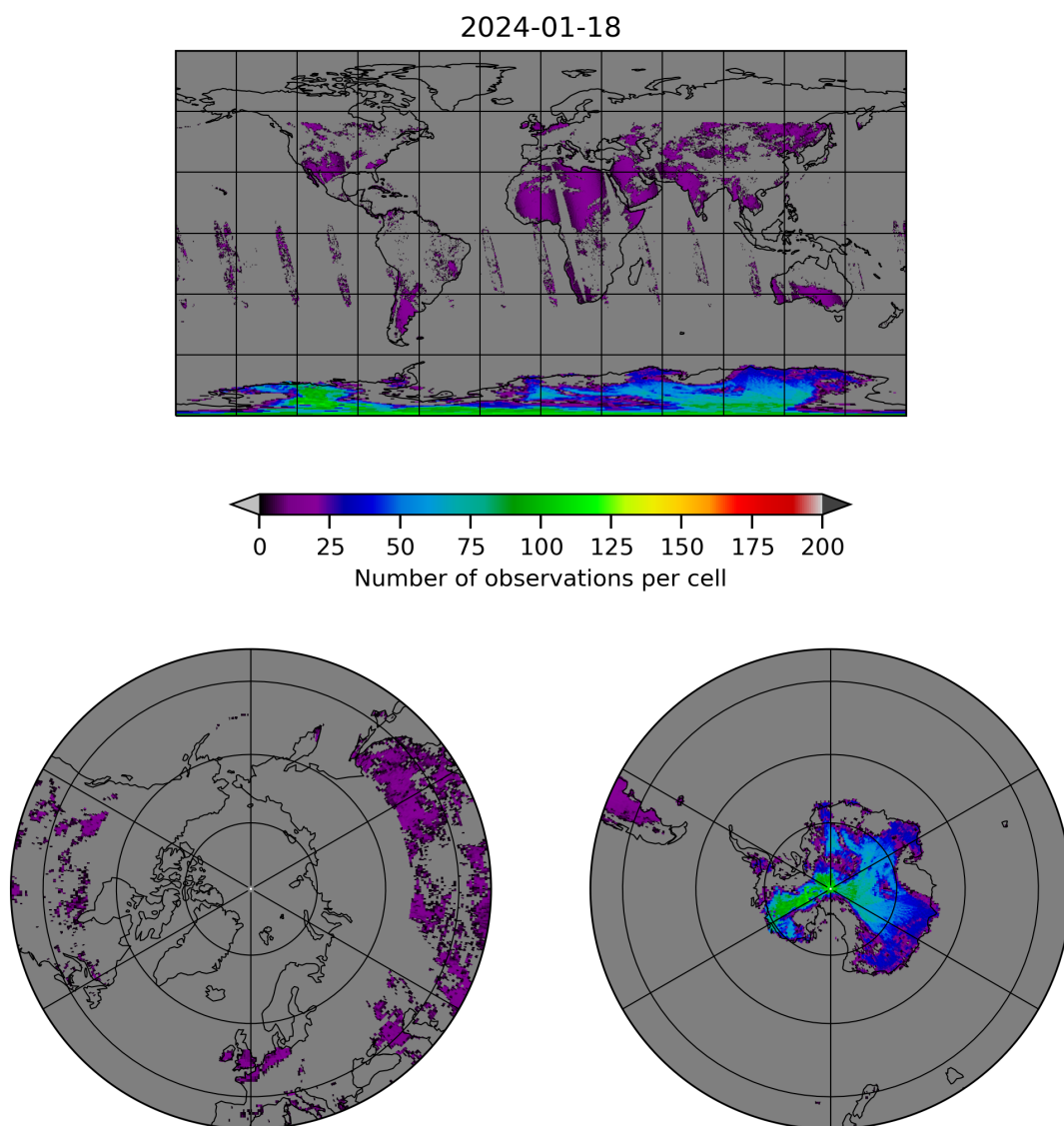
Figure 10: Map of the number of observations for 2024-01-17 to 2024-01-19
