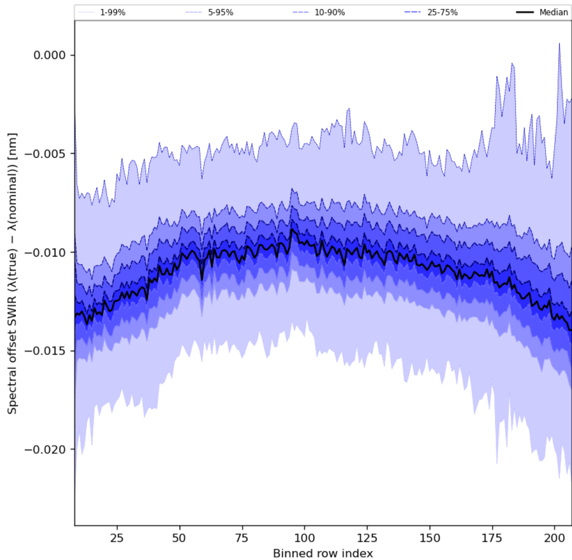
Figure 38: Along track statistics of “Spectral offset SWIR ( \lambda(\text{true}) - \lambda(\text{nominal}) )” for 2024-01-17 to 2024-01-19
