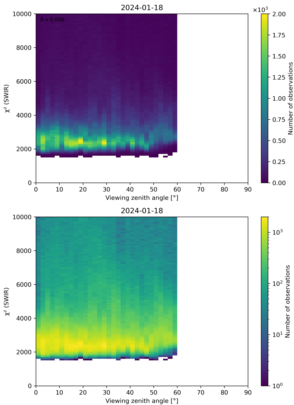
Figure 106: Scatter density plot of “Viewing zenith angle” against “ \chi^2 (SWIR)” for 2024-01-17 to 2024-01-19.
