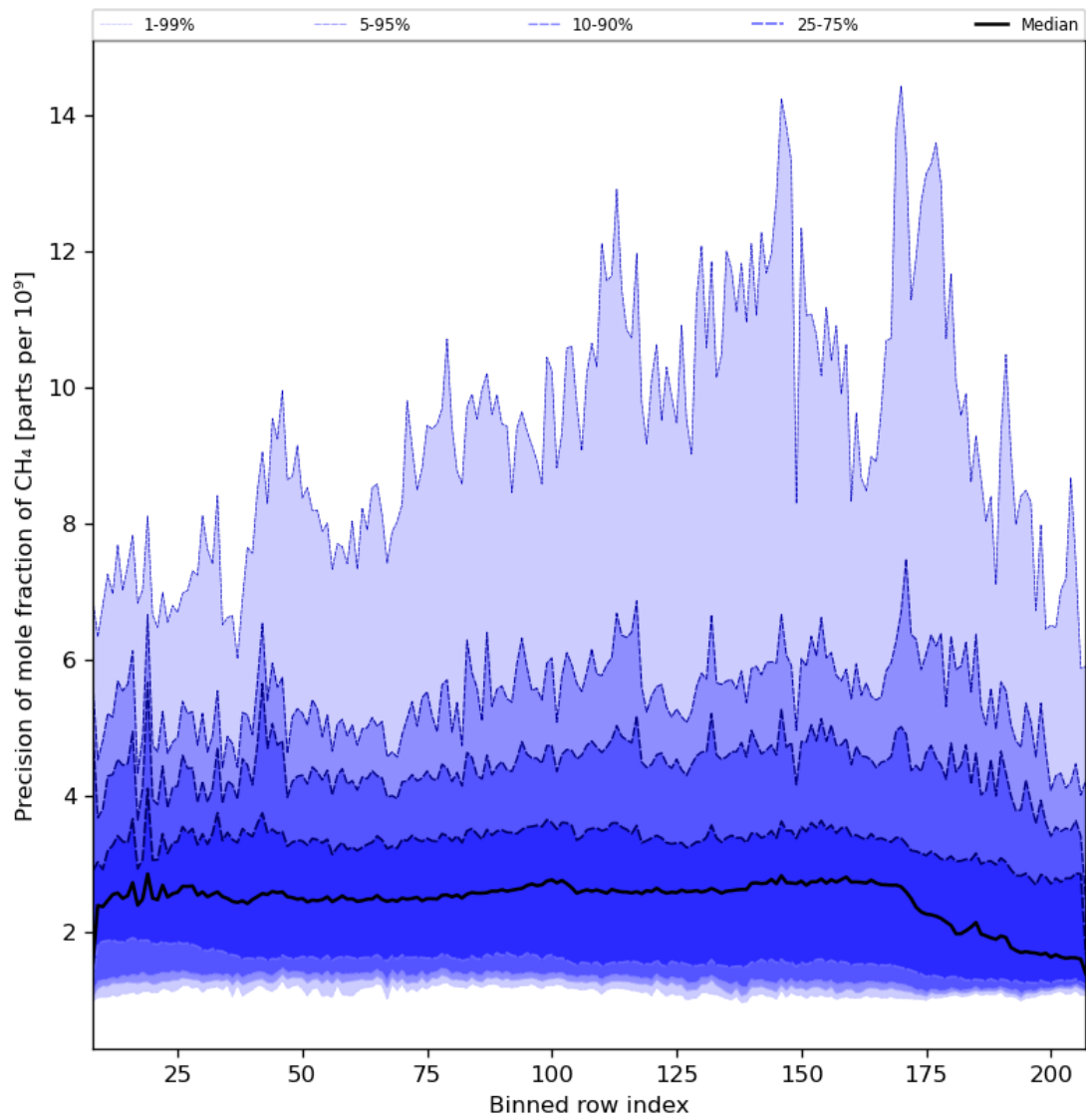
Figure 35: Along track statistics of “Precision of mole fraction of CH 4 ” for 2024-01-17 to 2024-01-19
