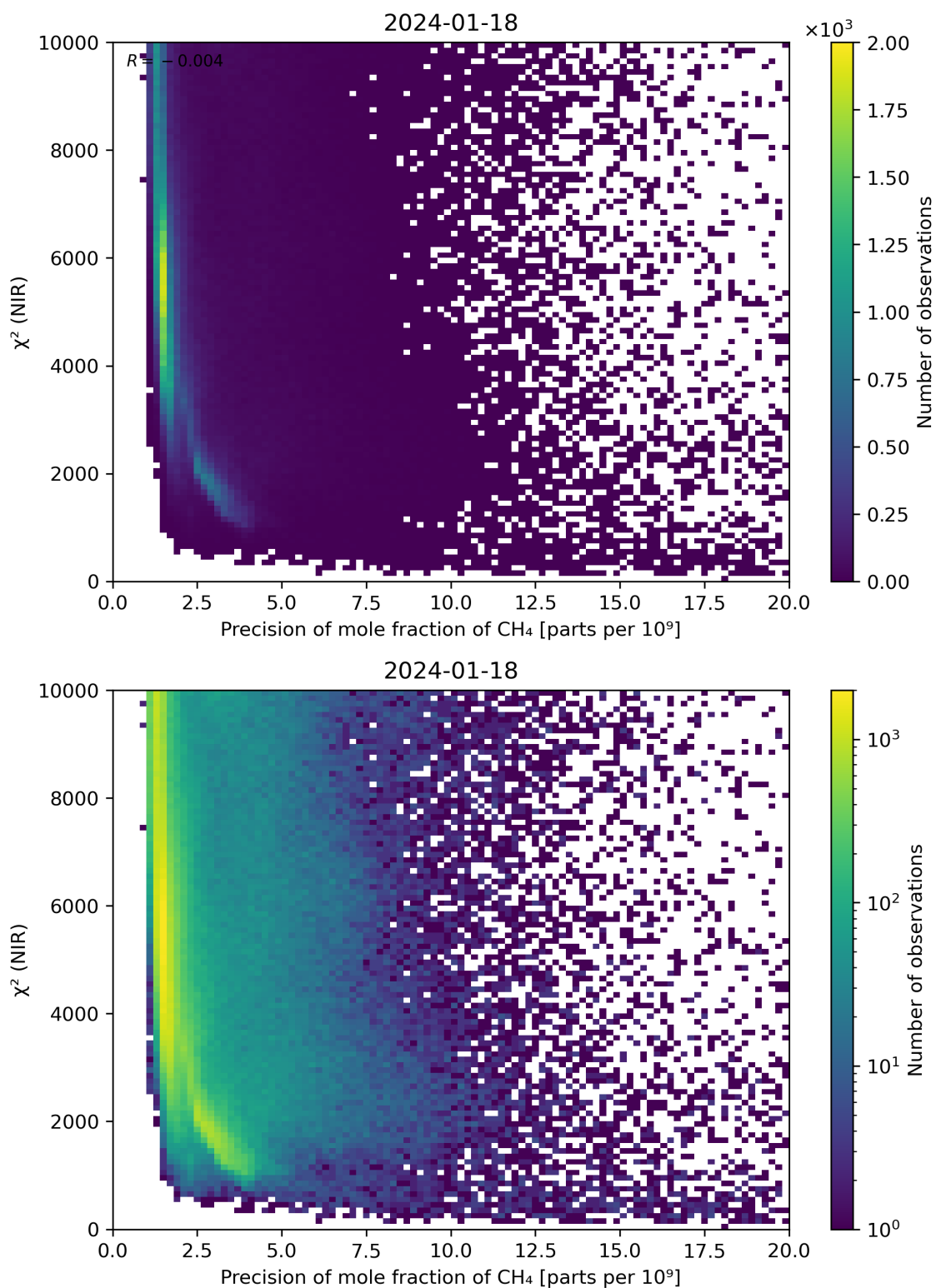
Figure 78: Scatter density plot of “Precision of mole fraction of \text{CH}_4 ” against “ \chi^2 (NIR)” for 2024-01-17 to 2024-01-19.
