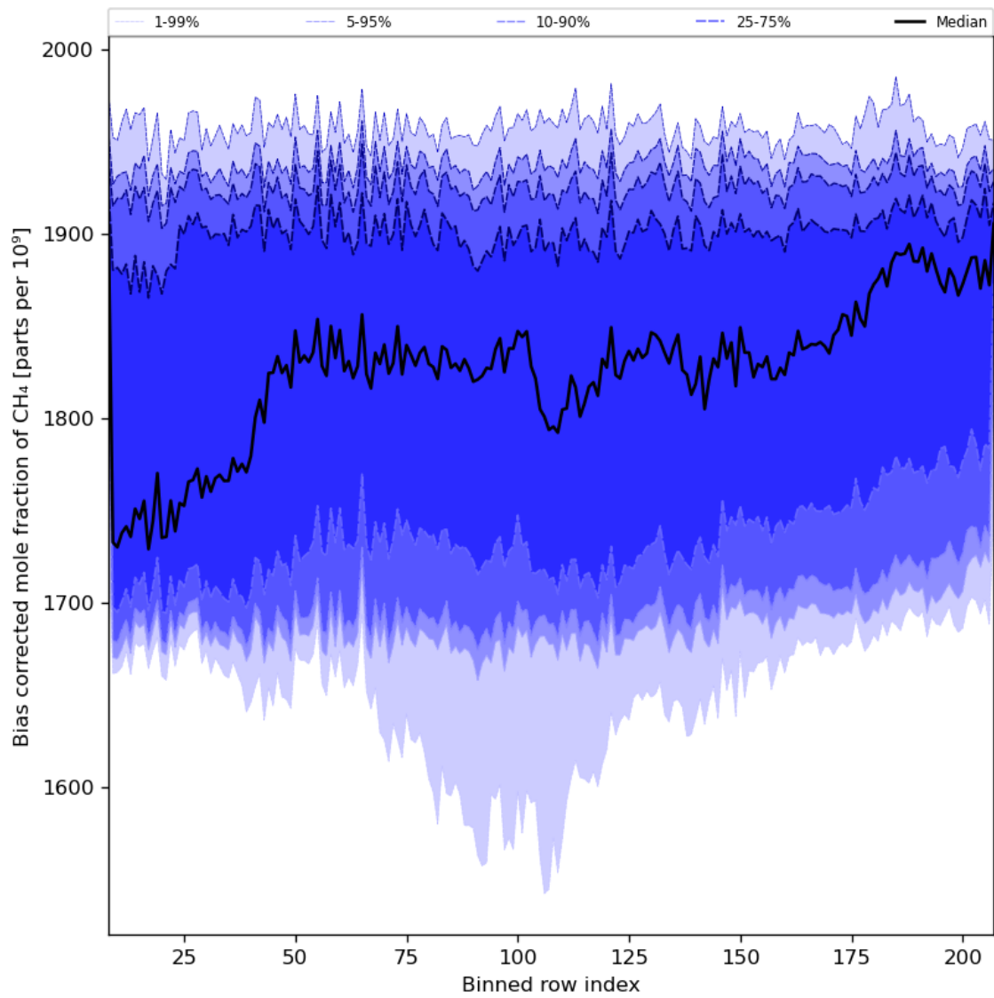
Figure 36: Along track statistics of “Bias corrected mole fraction of CH 4 ” for 2024-01-17 to 2024-01-19
