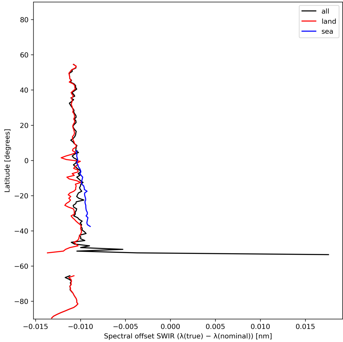
Figure 16: Zonal average of “Spectral offset SWIR ( \lambda(\text{true}) - \lambda(\text{nominal}) )” for 2024-01-17 to 2024-01-19.
