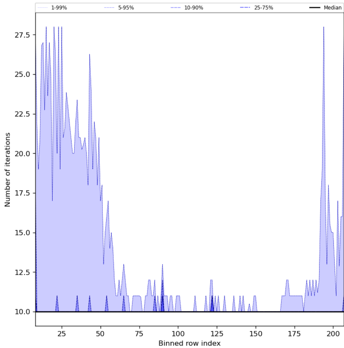
Figure 42: Along track statistics of “Number of iterations” for 2024-01-17 to 2024-01-19
