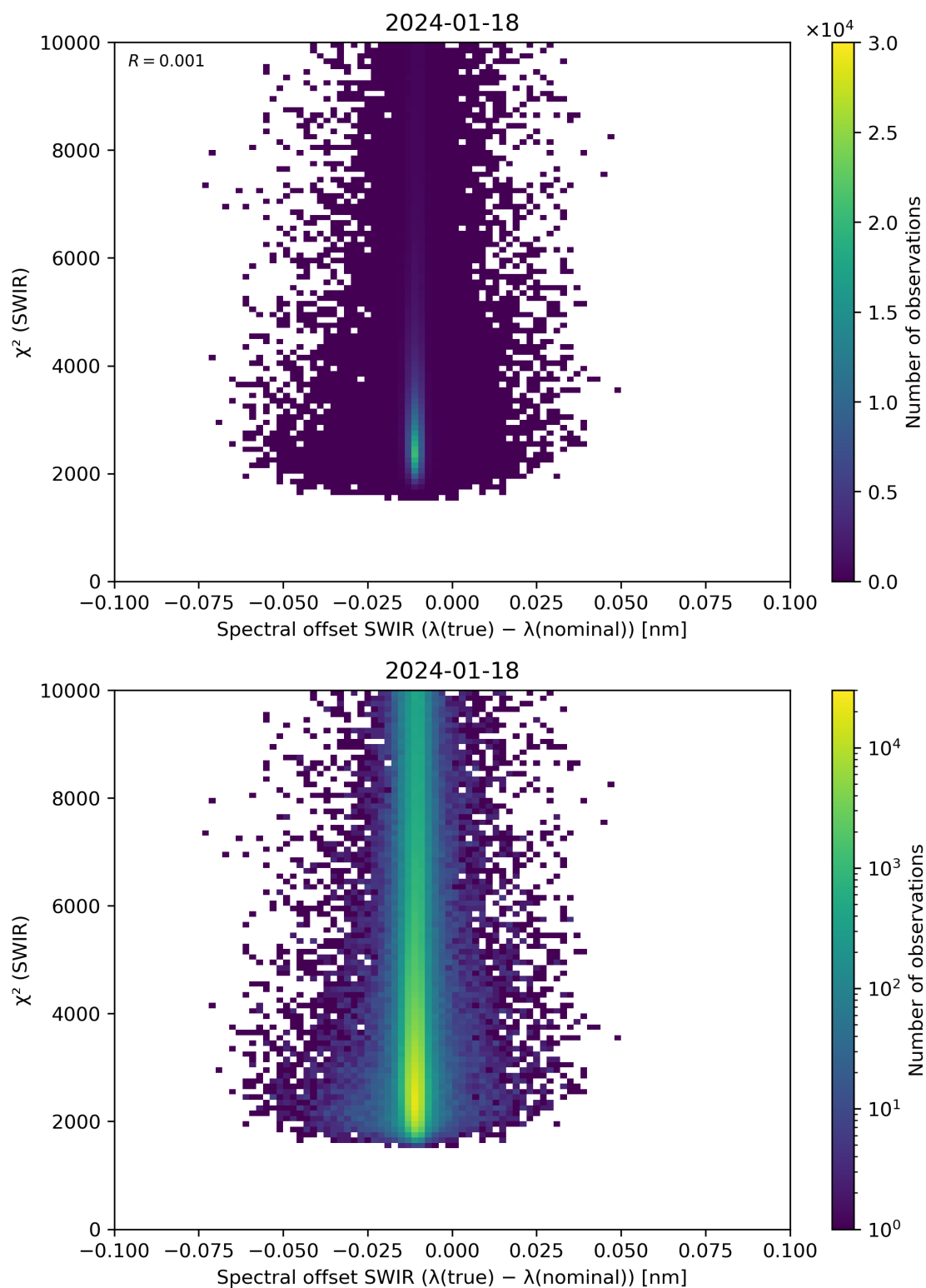
Figure 118: Scatter density plot of “Spectral offset SWIR ( \lambda(\text{true}) - \lambda(\text{nominal}) )” against “ \chi^2 (SWIR)” for 2024-01-17 to 2024-01-19.
