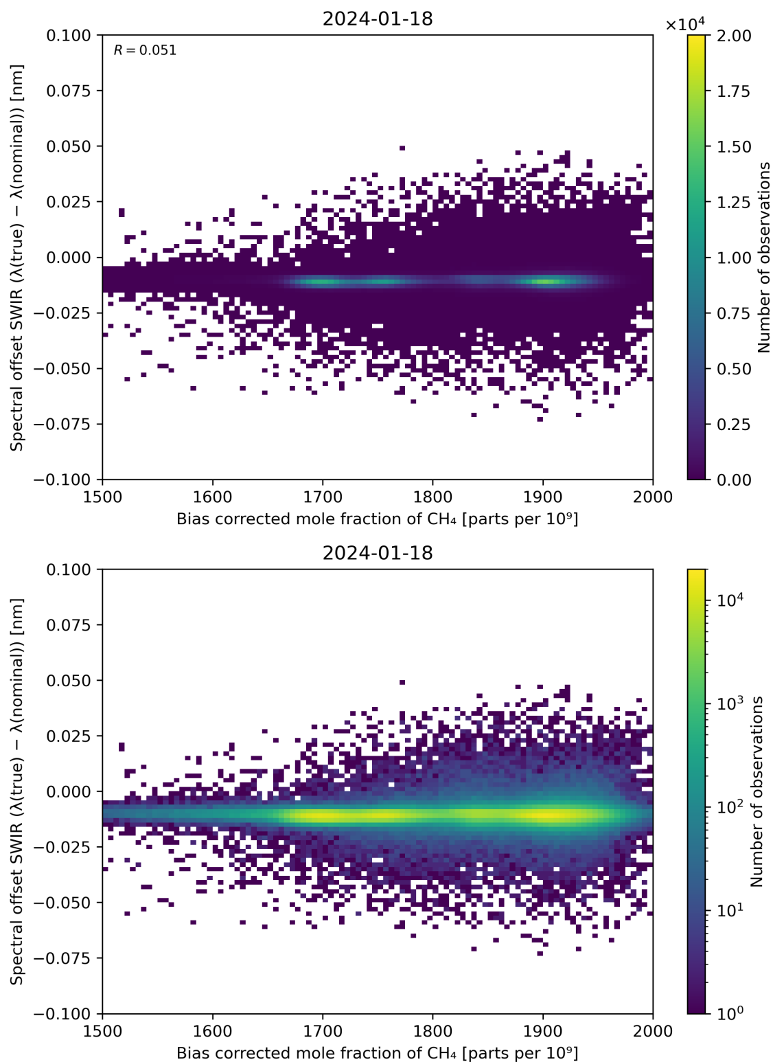
Figure 69: Scatter density plot of “Bias corrected mole fraction of \text{CH}_4 ” against “Spectral offset SWIR ( \lambda(\text{true}) - \lambda(\text{nominal}) )” for 2024-01-17 to 2024-01-19.
