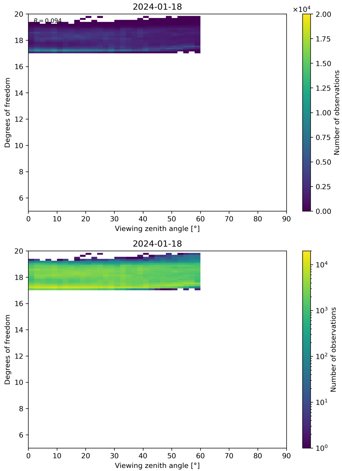
Figure 107: Scatter density plot of “Viewing zenith angle” against “Degrees of freedom” for 2024-01-17 to 2024-01-19.
