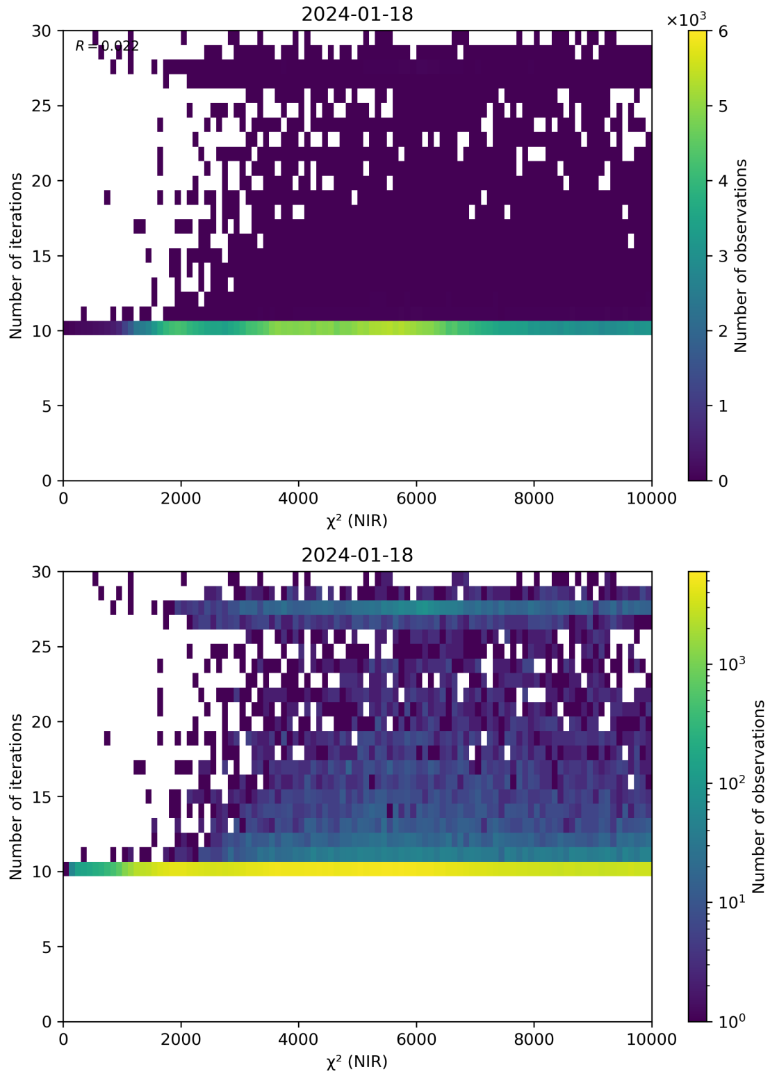
Figure 46: Scatter density plot of “ \chi^2 (NIR)” against “Number of iterations” for 2024-01-17 to 2024-01-19.
