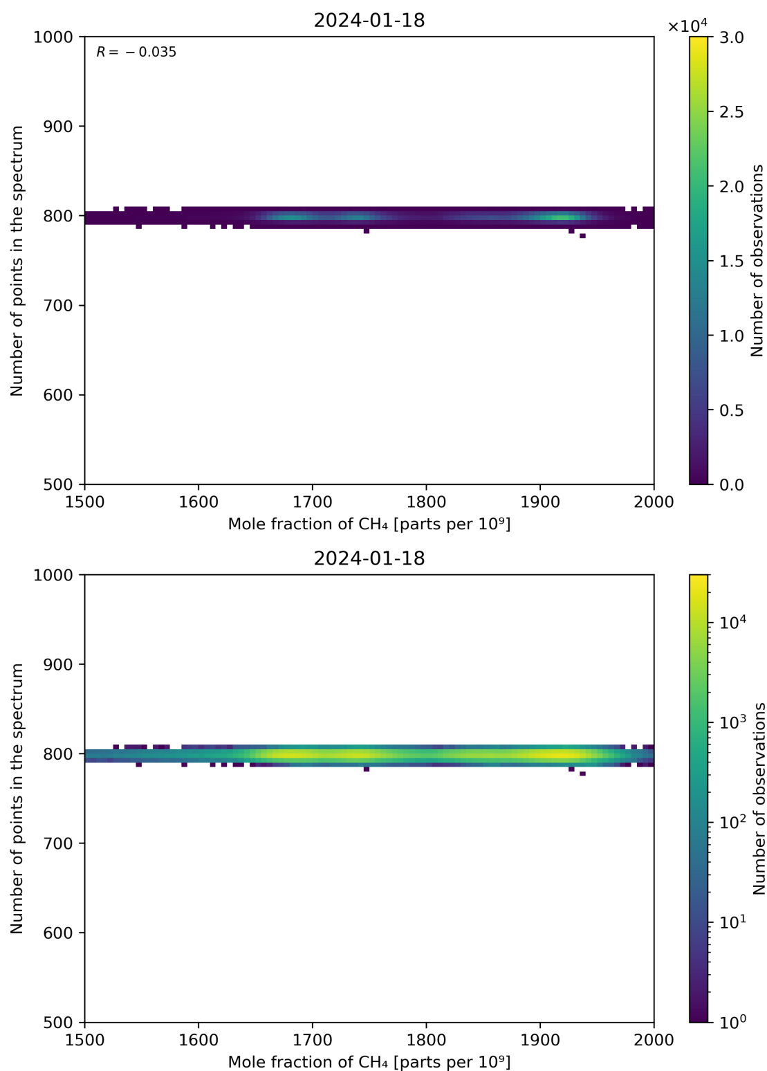
Figure 77: Scatter density plot of “Mole fraction of CH 4 ” against “Number of points in the spectrum” for 2024-01-17 to 2024-01-19.
