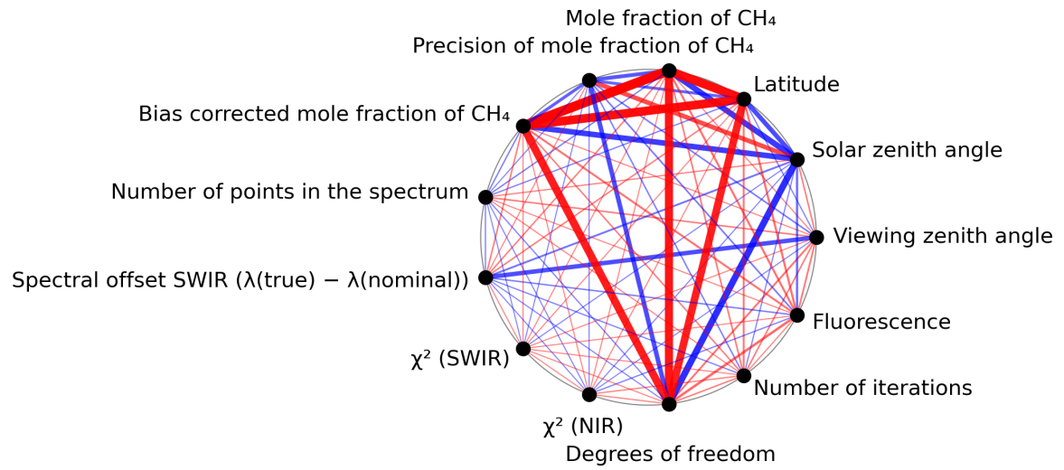
Figure 1: Map of correlation graph for 2024-01-17 to 2024-01-19.
