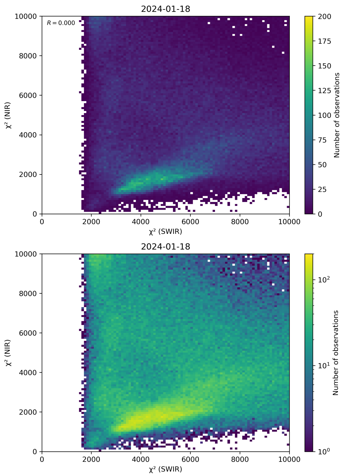
Figure 47: Scatter density plot of “ \chi^2 (SWIR)” against “ \chi^2 (NIR)” for 2024-01-17 to 2024-01-19.
