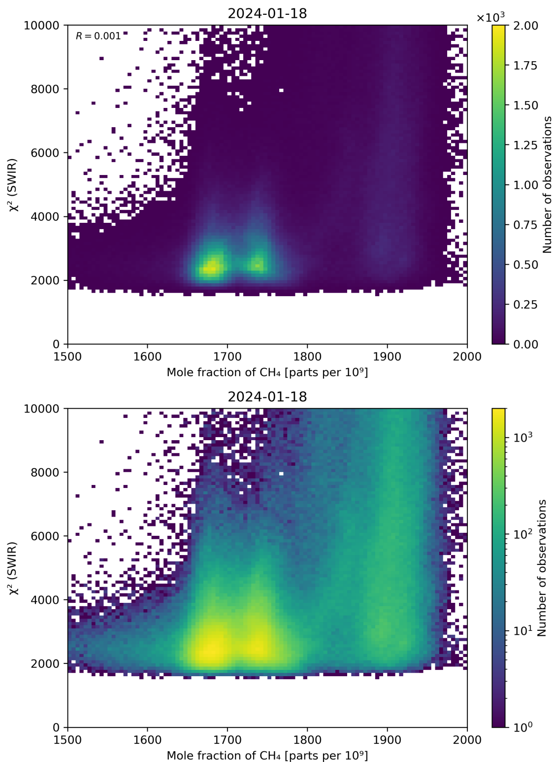
Figure 71: Scatter density plot of “Mole fraction of \text{CH}_4 ” against “ \chi^2 (SWIR)” for 2024-01-17 to 2024-01-19.
