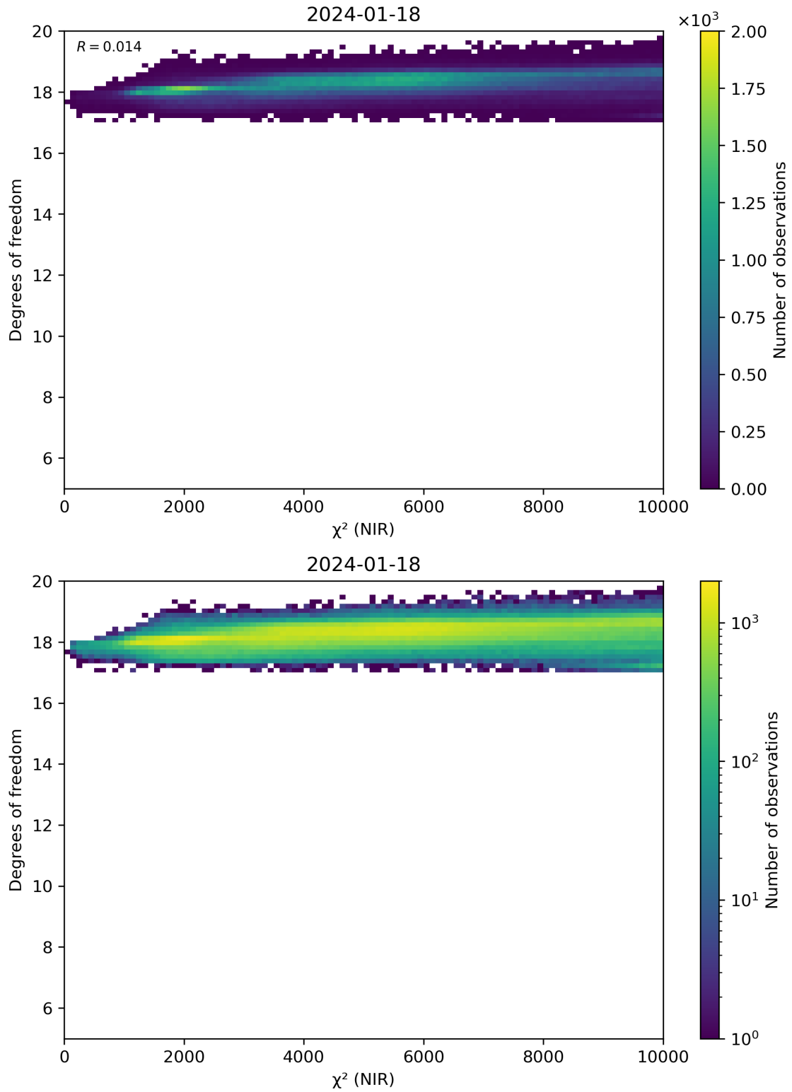
Figure 44: Scatter density plot of “ \chi^2 (NIR)” against “Degrees of freedom” for 2024-01-17 to 2024-01-19.
