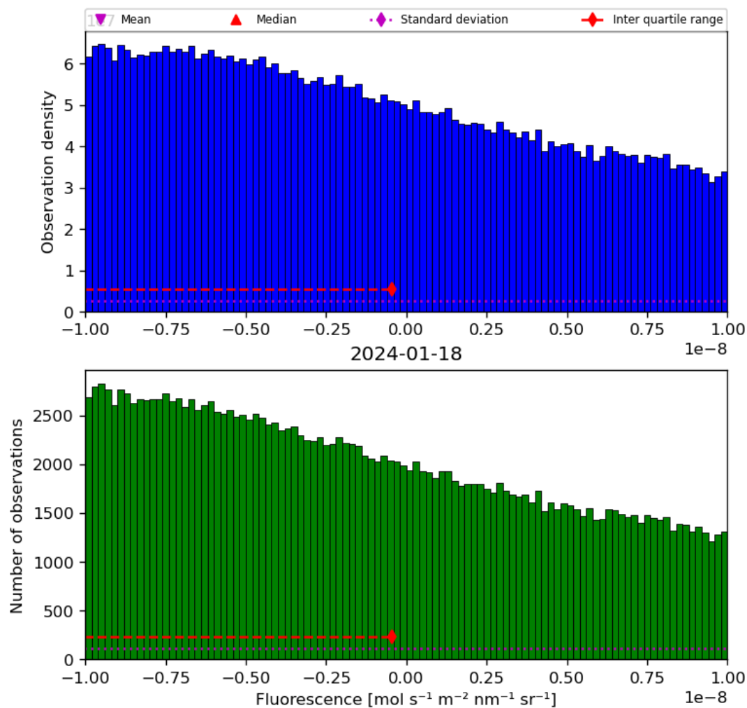
Figure 32: Histogram of “Fluorescence” for 2024-01-17 to 2024-01-19
