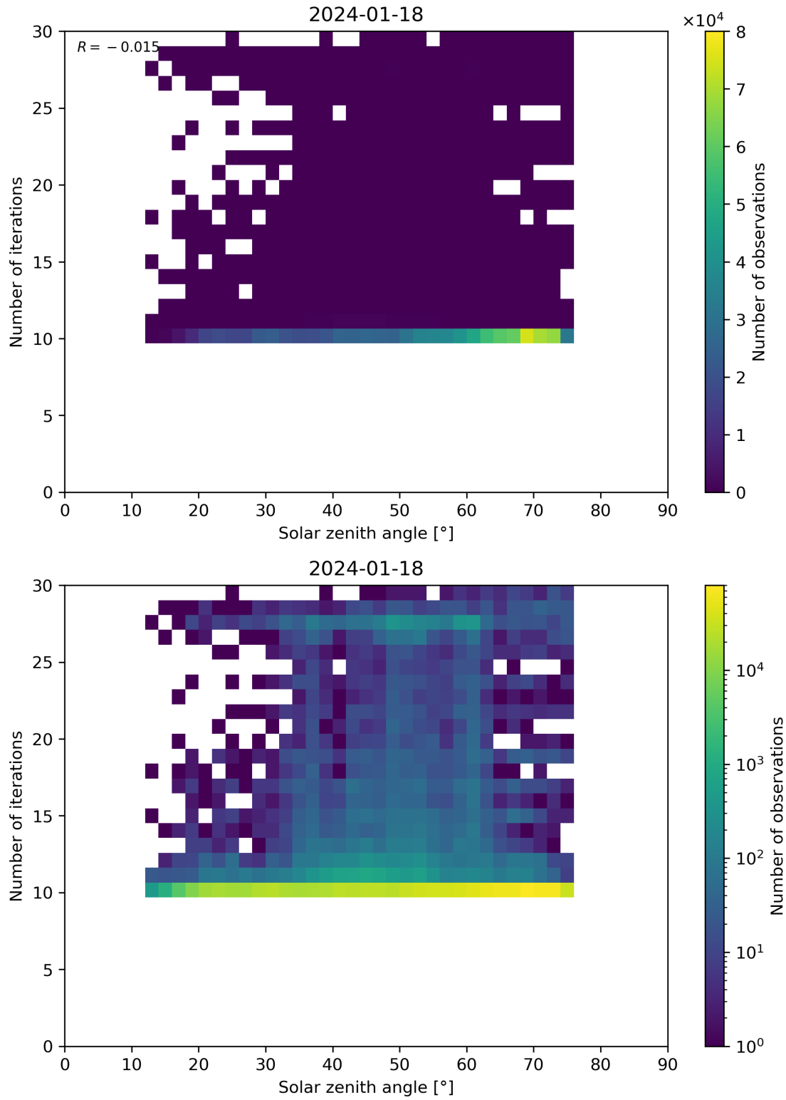
Figure 102: Scatter density plot of “Solar zenith angle” against “Number of iterations” for 2024-01-17 to 2024-01-19.
