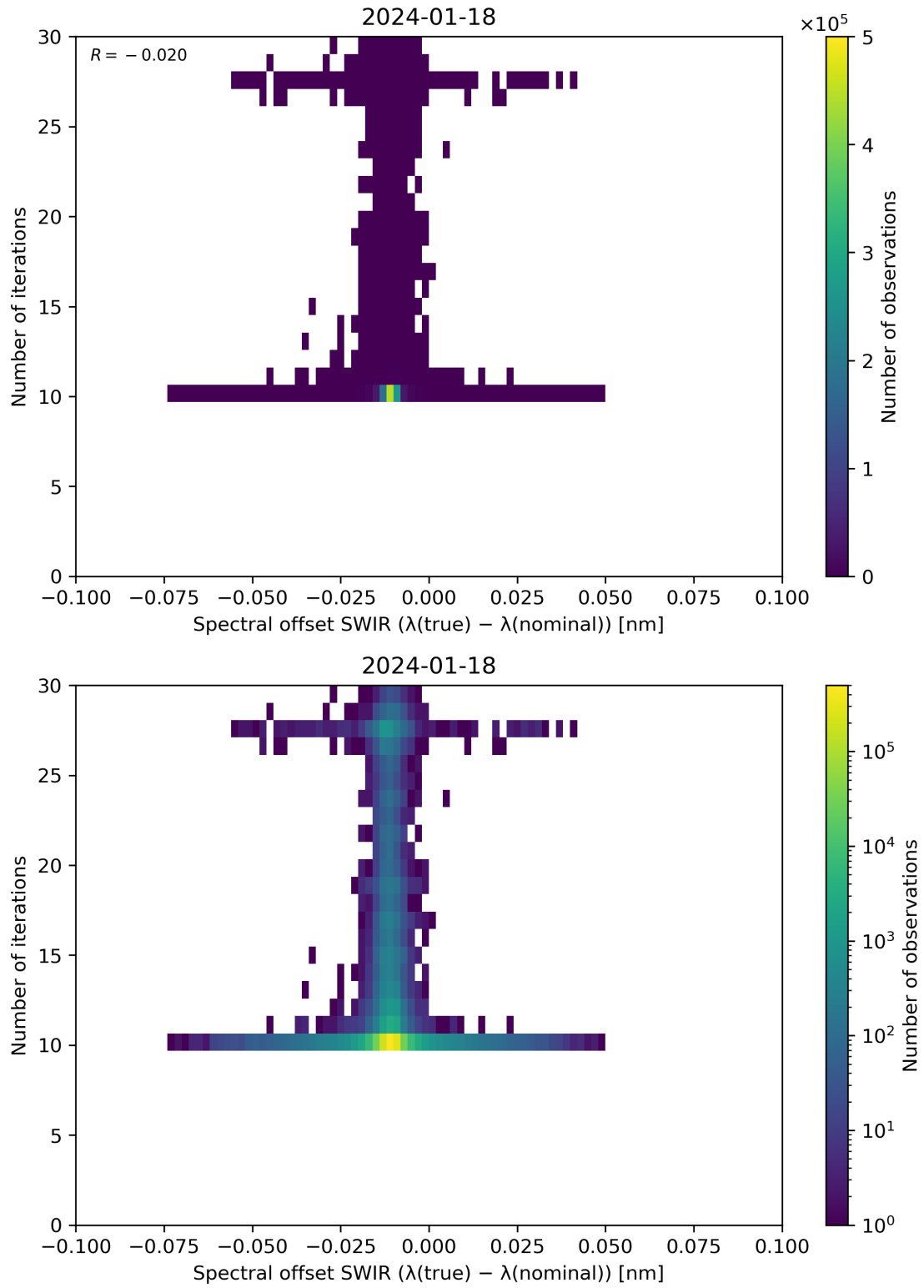
Figure 121: Scatter density plot of “Spectral offset SWIR ( \lambda(\text{true}) - \lambda(\text{nominal}) )” against “Number of iterations” for 2024-01-17 to 2024-01-19.
