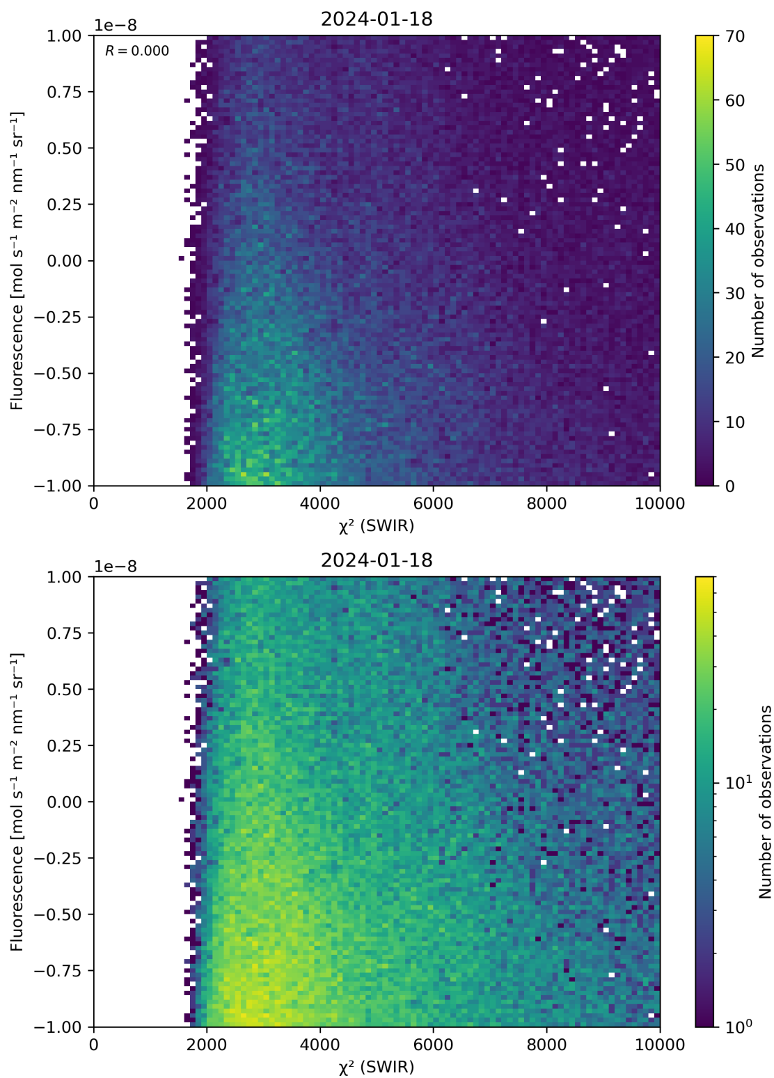
Figure 49: Scatter density plot of “ \chi^2 (SWIR)” against “Fluorescence” for 2024-01-17 to 2024-01-19.
