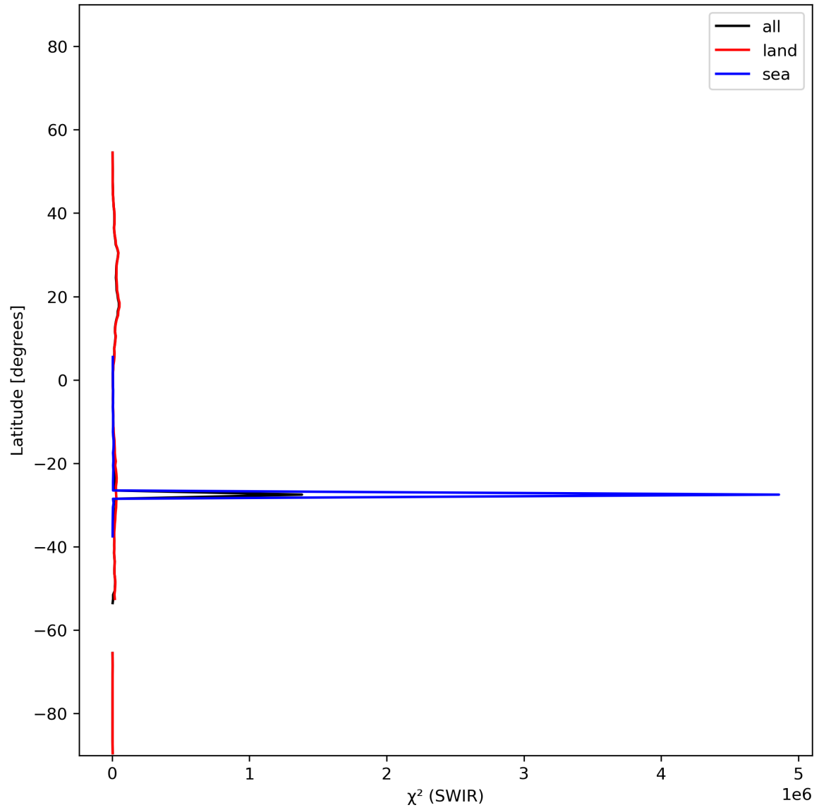
Figure 17: Zonal average of “ \chi^2 (SWIR)” for 2024-01-17 to 2024-01-19.
