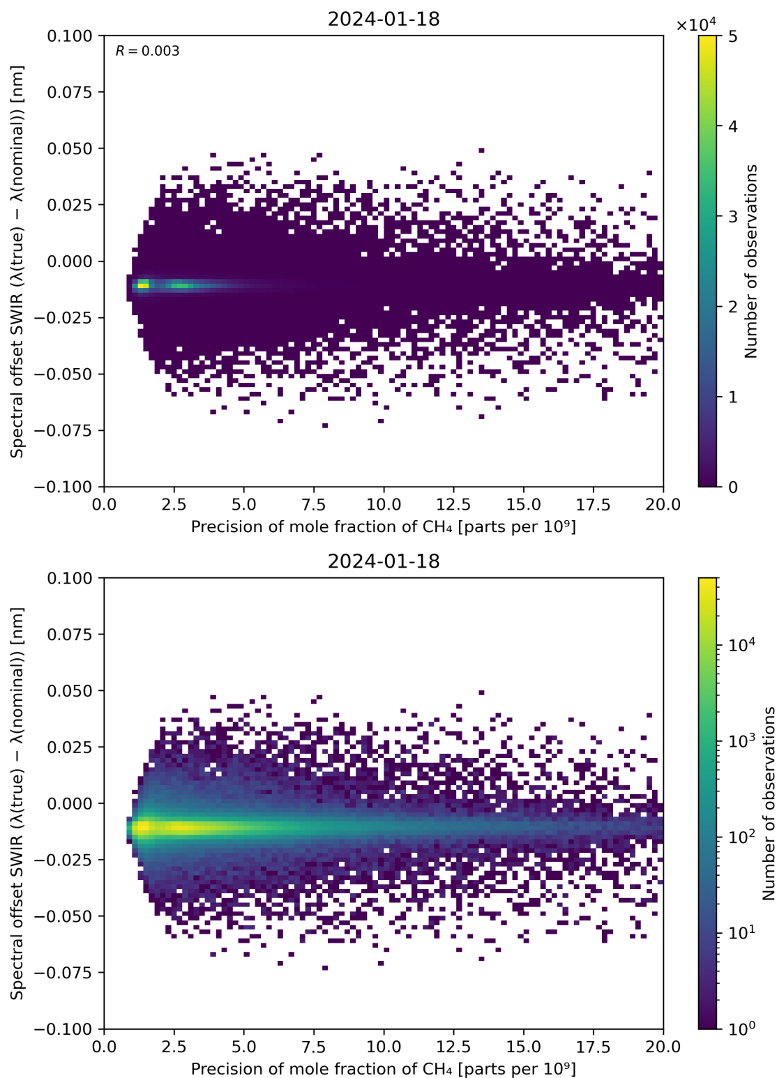
Figure 85: Scatter density plot of “Precision of mole fraction of CH 4 ” against “Spectral offset SWIR ( \lambda(\text{true}) - \lambda(\text{nominal}) )” for 2024-01-17 to 2024-01-19.
