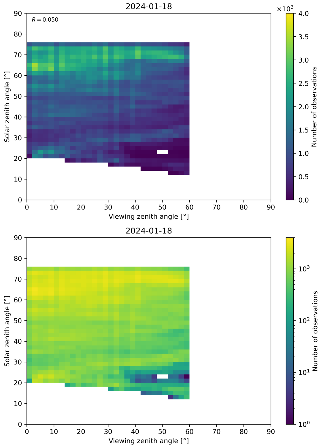
Figure 115: Scatter density plot of “Viewing zenith angle” against “Solar zenith angle” for 2024-01-17 to 2024-01-19.
