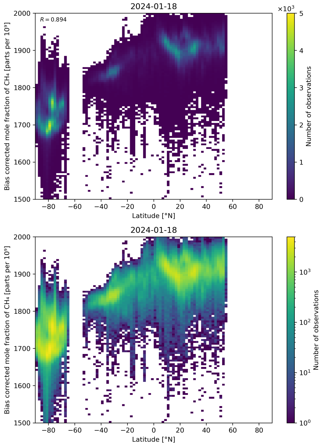
Figure 58: Scatter density plot of “Latitude” against “Bias corrected mole fraction of CH 4 ” for 2024-01-17 to 2024-01-19.
