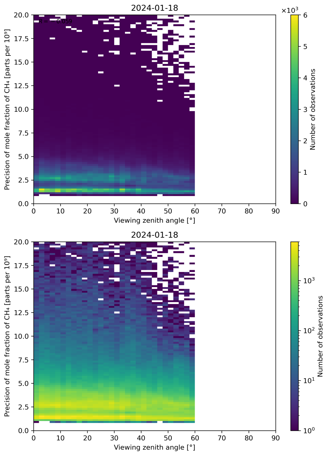
Figure 112: Scatter density plot of “Viewing zenith angle” against “Precision of mole fraction of CH 4 ” for 2024-01-17 to 2024-01-19.
