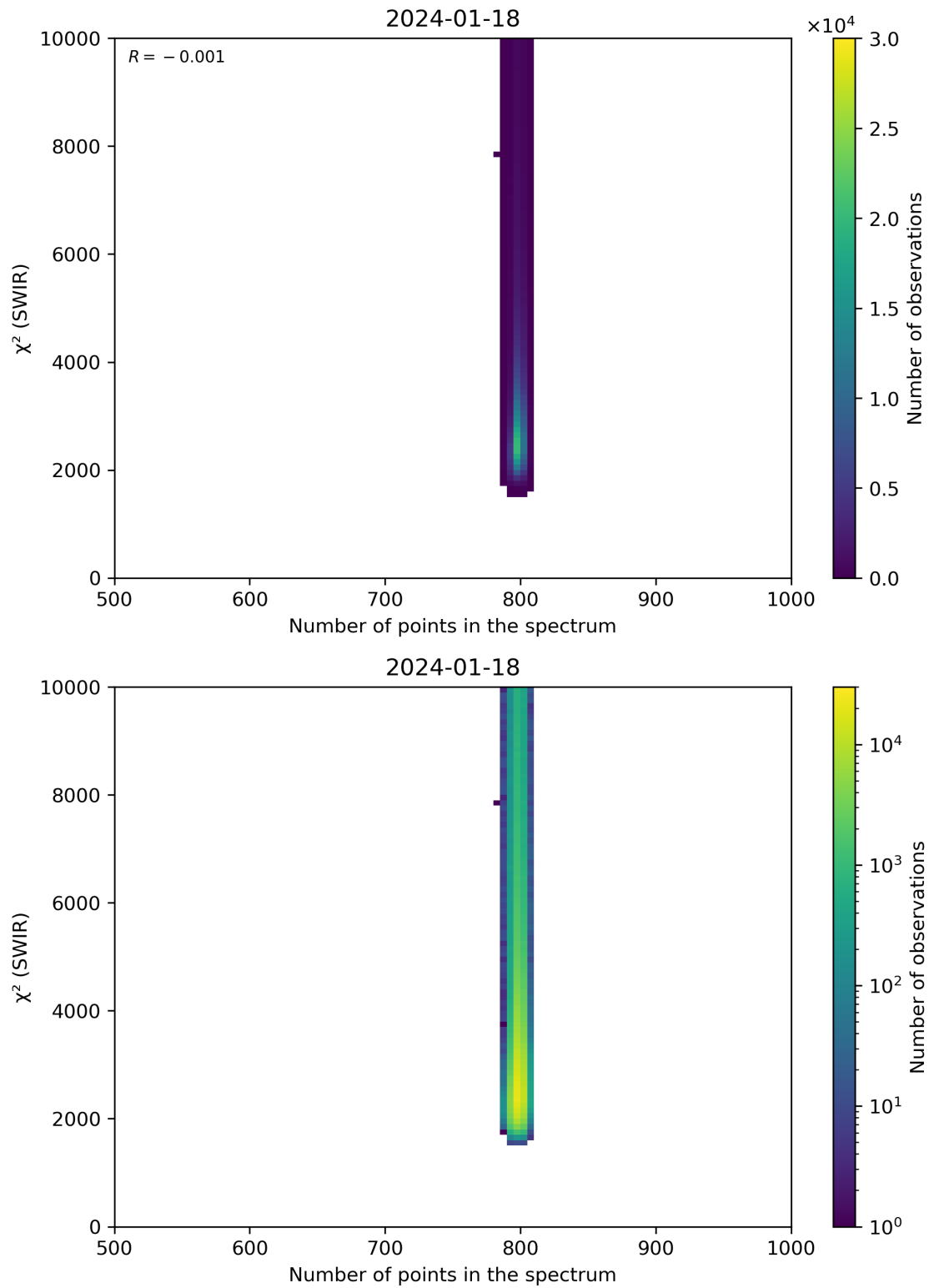
Figure 89: Scatter density plot of “Number of points in the spectrum” against “ \chi^2 (SWIR)” for 2024-01-17 to 2024-01-19.
