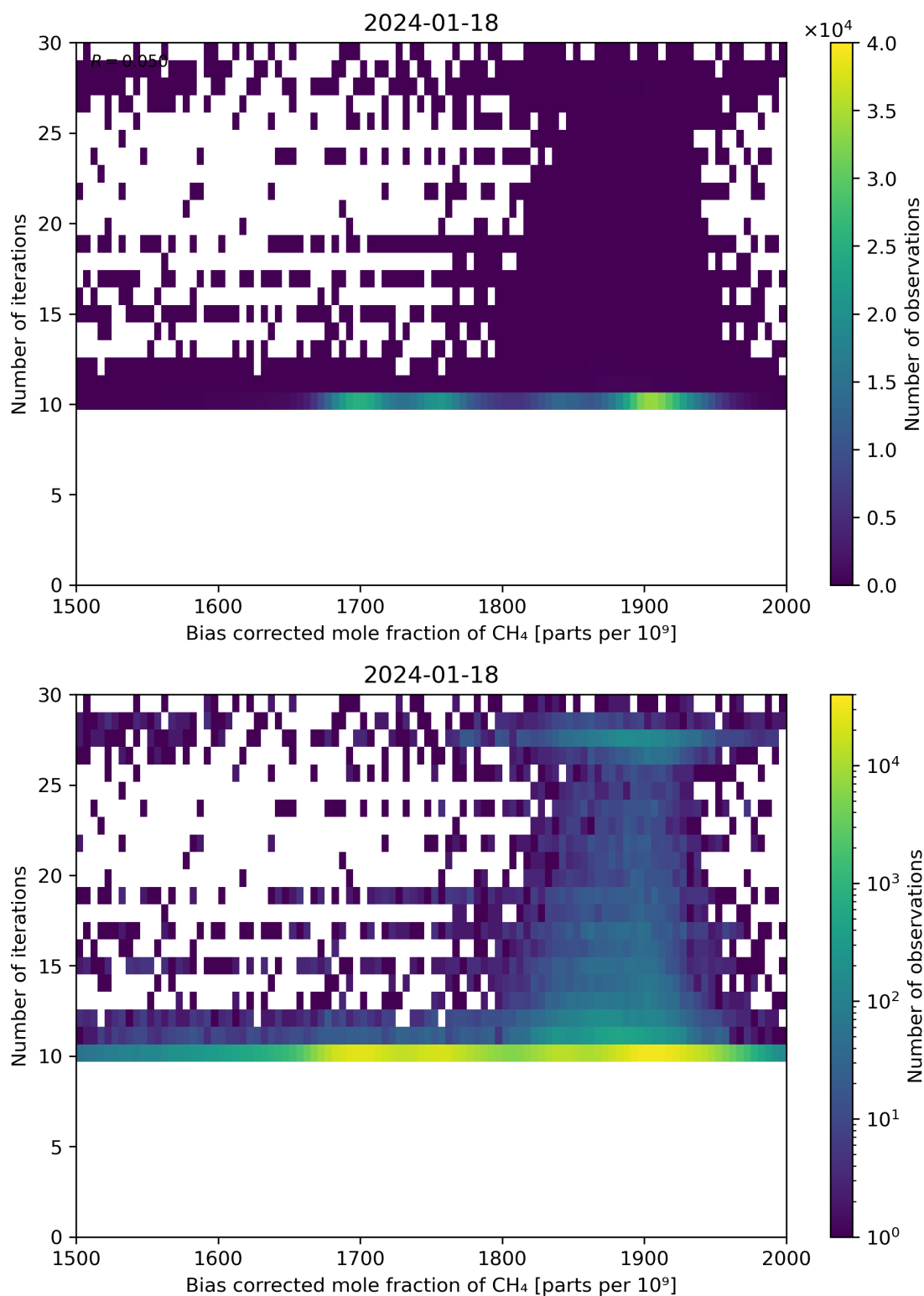
Figure 67: Scatter density plot of “Bias corrected mole fraction of \text{CH}_4 ” against “Number of iterations” for 2024-01-17 to 2024-01-19.
