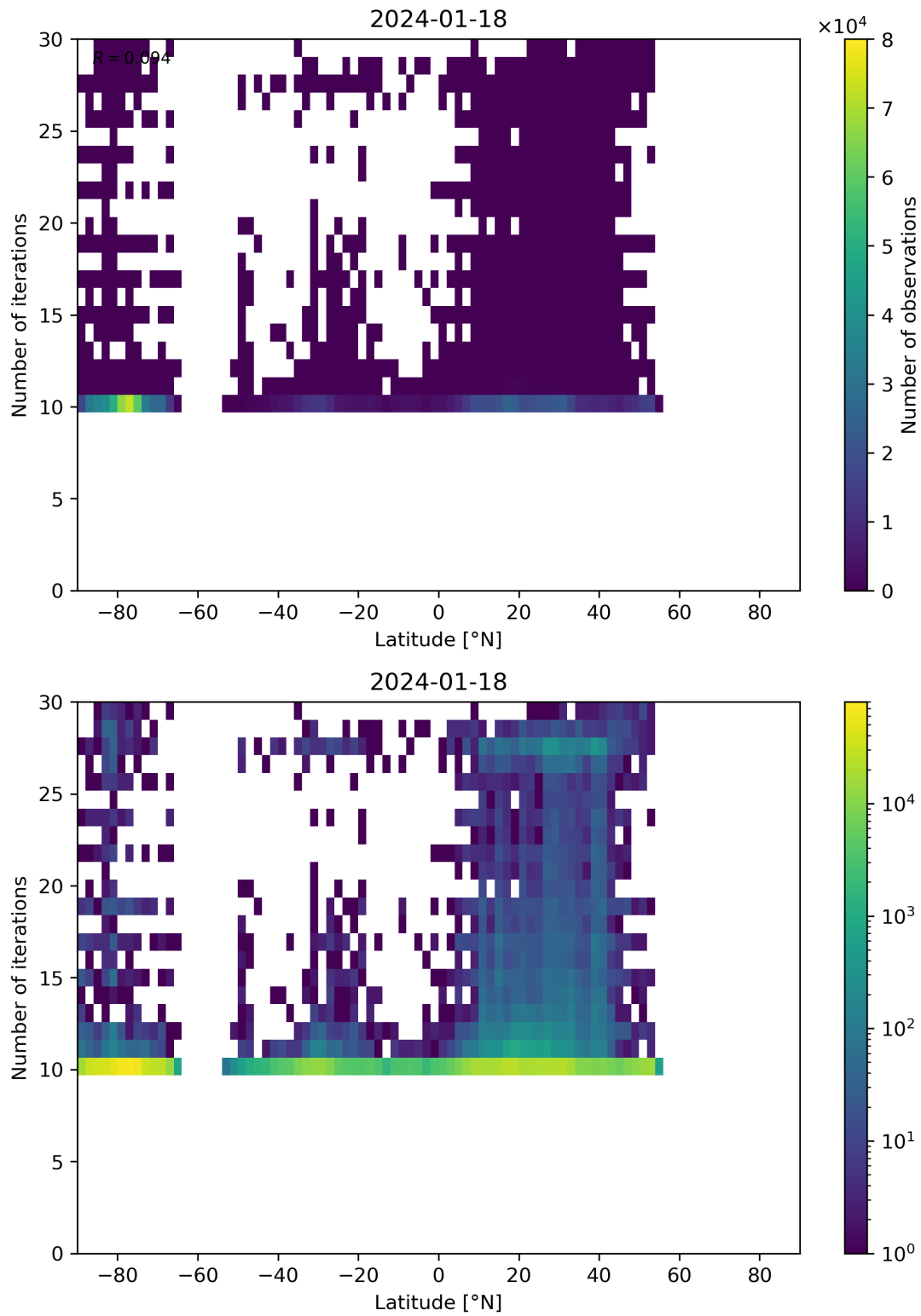
Figure 60: Scatter density plot of “Latitude” against “Number of iterations” for 2024-01-17 to 2024-01-19.
