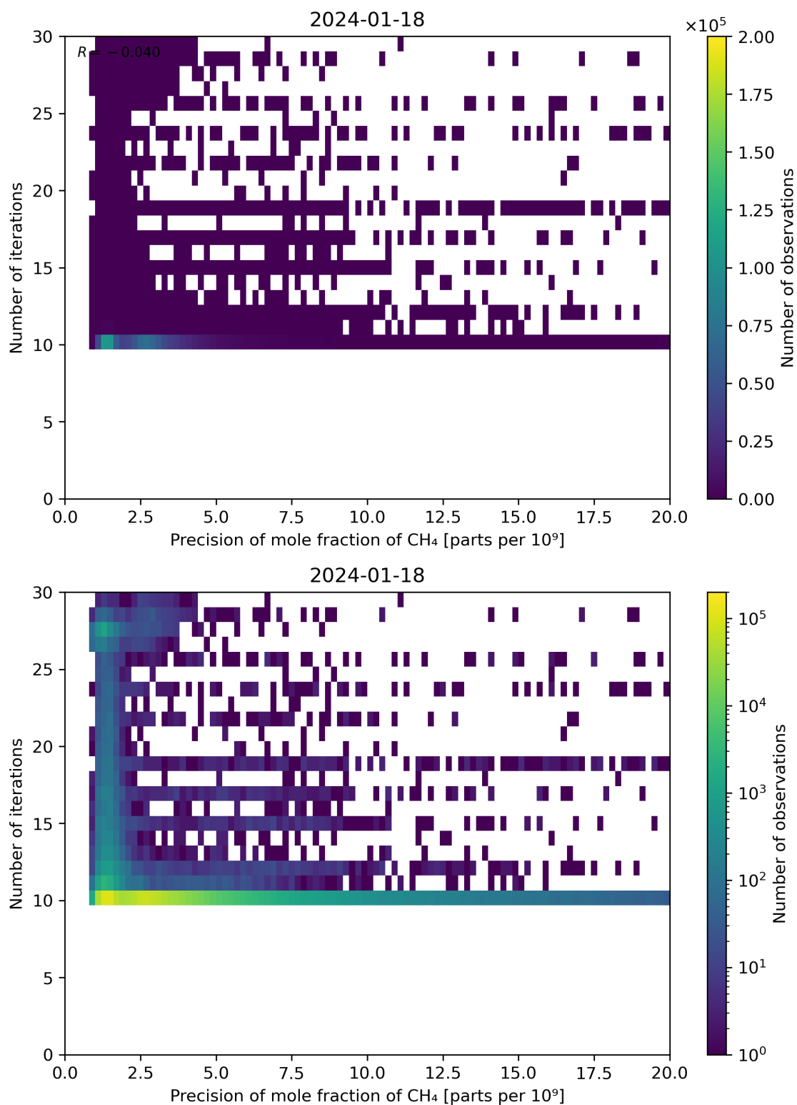
Figure 83: Scatter density plot of “Precision of mole fraction of CH 4 ” against “Number of iterations” for 2024-01-17 to 2024-01-19.
