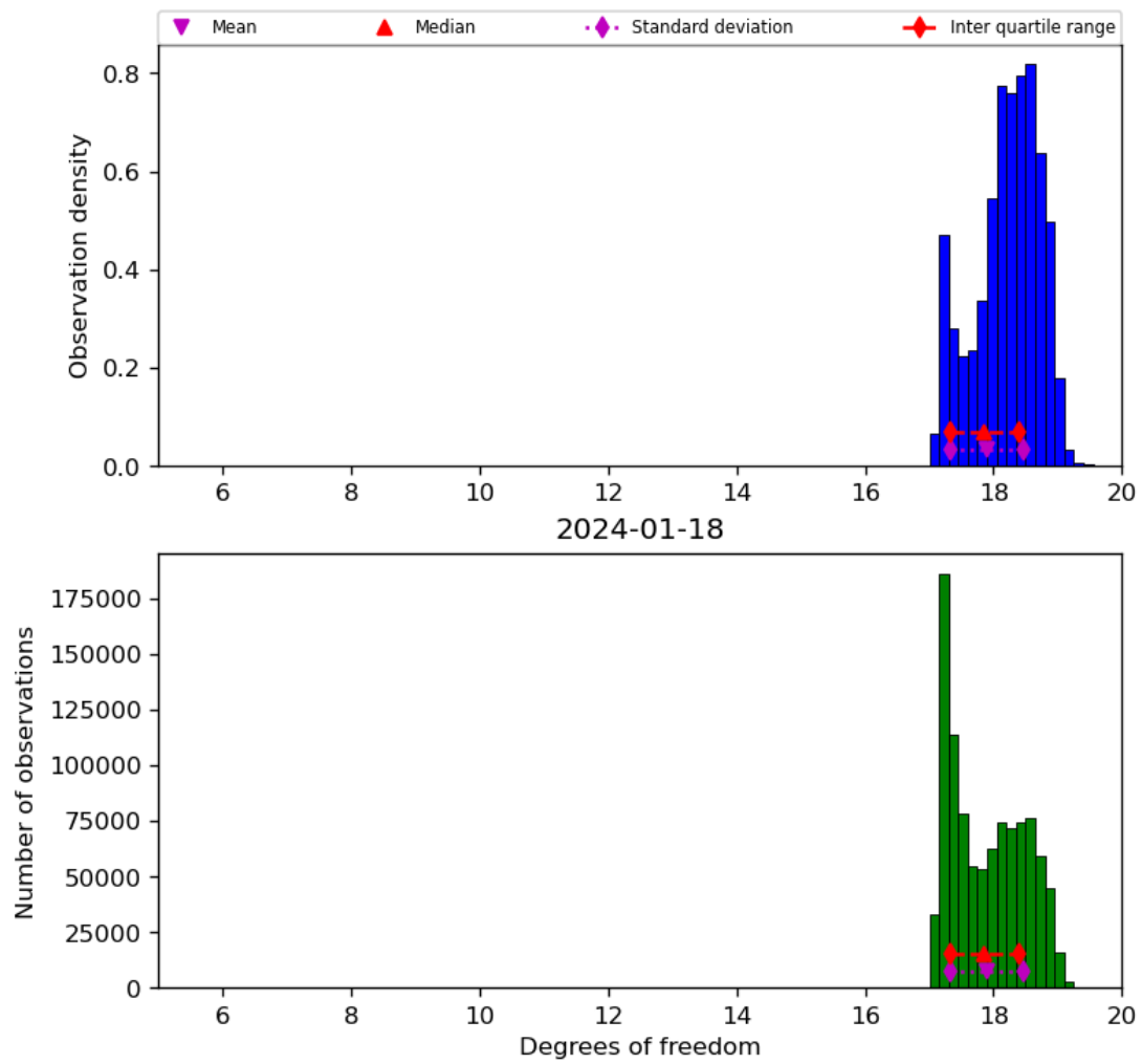
Figure 30: Histogram of “Degrees of freedom” for 2024-01-17 to 2024-01-19
