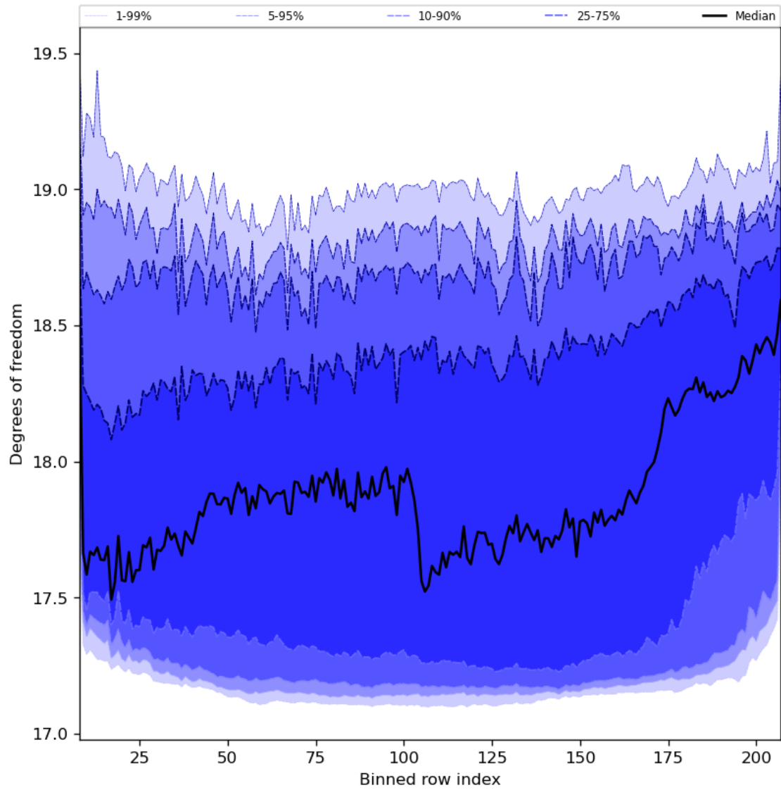
Figure 41: Along track statistics of “Degrees of freedom” for 2024-01-17 to 2024-01-19
