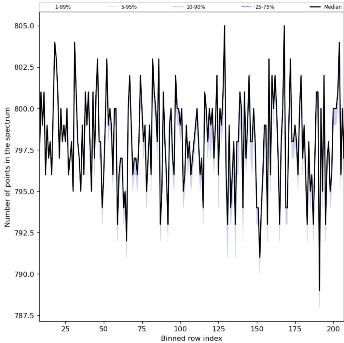
Figure 37: Along track statistics of “Number of points in the spectrum” for 2024-01-17 to 2024-01-19
