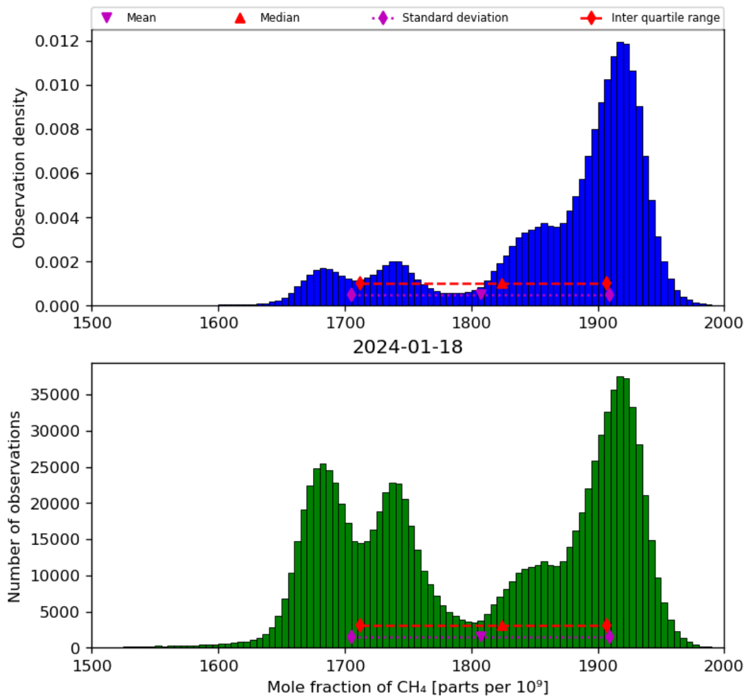
Figure 23: Histogram of “Mole fraction of CH 4 ” for 2024-01-17 to 2024-01-19
