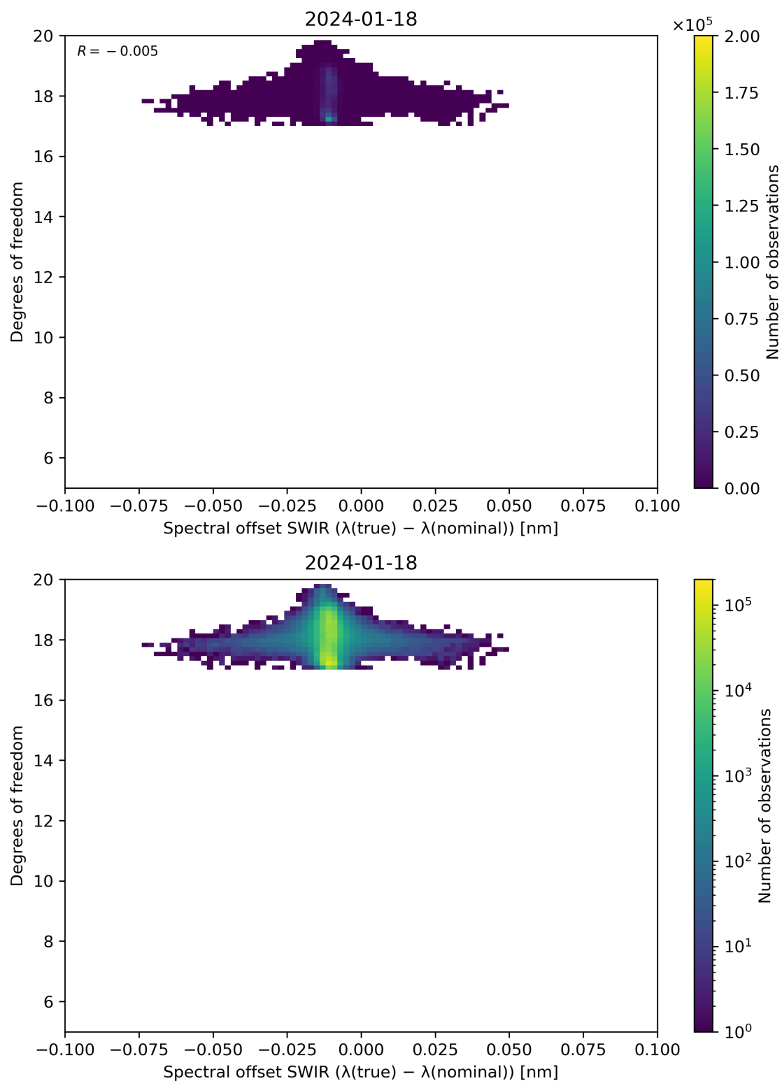
Figure 119: Scatter density plot of “Spectral offset SWIR ( \lambda(\text{true}) - \lambda(\text{nominal}) )” against “Degrees of freedom” for 2024-01-17 to 2024-01-19.
