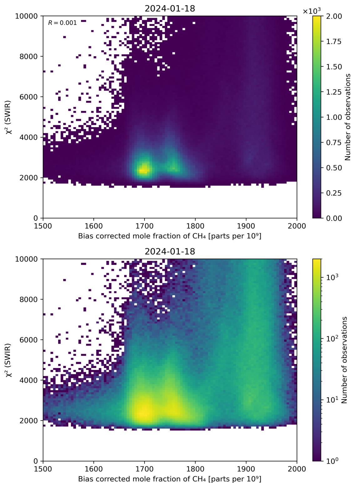
Figure 64: Scatter density plot of “Bias corrected mole fraction of \text{CH}_4 ” against “ \chi^2 (SWIR)” for 2024-01-17 to 2024-01-19.
