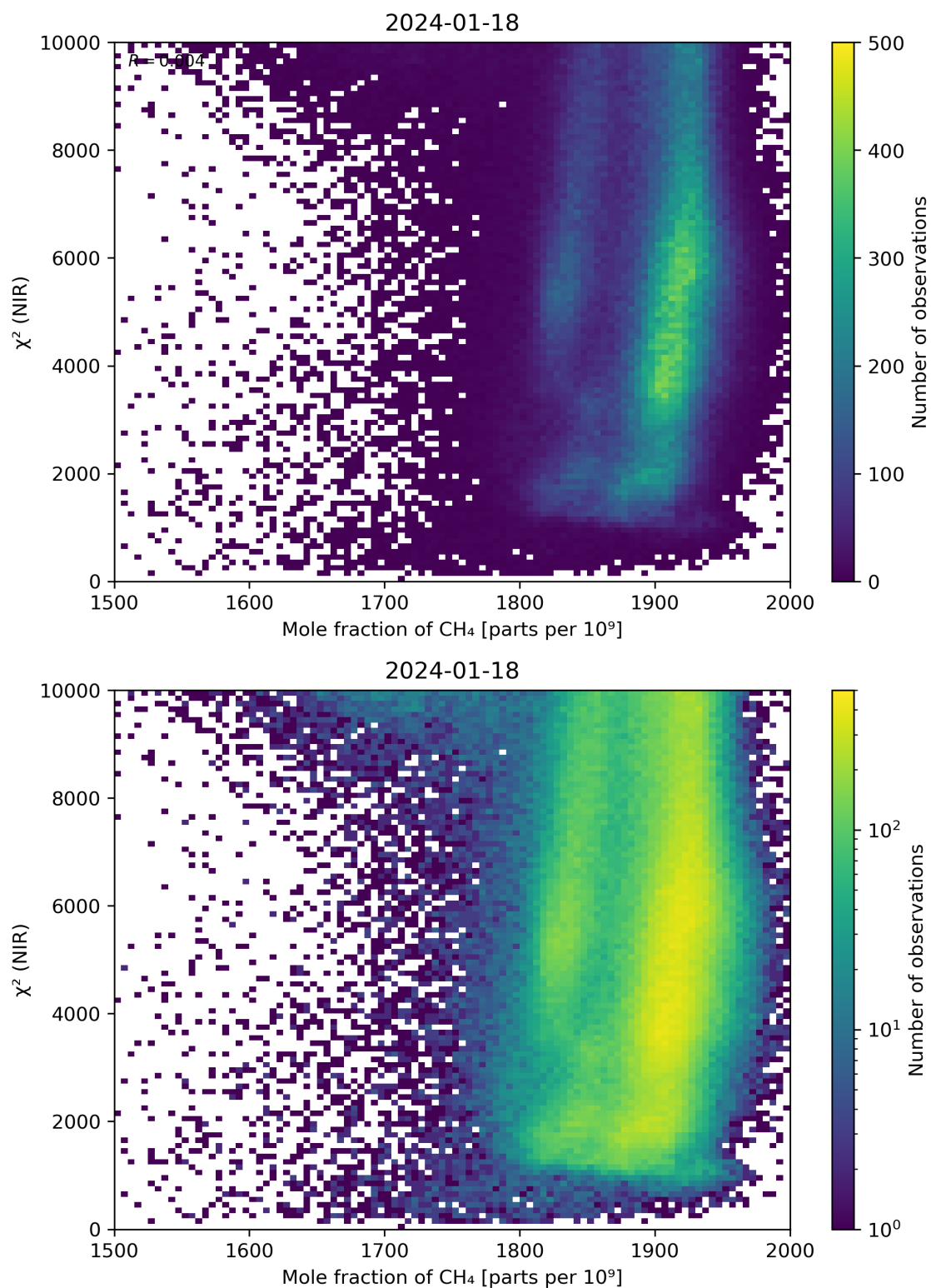
Figure 70: Scatter density plot of “Mole fraction of \text{CH}_4 ” against “ \chi^2 (NIR)” for 2024-01-17 to 2024-01-19.
