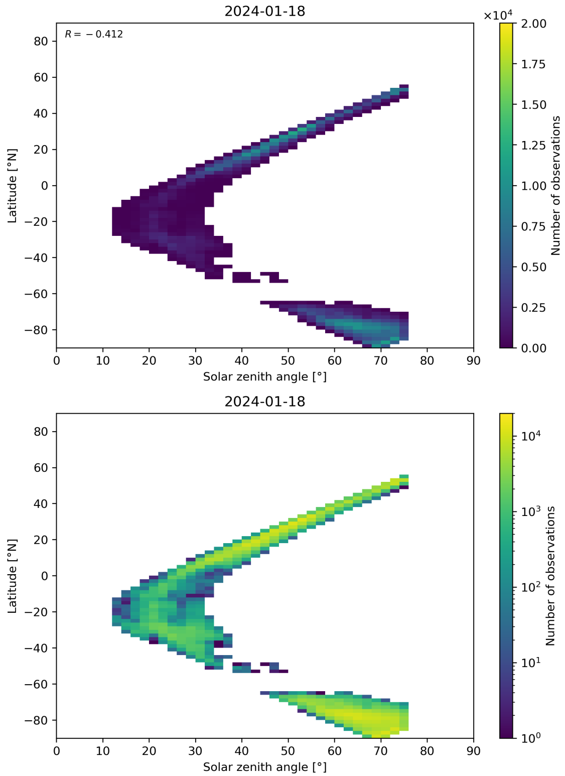
Figure 98: Scatter density plot of “Solar zenith angle” against “Latitude” for 2024-01-17 to 2024-01-19.
