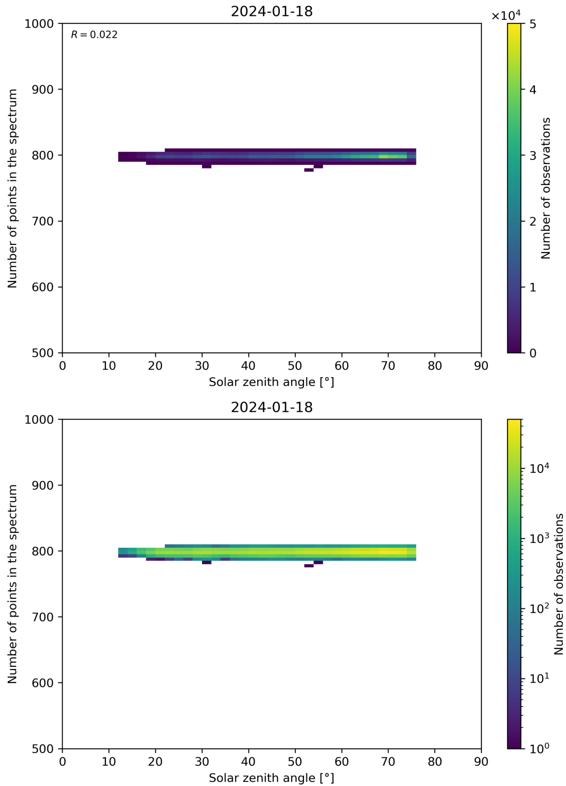
Figure 103: Scatter density plot of “Solar zenith angle” against “Number of points in the spectrum” for 2024-01-17 to 2024-01-19.
