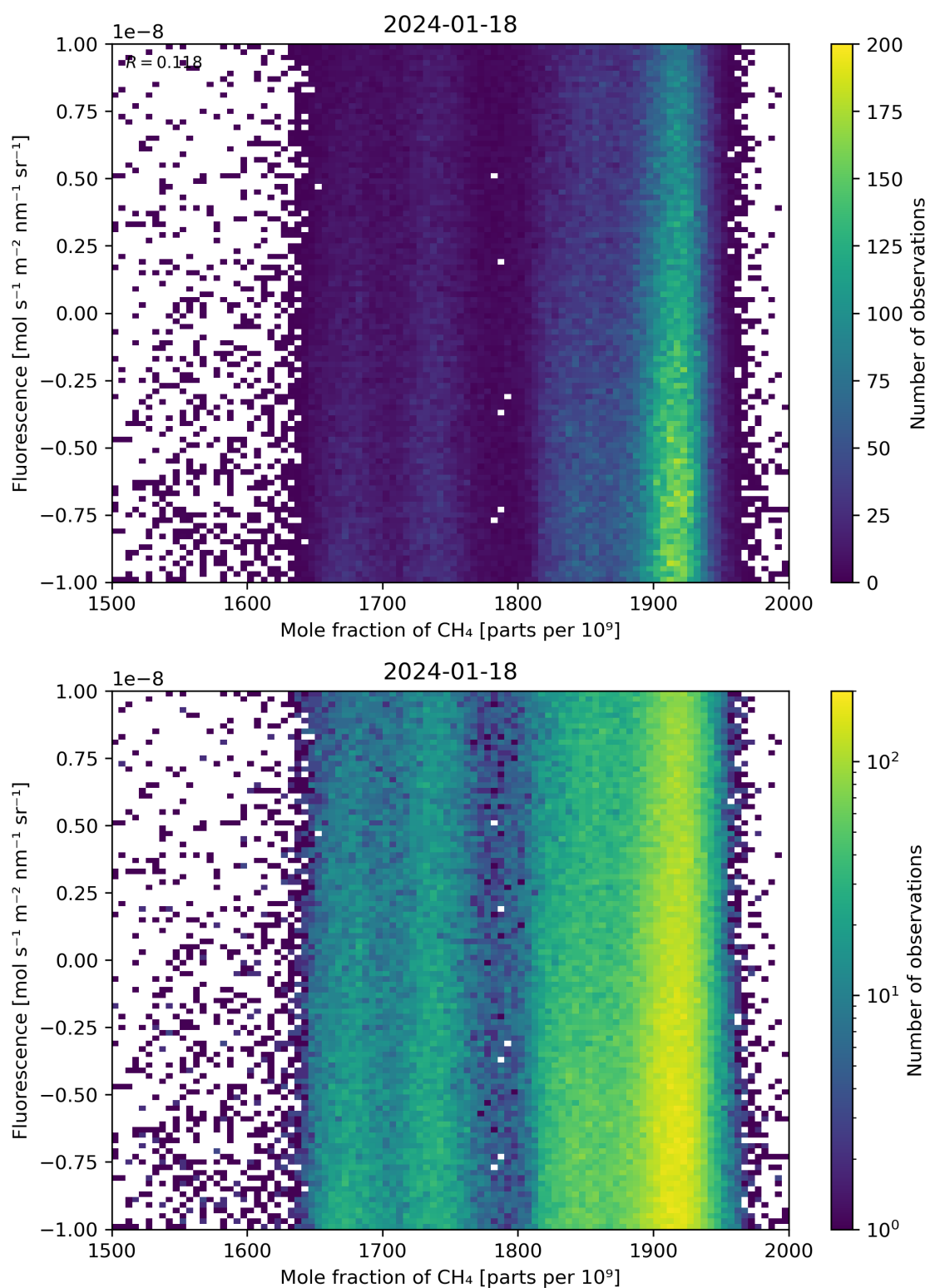
Figure 73: Scatter density plot of “Mole fraction of \text{CH}_4 ” against “Fluorescence” for 2024-01-17 to 2024-01-19.
