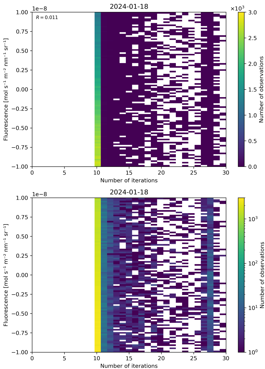
Figure 87: Scatter density plot of “Number of iterations” against “Fluorescence” for 2024-01-17 to 2024-01-19.
