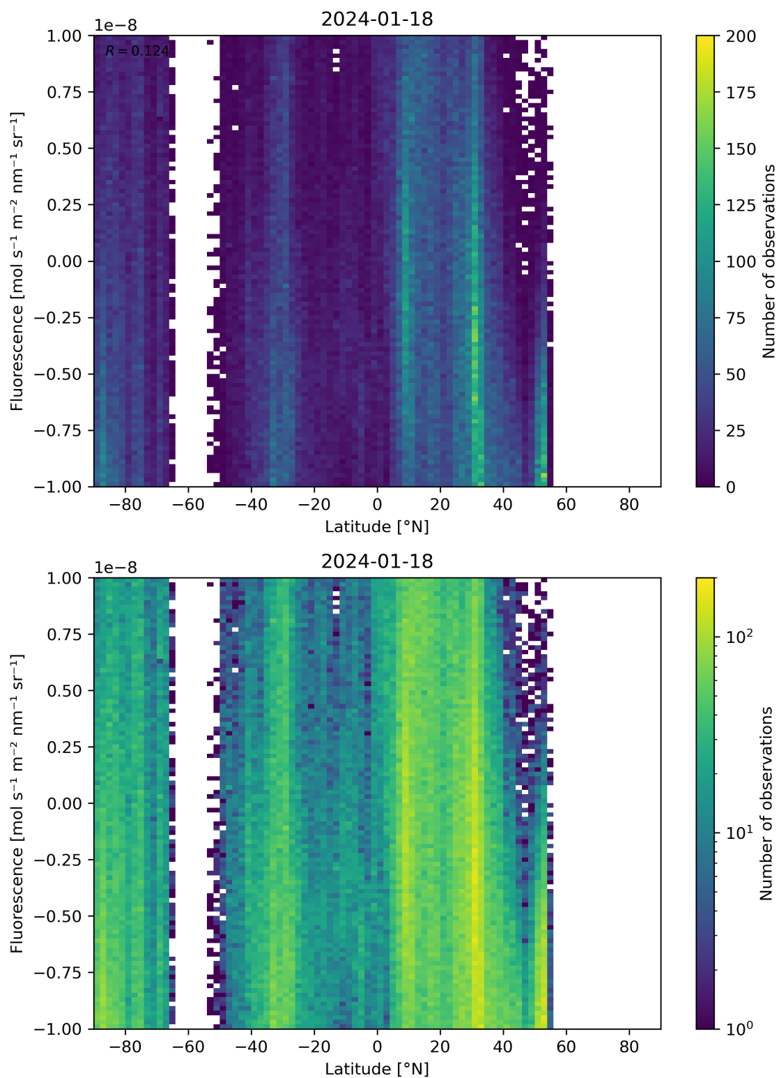
Figure 56: Scatter density plot of “Latitude” against “Fluorescence” for 2024-01-17 to 2024-01-19.
