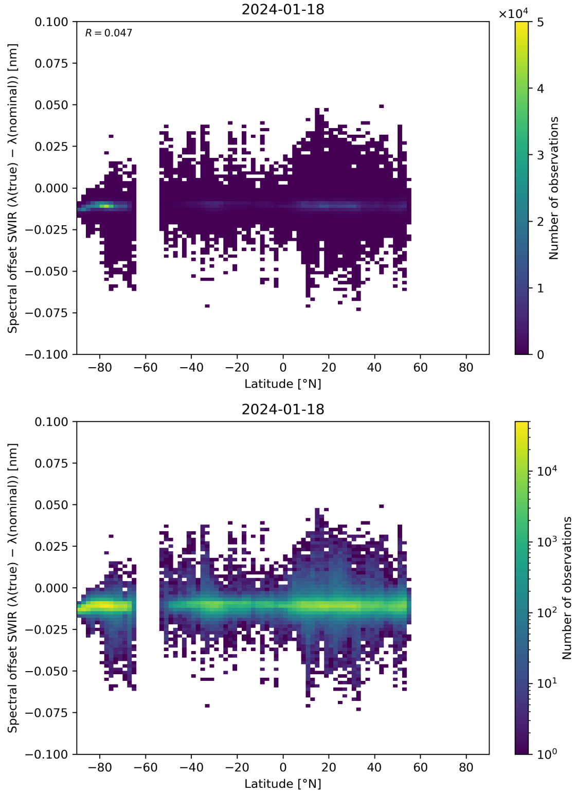
Figure 62: Scatter density plot of “Latitude” against “Spectral offset SWIR ( \lambda(\text{true}) - \lambda(\text{nominal}) )” for 2024-01-17 to 2024-01-19.
