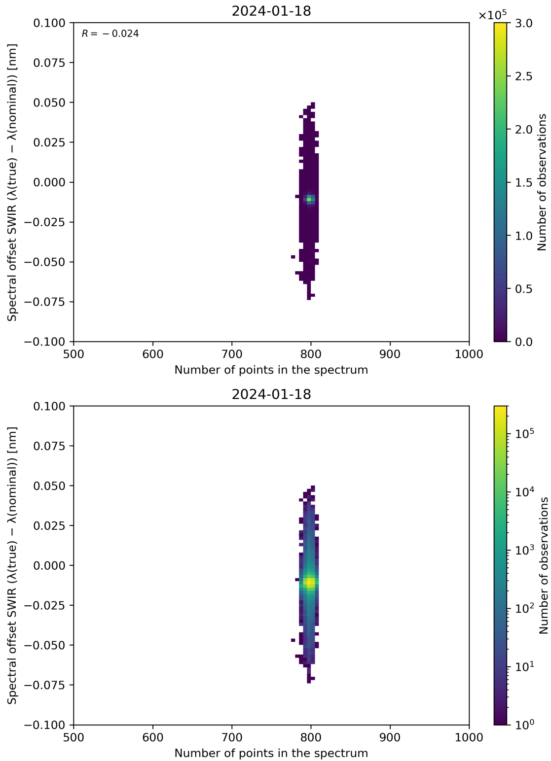
Figure 93: Scatter density plot of “Number of points in the spectrum” against “Spectral offset SWIR ( \lambda(\text{true}) - \lambda(\text{nominal}) )” for 2024-01-17 to 2024-01-19.
