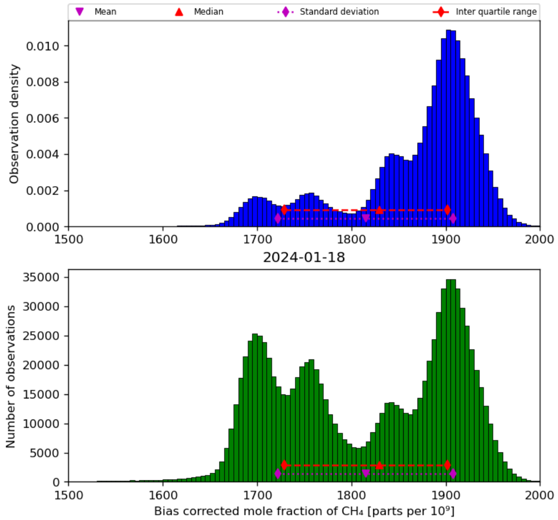
Figure 25: Histogram of “Bias corrected mole fraction of CH 4 ” for 2024-01-17 to 2024-01-19
