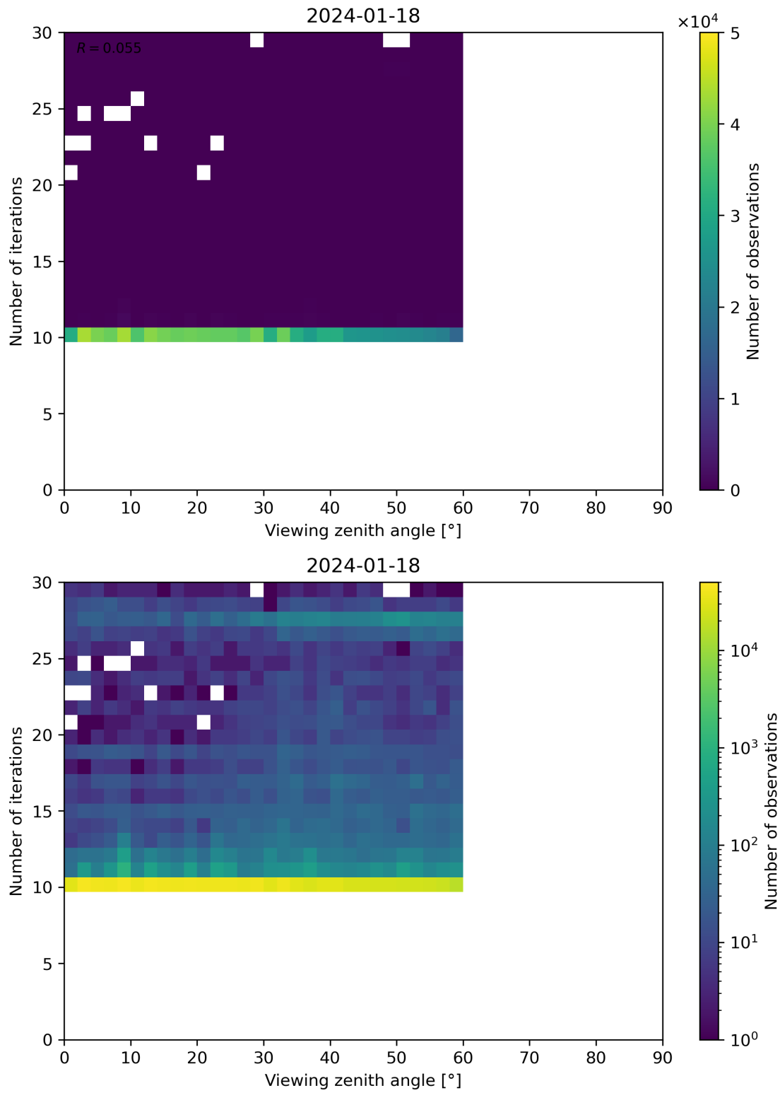
Figure 113: Scatter density plot of “Viewing zenith angle” against “Number of iterations” for 2024-01-17 to 2024-01-19.
