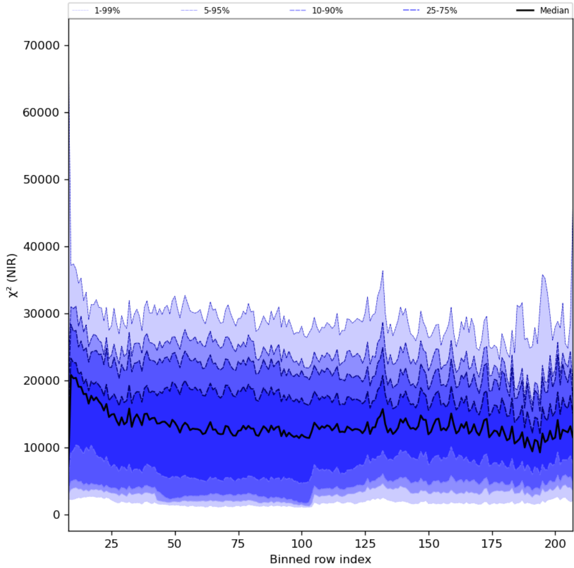
Figure 40: Along track statistics of “ \chi^2 (NIR)” for 2024-01-17 to 2024-01-19
