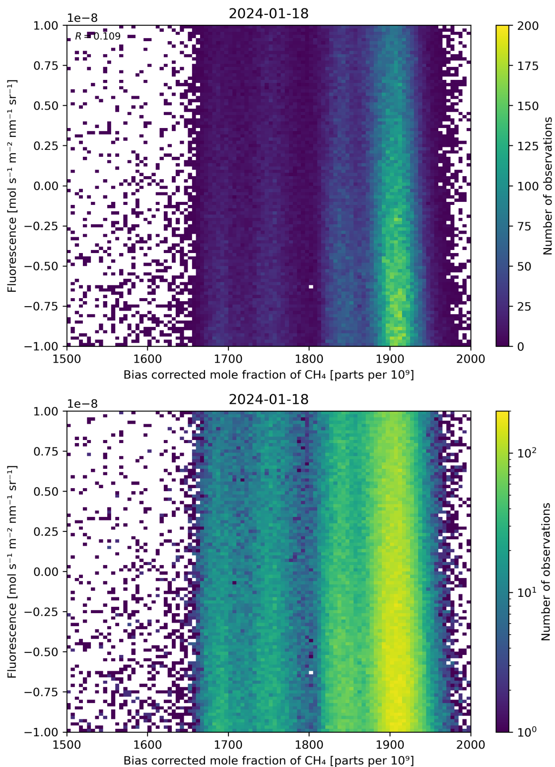
Figure 66: Scatter density plot of “Bias corrected mole fraction of \text{CH}_4 ” against “Fluorescence” for 2024-01-17 to 2024-01-19.
