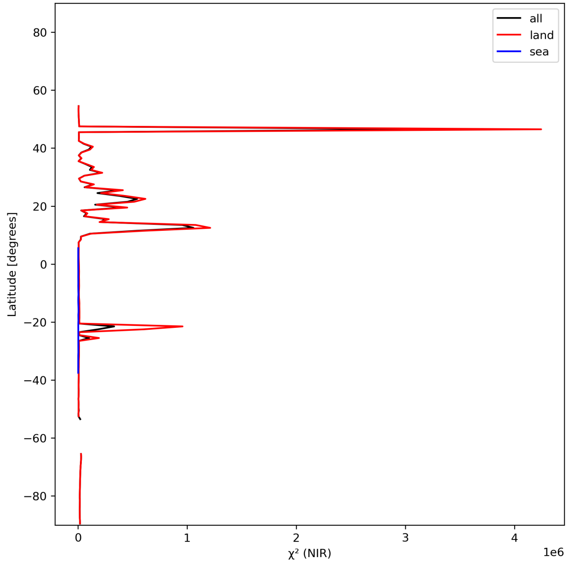
Figure 18: Zonal average of “ \chi^2 (NIR)” for 2024-01-17 to 2024-01-19.
