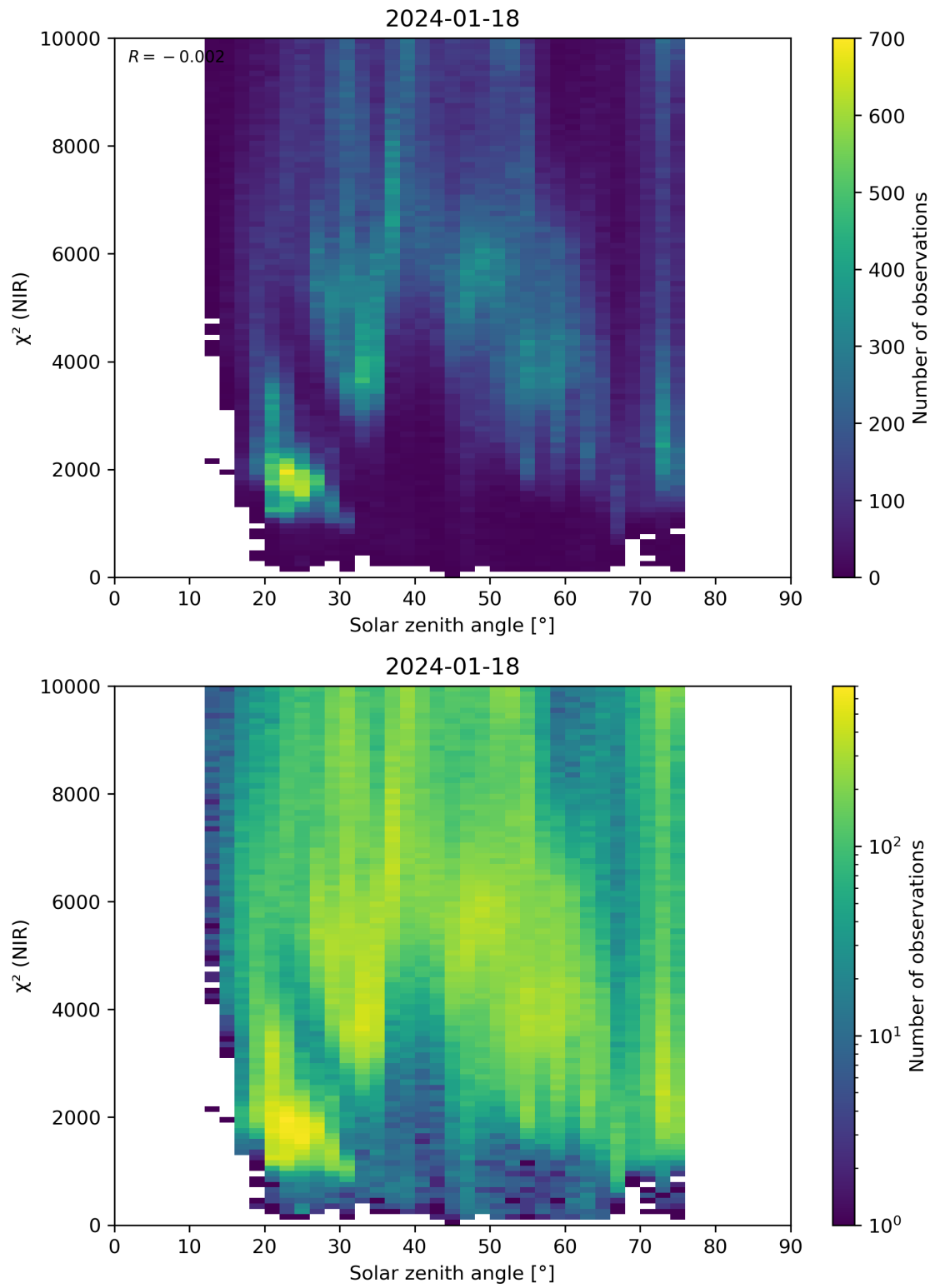
Figure 94: Scatter density plot of “Solar zenith angle” against “ \chi^2 (NIR)” for 2024-01-17 to 2024-01-19.
