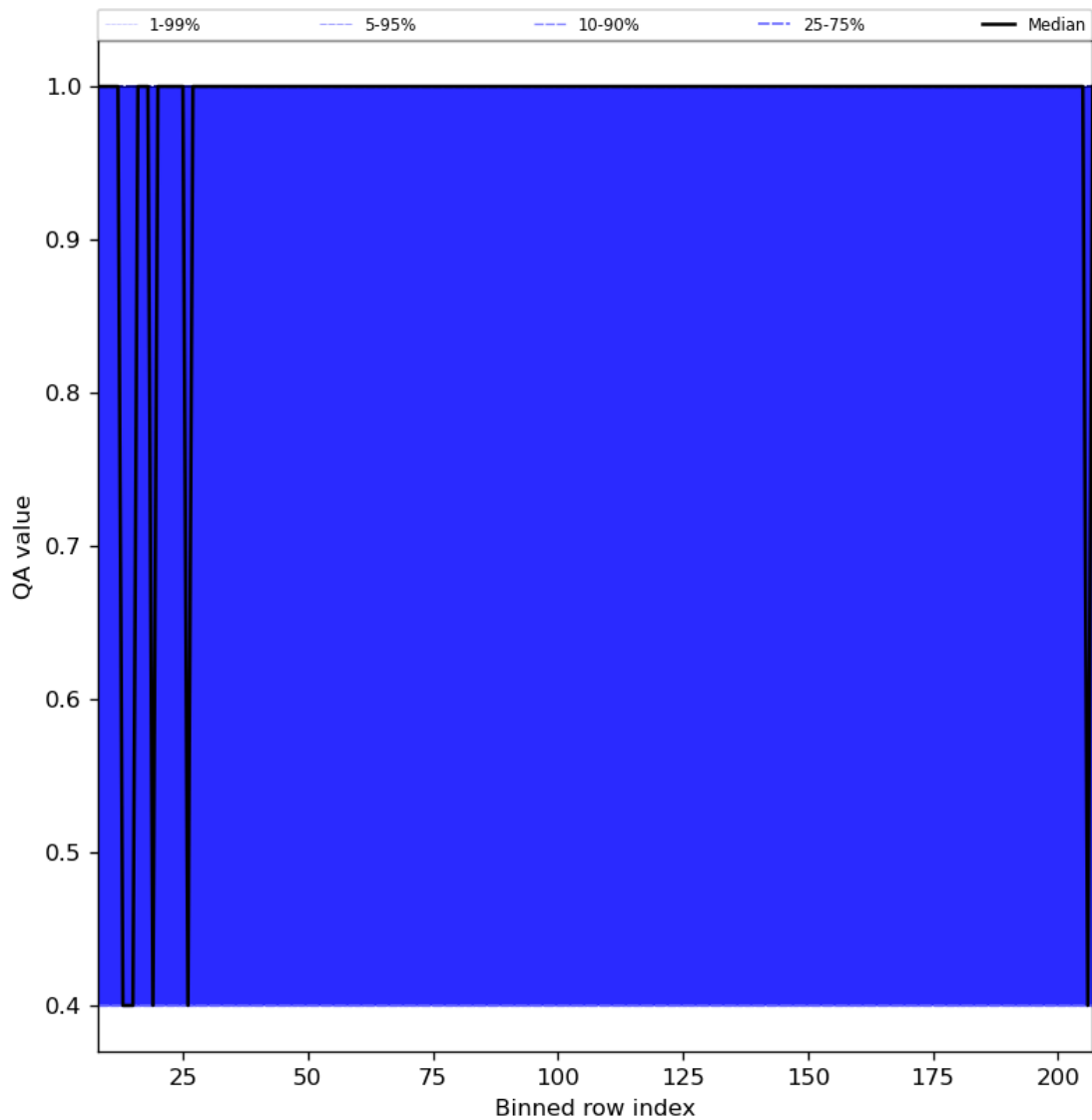
Figure 33: Along track statistics of “QA value” for 2024-01-17 to 2024-01-19
