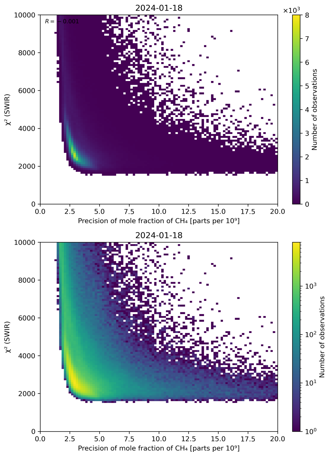
Figure 79: Scatter density plot of “Precision of mole fraction of \text{CH}_4 ” against “ \chi^2 (SWIR)” for 2024-01-17 to 2024-01-19.
