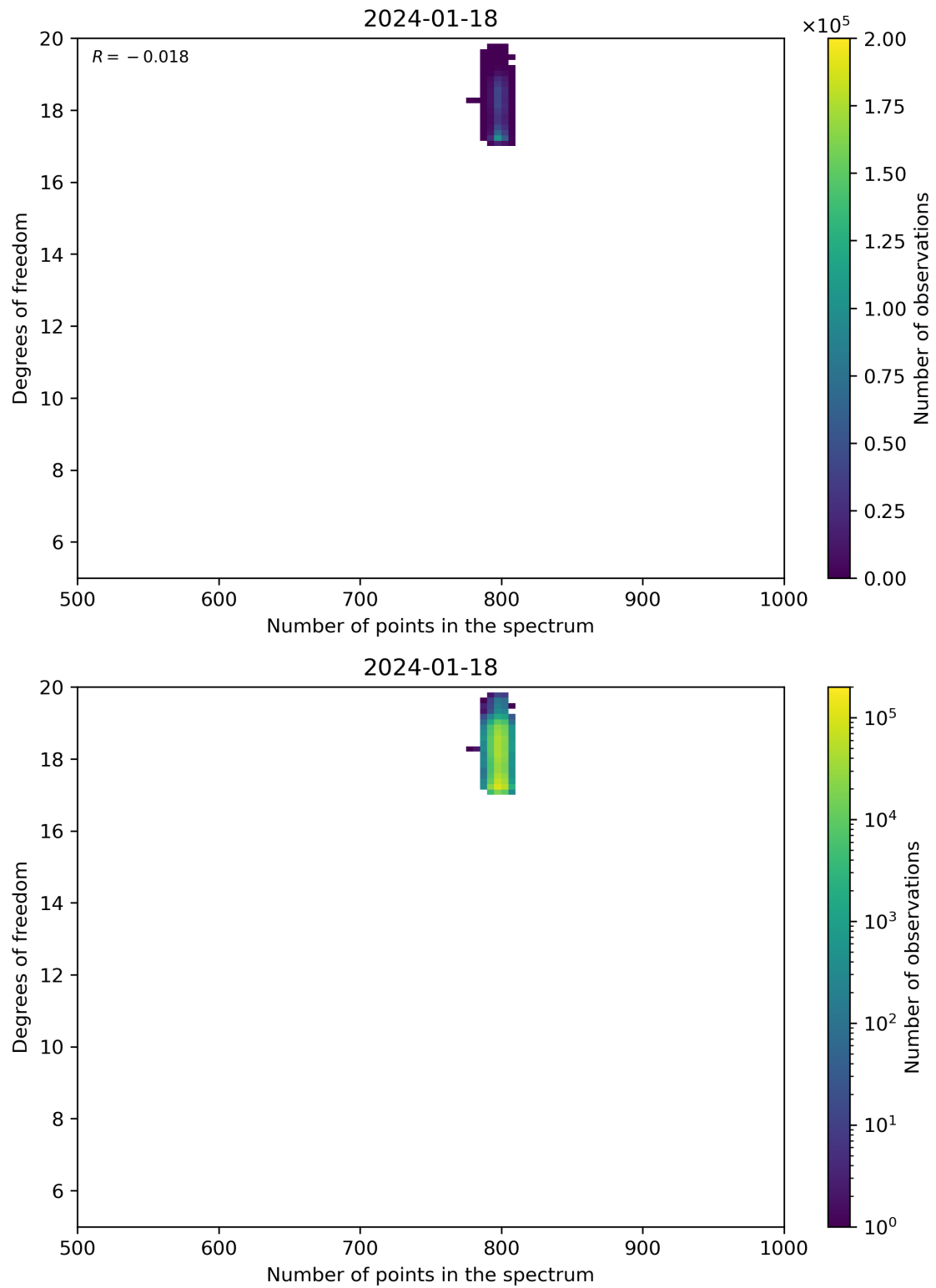
Figure 90: Scatter density plot of “Number of points in the spectrum” against “Degrees of freedom” for 2024-01-17 to 2024-01-19.
