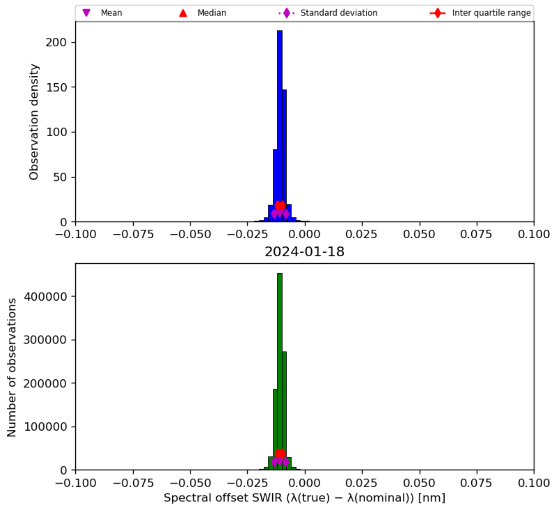
Figure 27: Histogram of “Spectral offset SWIR ( \lambda(\text{true}) - \lambda(\text{nominal}) )” for 2024-01-17 to 2024-01-19
