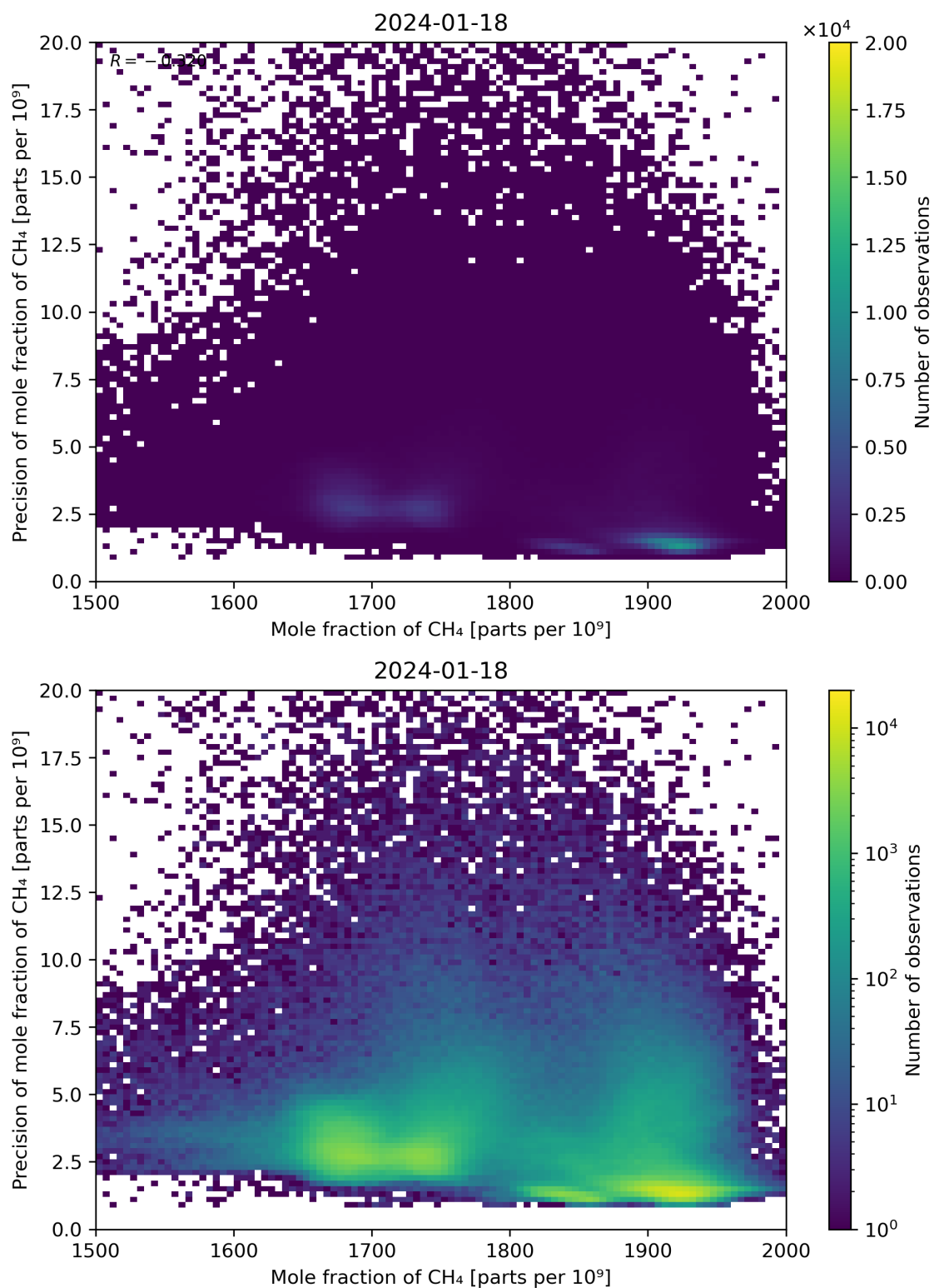
Figure 75: Scatter density plot of “Mole fraction of CH 4 ” against “Precision of mole fraction of CH 4 ” for 2024-01-17 to 2024-01-19.
