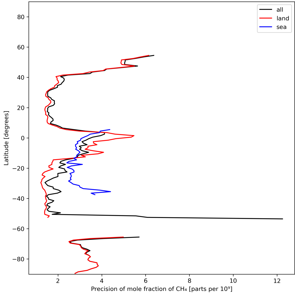
Figure 13: Zonal average of “Precision of mole fraction of CH 4 ” for 2024-01-17 to 2024-01-19.
