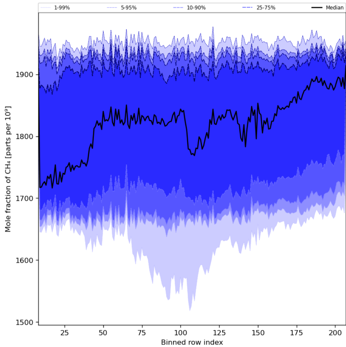
Figure 34: Along track statistics of “Mole fraction of CH 4 ” for 2024-01-17 to 2024-01-19
