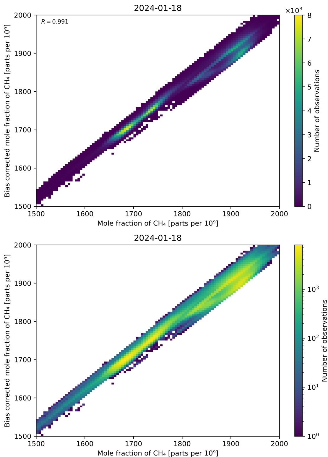
Figure 74: Scatter density plot of “Mole fraction of CH 4 ” against “Bias corrected mole fraction of CH 4 ” for 2024-01-17 to 2024-01-19.
