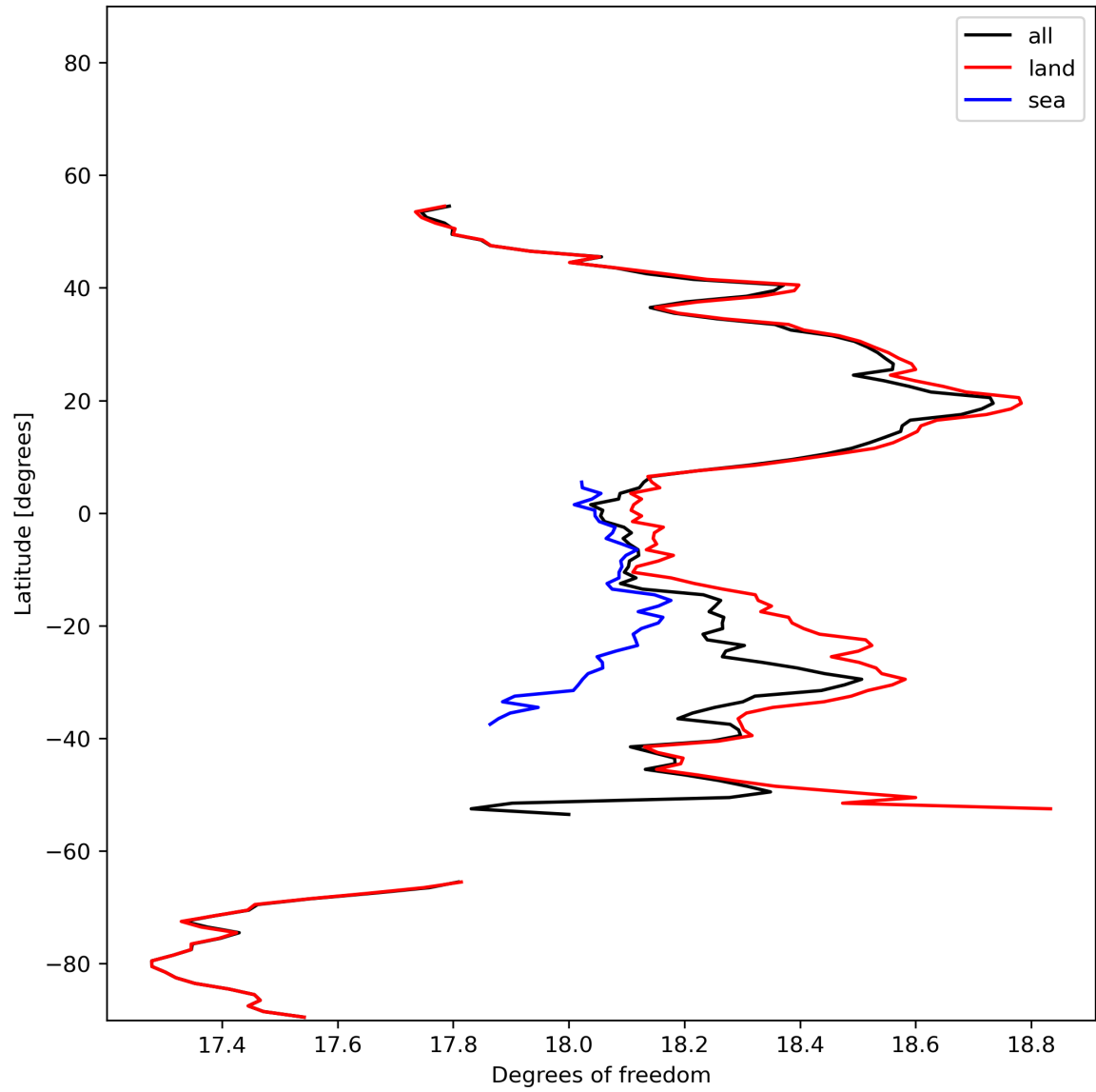
Figure 19: Zonal average of “Degrees of freedom” for 2024-01-17 to 2024-01-19.
