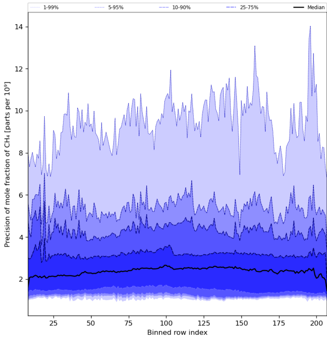
Figure 35: Along track statistics of “Precision of mole fraction of CH 4 ” for 2024-01-18 to 2024-01-20
