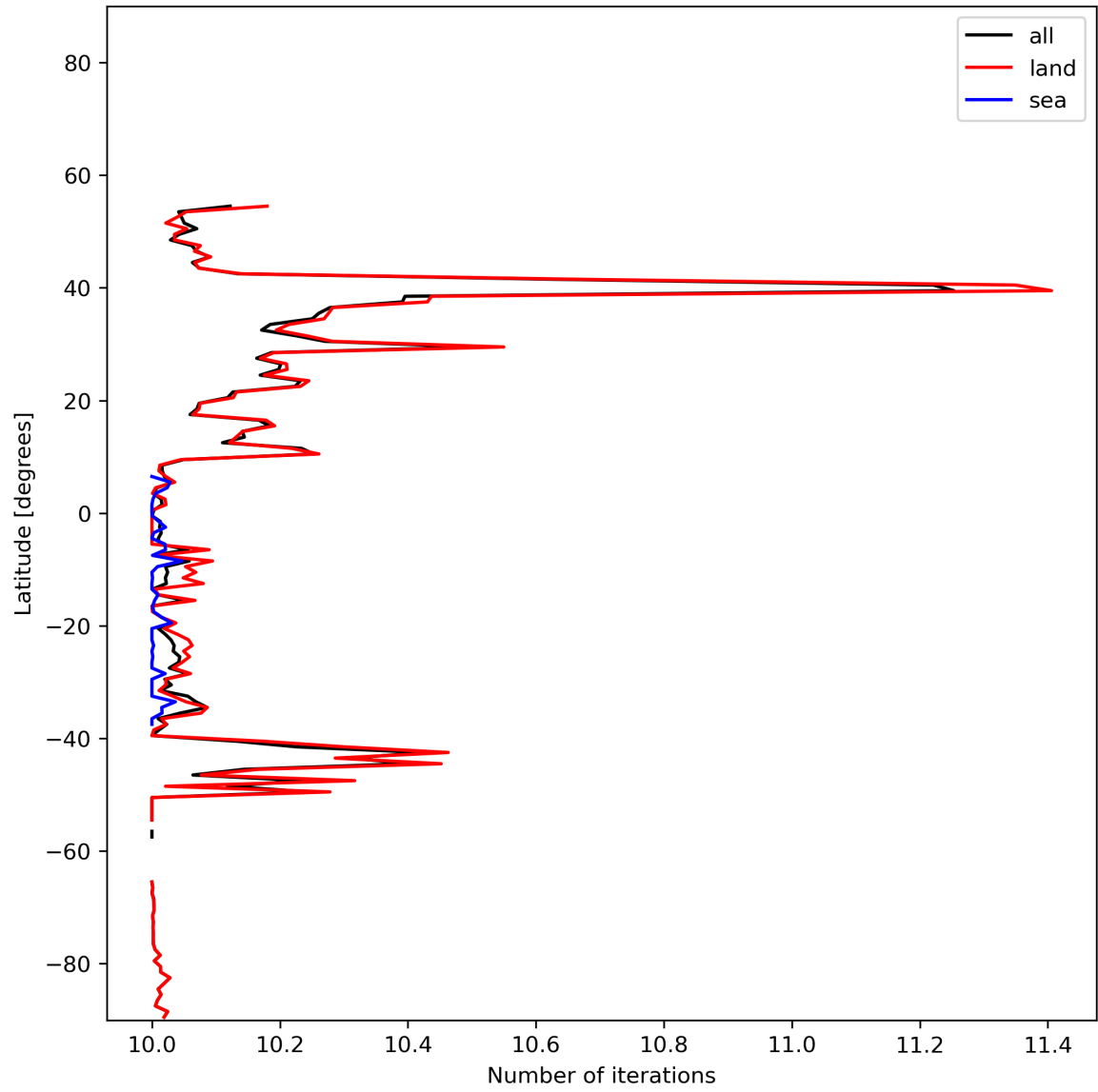
Figure 20: Zonal average of “Number of iterations” for 2024-01-18 to 2024-01-20.
