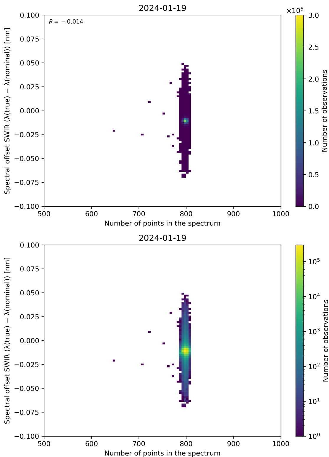
Figure 93: Scatter density plot of “Number of points in the spectrum” against “Spectral offset SWIR ( \lambda(\text{true}) - \lambda(\text{nominal}) )” for 2024-01-18 to 2024-01-20.
