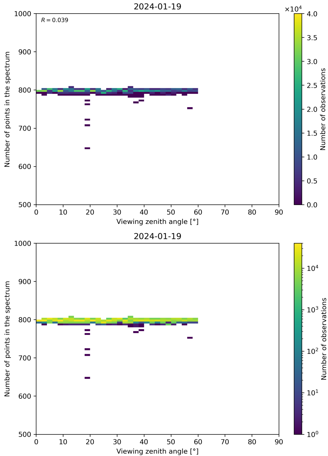
Figure 114: Scatter density plot of “Viewing zenith angle” against “Number of points in the spectrum” for 2024-01-18 to 2024-01-20.
