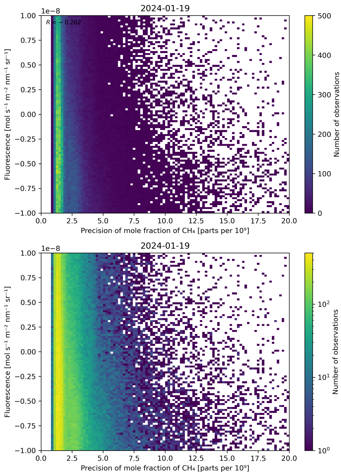
Figure 81: Scatter density plot of “Precision of mole fraction of \text{CH}_4 ” against “Fluorescence” for 2024-01-18 to 2024-01-20.
