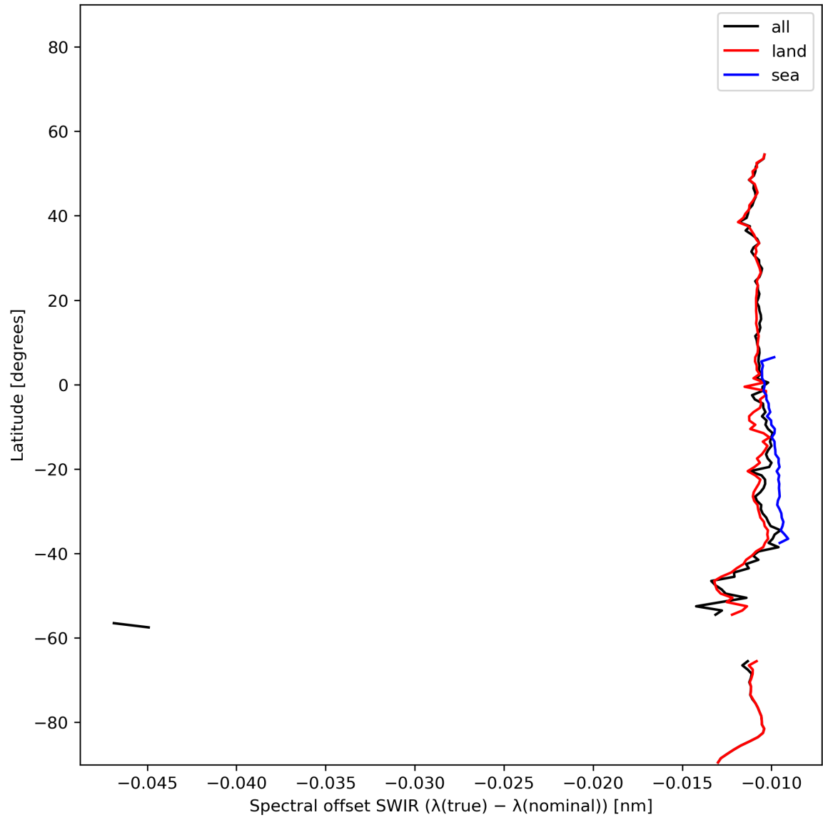
Figure 16: Zonal average of “Spectral offset SWIR ( \lambda(\text{true}) - \lambda(\text{nominal}) )” for 2024-01-18 to 2024-01-20.
