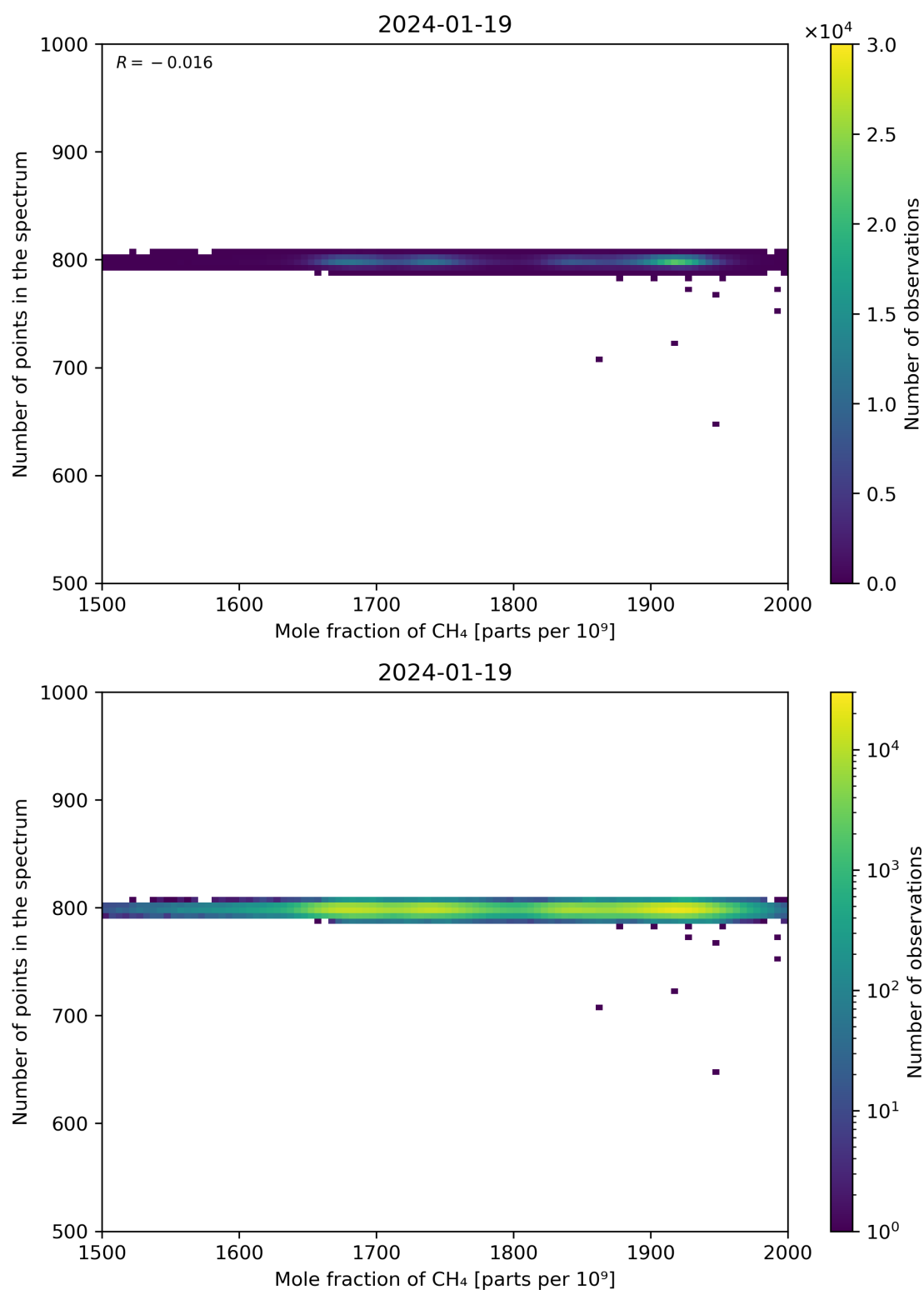
Figure 77: Scatter density plot of “Mole fraction of CH 4 ” against “Number of points in the spectrum” for 2024-01-18 to 2024-01-20.
