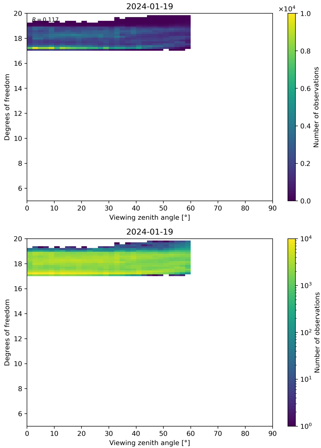
Figure 107: Scatter density plot of “Viewing zenith angle” against “Degrees of freedom” for 2024-01-18 to 2024-01-20.
