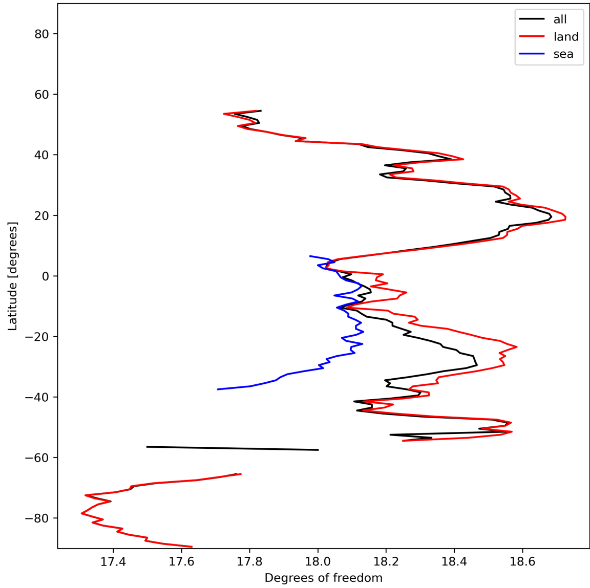
Figure 19: Zonal average of “Degrees of freedom” for 2024-01-18 to 2024-01-20.
