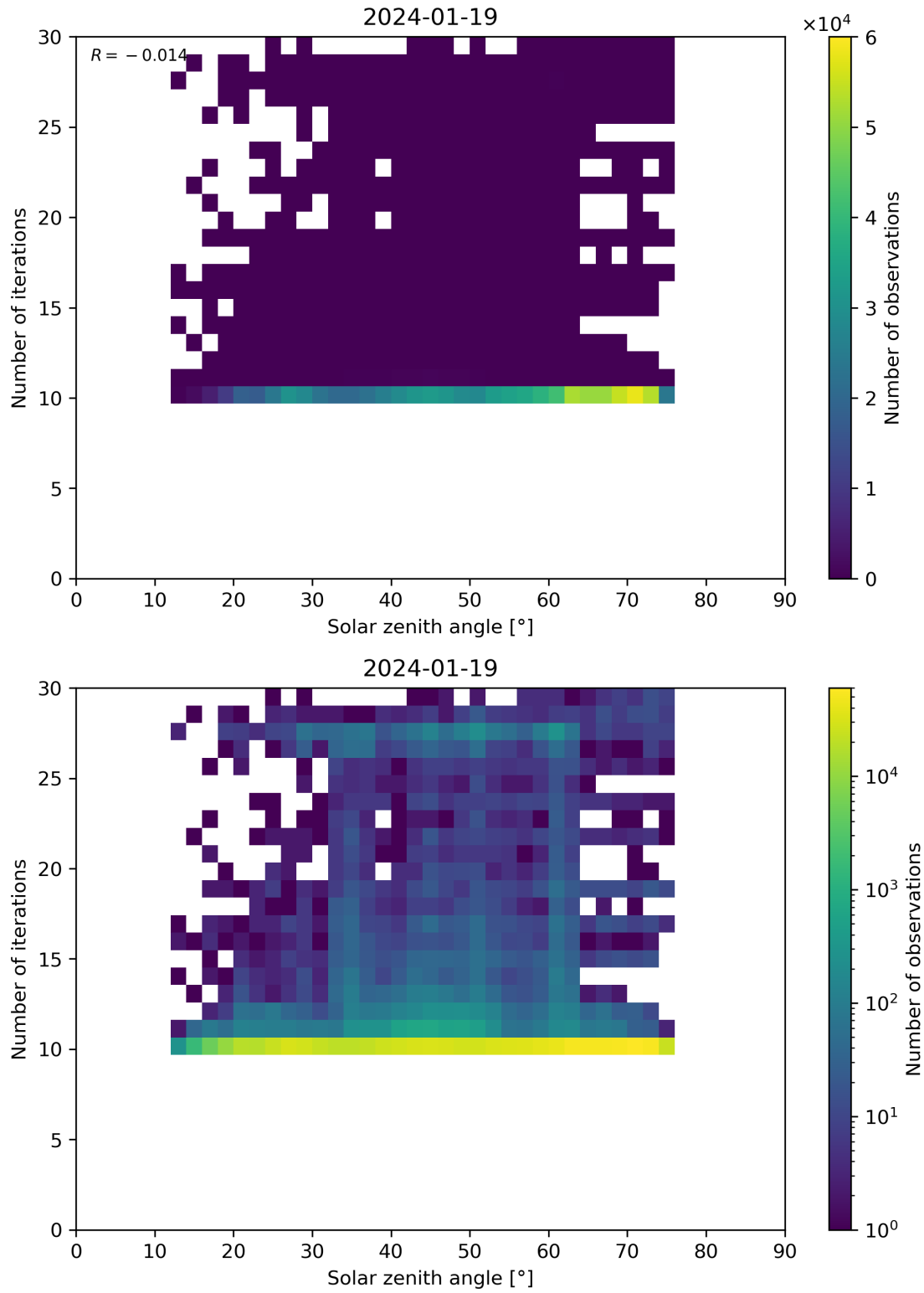
Figure 102: Scatter density plot of “Solar zenith angle” against “Number of iterations” for 2024-01-18 to 2024-01-20.
