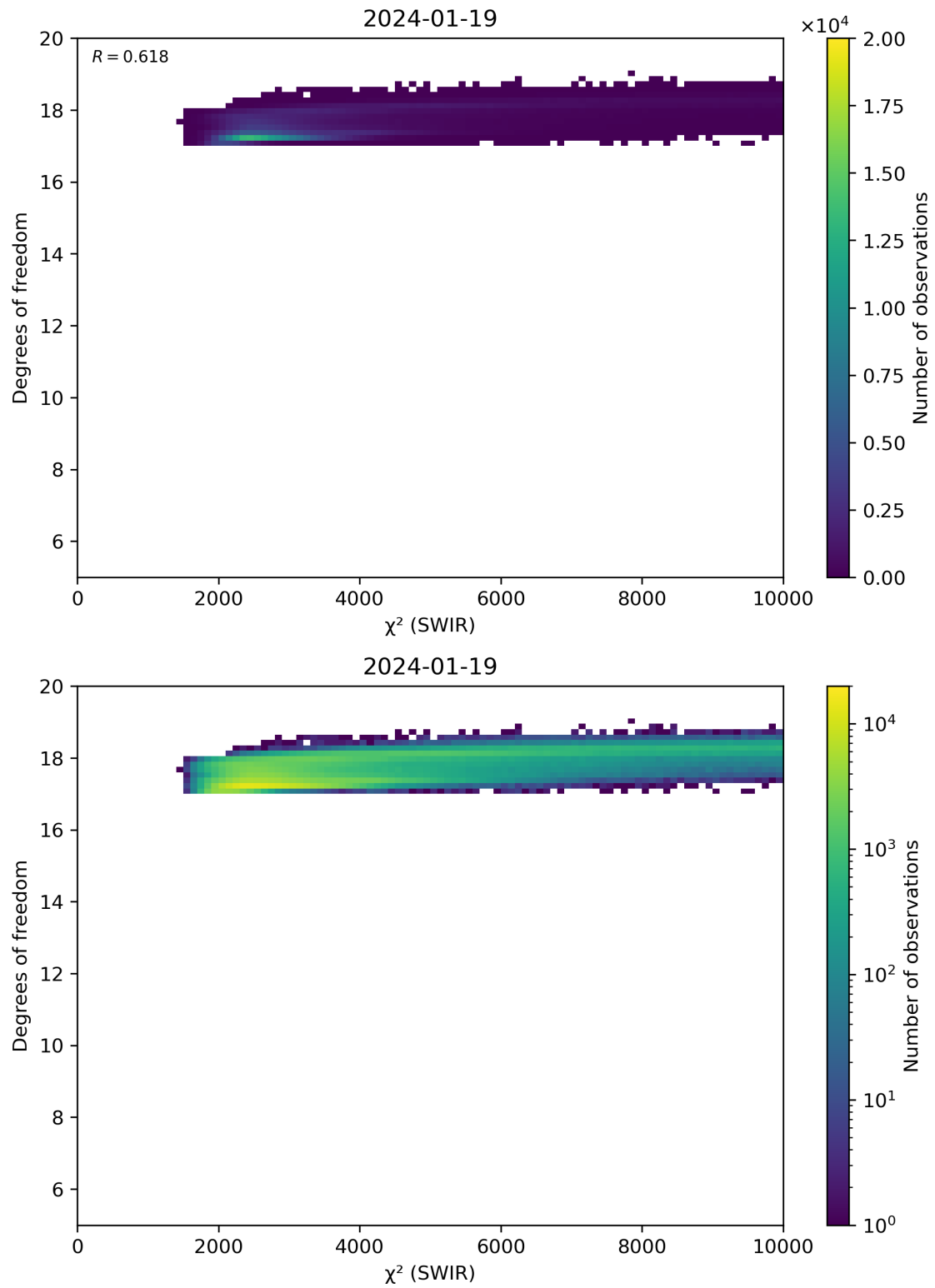
Figure 48: Scatter density plot of “ \chi^2 (SWIR)” against “Degrees of freedom” for 2024-01-18 to 2024-01-20.
