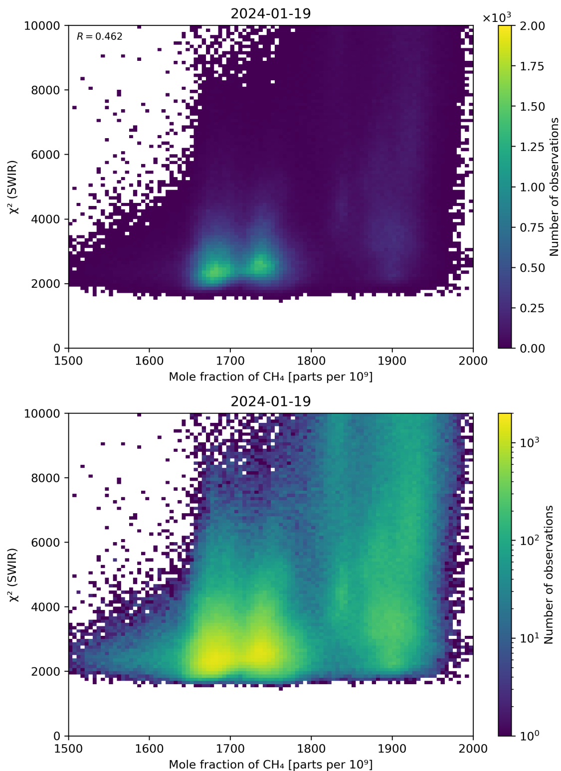
Figure 71: Scatter density plot of “Mole fraction of \text{CH}_4 ” against “ \chi^2 (SWIR)” for 2024-01-18 to 2024-01-20.
