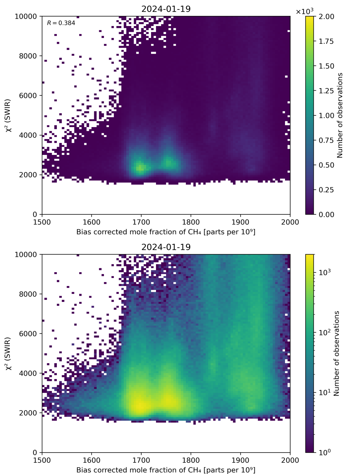
Figure 64: Scatter density plot of “Bias corrected mole fraction of \text{CH}_4 ” against “ \chi^2 (SWIR)” for 2024-01-18 to 2024-01-20.
