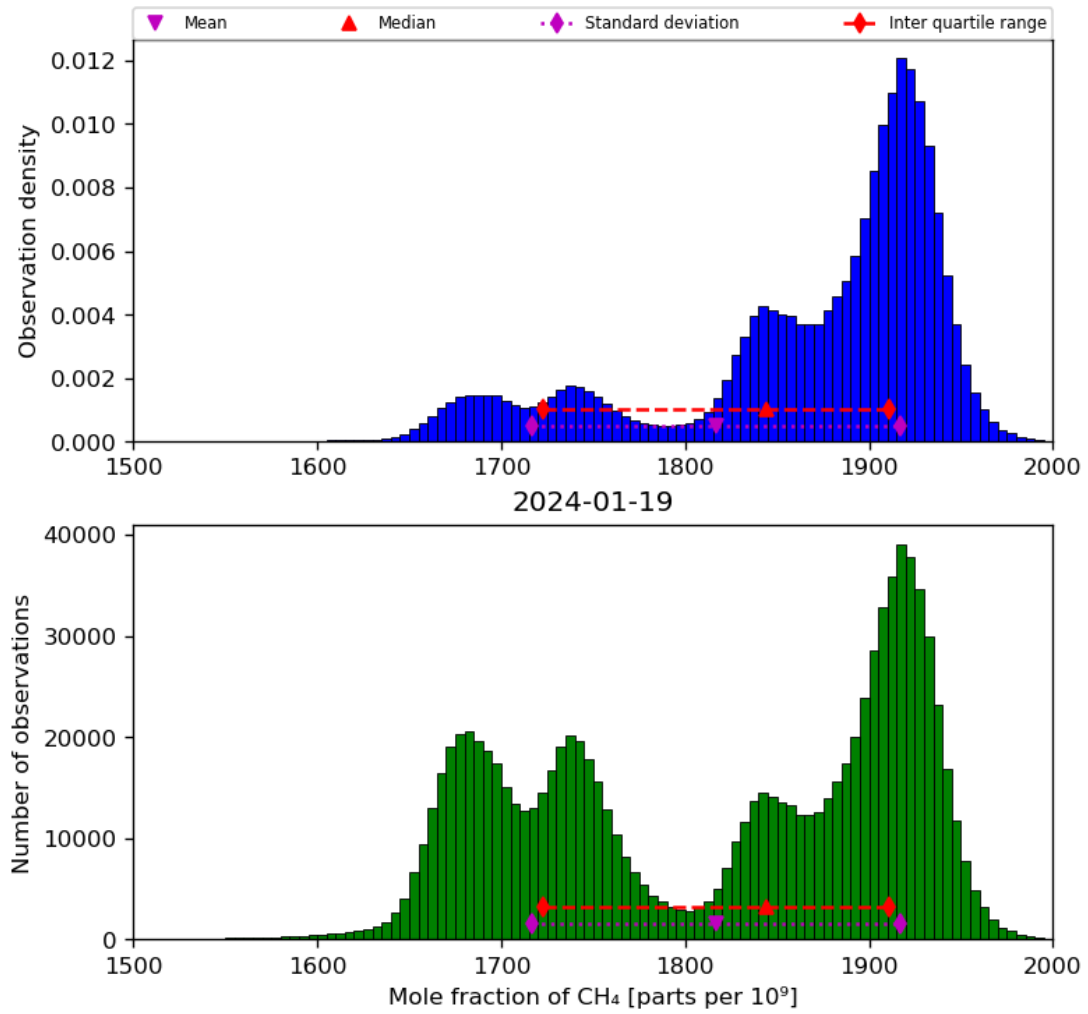
Figure 23: Histogram of “Mole fraction of CH 4 ” for 2024-01-18 to 2024-01-20
