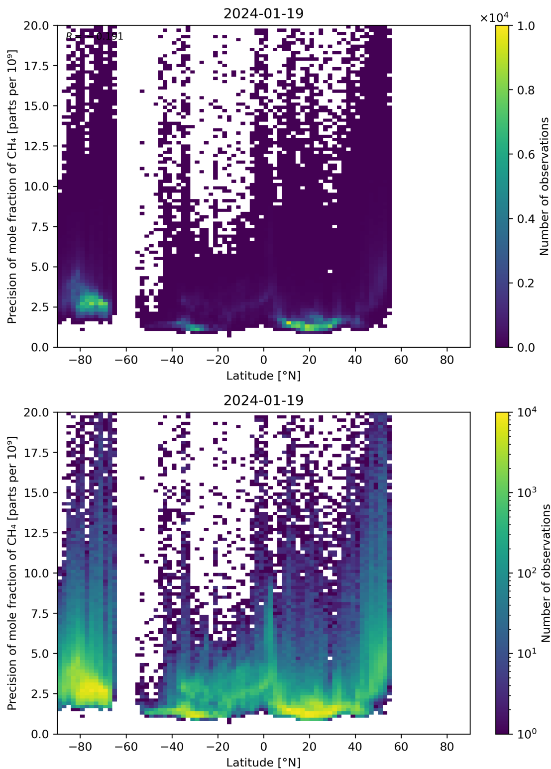
Figure 59: Scatter density plot of “Latitude” against “Precision of mole fraction of CH 4 ” for 2024-01-18 to 2024-01-20.
