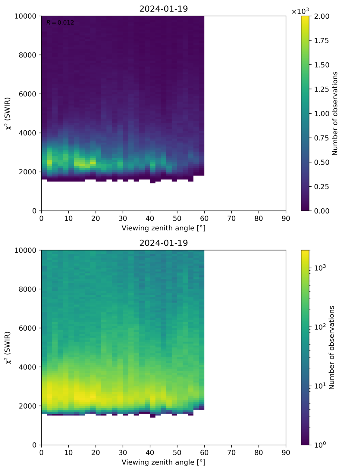
Figure 106: Scatter density plot of “Viewing zenith angle” against “ \chi^2 (SWIR)” for 2024-01-18 to 2024-01-20.
