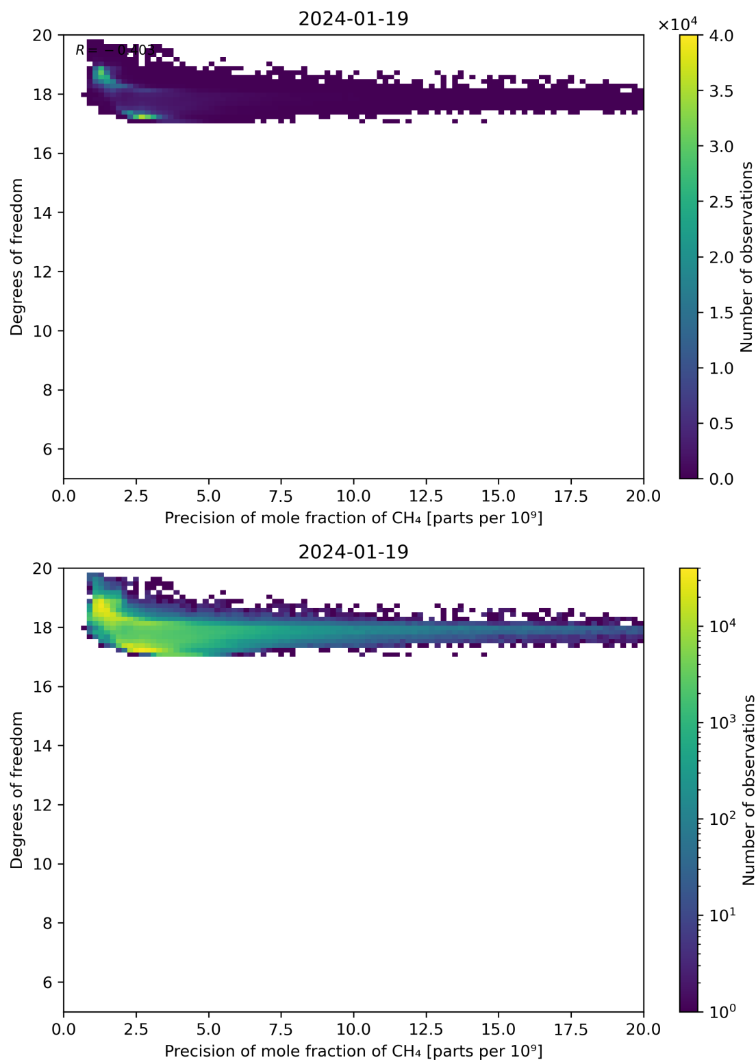
Figure 80: Scatter density plot of “Precision of mole fraction of CH 4 ” against “Degrees of freedom” for 2024-01-18 to 2024-01-20.
