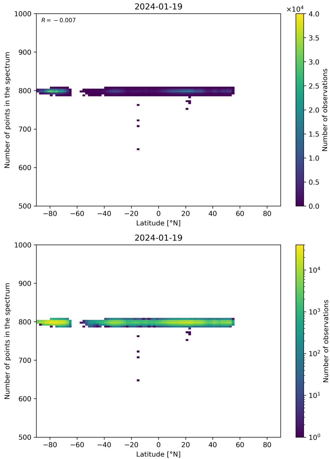
Figure 61: Scatter density plot of “Latitude” against “Number of points in the spectrum” for 2024-01-18 to 2024-01-20.
