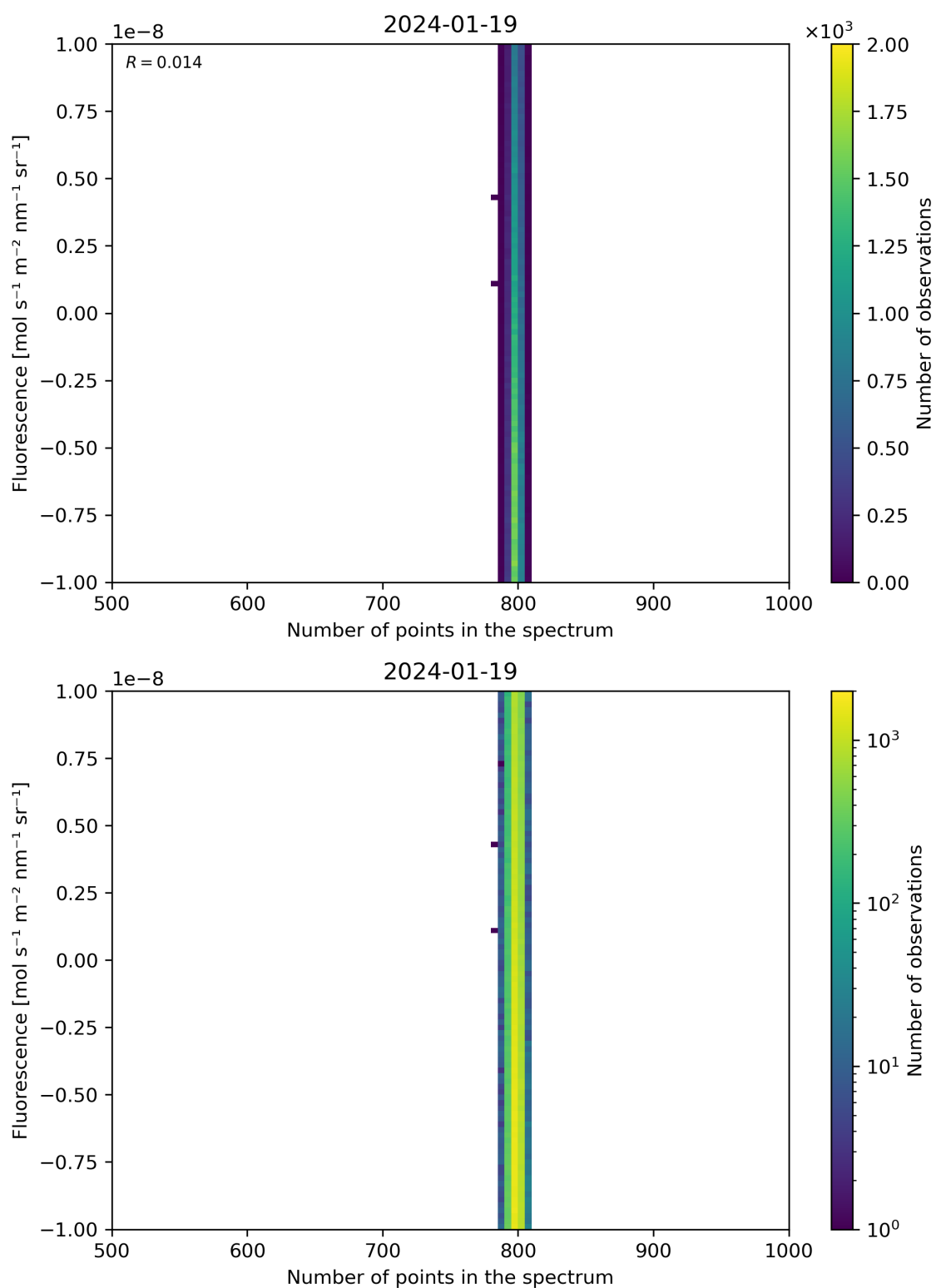
Figure 91: Scatter density plot of “Number of points in the spectrum” against “Fluorescence” for 2024-01-18 to 2024-01-20.
