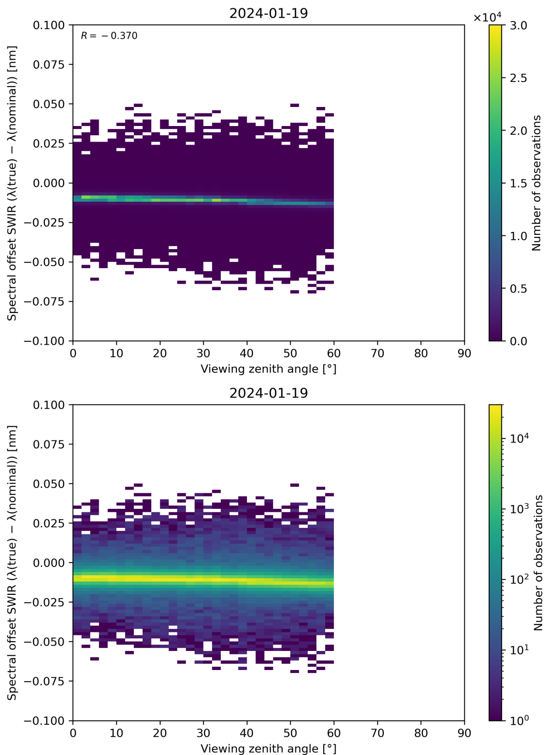
Figure 116: Scatter density plot of “Viewing zenith angle” against “Spectral offset SWIR ( \lambda(\text{true}) - \lambda(\text{nominal}) )” for 2024-01-18 to 2024-01-20.
