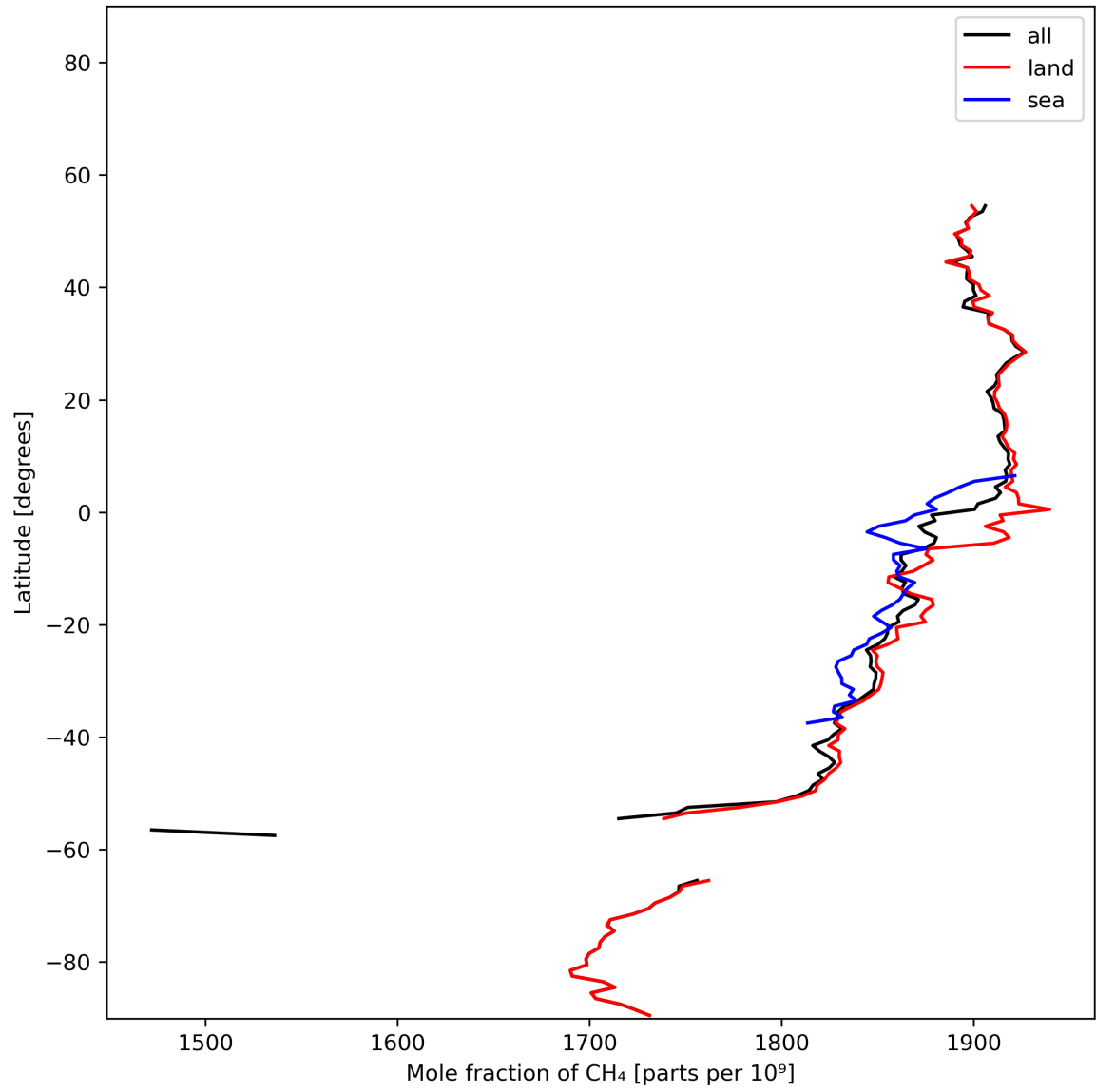
Figure 12: Zonal average of “Mole fraction of \text{CH}_4 ” for 2024-01-18 to 2024-01-20.
