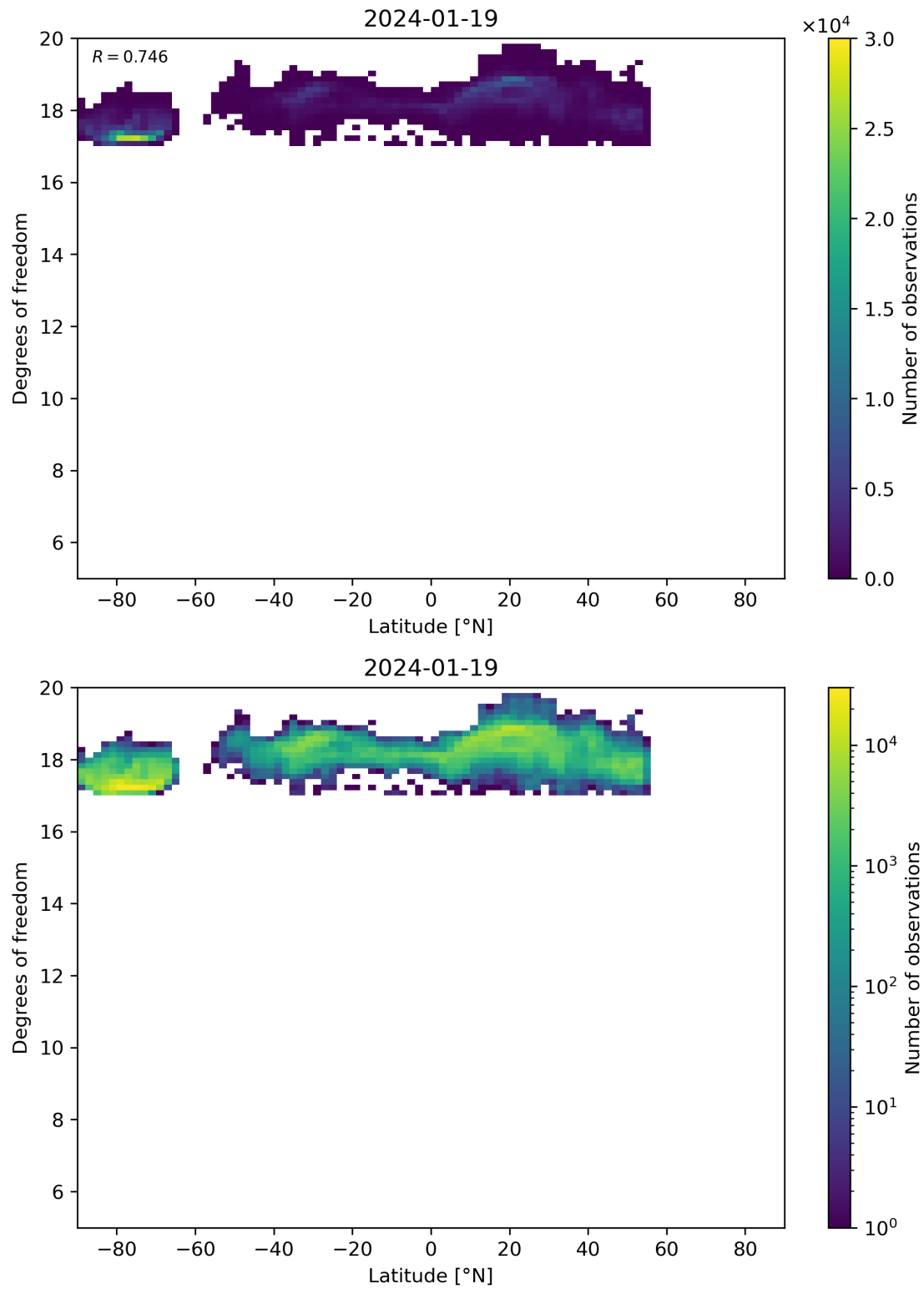
Figure 55: Scatter density plot of “Latitude” against “Degrees of freedom” for 2024-01-18 to 2024-01-20.
