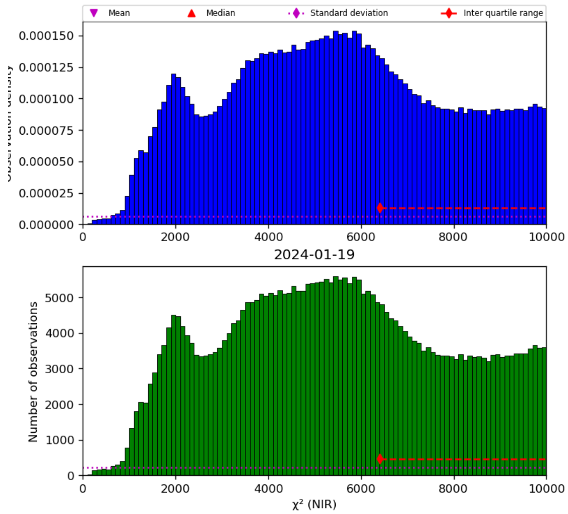
Figure 29: Histogram of “ \chi^2 (NIR)” for 2024-01-18 to 2024-01-20
