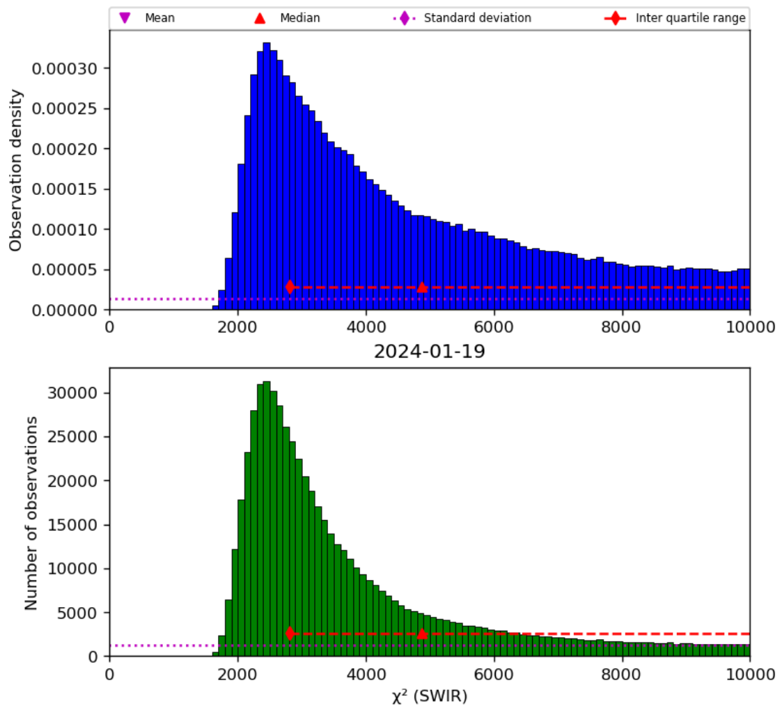
Figure 28: Histogram of “ \chi^2 (SWIR)” for 2024-01-18 to 2024-01-20
