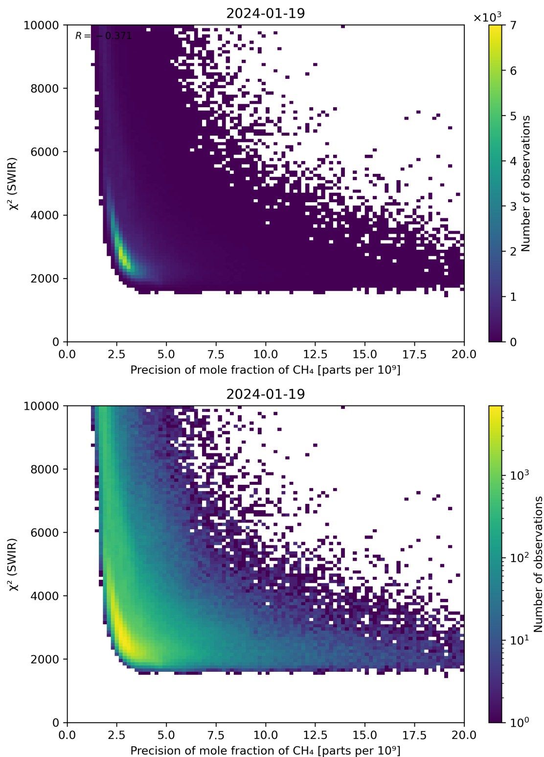
Figure 79: Scatter density plot of “Precision of mole fraction of CH 4 ” against “ \chi^2 (SWIR)” for 2024-01-18 to 2024-01-20.
