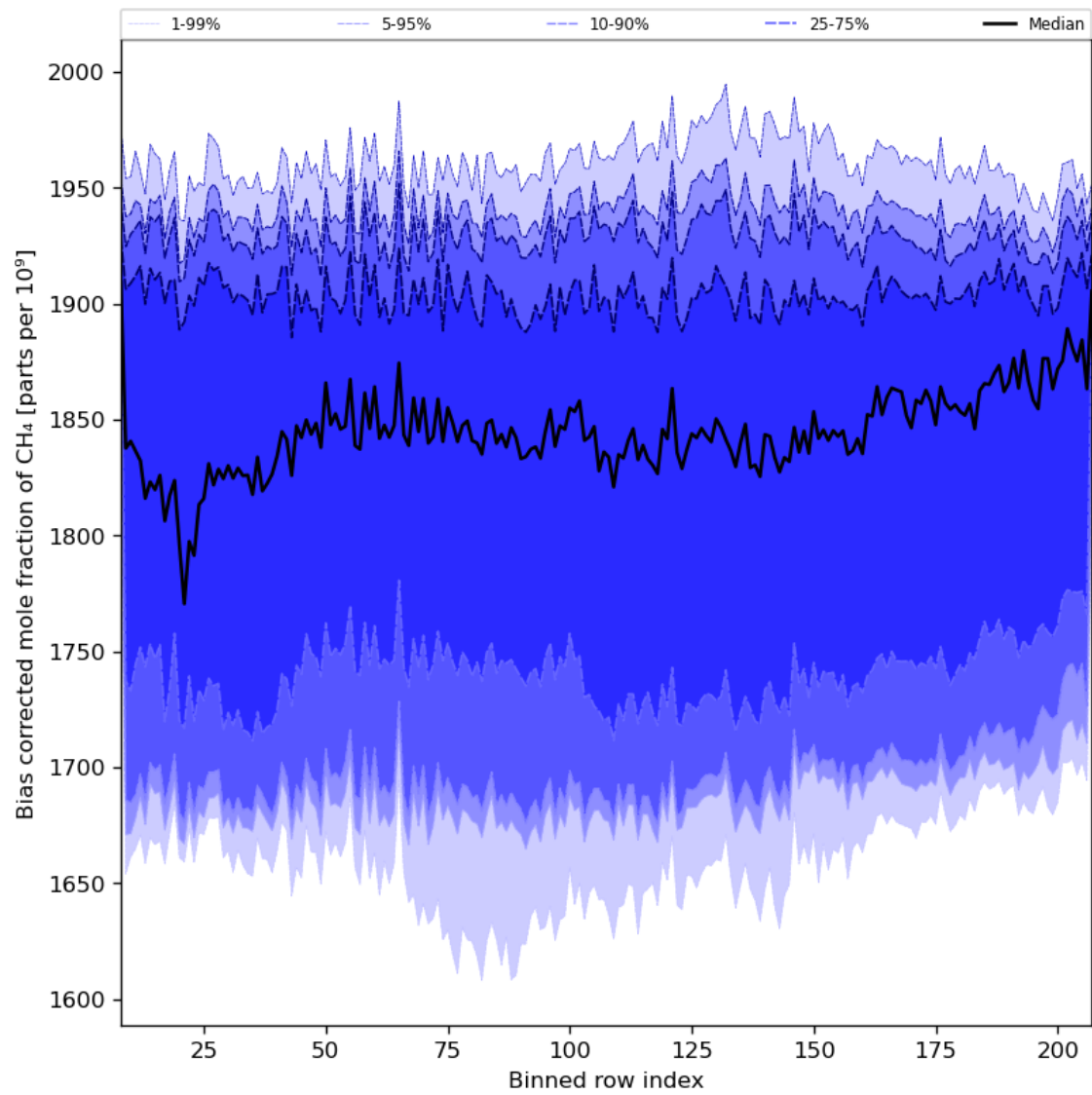
Figure 36: Along track statistics of “Bias corrected mole fraction of CH 4 ” for 2024-01-18 to 2024-01-20
