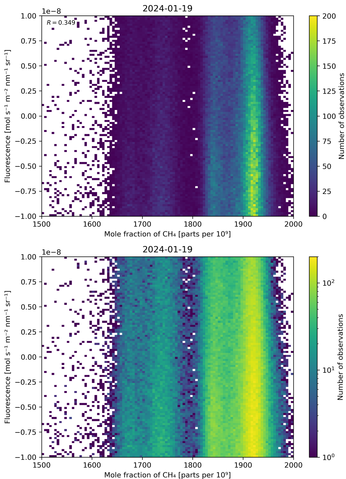
Figure 73: Scatter density plot of “Mole fraction of \text{CH}_4 ” against “Fluorescence” for 2024-01-18 to 2024-01-20.
