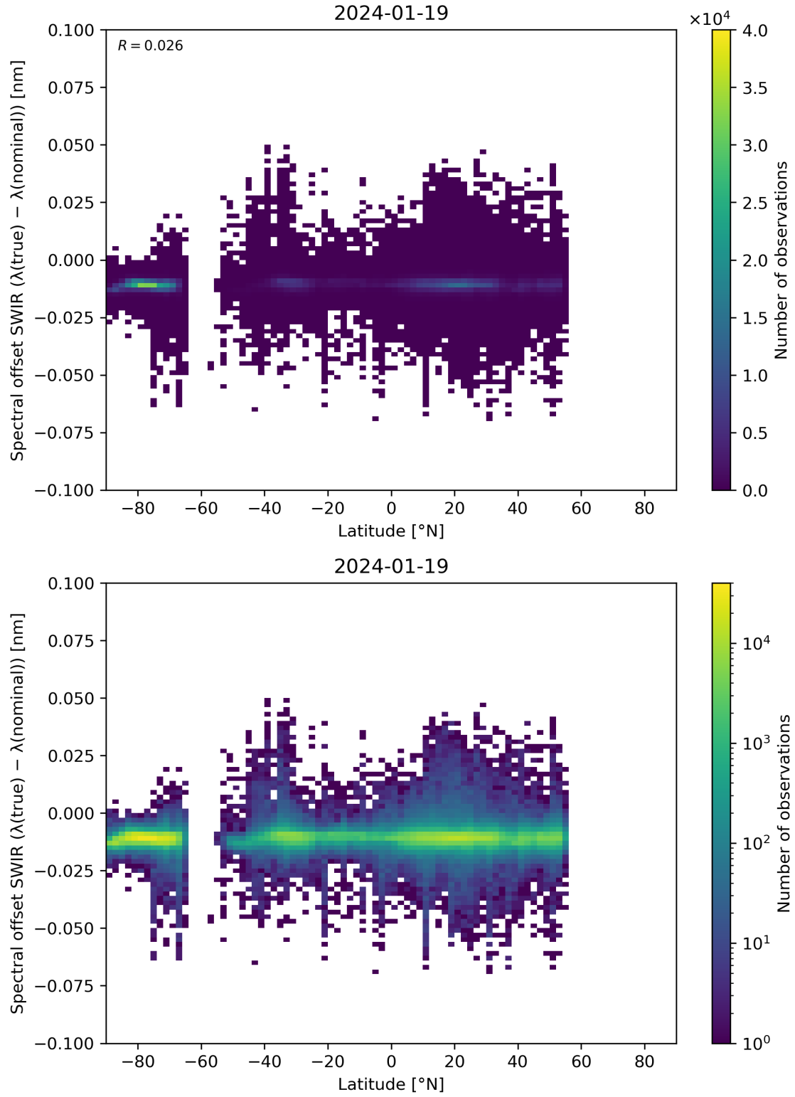
Figure 62: Scatter density plot of “Latitude” against “Spectral offset SWIR ( \lambda(\text{true}) - \lambda(\text{nominal}) )” for 2024-01-18 to 2024-01-20.
