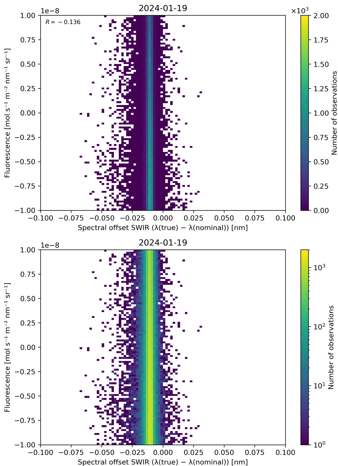
Figure 120: Scatter density plot of “Spectral offset SWIR ( \lambda(\text{true}) - \lambda(\text{nominal}) )” against “Fluorescence” for 2024-01-18 to 2024-01-20.
