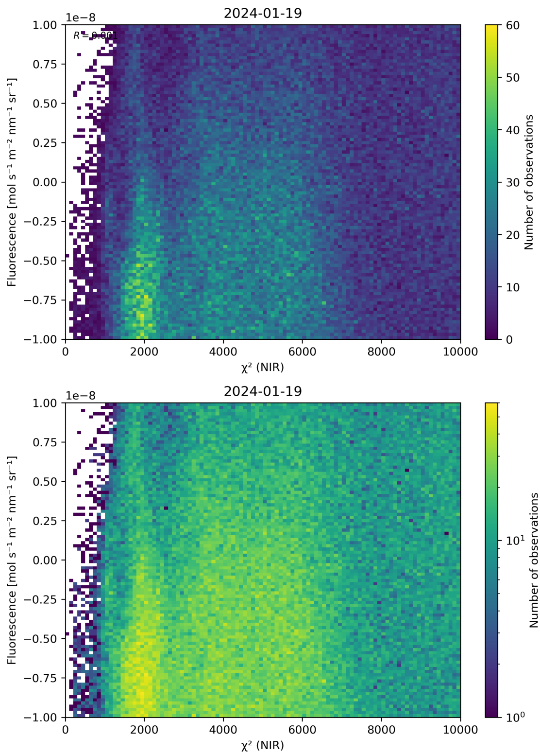
Figure 45: Scatter density plot of “ \chi^2 (NIR)” against “Fluorescence” for 2024-01-18 to 2024-01-20.
