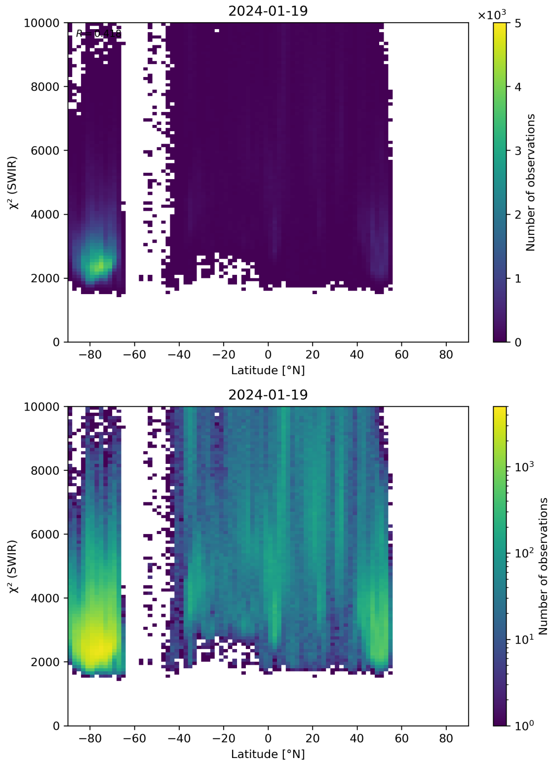
Figure 54: Scatter density plot of “Latitude” against “ \chi^2 (SWIR)” for 2024-01-18 to 2024-01-20.
