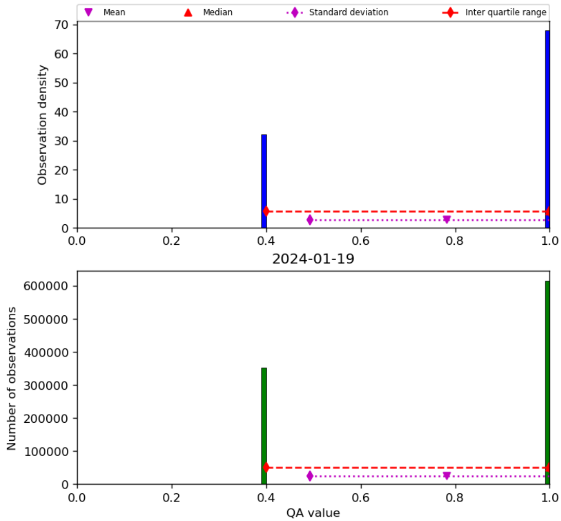
Figure 22: Histogram of “QA value” for 2024-01-18 to 2024-01-20
