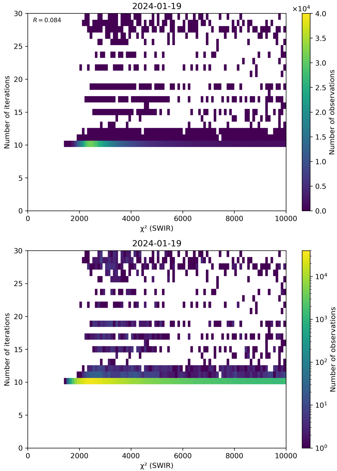
Figure 50: Scatter density plot of “ \chi^2 (SWIR)” against “Number of iterations” for 2024-01-18 to 2024-01-20.
