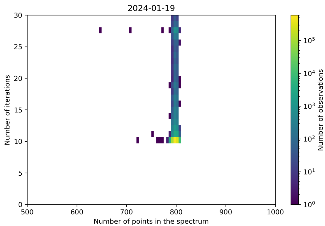
Figure 92: Scatter density plot of “Number of points in the spectrum” against “Number of iterations” for 2024-01-18 to 2024-01-20.
