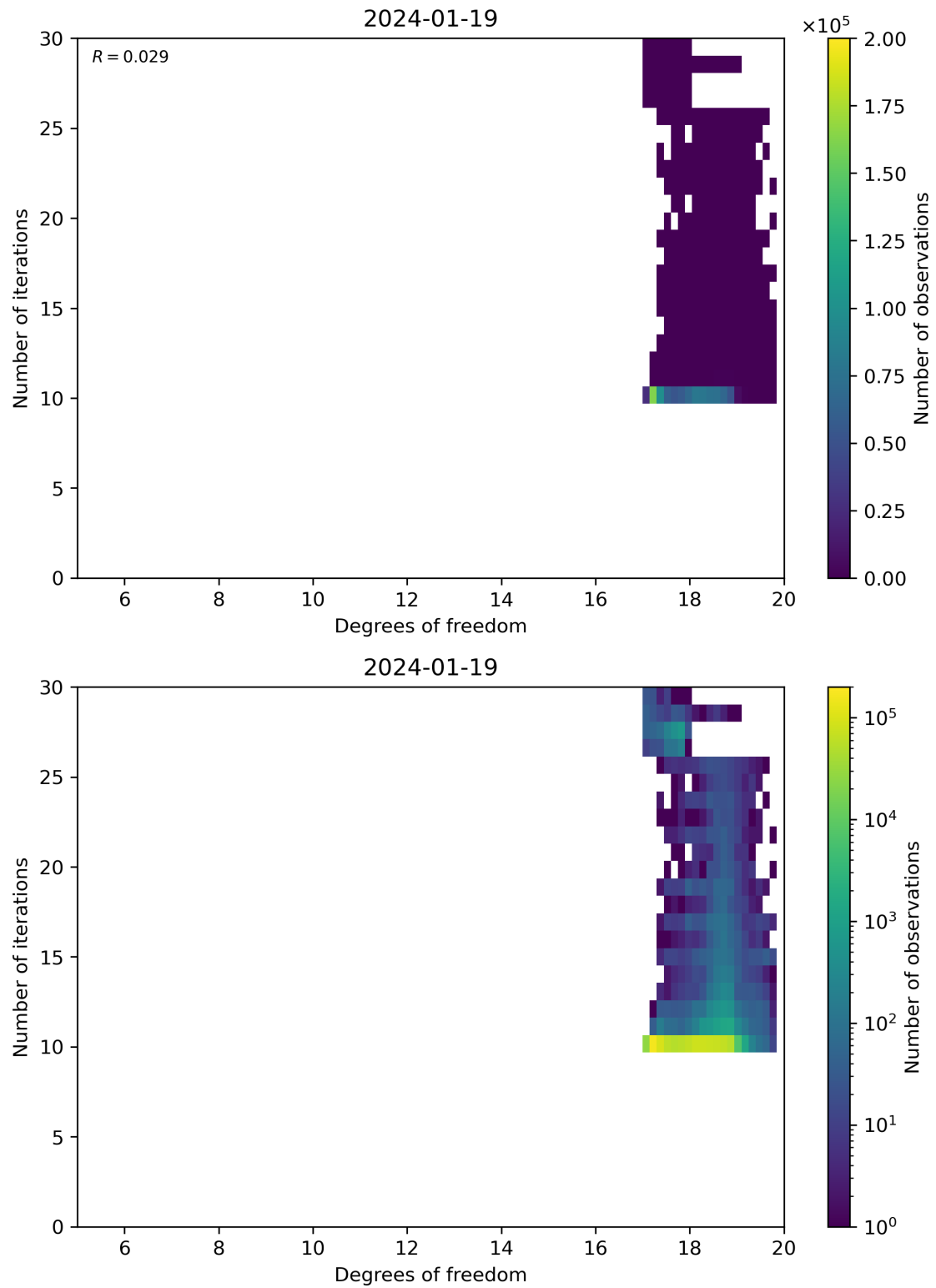
Figure 52: Scatter density plot of “Degrees of freedom” against “Number of iterations” for 2024-01-18 to 2024-01-20.
