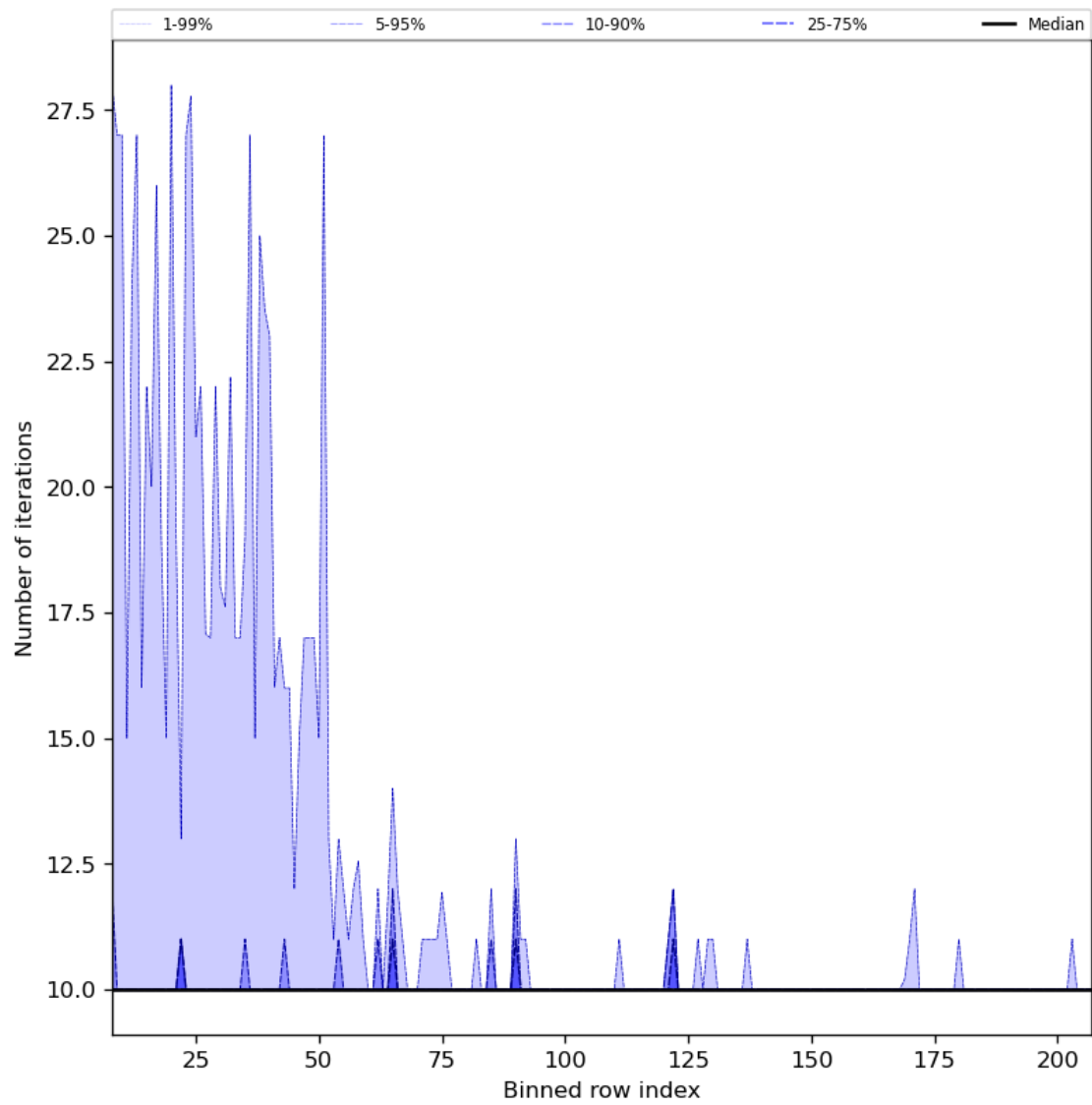
Figure 42: Along track statistics of “Number of iterations” for 2024-01-18 to 2024-01-20
