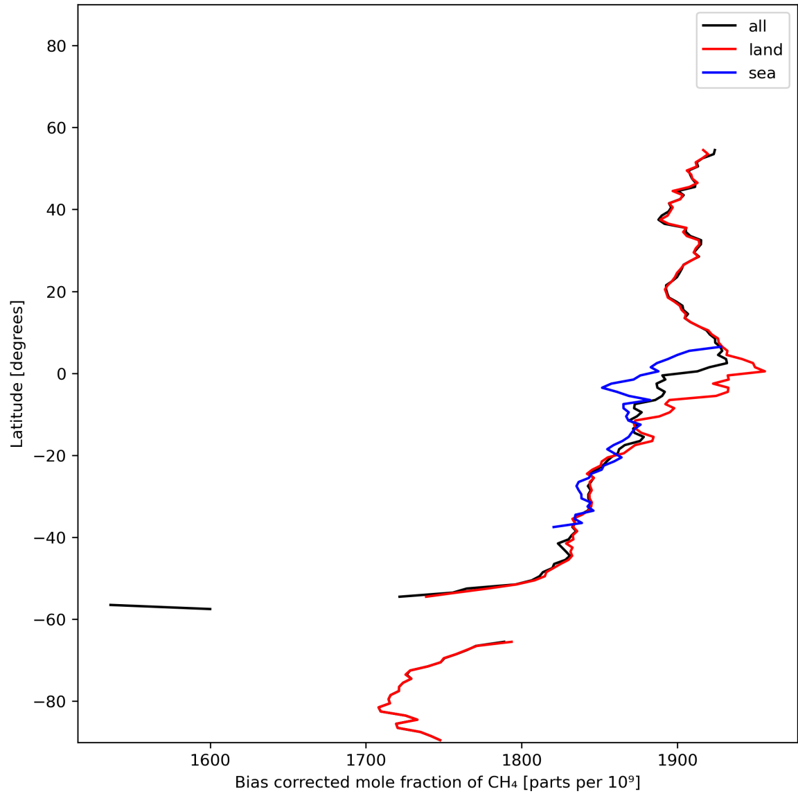
Figure 14: Zonal average of “Bias corrected mole fraction of CH 4 ” for 2024-01-18 to 2024-01-20.
