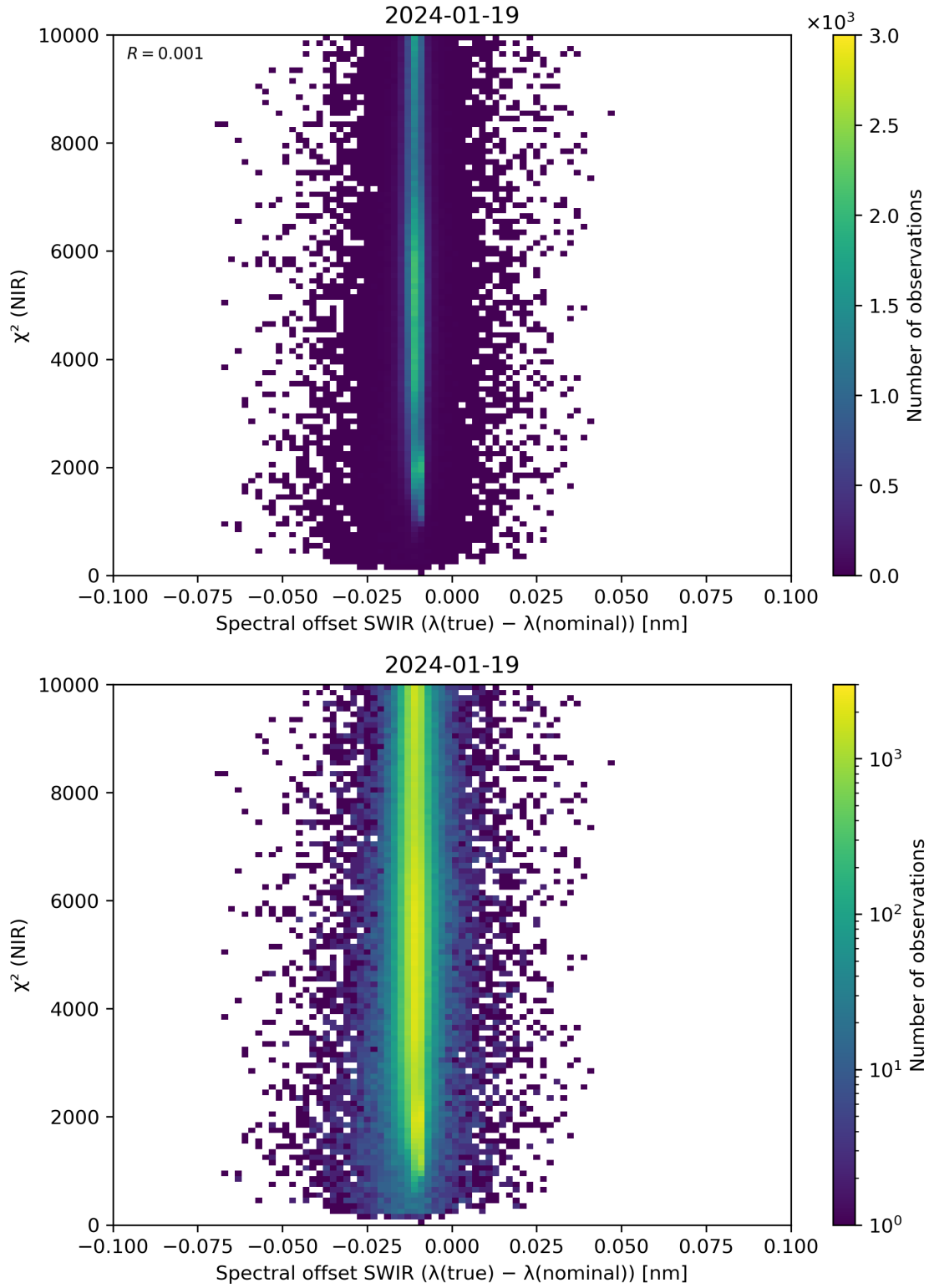
Figure 117: Scatter density plot of “Spectral offset SWIR ( \lambda(\text{true}) - \lambda(\text{nominal}) )” against “ \chi^2 (NIR)” for 2024-01-18 to 2024-01-20.
