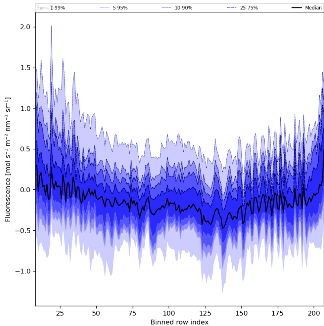
Figure 43: Along track statistics of “Fluorescence” for 2024-01-18 to 2024-01-20
