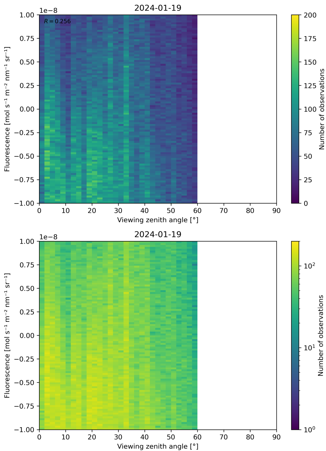
Figure 108: Scatter density plot of “Viewing zenith angle” against “Fluorescence” for 2024-01-18 to 2024-01-20.
