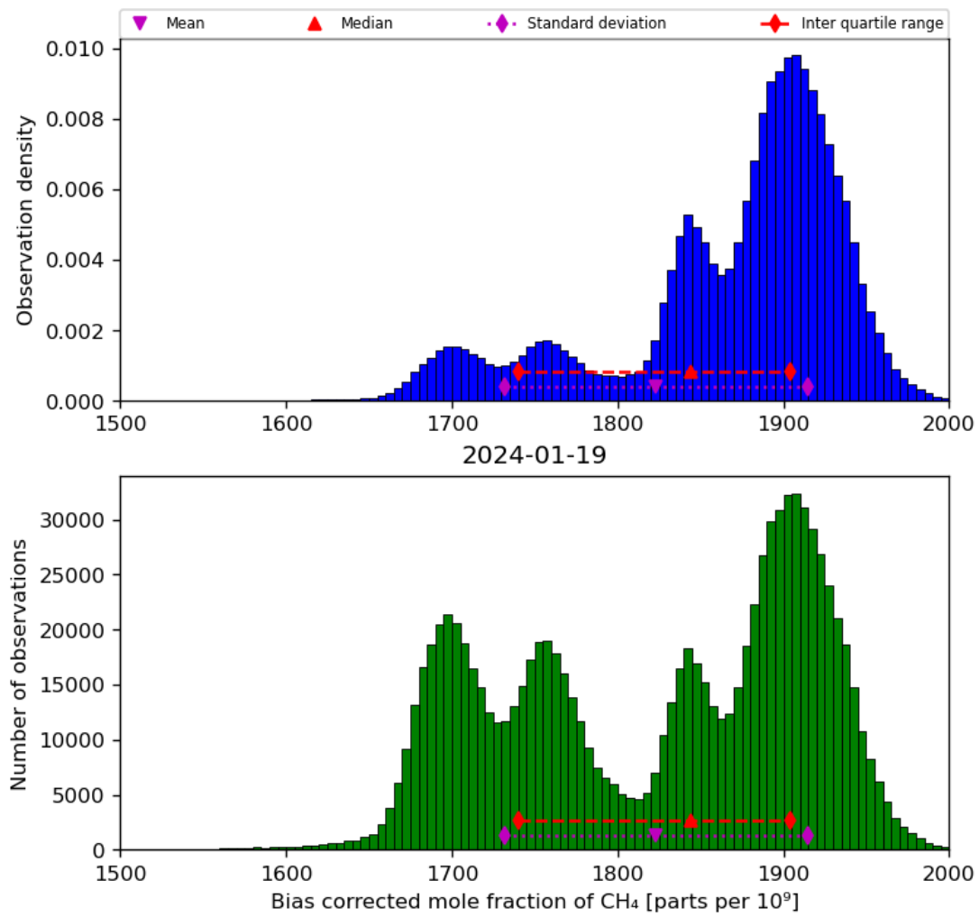
Figure 25: Histogram of “Bias corrected mole fraction of CH 4 ” for 2024-01-18 to 2024-01-20
