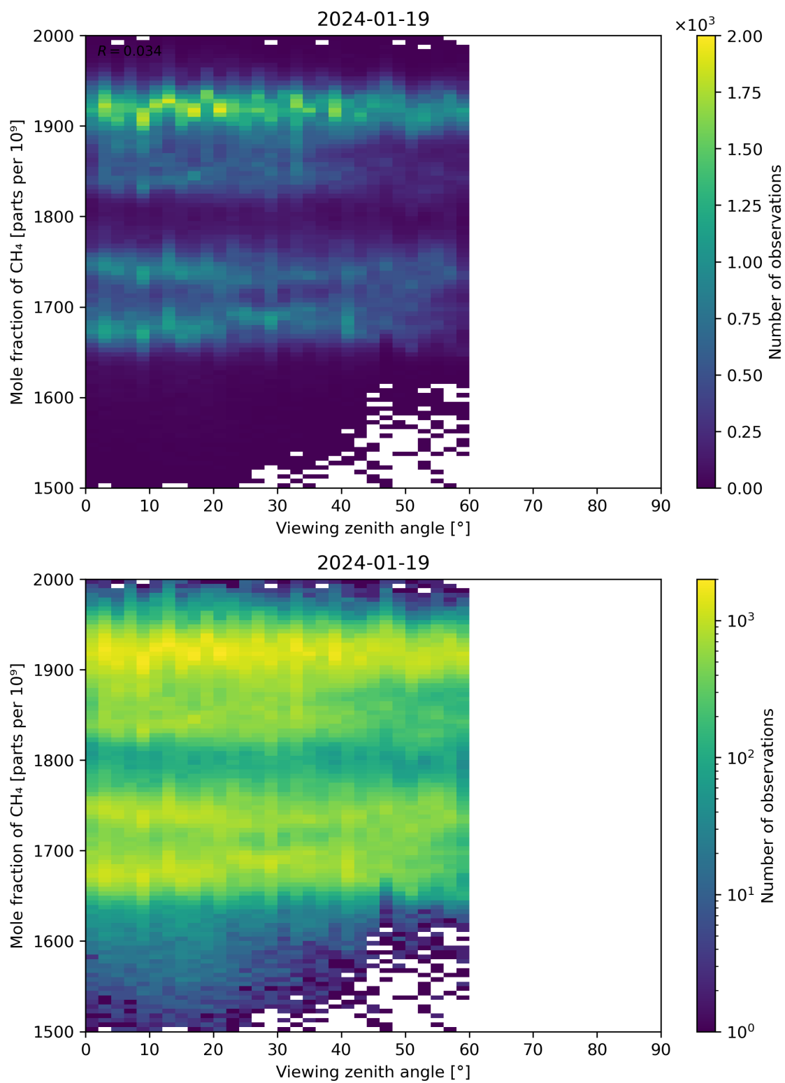
Figure 110: Scatter density plot of “Viewing zenith angle” against “Mole fraction of CH 4 ” for 2024-01-18 to 2024-01-20.
