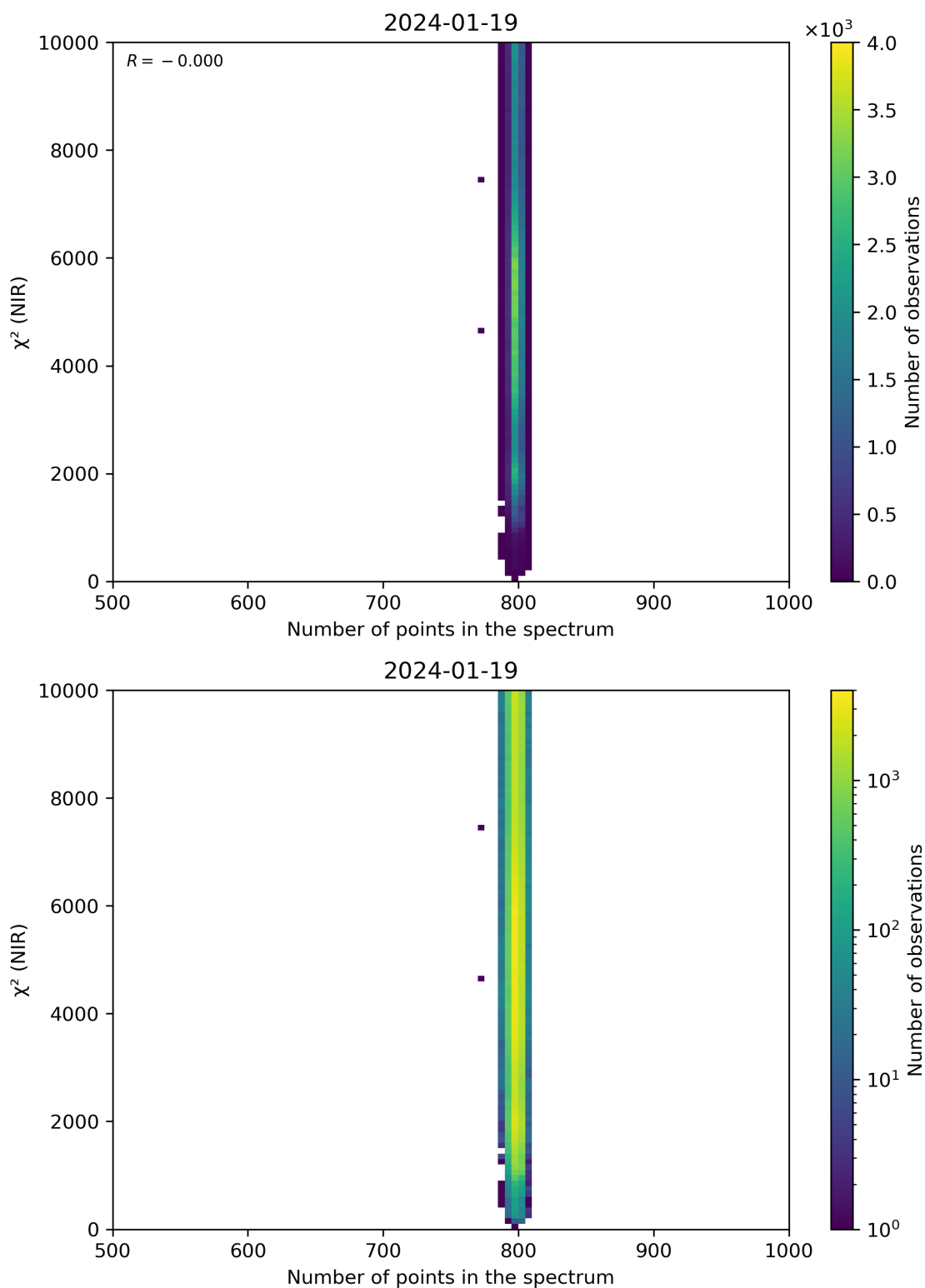
Figure 88: Scatter density plot of “Number of points in the spectrum” against “ \chi^2 (NIR)” for 2024-01-18 to 2024-01-20.
