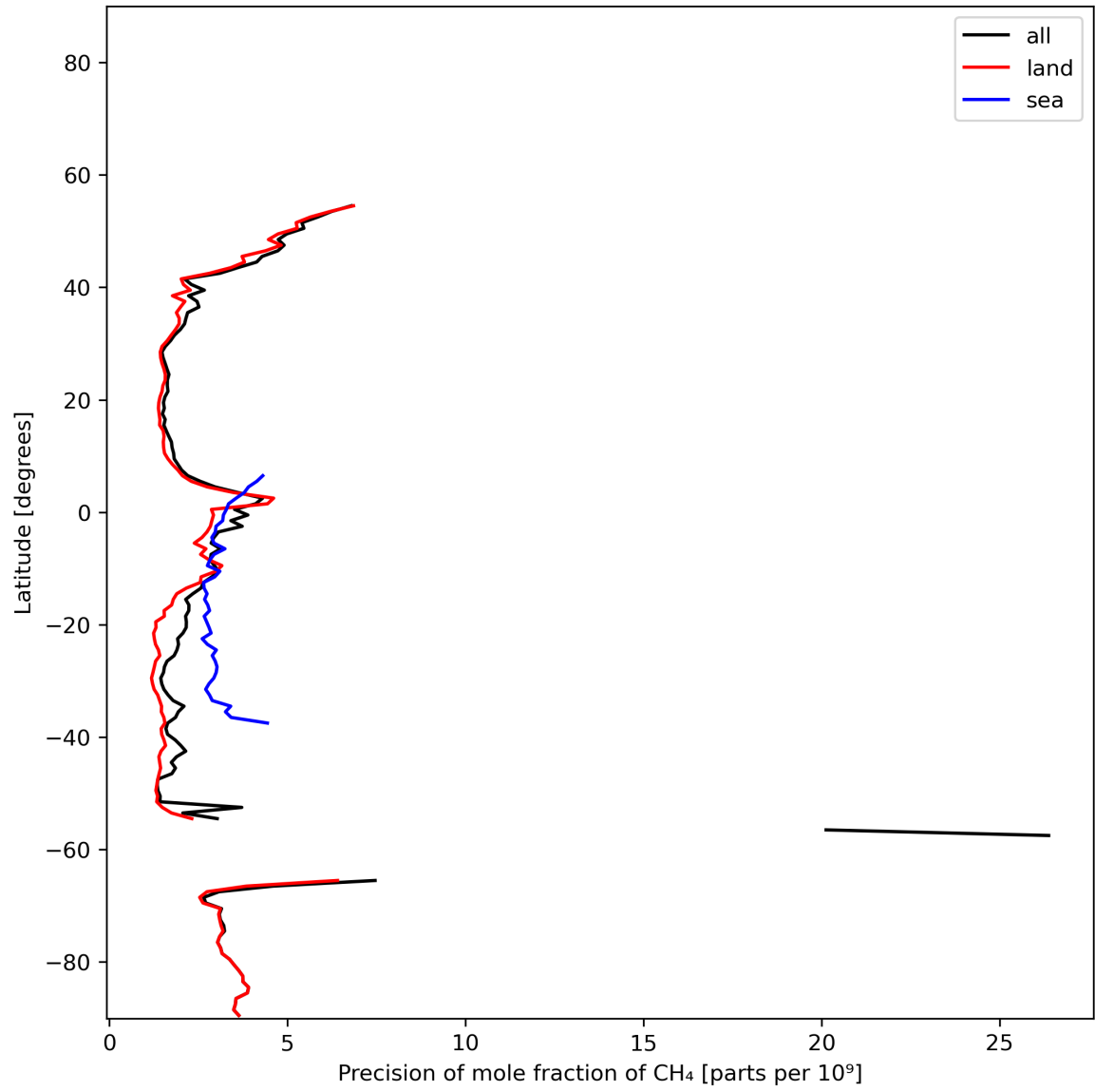
Figure 13: Zonal average of “Precision of mole fraction of CH 4 ” for 2024-01-18 to 2024-01-20.
