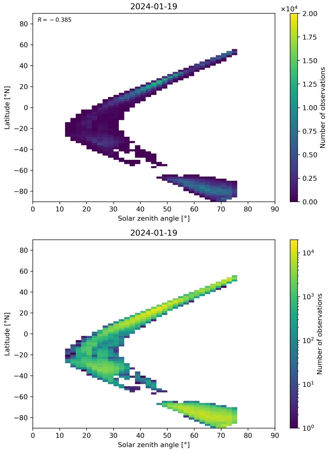
Figure 98: Scatter density plot of “Solar zenith angle” against “Latitude” for 2024-01-18 to 2024-01-20.
