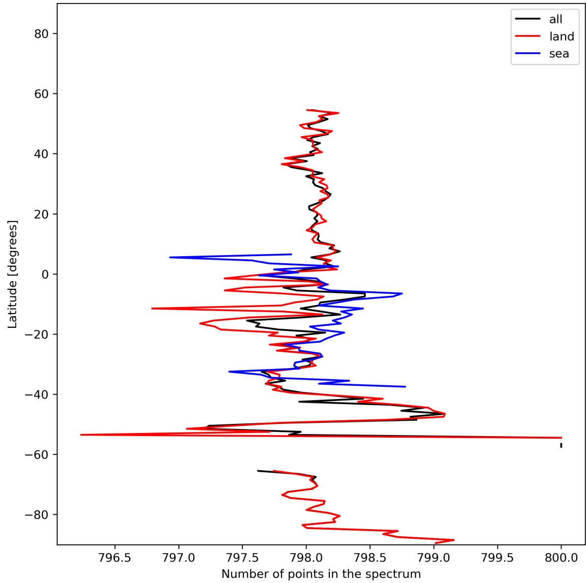
Figure 15: Zonal average of “Number of points in the spectrum” for 2024-01-18 to 2024-01-20.
