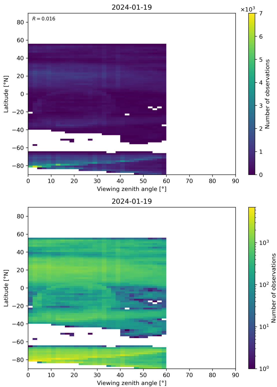
Figure 109: Scatter density plot of “Viewing zenith angle” against “Latitude” for 2024-01-18 to 2024-01-20.
