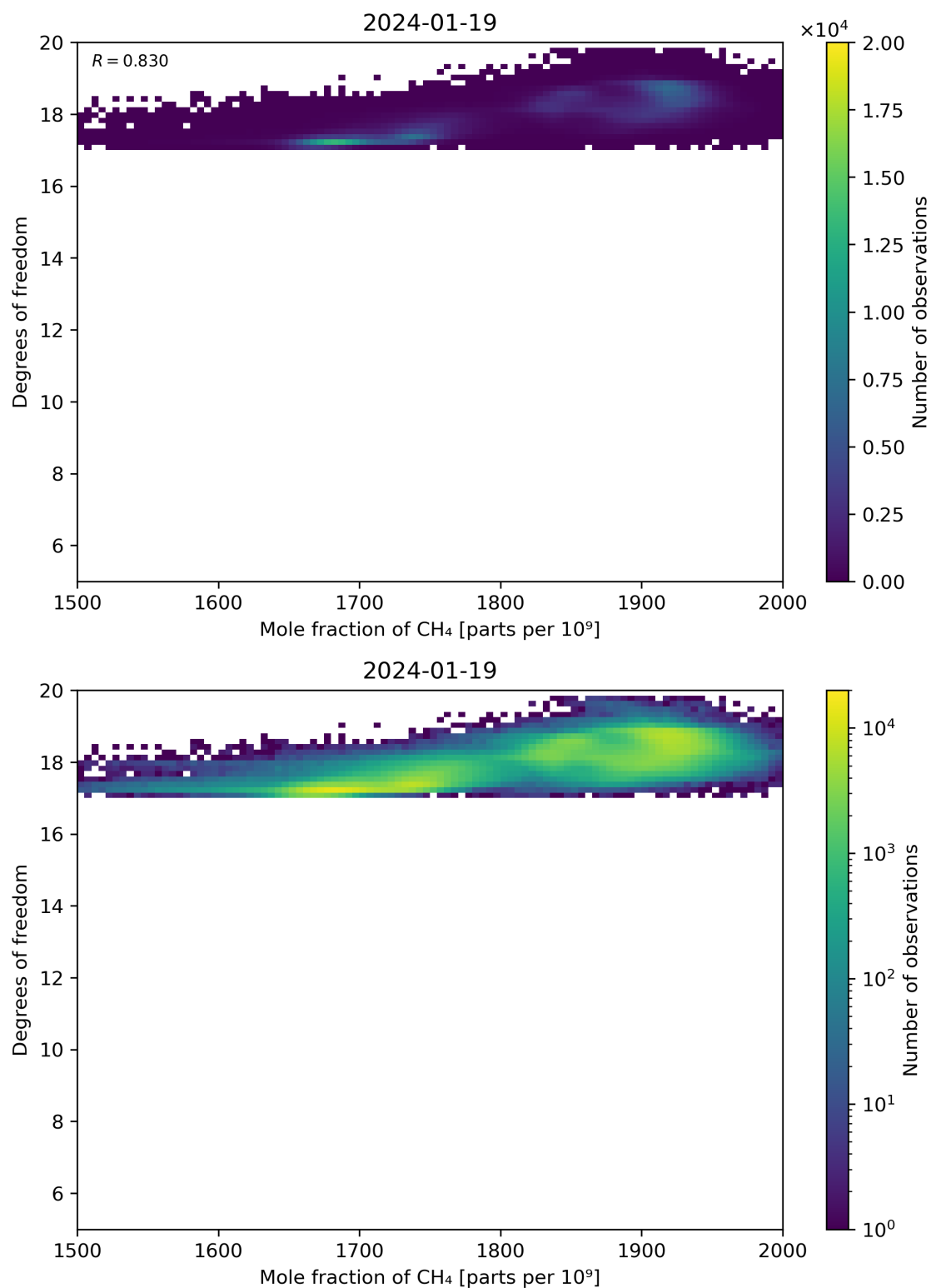
Figure 72: Scatter density plot of “Mole fraction of CH 4 ” against “Degrees of freedom” for 2024-01-18 to 2024-01-20.
