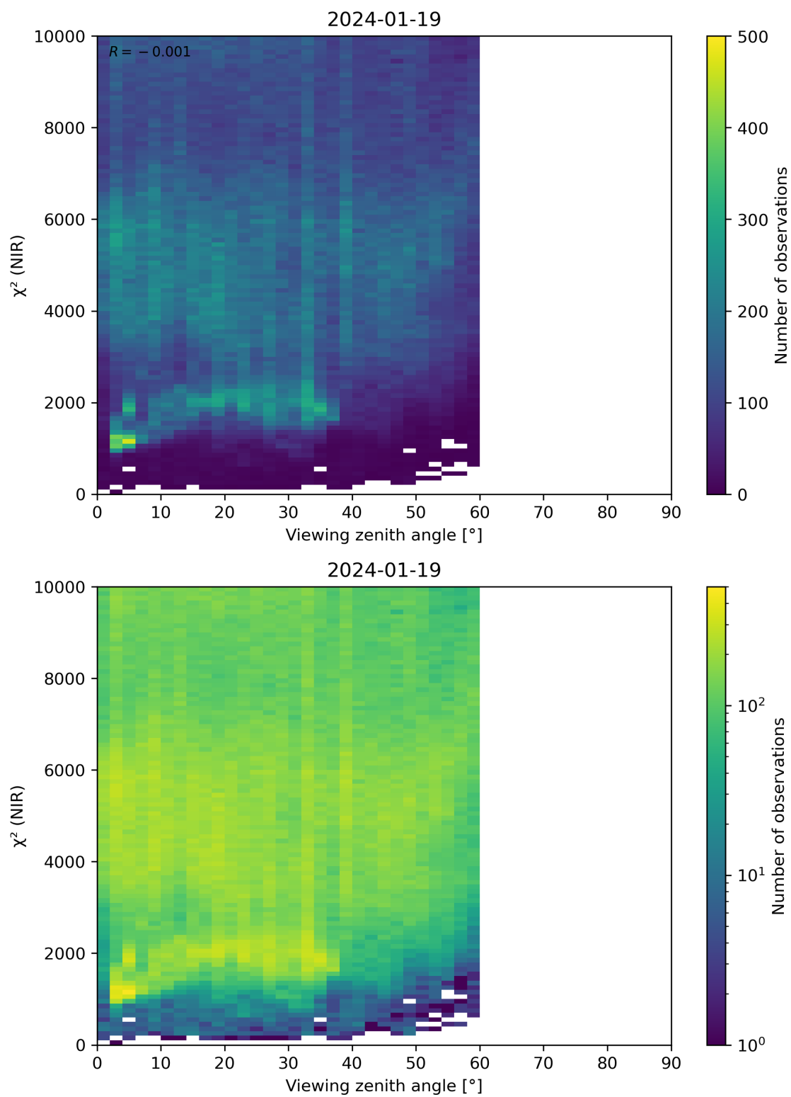
Figure 105: Scatter density plot of “Viewing zenith angle” against “ \chi^2 (NIR)” for 2024-01-18 to 2024-01-20.
