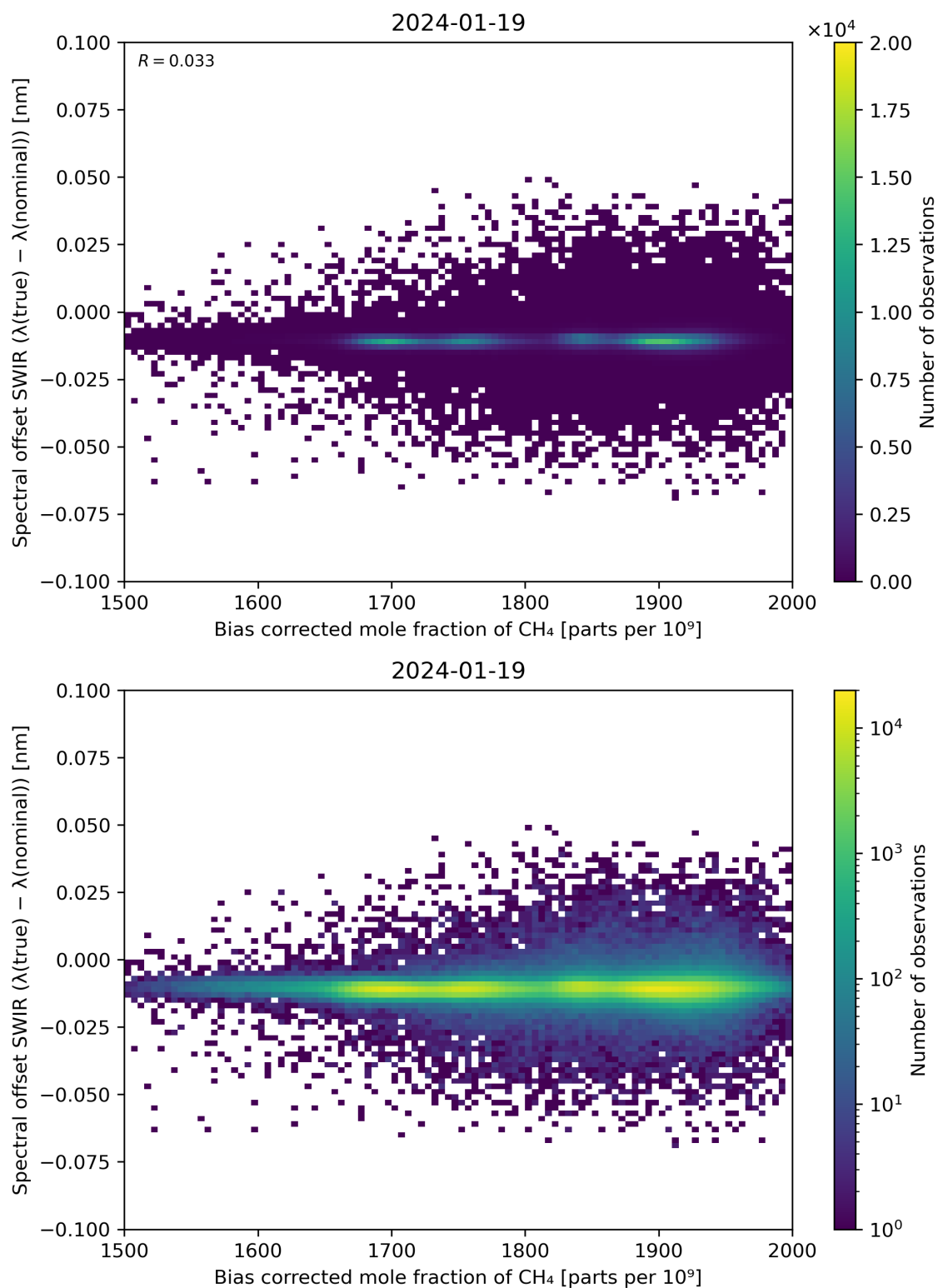
Figure 69: Scatter density plot of “Bias corrected mole fraction of \text{CH}_4 ” against “Spectral offset SWIR ( \lambda(\text{true}) - \lambda(\text{nominal}) )” for 2024-01-18 to 2024-01-20.
