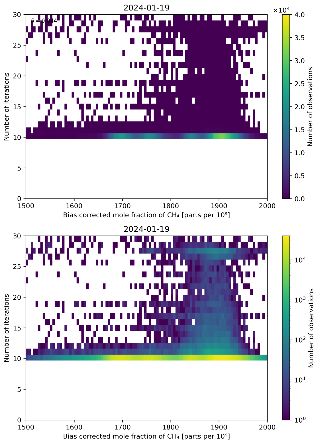
Figure 67: Scatter density plot of “Bias corrected mole fraction of \text{CH}_4 ” against “Number of iterations” for 2024-01-18 to 2024-01-20.
