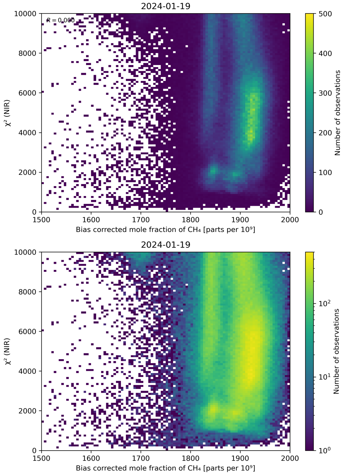
Figure 63: Scatter density plot of “Bias corrected mole fraction of \text{CH}_4 ” against “ \chi^2 (NIR)” for 2024-01-18 to 2024-01-20.
