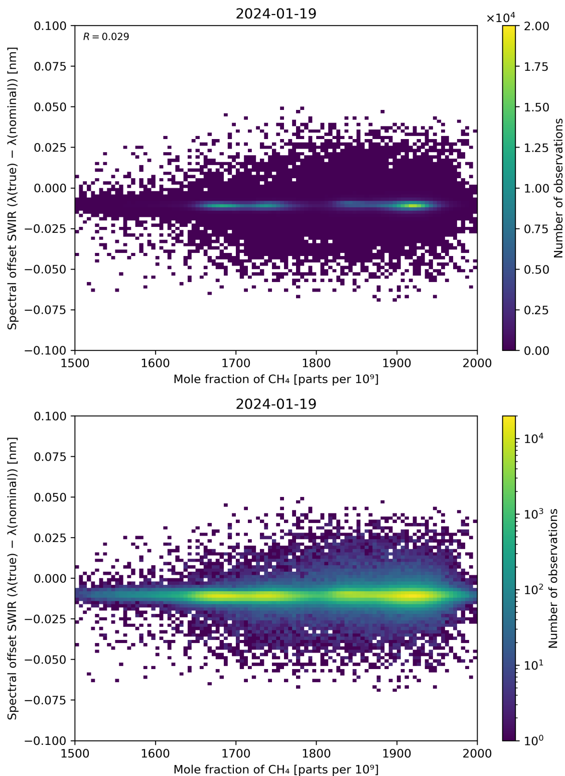
Figure 86: Scatter density plot of “Mole fraction of CH 4 ” against “Spectral offset SWIR ( \lambda(\text{true}) - \lambda(\text{nominal}) )” for 2024-01-18 to 2024-01-20.
