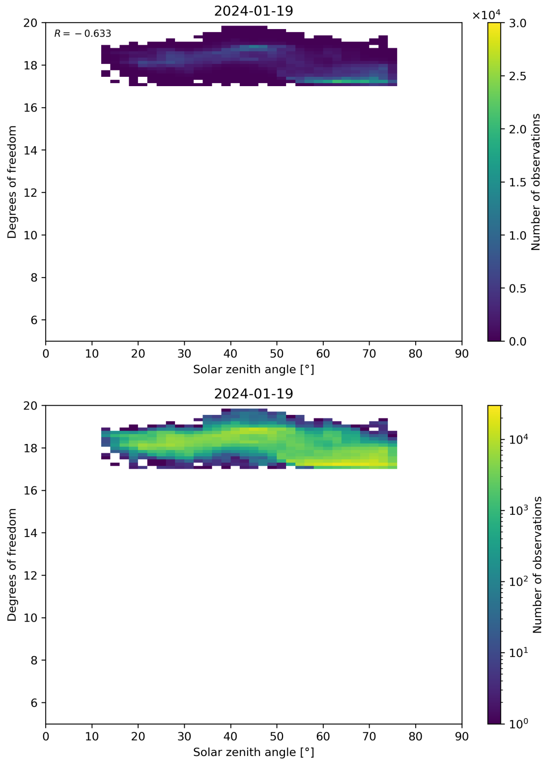
Figure 96: Scatter density plot of “Solar zenith angle” against “Degrees of freedom” for 2024-01-18 to 2024-01-20.
