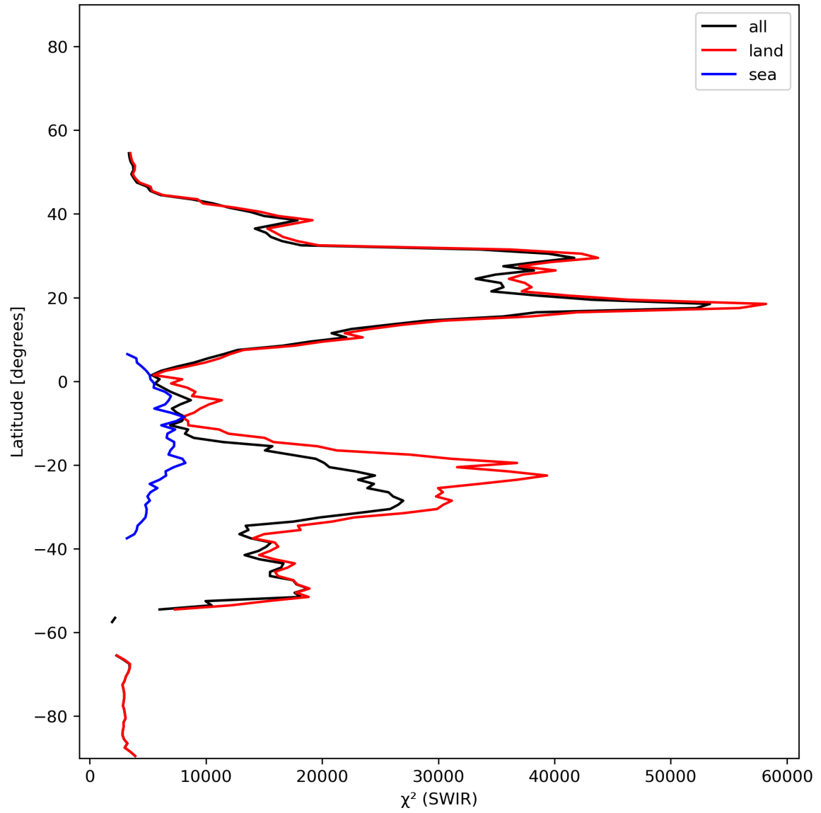
Figure 17: Zonal average of “ \chi^2 (SWIR)” for 2024-01-18 to 2024-01-20.
