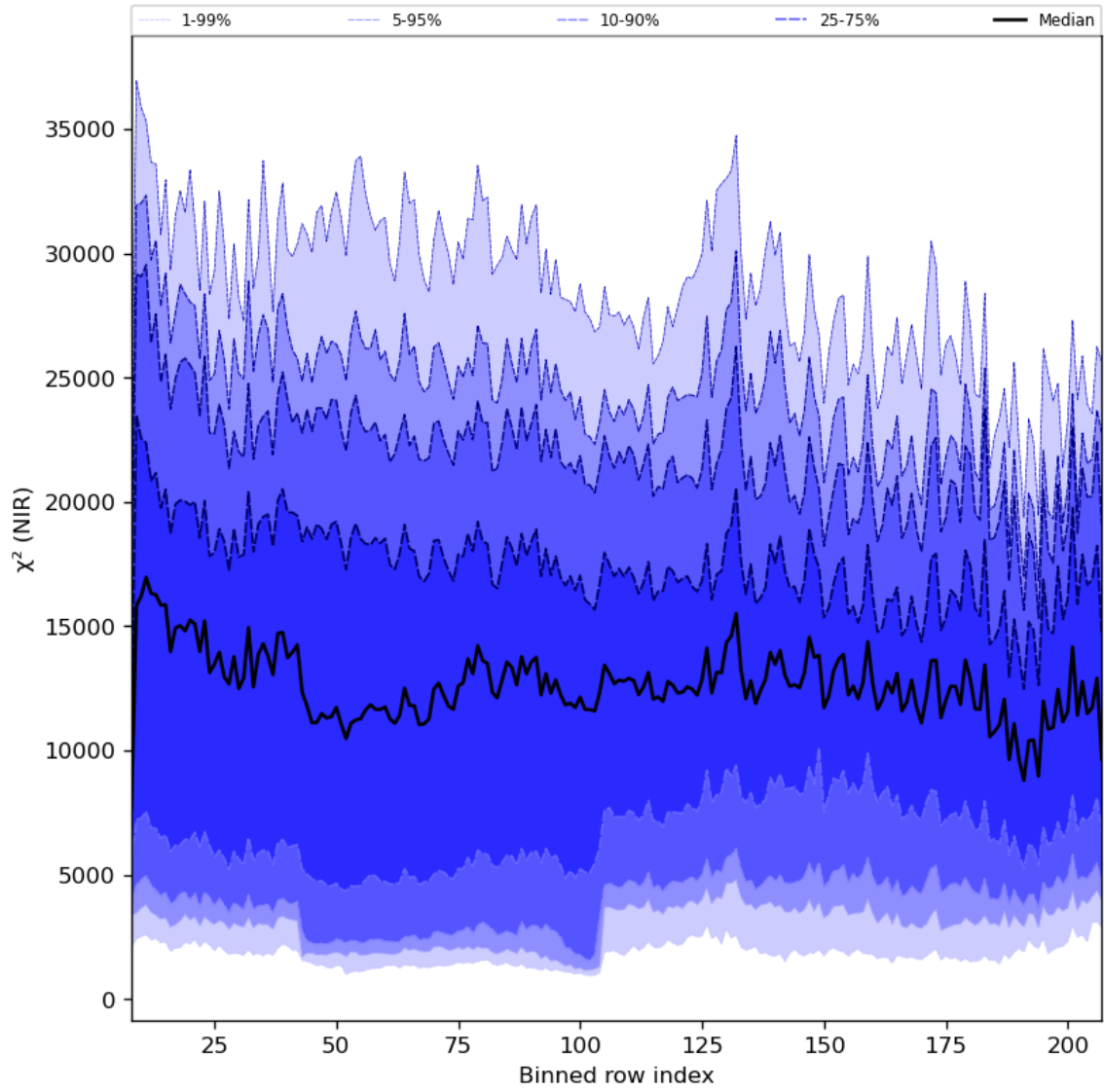
Figure 40: Along track statistics of “ \chi^2 (NIR)” for 2024-01-18 to 2024-01-20
