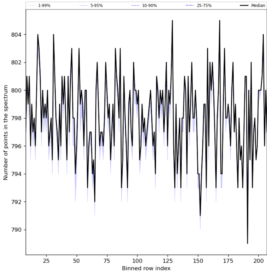
Figure 37: Along track statistics of “Number of points in the spectrum” for 2024-01-18 to 2024-01-20
