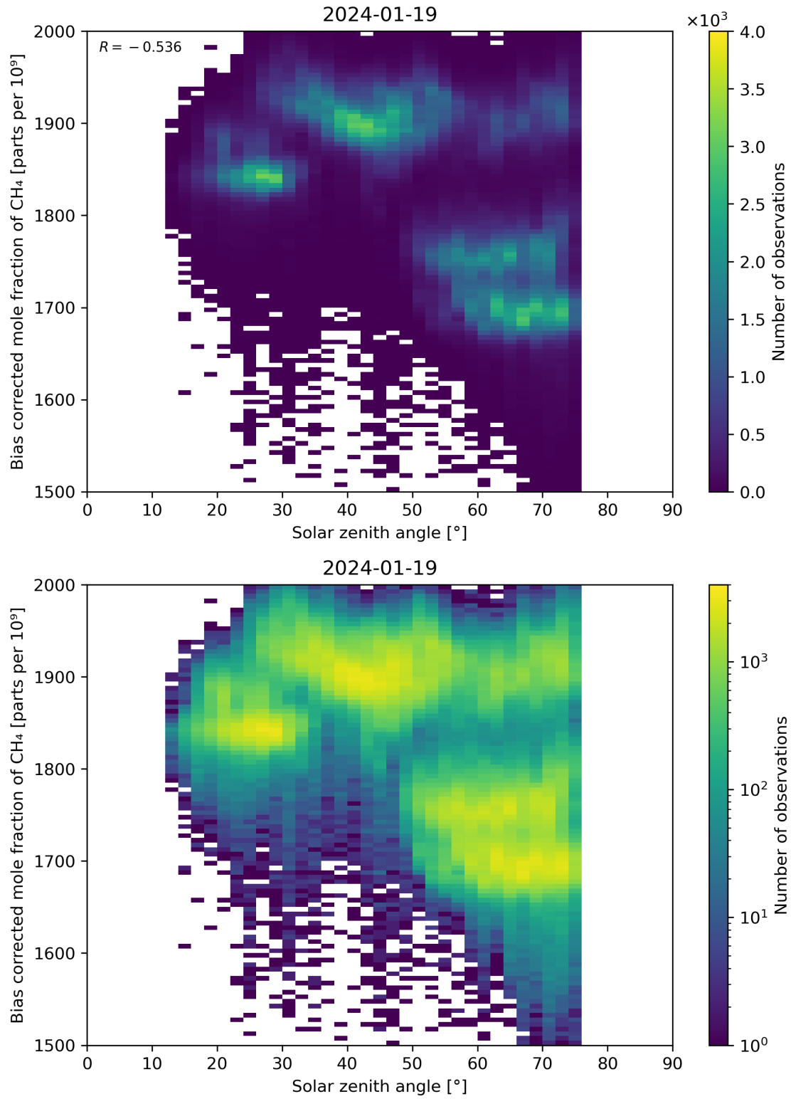
Figure 100: Scatter density plot of “Solar zenith angle” against “Bias corrected mole fraction of CH 4 ” for 2024-01-18 to 2024-01-20.
