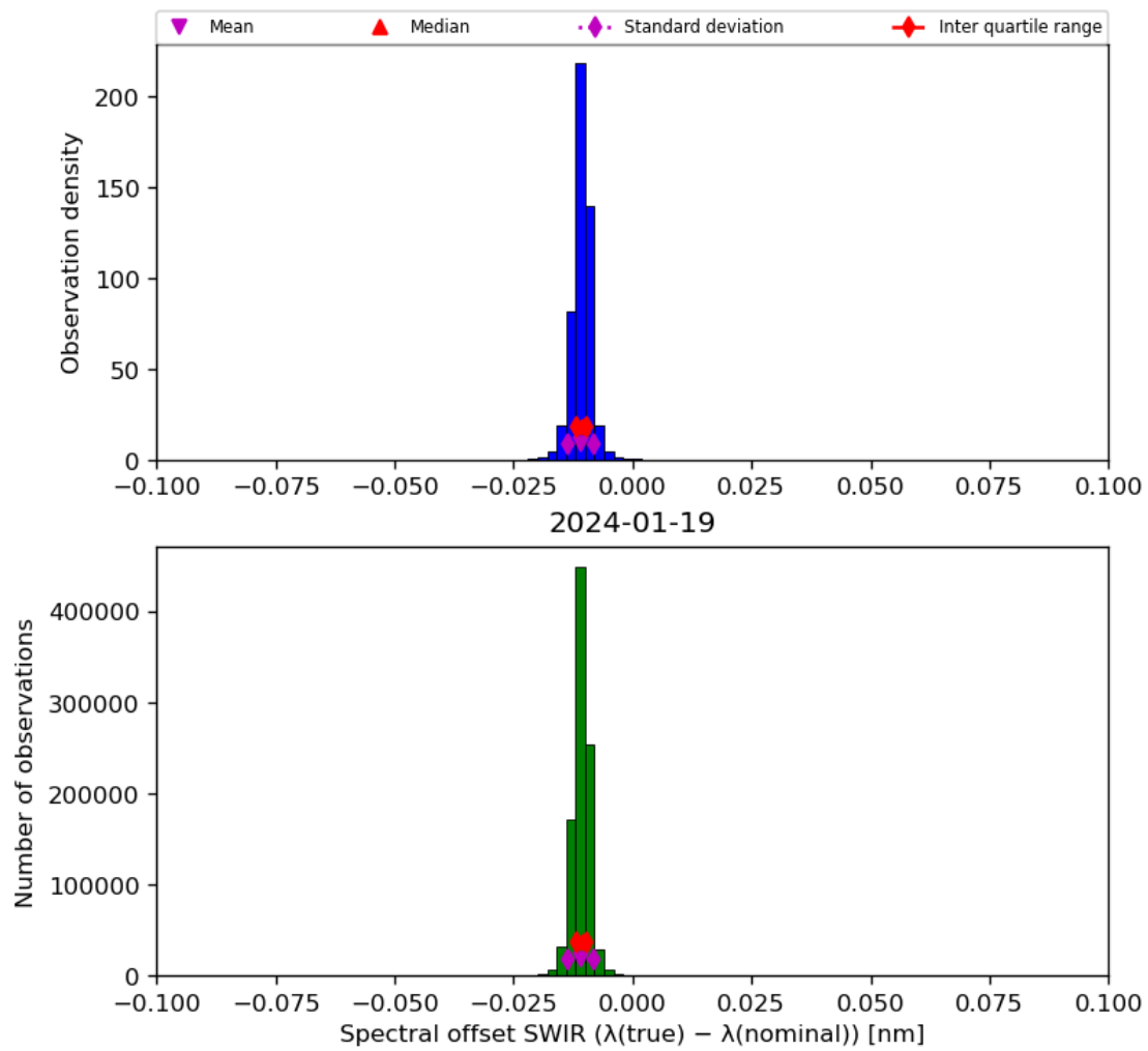
Figure 27: Histogram of “Spectral offset SWIR ( \lambda(\text{true}) - \lambda(\text{nominal}) )” for 2024-01-18 to 2024-01-20
