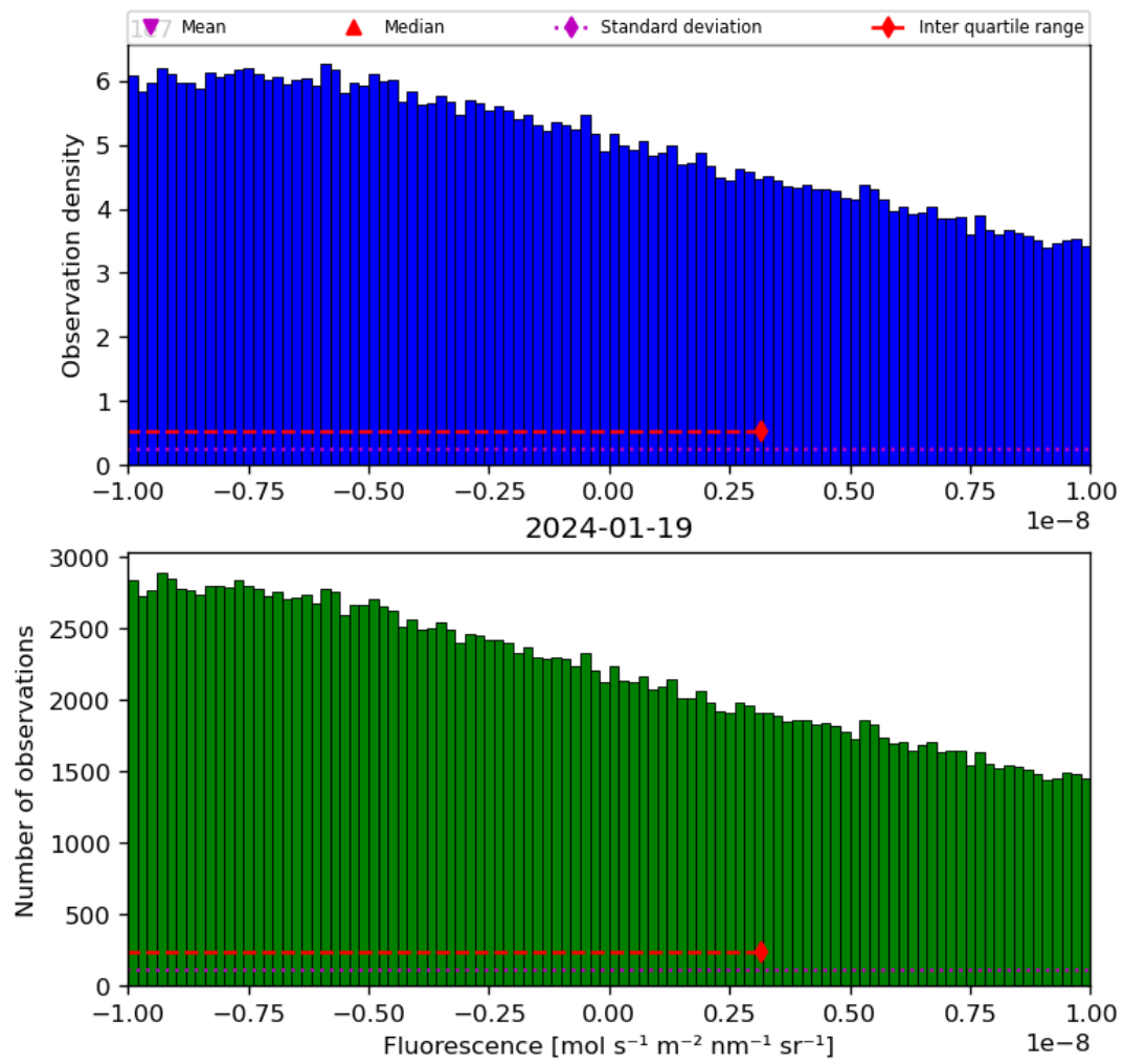
Figure 32: Histogram of “Fluorescence” for 2024-01-18 to 2024-01-20
