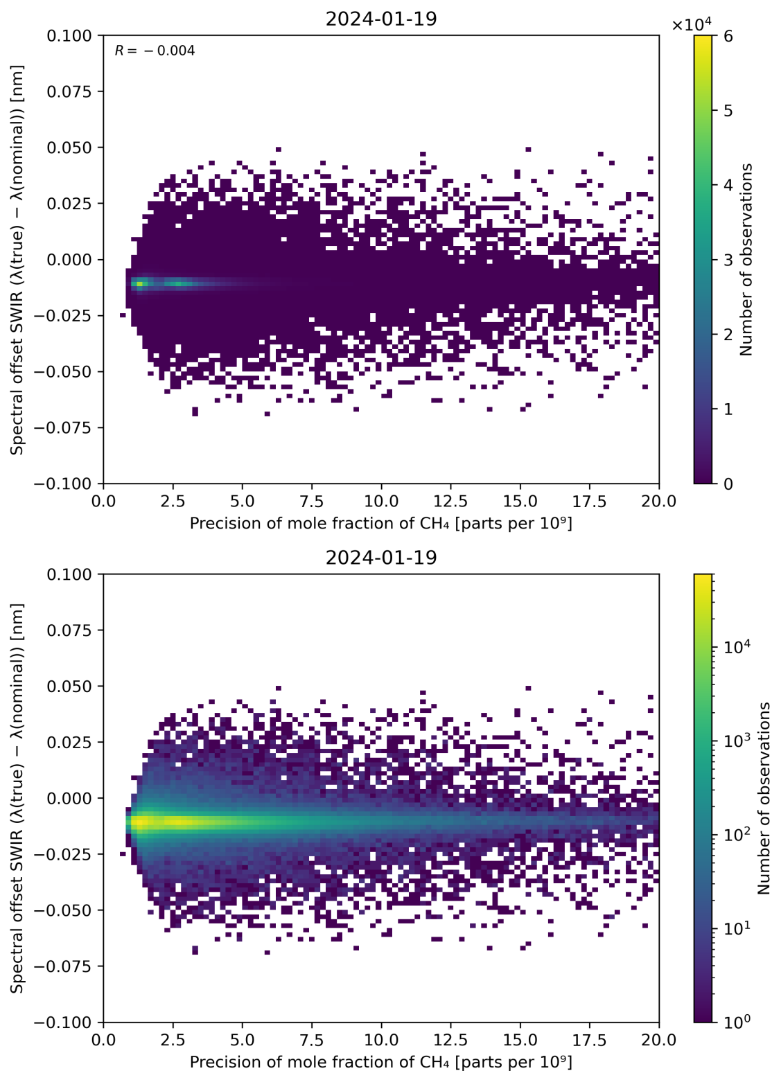
Figure 85: Scatter density plot of “Precision of mole fraction of \text{CH}_4 ” against “Spectral offset SWIR ( \lambda(\text{true}) - \lambda(\text{nominal}) )” for 2024-01-18 to 2024-01-20.
