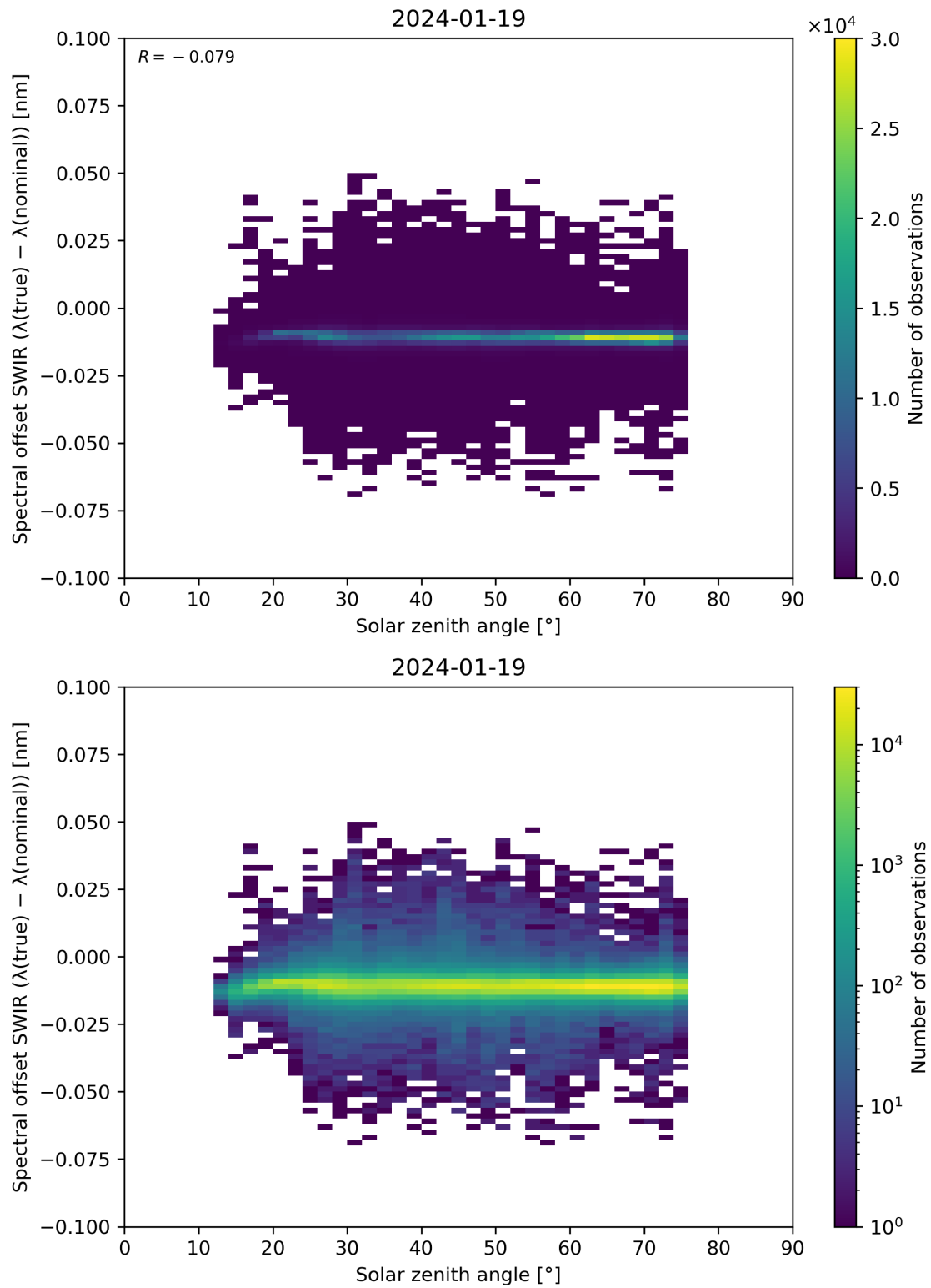
Figure 104: Scatter density plot of “Solar zenith angle” against “Spectral offset SWIR ( \lambda(\text{true}) - \lambda(\text{nominal}) )” for 2024-01-18 to 2024-01-20.
