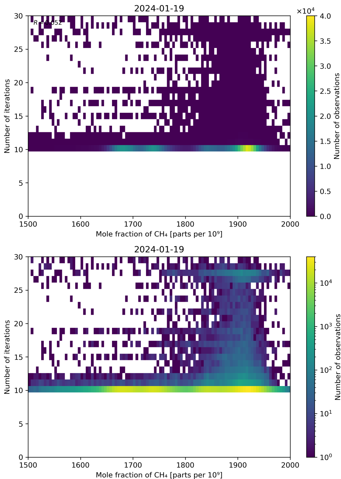
Figure 76: Scatter density plot of “Mole fraction of CH 4 ” against “Number of iterations” for 2024-01-18 to 2024-01-20.
