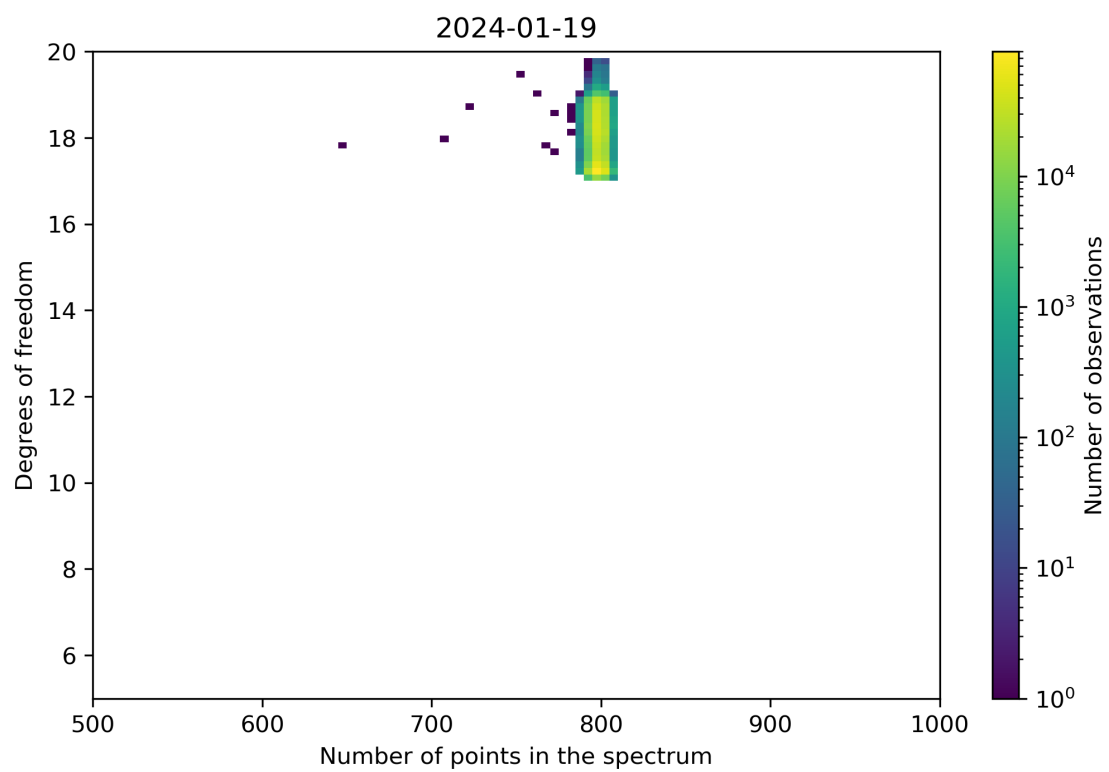
Figure 90: Scatter density plot of “Number of points in the spectrum” against “Degrees of freedom” for 2024-01-18 to 2024-01-20.
