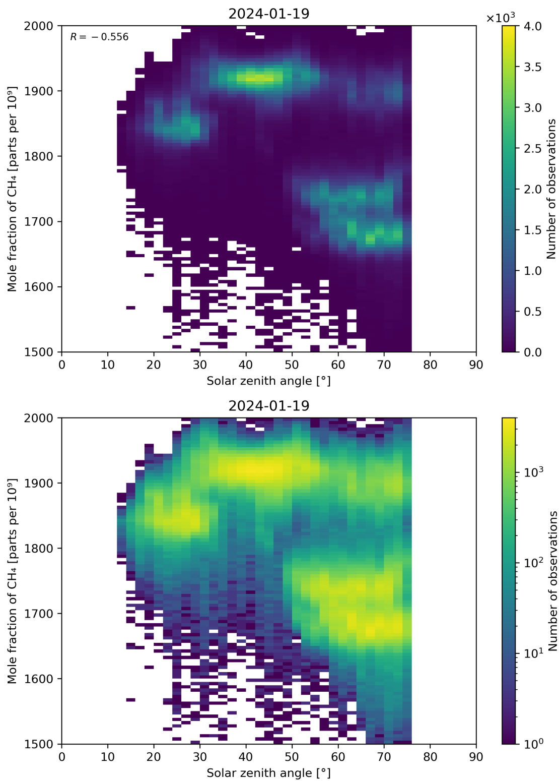
Figure 99: Scatter density plot of “Solar zenith angle” against “Mole fraction of CH 4 ” for 2024-01-18 to 2024-01-20.
