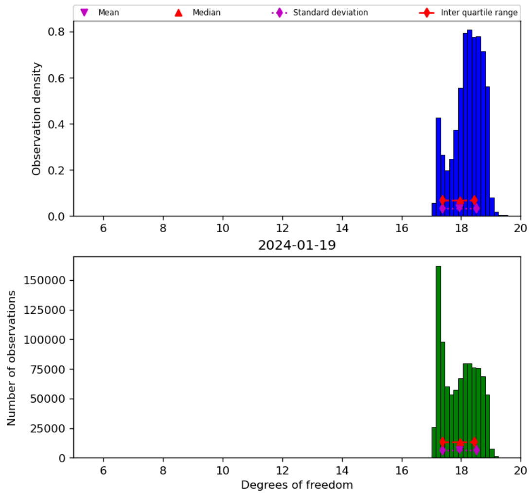
Figure 30: Histogram of “Degrees of freedom” for 2024-01-18 to 2024-01-20
