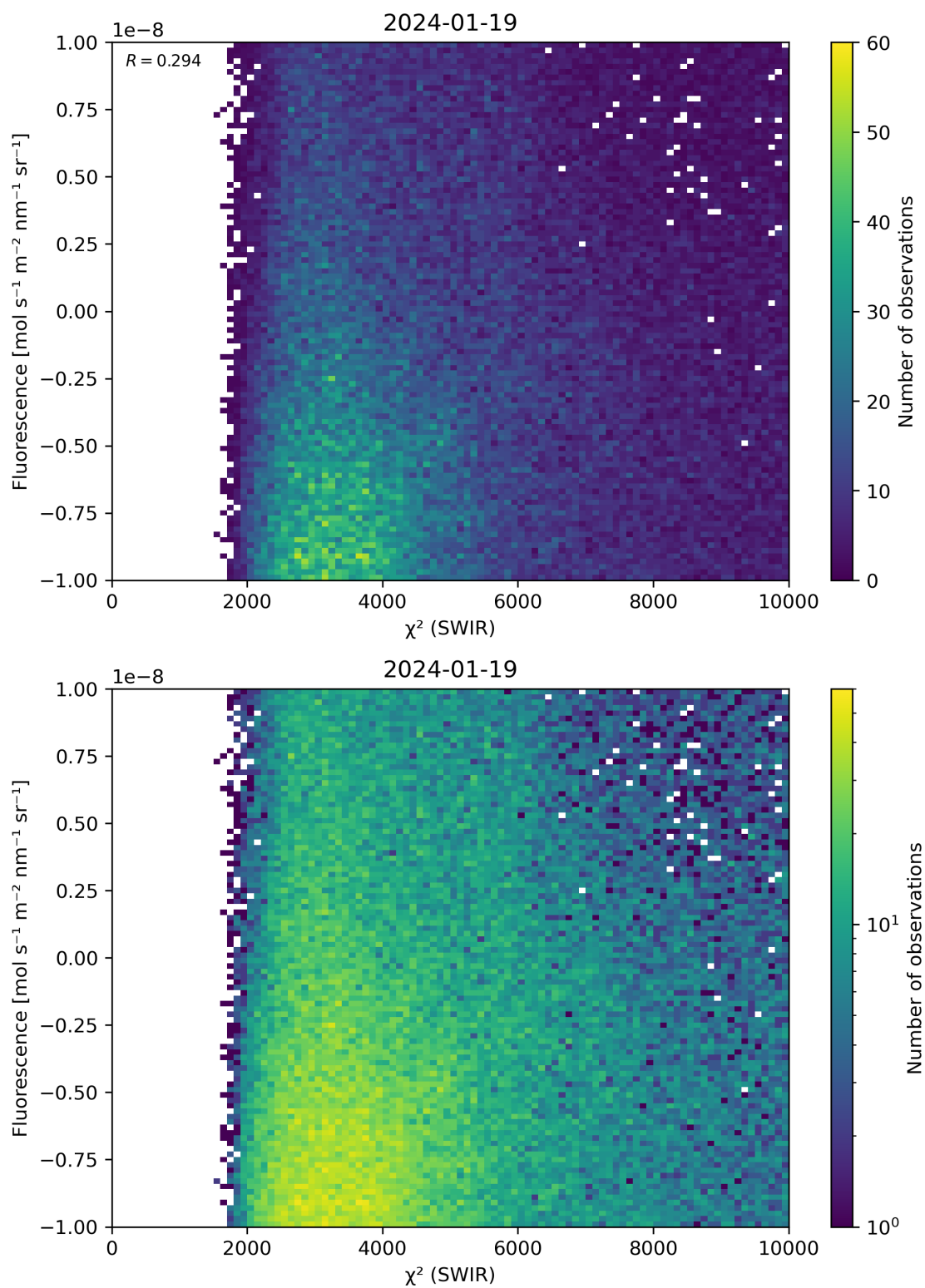
Figure 49: Scatter density plot of “ \chi^2 (SWIR)” against “Fluorescence” for 2024-01-18 to 2024-01-20.
