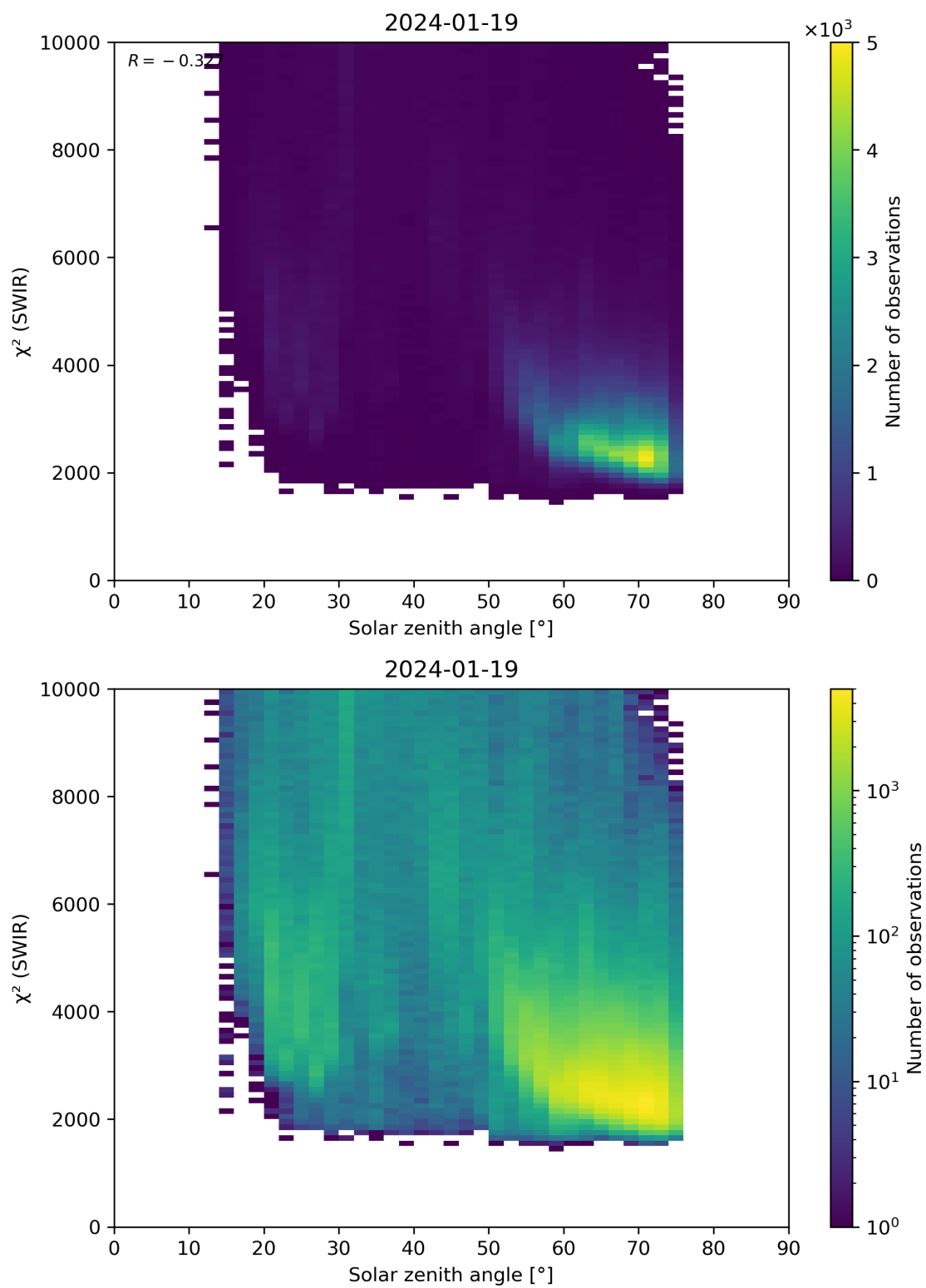
Figure 95: Scatter density plot of “Solar zenith angle” against “ \chi^2 (SWIR)” for 2024-01-18 to 2024-01-20.
