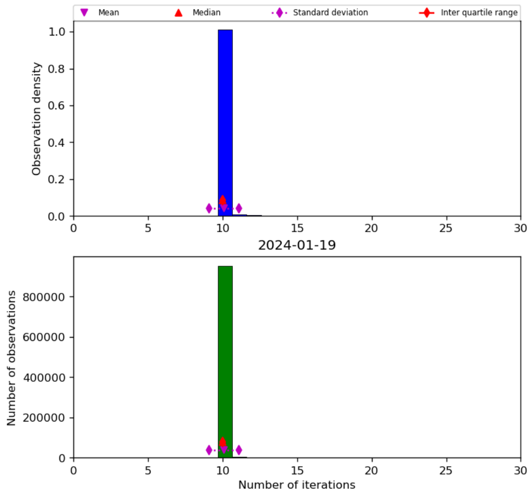
Figure 31: Histogram of “Number of iterations” for 2024-01-18 to 2024-01-20
