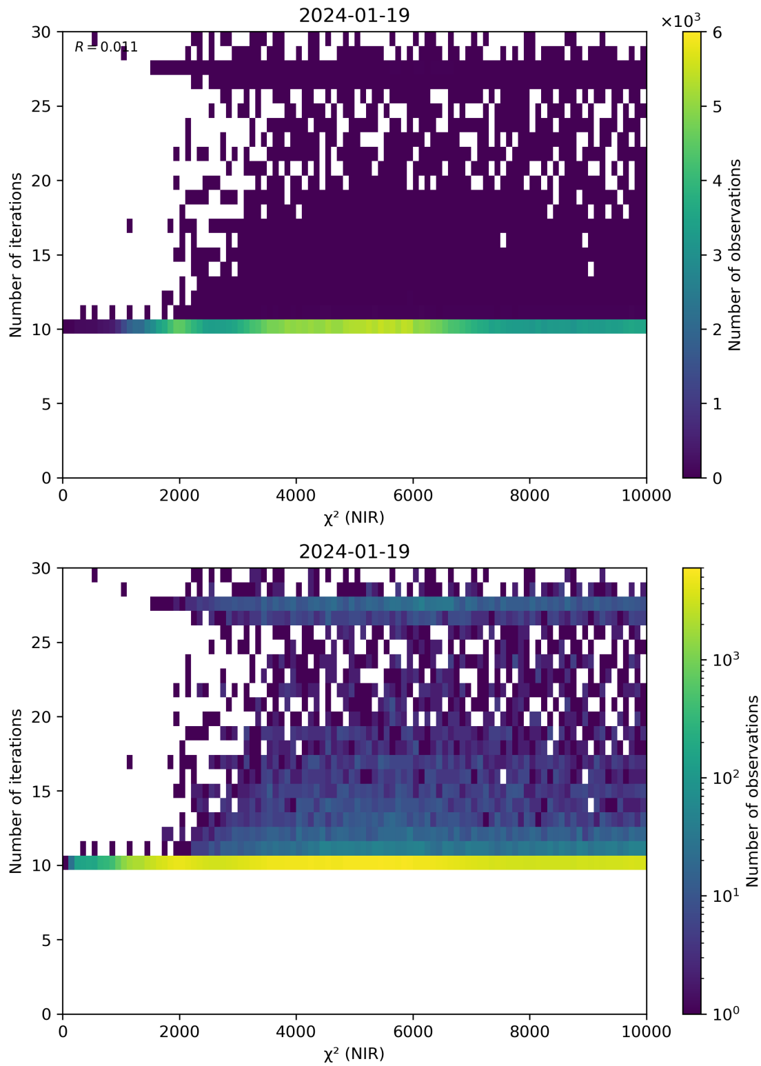
Figure 46: Scatter density plot of “ \chi^2 (NIR)” against “Number of iterations” for 2024-01-18 to 2024-01-20.
