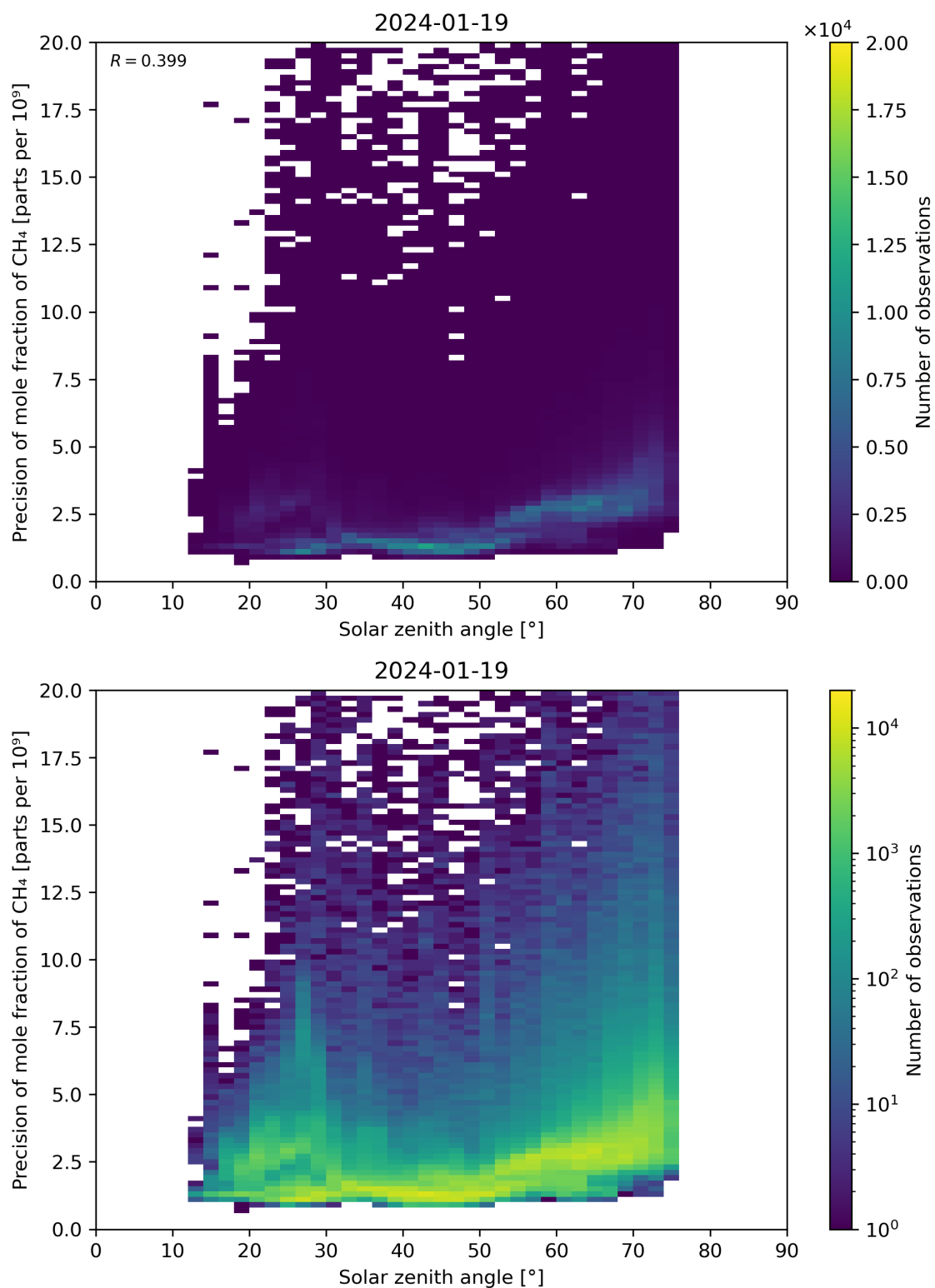
Figure 101: Scatter density plot of “Solar zenith angle” against “Precision of mole fraction of CH 4 ” for 2024-01-18 to 2024-01-20.
