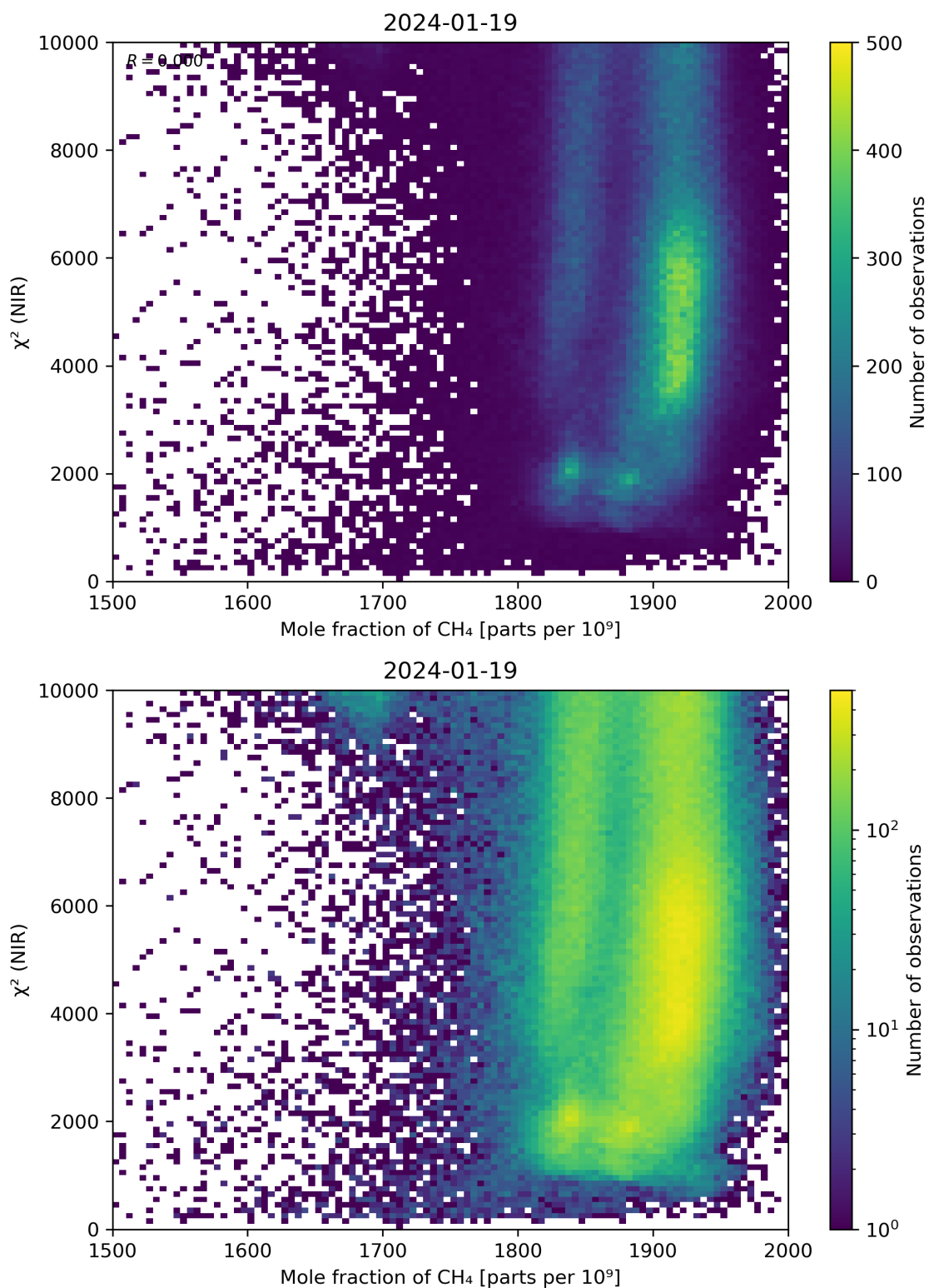
Figure 70: Scatter density plot of “Mole fraction of CH 4 ” against “ \chi^2 (NIR)” for 2024-01-18 to 2024-01-20.
