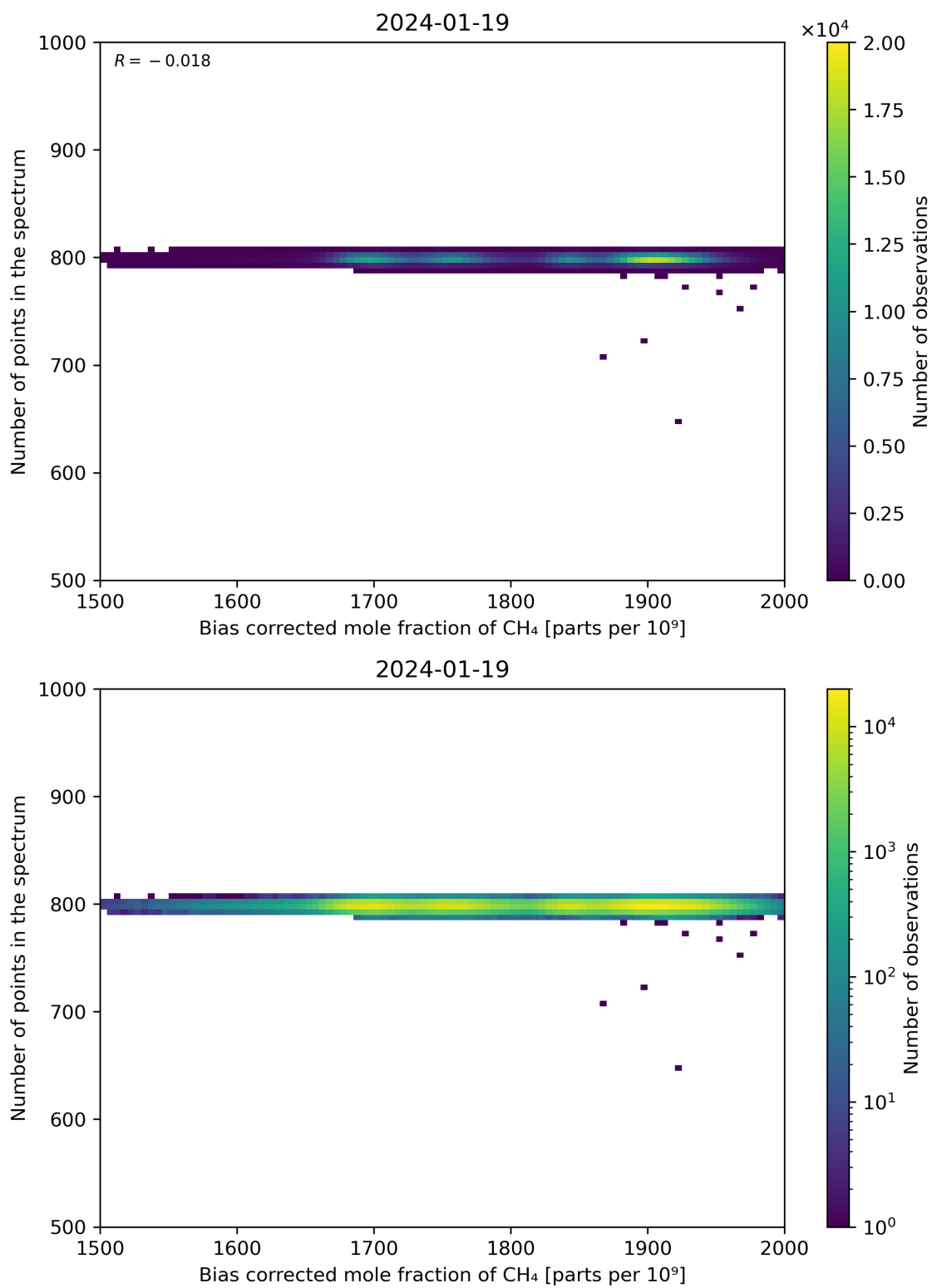
Figure 68: Scatter density plot of “Bias corrected mole fraction of CH 4 ” against “Number of points in the spectrum” for 2024-01-18 to 2024-01-20.
