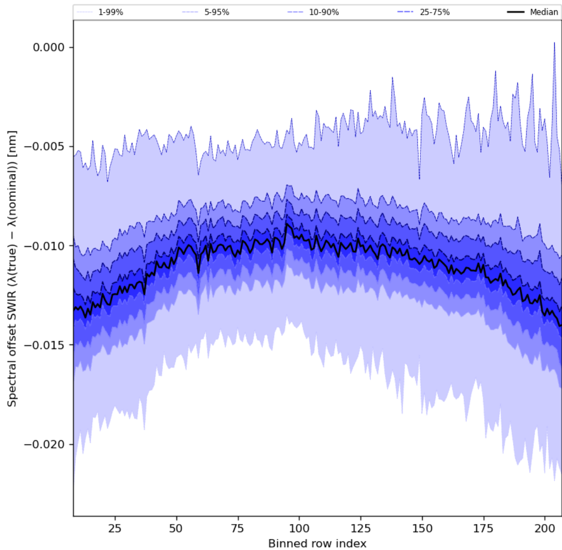
Figure 38: Along track statistics of “Spectral offset SWIR ( \lambda(\text{true}) - \lambda(\text{nominal}) )” for 2024-01-18 to 2024-01-20
