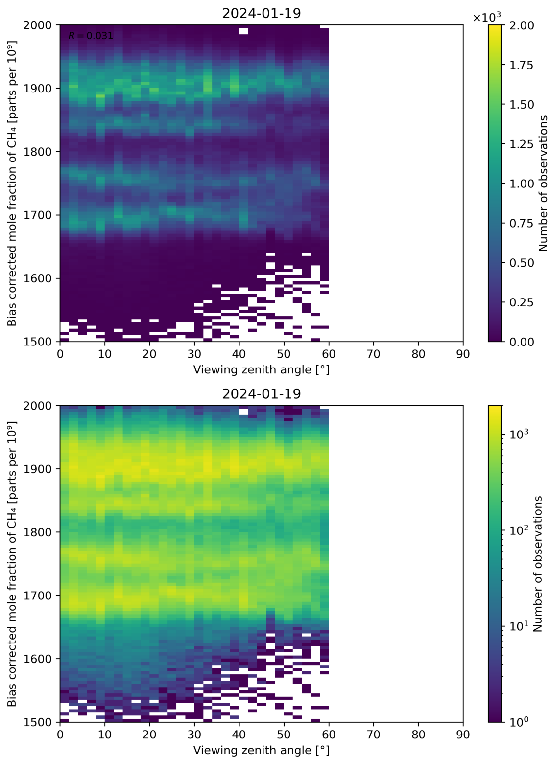
Figure 111: Scatter density plot of “Viewing zenith angle” against “Bias corrected mole fraction of CH 4 ” for 2024-01-18 to 2024-01-20.
