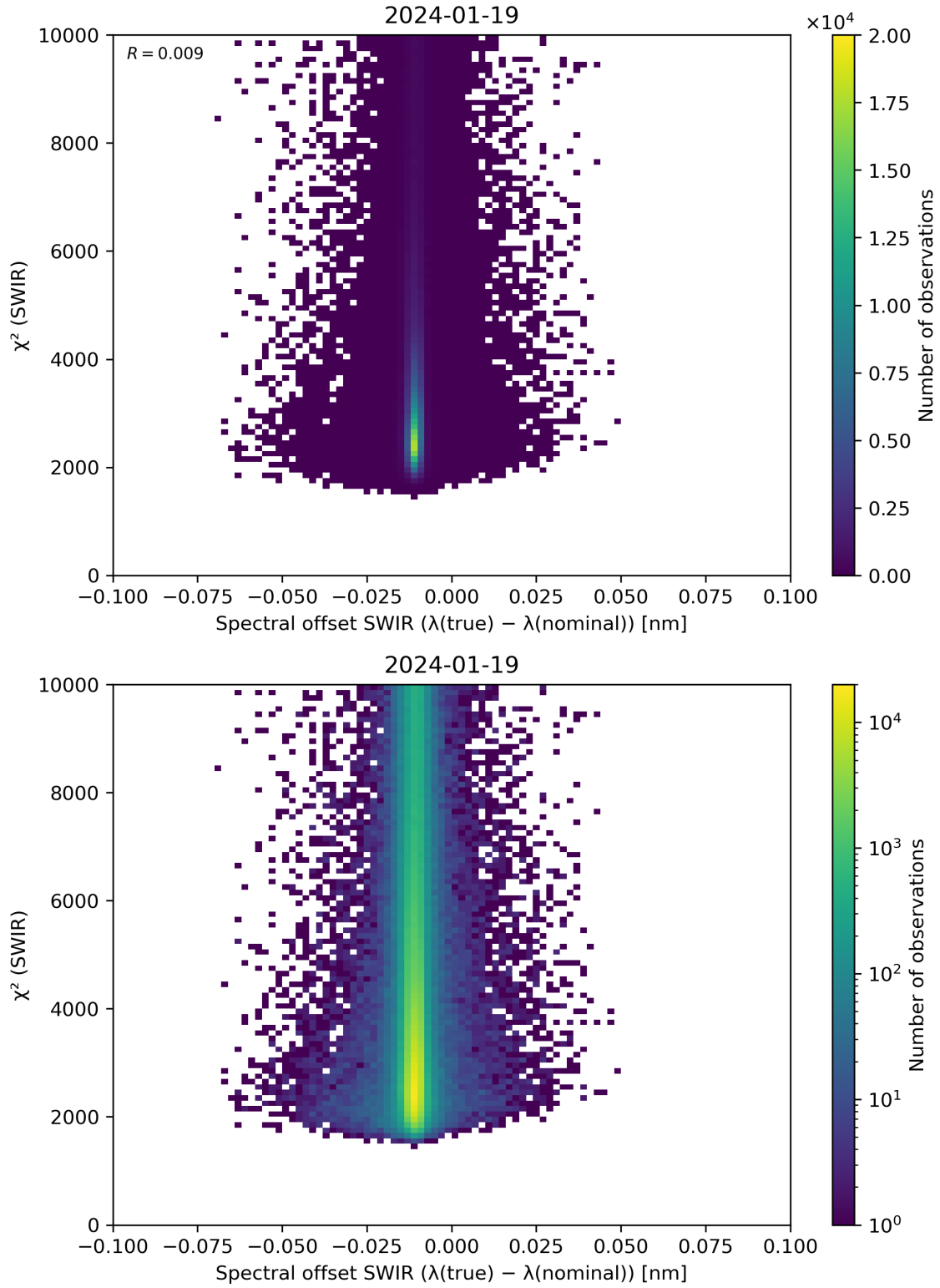
Figure 118: Scatter density plot of “Spectral offset SWIR ( \lambda(\text{true}) - \lambda(\text{nominal}) )” against “ \chi^2 (SWIR)” for 2024-01-18 to 2024-01-20.
