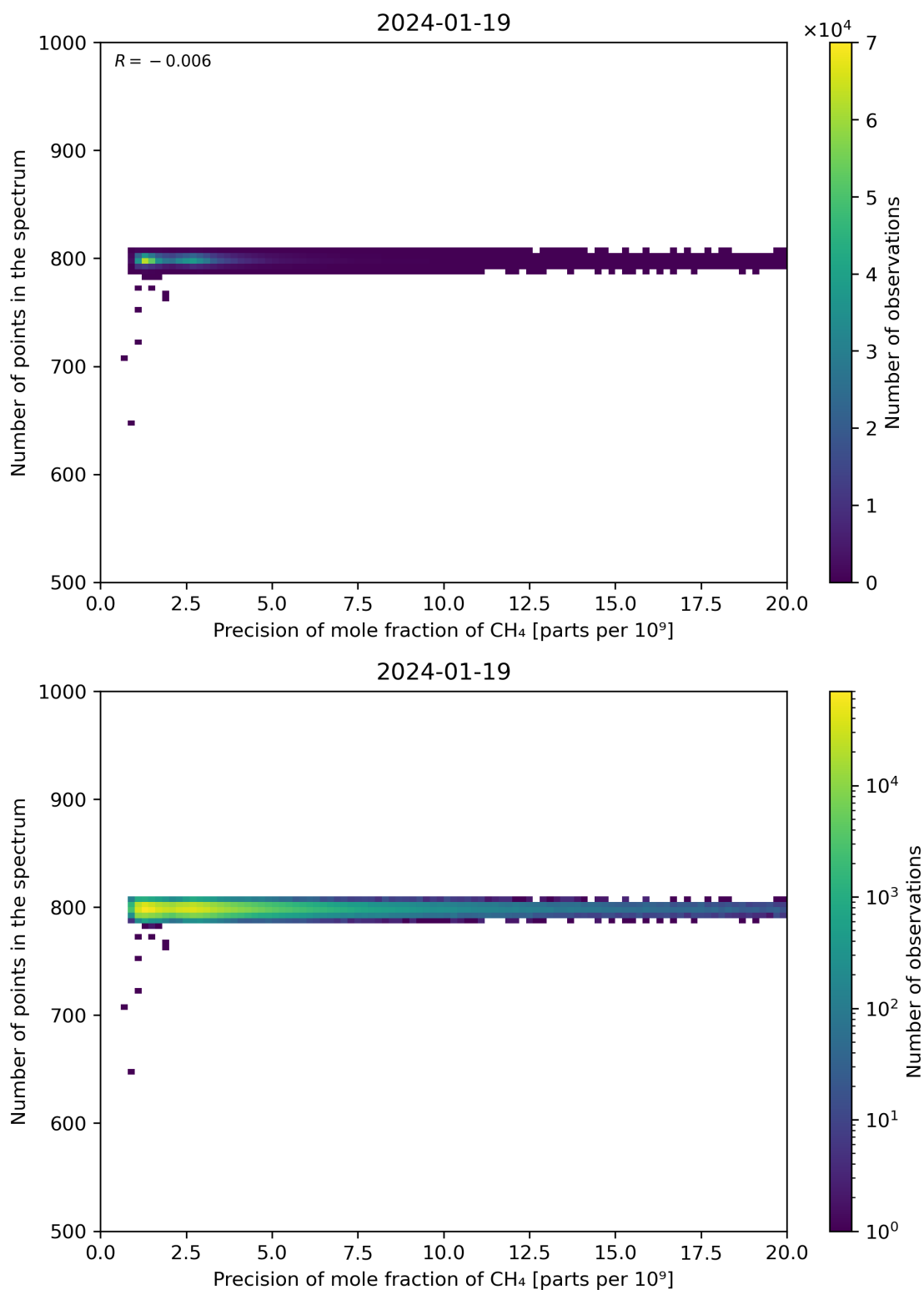
Figure 84: Scatter density plot of “Precision of mole fraction of CH 4 ” against “Number of points in the spectrum” for 2024-01-18 to 2024-01-20.
