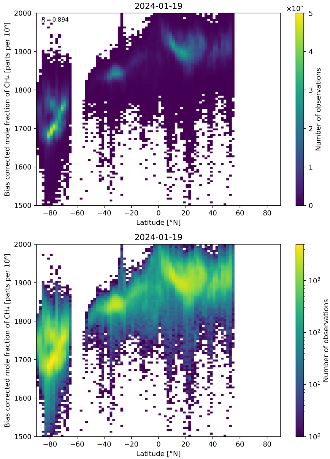
Figure 58: Scatter density plot of “Latitude” against “Bias corrected mole fraction of CH 4 ” for 2024-01-18 to 2024-01-20.
