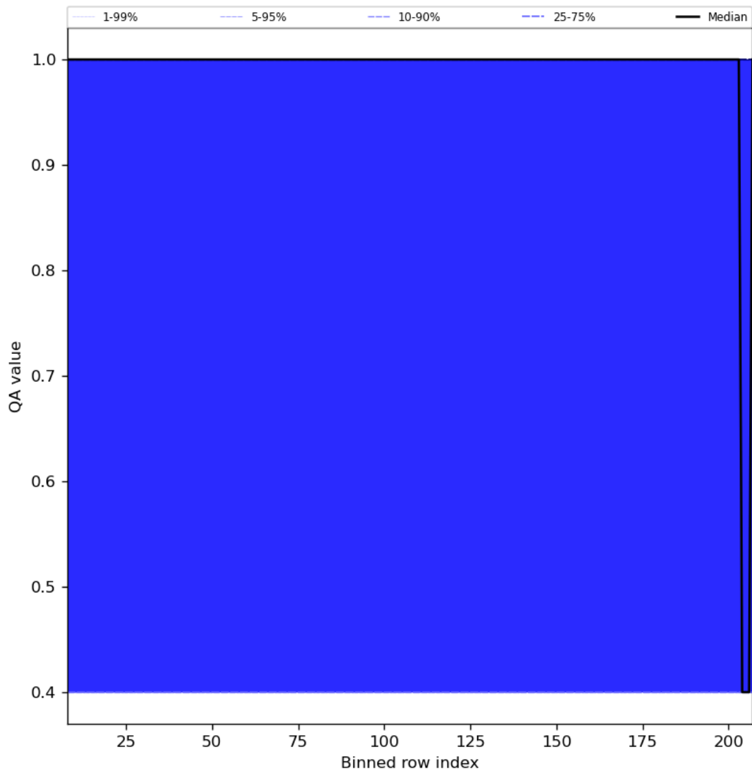
Figure 33: Along track statistics of “QA value” for 2024-01-18 to 2024-01-20
