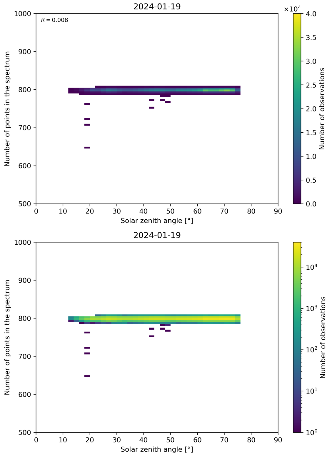
Figure 103: Scatter density plot of “Solar zenith angle” against “Number of points in the spectrum” for 2024-01-18 to 2024-01-20.
