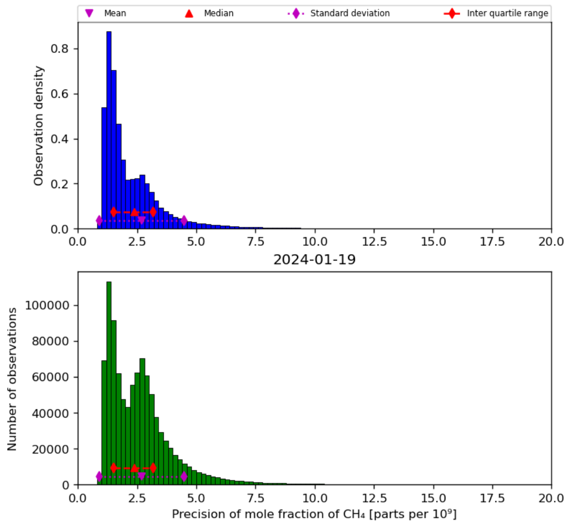
Figure 24: Histogram of “Precision of mole fraction of CH 4 ” for 2024-01-18 to 2024-01-20
