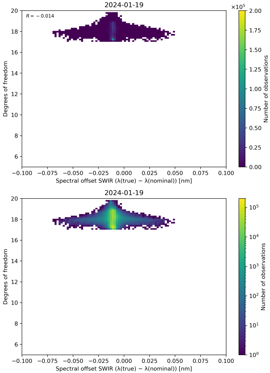
Figure 119: Scatter density plot of “Spectral offset SWIR ( \lambda(\text{true}) - \lambda(\text{nominal}) )” against “Degrees of freedom” for 2024-01-18 to 2024-01-20.
