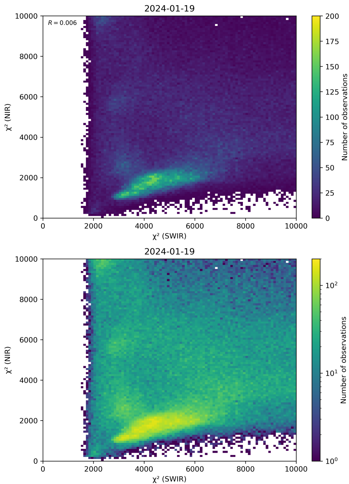
Figure 47: Scatter density plot of “ \chi^2 (SWIR)” against “ \chi^2 (NIR)” for 2024-01-18 to 2024-01-20.
