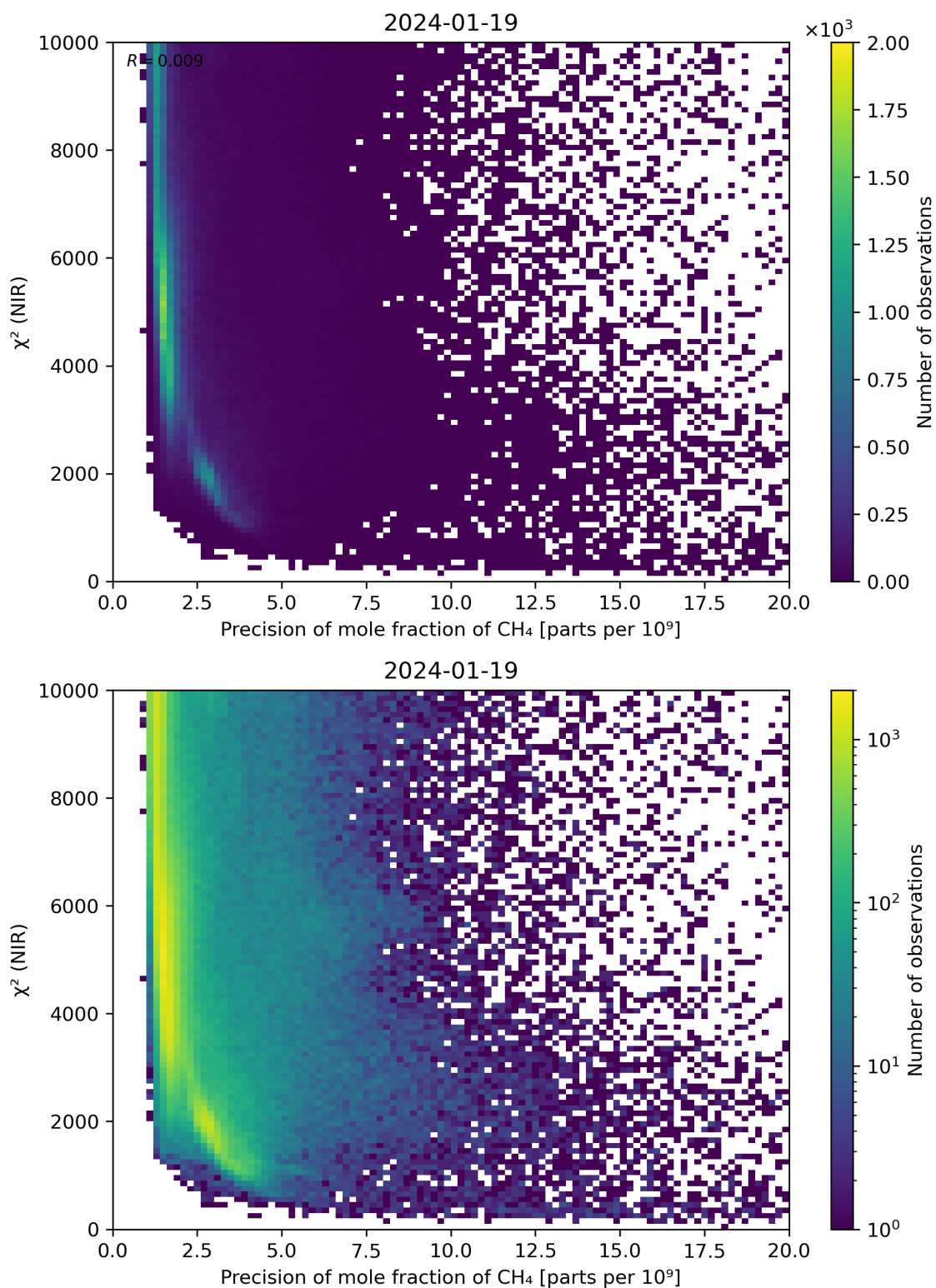
Figure 78: Scatter density plot of “Precision of mole fraction of \text{CH}_4 ” against “ \chi^2 (NIR)” for 2024-01-18 to 2024-01-20.
