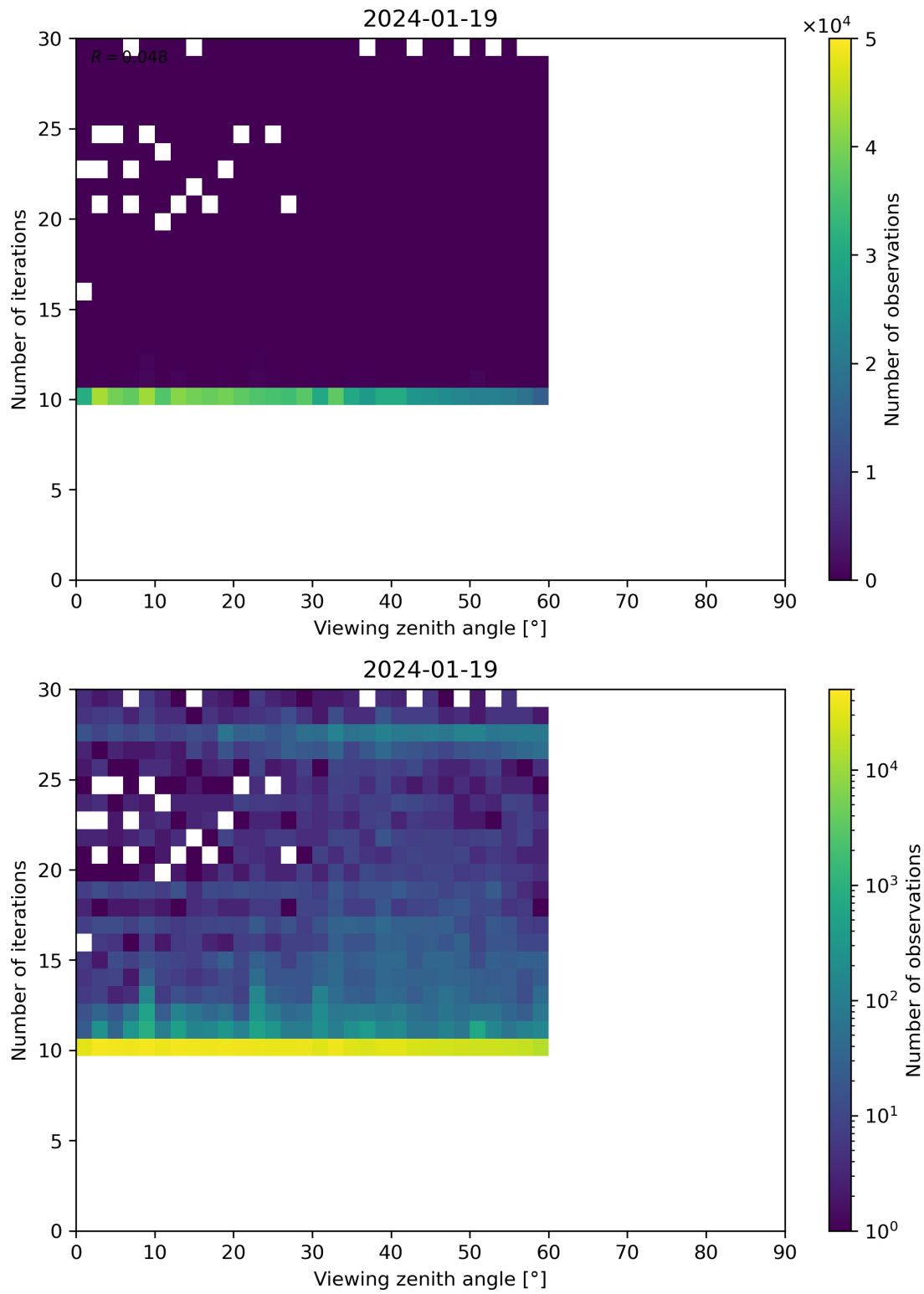
Figure 113: Scatter density plot of “Viewing zenith angle” against “Number of iterations” for 2024-01-18 to 2024-01-20.
