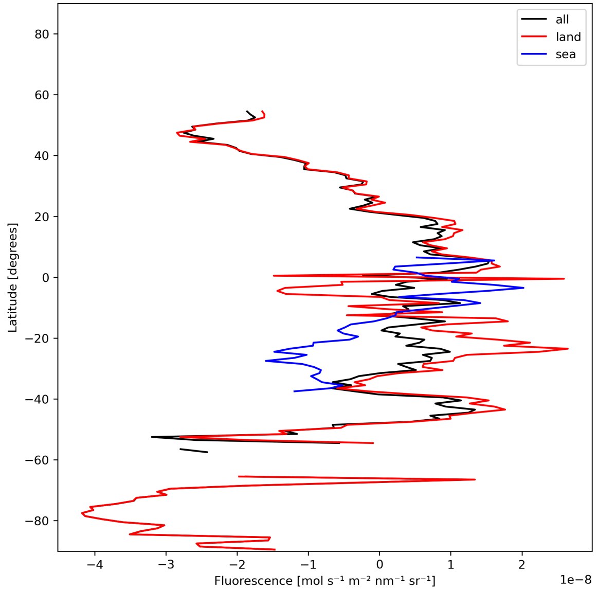
Figure 21: Zonal average of “Fluorescence” for 2024-01-18 to 2024-01-20.
