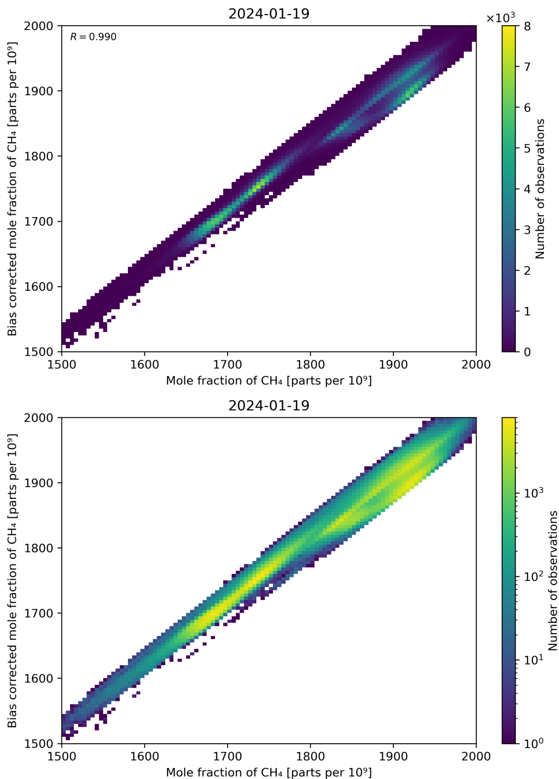
Figure 74: Scatter density plot of “Mole fraction of CH 4 ” against “Bias corrected mole fraction of CH 4 ” for 2024-01-18 to 2024-01-20.
