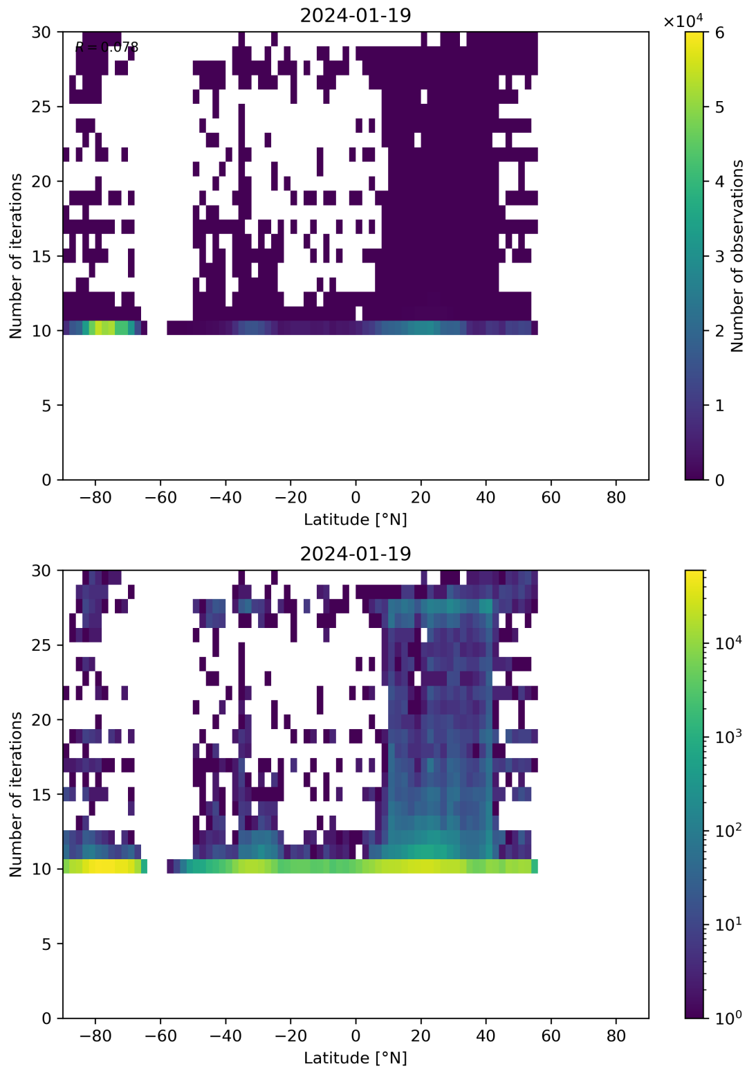
Figure 60: Scatter density plot of “Latitude” against “Number of iterations” for 2024-01-18 to 2024-01-20.
