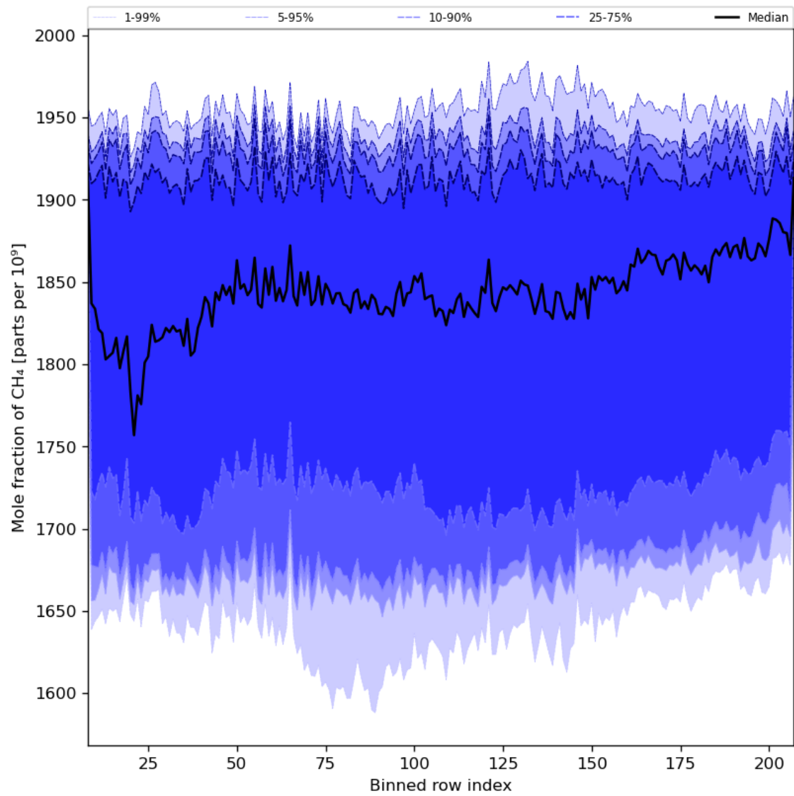
Figure 34: Along track statistics of “Mole fraction of CH 4 ” for 2024-01-18 to 2024-01-20
