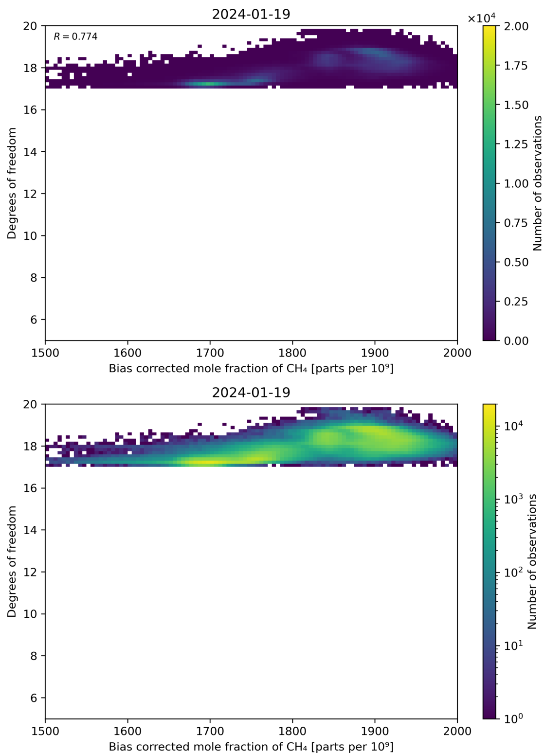
Figure 65: Scatter density plot of “Bias corrected mole fraction of CH 4 ” against “Degrees of freedom” for 2024-01-18 to 2024-01-20.
