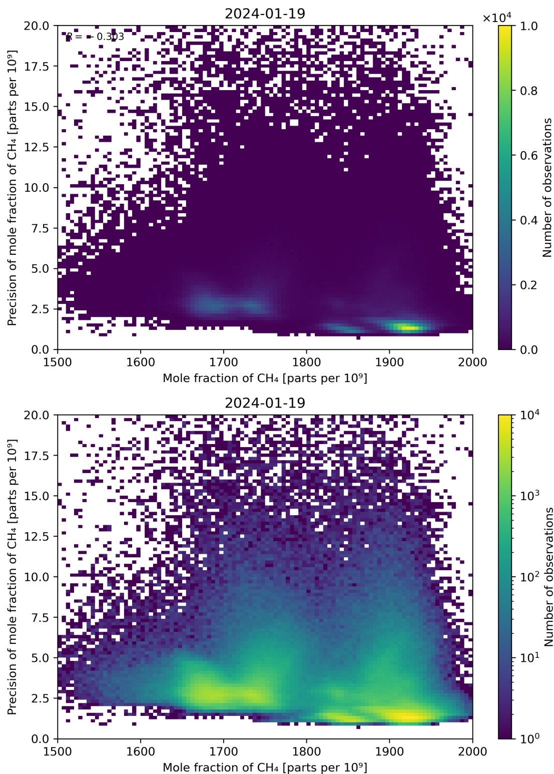
Figure 75: Scatter density plot of “Mole fraction of CH 4 ” against “Precision of mole fraction of CH 4 ” for 2024-01-18 to 2024-01-20.
