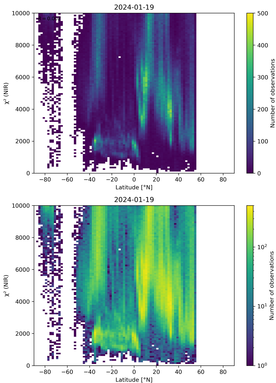
Figure 53: Scatter density plot of “Latitude” against “ \chi^2 (NIR)” for 2024-01-18 to 2024-01-20.
