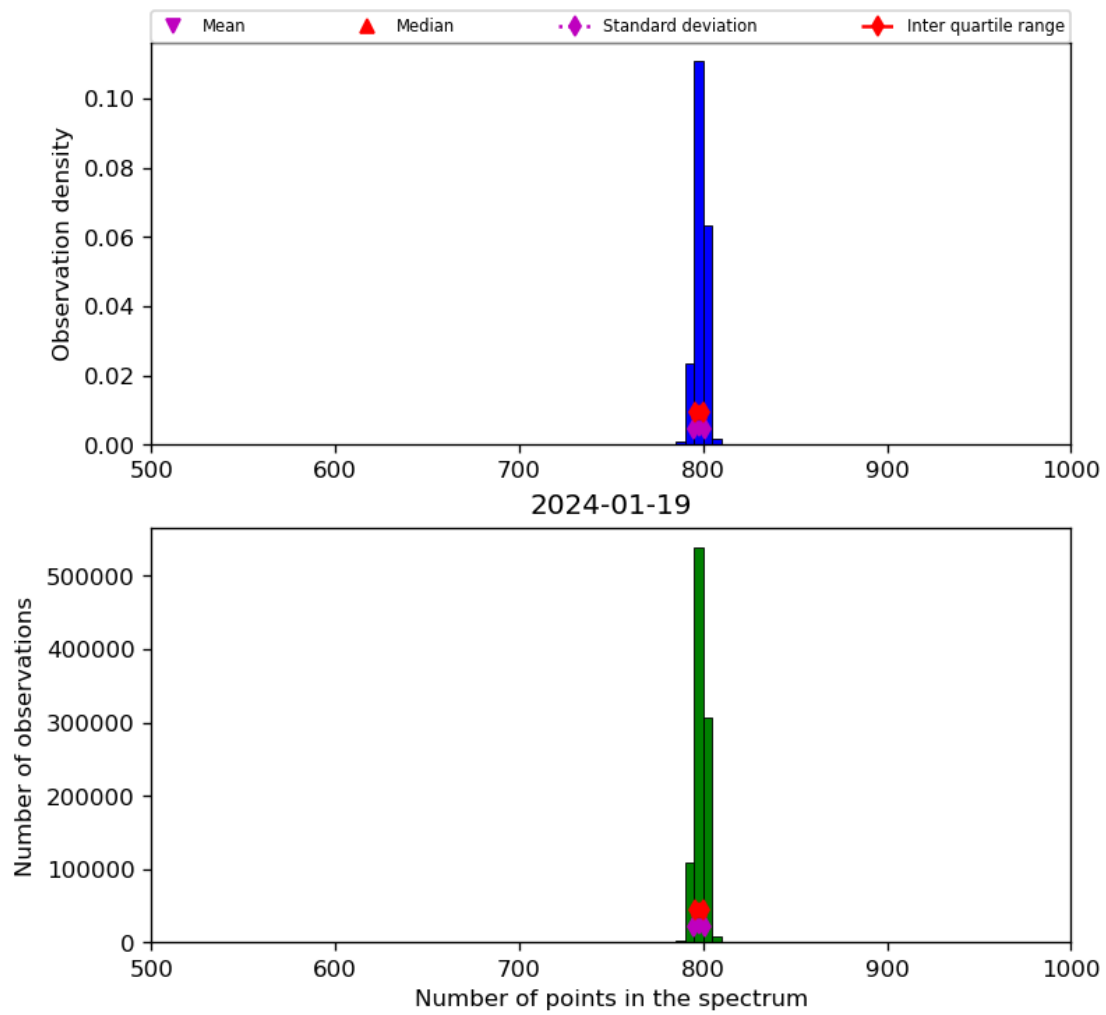
Figure 26: Histogram of “Number of points in the spectrum” for 2024-01-18 to 2024-01-20
