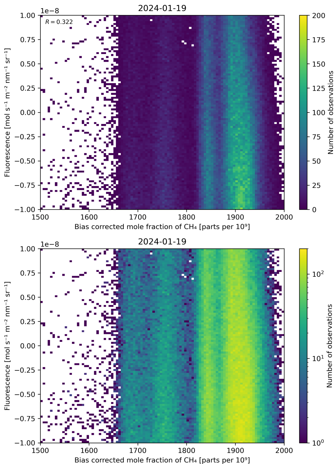
Figure 66: Scatter density plot of “Bias corrected mole fraction of \text{CH}_4 ” against “Fluorescence” for 2024-01-18 to 2024-01-20.
