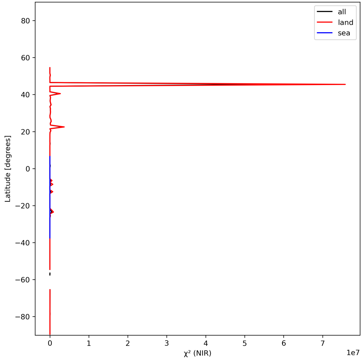
Figure 18: Zonal average of “ \chi^2 (NIR)” for 2024-01-18 to 2024-01-20.
