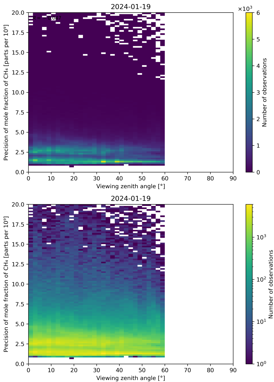
Figure 112: Scatter density plot of “Viewing zenith angle” against “Precision of mole fraction of CH 4 ” for 2024-01-18 to 2024-01-20.
