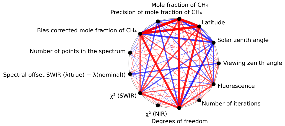
Figure 1: Map of correlation graph for 2024-01-18 to 2024-01-20.
