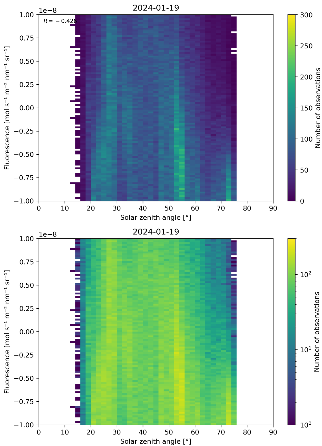
Figure 97: Scatter density plot of “Solar zenith angle” against “Fluorescence” for 2024-01-18 to 2024-01-20.
