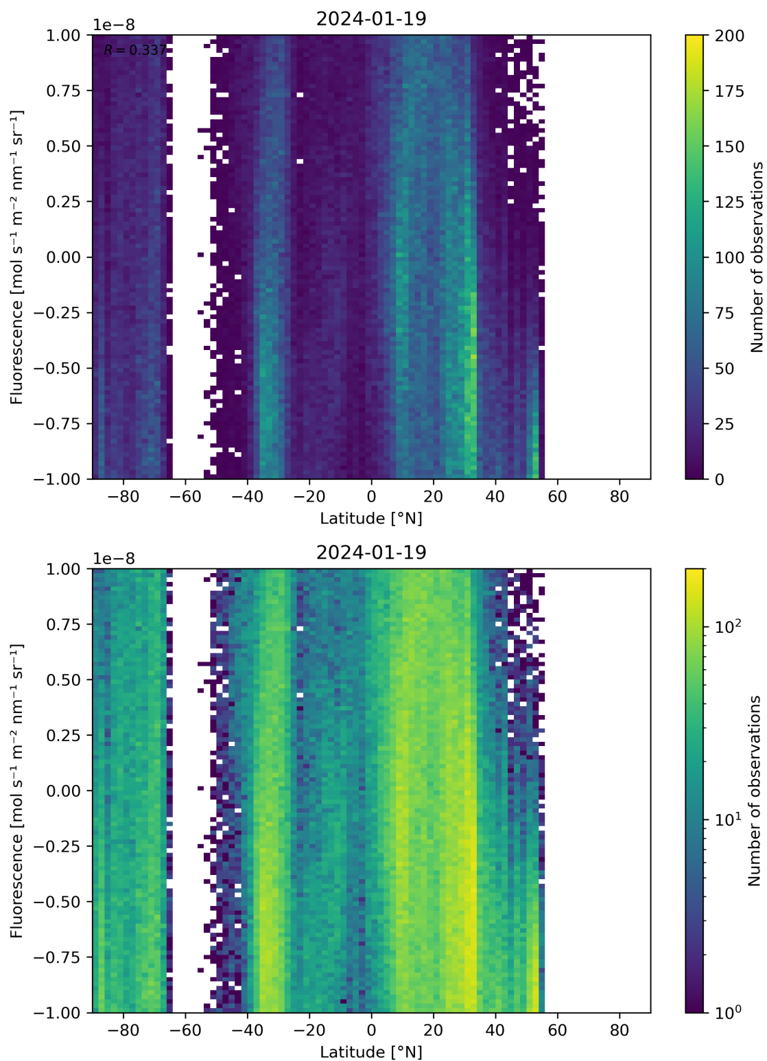
Figure 56: Scatter density plot of “Latitude” against “Fluorescence” for 2024-01-18 to 2024-01-20.
