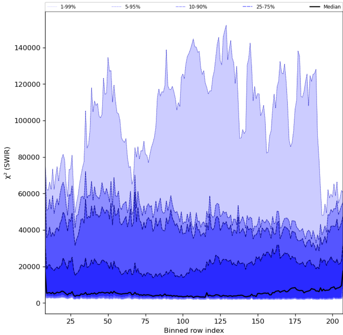
Figure 39: Along track statistics of “ \chi^2 (SWIR)” for 2024-01-18 to 2024-01-20
