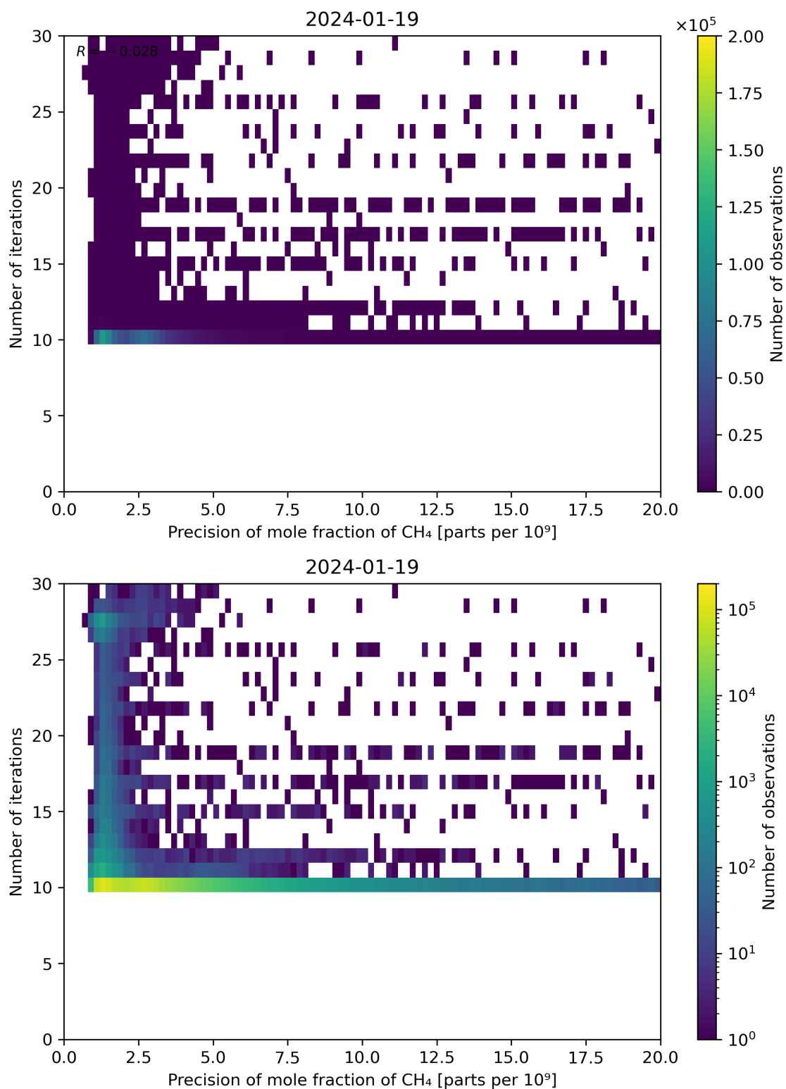
Figure 83: Scatter density plot of “Precision of mole fraction of CH 4 ” against “Number of iterations” for 2024-01-18 to 2024-01-20.
