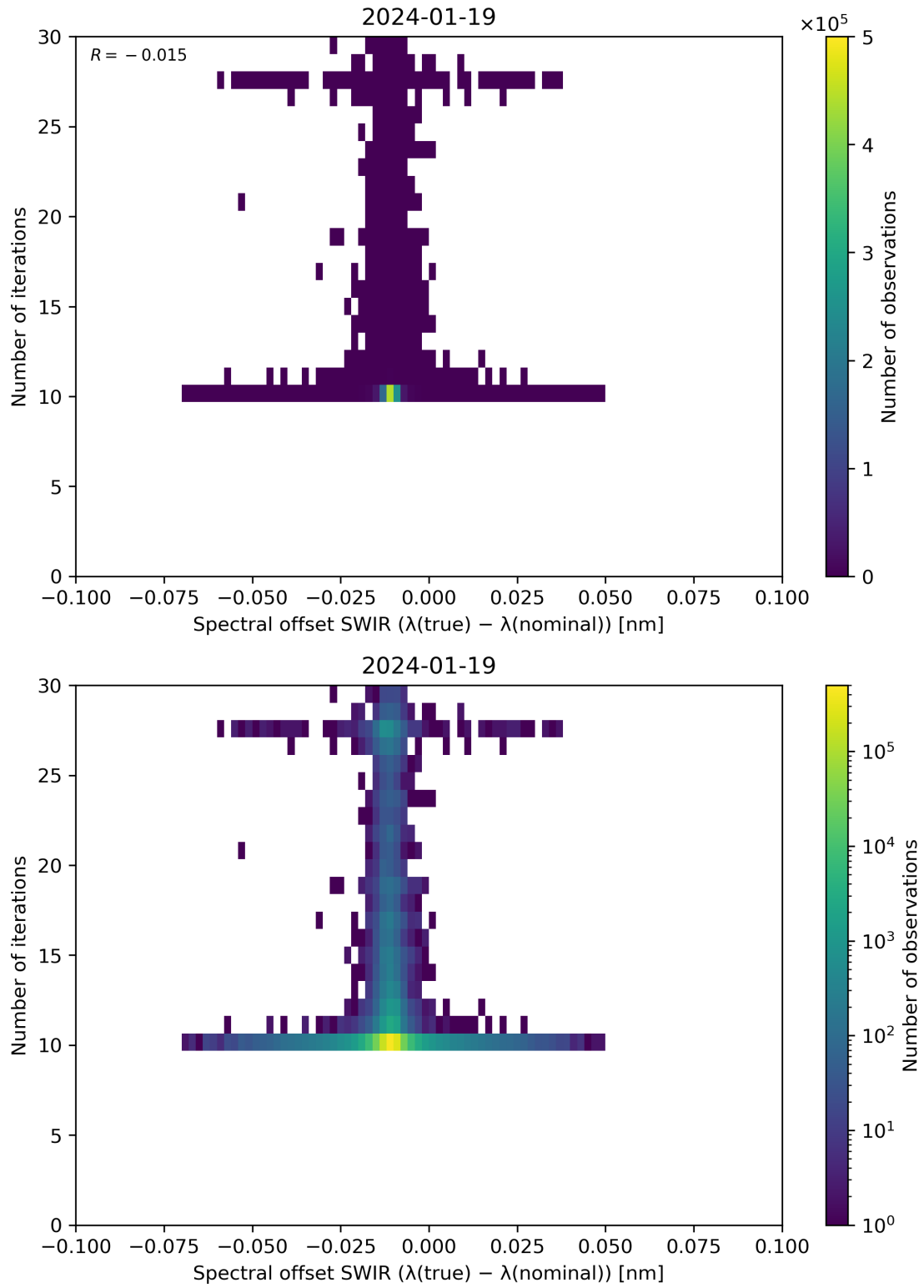
Figure 121: Scatter density plot of “Spectral offset SWIR ( \lambda(\text{true}) - \lambda(\text{nominal}) )” against “Number of iterations” for 2024-01-18 to 2024-01-20.
