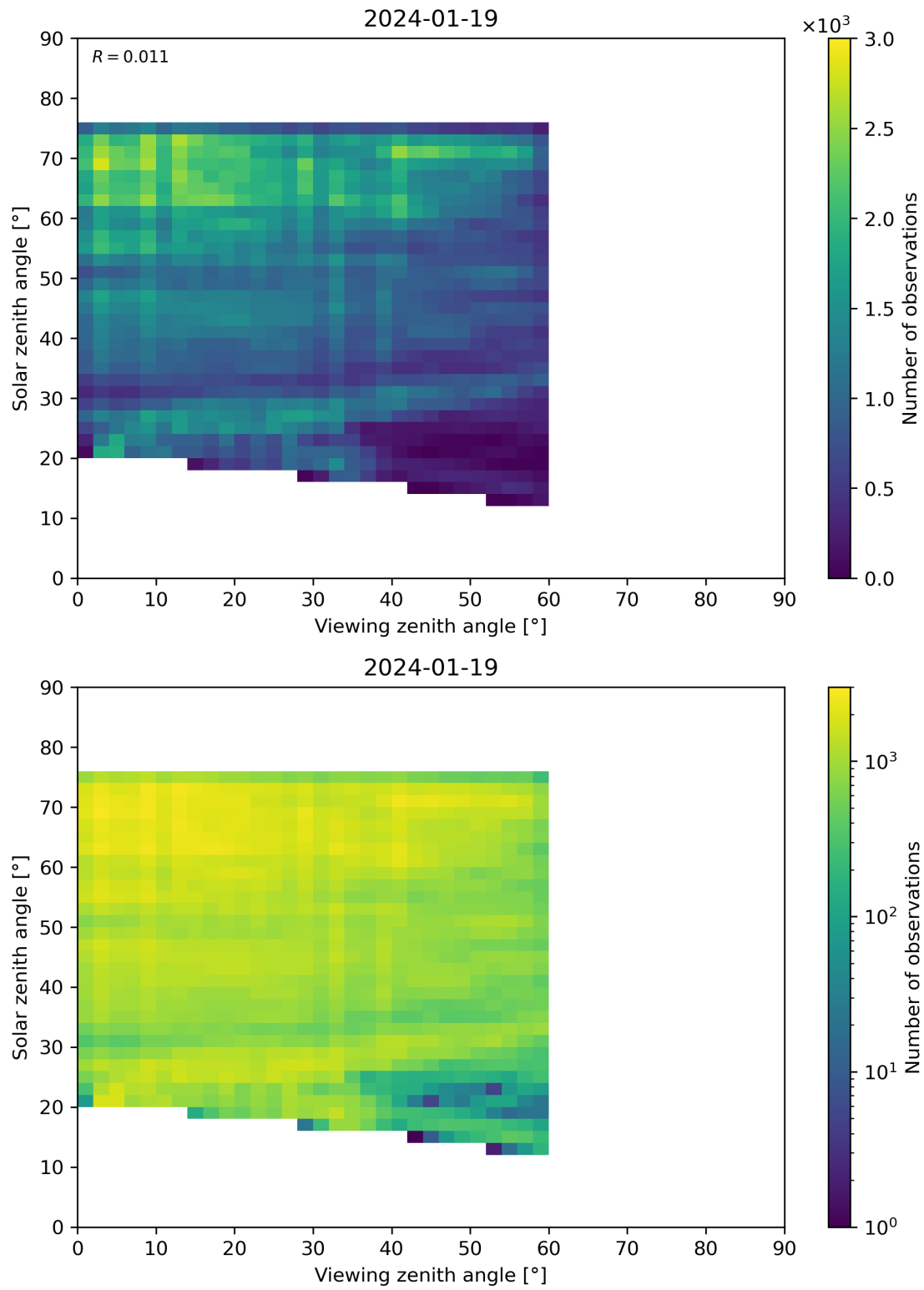
Figure 115: Scatter density plot of “Viewing zenith angle” against “Solar zenith angle” for 2024-01-18 to 2024-01-20.
