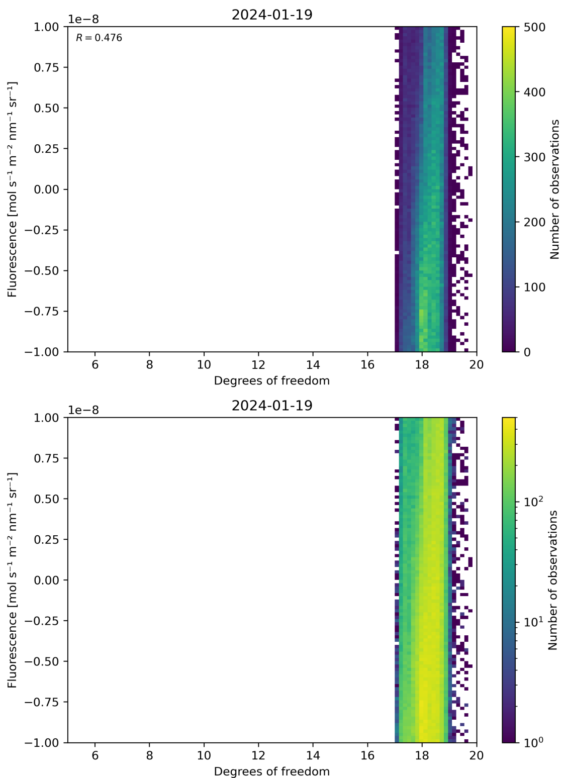
Figure 51: Scatter density plot of “Degrees of freedom” against “Fluorescence” for 2024-01-18 to 2024-01-20.
