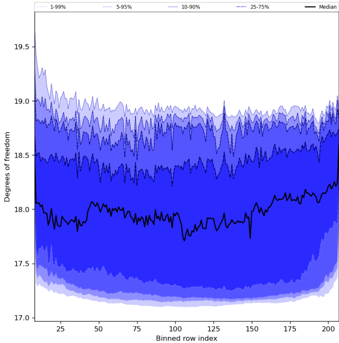
Figure 41: Along track statistics of “Degrees of freedom” for 2024-01-18 to 2024-01-20
