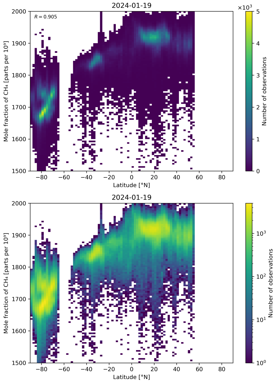
Figure 57: Scatter density plot of “Latitude” against “Mole fraction of CH 4 ” for 2024-01-18 to 2024-01-20.
