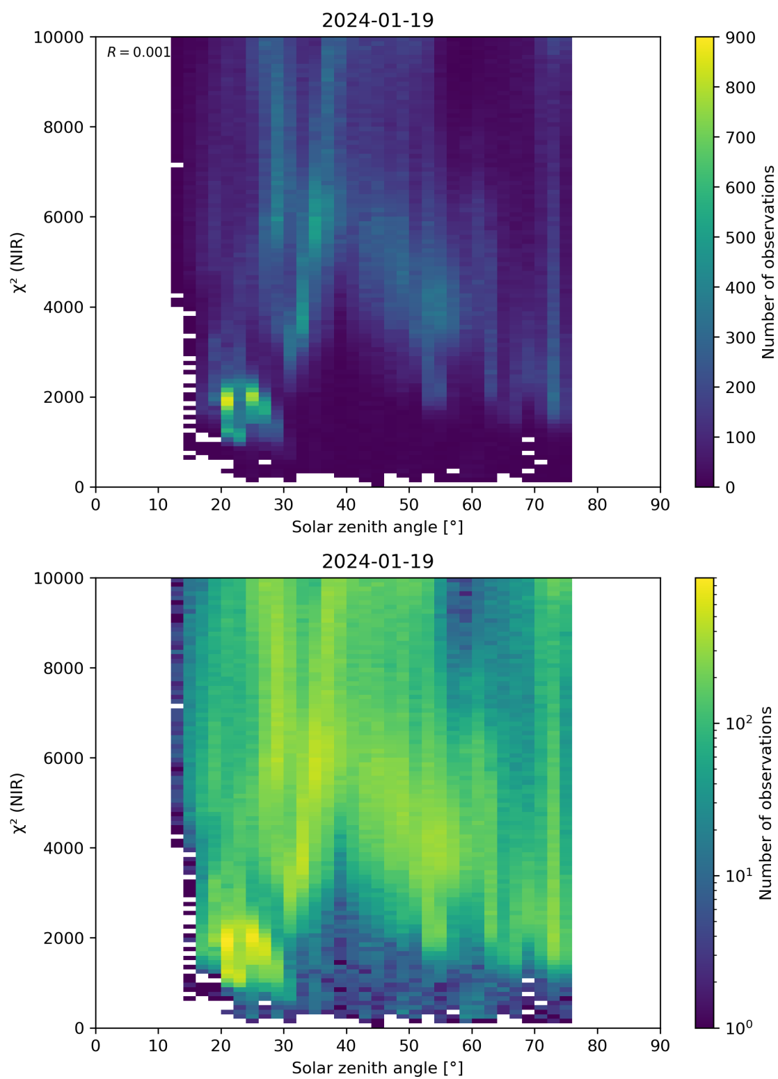
Figure 94: Scatter density plot of “Solar zenith angle” against “ \chi^2 (NIR)” for 2024-01-18 to 2024-01-20.
