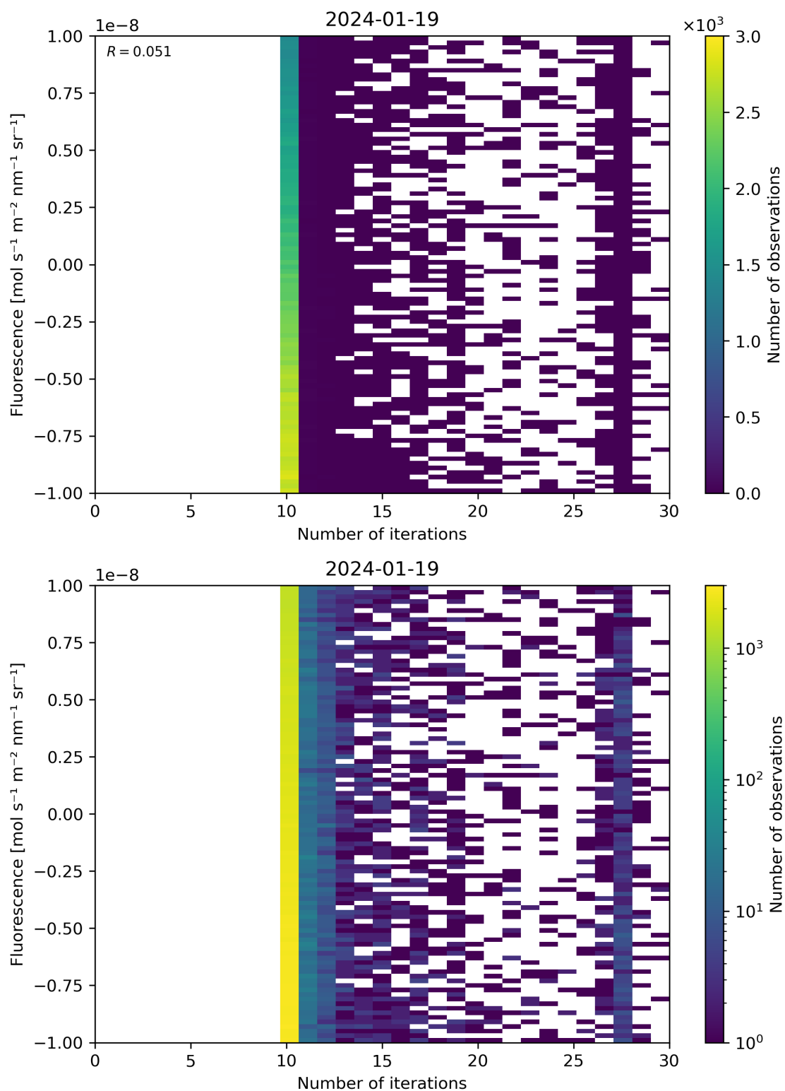
Figure 87: Scatter density plot of “Number of iterations” against “Fluorescence” for 2024-01-18 to 2024-01-20.
