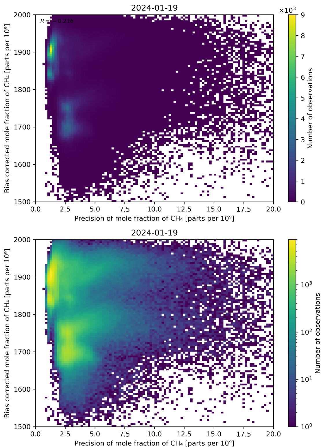
Figure 82: Scatter density plot of “Precision of mole fraction of CH 4 ” against “Bias corrected mole fraction of CH 4 ” for 2024-01-18 to 2024-01-20.
