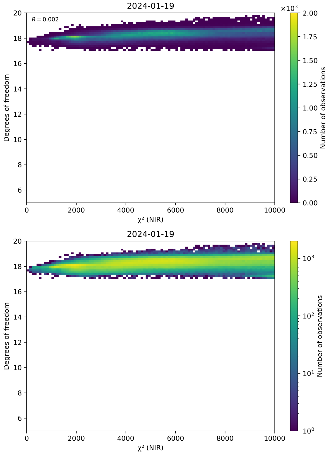
Figure 44: Scatter density plot of “ \chi^2 (NIR)” against “Degrees of freedom” for 2024-01-18 to 2024-01-20.
