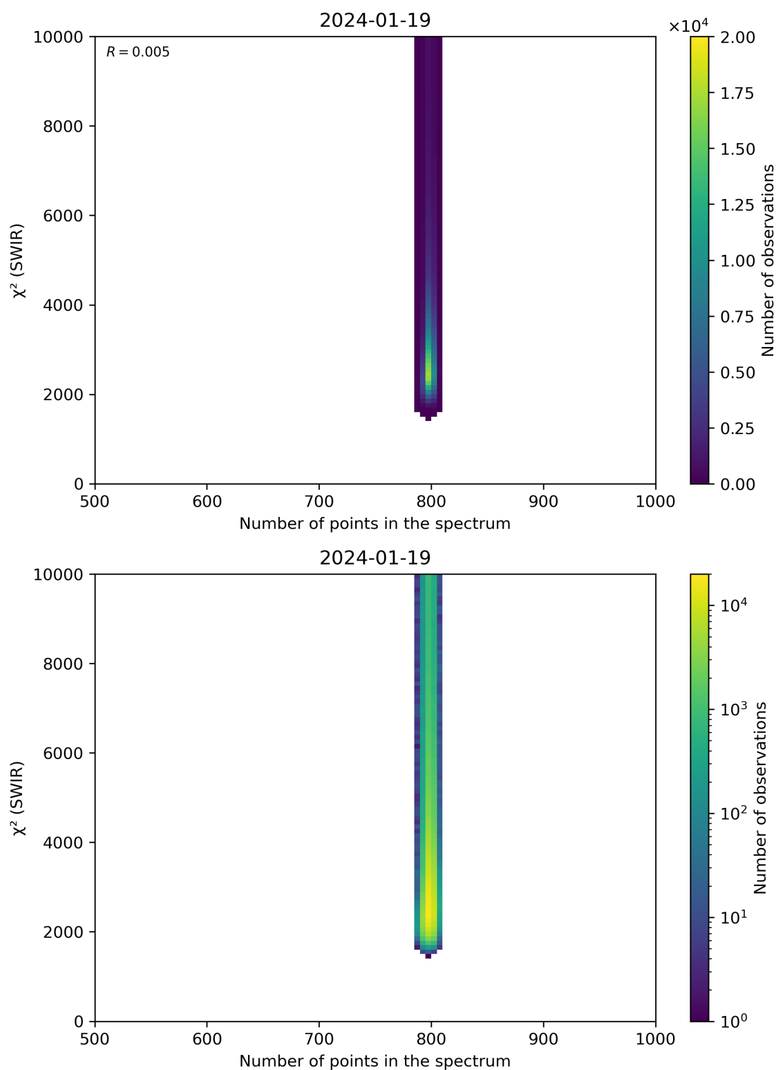
Figure 89: Scatter density plot of “Number of points in the spectrum” against “ \chi^2 (SWIR)” for 2024-01-18 to 2024-01-20.
