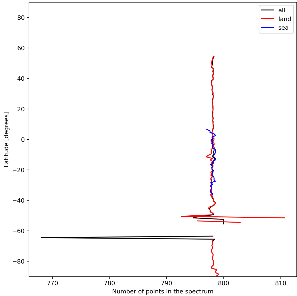
Figure 15: Zonal average of “Number of points in the spectrum” for 2024-01-19 to 2024-01-21.
