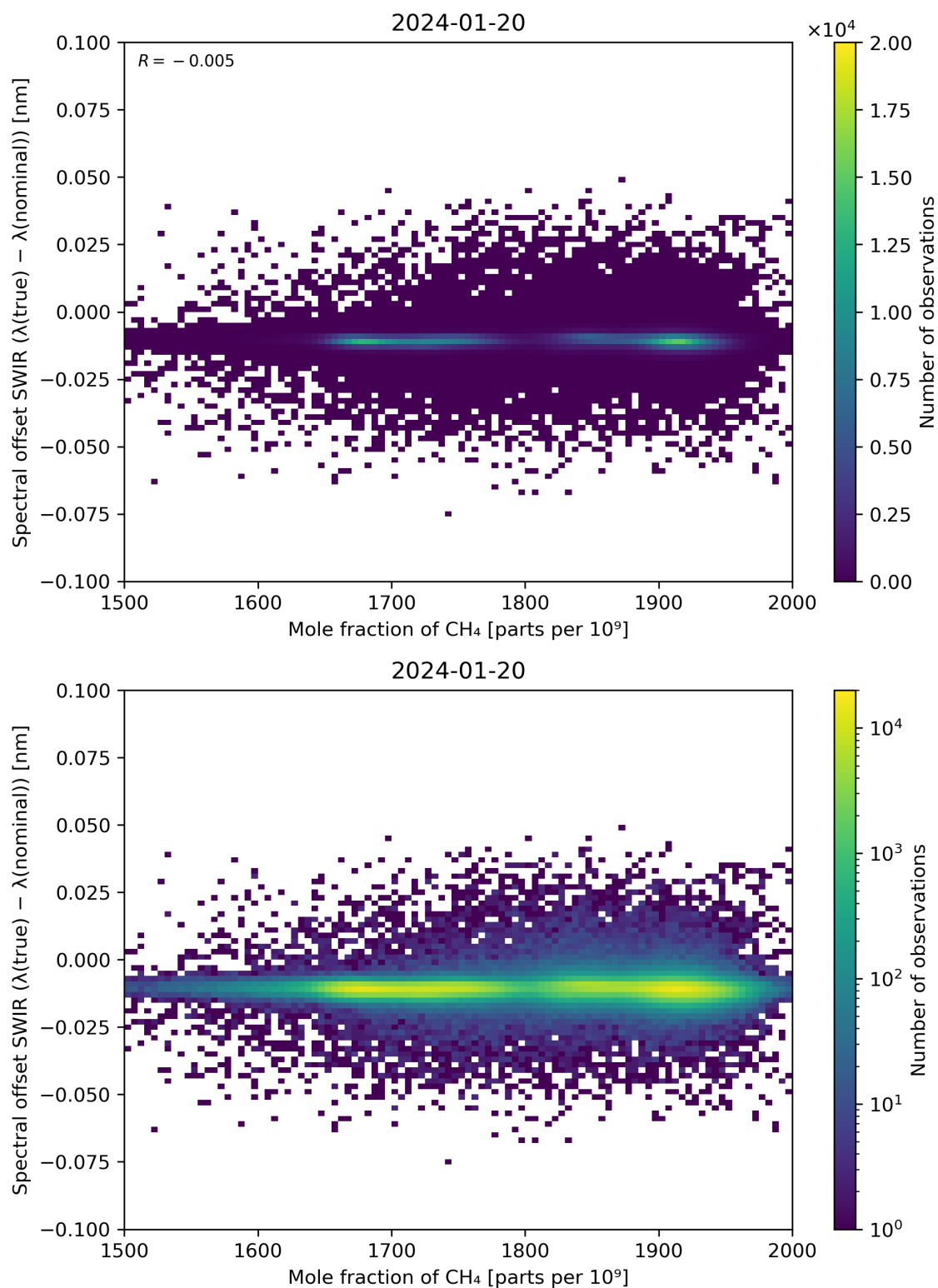
Figure 86: Scatter density plot of “Mole fraction of CH 4 ” against “Spectral offset SWIR ( \lambda(\text{true}) - \lambda(\text{nominal}) )” for 2024-01-19 to 2024-01-21.
