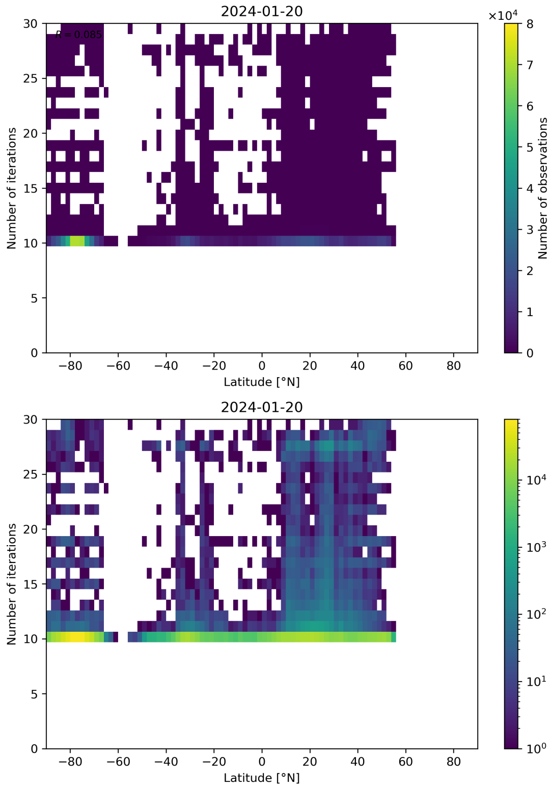
Figure 60: Scatter density plot of “Latitude” against “Number of iterations” for 2024-01-19 to 2024-01-21.
