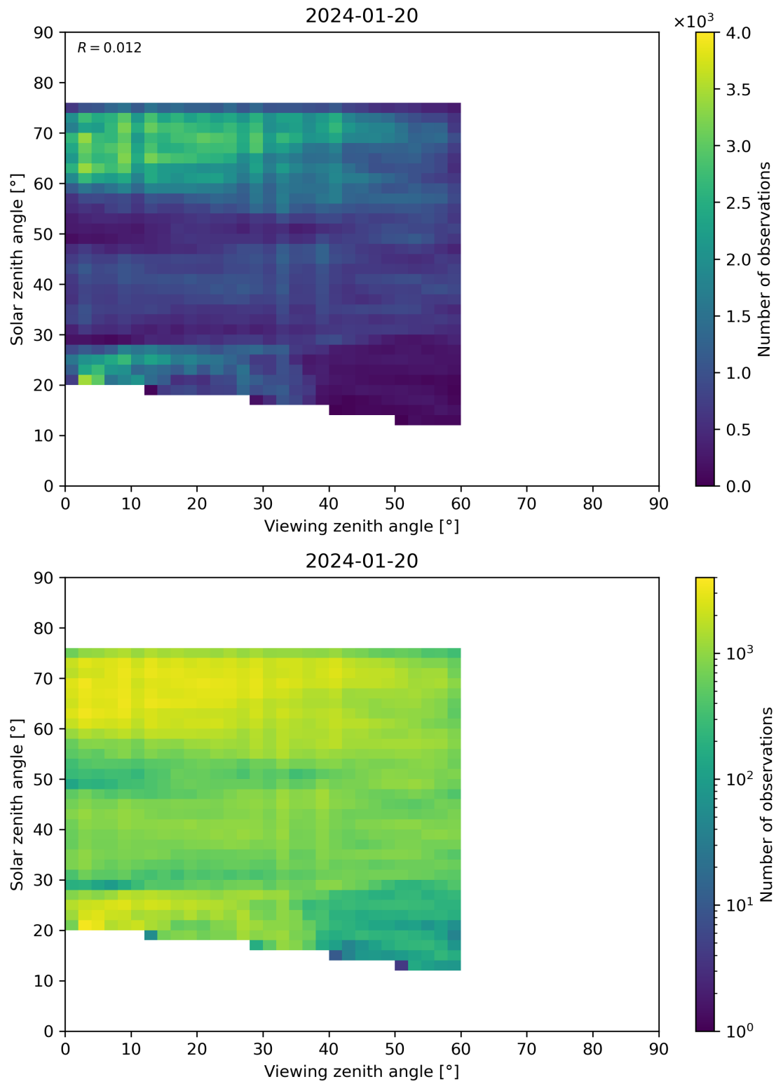
Figure 115: Scatter density plot of “Viewing zenith angle” against “Solar zenith angle” for 2024-01-19 to 2024-01-21.
