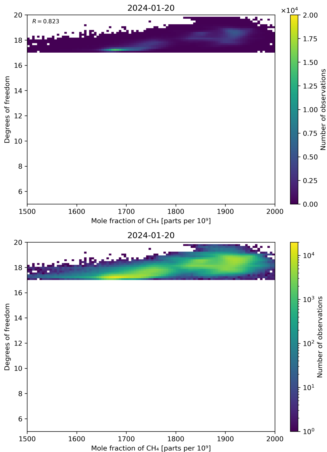
Figure 72: Scatter density plot of “Mole fraction of CH 4 ” against “Degrees of freedom” for 2024-01-19 to 2024-01-21.
