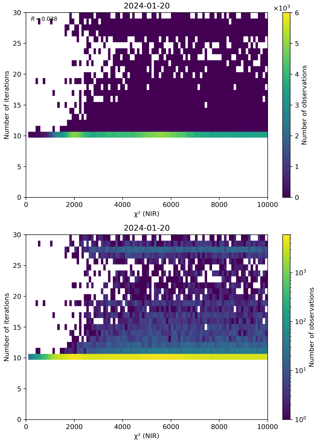
Figure 46: Scatter density plot of “ \chi^2 (NIR)” against “Number of iterations” for 2024-01-19 to 2024-01-21.
