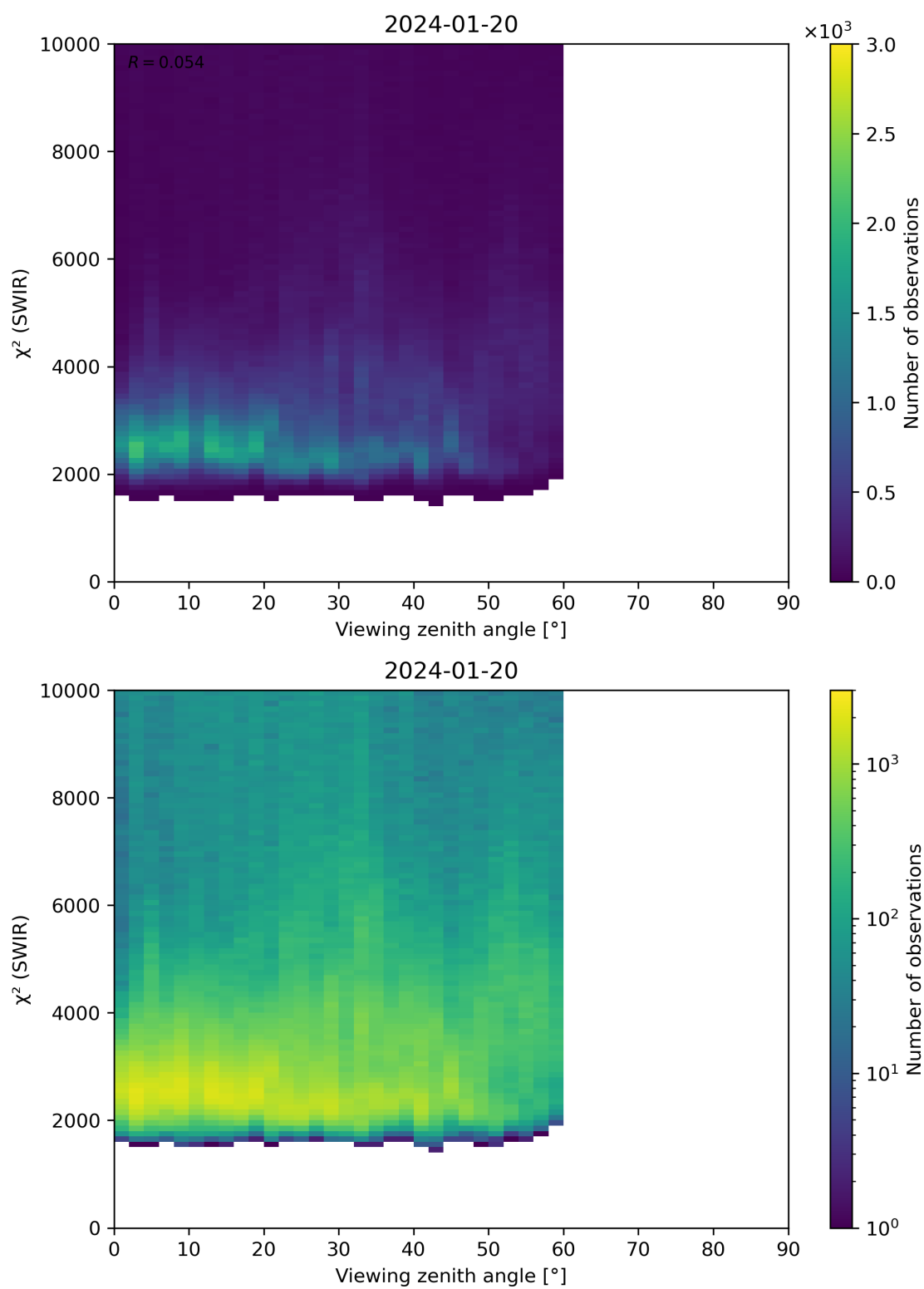
Figure 106: Scatter density plot of “Viewing zenith angle” against “ \chi^2 (SWIR)” for 2024-01-19 to 2024-01-21.
