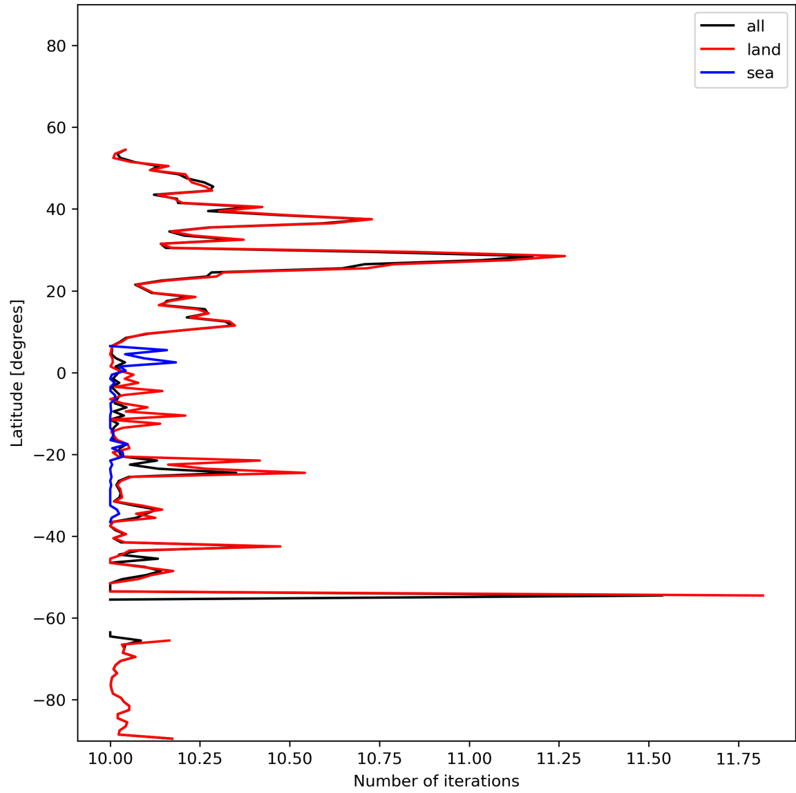
Figure 20: Zonal average of “Number of iterations” for 2024-01-19 to 2024-01-21.
