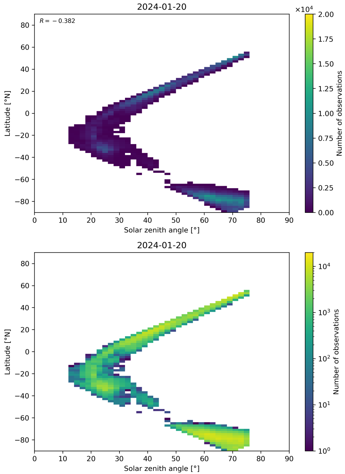
Figure 98: Scatter density plot of “Solar zenith angle” against “Latitude” for 2024-01-19 to 2024-01-21.
