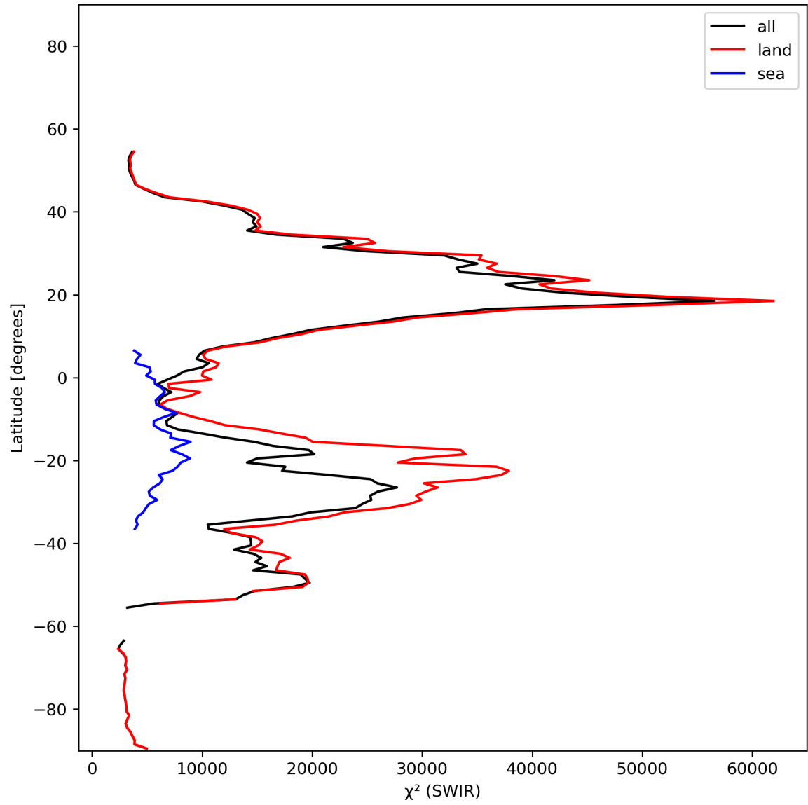
Figure 17: Zonal average of “ \chi^2 (SWIR)” for 2024-01-19 to 2024-01-21.
