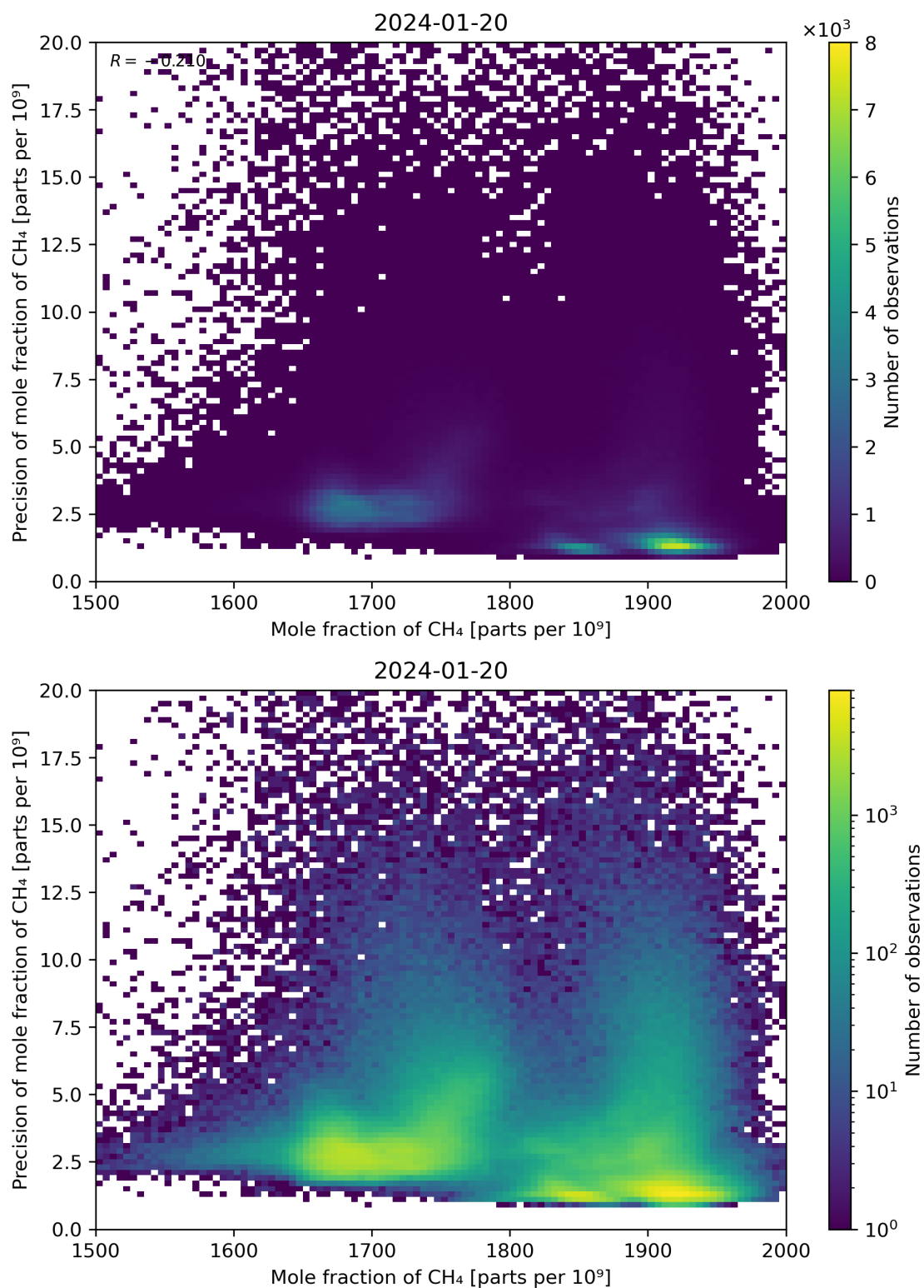
Figure 75: Scatter density plot of “Mole fraction of CH 4 ” against “Precision of mole fraction of CH 4 ” for 2024-01-19 to 2024-01-21.
