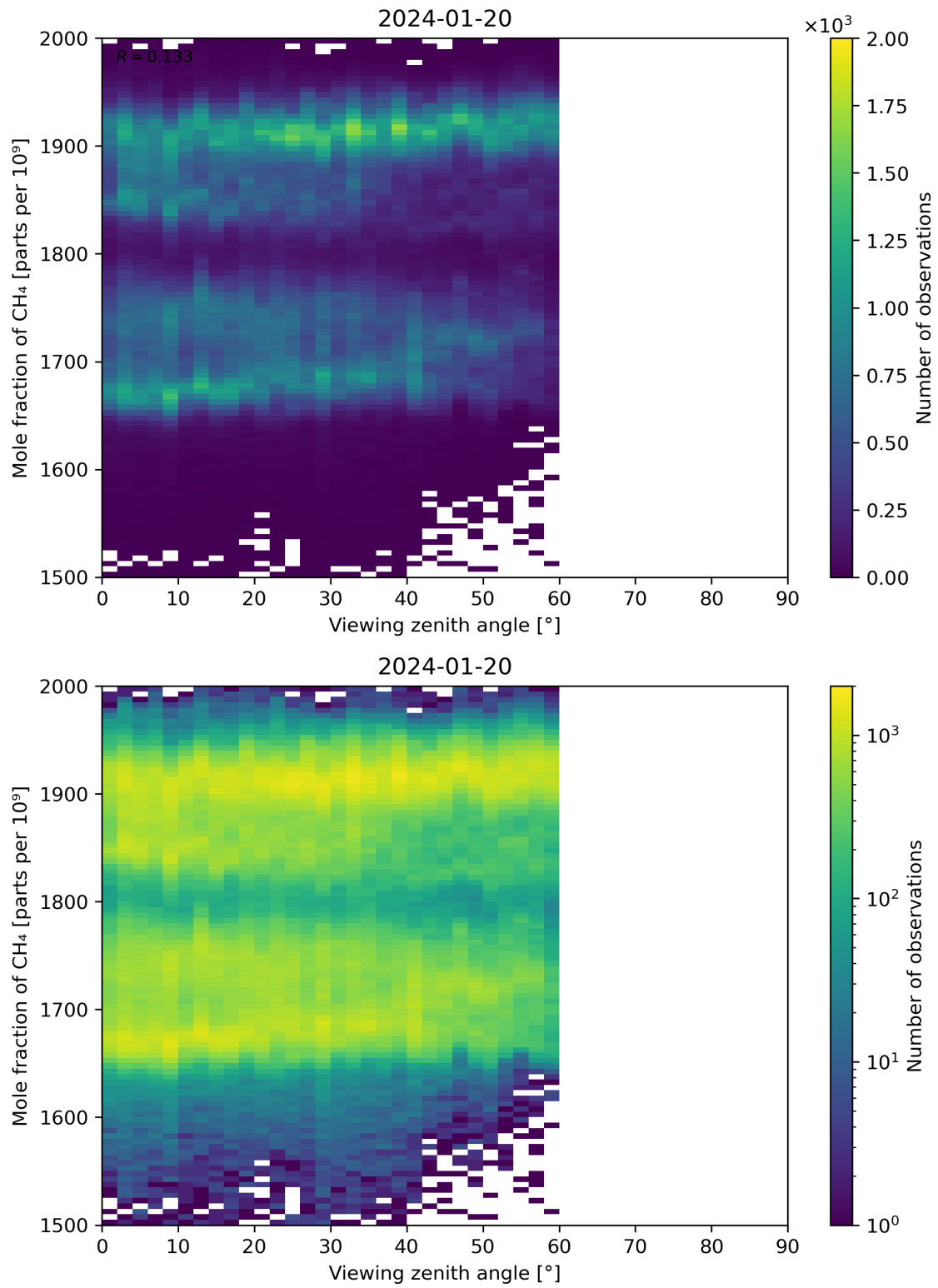
Figure 110: Scatter density plot of “Viewing zenith angle” against “Mole fraction of CH 4 ” for 2024-01-19 to 2024-01-21.
