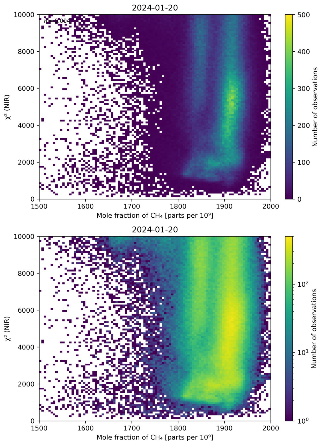
Figure 70: Scatter density plot of “Mole fraction of \text{CH}_4 ” against “ \chi^2 (NIR)” for 2024-01-19 to 2024-01-21.
