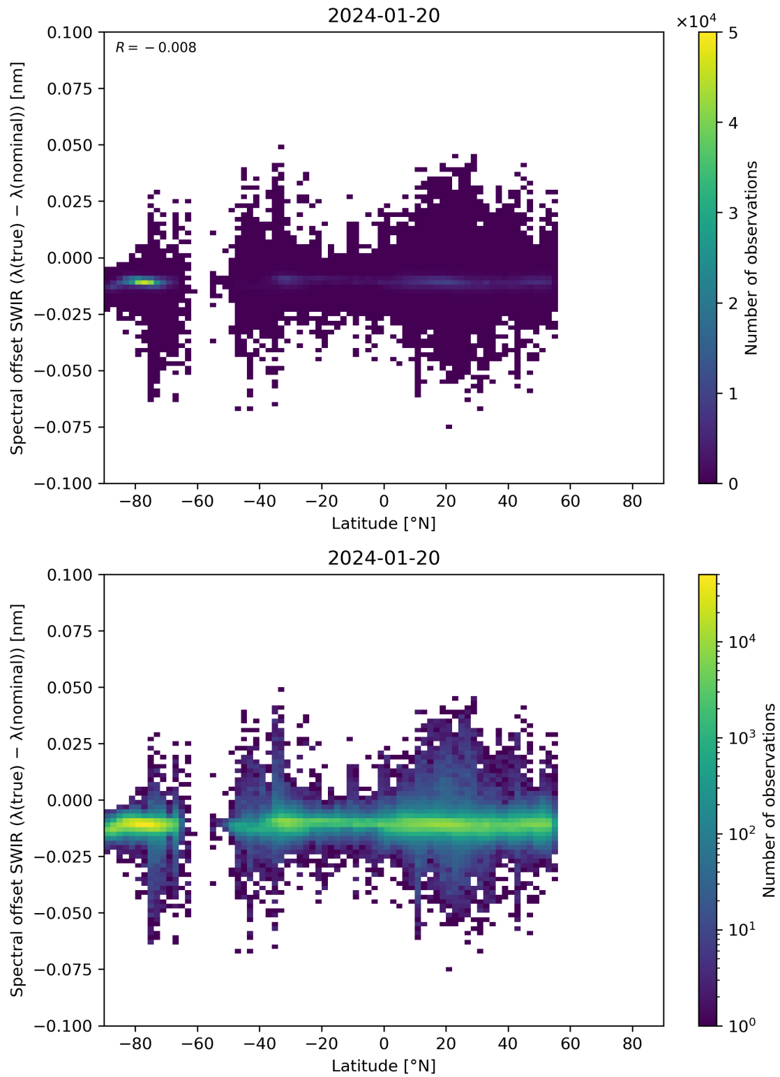
Figure 62: Scatter density plot of “Latitude” against “Spectral offset SWIR ( \lambda(\text{true}) - \lambda(\text{nominal}) )” for 2024-01-19 to 2024-01-21.
