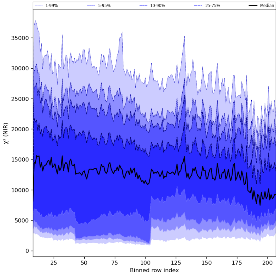
Figure 40: Along track statistics of “ \chi^2 (NIR)” for 2024-01-19 to 2024-01-21
