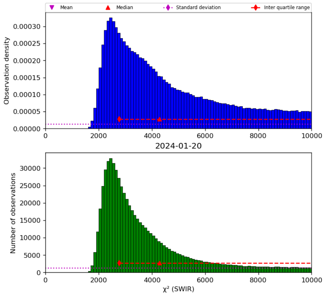
Figure 28: Histogram of “ \chi^2 (SWIR)” for 2024-01-19 to 2024-01-21
