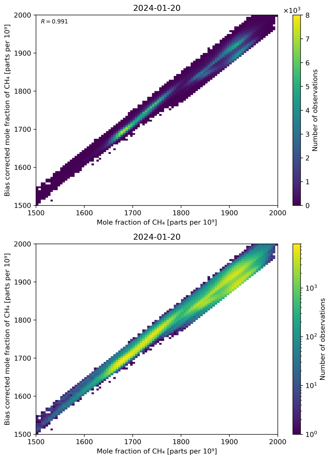
Figure 74: Scatter density plot of “Mole fraction of CH 4 ” against “Bias corrected mole fraction of CH 4 ” for 2024-01-19 to 2024-01-21.
