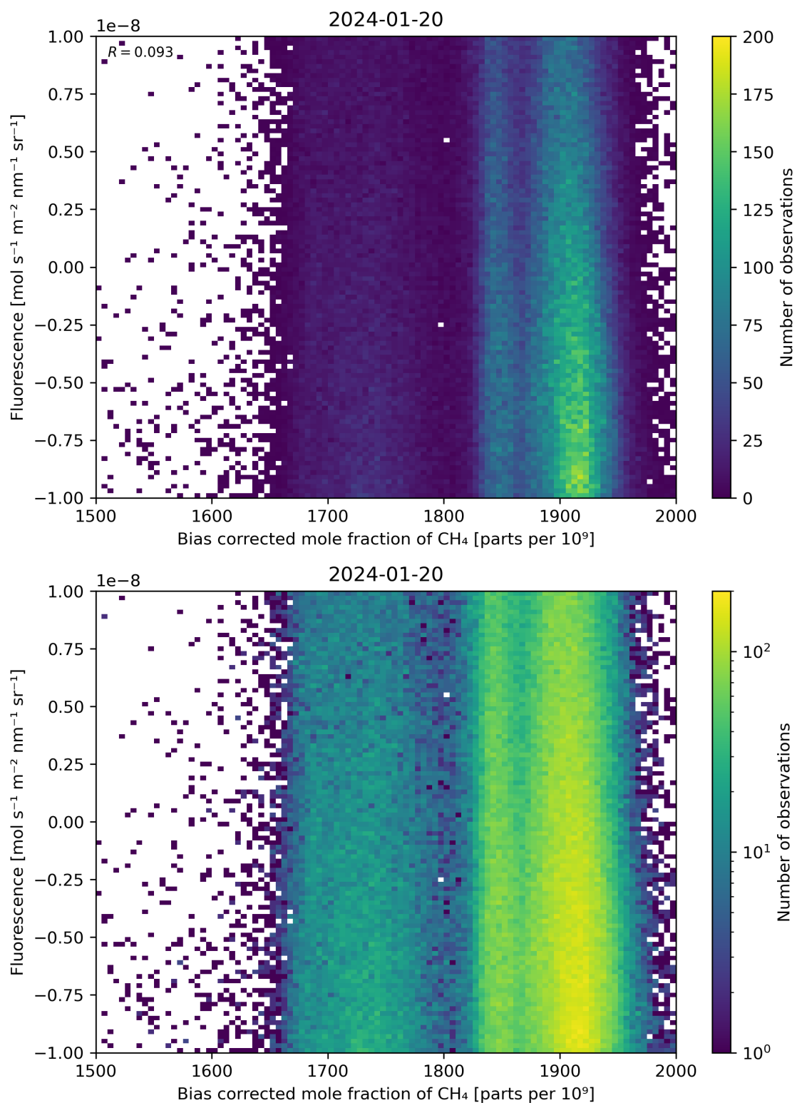
Figure 66: Scatter density plot of “Bias corrected mole fraction of \text{CH}_4 ” against “Fluorescence” for 2024-01-19 to 2024-01-21.
