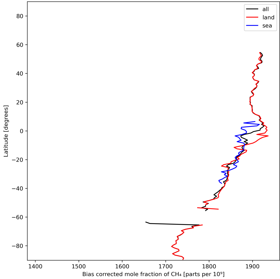
Figure 14: Zonal average of “Bias corrected mole fraction of CH 4 ” for 2024-01-19 to 2024-01-21.
