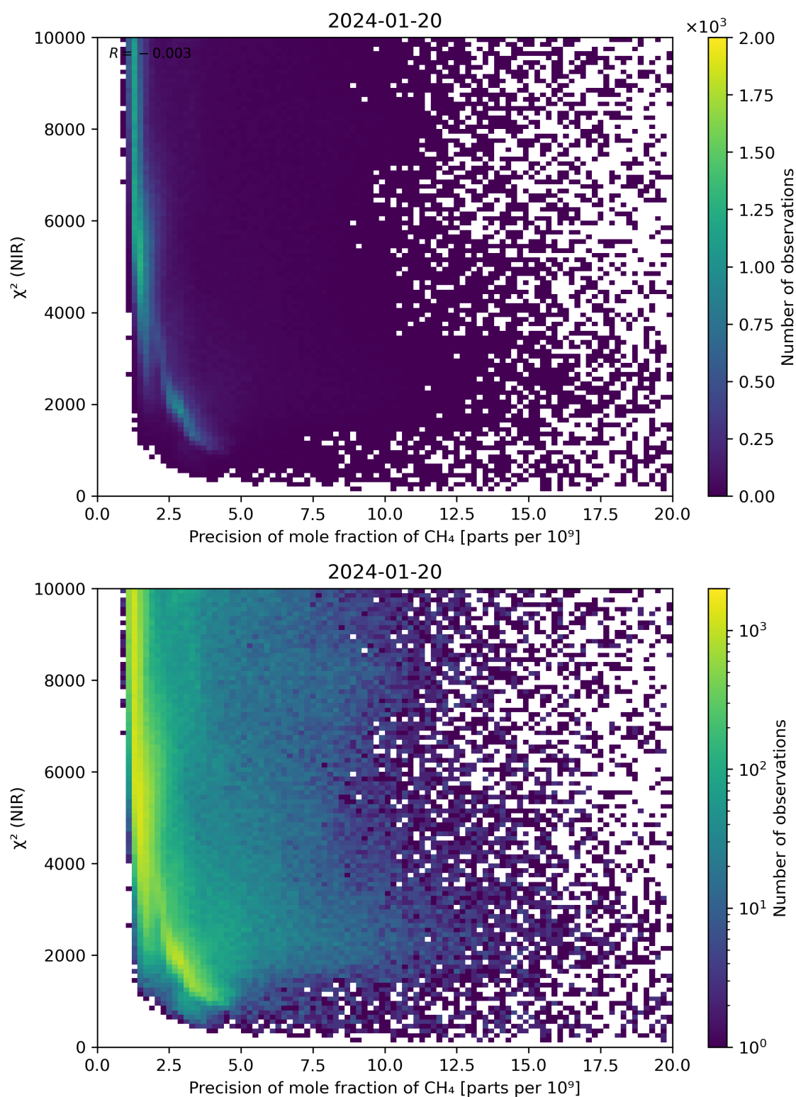
Figure 78: Scatter density plot of “Precision of mole fraction of CH 4 ” against “ \chi^2 (NIR)” for 2024-01-19 to 2024-01-21.
