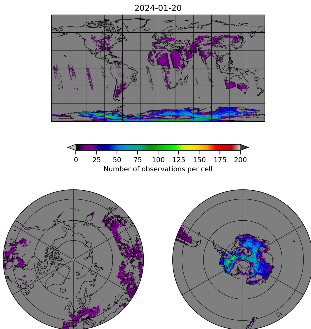
Figure 10: Map of the number of observations for 2024-01-19 to 2024-01-21
