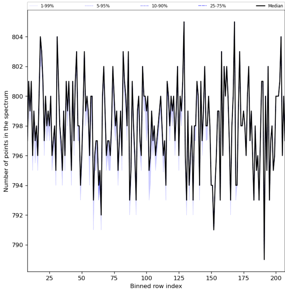
Figure 37: Along track statistics of “Number of points in the spectrum” for 2024-01-19 to 2024-01-21
