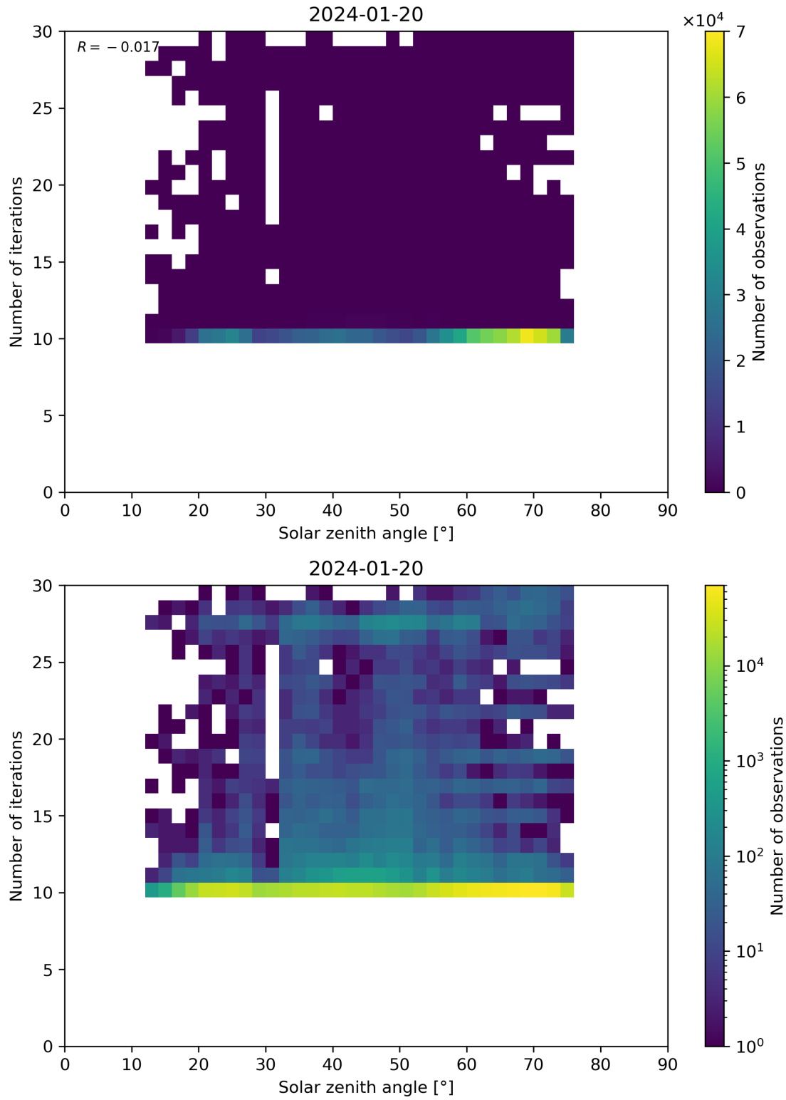
Figure 102: Scatter density plot of “Solar zenith angle” against “Number of iterations” for 2024-01-19 to 2024-01-21.
