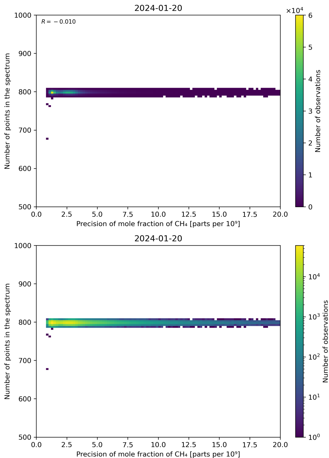
Figure 84: Scatter density plot of “Precision of mole fraction of CH 4 ” against “Number of points in the spectrum” for 2024-01-19 to 2024-01-21.
