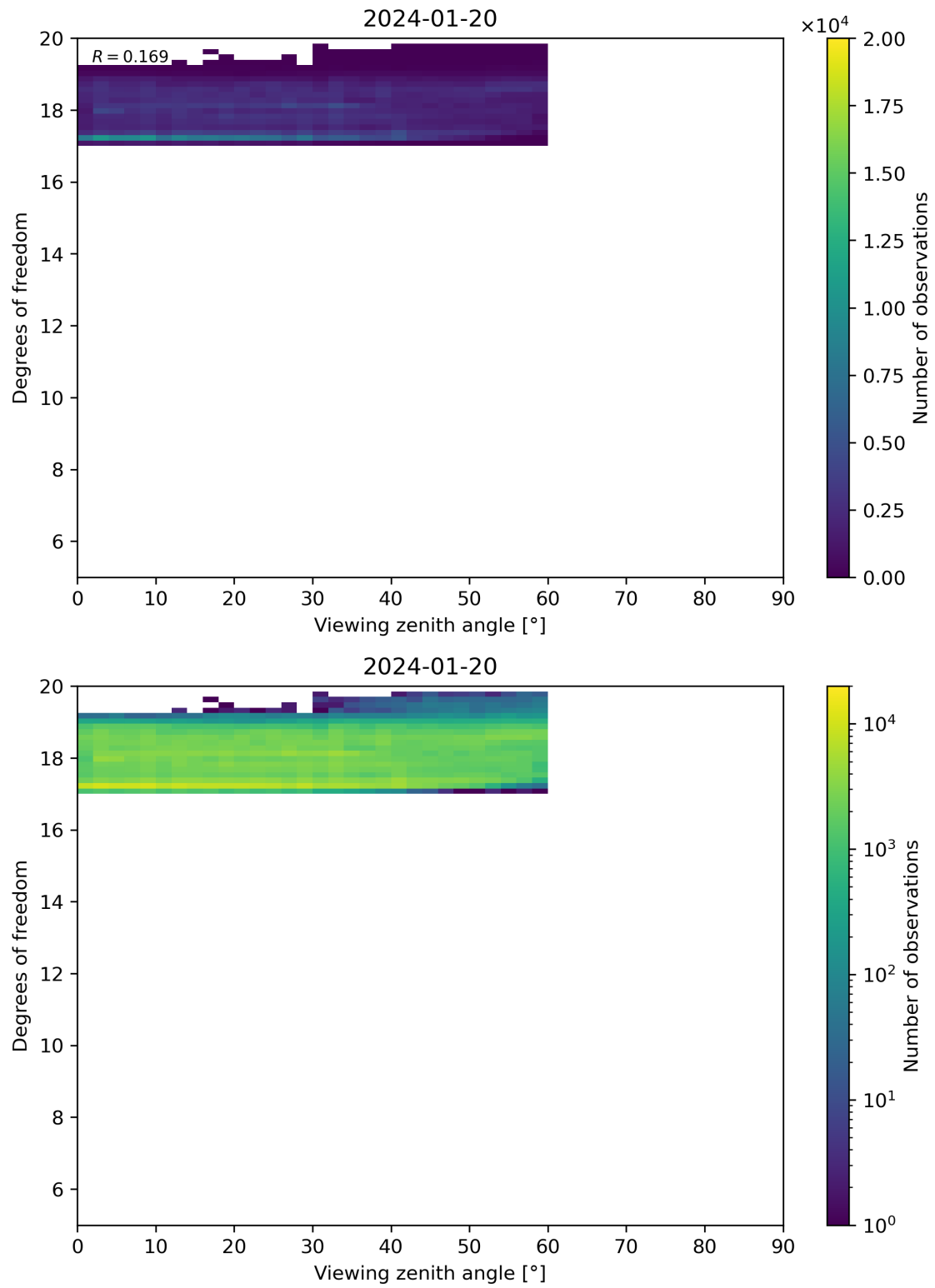
Figure 107: Scatter density plot of “Viewing zenith angle” against “Degrees of freedom” for 2024-01-19 to 2024-01-21.
