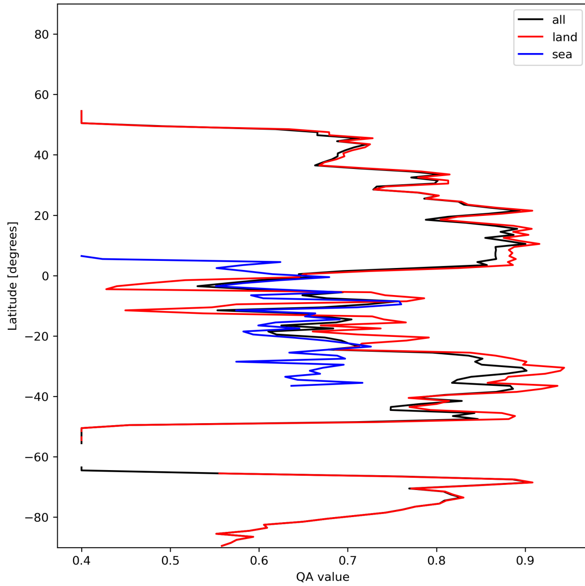
Figure 11: Zonal average of “QA value” for 2024-01-19 to 2024-01-21.
