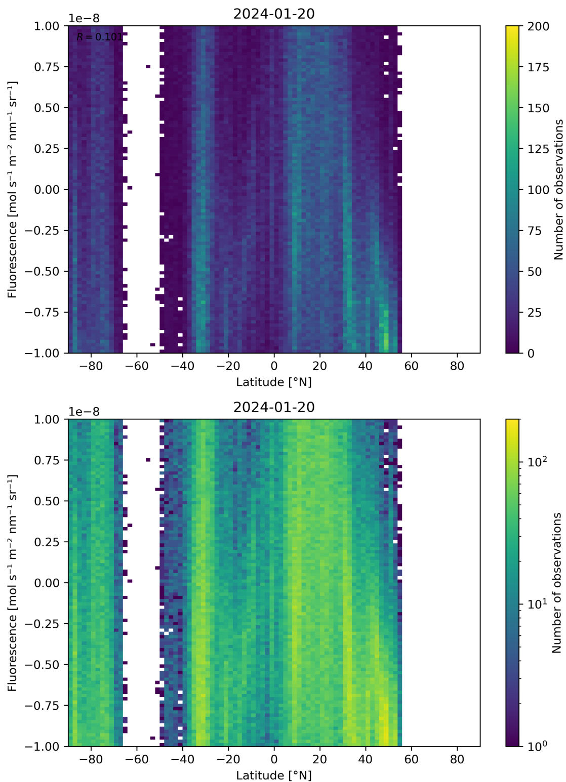
Figure 56: Scatter density plot of “Latitude” against “Fluorescence” for 2024-01-19 to 2024-01-21.
