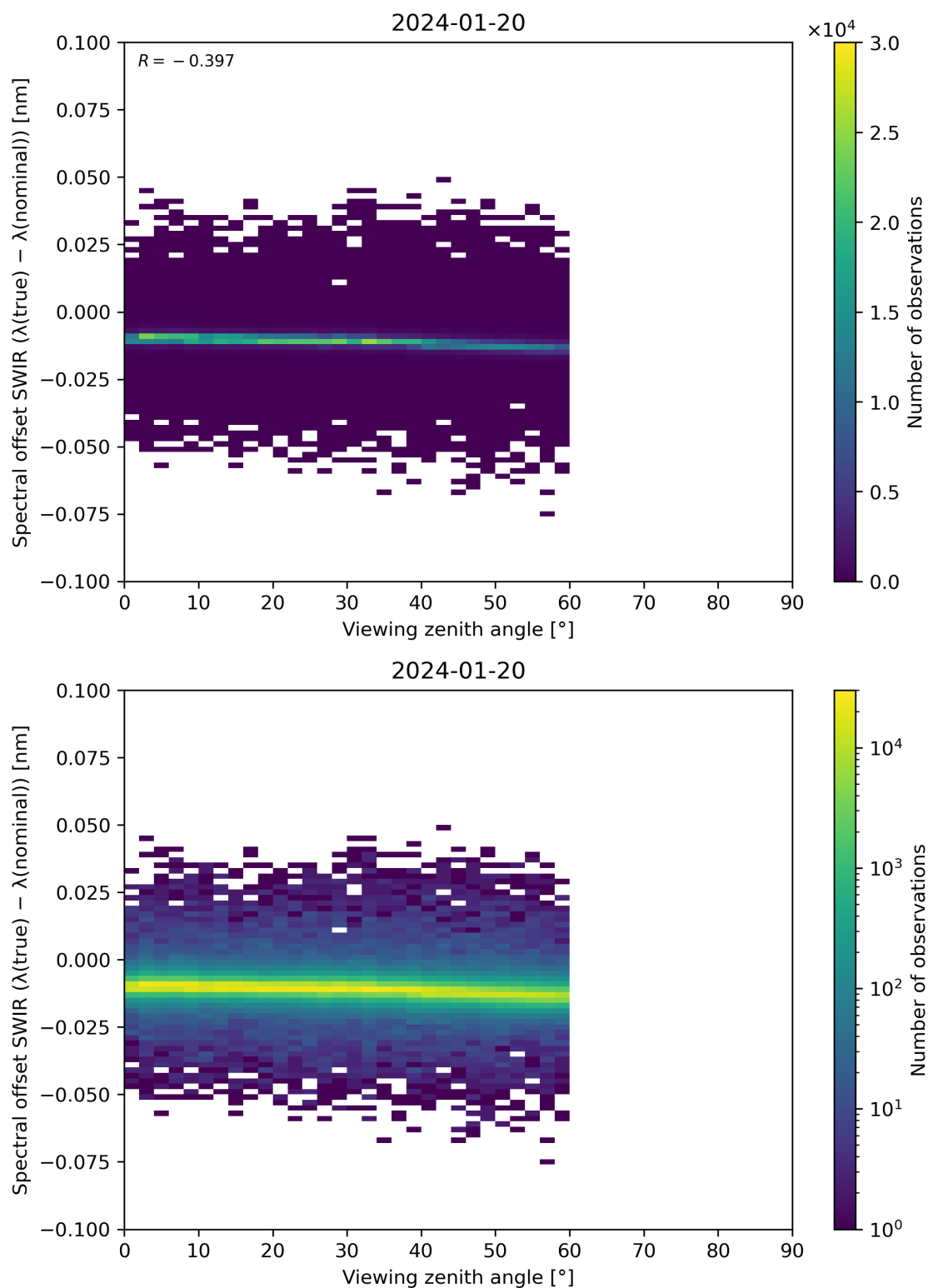
Figure 116: Scatter density plot of “Viewing zenith angle” against “Spectral offset SWIR ( \lambda(\text{true}) - \lambda(\text{nominal}) )” for 2024-01-19 to 2024-01-21.
