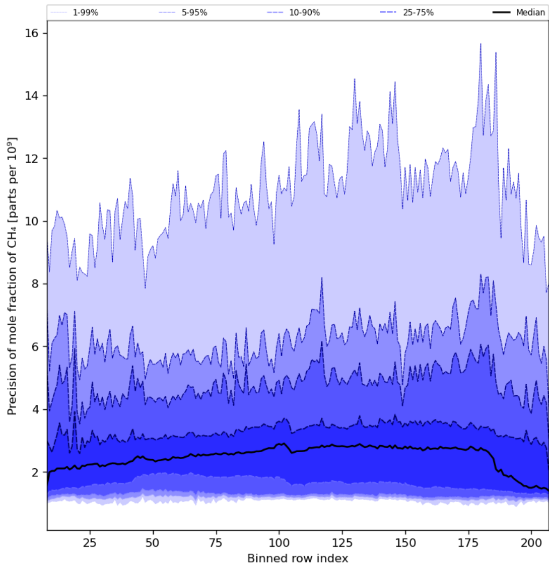
Figure 35: Along track statistics of “Precision of mole fraction of CH 4 ” for 2024-01-19 to 2024-01-21
