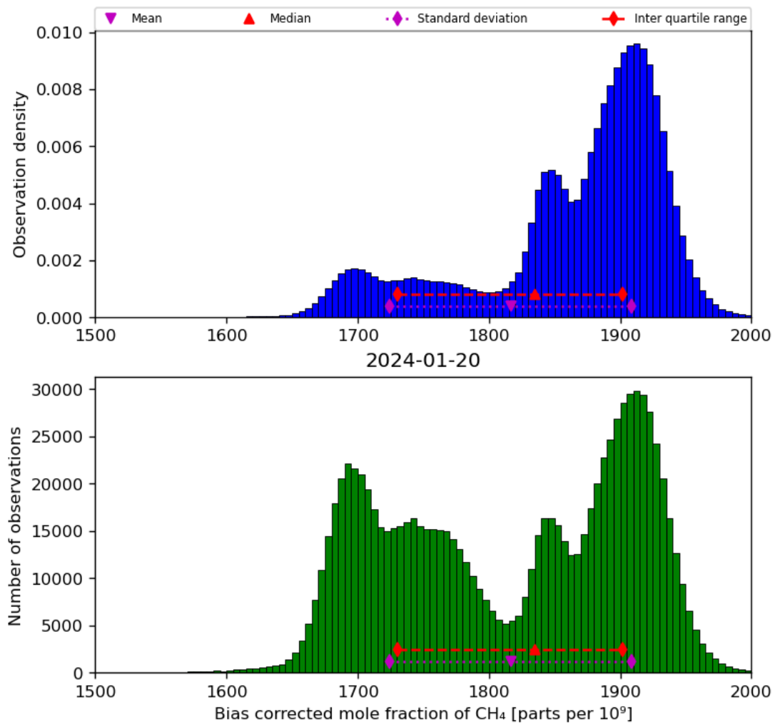
Figure 25: Histogram of “Bias corrected mole fraction of CH 4 ” for 2024-01-19 to 2024-01-21
