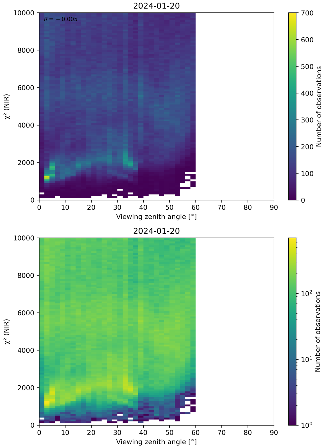
Figure 105: Scatter density plot of “Viewing zenith angle” against “ \chi^2 (NIR)” for 2024-01-19 to 2024-01-21.
