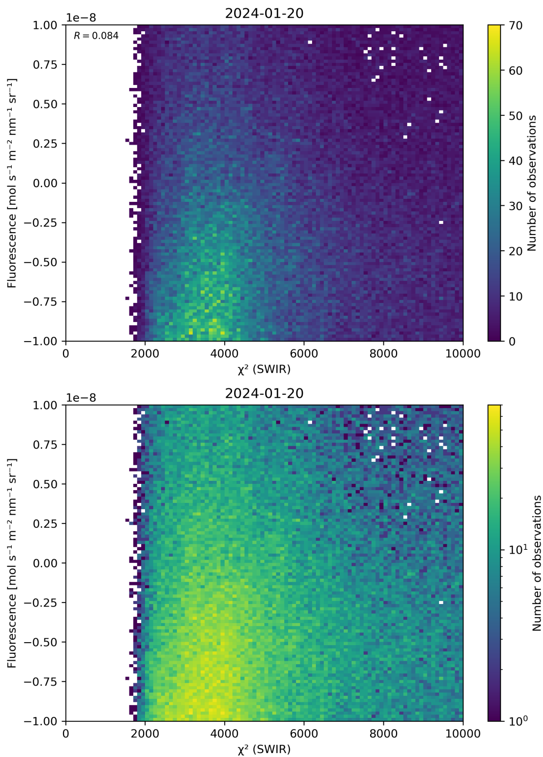
Figure 49: Scatter density plot of “ \chi^2 (SWIR)” against “Fluorescence” for 2024-01-19 to 2024-01-21.
