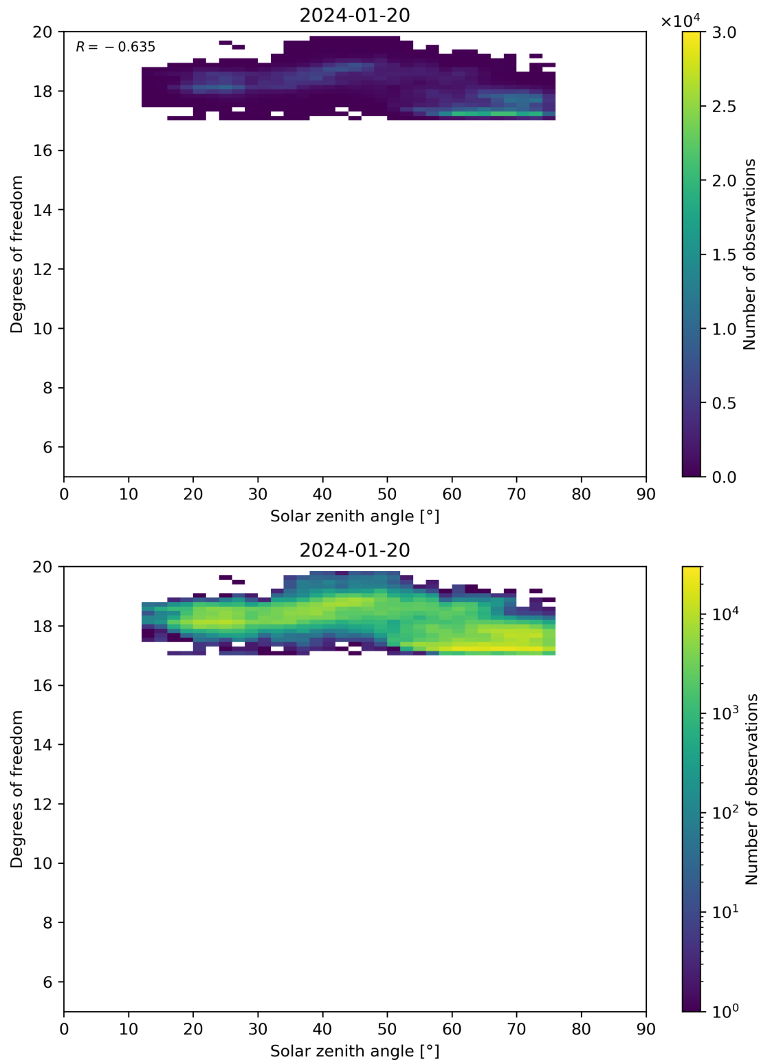
Figure 96: Scatter density plot of “Solar zenith angle” against “Degrees of freedom” for 2024-01-19 to 2024-01-21.
