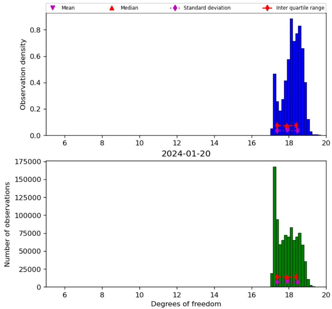
Figure 30: Histogram of “Degrees of freedom” for 2024-01-19 to 2024-01-21
