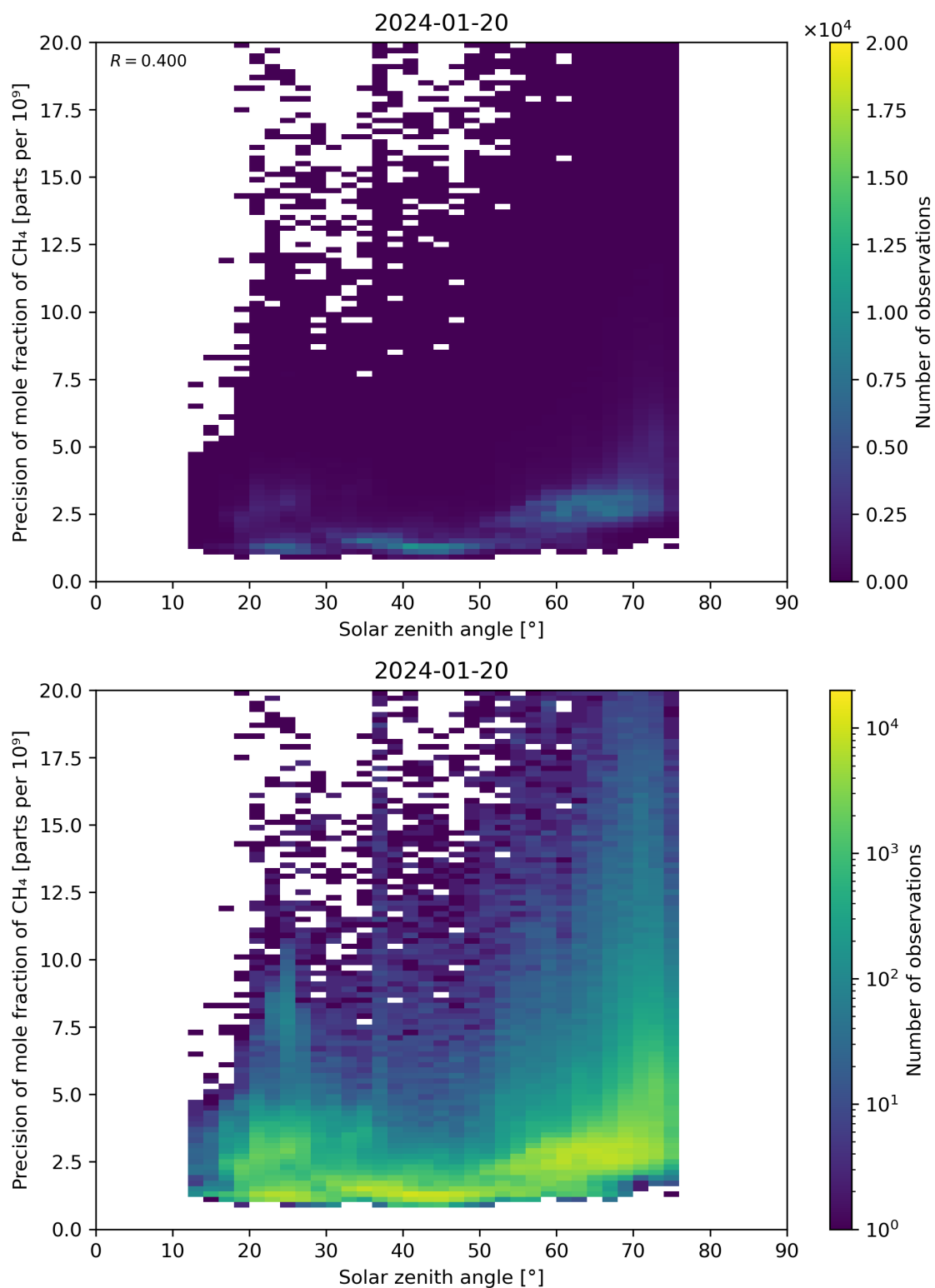
Figure 101: Scatter density plot of “Solar zenith angle” against “Precision of mole fraction of \text{CH}_4 ” for 2024-01-19 to 2024-01-21.
