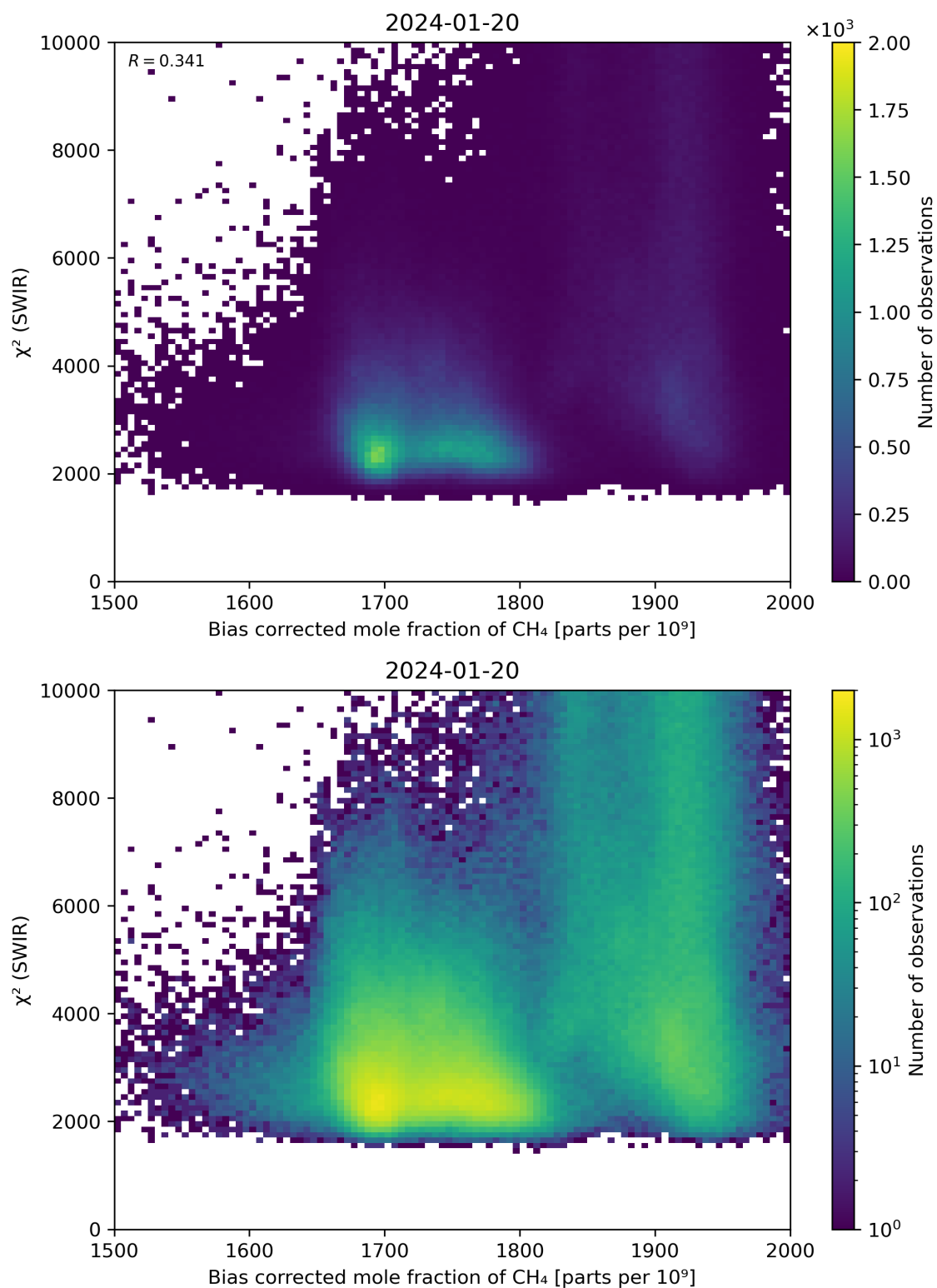
Figure 64: Scatter density plot of “Bias corrected mole fraction of CH 4 ” against “ \chi^2 (SWIR)” for 2024-01-19 to 2024-01-21.
