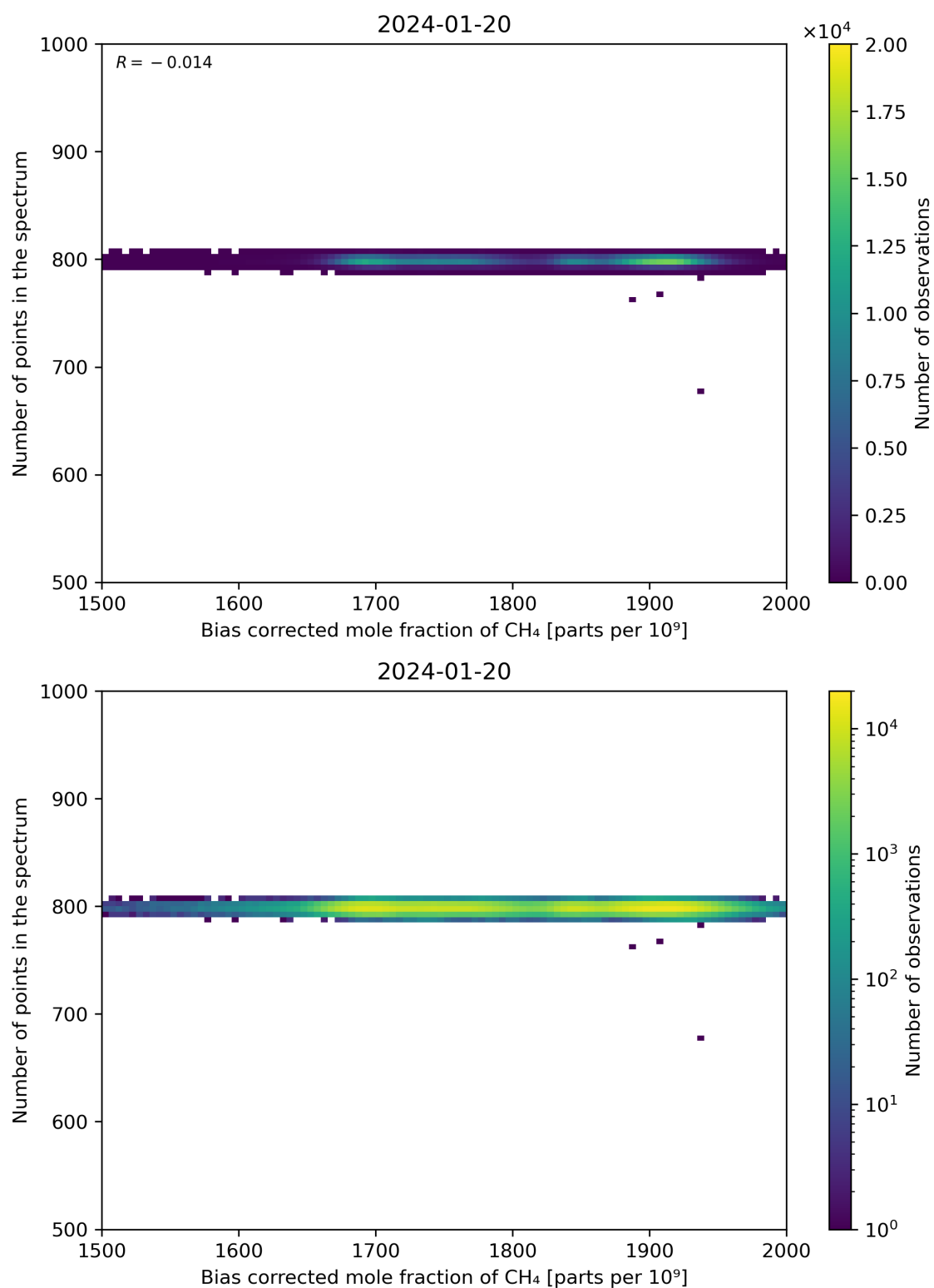
Figure 68: Scatter density plot of “Bias corrected mole fraction of CH 4 ” against “Number of points in the spectrum” for 2024-01-19 to 2024-01-21.
