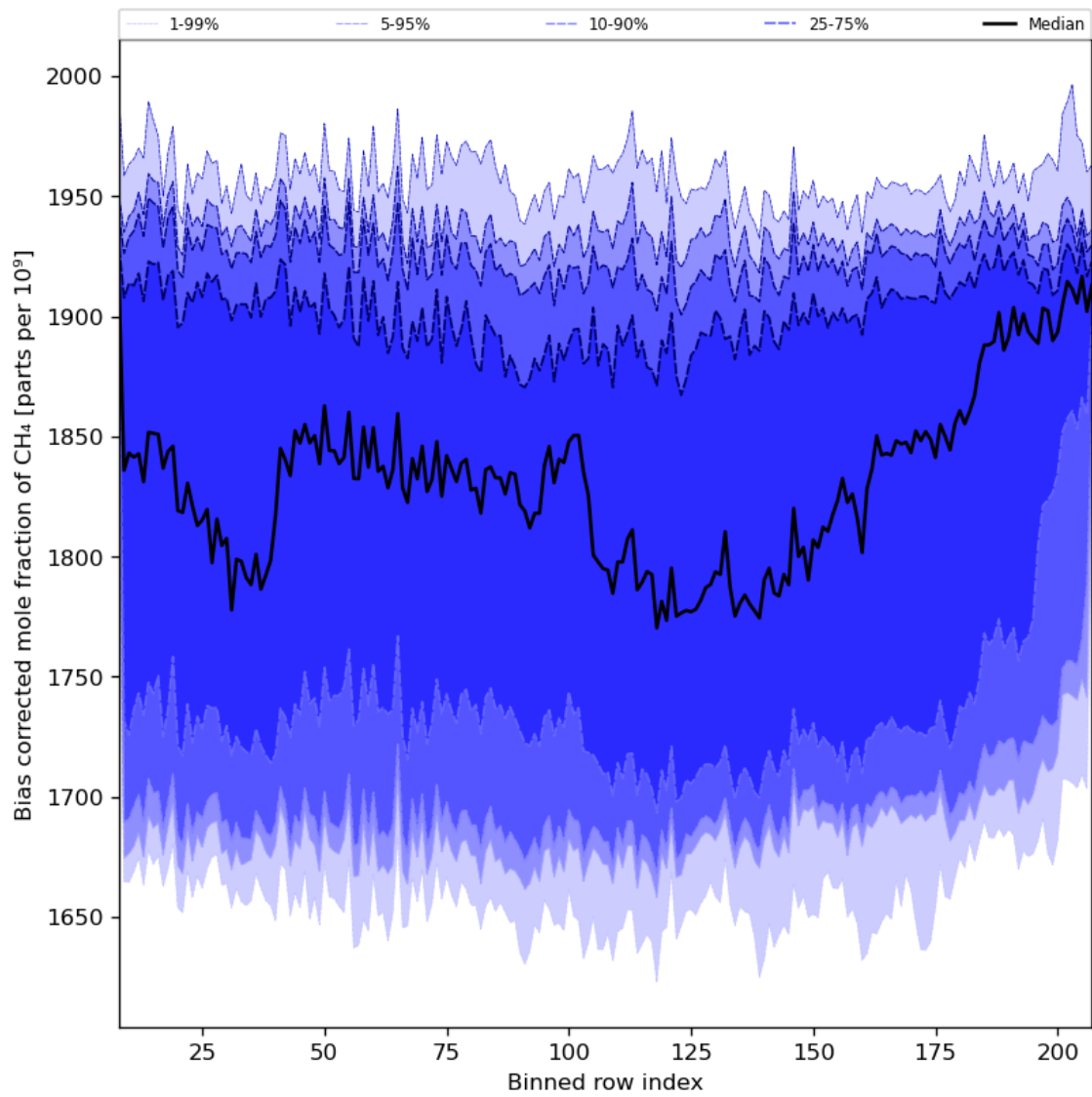
Figure 36: Along track statistics of “Bias corrected mole fraction of CH 4 ” for 2024-01-19 to 2024-01-21
