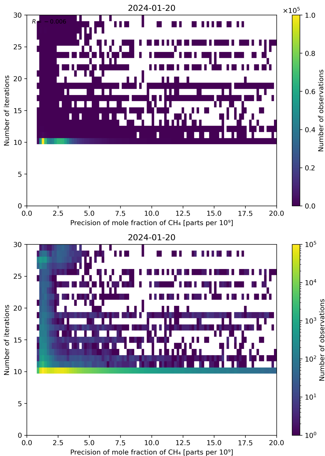
Figure 83: Scatter density plot of “Precision of mole fraction of CH 4 ” against “Number of iterations” for 2024-01-19 to 2024-01-21.
