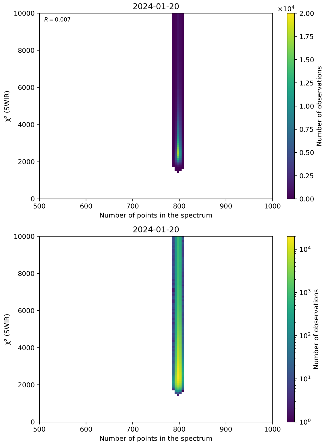
Figure 89: Scatter density plot of “Number of points in the spectrum” against “ \chi^2 (SWIR)” for 2024-01-19 to 2024-01-21.
