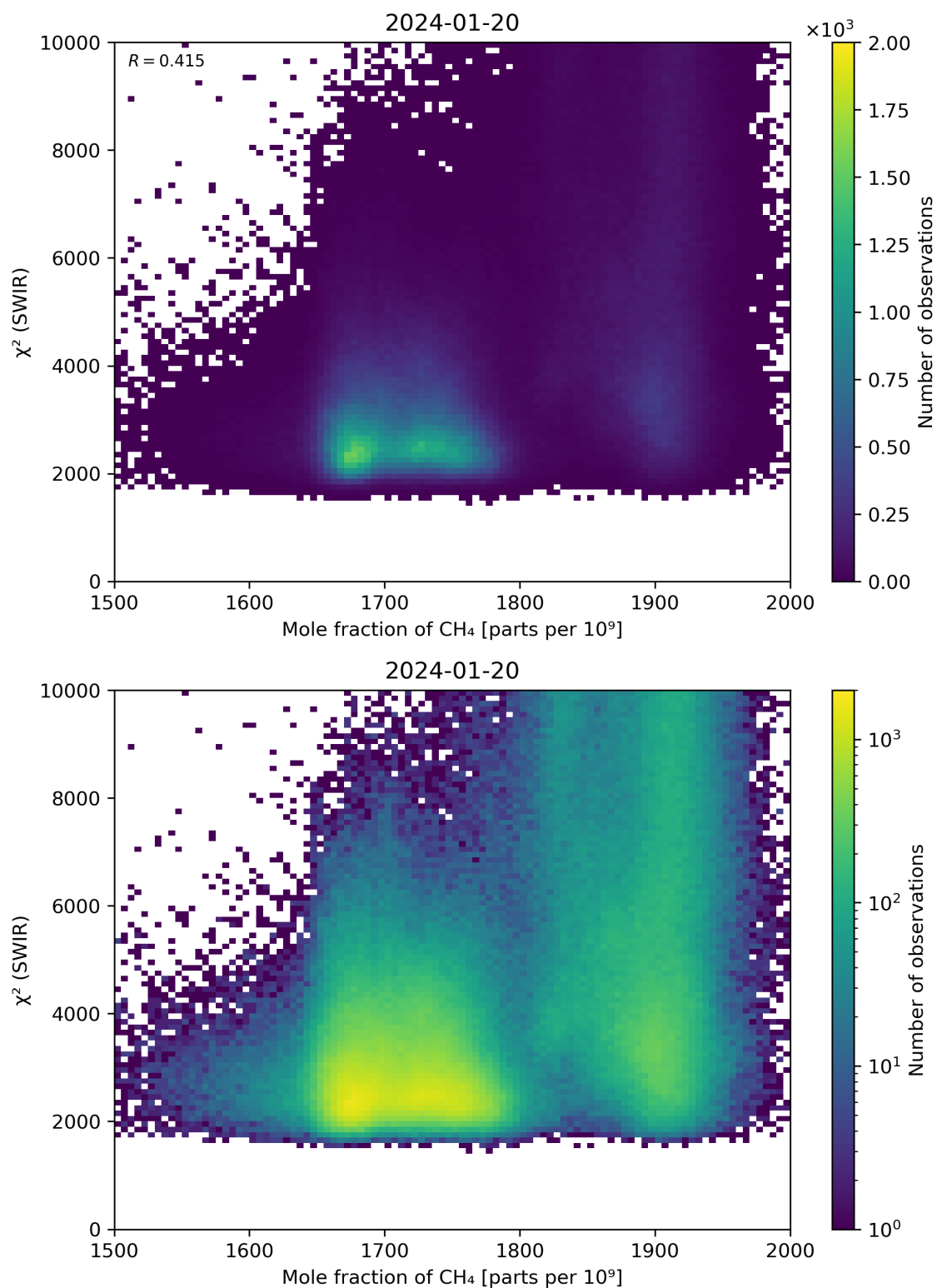
Figure 71: Scatter density plot of “Mole fraction of \text{CH}_4 ” against “ \chi^2 (SWIR)” for 2024-01-19 to 2024-01-21.
