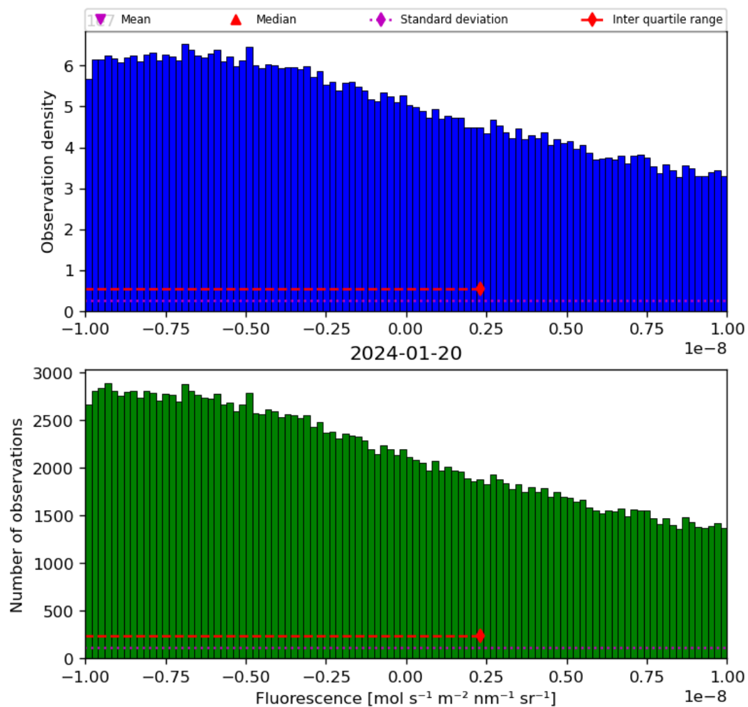
Figure 32: Histogram of “Fluorescence” for 2024-01-19 to 2024-01-21
