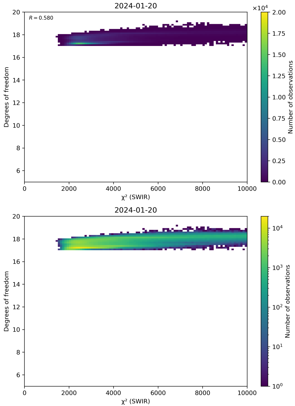
Figure 48: Scatter density plot of “ \chi^2 (SWIR)” against “Degrees of freedom” for 2024-01-19 to 2024-01-21.
