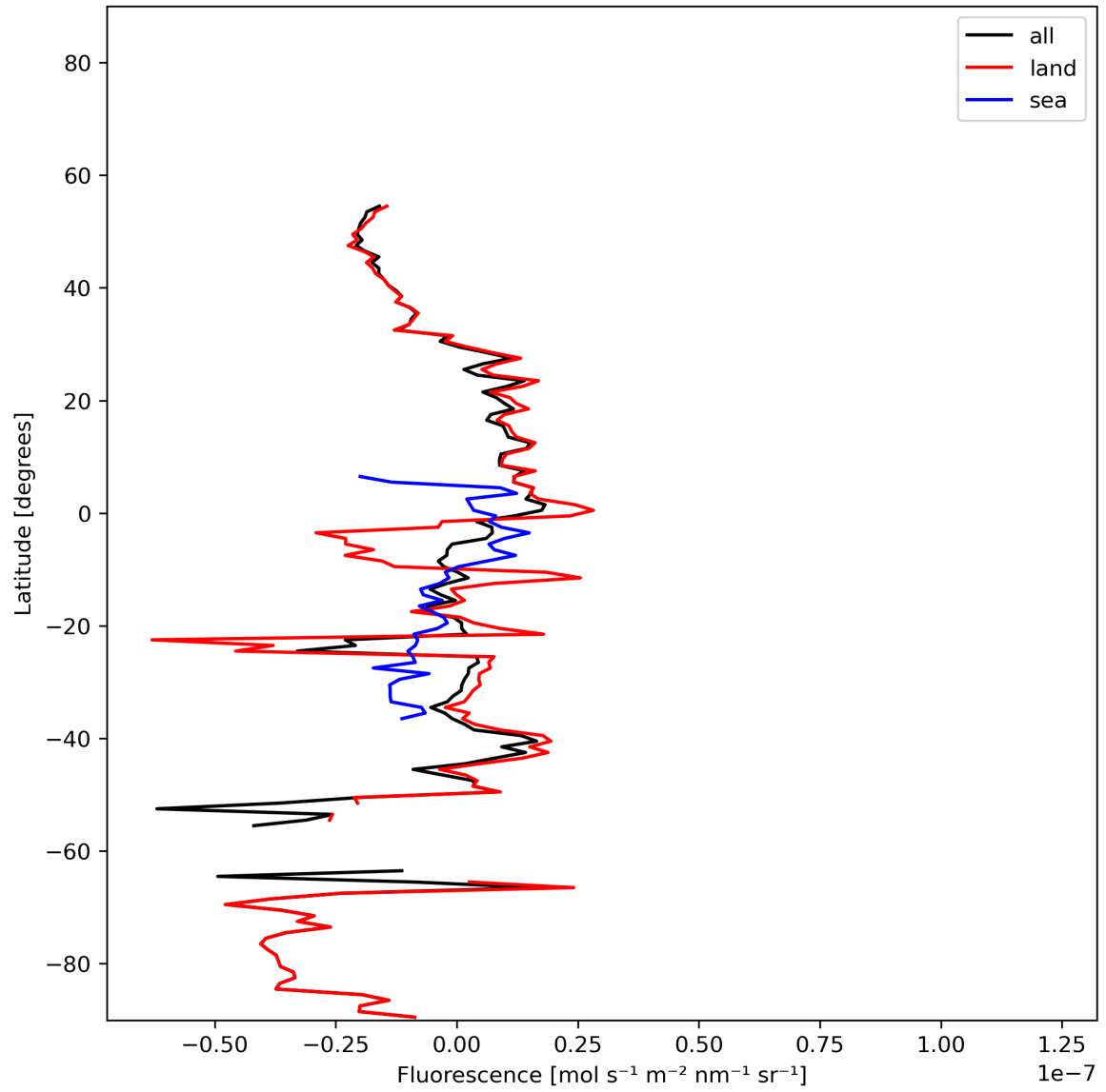
Figure 21: Zonal average of “Fluorescence” for 2024-01-19 to 2024-01-21.
