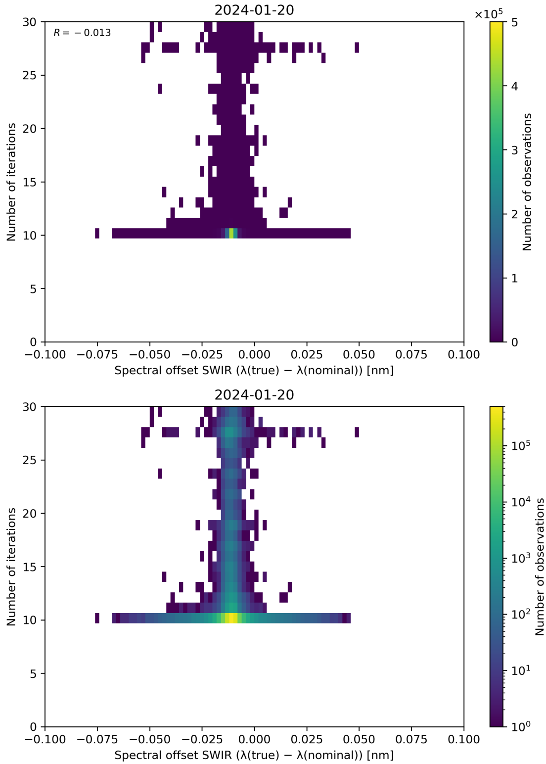
Figure 121: Scatter density plot of “Spectral offset SWIR ( \lambda(\text{true}) - \lambda(\text{nominal}) )” against “Number of iterations” for 2024-01-19 to 2024-01-21.
