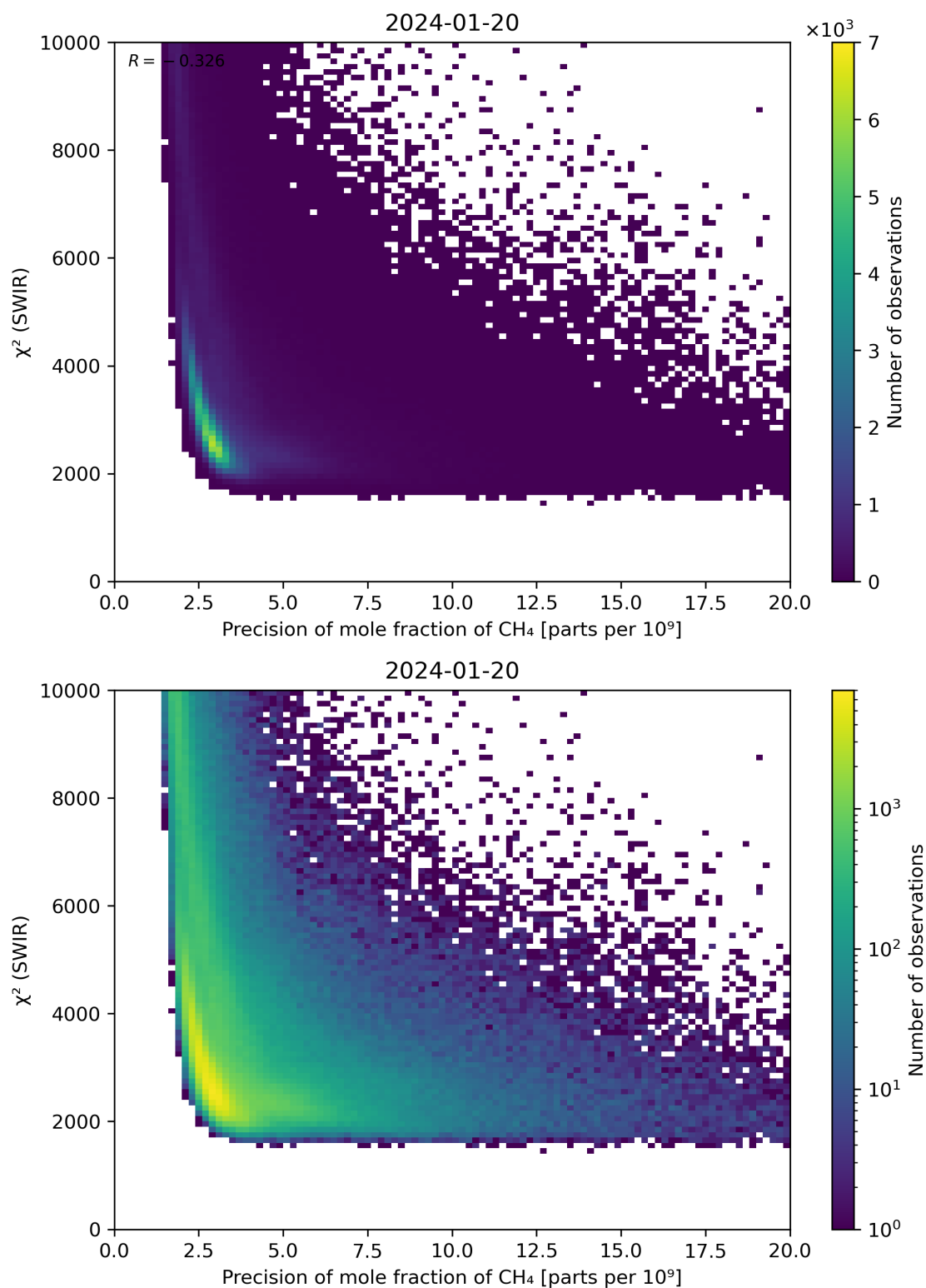
Figure 79: Scatter density plot of “Precision of mole fraction of \text{CH}_4 ” against “ \chi^2 (SWIR)” for 2024-01-19 to 2024-01-21.
