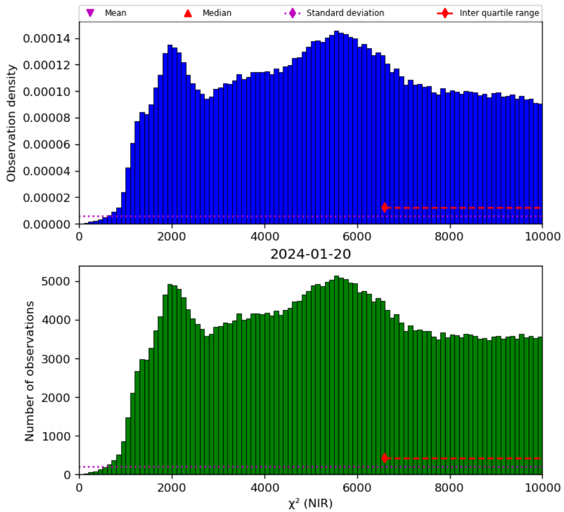
Figure 29: Histogram of “ \chi^2 (NIR)” for 2024-01-19 to 2024-01-21
