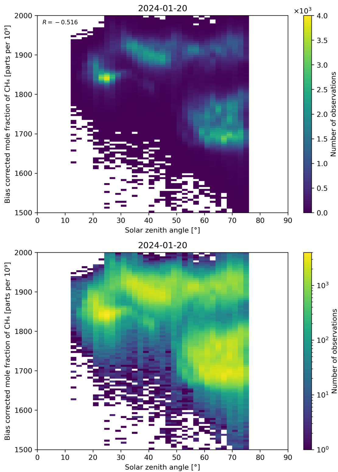
Figure 100: Scatter density plot of “Solar zenith angle” against “Bias corrected mole fraction of \text{CH}_4 ” for 2024-01-19 to 2024-01-21.
