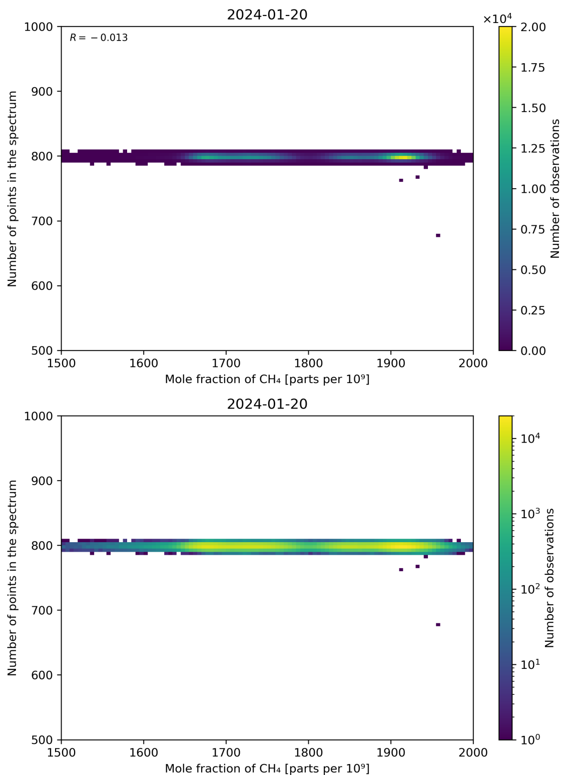
Figure 77: Scatter density plot of “Mole fraction of CH 4 ” against “Number of points in the spectrum” for 2024-01-19 to 2024-01-21.
