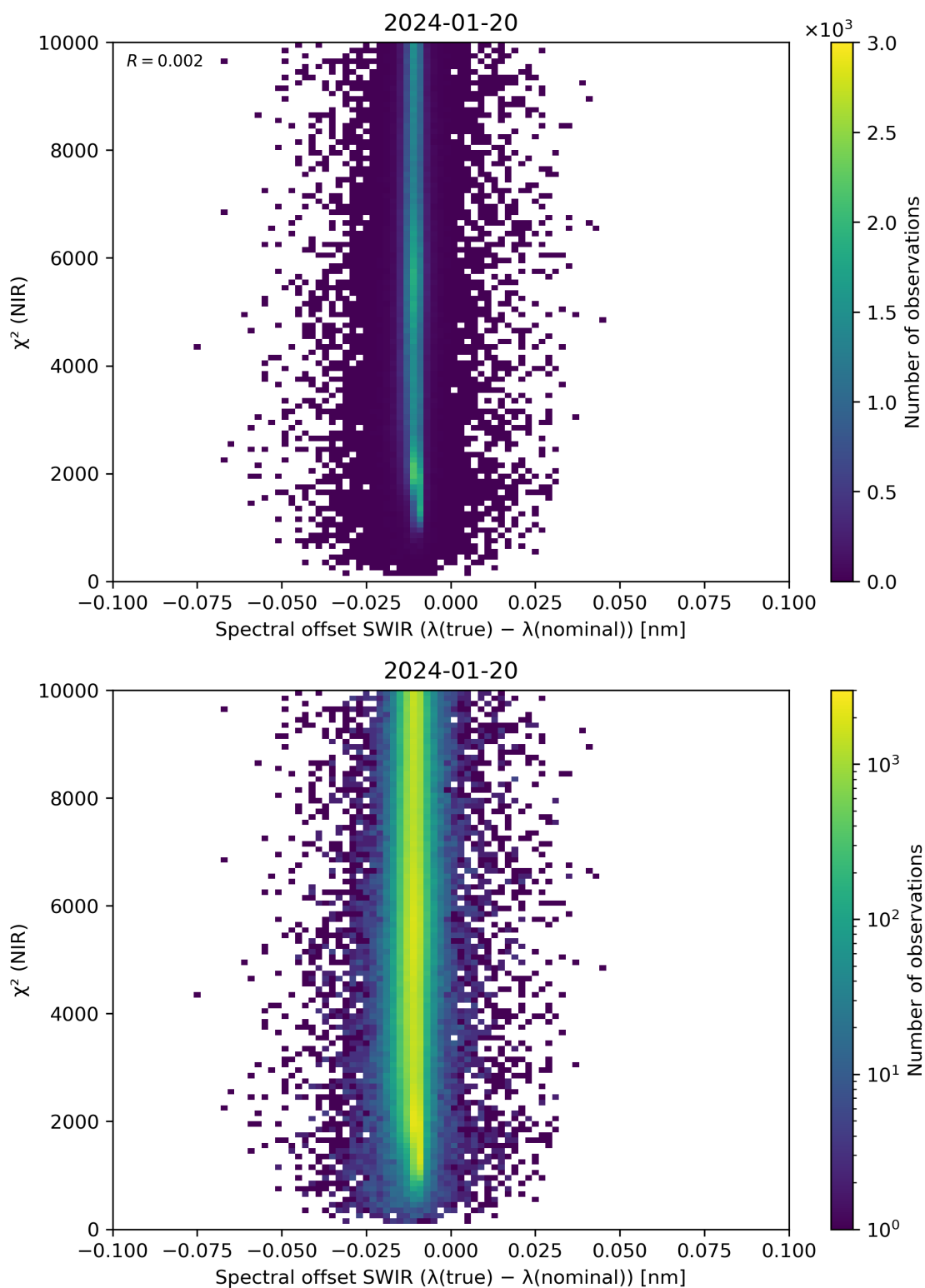
Figure 117: Scatter density plot of “Spectral offset SWIR ( \lambda(\text{true}) - \lambda(\text{nominal}) )” against “ \chi^2 (NIR)” for 2024-01-19 to 2024-01-21.
