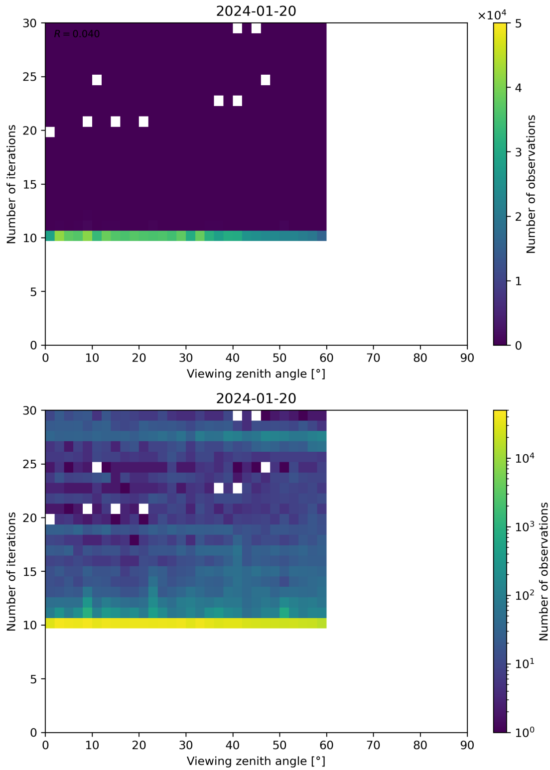
Figure 113: Scatter density plot of “Viewing zenith angle” against “Number of iterations” for 2024-01-19 to 2024-01-21.
