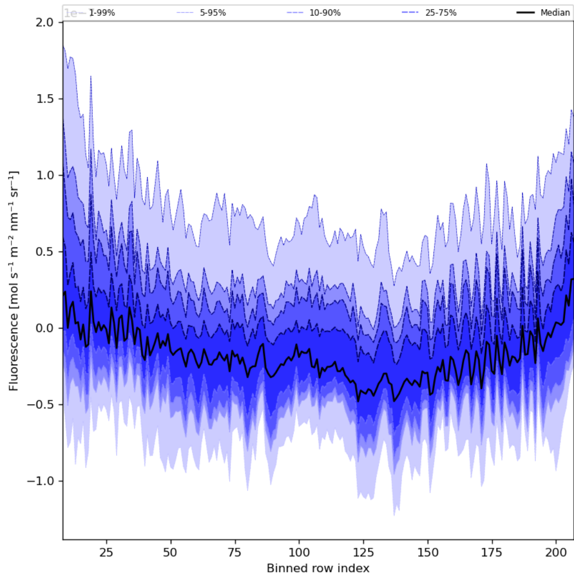
Figure 43: Along track statistics of “Fluorescence” for 2024-01-19 to 2024-01-21
