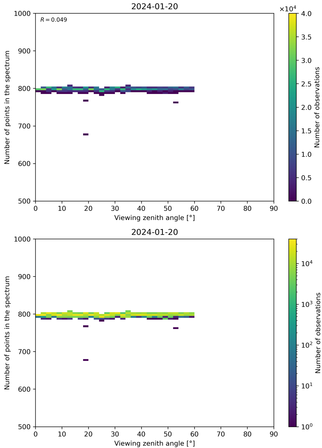
Figure 114: Scatter density plot of “Viewing zenith angle” against “Number of points in the spectrum” for 2024-01-19 to 2024-01-21.
