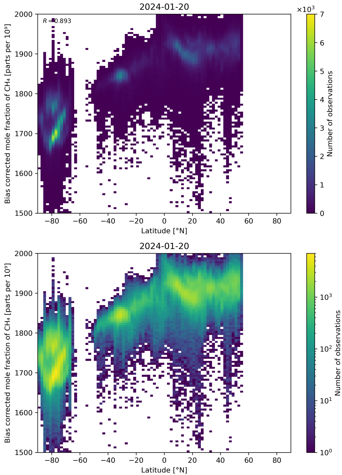
Figure 58: Scatter density plot of “Latitude” against “Bias corrected mole fraction of CH 4 ” for 2024-01-19 to 2024-01-21.
