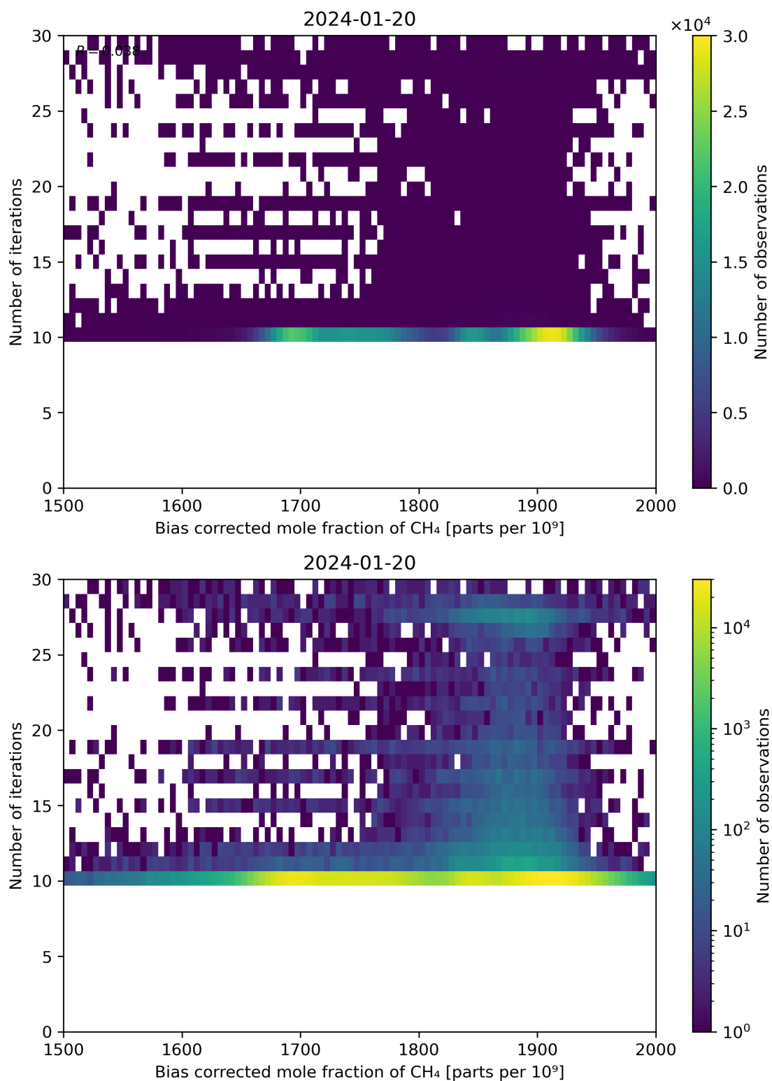
Figure 67: Scatter density plot of “Bias corrected mole fraction of \text{CH}_4 ” against “Number of iterations” for 2024-01-19 to 2024-01-21.
