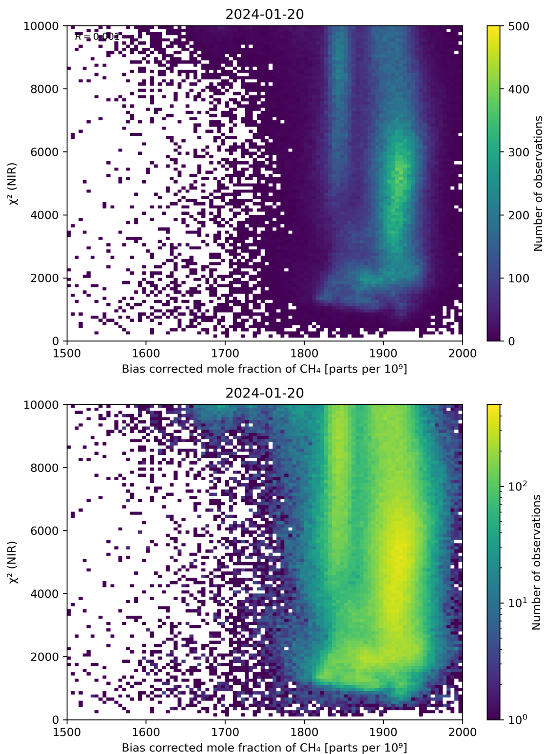
Figure 63: Scatter density plot of “Bias corrected mole fraction of CH 4 ” against “ \chi^2 (NIR)” for 2024-01-19 to 2024-01-21.
