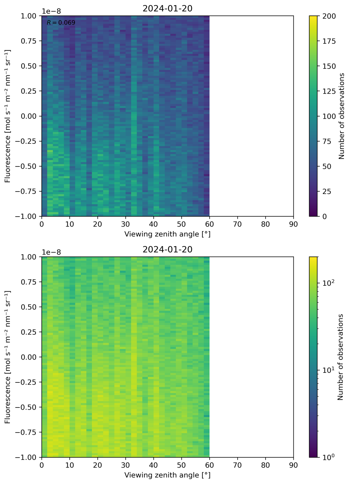
Figure 108: Scatter density plot of “Viewing zenith angle” against “Fluorescence” for 2024-01-19 to 2024-01-21.
