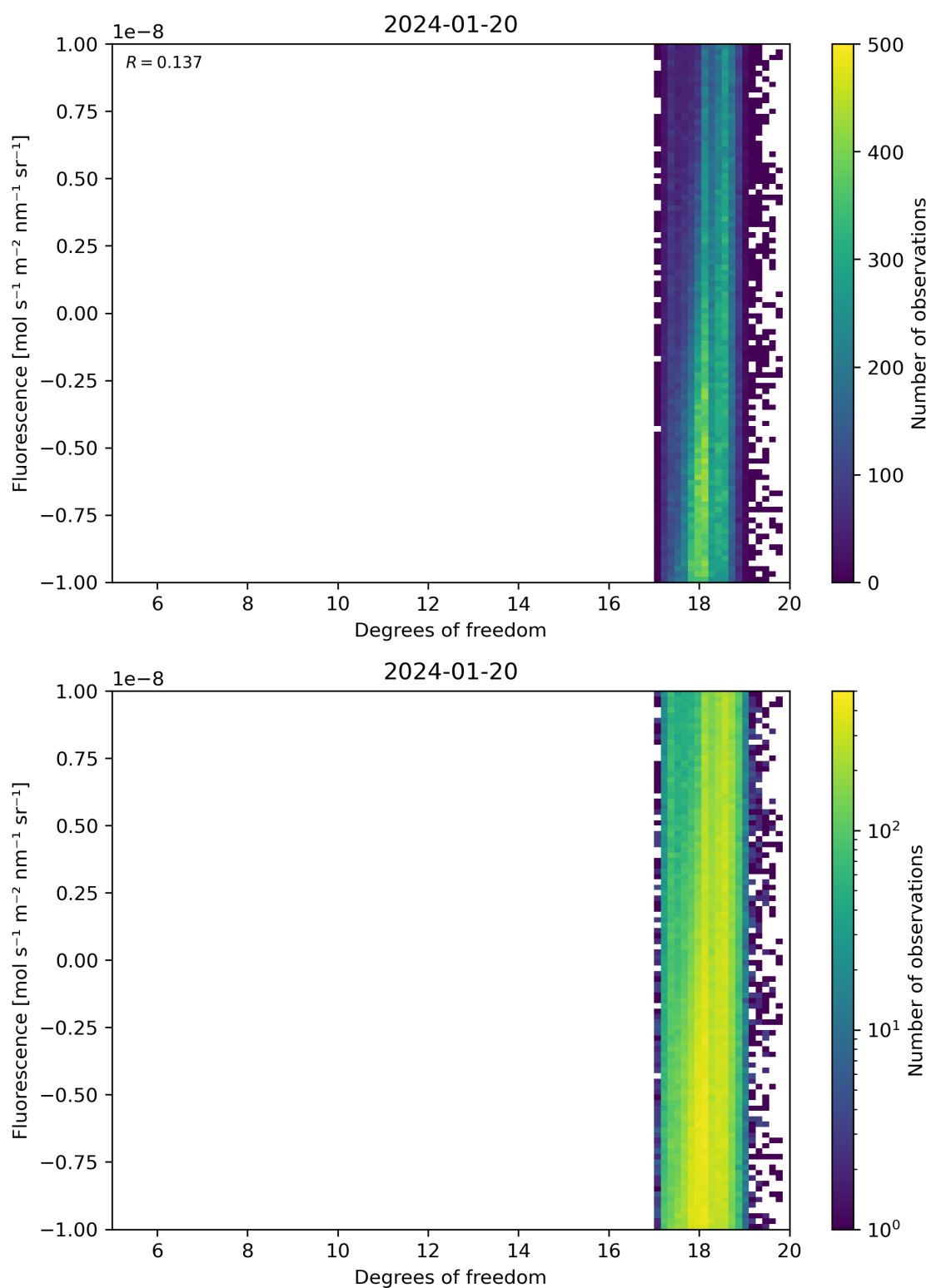
Figure 51: Scatter density plot of “Degrees of freedom” against “Fluorescence” for 2024-01-19 to 2024-01-21.
