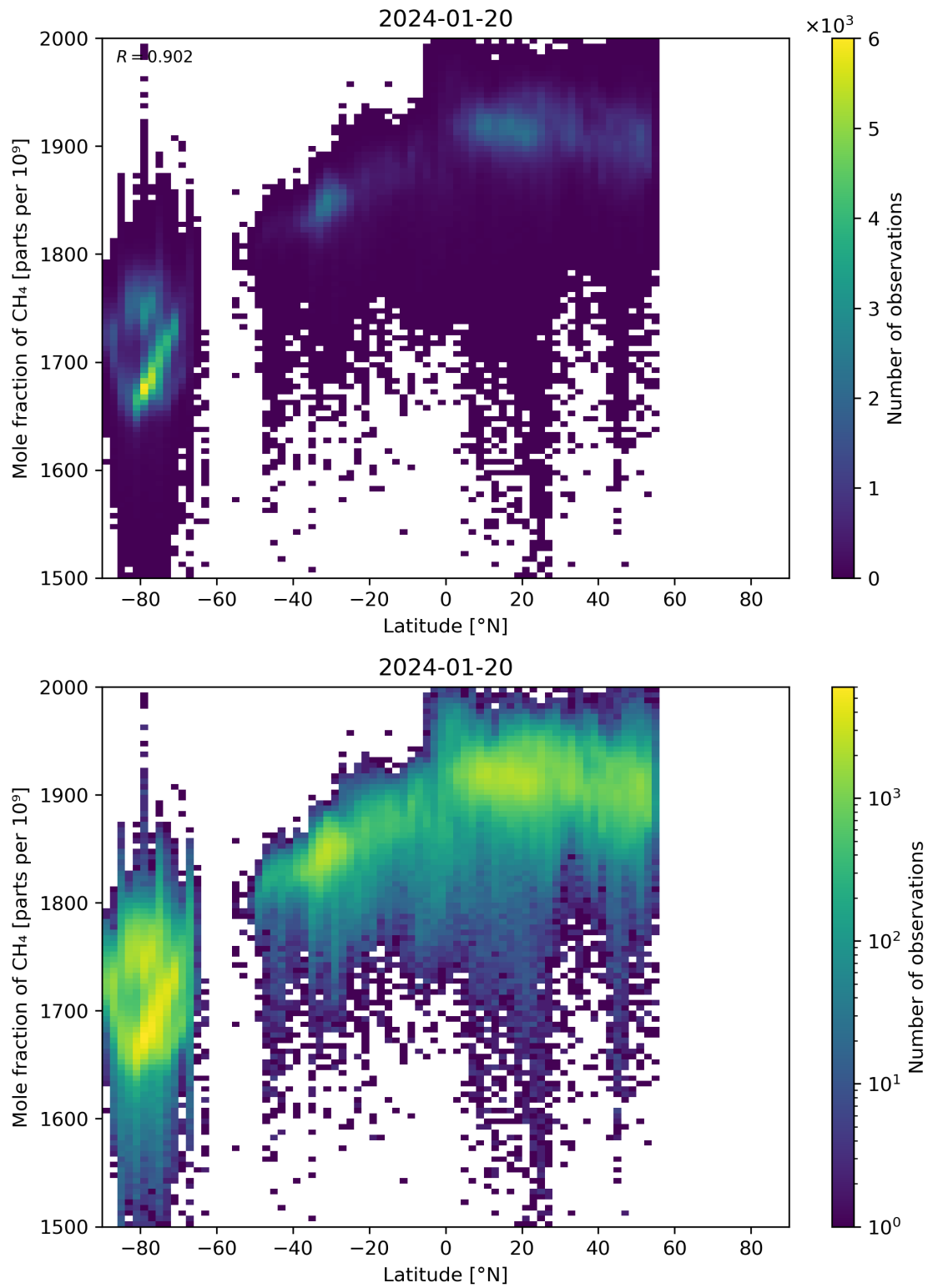
Figure 57: Scatter density plot of “Latitude” against “Mole fraction of CH 4 ” for 2024-01-19 to 2024-01-21.
