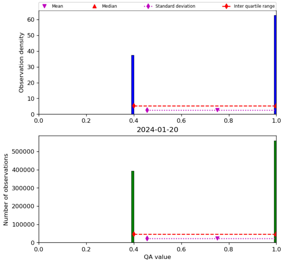
Figure 22: Histogram of “QA value” for 2024-01-19 to 2024-01-21
