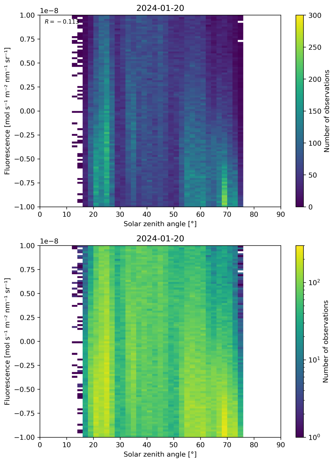
Figure 97: Scatter density plot of “Solar zenith angle” against “Fluorescence” for 2024-01-19 to 2024-01-21.
