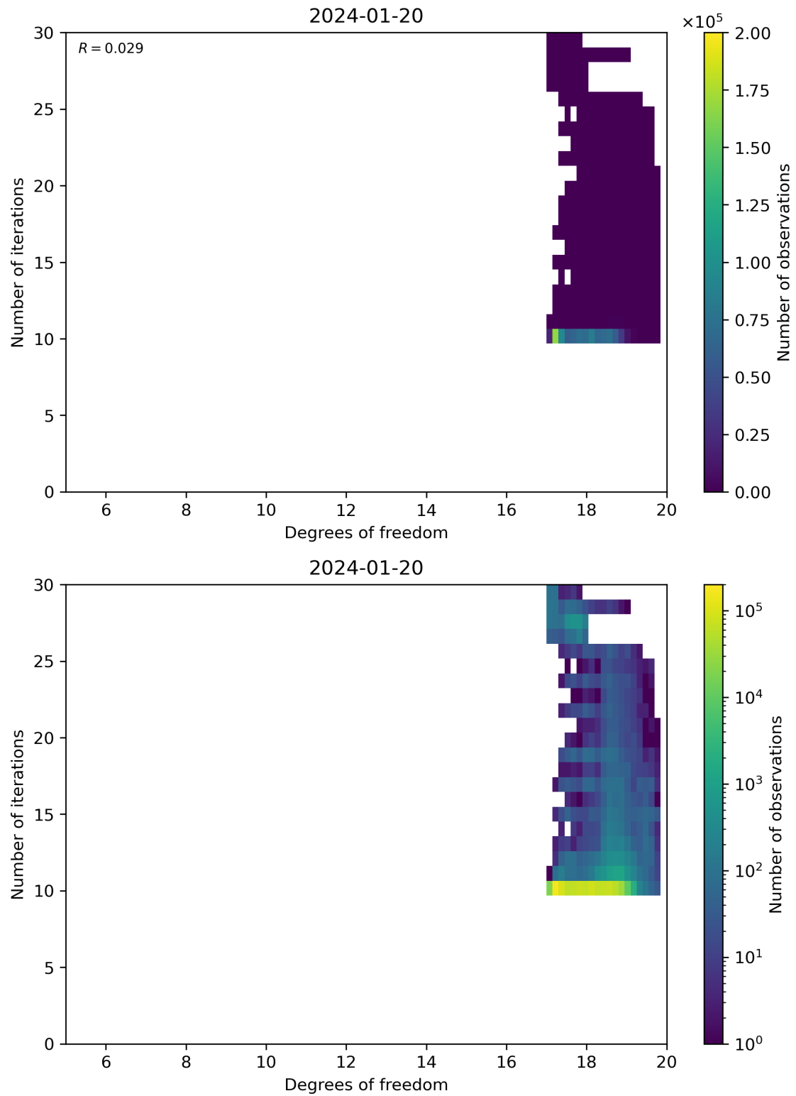
Figure 52: Scatter density plot of “Degrees of freedom” against “Number of iterations” for 2024-01-19 to 2024-01-21.
