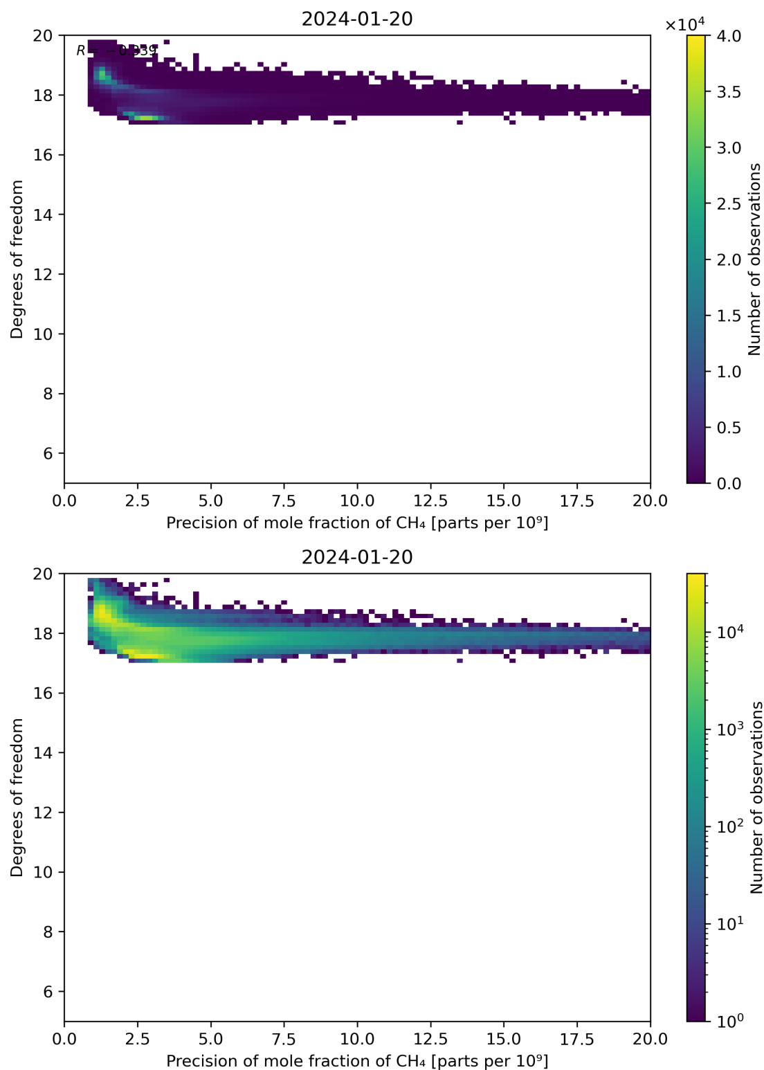
Figure 80: Scatter density plot of “Precision of mole fraction of CH 4 ” against “Degrees of freedom” for 2024-01-19 to 2024-01-21.
