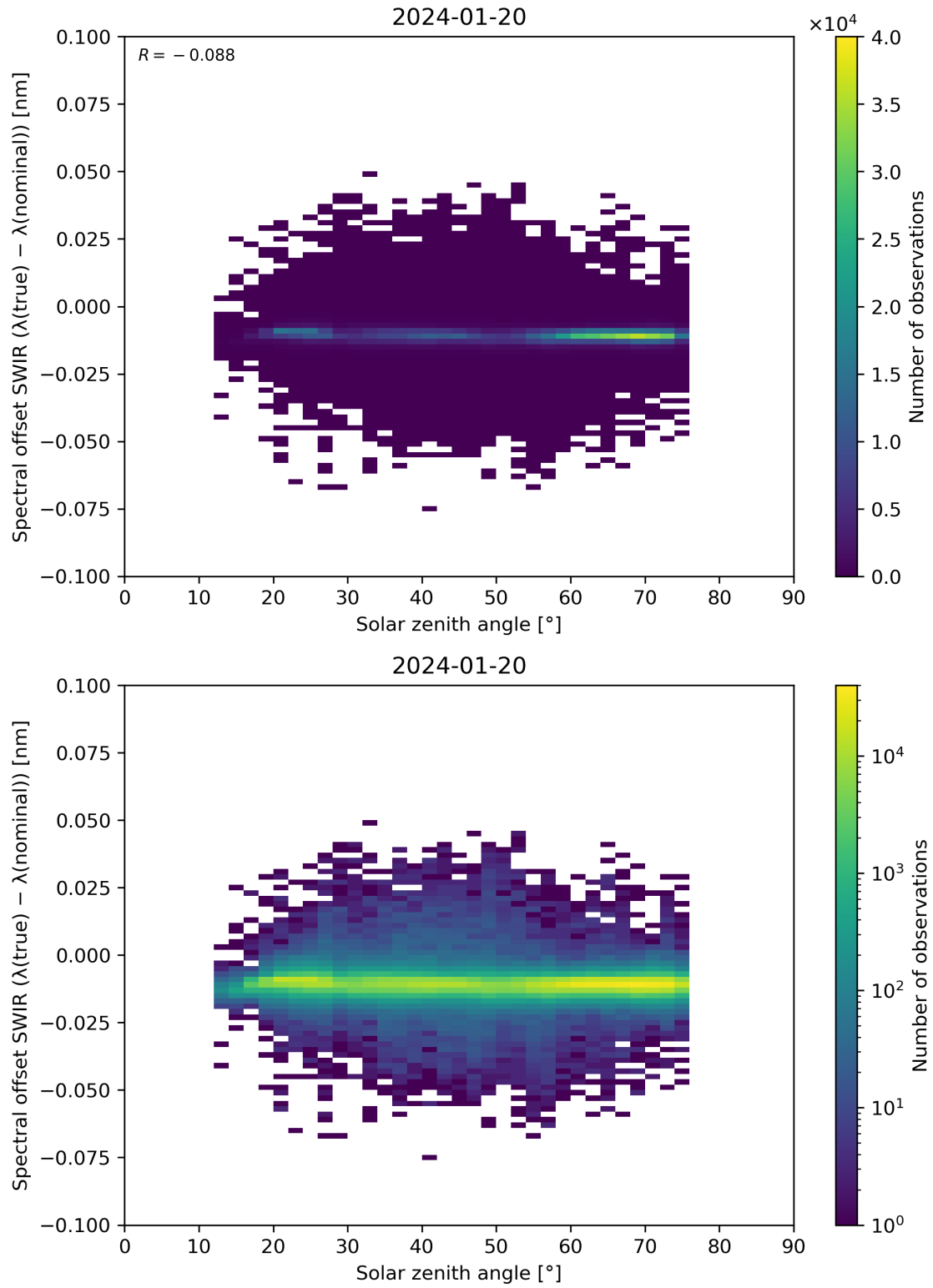
Figure 104: Scatter density plot of “Solar zenith angle” against “Spectral offset SWIR ( \lambda(\text{true}) - \lambda(\text{nominal}) )” for 2024-01-19 to 2024-01-21.
