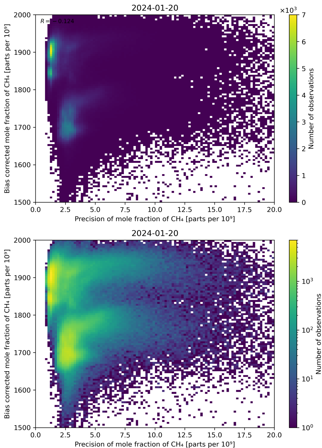
Figure 82: Scatter density plot of “Precision of mole fraction of CH 4 ” against “Bias corrected mole fraction of CH 4 ” for 2024-01-19 to 2024-01-21.
