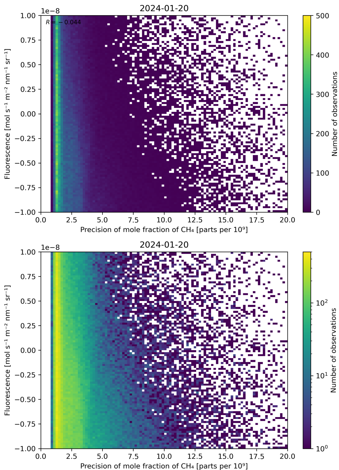
Figure 81: Scatter density plot of “Precision of mole fraction of \text{CH}_4 ” against “Fluorescence” for 2024-01-19 to 2024-01-21.
