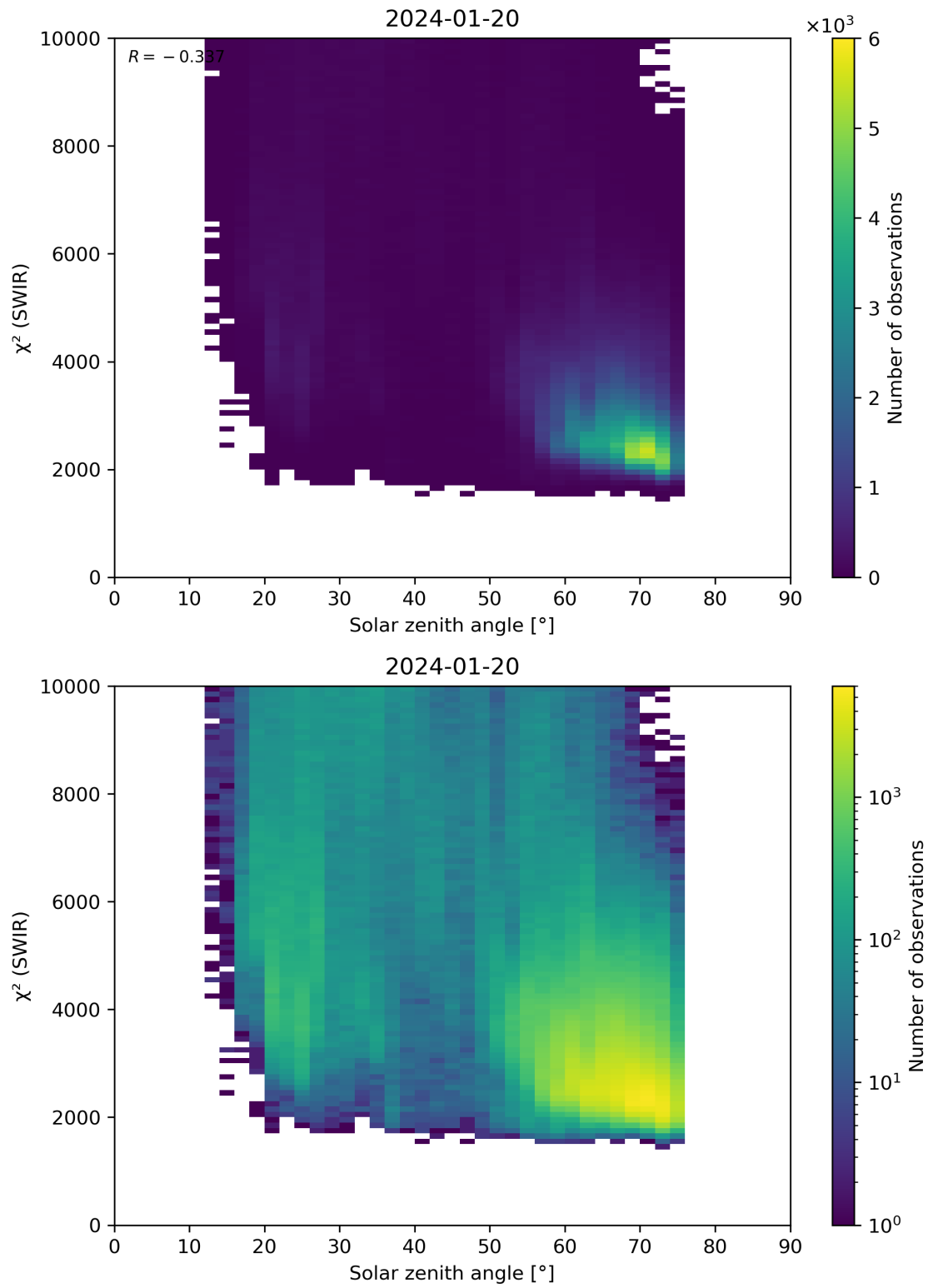
Figure 95: Scatter density plot of “Solar zenith angle” against “ \chi^2 (SWIR)” for 2024-01-19 to 2024-01-21.
