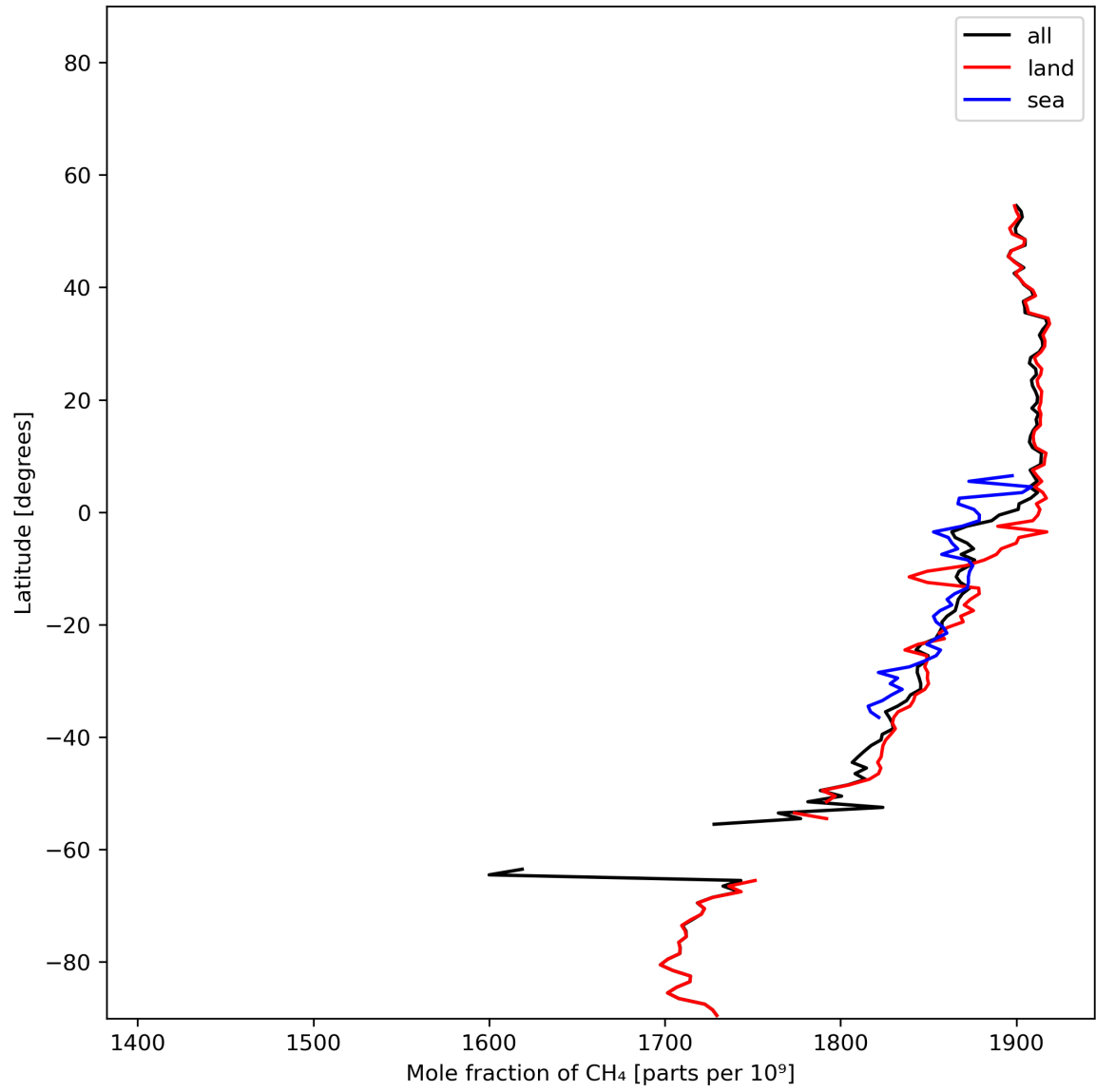
Figure 12: Zonal average of “Mole fraction of \text{CH}_4 ” for 2024-01-19 to 2024-01-21.
