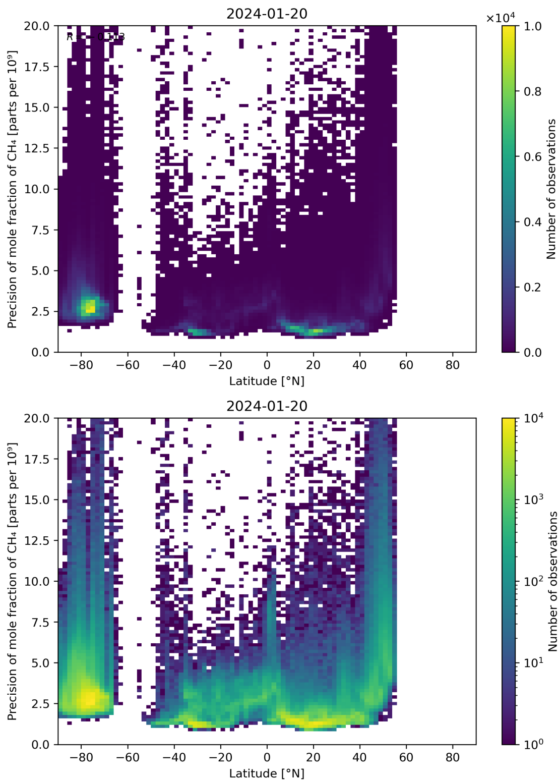
Figure 59: Scatter density plot of “Latitude” against “Precision of mole fraction of CH 4 ” for 2024-01-19 to 2024-01-21.
