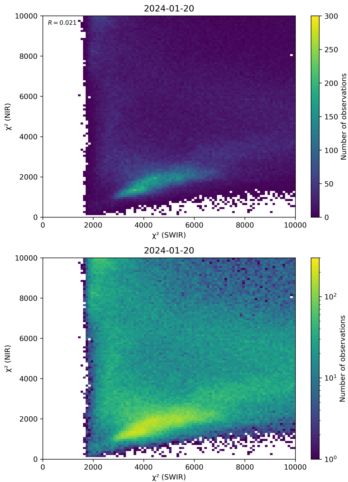
Figure 47: Scatter density plot of “ \chi^2 (SWIR)” against “ \chi^2 (NIR)” for 2024-01-19 to 2024-01-21.
