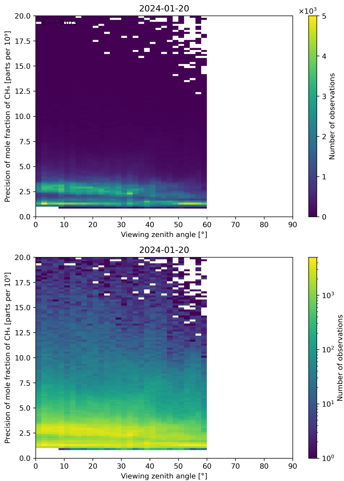
Figure 112: Scatter density plot of “Viewing zenith angle” against “Precision of mole fraction of CH 4 ” for 2024-01-19 to 2024-01-21.
