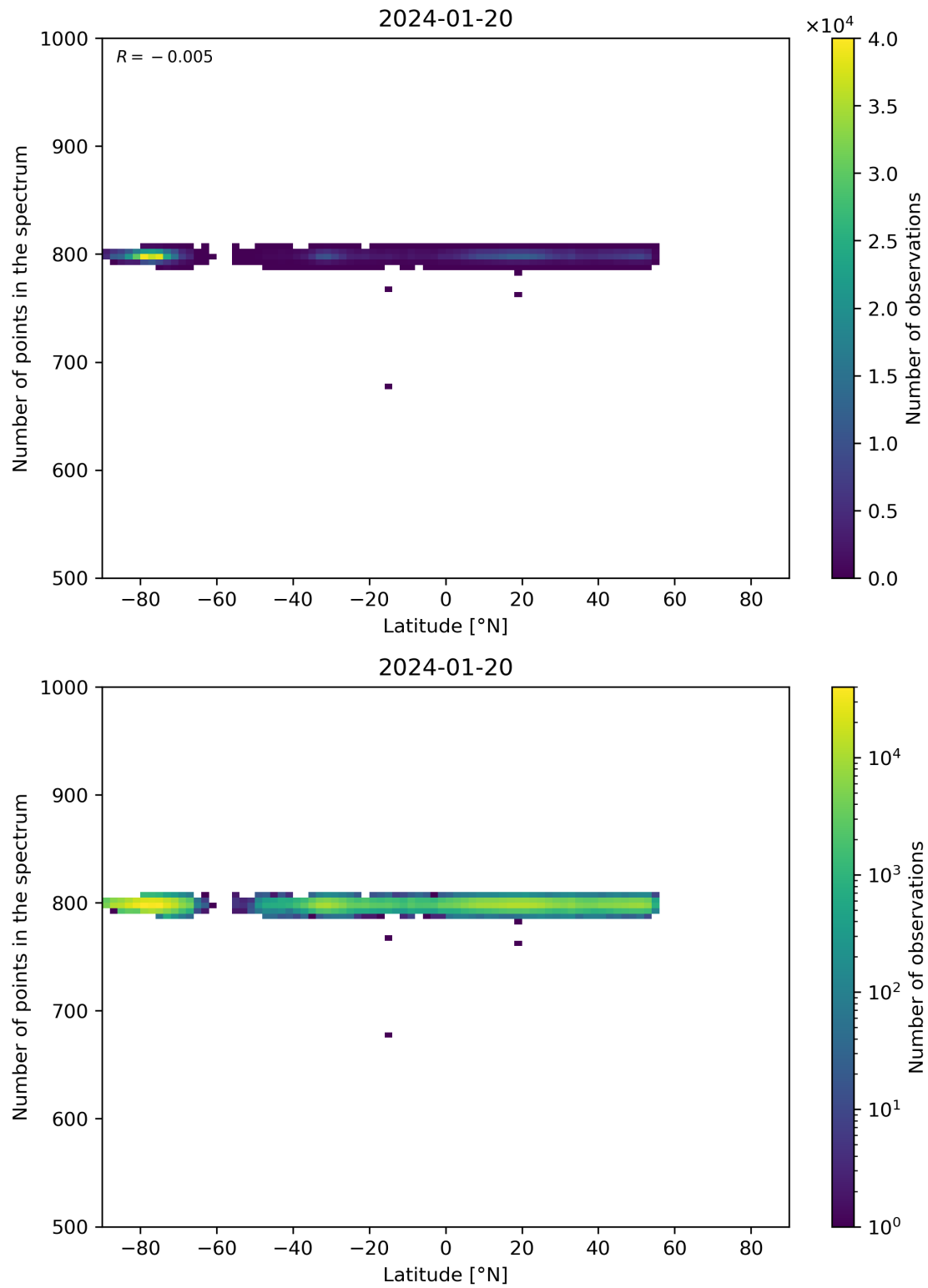
Figure 61: Scatter density plot of “Latitude” against “Number of points in the spectrum” for 2024-01-19 to 2024-01-21.
