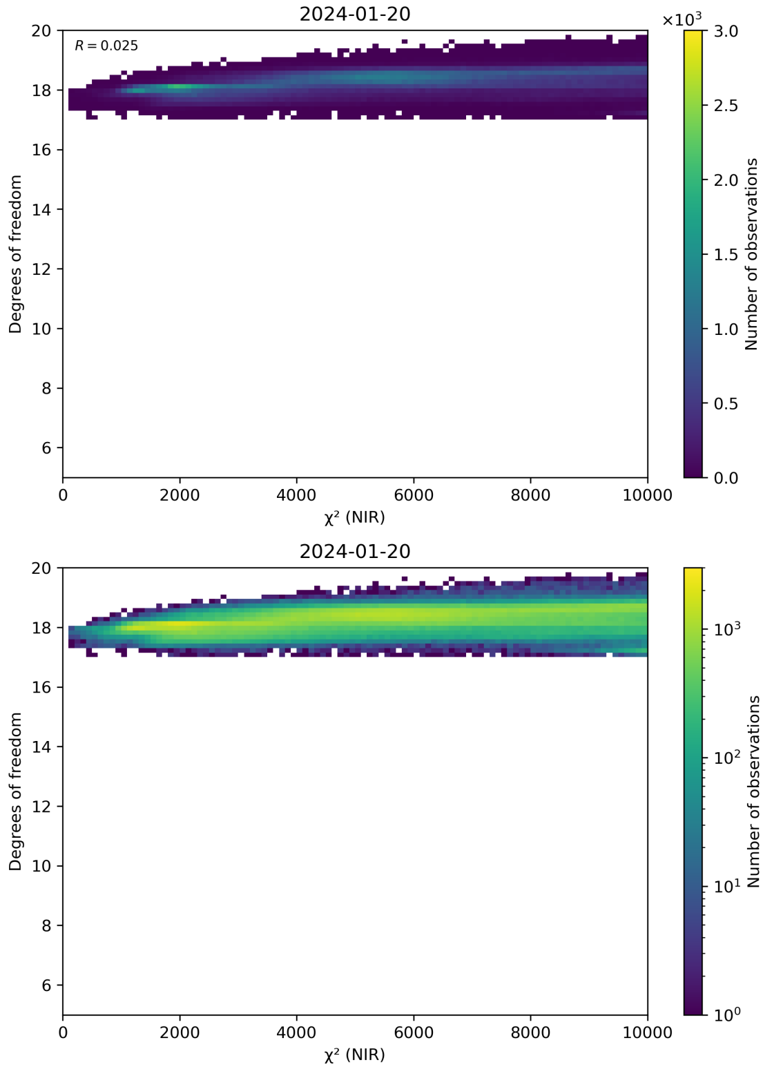
Figure 44: Scatter density plot of “ \chi^2 (NIR)” against “Degrees of freedom” for 2024-01-19 to 2024-01-21.
