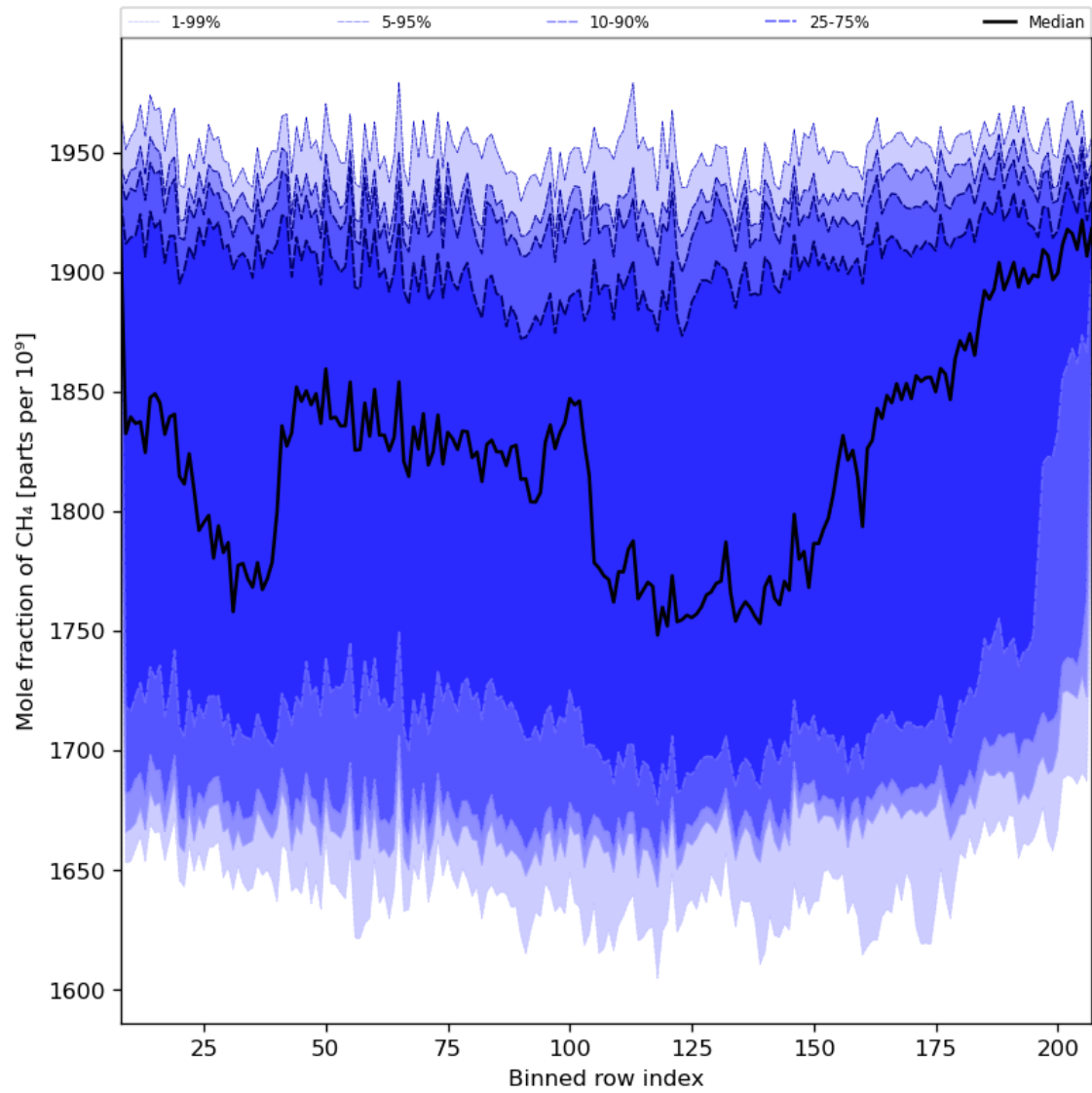
Figure 34: Along track statistics of “Mole fraction of CH 4 ” for 2024-01-19 to 2024-01-21
