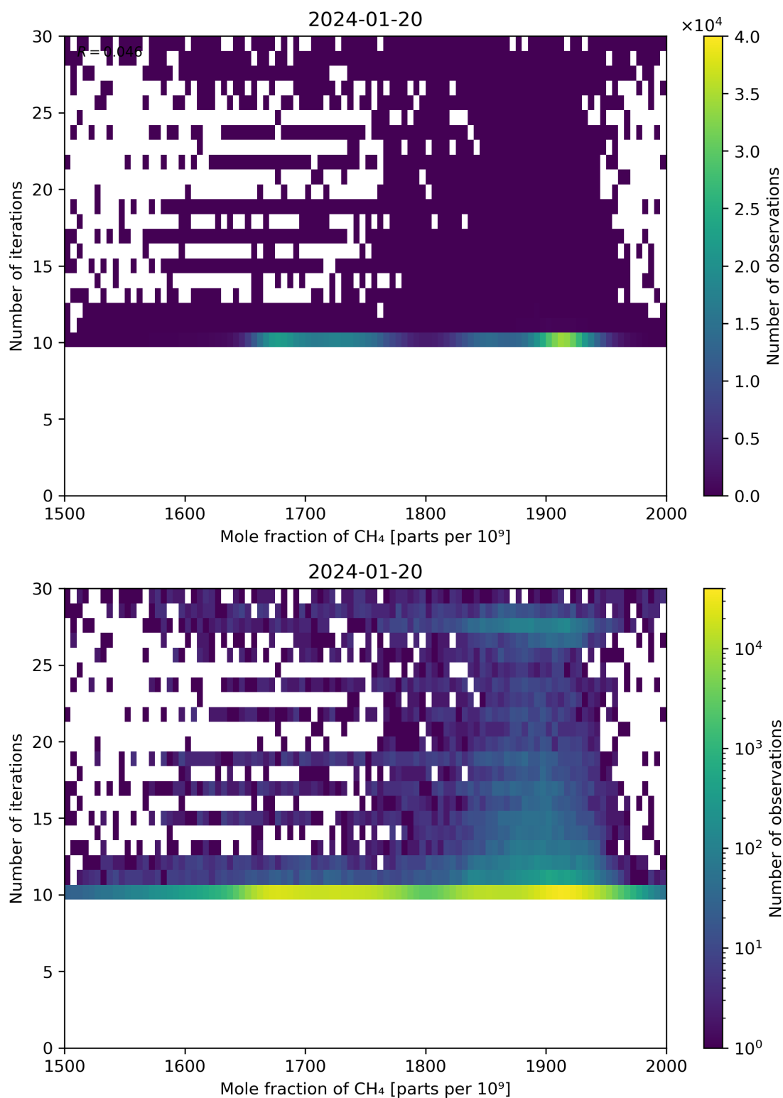
Figure 76: Scatter density plot of “Mole fraction of CH 4 ” against “Number of iterations” for 2024-01-19 to 2024-01-21.
