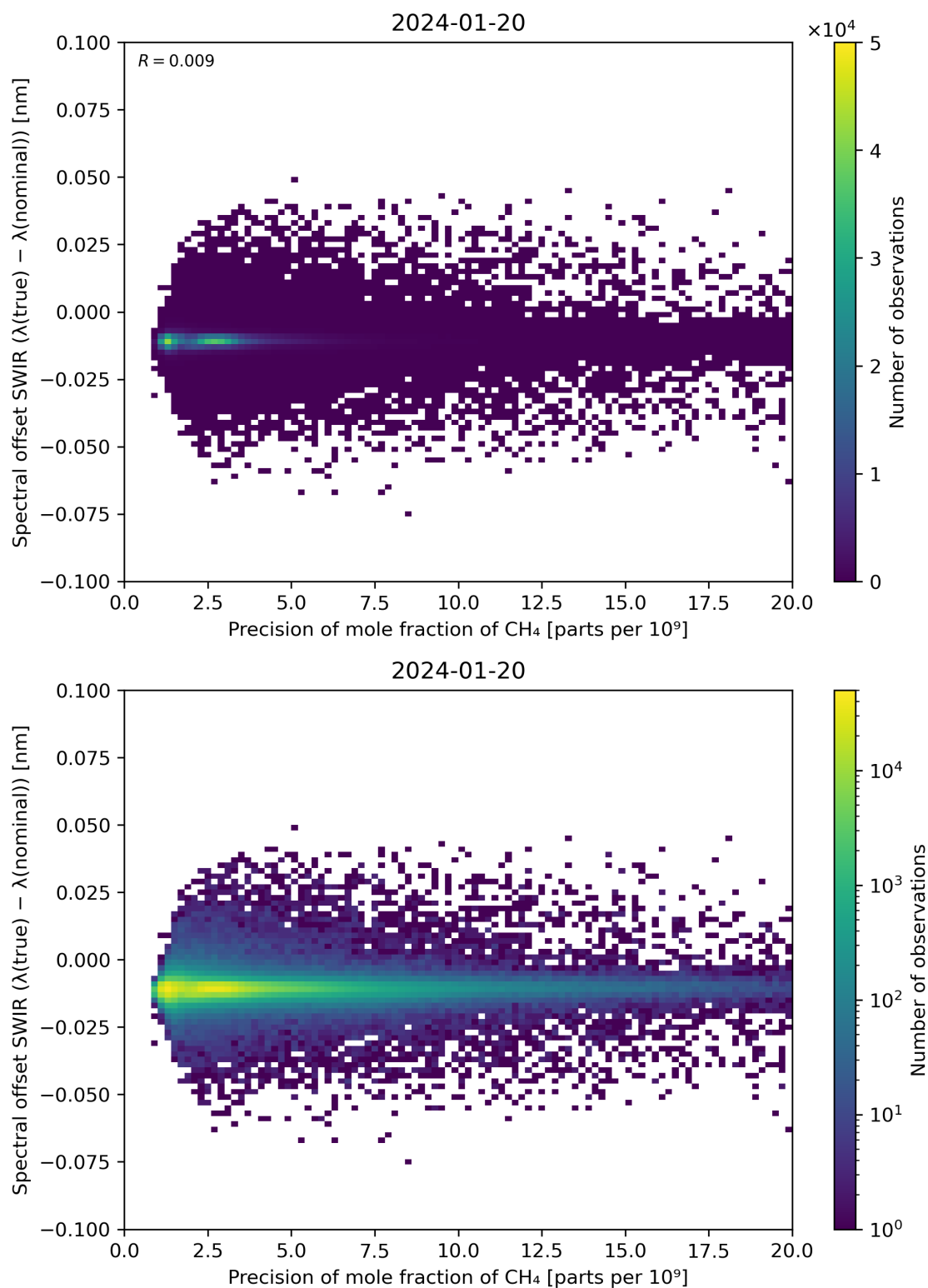
Figure 85: Scatter density plot of “Precision of mole fraction of \text{CH}_4 ” against “Spectral offset SWIR ( \lambda(\text{true}) - \lambda(\text{nominal}) )” for 2024-01-19 to 2024-01-21.
