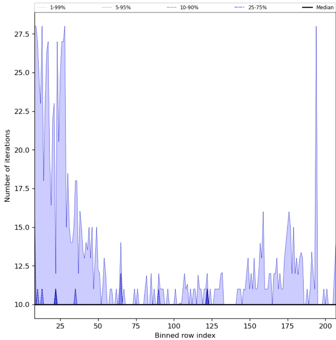
Figure 42: Along track statistics of “Number of iterations” for 2024-01-19 to 2024-01-21
