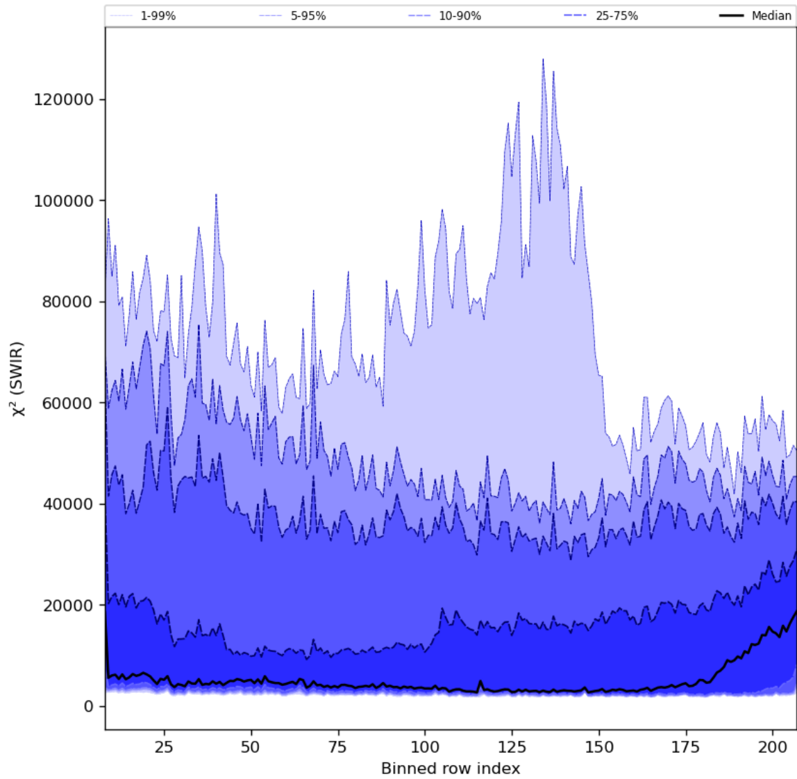
Figure 39: Along track statistics of “ \chi^2 (SWIR)” for 2024-01-19 to 2024-01-21
