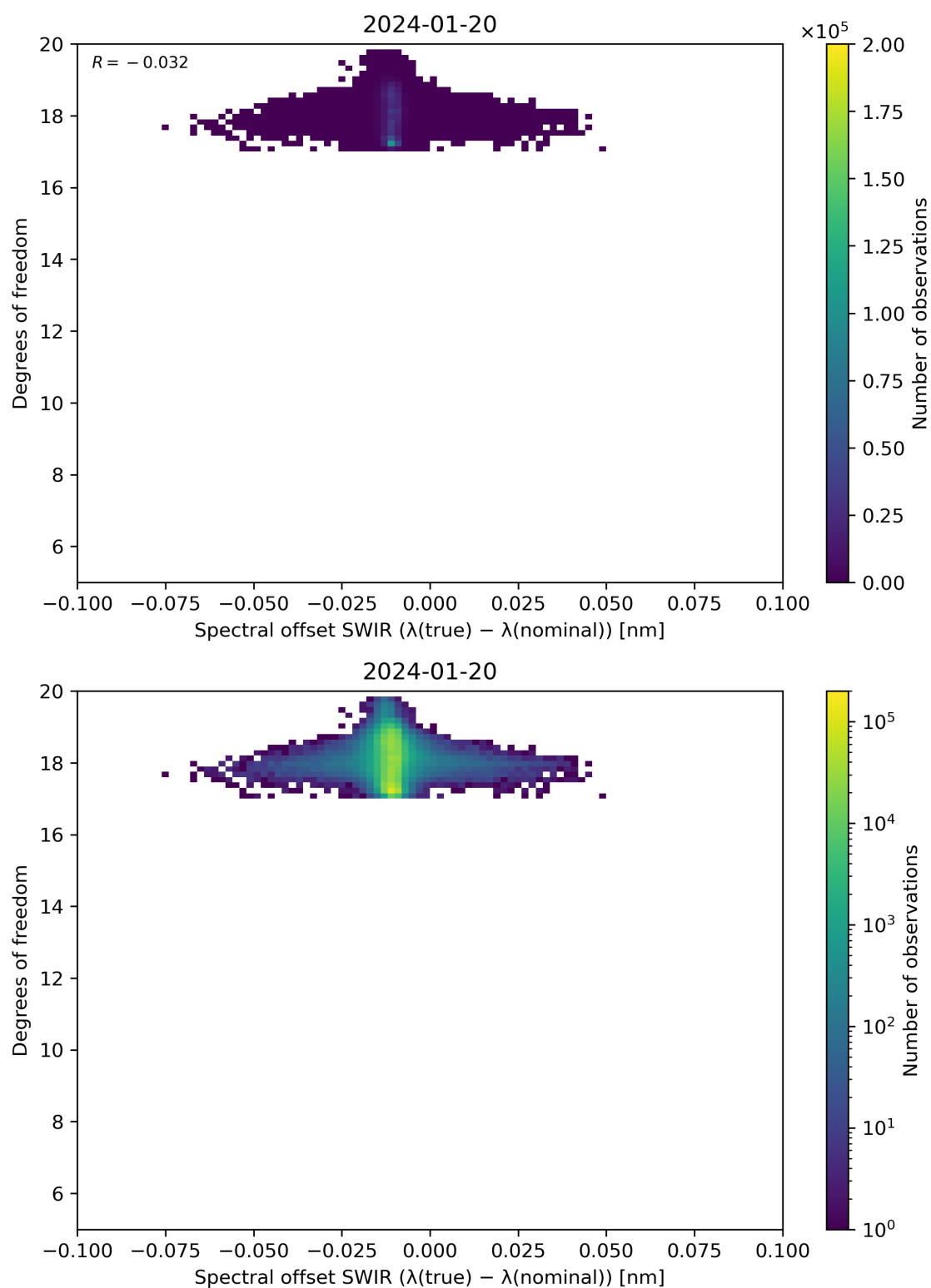
Figure 119: Scatter density plot of “Spectral offset SWIR ( \lambda(\text{true}) - \lambda(\text{nominal}) )” against “Degrees of freedom” for 2024-01-19 to 2024-01-21.
