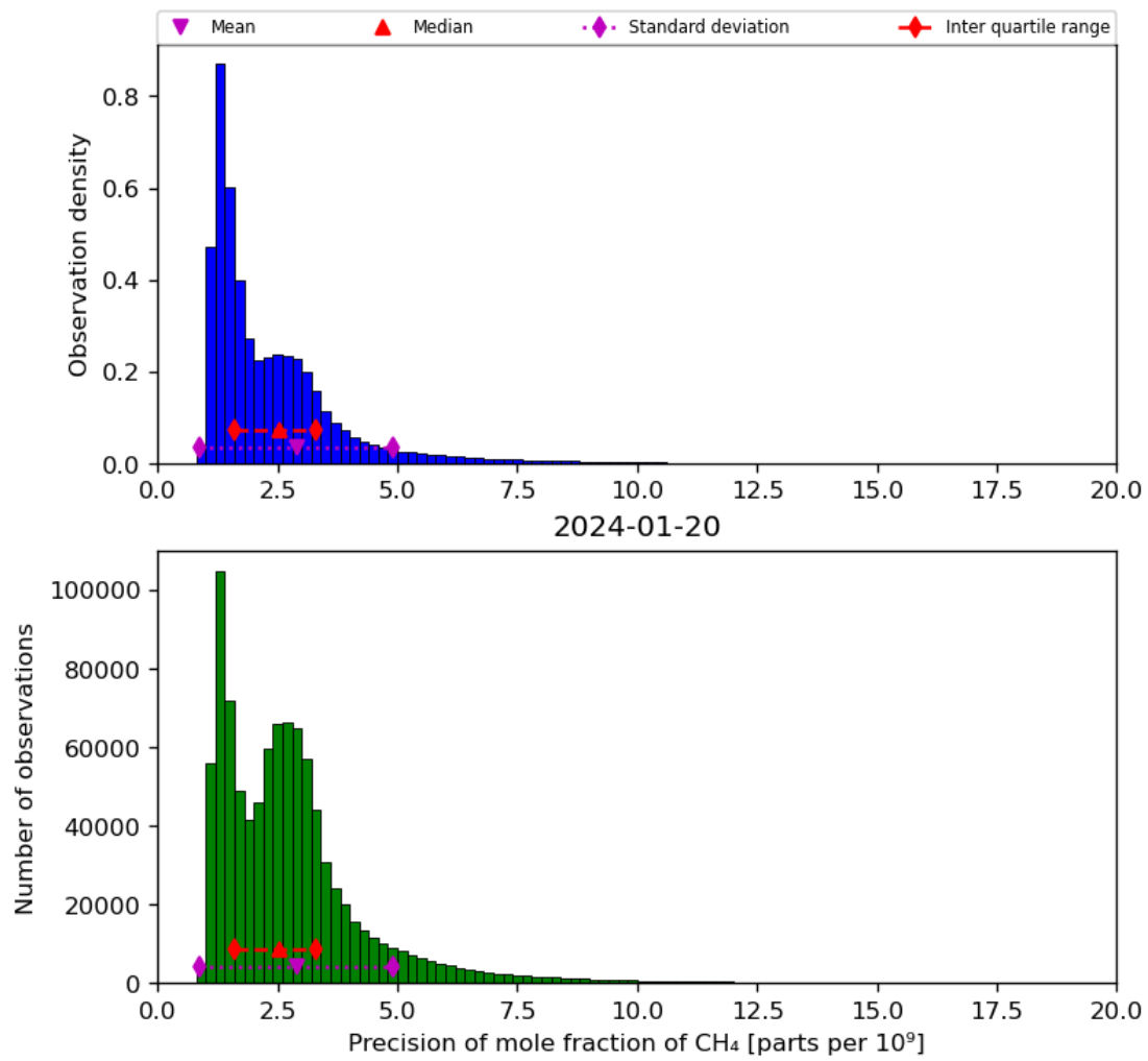
Figure 24: Histogram of “Precision of mole fraction of CH 4 ” for 2024-01-19 to 2024-01-21
