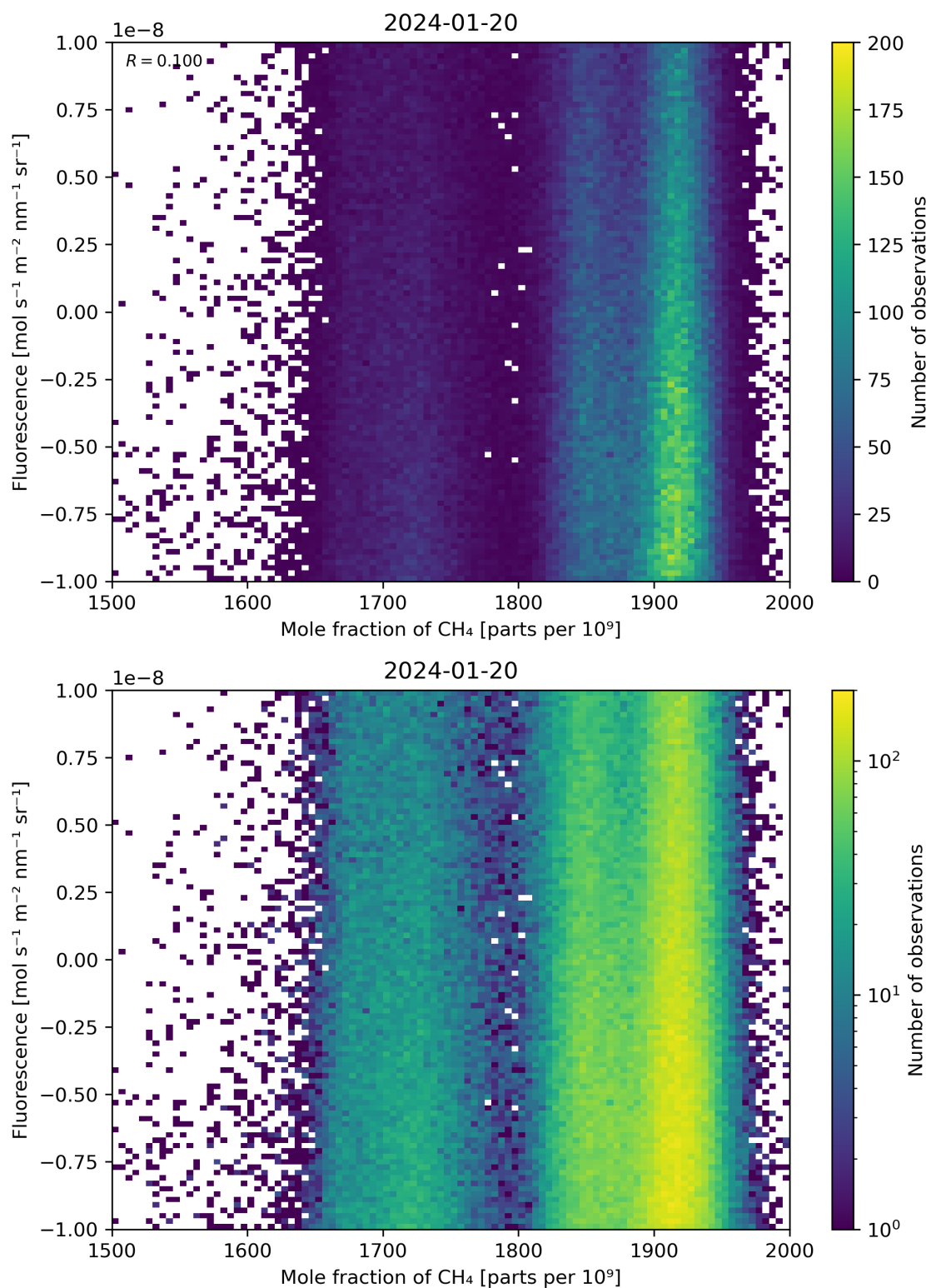
Figure 73: Scatter density plot of “Mole fraction of \text{CH}_4 ” against “Fluorescence” for 2024-01-19 to 2024-01-21.
