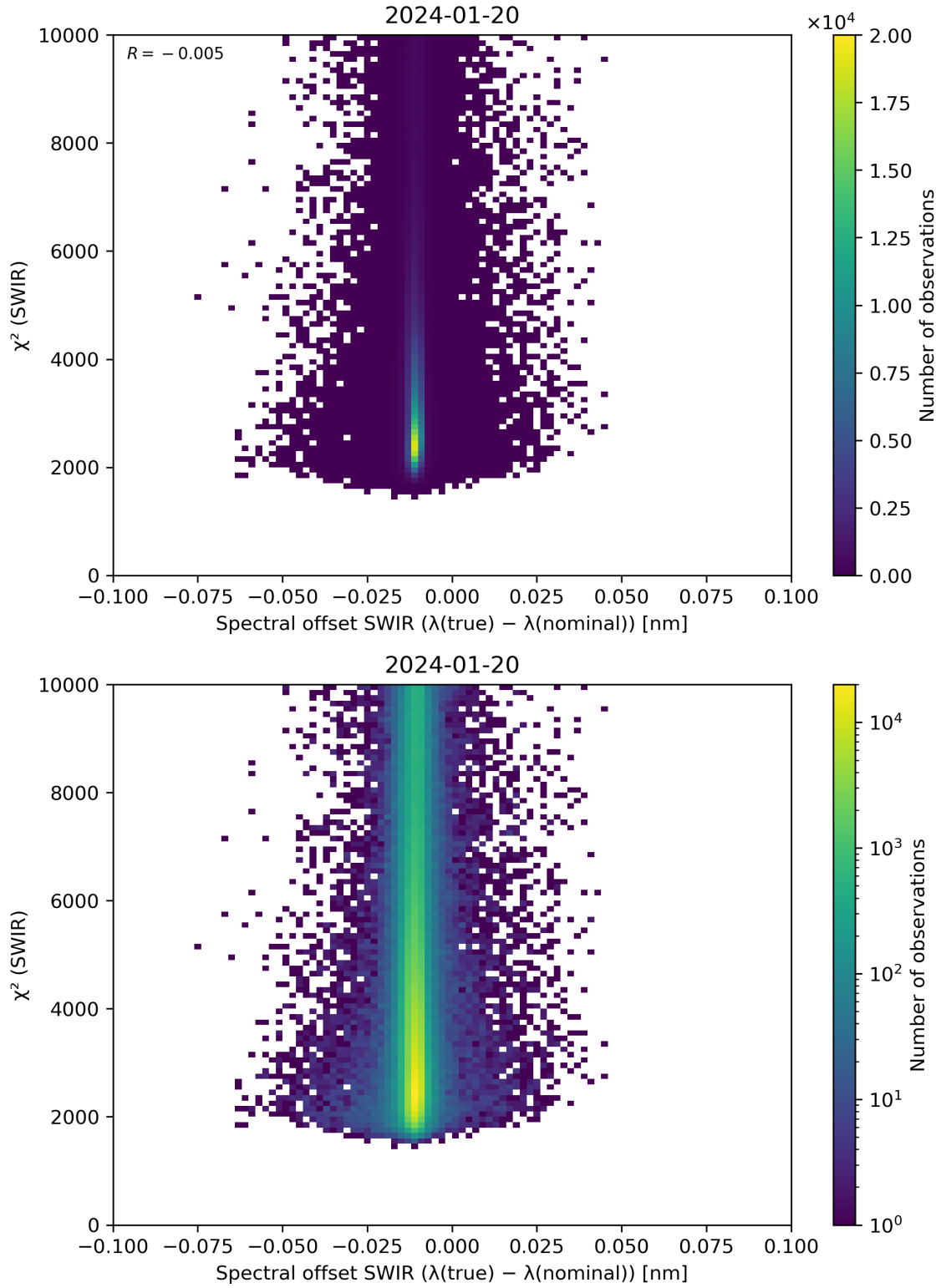
Figure 118: Scatter density plot of “Spectral offset SWIR ( \lambda(\text{true}) - \lambda(\text{nominal}) )” against “ \chi^2 (SWIR)” for 2024-01-19 to 2024-01-21.
