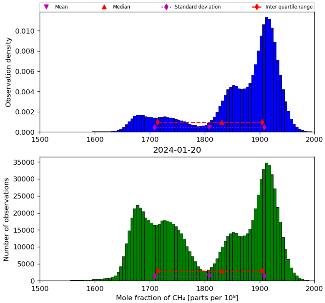
Figure 23: Histogram of “Mole fraction of CH 4 ” for 2024-01-19 to 2024-01-21
