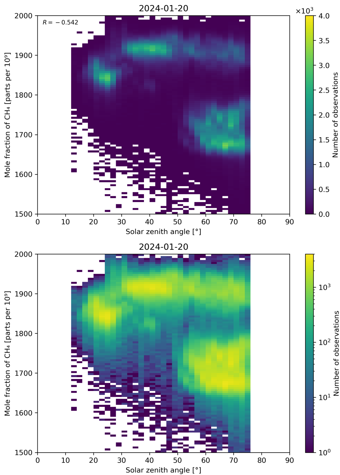
Figure 99: Scatter density plot of “Solar zenith angle” against “Mole fraction of CH 4 ” for 2024-01-19 to 2024-01-21.
