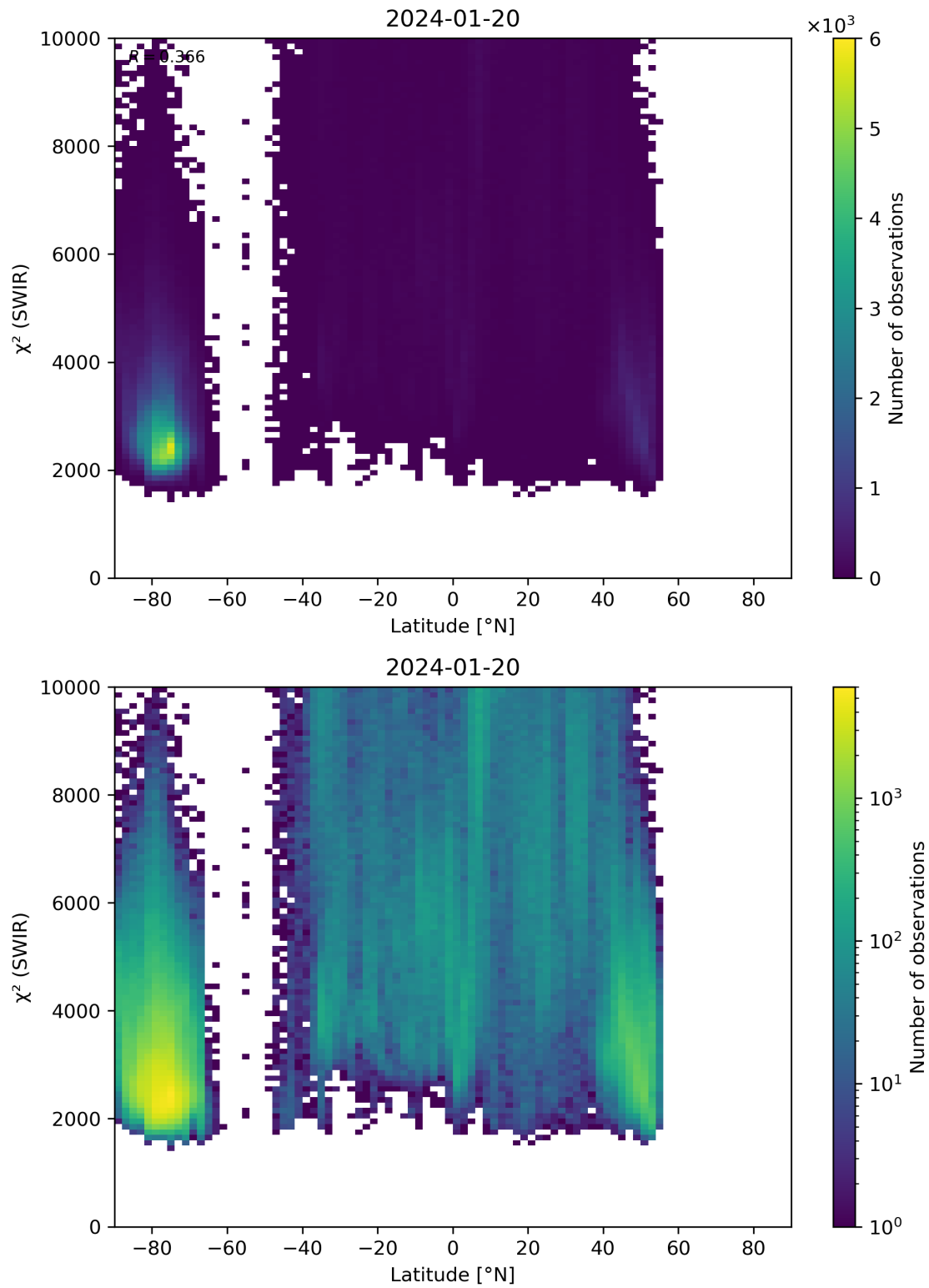
Figure 54: Scatter density plot of “Latitude” against “ \chi^2 (SWIR)” for 2024-01-19 to 2024-01-21.
