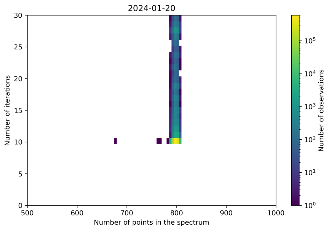
Figure 92: Scatter density plot of “Number of points in the spectrum” against “Number of iterations” for 2024-01-19 to 2024-01-21.
