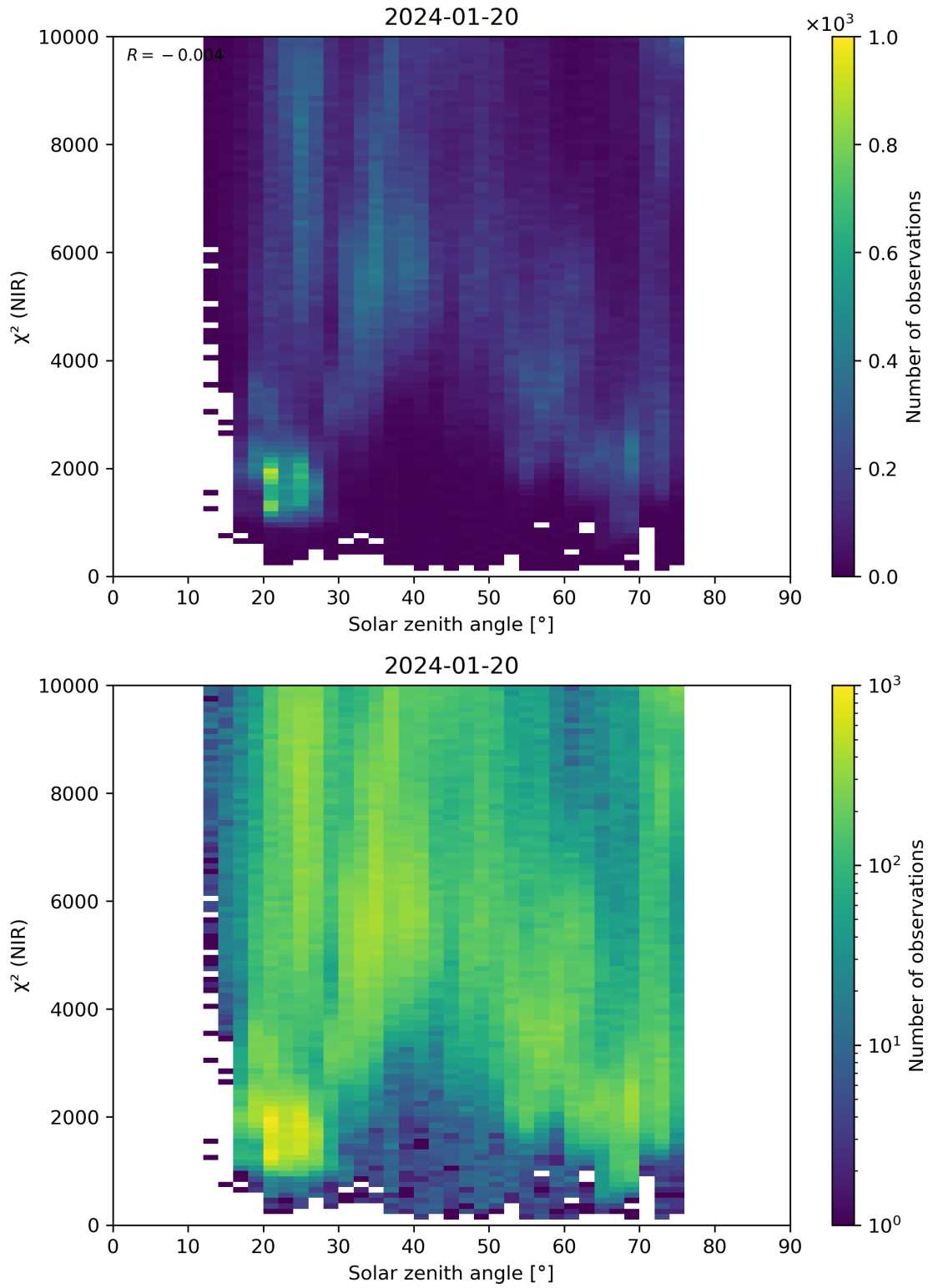
Figure 94: Scatter density plot of “Solar zenith angle” against “ \chi^2 (NIR)” for 2024-01-19 to 2024-01-21.
