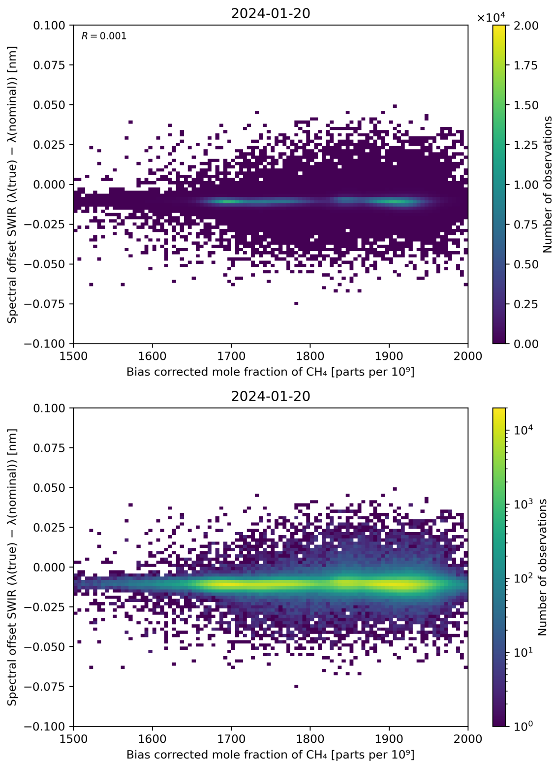
Figure 69: Scatter density plot of “Bias corrected mole fraction of \text{CH}_4 ” against “Spectral offset SWIR ( \lambda(\text{true}) - \lambda(\text{nominal}) )” for 2024-01-19 to 2024-01-21.
