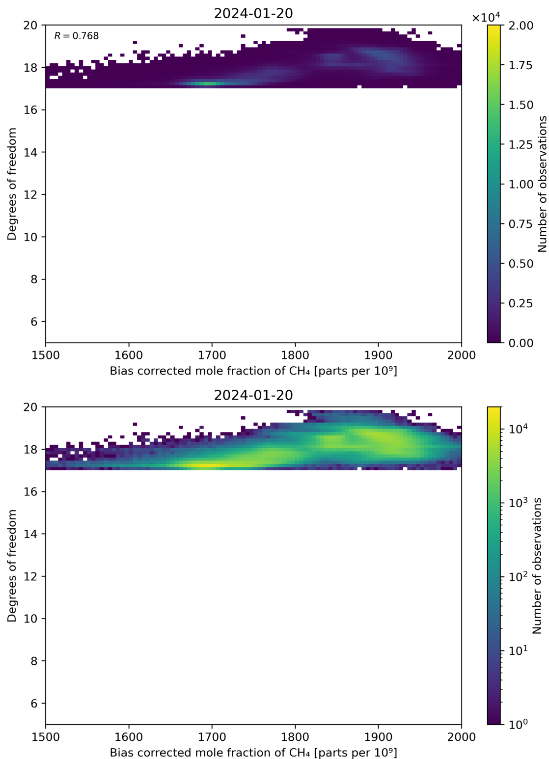
Figure 65: Scatter density plot of “Bias corrected mole fraction of CH 4 ” against “Degrees of freedom” for 2024-01-19 to 2024-01-21.
