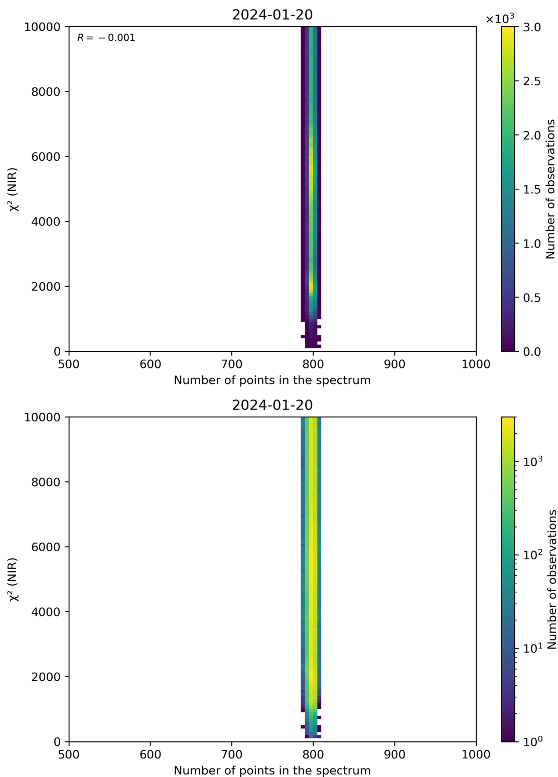
Figure 88: Scatter density plot of “Number of points in the spectrum” against “ \chi^2 (NIR)” for 2024-01-19 to 2024-01-21.
