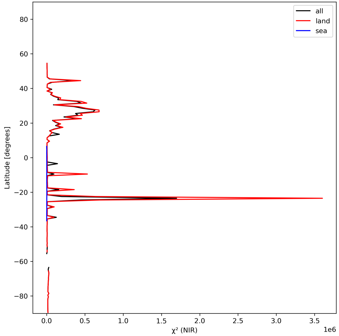
Figure 18: Zonal average of “ \chi^2 (NIR)” for 2024-01-19 to 2024-01-21.
