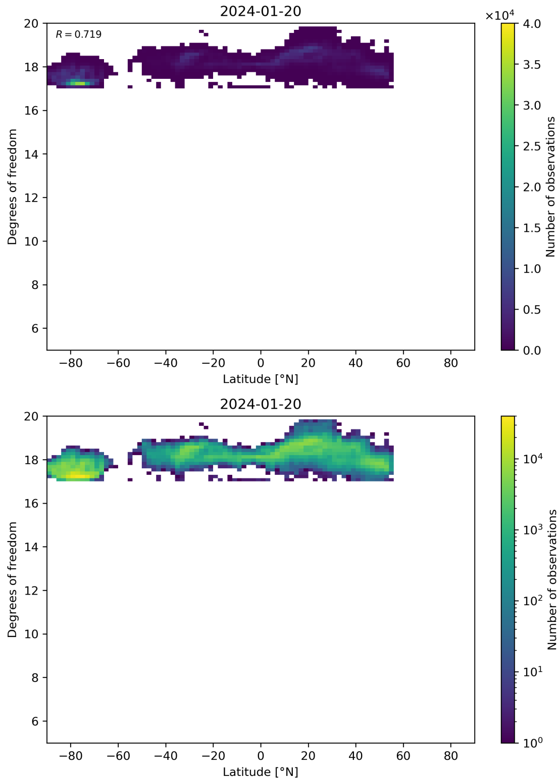
Figure 55: Scatter density plot of “Latitude” against “Degrees of freedom” for 2024-01-19 to 2024-01-21.
