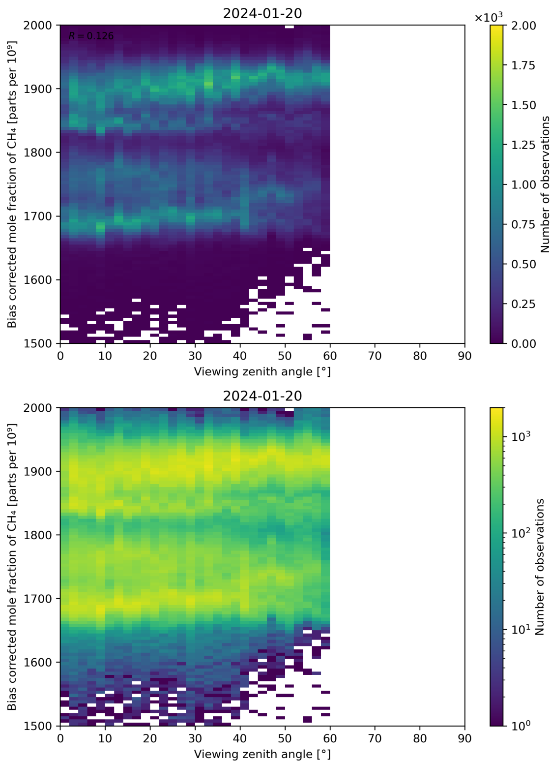
Figure 111: Scatter density plot of “Viewing zenith angle” against “Bias corrected mole fraction of CH 4 ” for 2024-01-19 to 2024-01-21.
