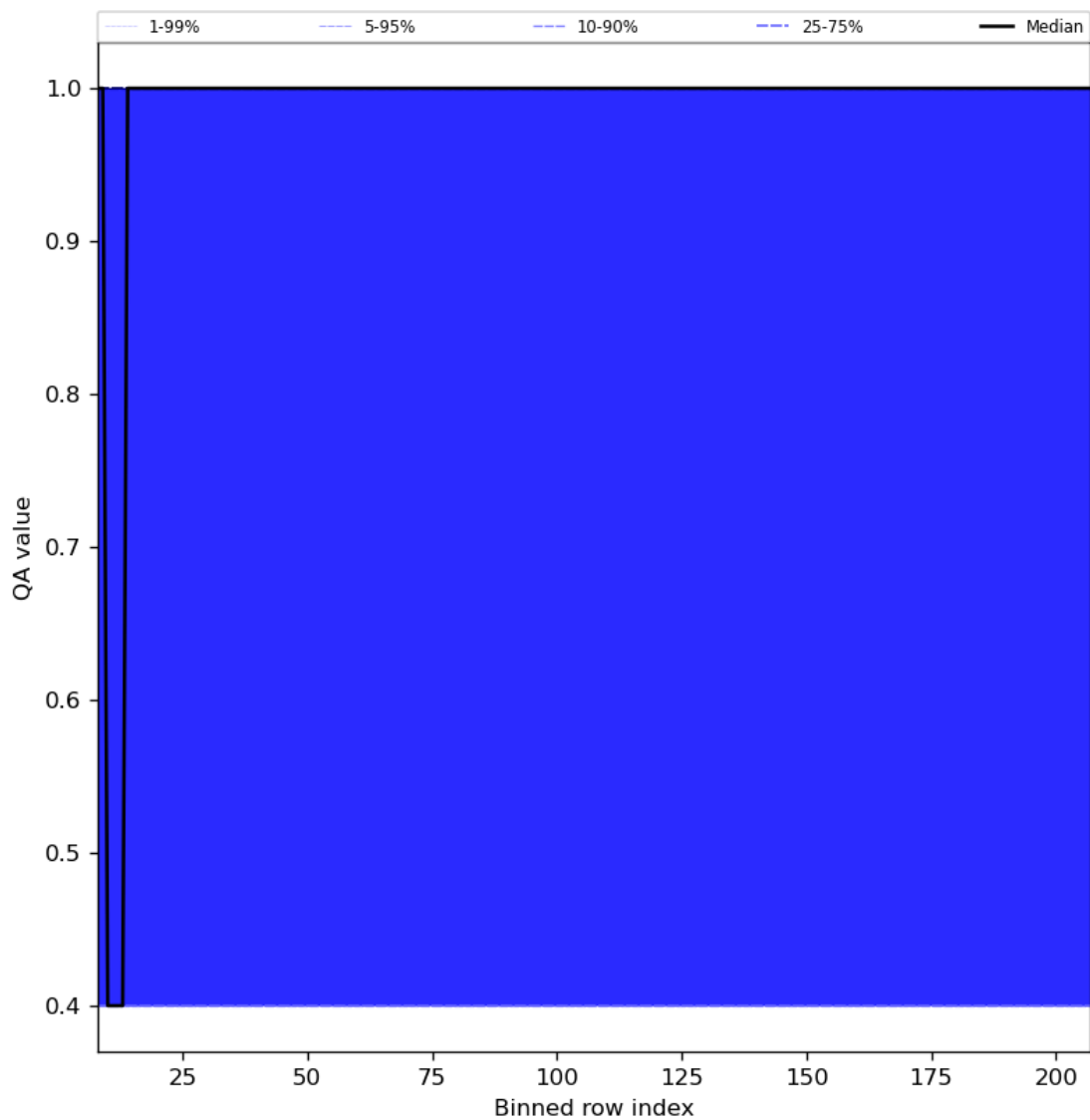
Figure 33: Along track statistics of “QA value” for 2024-01-19 to 2024-01-21
