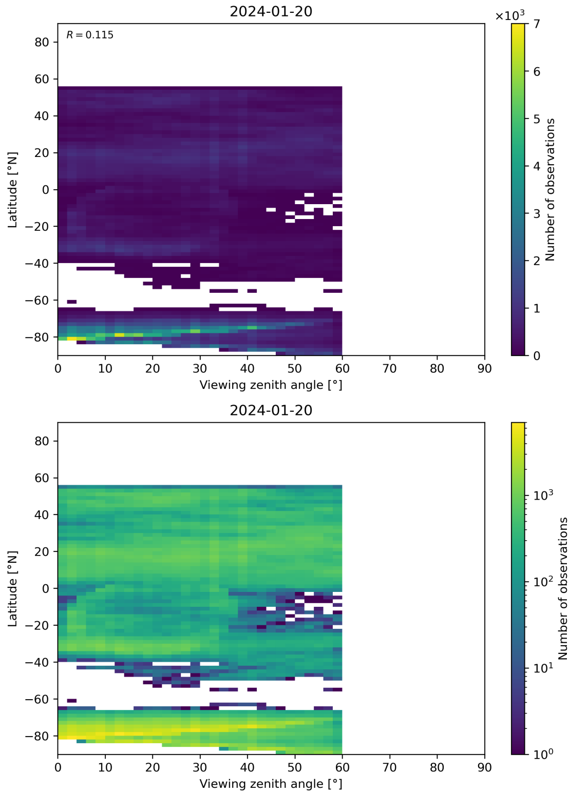
Figure 109: Scatter density plot of “Viewing zenith angle” against “Latitude” for 2024-01-19 to 2024-01-21.
