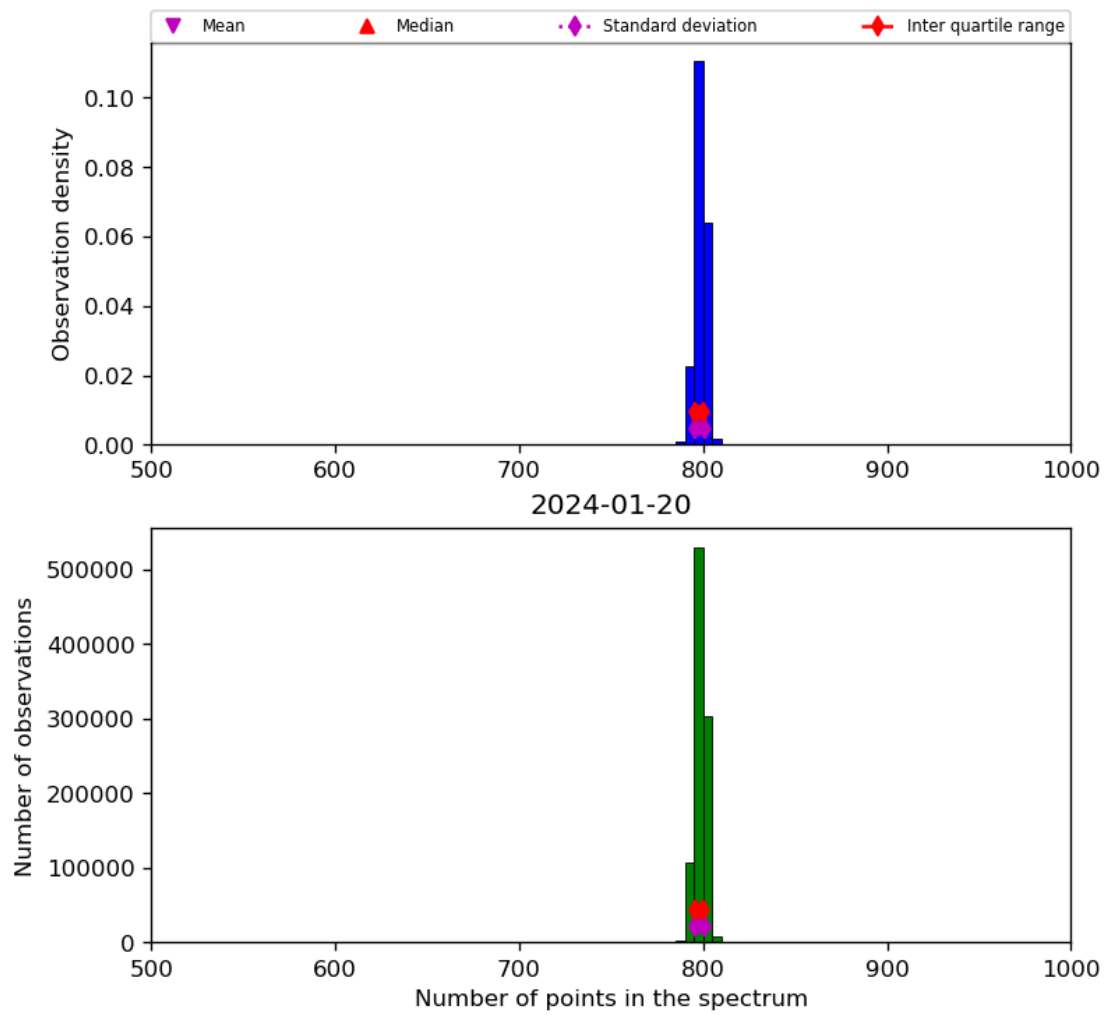
Figure 26: Histogram of “Number of points in the spectrum” for 2024-01-19 to 2024-01-21
