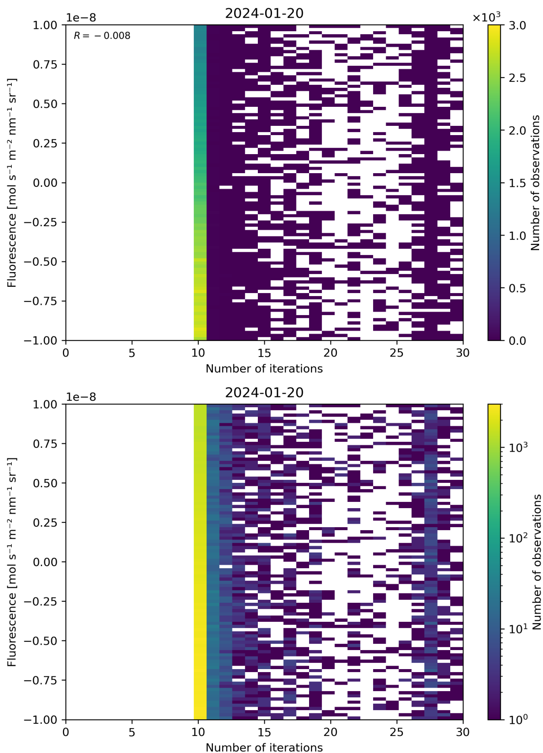
Figure 87: Scatter density plot of “Number of iterations” against “Fluorescence” for 2024-01-19 to 2024-01-21.
