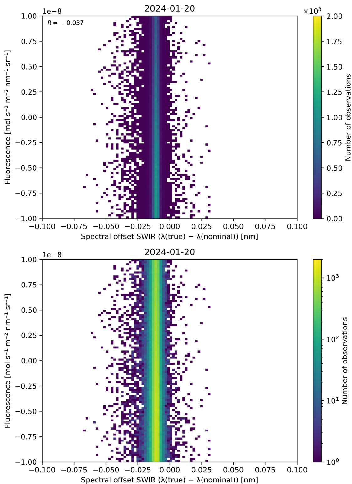
Figure 120: Scatter density plot of “Spectral offset SWIR ( \lambda(\text{true}) - \lambda(\text{nominal}) )” against “Fluorescence” for 2024-01-19 to 2024-01-21.
