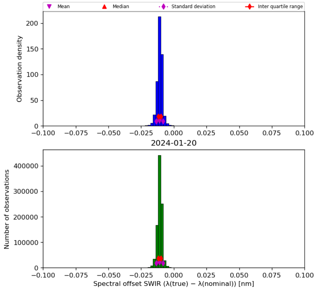
Figure 27: Histogram of “Spectral offset SWIR ( \lambda(\text{true}) - \lambda(\text{nominal}) )” for 2024-01-19 to 2024-01-21
