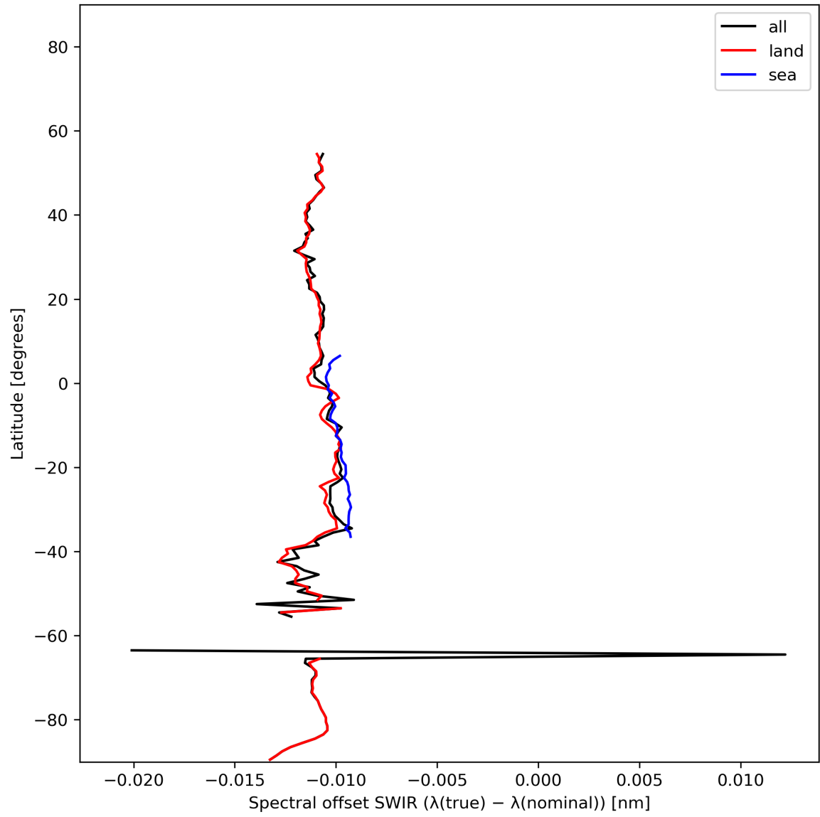
Figure 16: Zonal average of “Spectral offset SWIR ( \lambda(\text{true}) - \lambda(\text{nominal}) )” for 2024-01-19 to 2024-01-21.
