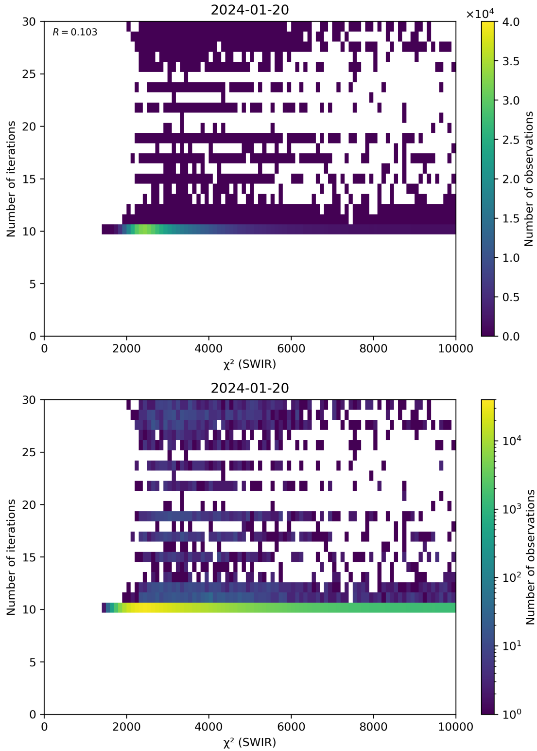
Figure 50: Scatter density plot of “ \chi^2 (SWIR)” against “Number of iterations” for 2024-01-19 to 2024-01-21.
