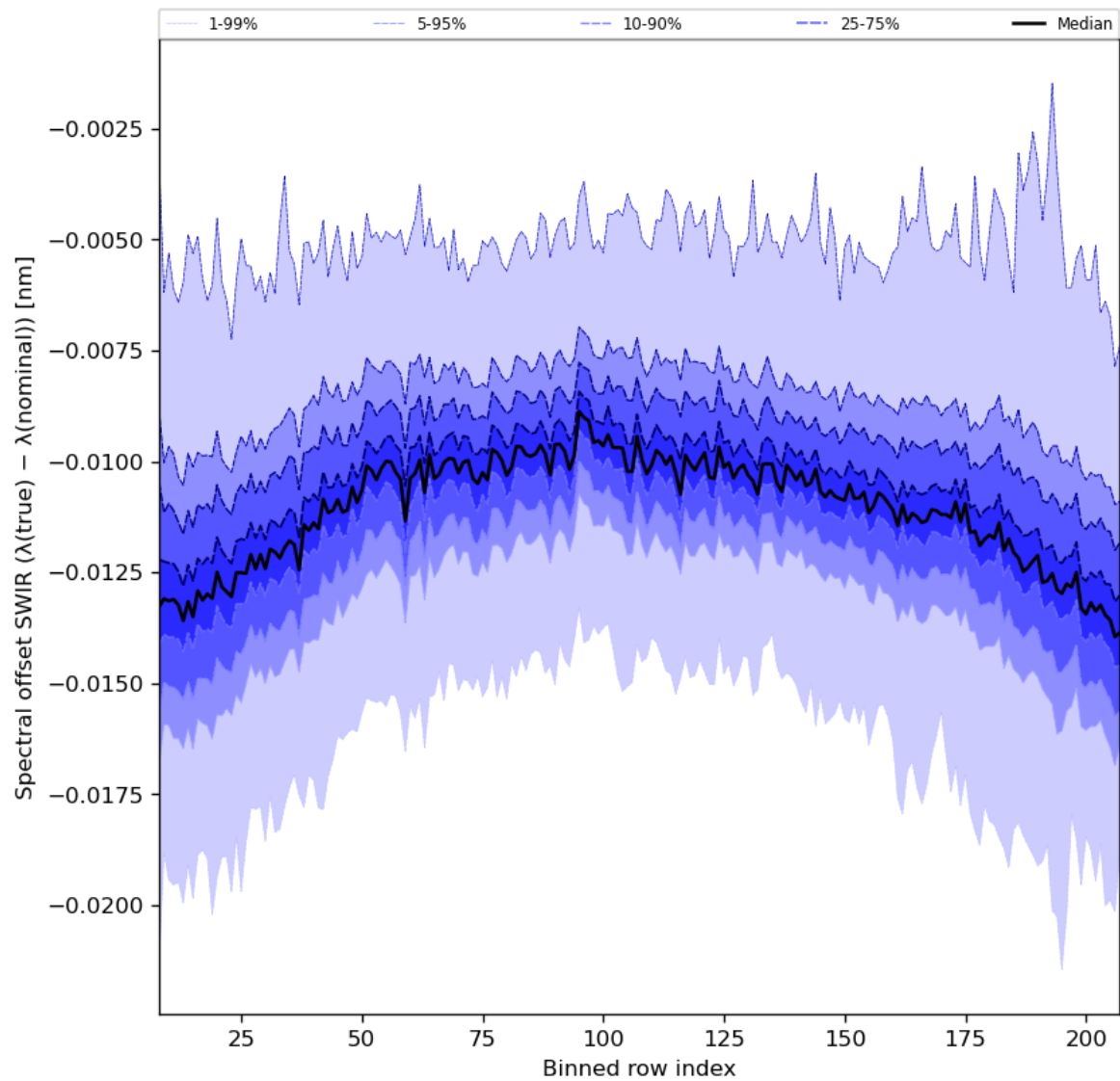
Figure 38: Along track statistics of “Spectral offset SWIR ( \lambda(\text{true}) - \lambda(\text{nominal}) )” for 2024-01-19 to 2024-01-21
