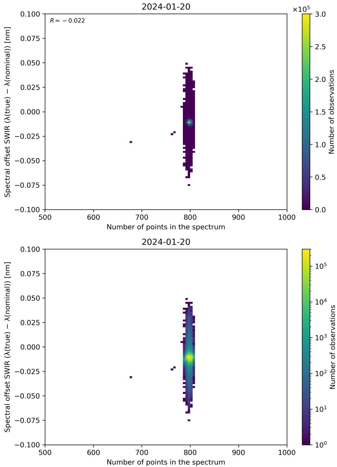
Figure 93: Scatter density plot of “Number of points in the spectrum” against “Spectral offset SWIR ( \lambda(\text{true}) - \lambda(\text{nominal}) )” for 2024-01-19 to 2024-01-21.
