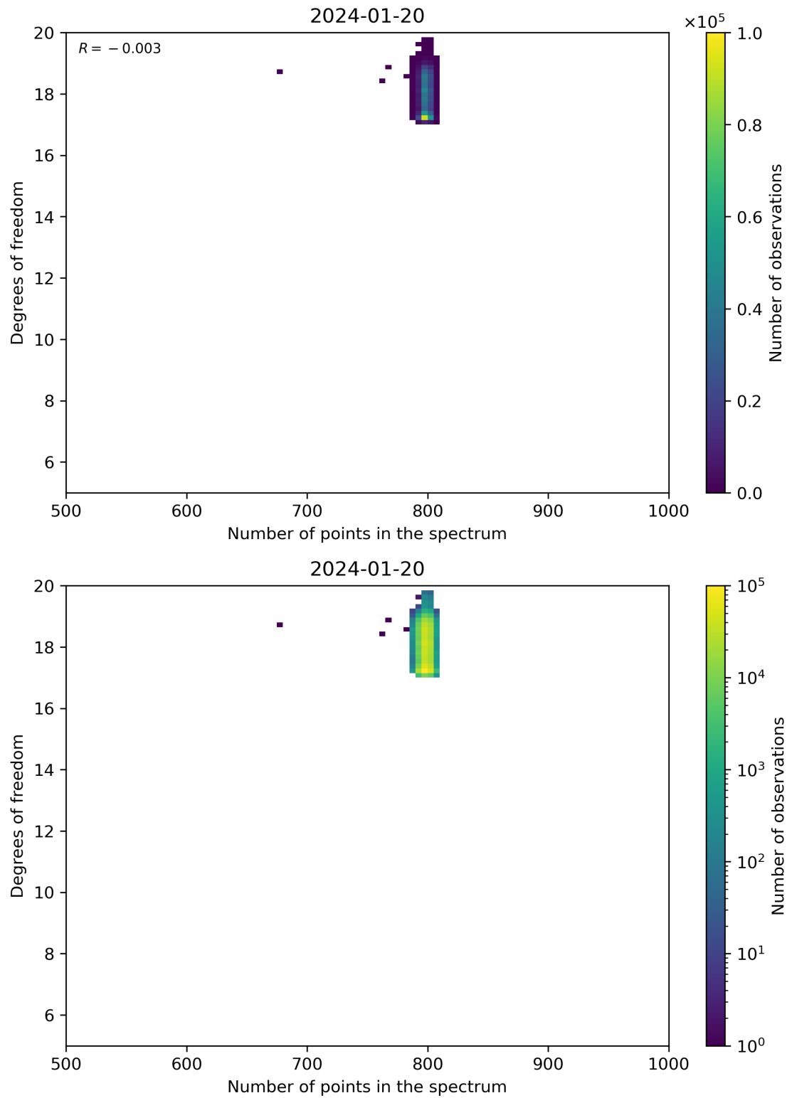
Figure 90: Scatter density plot of “Number of points in the spectrum” against “Degrees of freedom” for 2024-01-19 to 2024-01-21.
