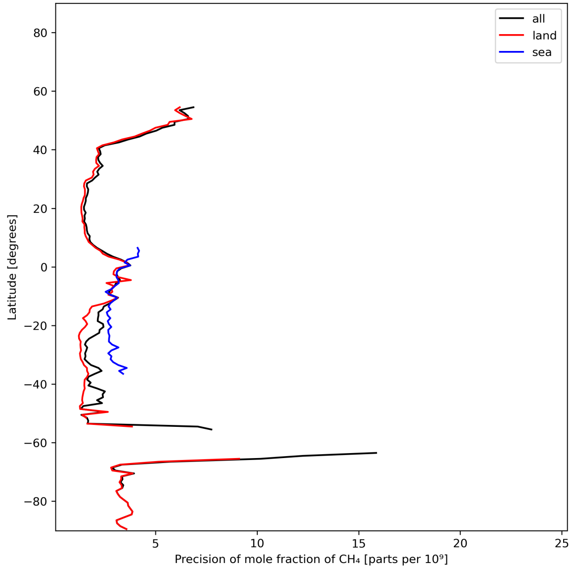
Figure 13: Zonal average of “Precision of mole fraction of CH 4 ” for 2024-01-19 to 2024-01-21.
