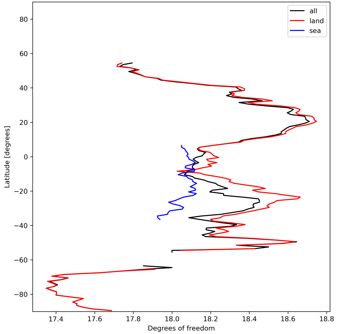
Figure 19: Zonal average of “Degrees of freedom” for 2024-01-19 to 2024-01-21.
