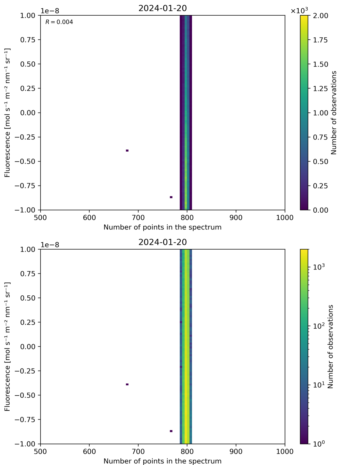
Figure 91: Scatter density plot of “Number of points in the spectrum” against “Fluorescence” for 2024-01-19 to 2024-01-21.
