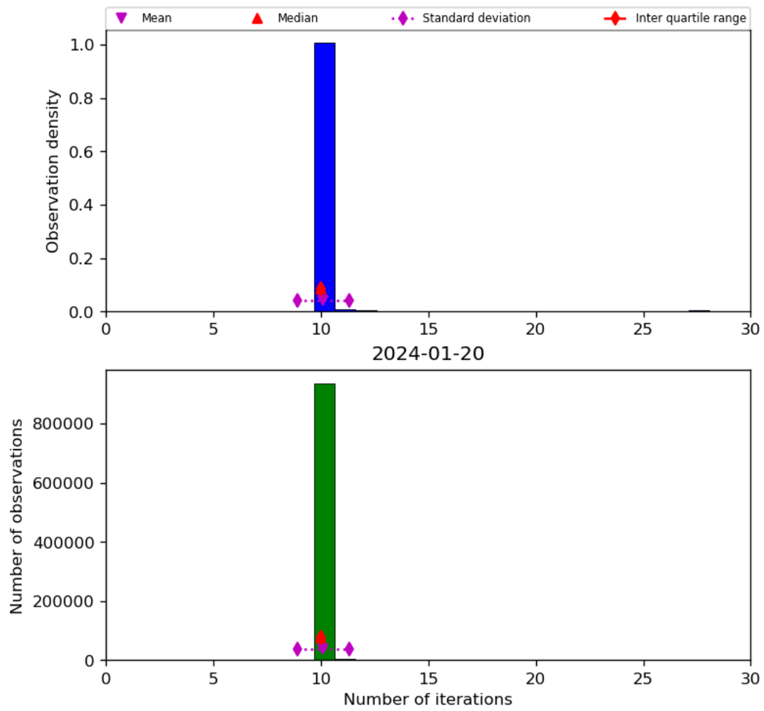
Figure 31: Histogram of “Number of iterations” for 2024-01-19 to 2024-01-21
