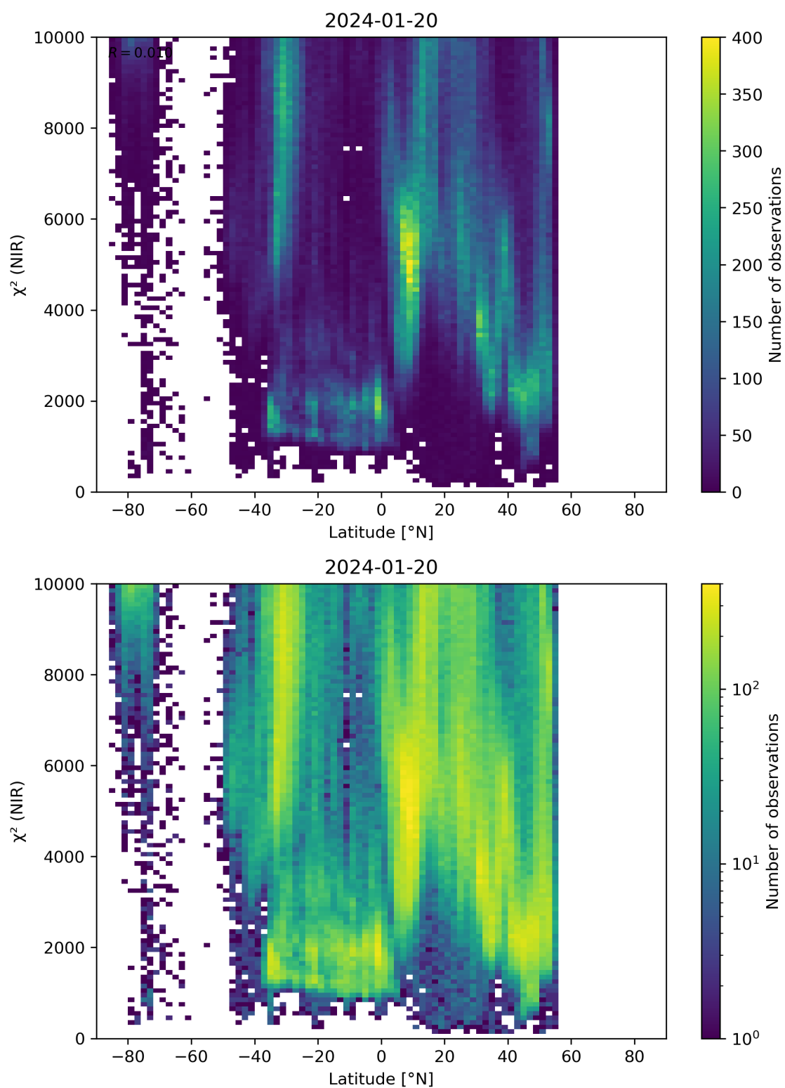
Figure 53: Scatter density plot of “Latitude” against “ \chi^2 (NIR)” for 2024-01-19 to 2024-01-21.
