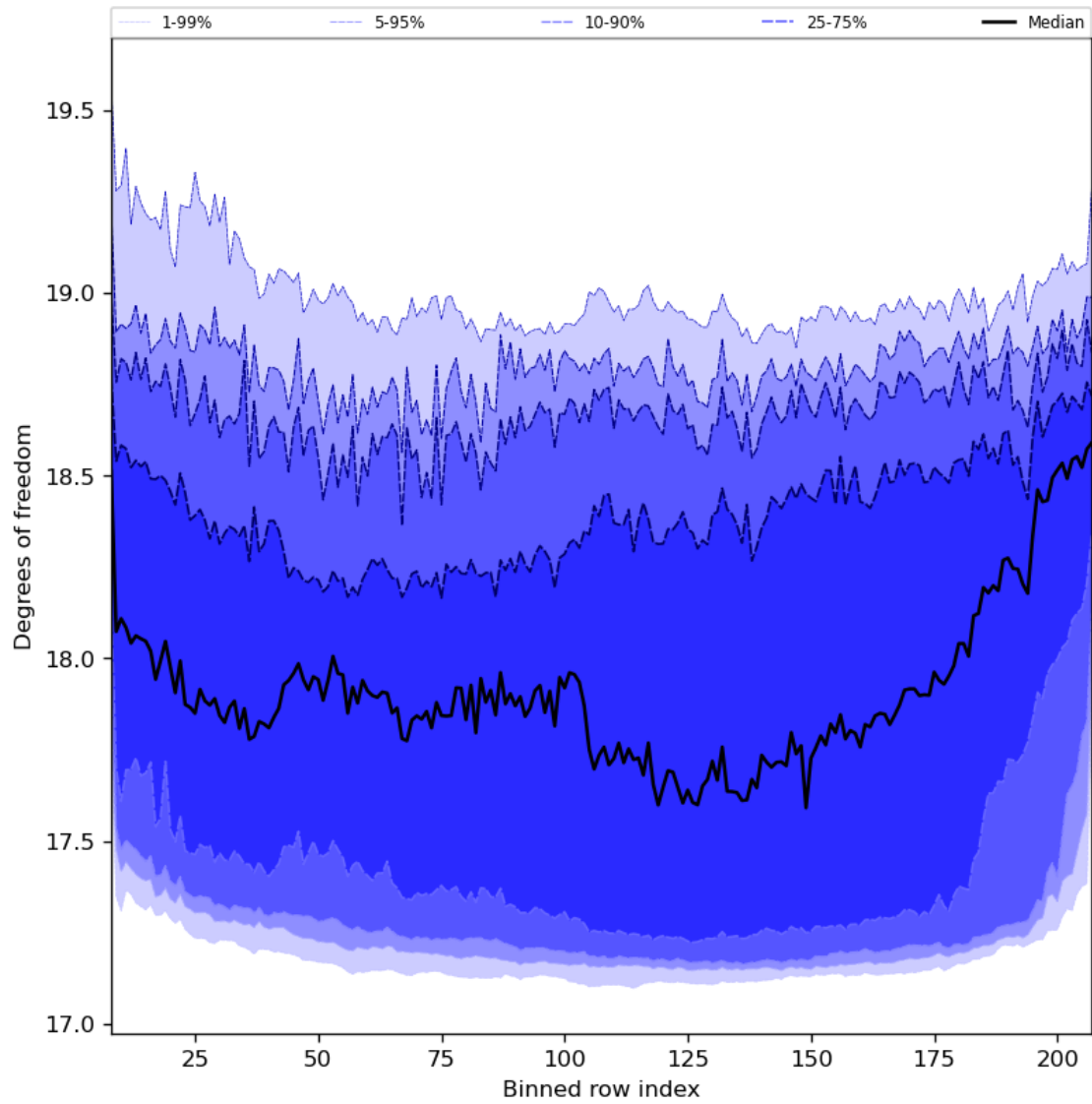
Figure 41: Along track statistics of “Degrees of freedom” for 2024-01-19 to 2024-01-21
