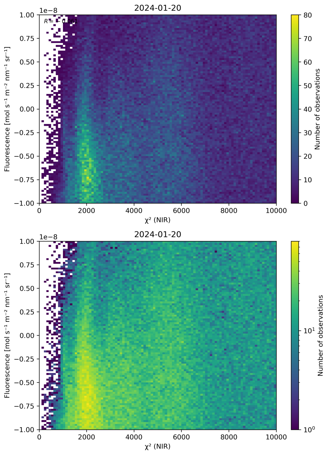
Figure 45: Scatter density plot of “ \chi^2 (NIR)” against “Fluorescence” for 2024-01-19 to 2024-01-21.
