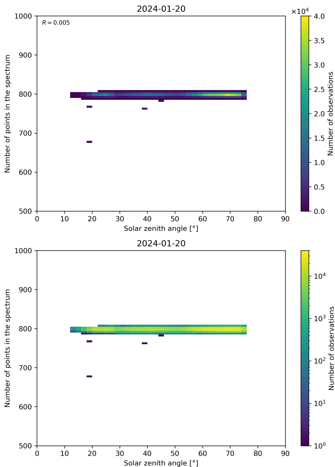
Figure 103: Scatter density plot of “Solar zenith angle” against “Number of points in the spectrum” for 2024-01-19 to 2024-01-21.
