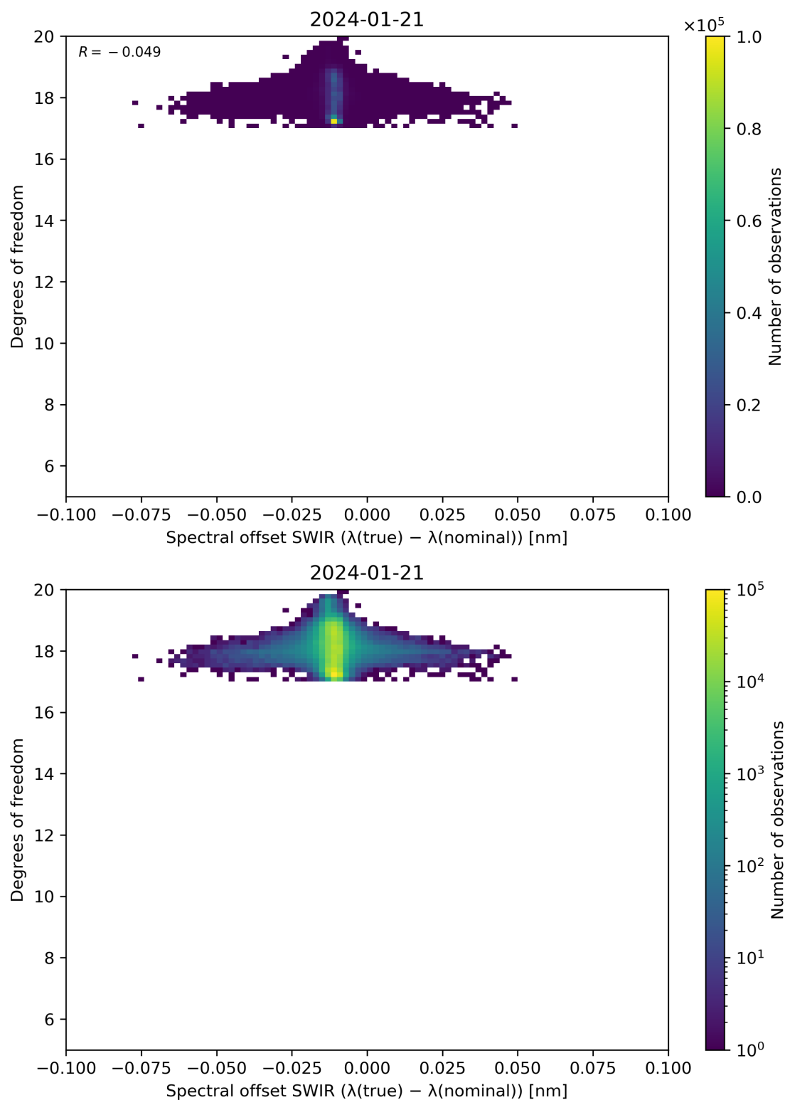
Figure 119: Scatter density plot of “Spectral offset SWIR ( \lambda(\text{true}) - \lambda(\text{nominal}) )” against “Degrees of freedom” for 2024-01-21 to 2024-01-22.
