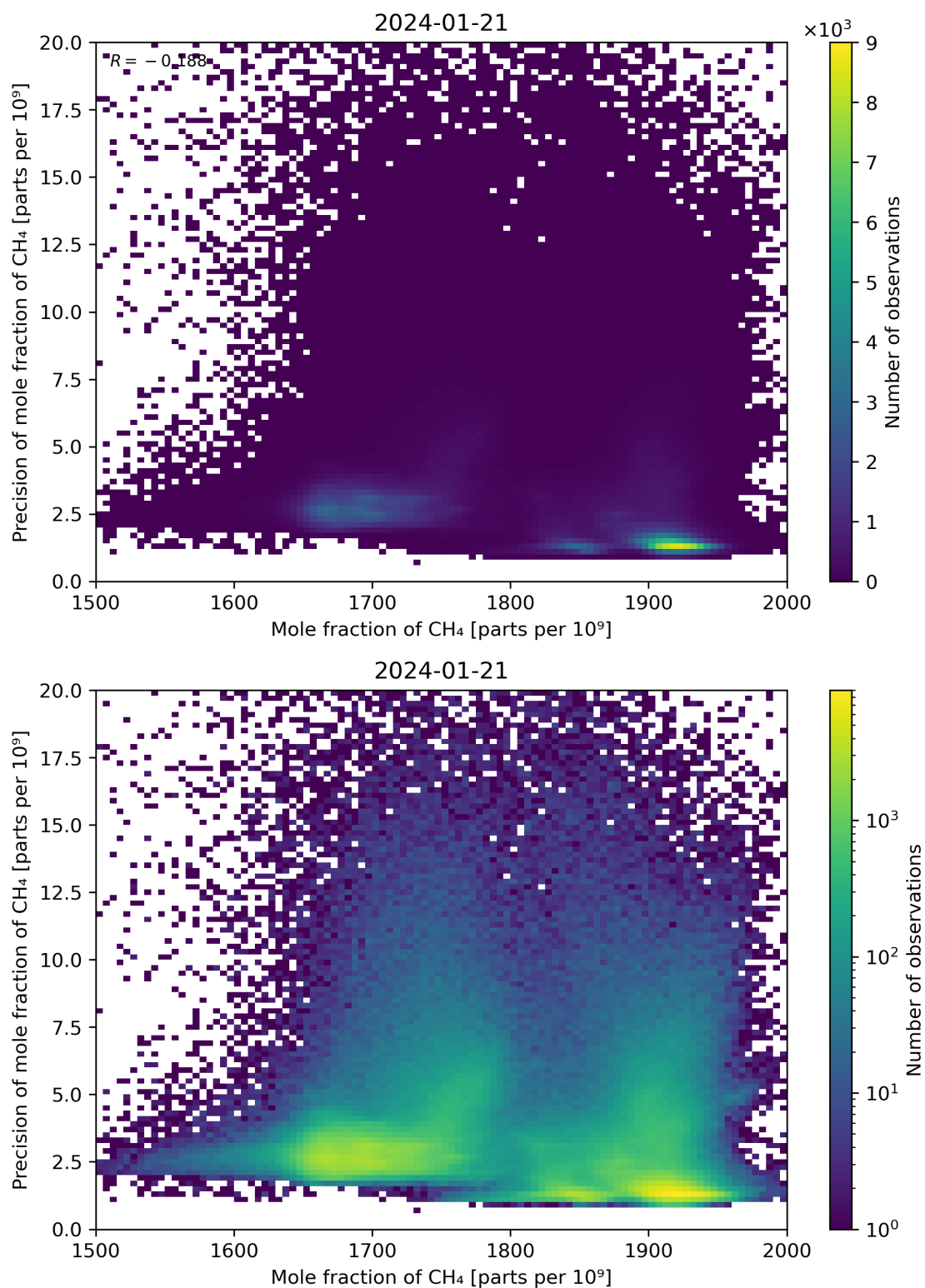
Figure 75: Scatter density plot of “Mole fraction of CH 4 ” against “Precision of mole fraction of CH 4 ” for 2024-01-21 to 2024-01-22.
