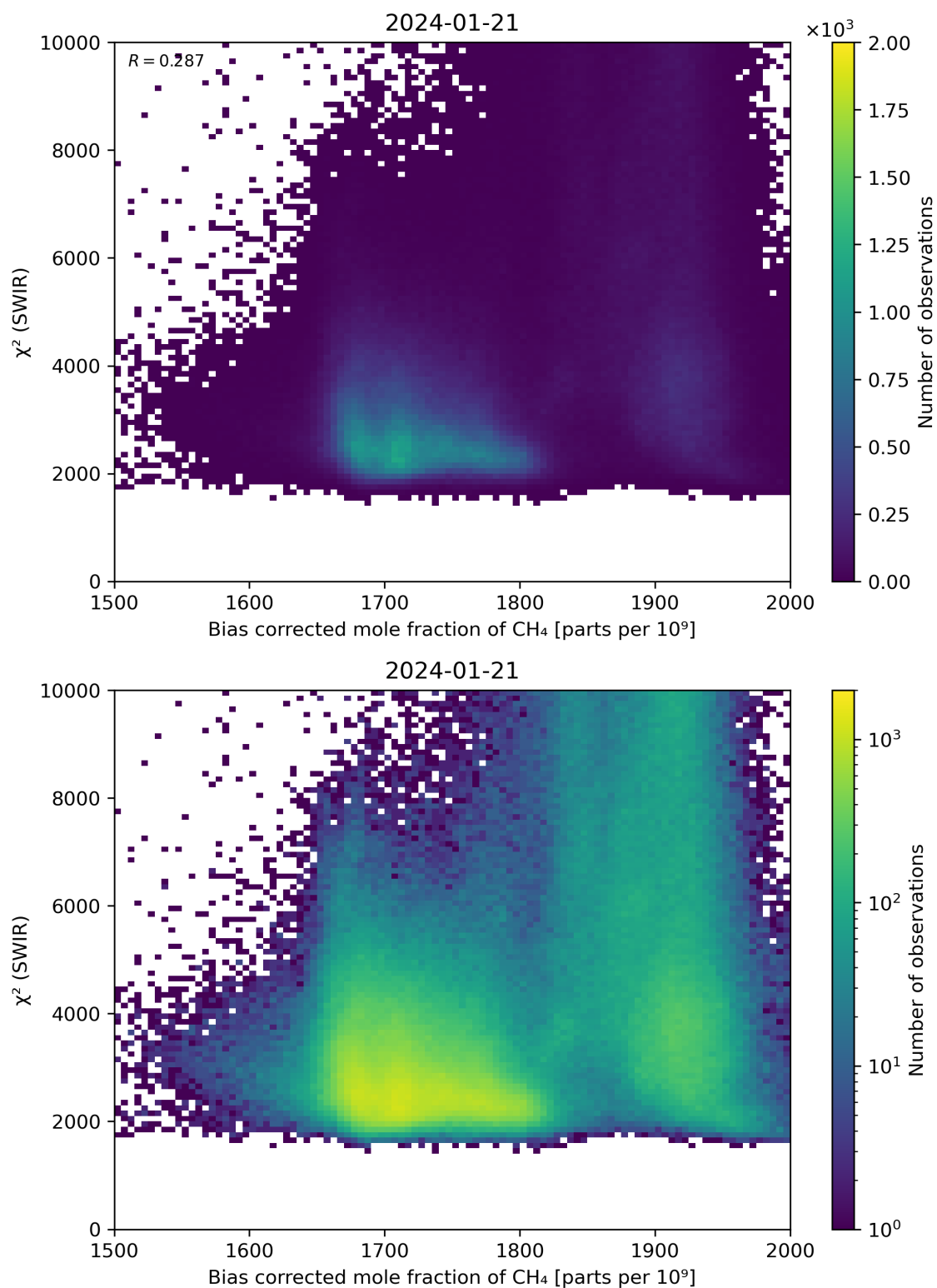
Figure 64: Scatter density plot of “Bias corrected mole fraction of CH 4 ” against “ \chi^2 (SWIR)” for 2024-01-21 to 2024-01-22.
