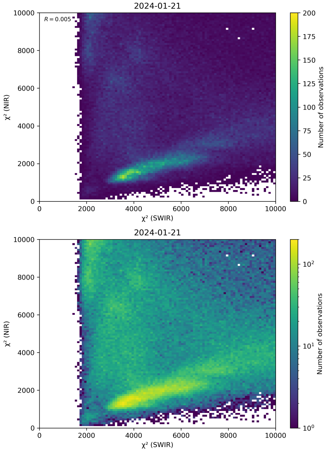
Figure 47: Scatter density plot of “ \chi^2 (SWIR)” against “ \chi^2 (NIR)” for 2024-01-21 to 2024-01-22.
