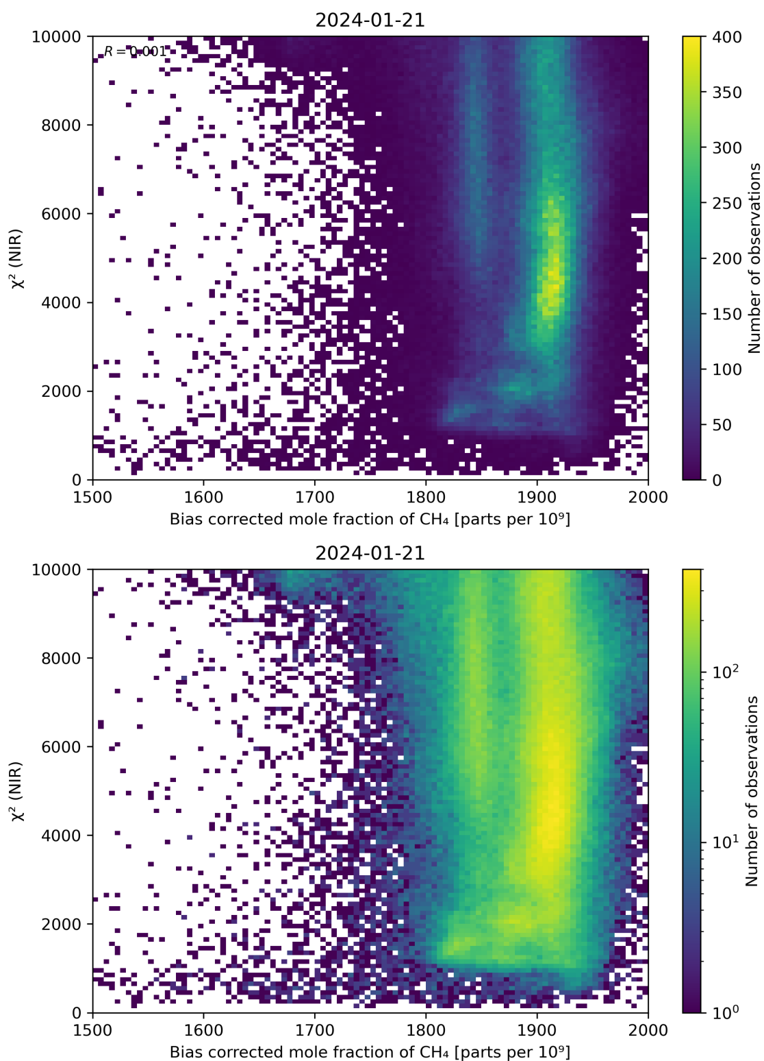
Figure 63: Scatter density plot of “Bias corrected mole fraction of CH 4 ” against “ \chi^2 (NIR)” for 2024-01-21 to 2024-01-22.
