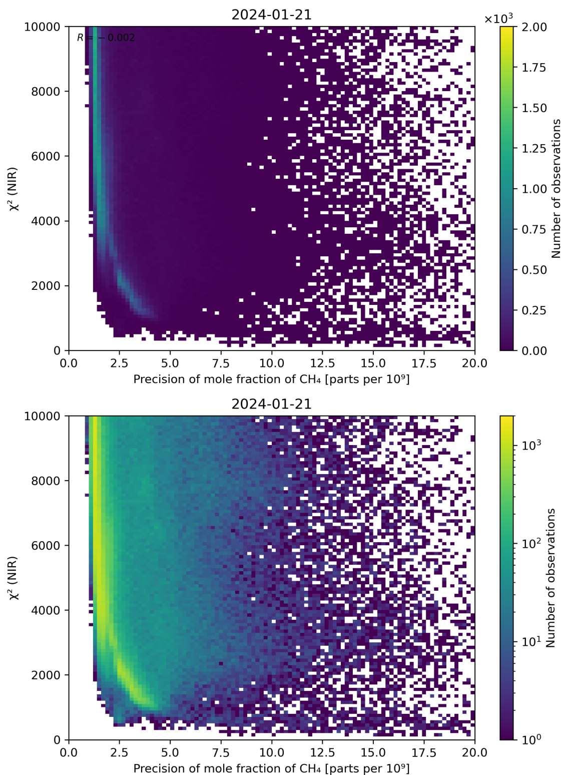
Figure 78: Scatter density plot of “Precision of mole fraction of CH 4 ” against “ \chi^2 (NIR)” for 2024-01-21 to 2024-01-22.
