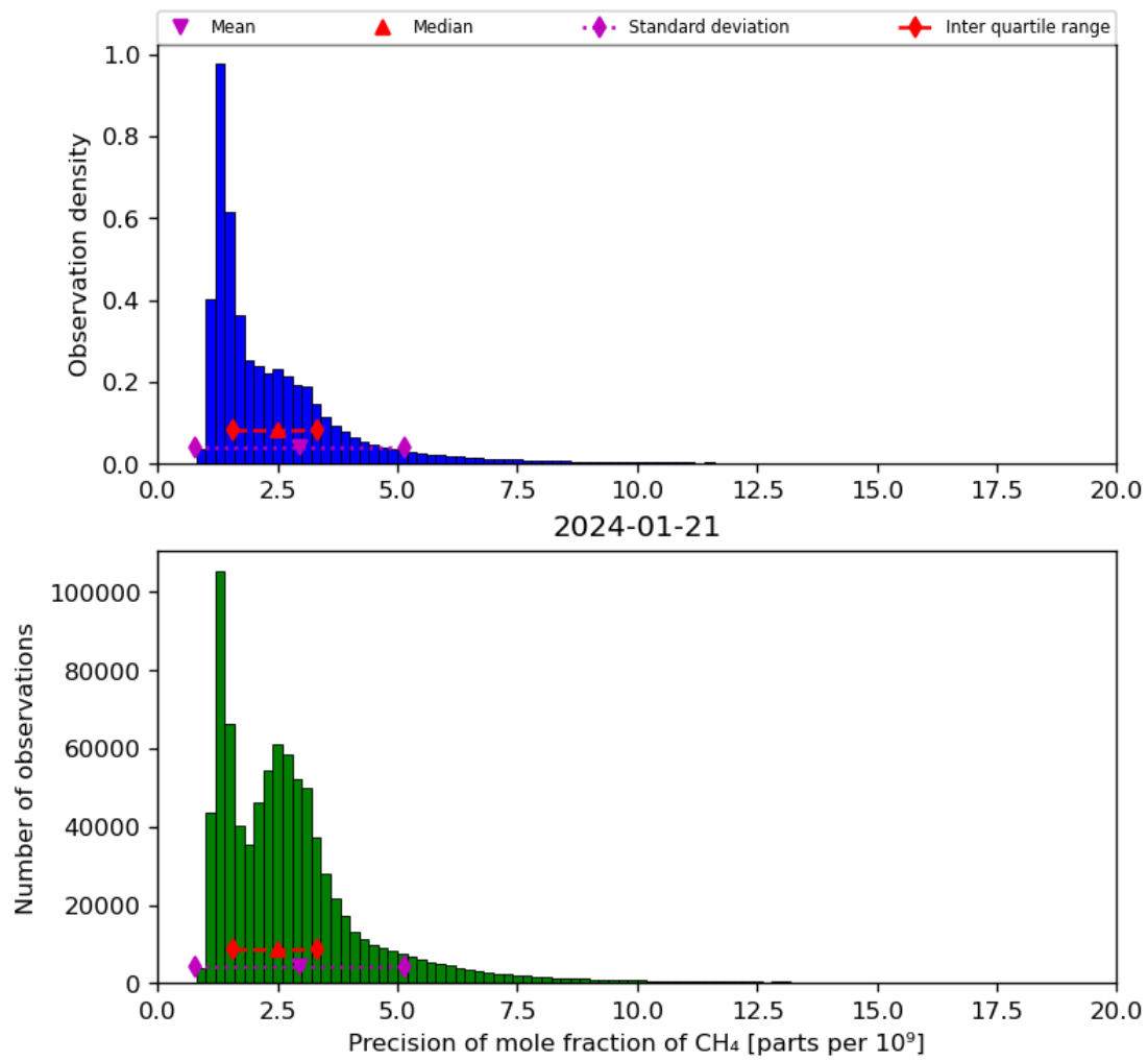
Figure 24: Histogram of “Precision of mole fraction of CH 4 ” for 2024-01-21 to 2024-01-22
