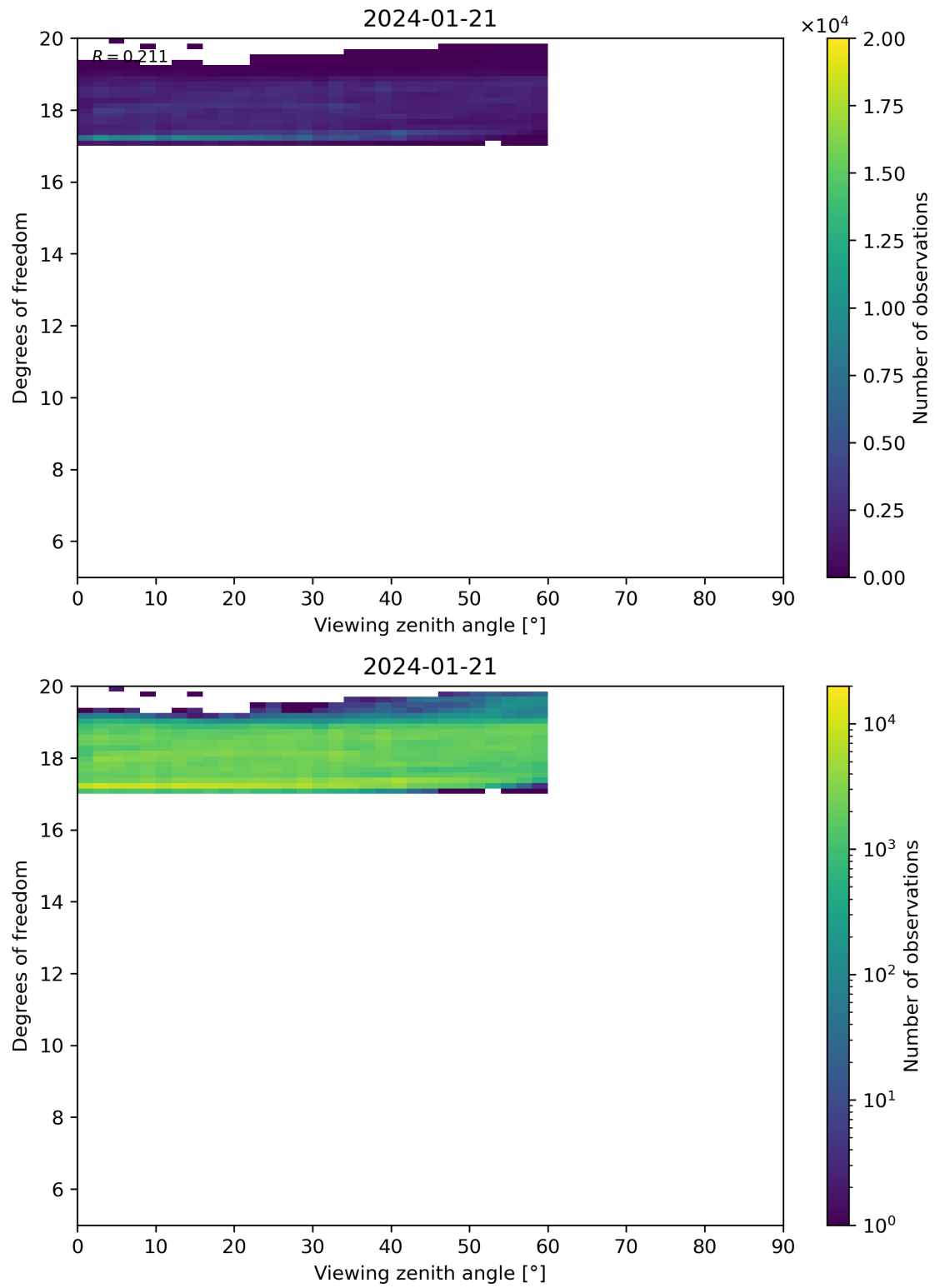
Figure 107: Scatter density plot of “Viewing zenith angle” against “Degrees of freedom” for 2024-01-21 to 2024-01-22.
