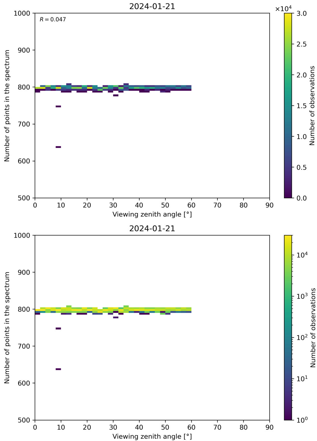
Figure 114: Scatter density plot of “Viewing zenith angle” against “Number of points in the spectrum” for 2024-01-21 to 2024-01-22.
