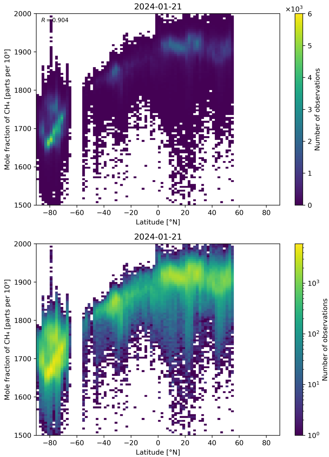
Figure 57: Scatter density plot of “Latitude” against “Mole fraction of CH 4 ” for 2024-01-21 to 2024-01-22.
