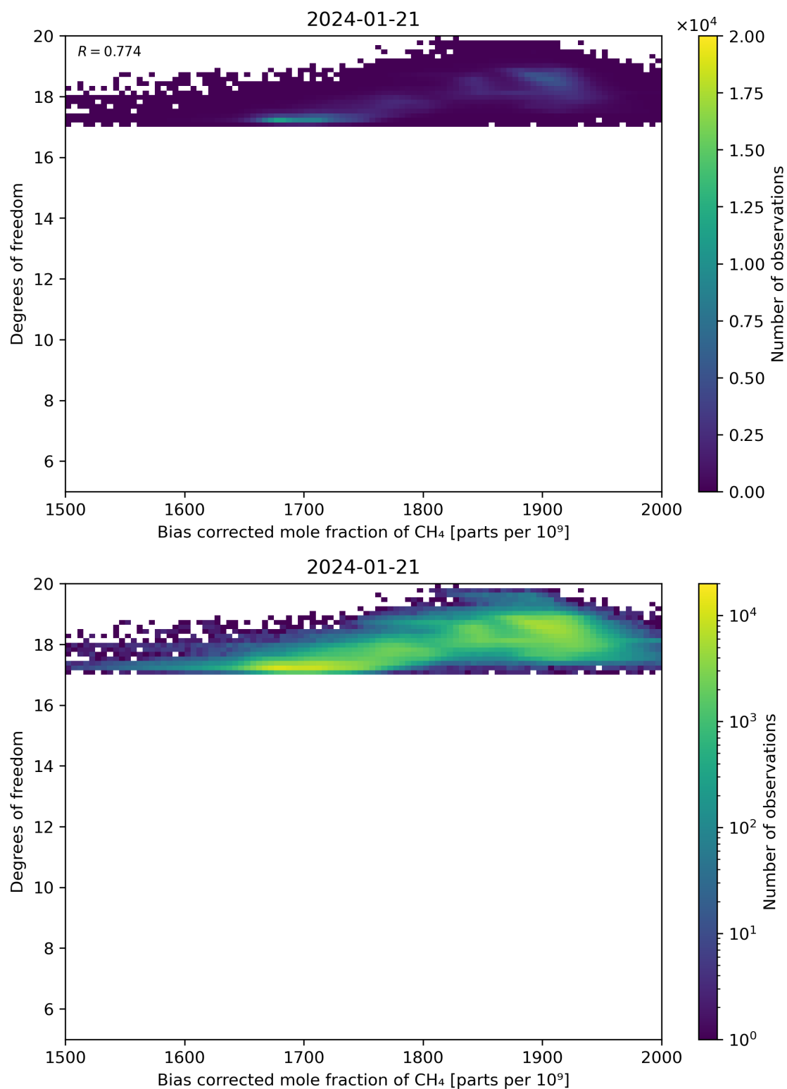
Figure 65: Scatter density plot of “Bias corrected mole fraction of CH 4 ” against “Degrees of freedom” for 2024-01-21 to 2024-01-22.
