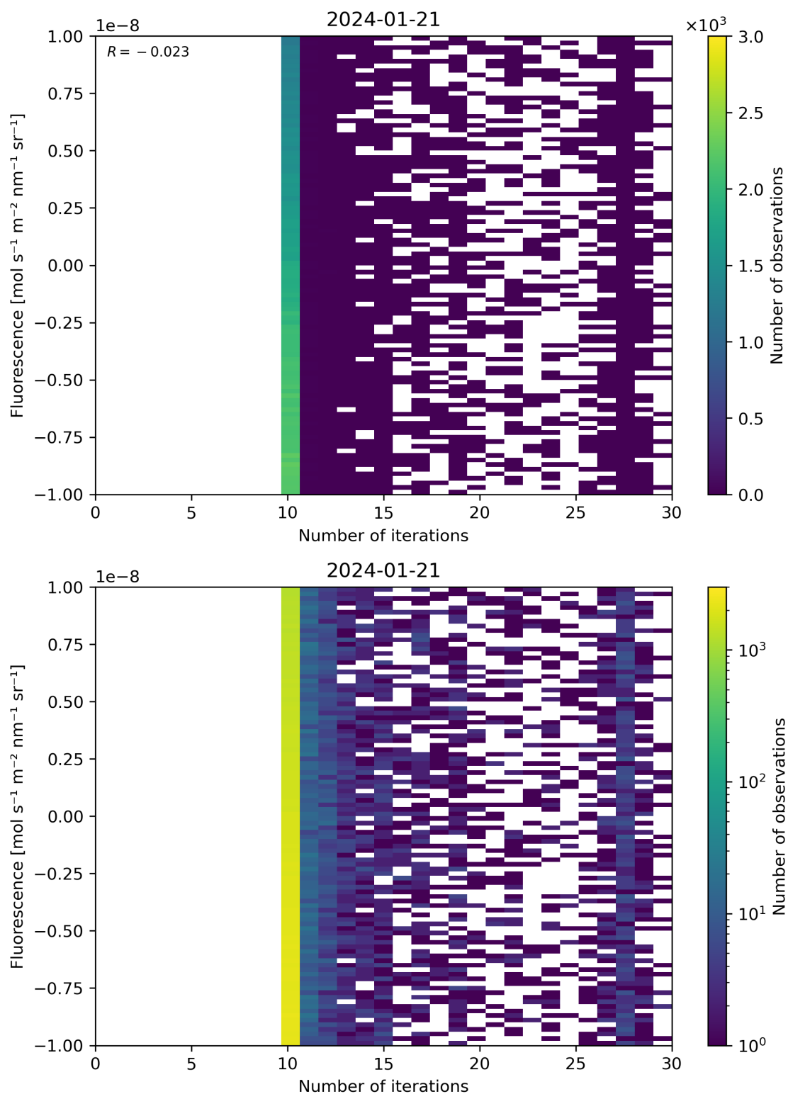
Figure 87: Scatter density plot of “Number of iterations” against “Fluorescence” for 2024-01-21 to 2024-01-22.
