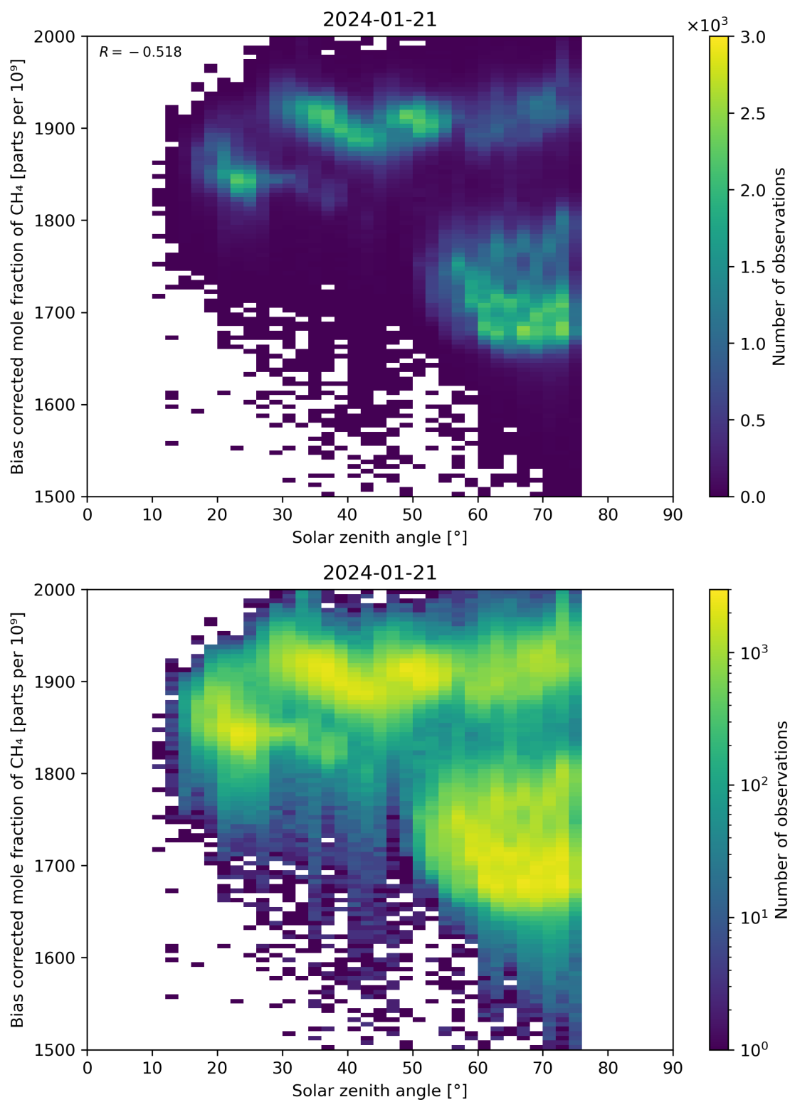
Figure 100: Scatter density plot of “Solar zenith angle” against “Bias corrected mole fraction of \text{CH}_4 ” for 2024-01-21 to 2024-01-22.
