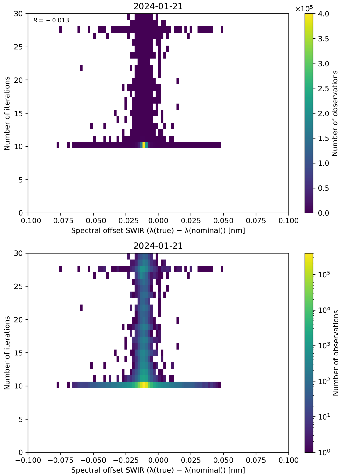
Figure 121: Scatter density plot of “Spectral offset SWIR ( \lambda(\text{true}) - \lambda(\text{nominal}) )” against “Number of iterations” for 2024-01-21 to 2024-01-22.
