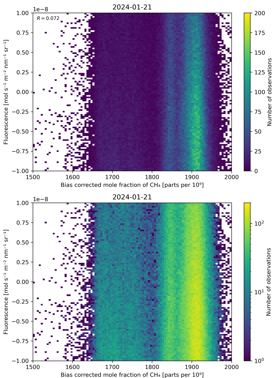
Figure 66: Scatter density plot of “Bias corrected mole fraction of \text{CH}_4 ” against “Fluorescence” for 2024-01-21 to 2024-01-22.
