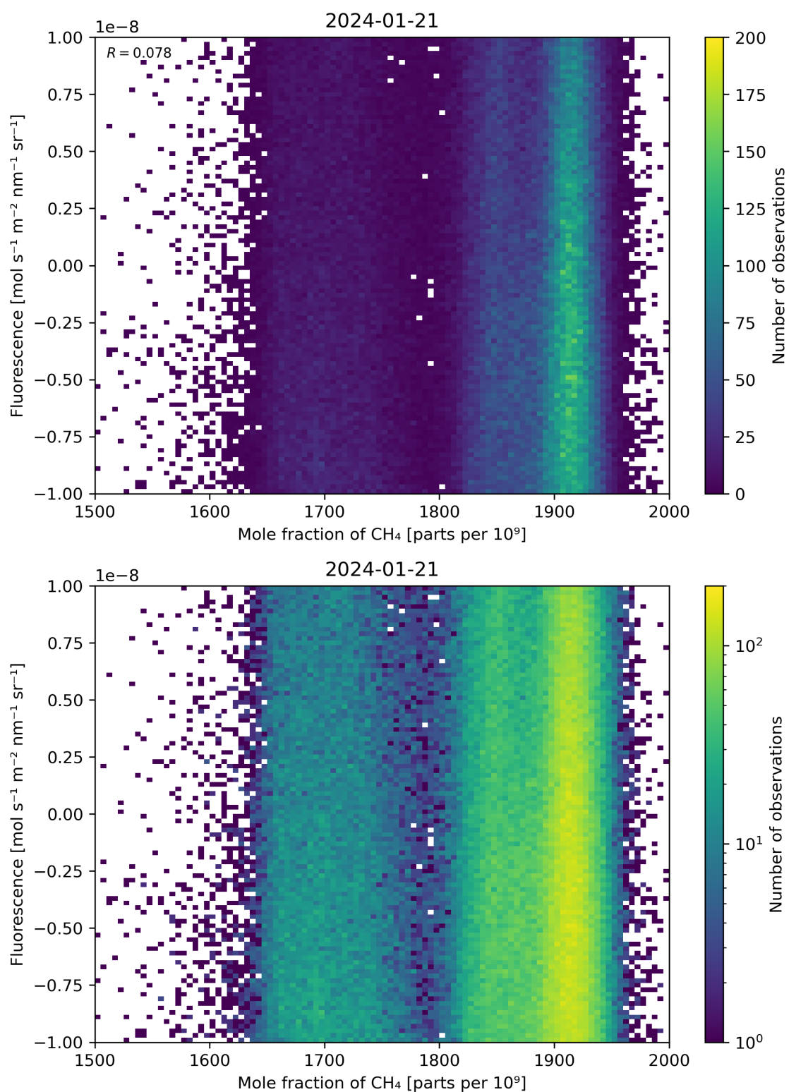
Figure 73: Scatter density plot of “Mole fraction of \text{CH}_4 ” against “Fluorescence” for 2024-01-21 to 2024-01-22.
