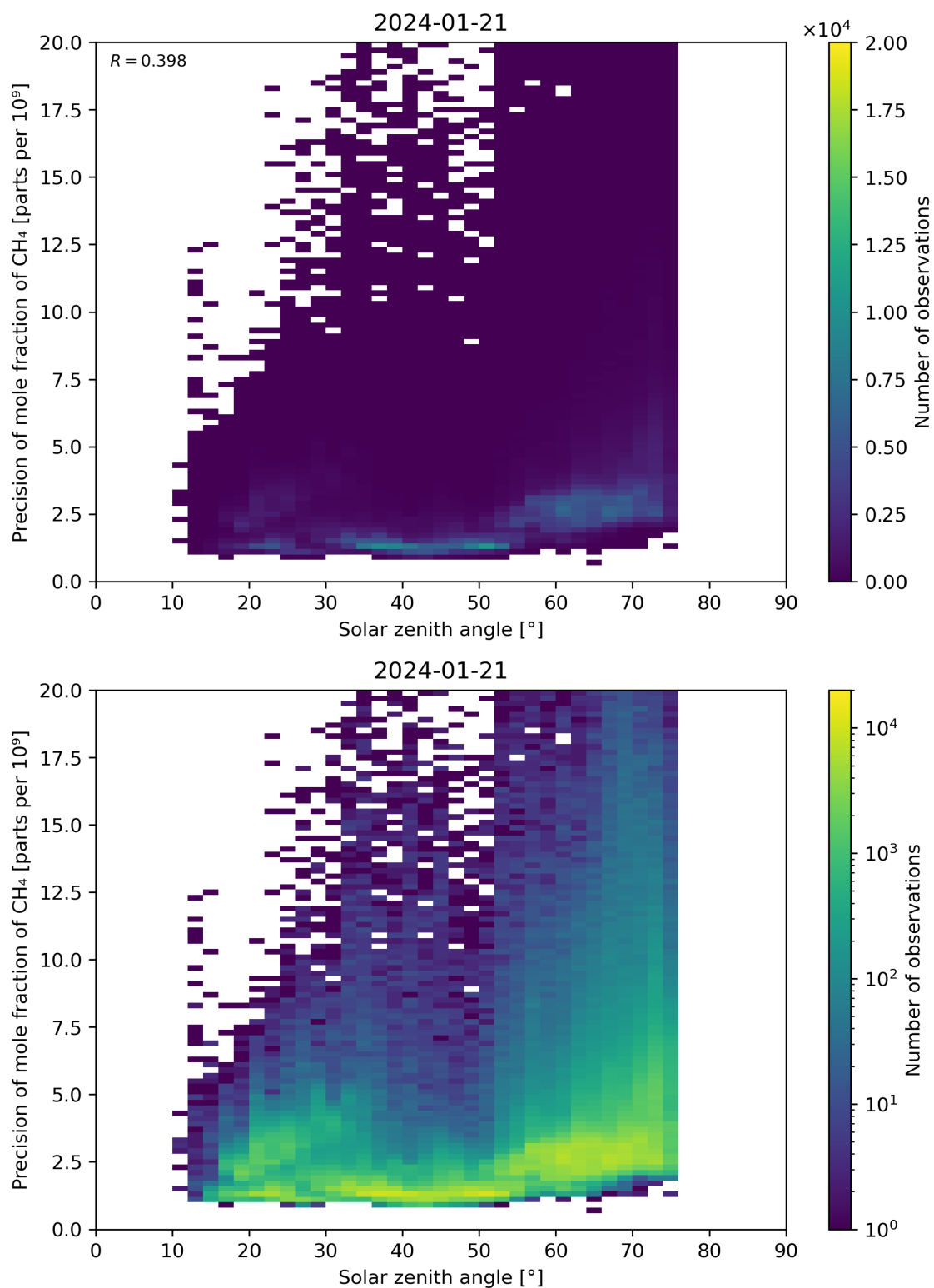
Figure 101: Scatter density plot of “Solar zenith angle” against “Precision of mole fraction of CH 4 ” for 2024-01-21 to 2024-01-22.
