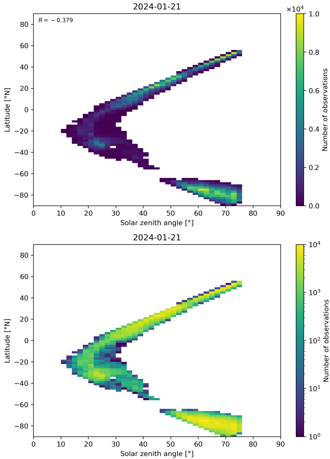
Figure 98: Scatter density plot of “Solar zenith angle” against “Latitude” for 2024-01-21 to 2024-01-22.
