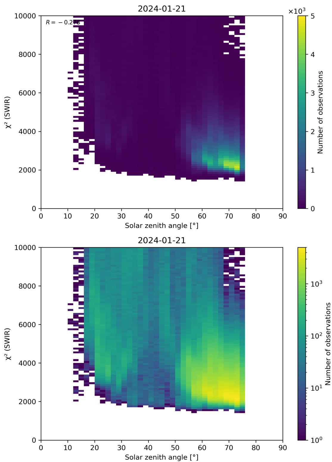
Figure 95: Scatter density plot of “Solar zenith angle” against “ \chi^2 (SWIR)” for 2024-01-21 to 2024-01-22.
