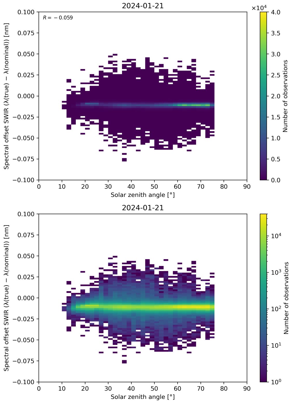
Figure 104: Scatter density plot of “Solar zenith angle” against “Spectral offset SWIR ( \lambda(\text{true}) - \lambda(\text{nominal}) )” for 2024-01-21 to 2024-01-22.
