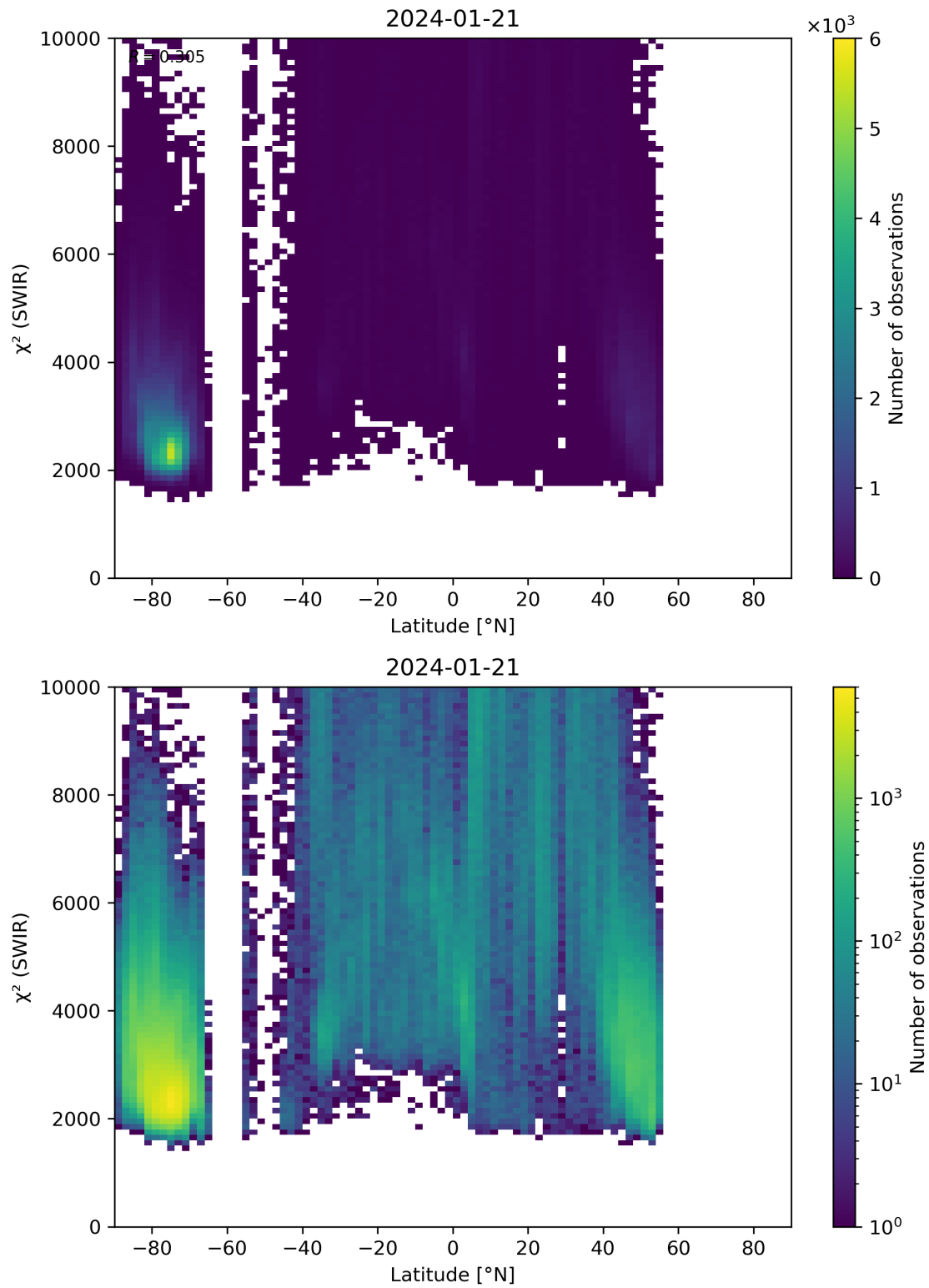
Figure 54: Scatter density plot of “Latitude” against “ \chi^2 (SWIR)” for 2024-01-21 to 2024-01-22.
