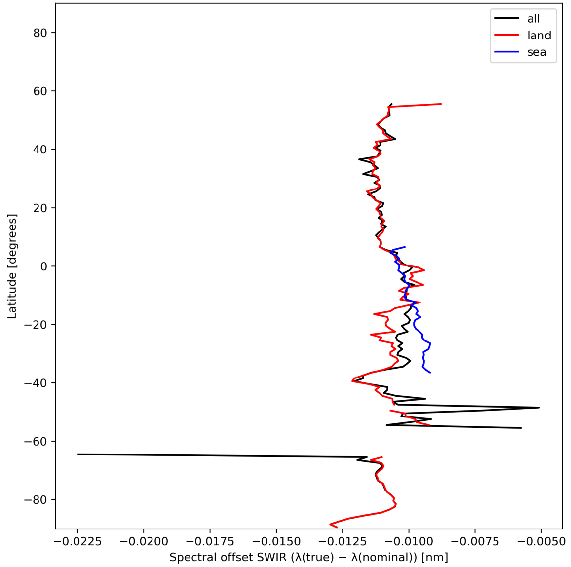
Figure 16: Zonal average of “Spectral offset SWIR ( \lambda(\text{true}) - \lambda(\text{nominal}) )” for 2024-01-21 to 2024-01-22.
