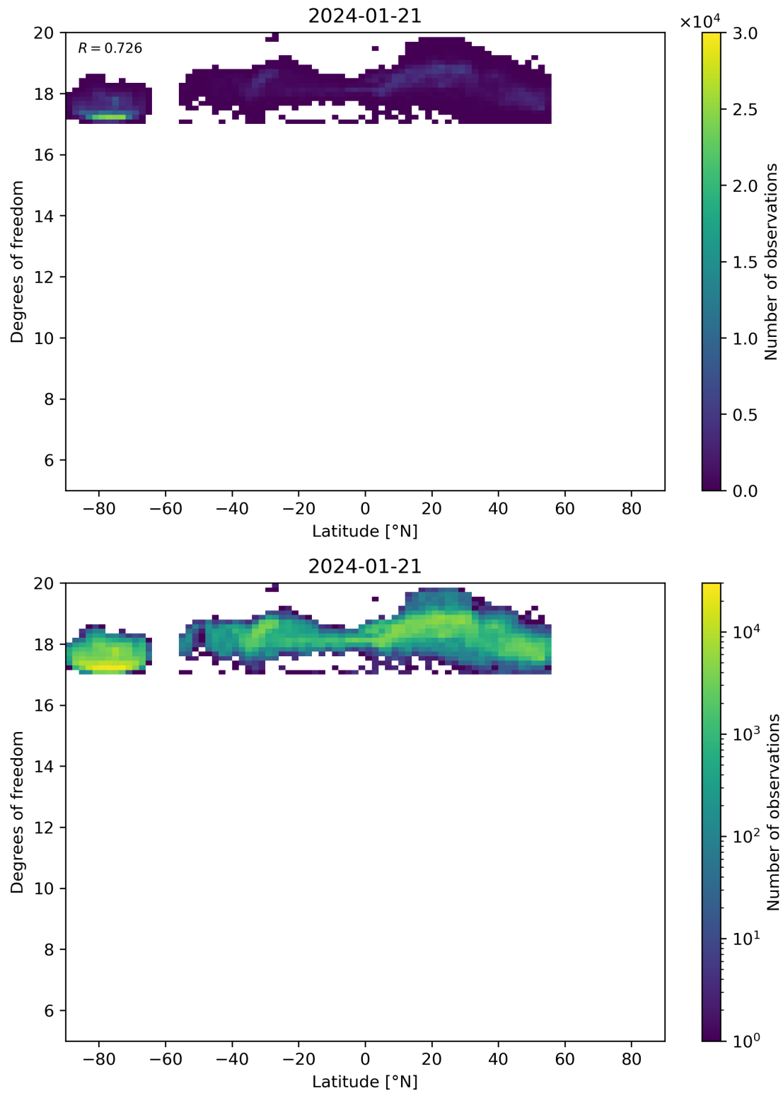
Figure 55: Scatter density plot of “Latitude” against “Degrees of freedom” for 2024-01-21 to 2024-01-22.
