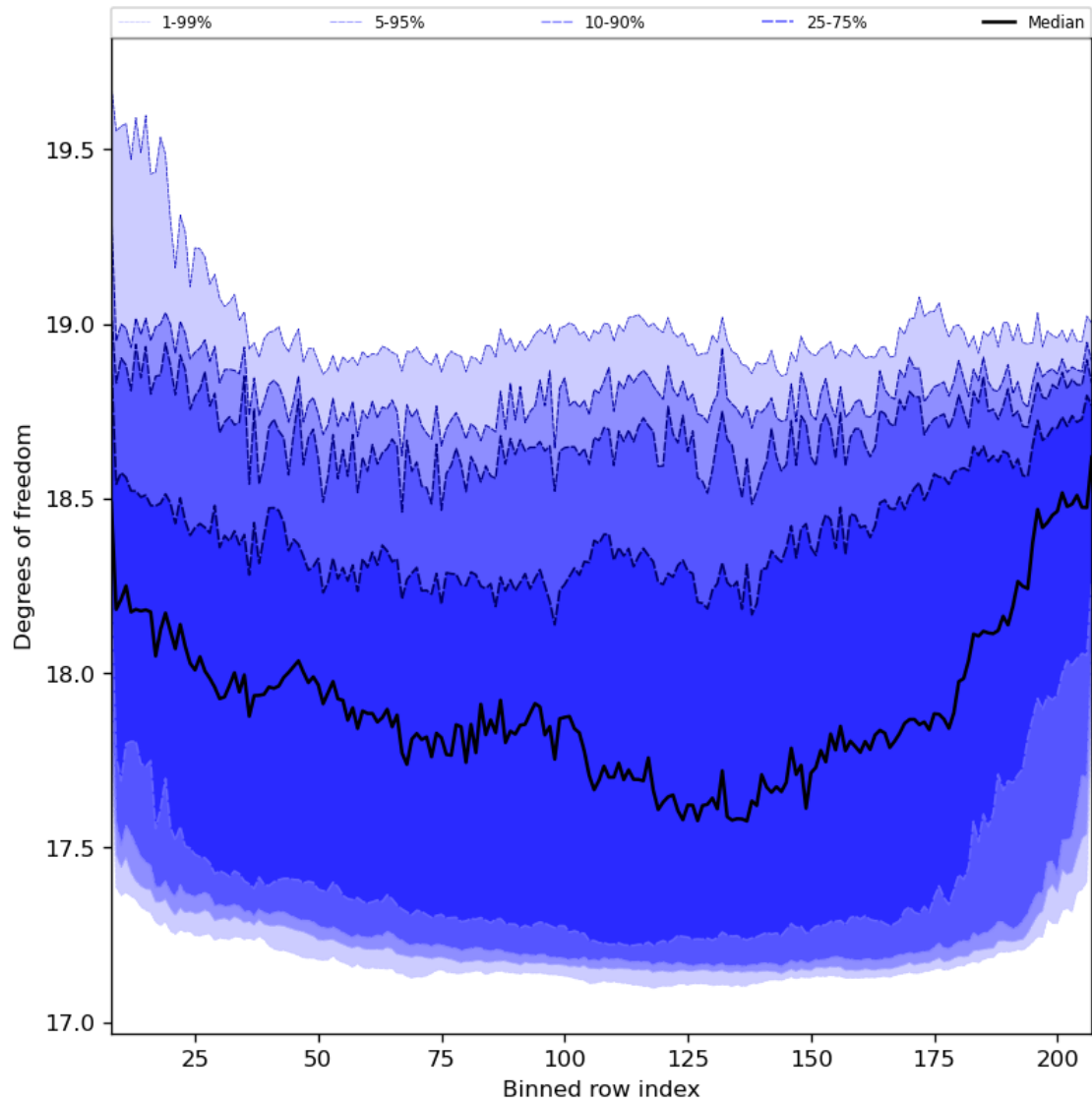
Figure 41: Along track statistics of “Degrees of freedom” for 2024-01-21 to 2024-01-22
