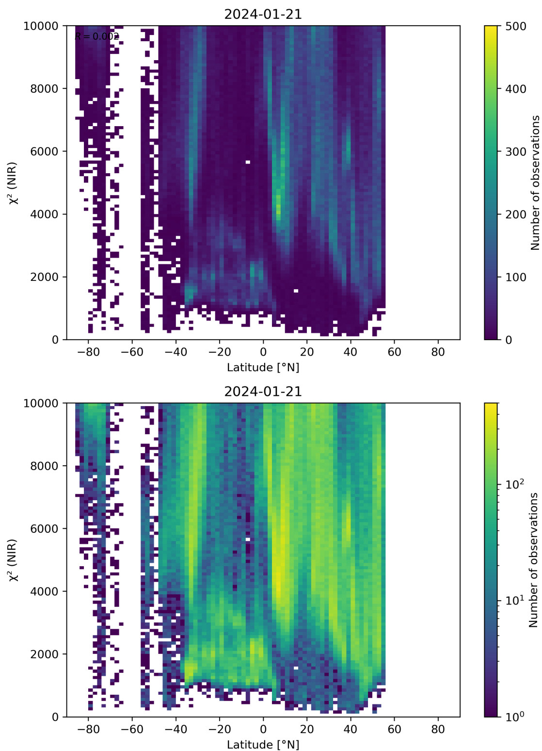
Figure 53: Scatter density plot of “Latitude” against “ \chi^2 (NIR)” for 2024-01-21 to 2024-01-22.
