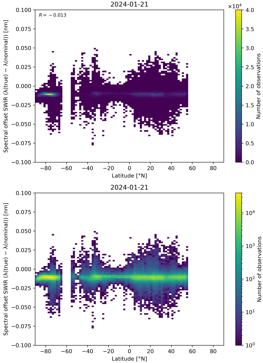
Figure 62: Scatter density plot of “Latitude” against “Spectral offset SWIR ( \lambda(\text{true}) - \lambda(\text{nominal}) )” for 2024-01-21 to 2024-01-22.
