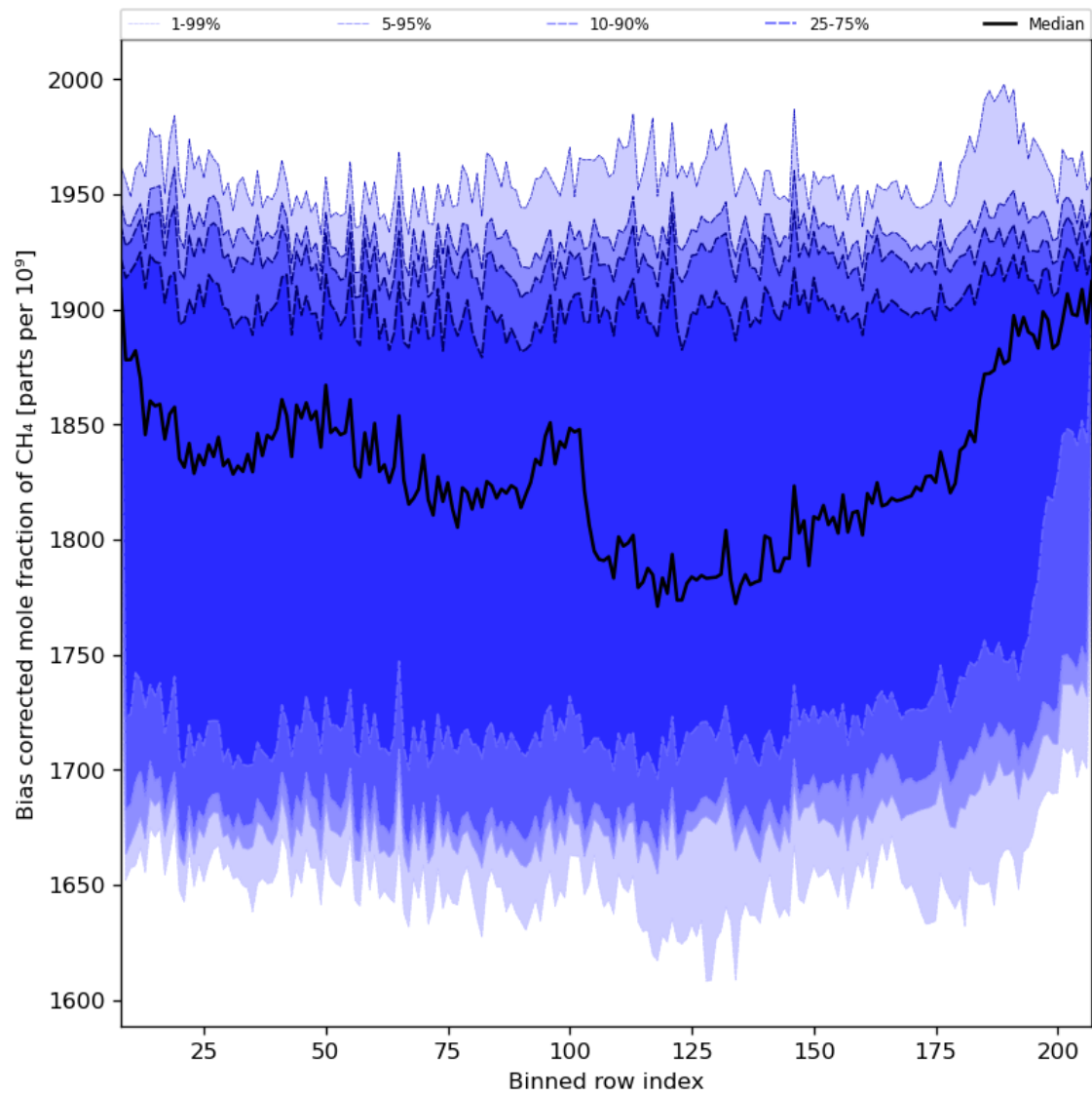
Figure 36: Along track statistics of “Bias corrected mole fraction of CH 4 ” for 2024-01-21 to 2024-01-22
