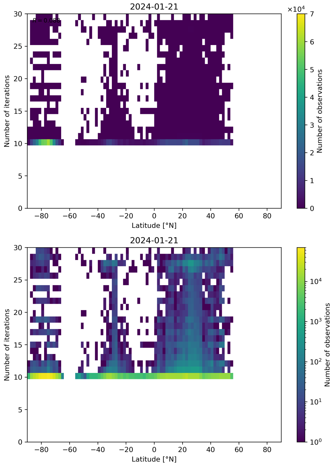
Figure 60: Scatter density plot of “Latitude” against “Number of iterations” for 2024-01-21 to 2024-01-22.
