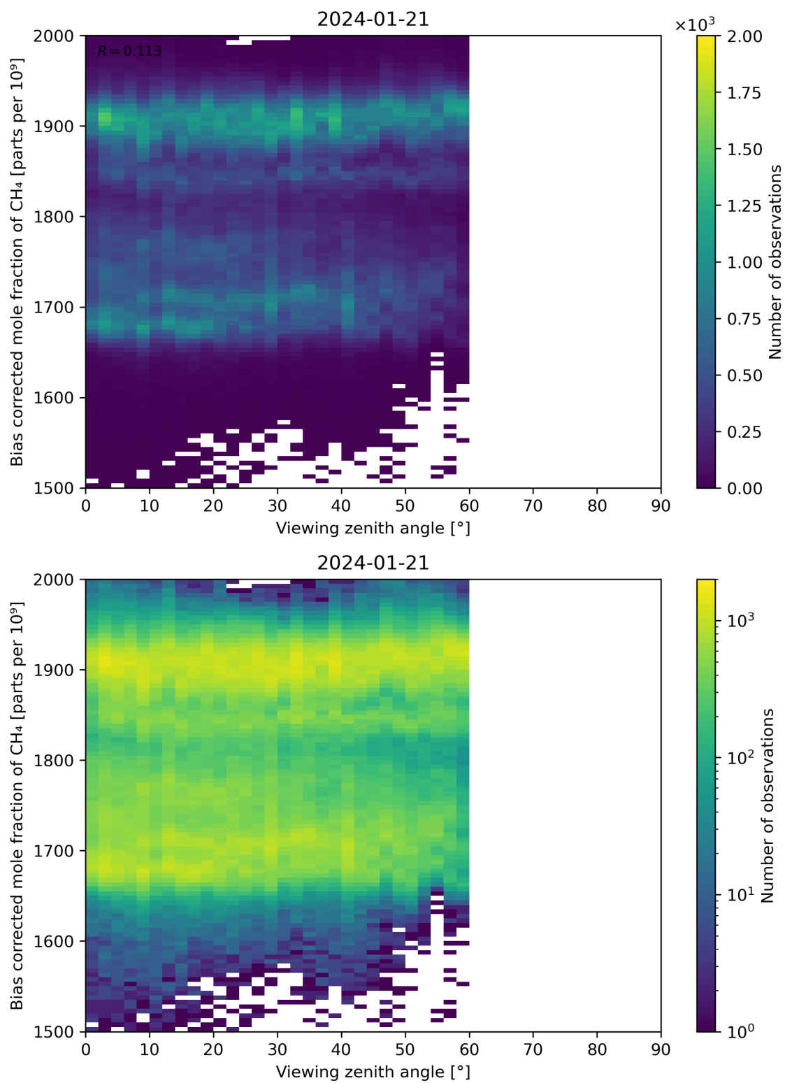
Figure 111: Scatter density plot of “Viewing zenith angle” against “Bias corrected mole fraction of CH 4 ” for 2024-01-21 to 2024-01-22.
