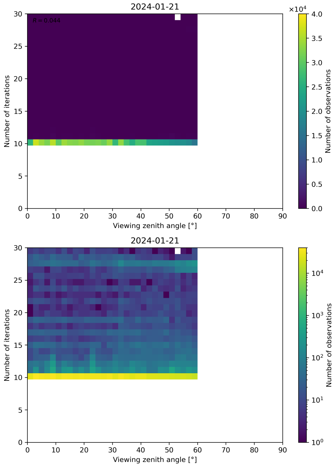
Figure 113: Scatter density plot of “Viewing zenith angle” against “Number of iterations” for 2024-01-21 to 2024-01-22.
