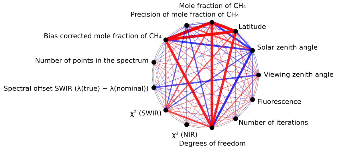
Figure 1: Map of correlation graph for 2024-01-21 to 2024-01-22.
