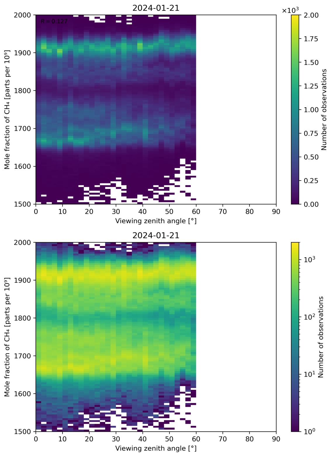
Figure 110: Scatter density plot of “Viewing zenith angle” against “Mole fraction of \text{CH}_4 ” for 2024-01-21 to 2024-01-22.
