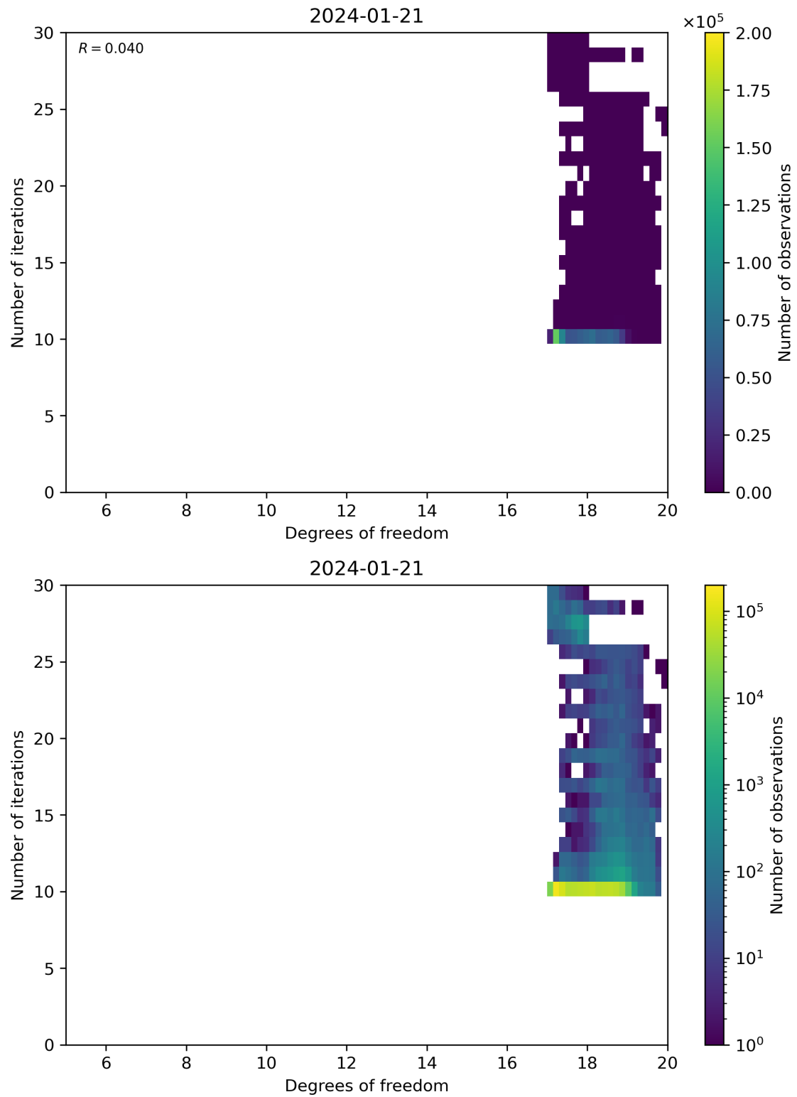
Figure 52: Scatter density plot of “Degrees of freedom” against “Number of iterations” for 2024-01-21 to 2024-01-22.
