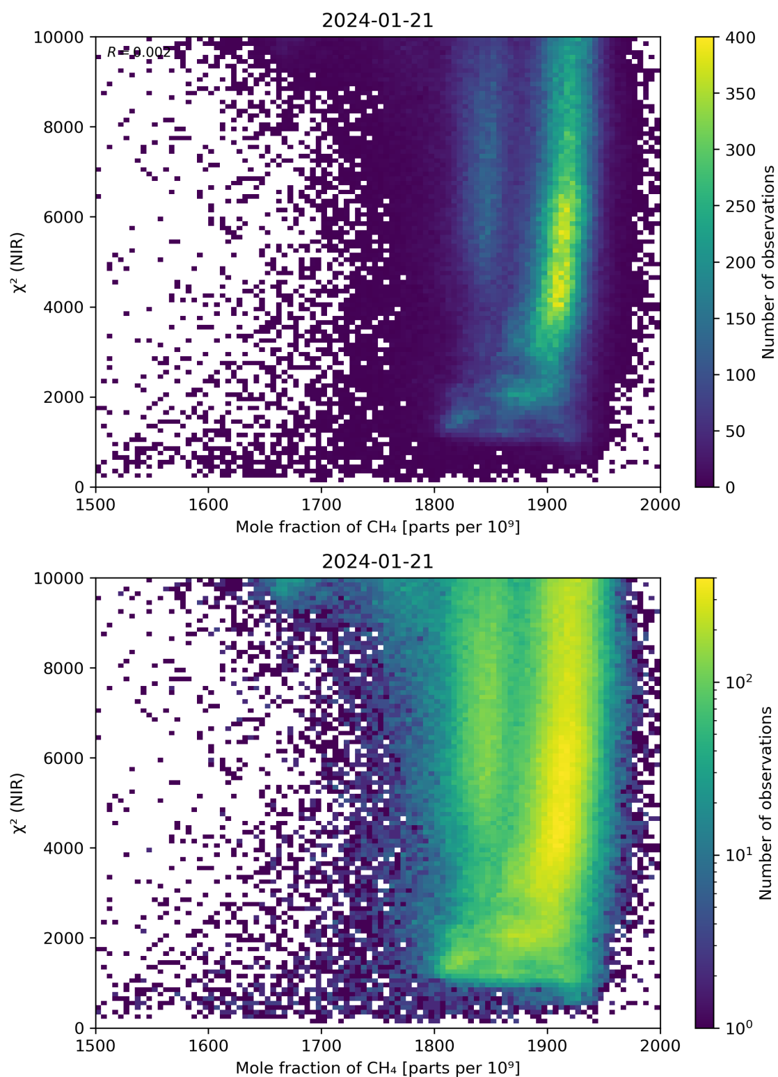
Figure 70: Scatter density plot of “Mole fraction of CH 4 ” against “ \chi^2 (NIR)” for 2024-01-21 to 2024-01-22.
