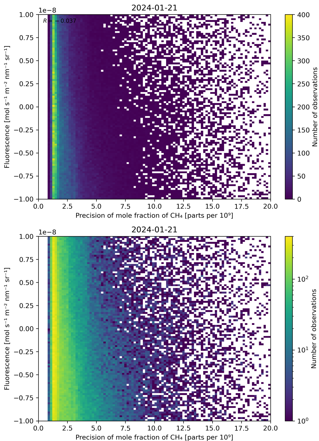
Figure 81: Scatter density plot of “Precision of mole fraction of \text{CH}_4 ” against “Fluorescence” for 2024-01-21 to 2024-01-22.
