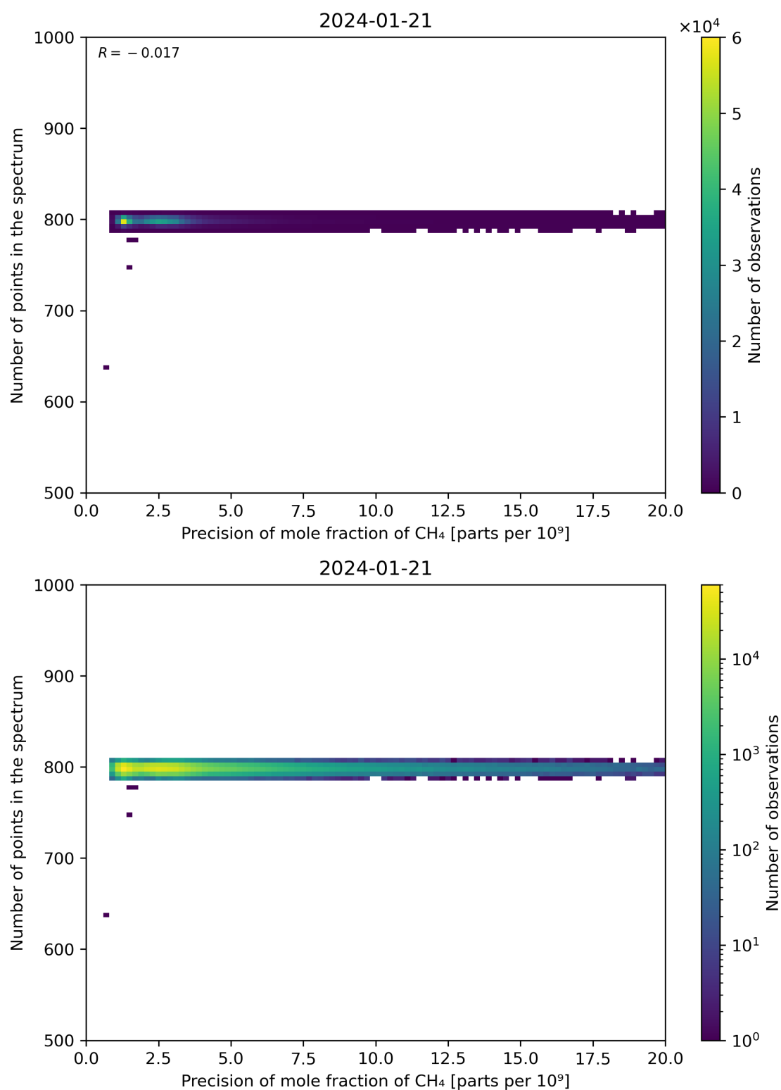
Figure 84: Scatter density plot of “Precision of mole fraction of CH 4 ” against “Number of points in the spectrum” for 2024-01-21 to 2024-01-22.
