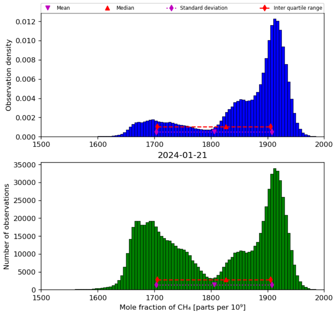
Figure 23: Histogram of “Mole fraction of CH 4 ” for 2024-01-21 to 2024-01-22
