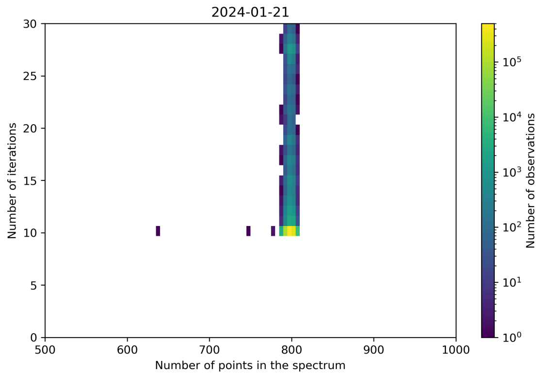
Figure 92: Scatter density plot of “Number of points in the spectrum” against “Number of iterations” for 2024-01-21 to 2024-01-22.
