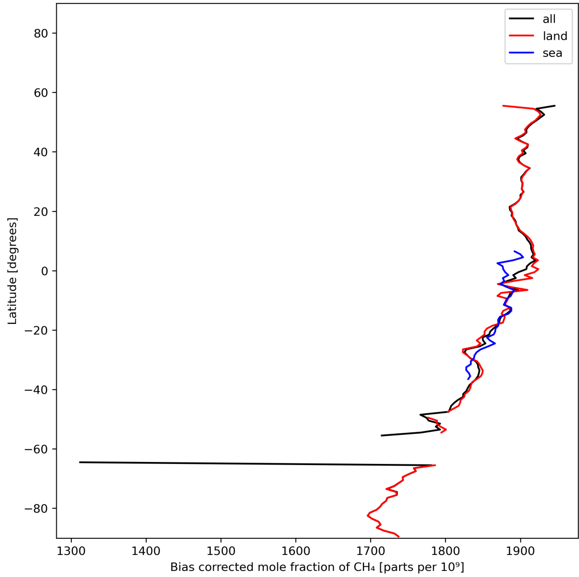
Figure 14: Zonal average of “Bias corrected mole fraction of CH 4 ” for 2024-01-21 to 2024-01-22.
