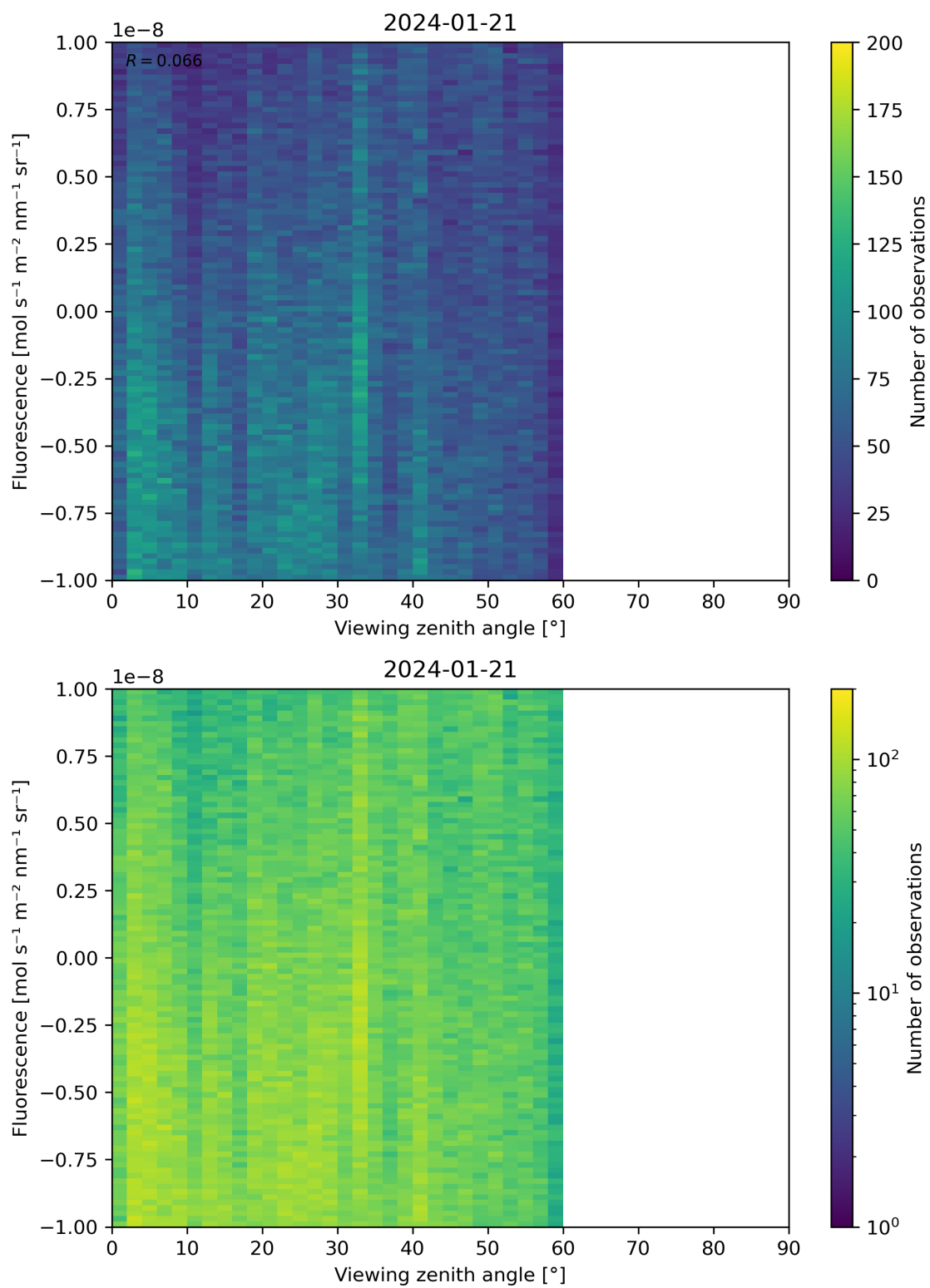
Figure 108: Scatter density plot of “Viewing zenith angle” against “Fluorescence” for 2024-01-21 to 2024-01-22.
