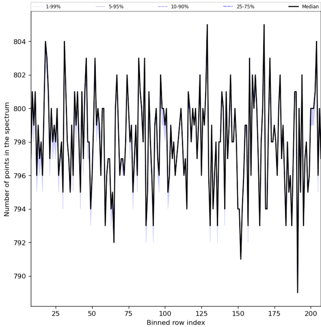
Figure 37: Along track statistics of “Number of points in the spectrum” for 2024-01-21 to 2024-01-22
