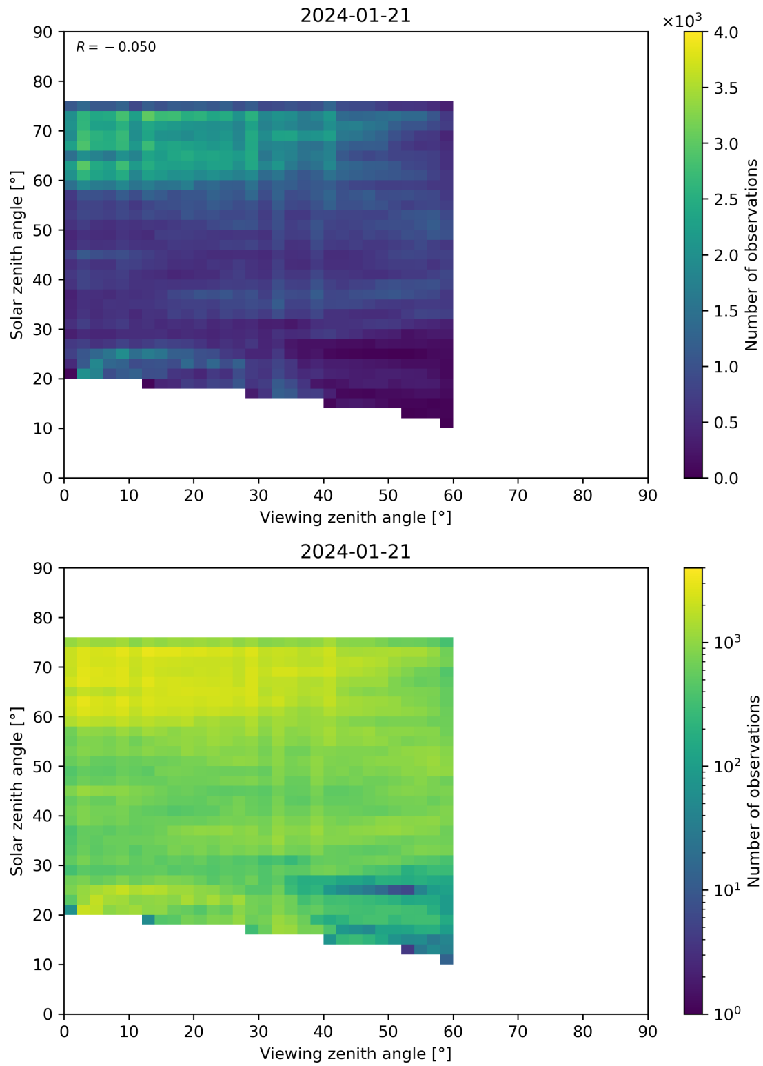
Figure 115: Scatter density plot of “Viewing zenith angle” against “Solar zenith angle” for 2024-01-21 to 2024-01-22.
