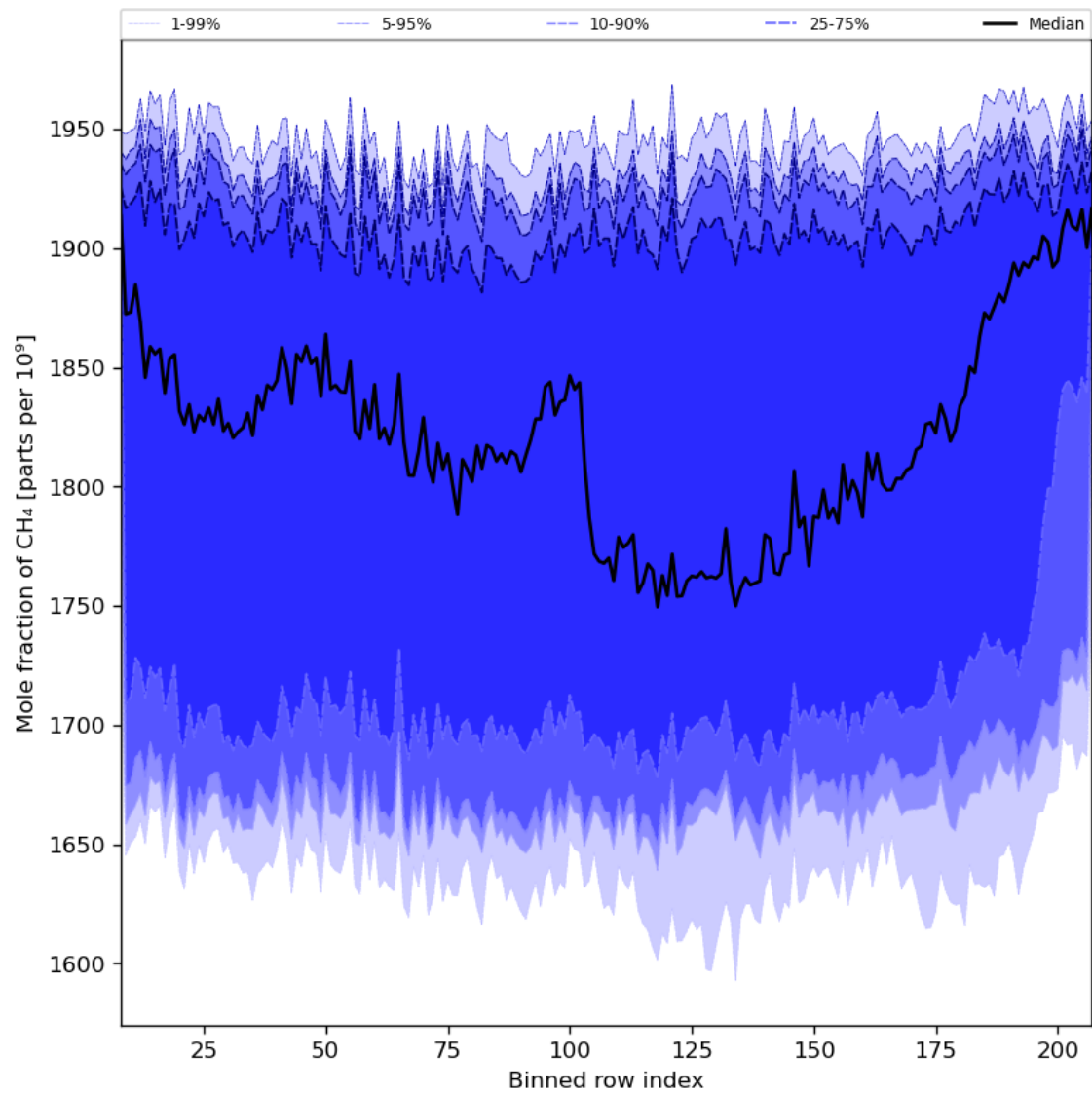
Figure 34: Along track statistics of “Mole fraction of CH 4 ” for 2024-01-21 to 2024-01-22
