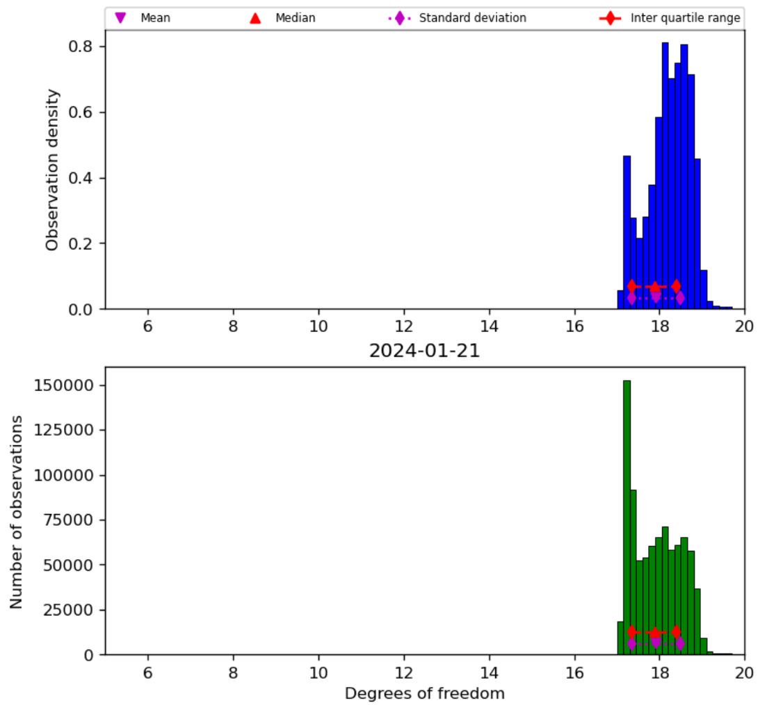
Figure 30: Histogram of “Degrees of freedom” for 2024-01-21 to 2024-01-22
