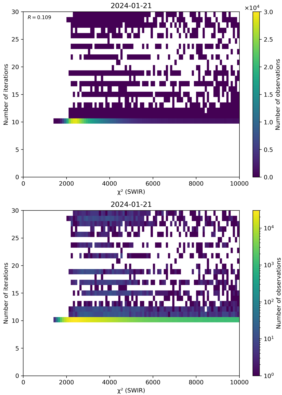
Figure 50: Scatter density plot of “ \chi^2 (SWIR)” against “Number of iterations” for 2024-01-21 to 2024-01-22.
