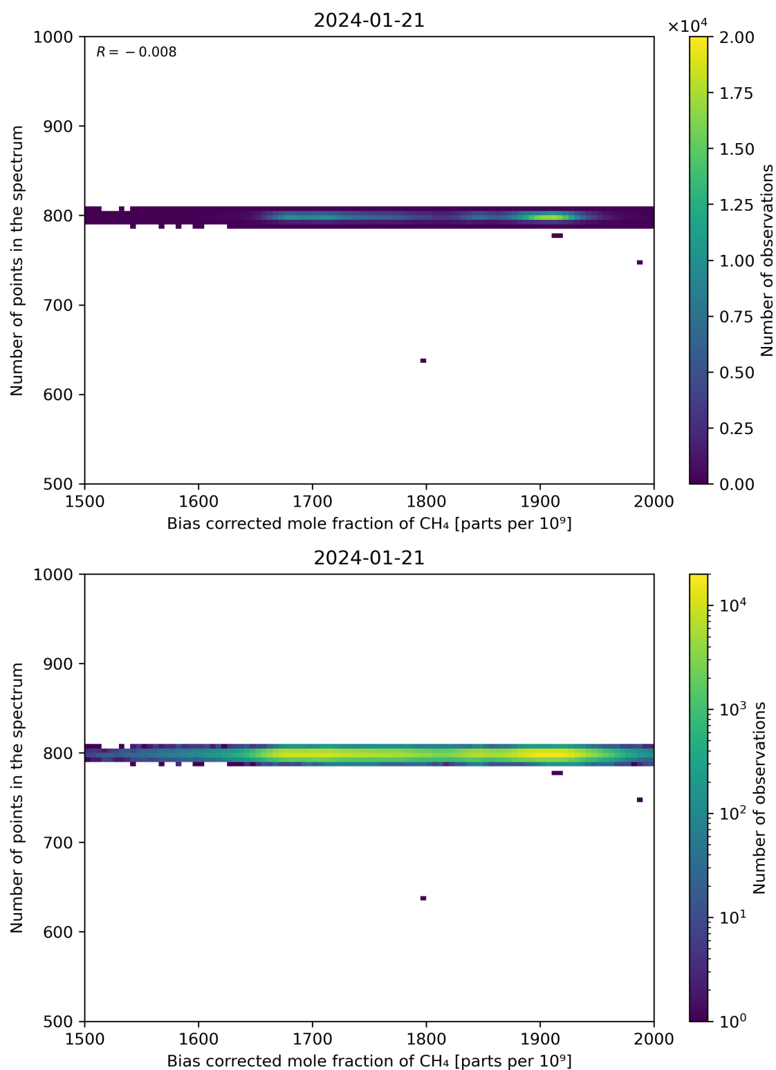
Figure 68: Scatter density plot of “Bias corrected mole fraction of CH 4 ” against “Number of points in the spectrum” for 2024-01-21 to 2024-01-22.
