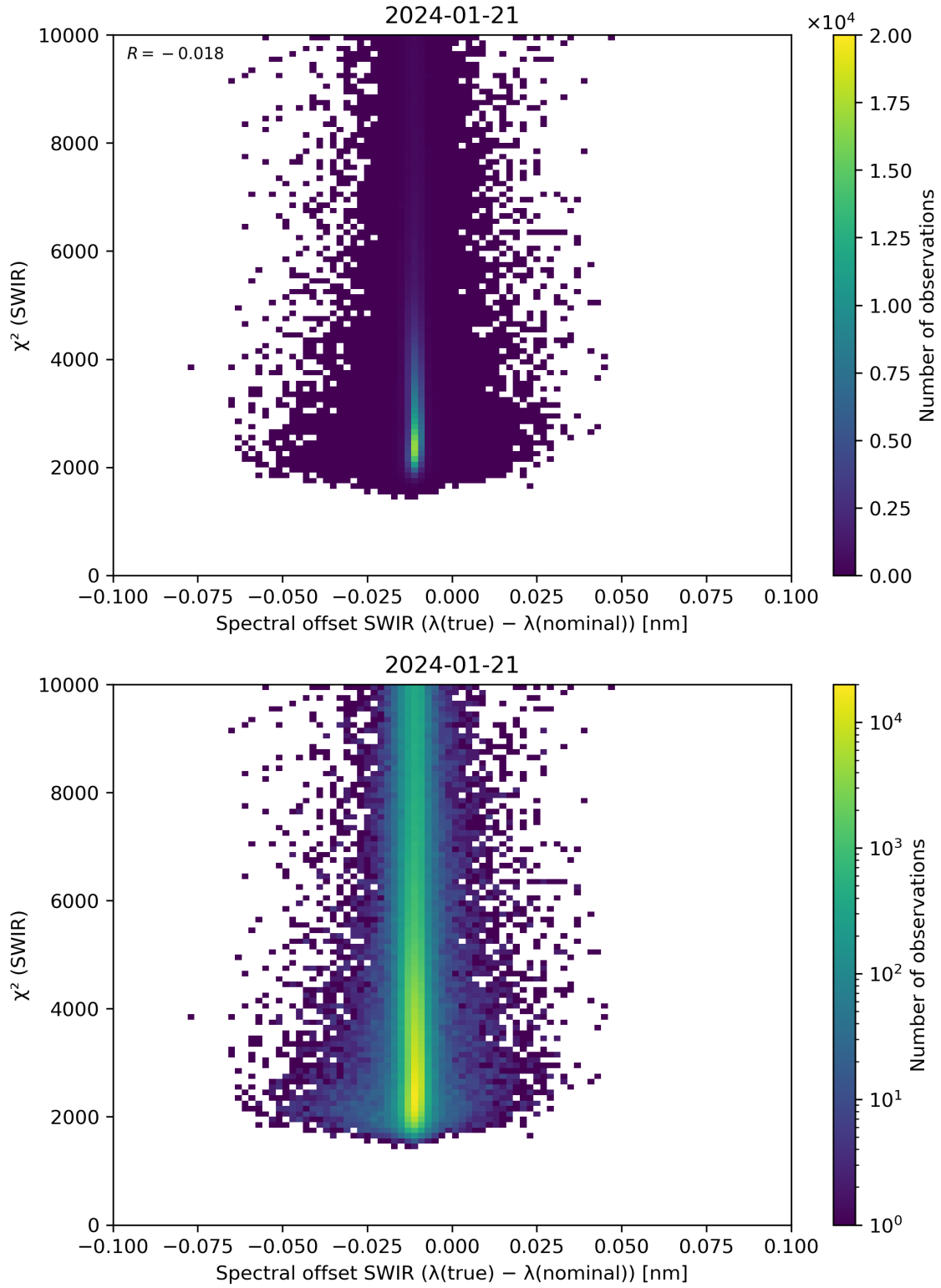
Figure 118: Scatter density plot of “Spectral offset SWIR ( \lambda(\text{true}) - \lambda(\text{nominal}) )” against “ \chi^2 (SWIR)” for 2024-01-21 to 2024-01-22.
