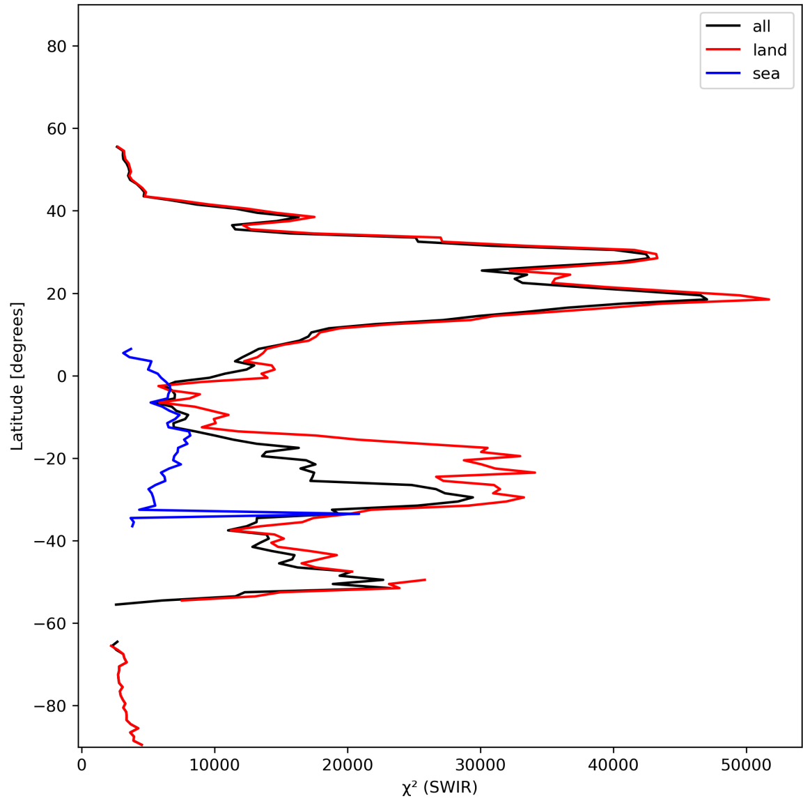
Figure 17: Zonal average of “ \chi^2 (SWIR)” for 2024-01-21 to 2024-01-22.
