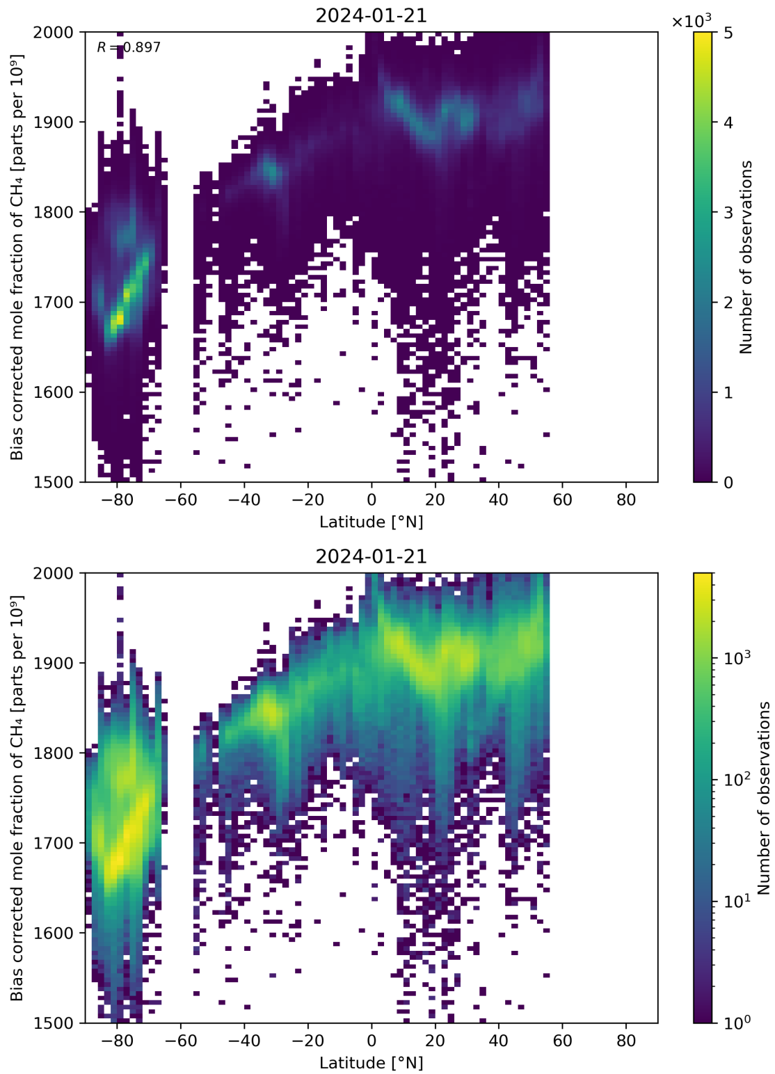
Figure 58: Scatter density plot of “Latitude” against “Bias corrected mole fraction of CH 4 ” for 2024-01-21 to 2024-01-22.
