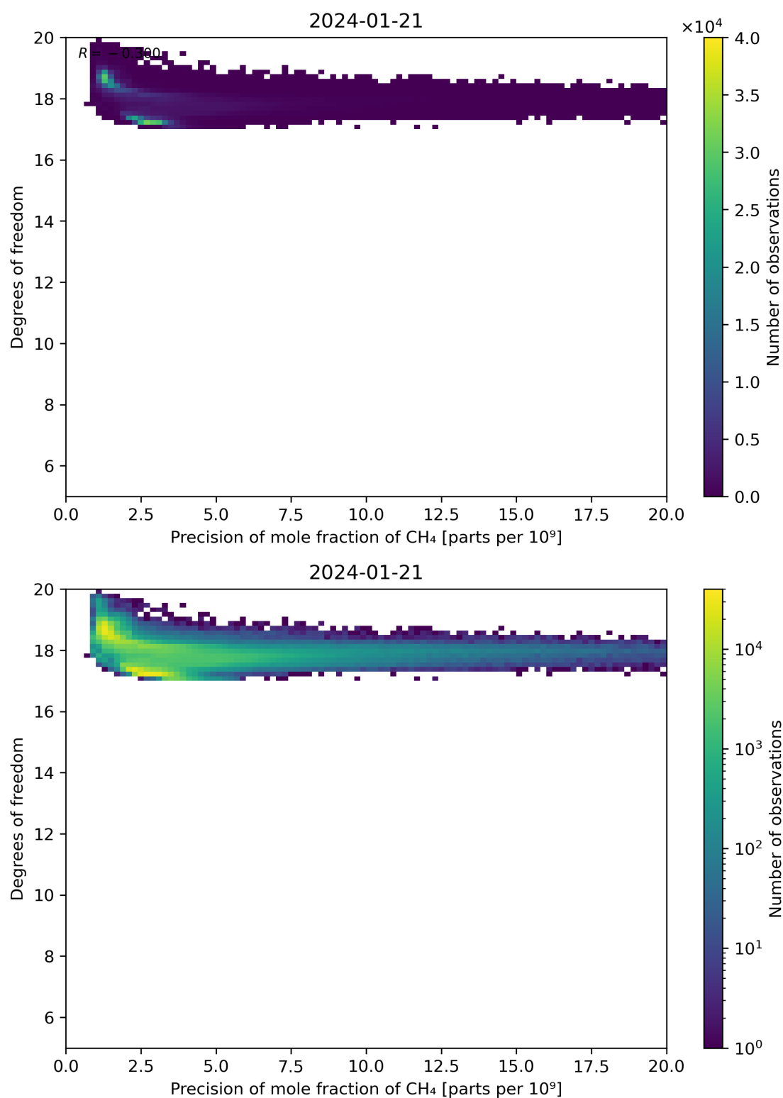
Figure 80: Scatter density plot of “Precision of mole fraction of \text{CH}_4 ” against “Degrees of freedom” for 2024-01-21 to 2024-01-22.
