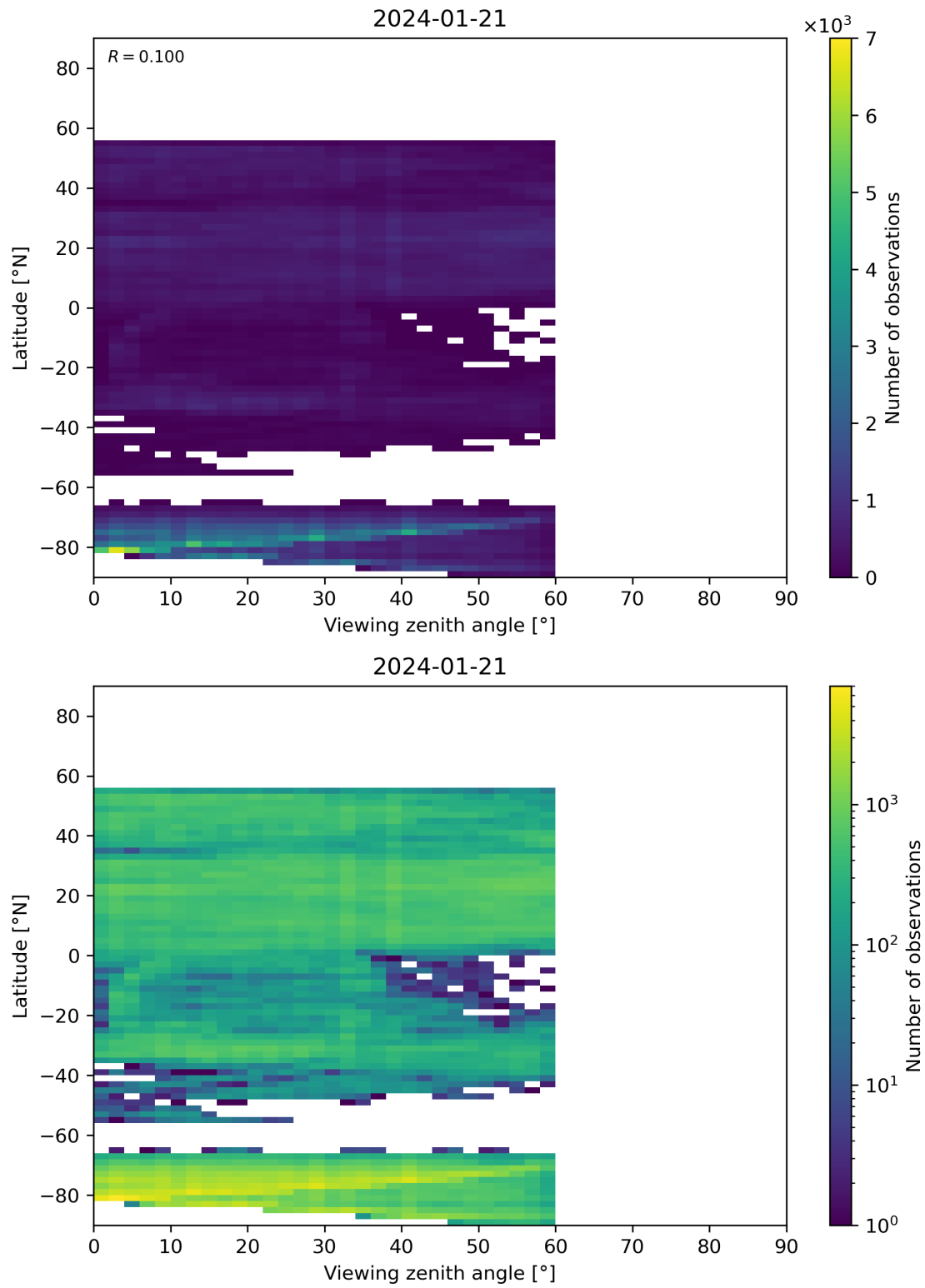
Figure 109: Scatter density plot of “Viewing zenith angle” against “Latitude” for 2024-01-21 to 2024-01-22.
