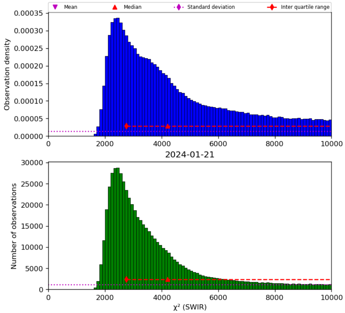
Figure 28: Histogram of “ \chi^2 (SWIR)” for 2024-01-21 to 2024-01-22
