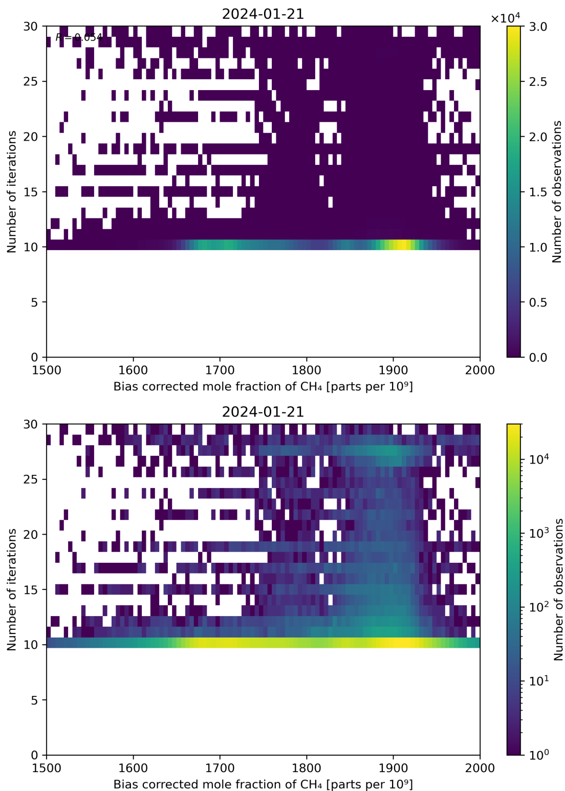
Figure 67: Scatter density plot of “Bias corrected mole fraction of CH 4 ” against “Number of iterations” for 2024-01-21 to 2024-01-22.
