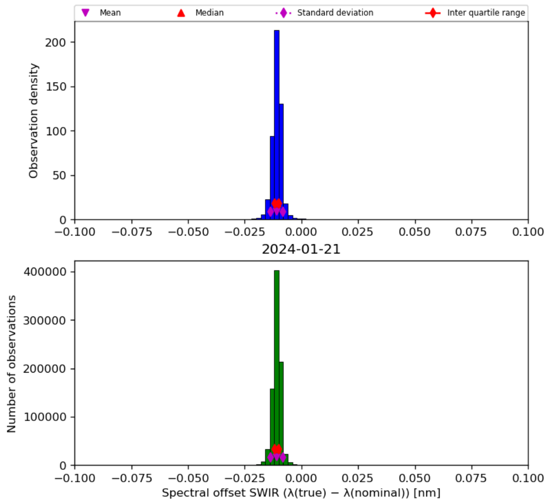
Figure 27: Histogram of “Spectral offset SWIR ( \lambda(\text{true}) - \lambda(\text{nominal}) )” for 2024-01-21 to 2024-01-22
