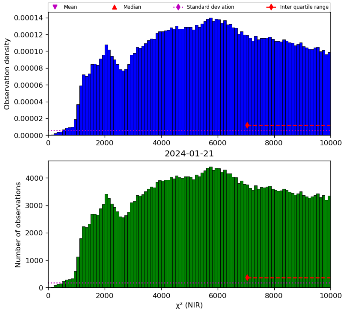
Figure 29: Histogram of “ \chi^2 (NIR)” for 2024-01-21 to 2024-01-22
