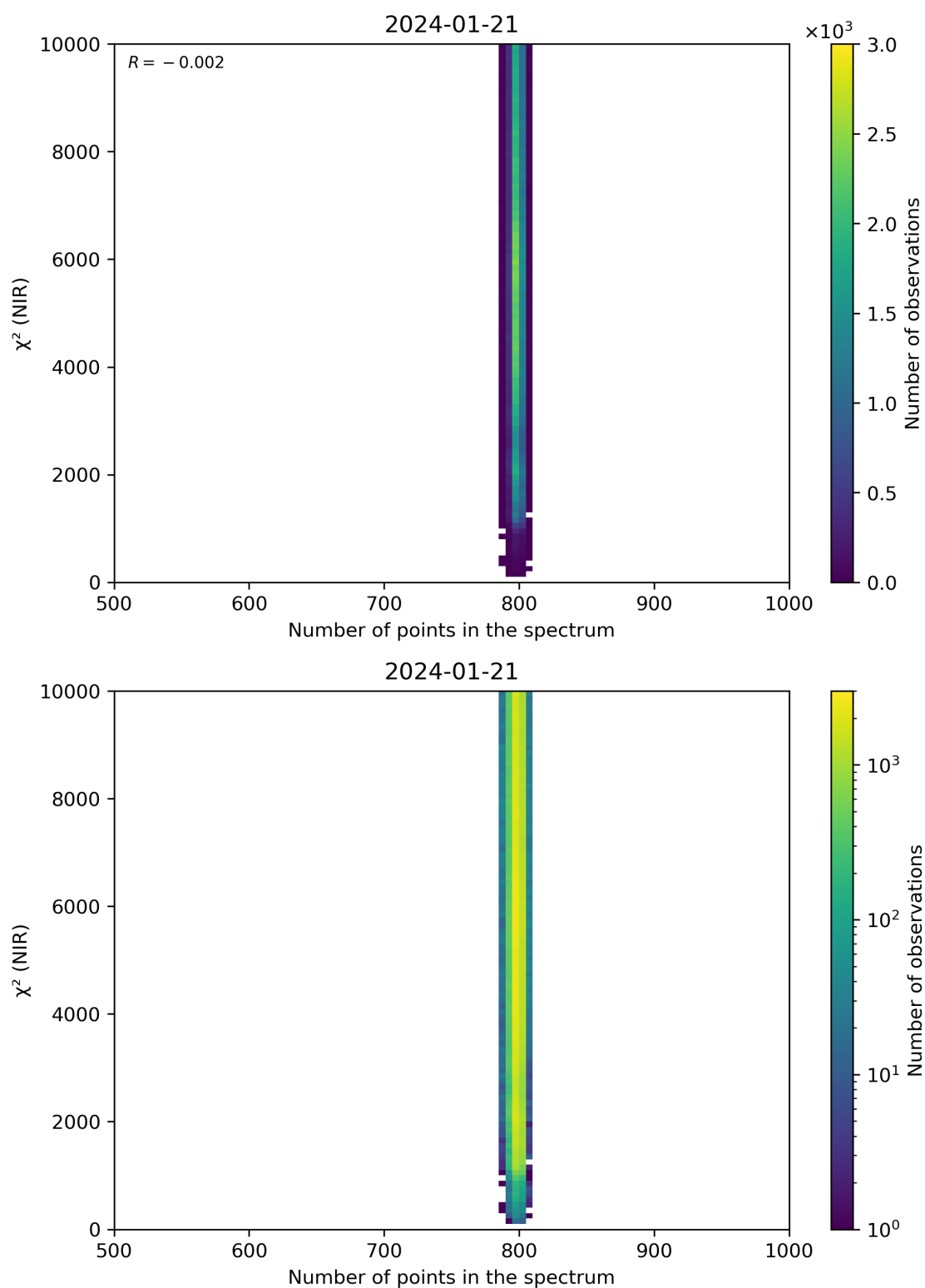
Figure 88: Scatter density plot of “Number of points in the spectrum” against “ \chi^2 (NIR)” for 2024-01-21 to 2024-01-22.
