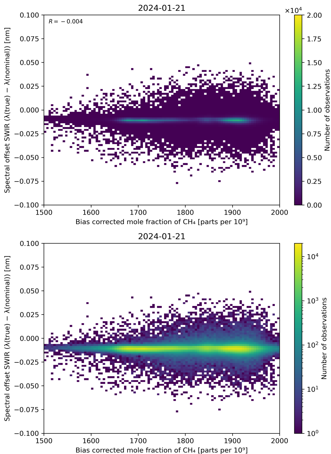
Figure 69: Scatter density plot of “Bias corrected mole fraction of \text{CH}_4 ” against “Spectral offset SWIR ( \lambda(\text{true}) - \lambda(\text{nominal}) )” for 2024-01-21 to 2024-01-22.
