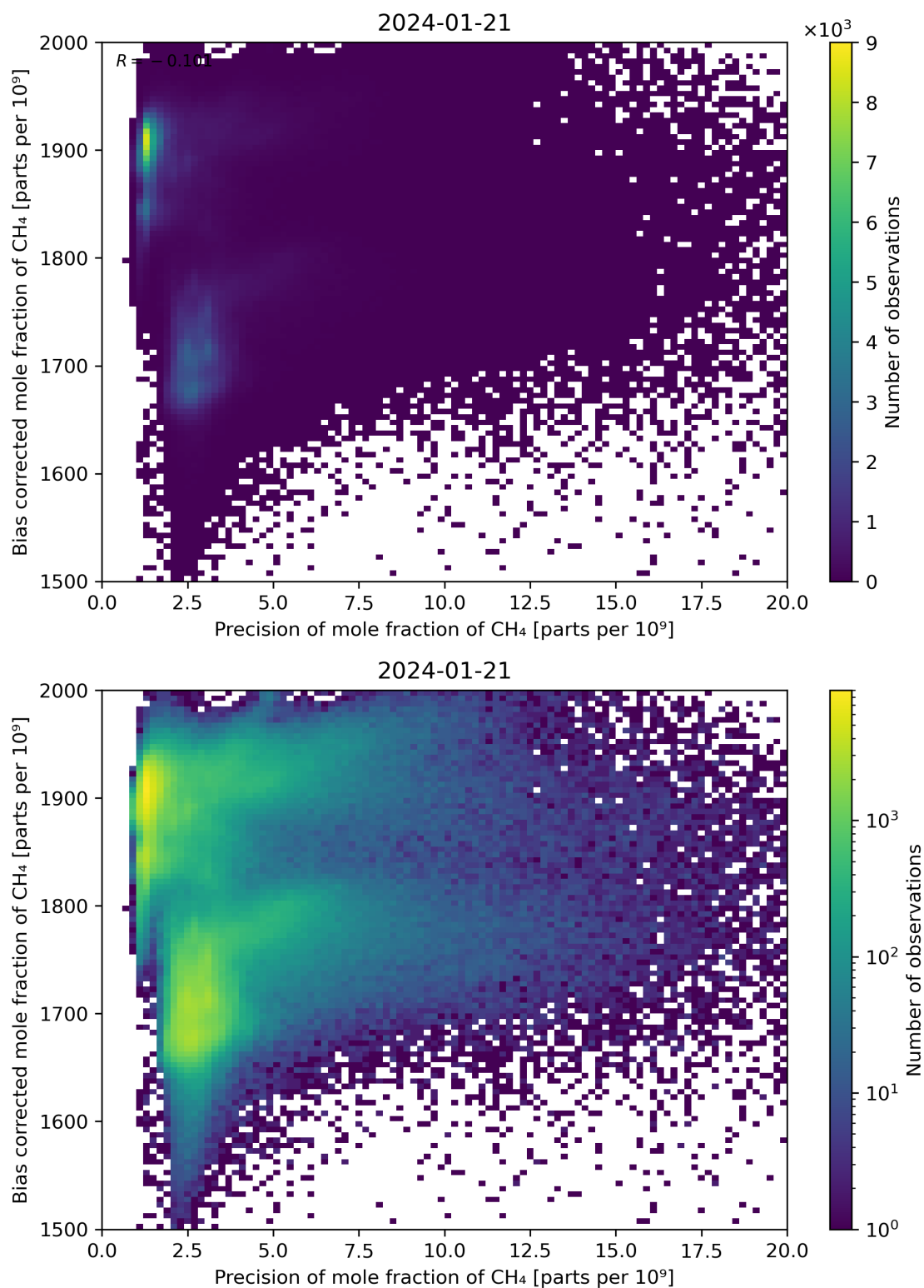
Figure 82: Scatter density plot of “Precision of mole fraction of CH 4 ” against “Bias corrected mole fraction of CH 4 ” for 2024-01-21 to 2024-01-22.
