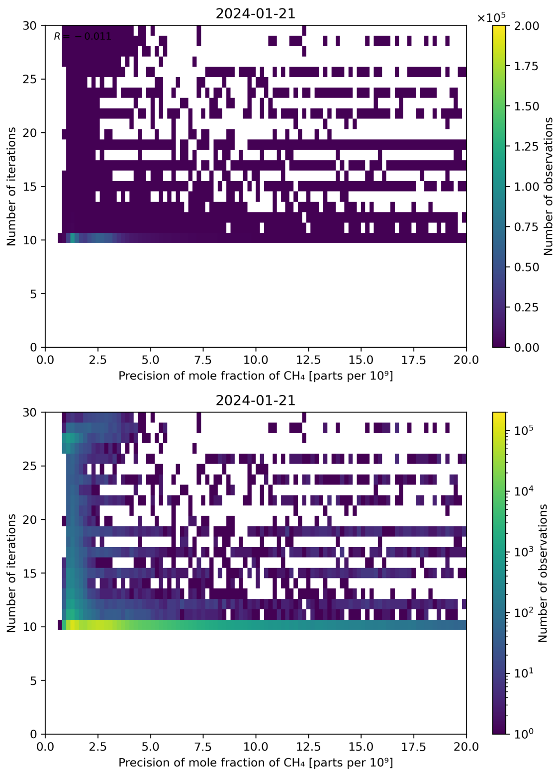
Figure 83: Scatter density plot of “Precision of mole fraction of CH 4 ” against “Number of iterations” for 2024-01-21 to 2024-01-22.
