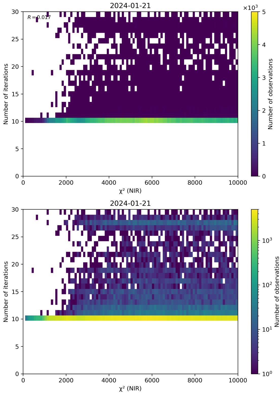
Figure 46: Scatter density plot of “ \chi^2 (NIR)” against “Number of iterations” for 2024-01-21 to 2024-01-22.
