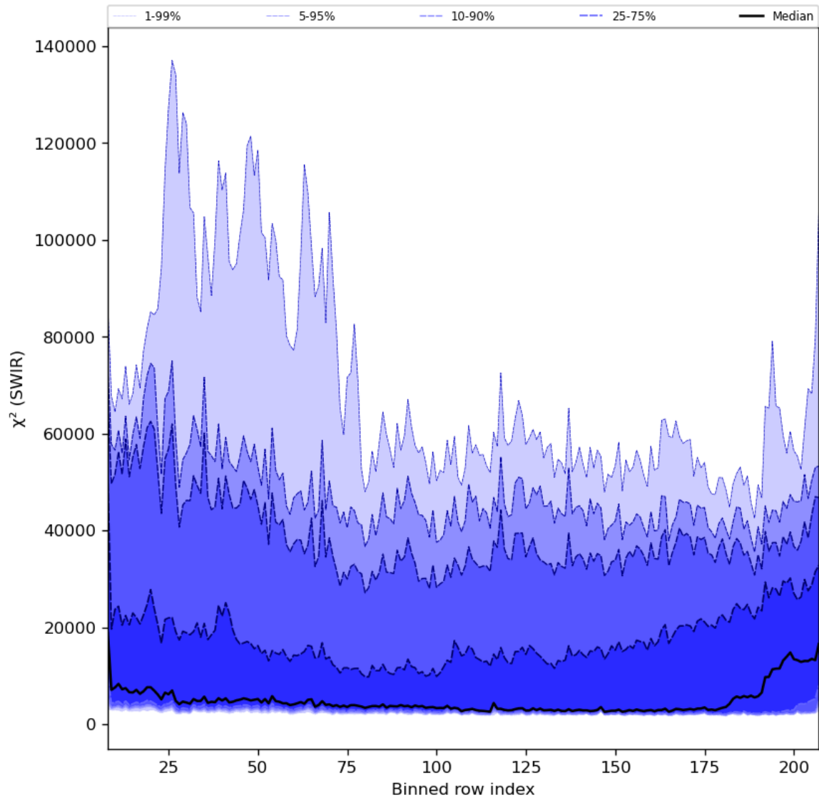
Figure 39: Along track statistics of " \chi^2 (SWIR)" for 2024-01-21 to 2024-01-22
