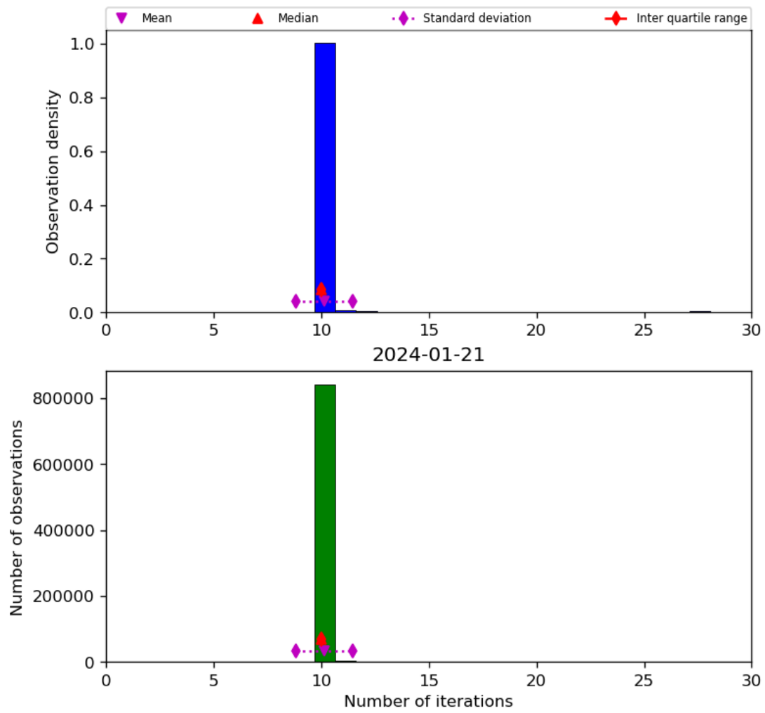
Figure 31: Histogram of “Number of iterations” for 2024-01-21 to 2024-01-22
