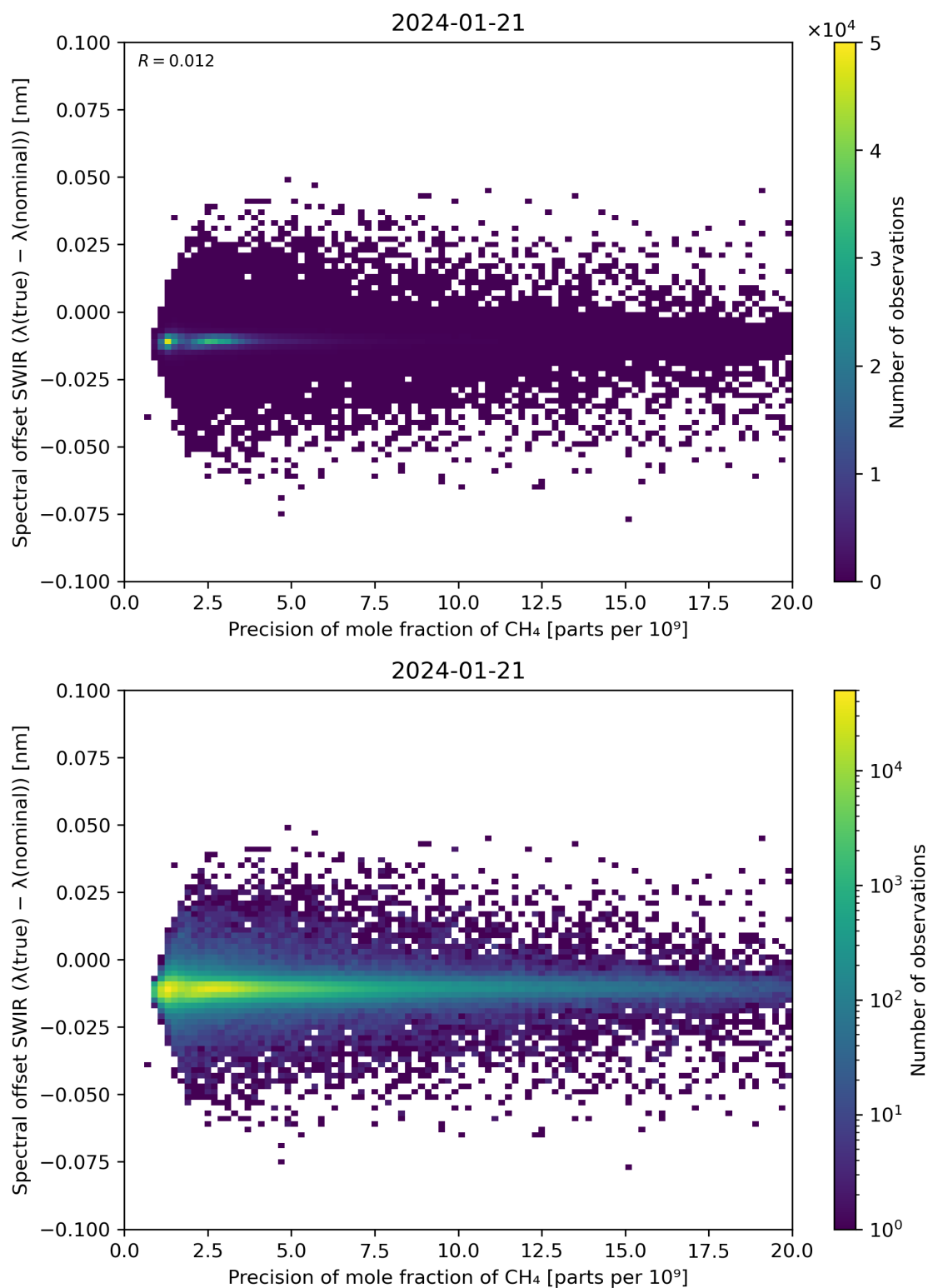
Figure 85: Scatter density plot of “Precision of mole fraction of \text{CH}_4 ” against “Spectral offset SWIR ( \lambda(\text{true}) - \lambda(\text{nominal}) )” for 2024-01-21 to 2024-01-22.
