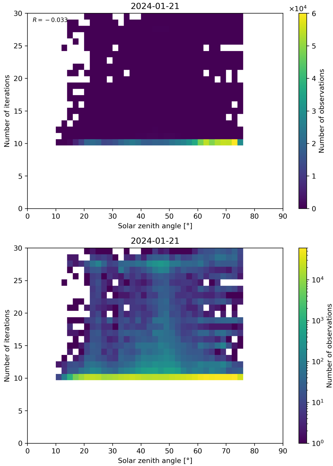
Figure 102: Scatter density plot of “Solar zenith angle” against “Number of iterations” for 2024-01-21 to 2024-01-22.
