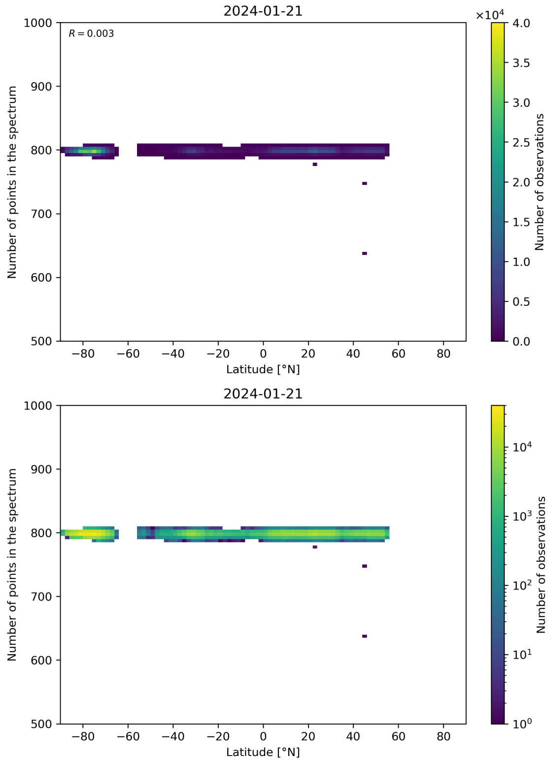
Figure 61: Scatter density plot of “Latitude” against “Number of points in the spectrum” for 2024-01-21 to 2024-01-22.
