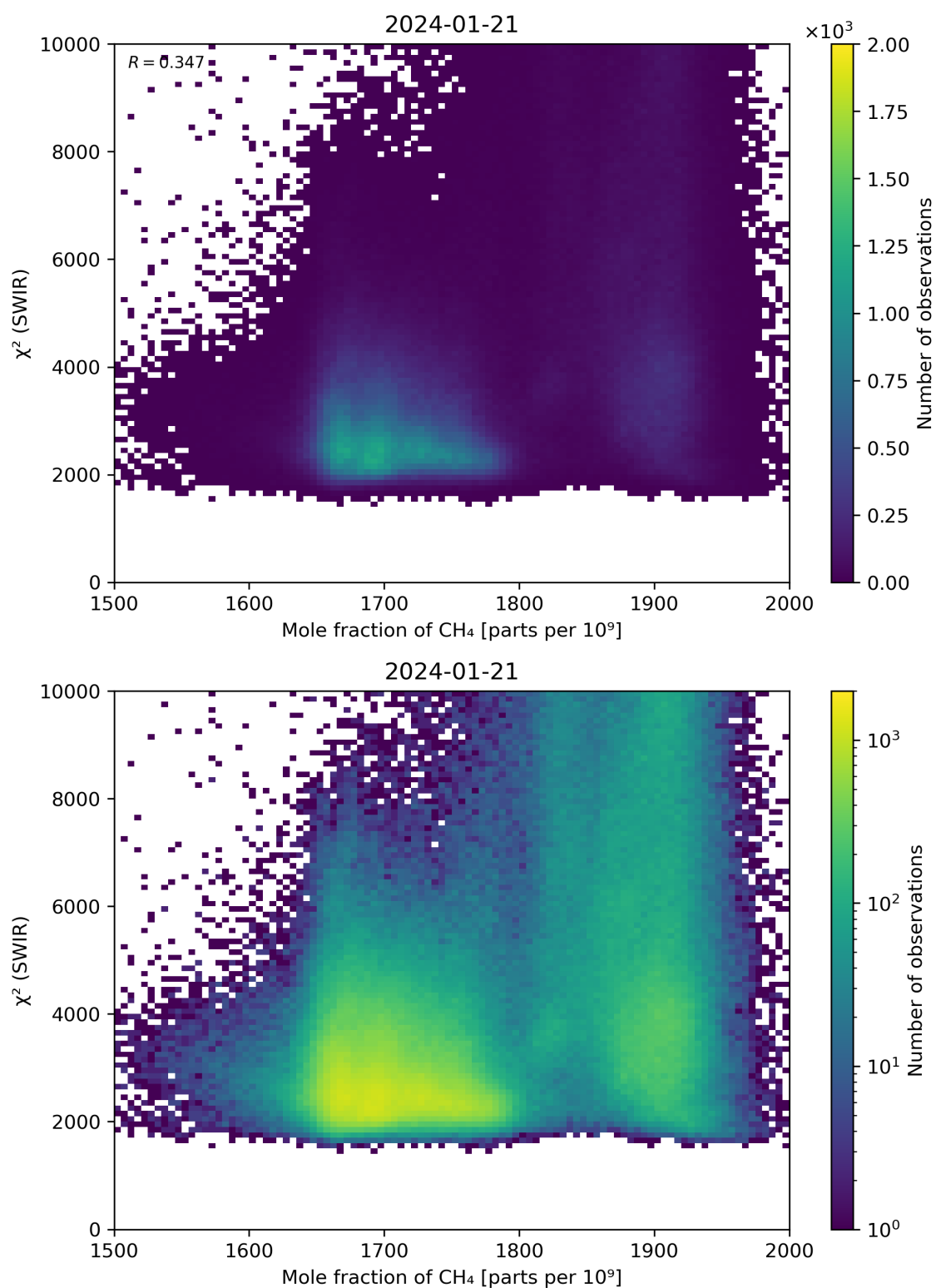
Figure 71: Scatter density plot of “Mole fraction of \text{CH}_4 ” against “ \chi^2 (SWIR)” for 2024-01-21 to 2024-01-22.
