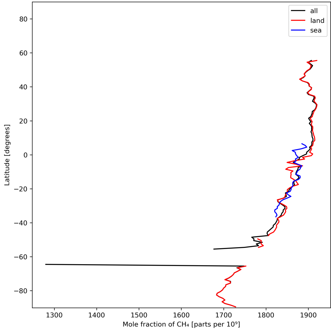
Figure 12: Zonal average of “Mole fraction of \text{CH}_4 ” for 2024-01-21 to 2024-01-22.
