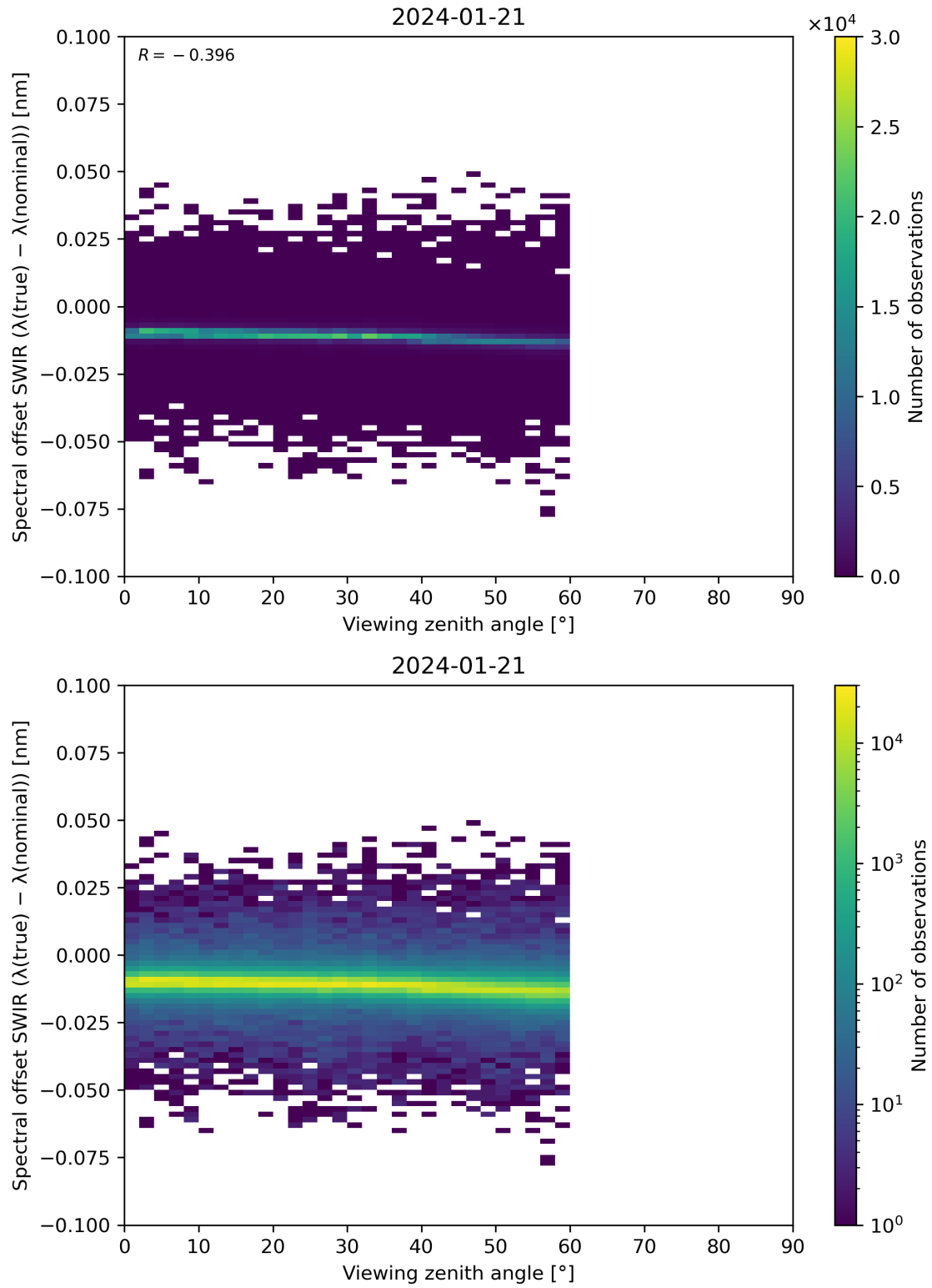
Figure 116: Scatter density plot of “Viewing zenith angle” against “Spectral offset SWIR ( \lambda(\text{true}) - \lambda(\text{nominal}) )” for 2024-01-21 to 2024-01-22.
