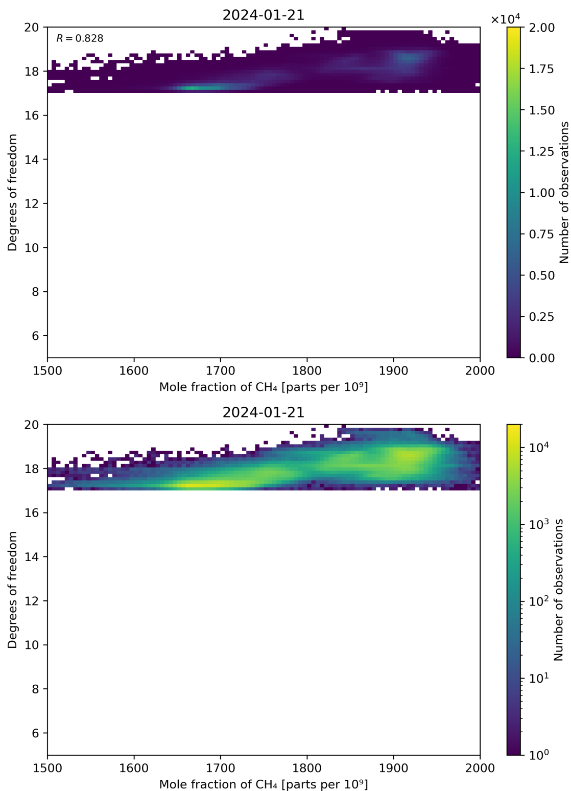
Figure 72: Scatter density plot of “Mole fraction of CH 4 ” against “Degrees of freedom” for 2024-01-21 to 2024-01-22.
