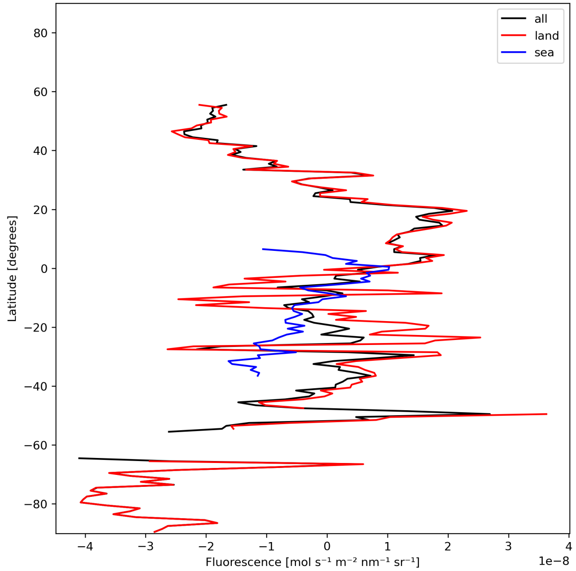
Figure 21: Zonal average of “Fluorescence” for 2024-01-21 to 2024-01-22.
