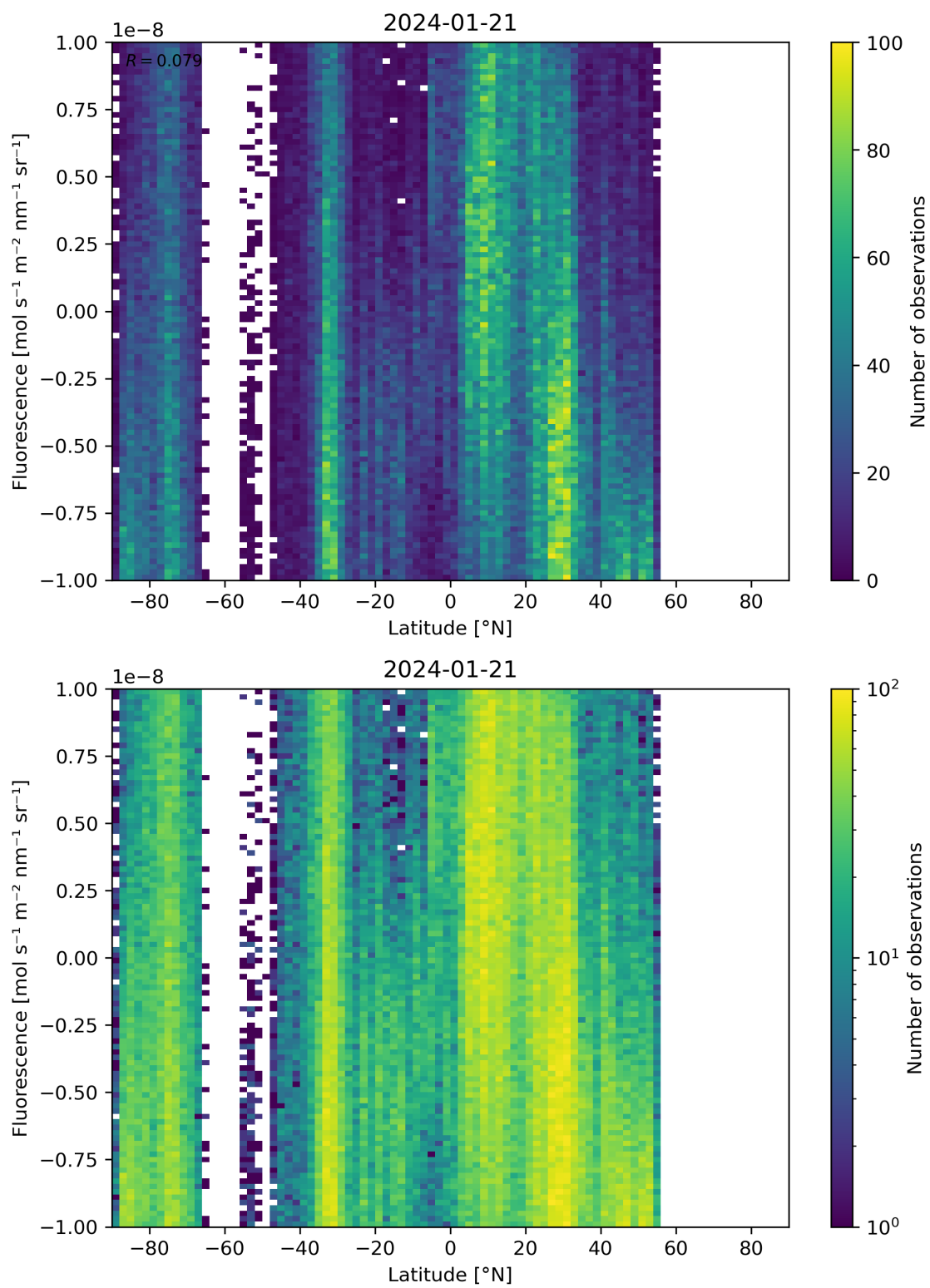
Figure 56: Scatter density plot of “Latitude” against “Fluorescence” for 2024-01-21 to 2024-01-22.
