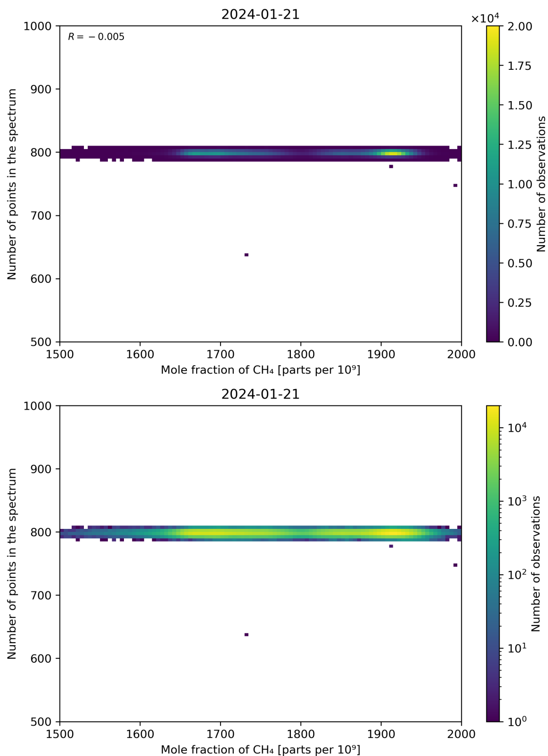
Figure 77: Scatter density plot of “Mole fraction of CH 4 ” against “Number of points in the spectrum” for 2024-01-21 to 2024-01-22.
