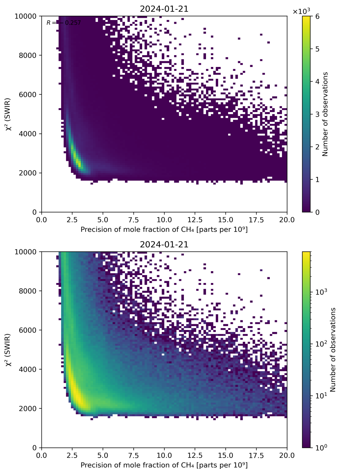
Figure 79: Scatter density plot of “Precision of mole fraction of CH 4 ” against “ \chi^2 (SWIR)” for 2024-01-21 to 2024-01-22.
