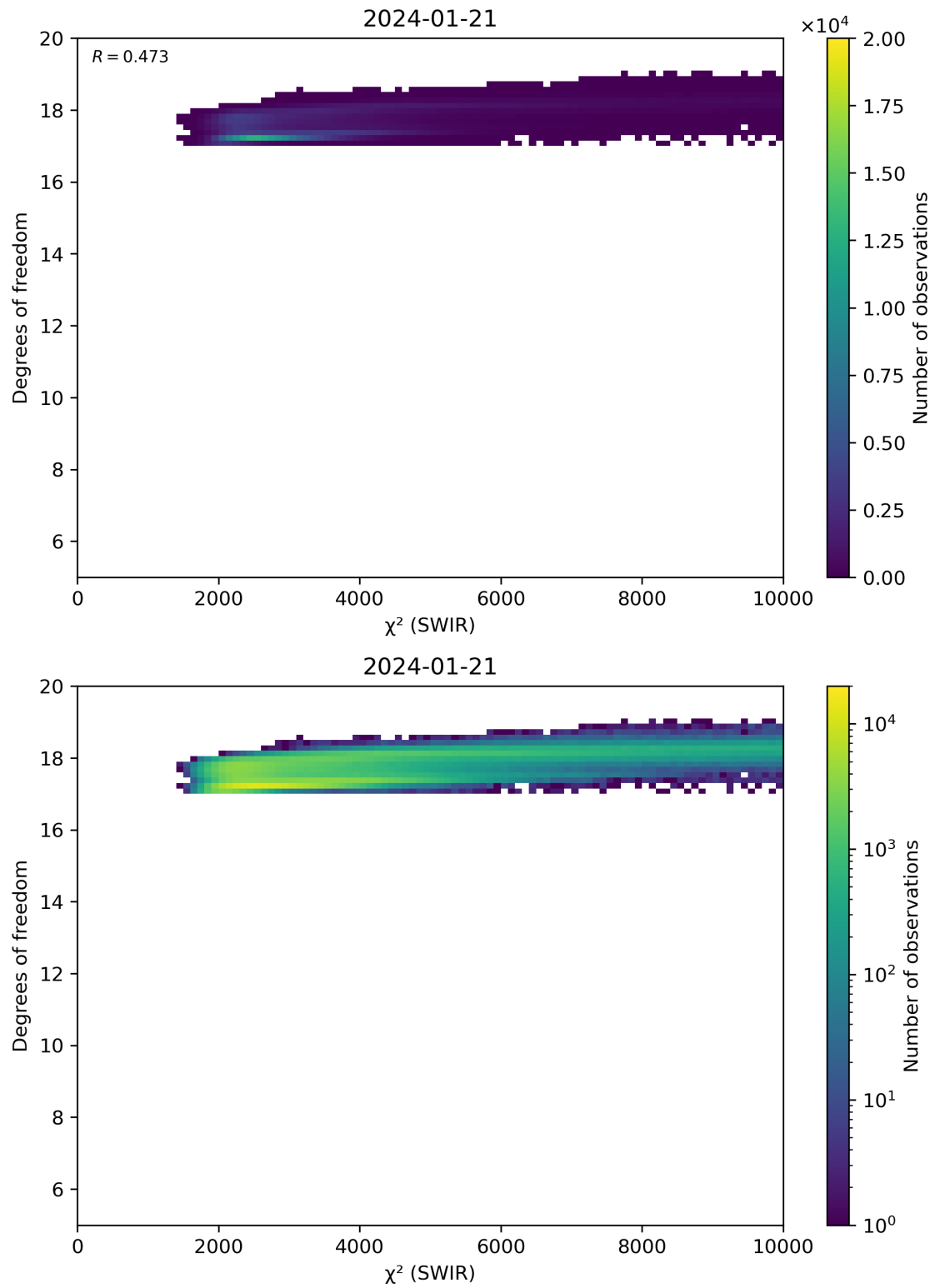
Figure 48: Scatter density plot of “ \chi^2 (SWIR)” against “Degrees of freedom” for 2024-01-21 to 2024-01-22.
