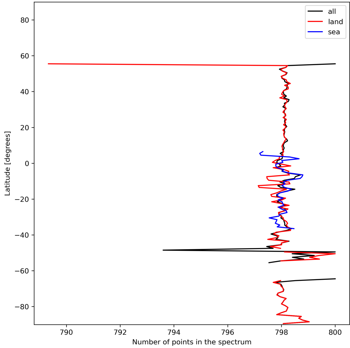
Figure 15: Zonal average of “Number of points in the spectrum” for 2024-01-21 to 2024-01-22.
