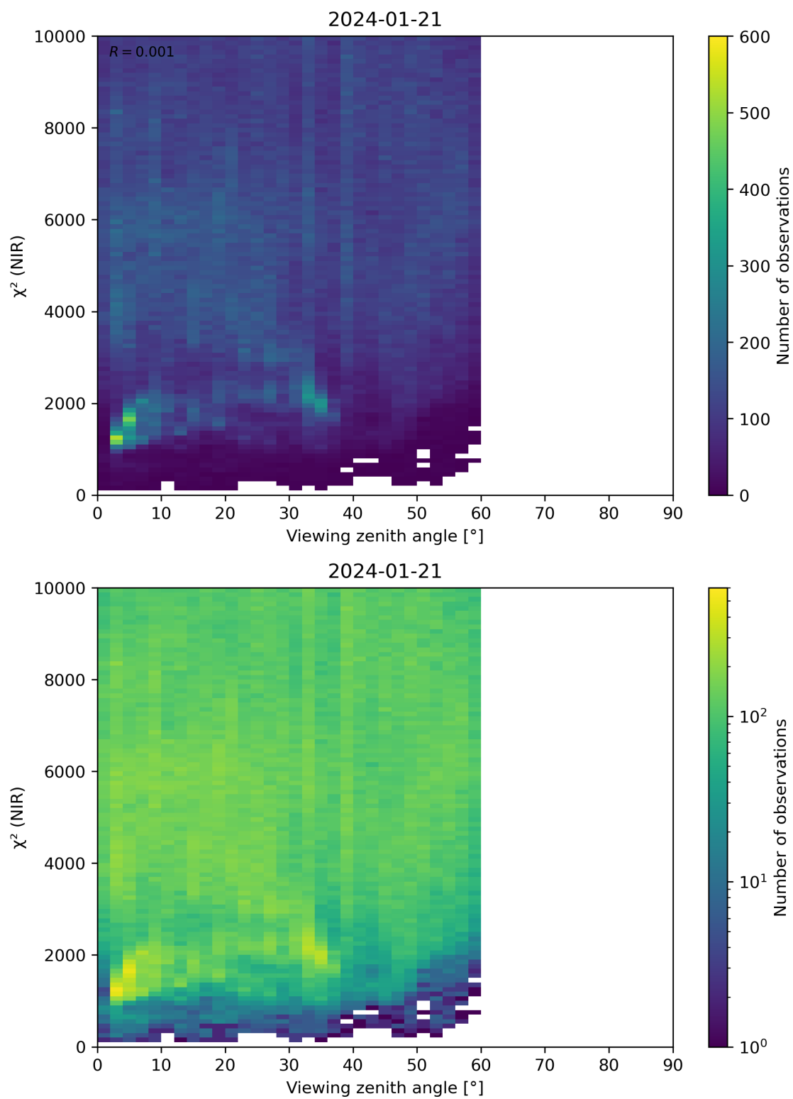
Figure 105: Scatter density plot of “Viewing zenith angle” against “ \chi^2 (NIR)” for 2024-01-21 to 2024-01-22.
