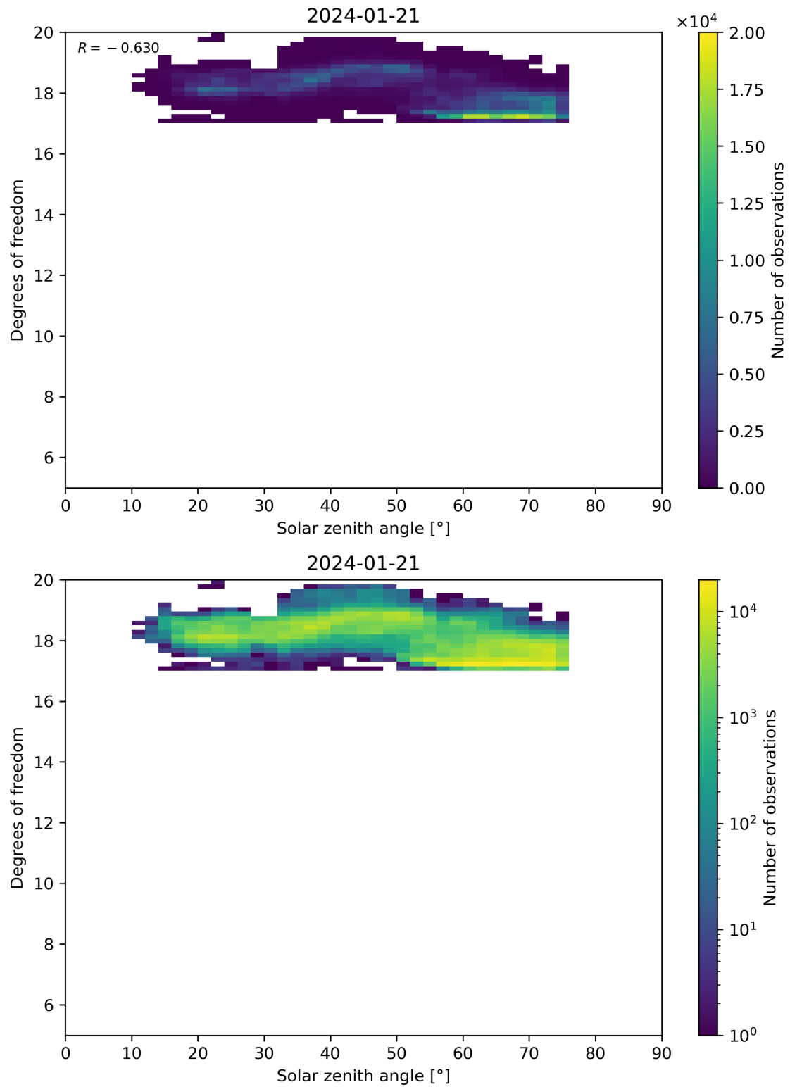
Figure 96: Scatter density plot of “Solar zenith angle” against “Degrees of freedom” for 2024-01-21 to 2024-01-22.
