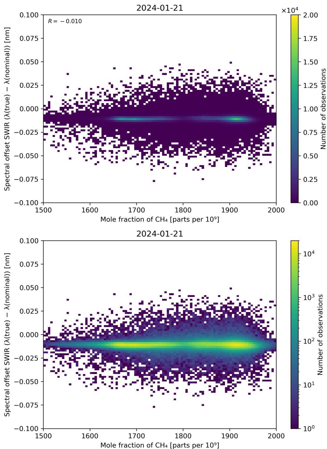
Figure 86: Scatter density plot of “Mole fraction of CH 4 ” against “Spectral offset SWIR ( \lambda(\text{true}) - \lambda(\text{nominal}) )” for 2024-01-21 to 2024-01-22.
