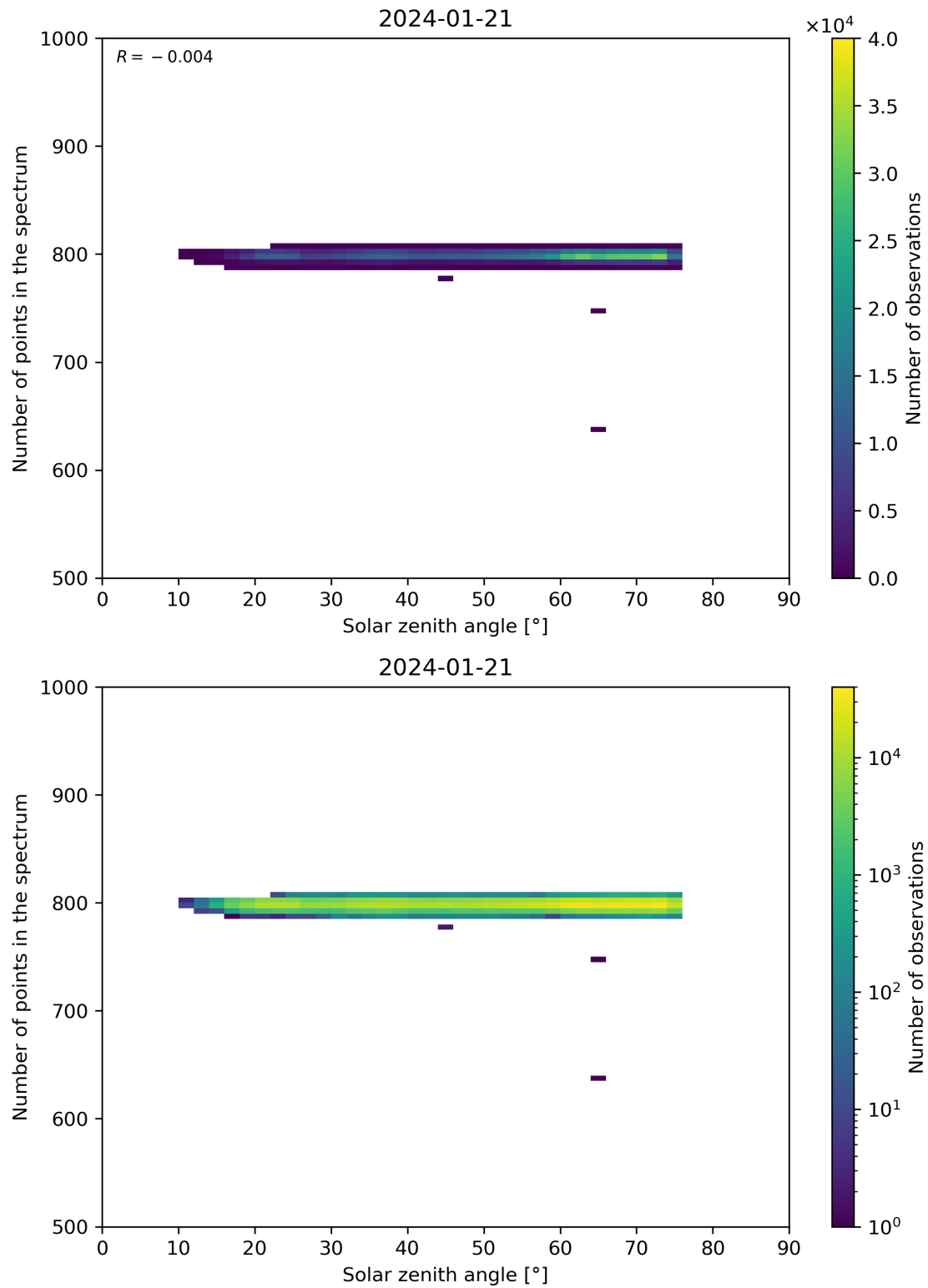
Figure 103: Scatter density plot of “Solar zenith angle” against “Number of points in the spectrum” for 2024-01-21 to 2024-01-22.
