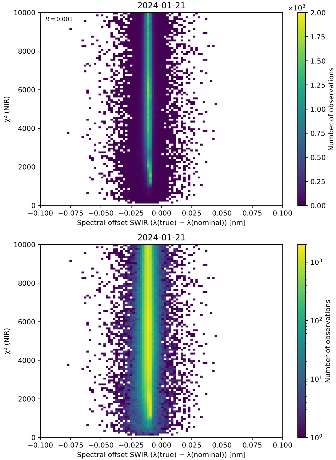
Figure 117: Scatter density plot of “Spectral offset SWIR ( \lambda(\text{true}) - \lambda(\text{nominal}) )” against “ \chi^2 (NIR)” for 2024-01-21 to 2024-01-22.
