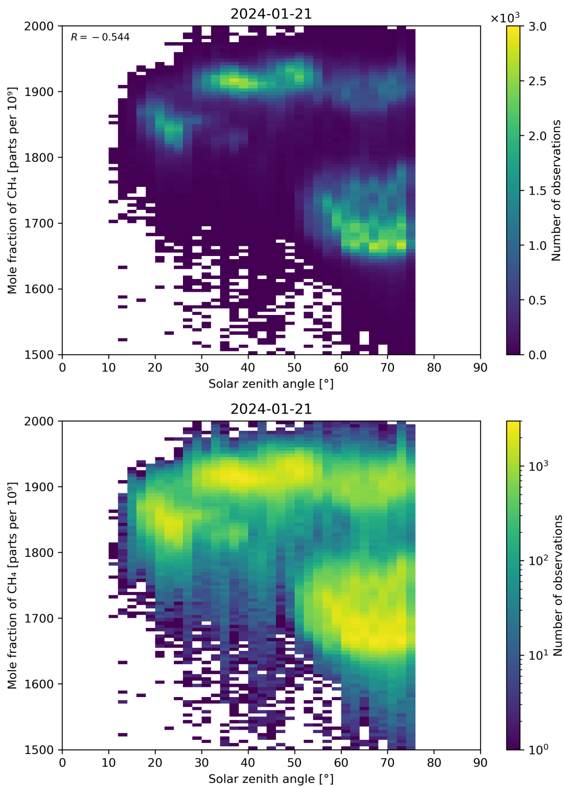
Figure 99: Scatter density plot of “Solar zenith angle” against “Mole fraction of CH 4 ” for 2024-01-21 to 2024-01-22.
