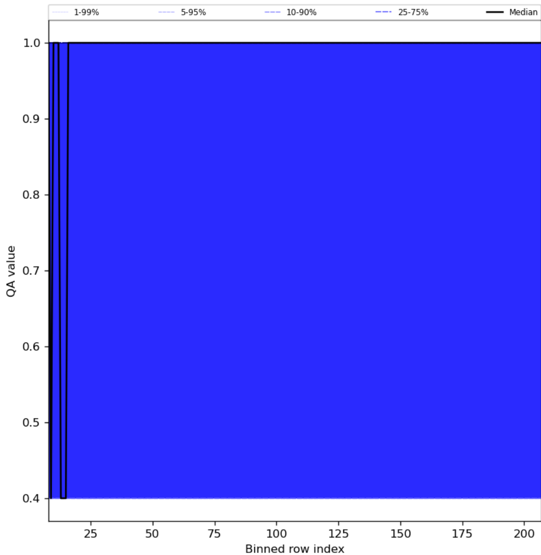
Figure 33: Along track statistics of “QA value” for 2024-01-21 to 2024-01-22
