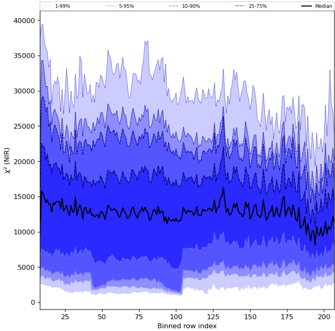
Figure 40: Along track statistics of “ \chi^2 (NIR)” for 2024-01-21 to 2024-01-22
