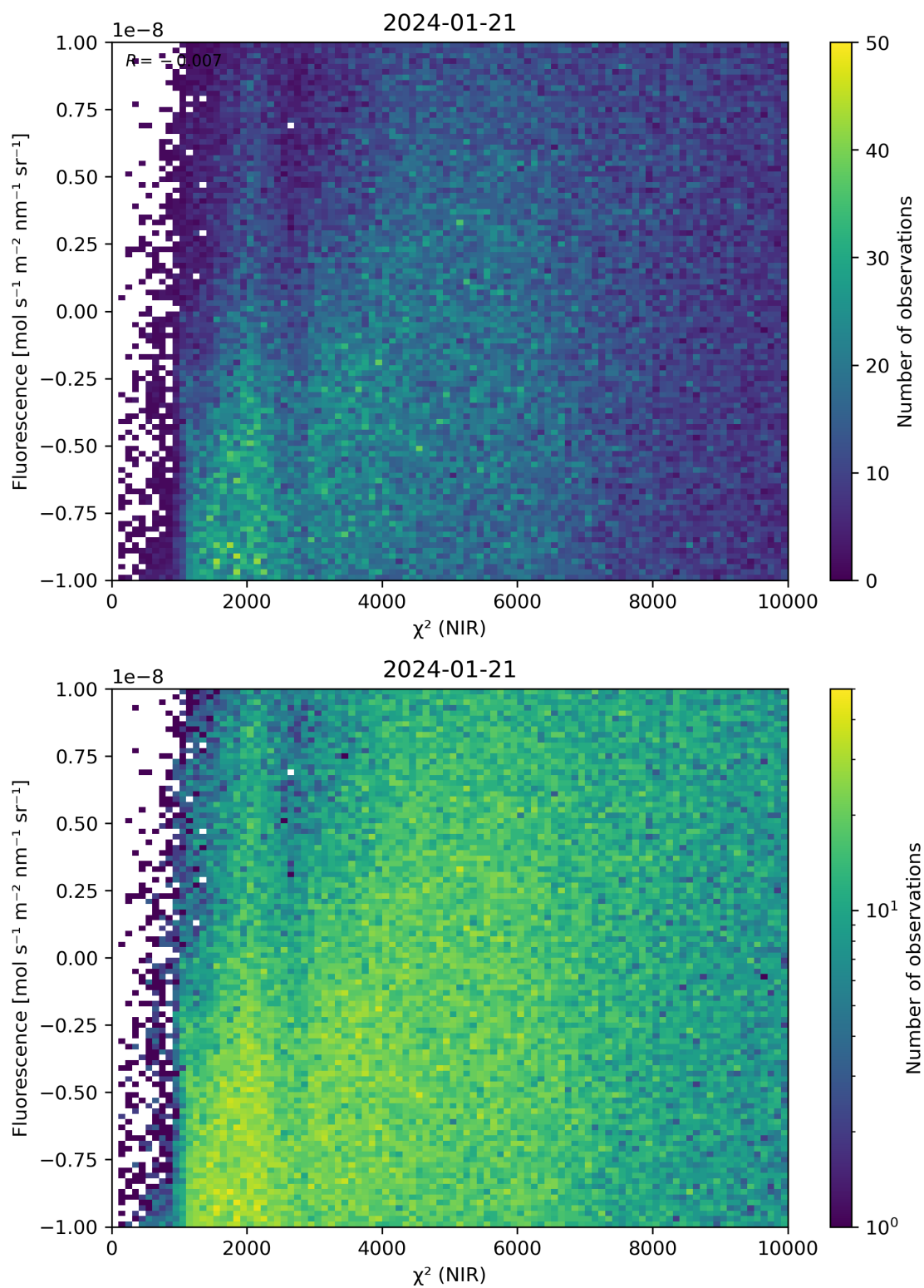
Figure 45: Scatter density plot of “ \chi^2 (NIR)” against “Fluorescence” for 2024-01-21 to 2024-01-22.
