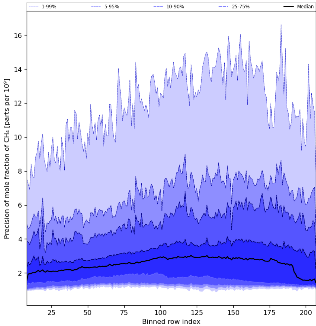
Figure 35: Along track statistics of “Precision of mole fraction of CH 4 ” for 2024-01-21 to 2024-01-22
