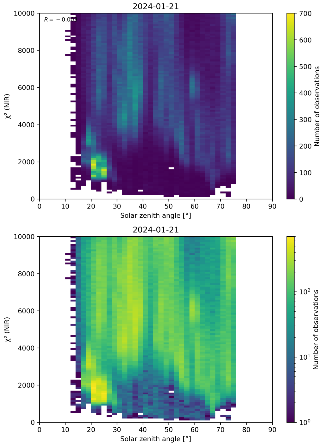
Figure 94: Scatter density plot of “Solar zenith angle” against “ \chi^2 (NIR)” for 2024-01-21 to 2024-01-22.
