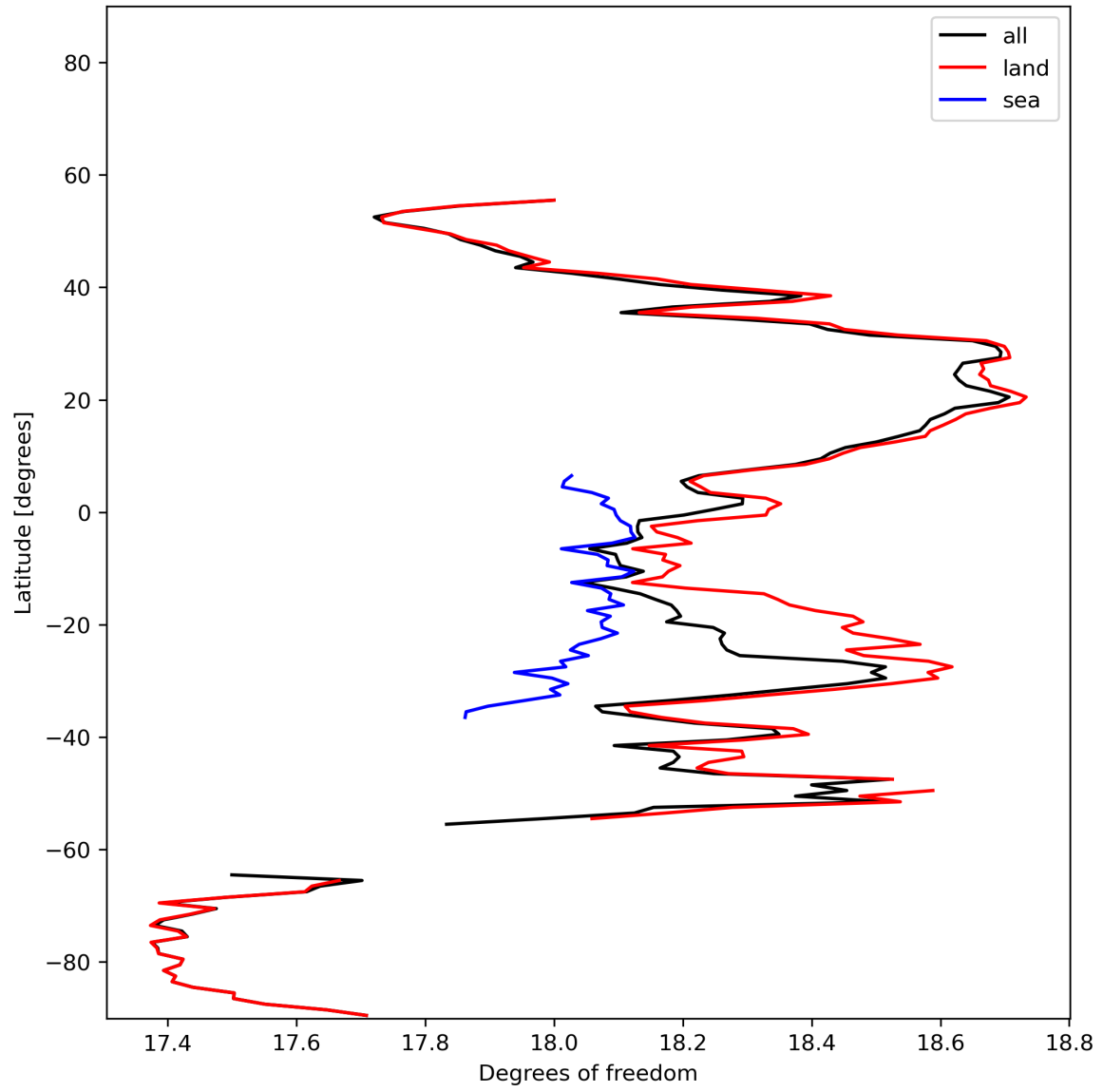
Figure 19: Zonal average of “Degrees of freedom” for 2024-01-21 to 2024-01-22.
