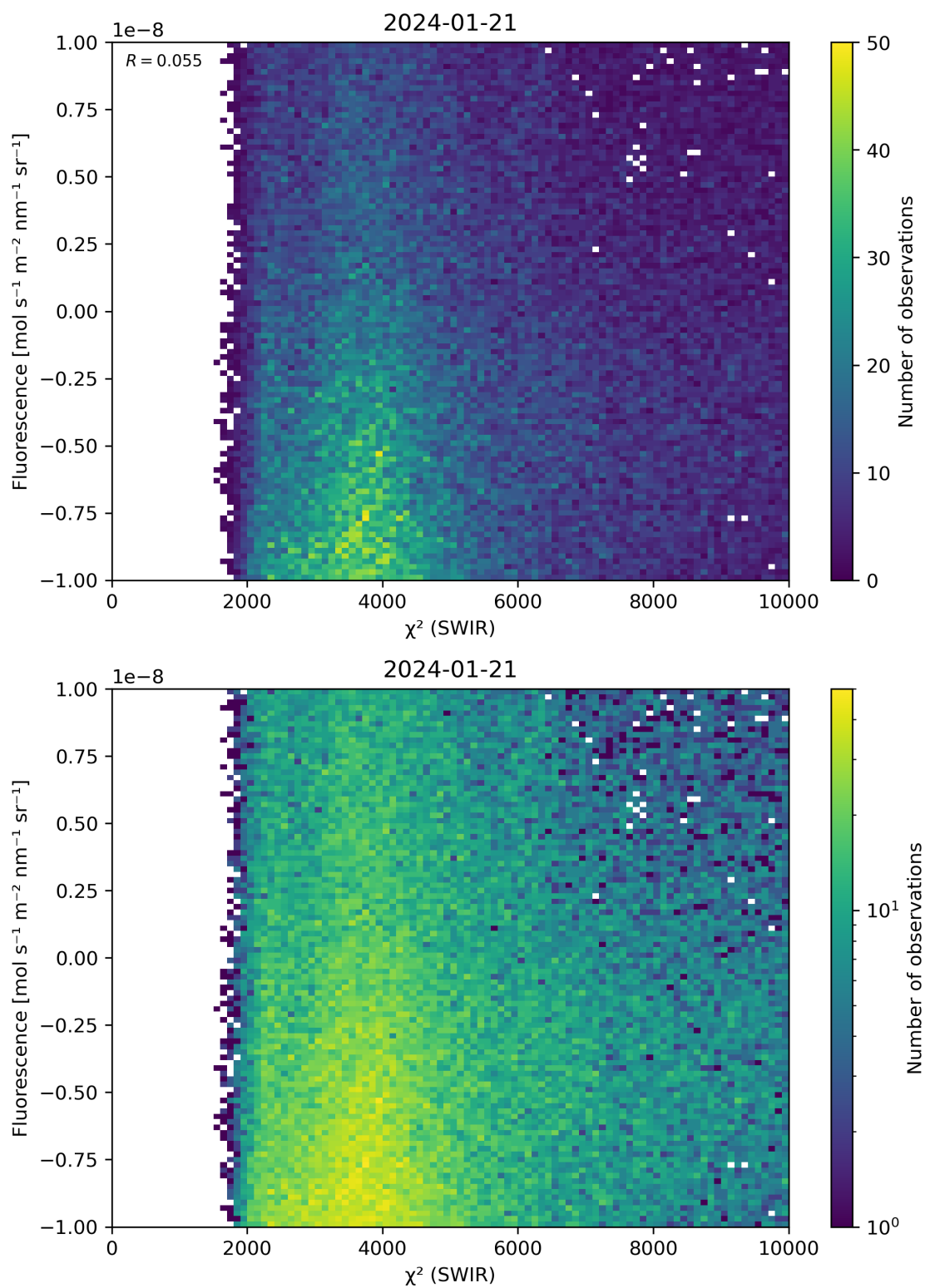
Figure 49: Scatter density plot of “ \chi^2 (SWIR)” against “Fluorescence” for 2024-01-21 to 2024-01-22.
