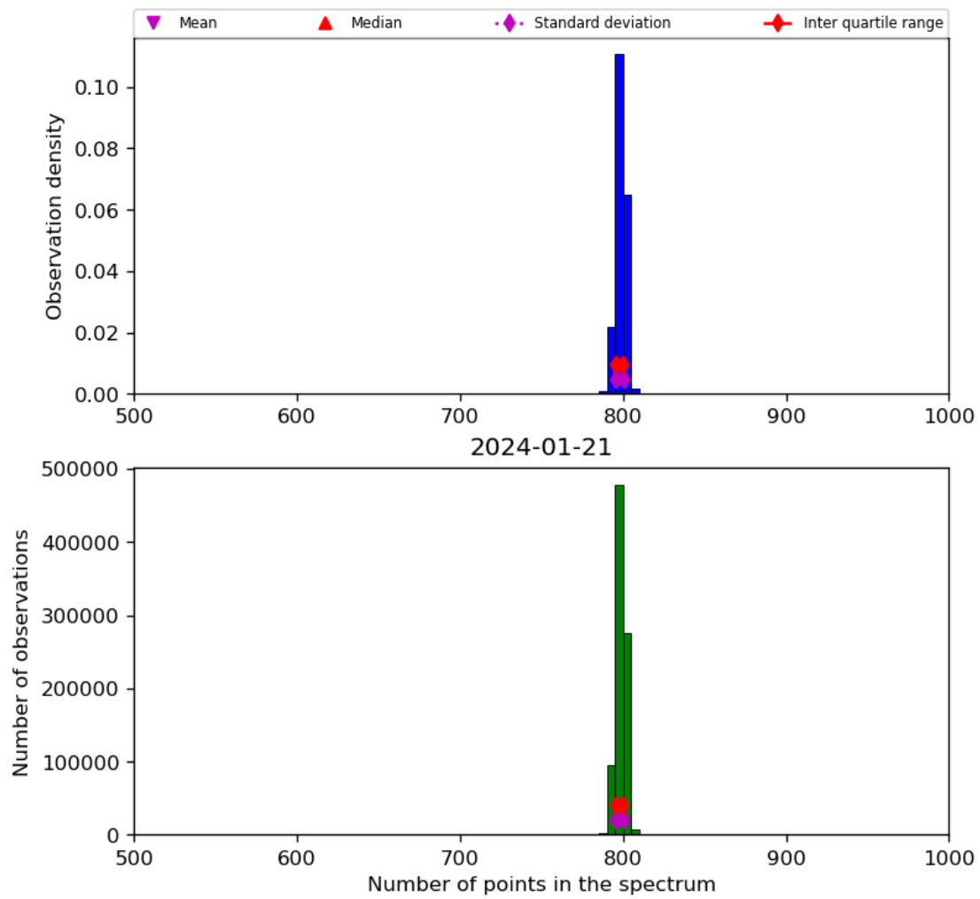
Figure 26: Histogram of “Number of points in the spectrum” for 2024-01-21 to 2024-01-22
