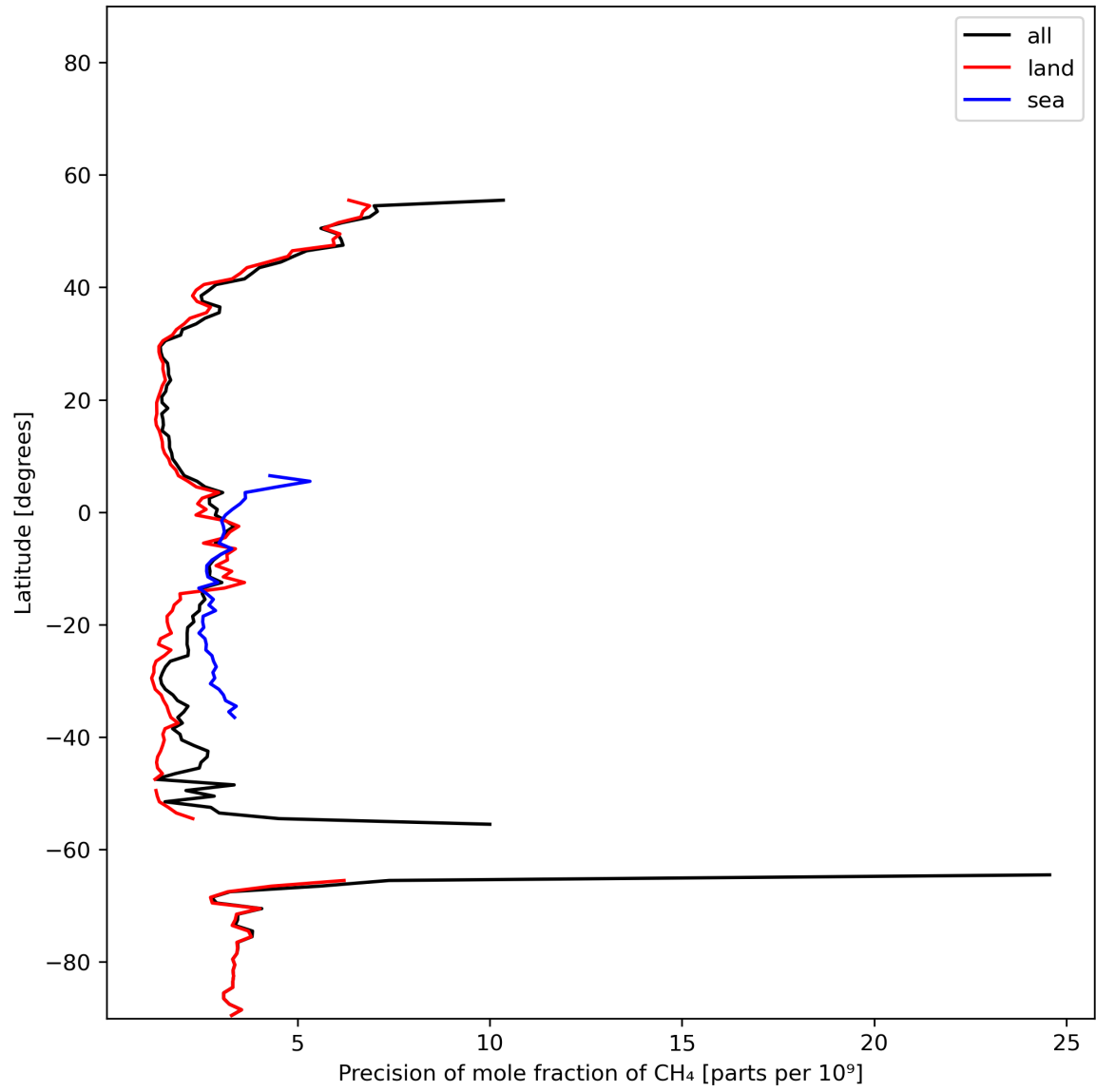
Figure 13: Zonal average of “Precision of mole fraction of CH 4 ” for 2024-01-21 to 2024-01-22.
