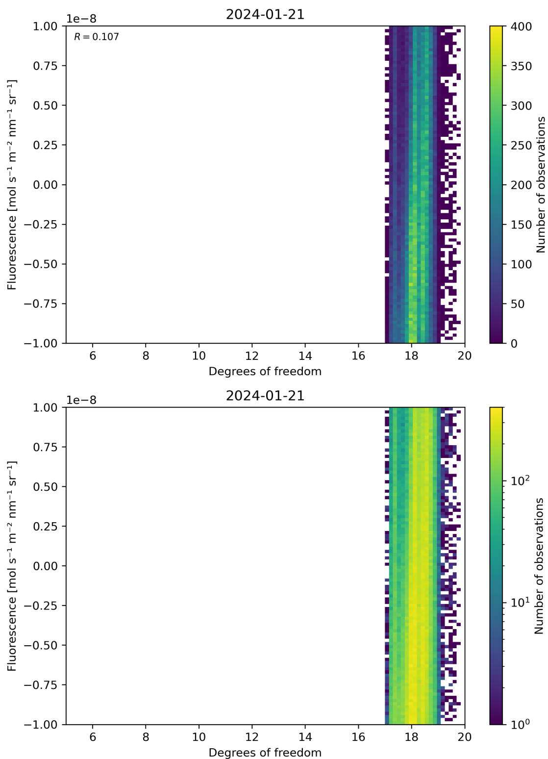
Figure 51: Scatter density plot of “Degrees of freedom” against “Fluorescence” for 2024-01-21 to 2024-01-22.
