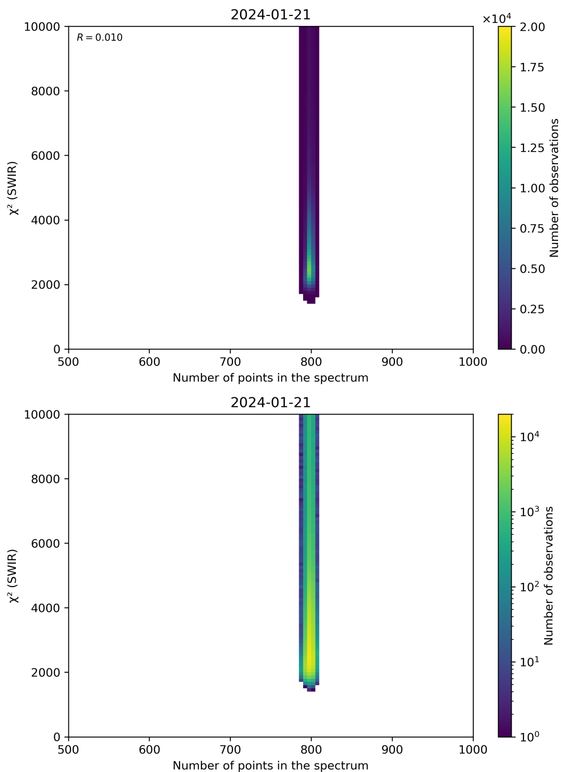
Figure 89: Scatter density plot of “Number of points in the spectrum” against “ \chi^2 (SWIR)” for 2024-01-21 to 2024-01-22.
