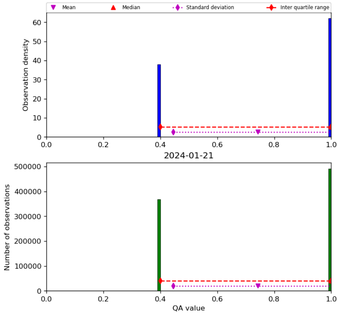
Figure 22: Histogram of “QA value” for 2024-01-21 to 2024-01-22
