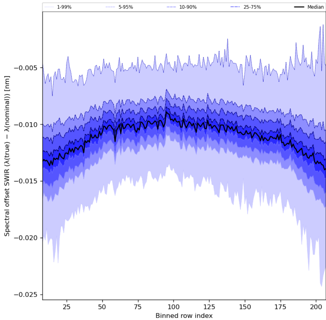
Figure 38: Along track statistics of “Spectral offset SWIR ( \lambda(\text{true}) - \lambda(\text{nominal}) )” for 2024-01-21 to 2024-01-22
