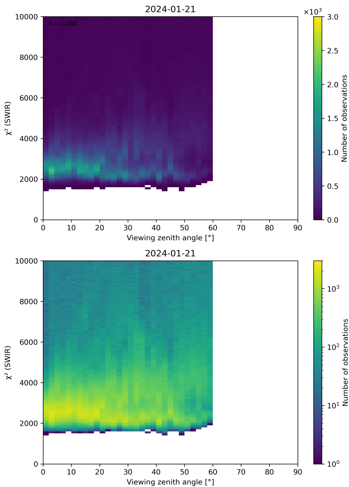
Figure 106: Scatter density plot of “Viewing zenith angle” against “ \chi^2 (SWIR)” for 2024-01-21 to 2024-01-22.
