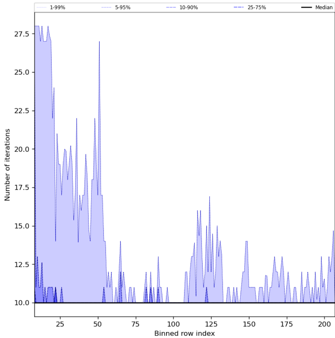
Figure 42: Along track statistics of “Number of iterations” for 2024-01-21 to 2024-01-22
