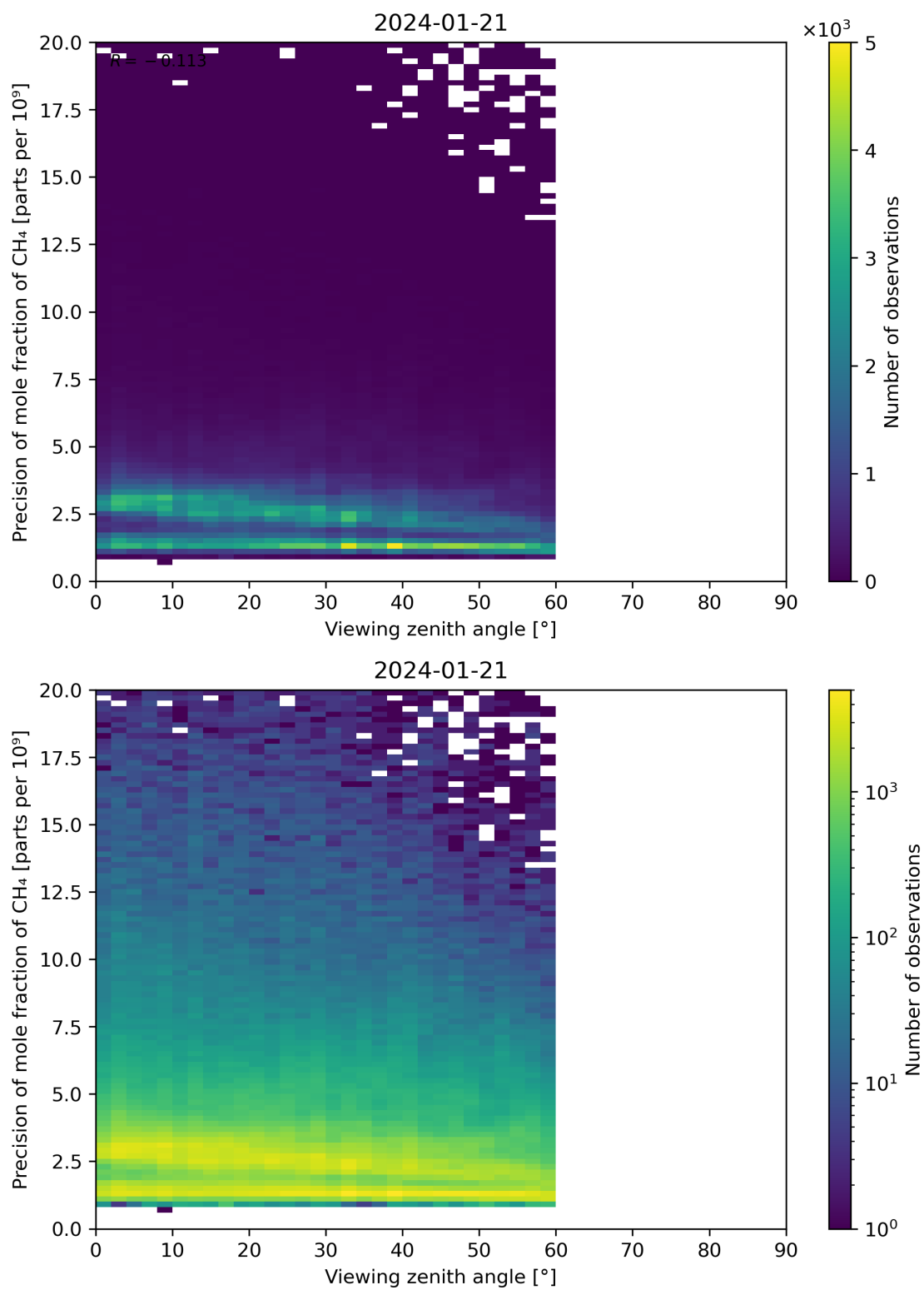
Figure 112: Scatter density plot of “Viewing zenith angle” against “Precision of mole fraction of CH 4 ” for 2024-01-21 to 2024-01-22.
