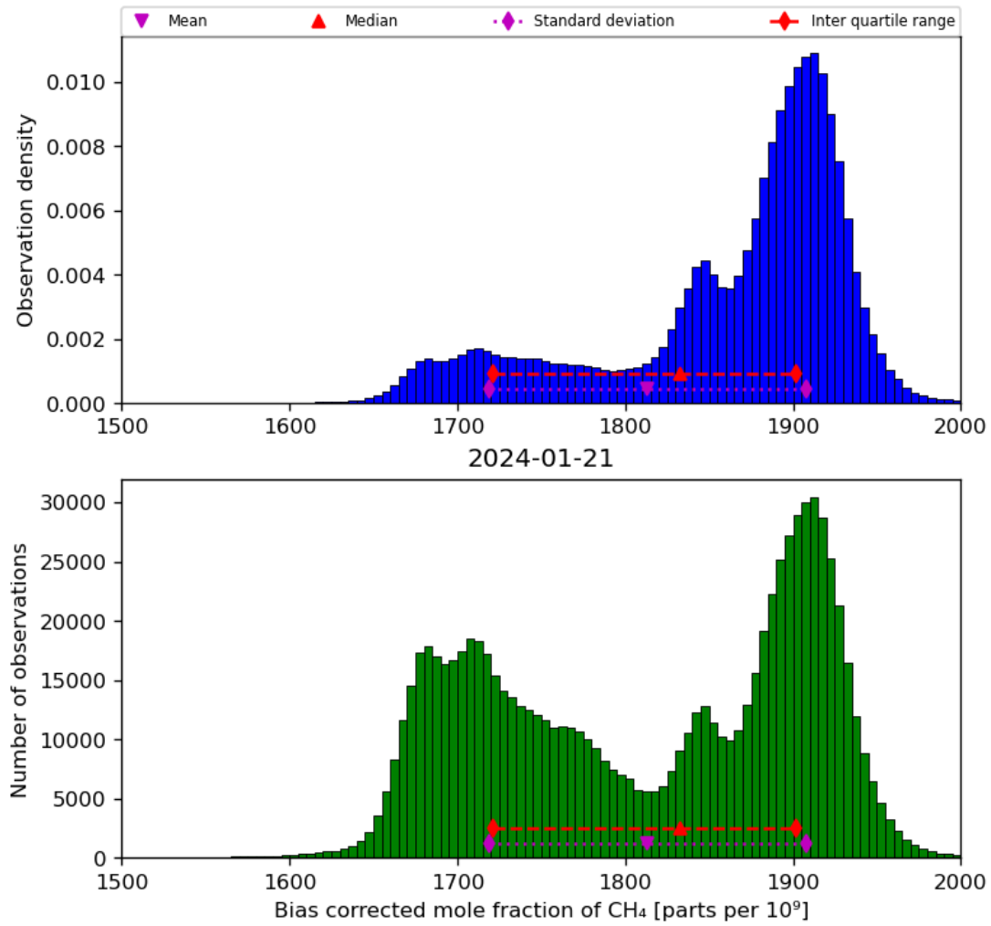
Figure 25: Histogram of “Bias corrected mole fraction of CH 4 ” for 2024-01-21 to 2024-01-22
