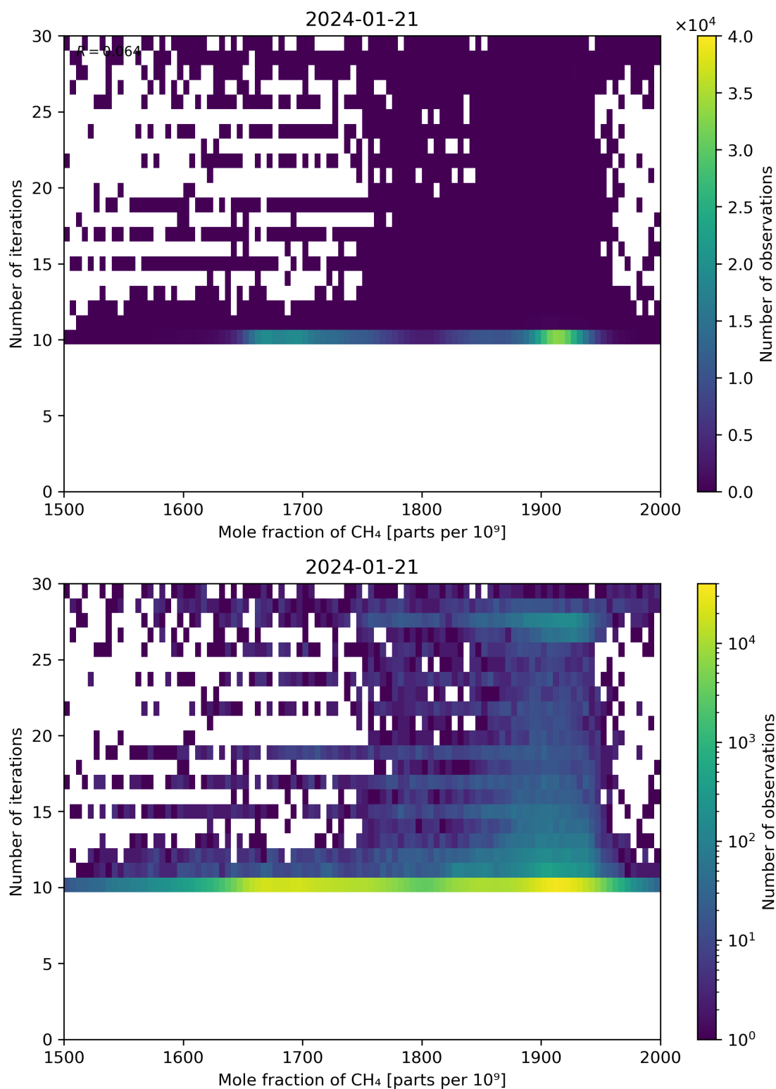
Figure 76: Scatter density plot of “Mole fraction of CH 4 ” against “Number of iterations” for 2024-01-21 to 2024-01-22.
