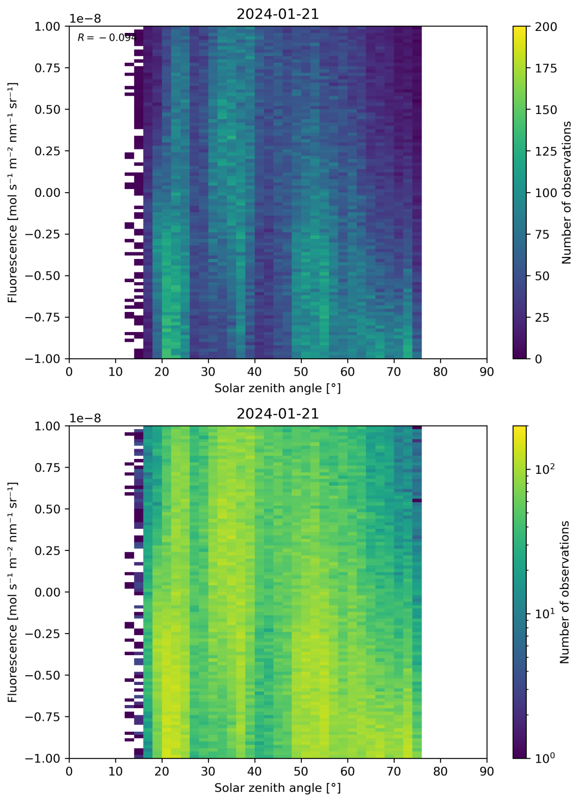
Figure 97: Scatter density plot of “Solar zenith angle” against “Fluorescence” for 2024-01-21 to 2024-01-22.
