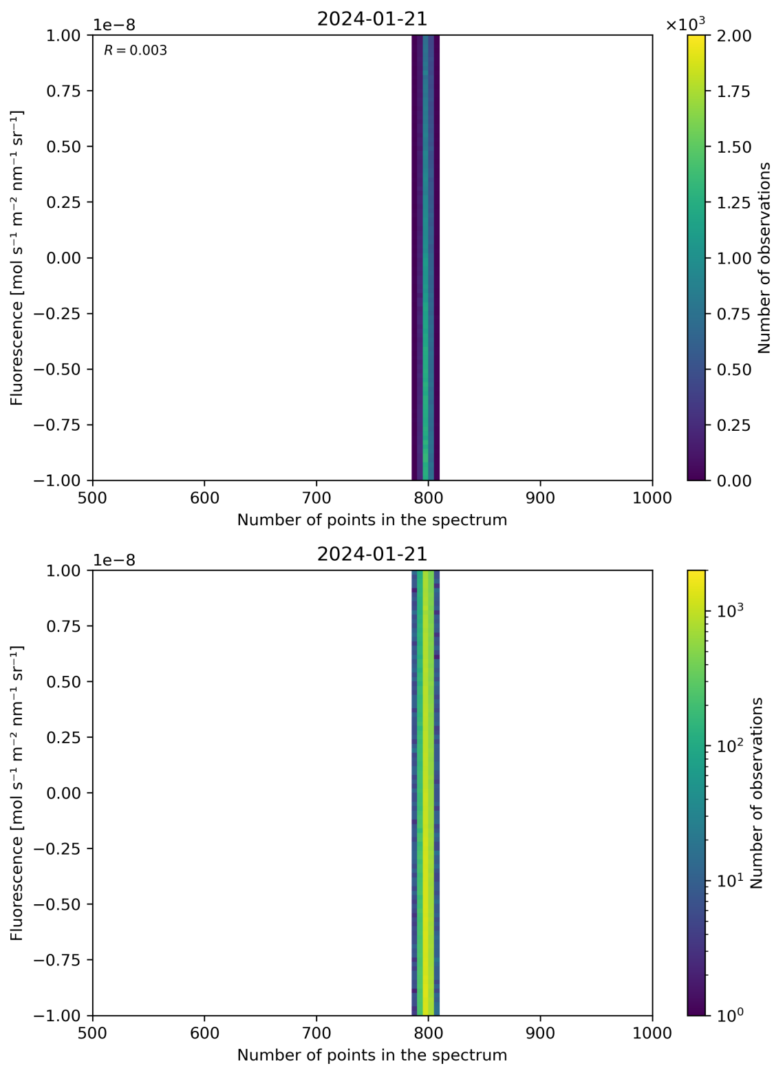
Figure 91: Scatter density plot of “Number of points in the spectrum” against “Fluorescence” for 2024-01-21 to 2024-01-22.
