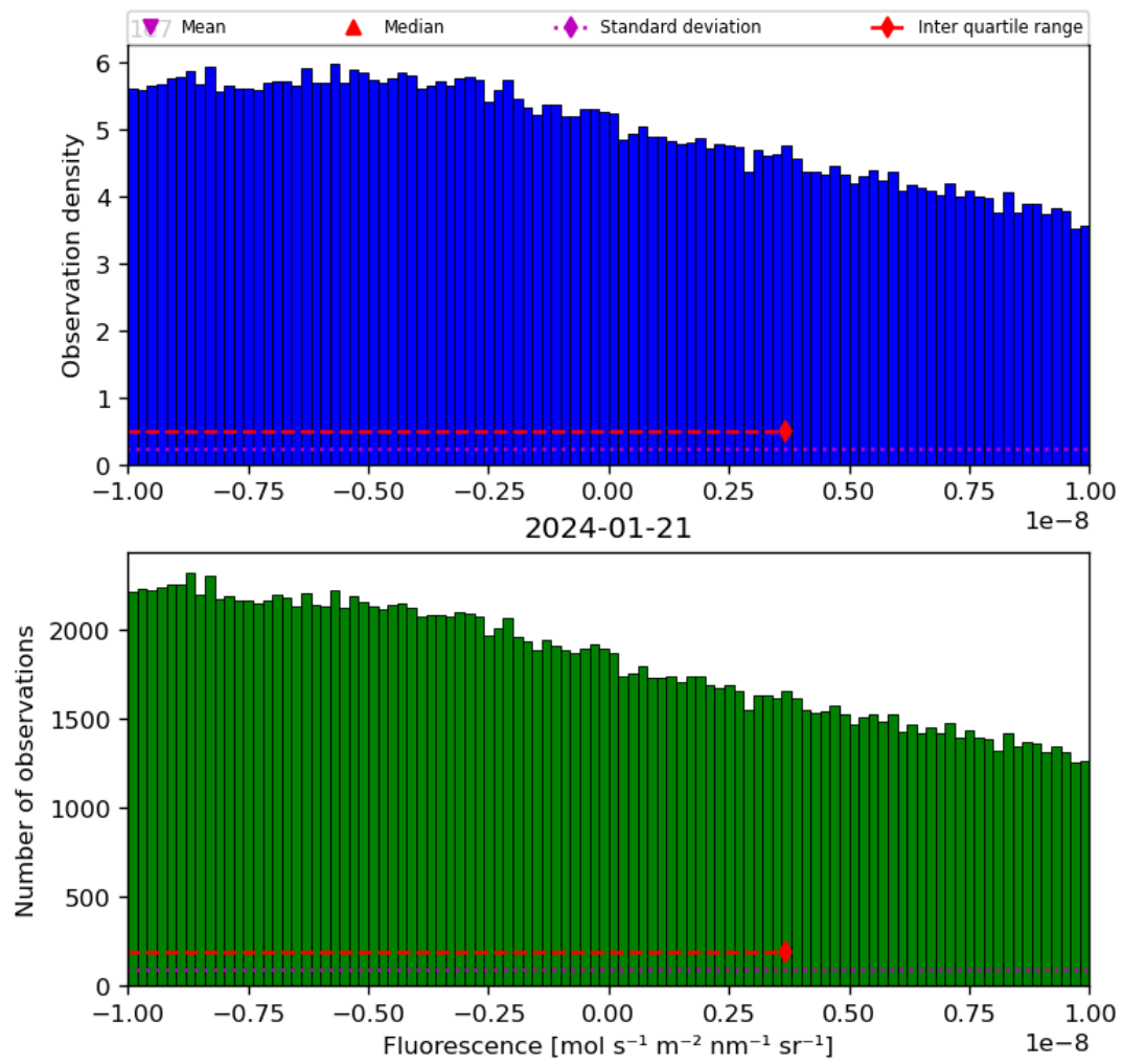
Figure 32: Histogram of “Fluorescence” for 2024-01-21 to 2024-01-22
