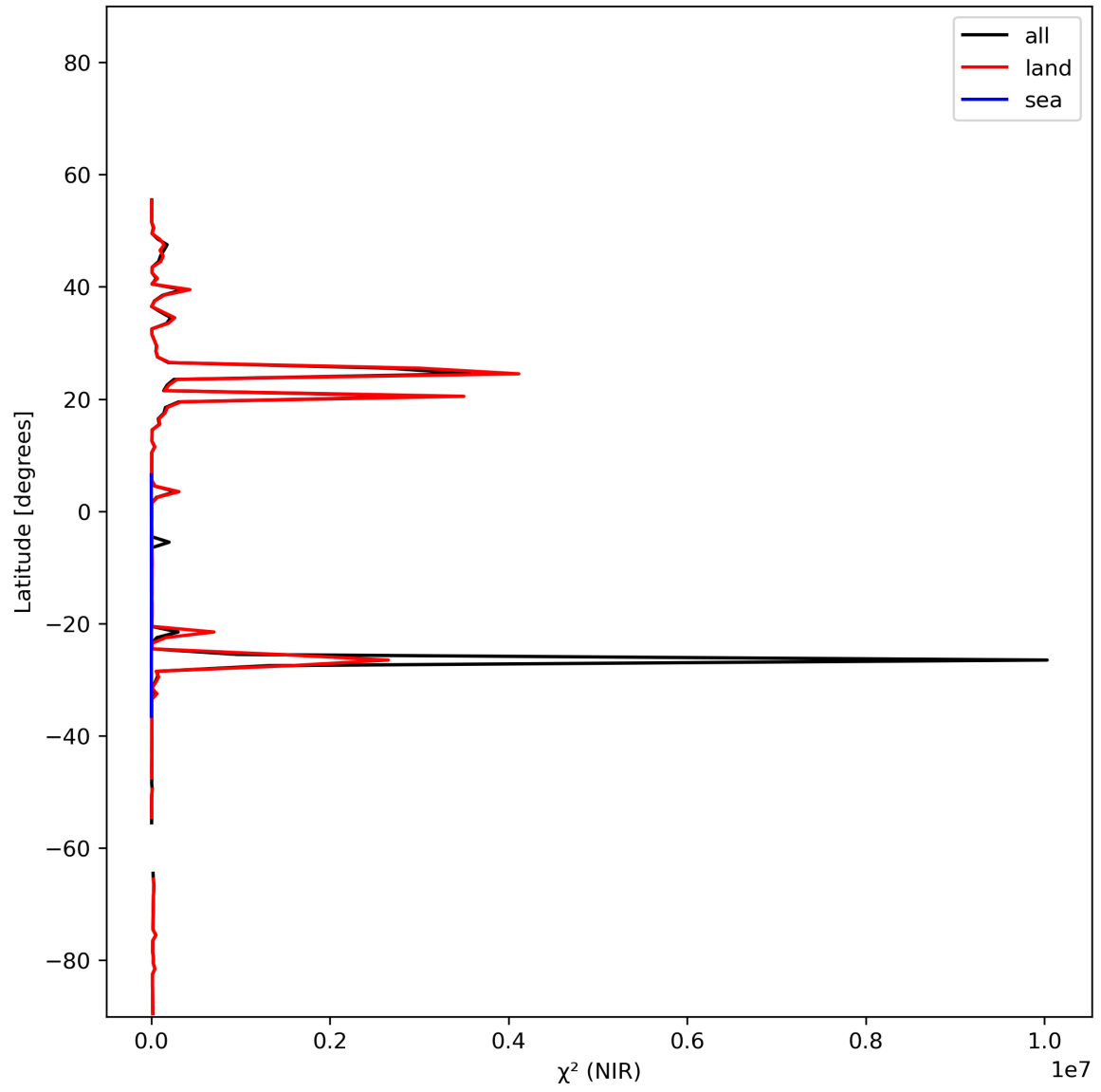
Figure 18: Zonal average of “ \chi^2 (NIR)” for 2024-01-21 to 2024-01-22.
