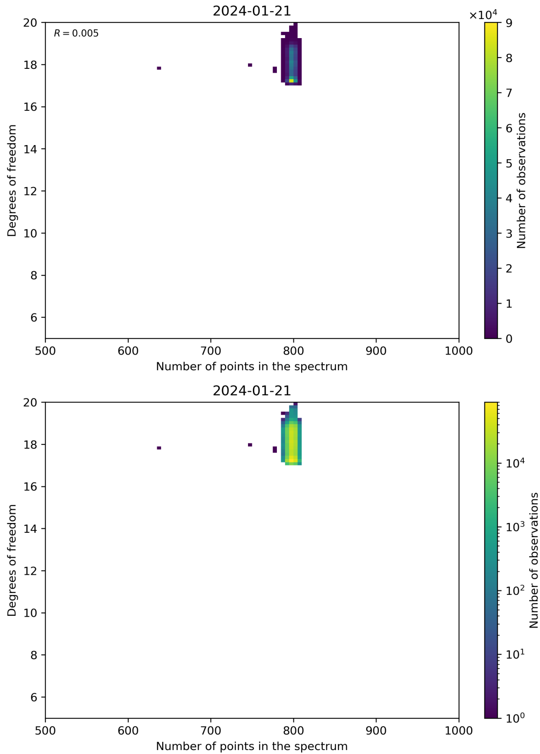
Figure 90: Scatter density plot of “Number of points in the spectrum” against “Degrees of freedom” for 2024-01-21 to 2024-01-22.
