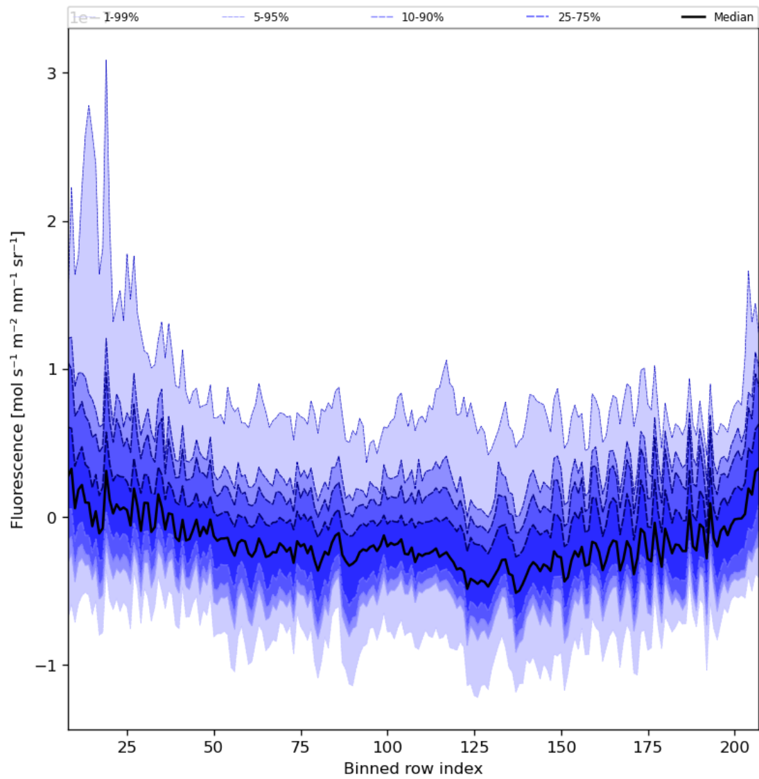
Figure 43: Along track statistics of “Fluorescence” for 2024-01-21 to 2024-01-22
