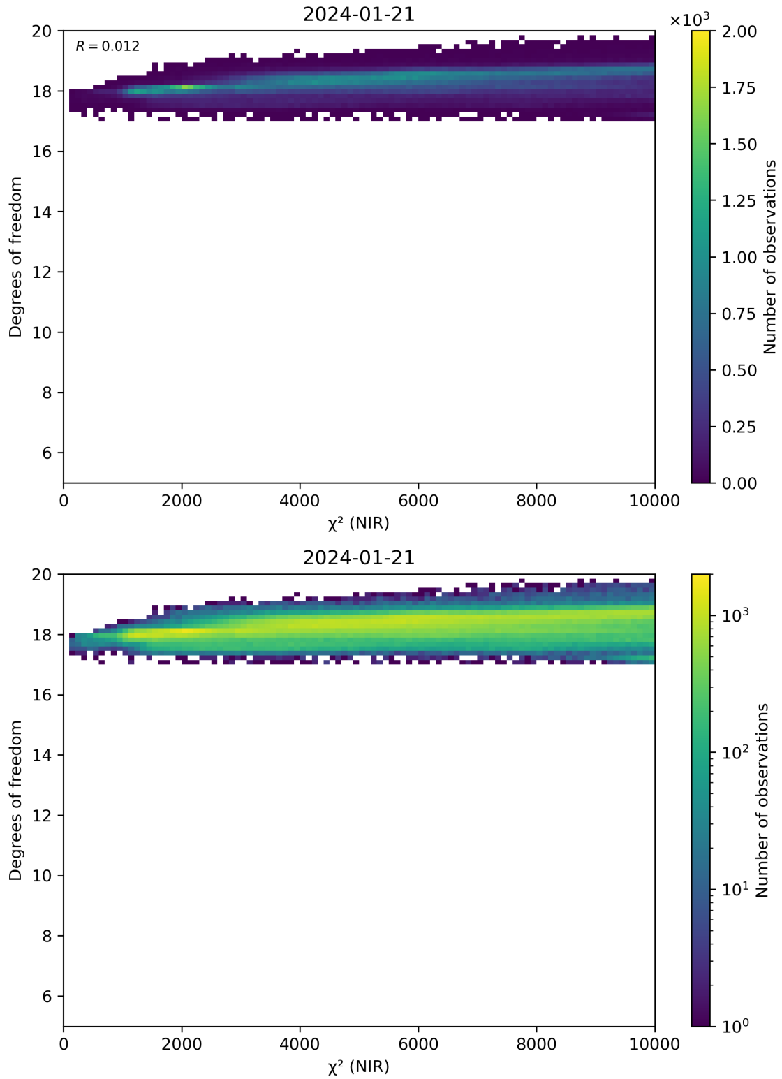
Figure 44: Scatter density plot of “ \chi^2 (NIR)” against “Degrees of freedom” for 2024-01-21 to 2024-01-22.
