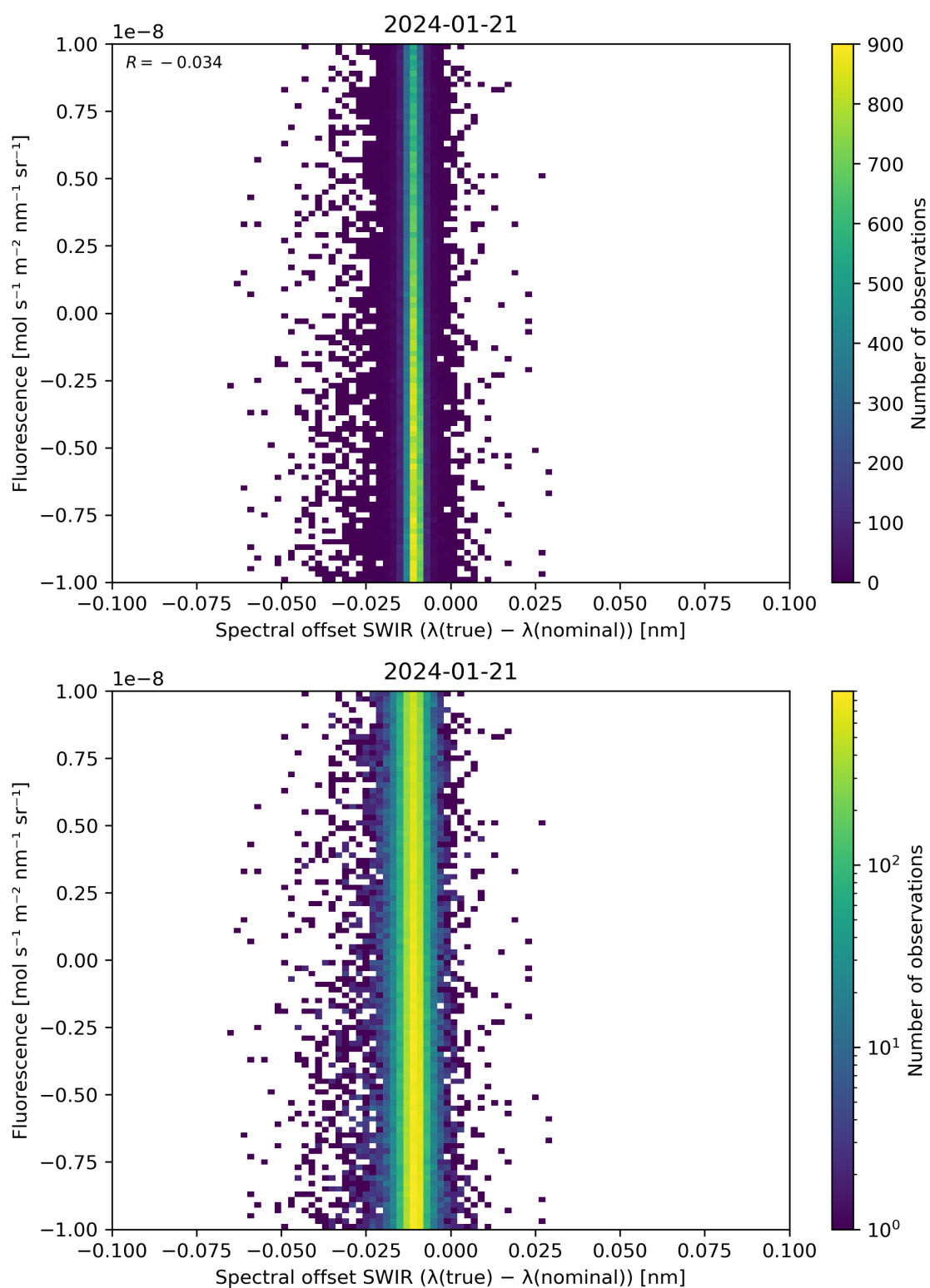
Figure 120: Scatter density plot of “Spectral offset SWIR ( \lambda(\text{true}) - \lambda(\text{nominal}) )” against “Fluorescence” for 2024-01-21 to 2024-01-22.
