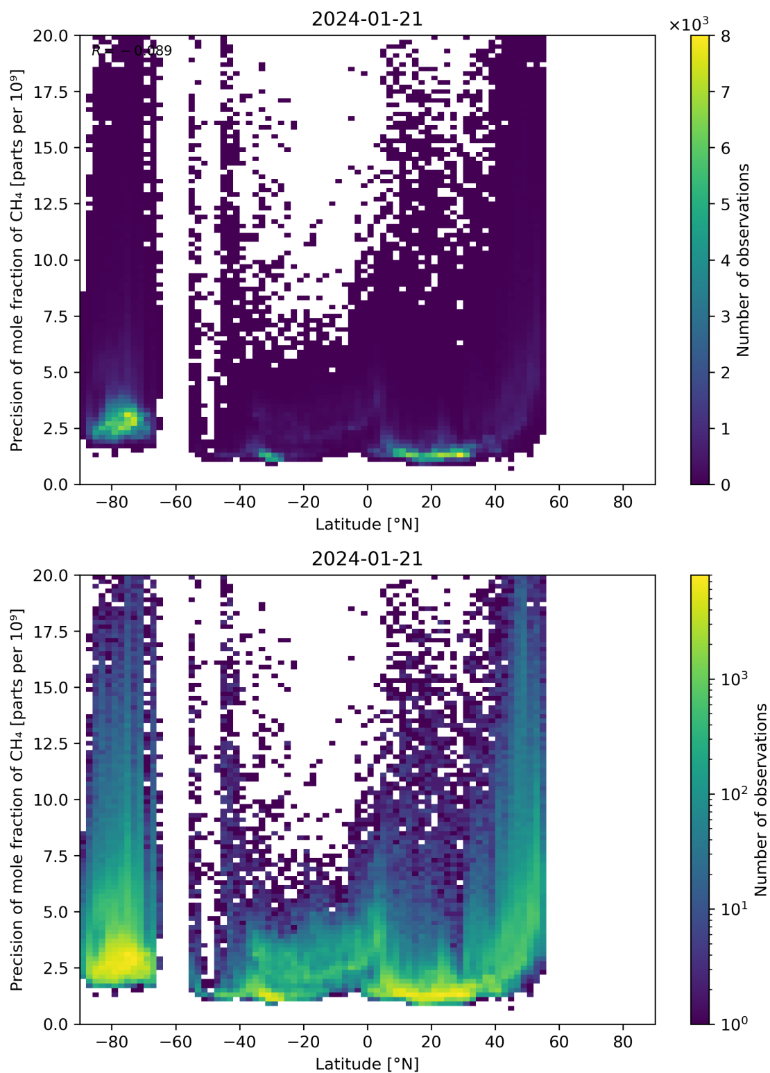
Figure 59: Scatter density plot of “Latitude” against “Precision of mole fraction of CH 4 ” for 2024-01-21 to 2024-01-22.
