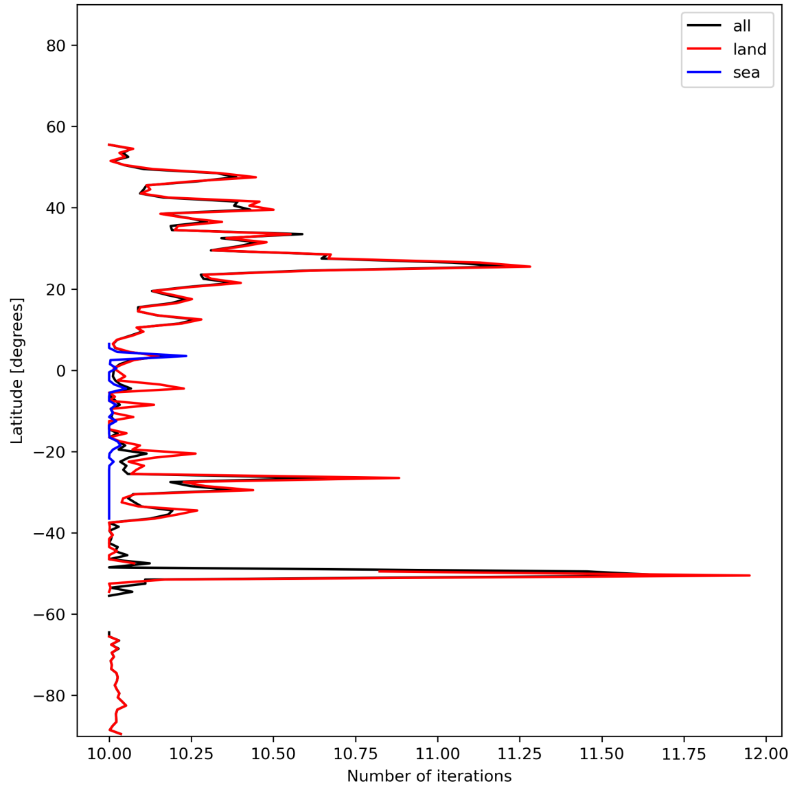
Figure 20: Zonal average of “Number of iterations” for 2024-01-21 to 2024-01-22.
