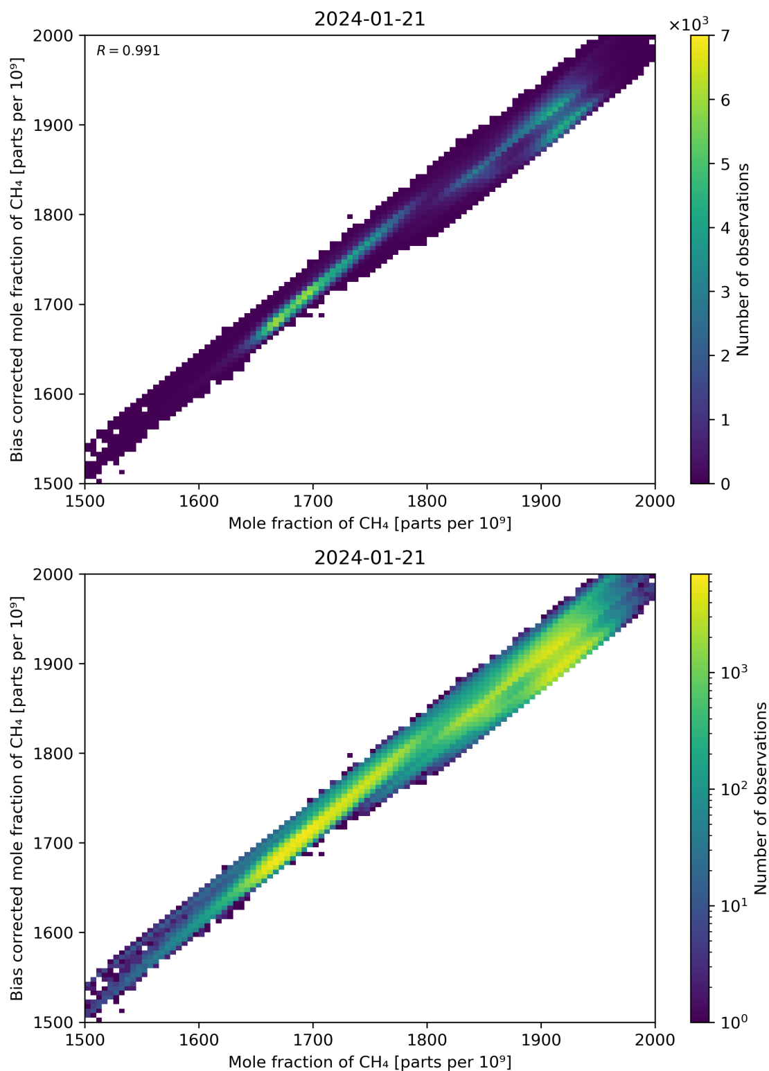
Figure 74: Scatter density plot of “Mole fraction of CH 4 ” against “Bias corrected mole fraction of CH 4 ” for 2024-01-21 to 2024-01-22.
