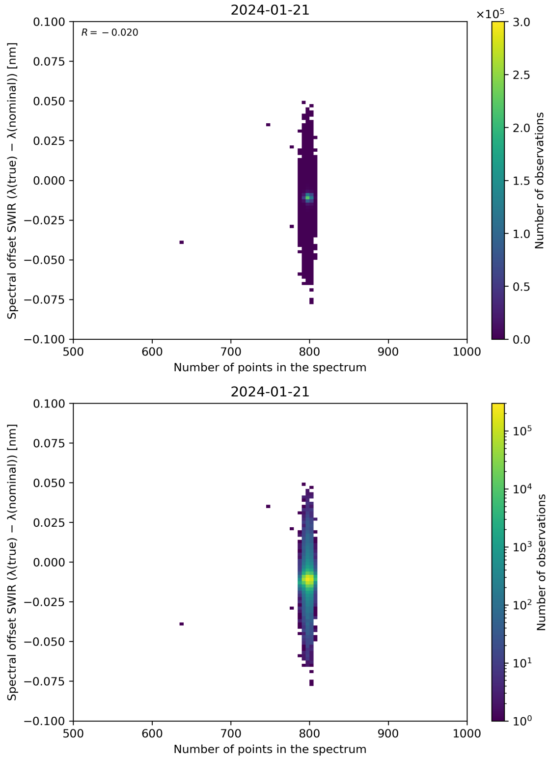
Figure 93: Scatter density plot of “Number of points in the spectrum” against “Spectral offset SWIR ( \lambda(\text{true}) - \lambda(\text{nominal}) )” for 2024-01-21 to 2024-01-22.
