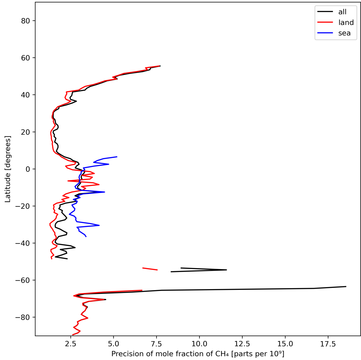
Figure 13: Zonal average of “Precision of mole fraction of \text{CH}_4 ” for 2024-01-21 to 2024-01-23.
