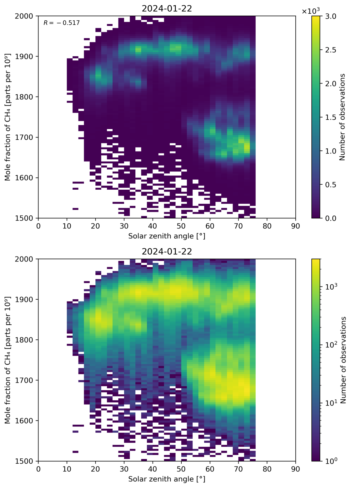
Figure 99: Scatter density plot of “Solar zenith angle” against “Mole fraction of \text{CH}_4 ” for 2024-01-21 to 2024-01-23.
