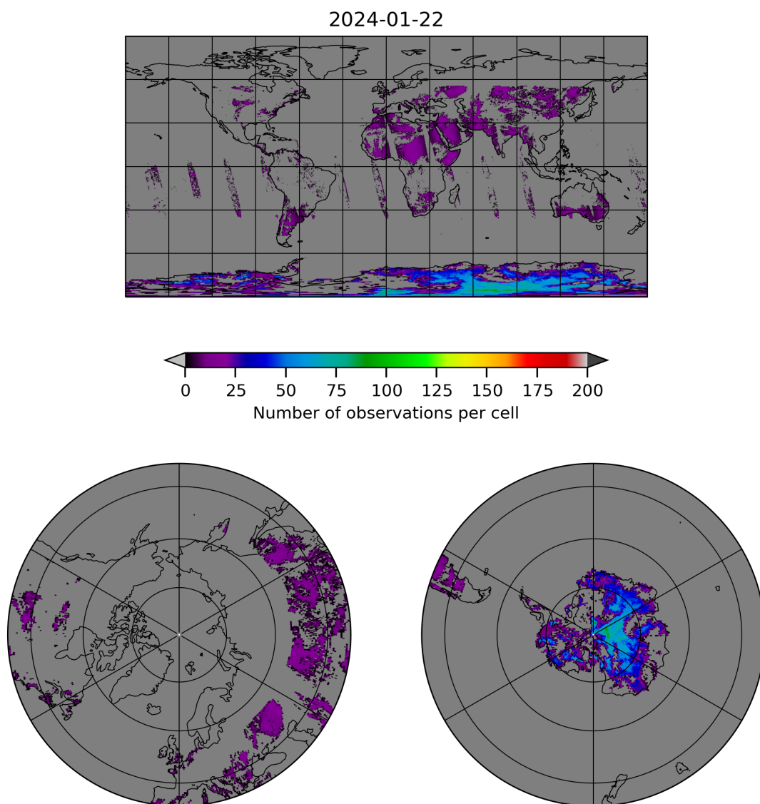
Figure 10: Map of the number of observations for 2024-01-21 to 2024-01-23
