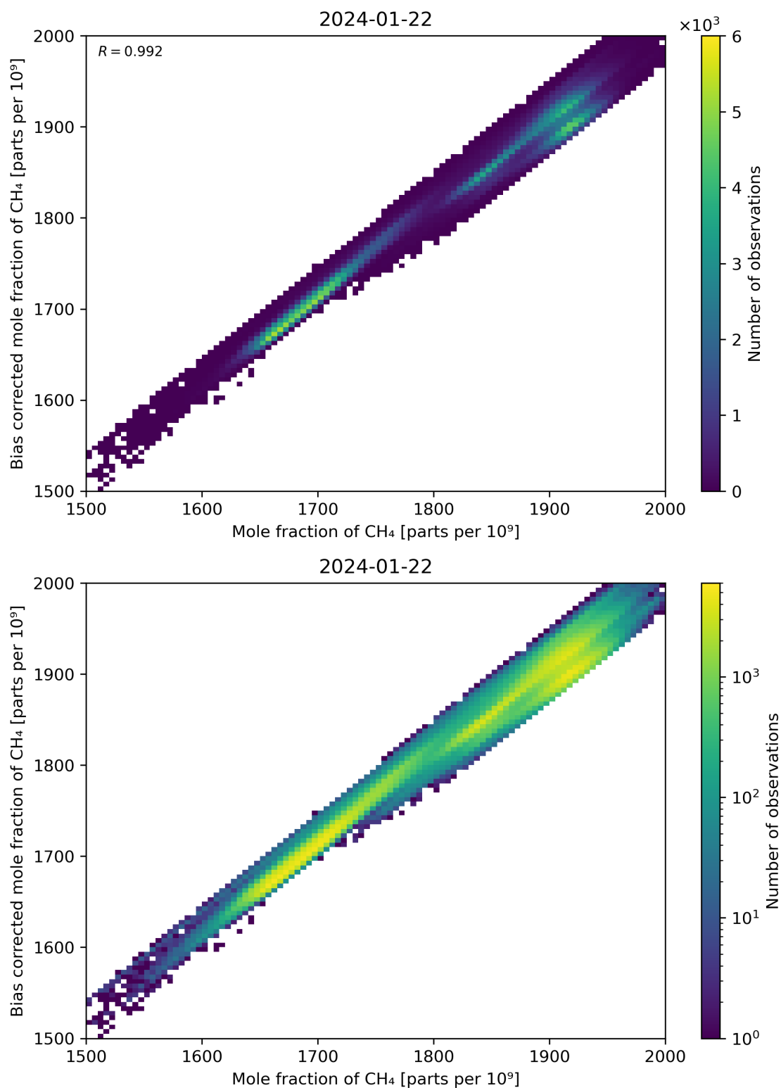
Figure 74: Scatter density plot of “Mole fraction of CH 4 ” against “Bias corrected mole fraction of CH 4 ” for 2024-01-21 to 2024-01-23.
