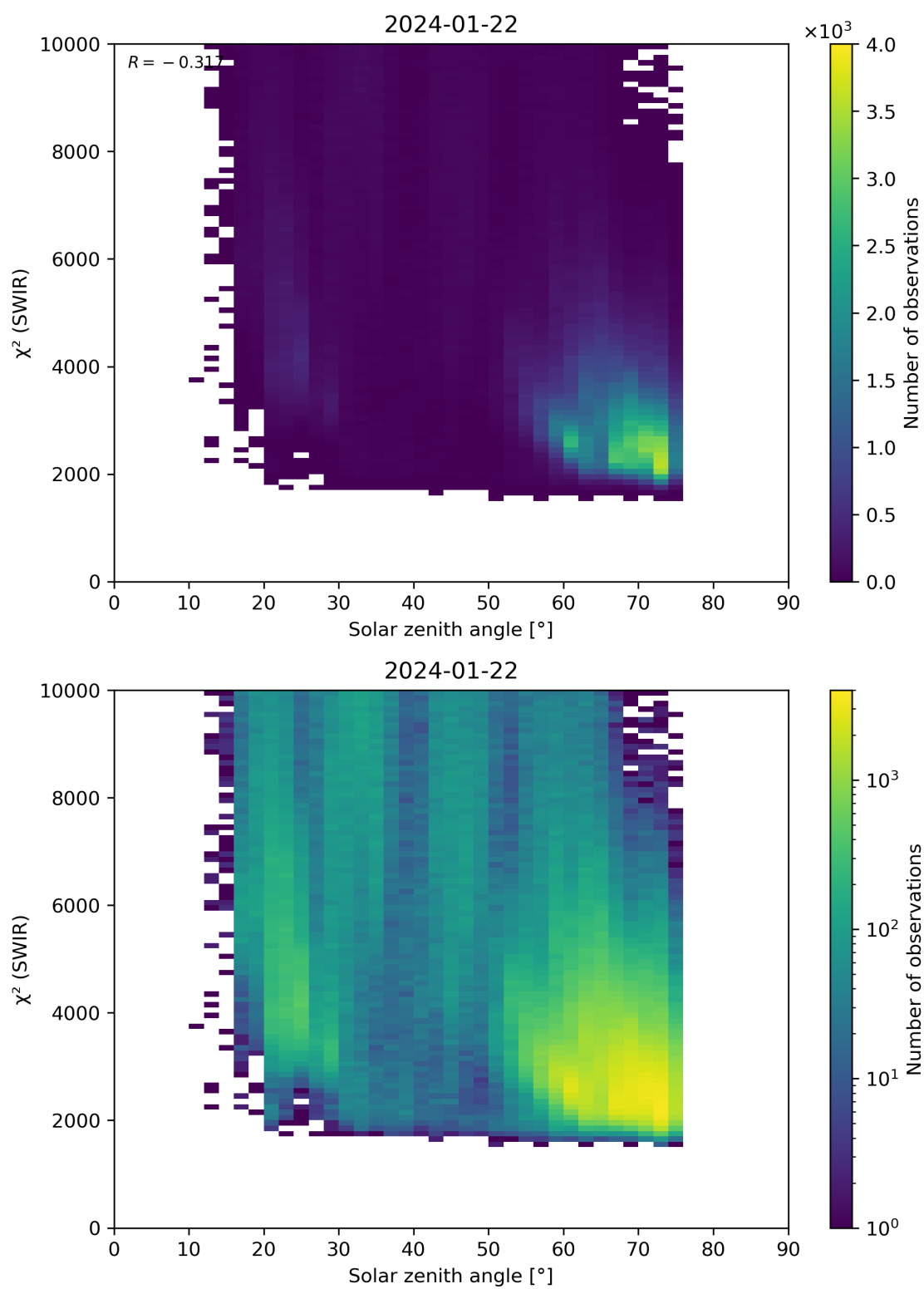
Figure 95: Scatter density plot of “Solar zenith angle” against “ \chi^2 (SWIR)” for 2024-01-21 to 2024-01-23.
