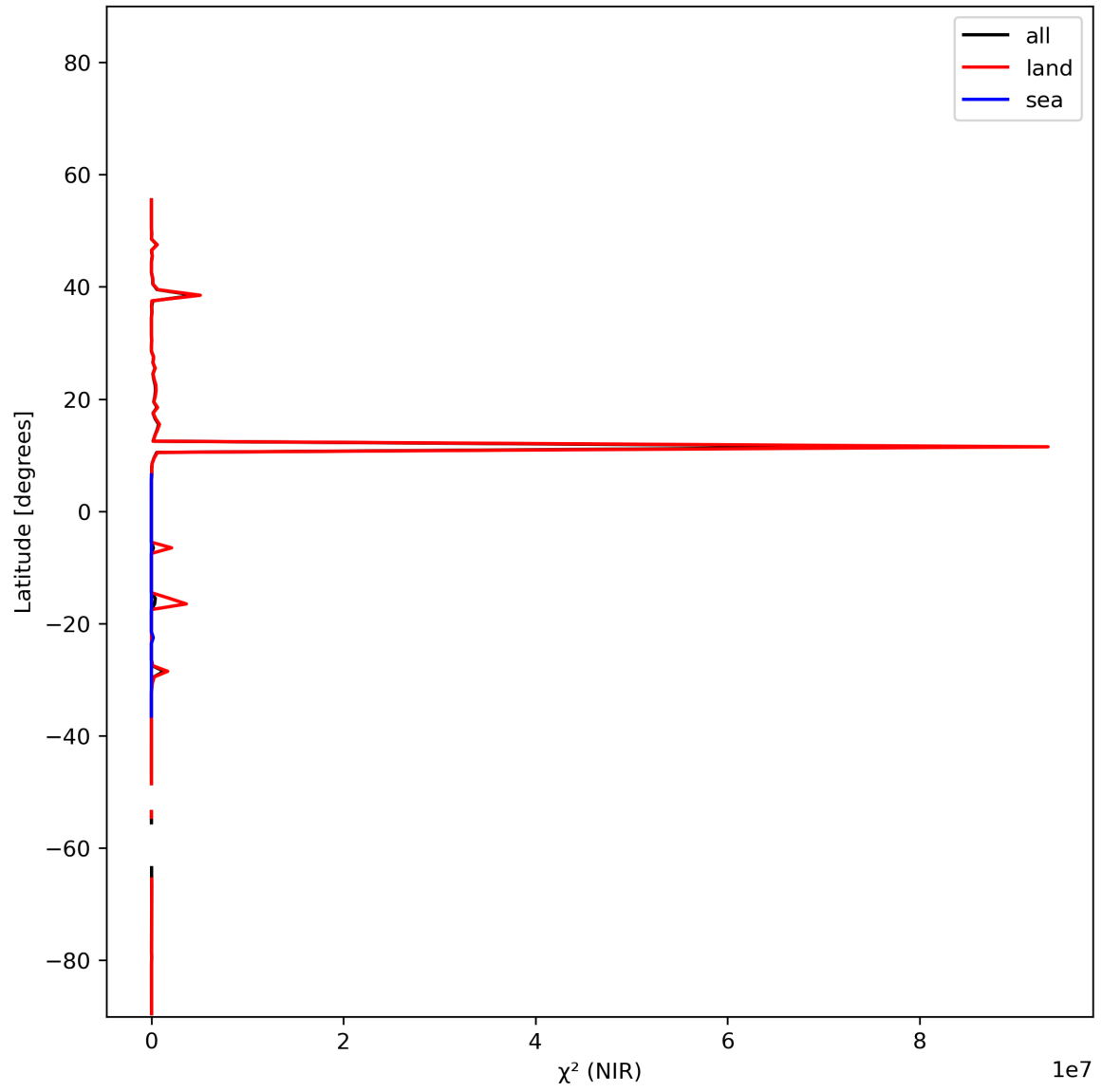
Figure 18: Zonal average of “ \chi^2 (NIR)” for 2024-01-21 to 2024-01-23.
