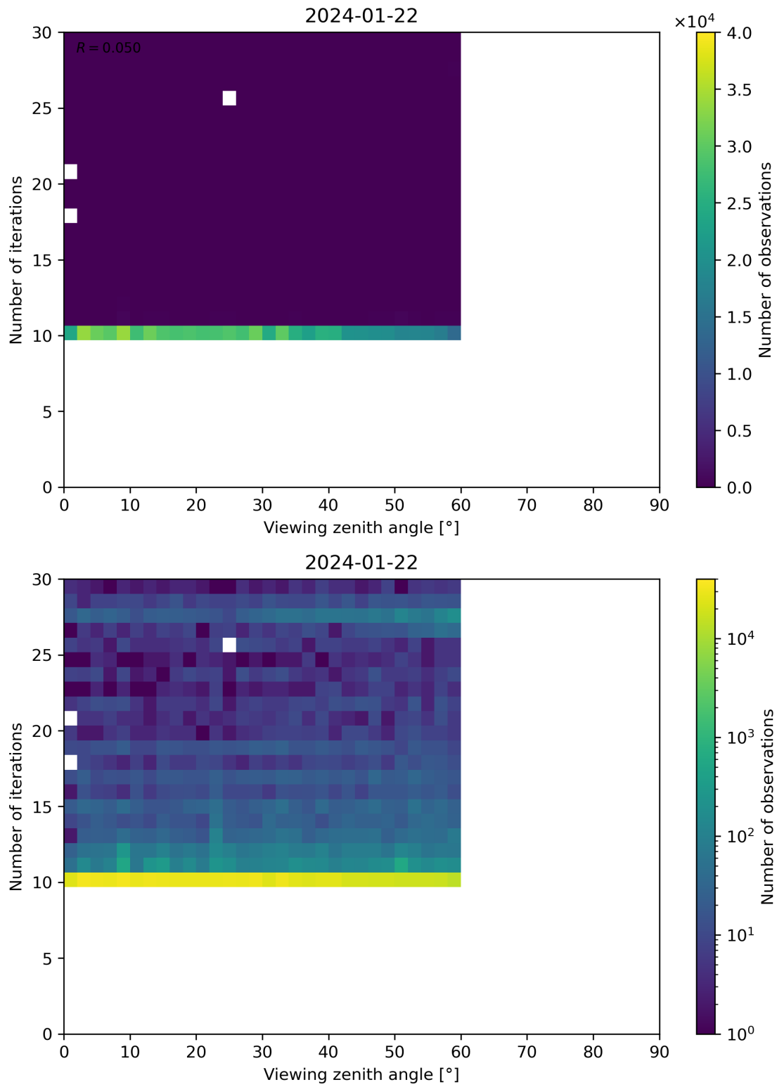
Figure 113: Scatter density plot of “Viewing zenith angle” against “Number of iterations” for 2024-01-21 to 2024-01-23.
