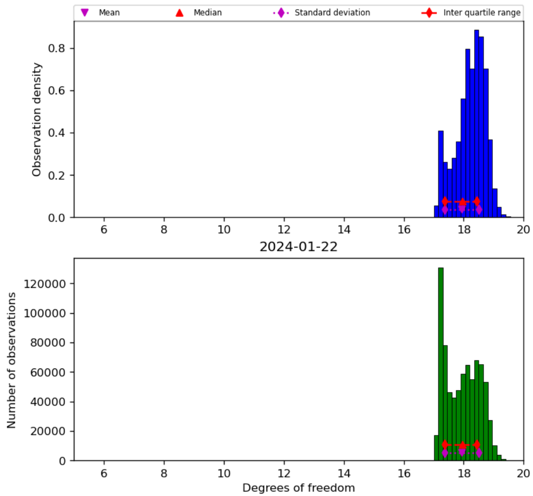
Figure 30: Histogram of “Degrees of freedom” for 2024-01-21 to 2024-01-23
