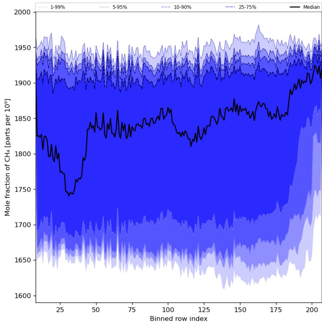
Figure 34: Along track statistics of “Mole fraction of CH 4 ” for 2024-01-21 to 2024-01-23
