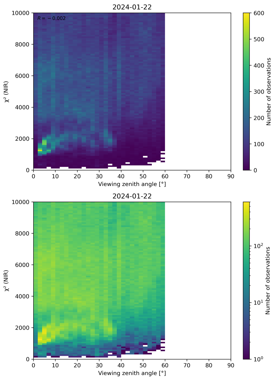
Figure 105: Scatter density plot of “Viewing zenith angle” against “ \chi^2 (NIR)” for 2024-01-21 to 2024-01-23.
