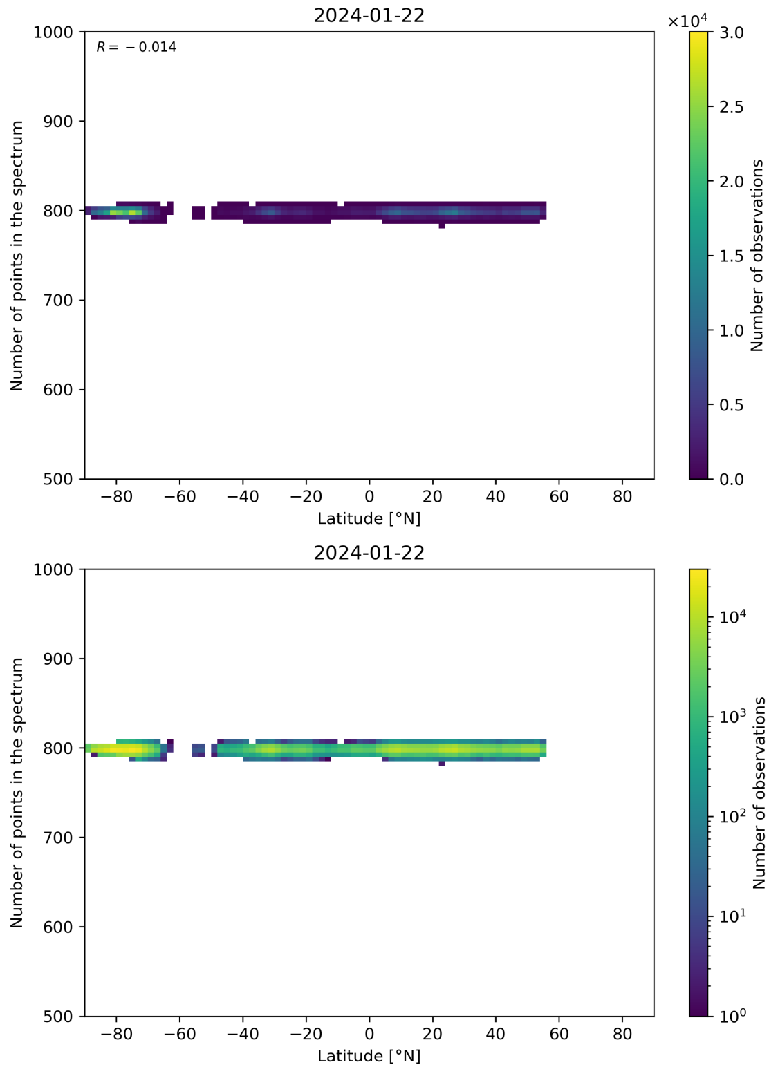
Figure 61: Scatter density plot of “Latitude” against “Number of points in the spectrum” for 2024-01-21 to 2024-01-23.
