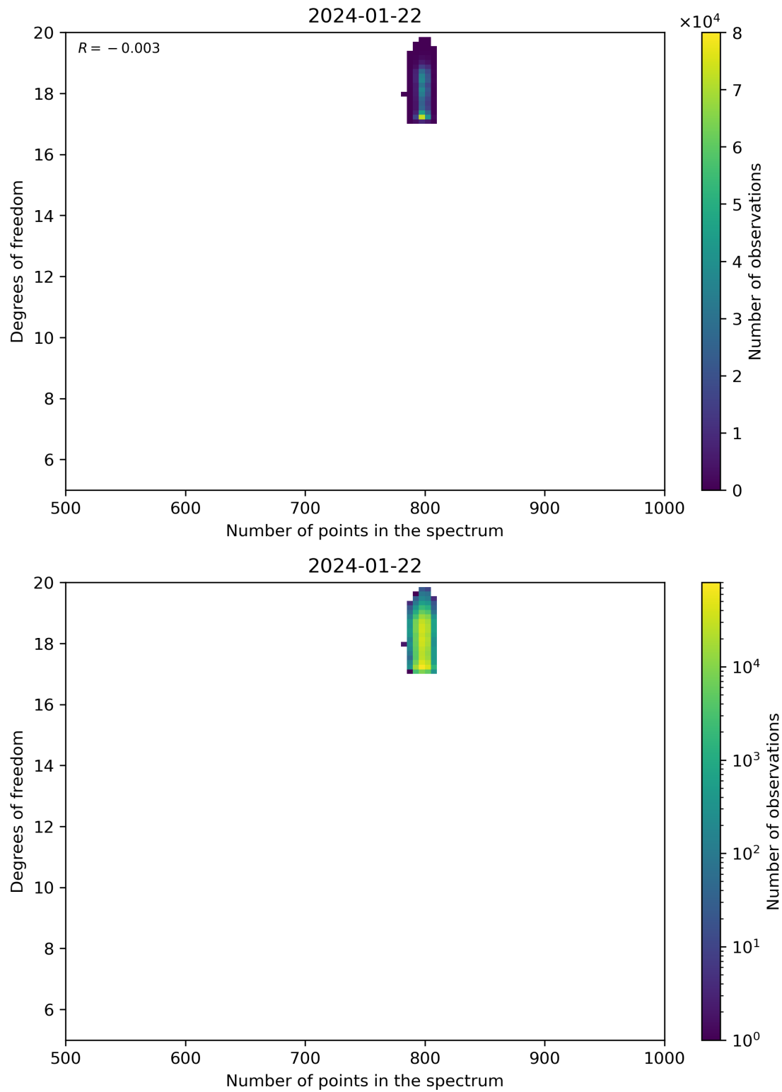
Figure 90: Scatter density plot of “Number of points in the spectrum” against “Degrees of freedom” for 2024-01-21 to 2024-01-23.
