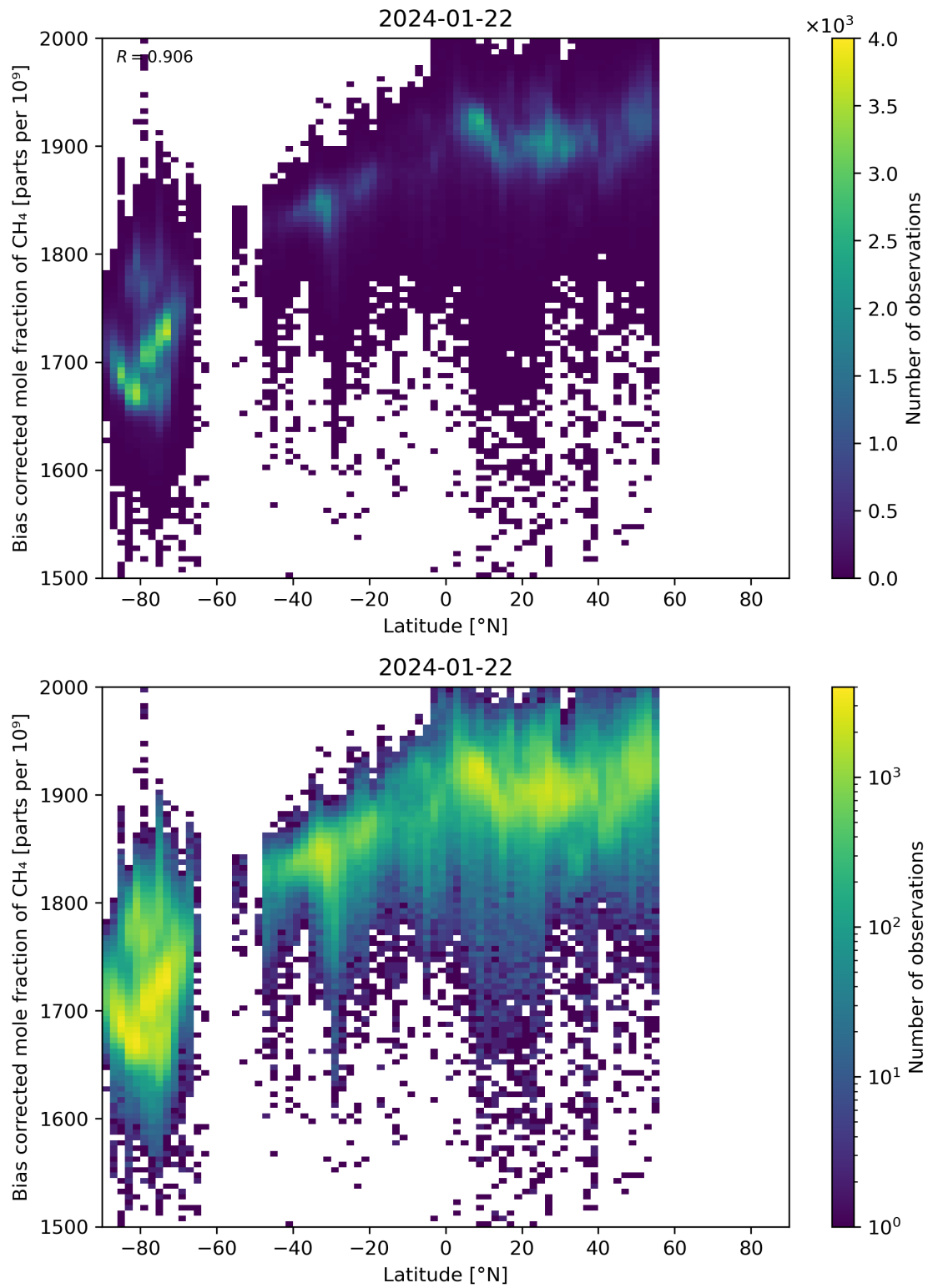
Figure 58: Scatter density plot of “Latitude” against “Bias corrected mole fraction of CH 4 ” for 2024-01-21 to 2024-01-23.
