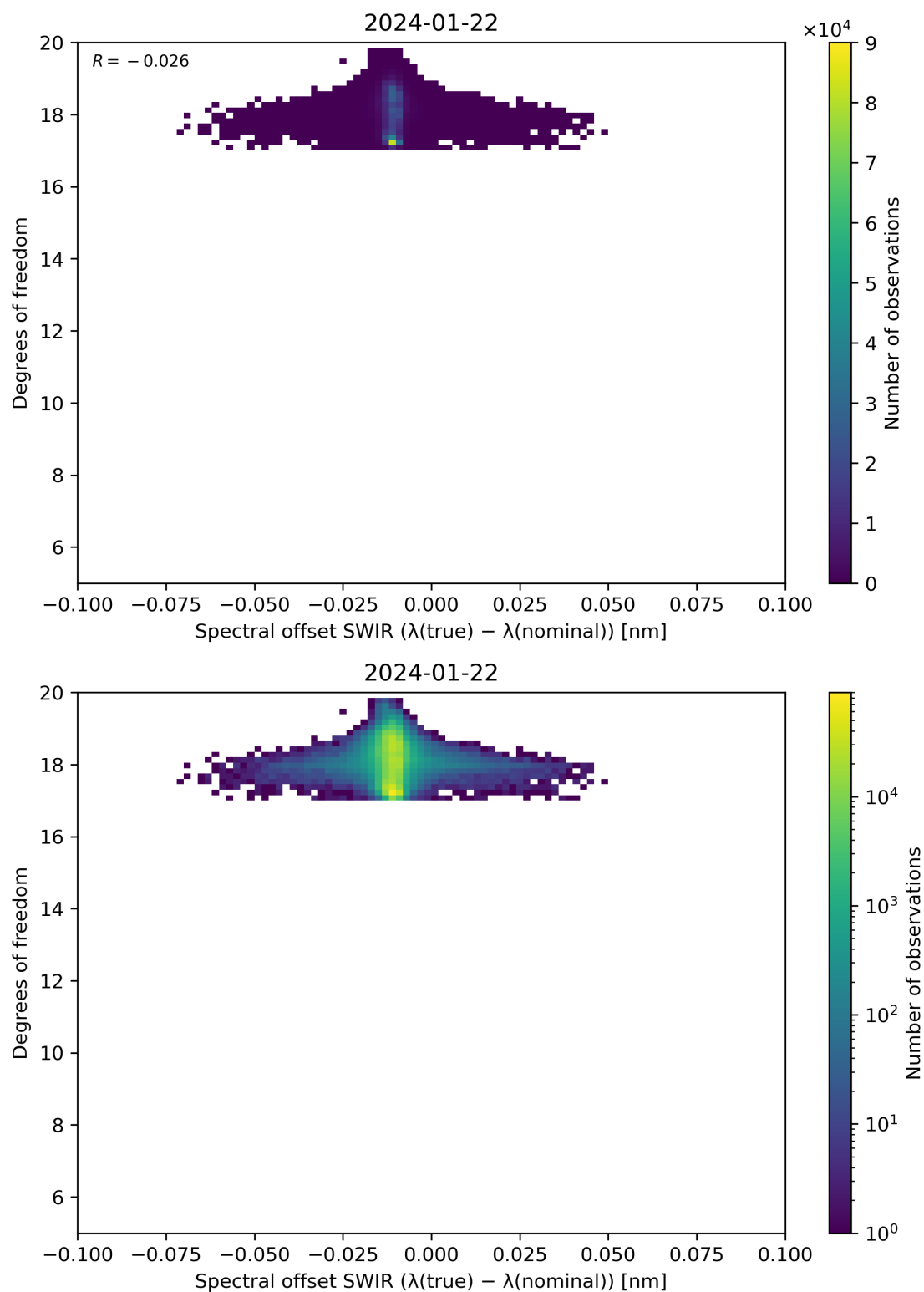
Figure 119: Scatter density plot of “Spectral offset SWIR ( \lambda(\text{true}) - \lambda(\text{nominal}) )” against “Degrees of freedom” for 2024-01-21 to 2024-01-23.
