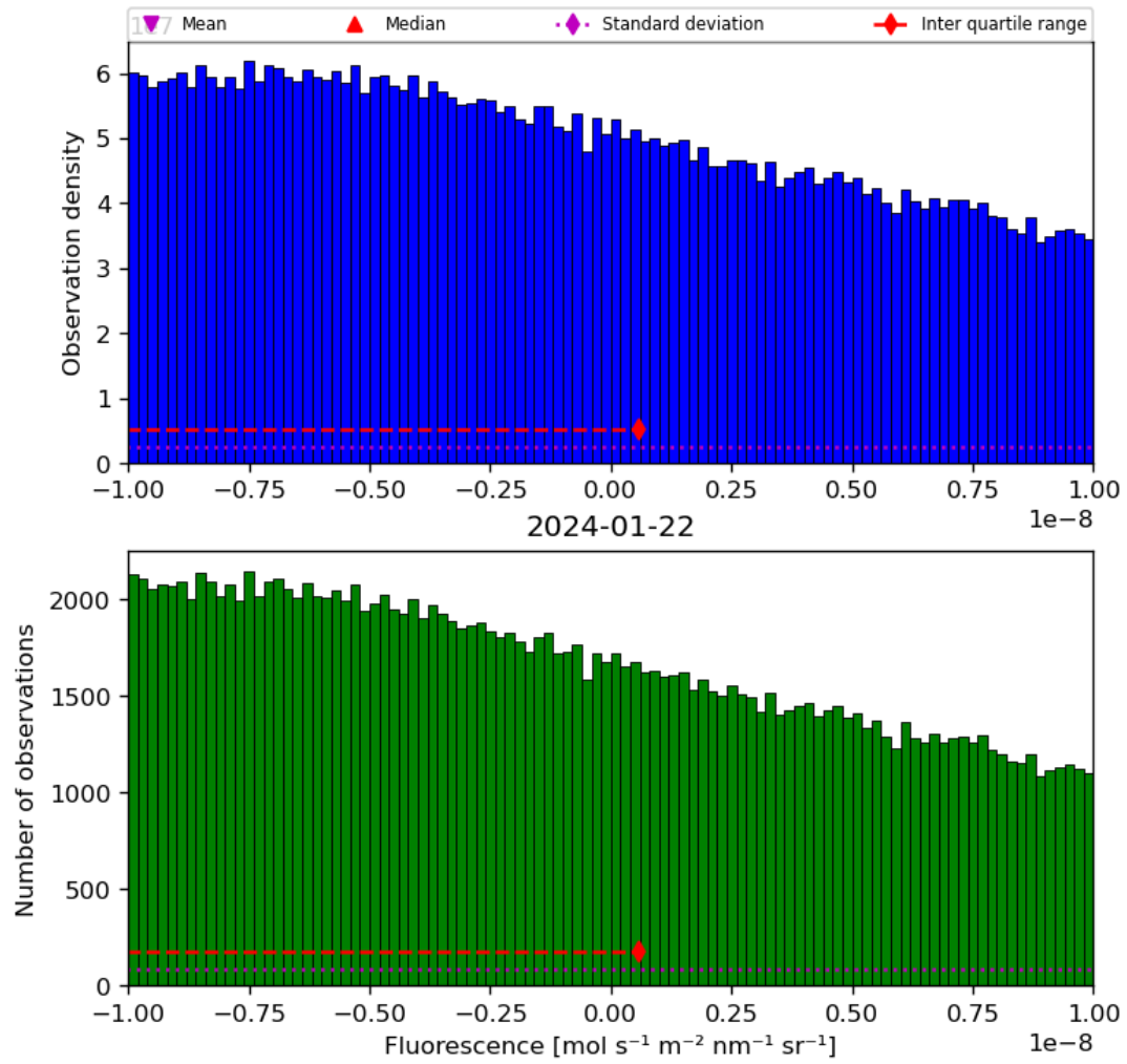
Figure 32: Histogram of “Fluorescence” for 2024-01-21 to 2024-01-23
