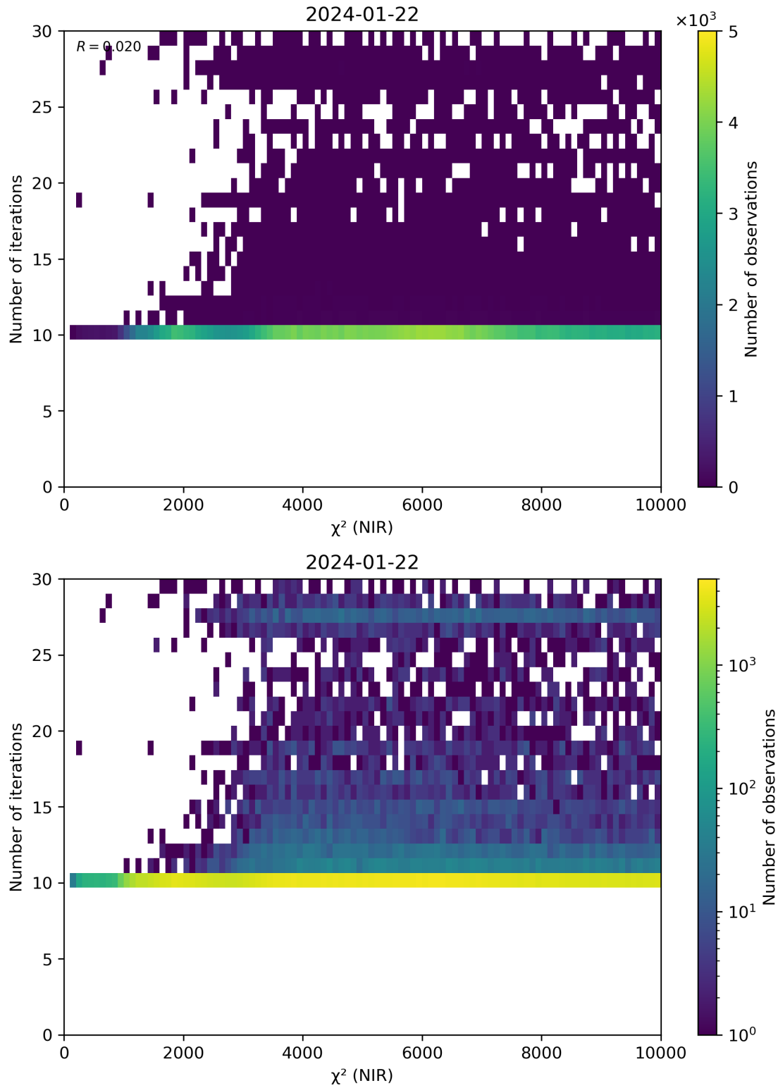
Figure 46: Scatter density plot of “ \chi^2 (NIR)” against “Number of iterations” for 2024-01-21 to 2024-01-23.
