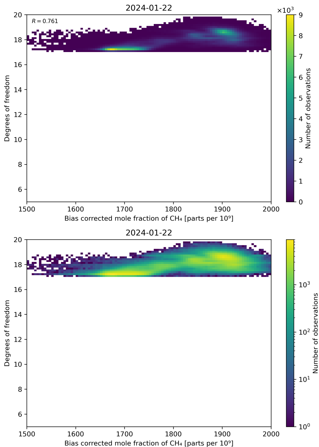
Figure 65: Scatter density plot of “Bias corrected mole fraction of CH 4 ” against “Degrees of freedom” for 2024-01-21 to 2024-01-23.
