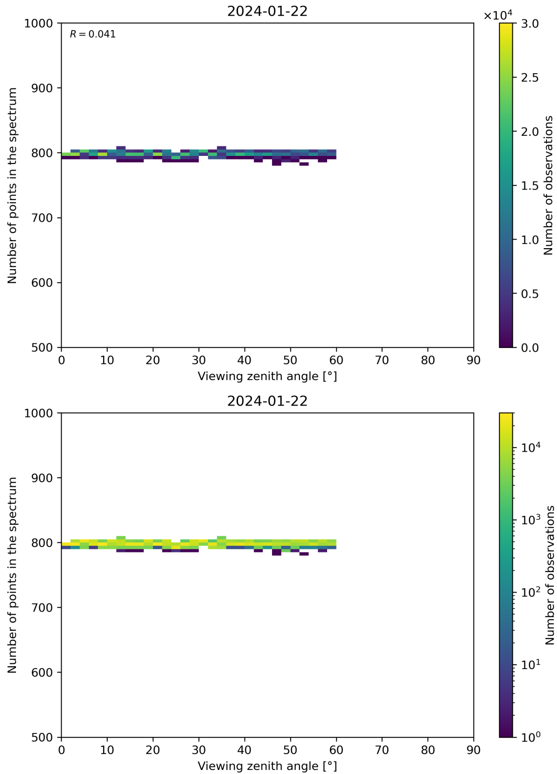
Figure 114: Scatter density plot of “Viewing zenith angle” against “Number of points in the spectrum” for 2024-01-21 to 2024-01-23.
