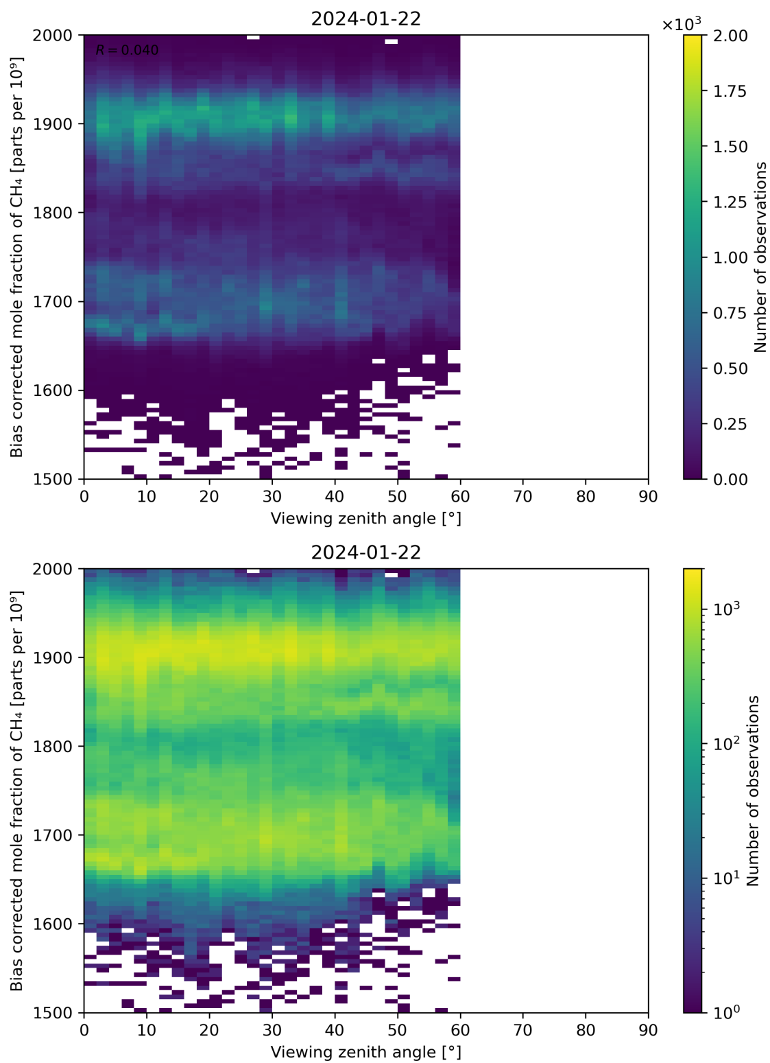
Figure 111: Scatter density plot of “Viewing zenith angle” against “Bias corrected mole fraction of CH 4 ” for 2024-01-21 to 2024-01-23.
