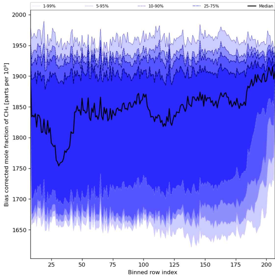
Figure 36: Along track statistics of “Bias corrected mole fraction of CH 4 ” for 2024-01-21 to 2024-01-23
