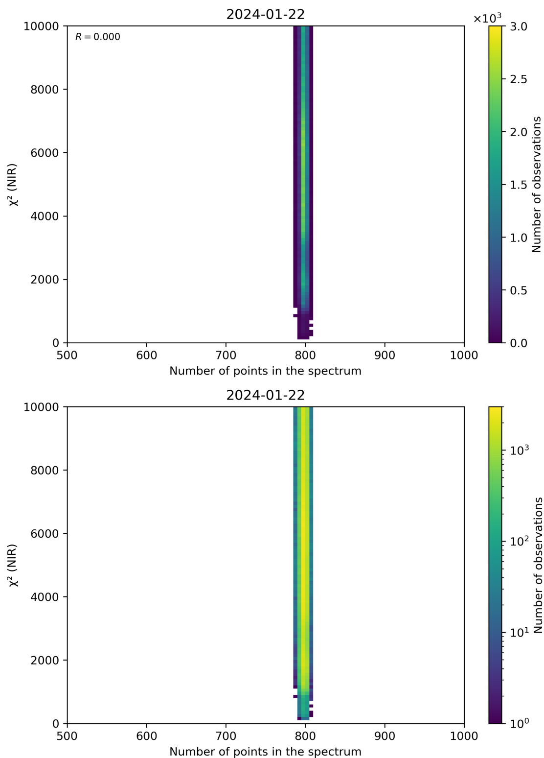
Figure 88: Scatter density plot of “Number of points in the spectrum” against “ \chi^2 (NIR)” for 2024-01-21 to 2024-01-23.
