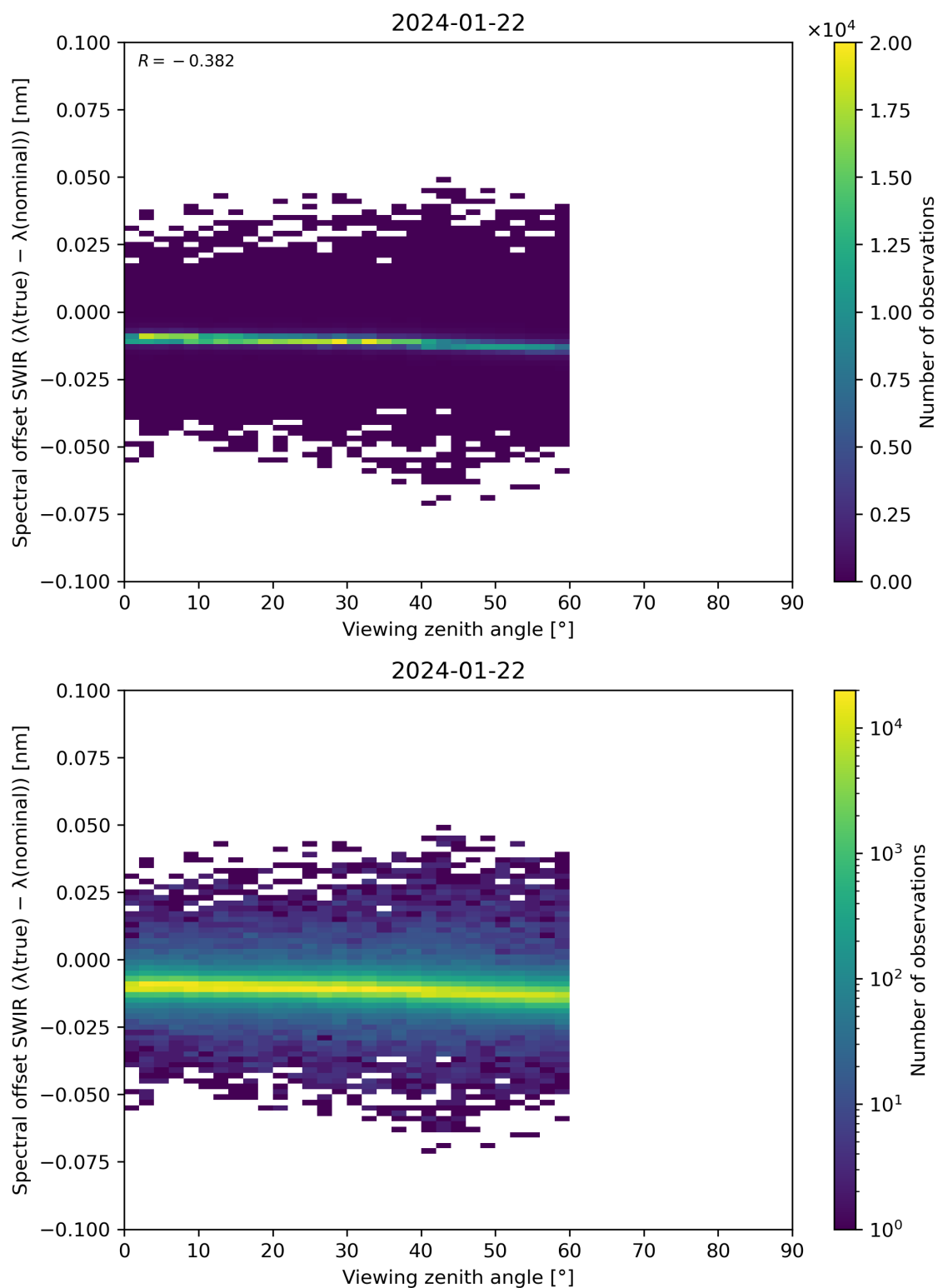
Figure 116: Scatter density plot of “Viewing zenith angle” against “Spectral offset SWIR ( \lambda(\text{true}) - \lambda(\text{nominal}) )” for 2024-01-21 to 2024-01-23.
