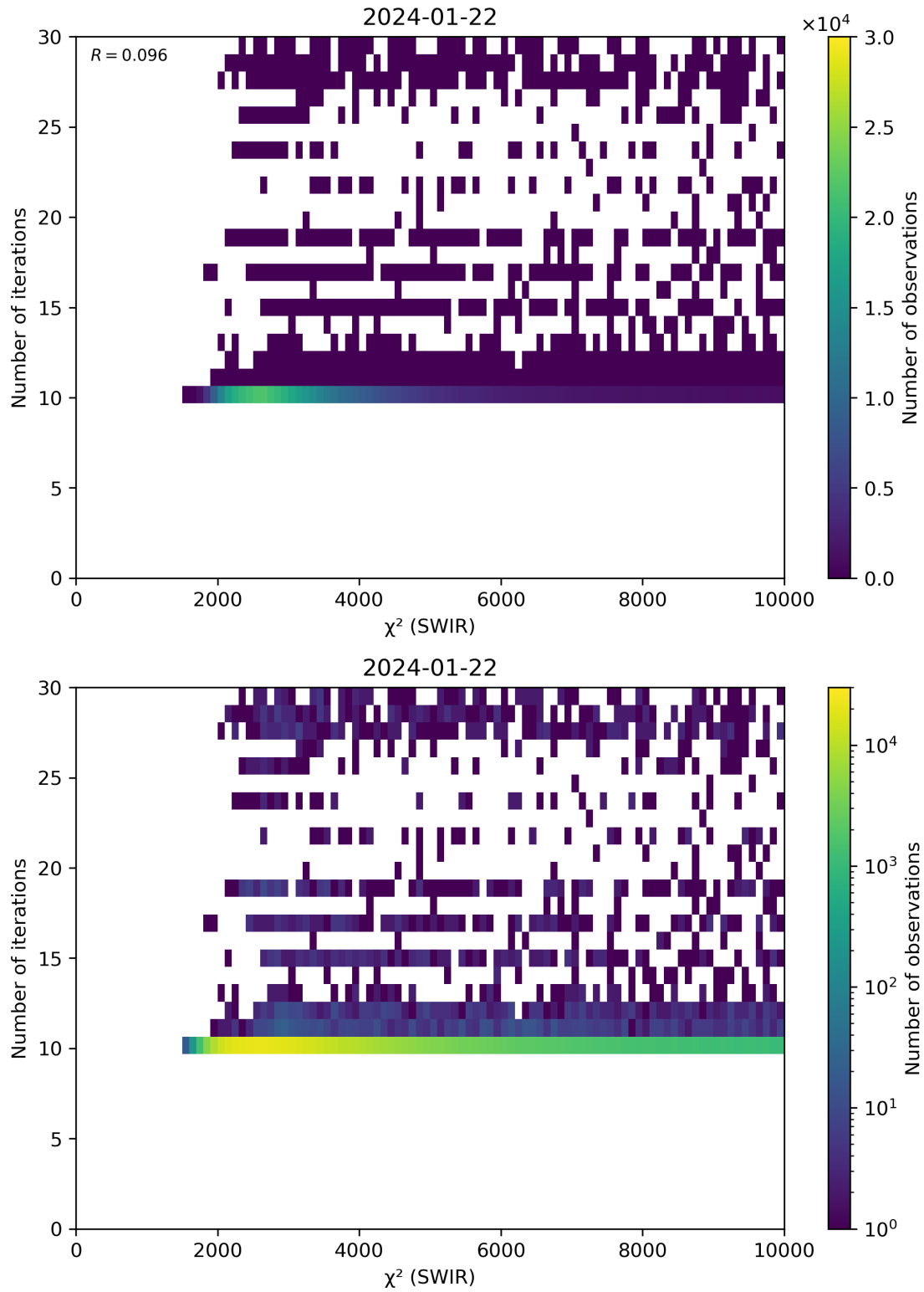
Figure 50: Scatter density plot of “ \chi^2 (SWIR)” against “Number of iterations” for 2024-01-21 to 2024-01-23.
