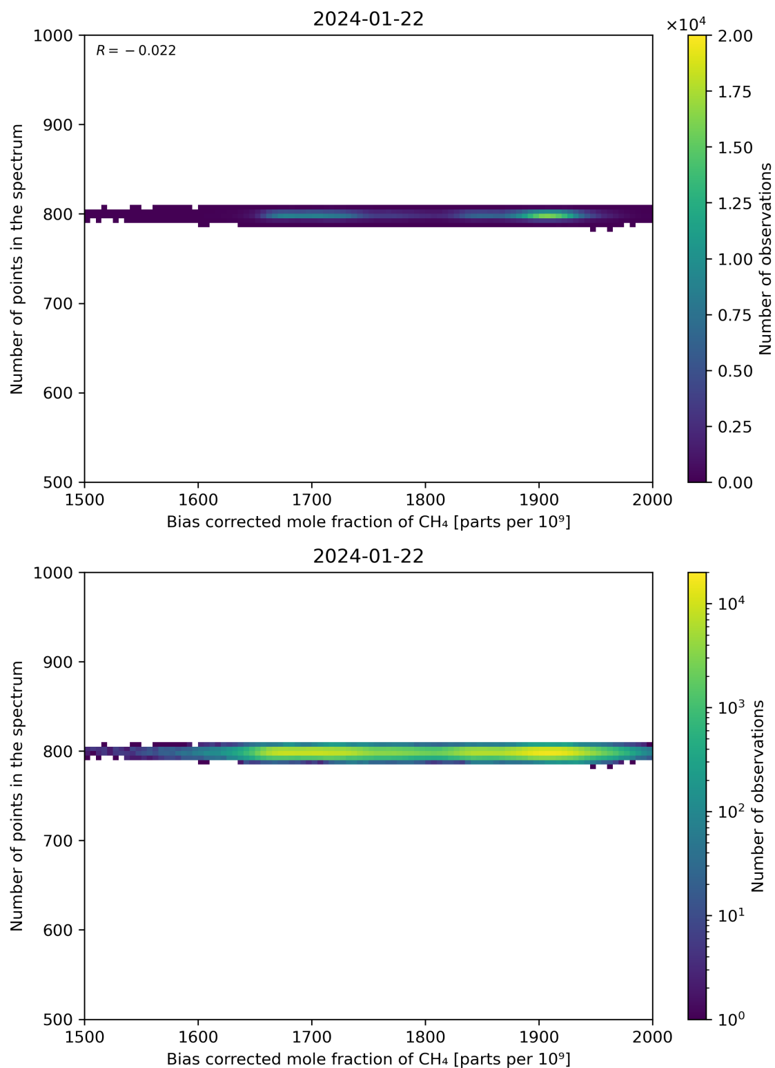
Figure 68: Scatter density plot of “Bias corrected mole fraction of CH 4 ” against “Number of points in the spectrum” for 2024-01-21 to 2024-01-23.
