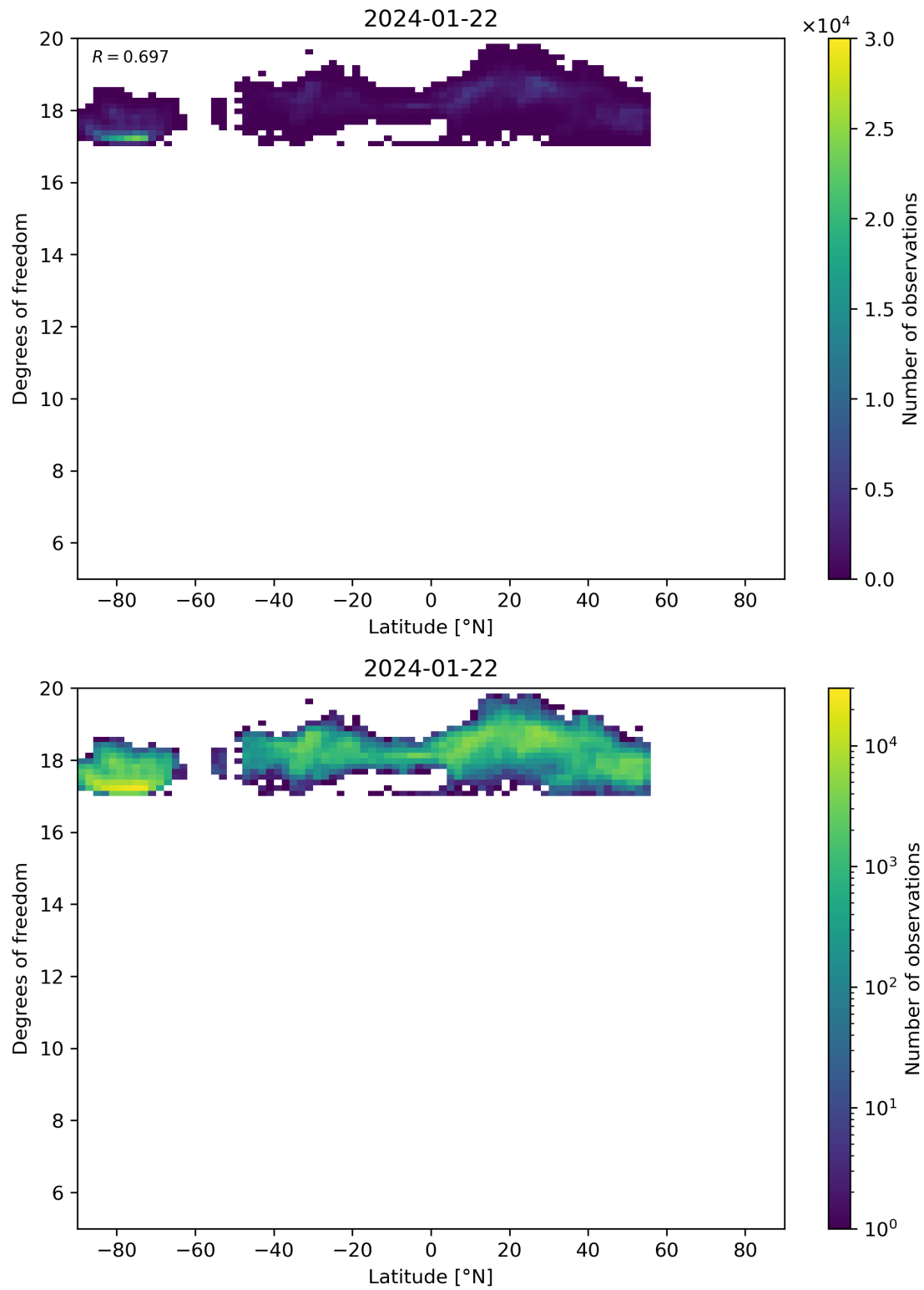
Figure 55: Scatter density plot of “Latitude” against “Degrees of freedom” for 2024-01-21 to 2024-01-23.
