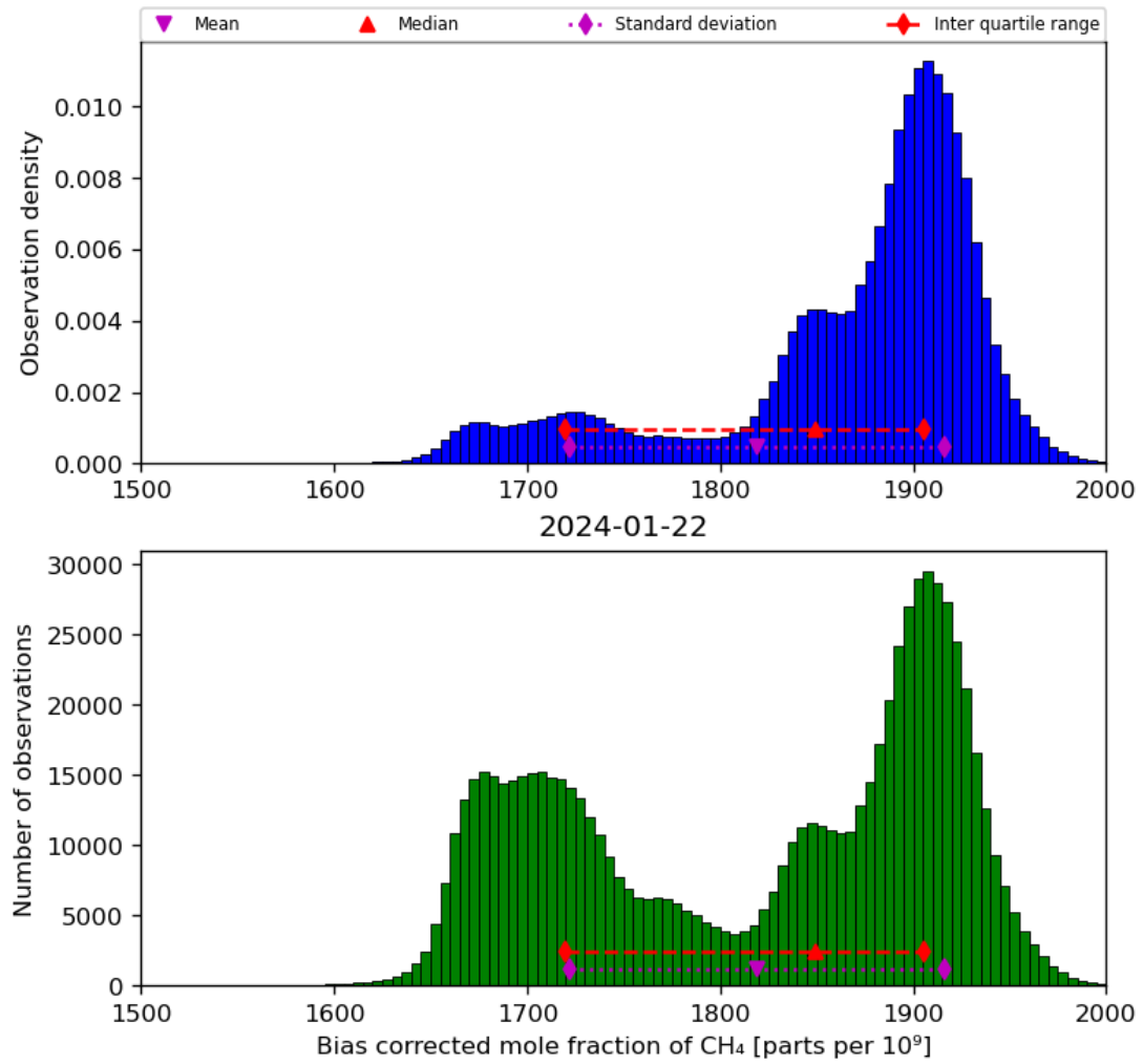
Figure 25: Histogram of “Bias corrected mole fraction of CH 4 ” for 2024-01-21 to 2024-01-23
