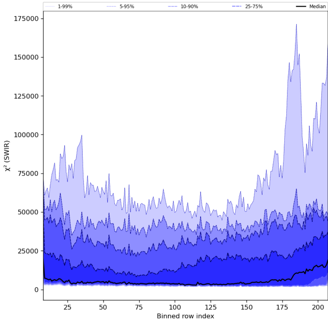
Figure 39: Along track statistics of “ \chi^2 (SWIR)” for 2024-01-21 to 2024-01-23
