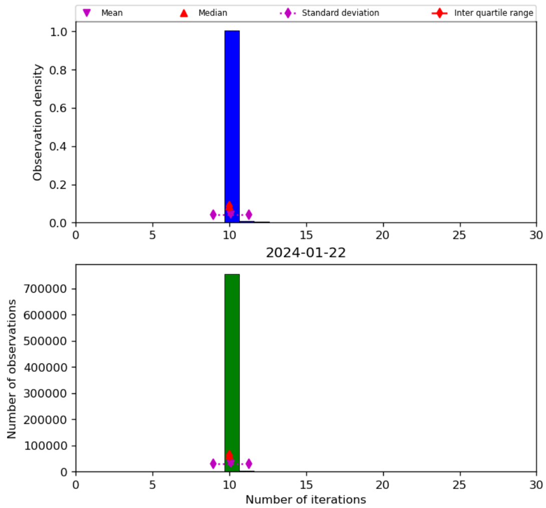
Figure 31: Histogram of “Number of iterations” for 2024-01-21 to 2024-01-23
