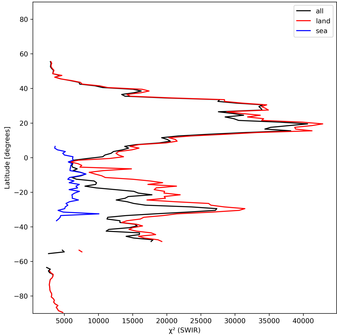
Figure 17: Zonal average of “ \chi^2 (SWIR)” for 2024-01-21 to 2024-01-23.
