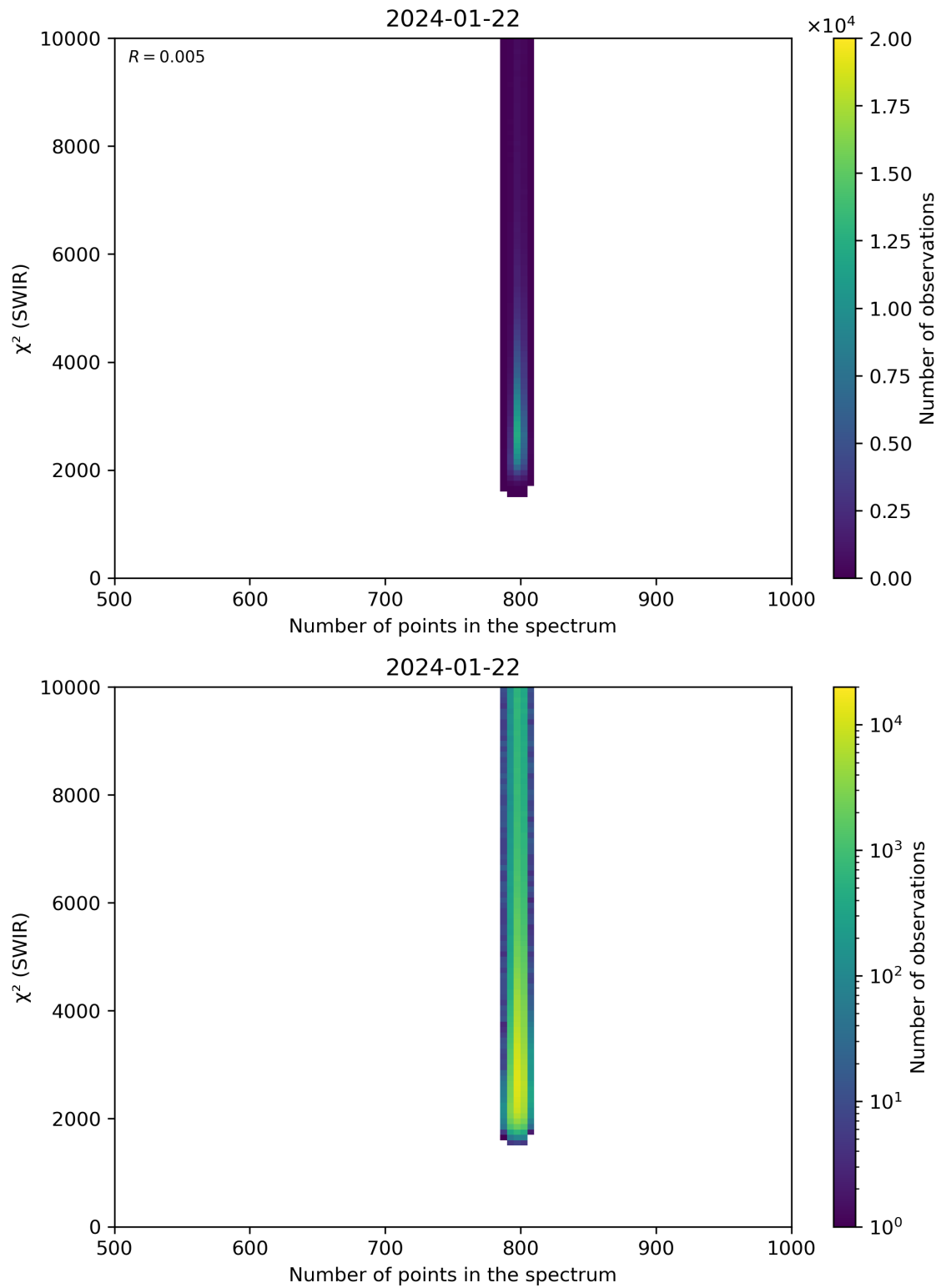
Figure 89: Scatter density plot of “Number of points in the spectrum” against “ \chi^2 (SWIR)” for 2024-01-21 to 2024-01-23.
