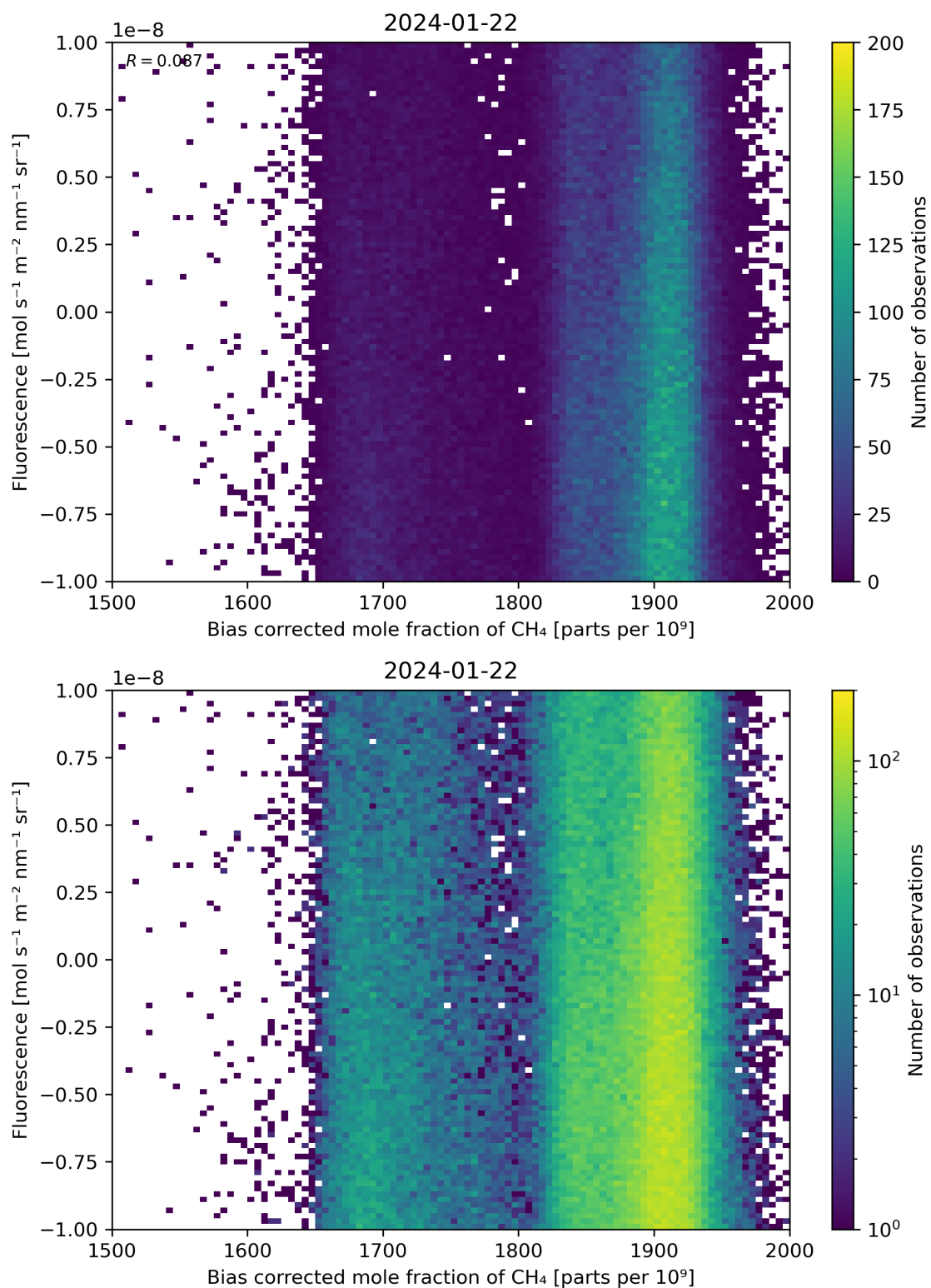
Figure 66: Scatter density plot of “Bias corrected mole fraction of \text{CH}_4 ” against “Fluorescence” for 2024-01-21 to 2024-01-23.
