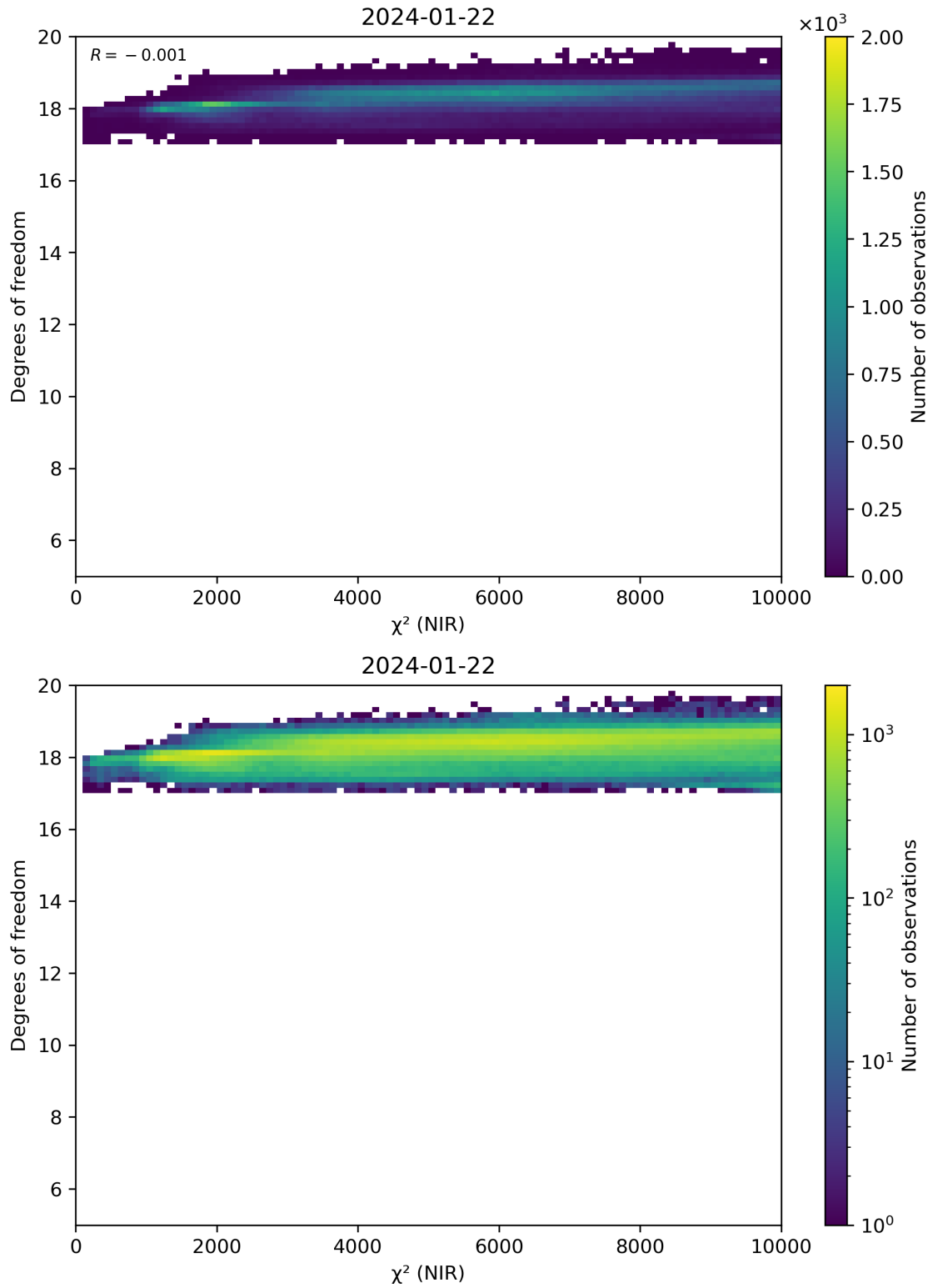
Figure 44: Scatter density plot of “ \chi^2 (NIR)” against “Degrees of freedom” for 2024-01-21 to 2024-01-23.
