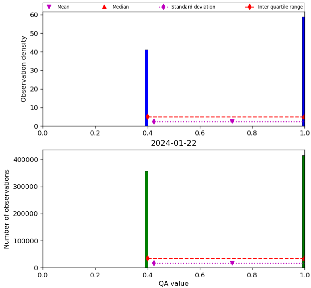
Figure 22: Histogram of “QA value” for 2024-01-21 to 2024-01-23
