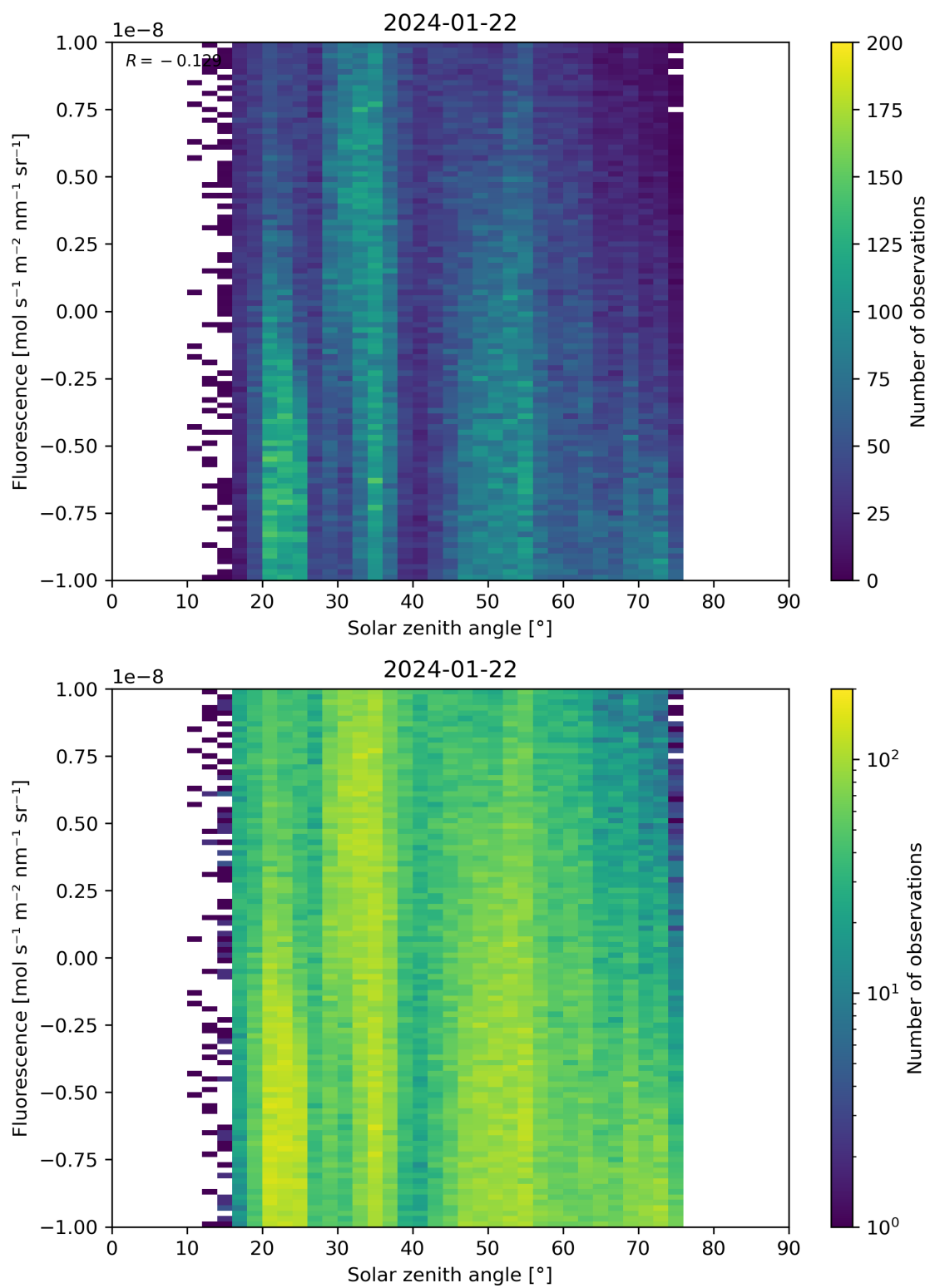
Figure 97: Scatter density plot of “Solar zenith angle” against “Fluorescence” for 2024-01-21 to 2024-01-23.
