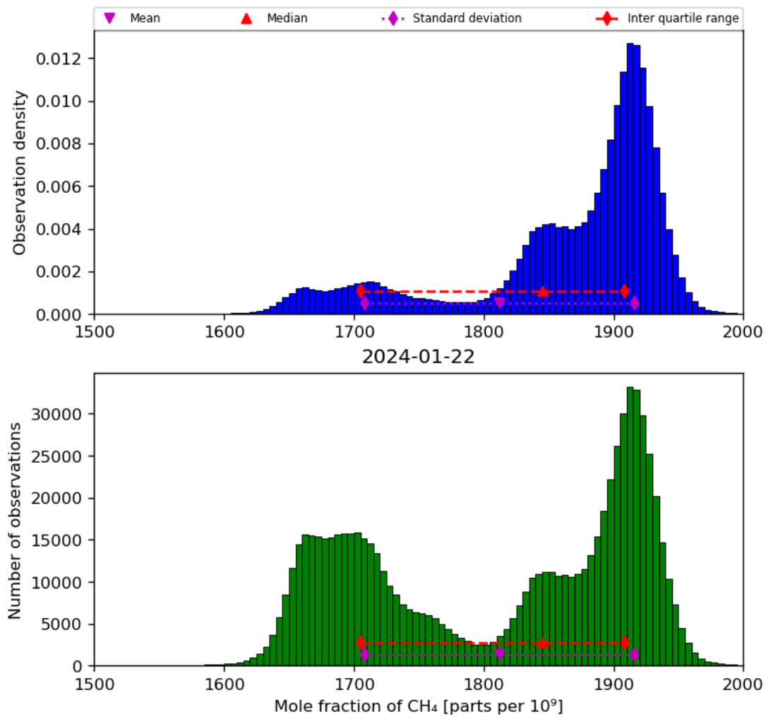
Figure 23: Histogram of “Mole fraction of CH 4 ” for 2024-01-21 to 2024-01-23
