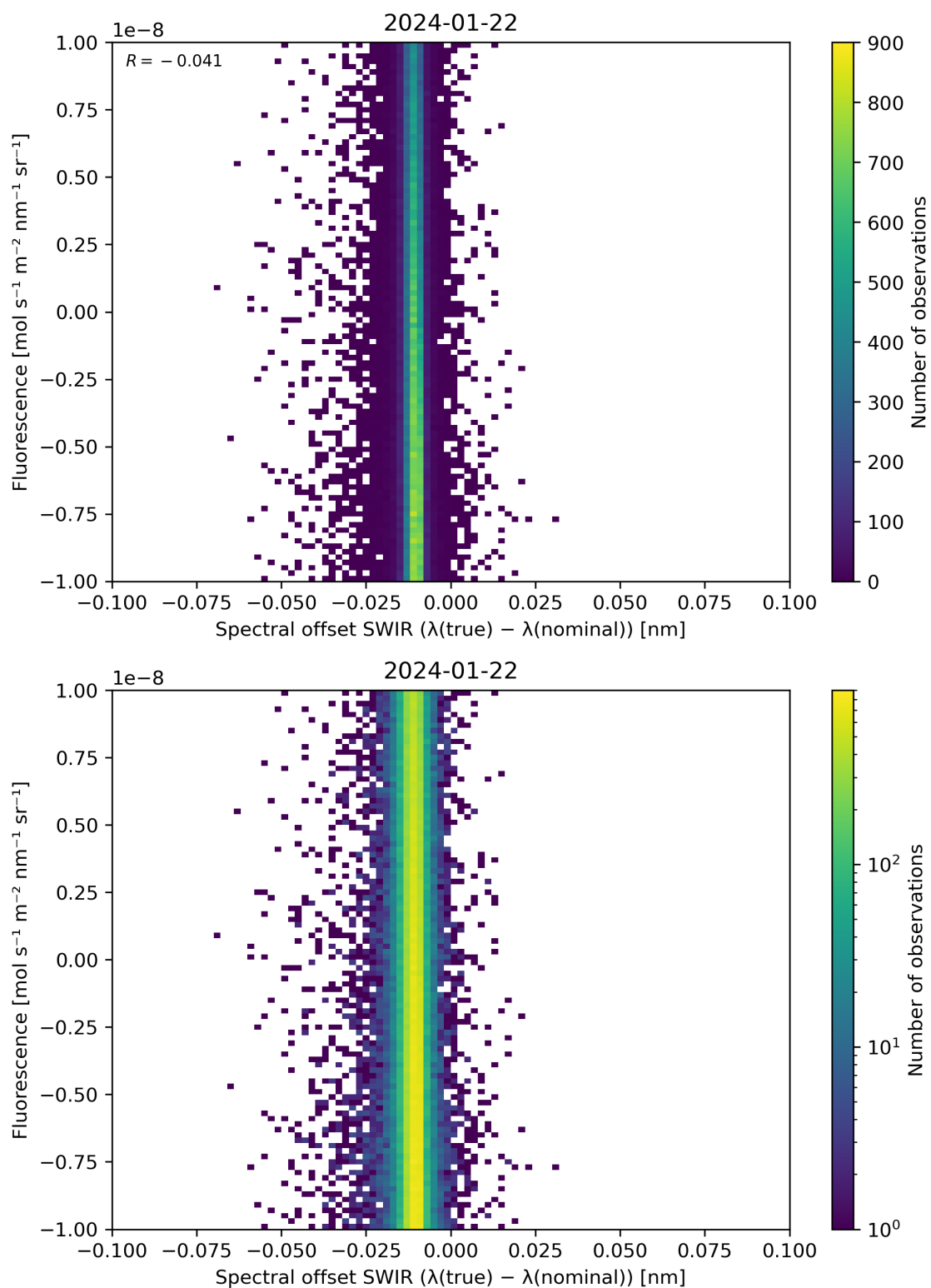
Figure 120: Scatter density plot of “Spectral offset SWIR ( \lambda(\text{true}) - \lambda(\text{nominal}) )” against “Fluorescence” for 2024-01-21 to 2024-01-23.
