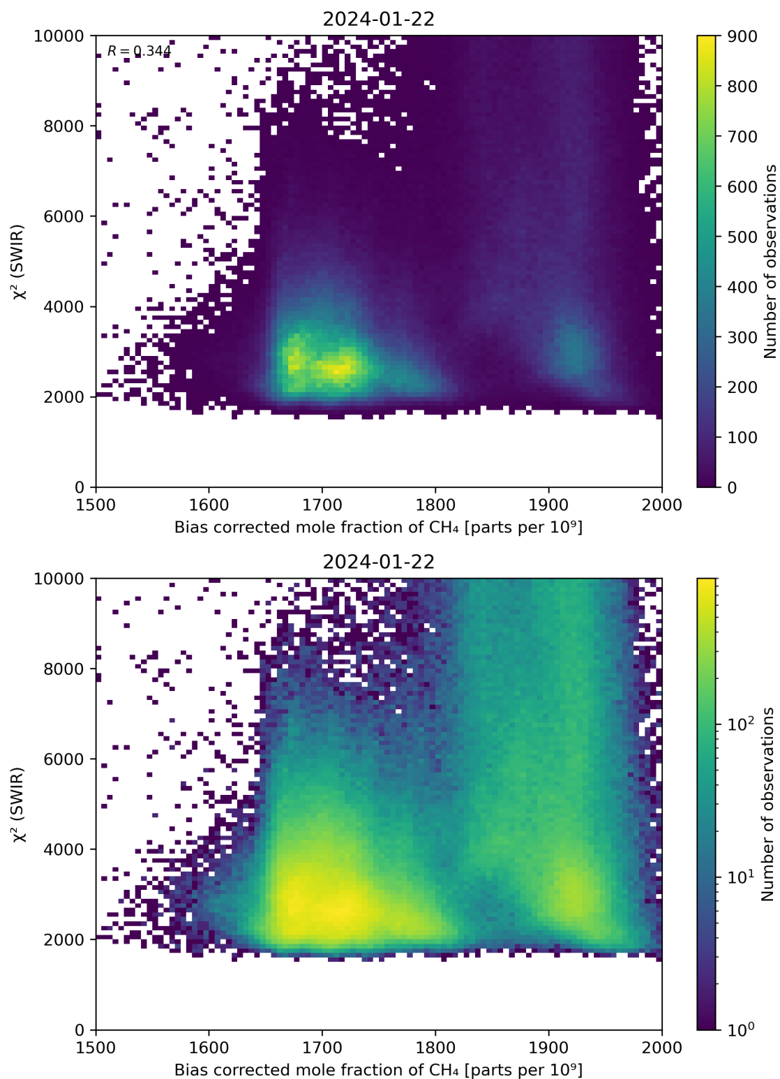
Figure 64: Scatter density plot of “Bias corrected mole fraction of CH 4 ” against “ \chi^2 (SWIR)” for 2024-01-21 to 2024-01-23.
