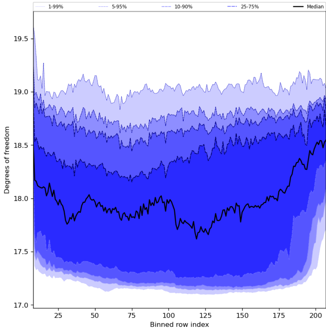
Figure 41: Along track statistics of “Degrees of freedom” for 2024-01-21 to 2024-01-23
