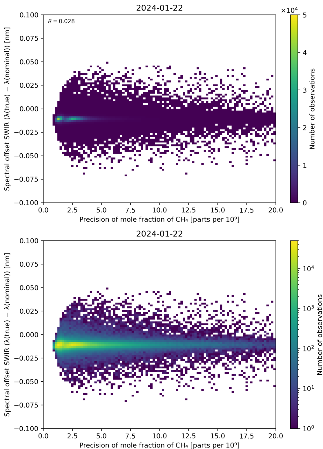
Figure 85: Scatter density plot of “Precision of mole fraction of CH 4 ” against “Spectral offset SWIR ( \lambda(\text{true}) - \lambda(\text{nominal}) )” for 2024-01-21 to 2024-01-23.
