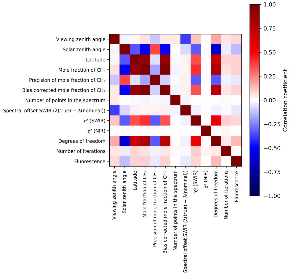
Figure 2: Map of correlation matrix for 2024-01-21 to 2024-01-23.
