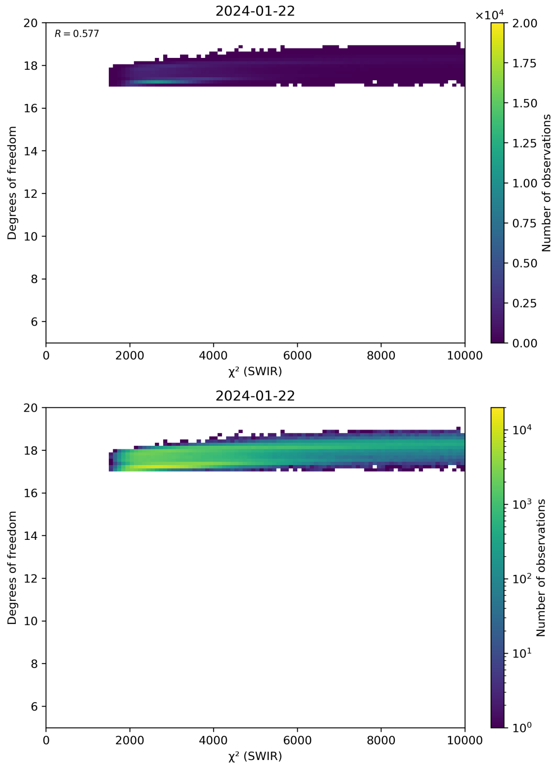
Figure 48: Scatter density plot of “ \chi^2 (SWIR)” against “Degrees of freedom” for 2024-01-21 to 2024-01-23.
