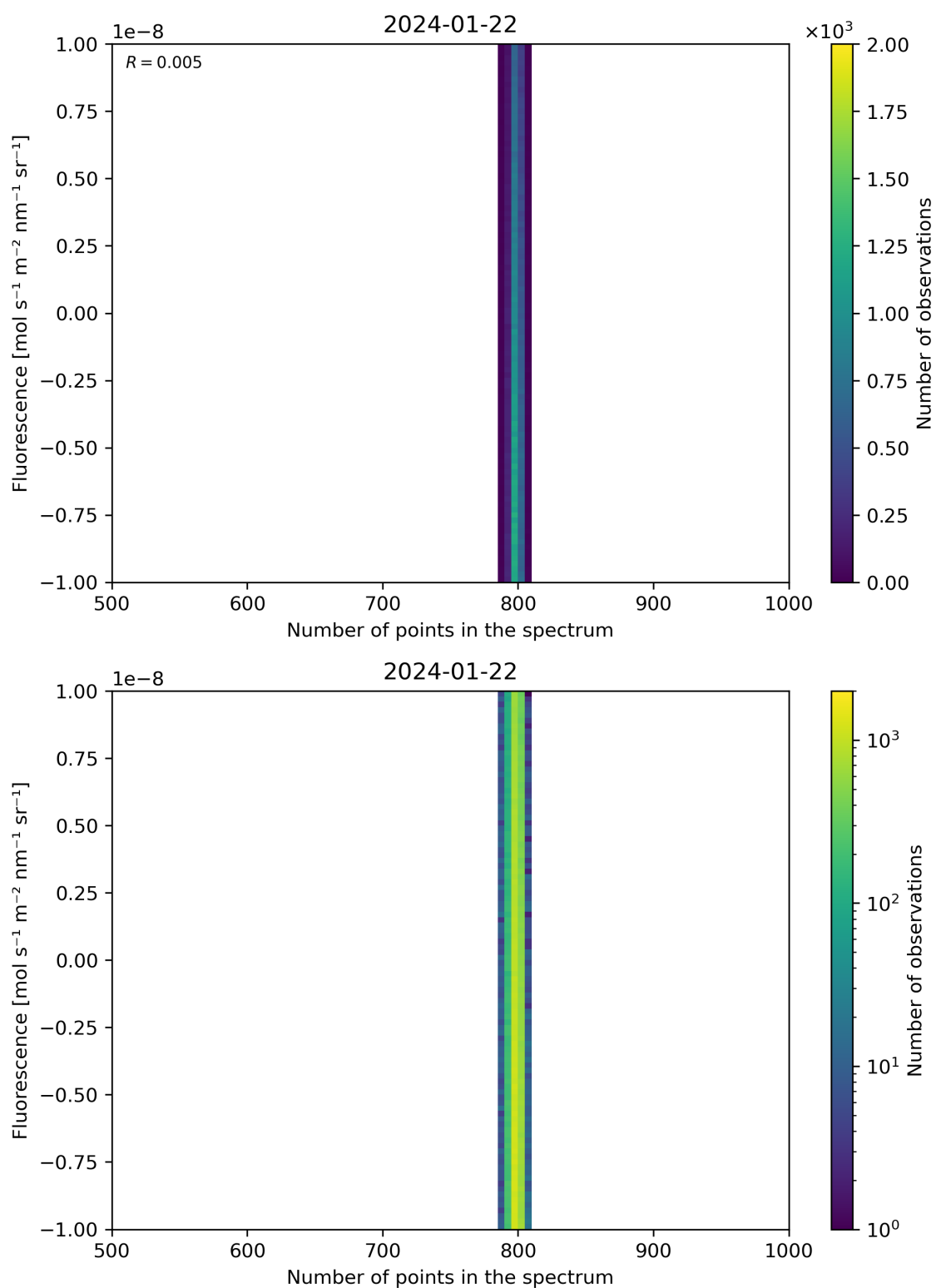
Figure 91: Scatter density plot of “Number of points in the spectrum” against “Fluorescence” for 2024-01-21 to 2024-01-23.
