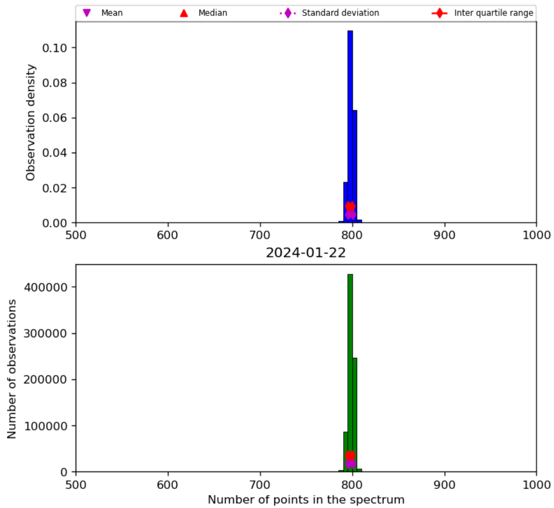
Figure 26: Histogram of “Number of points in the spectrum” for 2024-01-21 to 2024-01-23
