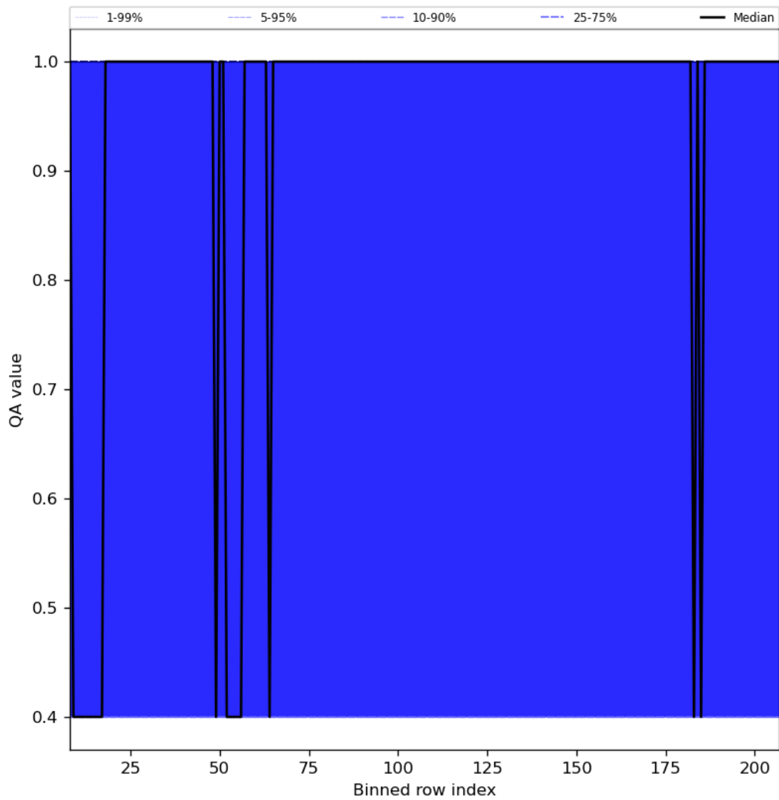
Figure 33: Along track statistics of “QA value” for 2024-01-21 to 2024-01-23
