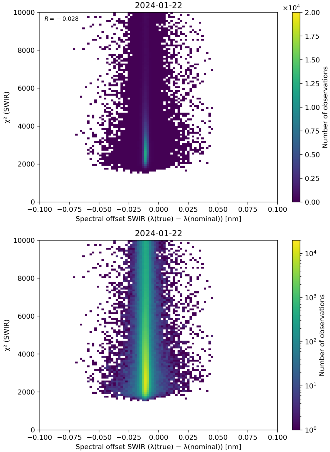
Figure 118: Scatter density plot of “Spectral offset SWIR ( \lambda(\text{true}) - \lambda(\text{nominal}) )” against “ \chi^2 (SWIR)” for 2024-01-21 to 2024-01-23.
