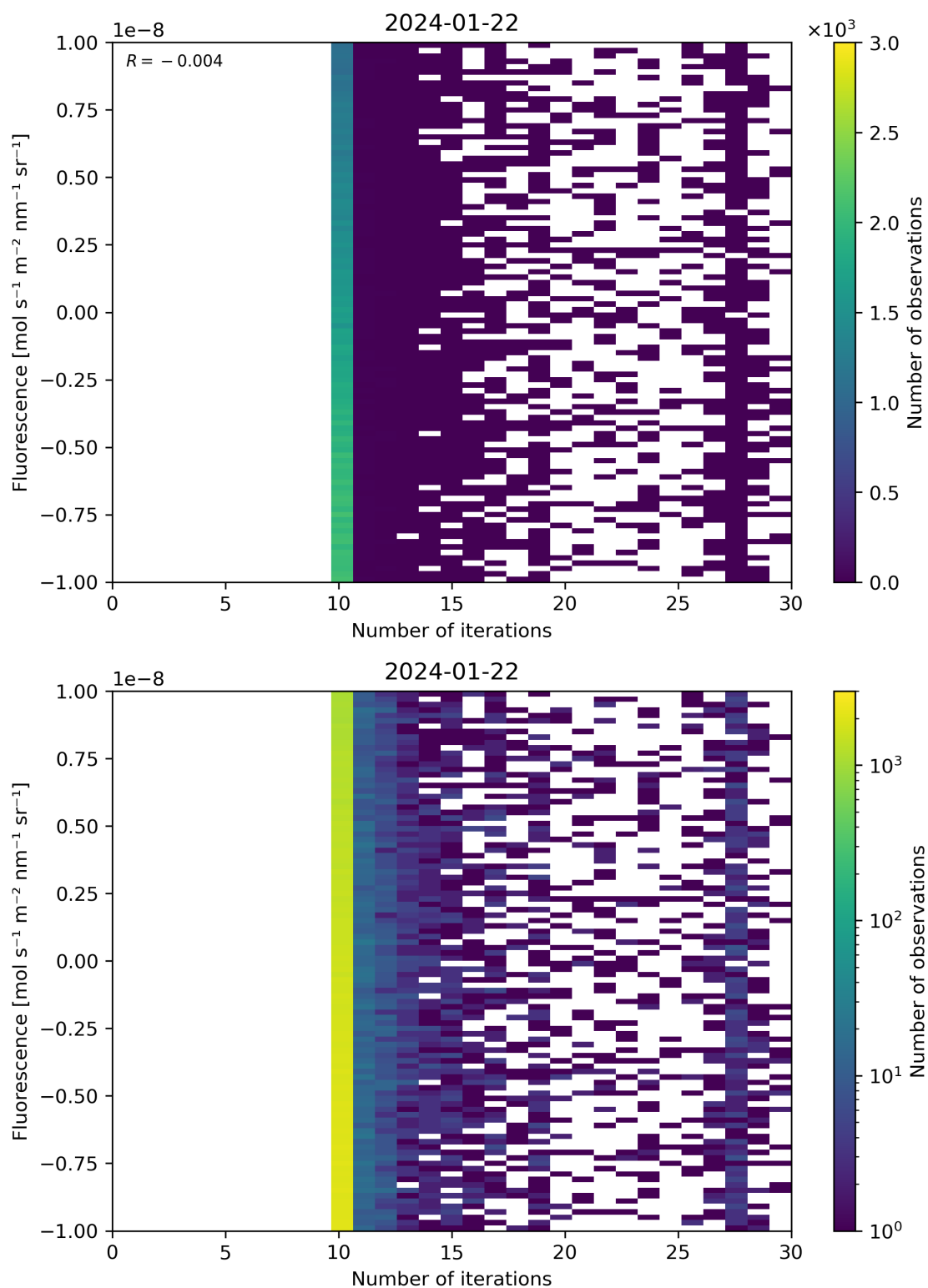
Figure 87: Scatter density plot of “Number of iterations” against “Fluorescence” for 2024-01-21 to 2024-01-23.
