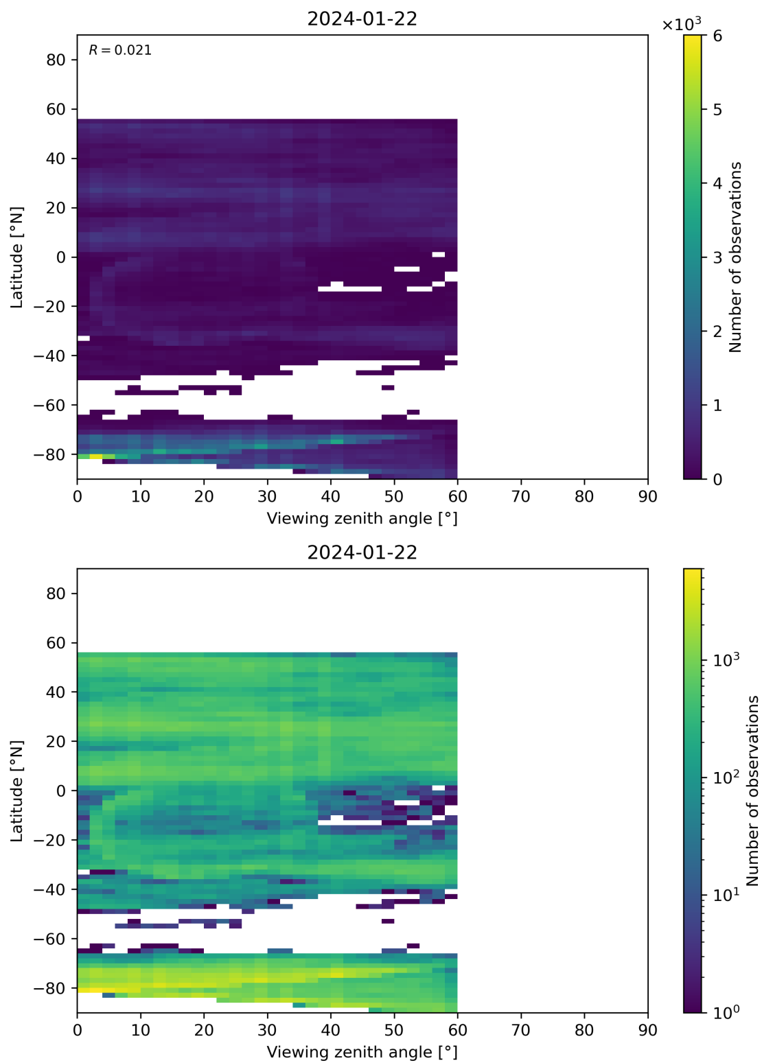
Figure 109: Scatter density plot of “Viewing zenith angle” against “Latitude” for 2024-01-21 to 2024-01-23.
