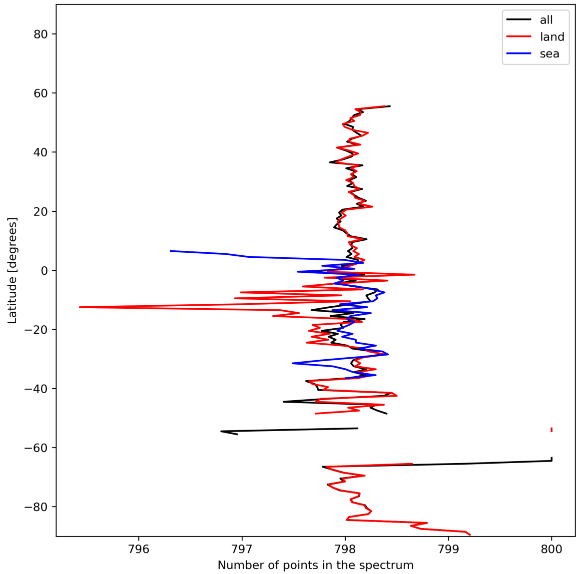
Figure 15: Zonal average of “Number of points in the spectrum” for 2024-01-21 to 2024-01-23.
