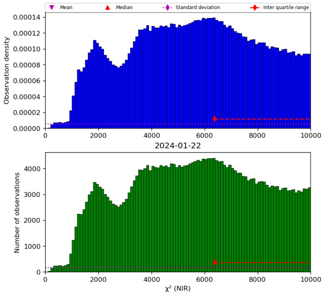
Figure 29: Histogram of “ \chi^2 (NIR)” for 2024-01-21 to 2024-01-23
