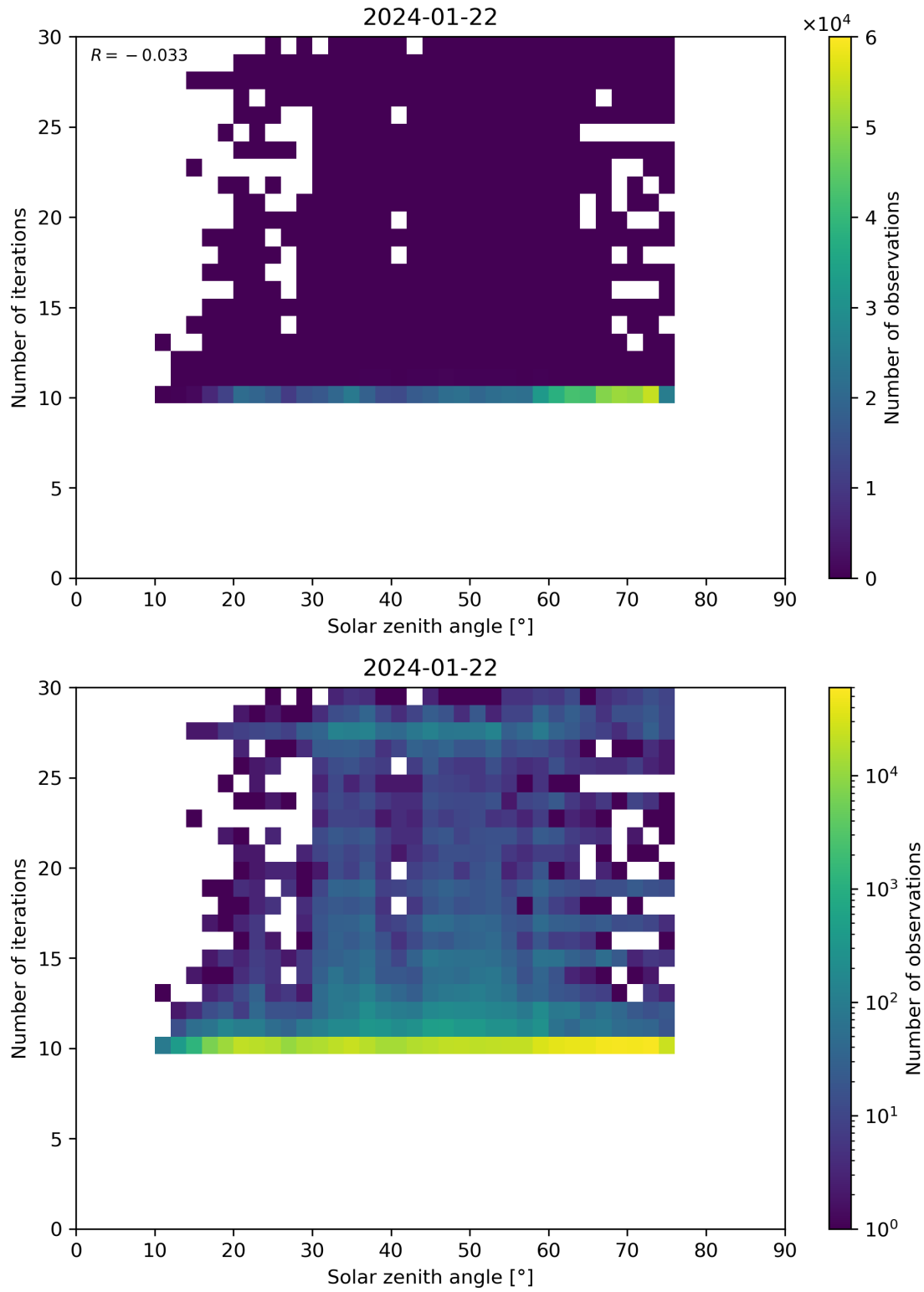
Figure 102: Scatter density plot of “Solar zenith angle” against “Number of iterations” for 2024-01-21 to 2024-01-23.
