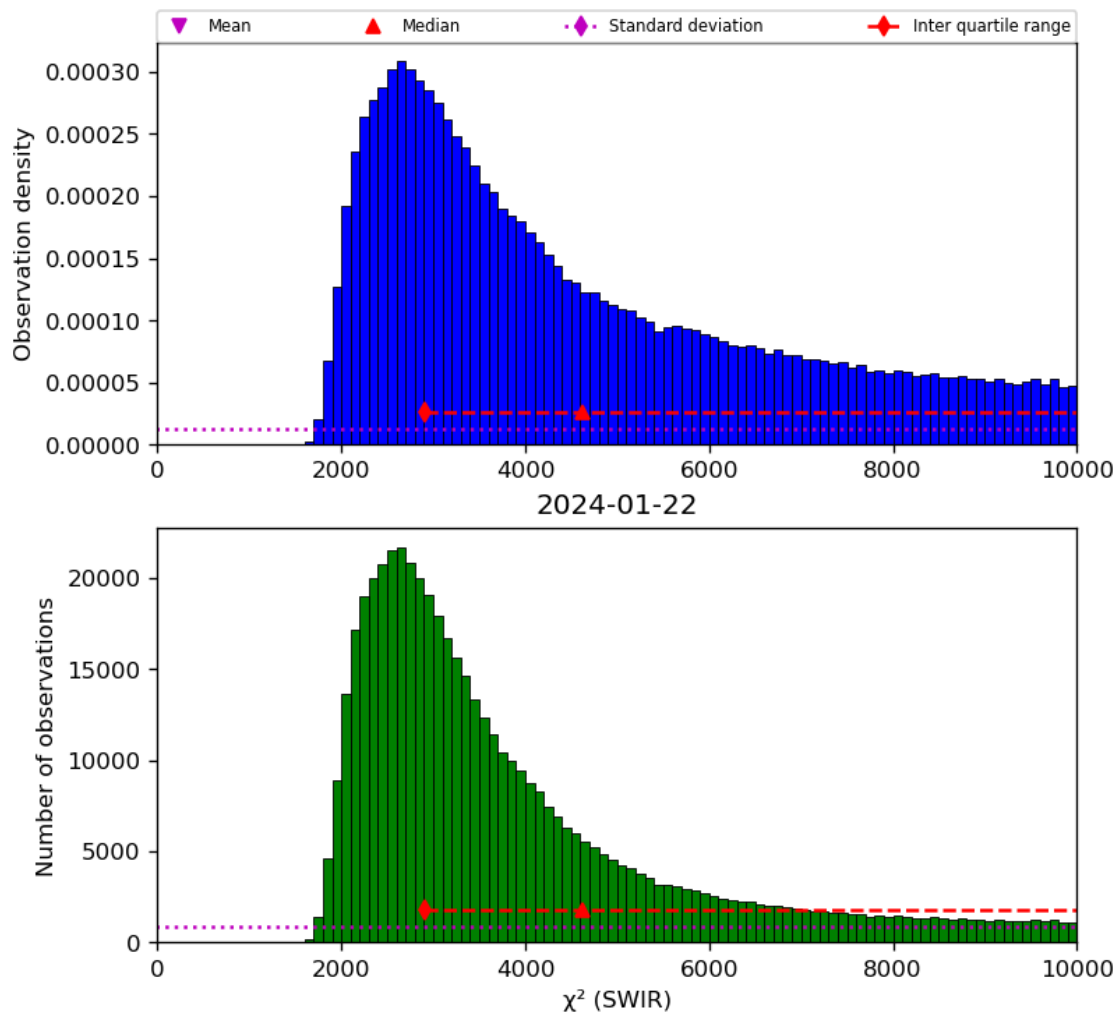
Figure 28: Histogram of “ \chi^2 (SWIR)” for 2024-01-21 to 2024-01-23
