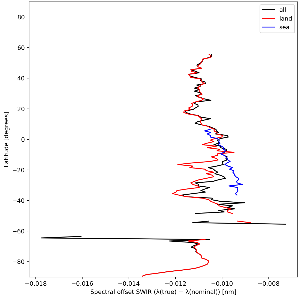
Figure 16: Zonal average of “Spectral offset SWIR ( \lambda(\text{true}) - \lambda(\text{nominal}) )” for 2024-01-21 to 2024-01-23.
