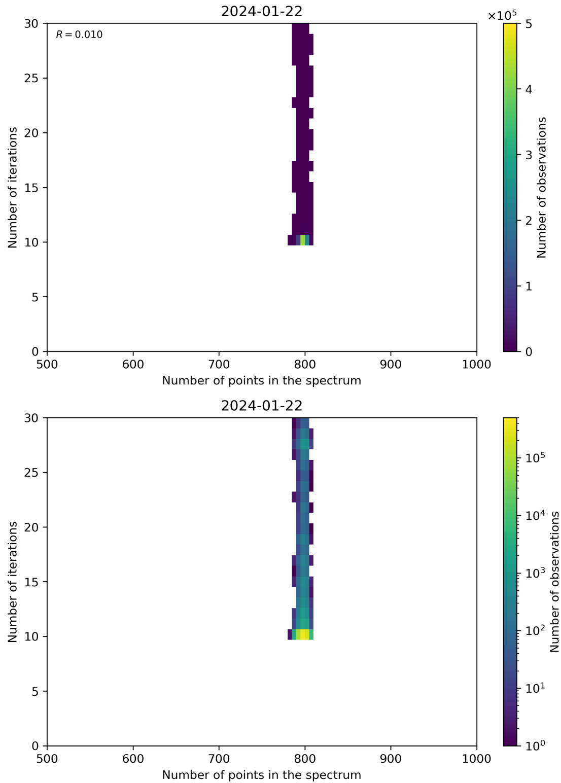
Figure 92: Scatter density plot of “Number of points in the spectrum” against “Number of iterations” for 2024-01-21 to 2024-01-23.
