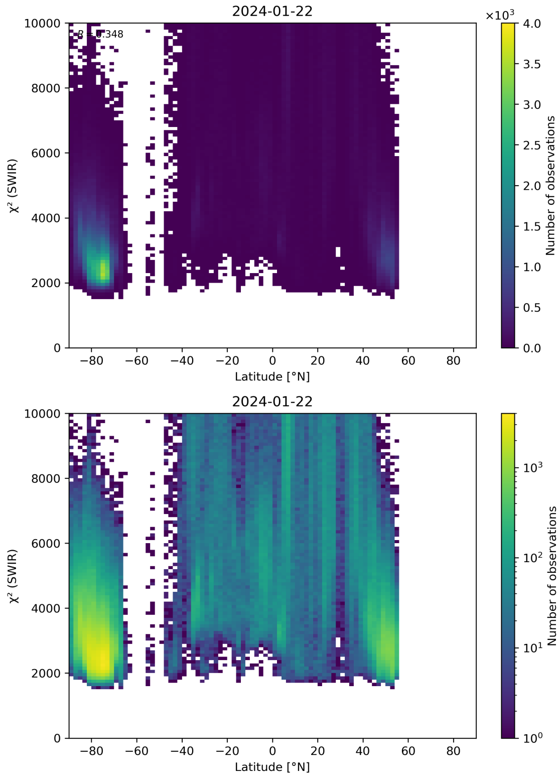
Figure 54: Scatter density plot of “Latitude” against “ \chi^2 (SWIR)” for 2024-01-21 to 2024-01-23.
