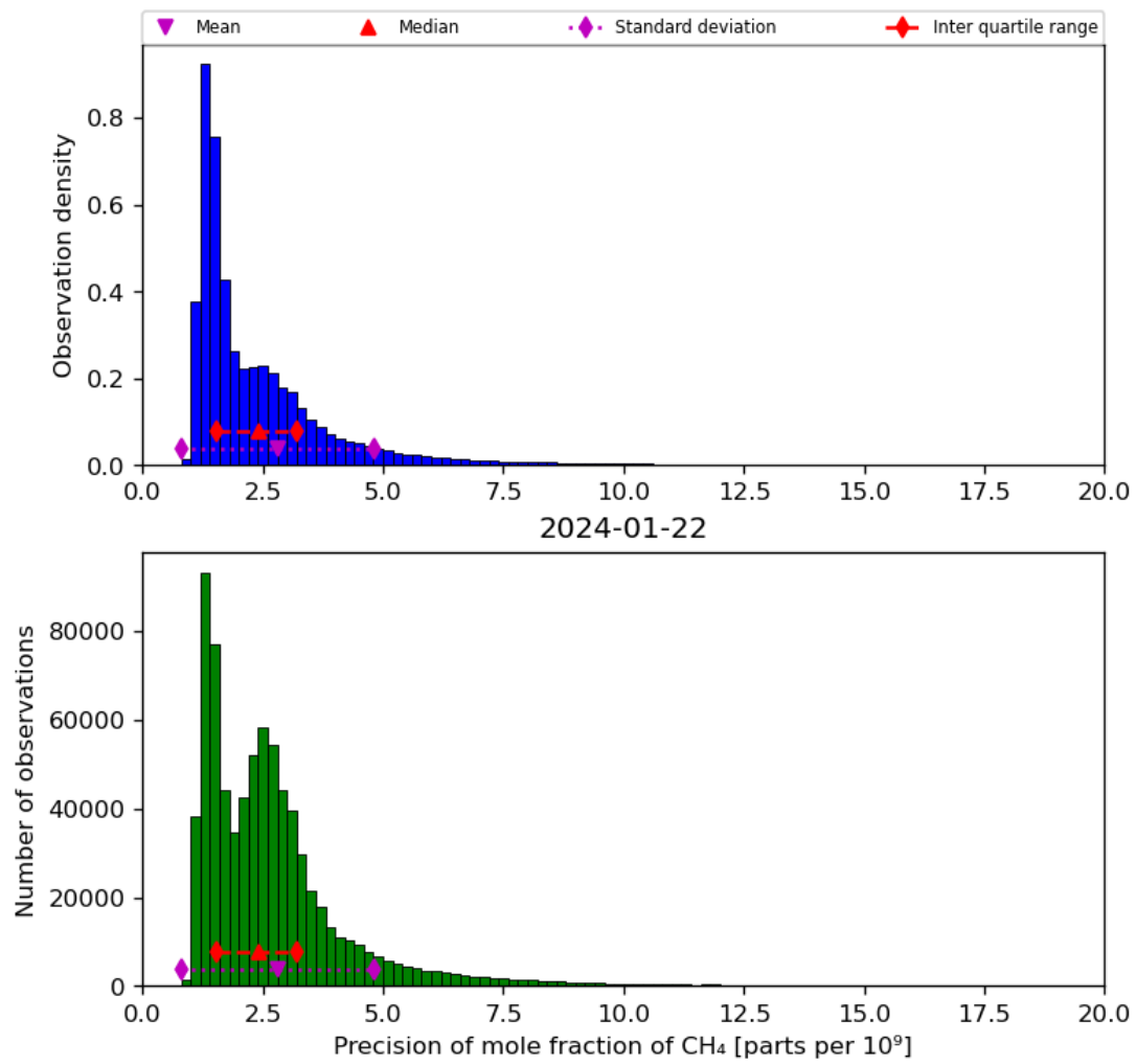
Figure 24: Histogram of “Precision of mole fraction of CH 4 ” for 2024-01-21 to 2024-01-23
