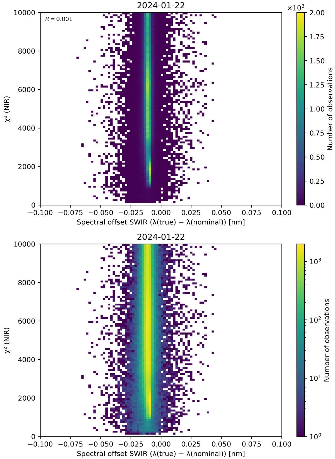
Figure 117: Scatter density plot of “Spectral offset SWIR ( \lambda(\text{true}) - \lambda(\text{nominal}) )” against “ \chi^2 (NIR)” for 2024-01-21 to 2024-01-23.
