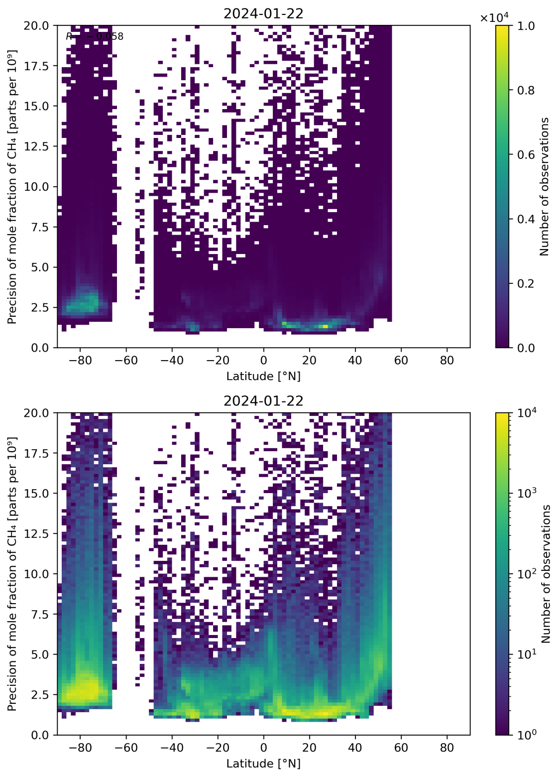
Figure 59: Scatter density plot of “Latitude” against “Precision of mole fraction of CH 4 ” for 2024-01-21 to 2024-01-23.
