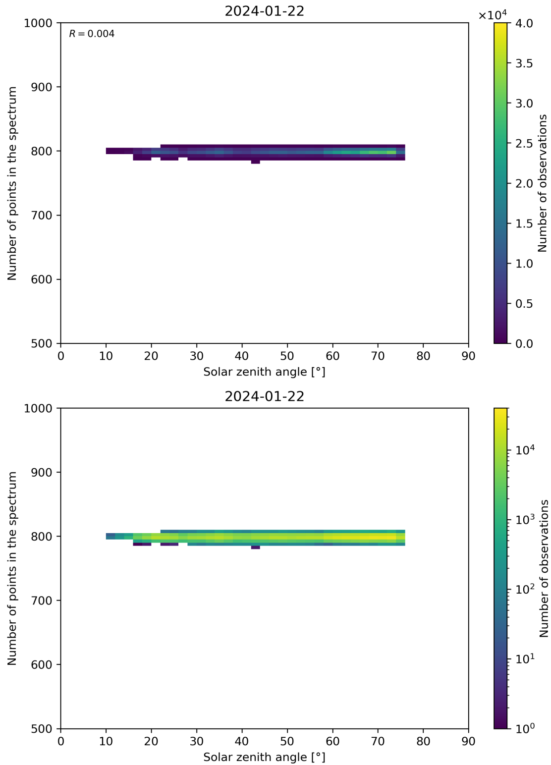
Figure 103: Scatter density plot of “Solar zenith angle” against “Number of points in the spectrum” for 2024-01-21 to 2024-01-23.
