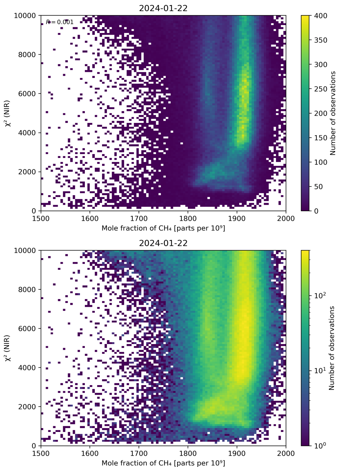
Figure 70: Scatter density plot of “Mole fraction of \text{CH}_4 ” against “ \chi^2 (NIR)” for 2024-01-21 to 2024-01-23.
