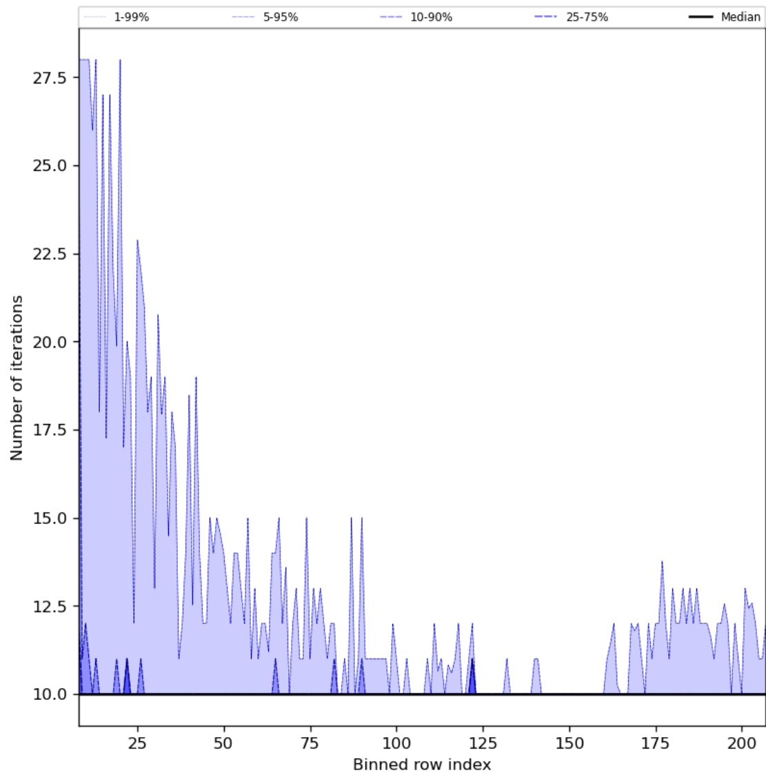
Figure 42: Along track statistics of “Number of iterations” for 2024-01-21 to 2024-01-23
