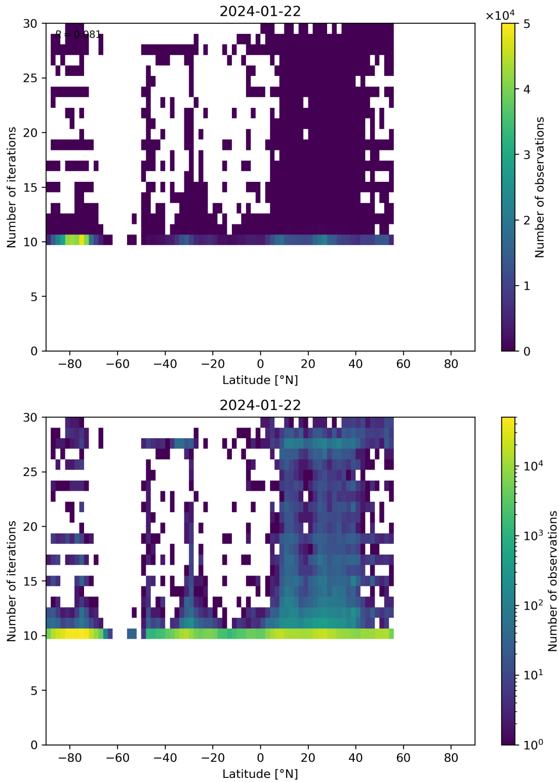
Figure 60: Scatter density plot of “Latitude” against “Number of iterations” for 2024-01-21 to 2024-01-23.
