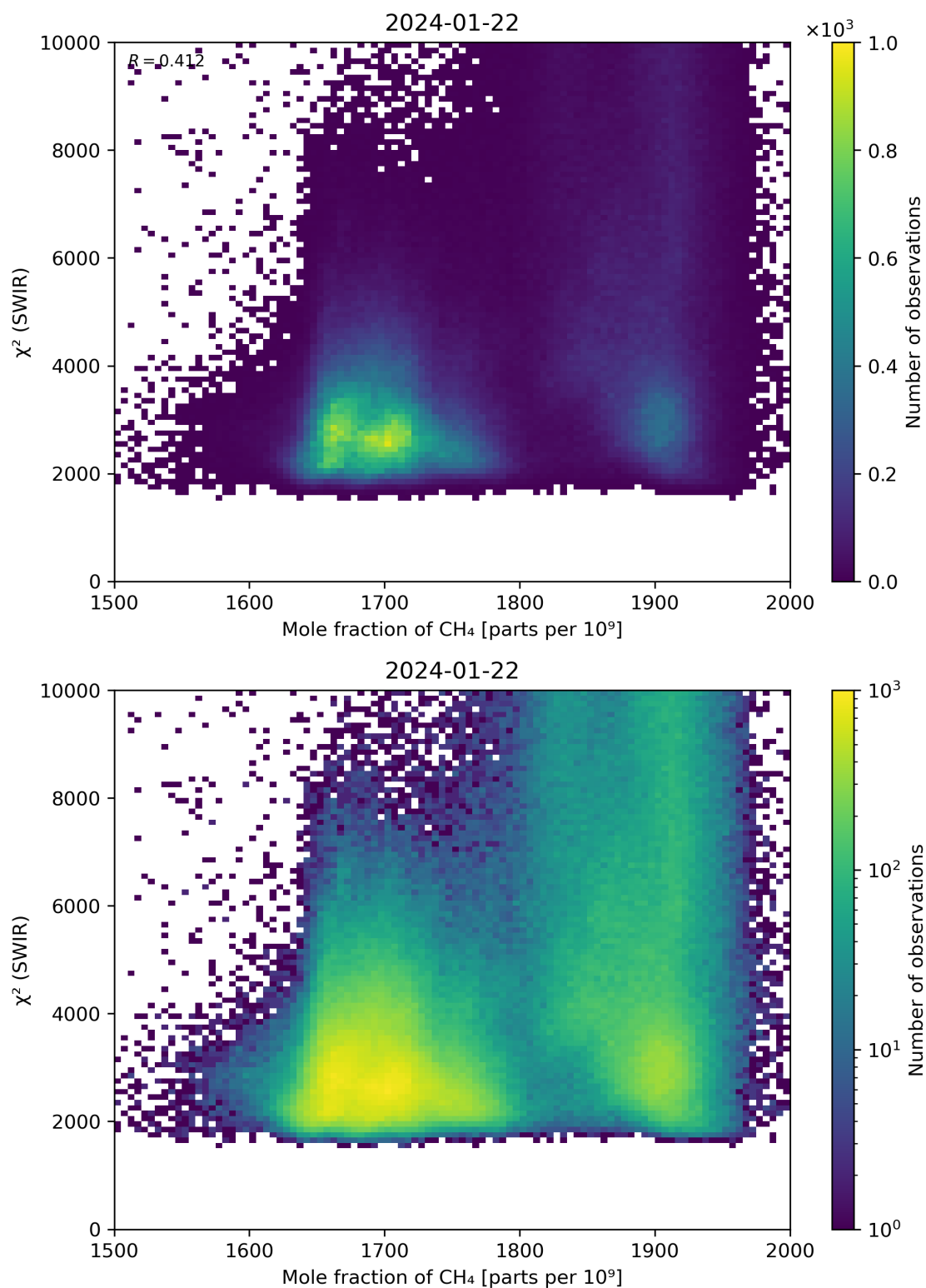
Figure 71: Scatter density plot of “Mole fraction of \text{CH}_4 ” against “ \chi^2 (SWIR)” for 2024-01-21 to 2024-01-23.
