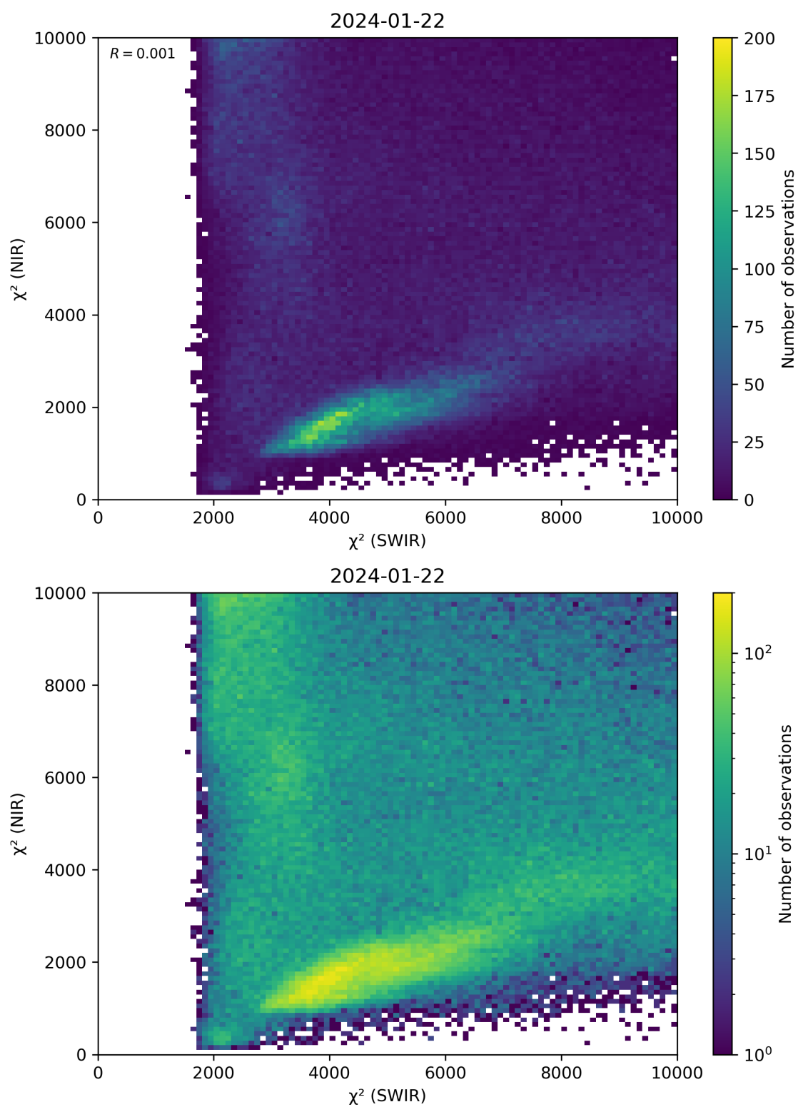
Figure 47: Scatter density plot of “ \chi^2 (SWIR)” against “ \chi^2 (NIR)” for 2024-01-21 to 2024-01-23.
