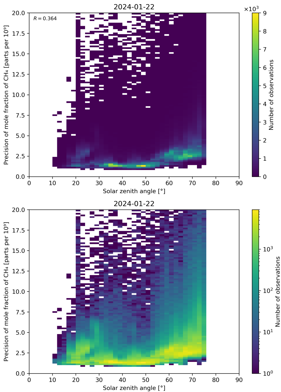
Figure 101: Scatter density plot of “Solar zenith angle” against “Precision of mole fraction of CH 4 ” for 2024-01-21 to 2024-01-23.
