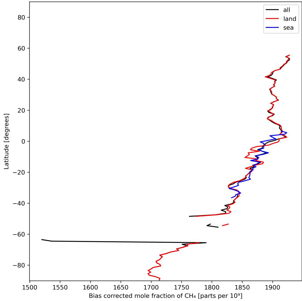
Figure 14: Zonal average of “Bias corrected mole fraction of CH 4 ” for 2024-01-21 to 2024-01-23.
