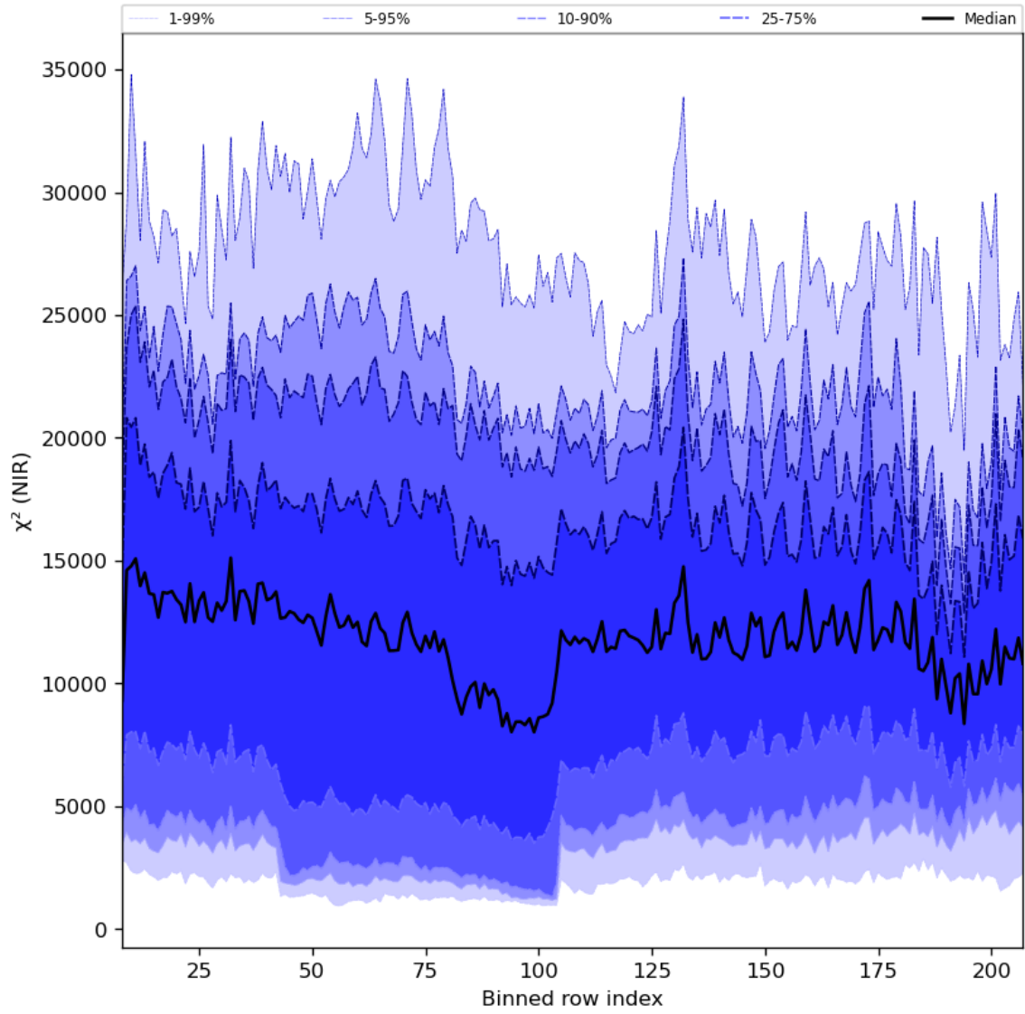
Figure 40: Along track statistics of “ \chi^2 (NIR)” for 2024-01-21 to 2024-01-23
