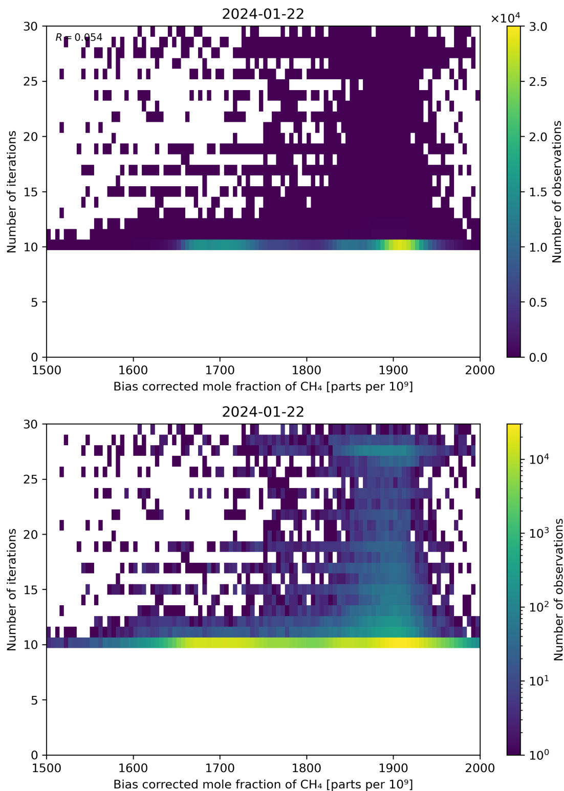
Figure 67: Scatter density plot of “Bias corrected mole fraction of \text{CH}_4 ” against “Number of iterations” for 2024-01-21 to 2024-01-23.
