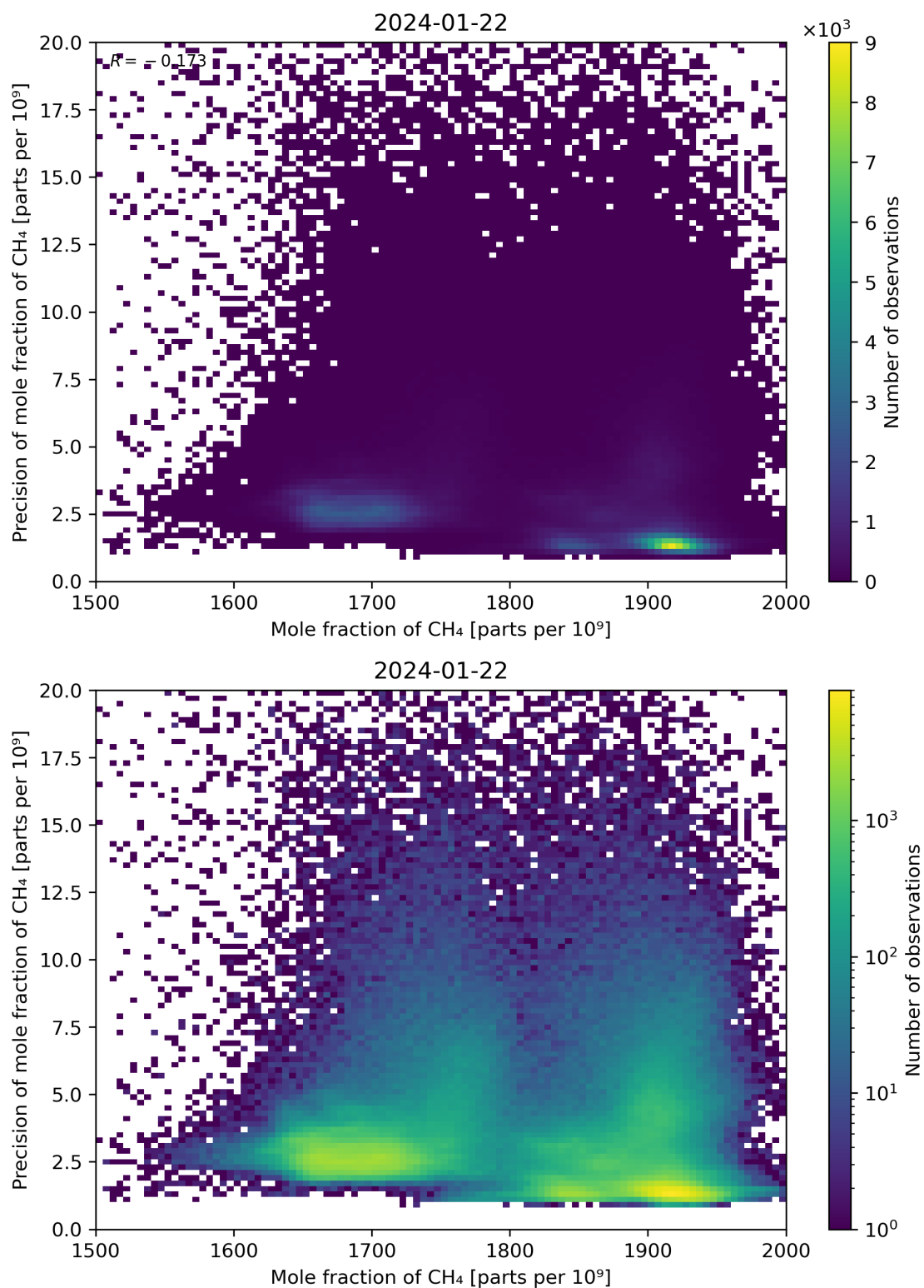
Figure 75: Scatter density plot of “Mole fraction of CH 4 ” against “Precision of mole fraction of CH 4 ” for 2024-01-21 to 2024-01-23.
