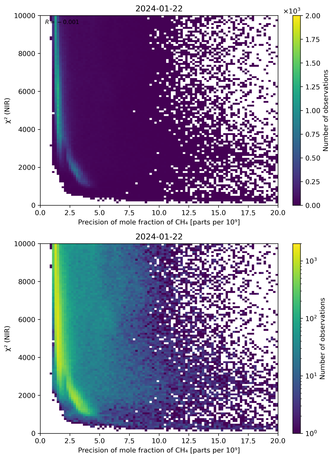
Figure 78: Scatter density plot of “Precision of mole fraction of CH 4 ” against “ \chi^2 (NIR)” for 2024-01-21 to 2024-01-23.
