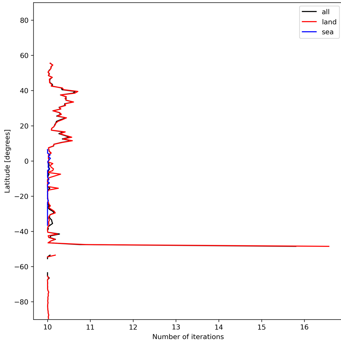
Figure 20: Zonal average of “Number of iterations” for 2024-01-21 to 2024-01-23.
