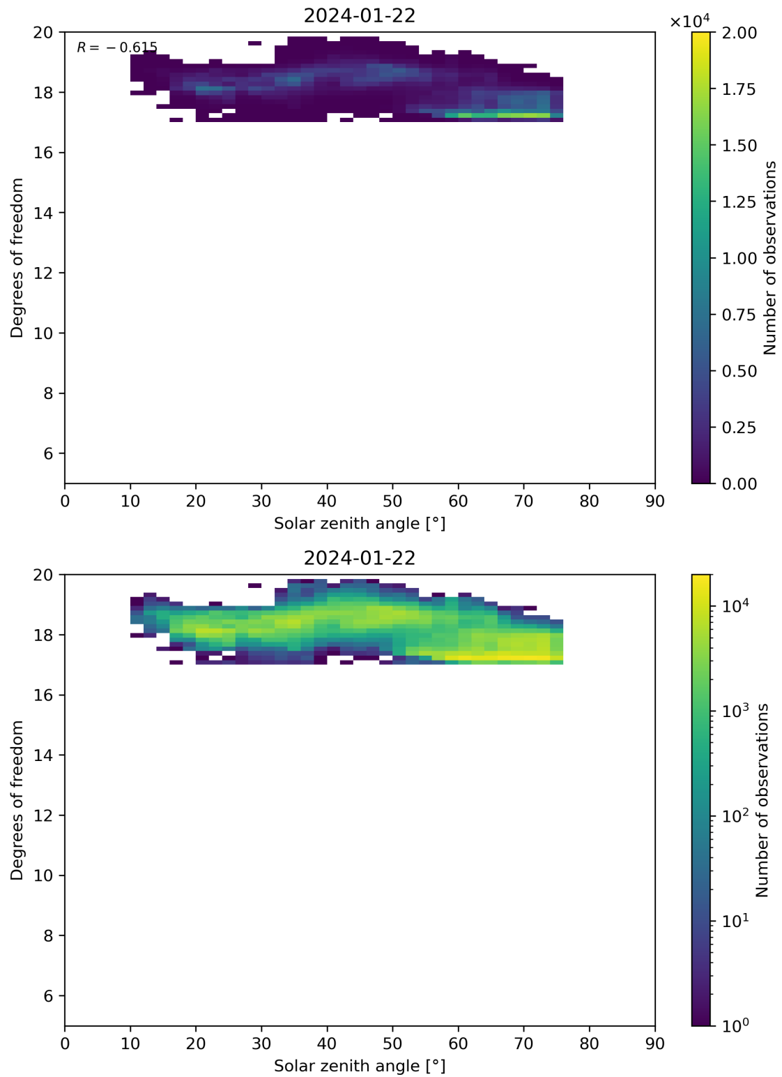
Figure 96: Scatter density plot of “Solar zenith angle” against “Degrees of freedom” for 2024-01-21 to 2024-01-23.
