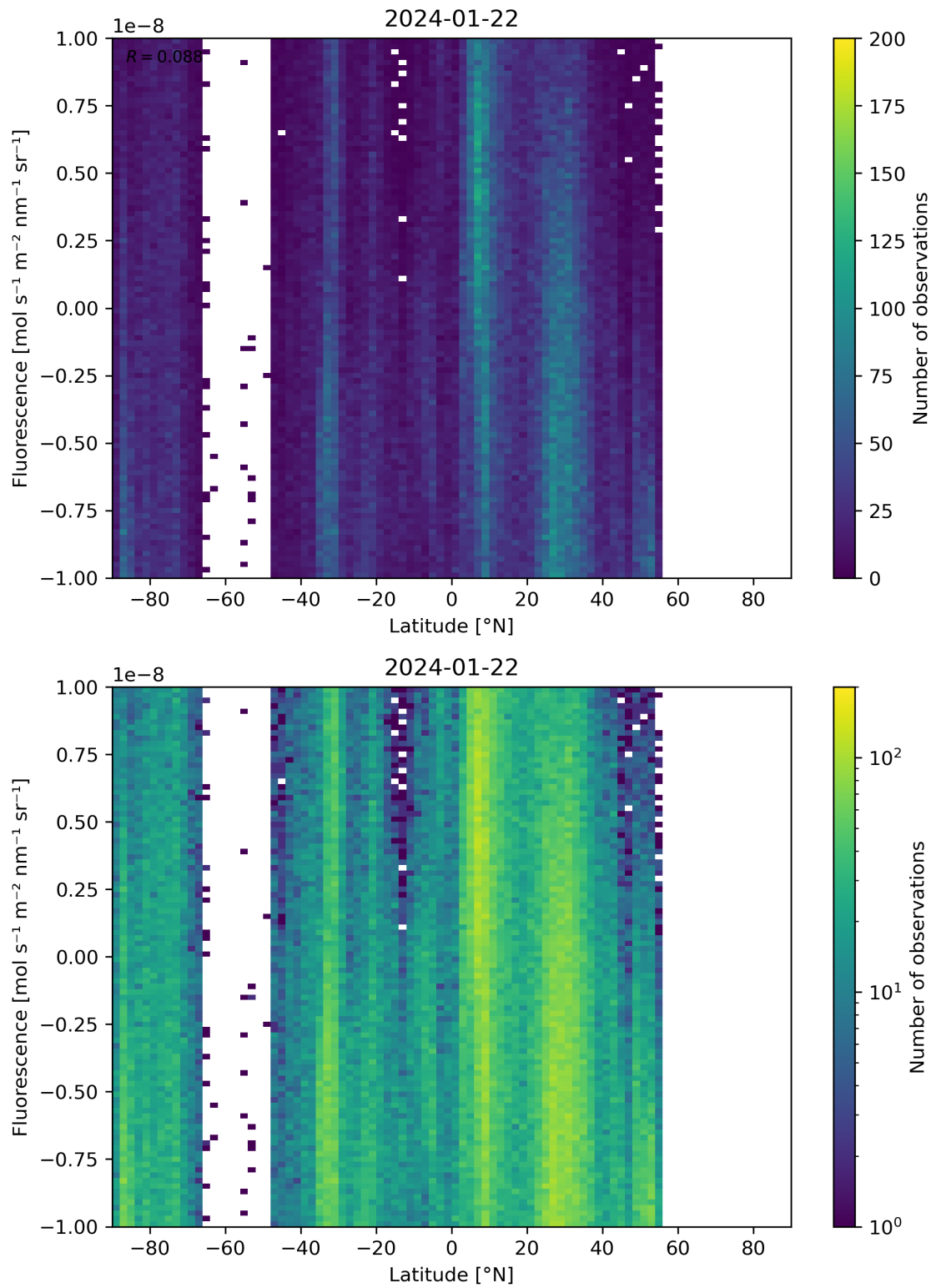
Figure 56: Scatter density plot of “Latitude” against “Fluorescence” for 2024-01-21 to 2024-01-23.
