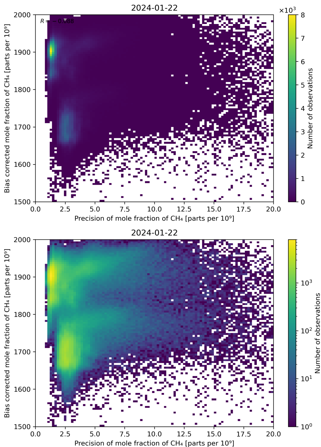
Figure 82: Scatter density plot of “Precision of mole fraction of CH 4 ” against “Bias corrected mole fraction of CH 4 ” for 2024-01-21 to 2024-01-23.
