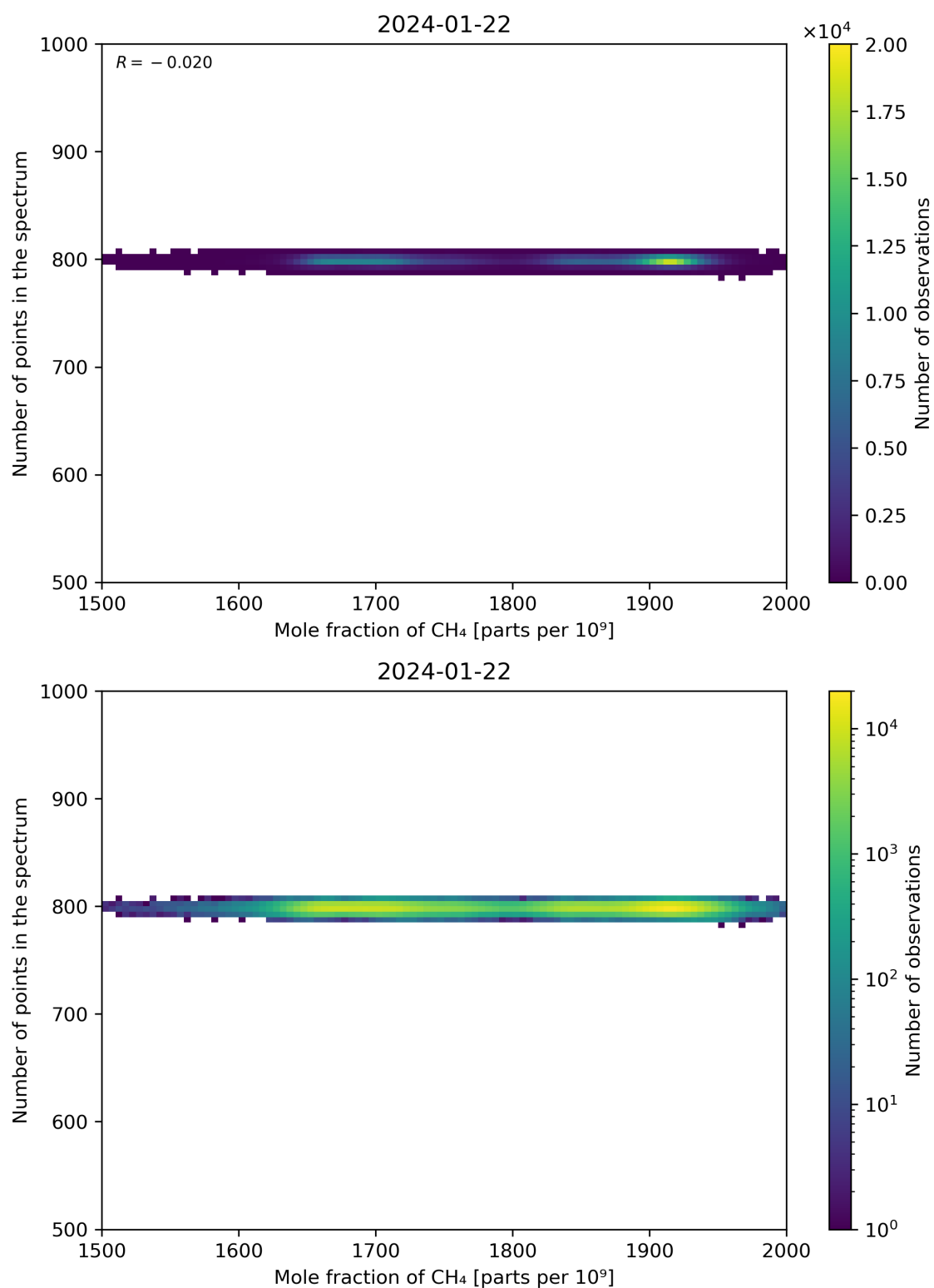
Figure 77: Scatter density plot of “Mole fraction of CH 4 ” against “Number of points in the spectrum” for 2024-01-21 to 2024-01-23.
