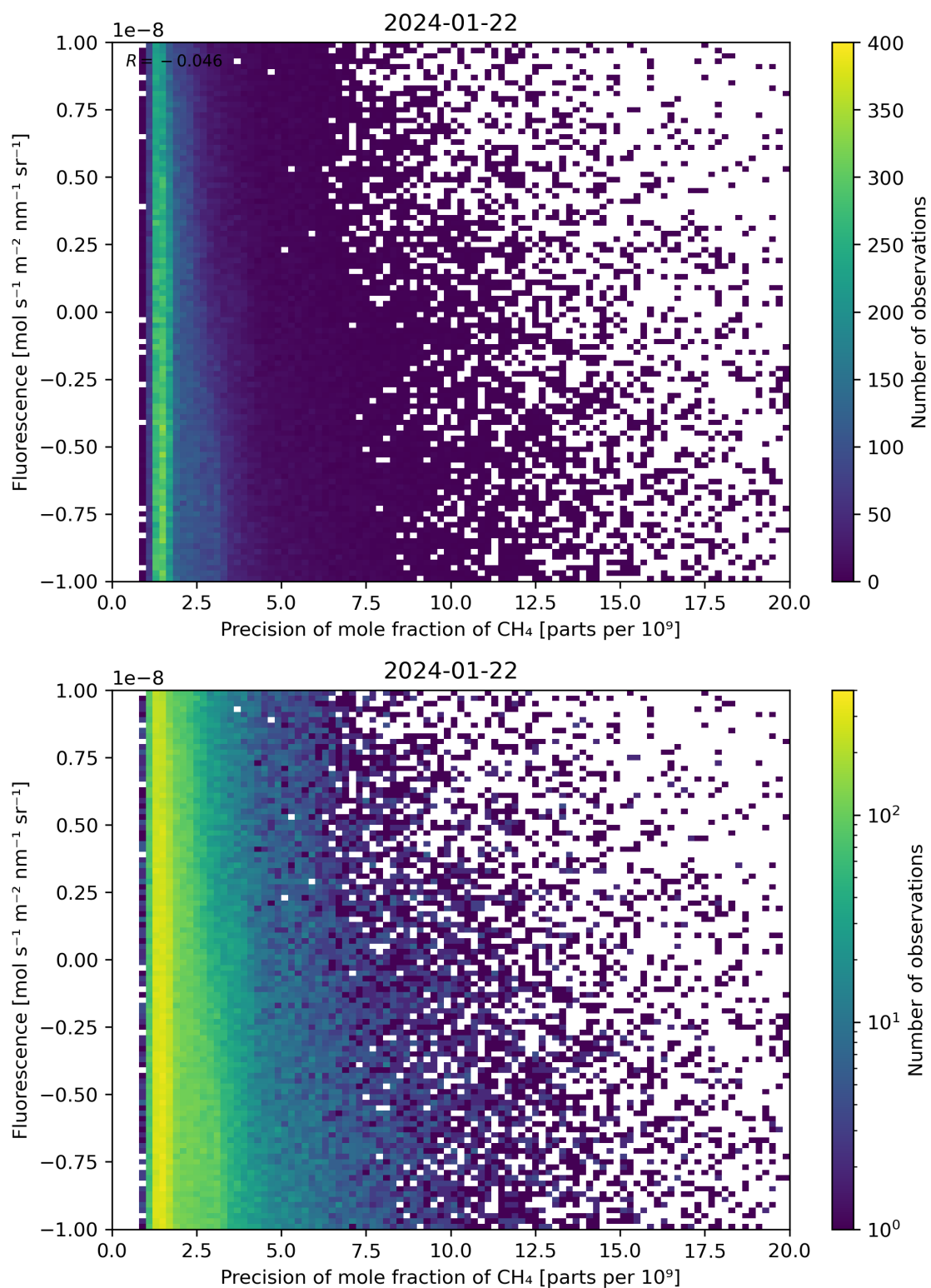
Figure 81: Scatter density plot of “Precision of mole fraction of CH 4 ” against “Fluorescence” for 2024-01-21 to 2024-01-23.
