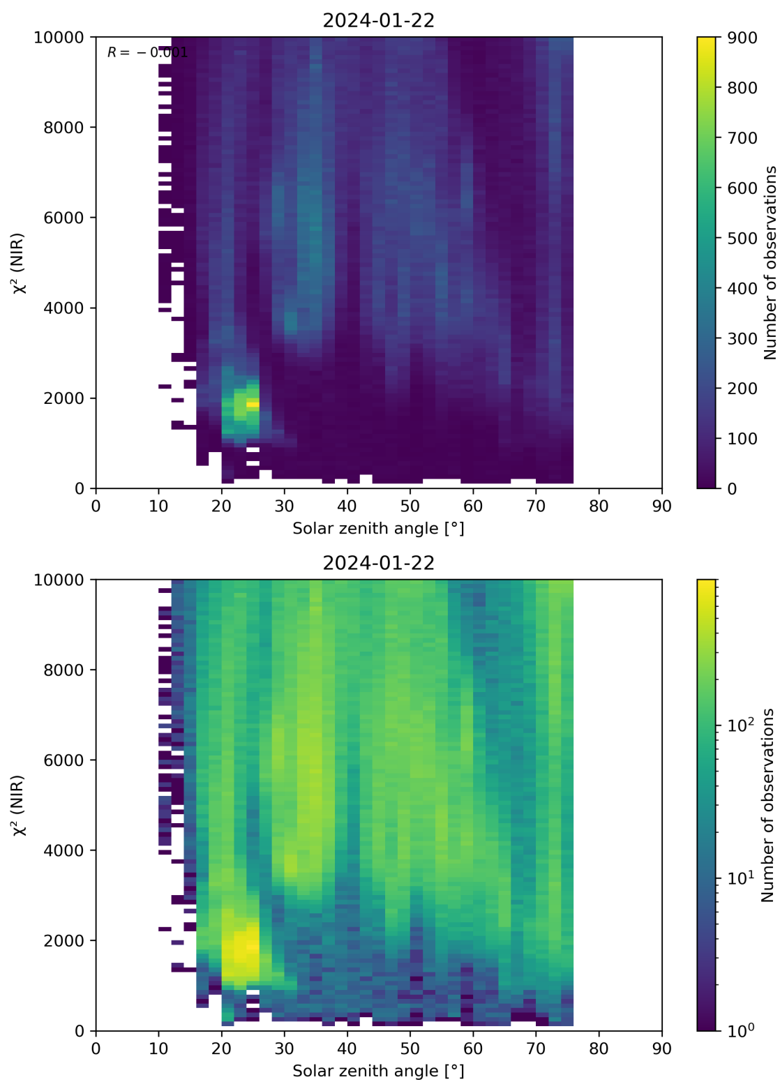
Figure 94: Scatter density plot of “Solar zenith angle” against “ \chi^2 (NIR)” for 2024-01-21 to 2024-01-23.
