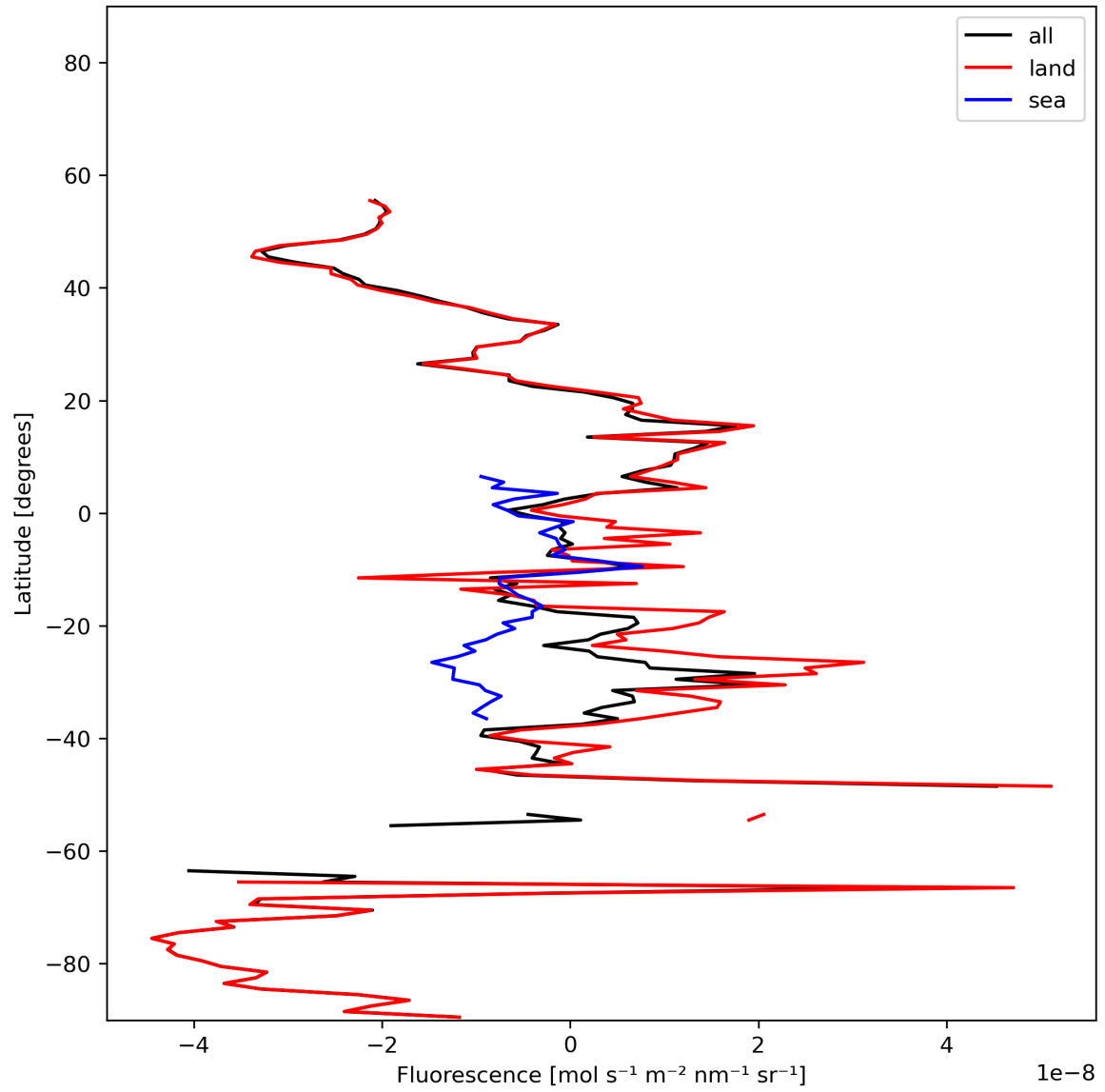
Figure 21: Zonal average of “Fluorescence” for 2024-01-21 to 2024-01-23.
