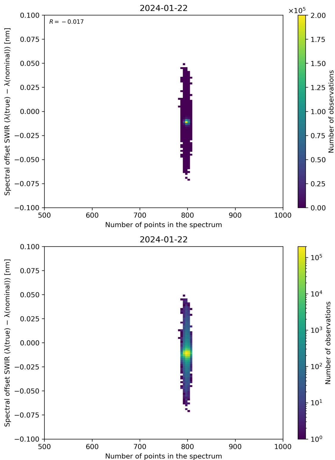
Figure 93: Scatter density plot of “Number of points in the spectrum” against “Spectral offset SWIR ( \lambda(\text{true}) - \lambda(\text{nominal}) )” for 2024-01-21 to 2024-01-23.
