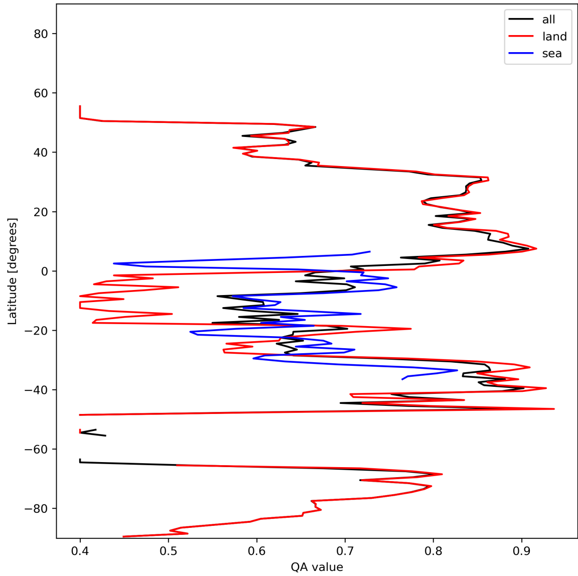
Figure 11: Zonal average of “QA value” for 2024-01-21 to 2024-01-23.
