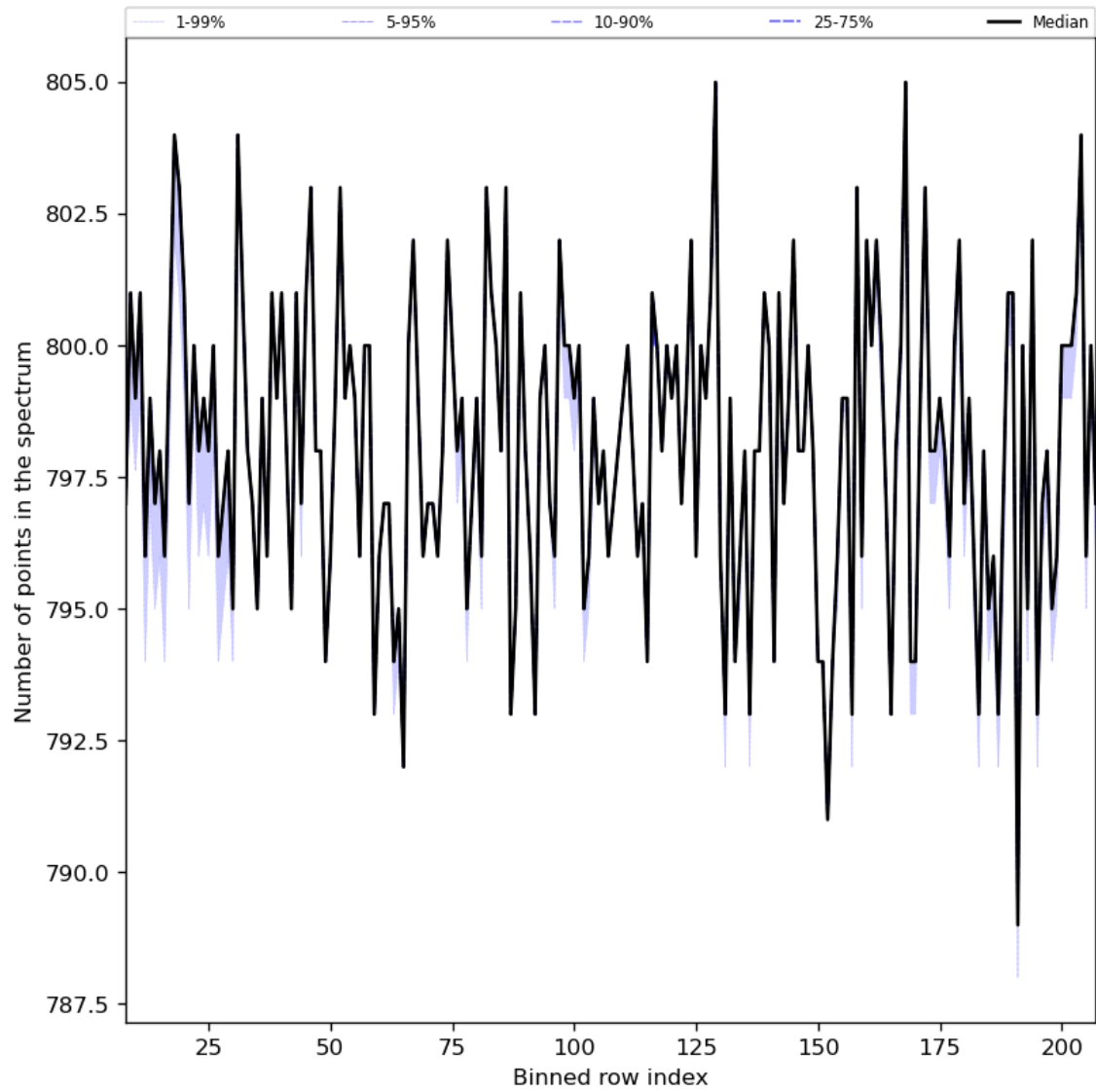
Figure 37: Along track statistics of “Number of points in the spectrum” for 2024-01-21 to 2024-01-23
