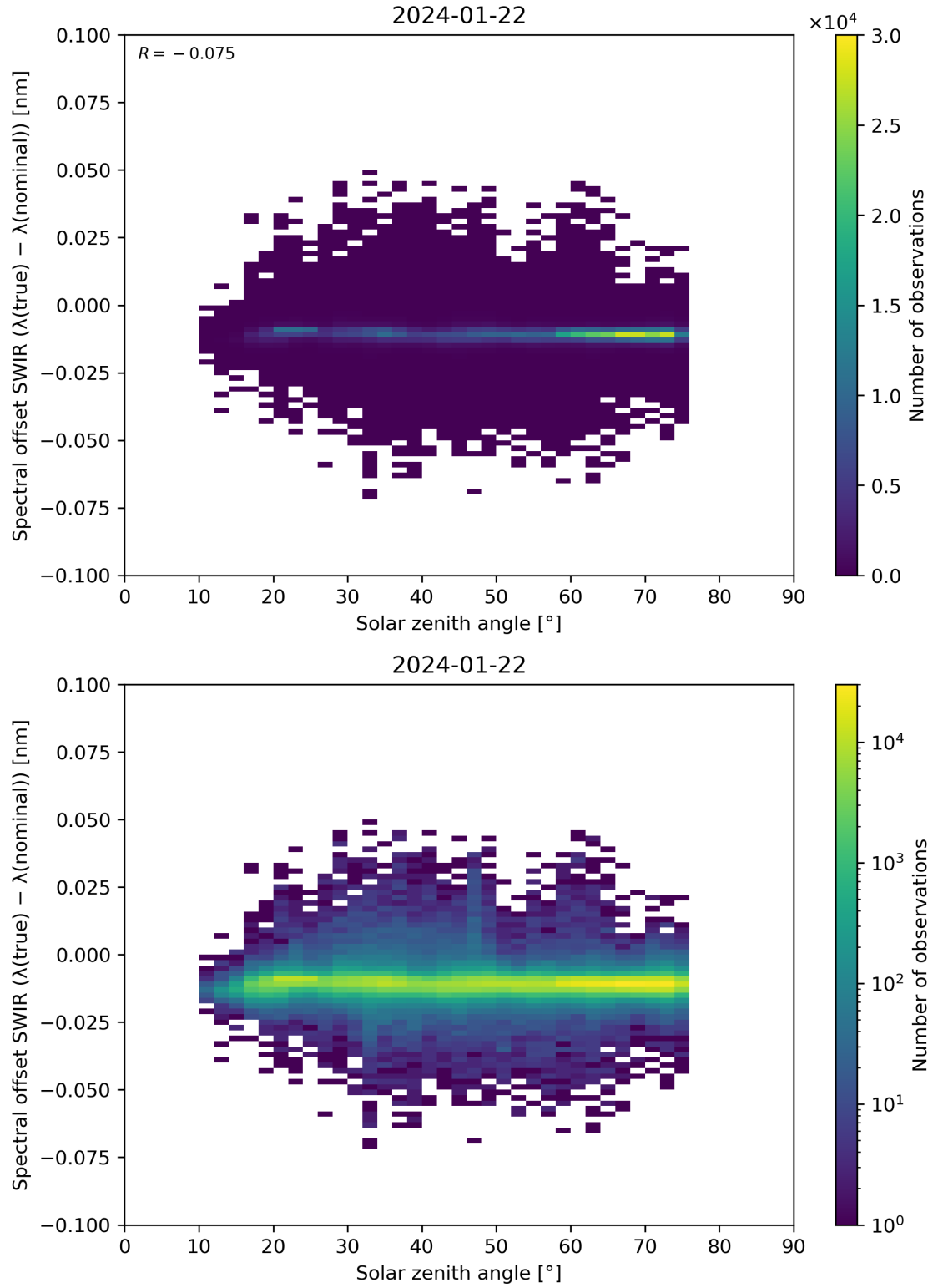
Figure 104: Scatter density plot of “Solar zenith angle” against “Spectral offset SWIR ( \lambda(\text{true}) - \lambda(\text{nominal}) )” for 2024-01-21 to 2024-01-23.
