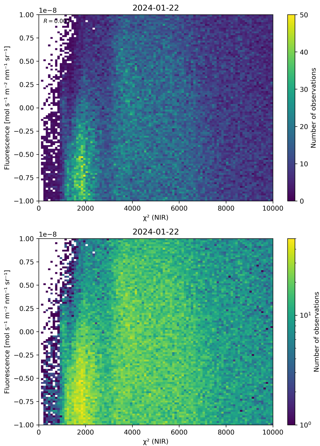
Figure 45: Scatter density plot of “ \chi^2 (NIR)” against “Fluorescence” for 2024-01-21 to 2024-01-23.
