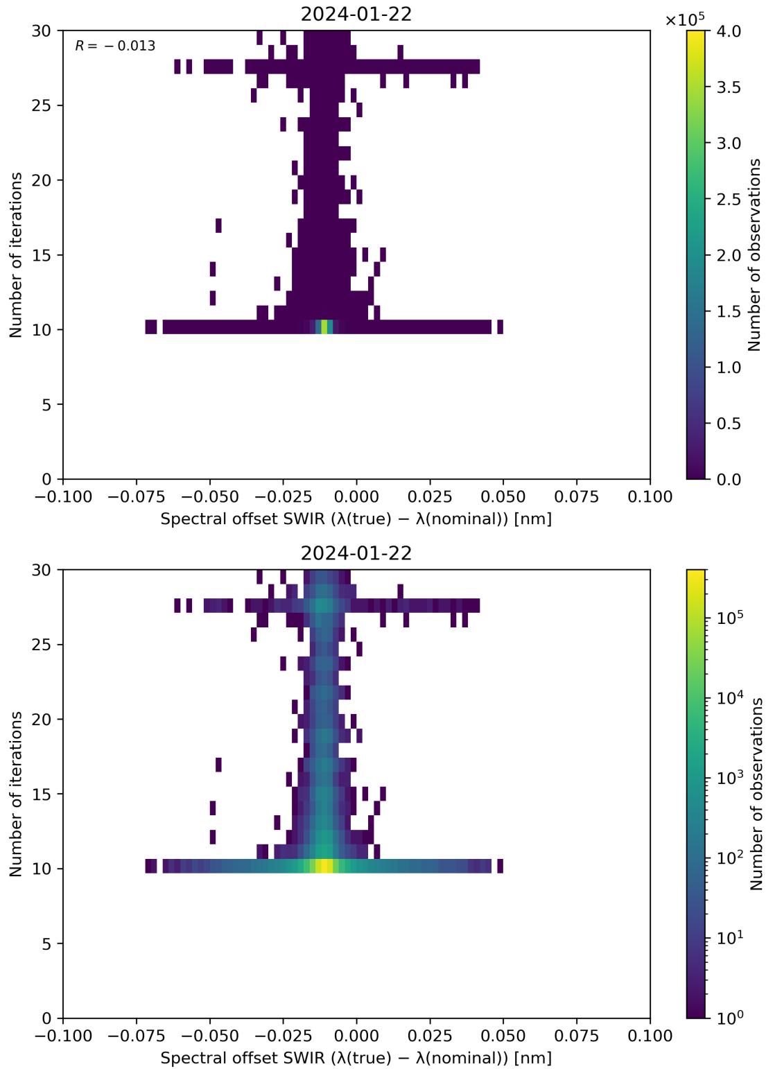
Figure 121: Scatter density plot of “Spectral offset SWIR ( \lambda(\text{true}) - \lambda(\text{nominal}) )” against “Number of iterations” for 2024-01-21 to 2024-01-23.
