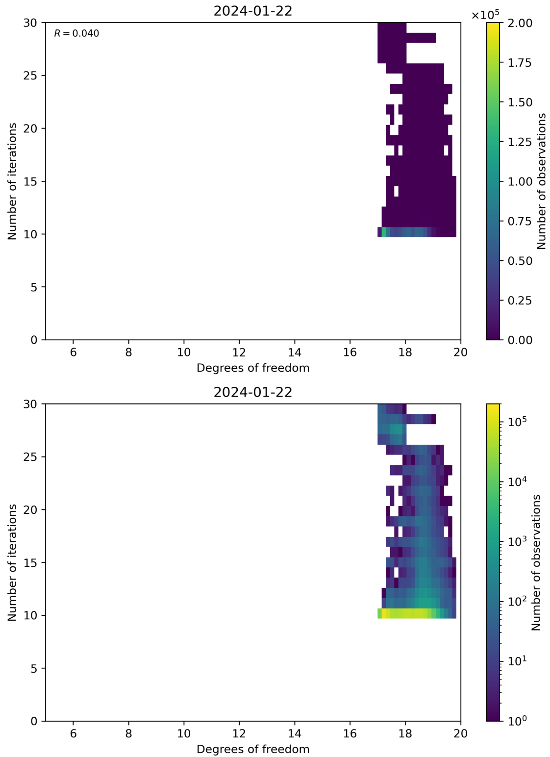
Figure 52: Scatter density plot of “Degrees of freedom” against “Number of iterations” for 2024-01-21 to 2024-01-23.
