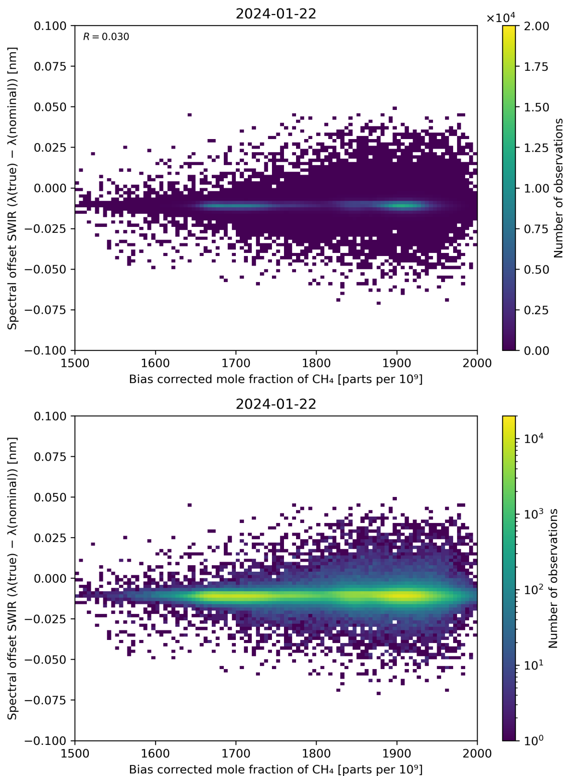
Figure 69: Scatter density plot of “Bias corrected mole fraction of \text{CH}_4 ” against “Spectral offset SWIR ( \lambda(\text{true}) - \lambda(\text{nominal}) )” for 2024-01-21 to 2024-01-23.
