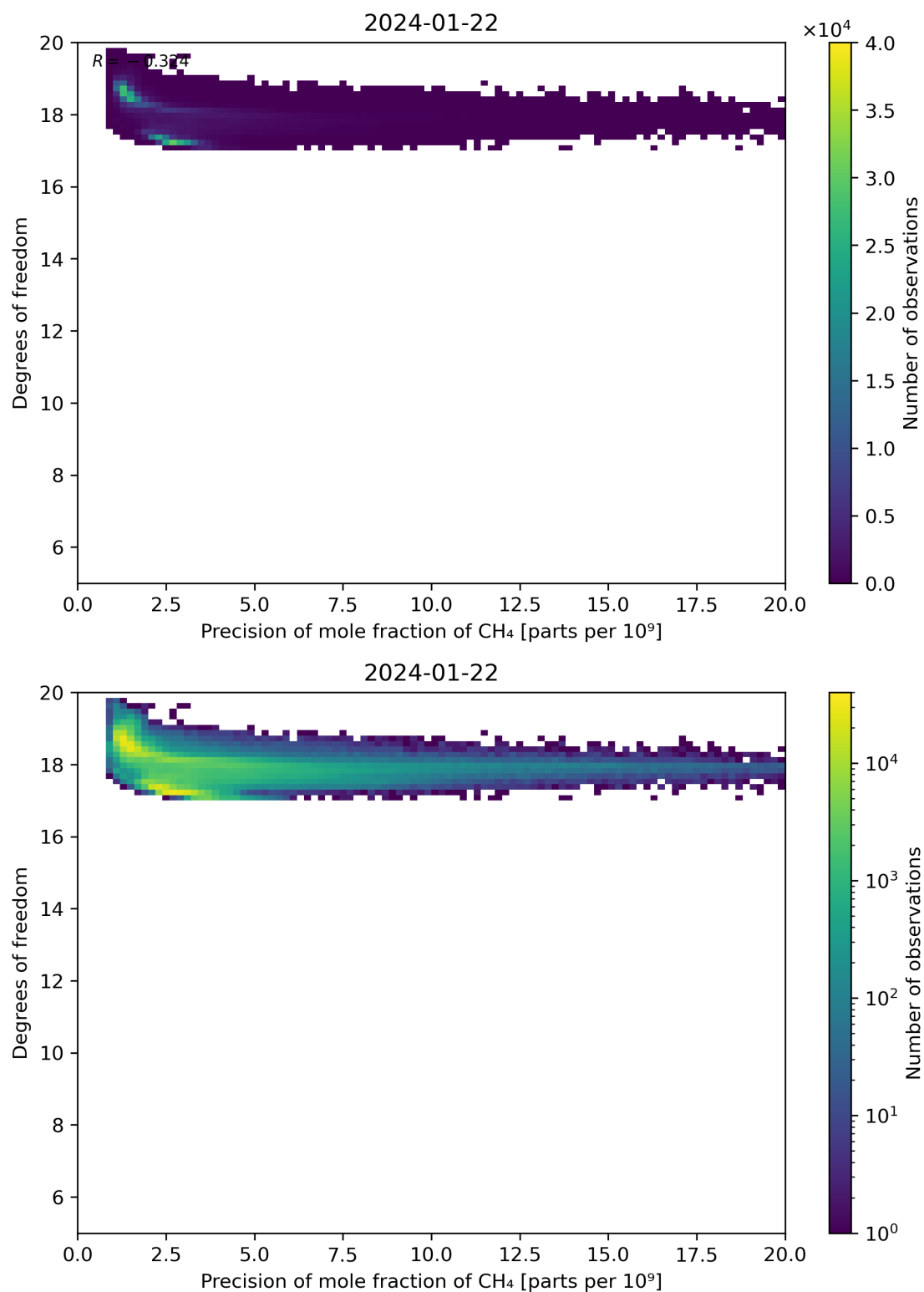
Figure 80: Scatter density plot of “Precision of mole fraction of CH 4 ” against “Degrees of freedom” for 2024-01-21 to 2024-01-23.
