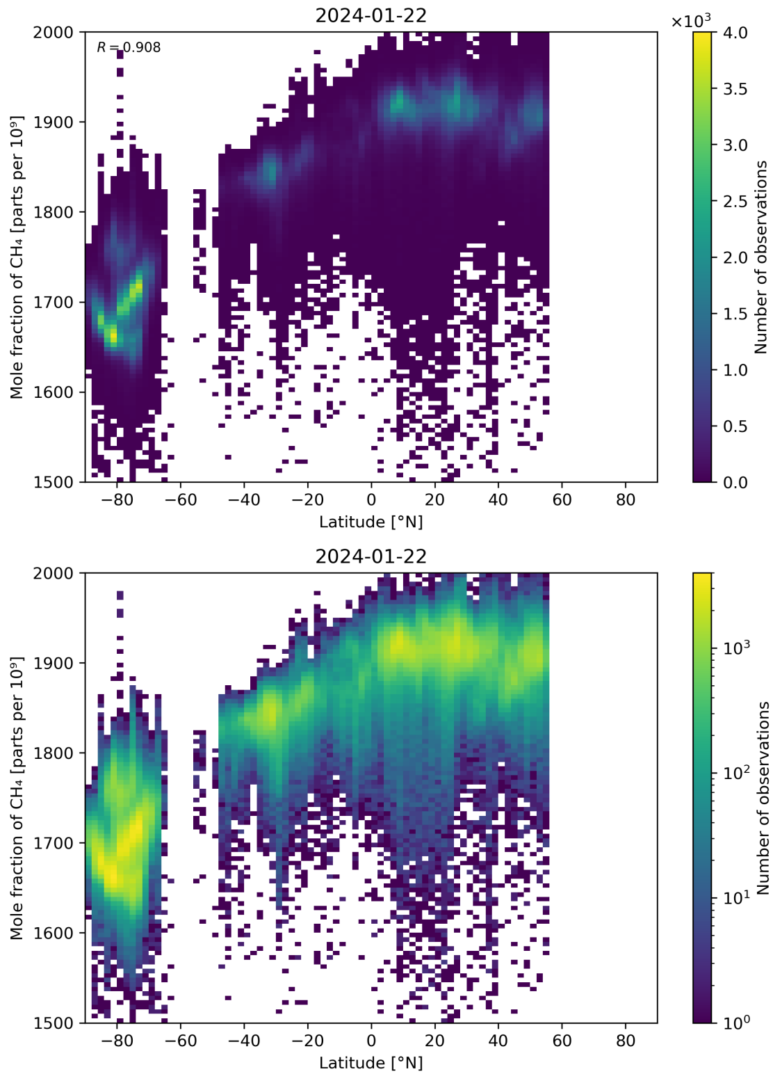
Figure 57: Scatter density plot of “Latitude” against “Mole fraction of CH 4 ” for 2024-01-21 to 2024-01-23.
