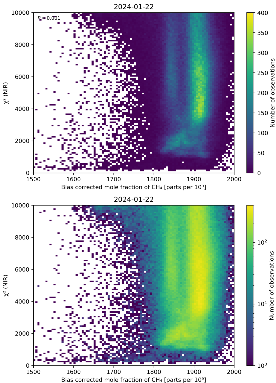
Figure 63: Scatter density plot of “Bias corrected mole fraction of \text{CH}_4 ” against “ \chi^2 (NIR)” for 2024-01-21 to 2024-01-23.
