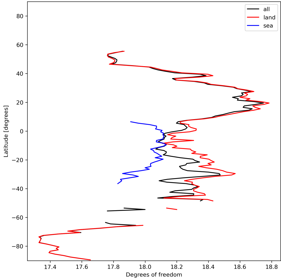
Figure 19: Zonal average of “Degrees of freedom” for 2024-01-21 to 2024-01-23.
