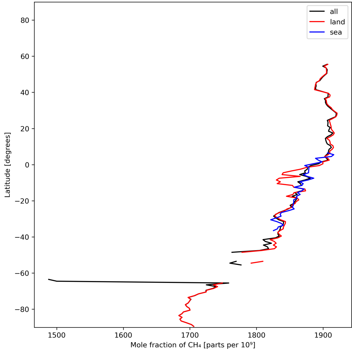
Figure 12: Zonal average of “Mole fraction of \text{CH}_4 ” for 2024-01-21 to 2024-01-23.
