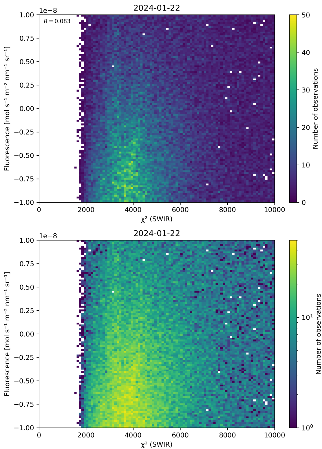
Figure 49: Scatter density plot of “ \chi^2 (SWIR)” against “Fluorescence” for 2024-01-21 to 2024-01-23.
