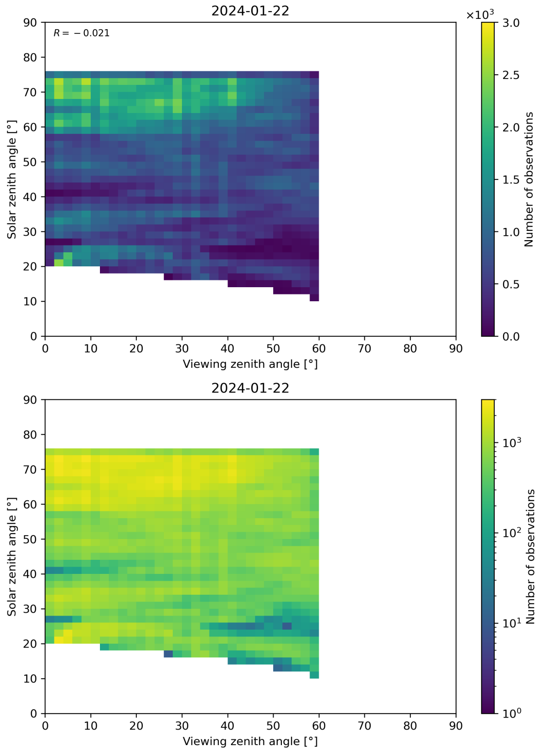
Figure 115: Scatter density plot of “Viewing zenith angle” against “Solar zenith angle” for 2024-01-21 to 2024-01-23.
