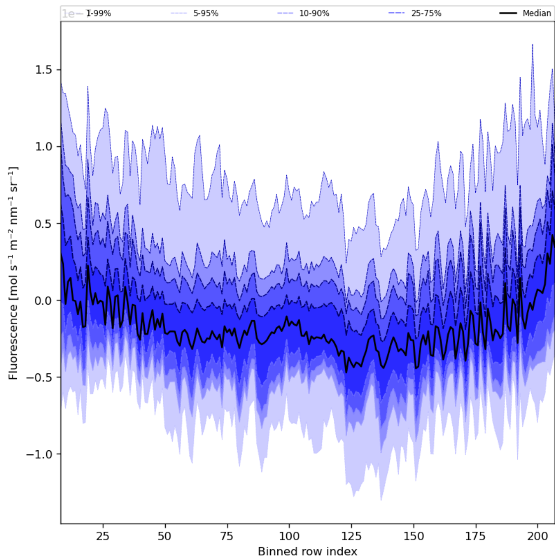
Figure 43: Along track statistics of “Fluorescence” for 2024-01-21 to 2024-01-23
