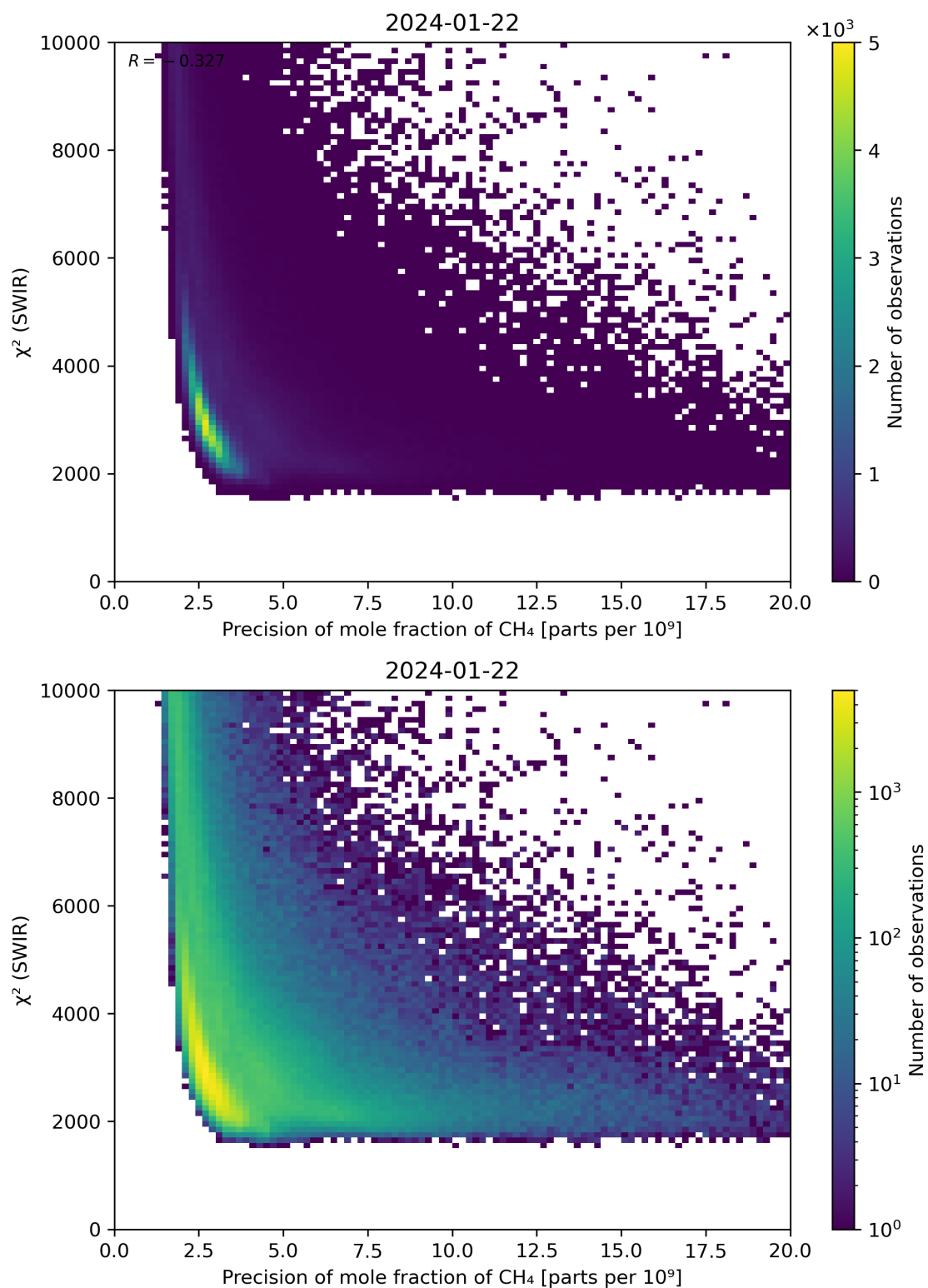
Figure 79: Scatter density plot of “Precision of mole fraction of \text{CH}_4 ” against “ \chi^2 (SWIR)” for 2024-01-21 to 2024-01-23.
