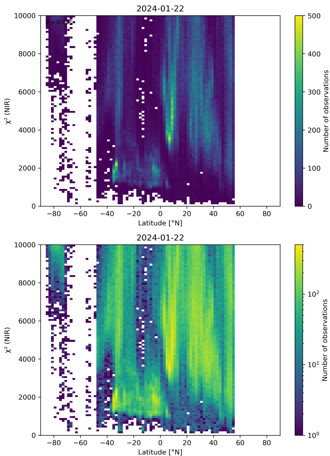
Figure 53: Scatter density plot of “Latitude” against “ \chi^2 (NIR)” for 2024-01-21 to 2024-01-23.
