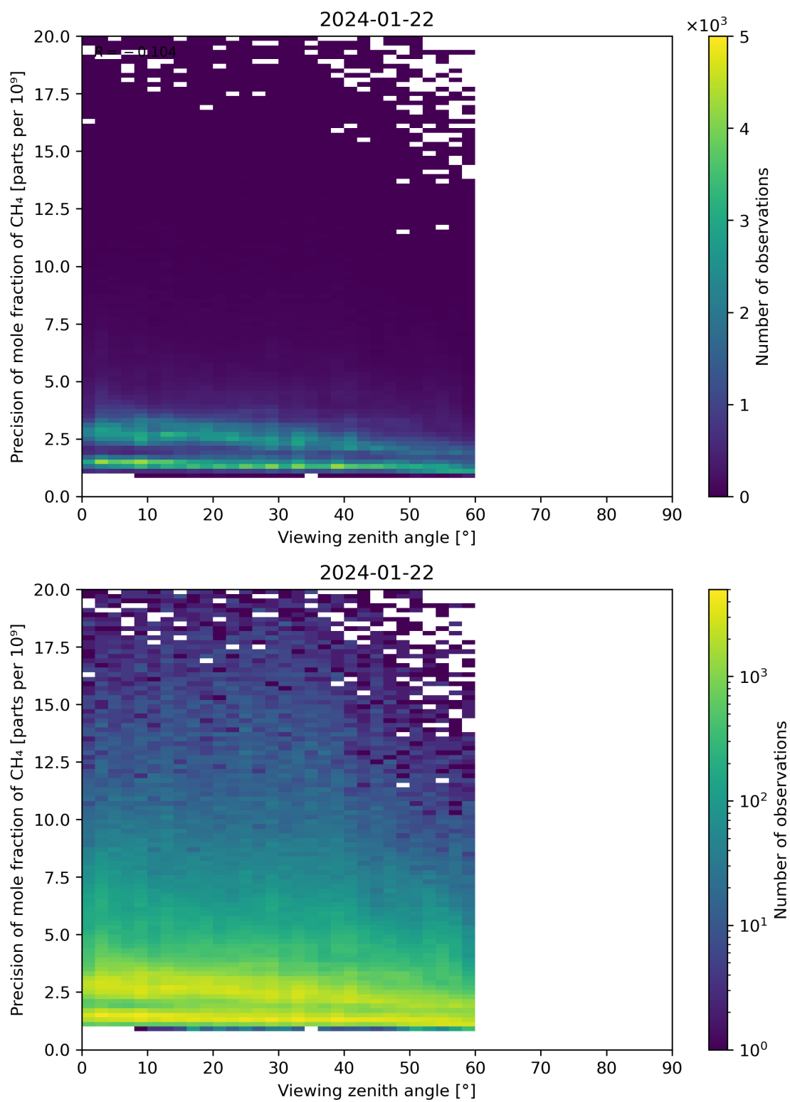
Figure 112: Scatter density plot of “Viewing zenith angle” against “Precision of mole fraction of CH 4 ” for 2024-01-21 to 2024-01-23.
