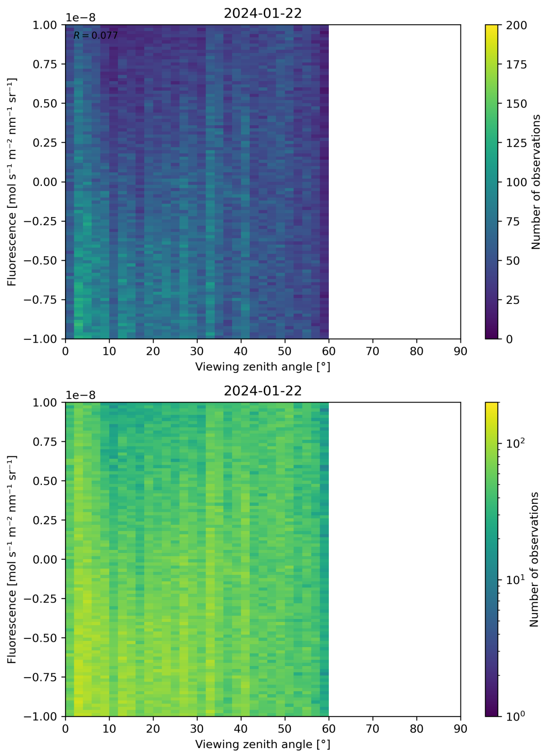
Figure 108: Scatter density plot of “Viewing zenith angle” against “Fluorescence” for 2024-01-21 to 2024-01-23.
