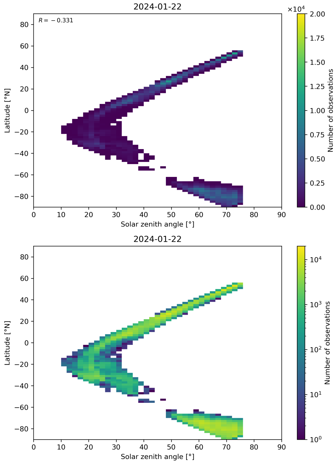
Figure 98: Scatter density plot of “Solar zenith angle” against “Latitude” for 2024-01-21 to 2024-01-23.
