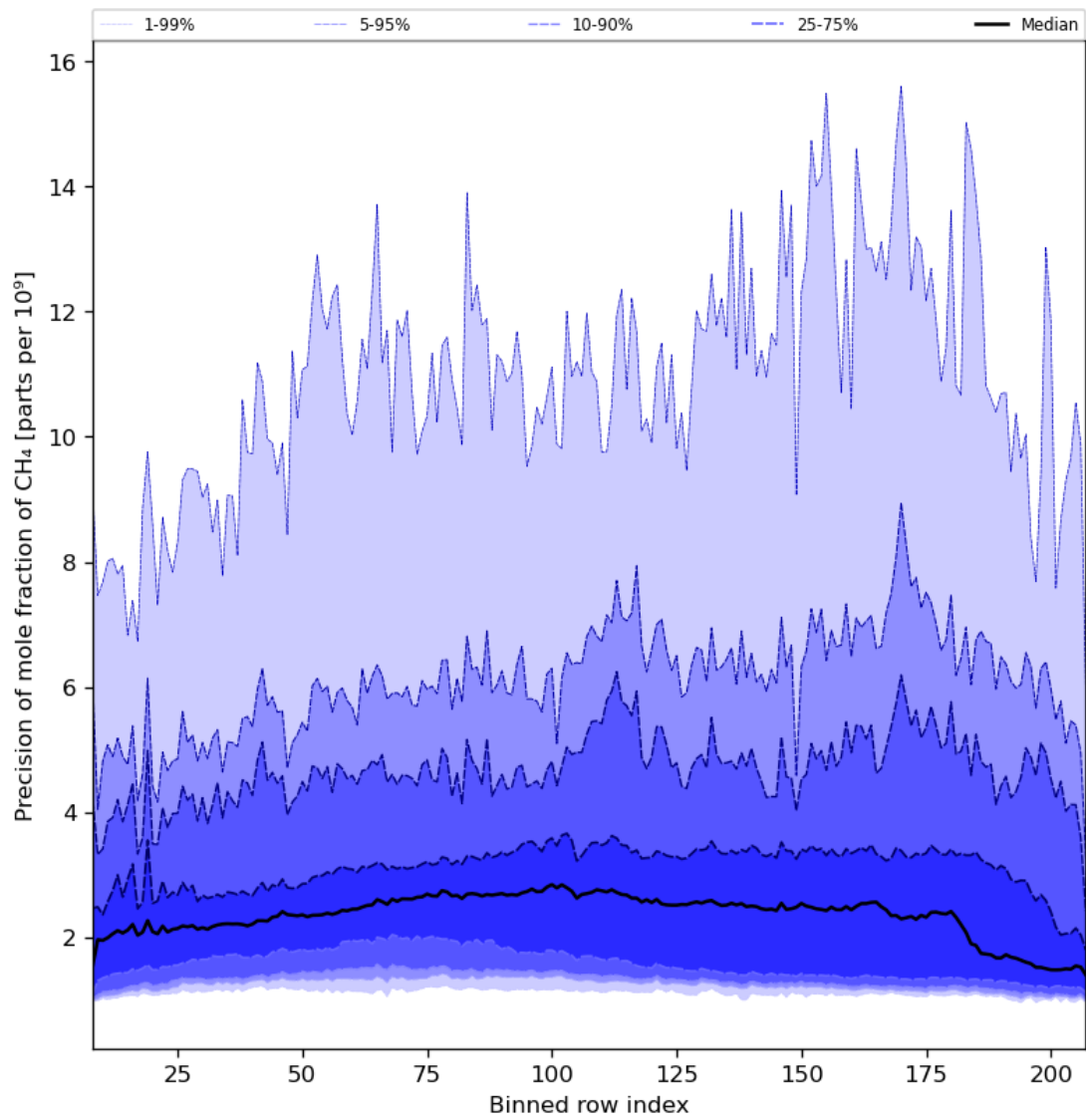
Figure 35: Along track statistics of “Precision of mole fraction of CH 4 ” for 2024-01-21 to 2024-01-23
