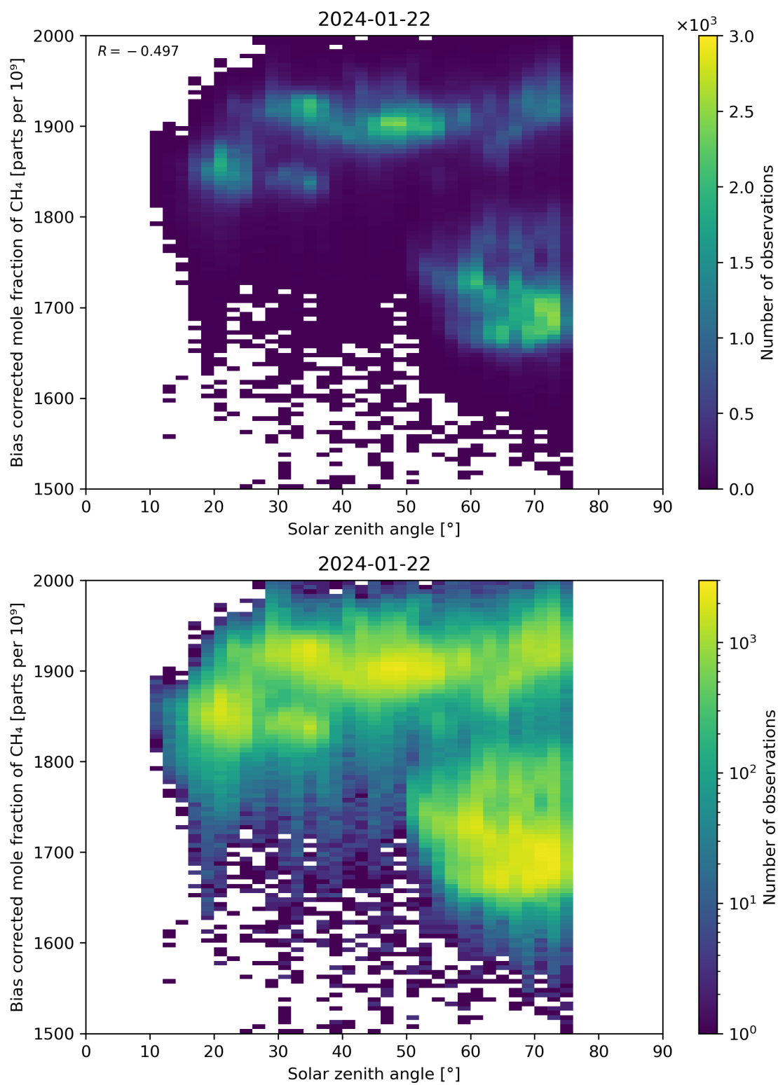
Figure 100: Scatter density plot of “Solar zenith angle” against “Bias corrected mole fraction of CH 4 ” for 2024-01-21 to 2024-01-23.
