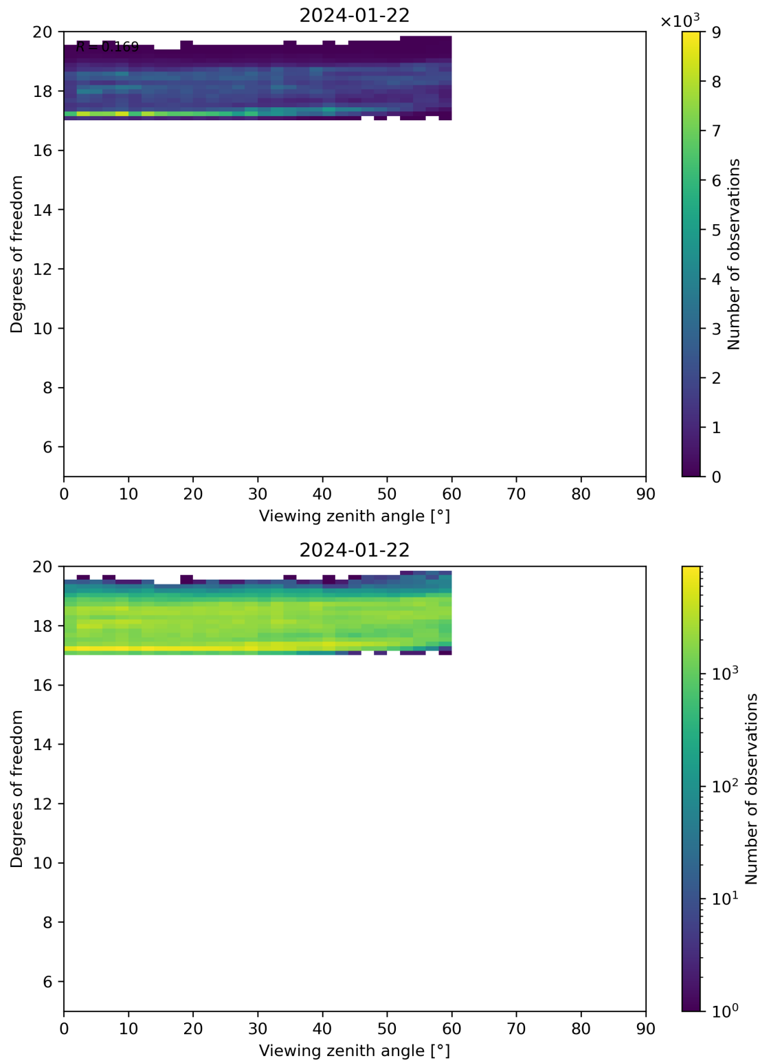
Figure 107: Scatter density plot of “Viewing zenith angle” against “Degrees of freedom” for 2024-01-21 to 2024-01-23.
