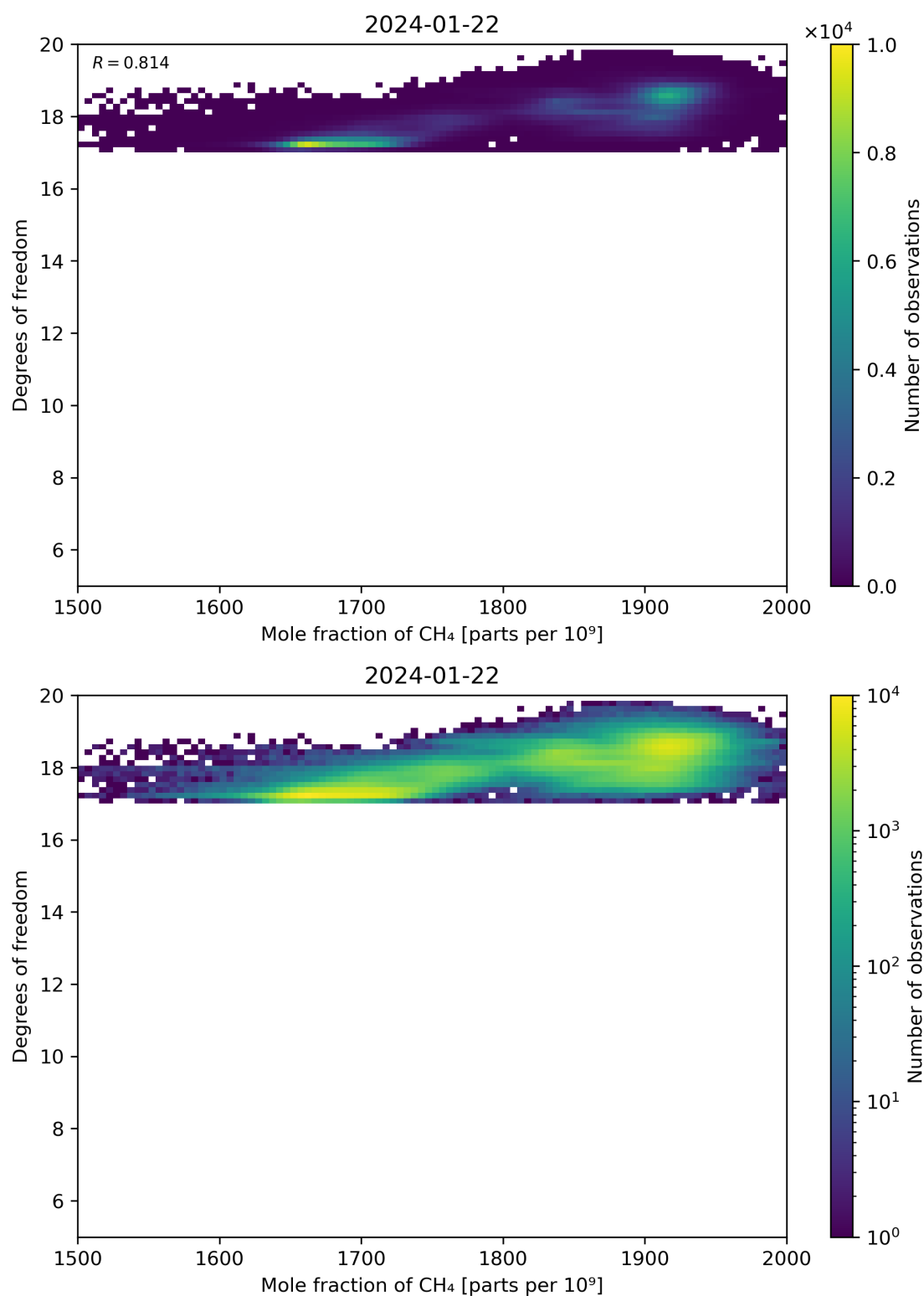
Figure 72: Scatter density plot of “Mole fraction of CH 4 ” against “Degrees of freedom” for 2024-01-21 to 2024-01-23.
