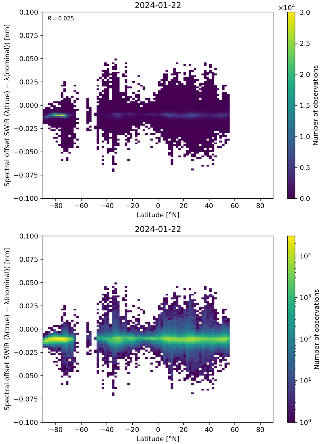
Figure 62: Scatter density plot of “Latitude” against “Spectral offset SWIR ( \lambda(\text{true}) - \lambda(\text{nominal}) )” for 2024-01-21 to 2024-01-23.
