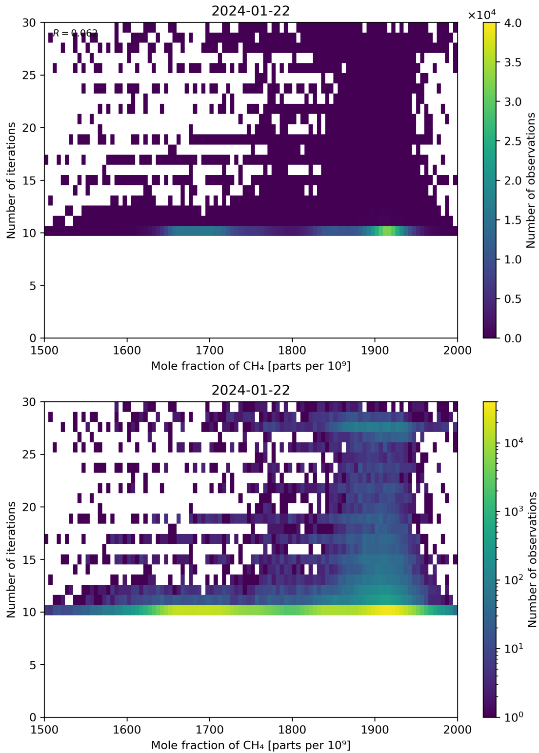
Figure 76: Scatter density plot of “Mole fraction of CH 4 ” against “Number of iterations” for 2024-01-21 to 2024-01-23.
