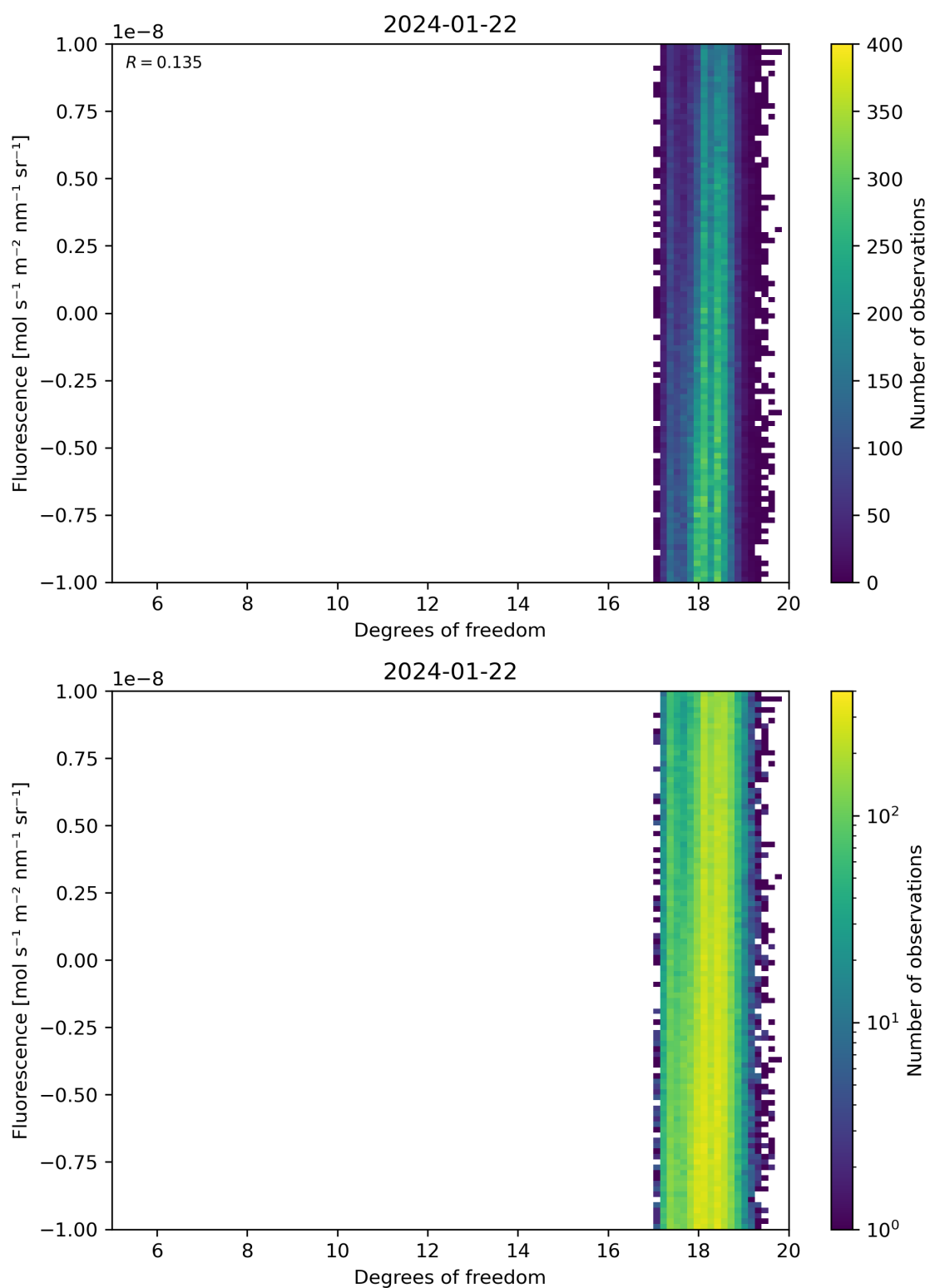
Figure 51: Scatter density plot of “Degrees of freedom” against “Fluorescence” for 2024-01-21 to 2024-01-23.
