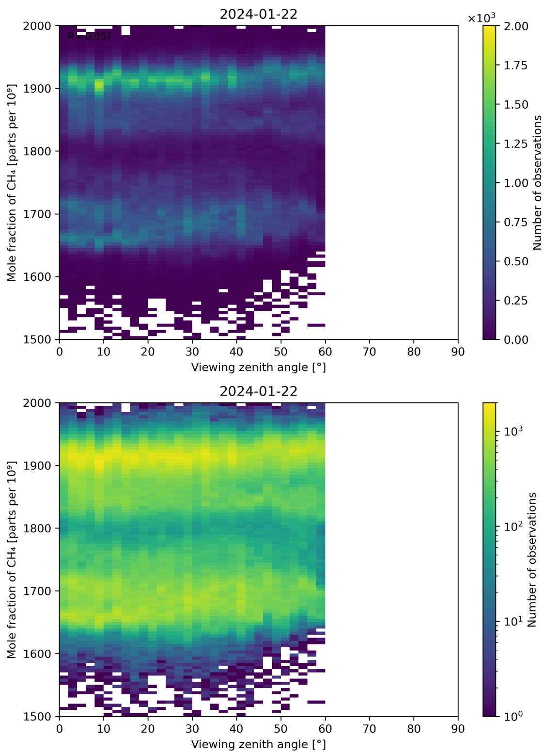
Figure 110: Scatter density plot of “Viewing zenith angle” against “Mole fraction of \text{CH}_4 ” for 2024-01-21 to 2024-01-23.
