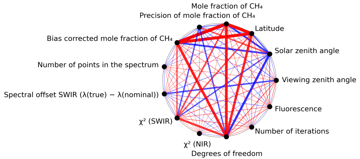
Figure 1: Map of correlation graph for 2024-01-21 to 2024-01-23.
