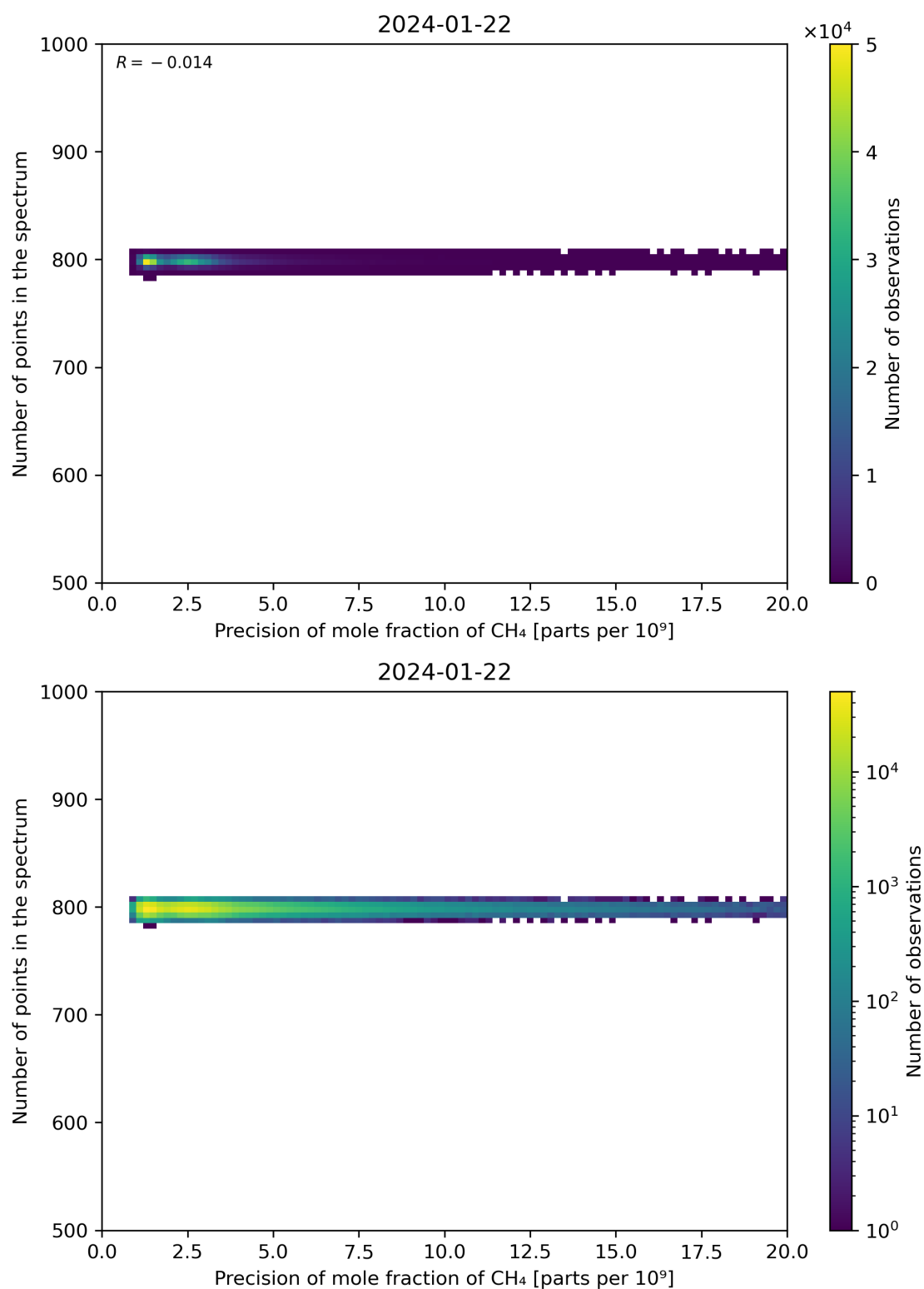
Figure 84: Scatter density plot of “Precision of mole fraction of CH 4 ” against “Number of points in the spectrum” for 2024-01-21 to 2024-01-23.
