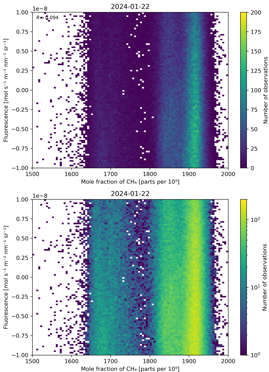
Figure 73: Scatter density plot of “Mole fraction of \text{CH}_4 ” against “Fluorescence” for 2024-01-21 to 2024-01-23.
