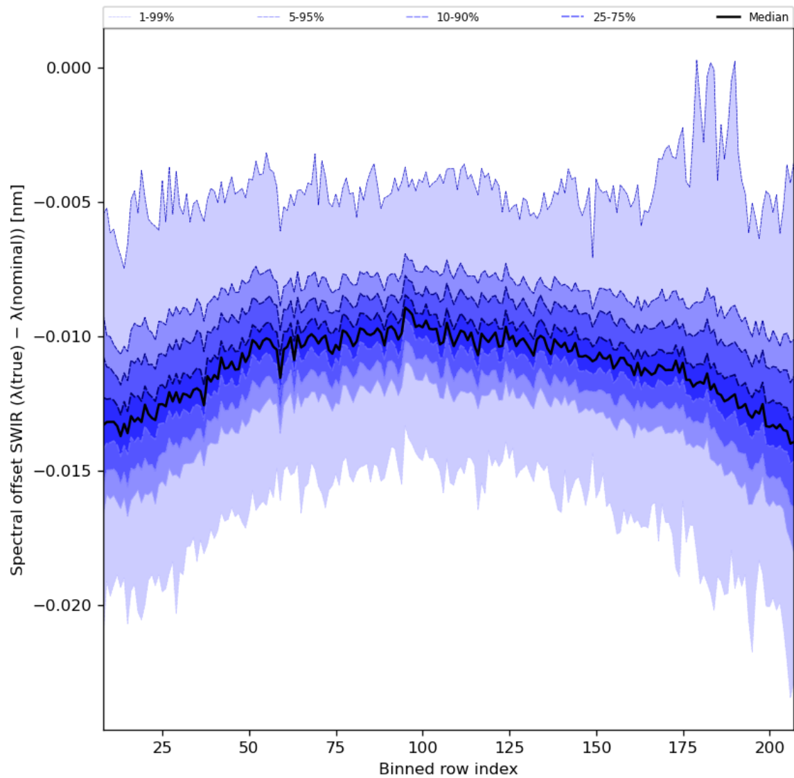
Figure 38: Along track statistics of “Spectral offset SWIR ( \lambda(\text{true}) - \lambda(\text{nominal}) )” for 2024-01-21 to 2024-01-23
