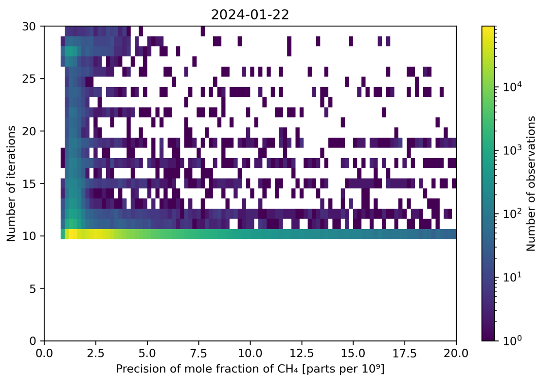
Figure 83: Scatter density plot of “Precision of mole fraction of CH 4 ” against “Number of iterations” for 2024-01-21 to 2024-01-23.
