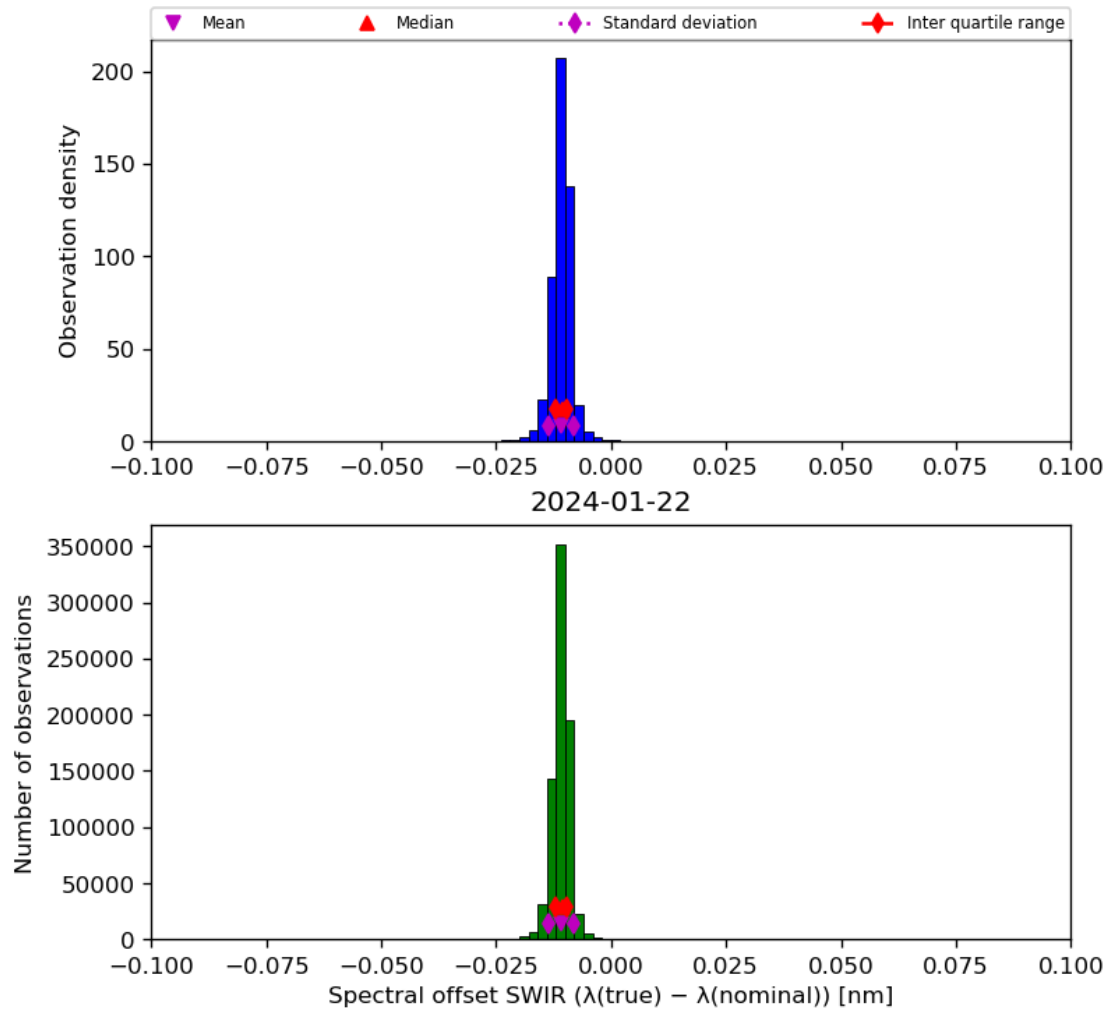
Figure 27: Histogram of “Spectral offset SWIR ( \lambda(\text{true}) - \lambda(\text{nominal}) )” for 2024-01-21 to 2024-01-23
