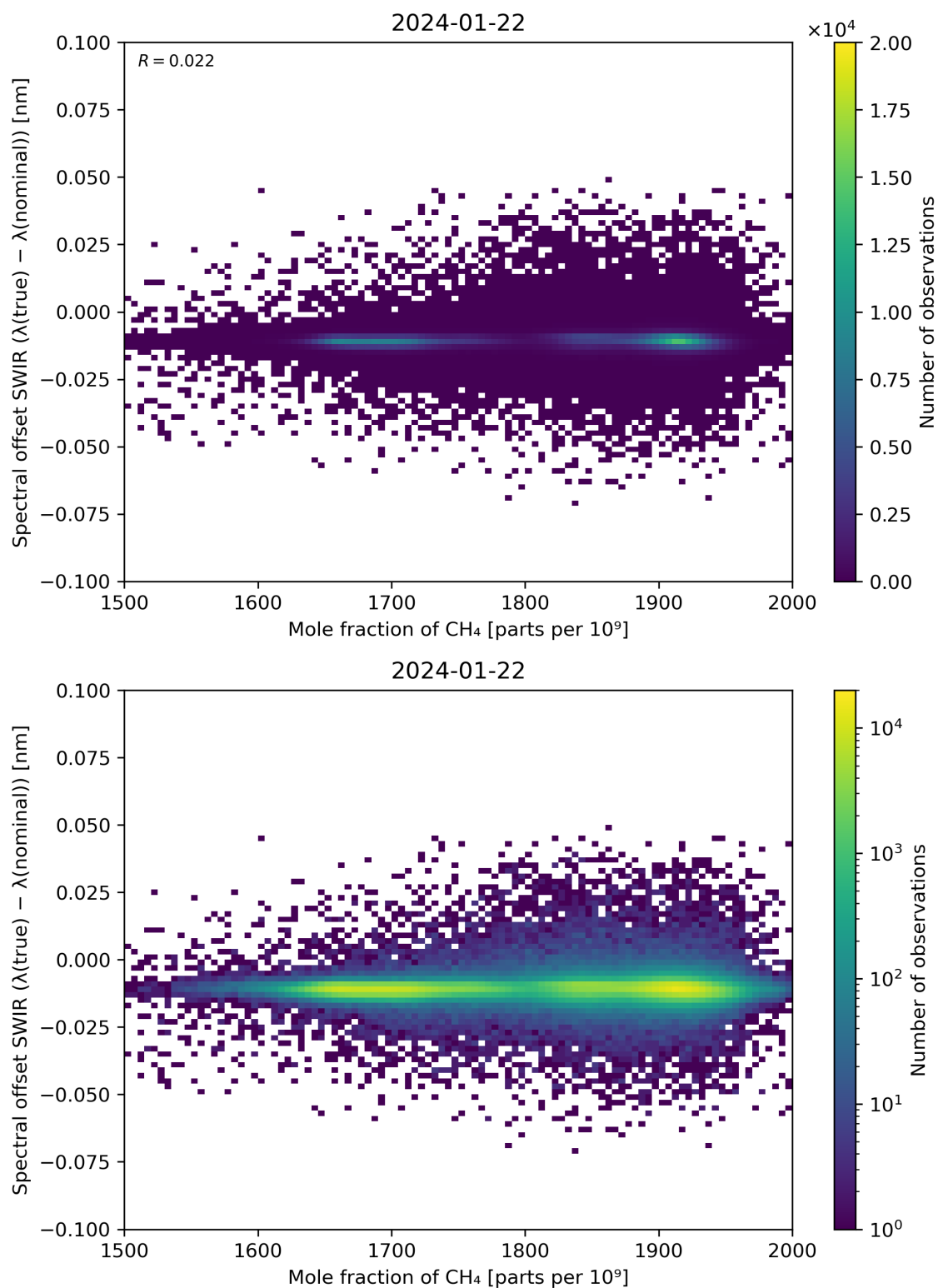
Figure 86: Scatter density plot of “Mole fraction of CH 4 ” against “Spectral offset SWIR ( \lambda(\text{true}) - \lambda(\text{nominal}) )” for 2024-01-21 to 2024-01-23.
