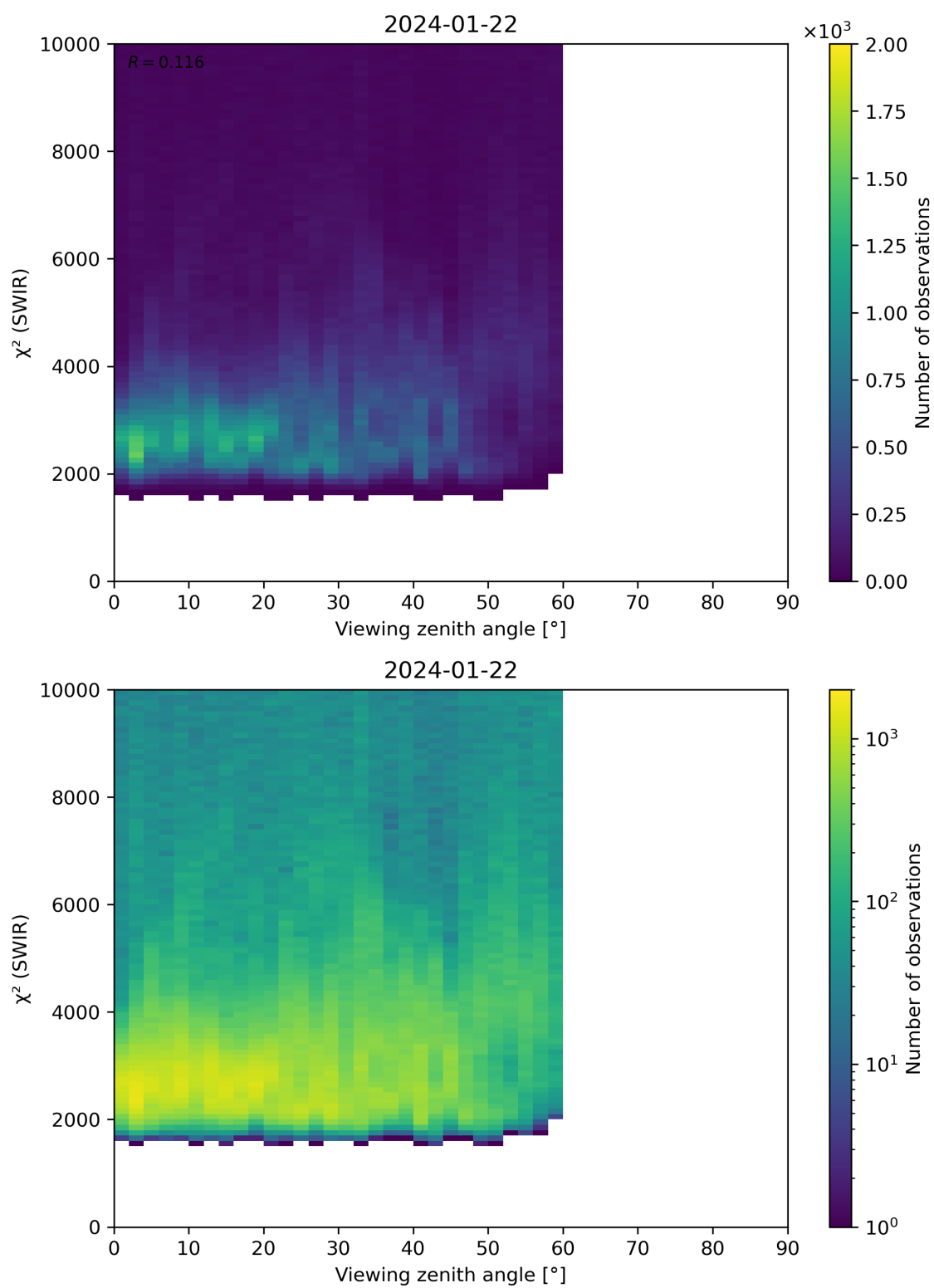
Figure 106: Scatter density plot of “Viewing zenith angle” against “ \chi^2 (SWIR)” for 2024-01-21 to 2024-01-23.
